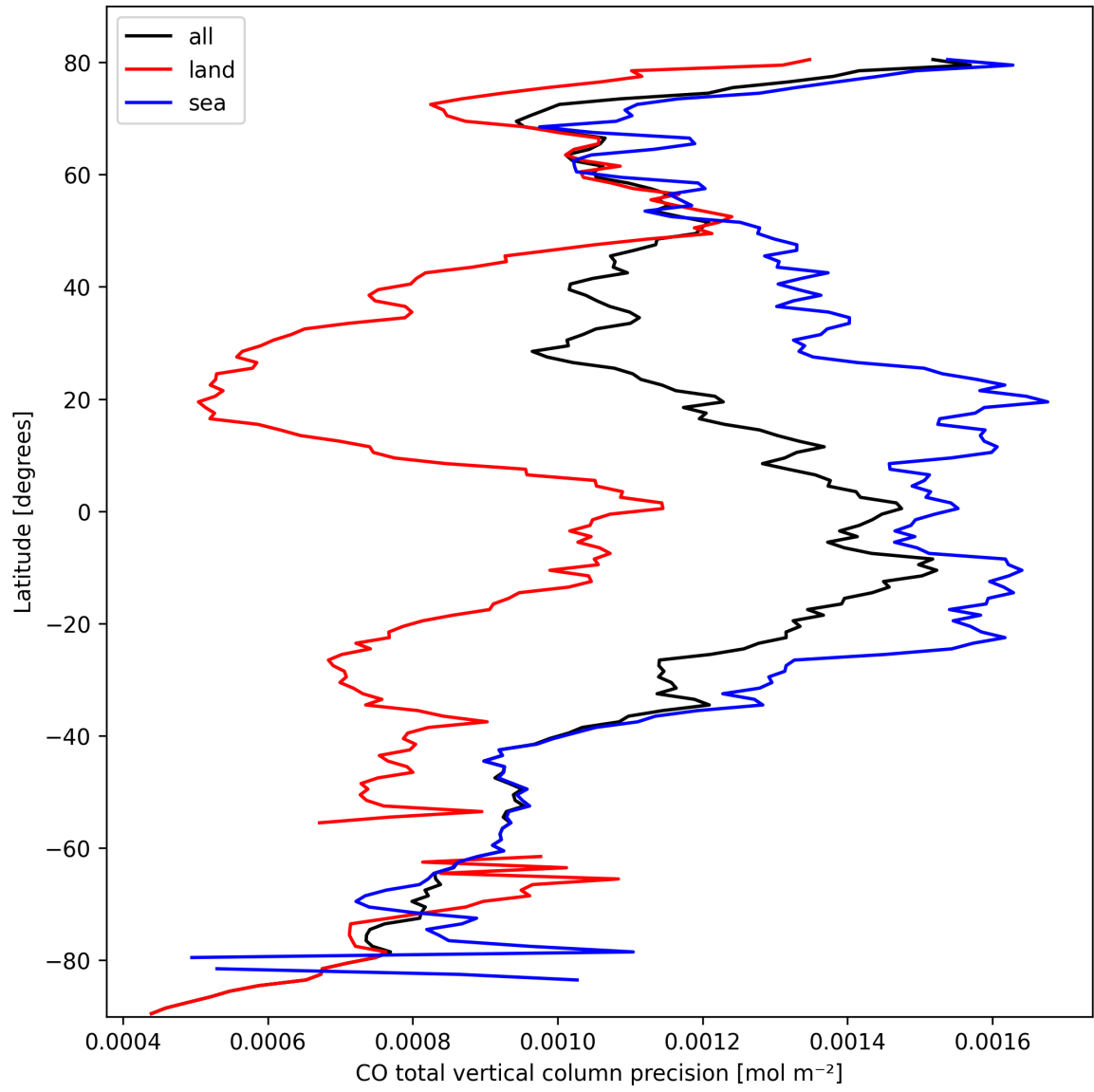
Figure 8: Zonal average of “CO total vertical column precision” for 2025-03-08 to 2025-03-09.
