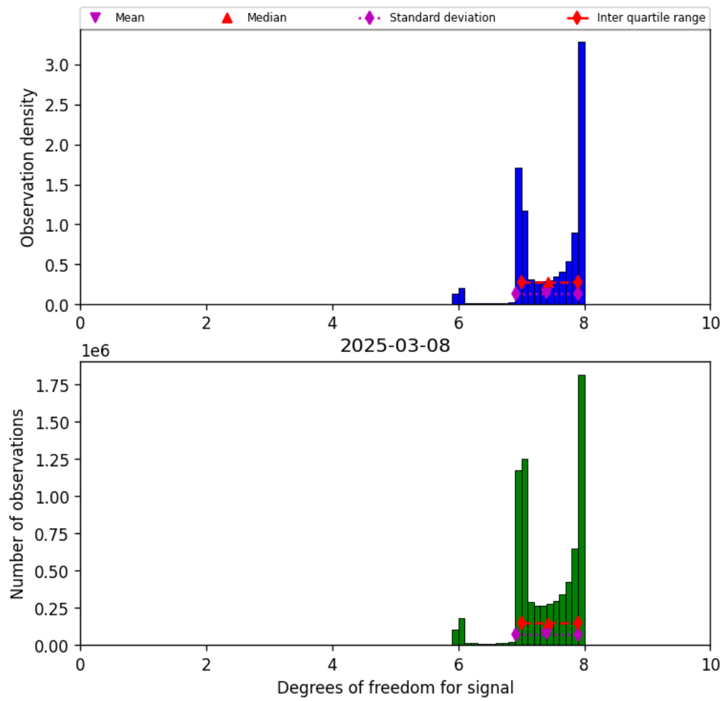
Figure 18: Histogram of “Degrees of freedom for signal” for 2025-03-08 to 2025-03-09
