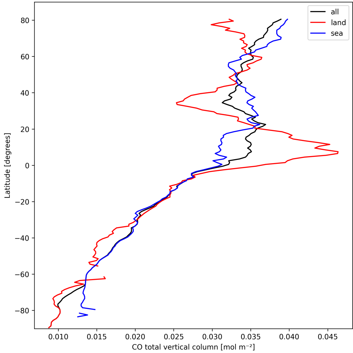
Figure 7: Zonal average of “CO total vertical column” for 2025-03-08 to 2025-03-09.
