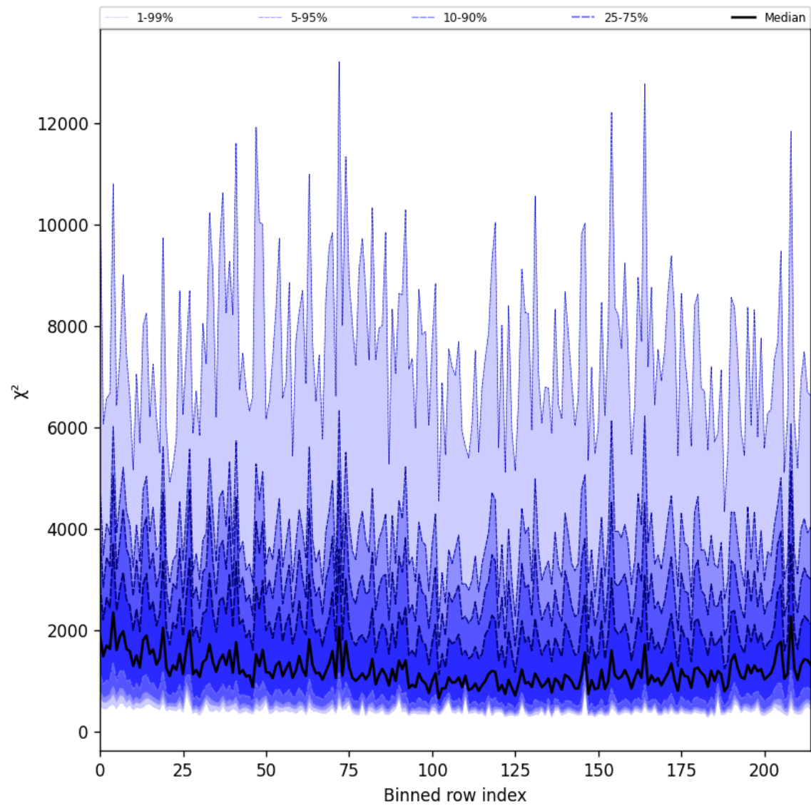
Figure 24: Along track statistics of “ \chi^2 ” for 2025-03-08 to 2025-03-09
