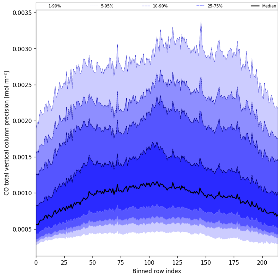
Figure 22: Along track statistics of “CO total vertical column precision” for 2025-03-08 to 2025-03-09
