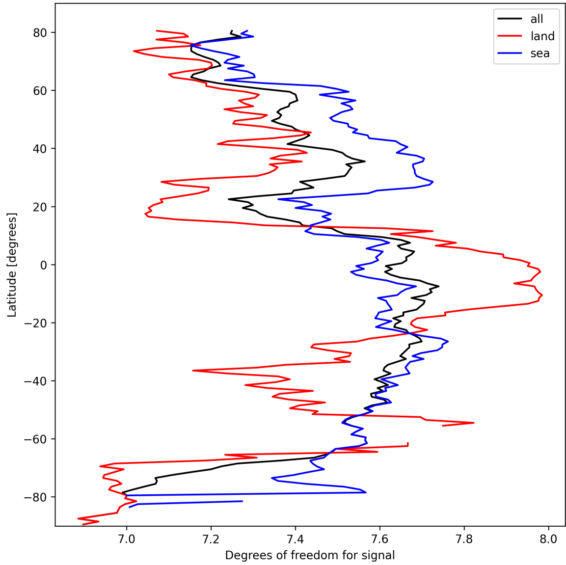
Figure 11: Zonal average of “Degrees of freedom for signal” for 2025-03-08 to 2025-03-09.
