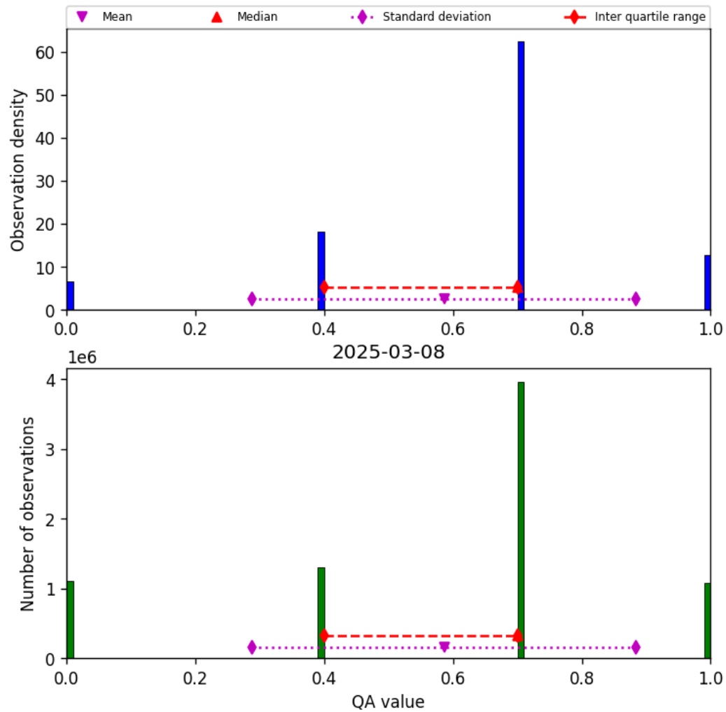
Figure 13: Histogram of “QA value” for 2025-03-08 to 2025-03-09
