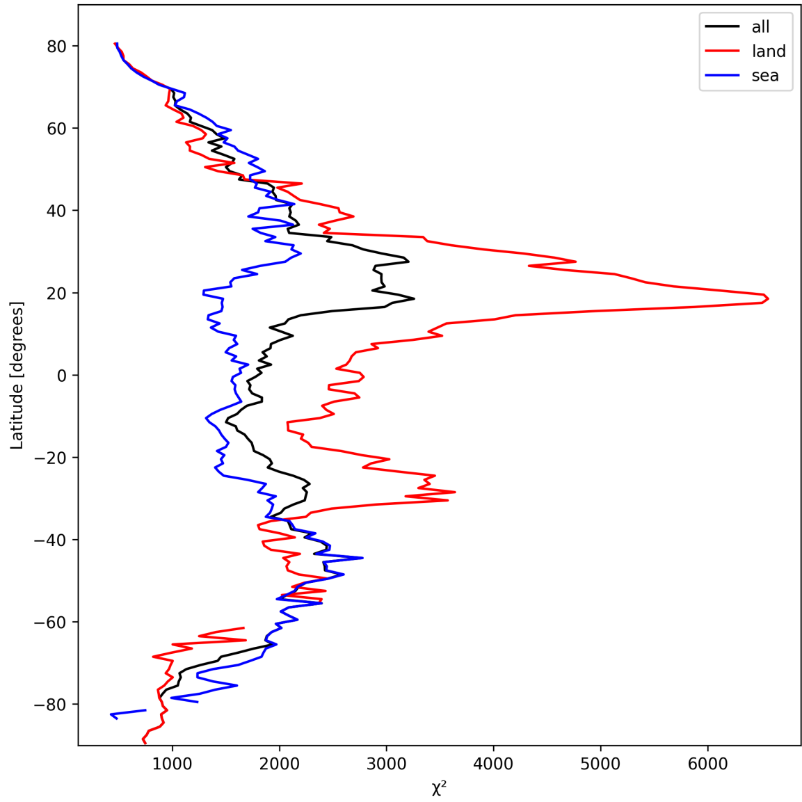
Figure 10: Zonal average of “ \chi^2 ” for 2025-03-08 to 2025-03-09.
