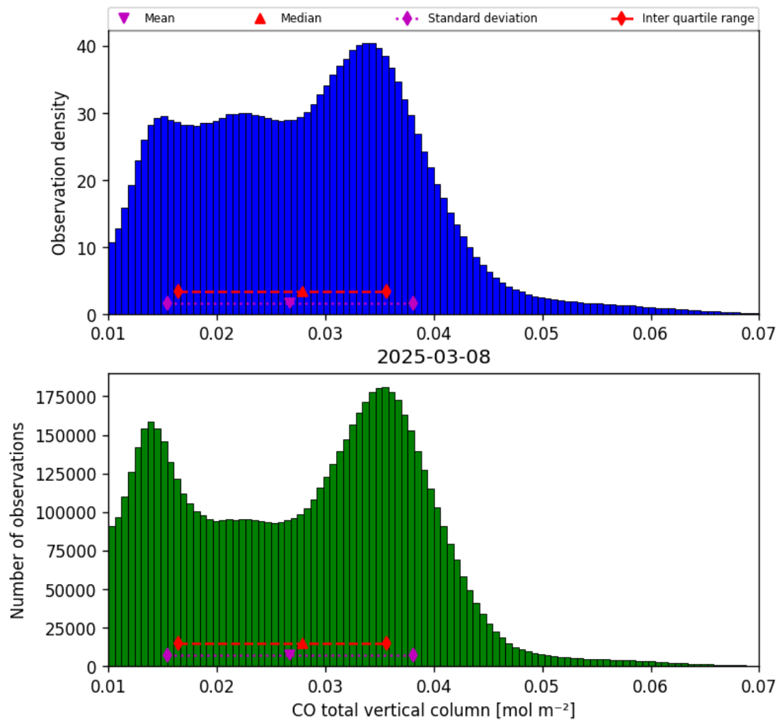
Figure 14: Histogram of “CO total vertical column” for 2025-03-08 to 2025-03-09
