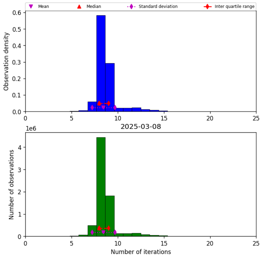
Figure 19: Histogram of “Number of iterations” for 2025-03-08 to 2025-03-09
