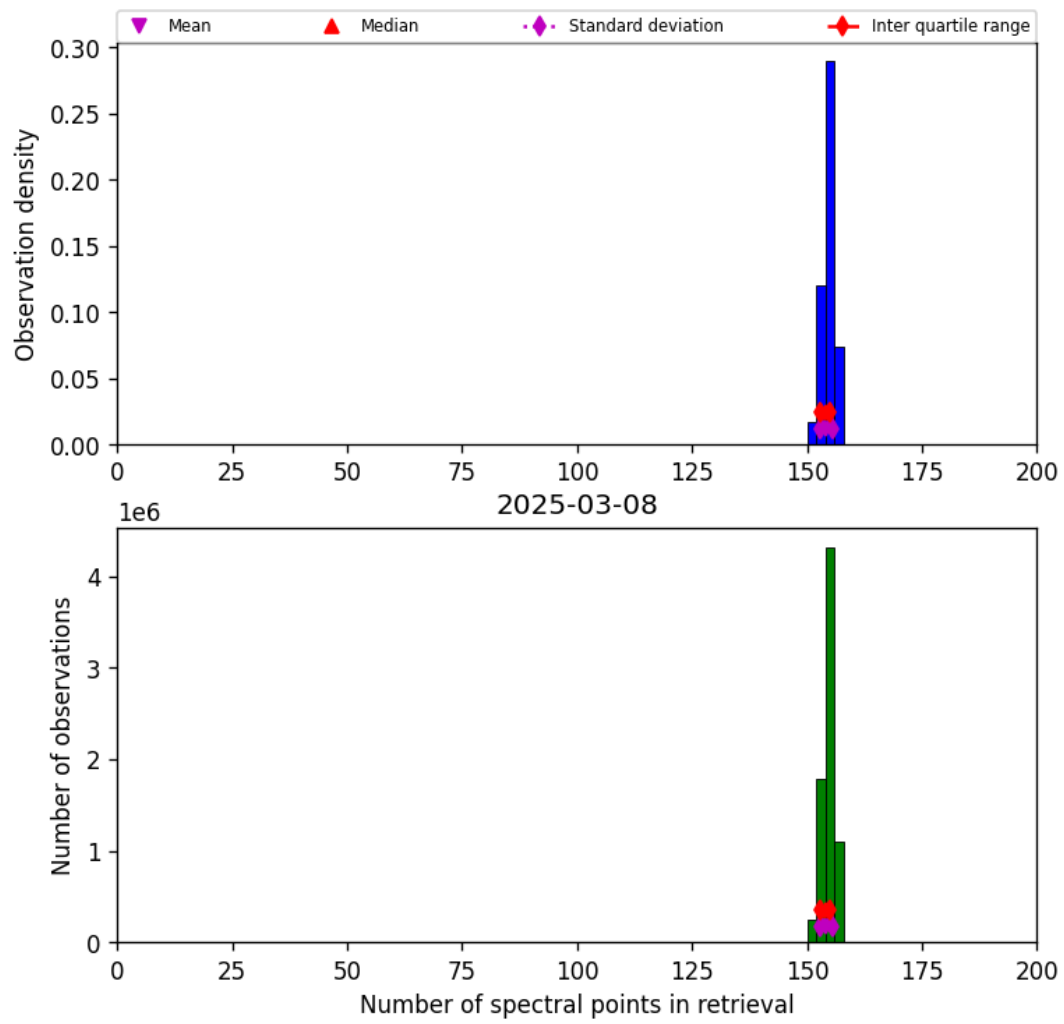
Figure 16: Histogram of “Number of spectral points in retrieval” for 2025-03-08 to 2025-03-09
