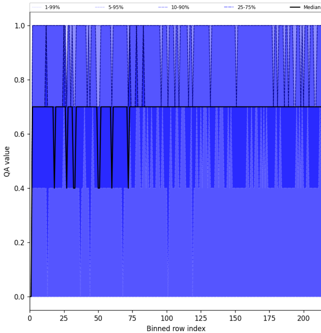
Figure 20: Along track statistics of "QA value" for 2025-03-08 to 2025-03-09
