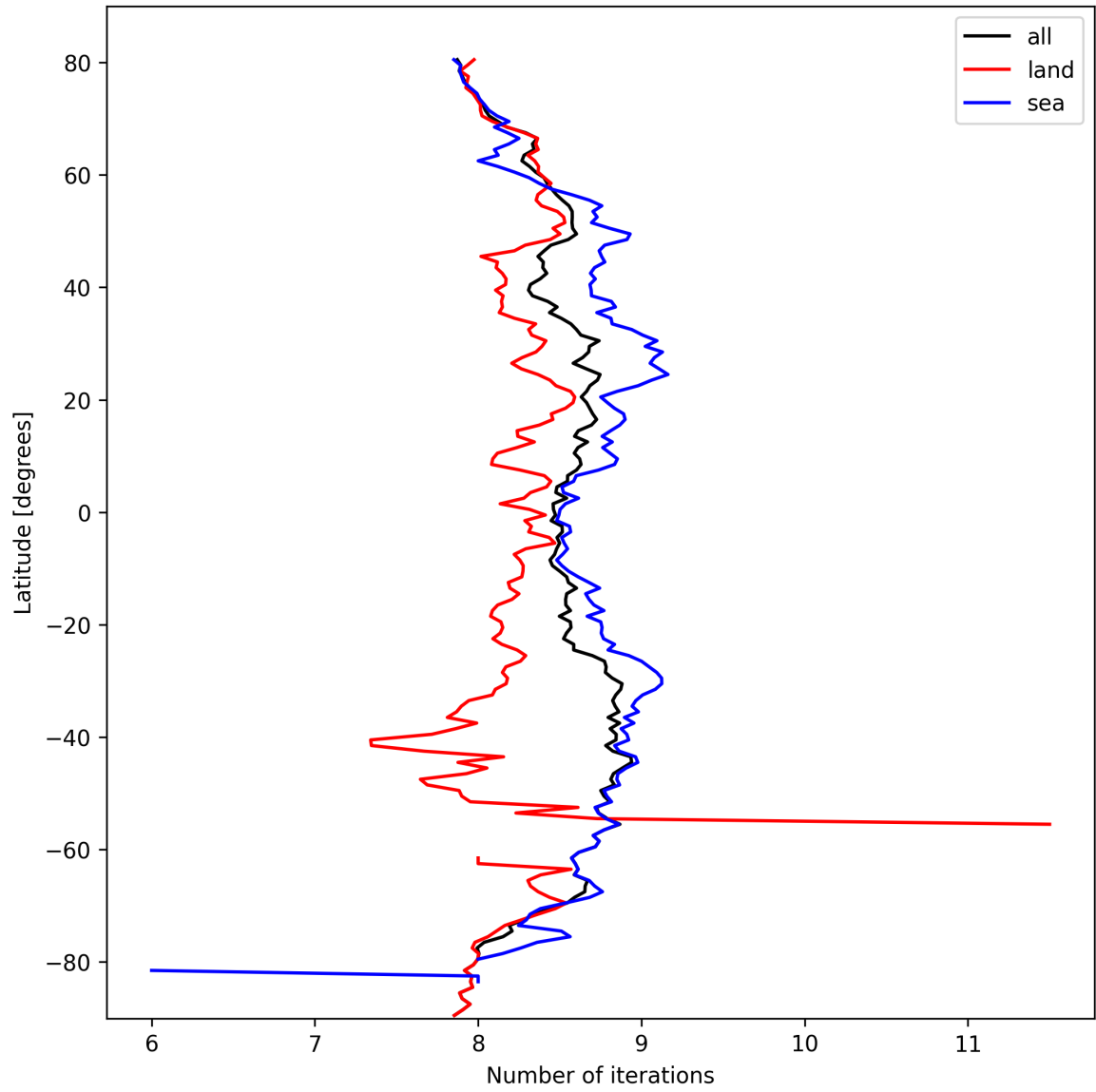
Figure 12: Zonal average of “Number of iterations” for 2025-03-08 to 2025-03-09.
