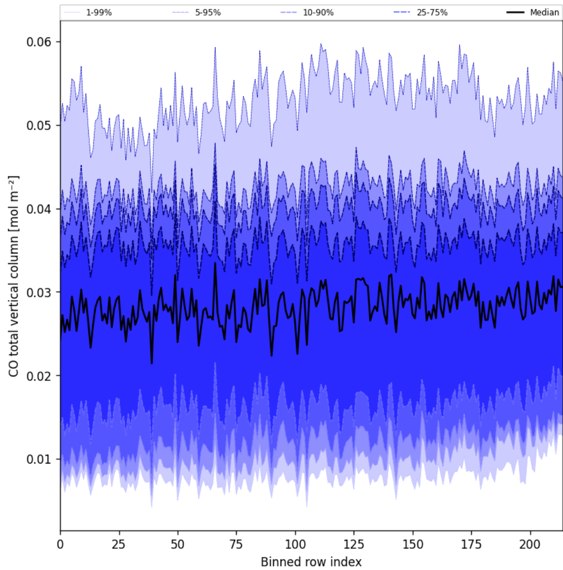
Figure 21: Along track statistics of “CO total vertical column” for 2025-03-08 to 2025-03-09
