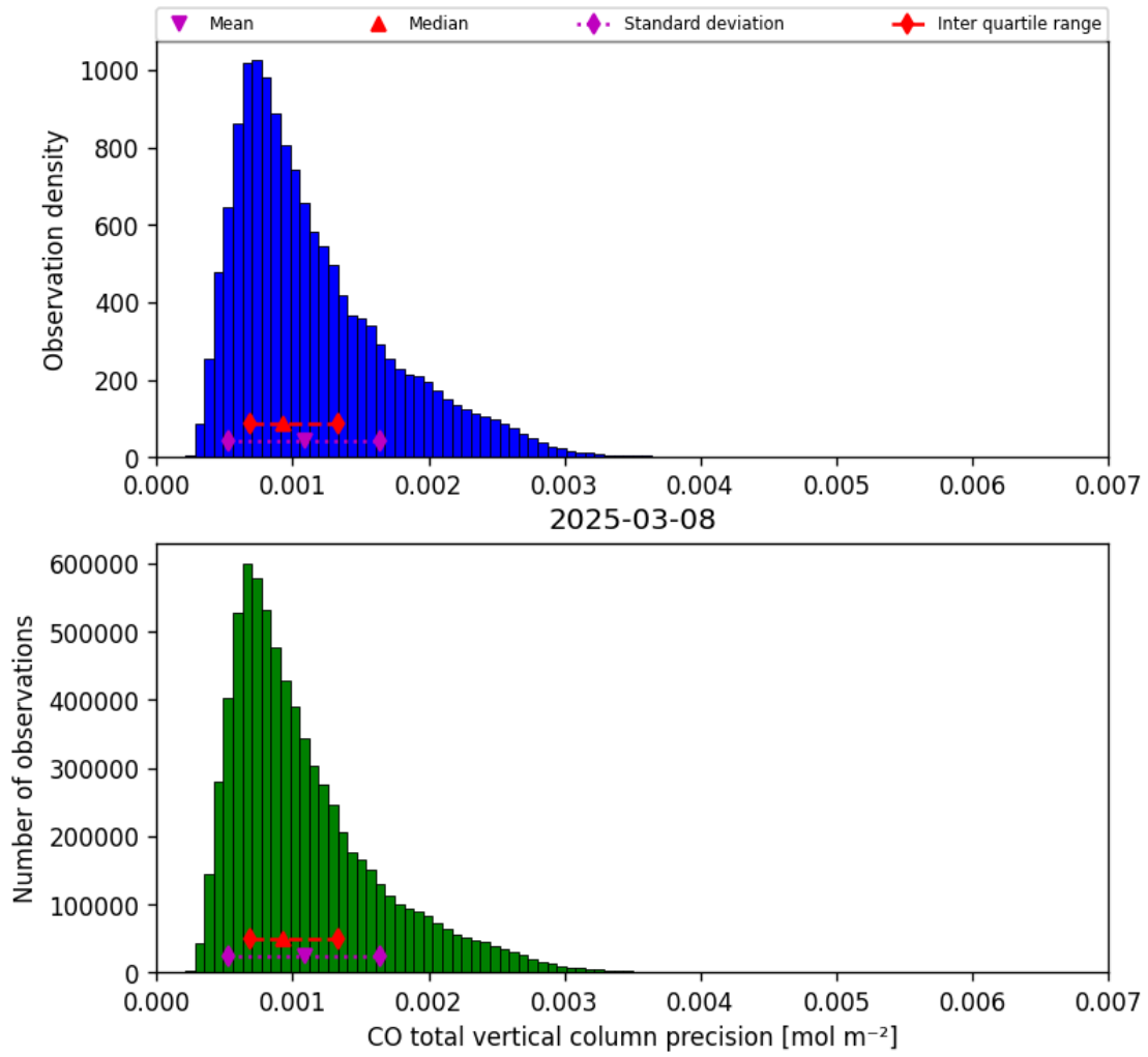
Figure 15: Histogram of “CO total vertical column precision” for 2025-03-08 to 2025-03-09
