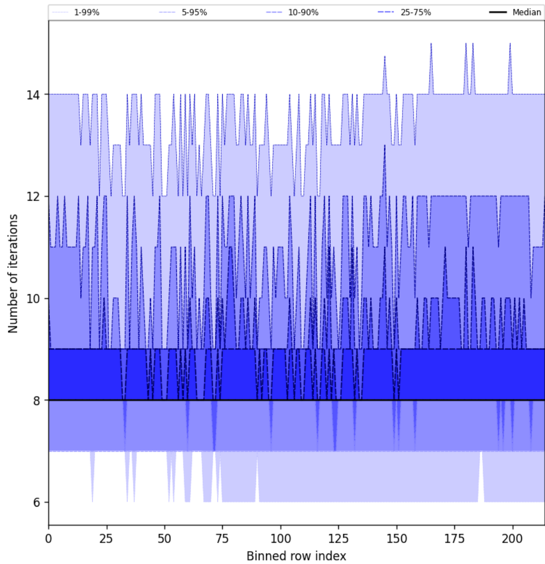
Figure 26: Along track statistics of “Number of iterations” for 2025-03-08 to 2025-03-09
