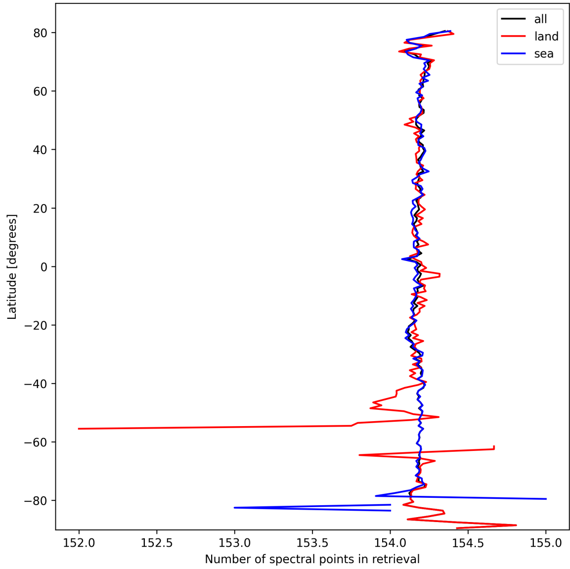
Figure 9: Zonal average of “Number of spectral points in retrieval” for 2025-03-08 to 2025-03-09.
