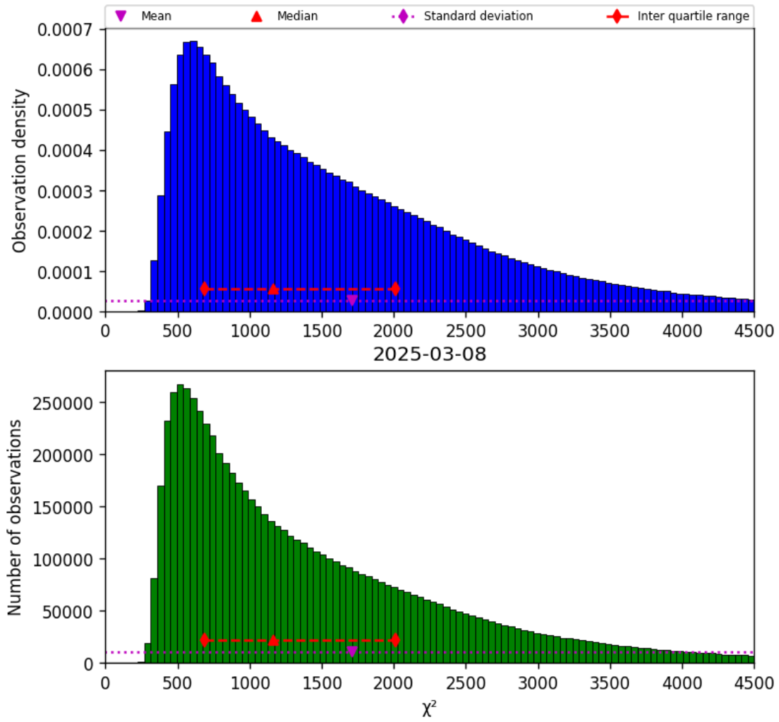
Figure 17: Histogram of " \chi^2 " for 2025-03-08 to 2025-03-09
