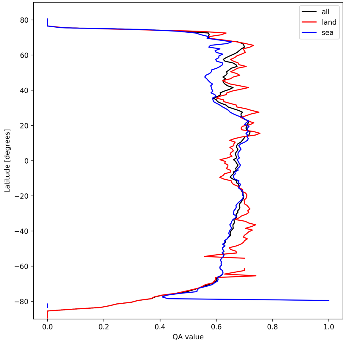
Figure 6: Zonal average of “QA value” for 2025-03-08 to 2025-03-09.
