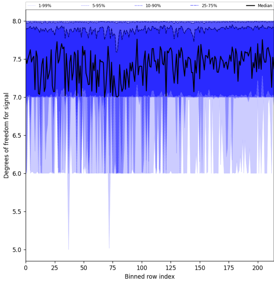
Figure 25: Along track statistics of “Degrees of freedom for signal” for 2025-03-08 to 2025-03-09
