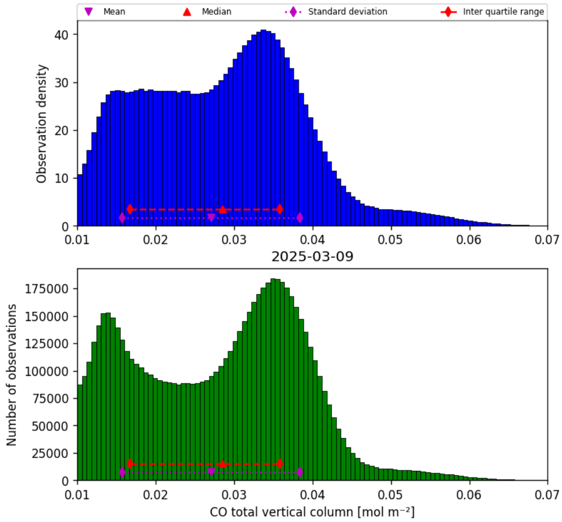
Figure 14: Histogram of “CO total vertical column” for 2025-03-09 to 2025-03-10
