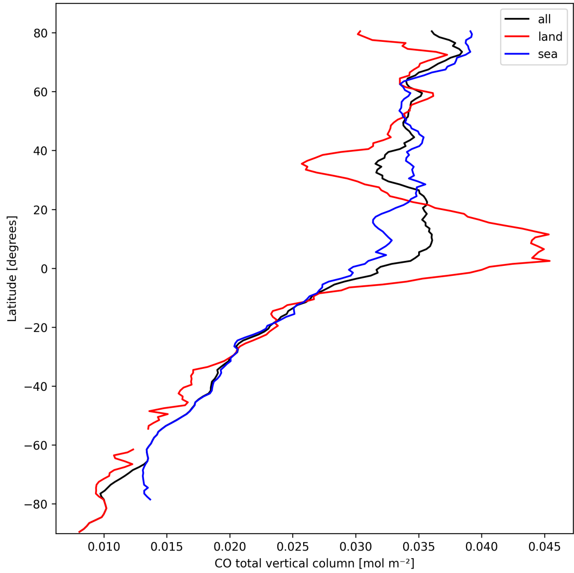
Figure 7: Zonal average of “CO total vertical column” for 2025-03-09 to 2025-03-10.
