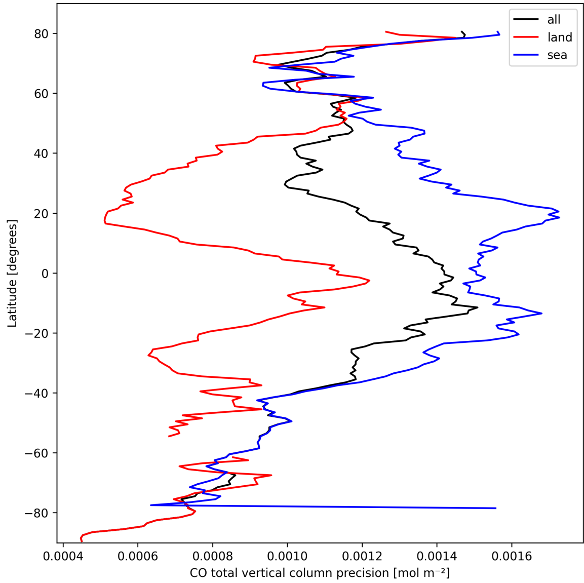
Figure 8: Zonal average of “CO total vertical column precision” for 2025-03-09 to 2025-03-10.
