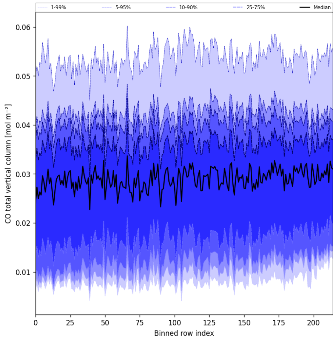
Figure 21: Along track statistics of “CO total vertical column” for 2025-03-09 to 2025-03-10
