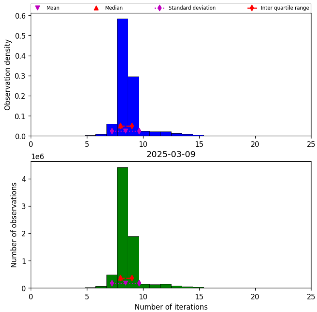
Figure 19: Histogram of “Number of iterations” for 2025-03-09 to 2025-03-10
