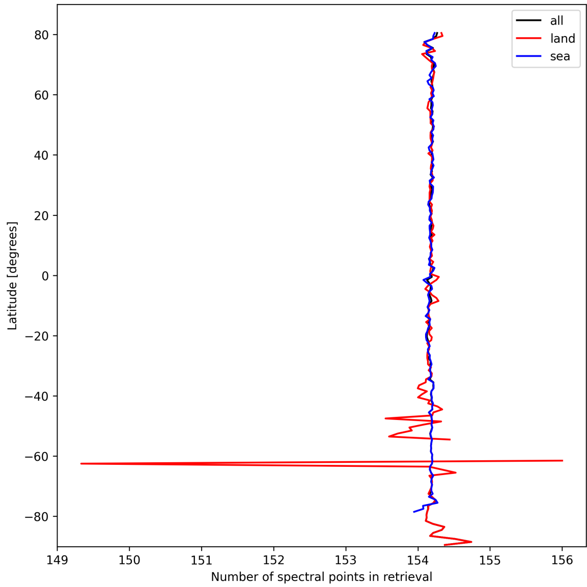
Figure 9: Zonal average of “Number of spectral points in retrieval” for 2025-03-09 to 2025-03-10.
