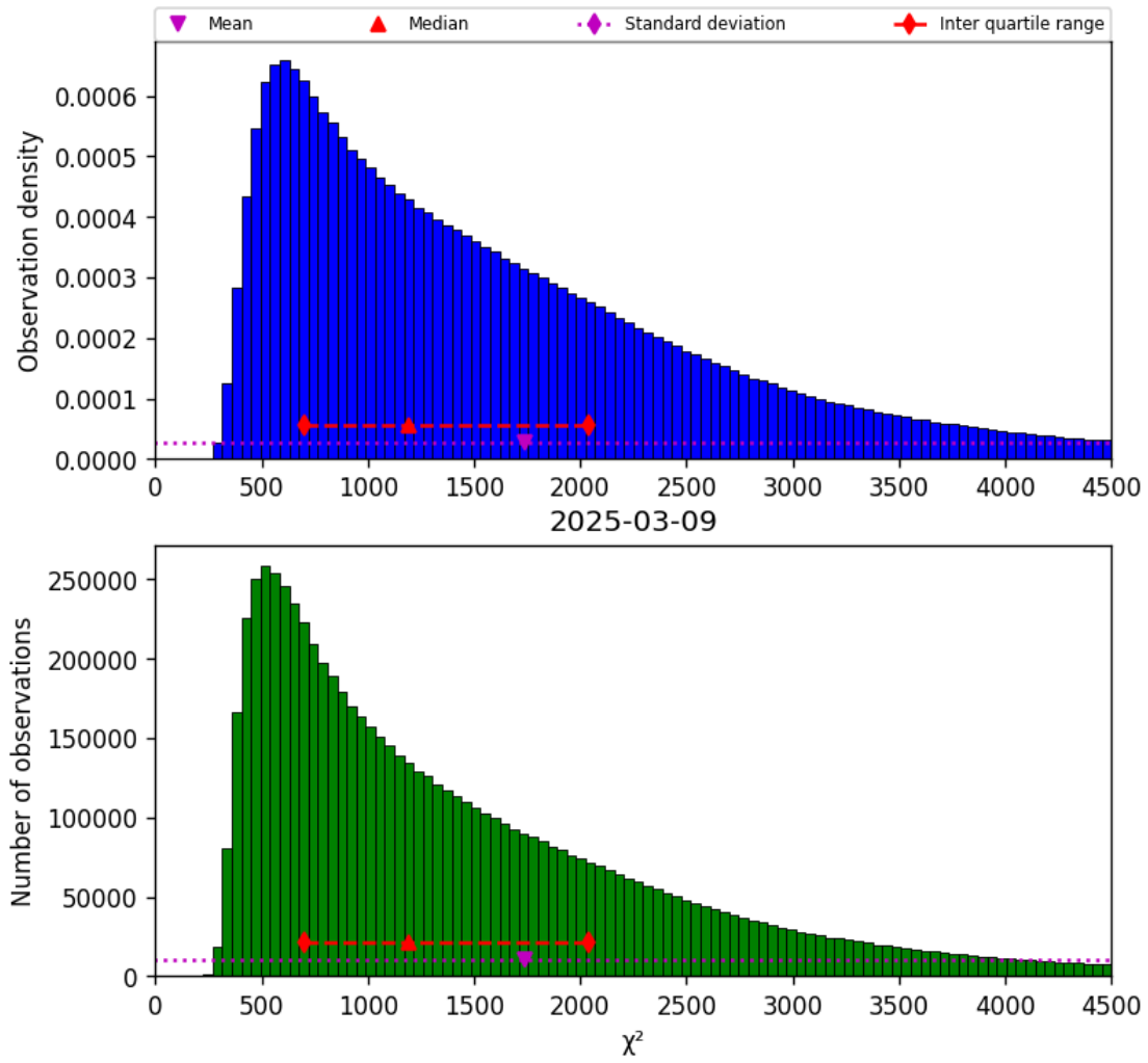
Figure 17: Histogram of “ \chi^2 ” for 2025-03-09 to 2025-03-10
