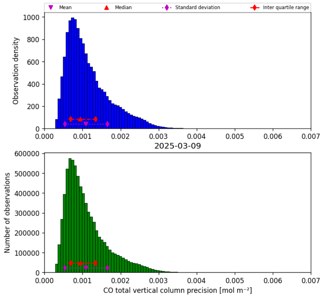
Figure 15: Histogram of “CO total vertical column precision” for 2025-03-09 to 2025-03-10
