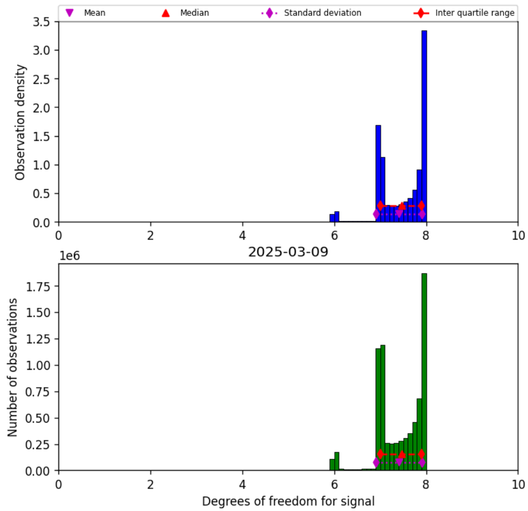
Figure 18: Histogram of “Degrees of freedom for signal” for 2025-03-09 to 2025-03-10
