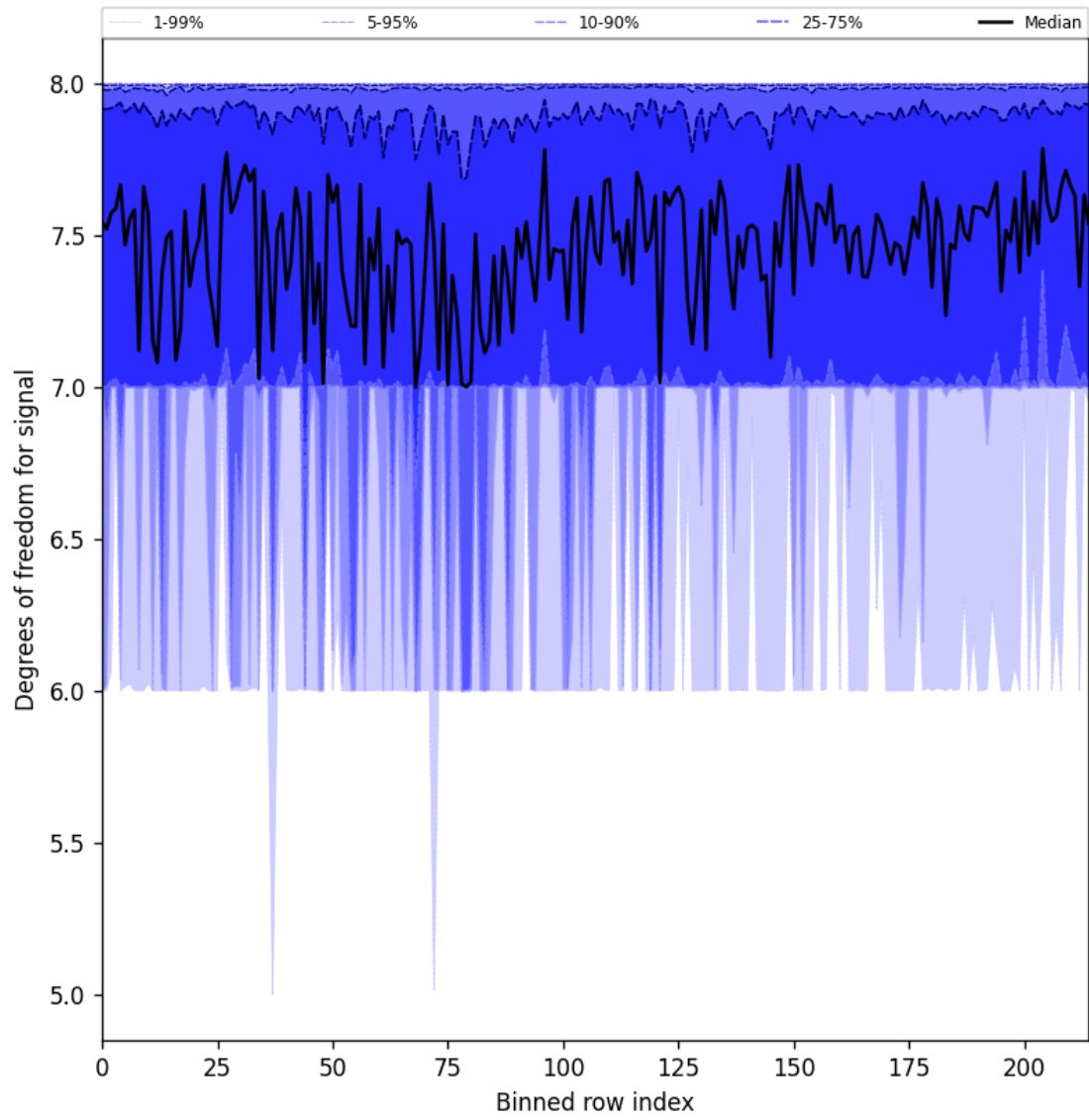
Figure 25: Along track statistics of “Degrees of freedom for signal” for 2025-03-09 to 2025-03-10
