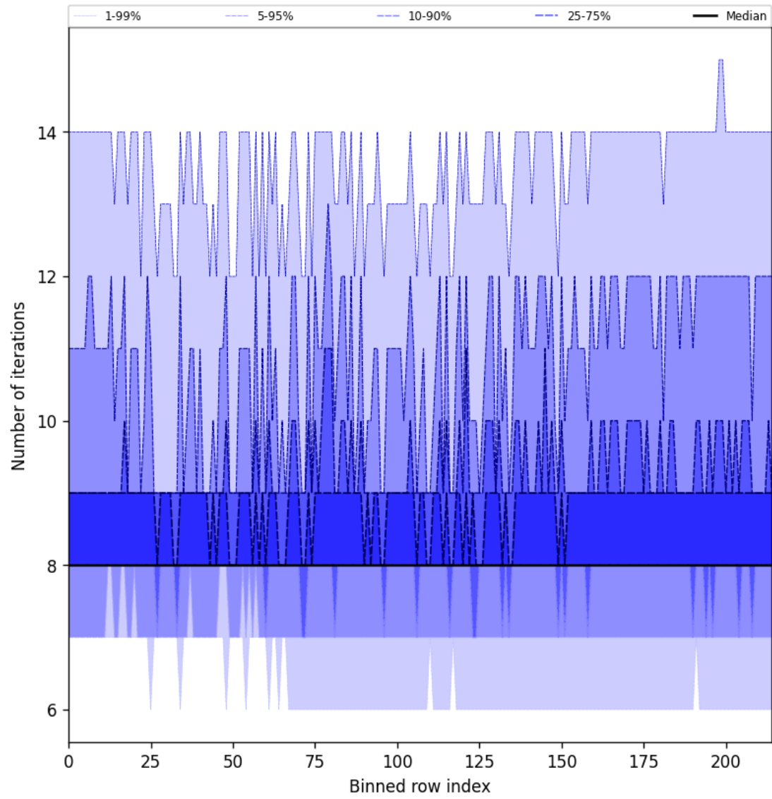
Figure 26: Along track statistics of “Number of iterations” for 2025-03-09 to 2025-03-10
