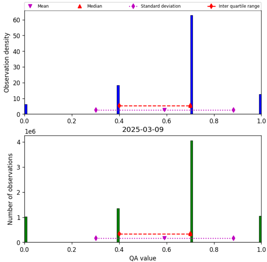
Figure 13: Histogram of “QA value” for 2025-03-09 to 2025-03-10
