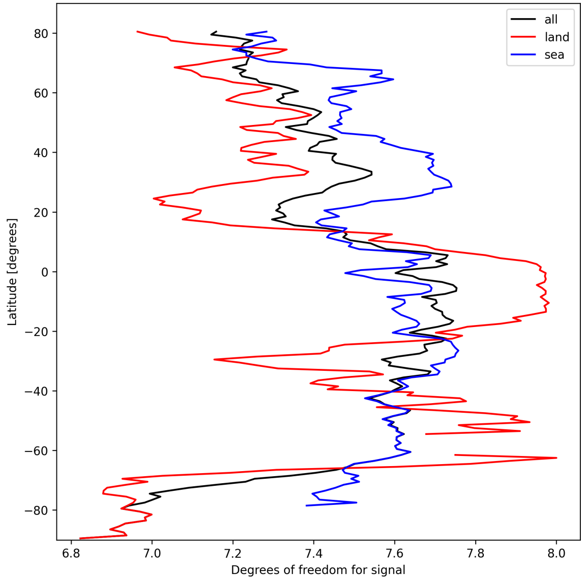
Figure 11: Zonal average of “Degrees of freedom for signal” for 2025-03-09 to 2025-03-10.
