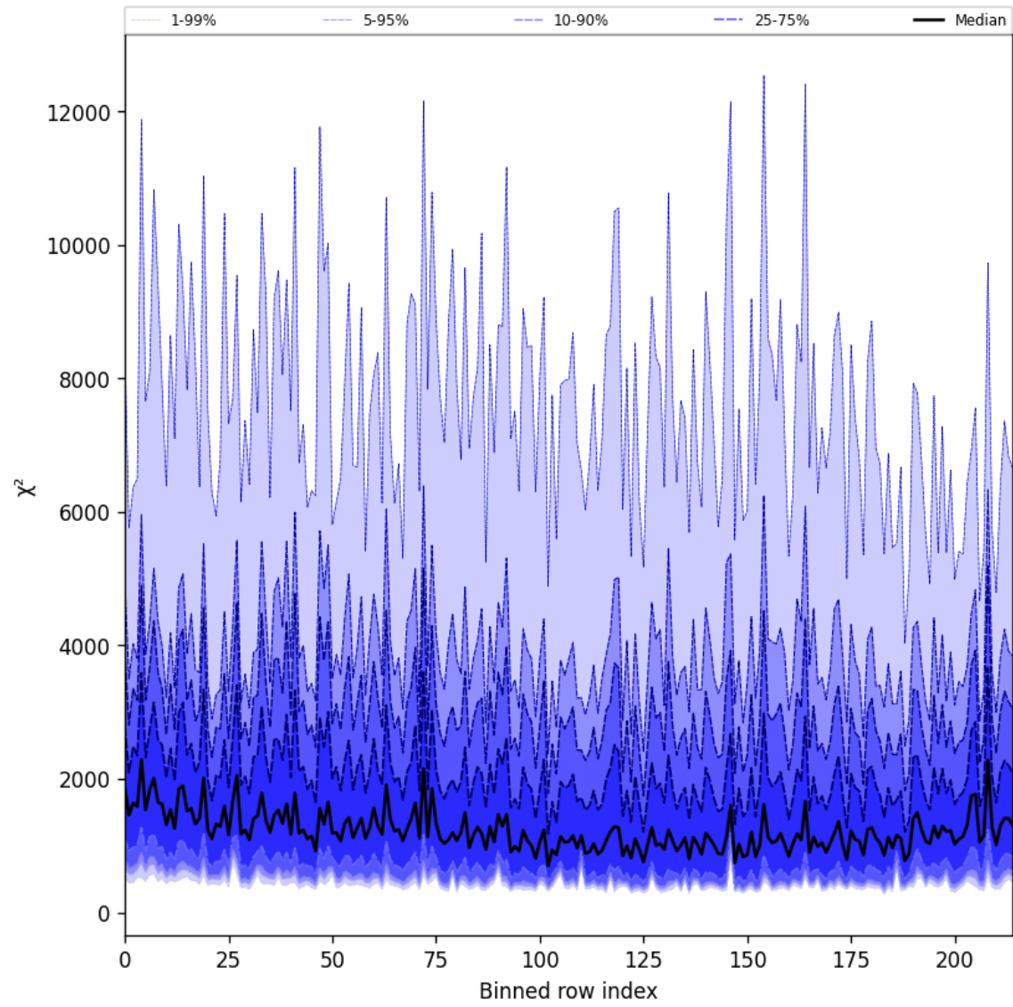
Figure 24: Along track statistics of “ \chi^2 ” for 2025-03-09 to 2025-03-10
