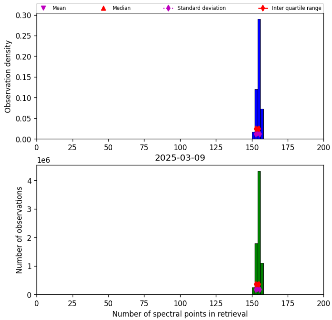
Figure 16: Histogram of “Number of spectral points in retrieval” for 2025-03-09 to 2025-03-10
