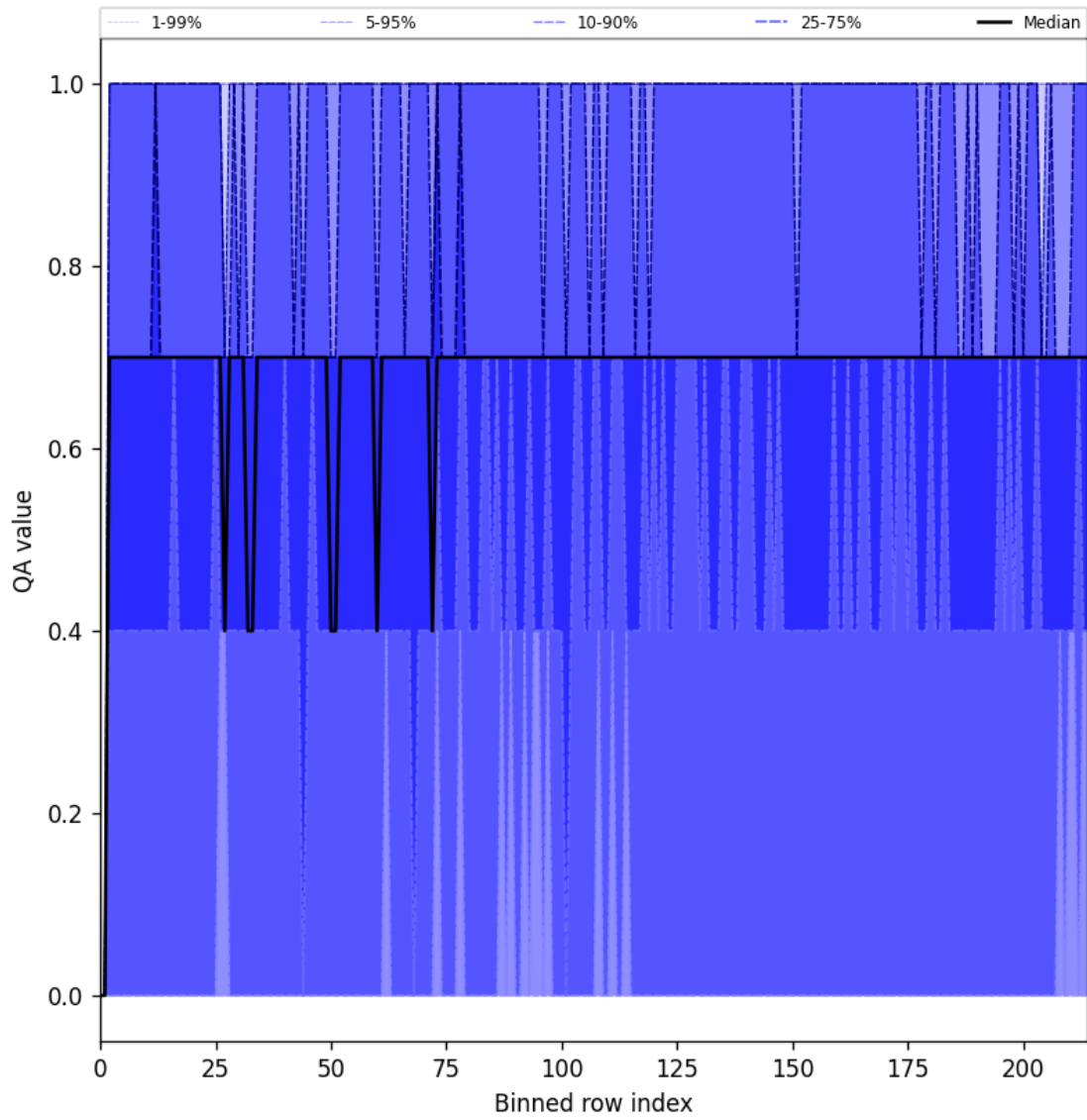
Figure 20: Along track statistics of “QA value” for 2025-03-09 to 2025-03-10
