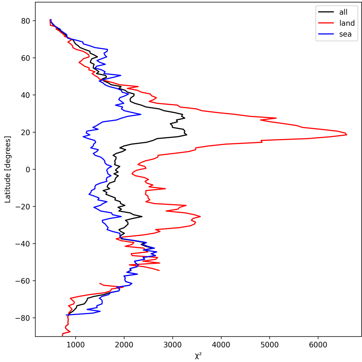
Figure 10: Zonal average of “ \chi^2 ” for 2025-03-09 to 2025-03-10.
