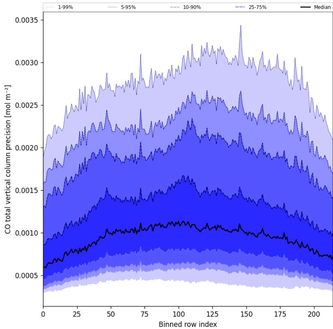
Figure 22: Along track statistics of “CO total vertical column precision” for 2025-03-09 to 2025-03-10
