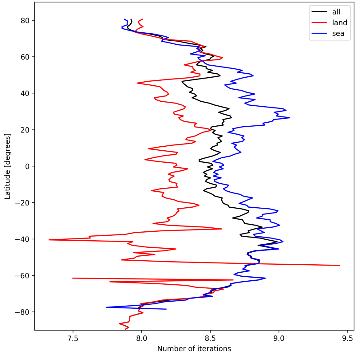
Figure 12: Zonal average of “Number of iterations” for 2025-03-09 to 2025-03-10.
