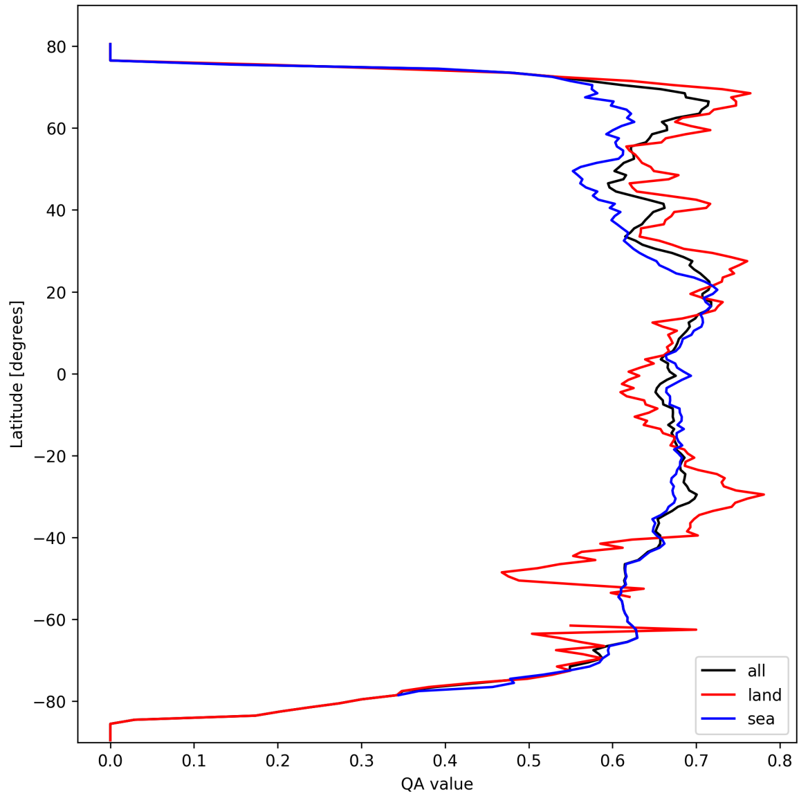
Figure 6: Zonal average of “QA value” for 2025-03-09 to 2025-03-10.
