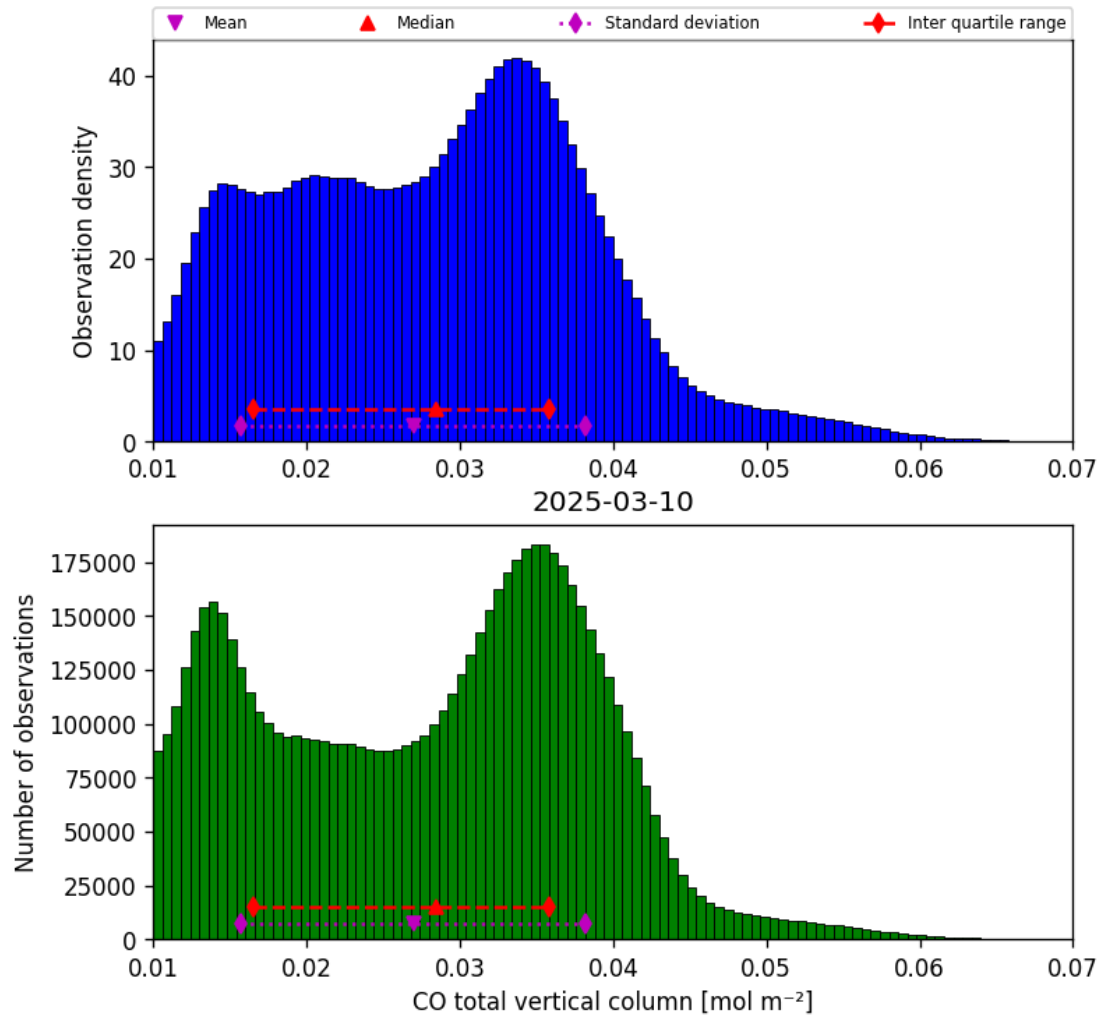
Figure 14: Histogram of “CO total vertical column” for 2025-03-10 to 2025-03-10
