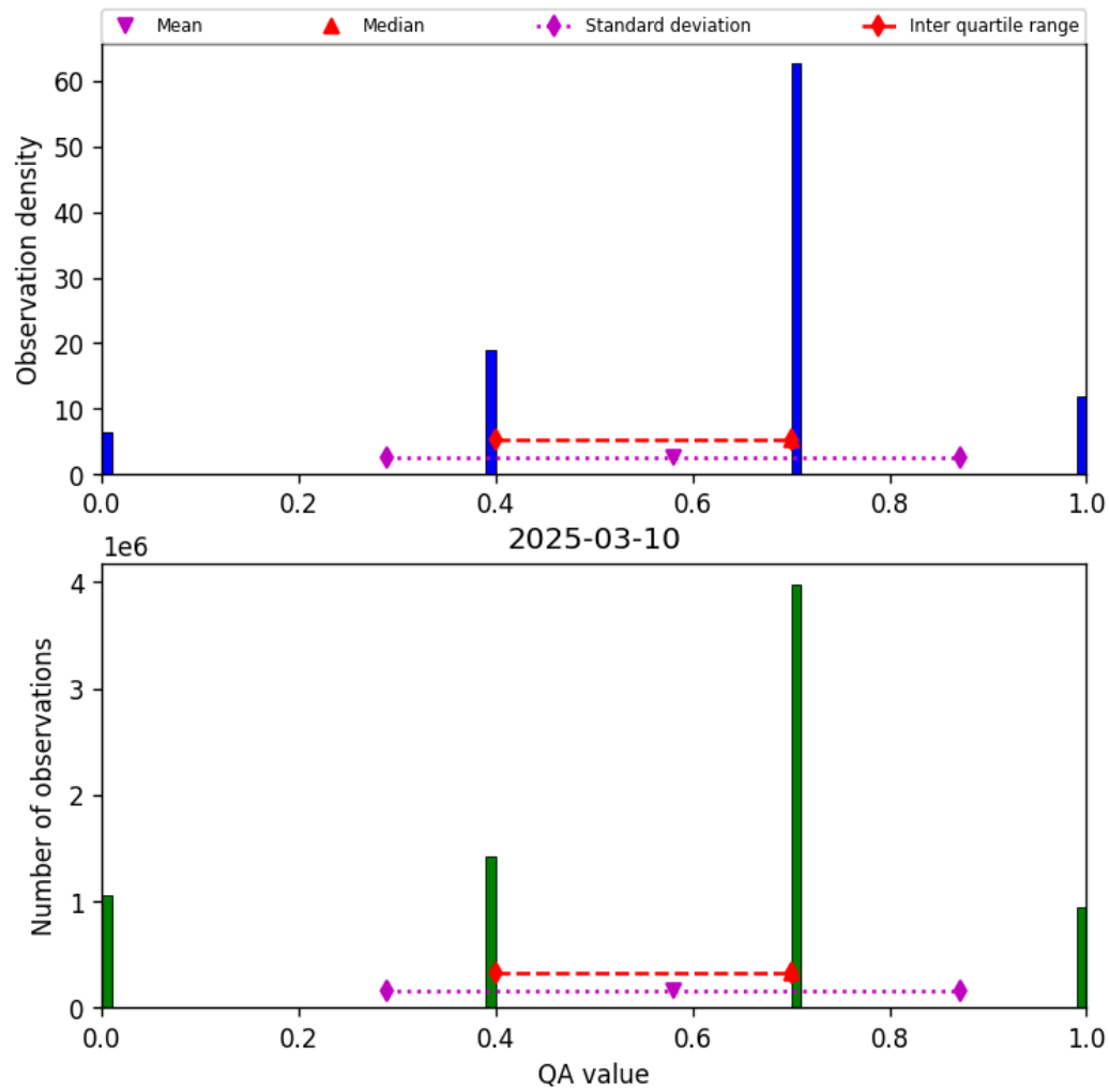
Figure 13: Histogram of “QA value” for 2025-03-10 to 2025-03-10
