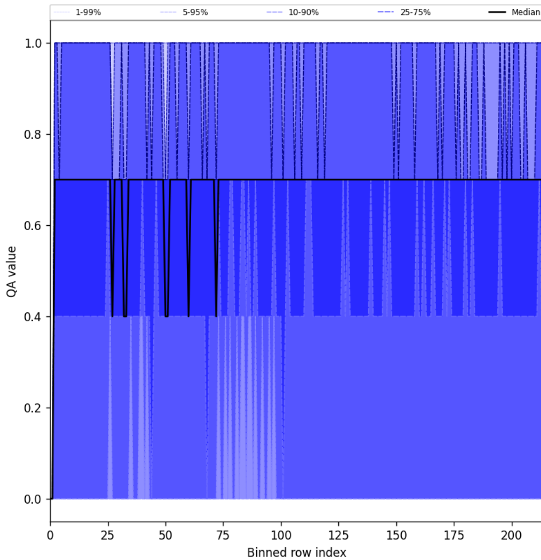
Figure 20: Along track statistics of “QA value” for 2025-03-10 to 2025-03-10
