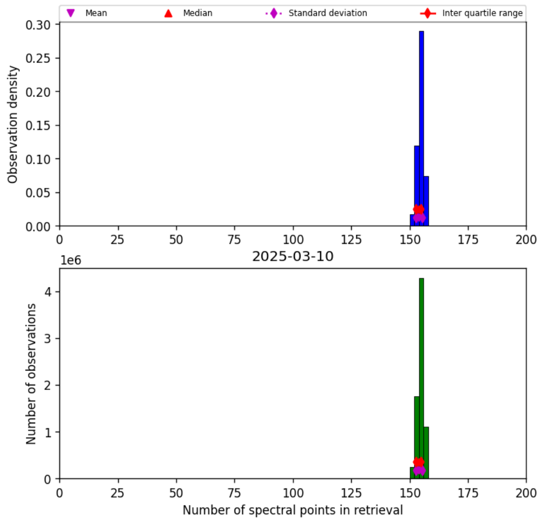
Figure 16: Histogram of “Number of spectral points in retrieval” for 2025-03-10 to 2025-03-10
