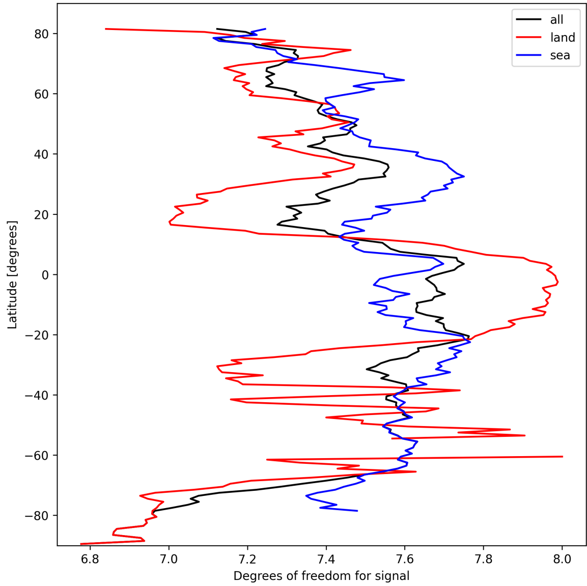
Figure 11: Zonal average of “Degrees of freedom for signal” for 2025-03-10 to 2025-03-10.
