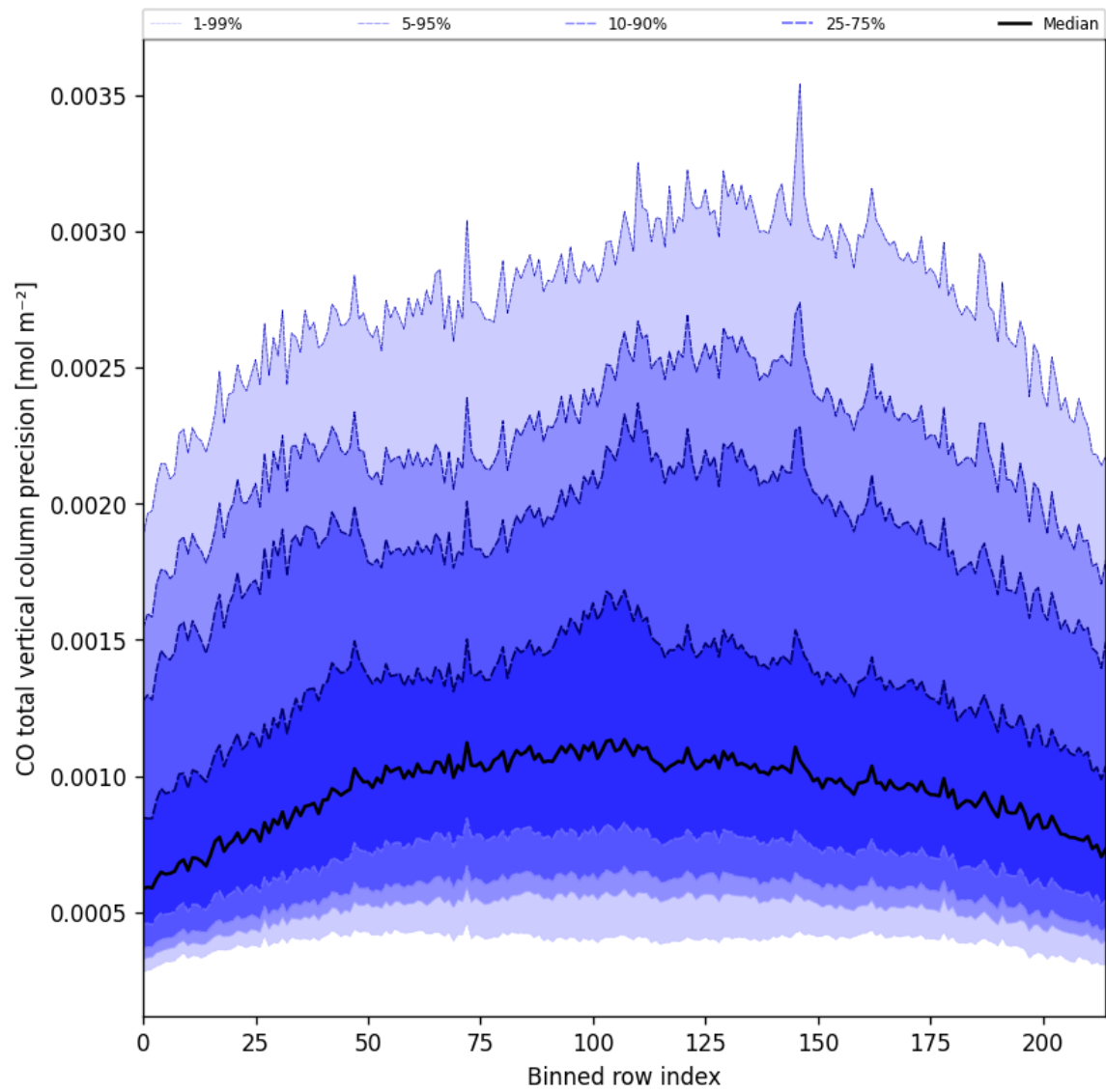
Figure 22: Along track statistics of “CO total vertical column precision” for 2025-03-10 to 2025-03-10
