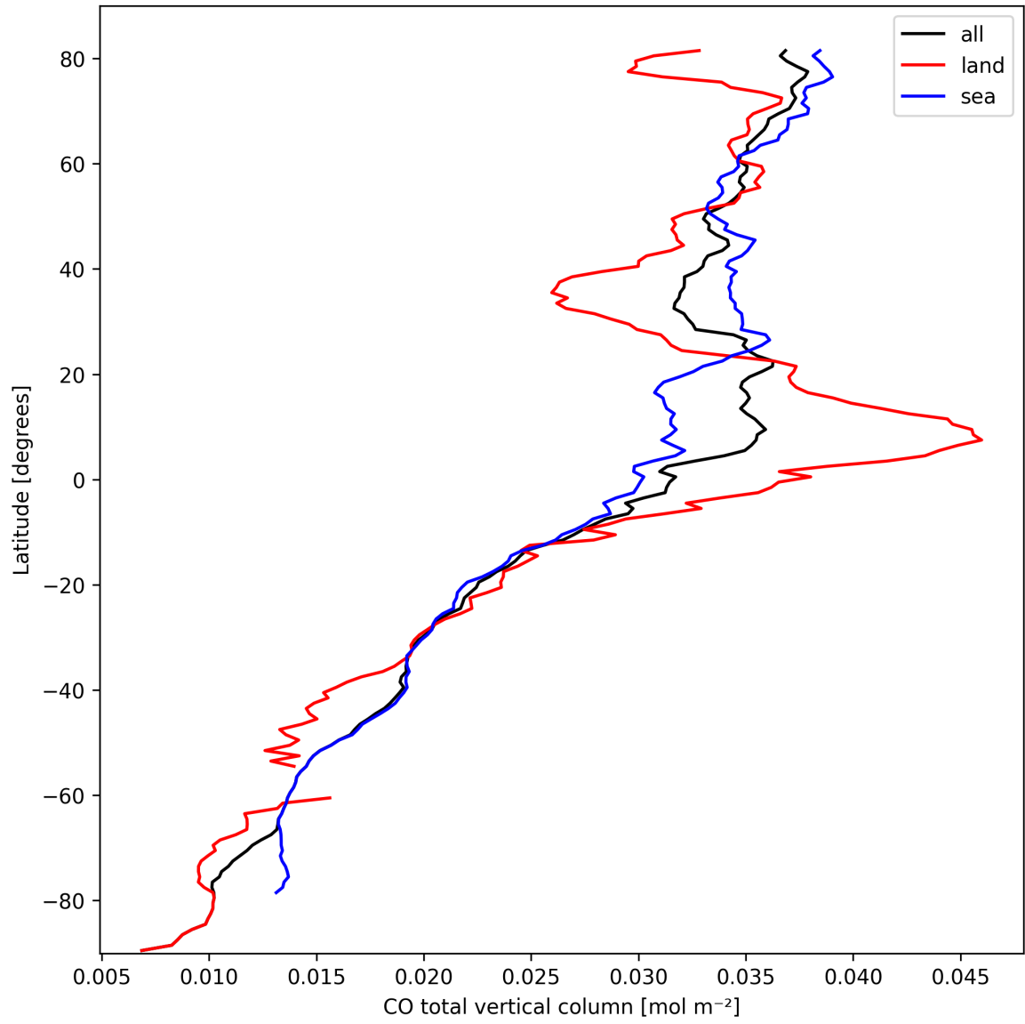
Figure 7: Zonal average of “CO total vertical column” for 2025-03-10 to 2025-03-10.
