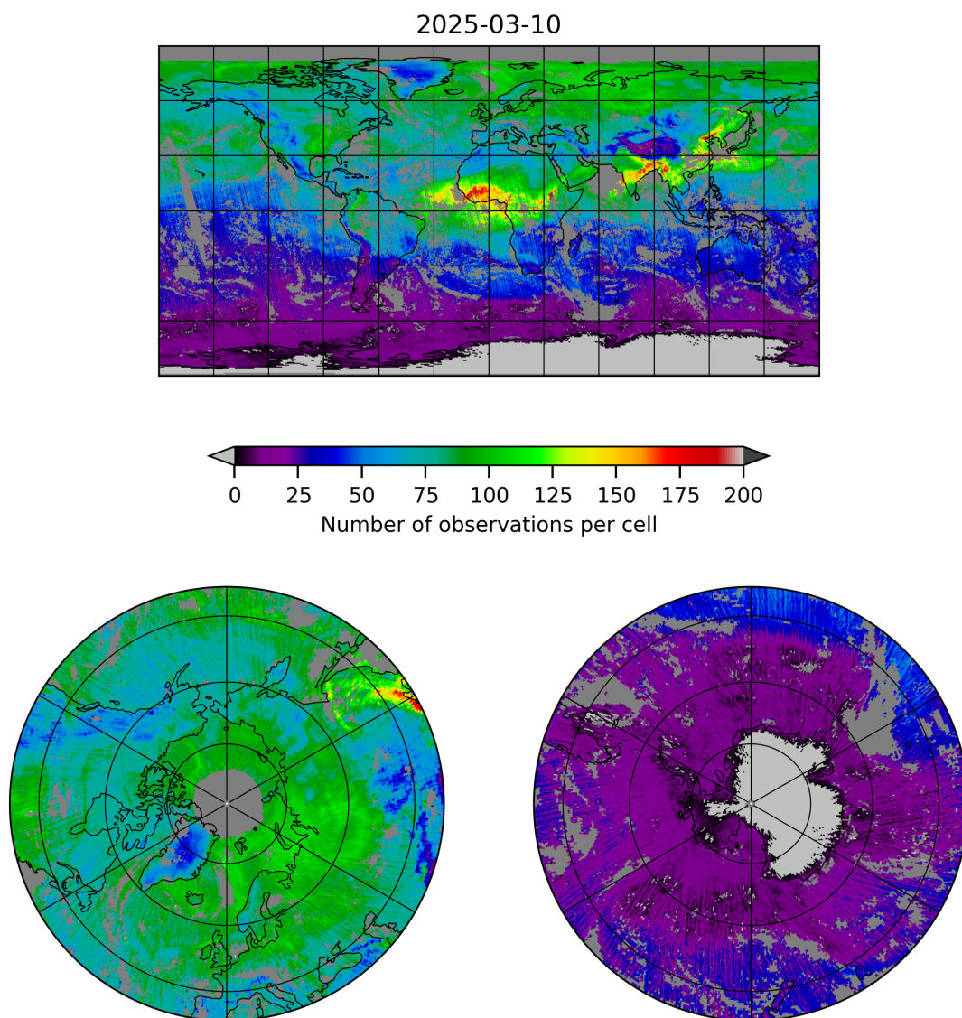
Figure 5: Map of the number of observations for 2025-03-10 to 2025-03-10
