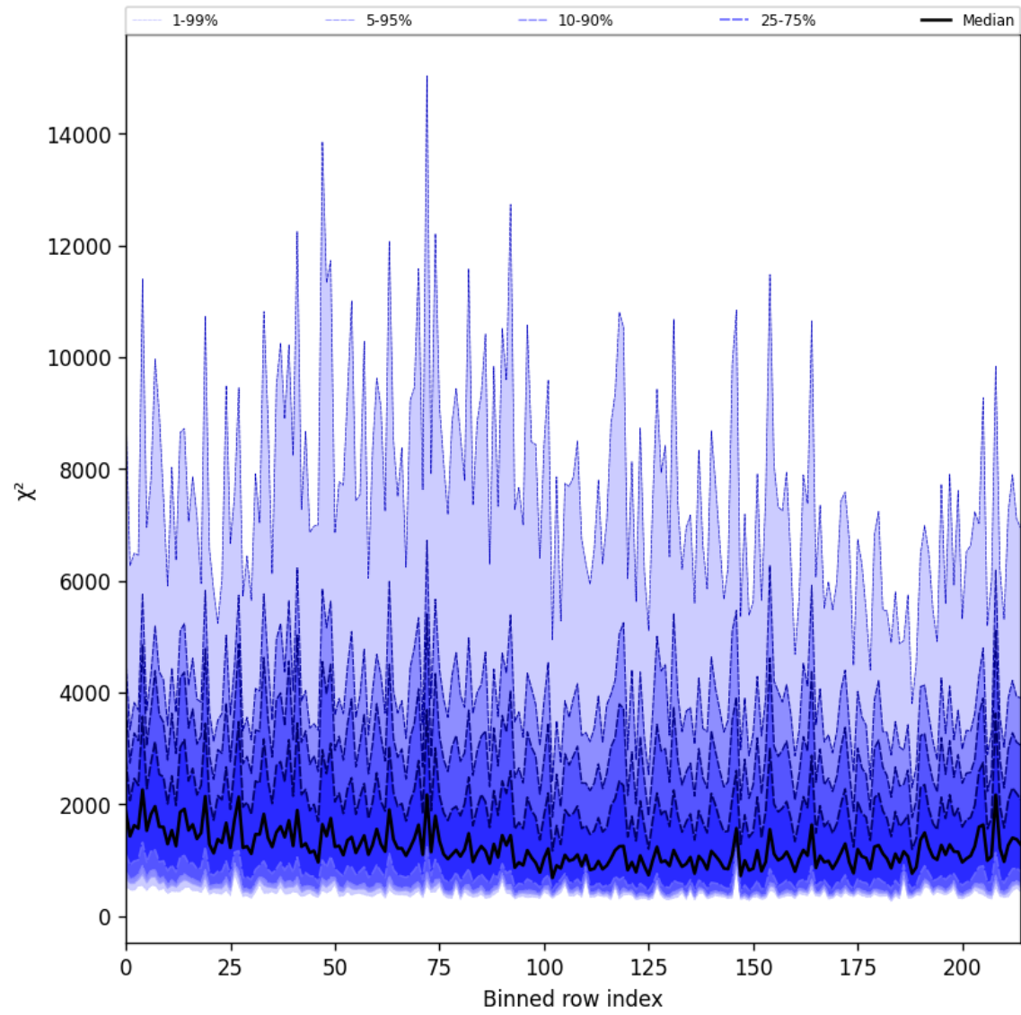
Figure 24: Along track statistics of “ \chi^2 ” for 2025-03-10 to 2025-03-10
