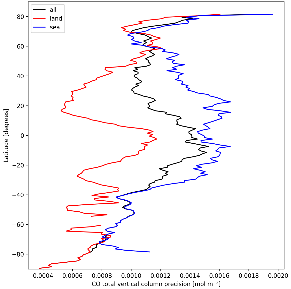
Figure 8: Zonal average of “CO total vertical column precision” for 2025-03-10 to 2025-03-10.
