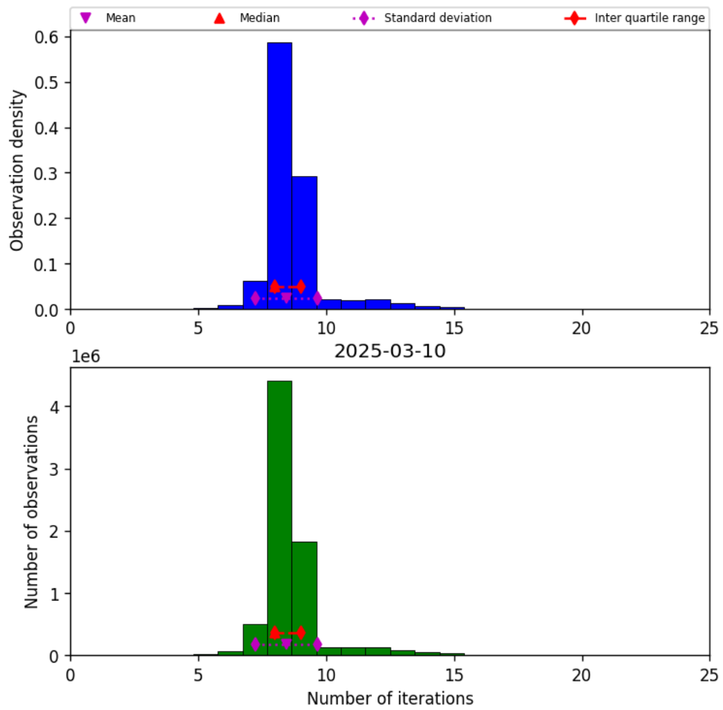
Figure 19: Histogram of “Number of iterations” for 2025-03-10 to 2025-03-10
