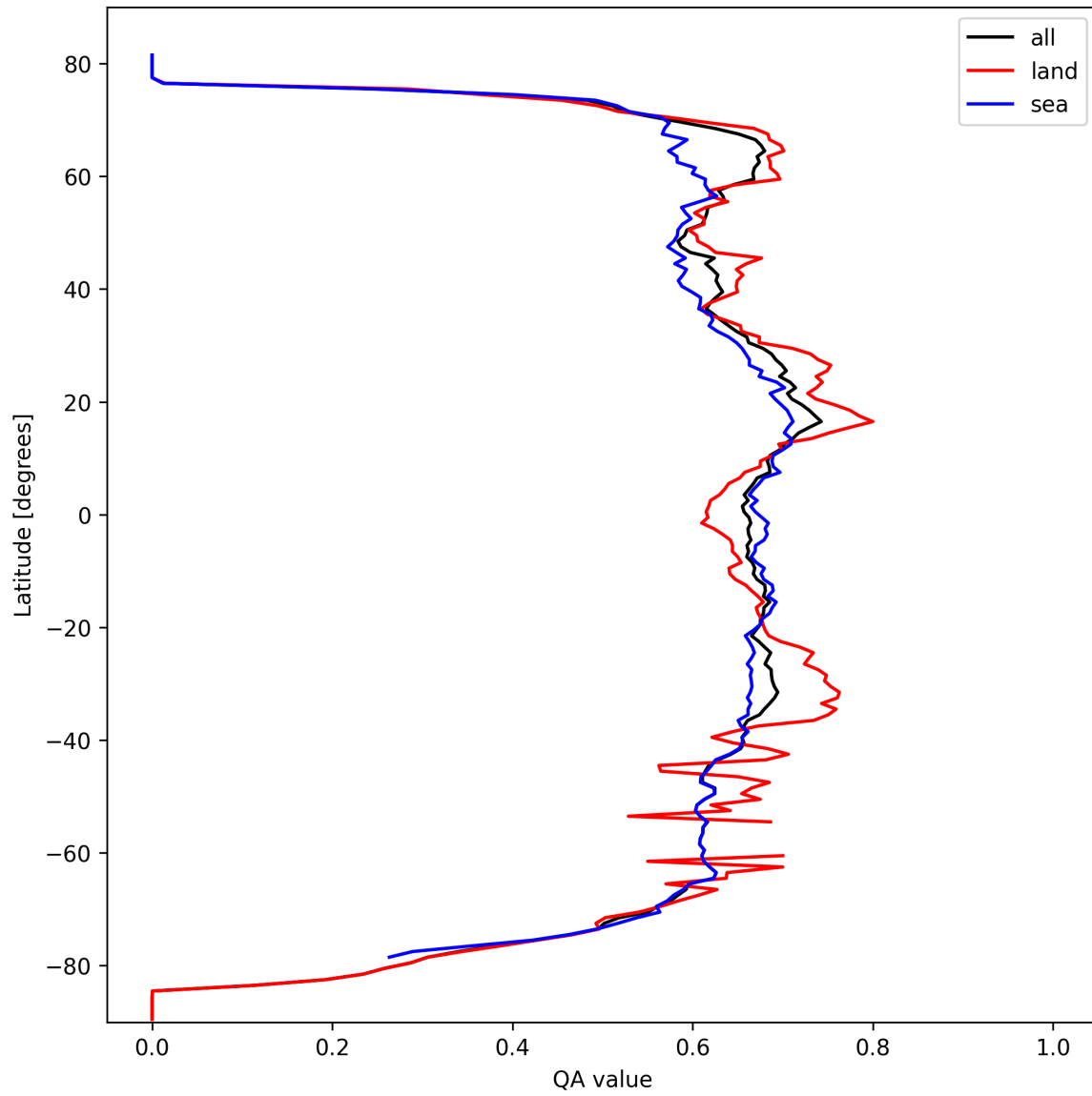
Figure 6: Zonal average of “QA value” for 2025-03-10 to 2025-03-10.
