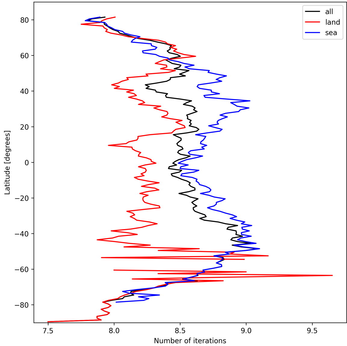
Figure 12: Zonal average of “Number of iterations” for 2025-03-10 to 2025-03-10.
