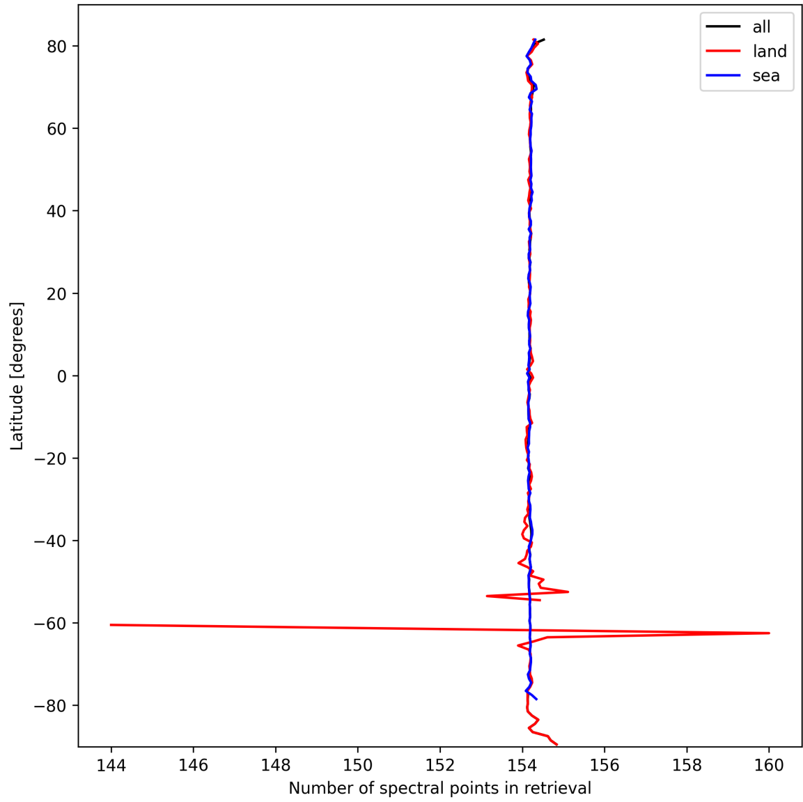
Figure 9: Zonal average of “Number of spectral points in retrieval” for 2025-03-10 to 2025-03-10.
