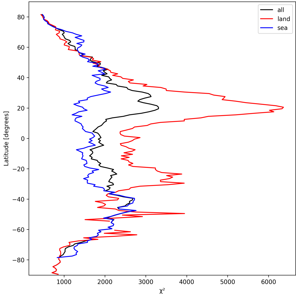
Figure 10: Zonal average of “ \chi^2 ” for 2025-03-10 to 2025-03-10.
