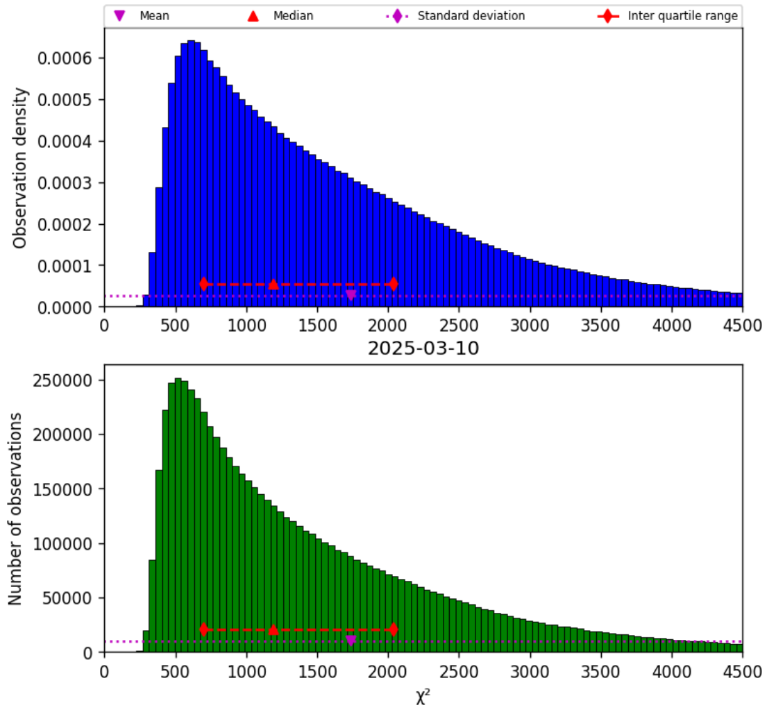
Figure 17: Histogram of " \chi^2 " for 2025-03-10 to 2025-03-10
