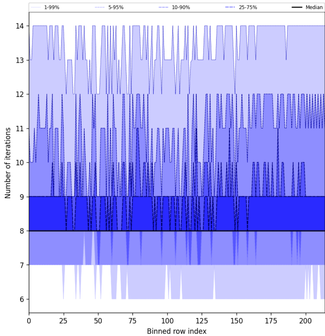
Figure 26: Along track statistics of “Number of iterations” for 2025-03-10 to 2025-03-10
