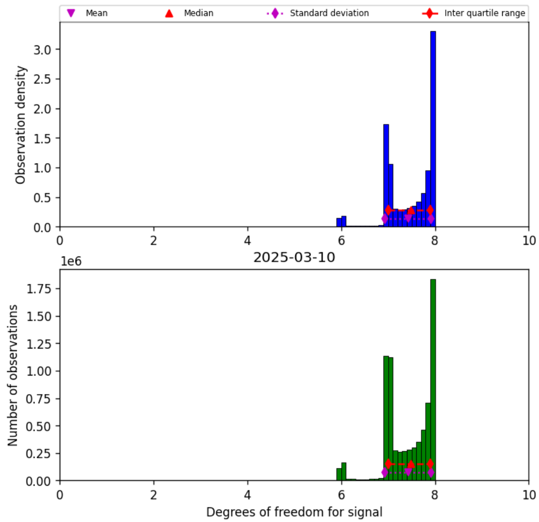
Figure 18: Histogram of “Degrees of freedom for signal” for 2025-03-10 to 2025-03-10
