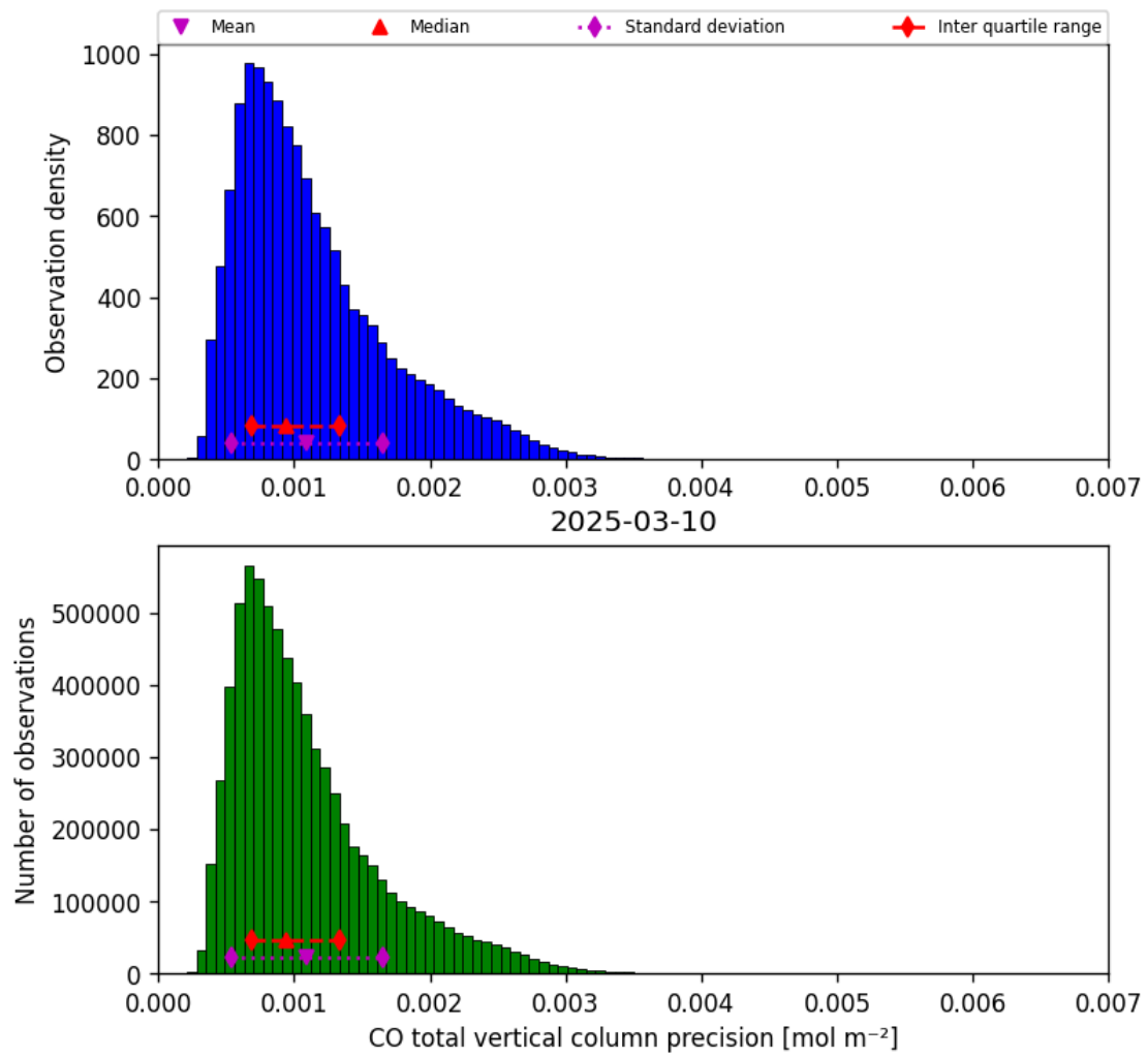
Figure 15: Histogram of “CO total vertical column precision” for 2025-03-10 to 2025-03-10
