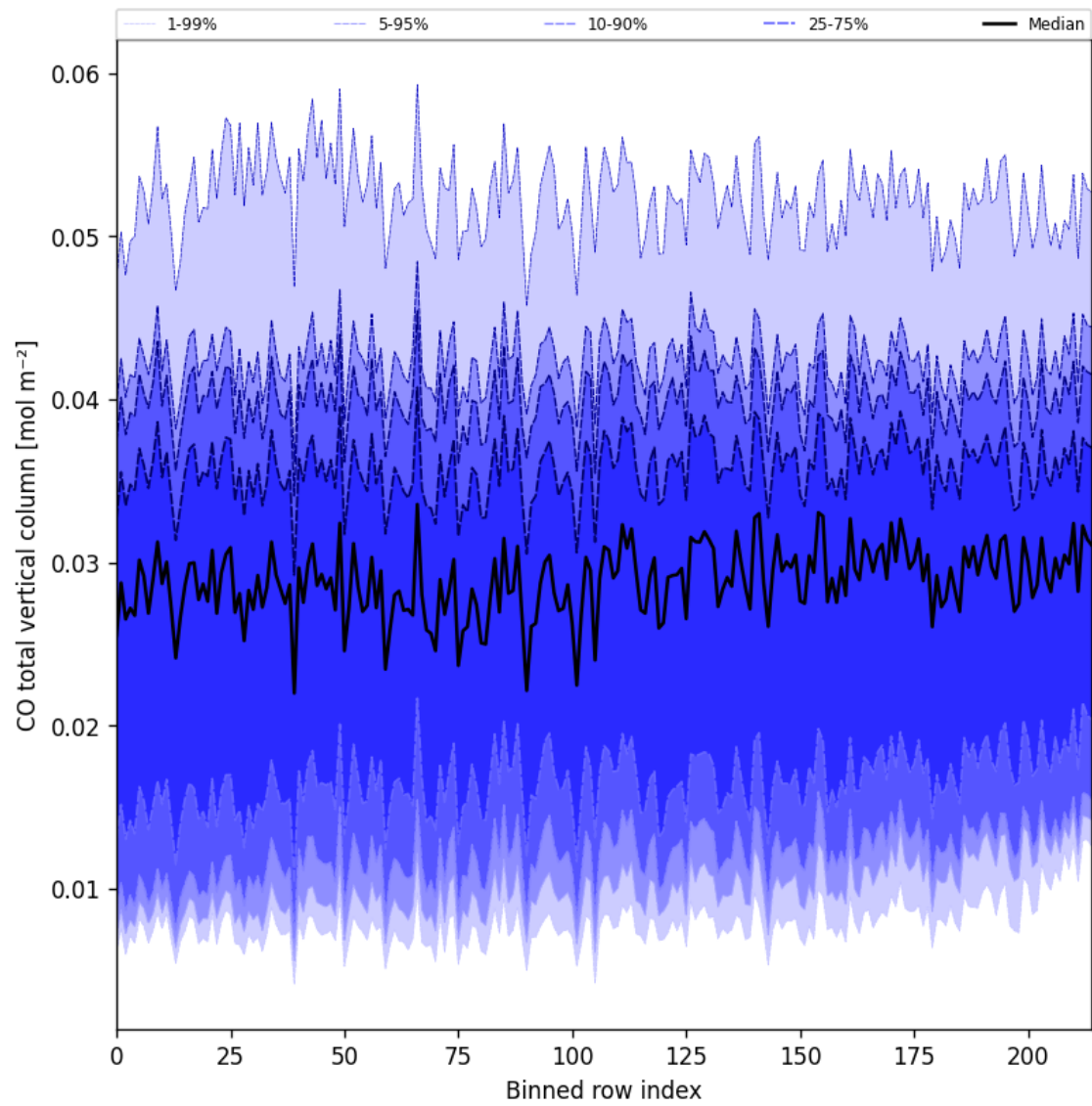
Figure 21: Along track statistics of "CO total vertical column" for 2025-03-10 to 2025-03-10
