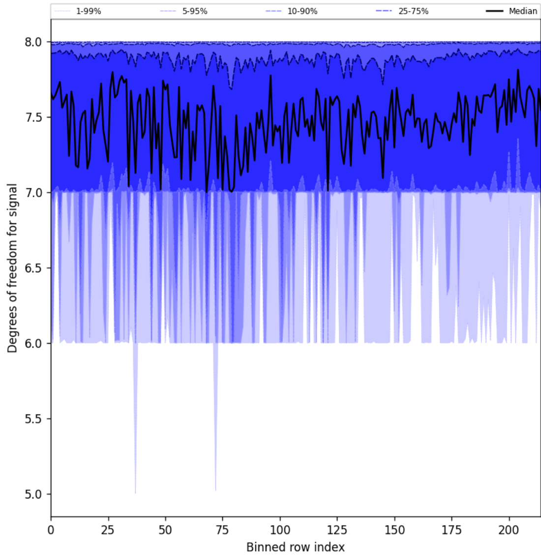
Figure 25: Along track statistics of “Degrees of freedom for signal” for 2025-03-10 to 2025-03-10
