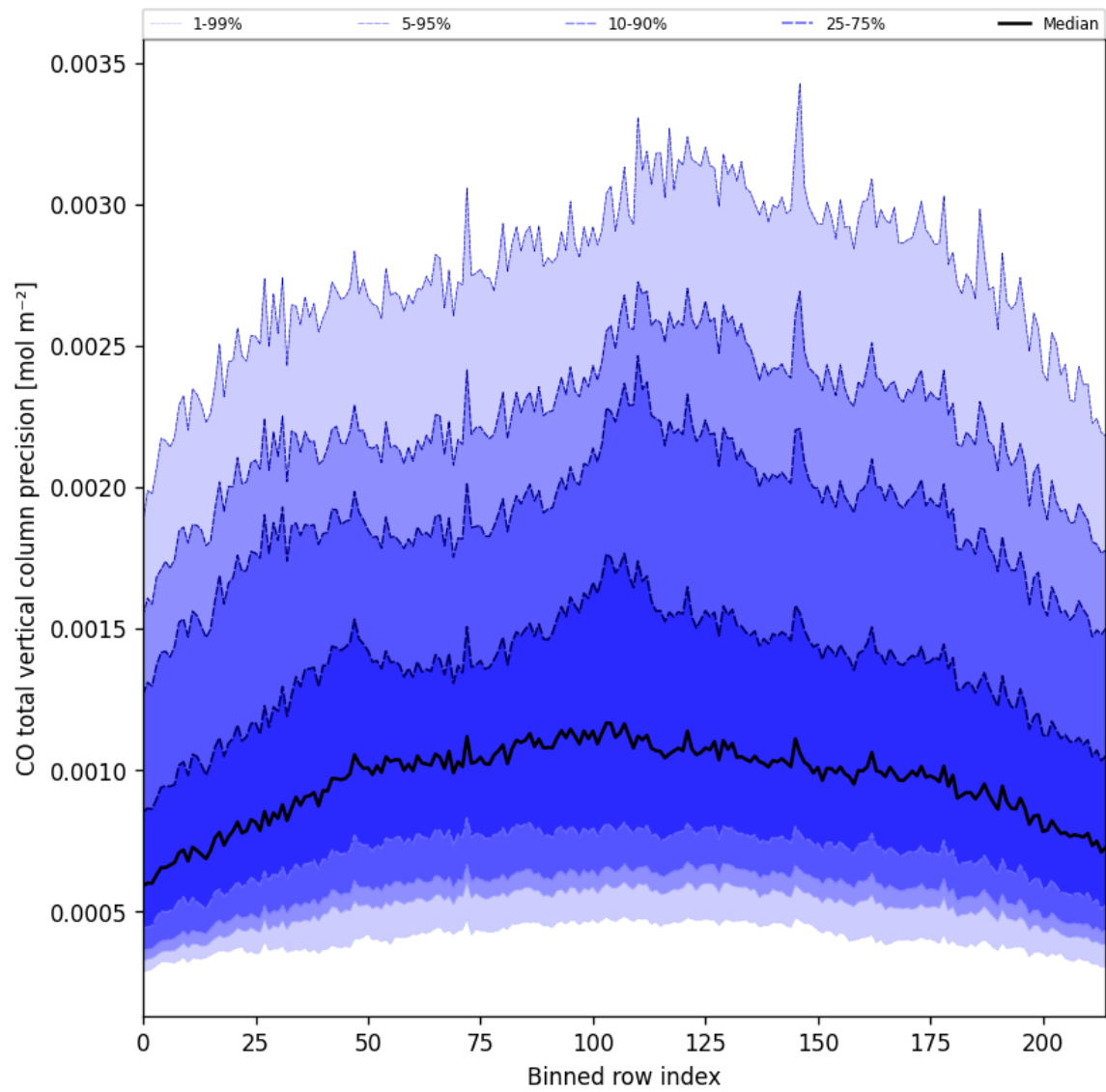
Figure 22: Along track statistics of “CO total vertical column precision” for 2025-03-11 to 2025-03-12
