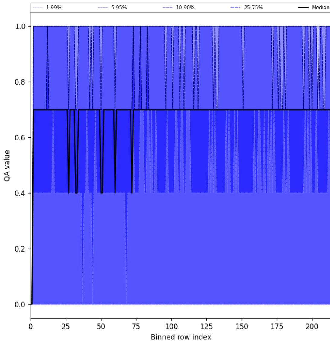
Figure 20: Along track statistics of “QA value” for 2025-03-11 to 2025-03-12
