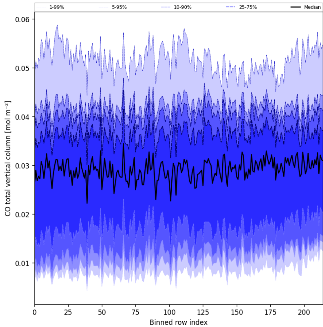
Figure 21: Along track statistics of “CO total vertical column” for 2025-03-11 to 2025-03-12
