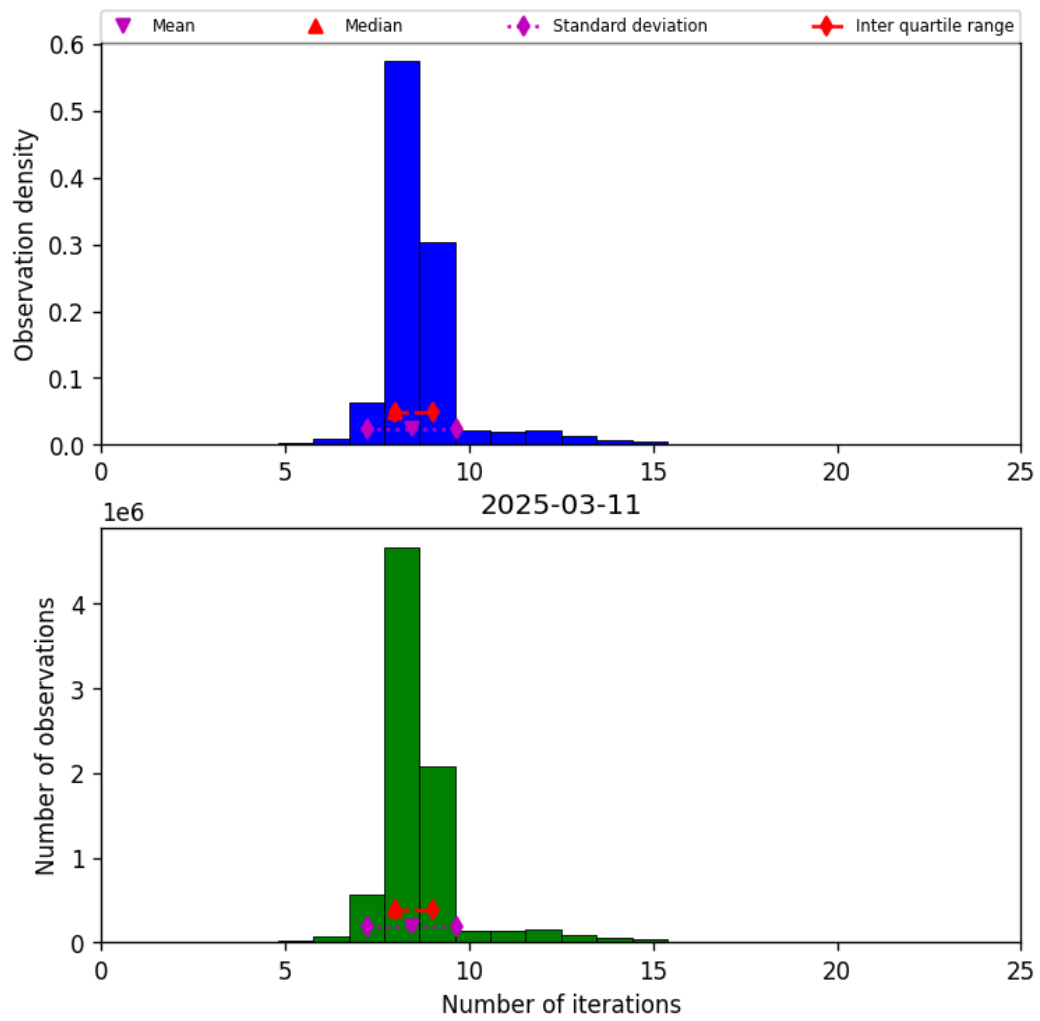
Figure 19: Histogram of “Number of iterations” for 2025-03-11 to 2025-03-12
