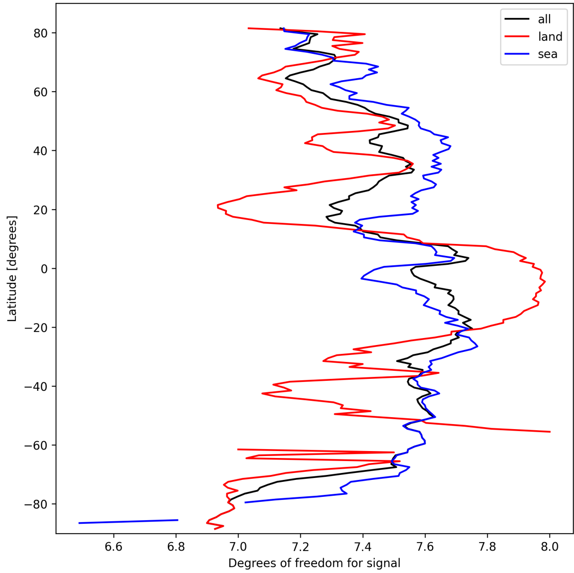
Figure 11: Zonal average of “Degrees of freedom for signal” for 2025-03-11 to 2025-03-12.
