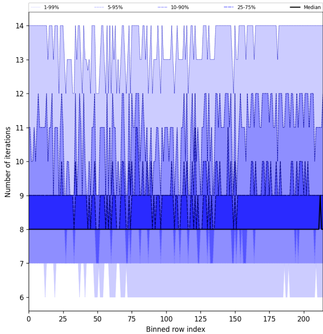
Figure 26: Along track statistics of “Number of iterations” for 2025-03-11 to 2025-03-12
