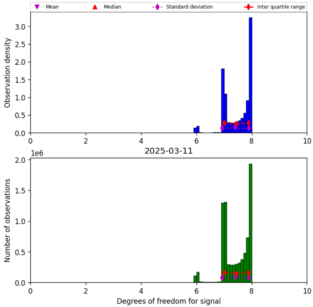
Figure 18: Histogram of “Degrees of freedom for signal” for 2025-03-11 to 2025-03-12
