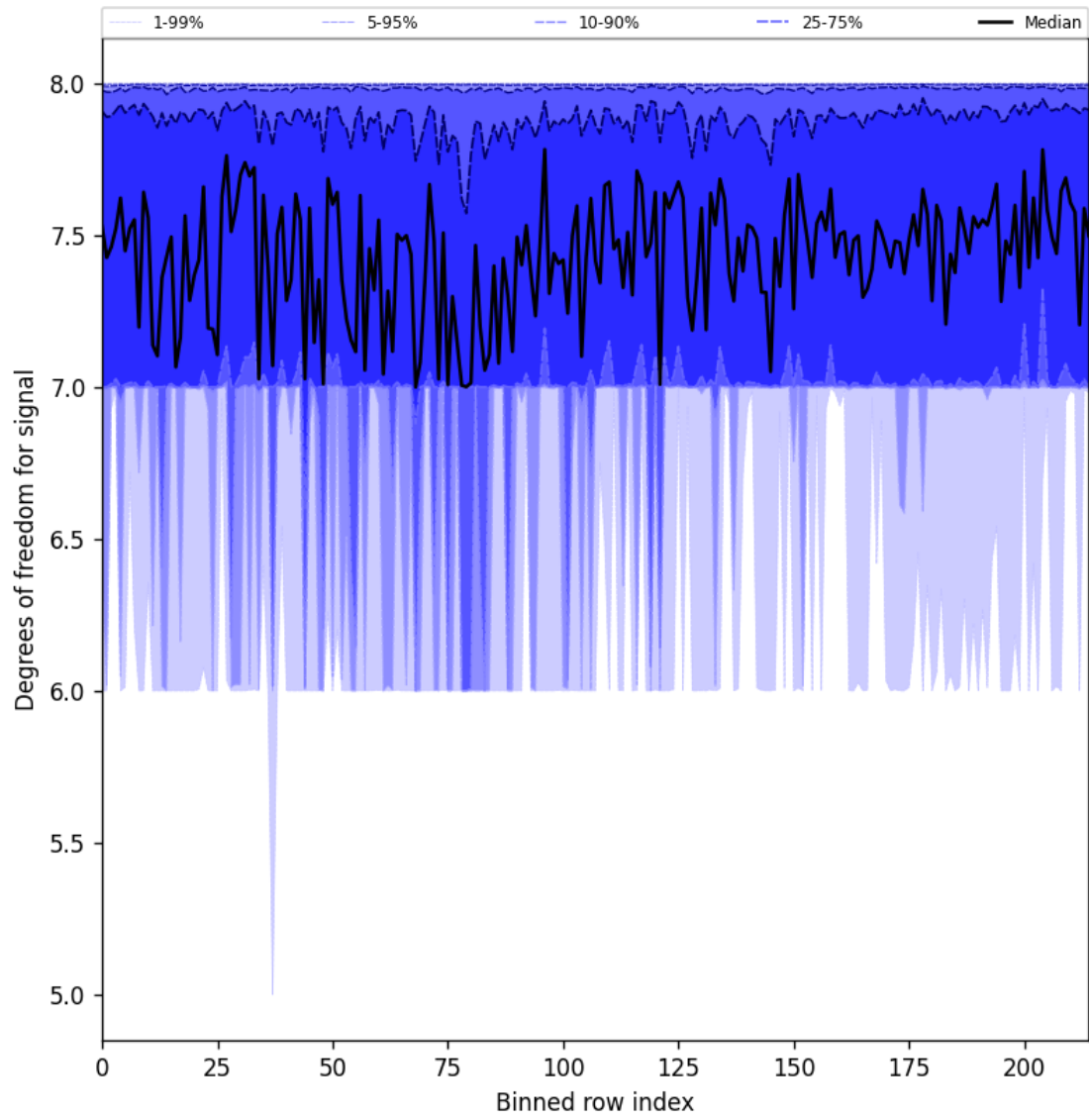
Figure 25: Along track statistics of “Degrees of freedom for signal” for 2025-03-11 to 2025-03-12
