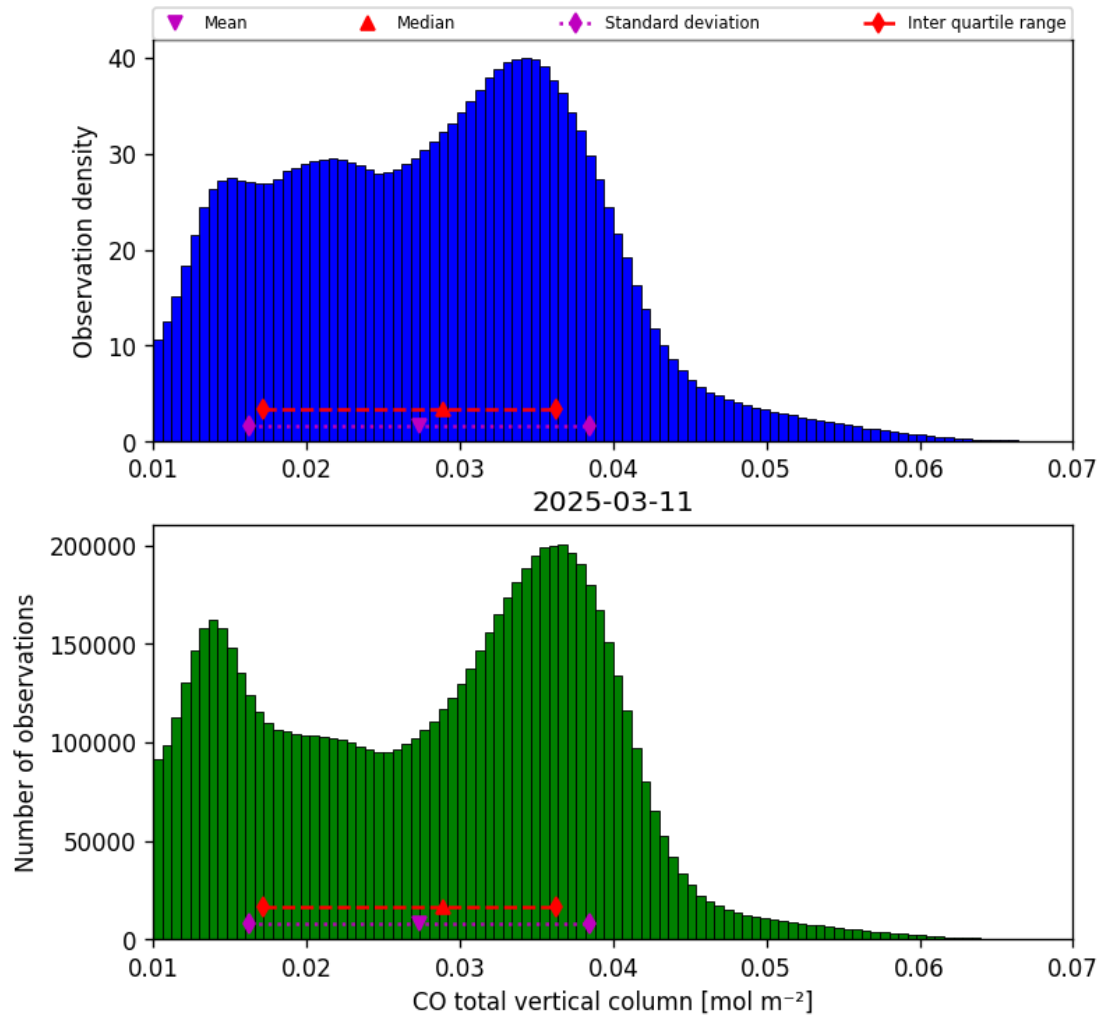
Figure 14: Histogram of “CO total vertical column” for 2025-03-11 to 2025-03-12
