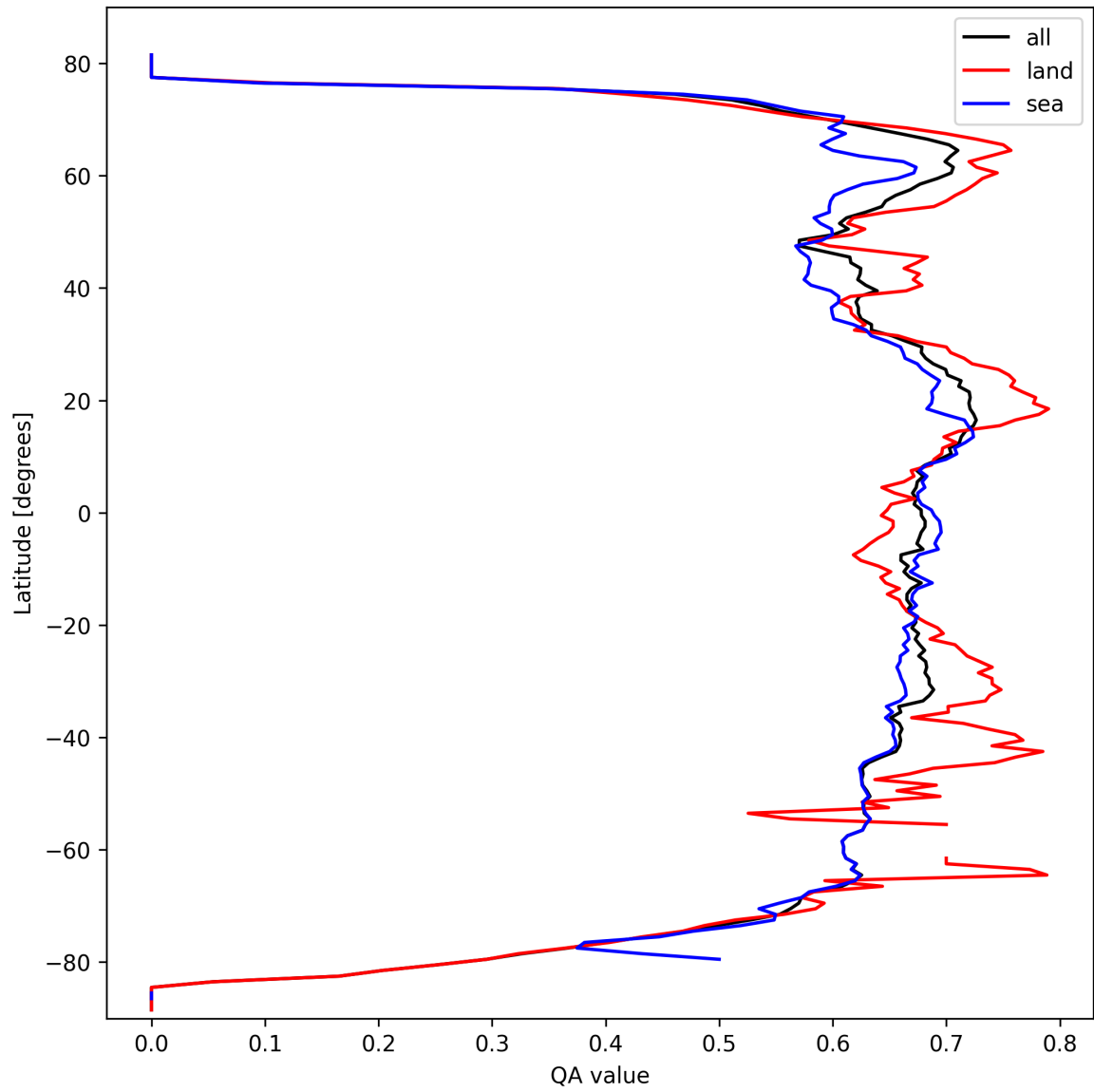
Figure 6: Zonal average of “QA value” for 2025-03-11 to 2025-03-12.
