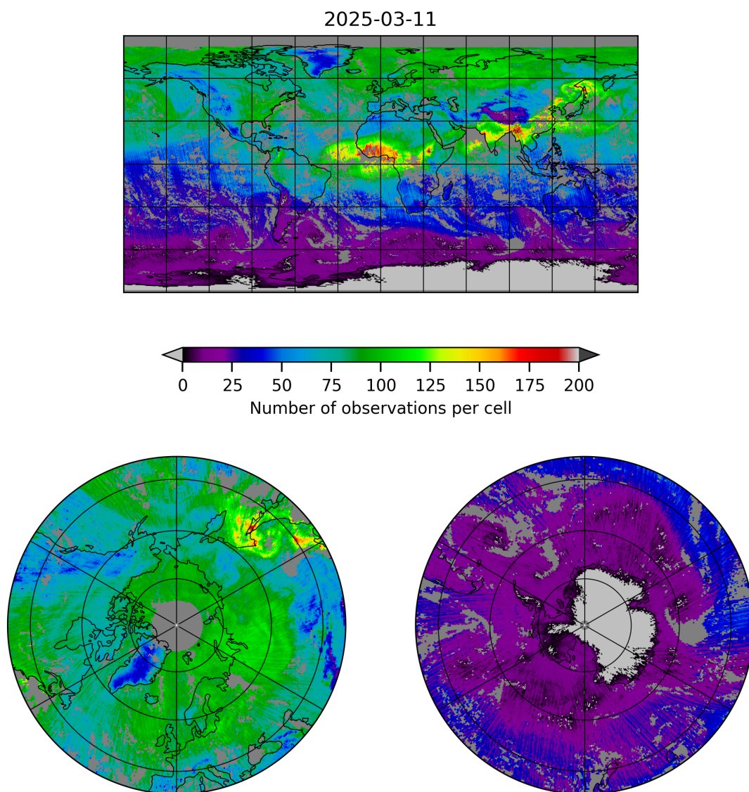
Figure 5: Map of the number of observations for 2025-03-11 to 2025-03-12
