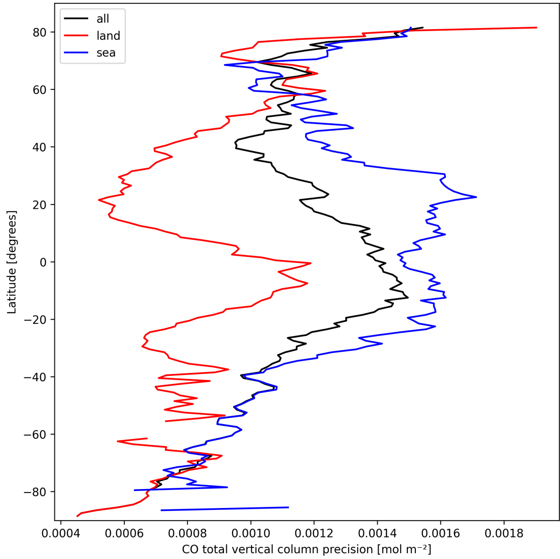
Figure 8: Zonal average of “CO total vertical column precision” for 2025-03-11 to 2025-03-12.
