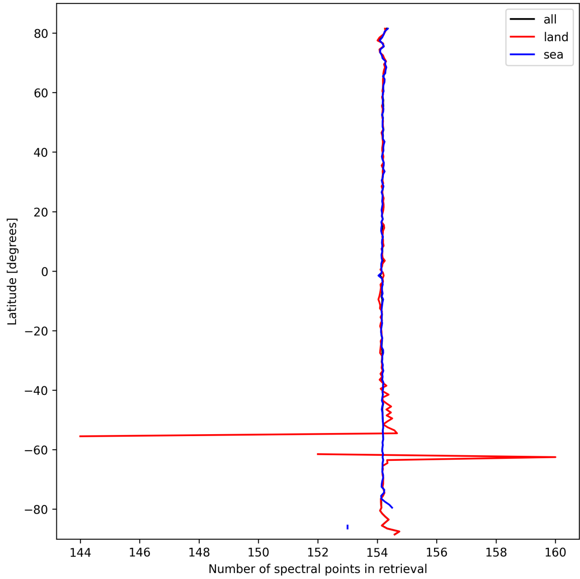
Figure 9: Zonal average of “Number of spectral points in retrieval” for 2025-03-11 to 2025-03-12.
