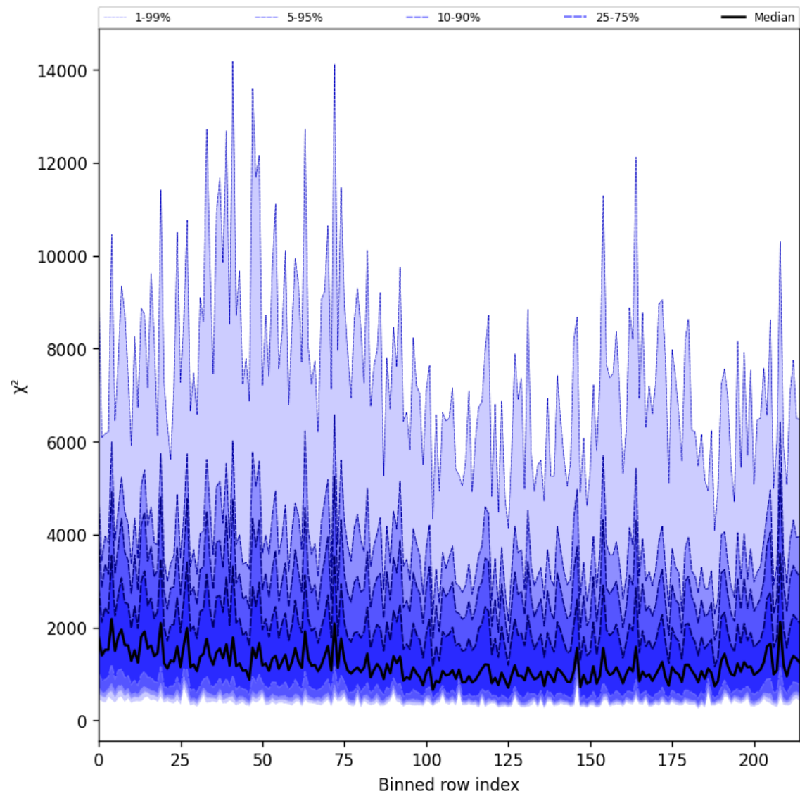
Figure 24: Along track statistics of “ \chi^2 ” for 2025-03-11 to 2025-03-12
