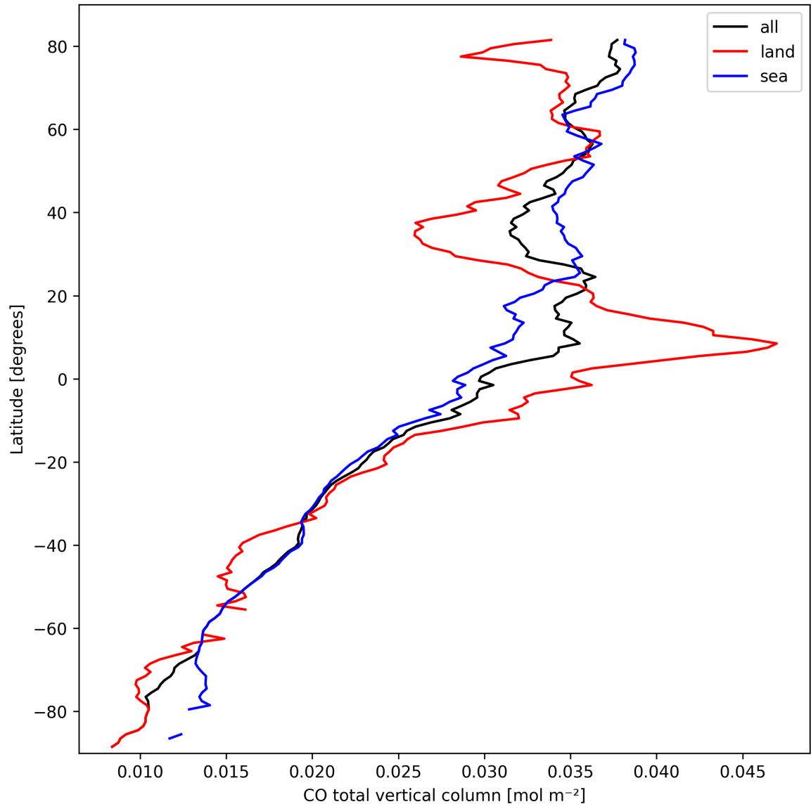
Figure 7: Zonal average of “CO total vertical column” for 2025-03-11 to 2025-03-12.
