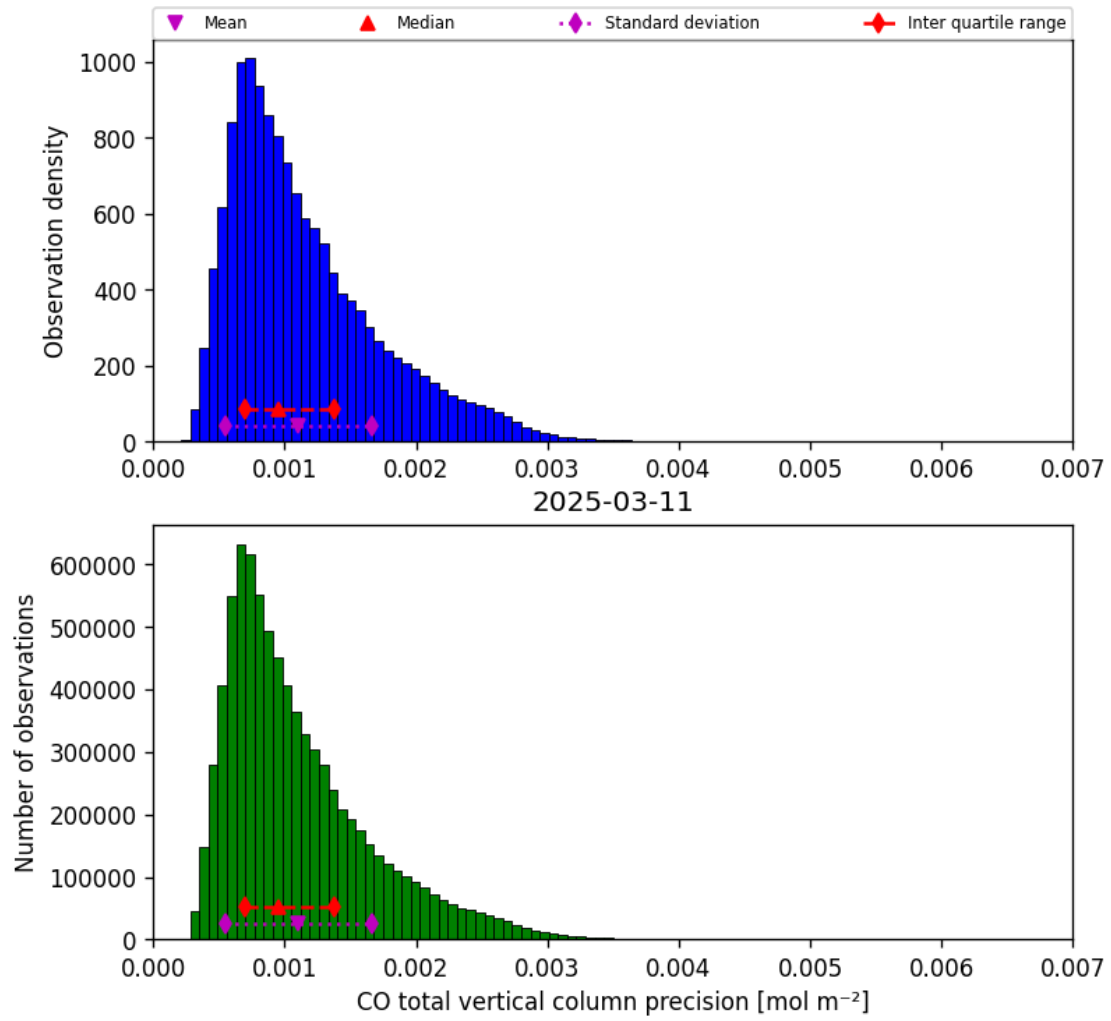
Figure 15: Histogram of “CO total vertical column precision” for 2025-03-11 to 2025-03-12
