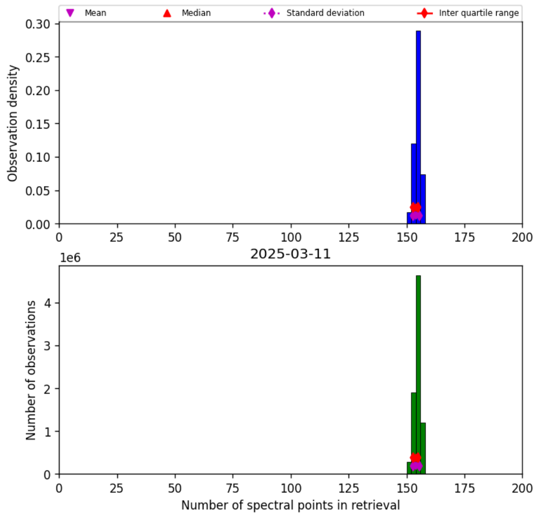
Figure 16: Histogram of “Number of spectral points in retrieval” for 2025-03-11 to 2025-03-12
