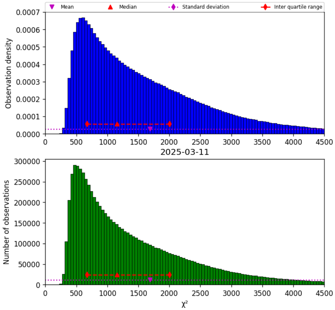
Figure 17: Histogram of “ \chi^2 ” for 2025-03-11 to 2025-03-12
