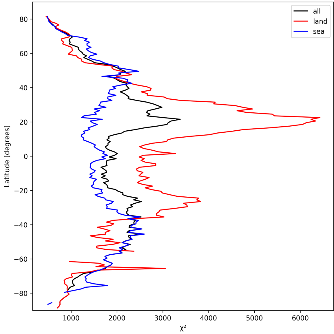
Figure 10: Zonal average of “ \chi^2 ” for 2025-03-11 to 2025-03-12.
