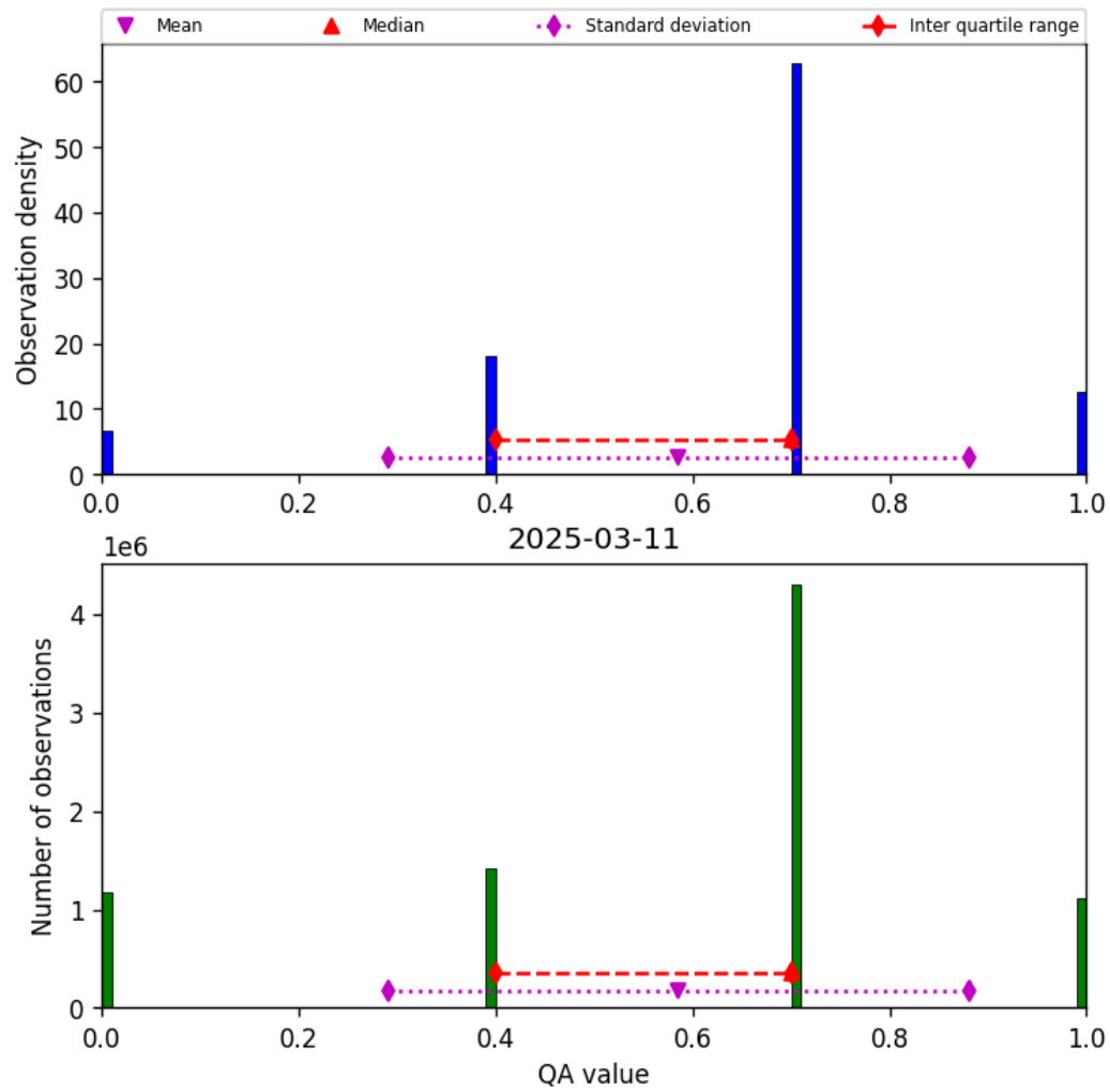
Figure 13: Histogram of “QA value” for 2025-03-11 to 2025-03-12
