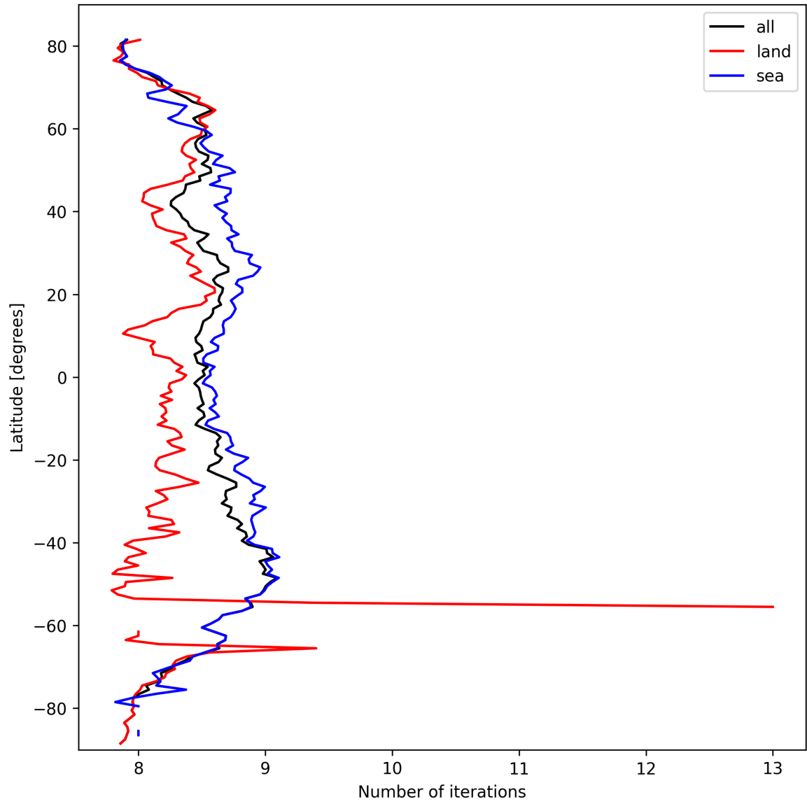
Figure 12: Zonal average of “Number of iterations” for 2025-03-11 to 2025-03-12.
