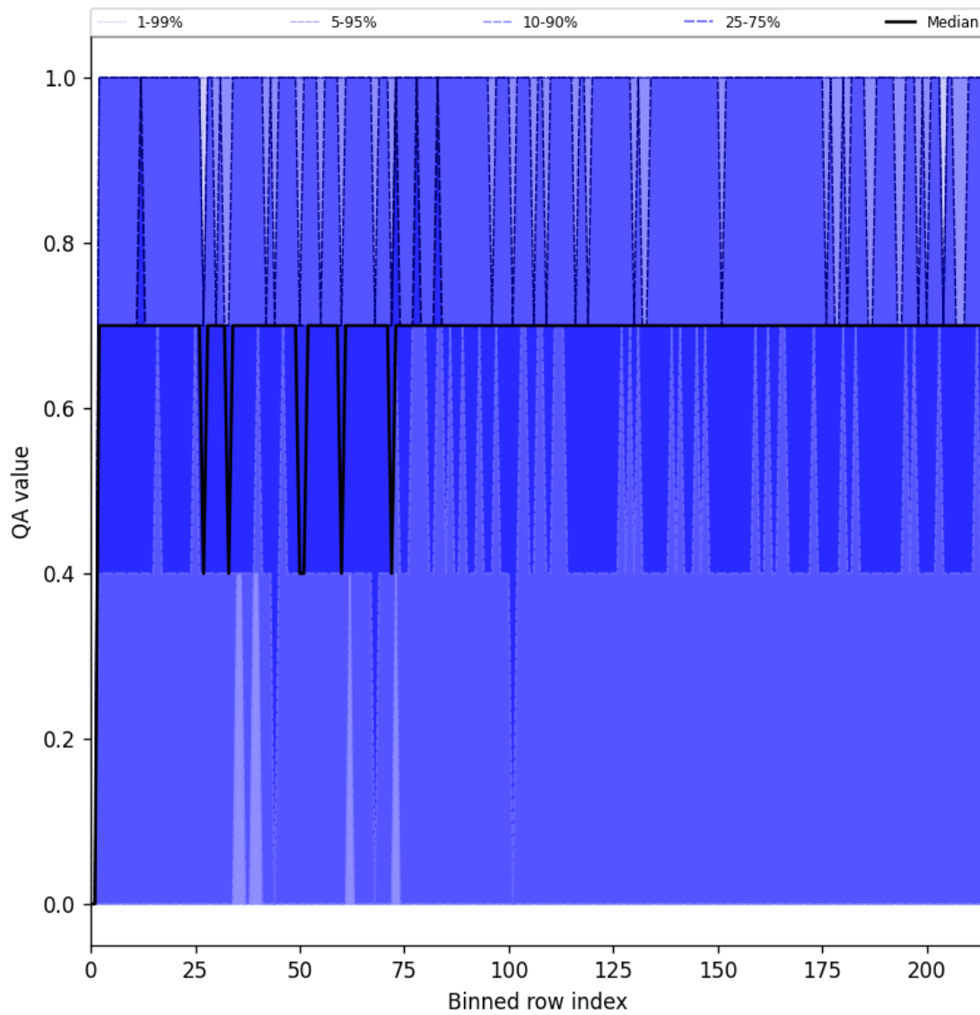
Figure 20: Along track statistics of “QA value” for 2025-03-12 to 2025-03-13
