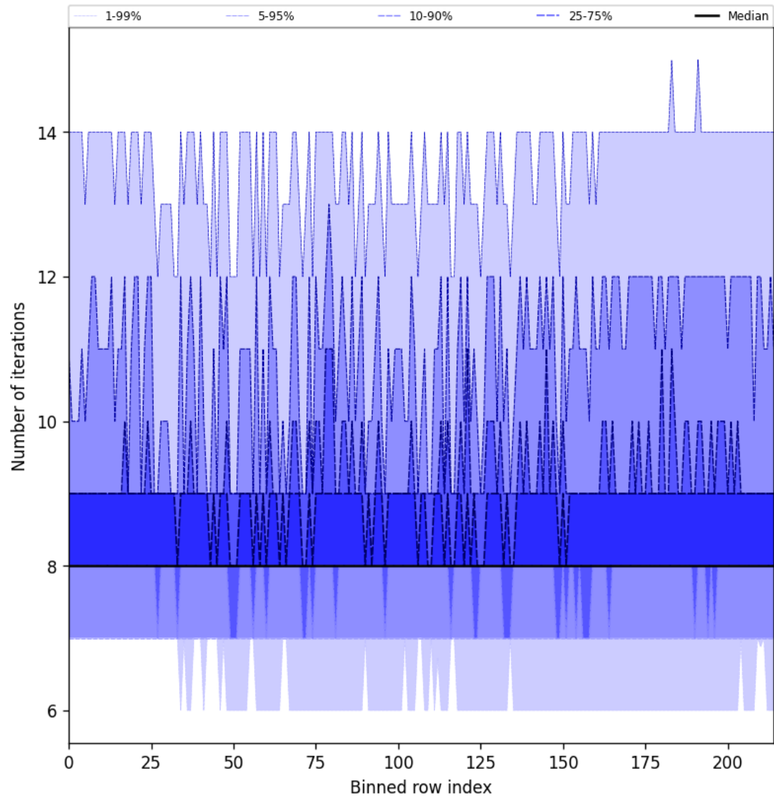
Figure 26: Along track statistics of “Number of iterations” for 2025-03-12 to 2025-03-13
