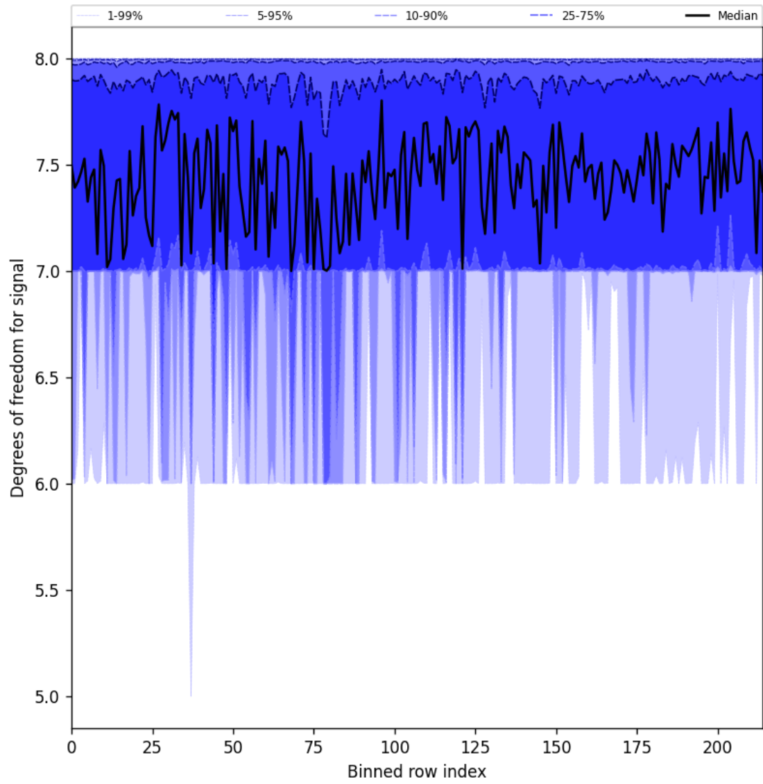
Figure 25: Along track statistics of “Degrees of freedom for signal” for 2025-03-12 to 2025-03-13
