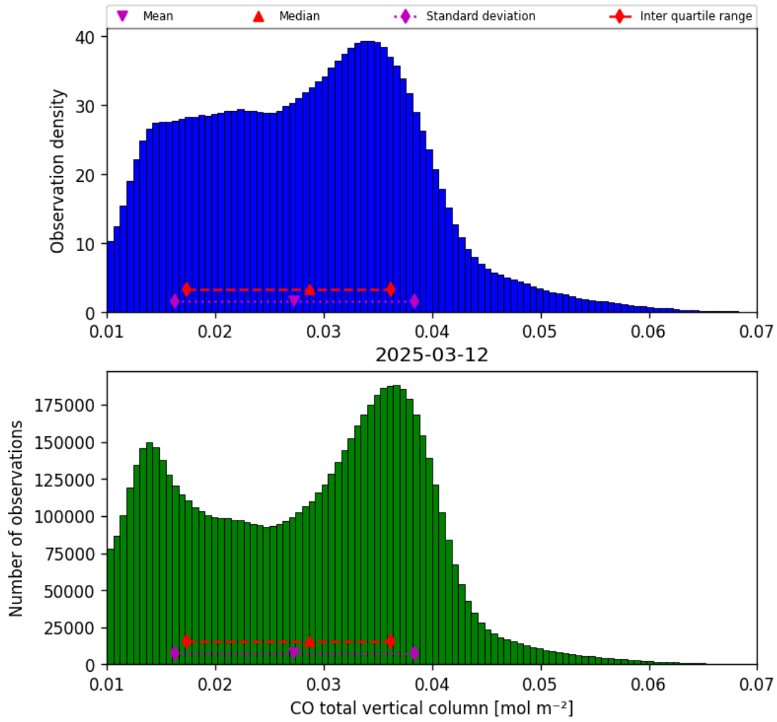
Figure 14: Histogram of “CO total vertical column” for 2025-03-12 to 2025-03-13
