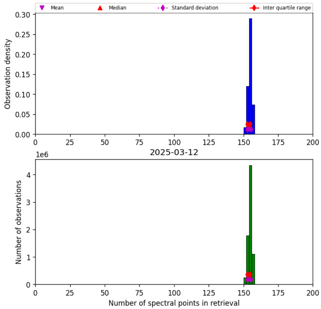
Figure 16: Histogram of “Number of spectral points in retrieval” for 2025-03-12 to 2025-03-13
