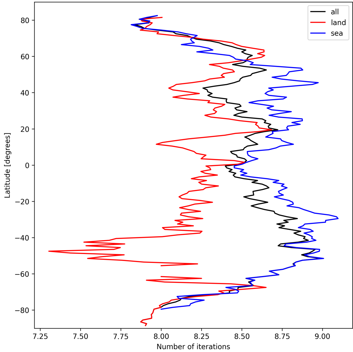
Figure 12: Zonal average of “Number of iterations” for 2025-03-12 to 2025-03-13.
