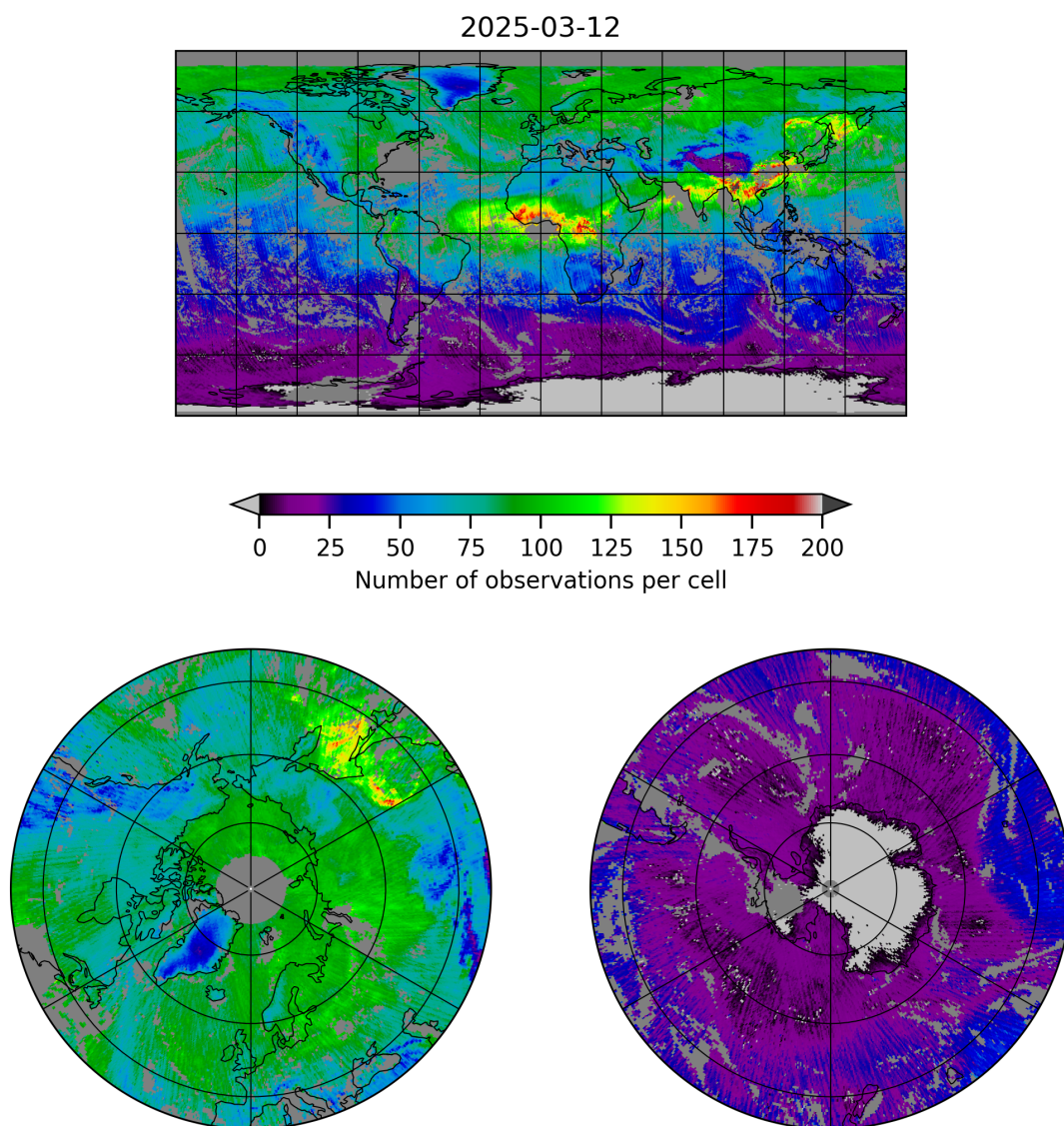
Figure 5: Map of the number of observations for 2025-03-12 to 2025-03-13
