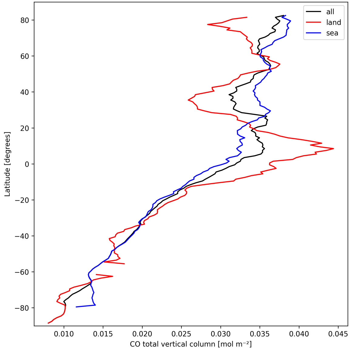
Figure 7: Zonal average of “CO total vertical column” for 2025-03-12 to 2025-03-13.
