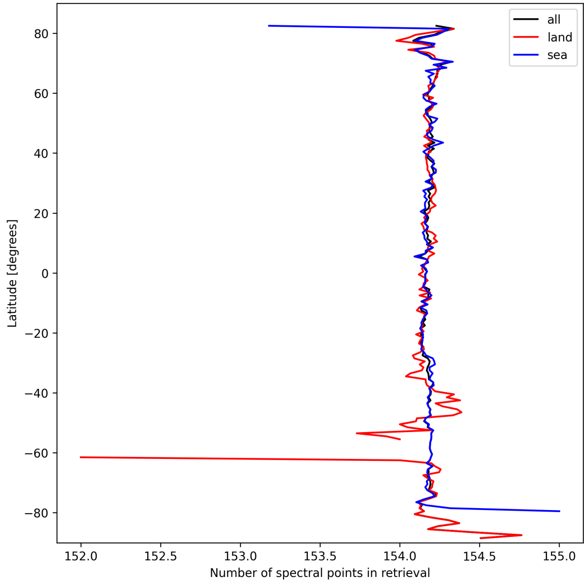
Figure 9: Zonal average of “Number of spectral points in retrieval” for 2025-03-12 to 2025-03-13.
