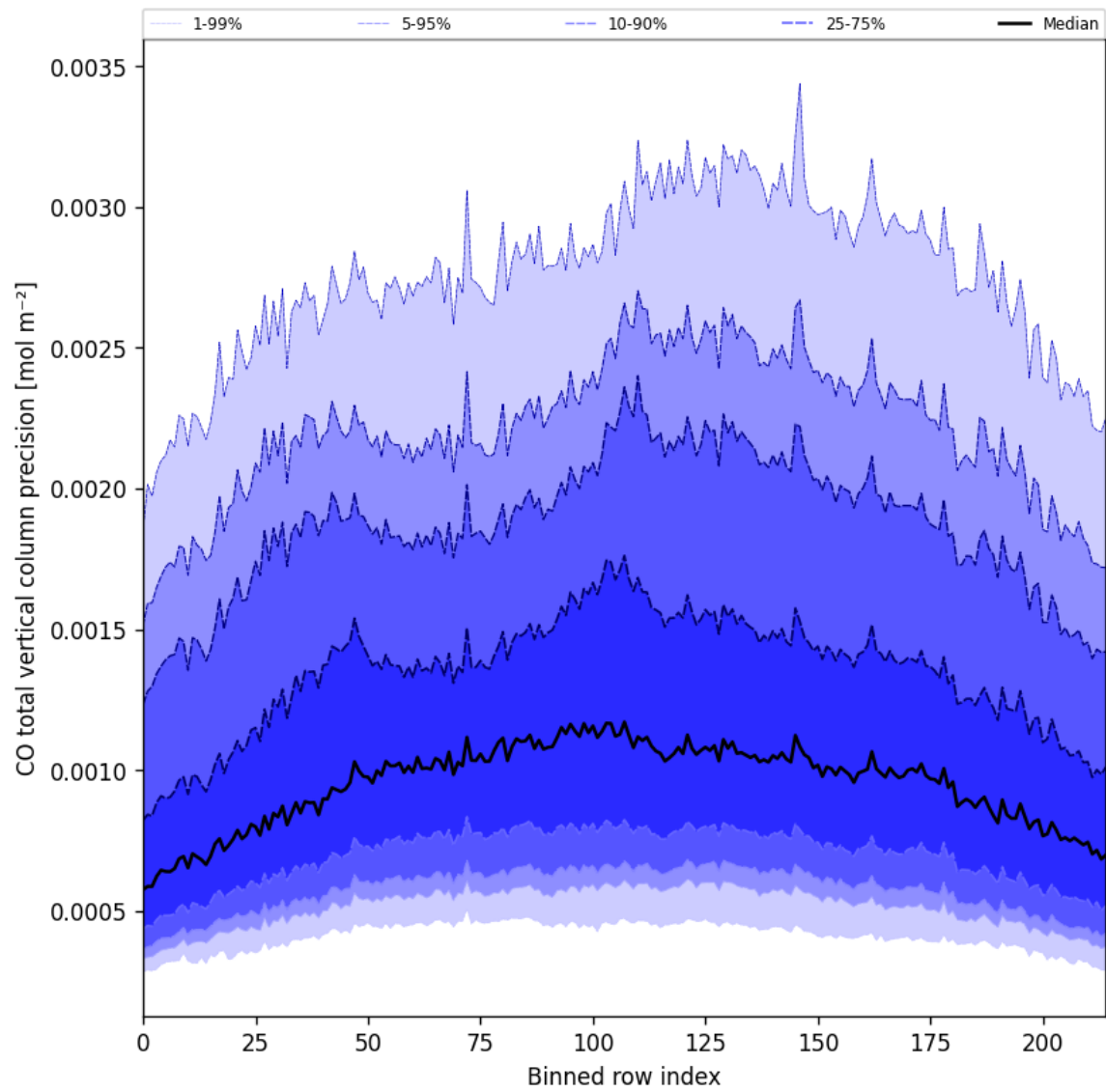
Figure 22: Along track statistics of “CO total vertical column precision” for 2025-03-12 to 2025-03-13
