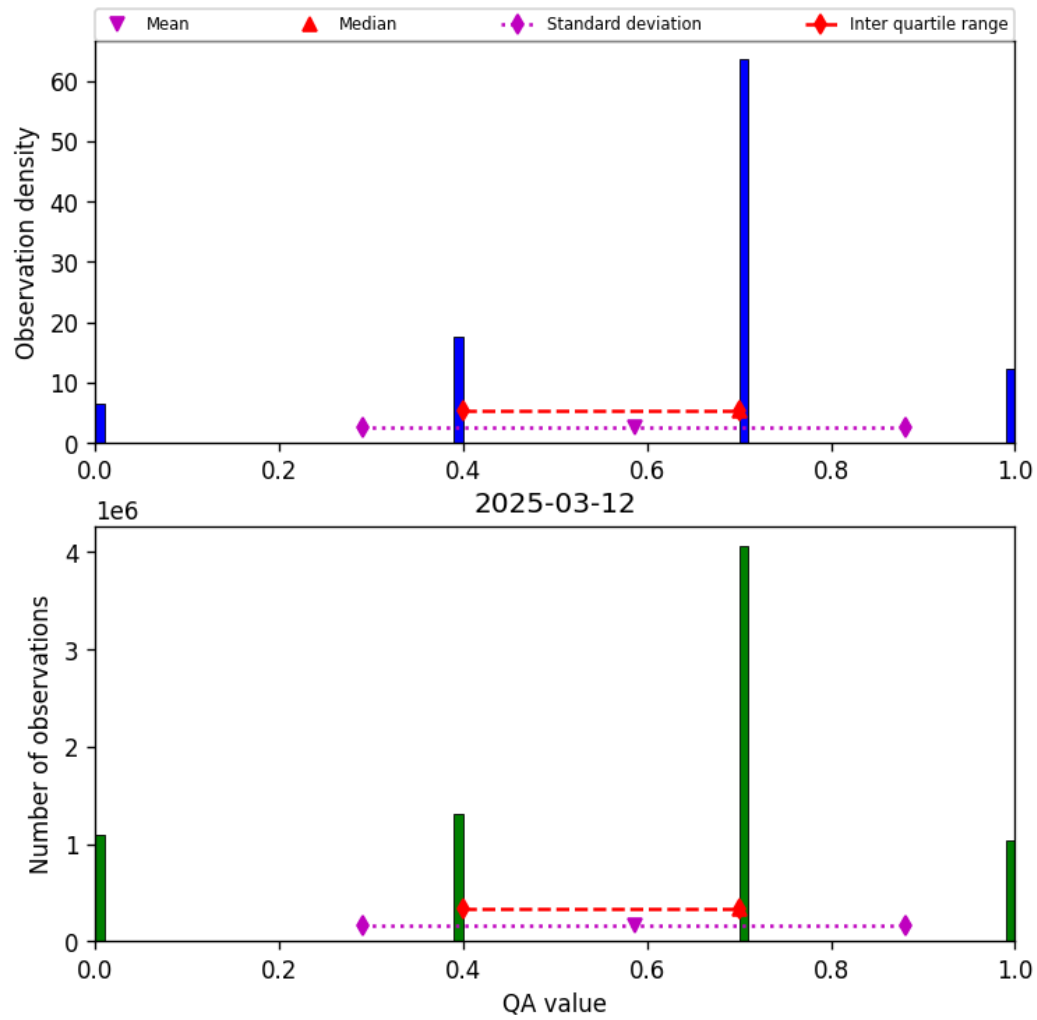
Figure 13: Histogram of “QA value” for 2025-03-12 to 2025-03-13
