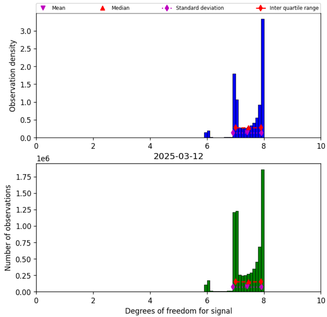
Figure 18: Histogram of “Degrees of freedom for signal” for 2025-03-12 to 2025-03-13
