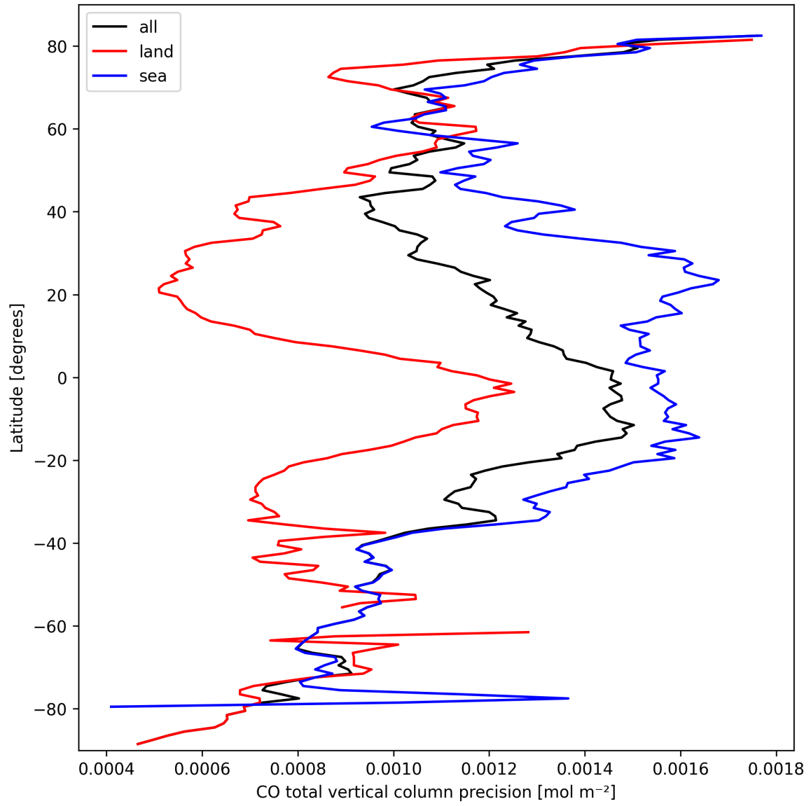
Figure 8: Zonal average of “CO total vertical column precision” for 2025-03-12 to 2025-03-13.
