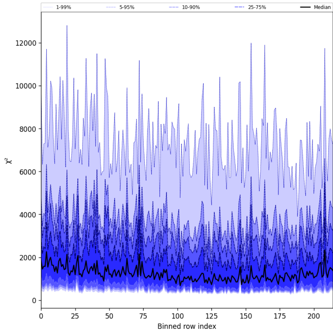
Figure 24: Along track statistics of “ \chi^2 ” for 2025-03-12 to 2025-03-13
