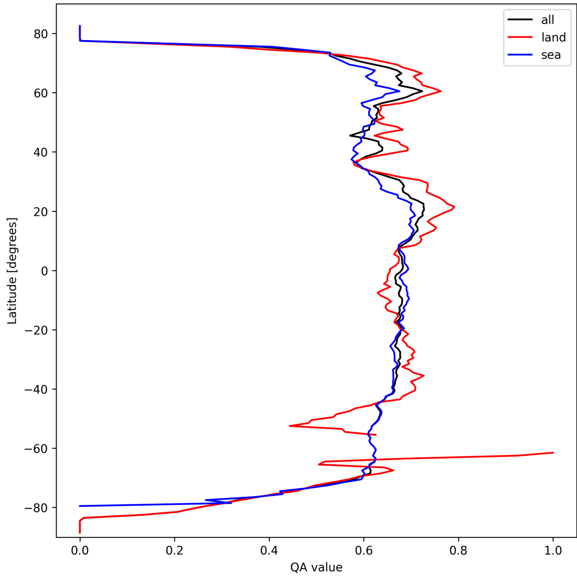
Figure 6: Zonal average of “QA value” for 2025-03-12 to 2025-03-13.
