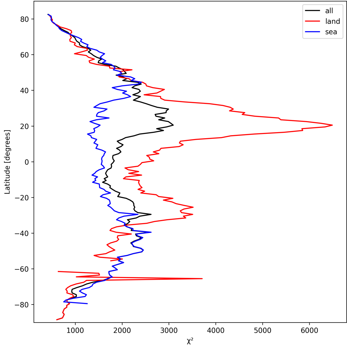
Figure 10: Zonal average of “ \chi^2 ” for 2025-03-12 to 2025-03-13.
