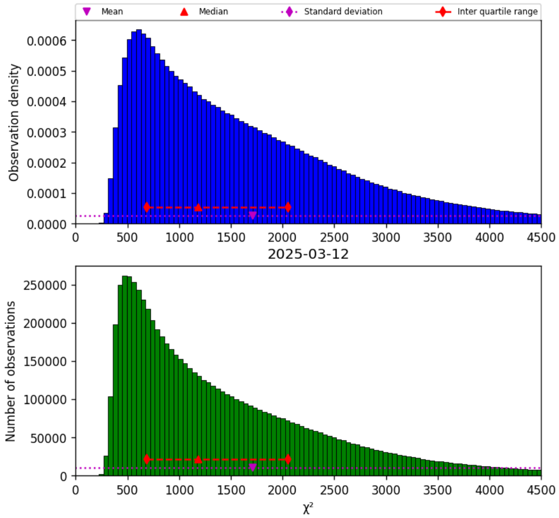
Figure 17: Histogram of “ \chi^2 ” for 2025-03-12 to 2025-03-13
