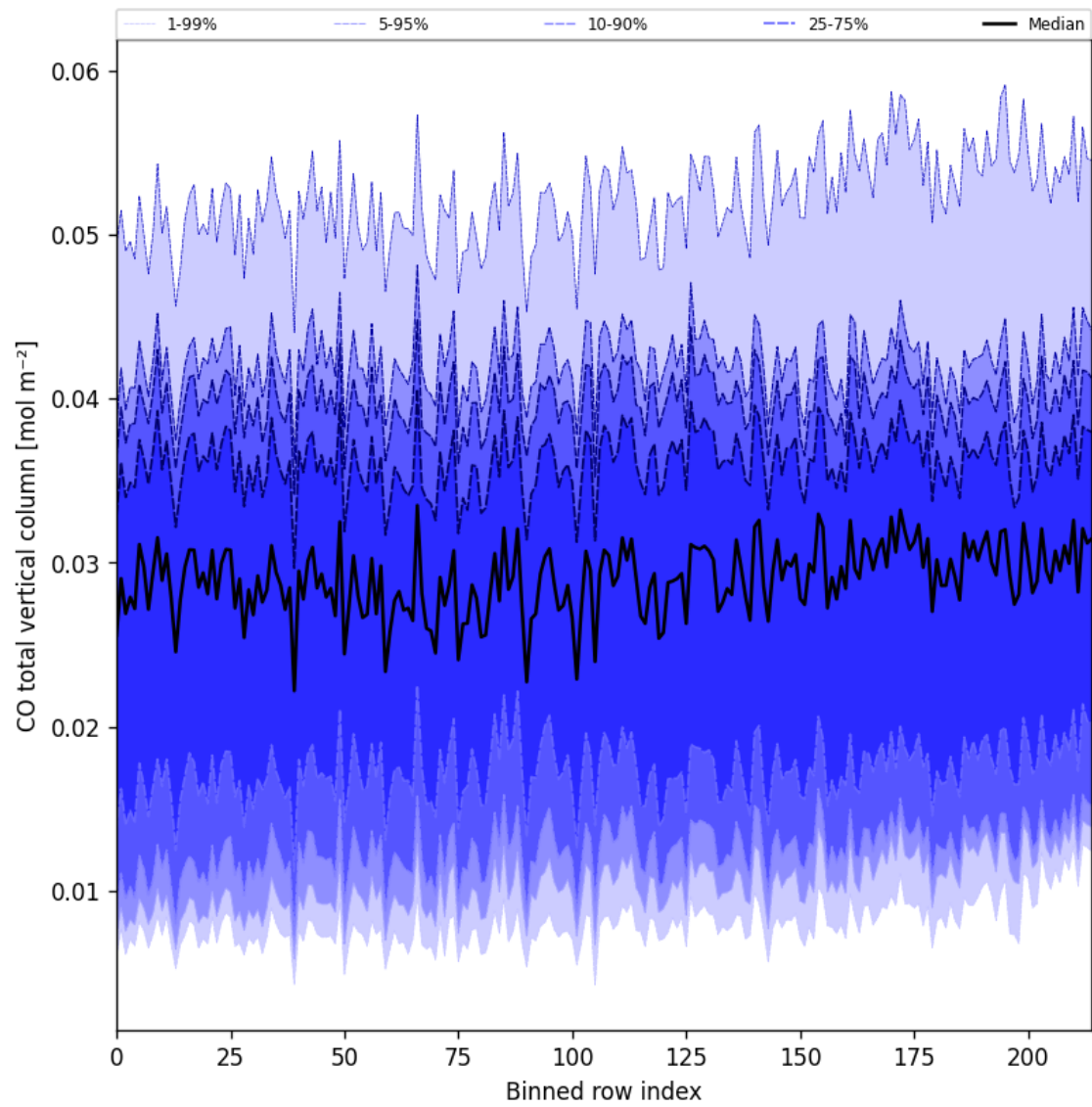
Figure 21: Along track statistics of “CO total vertical column” for 2025-03-12 to 2025-03-13
