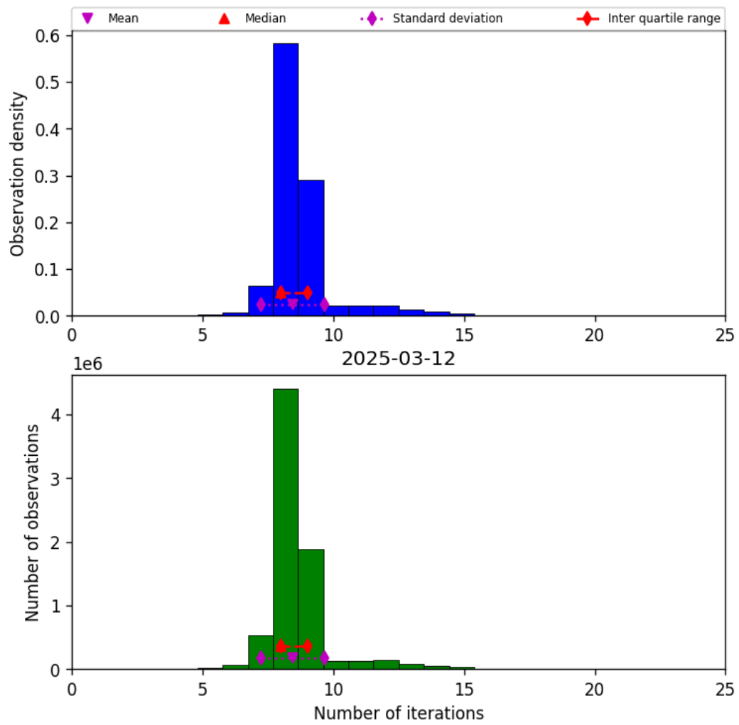
Figure 19: Histogram of “Number of iterations” for 2025-03-12 to 2025-03-13
