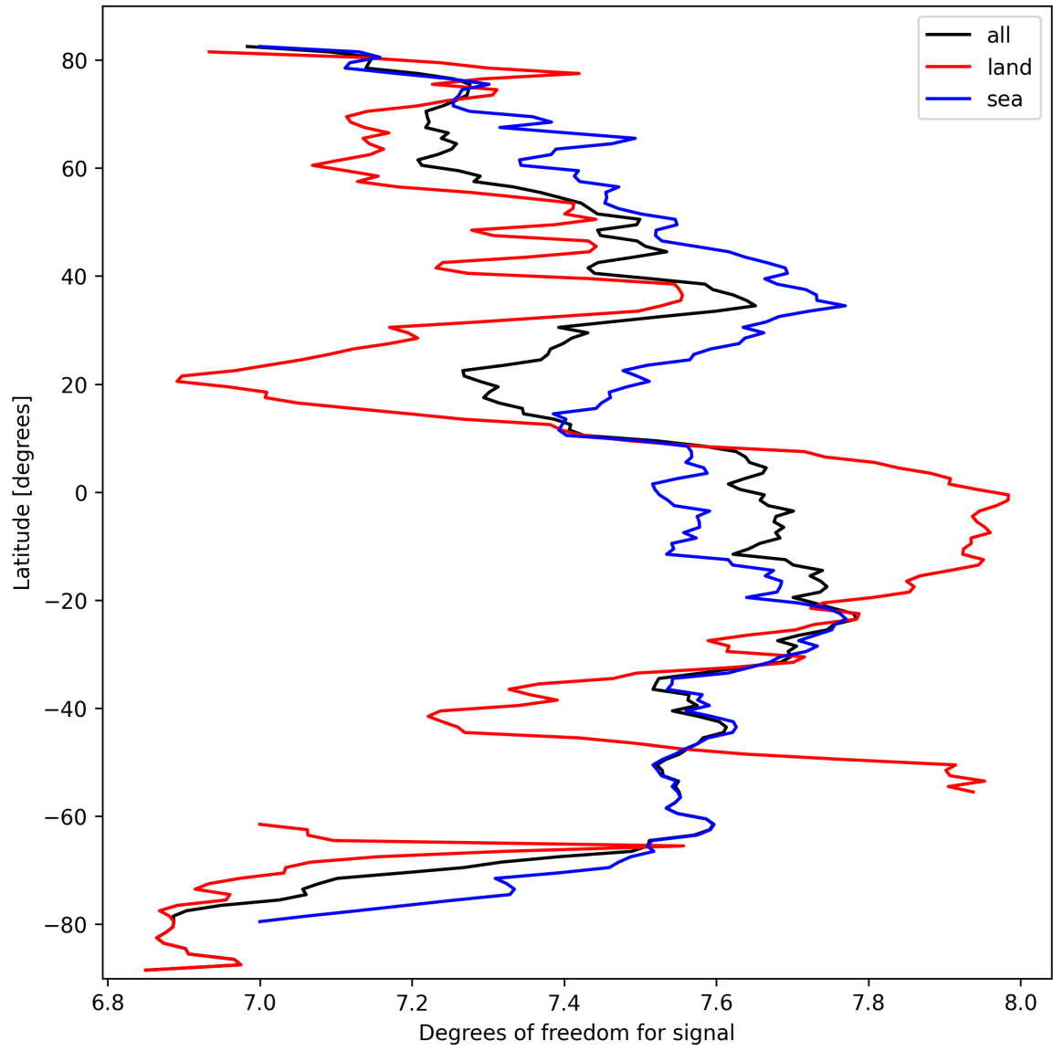
Figure 11: Zonal average of “Degrees of freedom for signal” for 2025-03-12 to 2025-03-13.
