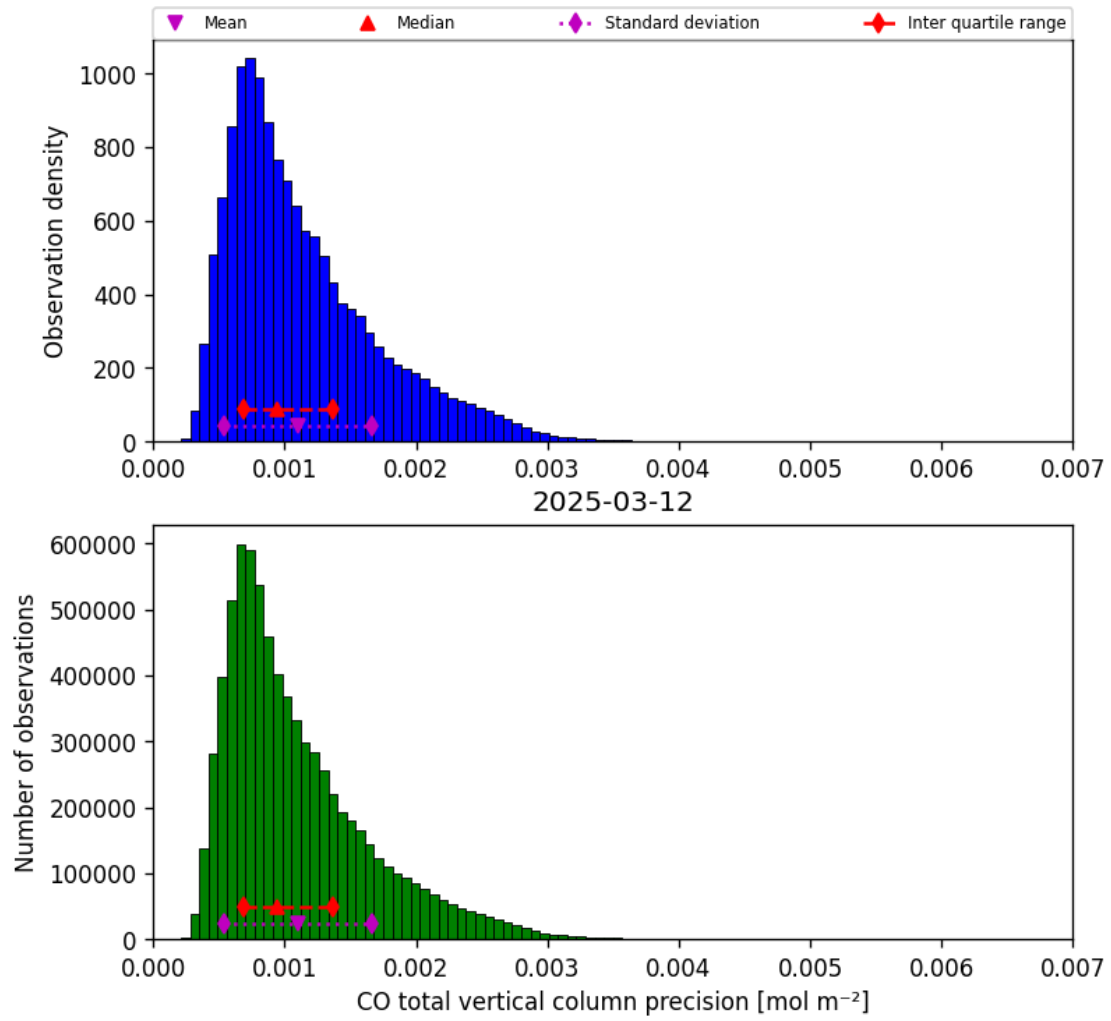
Figure 15: Histogram of “CO total vertical column precision” for 2025-03-12 to 2025-03-13
