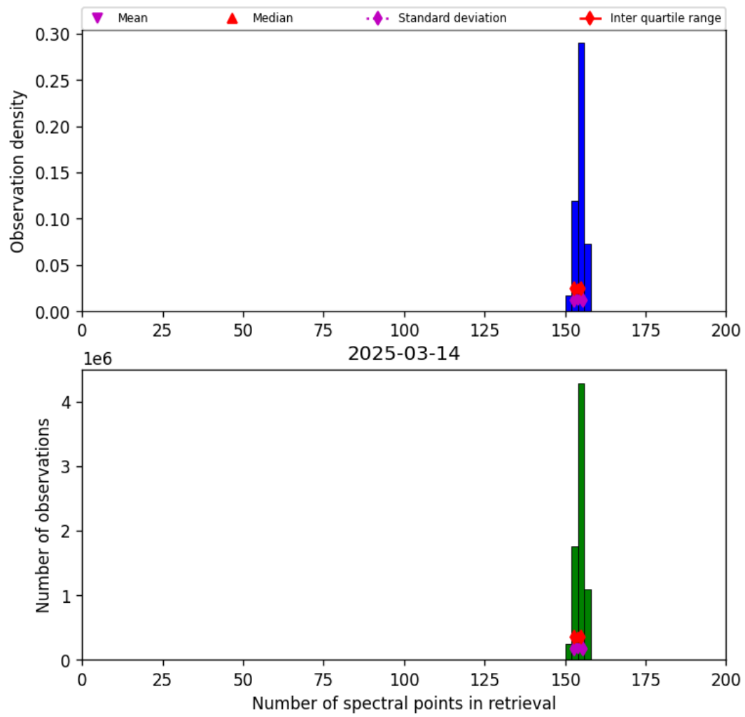
Figure 16: Histogram of “Number of spectral points in retrieval” for 2025-03-14 to 2025-03-15
