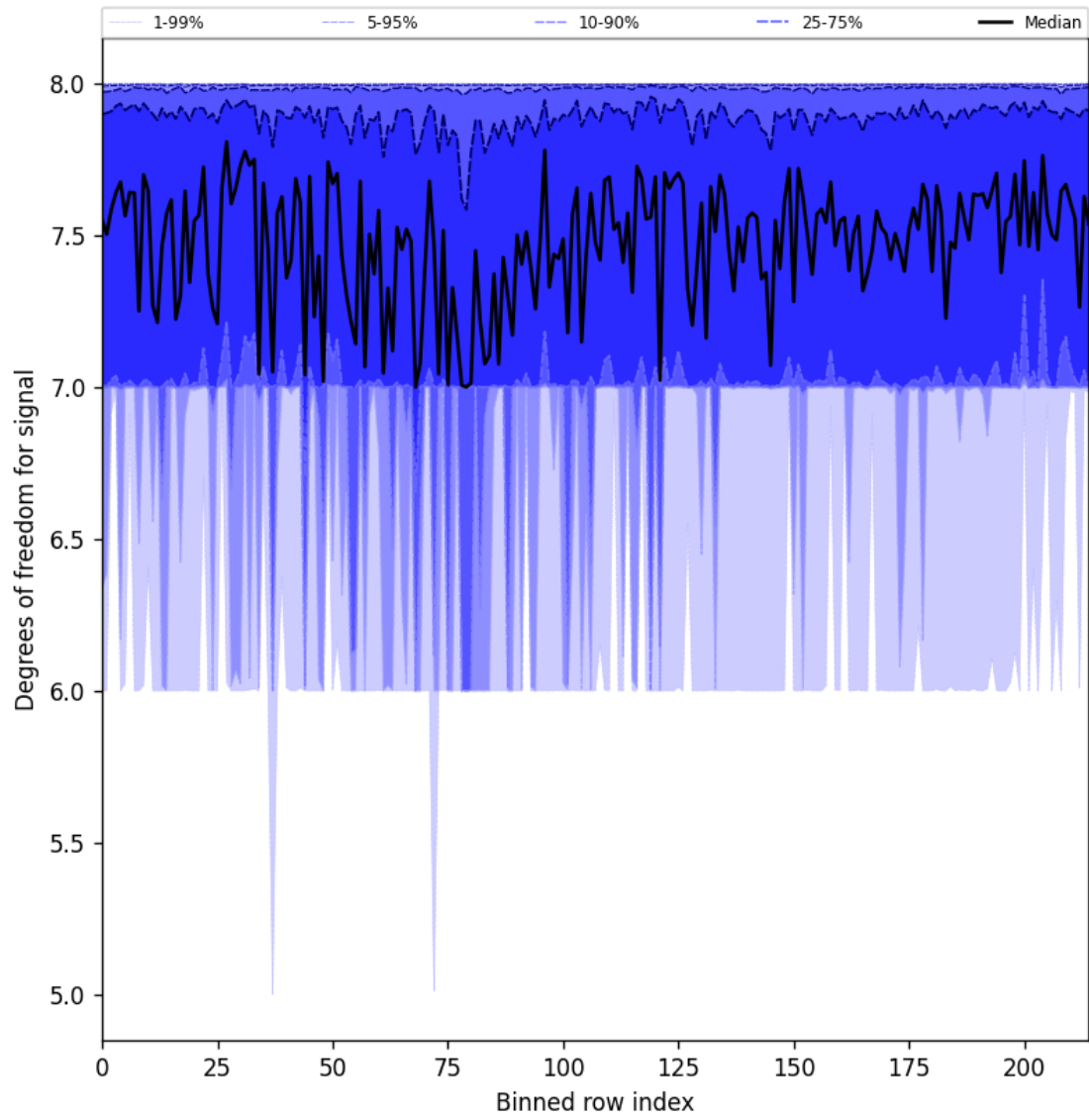
Figure 25: Along track statistics of “Degrees of freedom for signal” for 2025-03-14 to 2025-03-15
