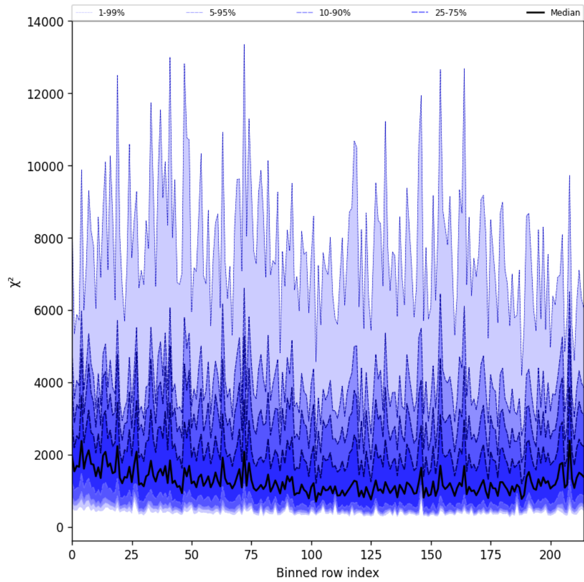
Figure 24: Along track statistics of “ \chi^2 ” for 2025-03-14 to 2025-03-15
