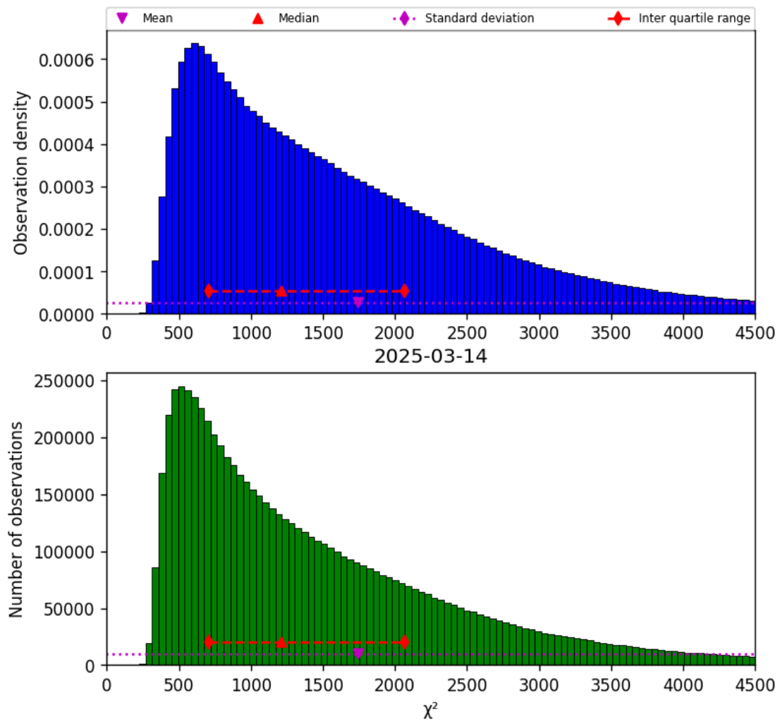
Figure 17: Histogram of " \chi^2 " for 2025-03-14 to 2025-03-15
