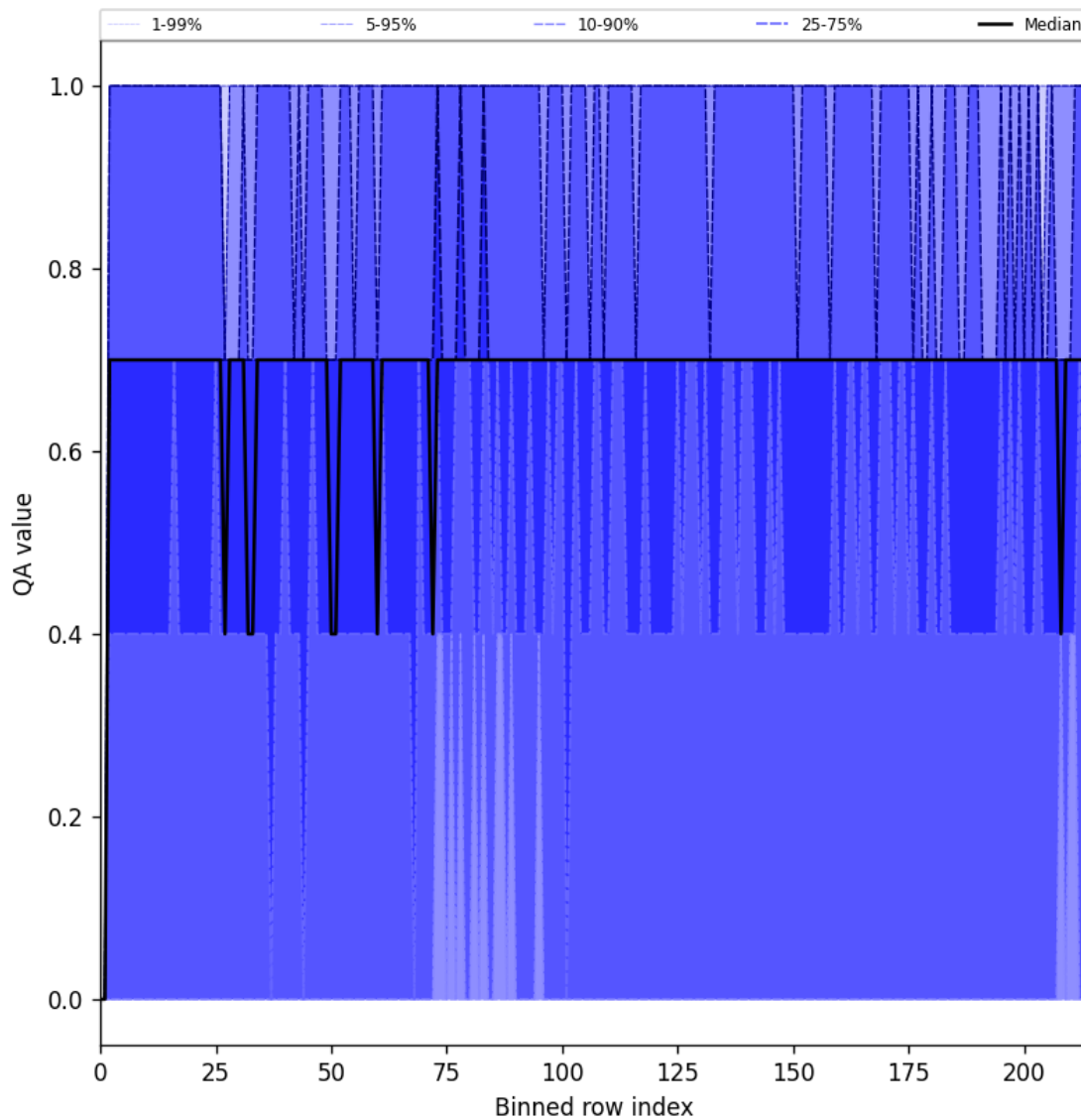
Figure 20: Along track statistics of “QA value” for 2025-03-14 to 2025-03-15
