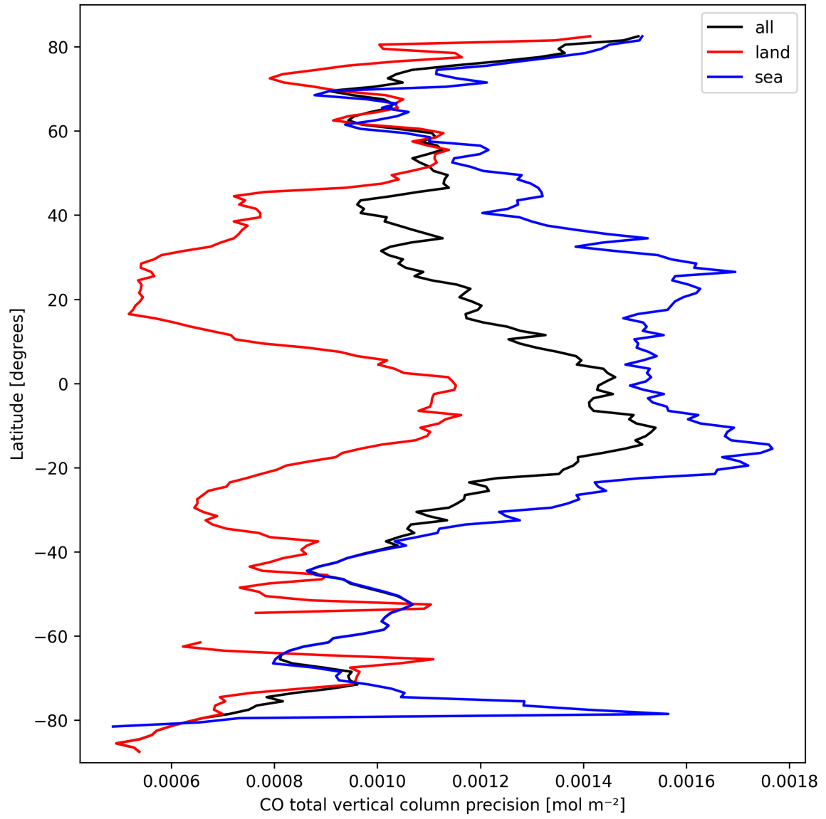
Figure 8: Zonal average of “CO total vertical column precision” for 2025-03-14 to 2025-03-15.
