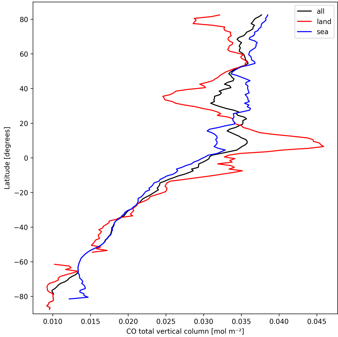
Figure 7: Zonal average of “CO total vertical column” for 2025-03-14 to 2025-03-15.
