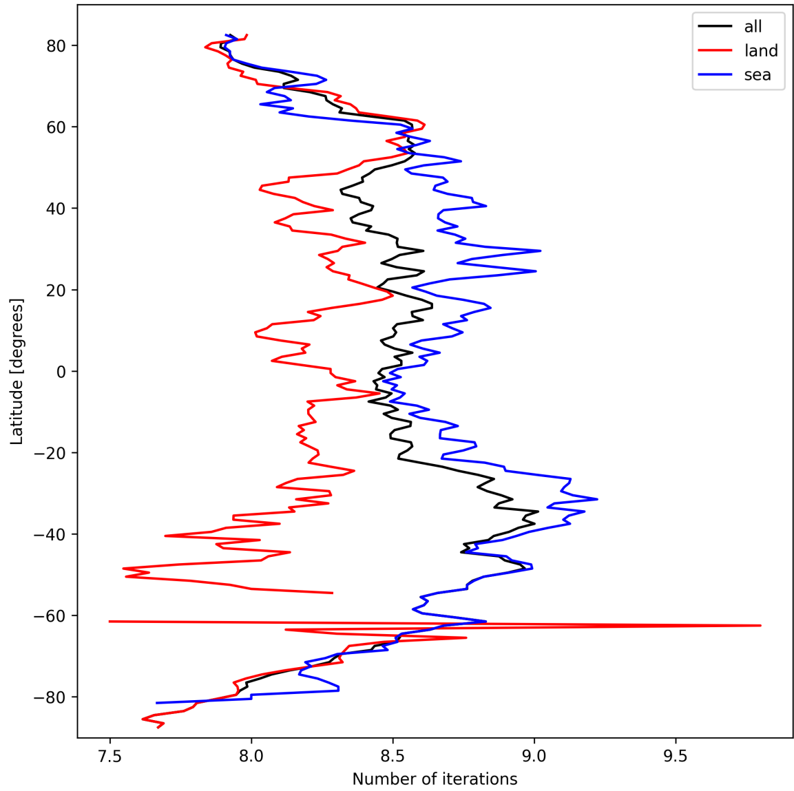
Figure 12: Zonal average of “Number of iterations” for 2025-03-14 to 2025-03-15.
