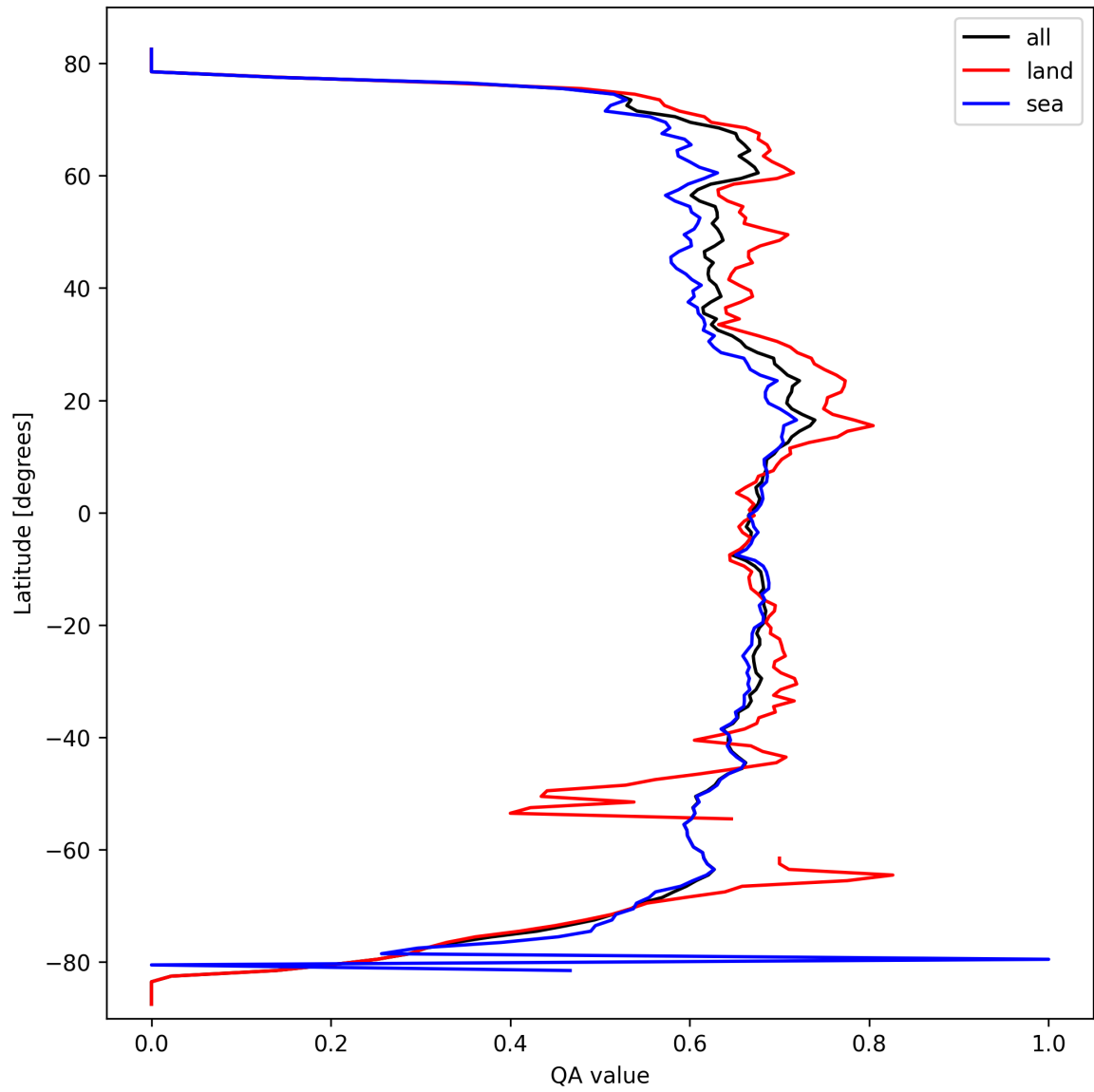
Figure 6: Zonal average of “QA value” for 2025-03-14 to 2025-03-15.
