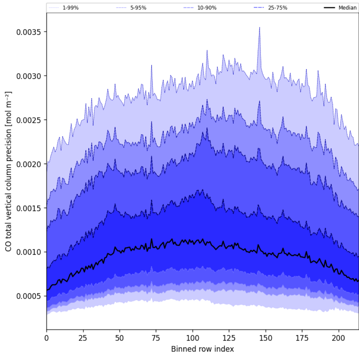
Figure 22: Along track statistics of “CO total vertical column precision” for 2025-03-14 to 2025-03-15
