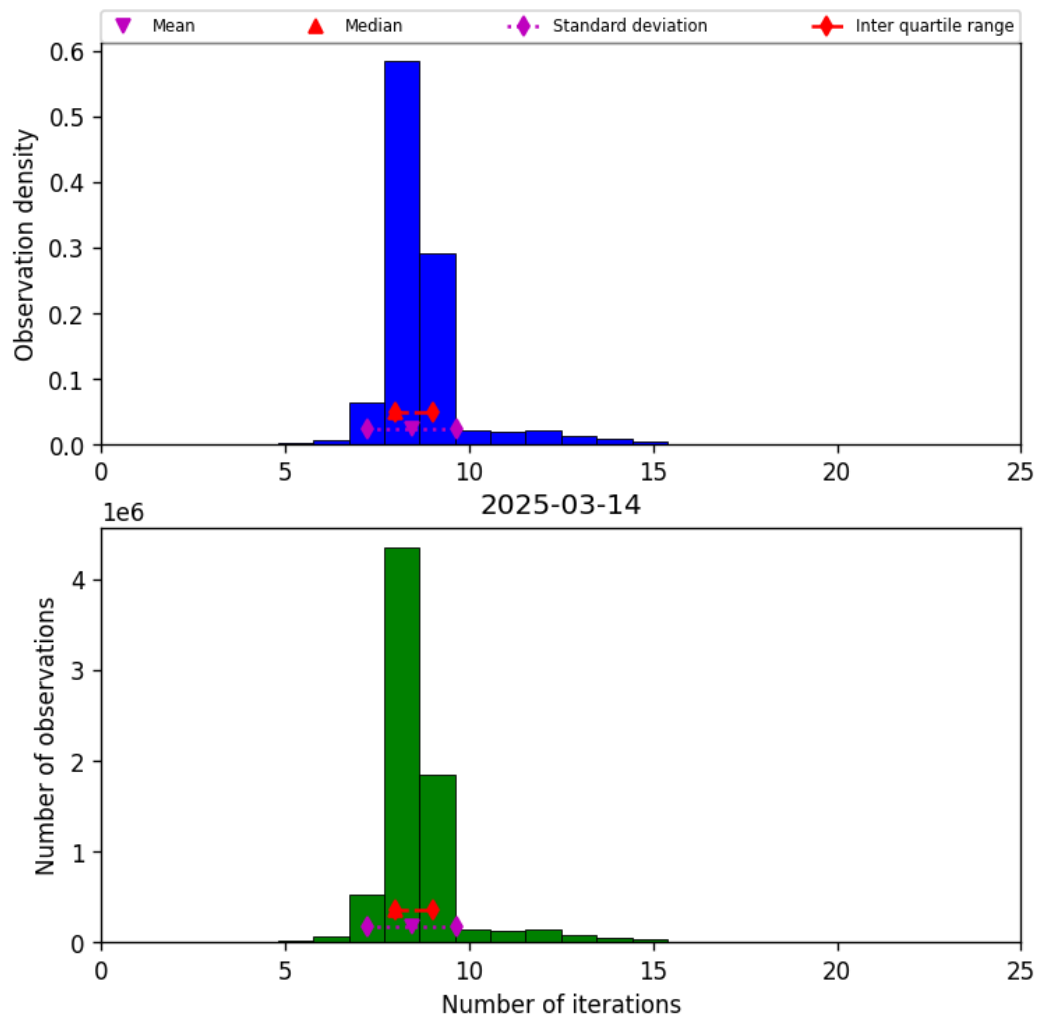
Figure 19: Histogram of “Number of iterations” for 2025-03-14 to 2025-03-15
