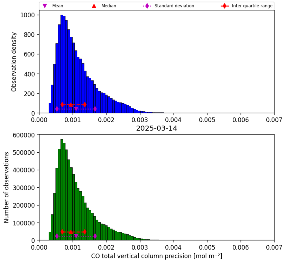
Figure 15: Histogram of “CO total vertical column precision” for 2025-03-14 to 2025-03-15
