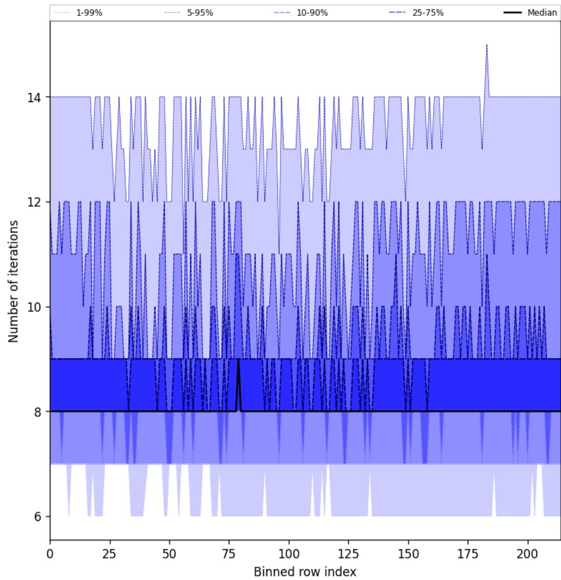
Figure 26: Along track statistics of “Number of iterations” for 2025-03-14 to 2025-03-15
