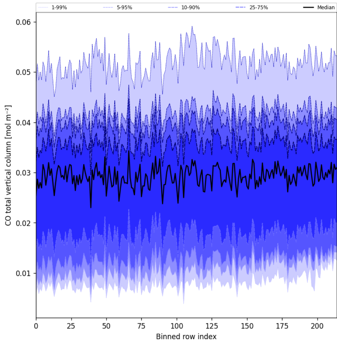
Figure 21: Along track statistics of “CO total vertical column” for 2025-03-14 to 2025-03-15
