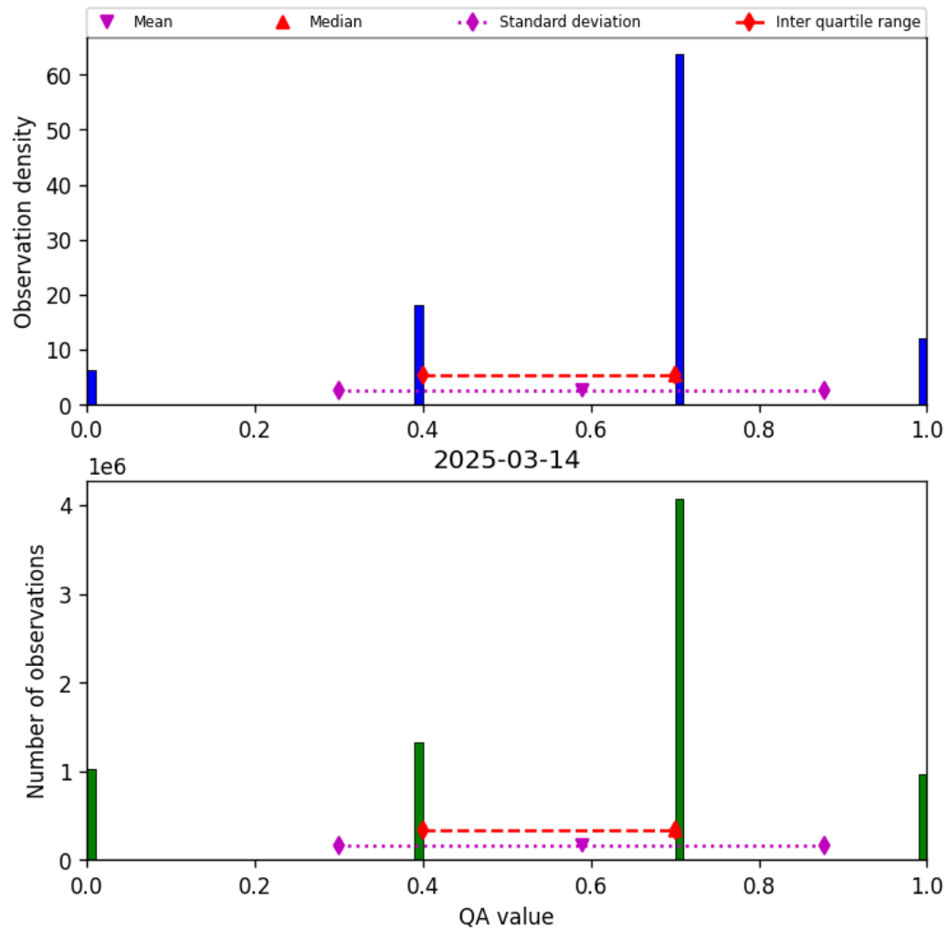
Figure 13: Histogram of “QA value” for 2025-03-14 to 2025-03-15
