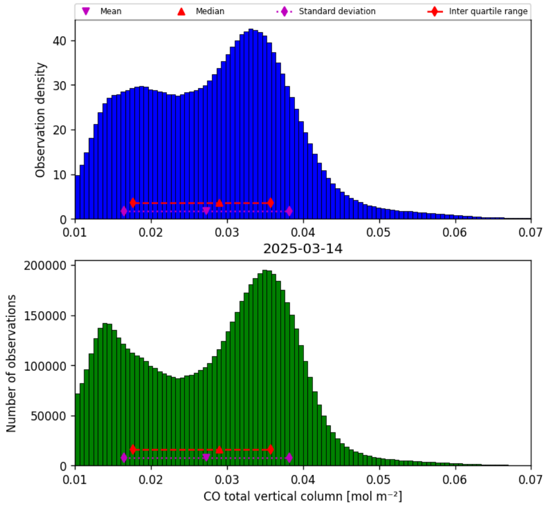
Figure 14: Histogram of “CO total vertical column” for 2025-03-14 to 2025-03-15
