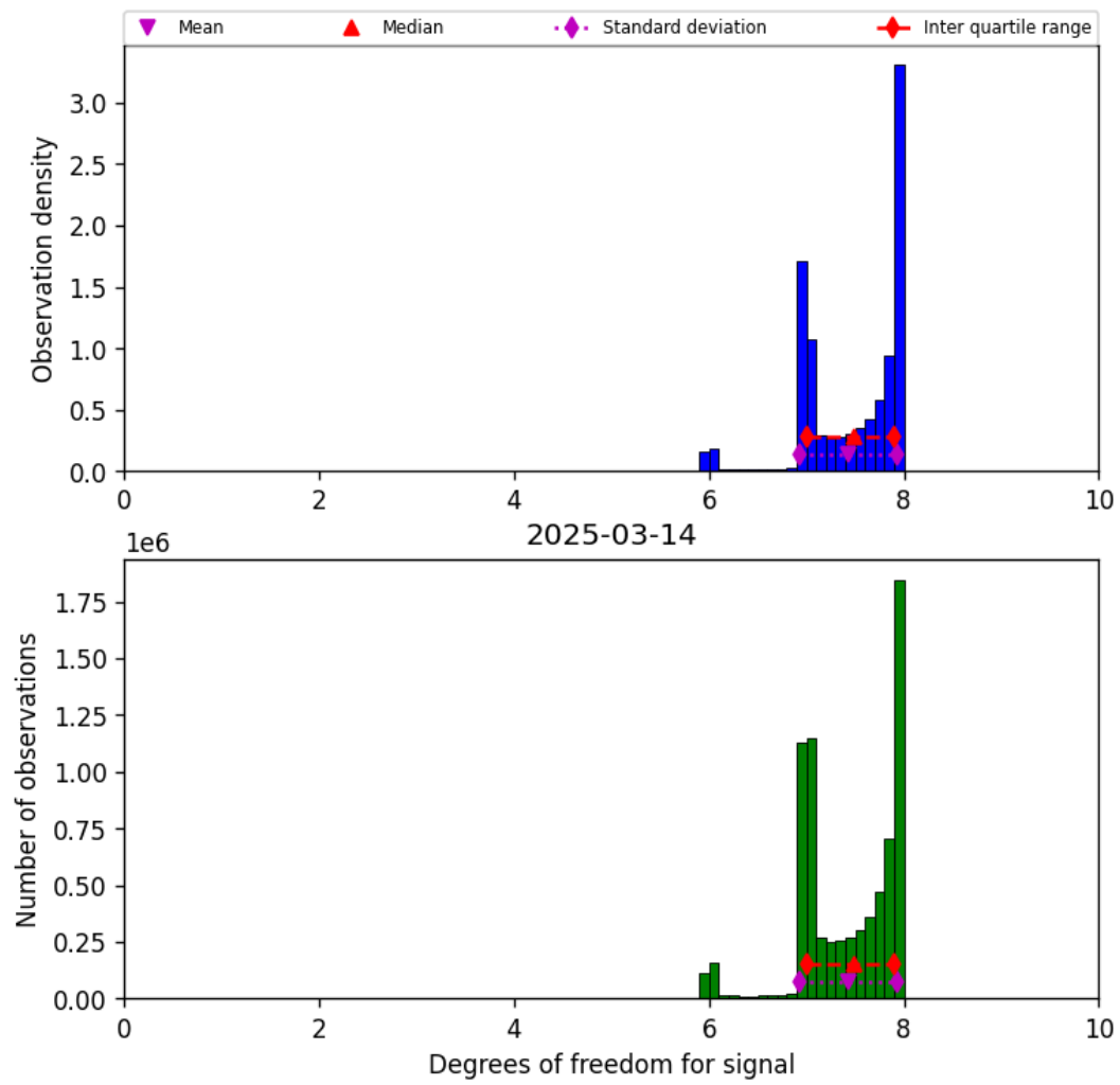
Figure 18: Histogram of “Degrees of freedom for signal” for 2025-03-14 to 2025-03-15
