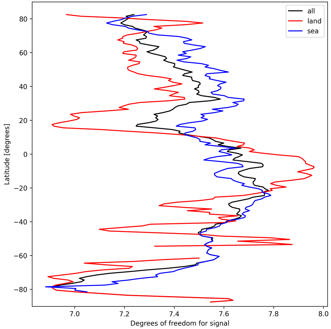
Figure 11: Zonal average of “Degrees of freedom for signal” for 2025-03-14 to 2025-03-15.
