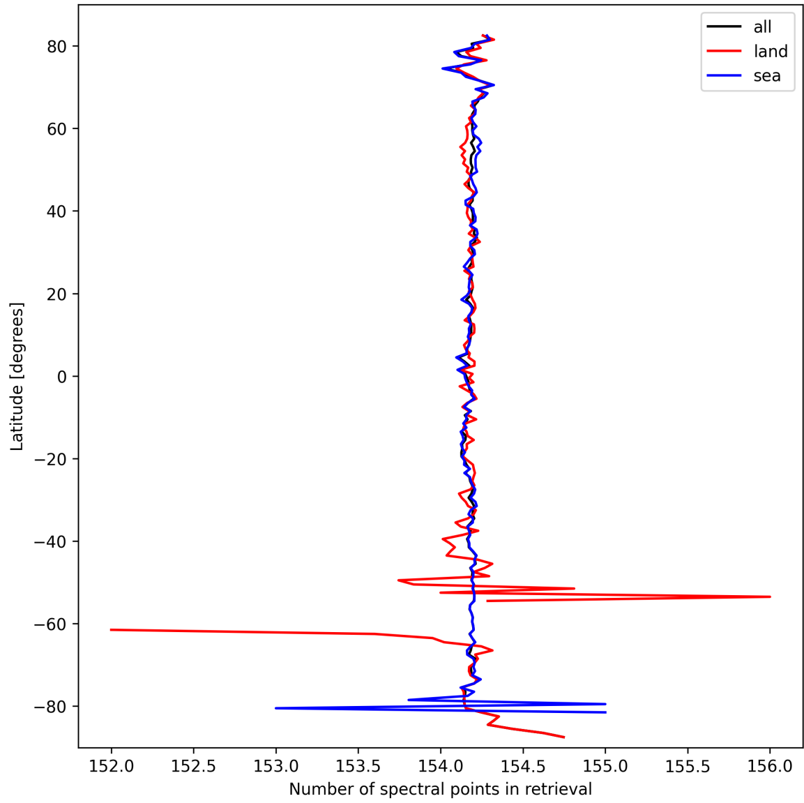
Figure 9: Zonal average of “Number of spectral points in retrieval” for 2025-03-14 to 2025-03-15.
