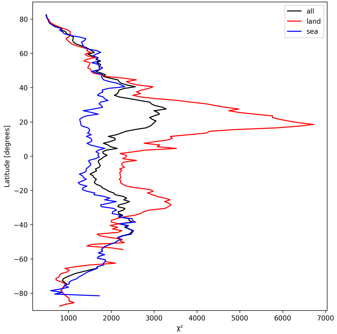
Figure 10: Zonal average of “ \chi^2 ” for 2025-03-14 to 2025-03-15.
