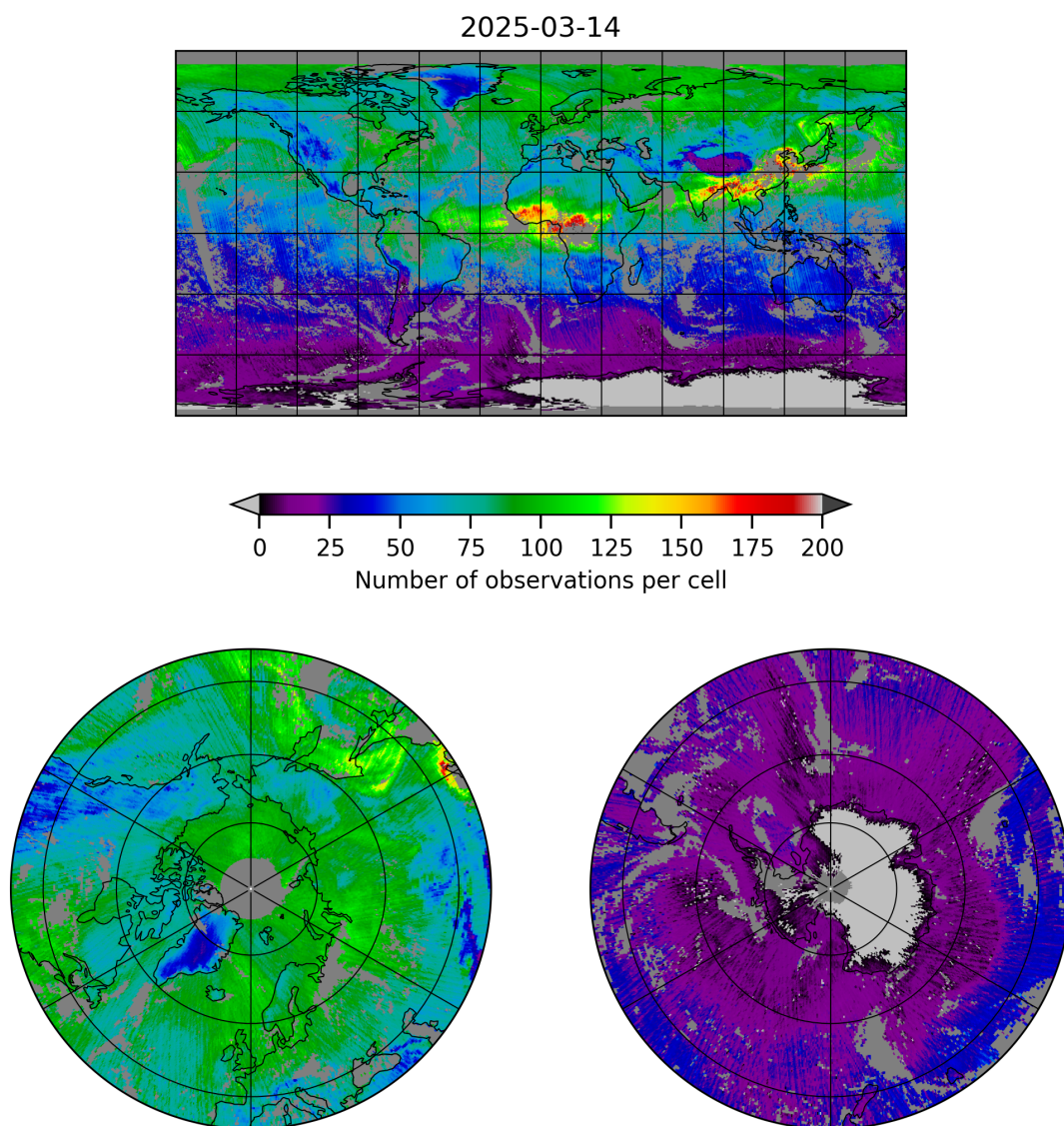
Figure 5: Map of the number of observations for 2025-03-14 to 2025-03-15
