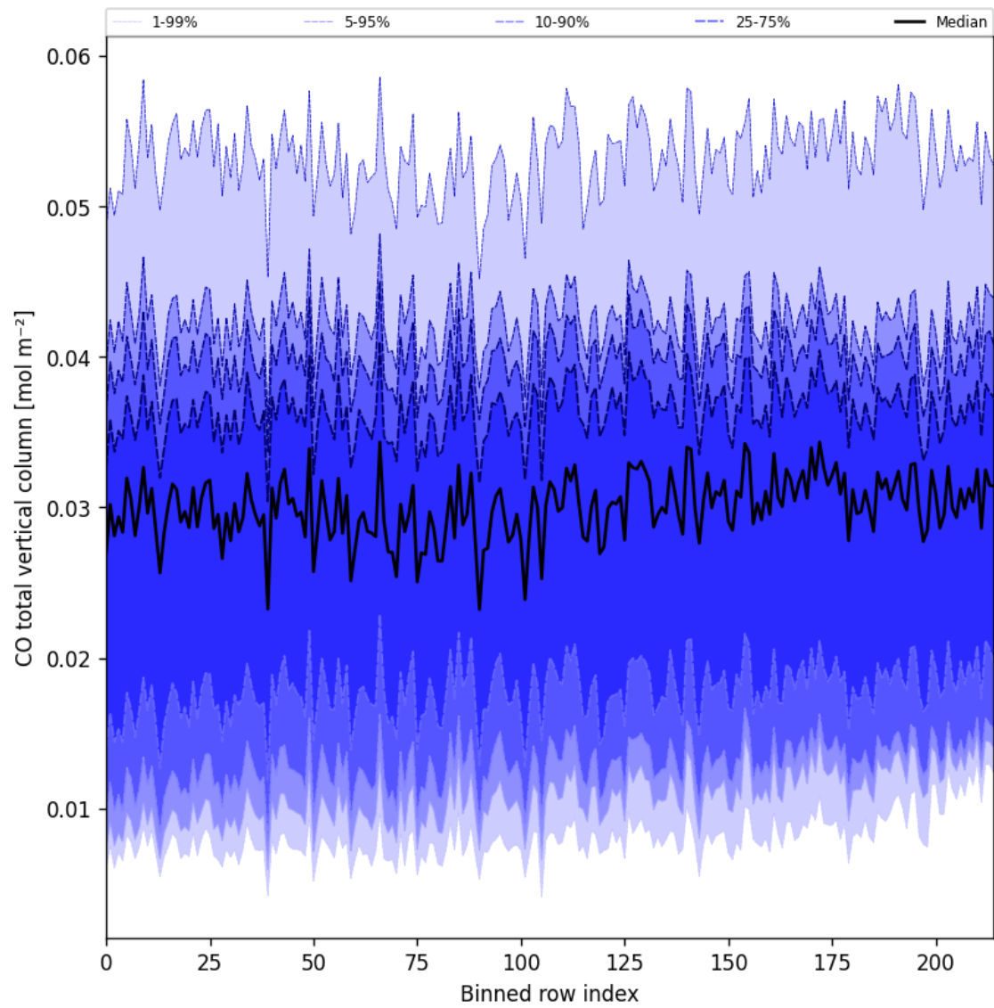
Figure 21: Along track statistics of “CO total vertical column” for 2025-03-16 to 2025-03-17
