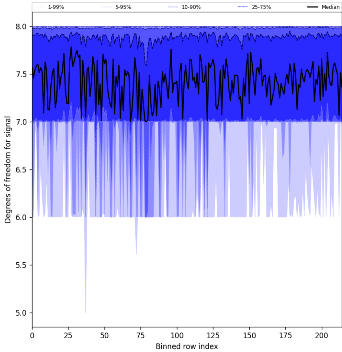
Figure 25: Along track statistics of “Degrees of freedom for signal” for 2025-03-16 to 2025-03-17
