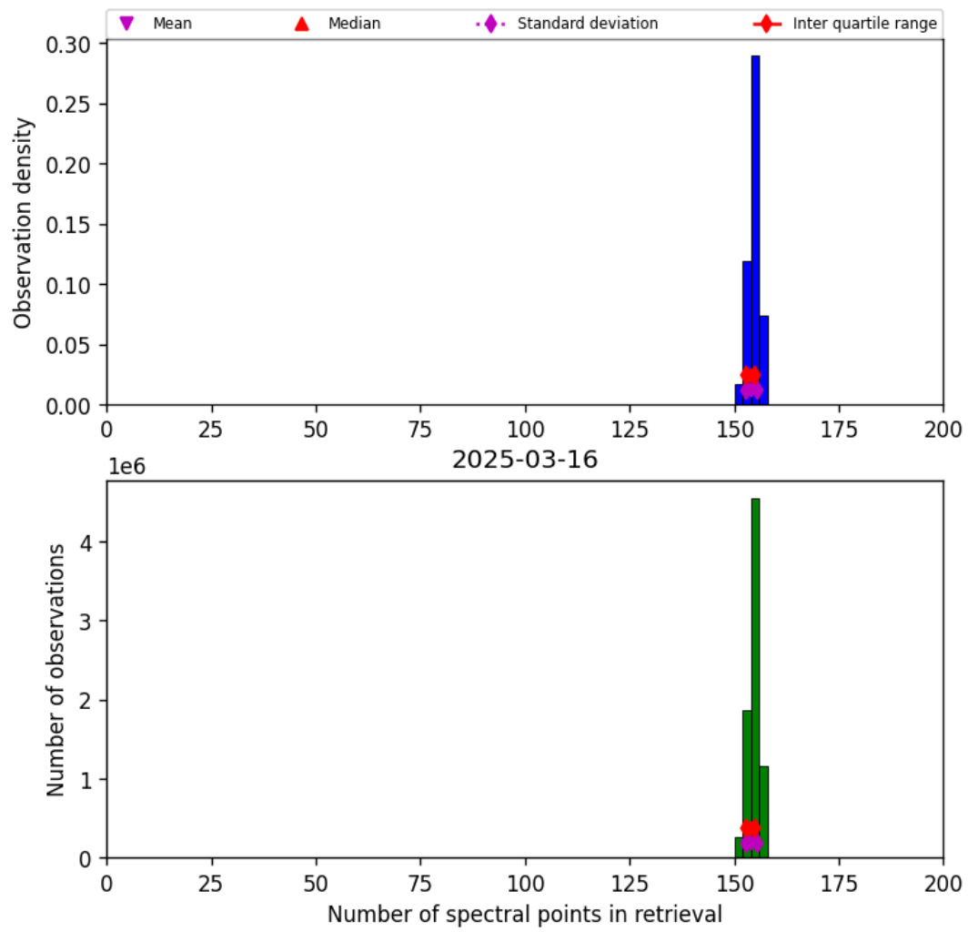
Figure 16: Histogram of “Number of spectral points in retrieval” for 2025-03-16 to 2025-03-17
