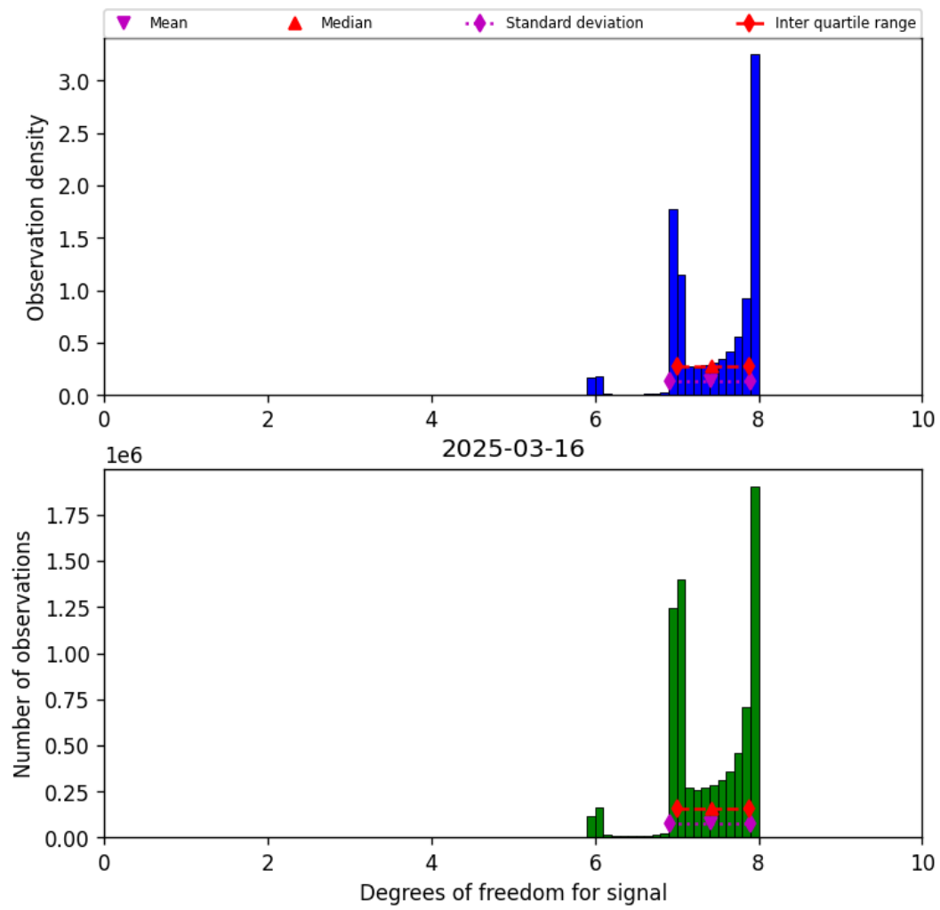
Figure 18: Histogram of “Degrees of freedom for signal” for 2025-03-16 to 2025-03-17
