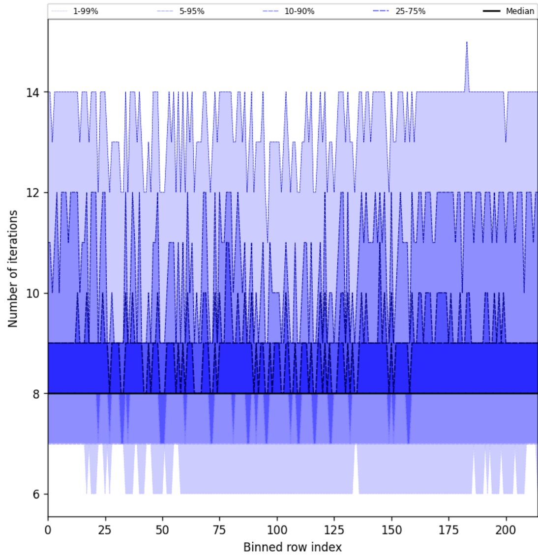
Figure 26: Along track statistics of “Number of iterations” for 2025-03-16 to 2025-03-17
