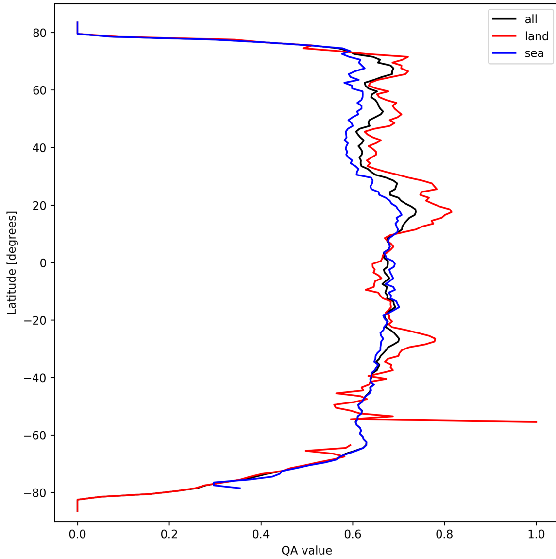
Figure 6: Zonal average of “QA value” for 2025-03-16 to 2025-03-17.
