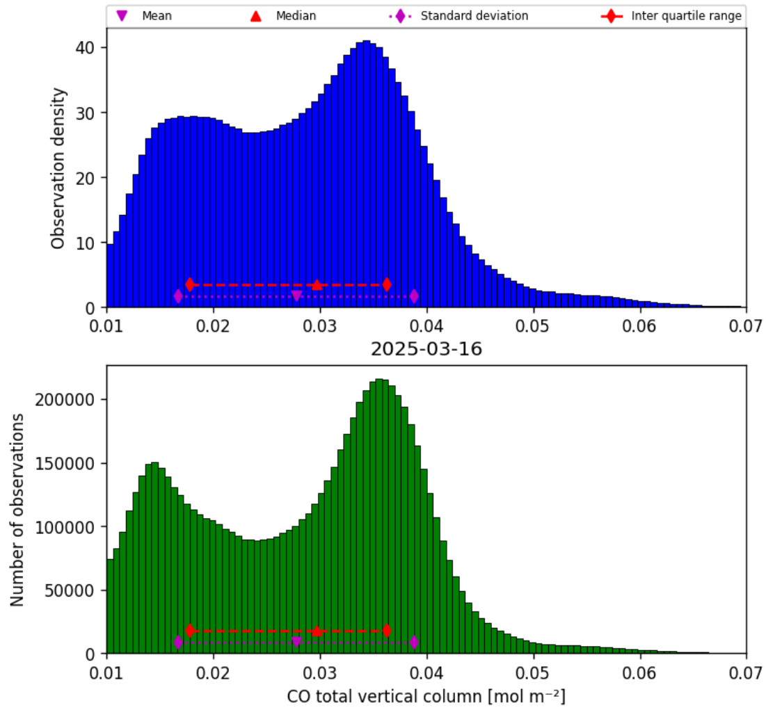
Figure 14: Histogram of “CO total vertical column” for 2025-03-16 to 2025-03-17
