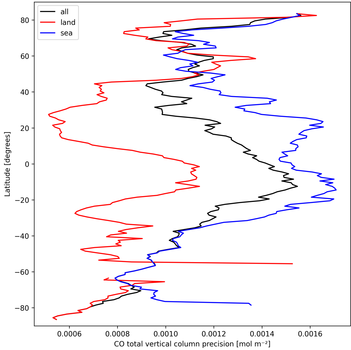
Figure 8: Zonal average of "CO total vertical column precision" for 2025-03-16 to 2025-03-17.
