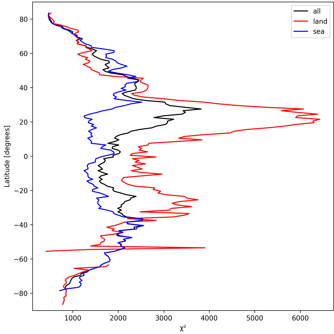
Figure 10: Zonal average of “ \chi^2 ” for 2025-03-16 to 2025-03-17.
