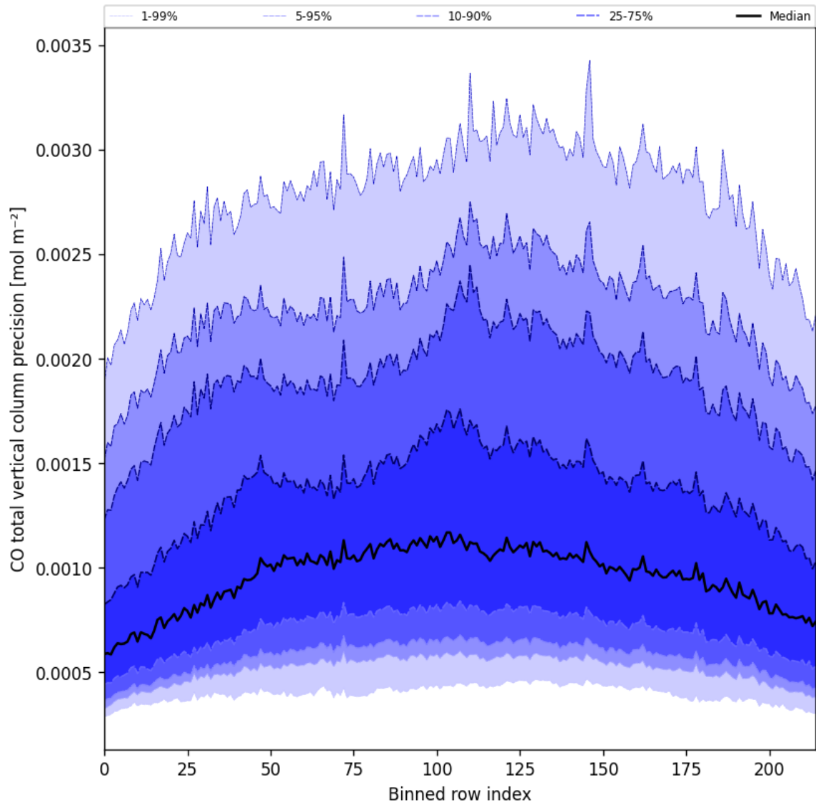
Figure 22: Along track statistics of “CO total vertical column precision” for 2025-03-16 to 2025-03-17
