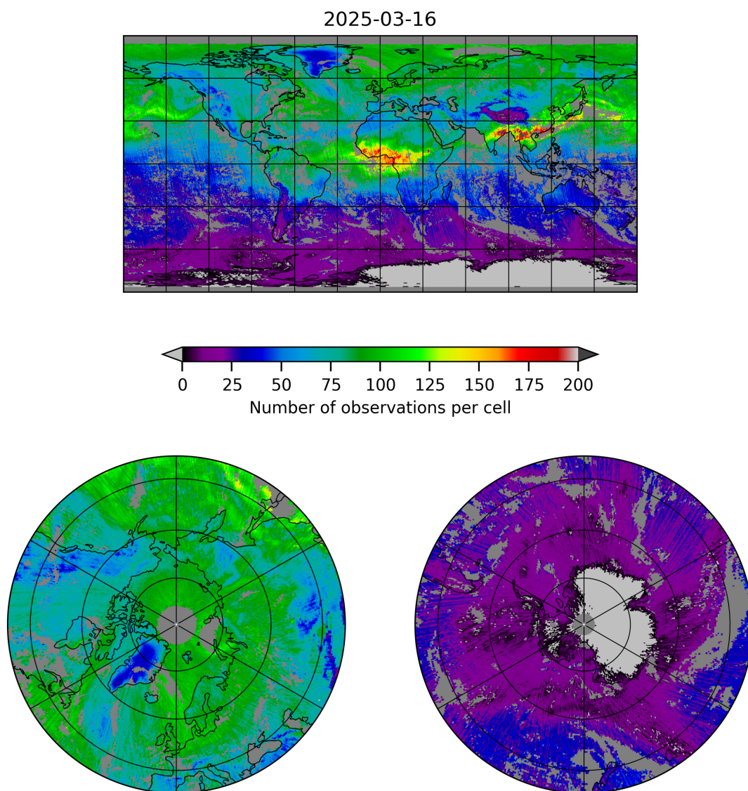
Figure 5: Map of the number of observations for 2025-03-16 to 2025-03-17
