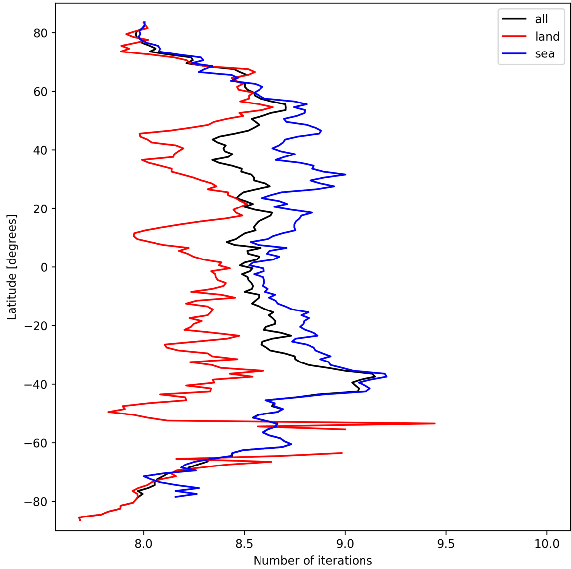
Figure 12: Zonal average of “Number of iterations” for 2025-03-16 to 2025-03-17.
