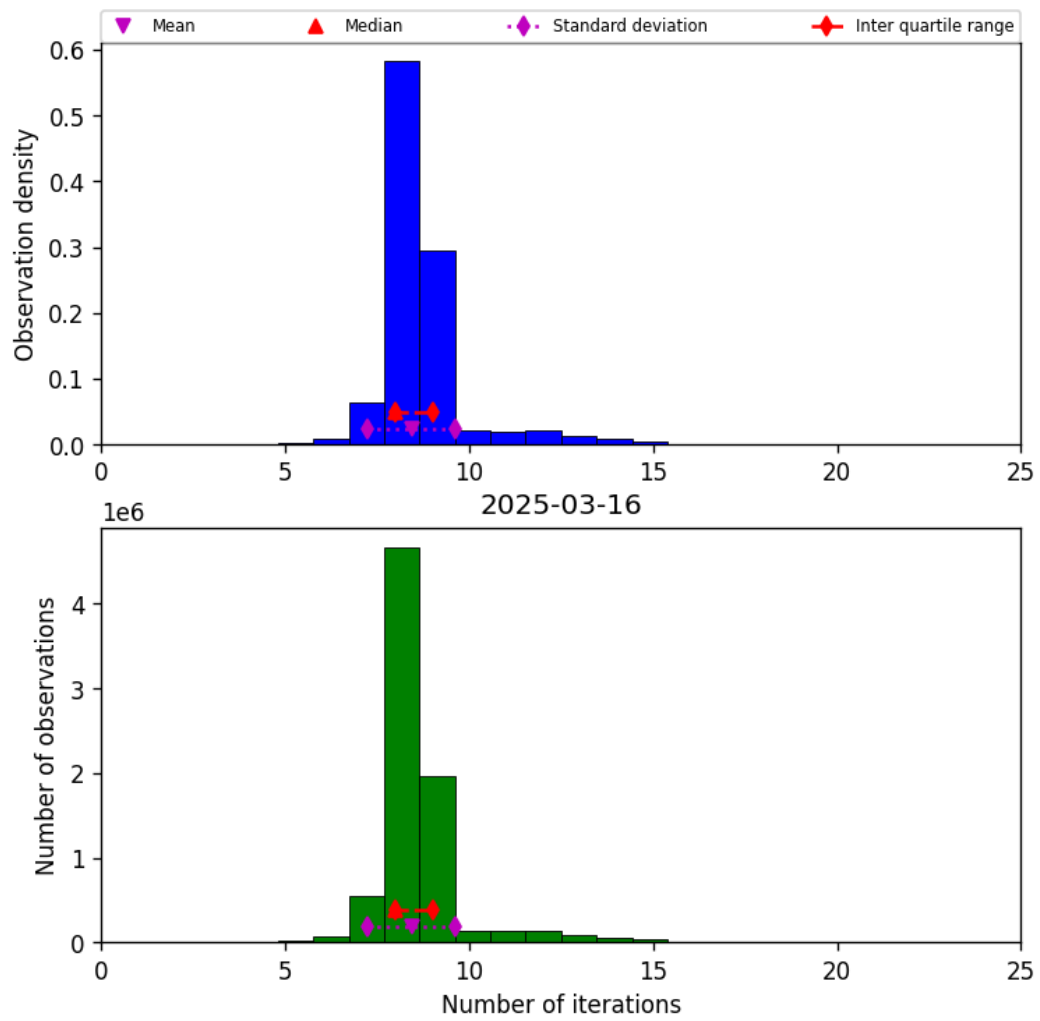
Figure 19: Histogram of “Number of iterations” for 2025-03-16 to 2025-03-17
