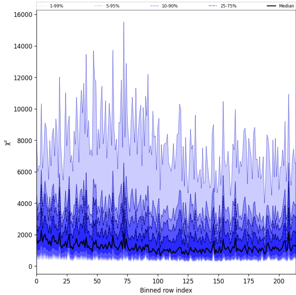
Figure 24: Along track statistics of “ \chi^2 ” for 2025-03-16 to 2025-03-17
