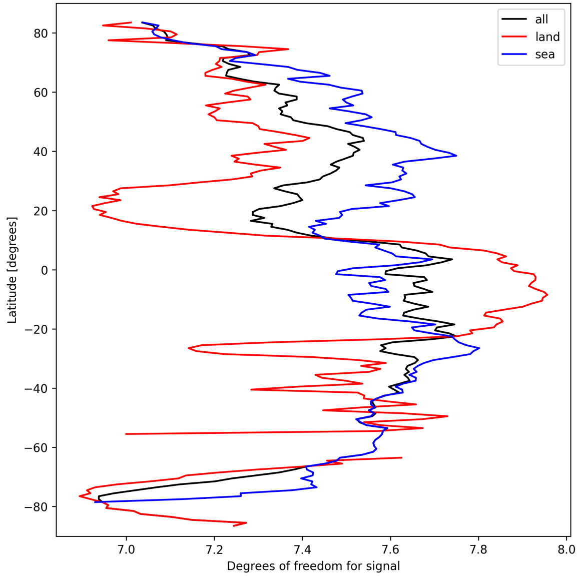
Figure 11: Zonal average of “Degrees of freedom for signal” for 2025-03-16 to 2025-03-17.
