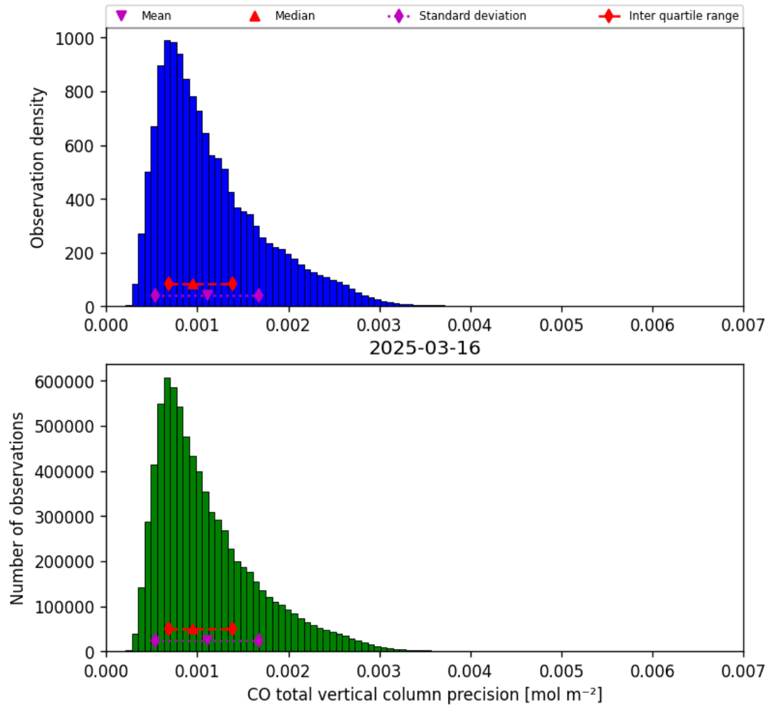
Figure 15: Histogram of “CO total vertical column precision” for 2025-03-16 to 2025-03-17
