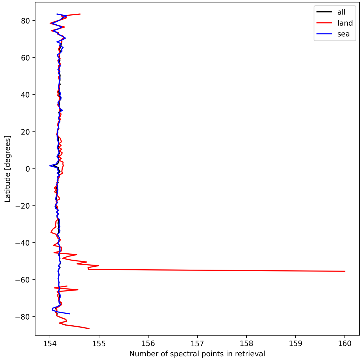
Figure 9: Zonal average of “Number of spectral points in retrieval” for 2025-03-16 to 2025-03-17.
