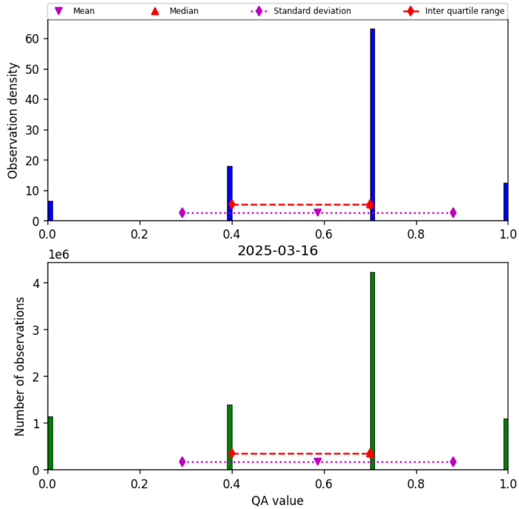
Figure 13: Histogram of “QA value” for 2025-03-16 to 2025-03-17
