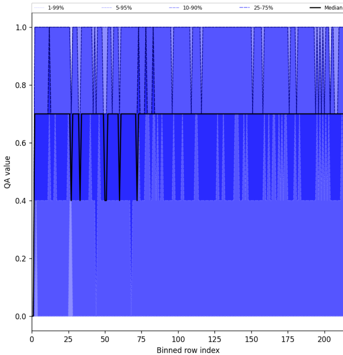
Figure 20: Along track statistics of “QA value” for 2025-03-16 to 2025-03-17
