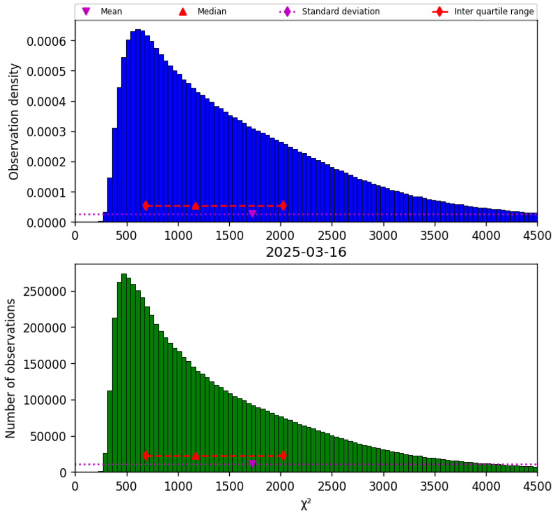
Figure 17: Histogram of “ \chi^2 ” for 2025-03-16 to 2025-03-17
