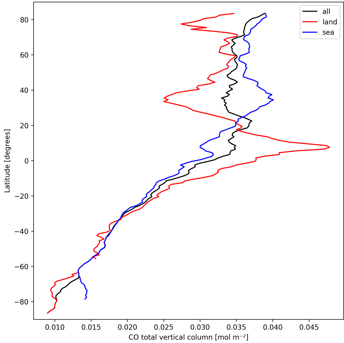
Figure 7: Zonal average of “CO total vertical column” for 2025-03-16 to 2025-03-17.
