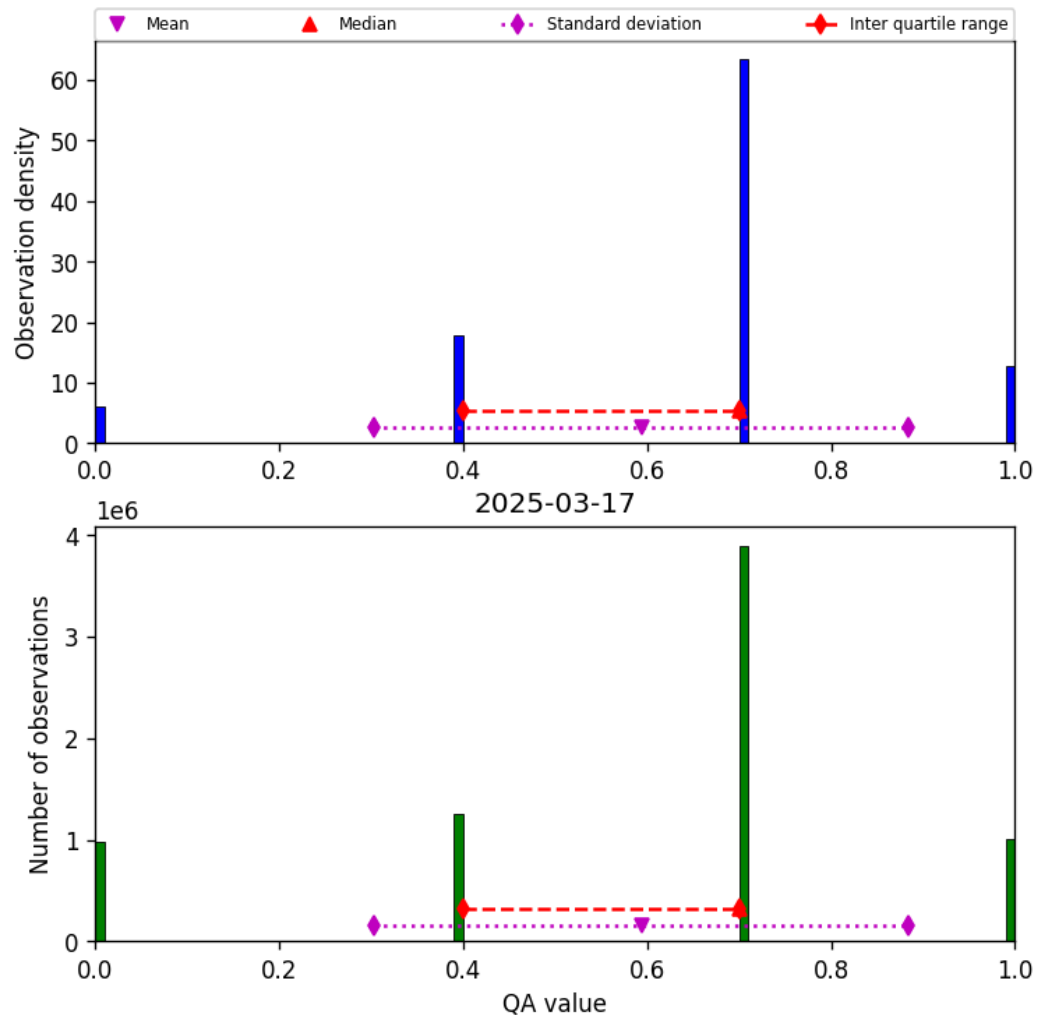
Figure 13: Histogram of “QA value” for 2025-03-17 to 2025-03-18
