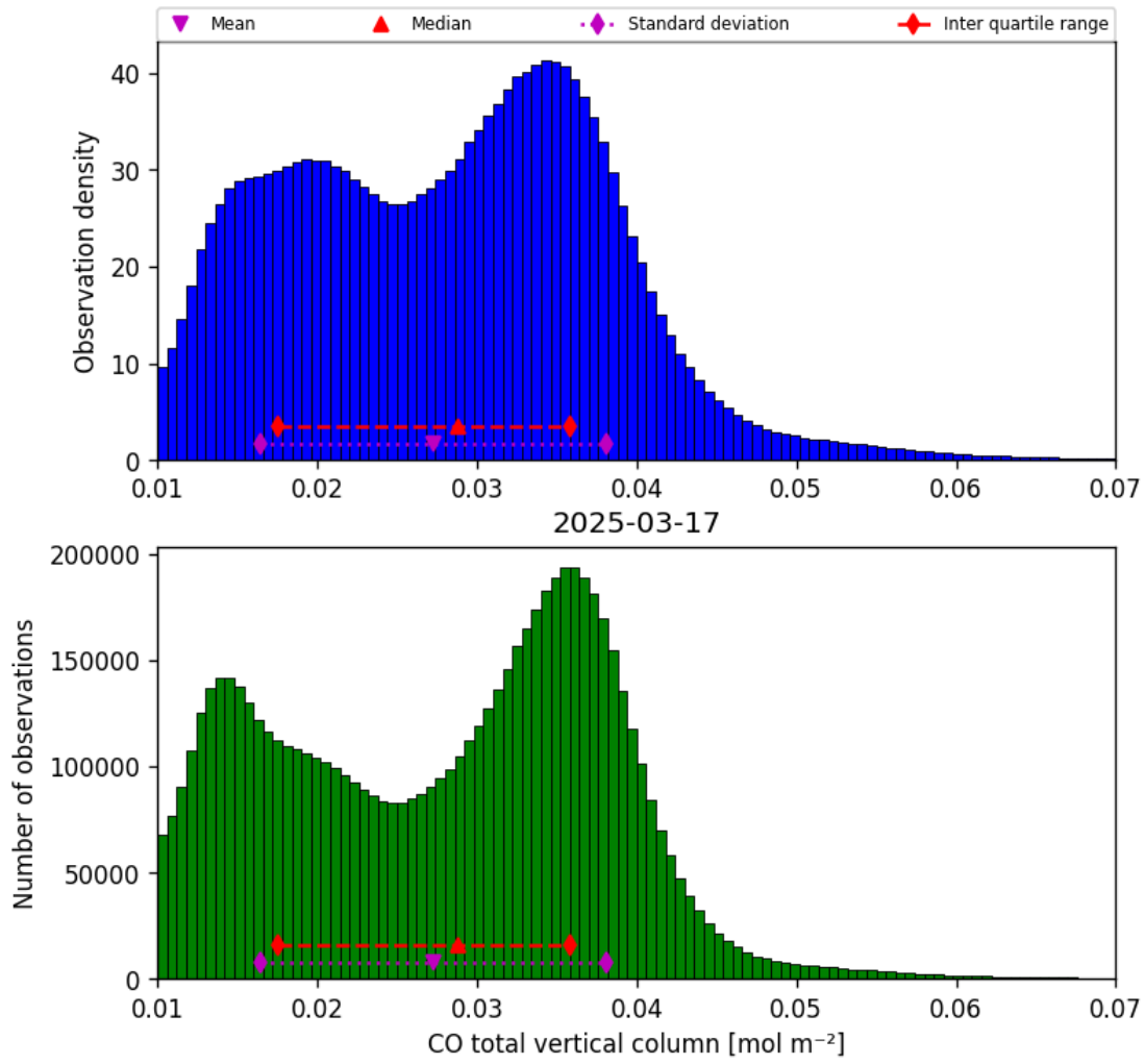
Figure 14: Histogram of “CO total vertical column” for 2025-03-17 to 2025-03-18
