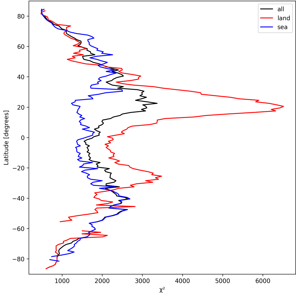
Figure 10: Zonal average of “ \chi^2 ” for 2025-03-17 to 2025-03-18.
