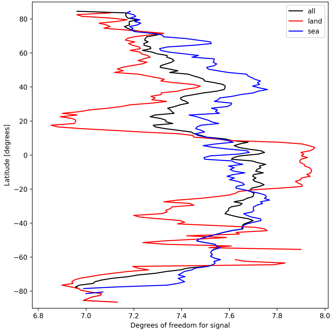
Figure 11: Zonal average of “Degrees of freedom for signal” for 2025-03-17 to 2025-03-18.
