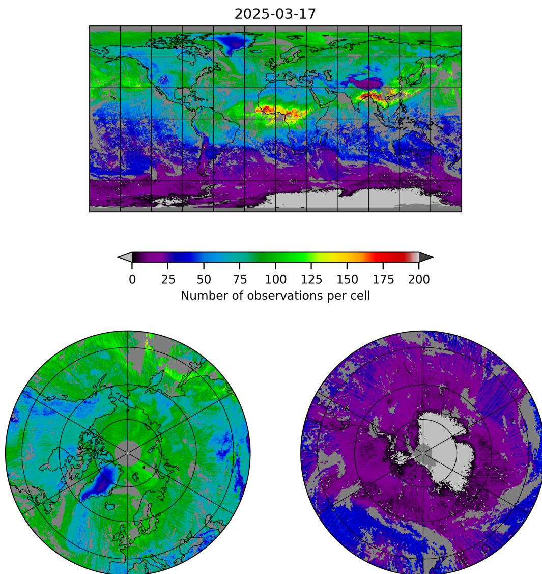
Figure 5: Map of the number of observations for 2025-03-17 to 2025-03-18
