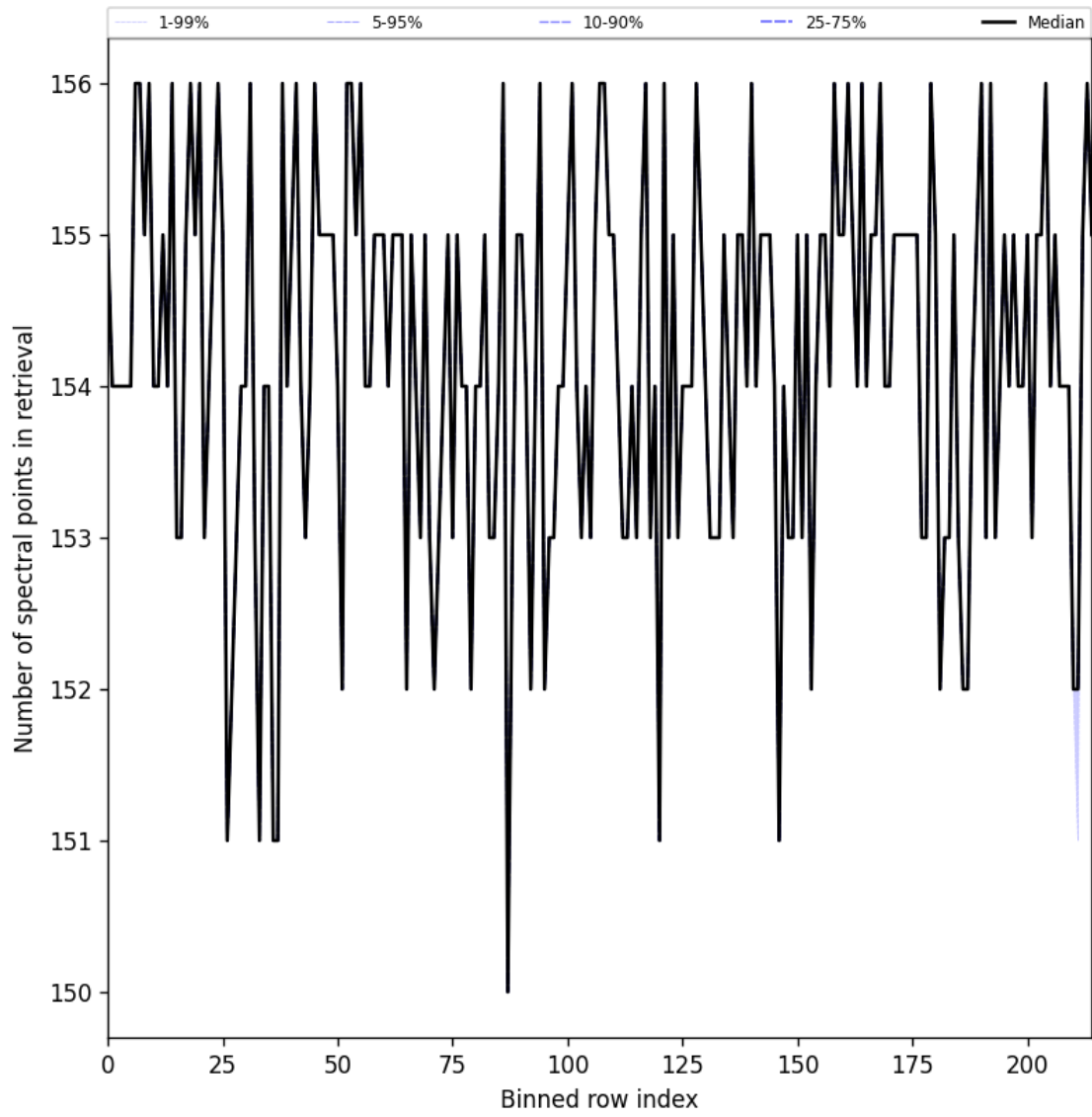
Figure 23: Along track statistics of “Number of spectral points in retrieval” for 2025-03-17 to 2025-03-18
