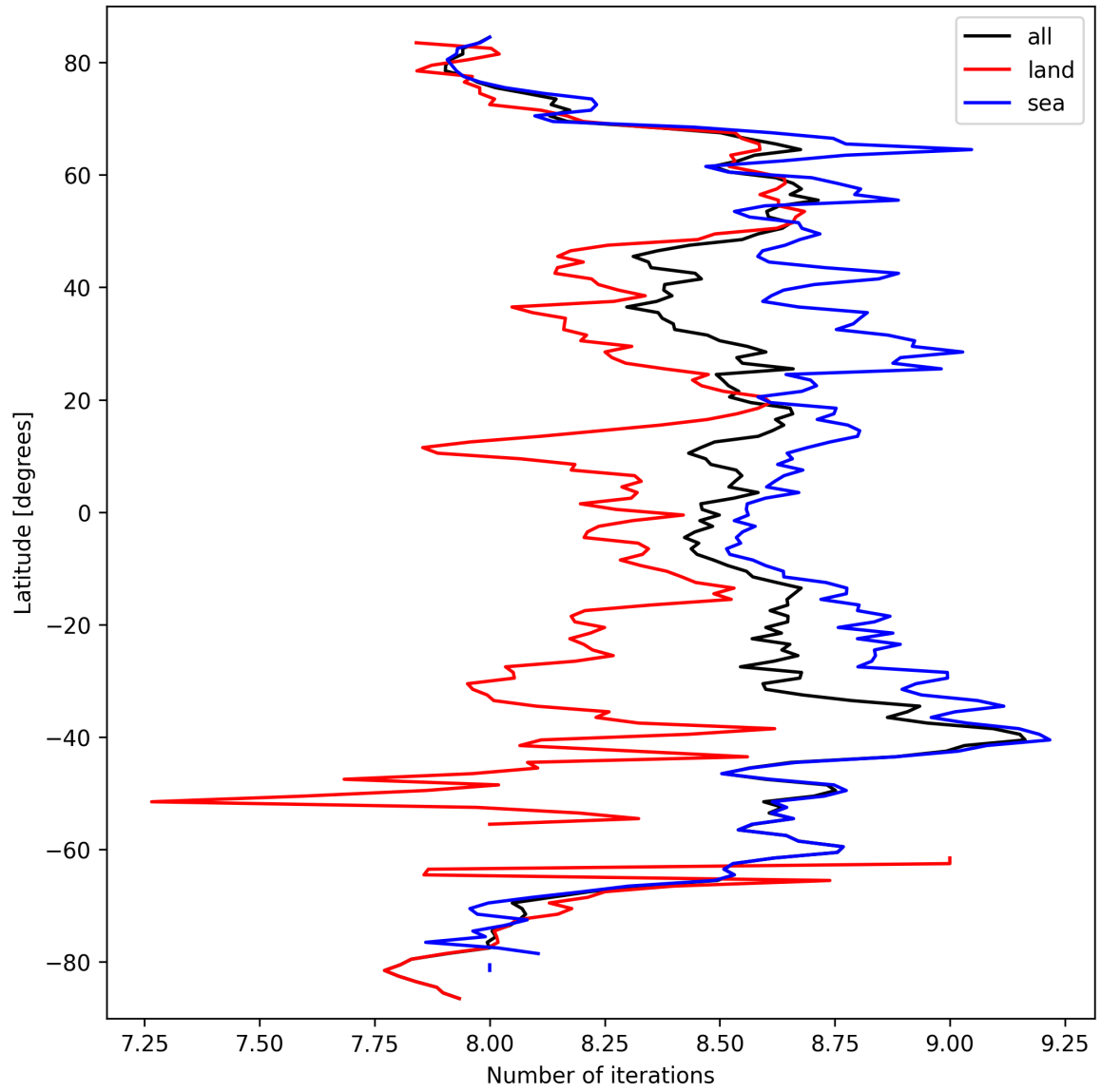
Figure 12: Zonal average of “Number of iterations” for 2025-03-17 to 2025-03-18.
