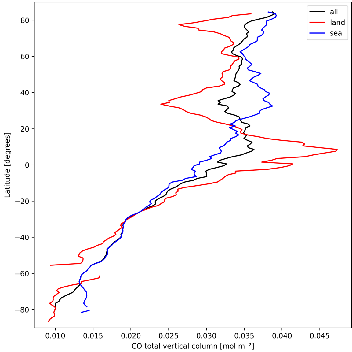
Figure 7: Zonal average of “CO total vertical column” for 2025-03-17 to 2025-03-18.
