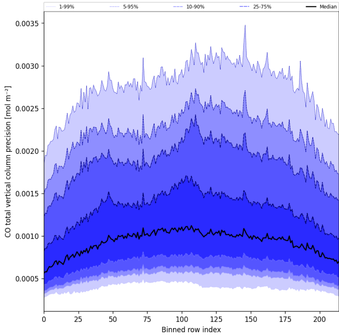
Figure 22: Along track statistics of “CO total vertical column precision” for 2025-03-17 to 2025-03-18
