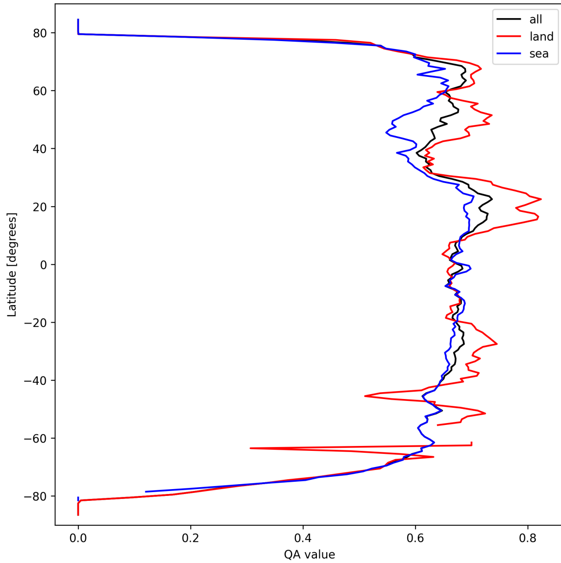
Figure 6: Zonal average of “QA value” for 2025-03-17 to 2025-03-18.
