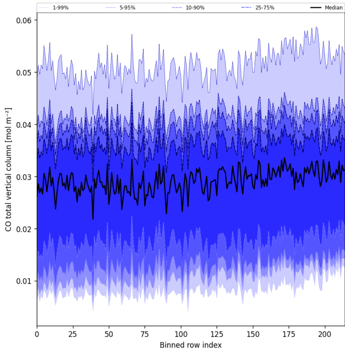
Figure 21: Along track statistics of “CO total vertical column” for 2025-03-17 to 2025-03-18
