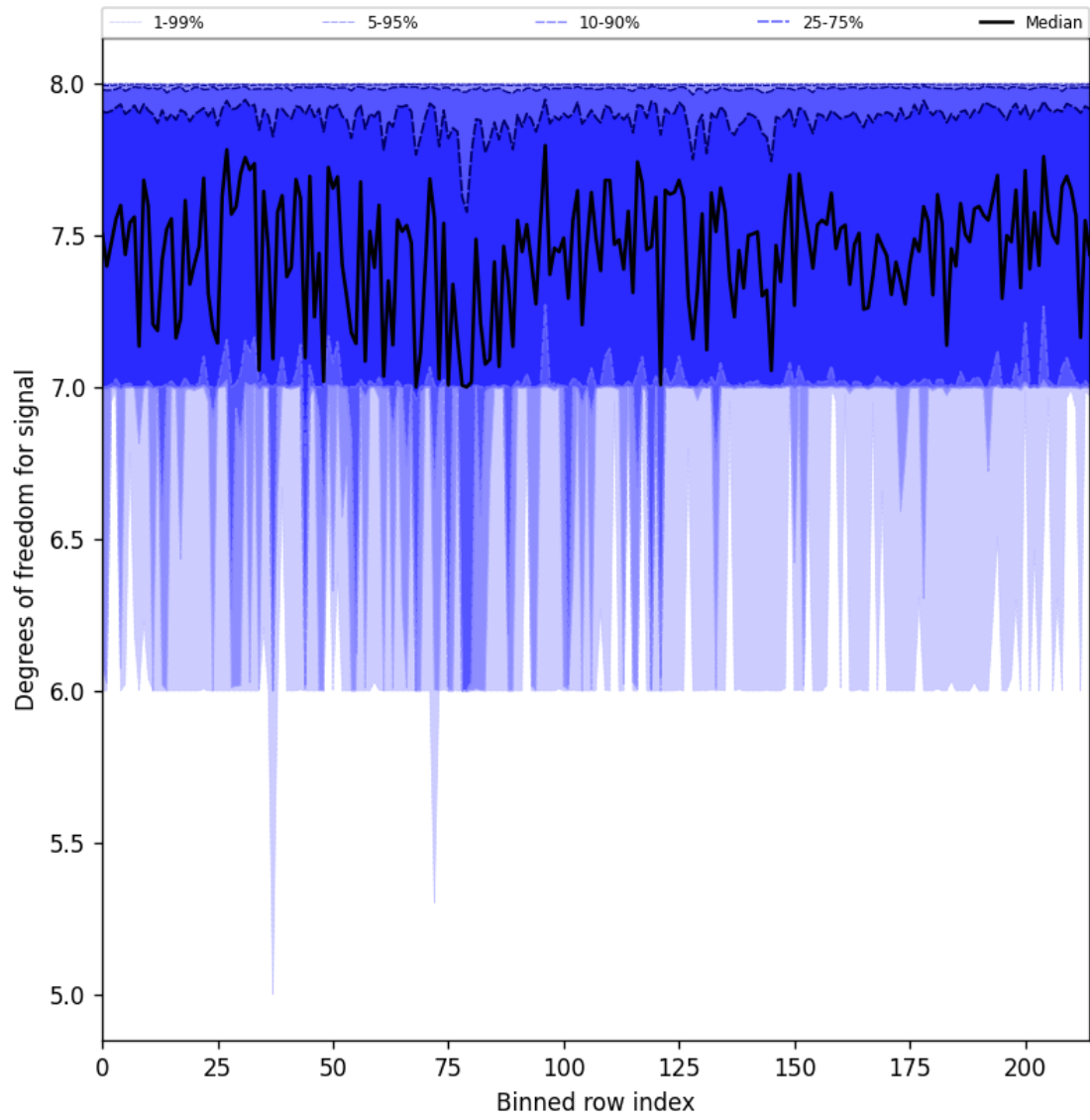
Figure 25: Along track statistics of “Degrees of freedom for signal” for 2025-03-17 to 2025-03-18
