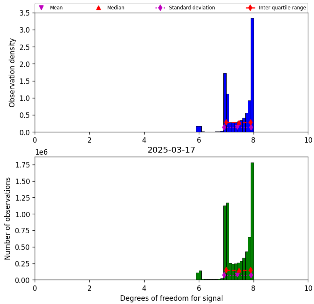
Figure 18: Histogram of “Degrees of freedom for signal” for 2025-03-17 to 2025-03-18
