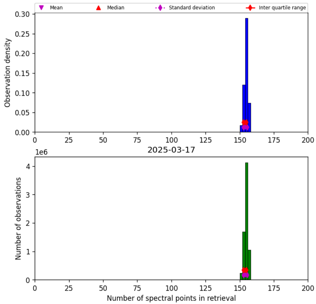
Figure 16: Histogram of “Number of spectral points in retrieval” for 2025-03-17 to 2025-03-18
