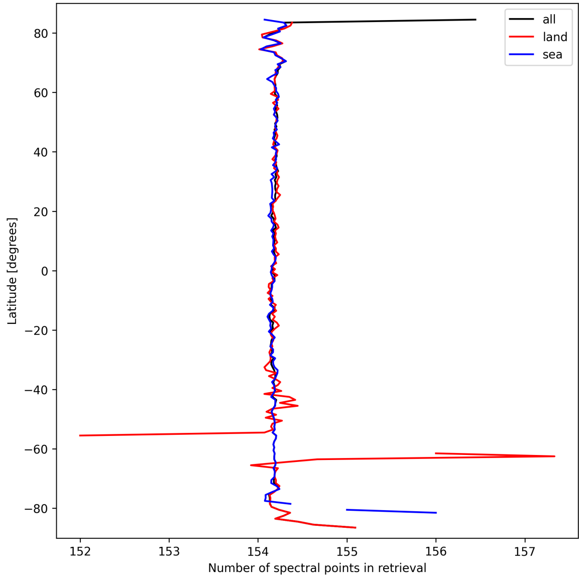
Figure 9: Zonal average of “Number of spectral points in retrieval” for 2025-03-17 to 2025-03-18.
