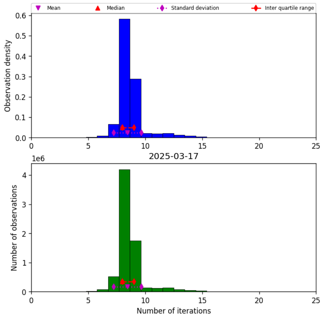
Figure 19: Histogram of “Number of iterations” for 2025-03-17 to 2025-03-18
