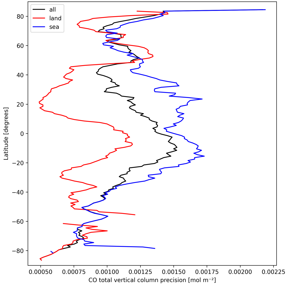
Figure 8: Zonal average of “CO total vertical column precision” for 2025-03-17 to 2025-03-18.
