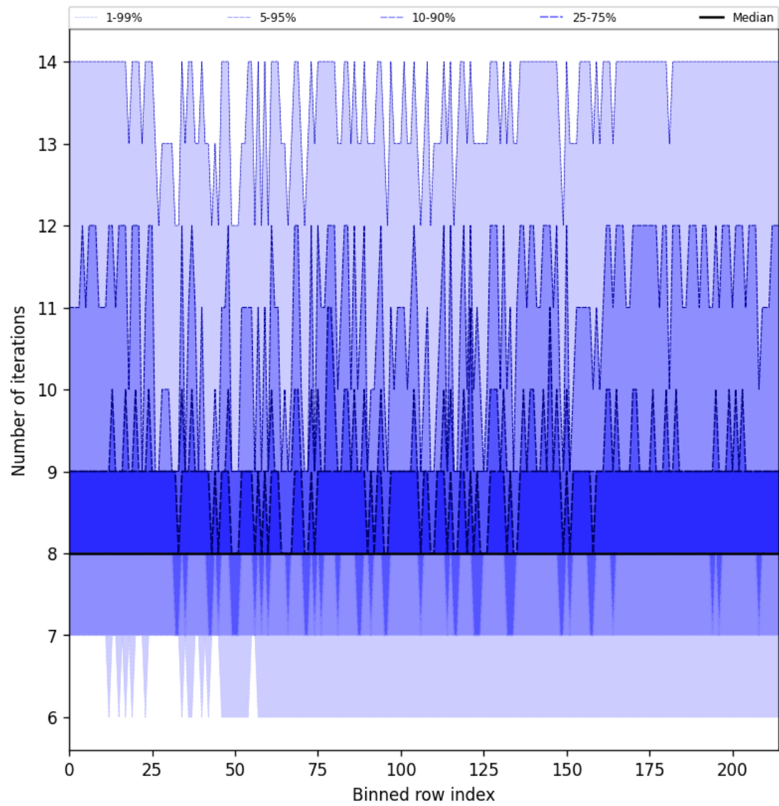
Figure 26: Along track statistics of “Number of iterations” for 2025-03-17 to 2025-03-18
