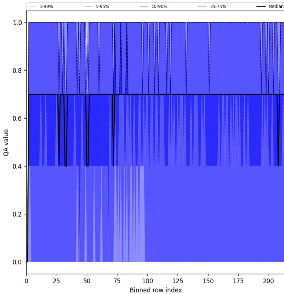
Figure 20: Along track statistics of “QA value” for 2025-03-17 to 2025-03-18
