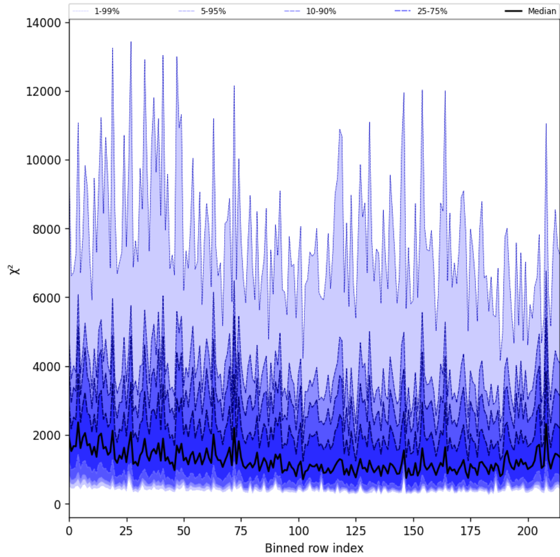
Figure 24: Along track statistics of “ \chi^2 ” for 2025-03-17 to 2025-03-18
