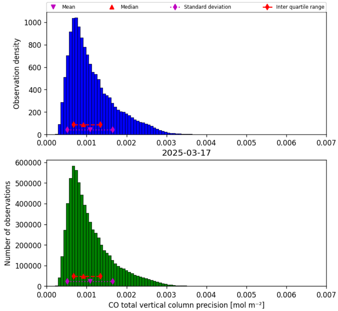
Figure 15: Histogram of “CO total vertical column precision” for 2025-03-17 to 2025-03-18
