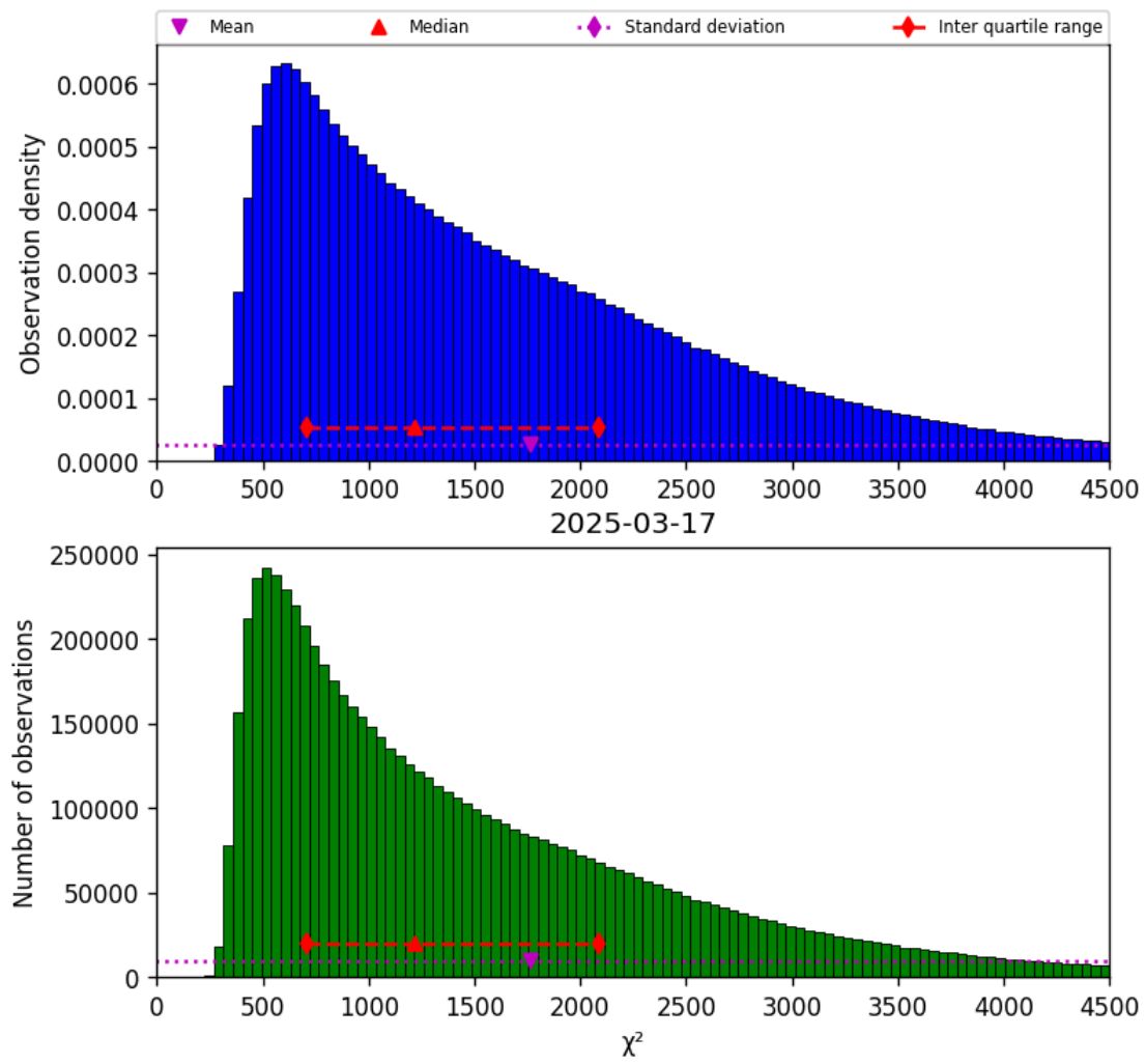
Figure 17: Histogram of “ \chi^2 ” for 2025-03-17 to 2025-03-18
