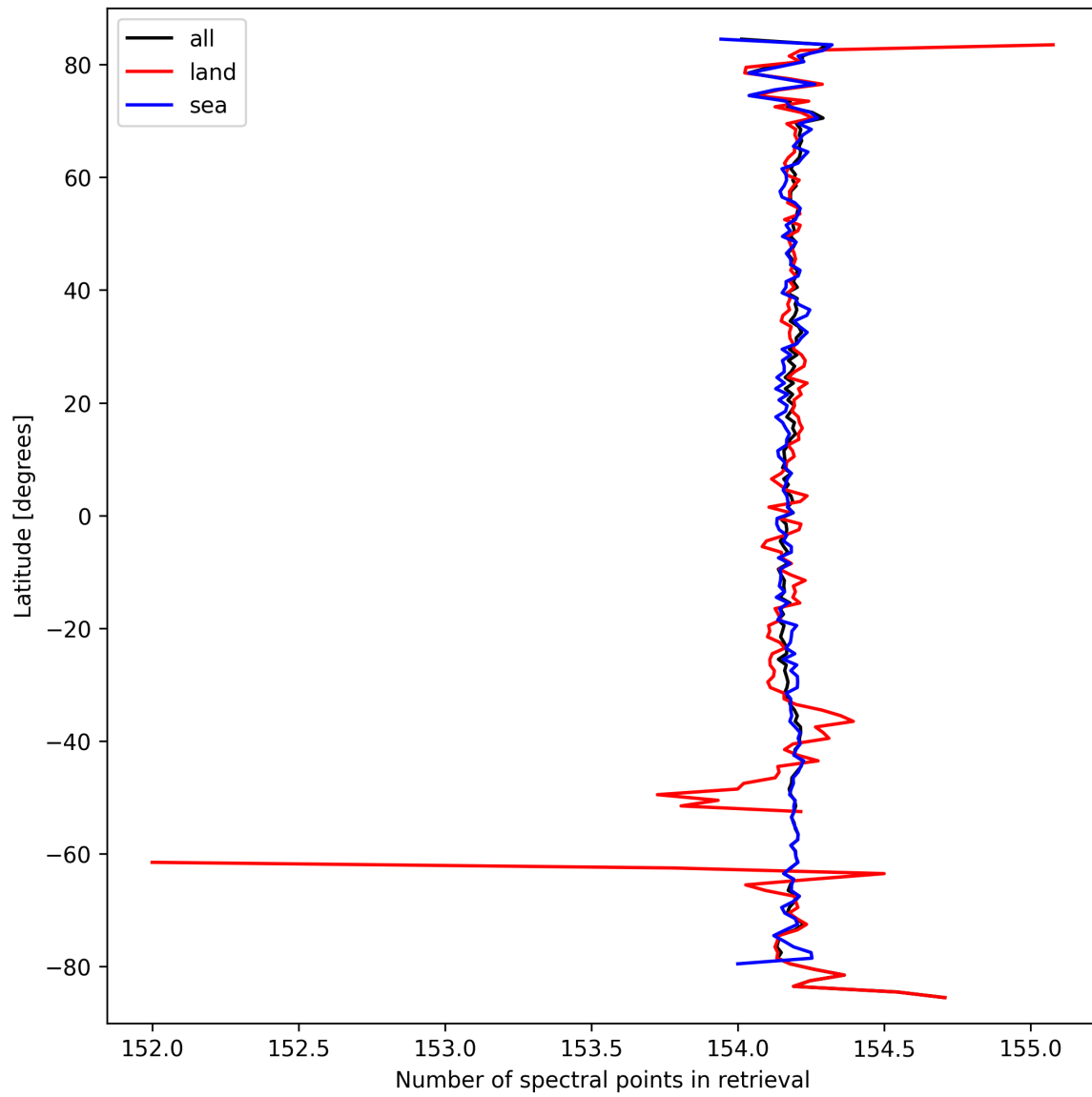
Figure 9: Zonal average of “Number of spectral points in retrieval” for 2025-03-18 to 2025-03-19.
