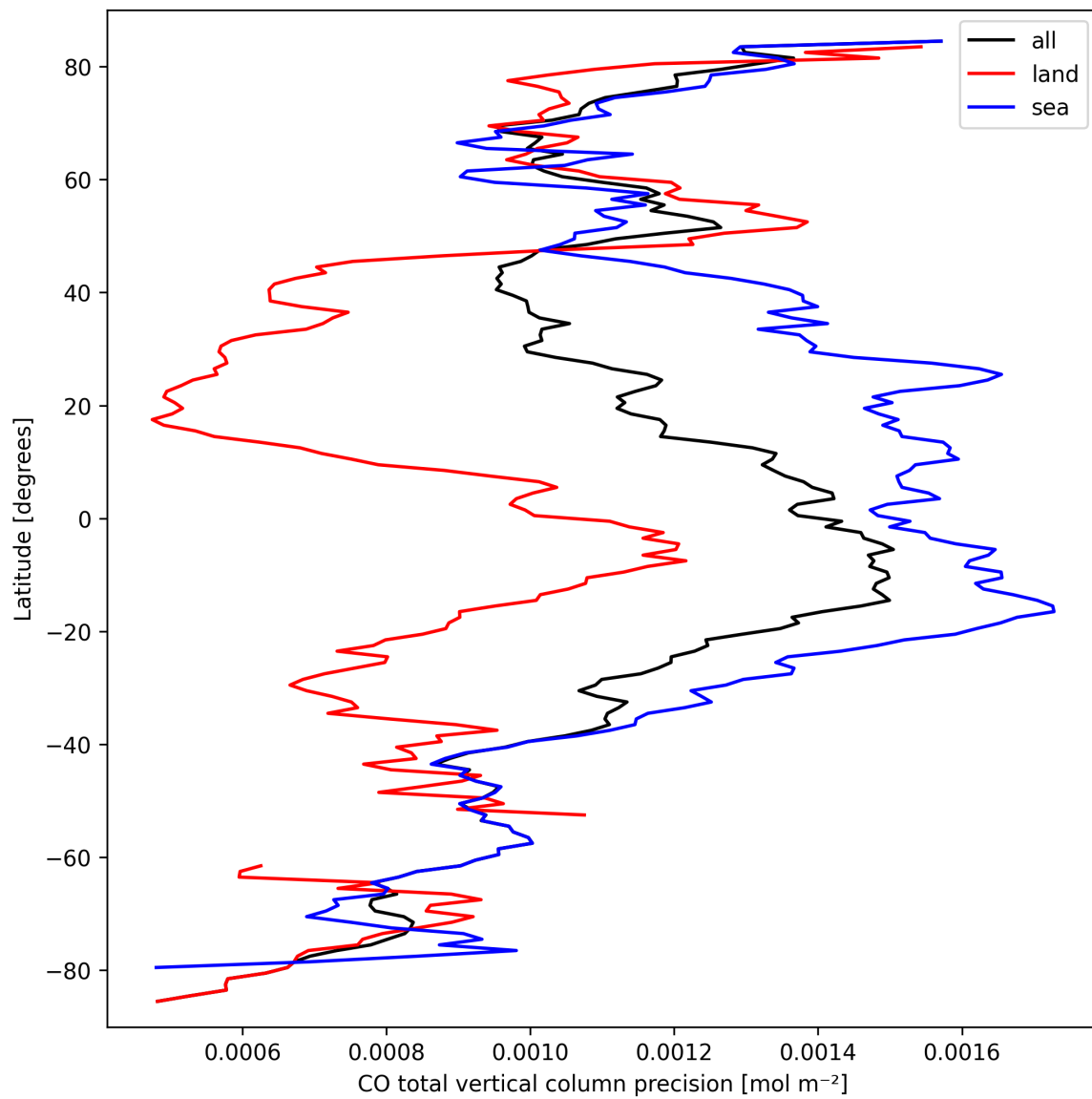
Figure 8: Zonal average of “CO total vertical column precision” for 2025-03-18 to 2025-03-19.
