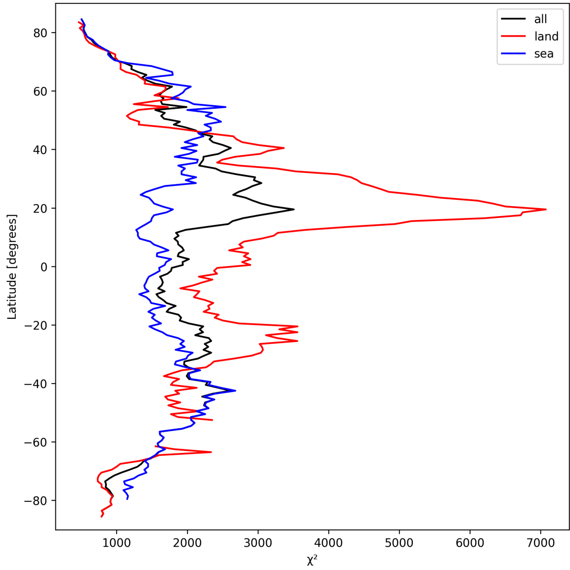
Figure 10: Zonal average of “ \chi^2 ” for 2025-03-18 to 2025-03-19.
