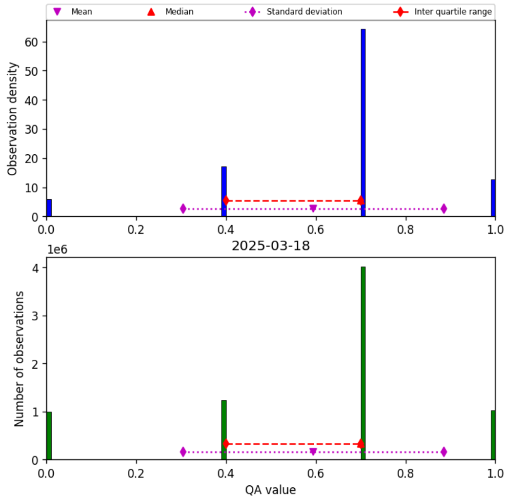
Figure 13: Histogram of “QA value” for 2025-03-18 to 2025-03-19
