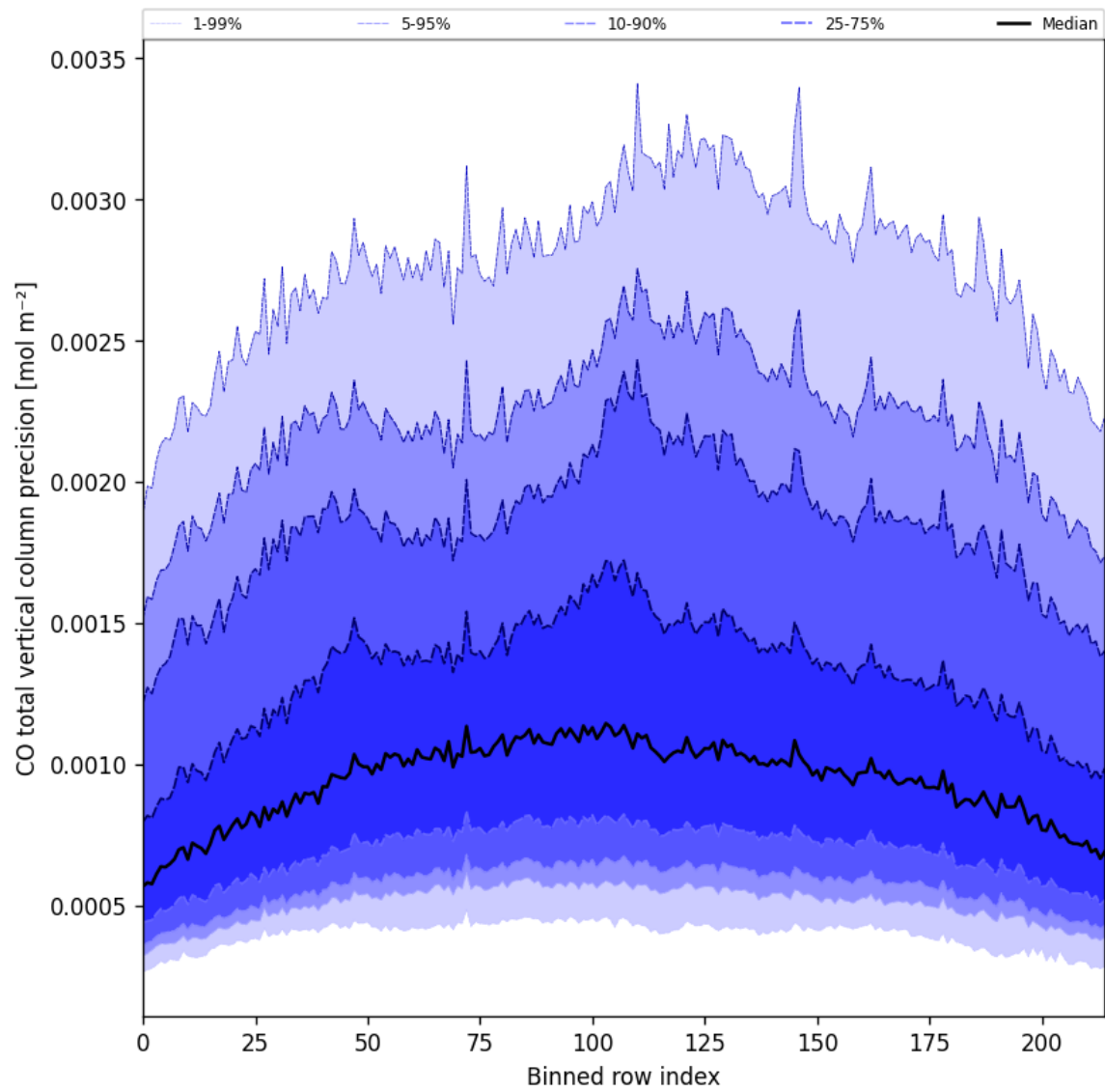
Figure 22: Along track statistics of “CO total vertical column precision” for 2025-03-18 to 2025-03-19
