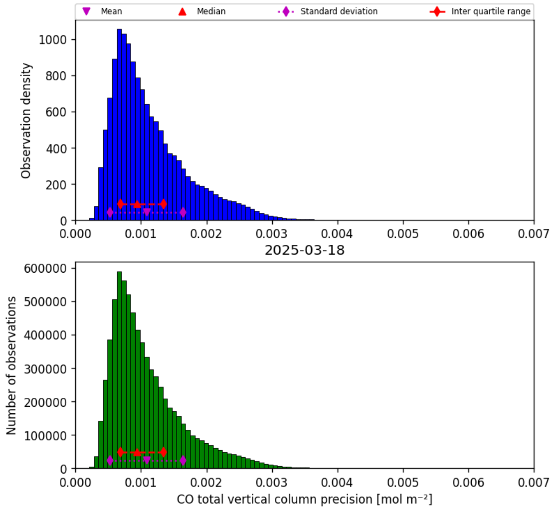
Figure 15: Histogram of “CO total vertical column precision” for 2025-03-18 to 2025-03-19
