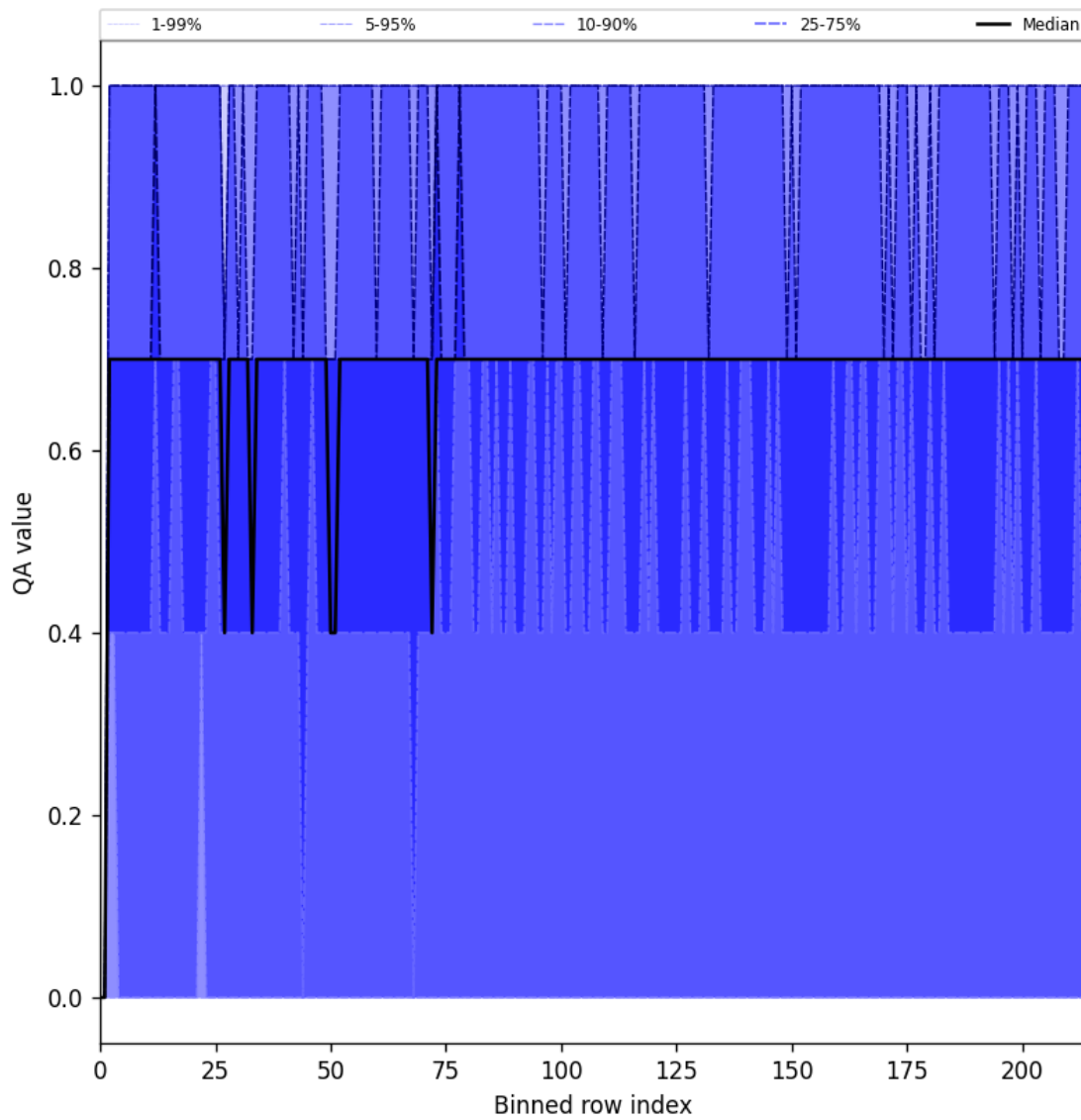
Figure 20: Along track statistics of “QA value” for 2025-03-18 to 2025-03-19
