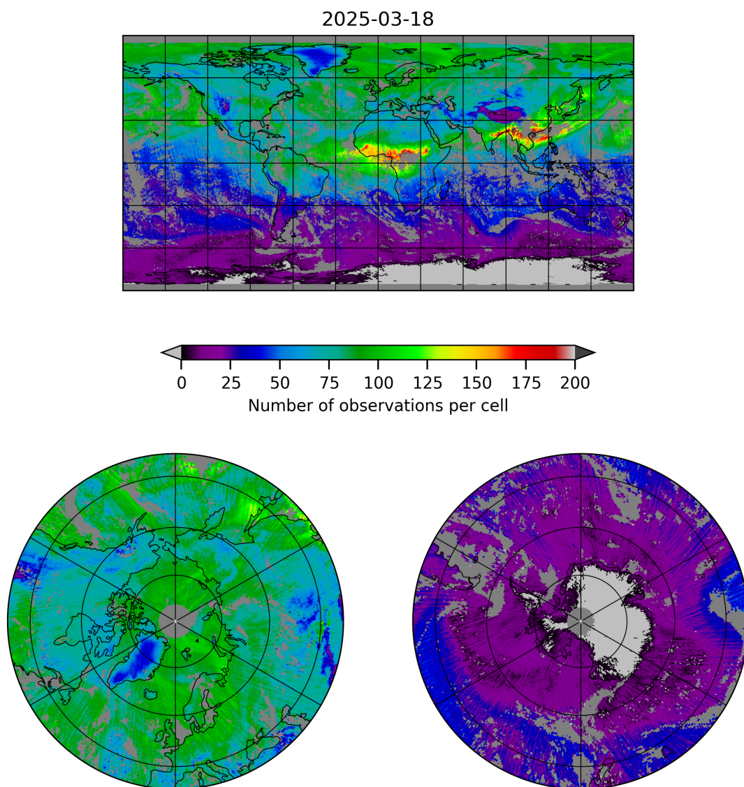
Figure 5: Map of the number of observations for 2025-03-18 to 2025-03-19
