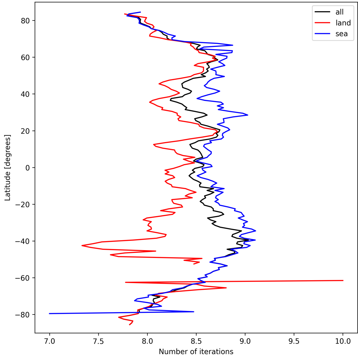
Figure 12: Zonal average of “Number of iterations” for 2025-03-18 to 2025-03-19.
