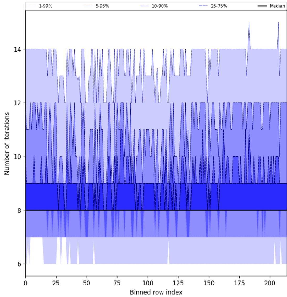
Figure 26: Along track statistics of “Number of iterations” for 2025-03-18 to 2025-03-19
