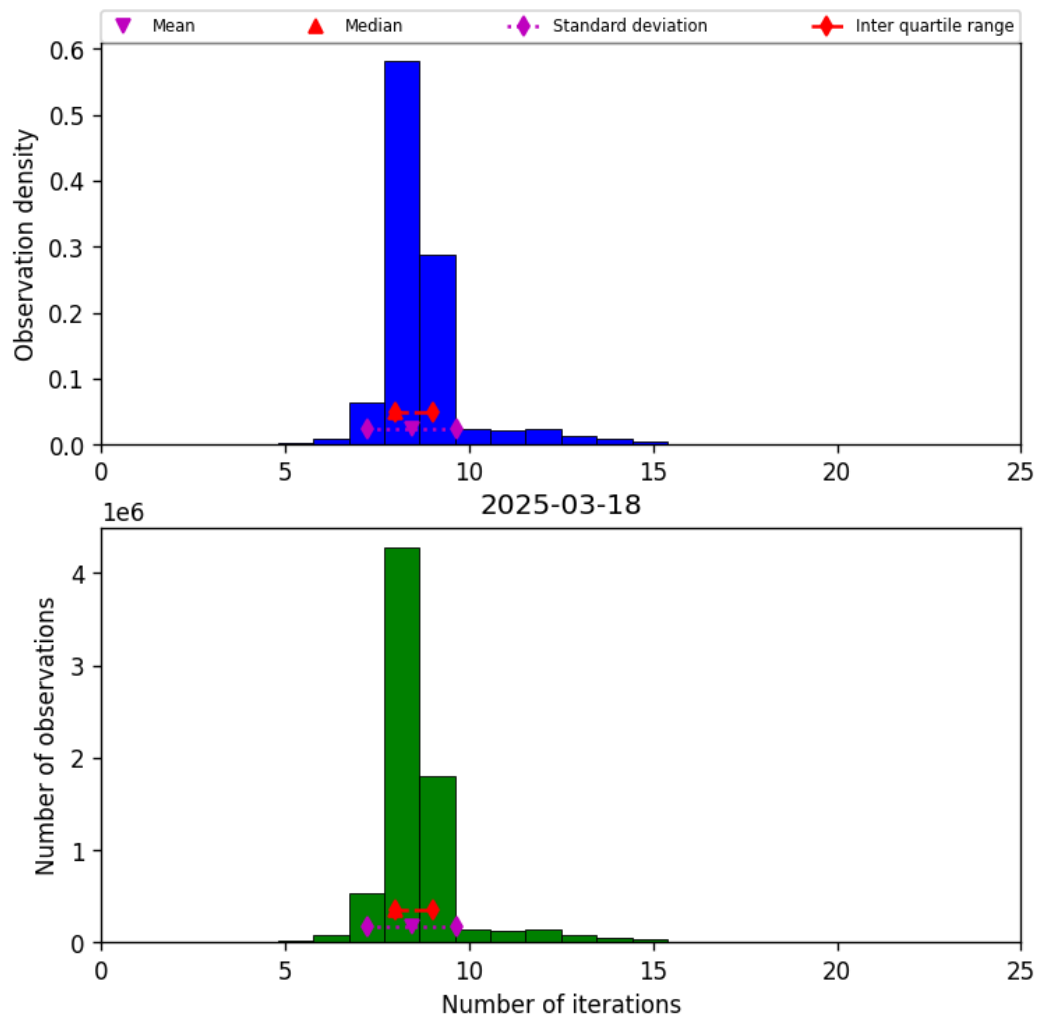
Figure 19: Histogram of “Number of iterations” for 2025-03-18 to 2025-03-19
