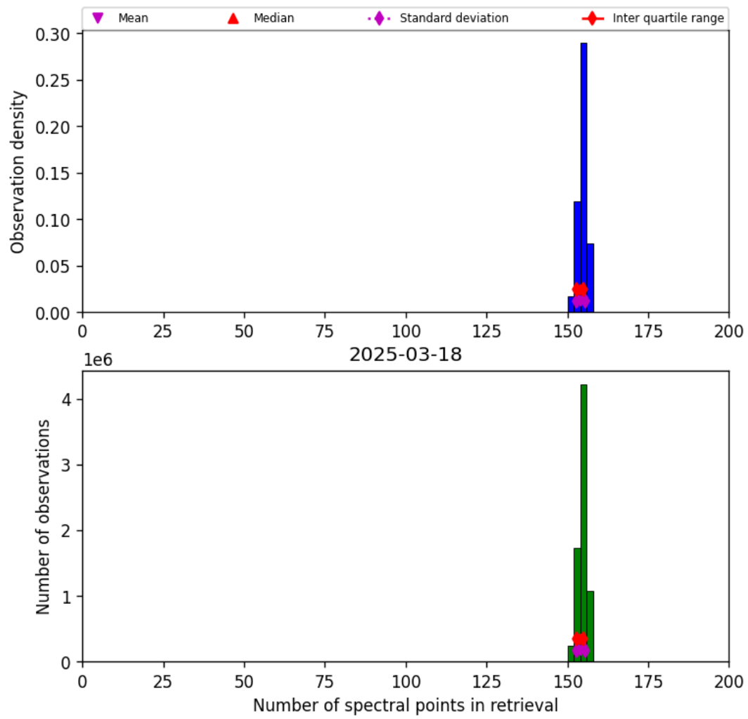
Figure 16: Histogram of “Number of spectral points in retrieval” for 2025-03-18 to 2025-03-19
