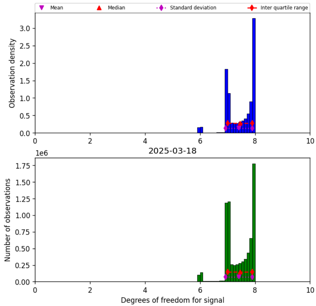
Figure 18: Histogram of “Degrees of freedom for signal” for 2025-03-18 to 2025-03-19
