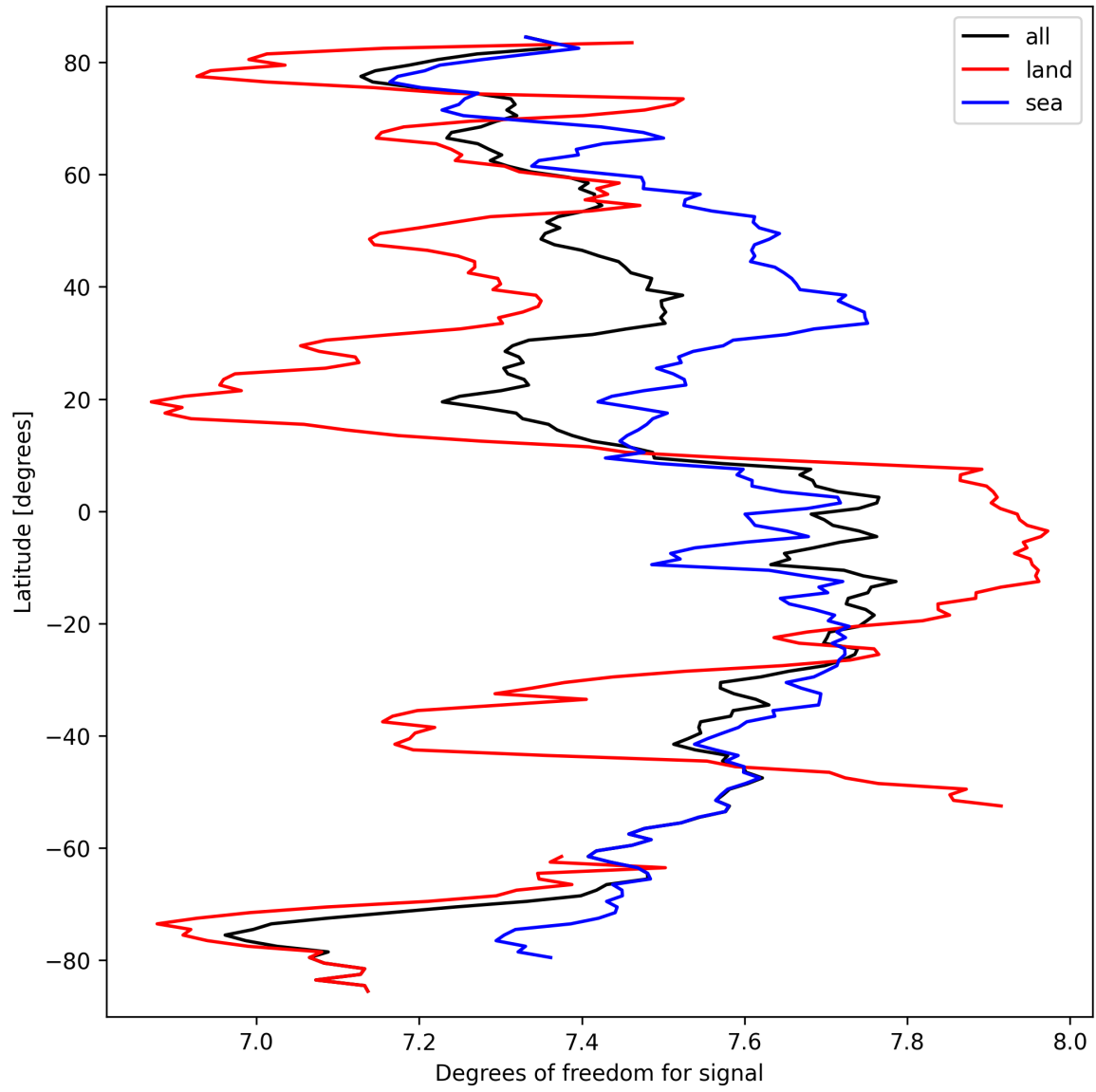
Figure 11: Zonal average of “Degrees of freedom for signal” for 2025-03-18 to 2025-03-19.
