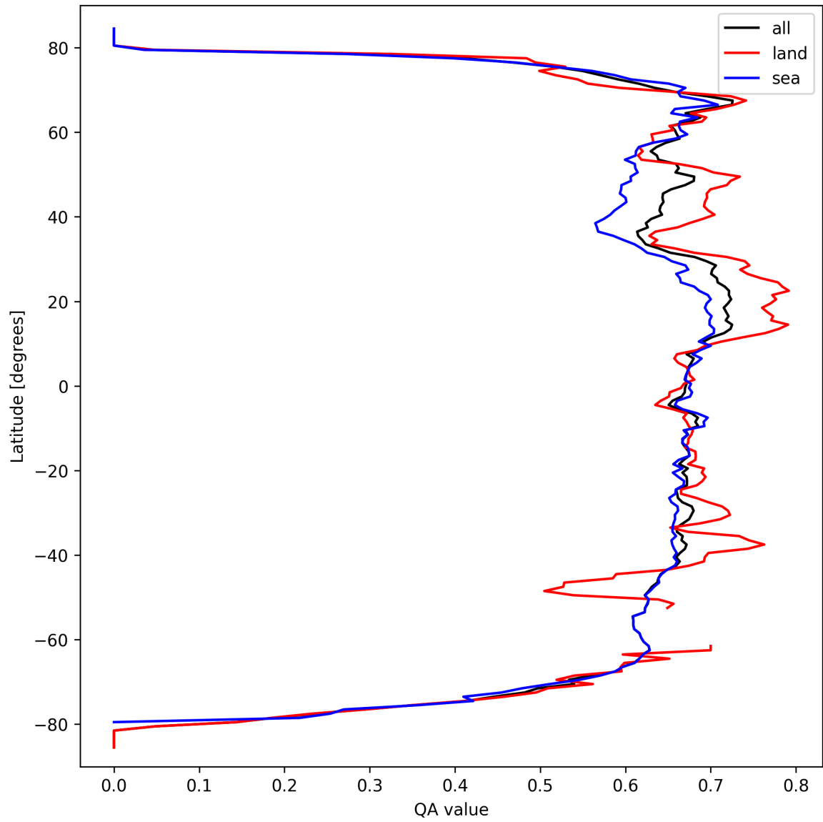
Figure 6: Zonal average of “QA value” for 2025-03-18 to 2025-03-19.
