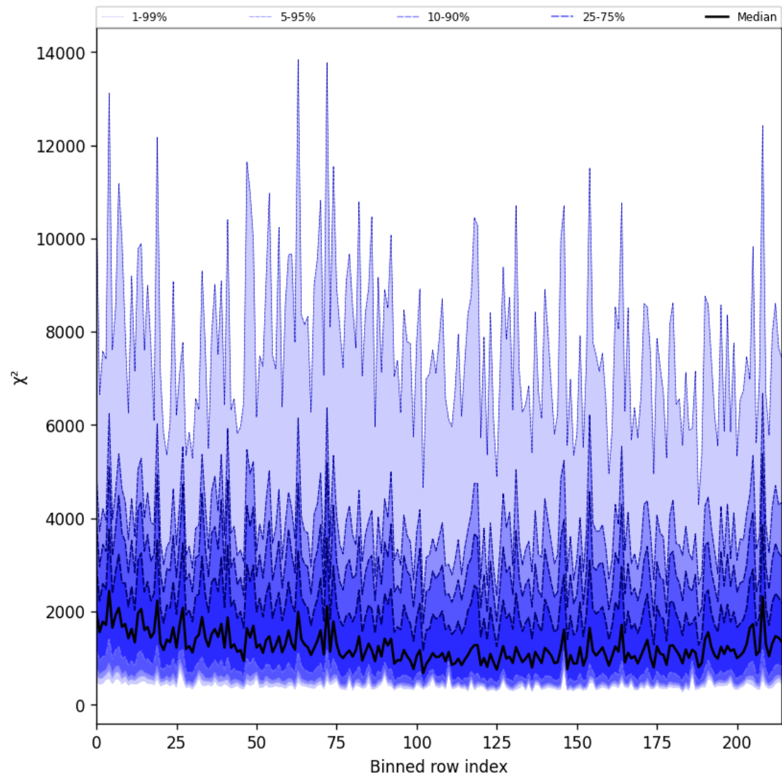
Figure 24: Along track statistics of “ \chi^2 ” for 2025-03-18 to 2025-03-19
