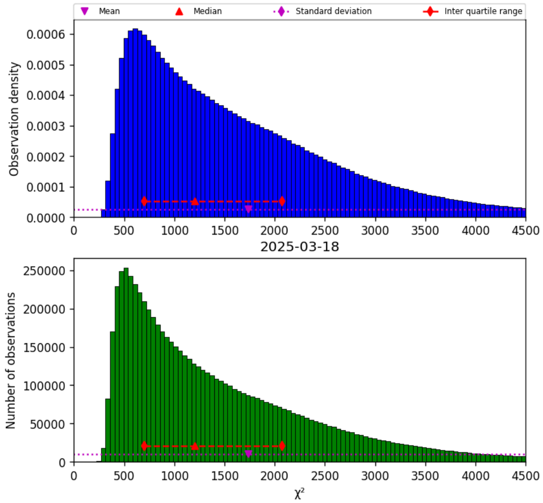
Figure 17: Histogram of “ \chi^2 ” for 2025-03-18 to 2025-03-19
