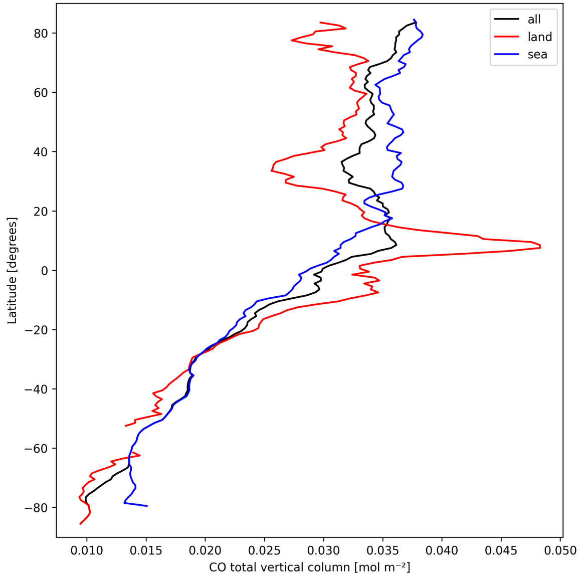
Figure 7: Zonal average of “CO total vertical column” for 2025-03-18 to 2025-03-19.
