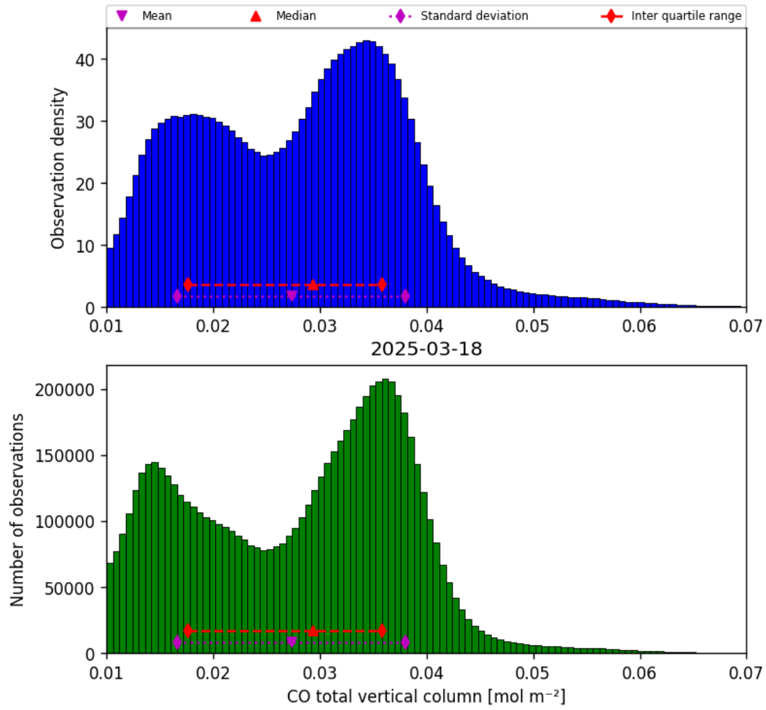
Figure 14: Histogram of “CO total vertical column” for 2025-03-18 to 2025-03-19
