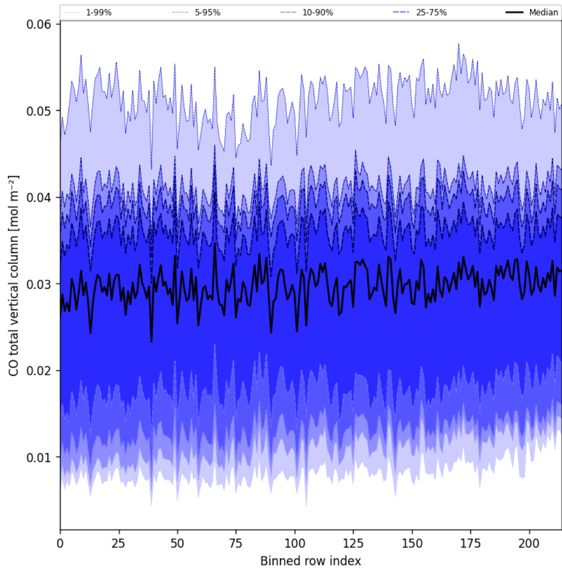
Figure 21: Along track statistics of “CO total vertical column” for 2025-03-18 to 2025-03-19
