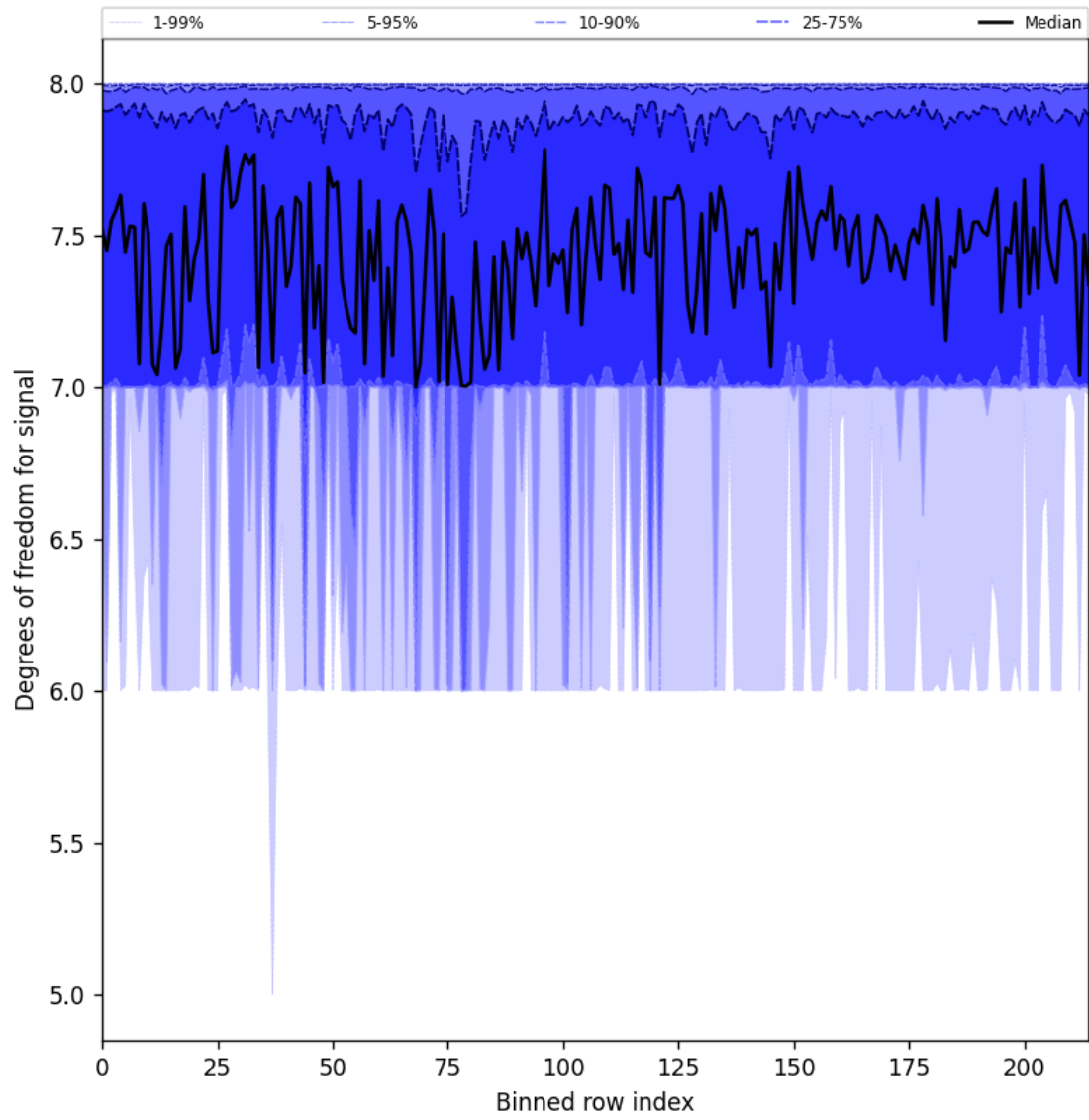
Figure 25: Along track statistics of “Degrees of freedom for signal” for 2025-03-18 to 2025-03-19
