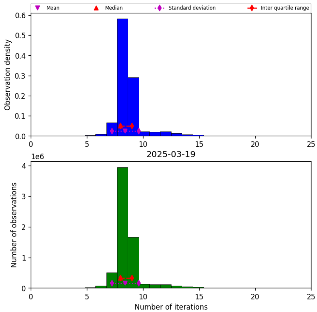
Figure 19: Histogram of “Number of iterations” for 2025-03-19 to 2025-03-20
