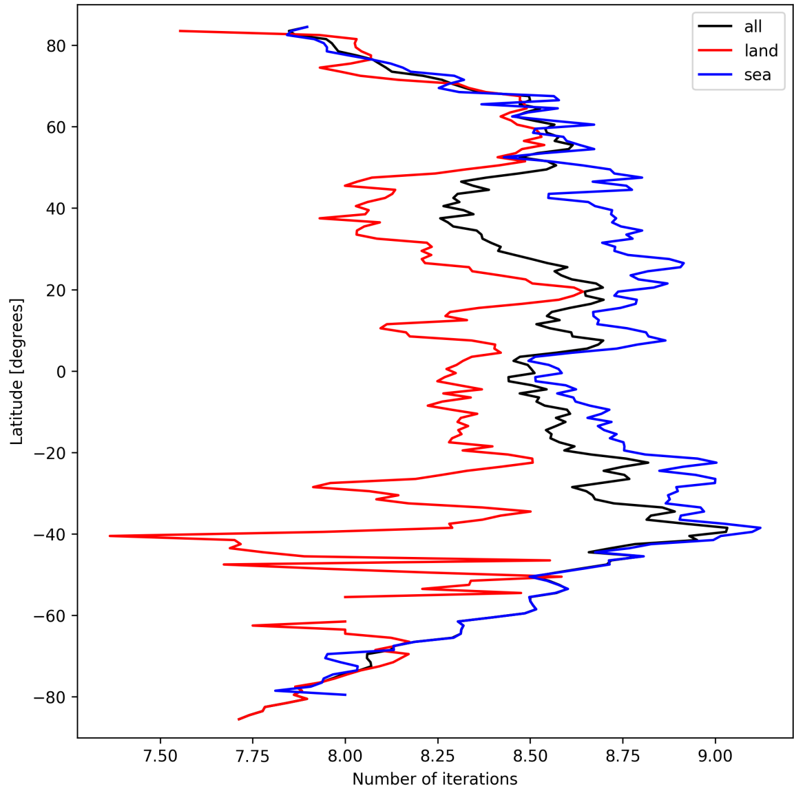
Figure 12: Zonal average of “Number of iterations” for 2025-03-19 to 2025-03-20.
