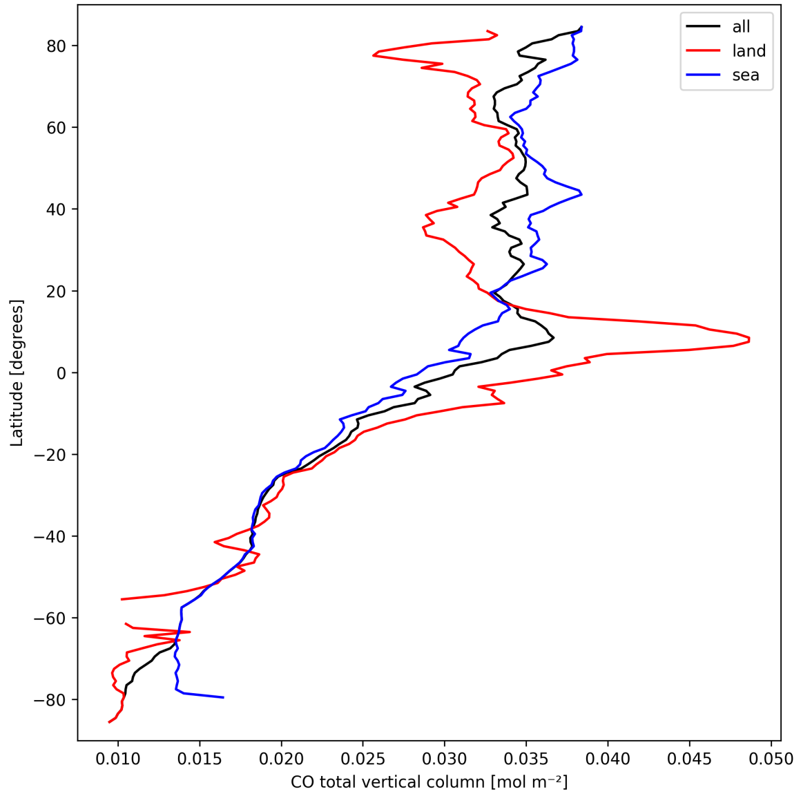
Figure 7: Zonal average of “CO total vertical column” for 2025-03-19 to 2025-03-20.
