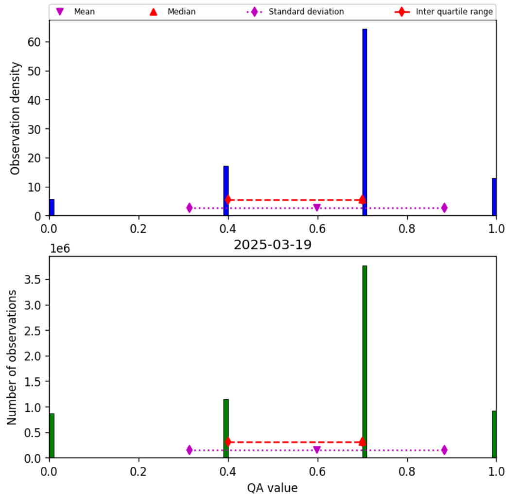
Figure 13: Histogram of “QA value” for 2025-03-19 to 2025-03-20
