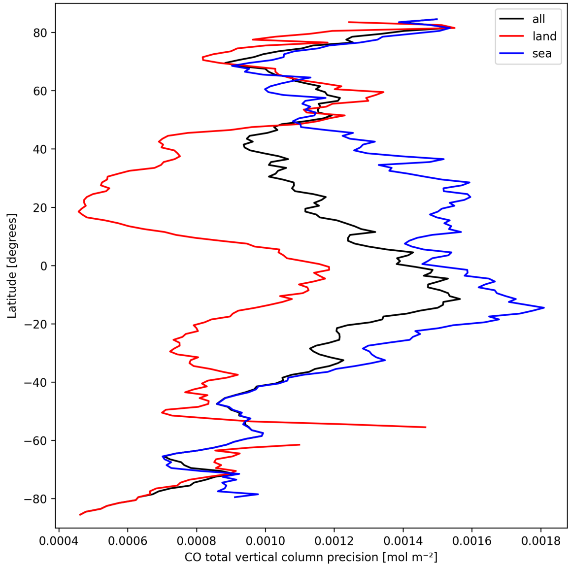
Figure 8: Zonal average of “CO total vertical column precision” for 2025-03-19 to 2025-03-20.
