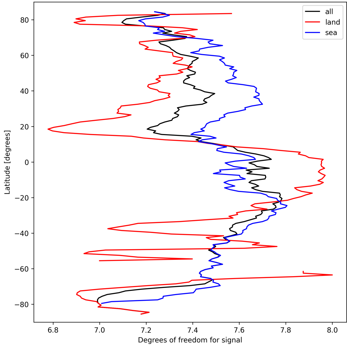
Figure 11: Zonal average of “Degrees of freedom for signal” for 2025-03-19 to 2025-03-20.
