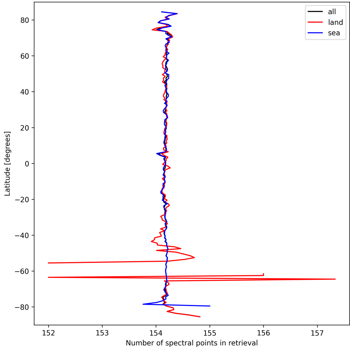
Figure 9: Zonal average of “Number of spectral points in retrieval” for 2025-03-19 to 2025-03-20.
