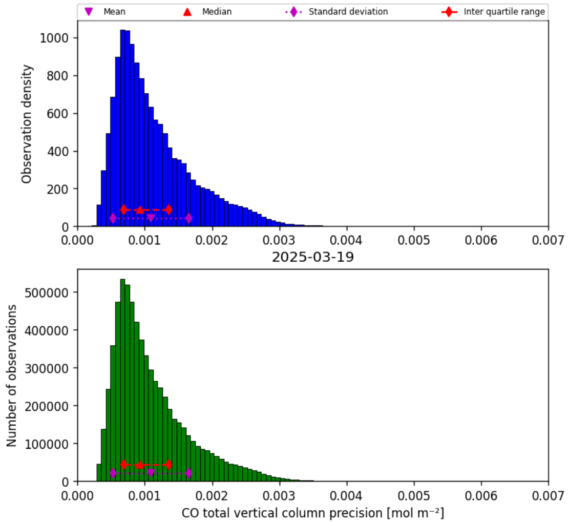
Figure 15: Histogram of “CO total vertical column precision” for 2025-03-19 to 2025-03-20
