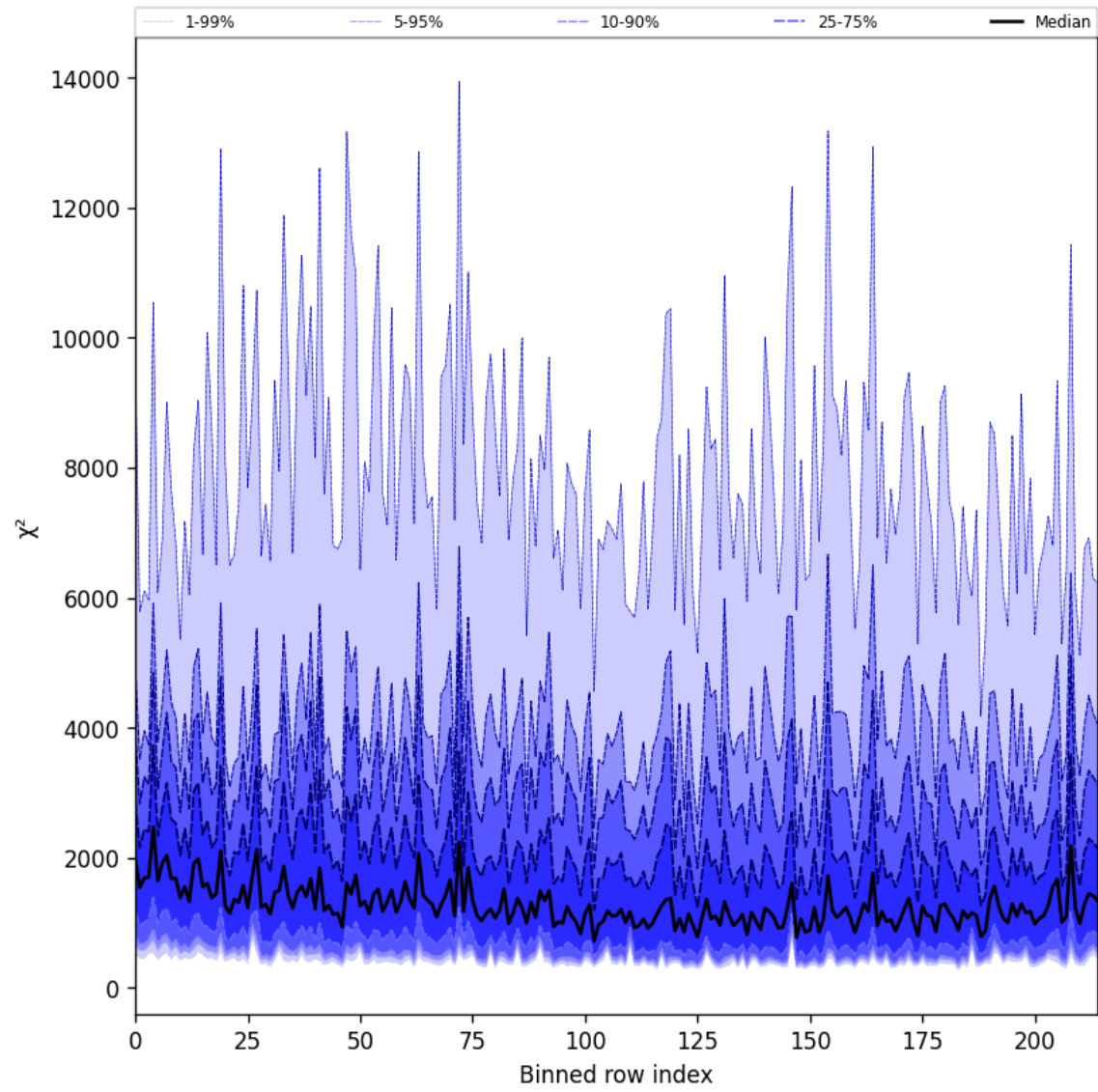
Figure 24: Along track statistics of “ \chi^2 ” for 2025-03-19 to 2025-03-20
