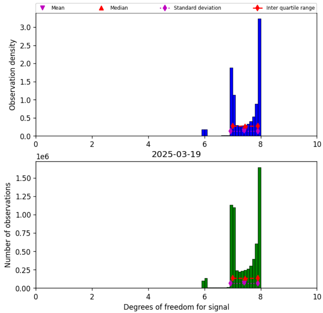
Figure 18: Histogram of “Degrees of freedom for signal” for 2025-03-19 to 2025-03-20
