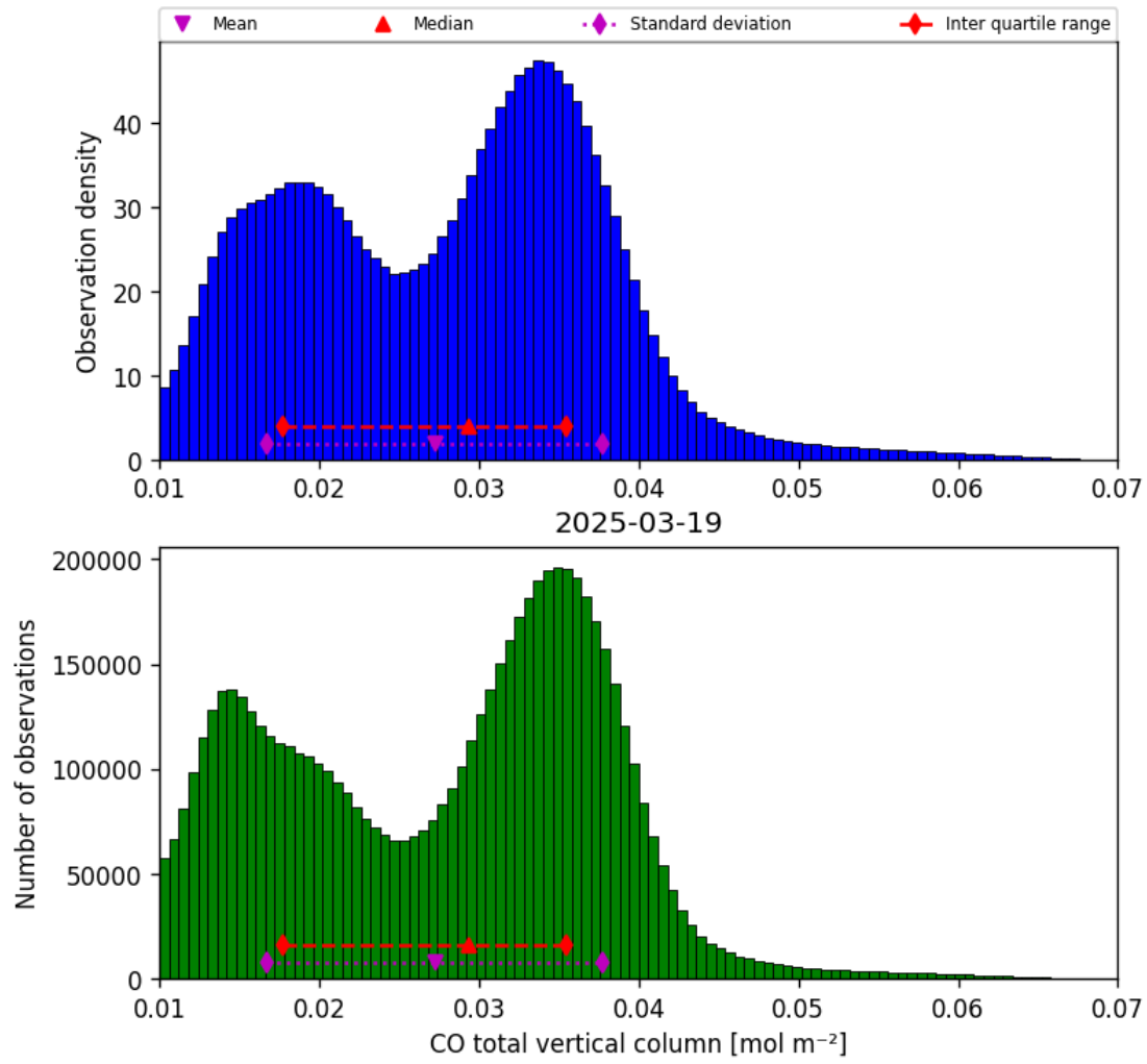
Figure 14: Histogram of “CO total vertical column” for 2025-03-19 to 2025-03-20
