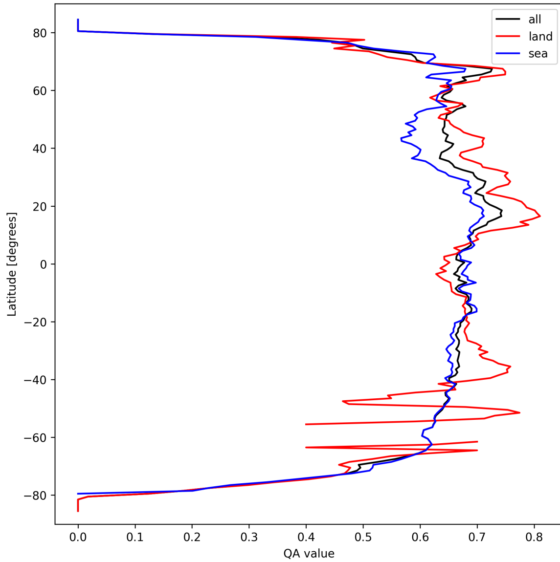
Figure 6: Zonal average of “QA value” for 2025-03-19 to 2025-03-20.
