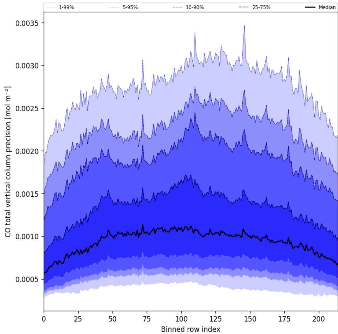
Figure 22: Along track statistics of “CO total vertical column precision” for 2025-03-19 to 2025-03-20
