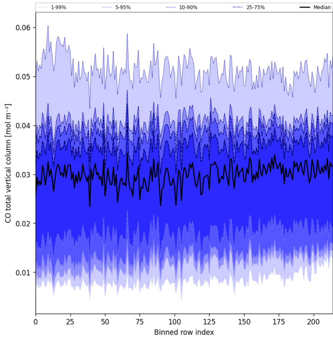
Figure 21: Along track statistics of “CO total vertical column” for 2025-03-19 to 2025-03-20
