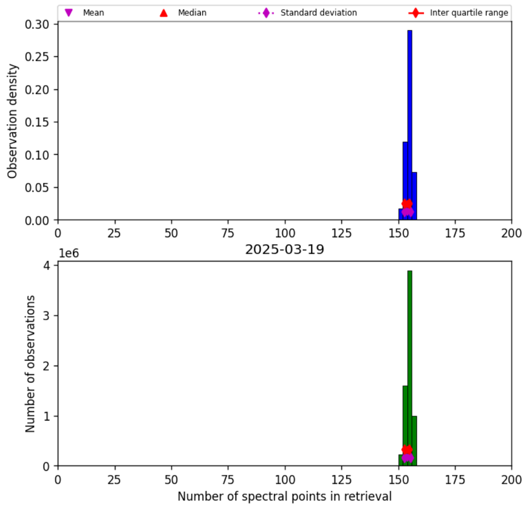
Figure 16: Histogram of “Number of spectral points in retrieval” for 2025-03-19 to 2025-03-20
