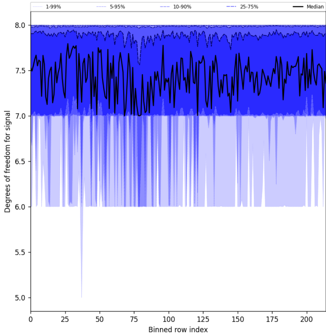
Figure 25: Along track statistics of “Degrees of freedom for signal” for 2025-03-19 to 2025-03-20
