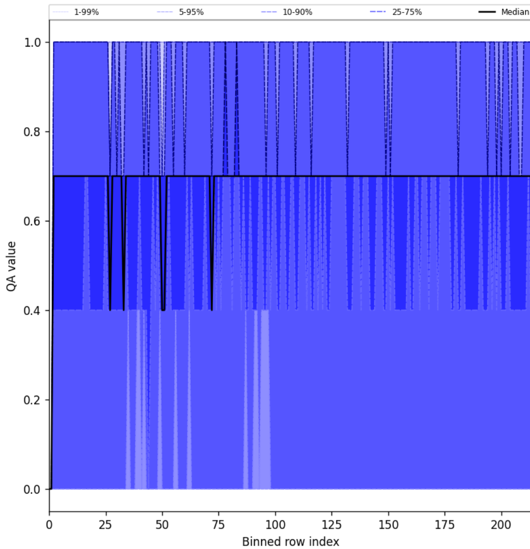
Figure 20: Along track statistics of “QA value” for 2025-03-19 to 2025-03-20
