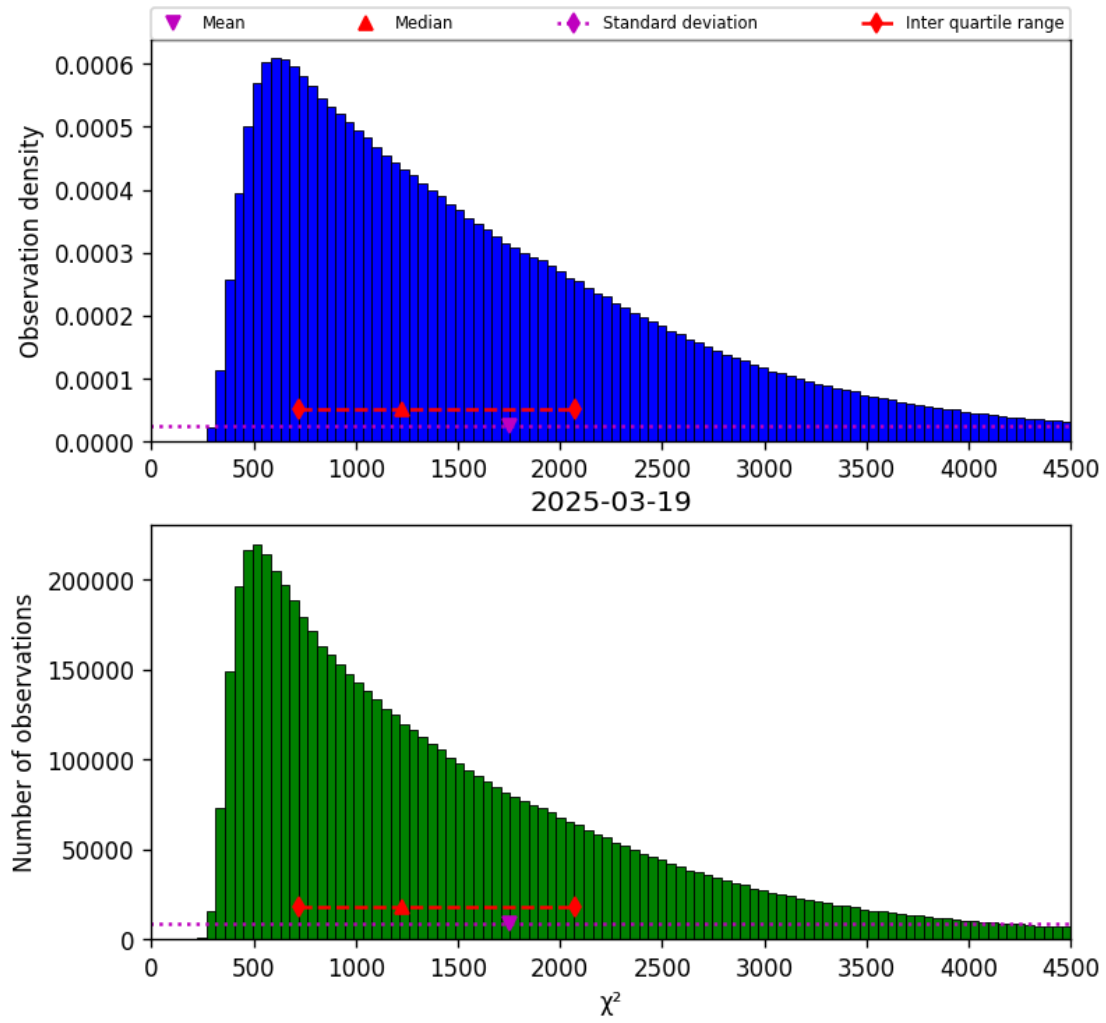
Figure 17: Histogram of “ \chi^2 ” for 2025-03-19 to 2025-03-20
