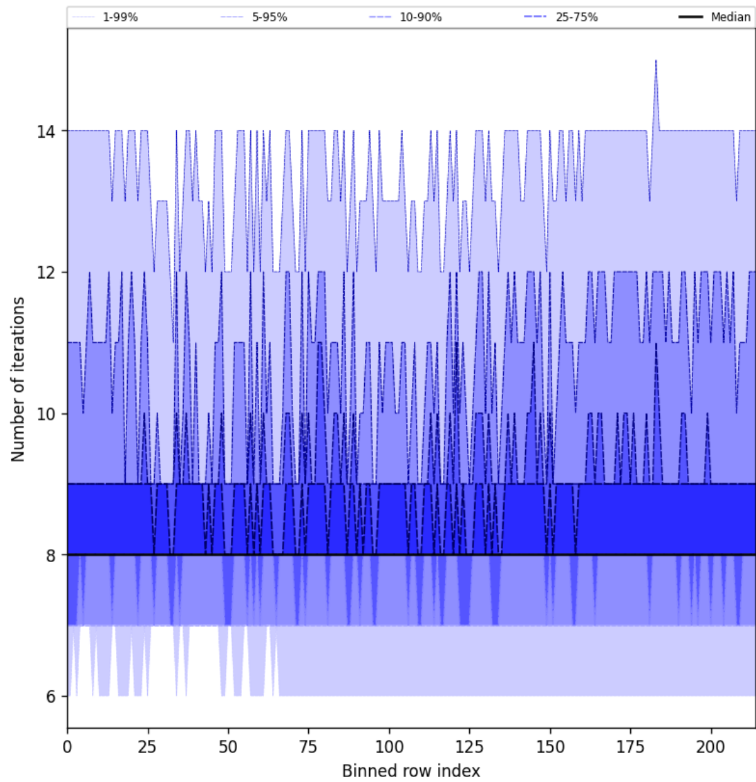
Figure 26: Along track statistics of “Number of iterations” for 2025-03-19 to 2025-03-20
