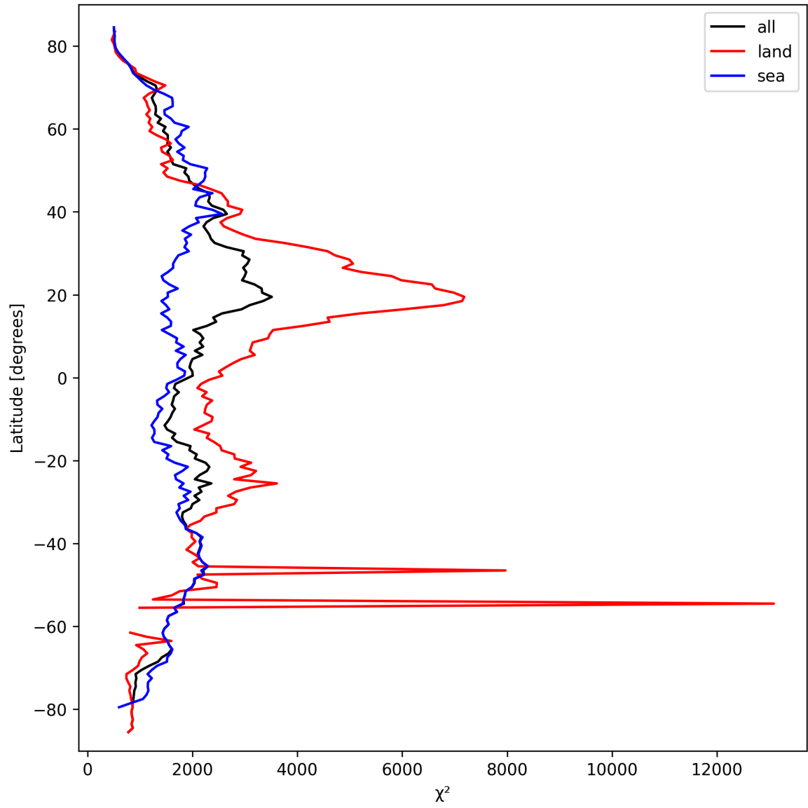
Figure 10: Zonal average of “ \chi^2 ” for 2025-03-19 to 2025-03-20.
