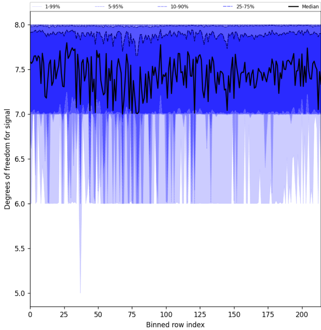
Figure 25: Along track statistics of “Degrees of freedom for signal” for 2025-03-20 to 2025-03-21
