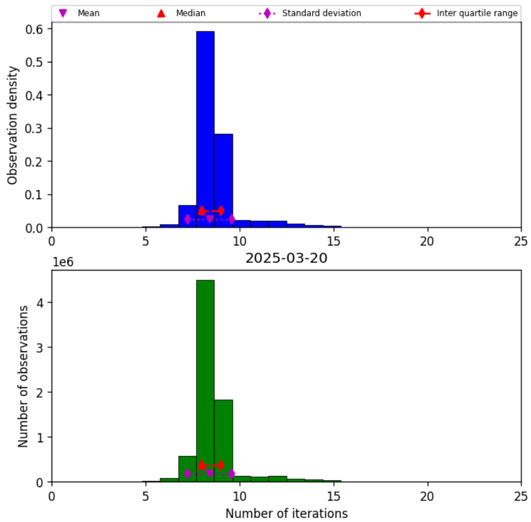
Figure 19: Histogram of “Number of iterations” for 2025-03-20 to 2025-03-21
