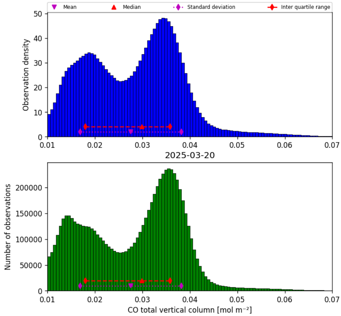
Figure 14: Histogram of “CO total vertical column” for 2025-03-20 to 2025-03-21
