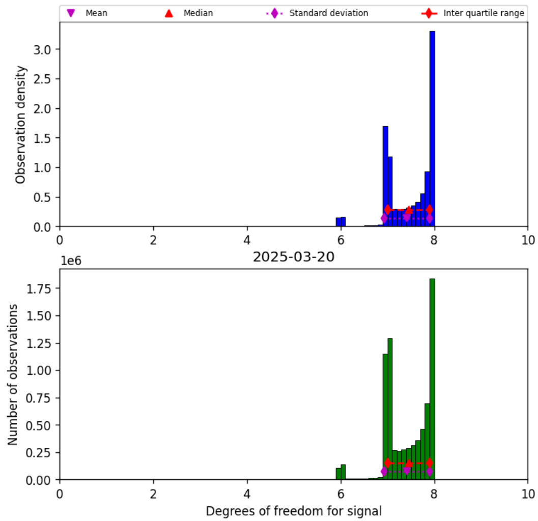
Figure 18: Histogram of “Degrees of freedom for signal” for 2025-03-20 to 2025-03-21
