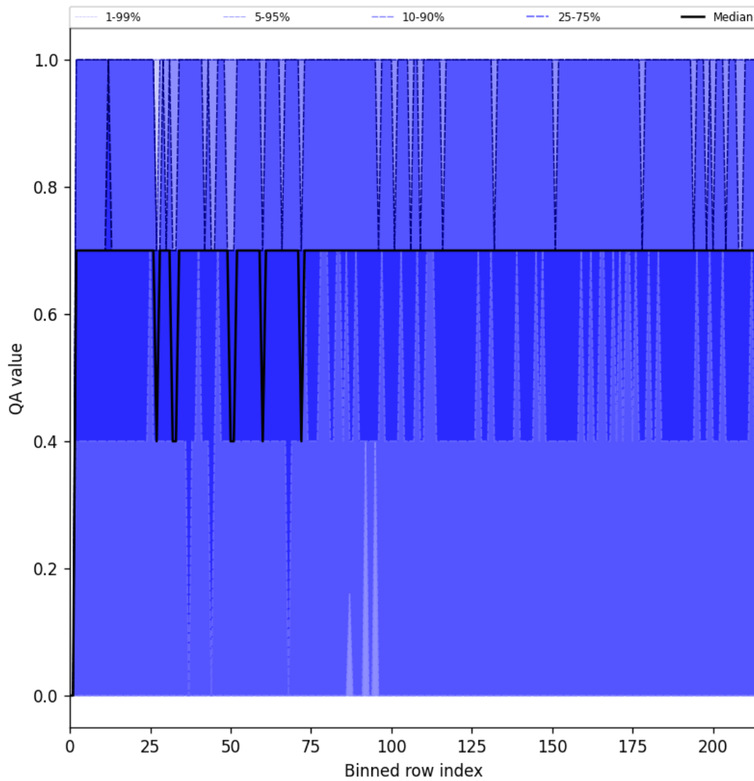
Figure 20: Along track statistics of “QA value” for 2025-03-20 to 2025-03-21
