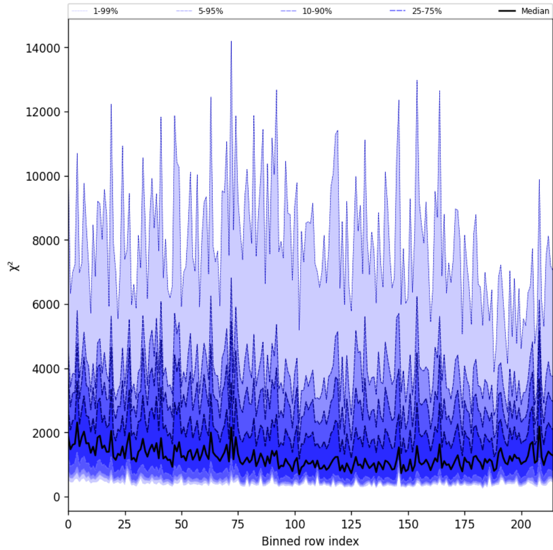
Figure 24: Along track statistics of “ \chi^2 ” for 2025-03-20 to 2025-03-21
