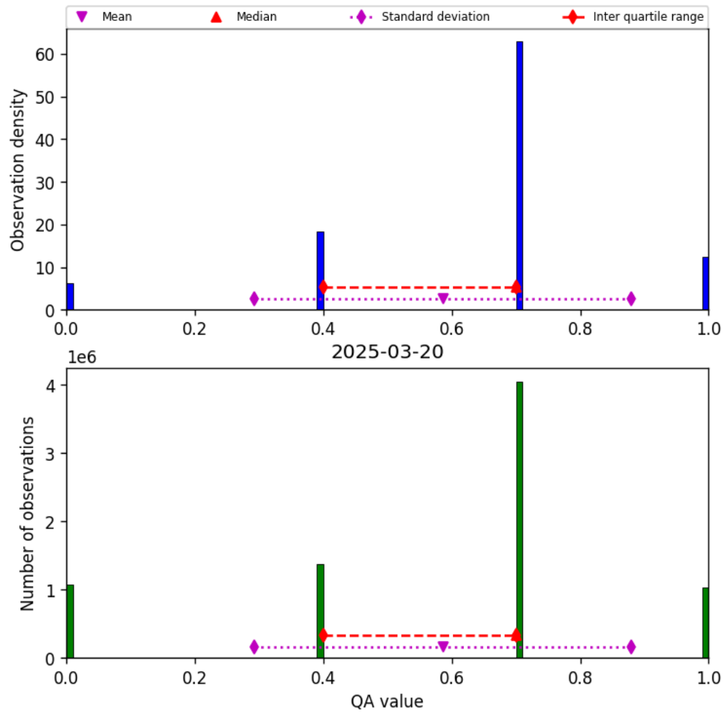
Figure 13: Histogram of “QA value” for 2025-03-20 to 2025-03-21
