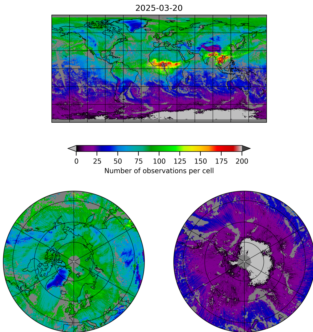
Figure 5: Map of the number of observations for 2025-03-20 to 2025-03-21
