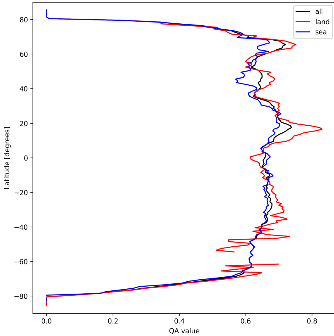
Figure 6: Zonal average of “QA value” for 2025-03-20 to 2025-03-21.
