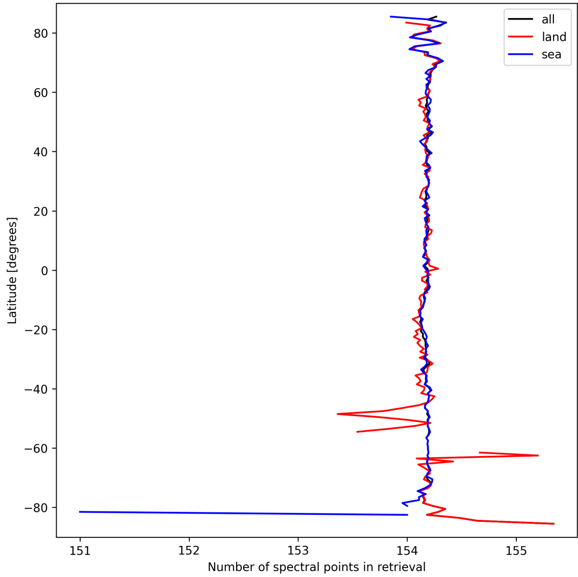
Figure 9: Zonal average of “Number of spectral points in retrieval” for 2025-03-20 to 2025-03-21.
