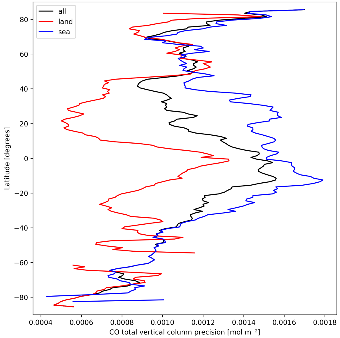
Figure 8: Zonal average of "CO total vertical column precision" for 2025-03-20 to 2025-03-21.
