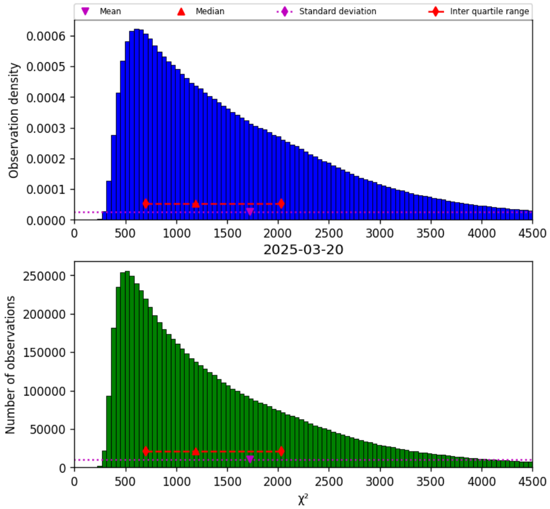
Figure 17: Histogram of “ \chi^2 ” for 2025-03-20 to 2025-03-21
