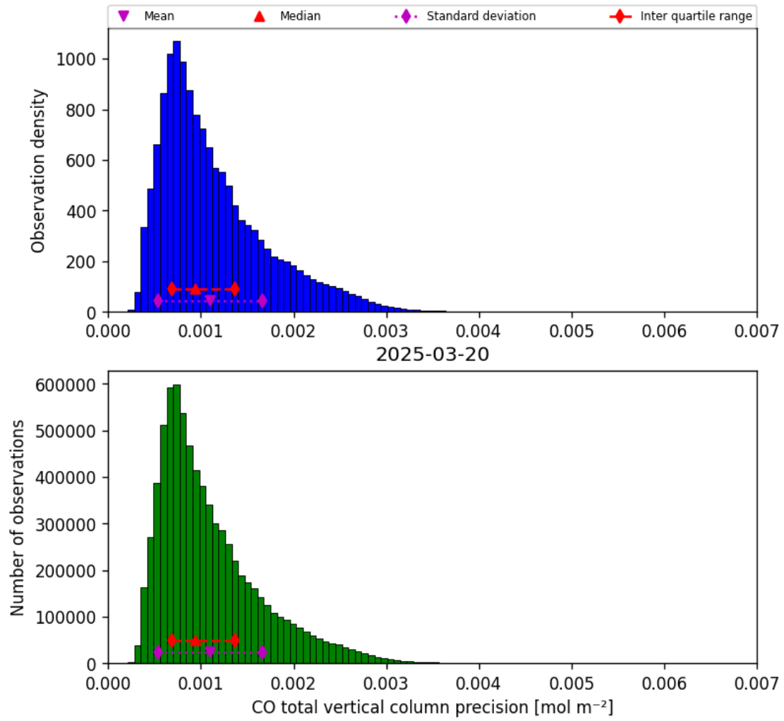
Figure 15: Histogram of “CO total vertical column precision” for 2025-03-20 to 2025-03-21
