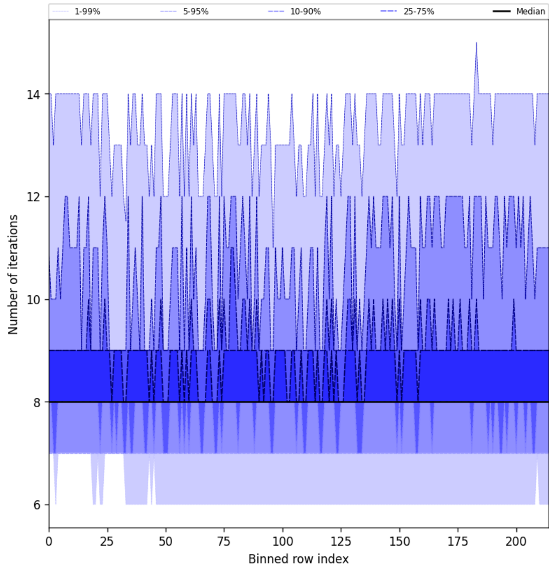
Figure 26: Along track statistics of “Number of iterations” for 2025-03-20 to 2025-03-21
