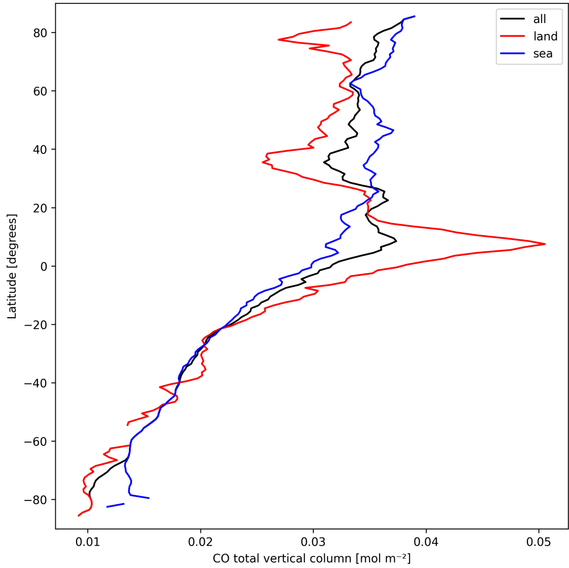
Figure 7: Zonal average of “CO total vertical column” for 2025-03-20 to 2025-03-21.
