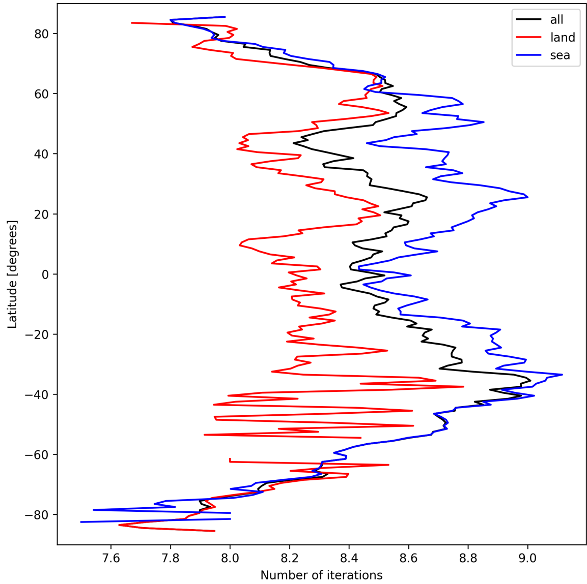
Figure 12: Zonal average of “Number of iterations” for 2025-03-20 to 2025-03-21.
