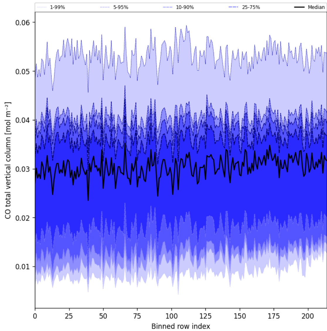
Figure 21: Along track statistics of “CO total vertical column” for 2025-03-20 to 2025-03-21
