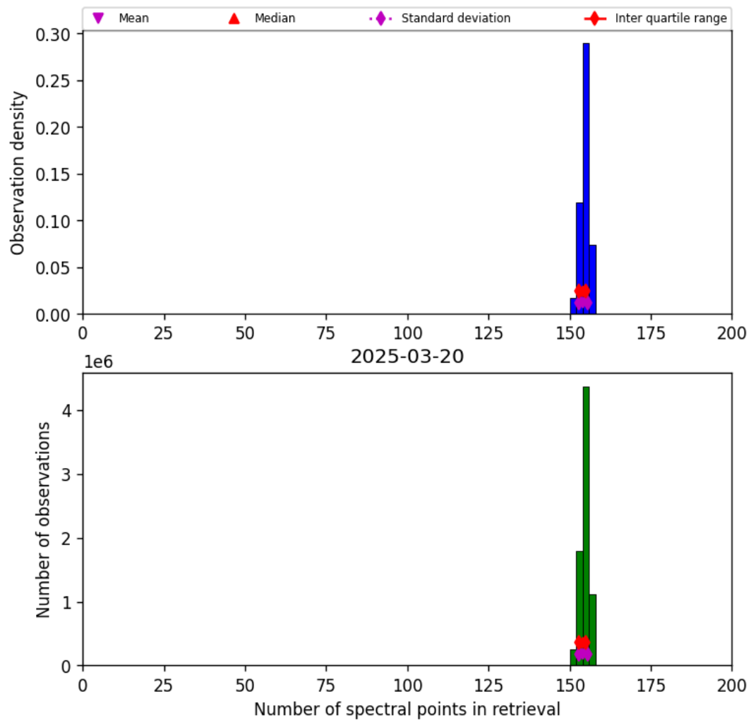
Figure 16: Histogram of “Number of spectral points in retrieval” for 2025-03-20 to 2025-03-21
