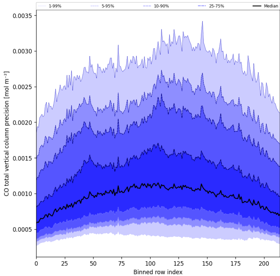
Figure 22: Along track statistics of “CO total vertical column precision” for 2025-03-20 to 2025-03-21
