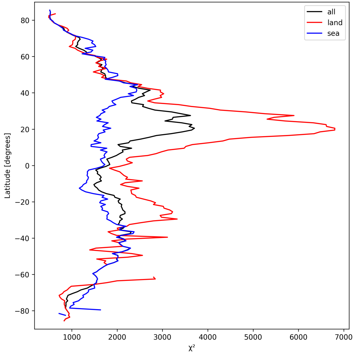
Figure 10: Zonal average of “ \chi^2 ” for 2025-03-20 to 2025-03-21.
