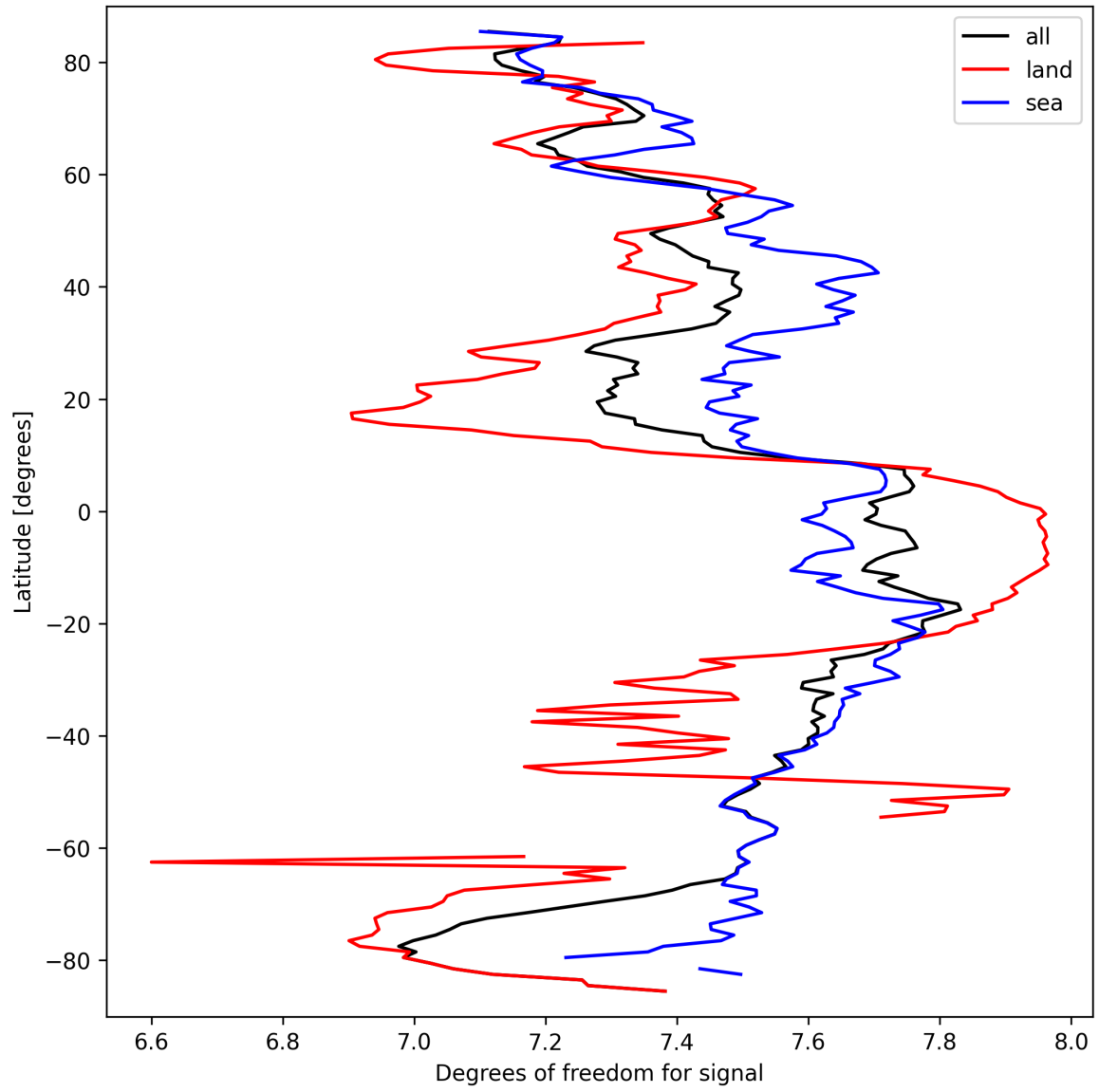
Figure 11: Zonal average of “Degrees of freedom for signal” for 2025-03-20 to 2025-03-21.
