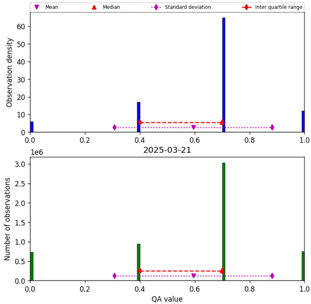
Figure 13: Histogram of “QA value” for 2025-03-21 to 2025-03-21
