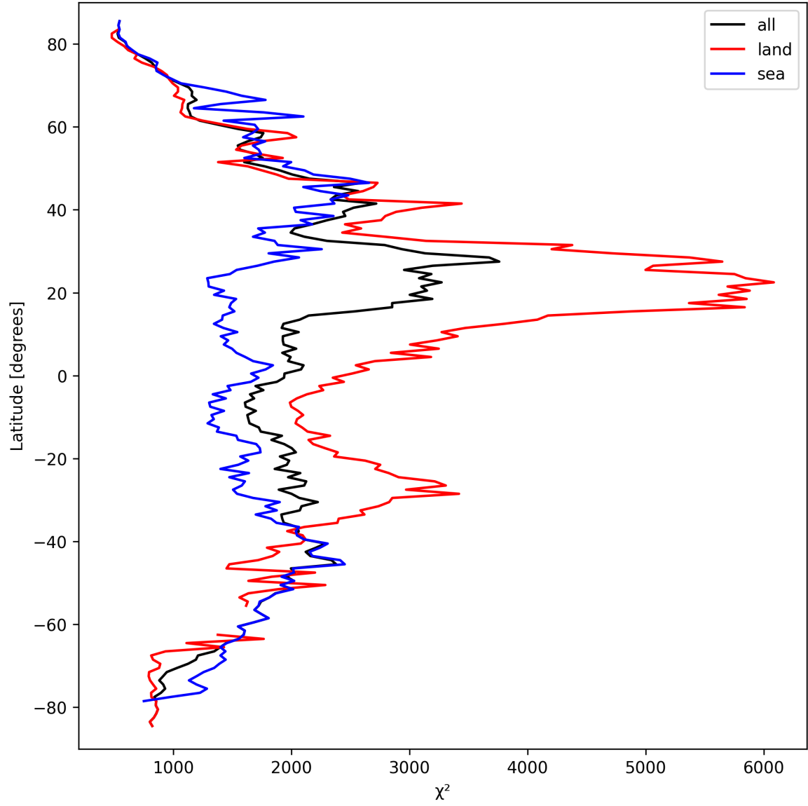
Figure 10: Zonal average of “ \chi^2 ” for 2025-03-21 to 2025-03-21.
