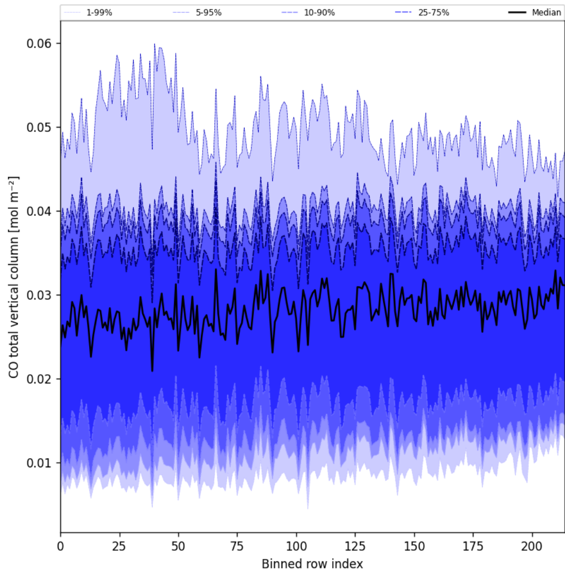
Figure 21: Along track statistics of “CO total vertical column” for 2025-03-21 to 2025-03-21
