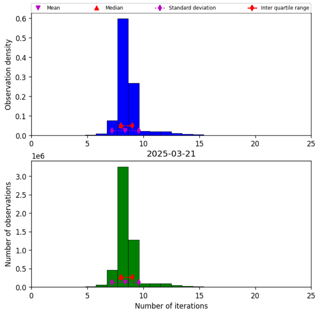
Figure 19: Histogram of “Number of iterations” for 2025-03-21 to 2025-03-21
