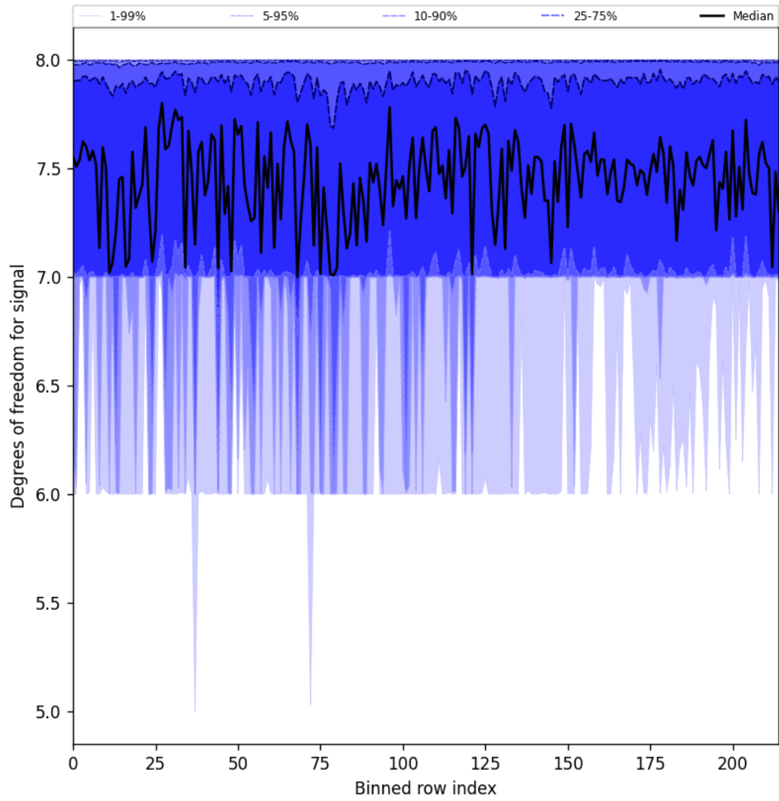
Figure 25: Along track statistics of “Degrees of freedom for signal” for 2025-03-21 to 2025-03-21
