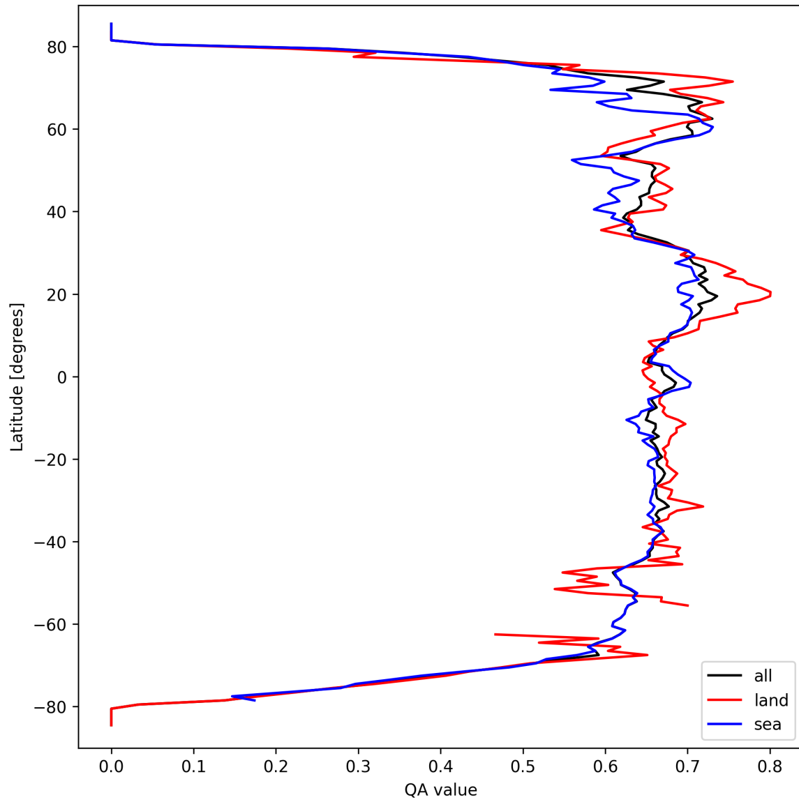
Figure 6: Zonal average of “QA value” for 2025-03-21 to 2025-03-21.
