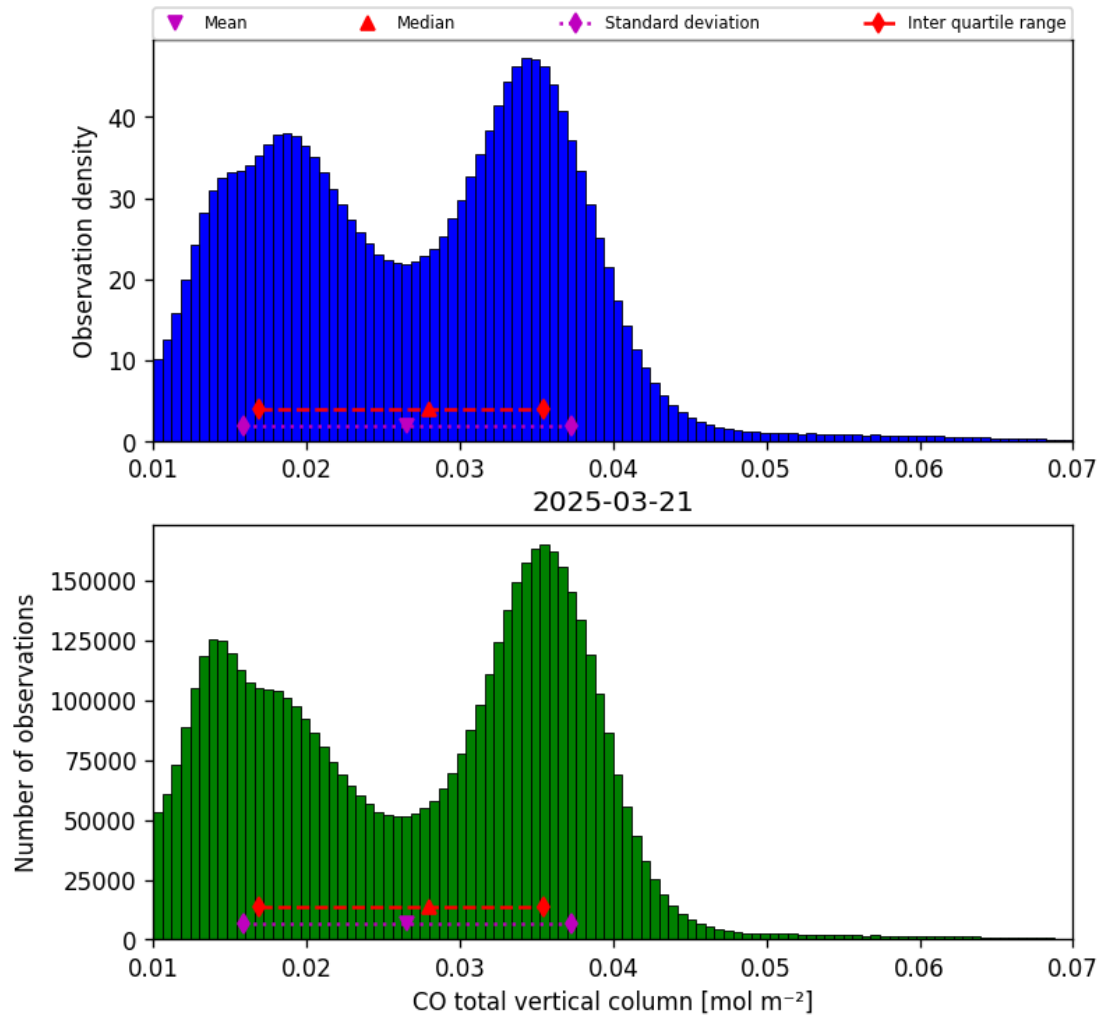
Figure 14: Histogram of “CO total vertical column” for 2025-03-21 to 2025-03-21
