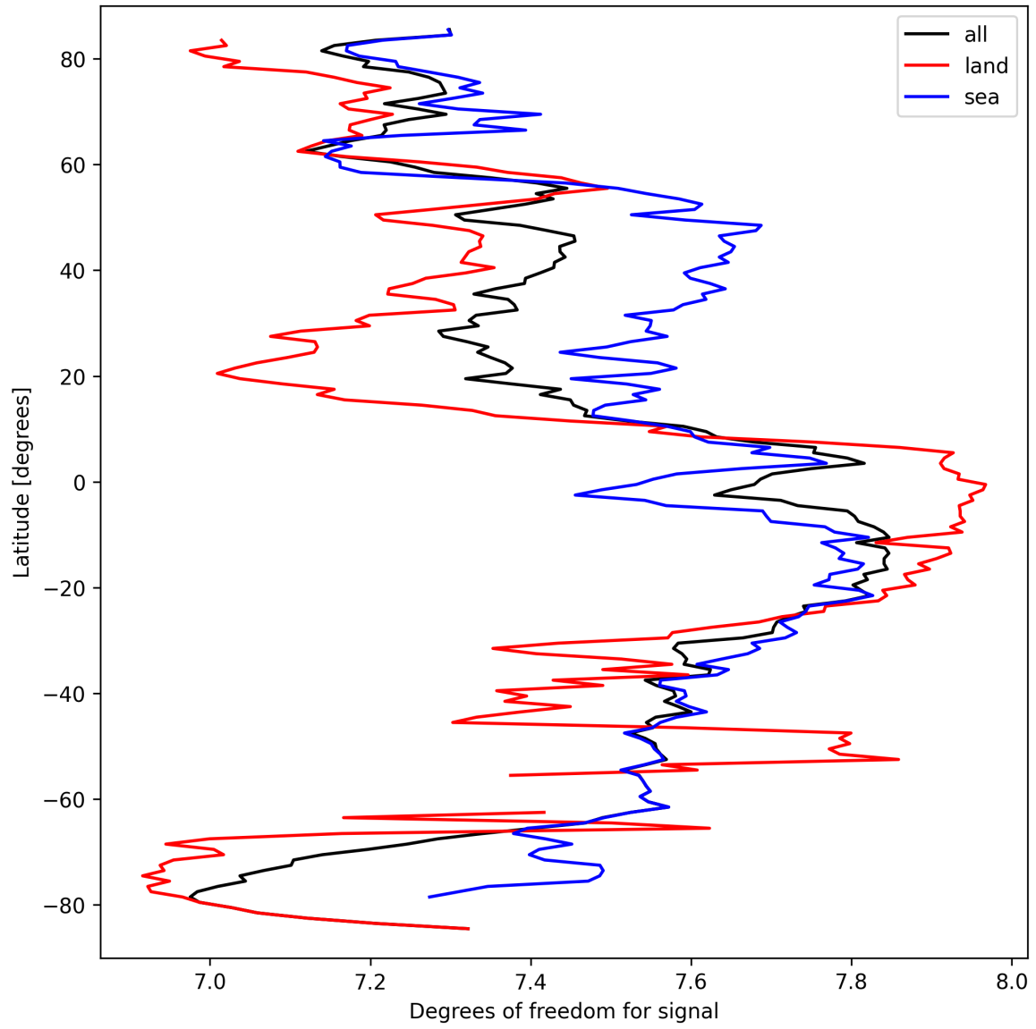
Figure 11: Zonal average of “Degrees of freedom for signal” for 2025-03-21 to 2025-03-21.
