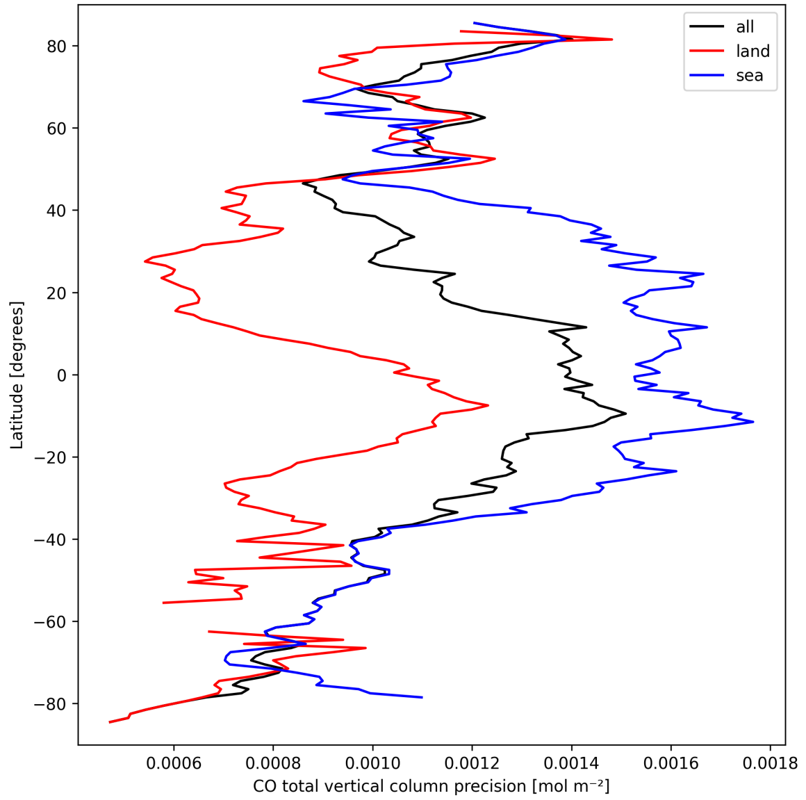
Figure 8: Zonal average of “CO total vertical column precision” for 2025-03-21 to 2025-03-21.
