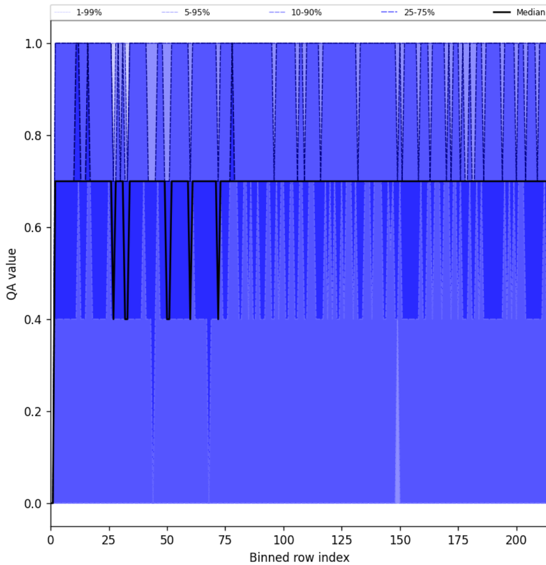
Figure 20: Along track statistics of “QA value” for 2025-03-21 to 2025-03-21
