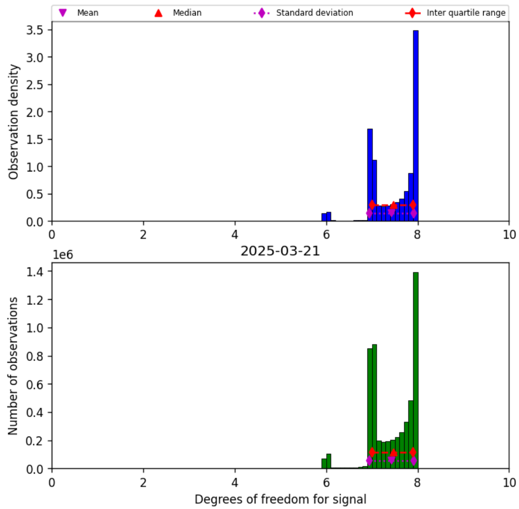
Figure 18: Histogram of “Degrees of freedom for signal” for 2025-03-21 to 2025-03-21
