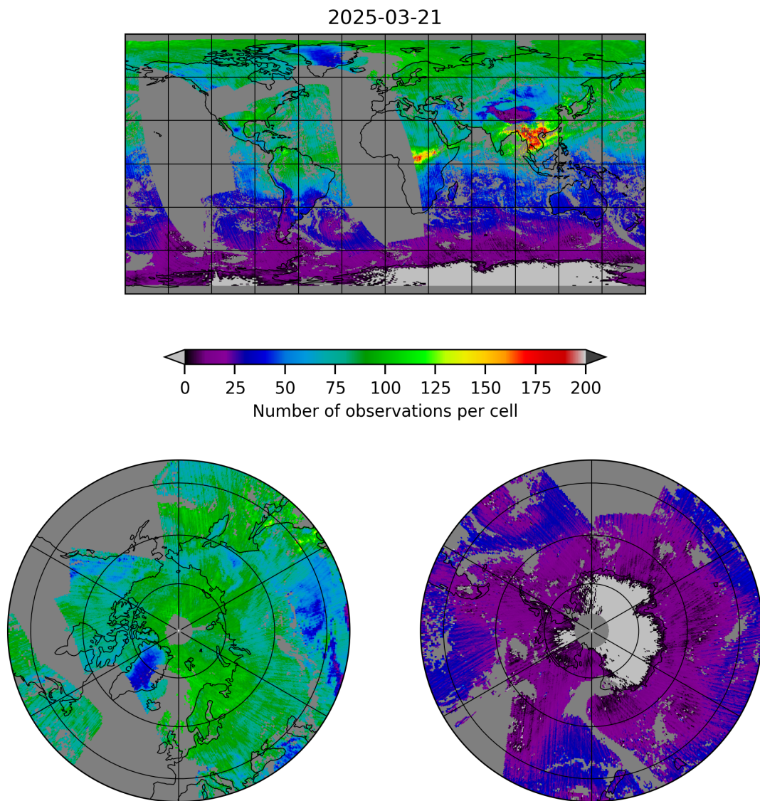
Figure 5: Map of the number of observations for 2025-03-21 to 2025-03-21
