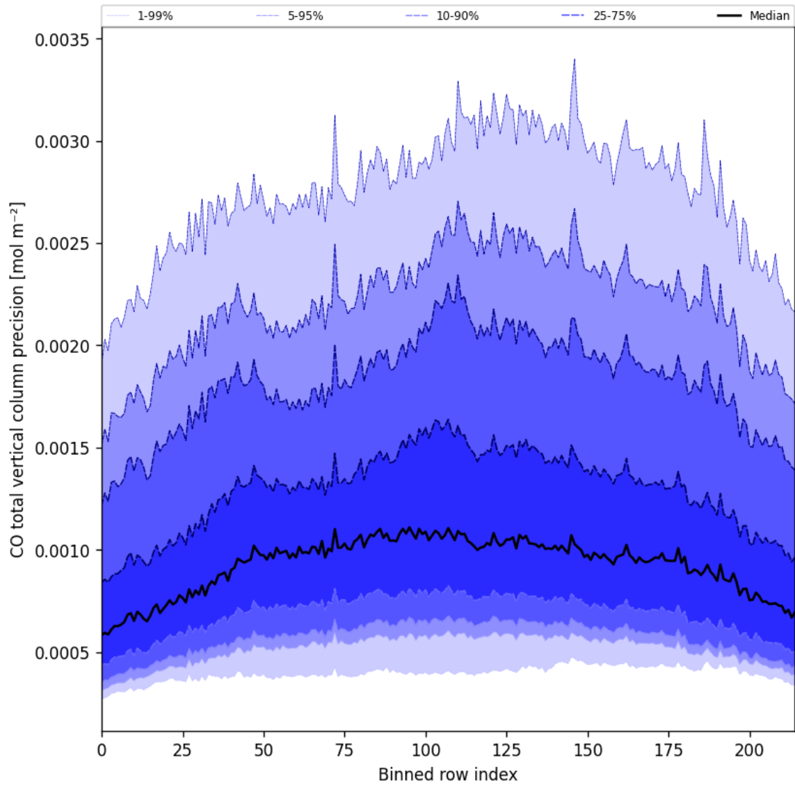
Figure 22: Along track statistics of “CO total vertical column precision” for 2025-03-21 to 2025-03-21
