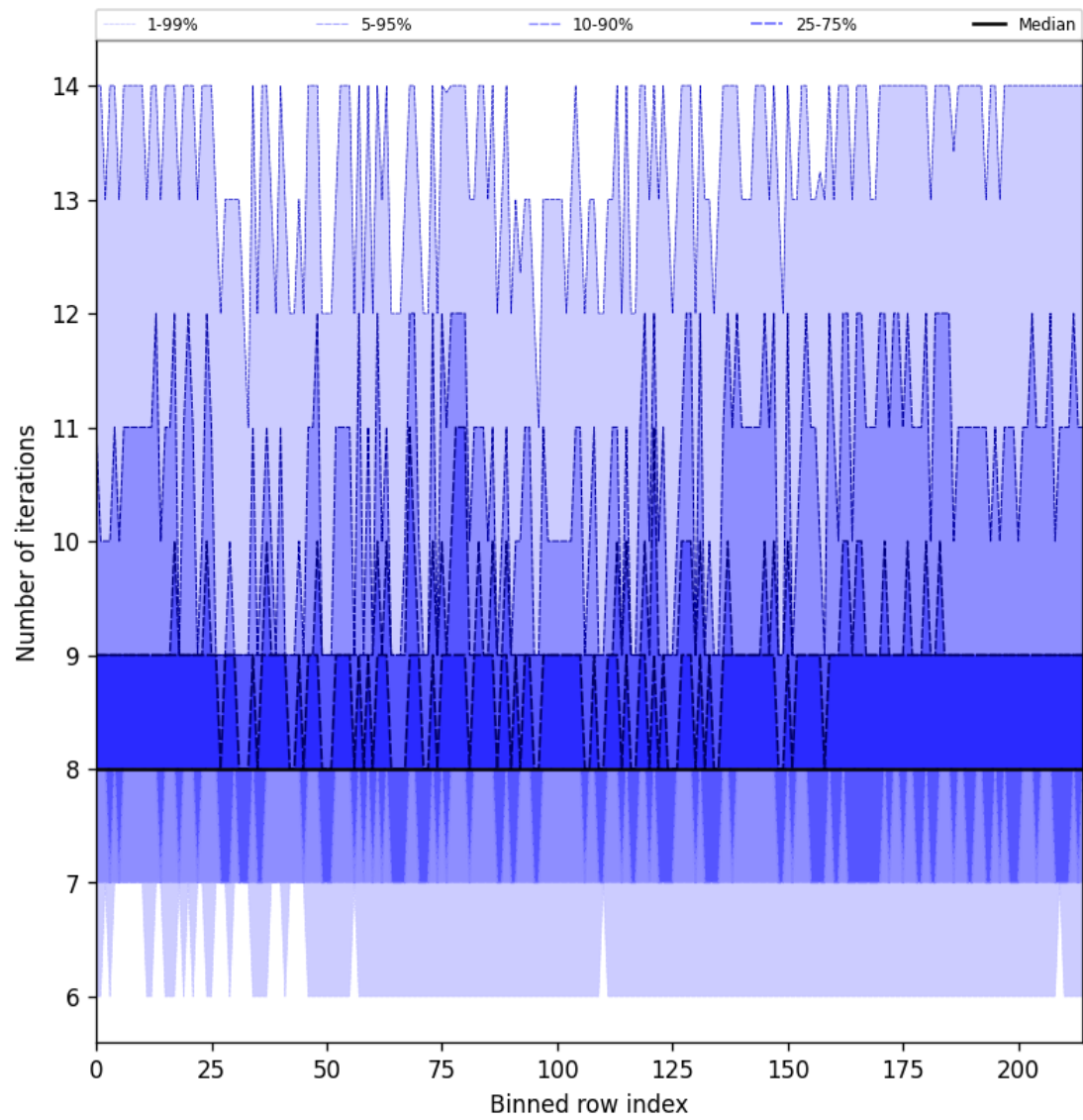
Figure 26: Along track statistics of “Number of iterations” for 2025-03-21 to 2025-03-21
