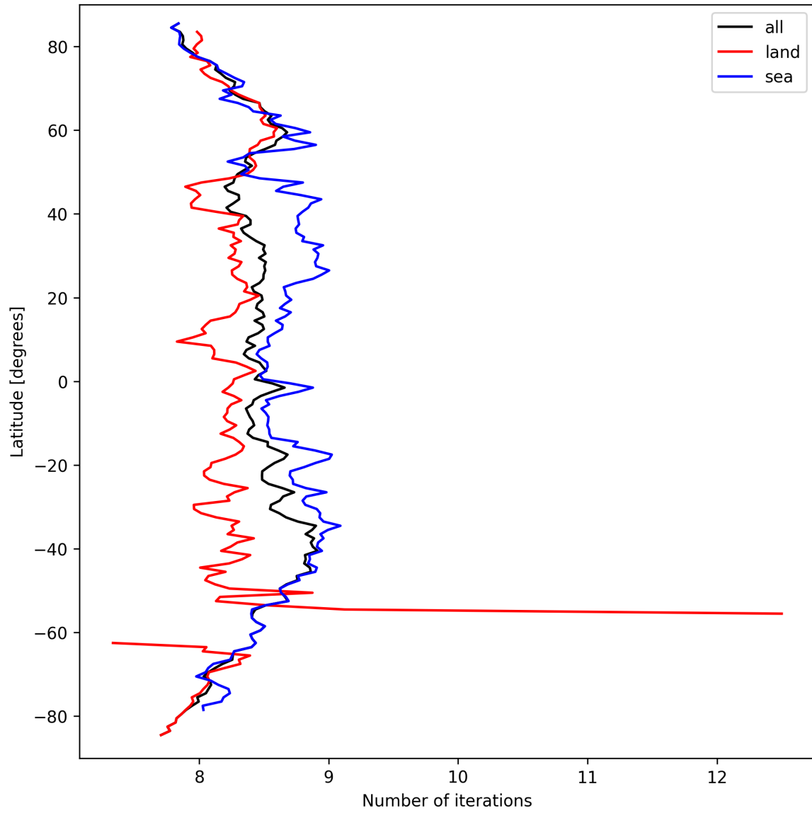
Figure 12: Zonal average of “Number of iterations” for 2025-03-21 to 2025-03-21.
