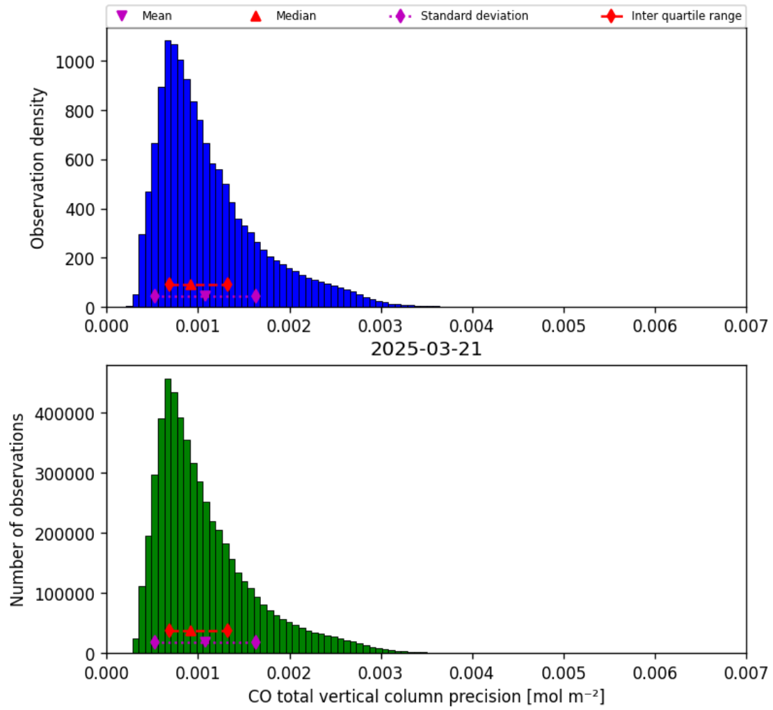
Figure 15: Histogram of “CO total vertical column precision” for 2025-03-21 to 2025-03-21
