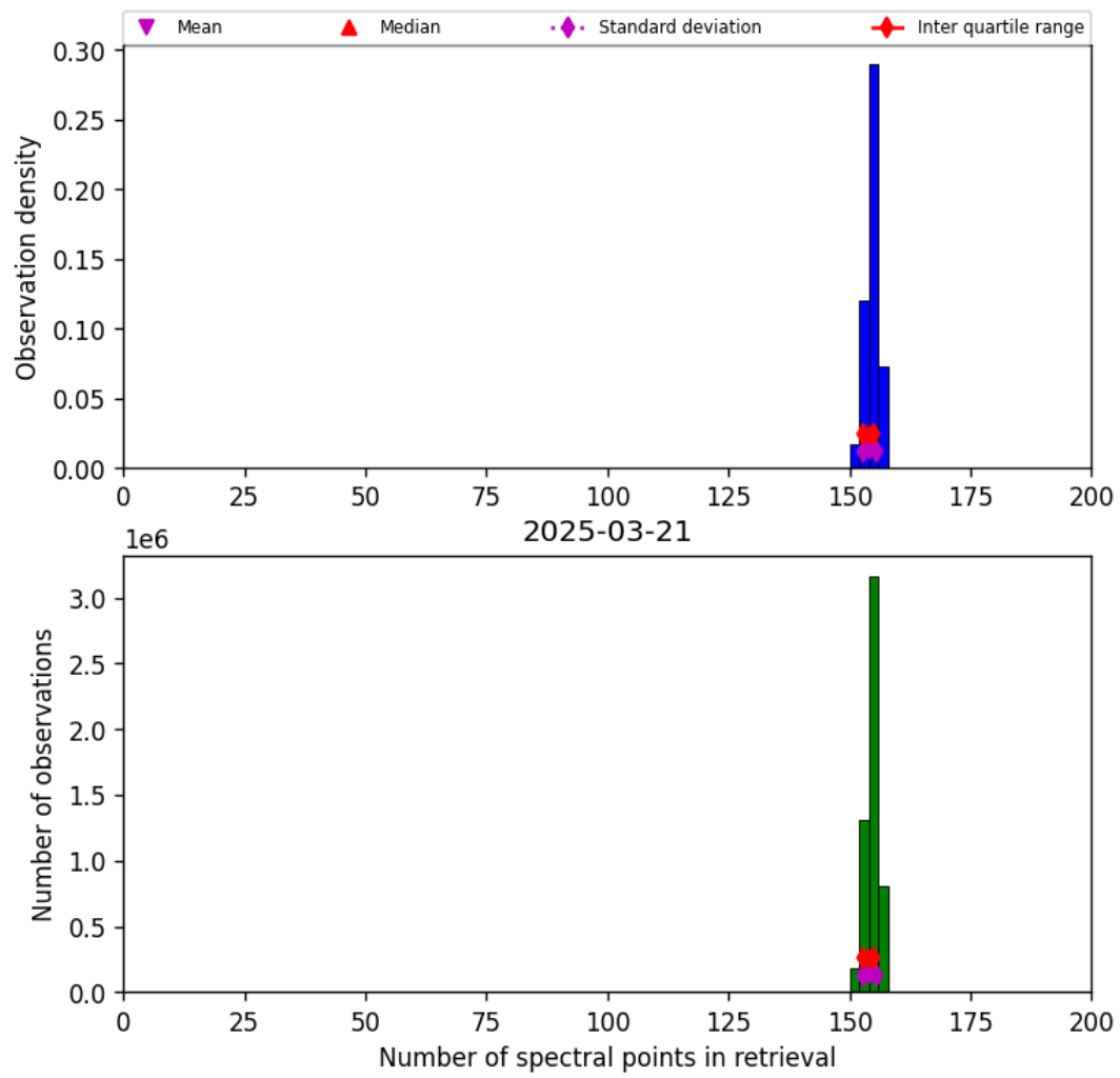
Figure 16: Histogram of “Number of spectral points in retrieval” for 2025-03-21 to 2025-03-21
