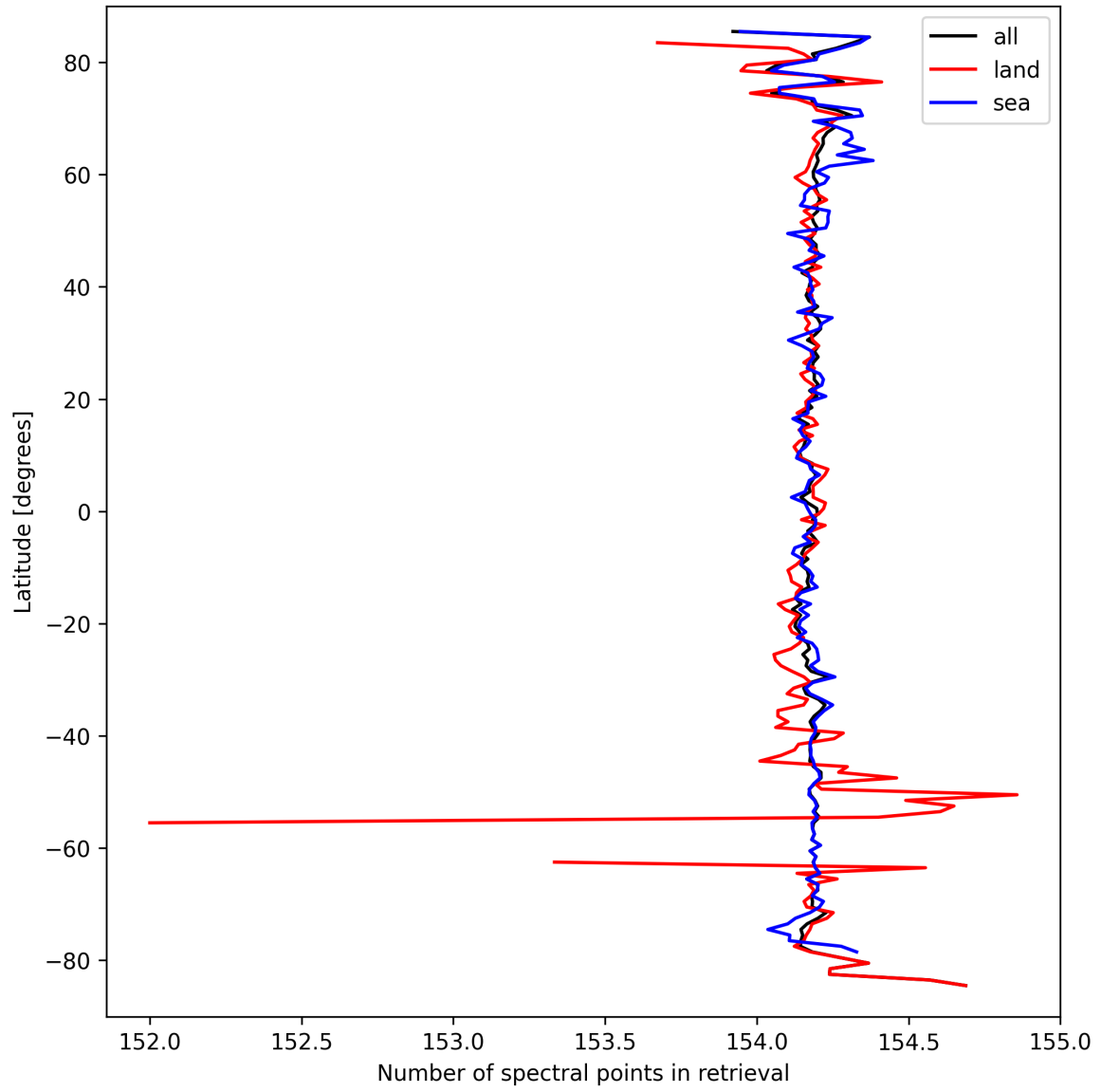
Figure 9: Zonal average of “Number of spectral points in retrieval” for 2025-03-21 to 2025-03-21.
