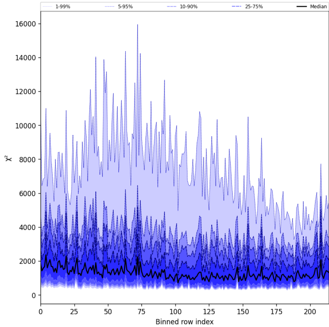
Figure 24: Along track statistics of “ \chi^2 ” for 2025-03-21 to 2025-03-21
