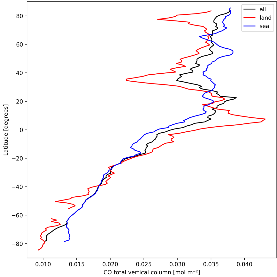
Figure 7: Zonal average of “CO total vertical column” for 2025-03-21 to 2025-03-21.
