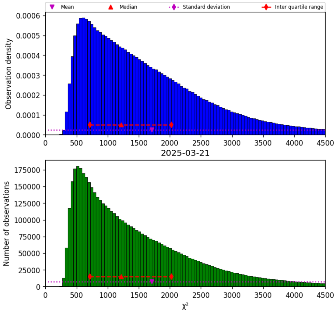
Figure 17: Histogram of " \chi^2 " for 2025-03-21 to 2025-03-21
