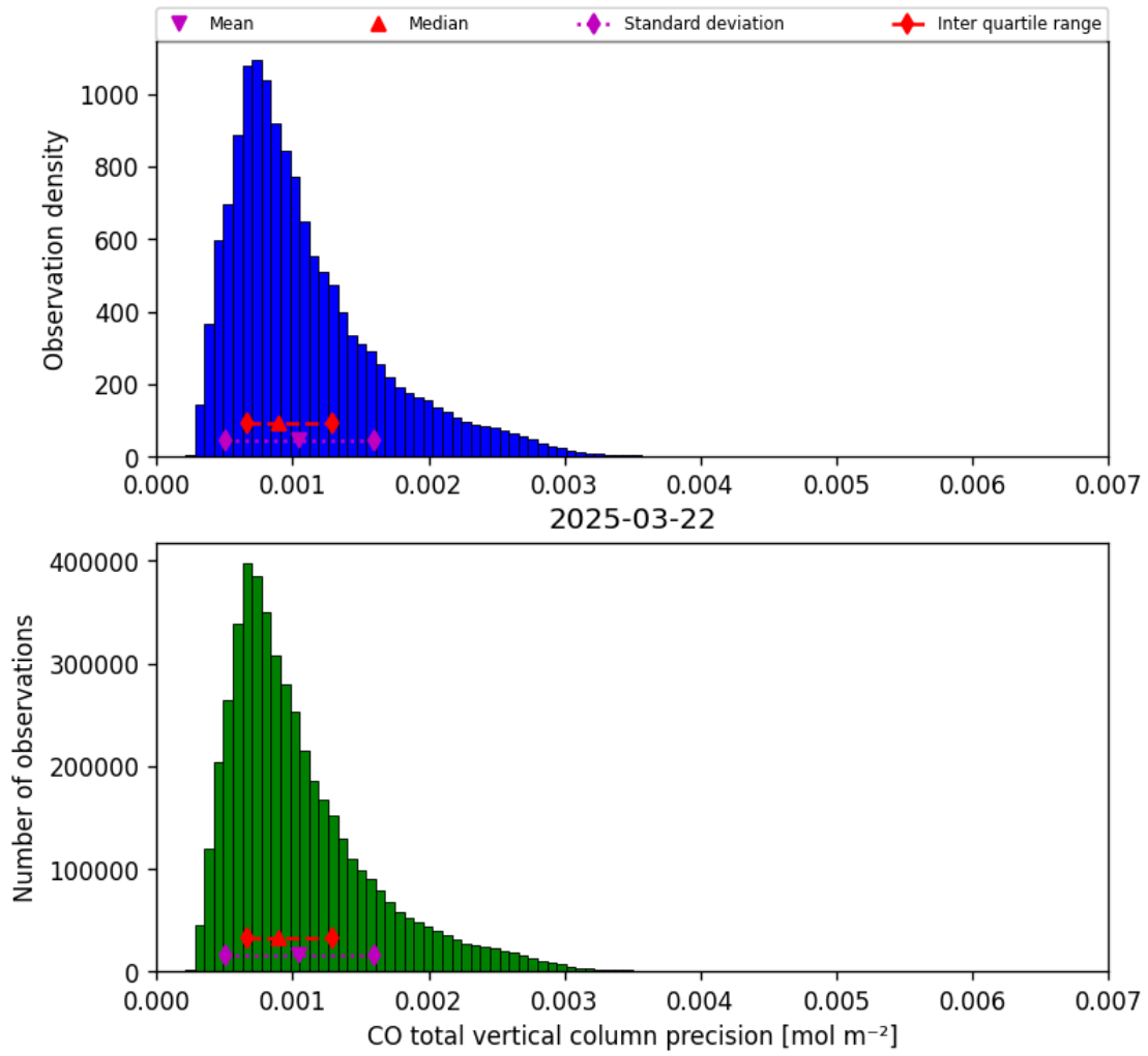
Figure 15: Histogram of “CO total vertical column precision” for 2025-03-22 to 2025-03-22
