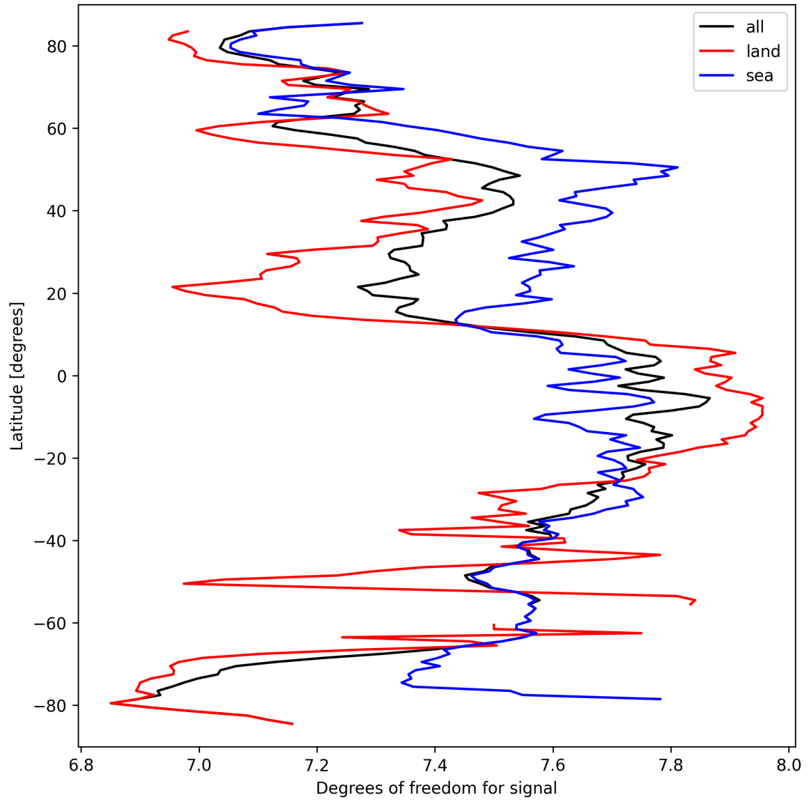
Figure 11: Zonal average of “Degrees of freedom for signal” for 2025-03-22 to 2025-03-22.
