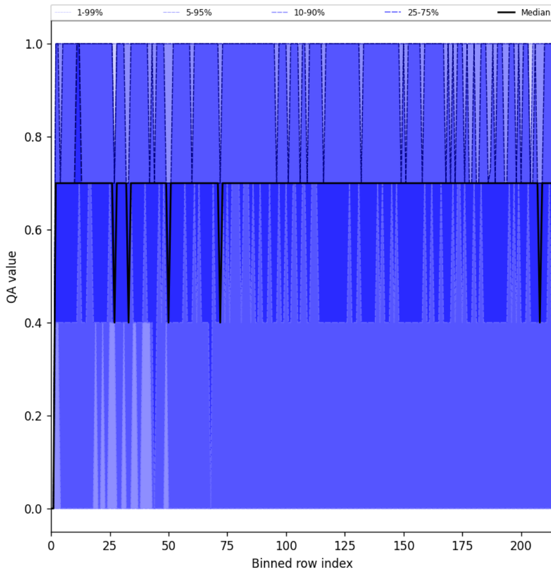
Figure 20: Along track statistics of “QA value” for 2025-03-22 to 2025-03-22
