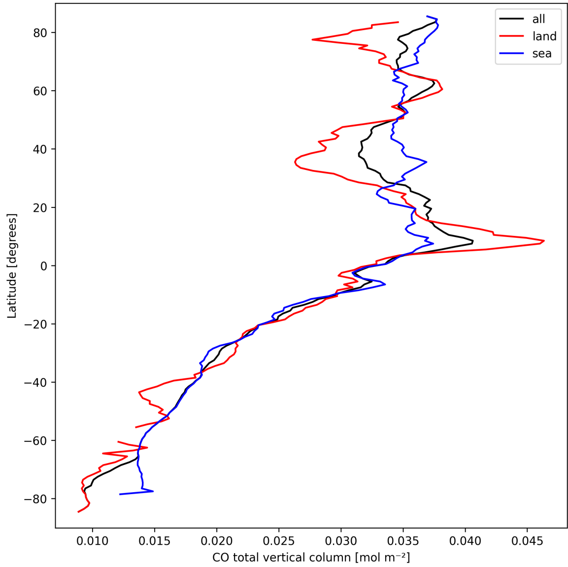
Figure 7: Zonal average of “CO total vertical column” for 2025-03-22 to 2025-03-22.
