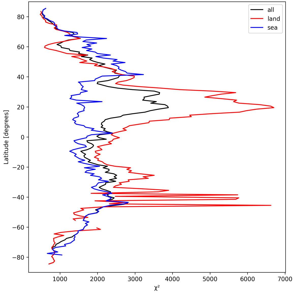
Figure 10: Zonal average of “ \chi^2 ” for 2025-03-22 to 2025-03-22.
