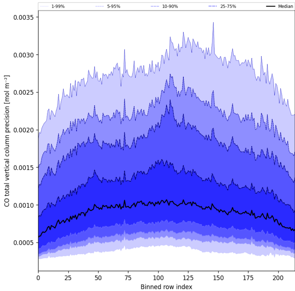
Figure 22: Along track statistics of “CO total vertical column precision” for 2025-03-22 to 2025-03-22
