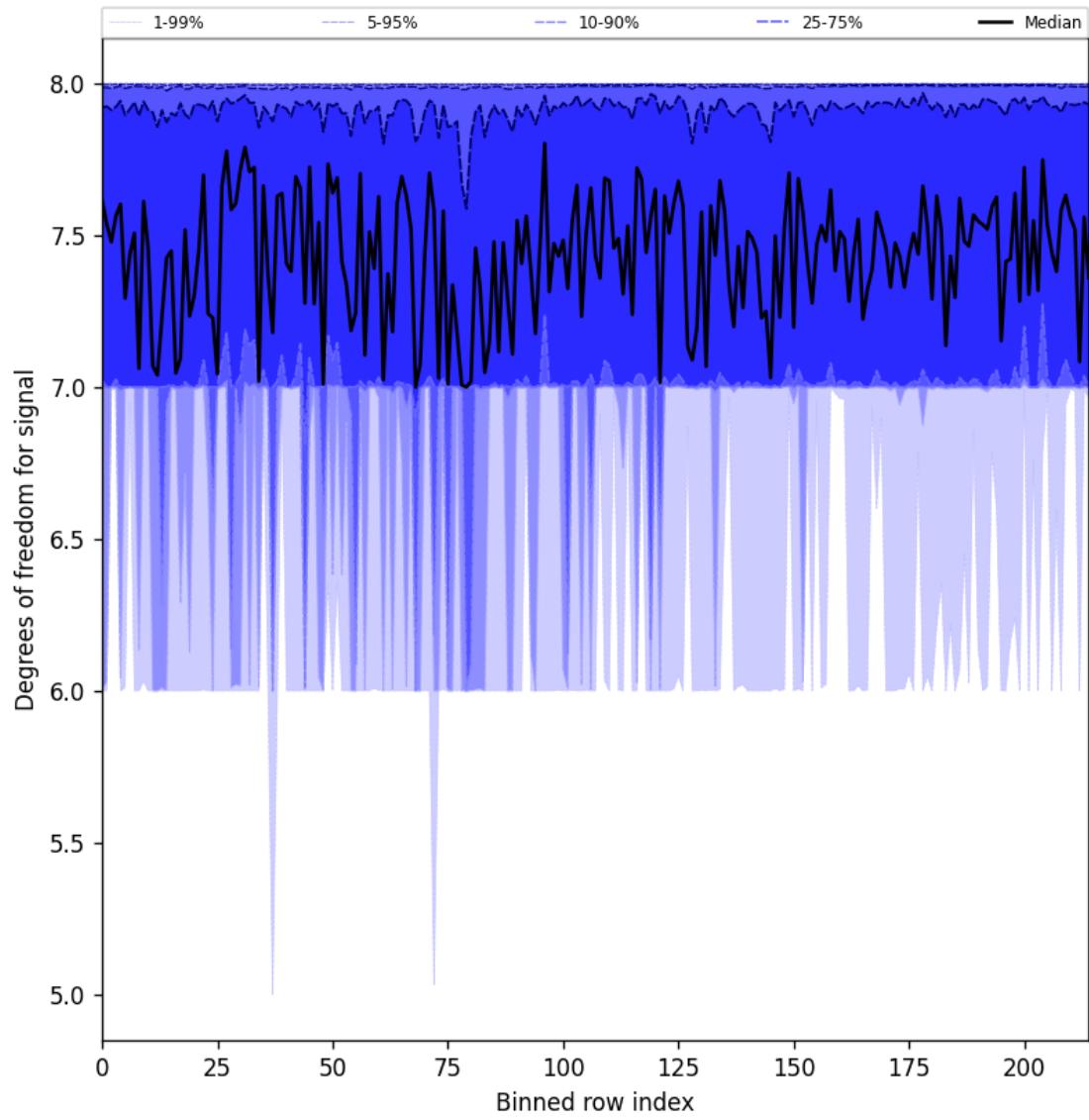
Figure 25: Along track statistics of “Degrees of freedom for signal” for 2025-03-22 to 2025-03-22
