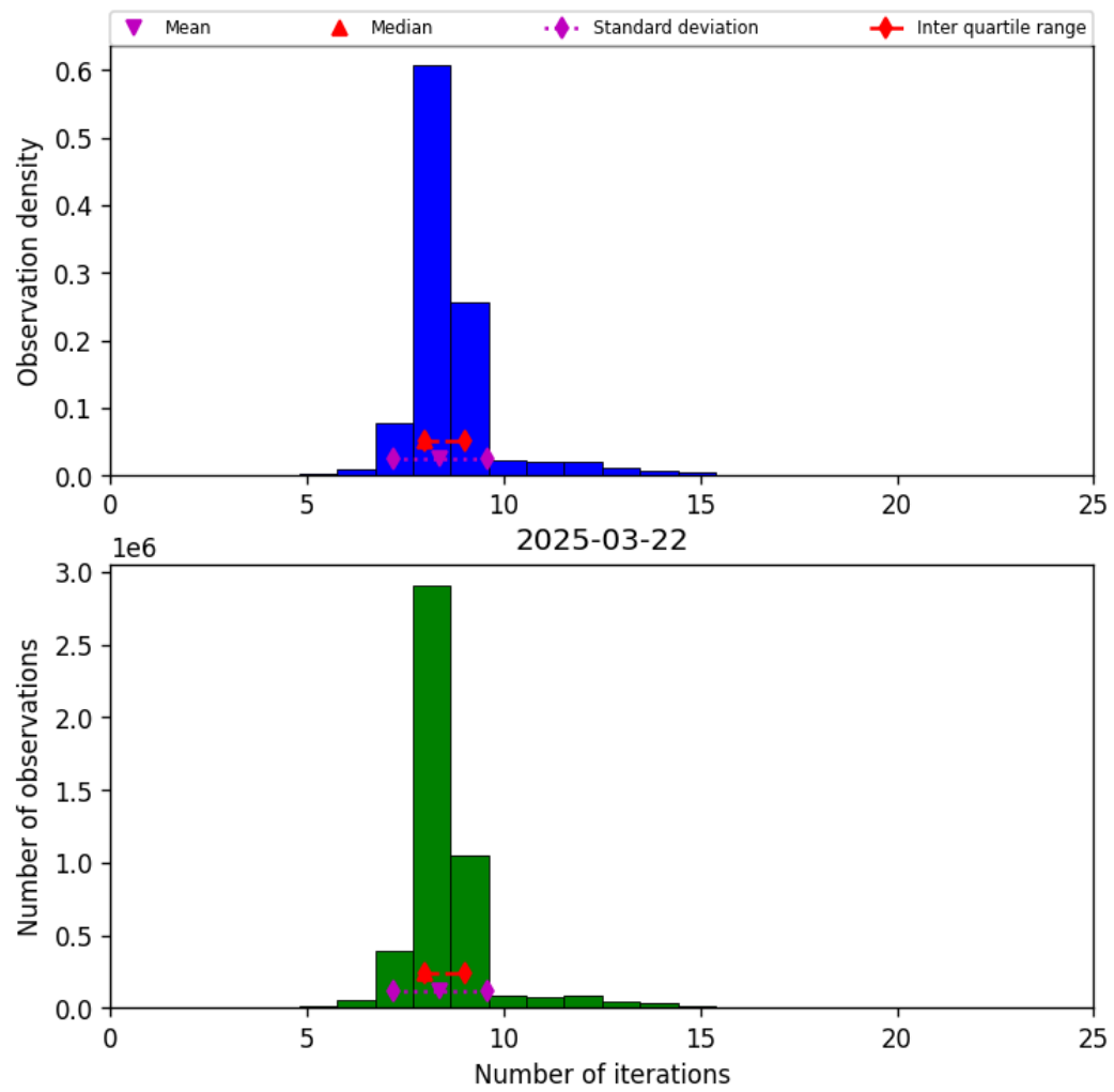
Figure 19: Histogram of “Number of iterations” for 2025-03-22 to 2025-03-22
