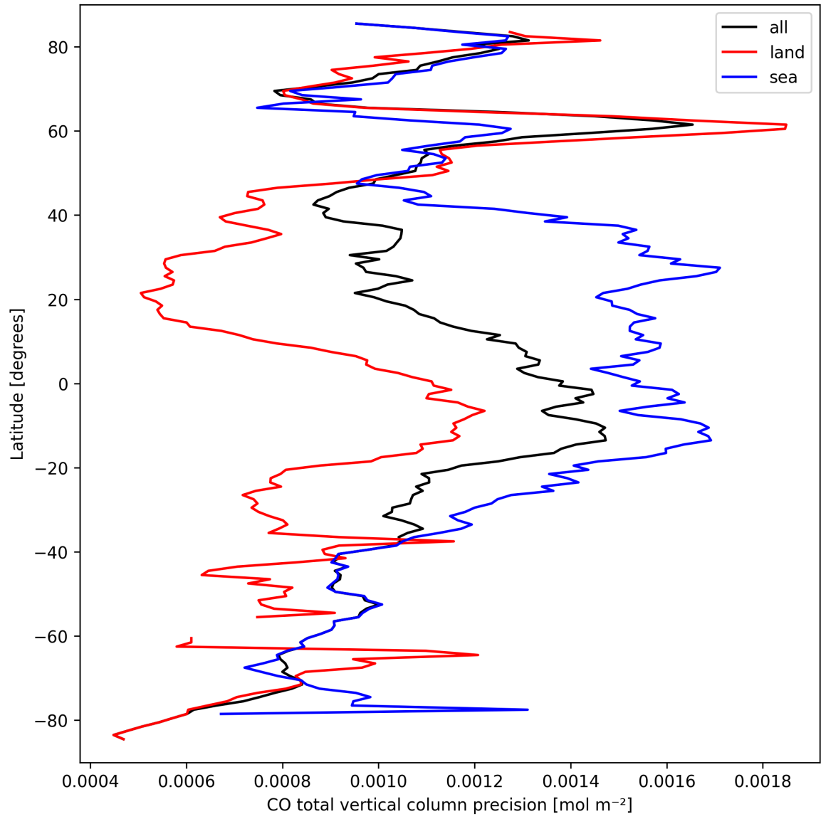
Figure 8: Zonal average of “CO total vertical column precision” for 2025-03-22 to 2025-03-22.
