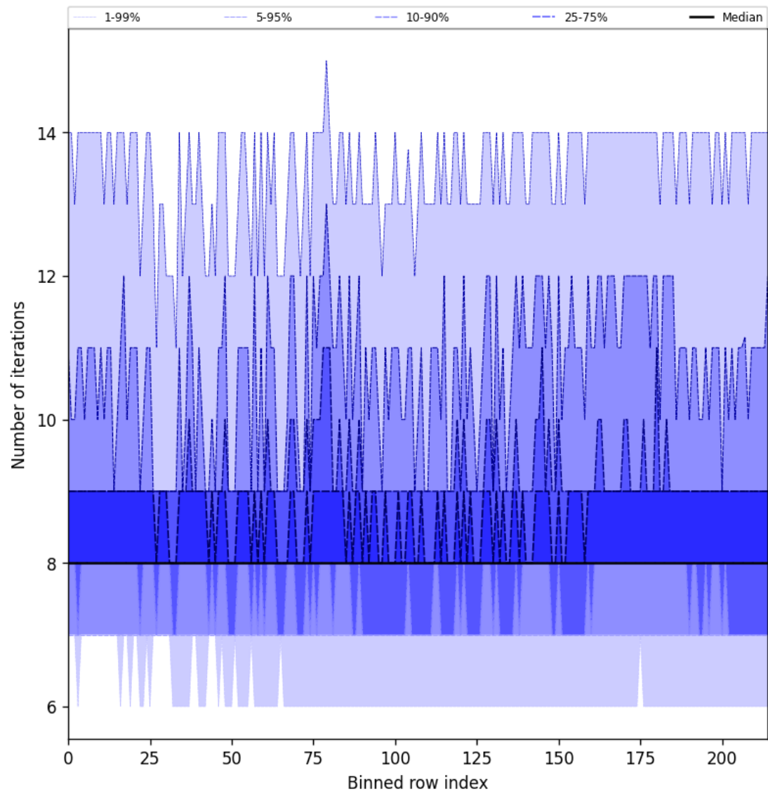
Figure 26: Along track statistics of “Number of iterations” for 2025-03-22 to 2025-03-22
