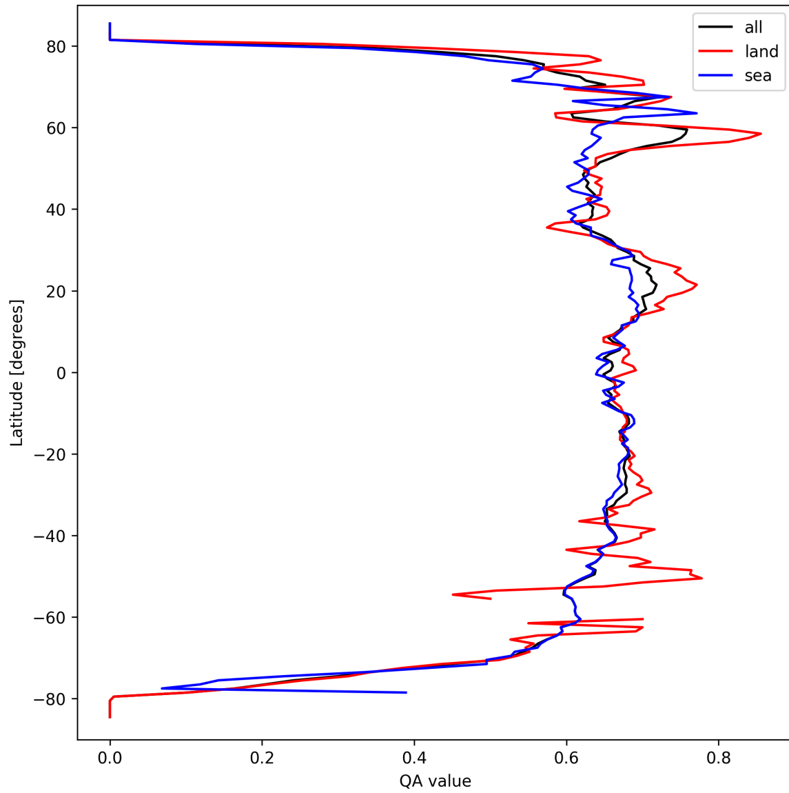
Figure 6: Zonal average of “QA value” for 2025-03-22 to 2025-03-22.
