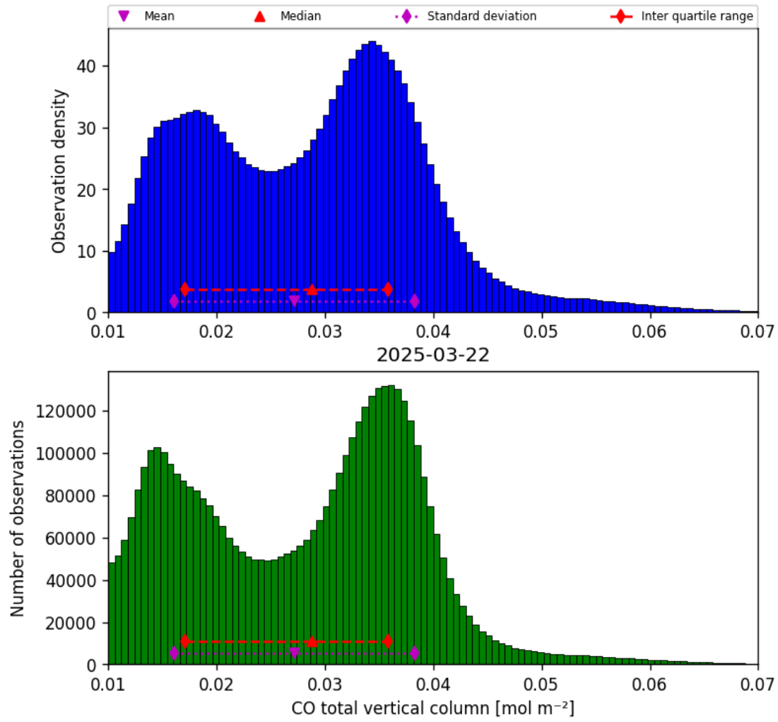
Figure 14: Histogram of “CO total vertical column” for 2025-03-22 to 2025-03-22
