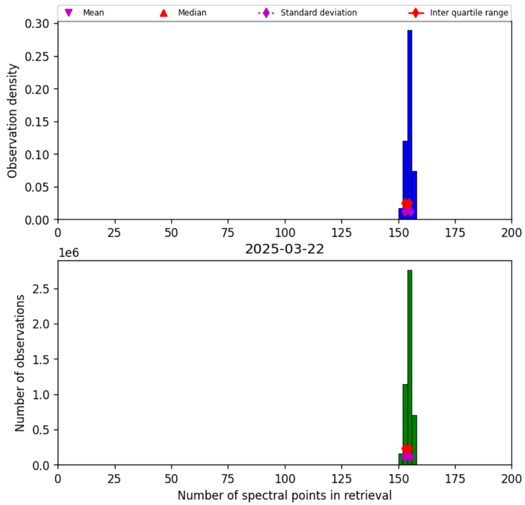
Figure 16: Histogram of “Number of spectral points in retrieval” for 2025-03-22 to 2025-03-22
