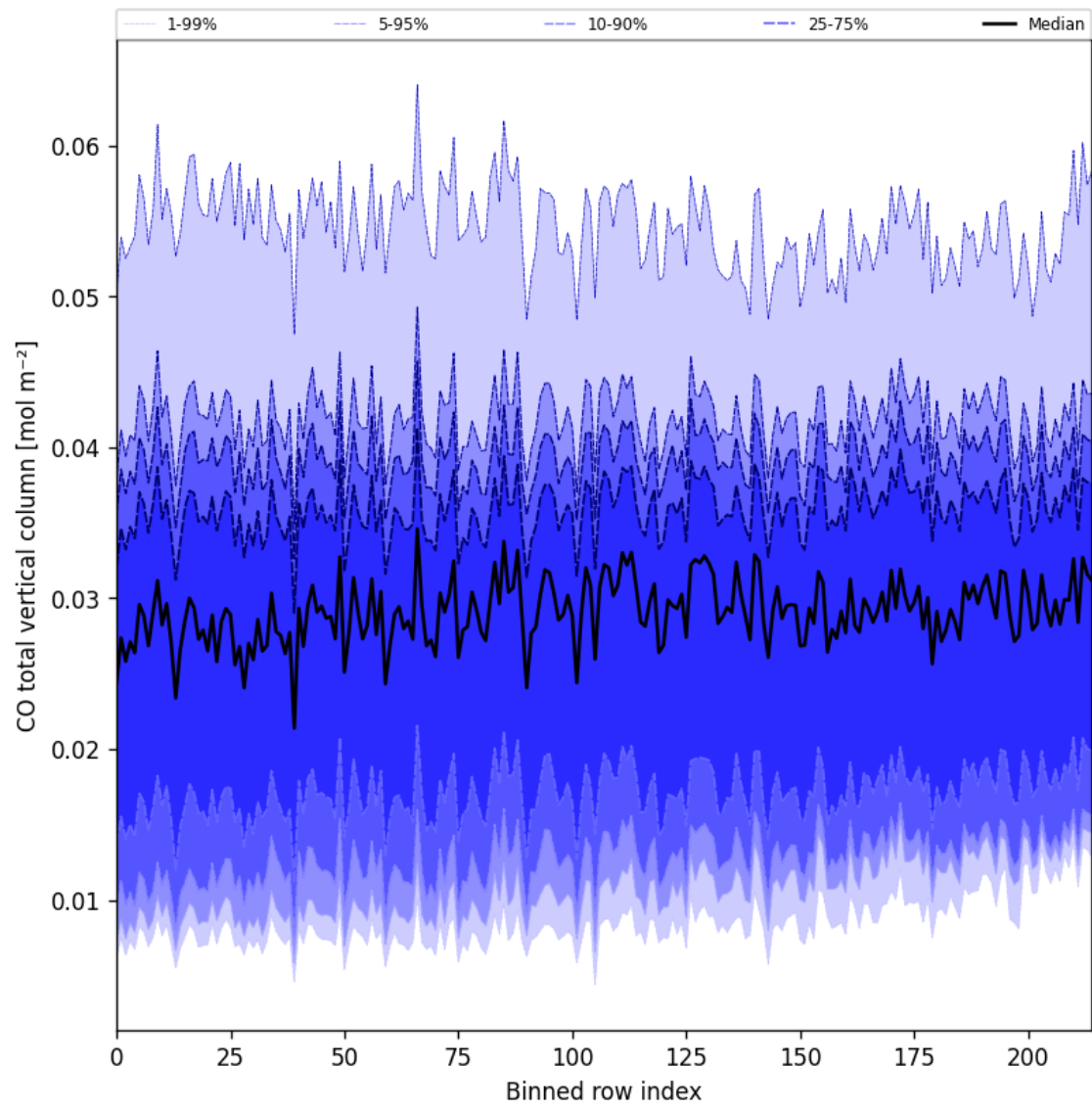
Figure 21: Along track statistics of “CO total vertical column” for 2025-03-22 to 2025-03-22
