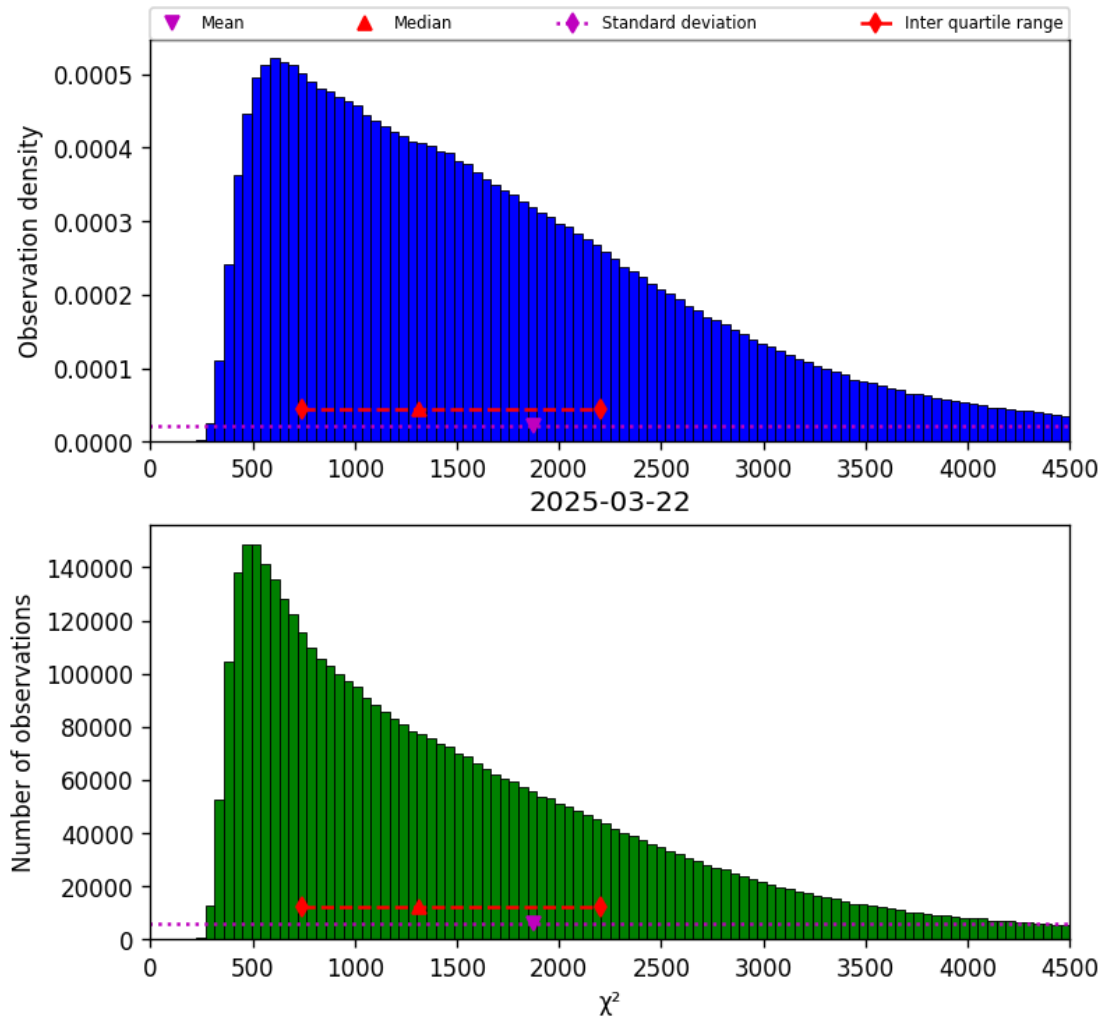
Figure 17: Histogram of " \chi^2 " for 2025-03-22 to 2025-03-22
