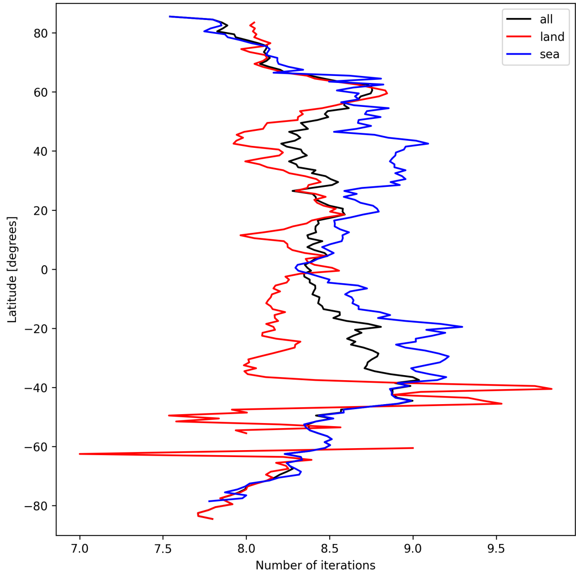
Figure 12: Zonal average of “Number of iterations” for 2025-03-22 to 2025-03-22.
