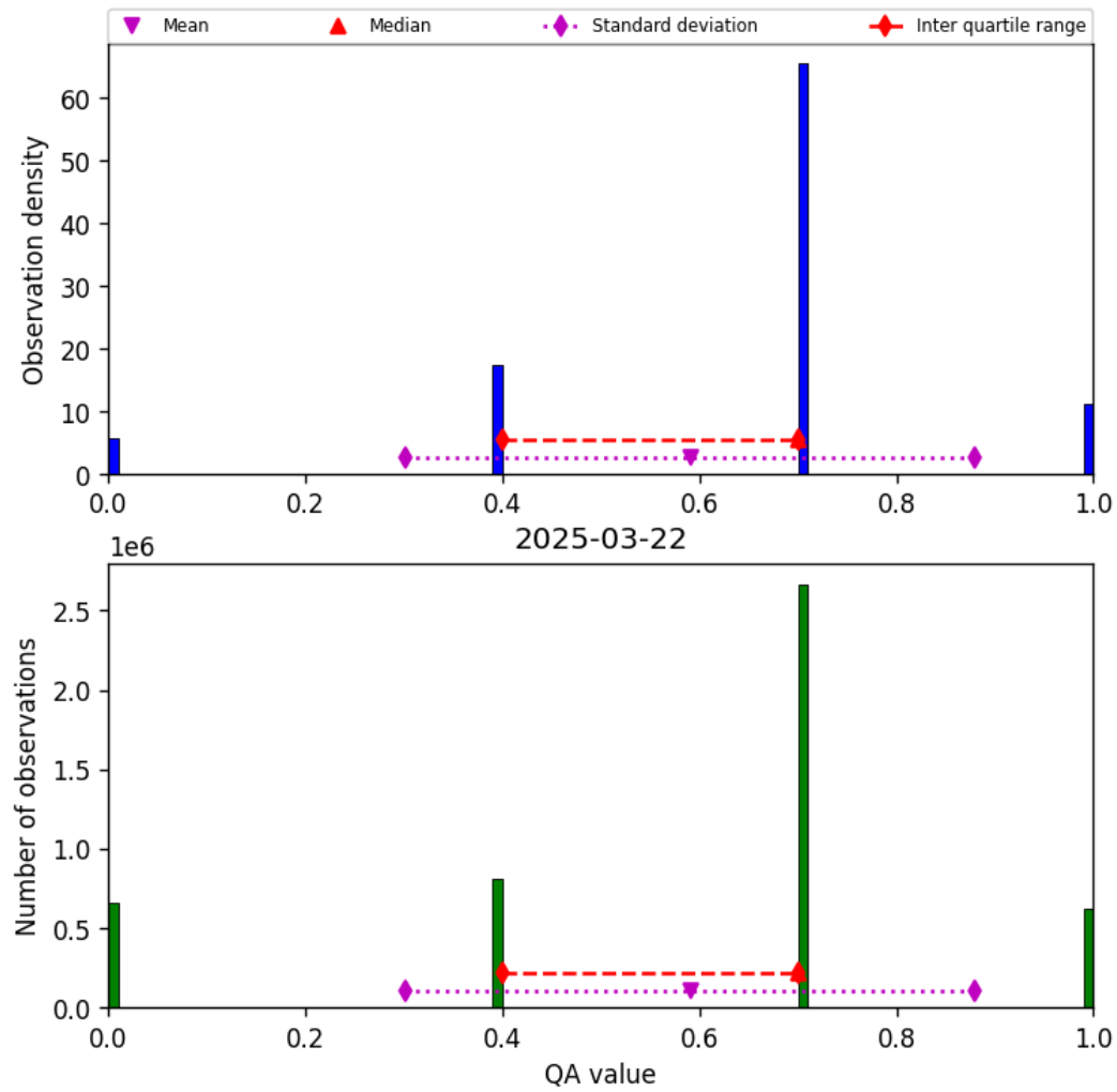
Figure 13: Histogram of “QA value” for 2025-03-22 to 2025-03-22
