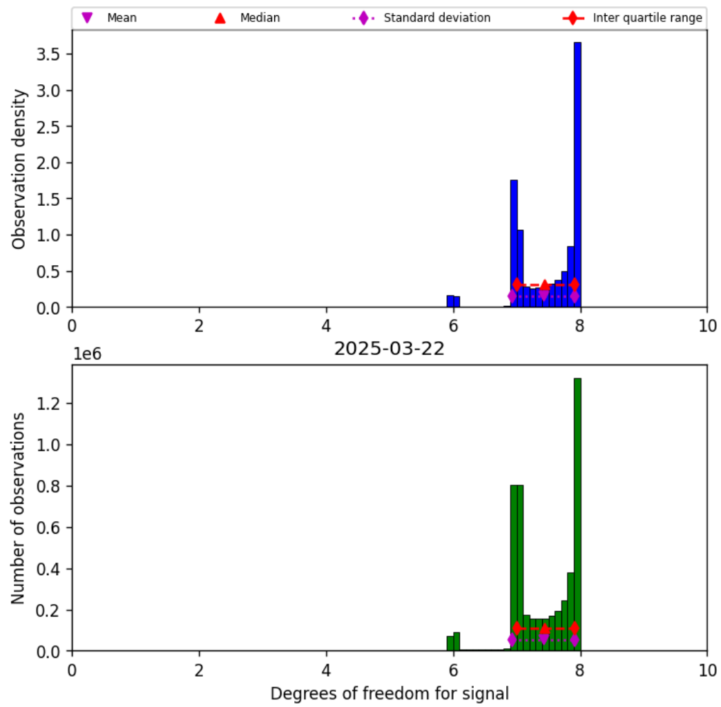
Figure 18: Histogram of “Degrees of freedom for signal” for 2025-03-22 to 2025-03-22
