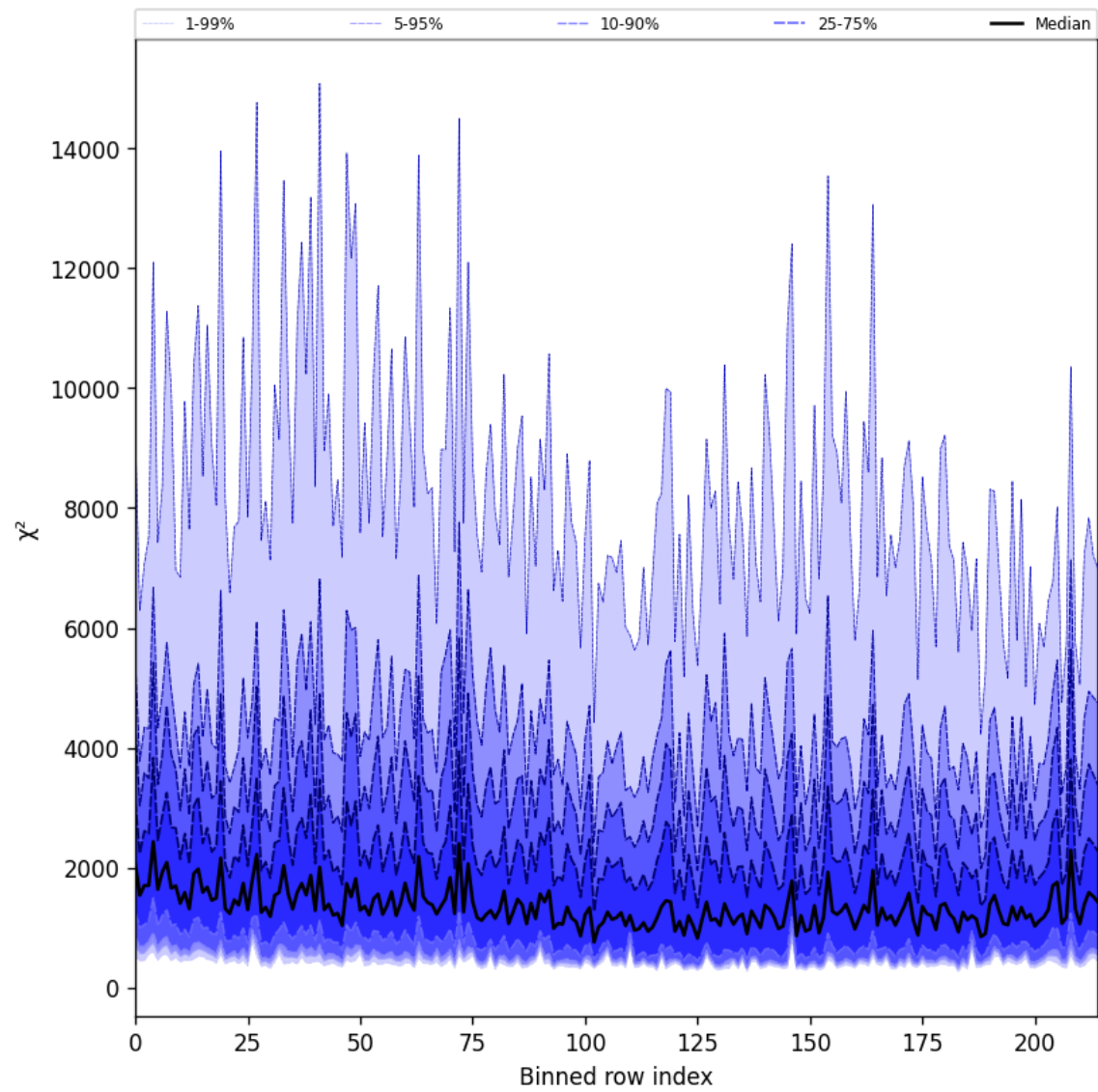
Figure 24: Along track statistics of “ \chi^2 ” for 2025-03-22 to 2025-03-22
