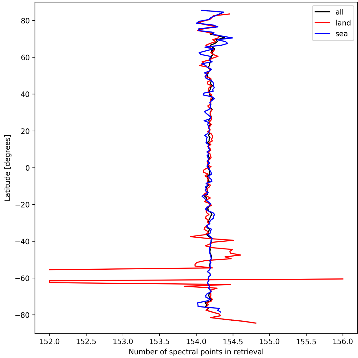
Figure 9: Zonal average of “Number of spectral points in retrieval” for 2025-03-22 to 2025-03-22.
