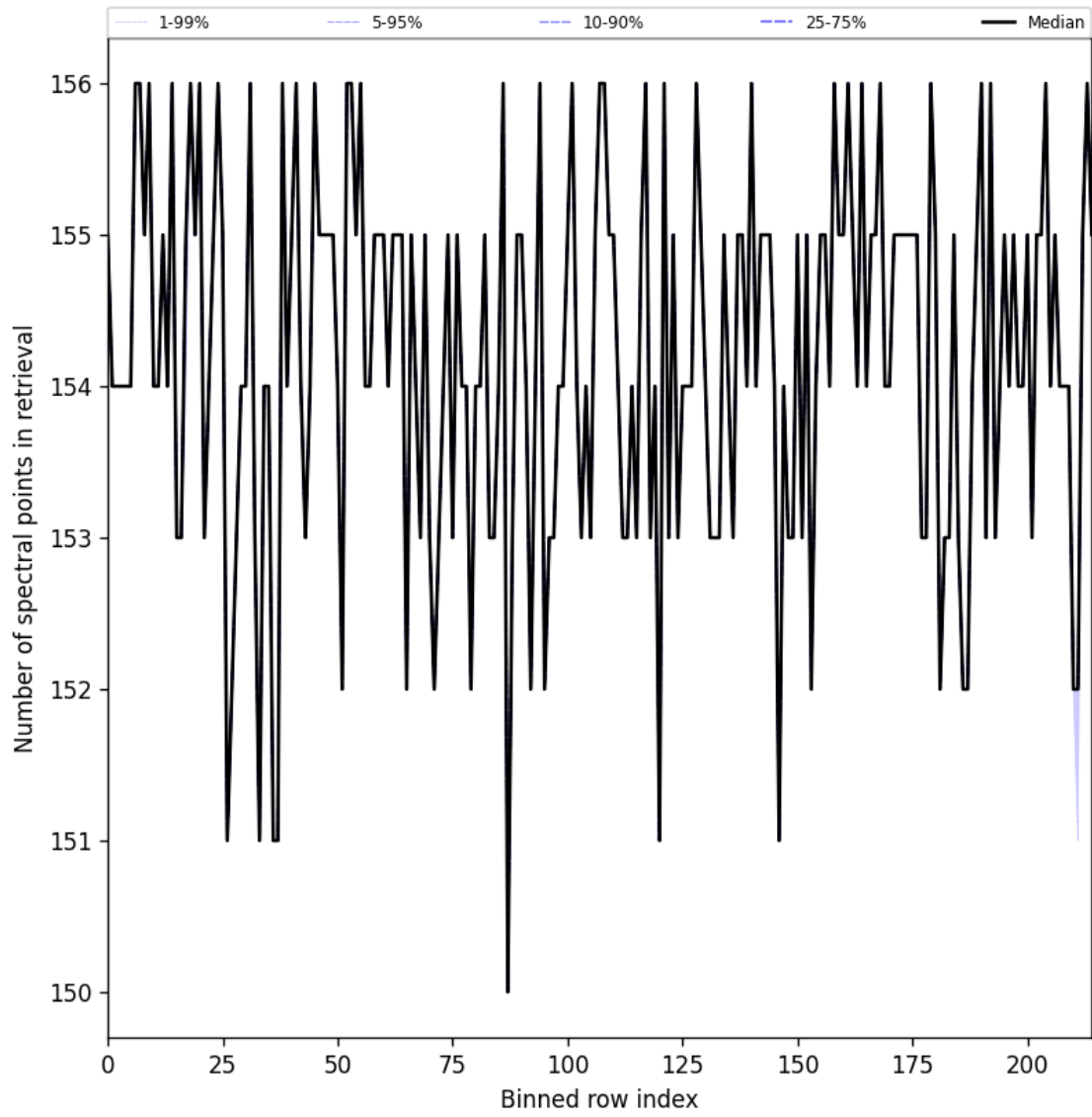
Figure 23: Along track statistics of “Number of spectral points in retrieval” for 2025-03-22 to 2025-03-22
