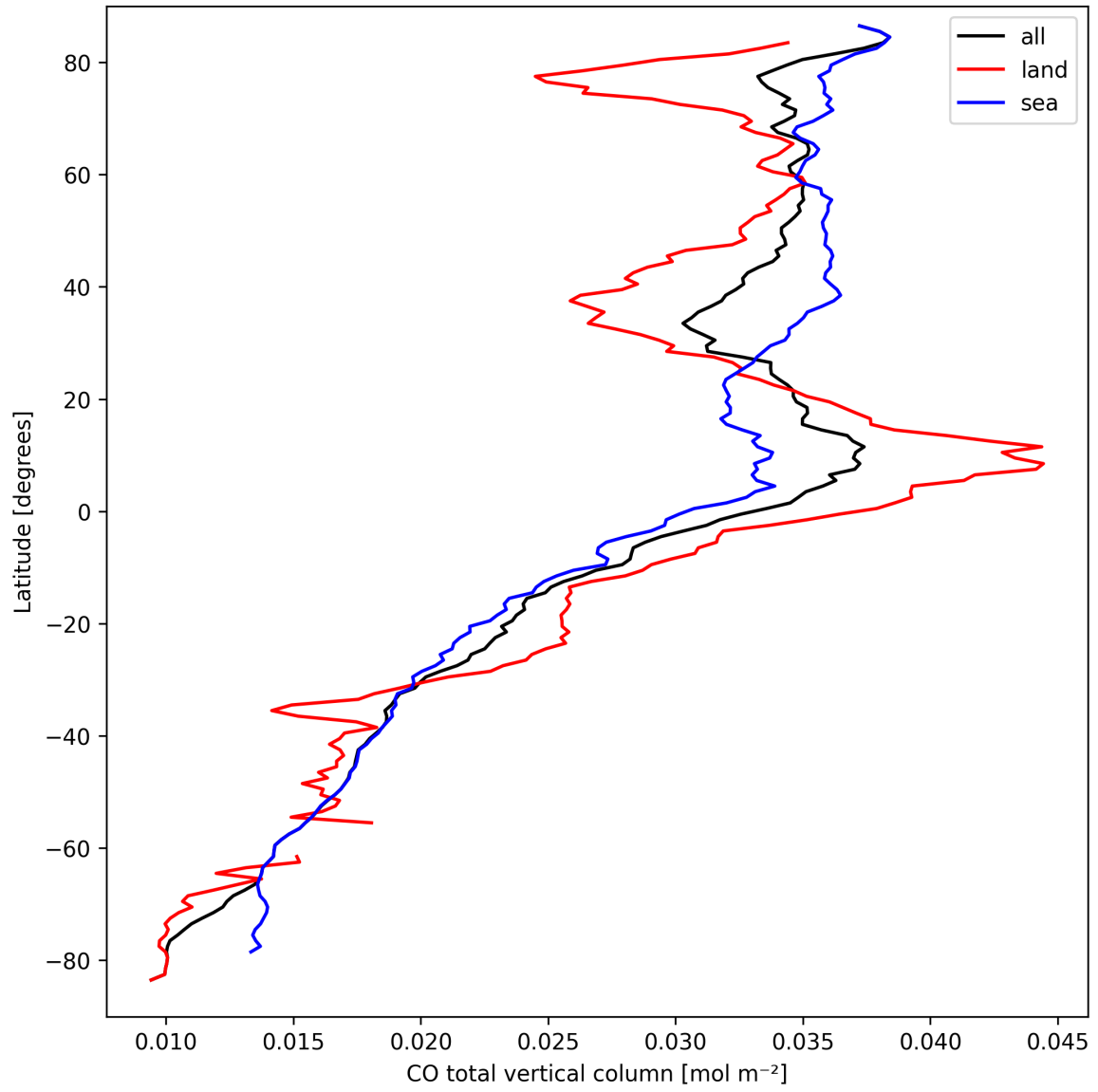
Figure 7: Zonal average of “CO total vertical column” for 2025-03-24 to 2025-03-25.
