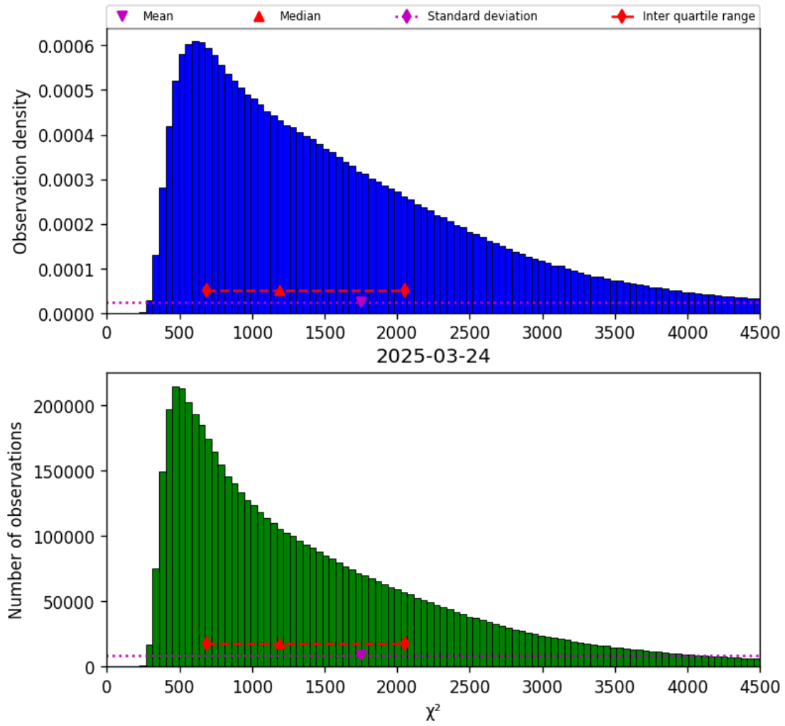
Figure 17: Histogram of “ \chi^2 ” for 2025-03-24 to 2025-03-25
