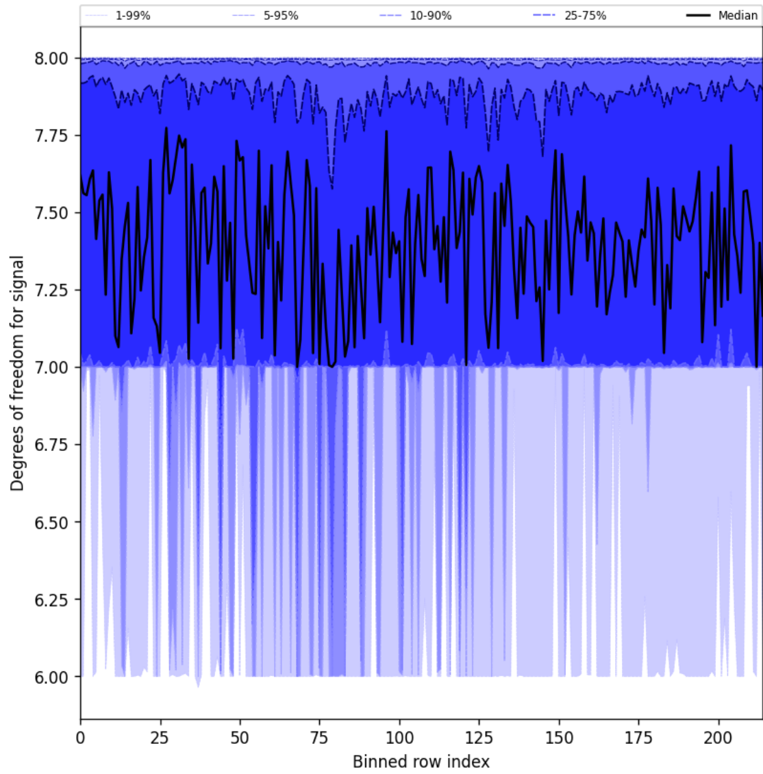
Figure 25: Along track statistics of “Degrees of freedom for signal” for 2025-03-24 to 2025-03-25
