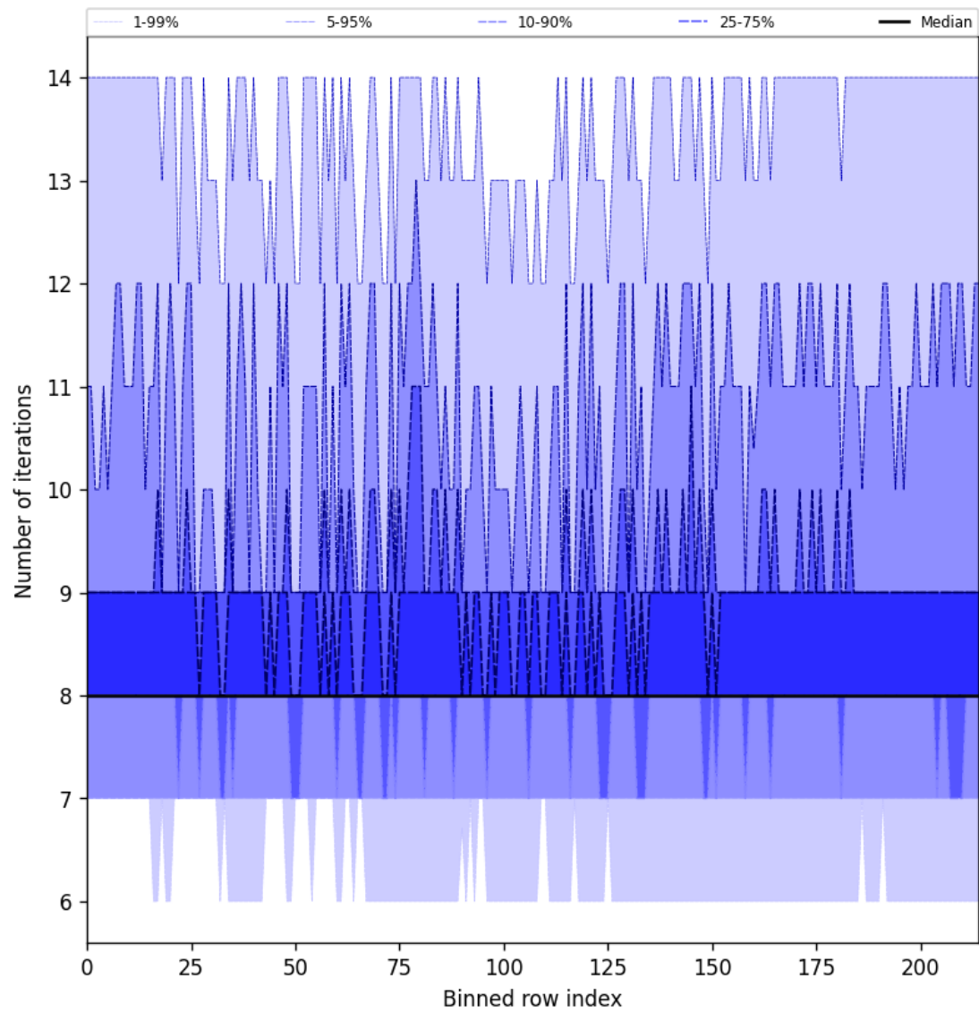
Figure 26: Along track statistics of “Number of iterations” for 2025-03-24 to 2025-03-25
