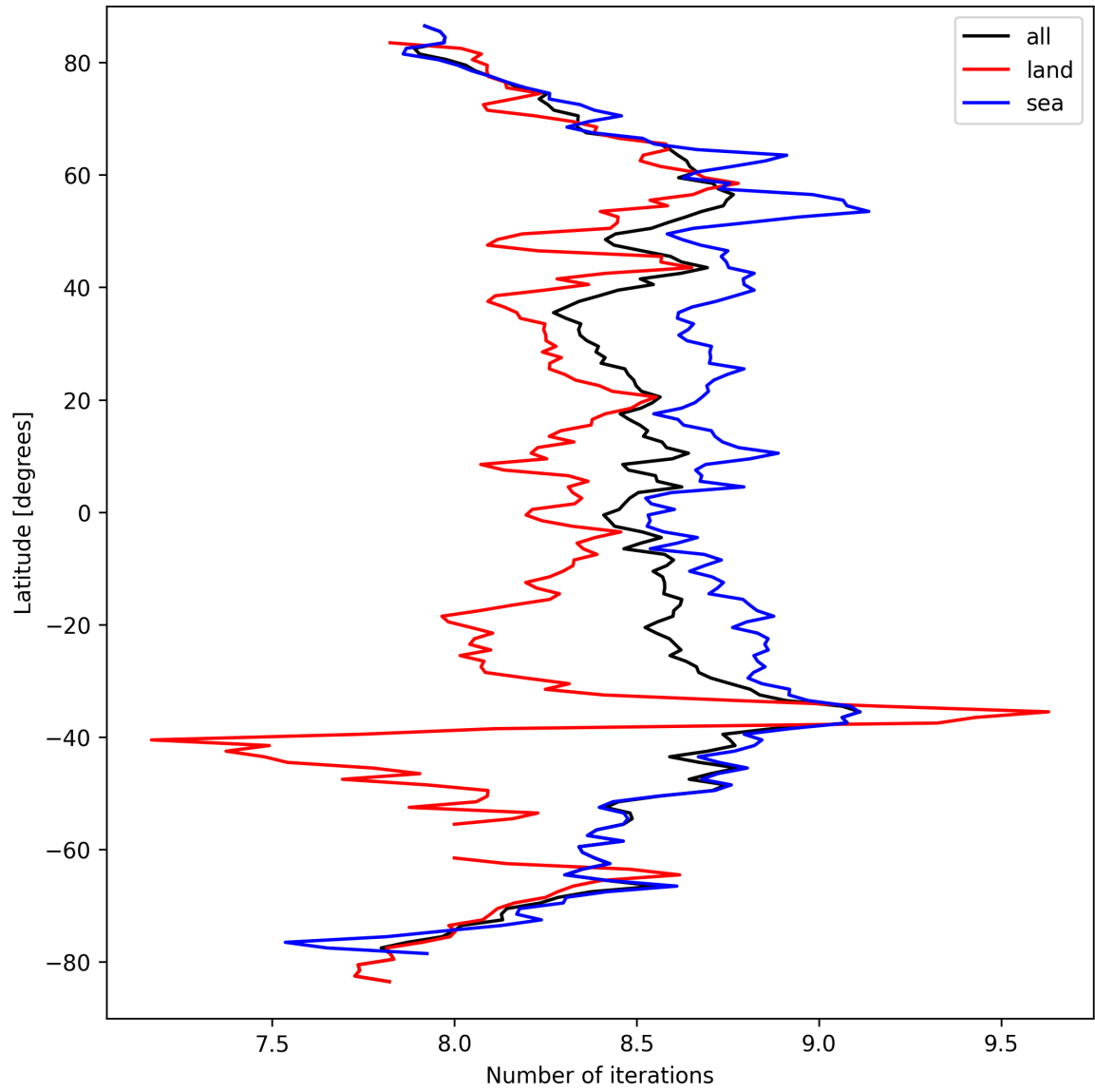
Figure 12: Zonal average of “Number of iterations” for 2025-03-24 to 2025-03-25.
