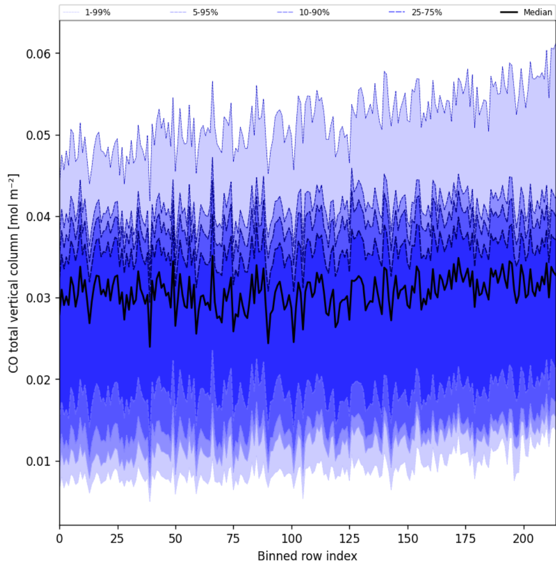
Figure 21: Along track statistics of “CO total vertical column” for 2025-03-24 to 2025-03-25
