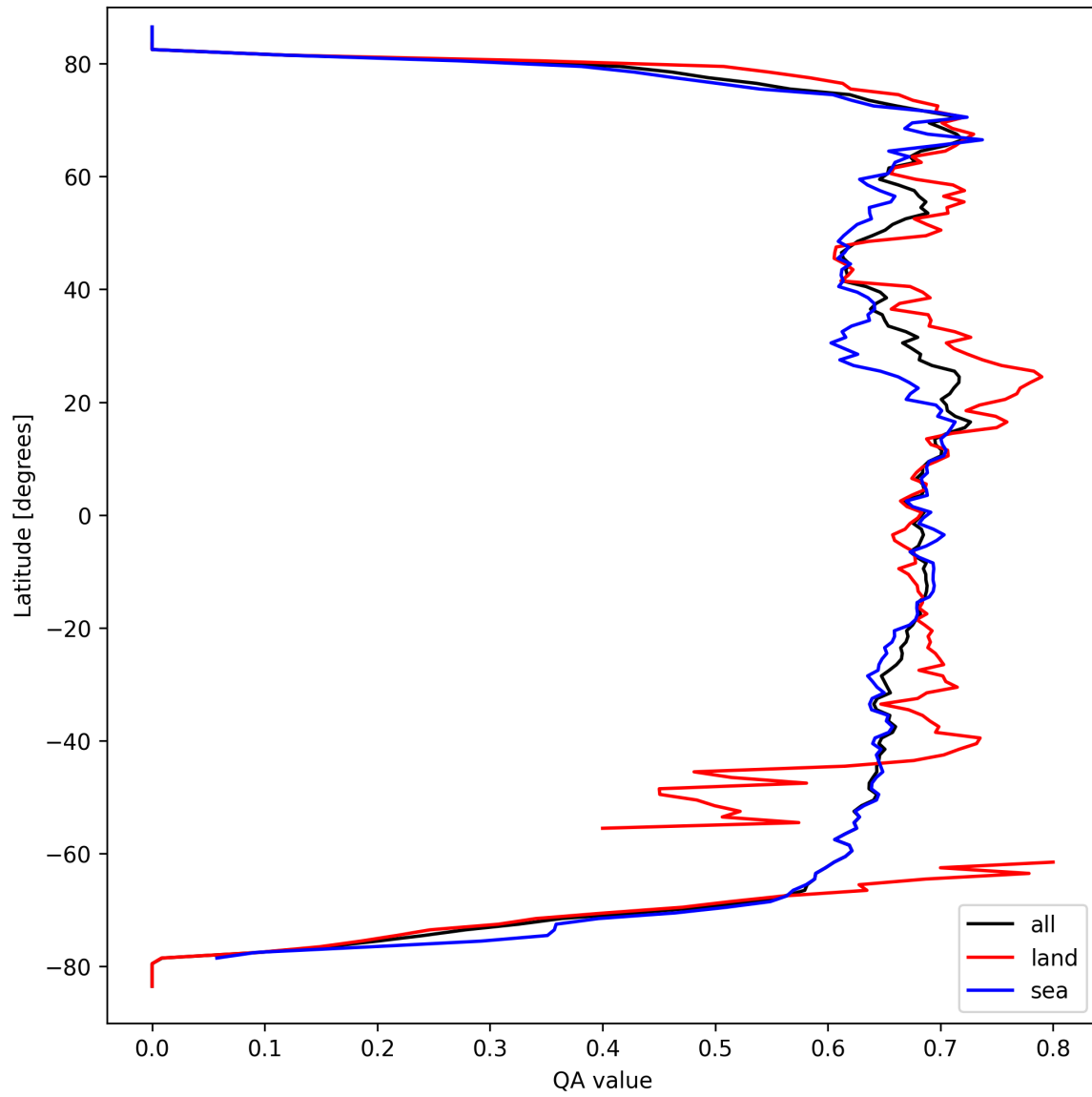
Figure 6: Zonal average of “QA value” for 2025-03-24 to 2025-03-25.
