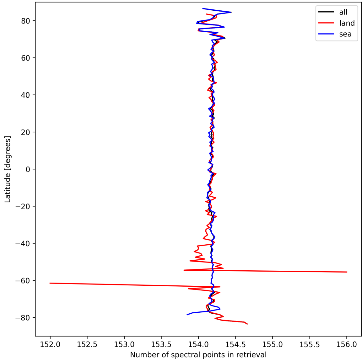
Figure 9: Zonal average of “Number of spectral points in retrieval” for 2025-03-24 to 2025-03-25.
