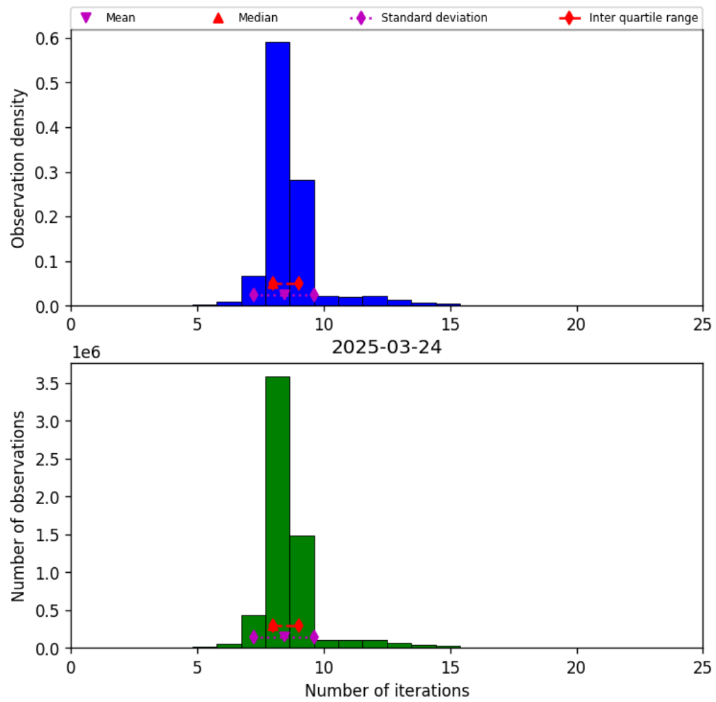
Figure 19: Histogram of “Number of iterations” for 2025-03-24 to 2025-03-25
