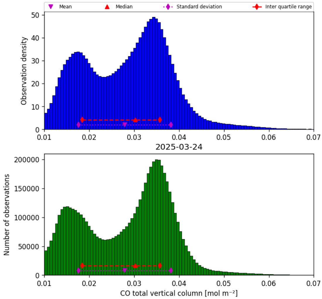
Figure 14: Histogram of “CO total vertical column” for 2025-03-24 to 2025-03-25
