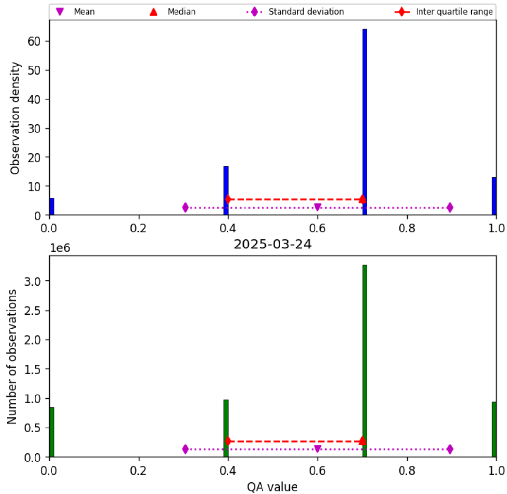
Figure 13: Histogram of “QA value” for 2025-03-24 to 2025-03-25
