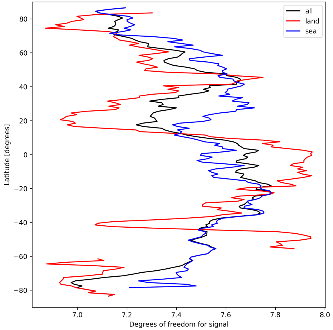
Figure 11: Zonal average of “Degrees of freedom for signal” for 2025-03-24 to 2025-03-25.
