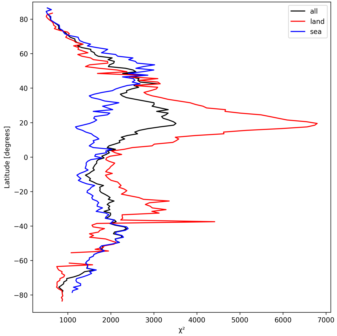
Figure 10: Zonal average of “ \chi^2 ” for 2025-03-24 to 2025-03-25.
