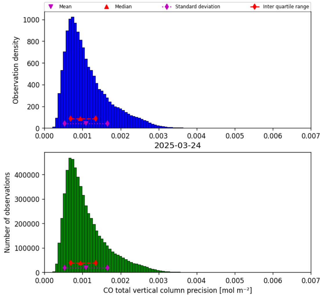
Figure 15: Histogram of “CO total vertical column precision” for 2025-03-24 to 2025-03-25
