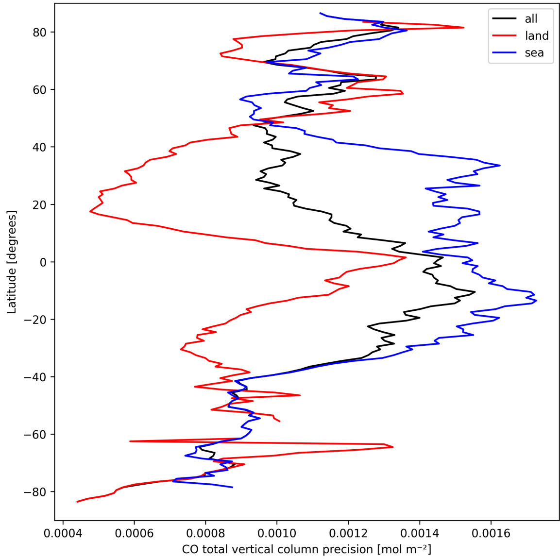
Figure 8: Zonal average of "CO total vertical column precision" for 2025-03-24 to 2025-03-25.
