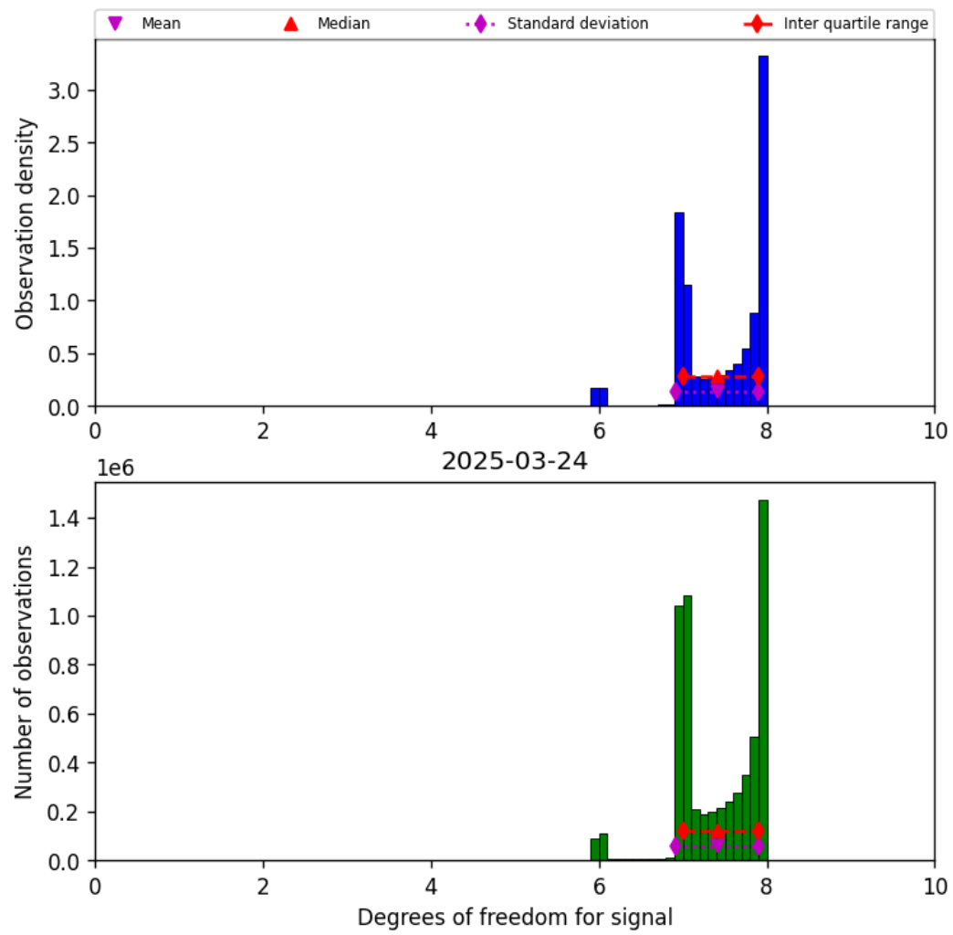
Figure 18: Histogram of “Degrees of freedom for signal” for 2025-03-24 to 2025-03-25
