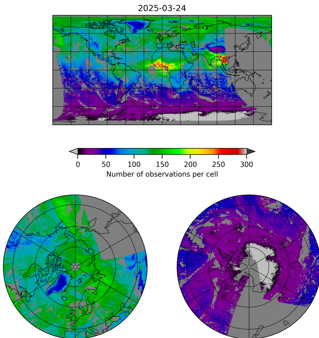
Figure 5: Map of the number of observations for 2025-03-24 to 2025-03-25
