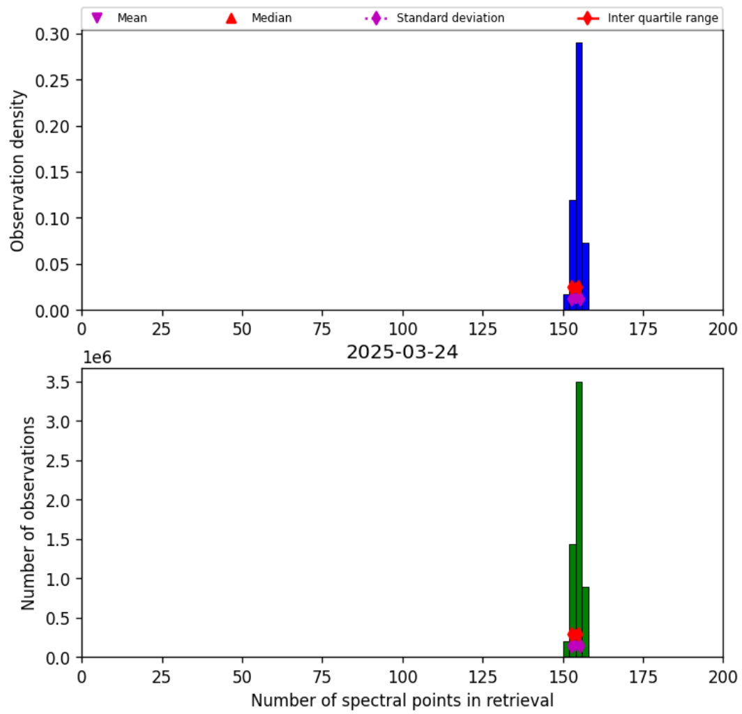
Figure 16: Histogram of “Number of spectral points in retrieval” for 2025-03-24 to 2025-03-25
