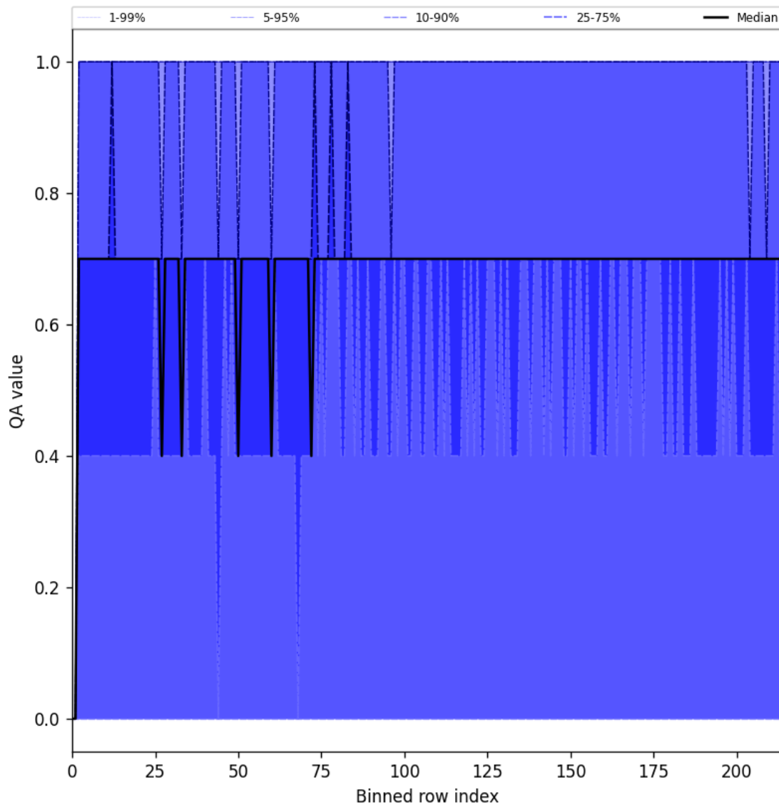
Figure 20: Along track statistics of “QA value” for 2025-03-24 to 2025-03-25
