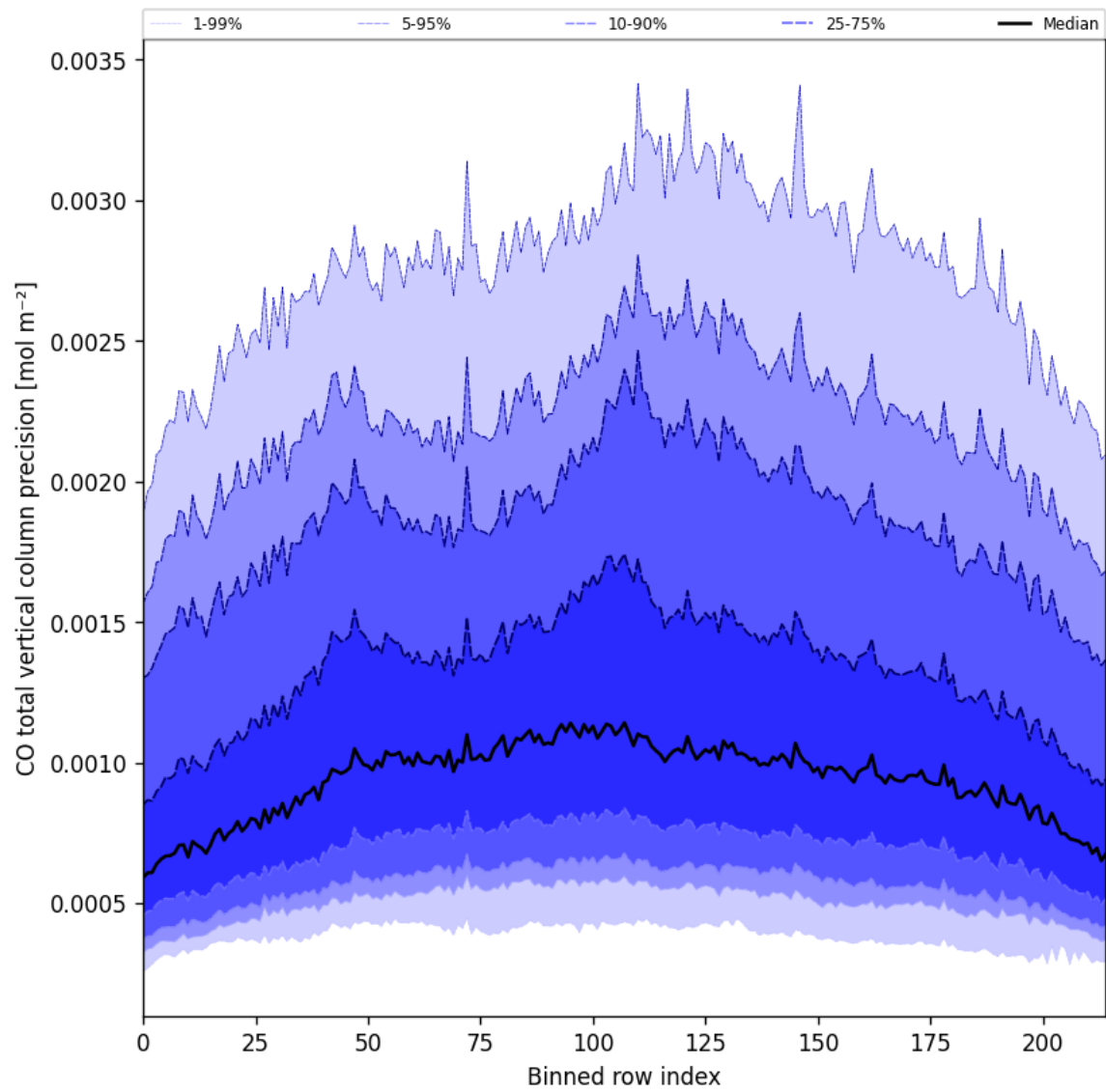
Figure 22: Along track statistics of “CO total vertical column precision” for 2025-03-24 to 2025-03-25
