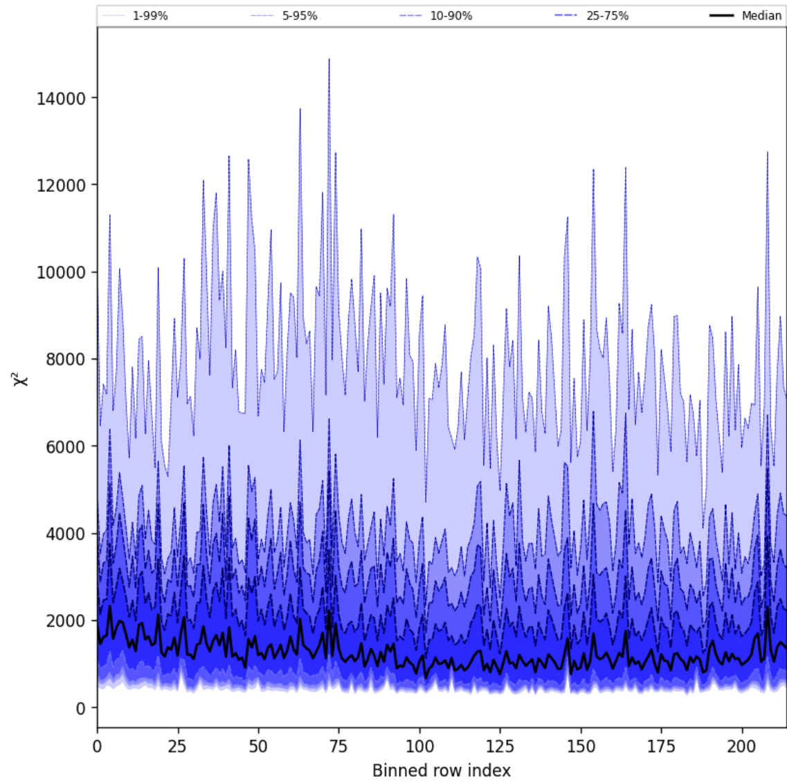
Figure 24: Along track statistics of “ \chi^2 ” for 2025-03-24 to 2025-03-25
