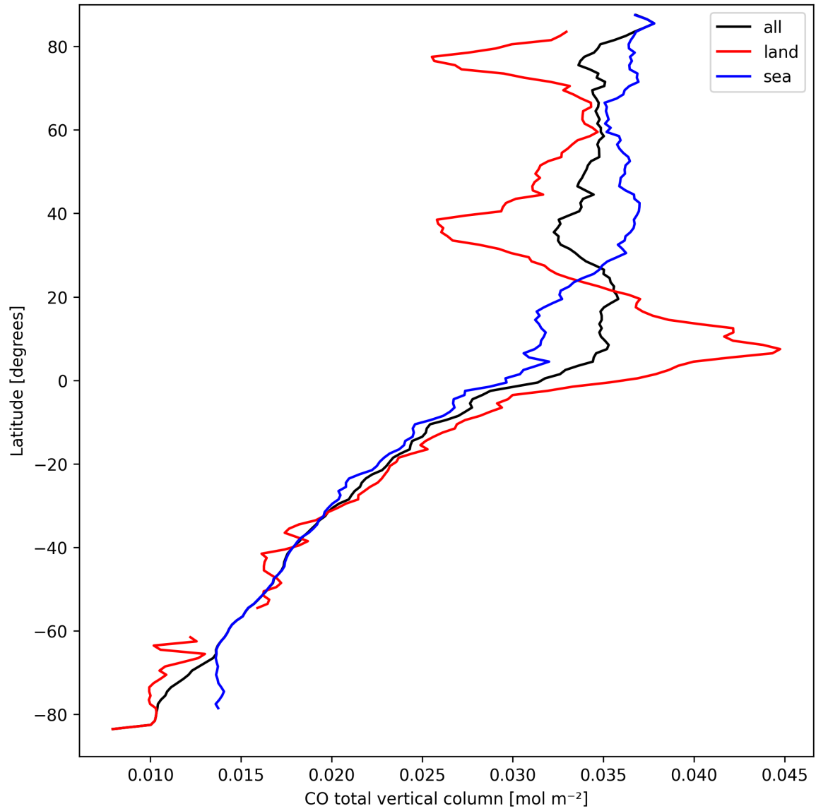
Figure 7: Zonal average of “CO total vertical column” for 2025-03-25 to 2025-03-26.
