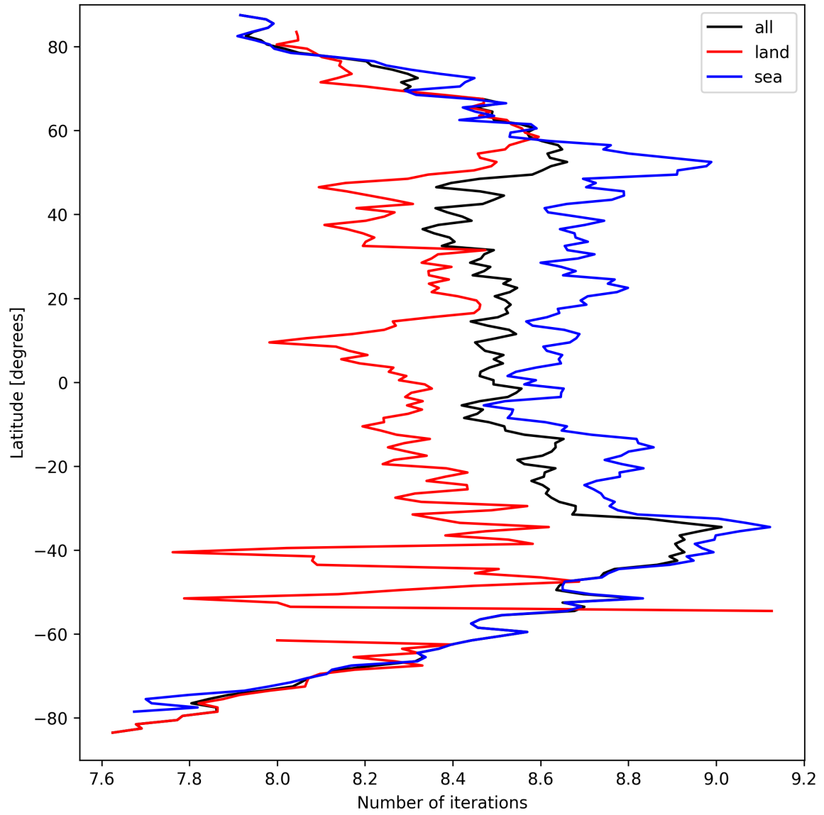
Figure 12: Zonal average of “Number of iterations” for 2025-03-25 to 2025-03-26.
