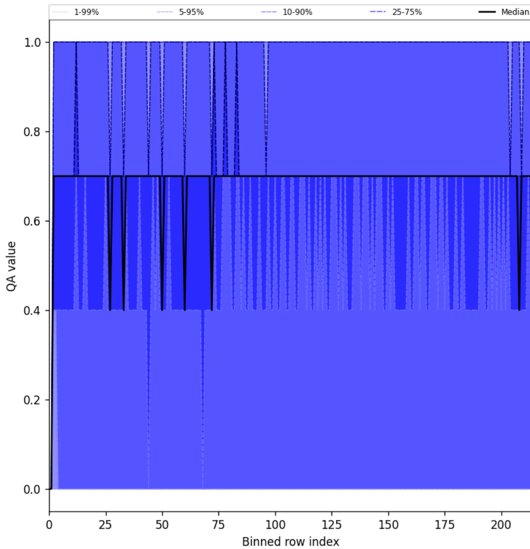
Figure 20: Along track statistics of “QA value” for 2025-03-25 to 2025-03-26
