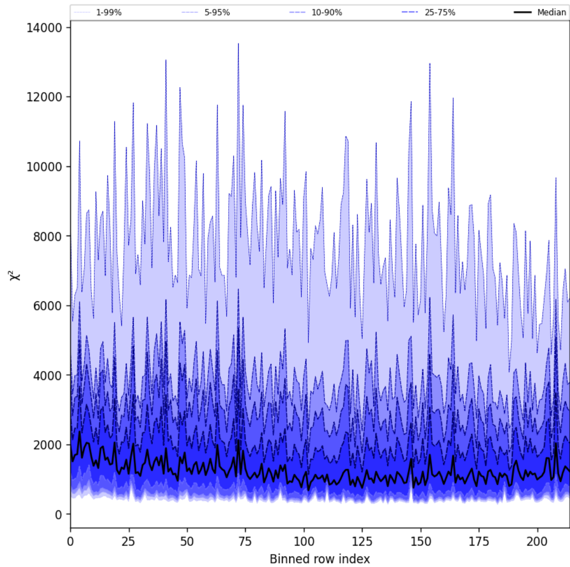
Figure 24: Along track statistics of “ \chi^2 ” for 2025-03-25 to 2025-03-26
