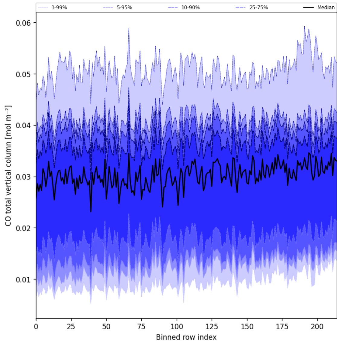
Figure 21: Along track statistics of “CO total vertical column” for 2025-03-25 to 2025-03-26
