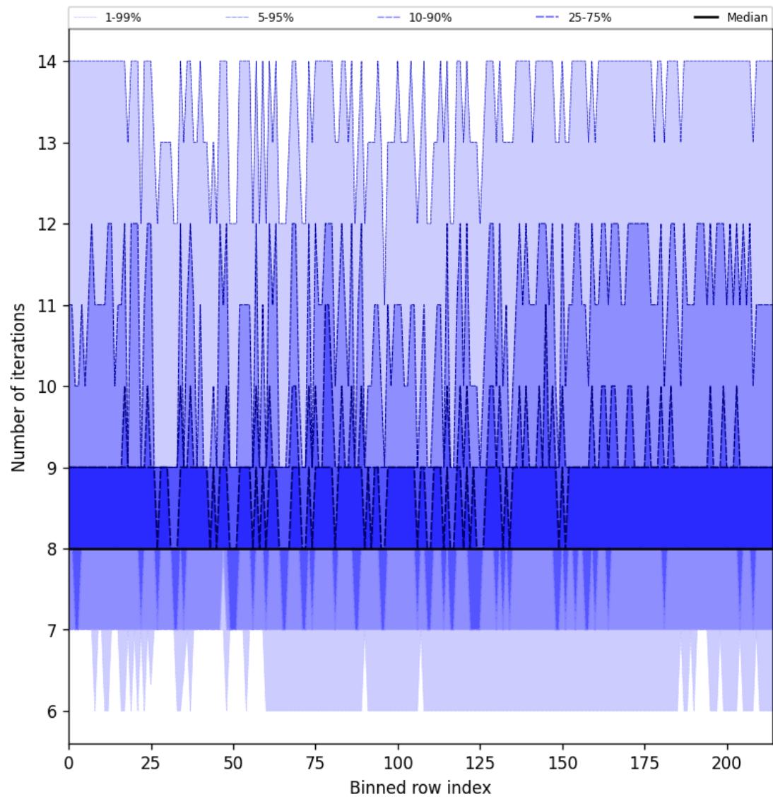
Figure 26: Along track statistics of “Number of iterations” for 2025-03-25 to 2025-03-26
