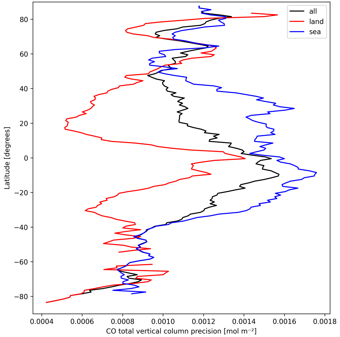
Figure 8: Zonal average of “CO total vertical column precision” for 2025-03-25 to 2025-03-26.
