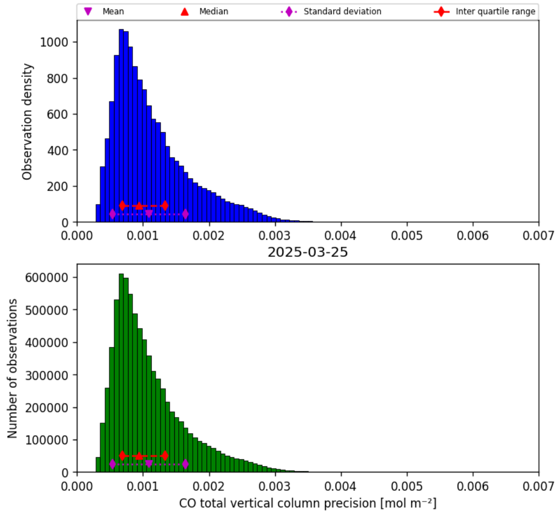
Figure 15: Histogram of “CO total vertical column precision” for 2025-03-25 to 2025-03-26
