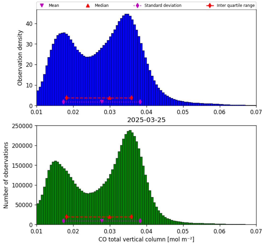
Figure 14: Histogram of “CO total vertical column” for 2025-03-25 to 2025-03-26
