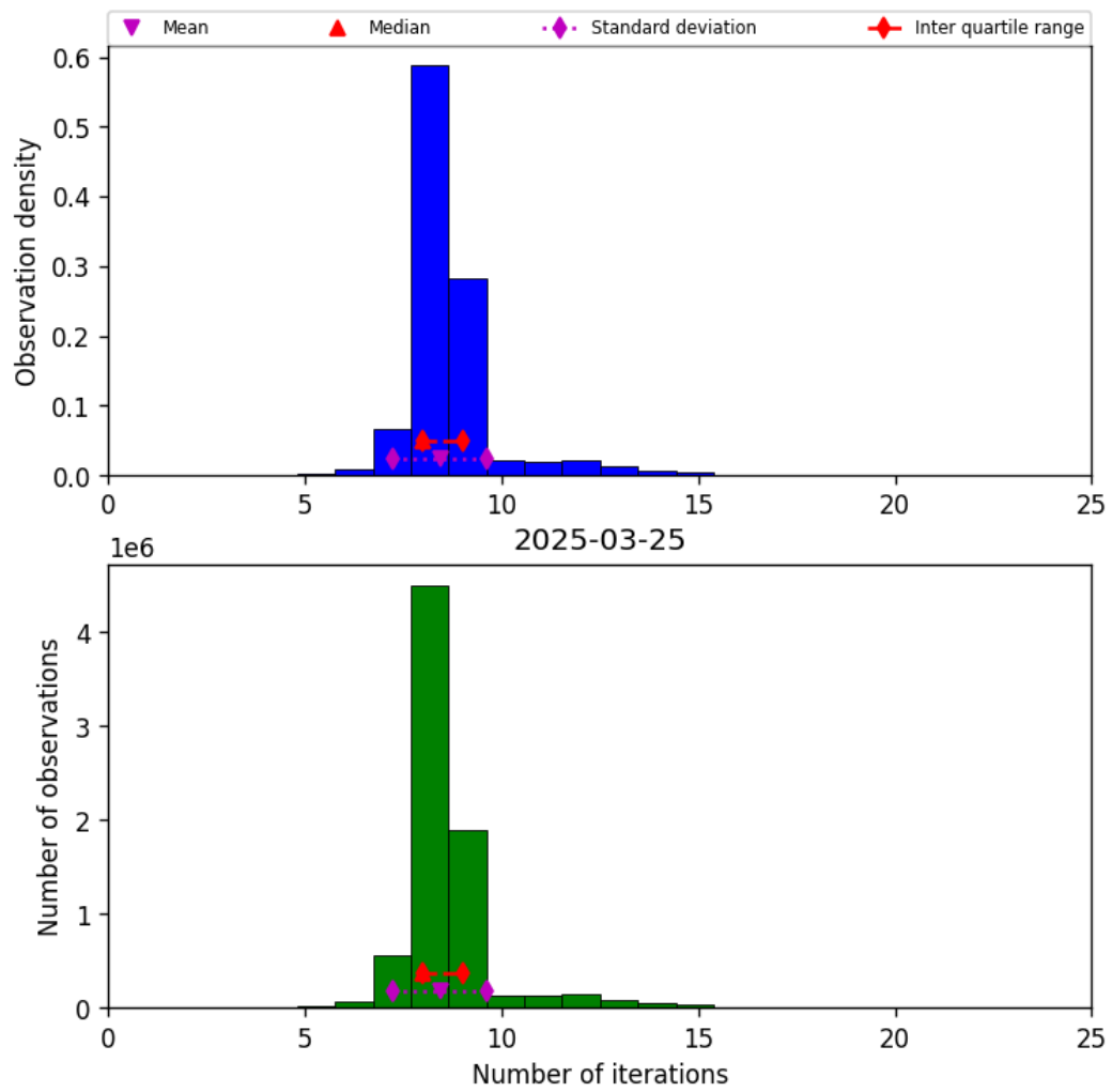
Figure 19: Histogram of “Number of iterations” for 2025-03-25 to 2025-03-26
