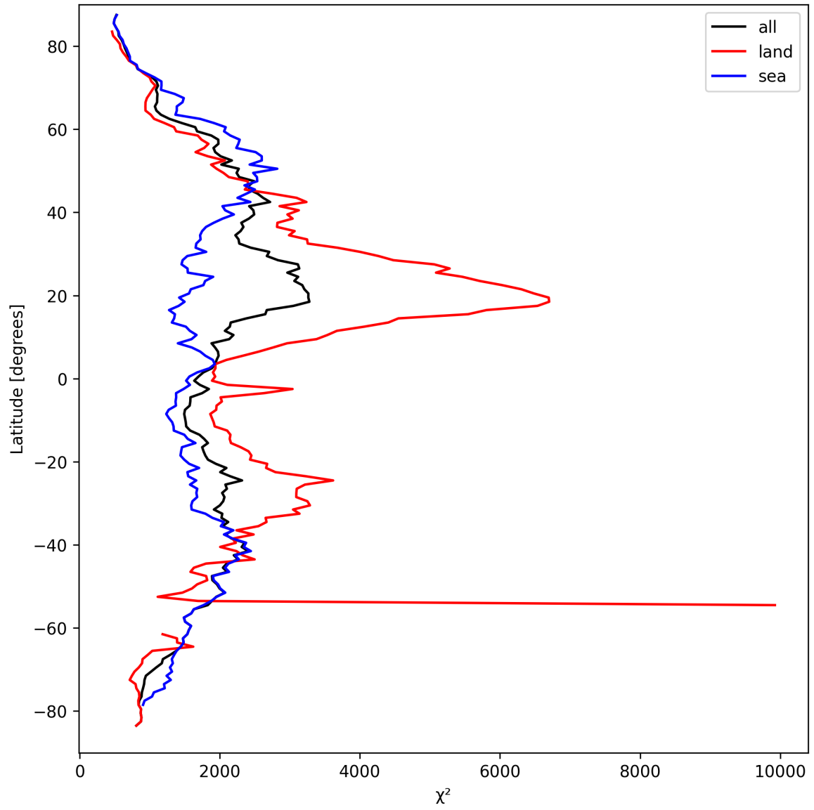
Figure 10: Zonal average of “ \chi^2 ” for 2025-03-25 to 2025-03-26.
