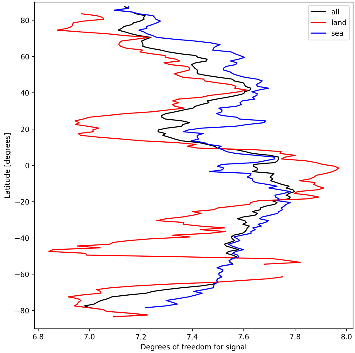
Figure 11: Zonal average of “Degrees of freedom for signal” for 2025-03-25 to 2025-03-26.
