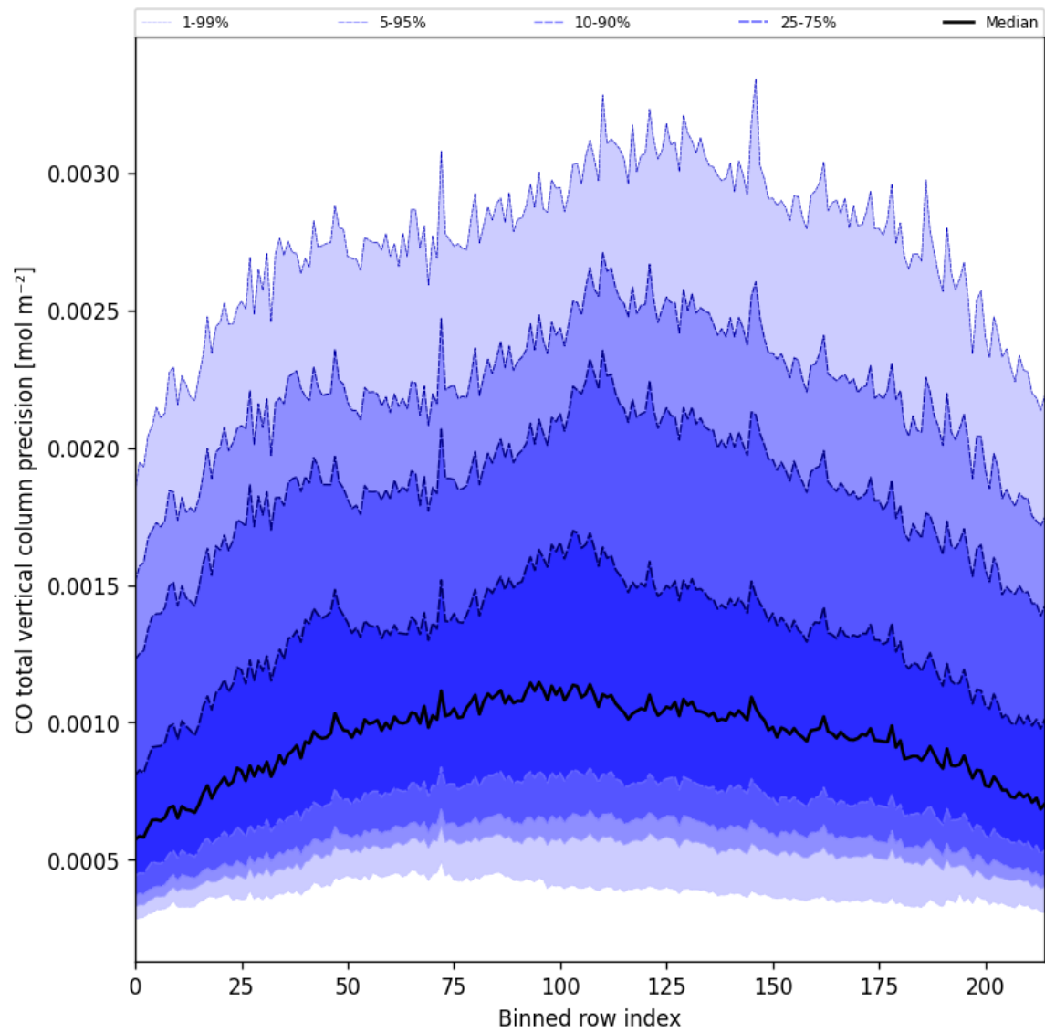
Figure 22: Along track statistics of “CO total vertical column precision” for 2025-03-25 to 2025-03-26
