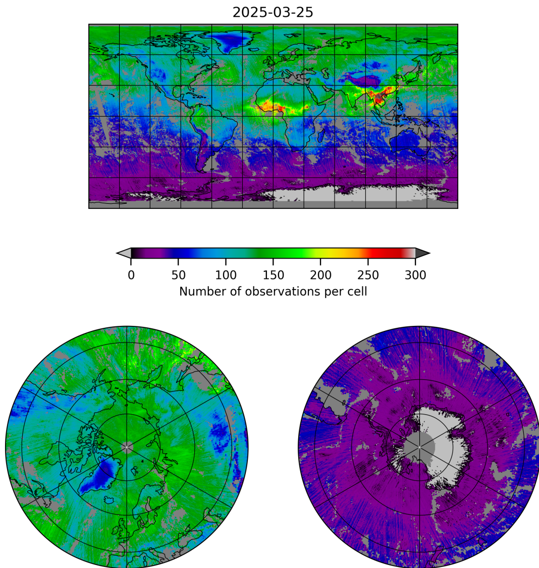
Figure 5: Map of the number of observations for 2025-03-25 to 2025-03-26
