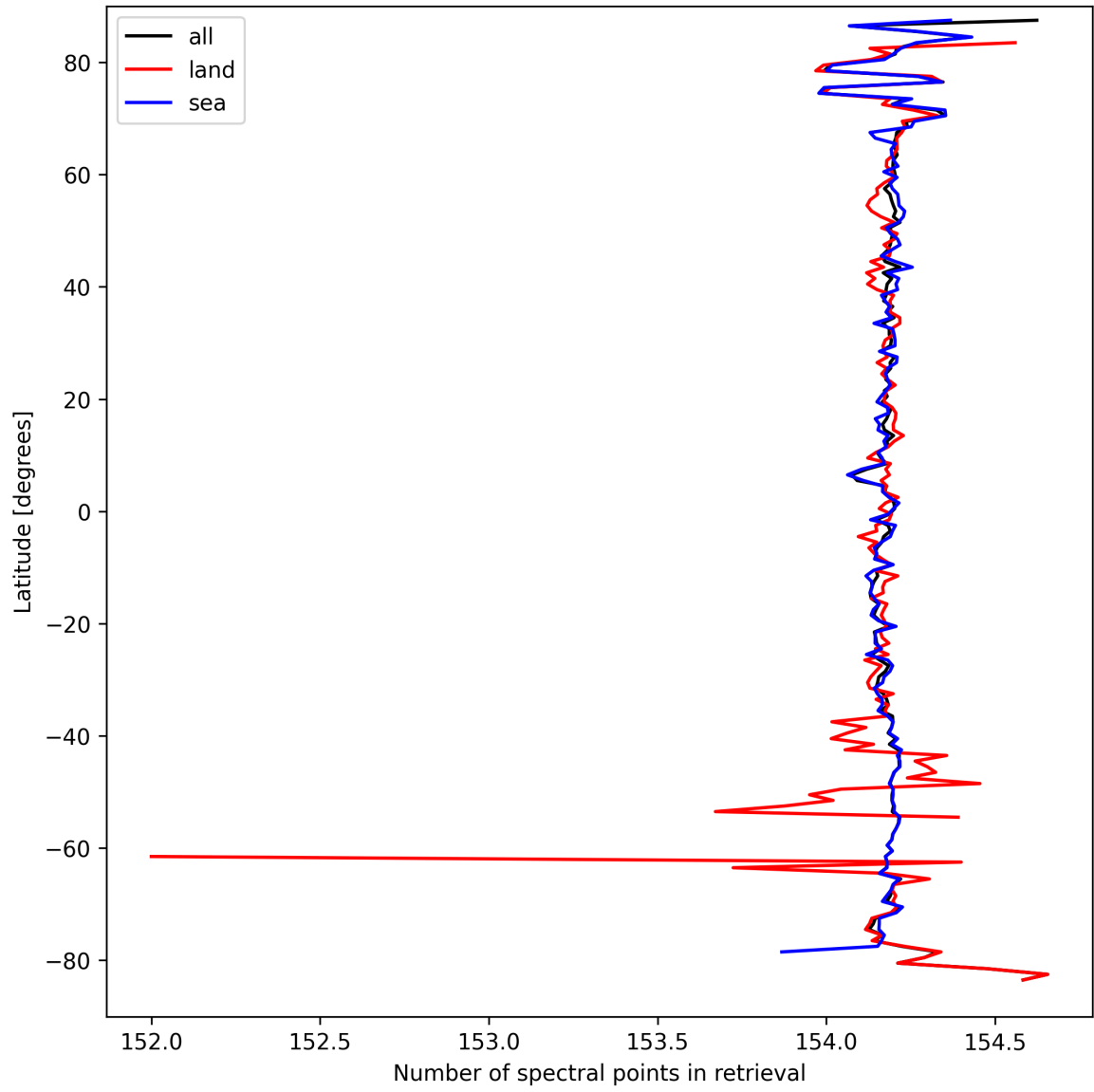
Figure 9: Zonal average of “Number of spectral points in retrieval” for 2025-03-25 to 2025-03-26.
