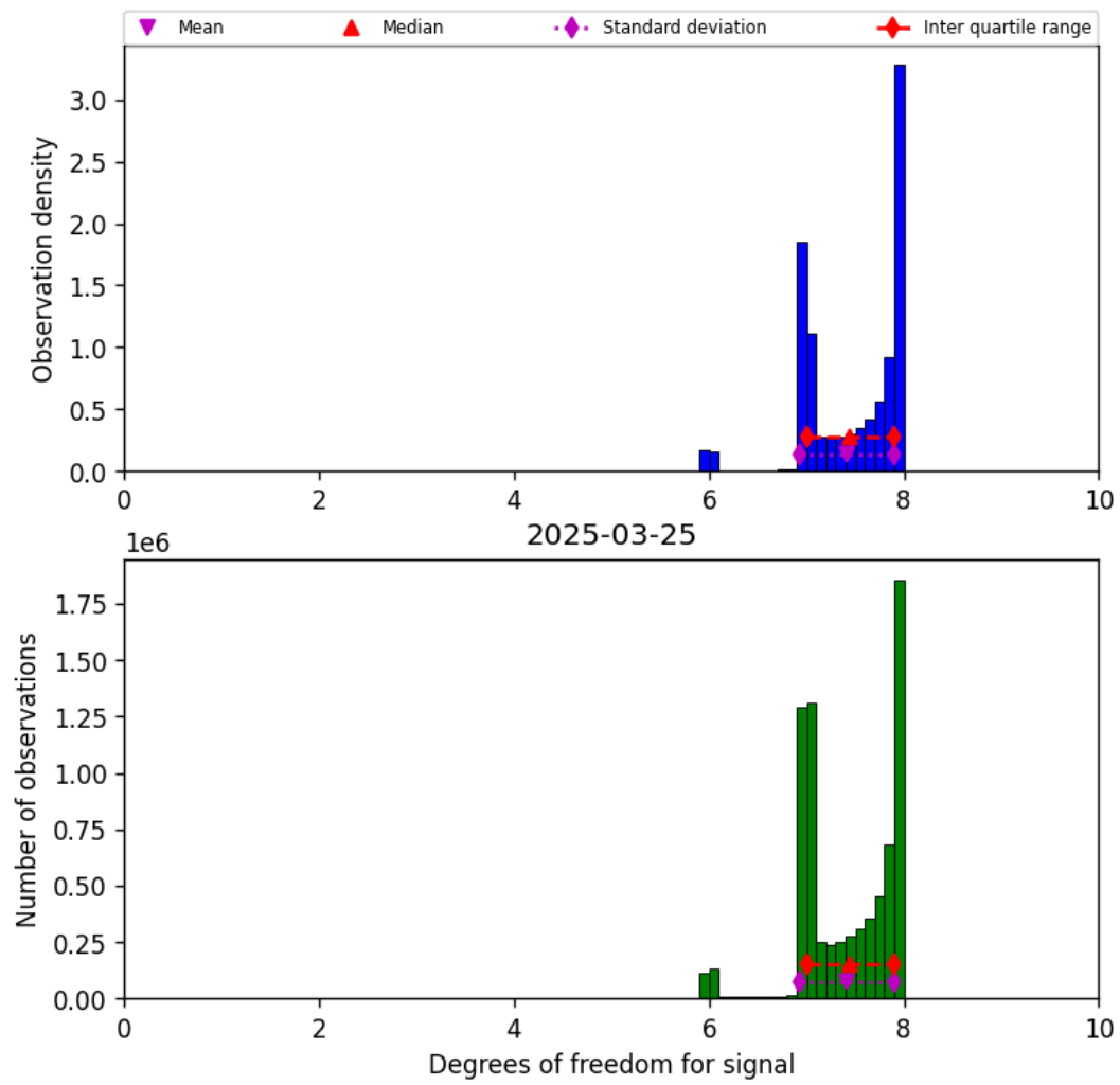
Figure 18: Histogram of “Degrees of freedom for signal” for 2025-03-25 to 2025-03-26
