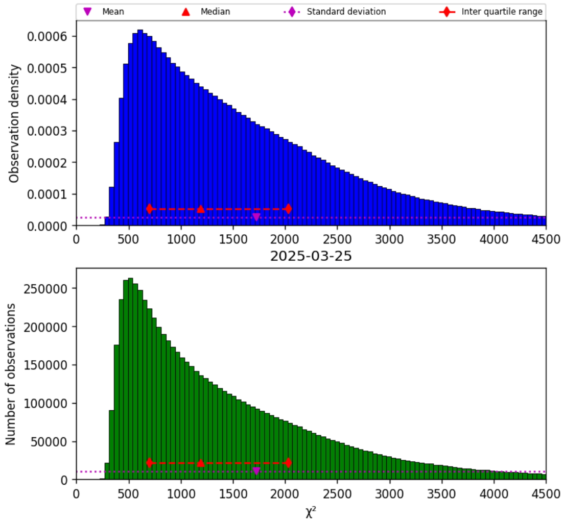
Figure 17: Histogram of “ \chi^2 ” for 2025-03-25 to 2025-03-26
