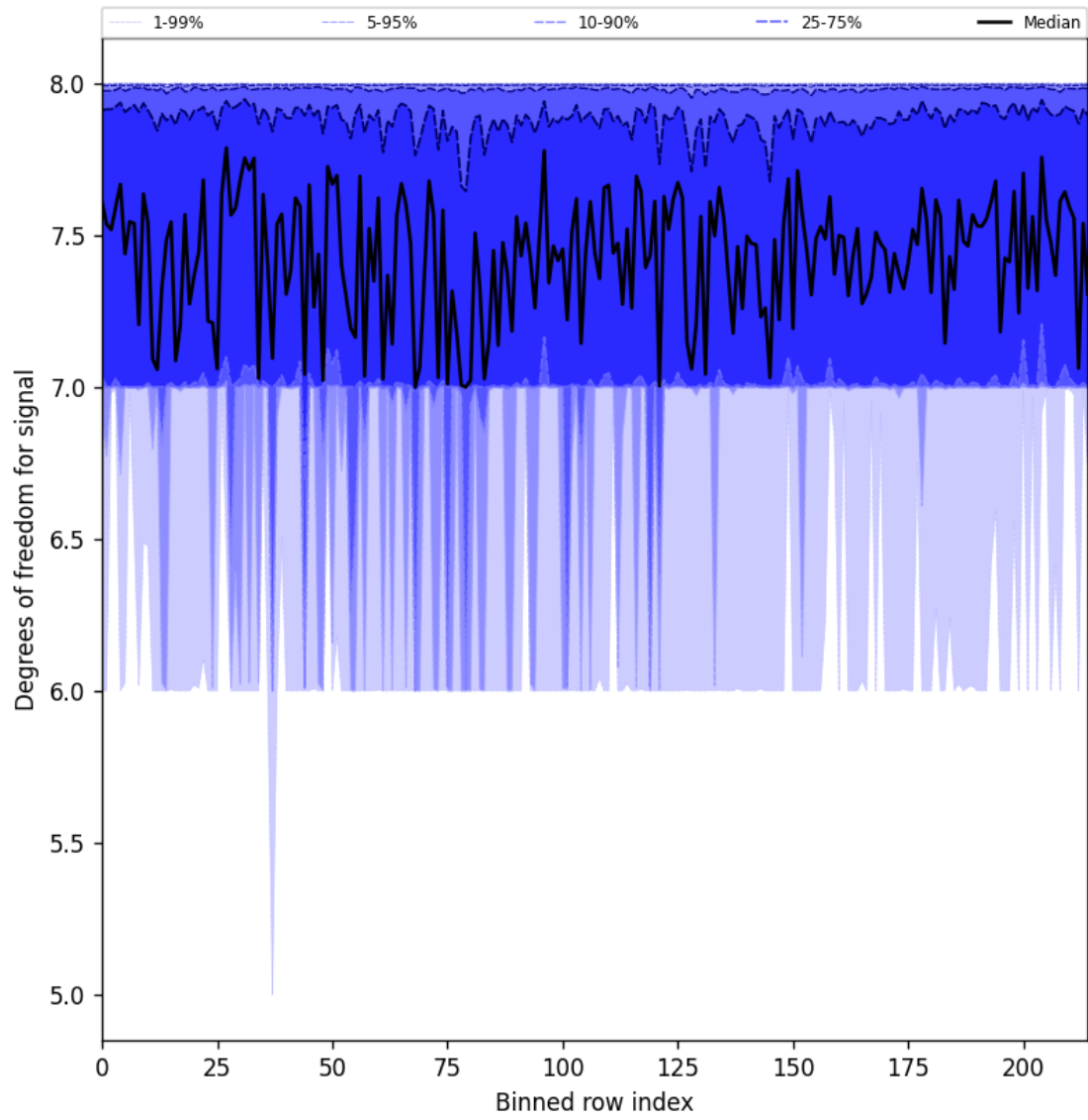
Figure 25: Along track statistics of “Degrees of freedom for signal” for 2025-03-25 to 2025-03-26
