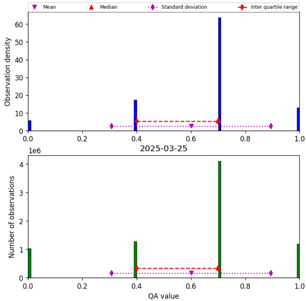
Figure 13: Histogram of “QA value” for 2025-03-25 to 2025-03-26
