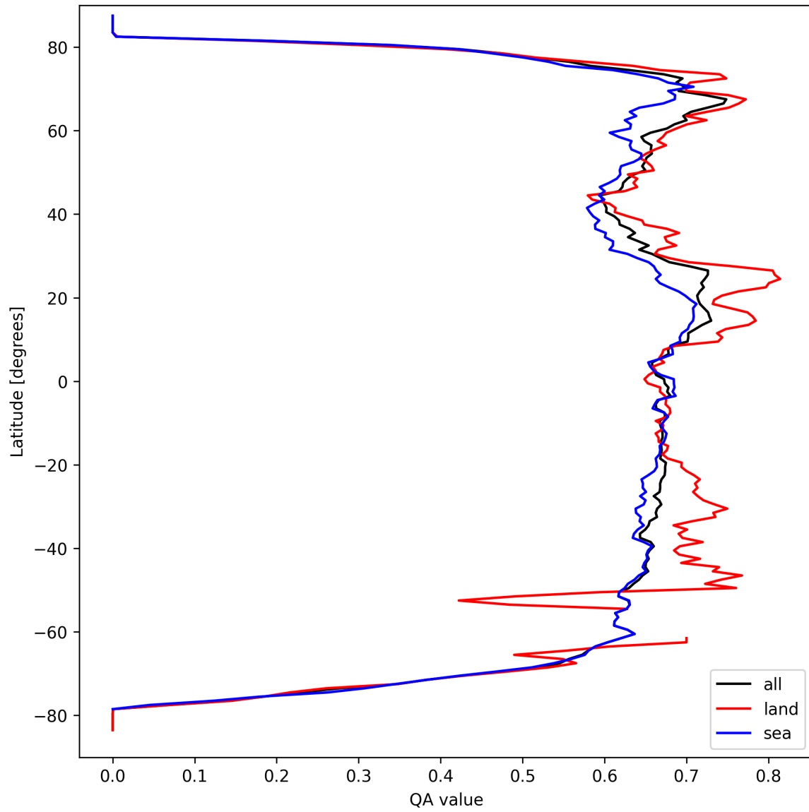
Figure 6: Zonal average of “QA value” for 2025-03-25 to 2025-03-26.
