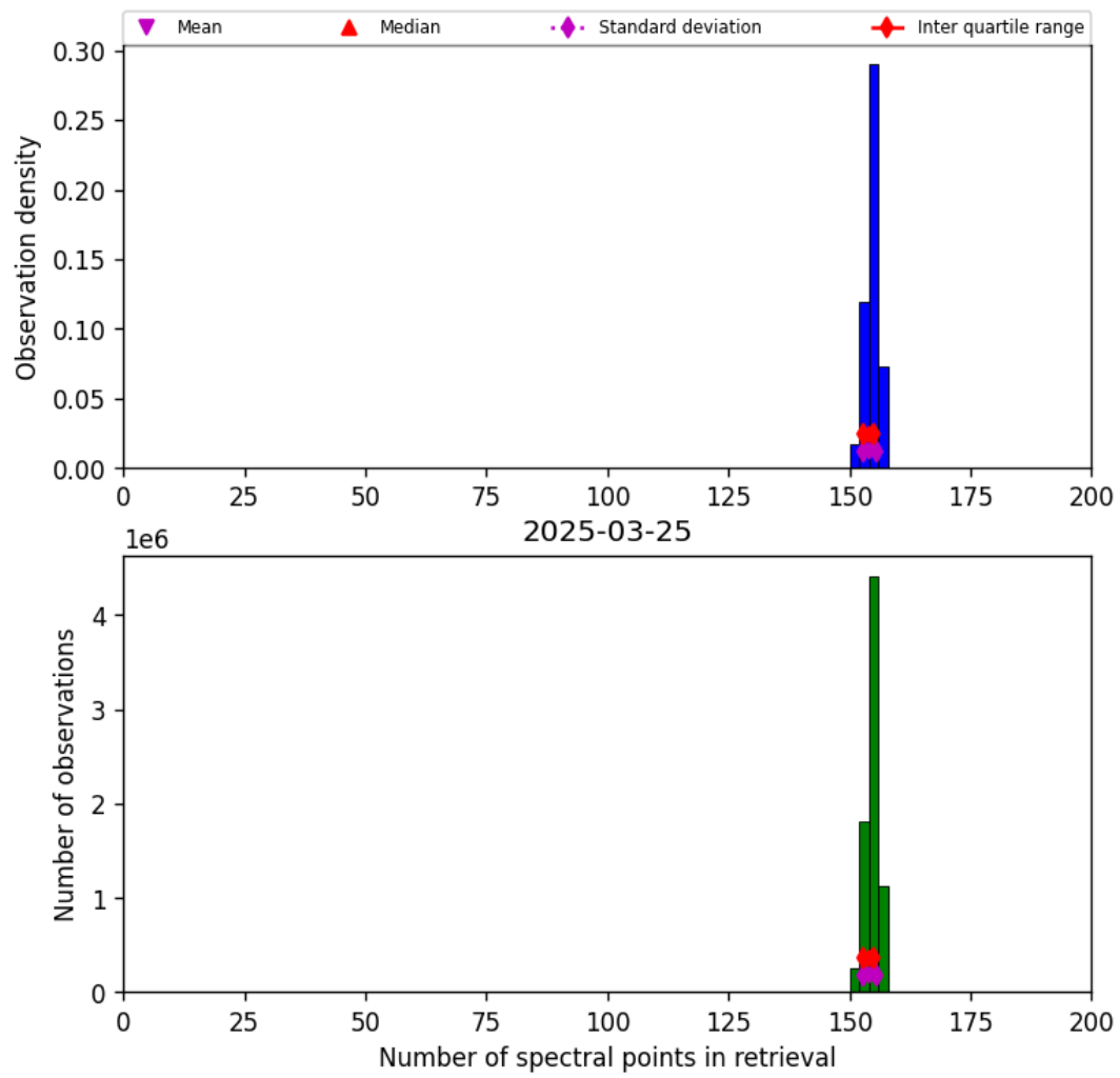
Figure 16: Histogram of “Number of spectral points in retrieval” for 2025-03-25 to 2025-03-26
