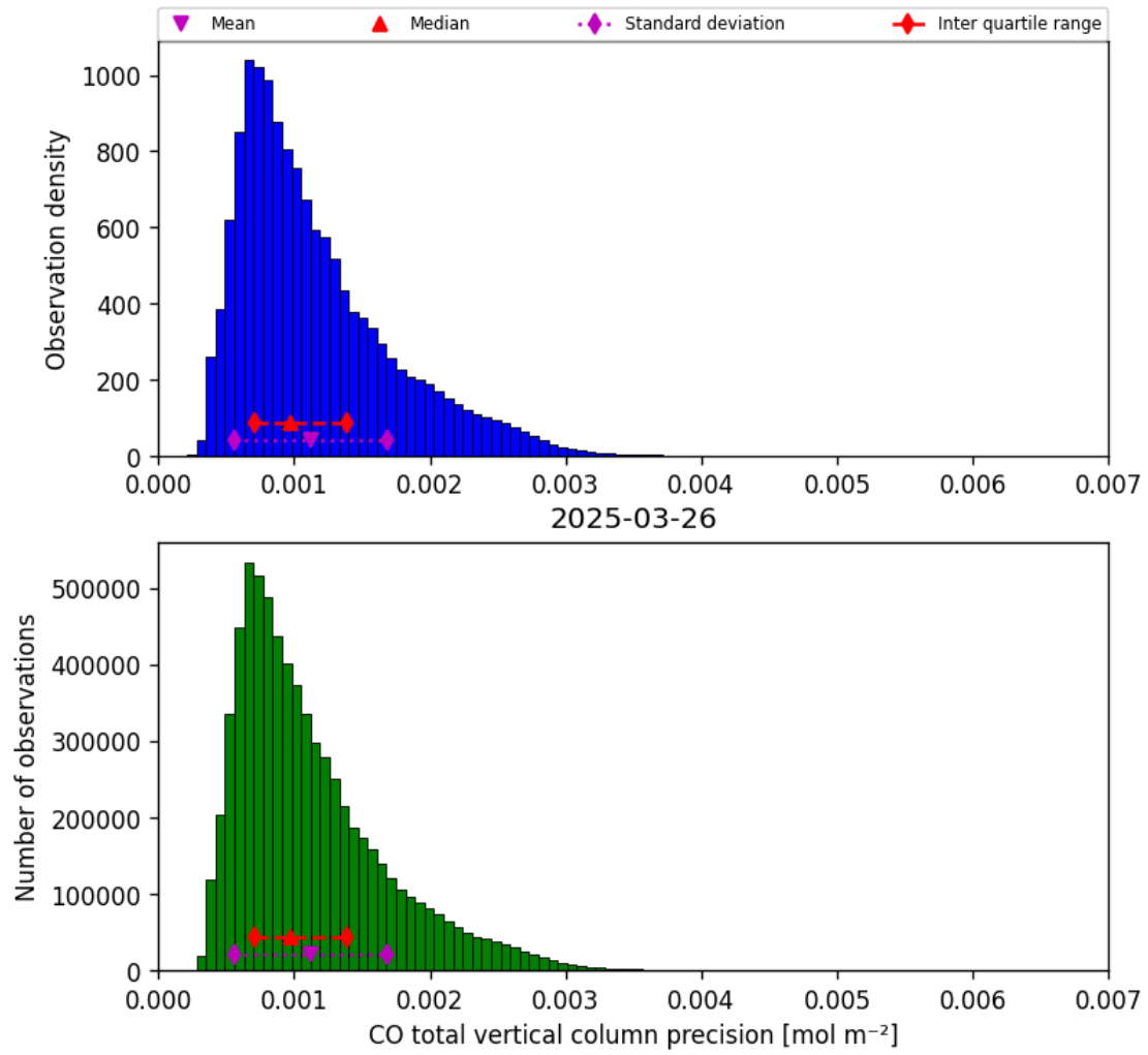
Figure 15: Histogram of “CO total vertical column precision” for 2025-03-26 to 2025-03-26
