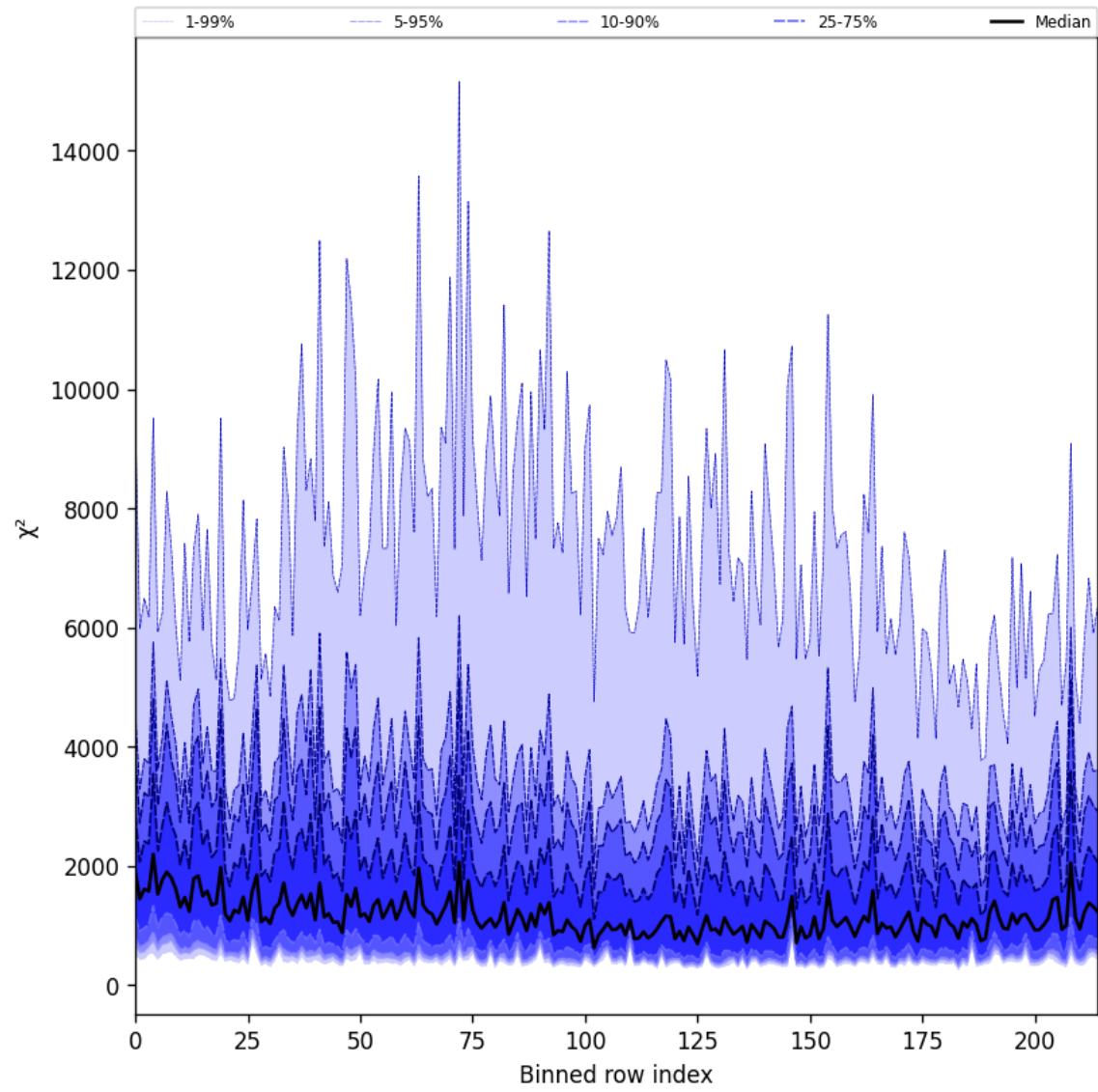
Figure 24: Along track statistics of “ \chi^2 ” for 2025-03-26 to 2025-03-26
