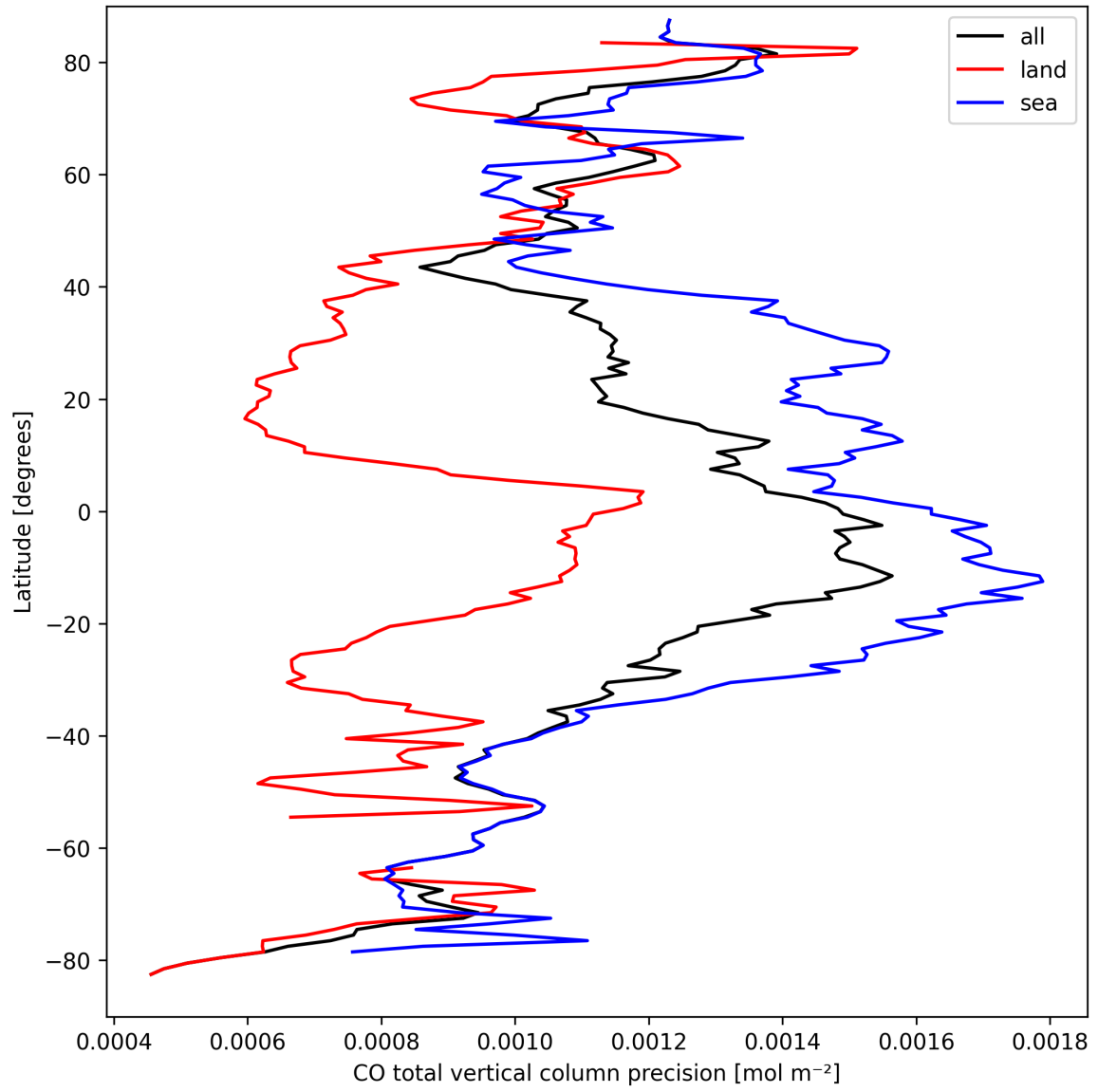
Figure 8: Zonal average of “CO total vertical column precision” for 2025-03-26 to 2025-03-26.
