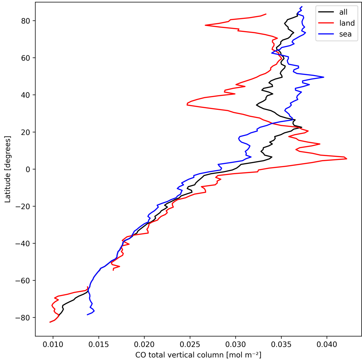
Figure 7: Zonal average of “CO total vertical column” for 2025-03-26 to 2025-03-26.
