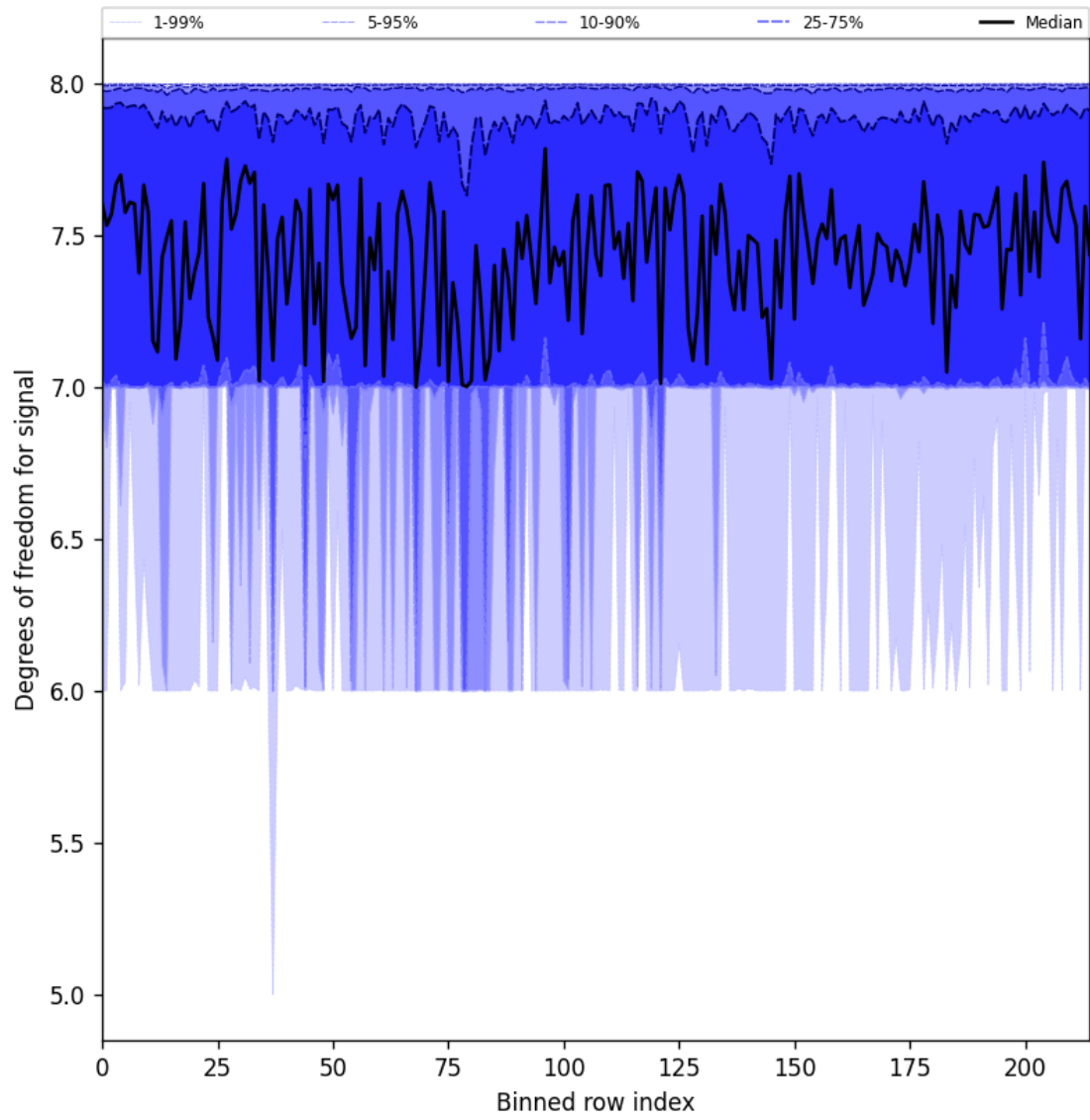
Figure 25: Along track statistics of “Degrees of freedom for signal” for 2025-03-26 to 2025-03-26
