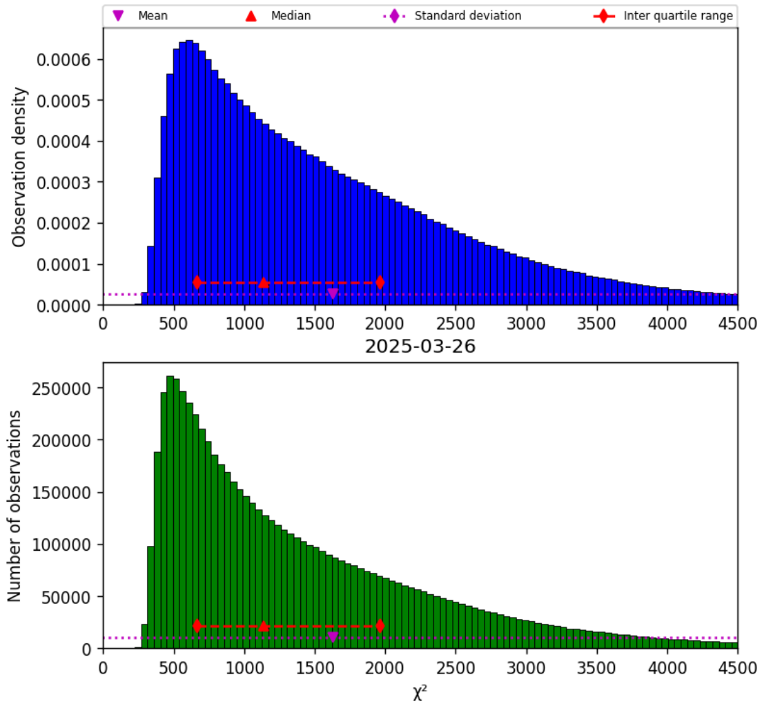
Figure 17: Histogram of “ \chi^2 ” for 2025-03-26 to 2025-03-26
