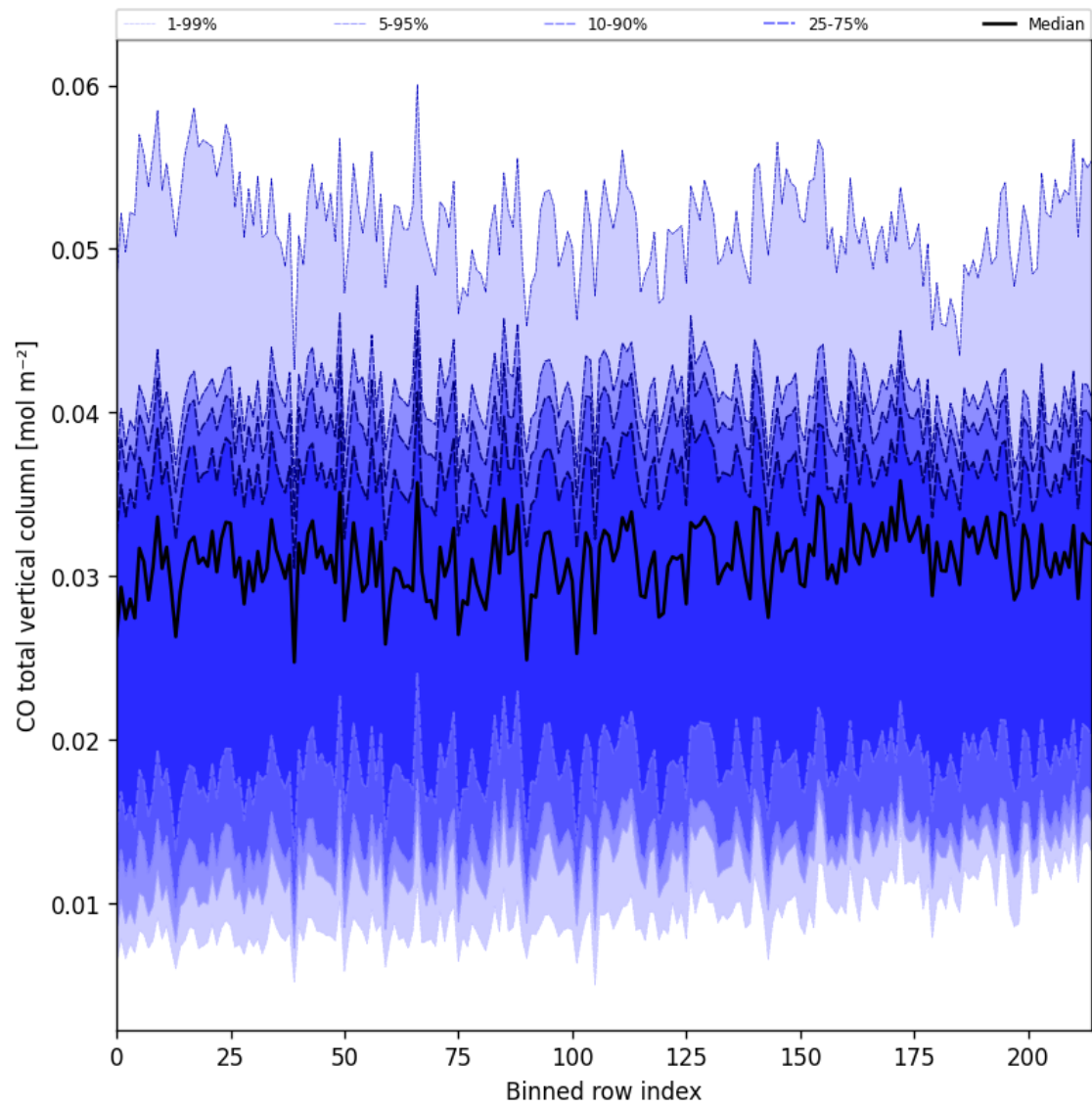
Figure 21: Along track statistics of “CO total vertical column” for 2025-03-26 to 2025-03-26
