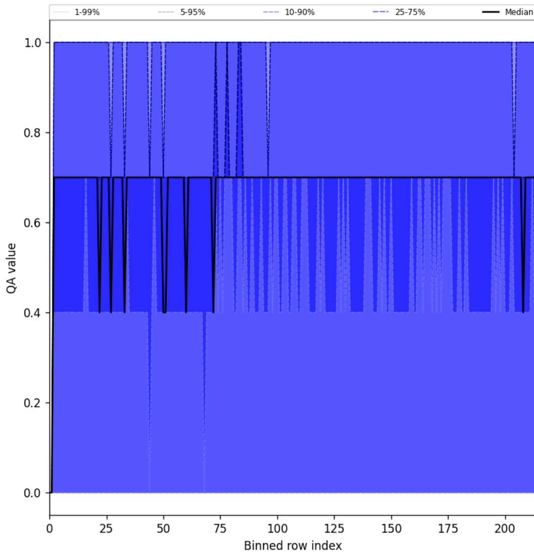
Figure 20: Along track statistics of “QA value” for 2025-03-26 to 2025-03-26
