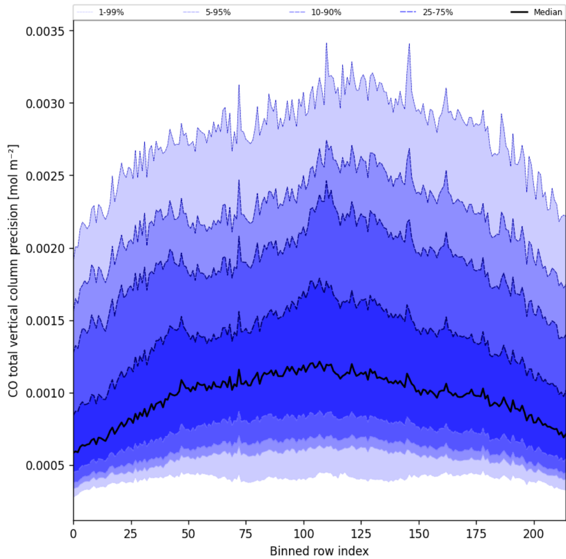
Figure 22: Along track statistics of “CO total vertical column precision” for 2025-03-26 to 2025-03-26
