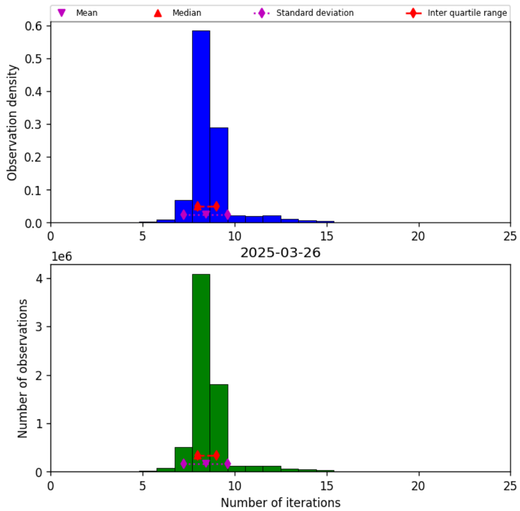
Figure 19: Histogram of “Number of iterations” for 2025-03-26 to 2025-03-26
