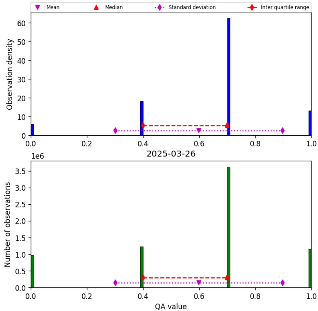
Figure 13: Histogram of “QA value” for 2025-03-26 to 2025-03-26
