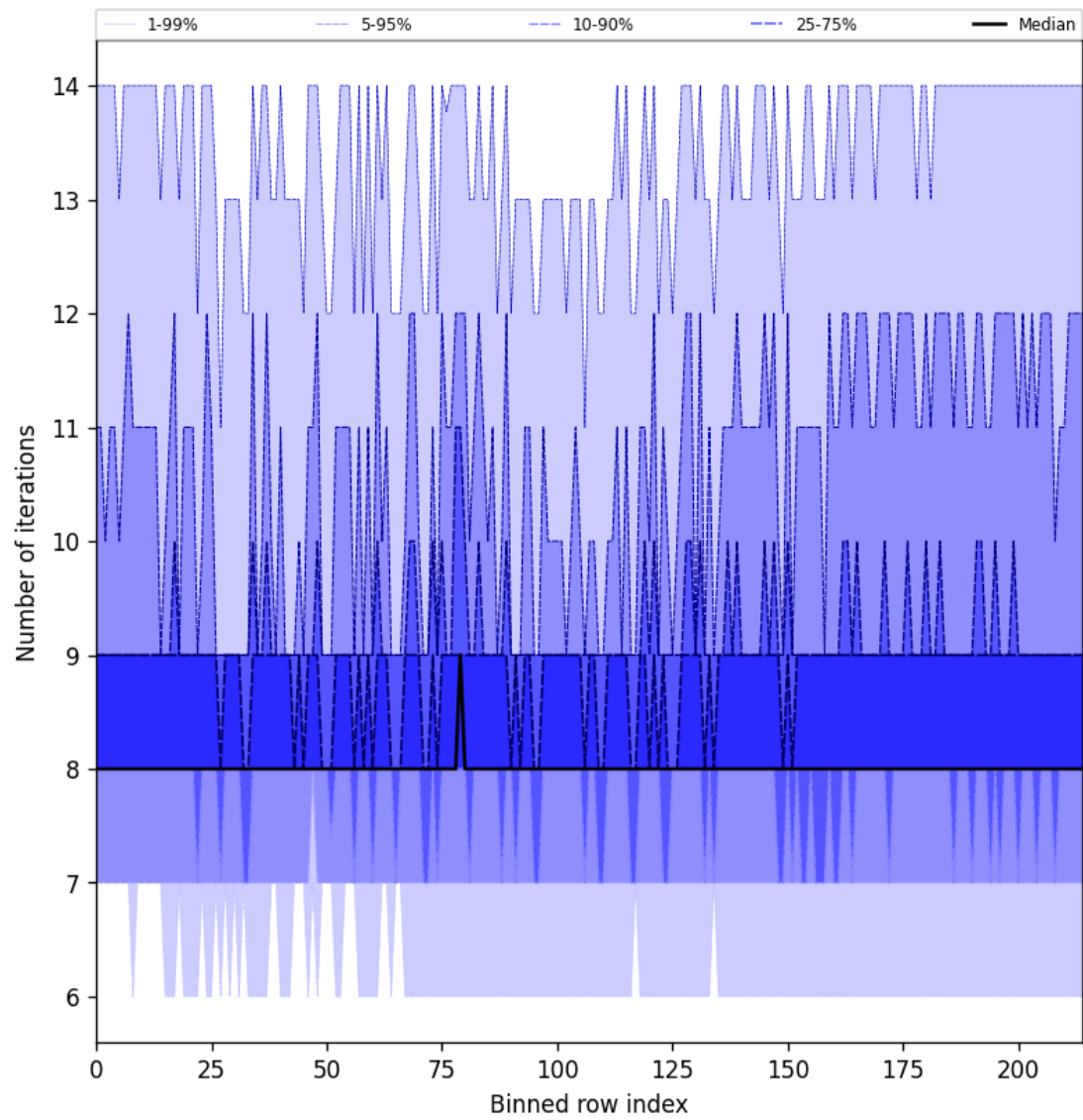
Figure 26: Along track statistics of “Number of iterations” for 2025-03-26 to 2025-03-26
