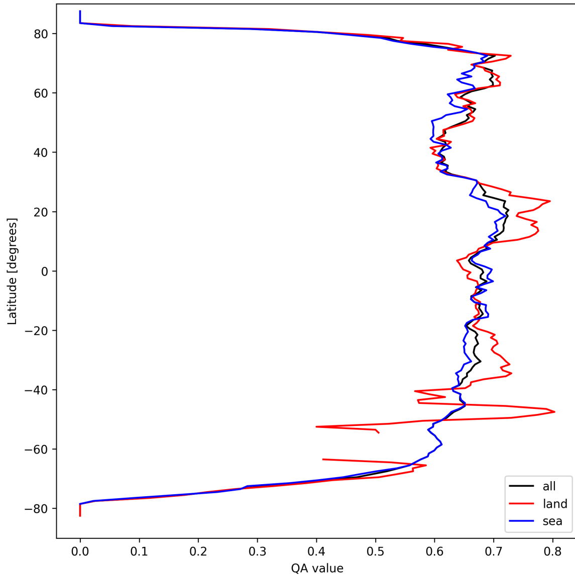
Figure 6: Zonal average of “QA value” for 2025-03-26 to 2025-03-26.
