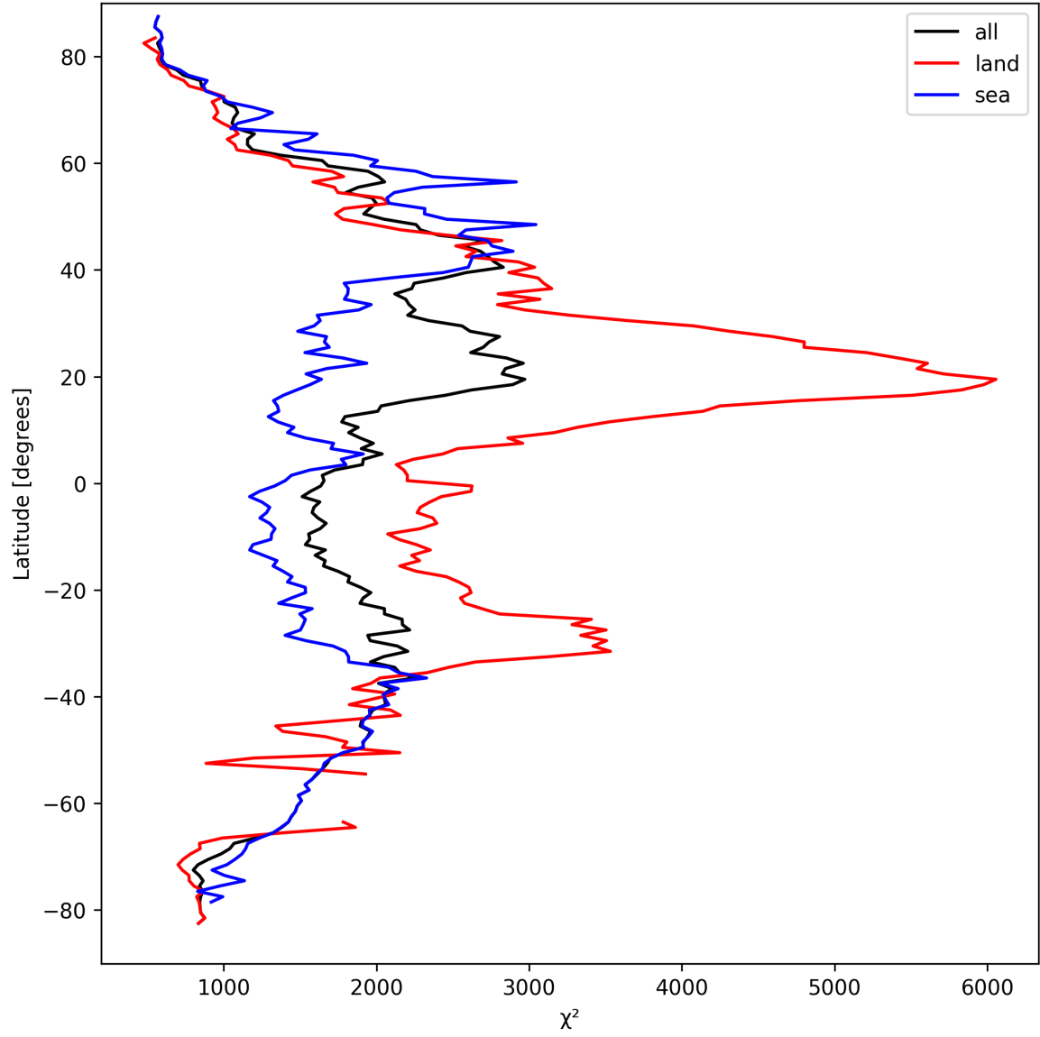
Figure 10: Zonal average of “ \chi^2 ” for 2025-03-26 to 2025-03-26.
