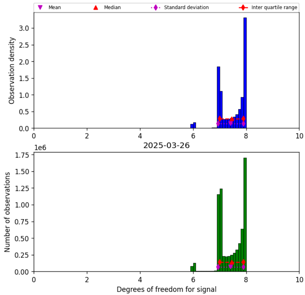
Figure 18: Histogram of “Degrees of freedom for signal” for 2025-03-26 to 2025-03-26
