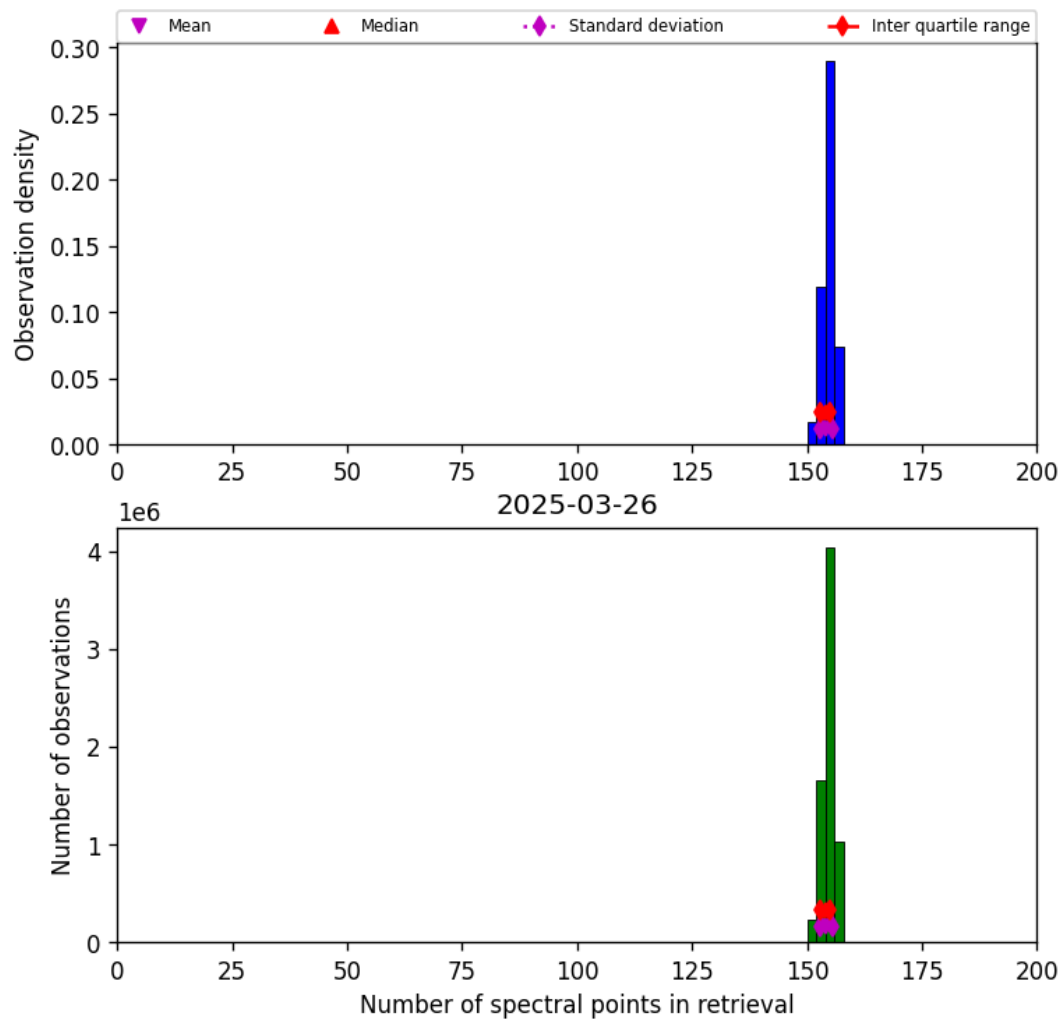
Figure 16: Histogram of “Number of spectral points in retrieval” for 2025-03-26 to 2025-03-26
