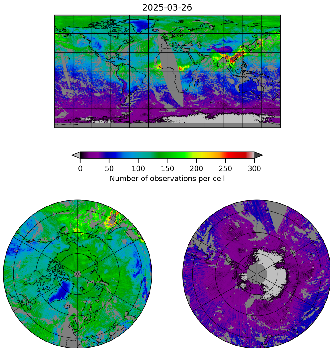
Figure 5: Map of the number of observations for 2025-03-26 to 2025-03-26
