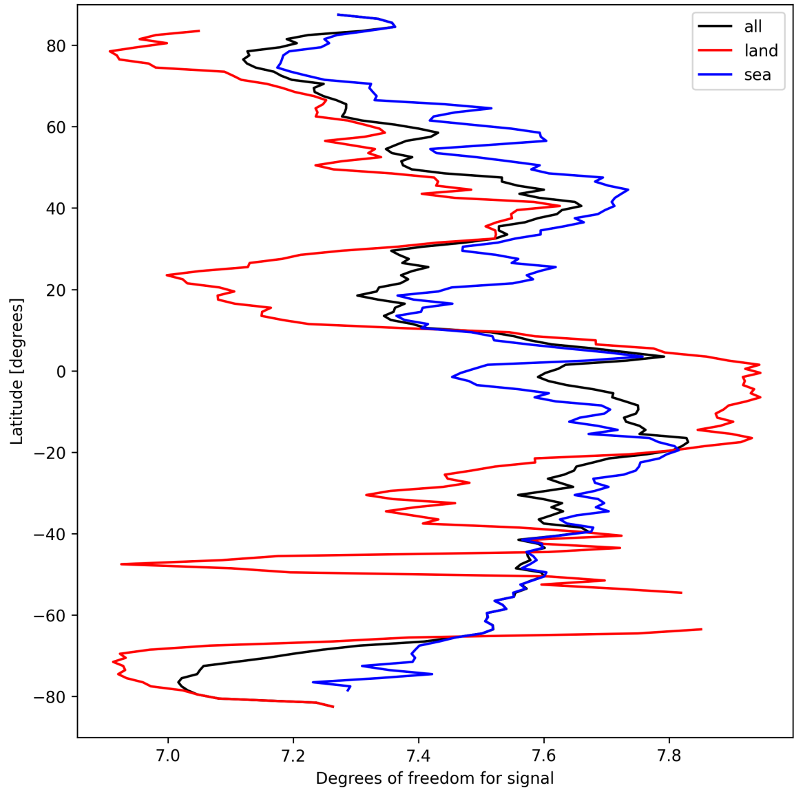
Figure 11: Zonal average of “Degrees of freedom for signal” for 2025-03-26 to 2025-03-26.
