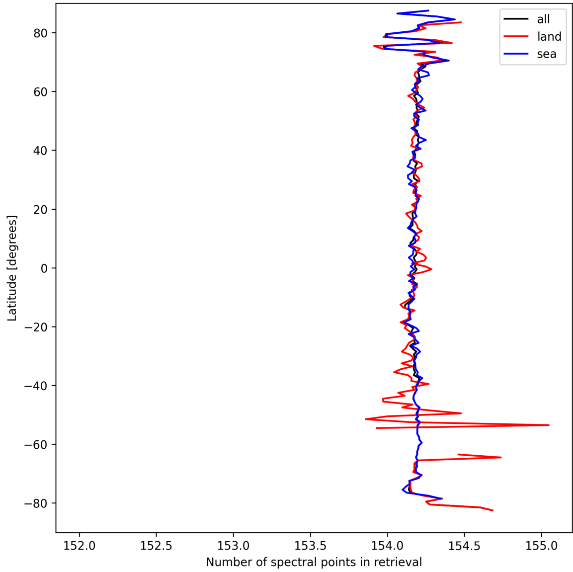
Figure 9: Zonal average of “Number of spectral points in retrieval” for 2025-03-26 to 2025-03-26.
