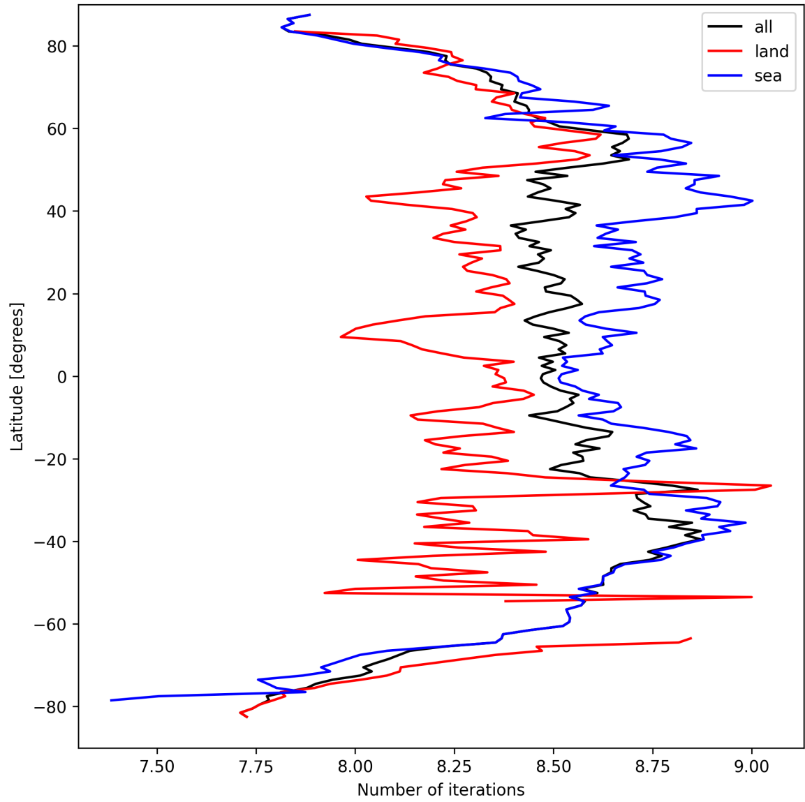
Figure 12: Zonal average of “Number of iterations” for 2025-03-26 to 2025-03-26.
