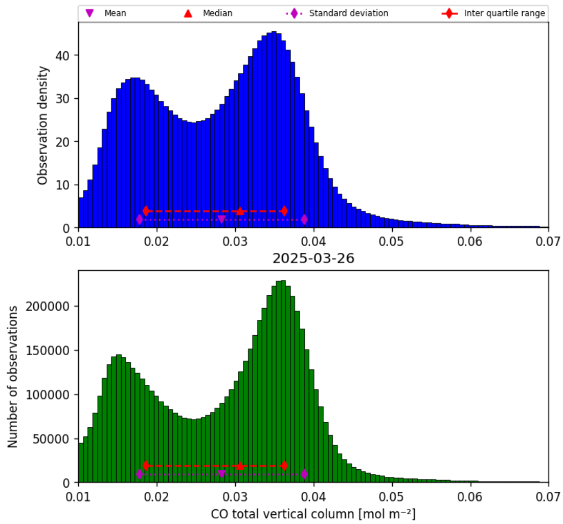
Figure 14: Histogram of “CO total vertical column” for 2025-03-26 to 2025-03-26
