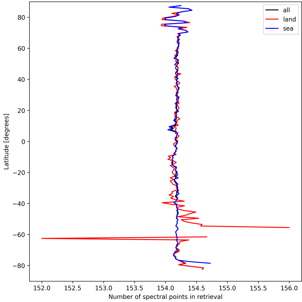
Figure 9: Zonal average of “Number of spectral points in retrieval” for 2025-03-27 to 2025-03-28.
