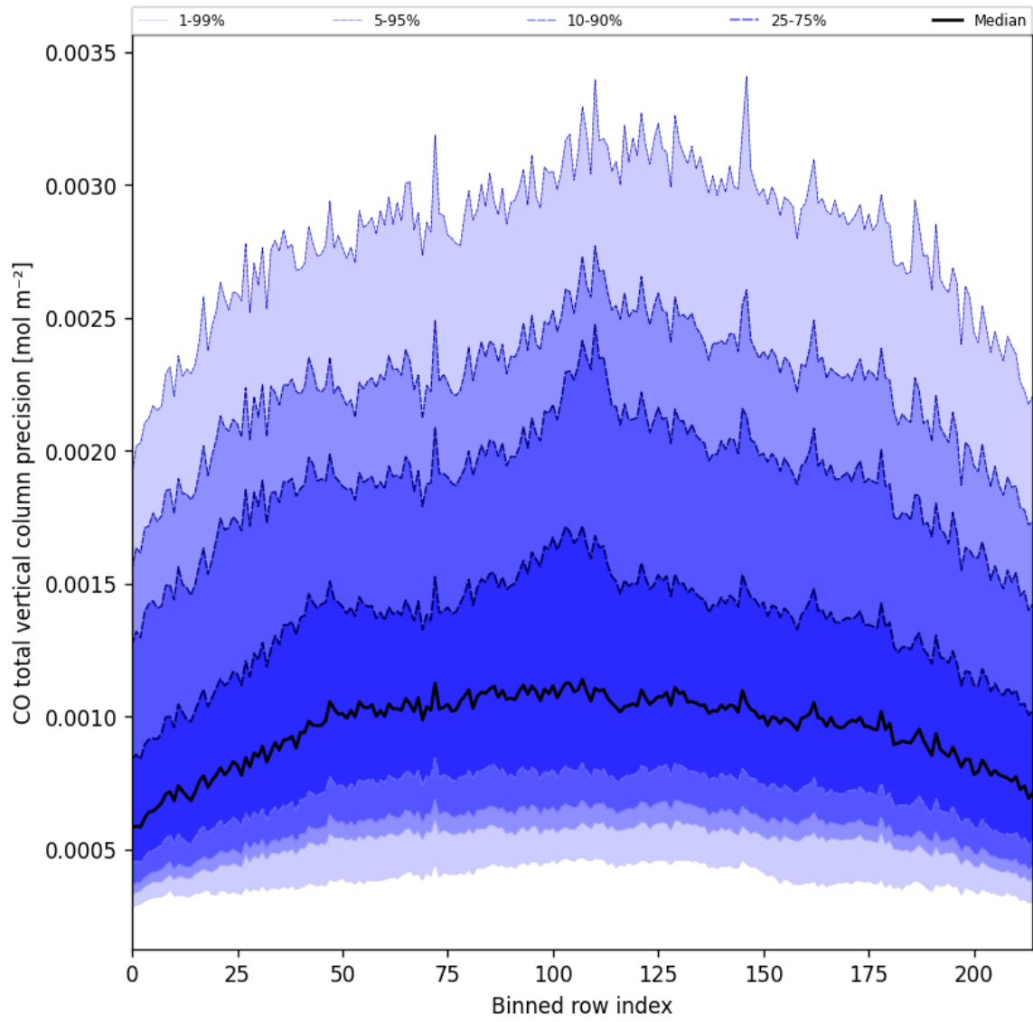
Figure 22: Along track statistics of “CO total vertical column precision” for 2025-03-27 to 2025-03-28
