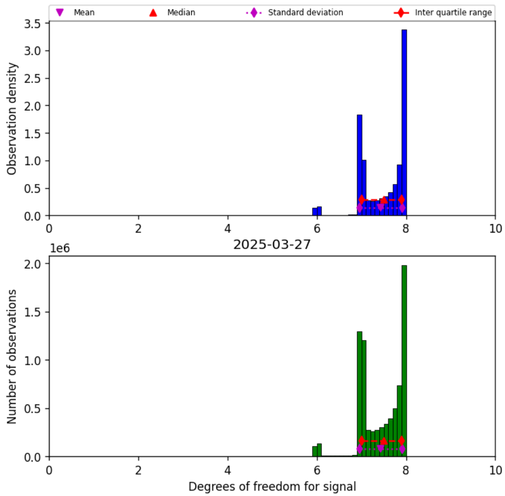
Figure 18: Histogram of “Degrees of freedom for signal” for 2025-03-27 to 2025-03-28
