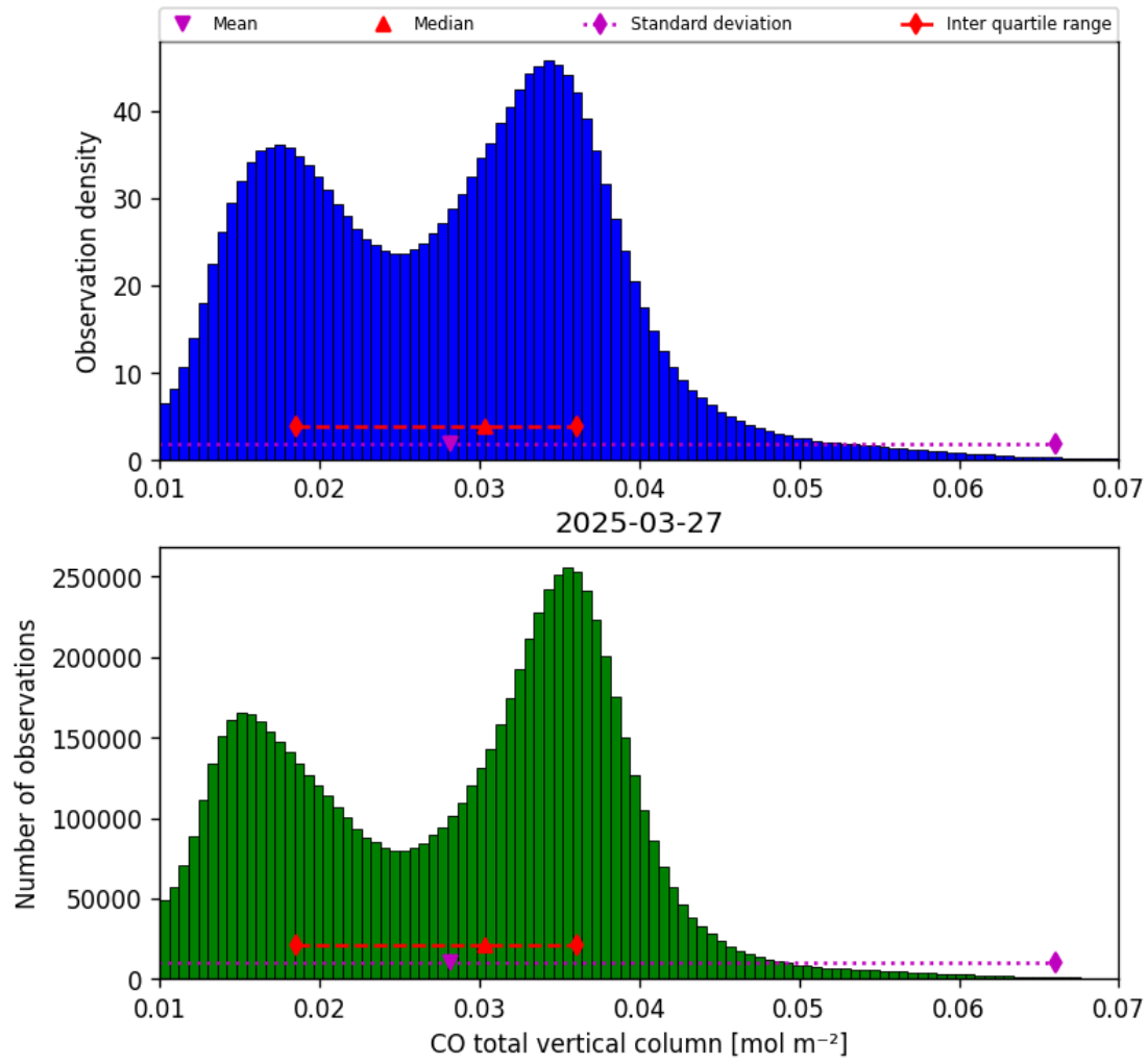
Figure 14: Histogram of “CO total vertical column” for 2025-03-27 to 2025-03-28
