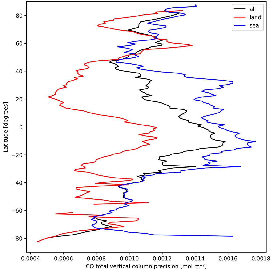
Figure 8: Zonal average of “CO total vertical column precision” for 2025-03-27 to 2025-03-28.
