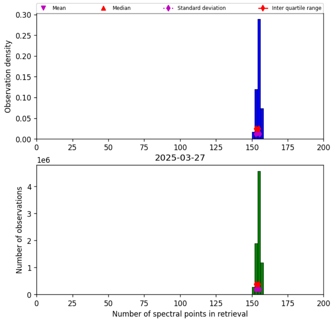
Figure 16: Histogram of “Number of spectral points in retrieval” for 2025-03-27 to 2025-03-28
