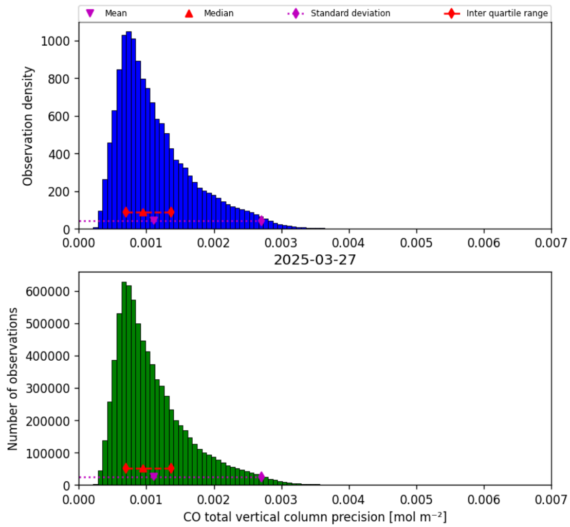
Figure 15: Histogram of “CO total vertical column precision” for 2025-03-27 to 2025-03-28
