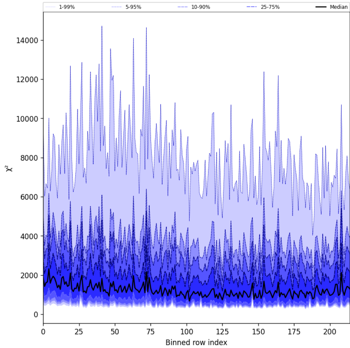
Figure 24: Along track statistics of “ \chi^2 ” for 2025-03-27 to 2025-03-28
