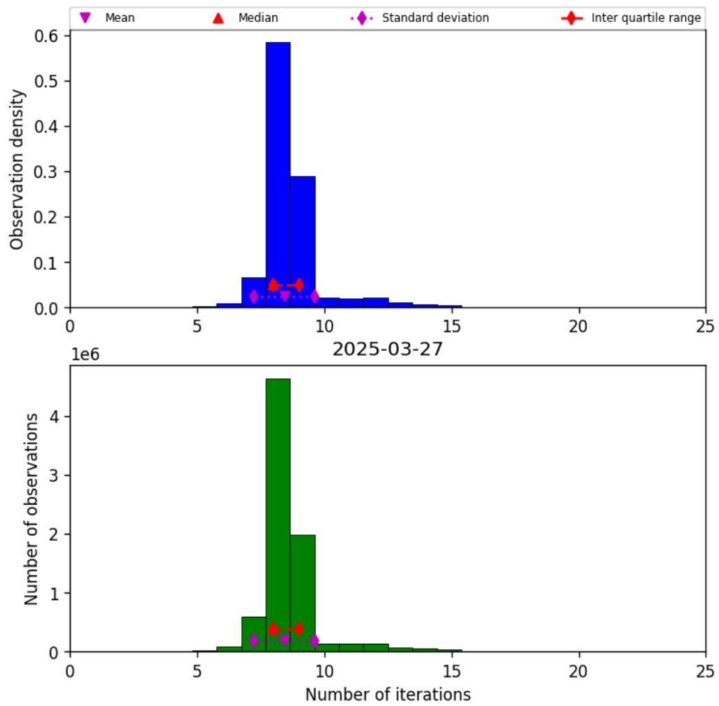
Figure 19: Histogram of “Number of iterations” for 2025-03-27 to 2025-03-28
