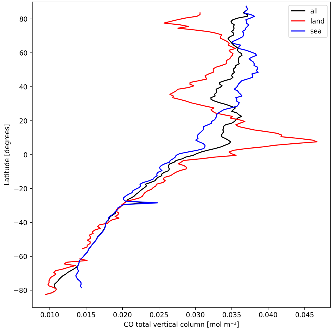
Figure 7: Zonal average of “CO total vertical column” for 2025-03-27 to 2025-03-28.
