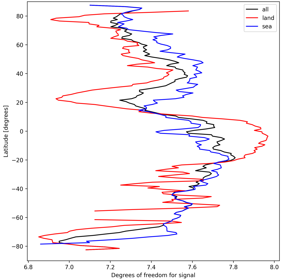
Figure 11: Zonal average of “Degrees of freedom for signal” for 2025-03-27 to 2025-03-28.
