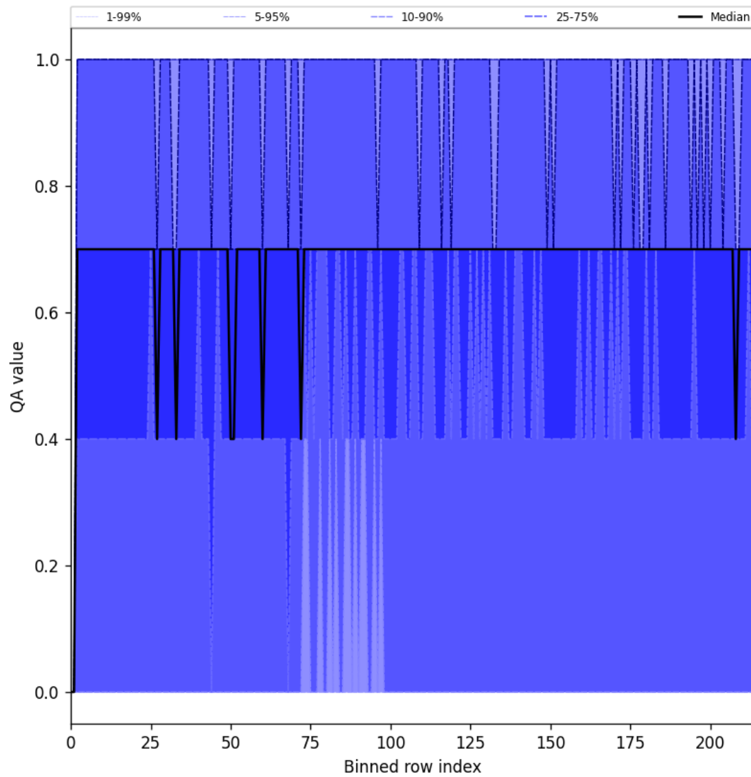
Figure 20: Along track statistics of “QA value” for 2025-03-27 to 2025-03-28
