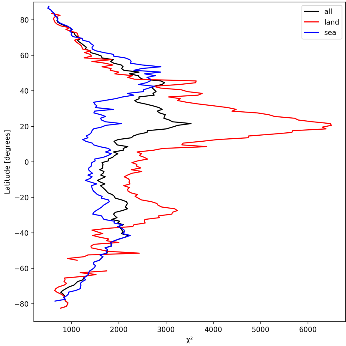
Figure 10: Zonal average of “ \chi^2 ” for 2025-03-27 to 2025-03-28.
