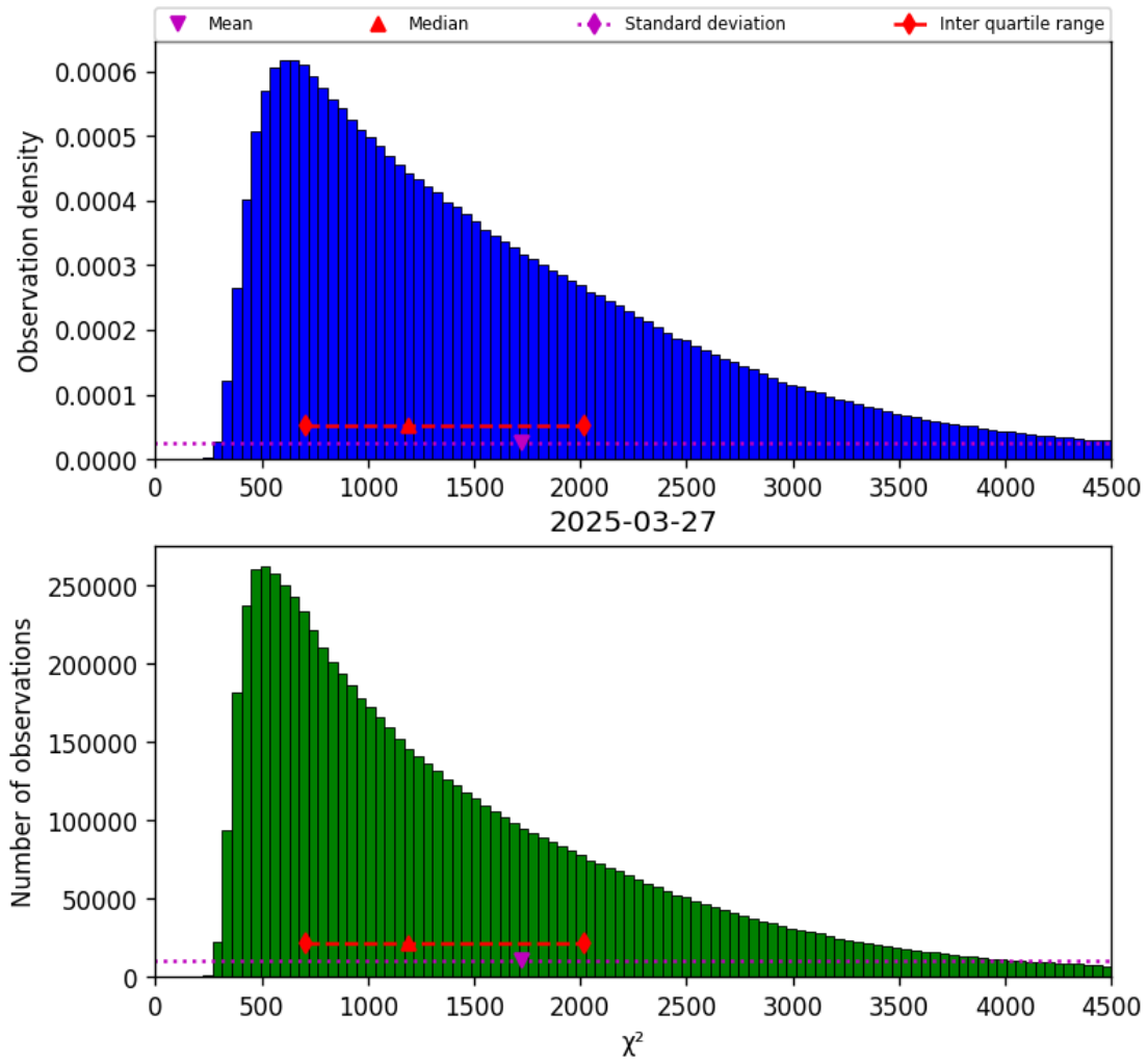
Figure 17: Histogram of “ \chi^2 ” for 2025-03-27 to 2025-03-28
