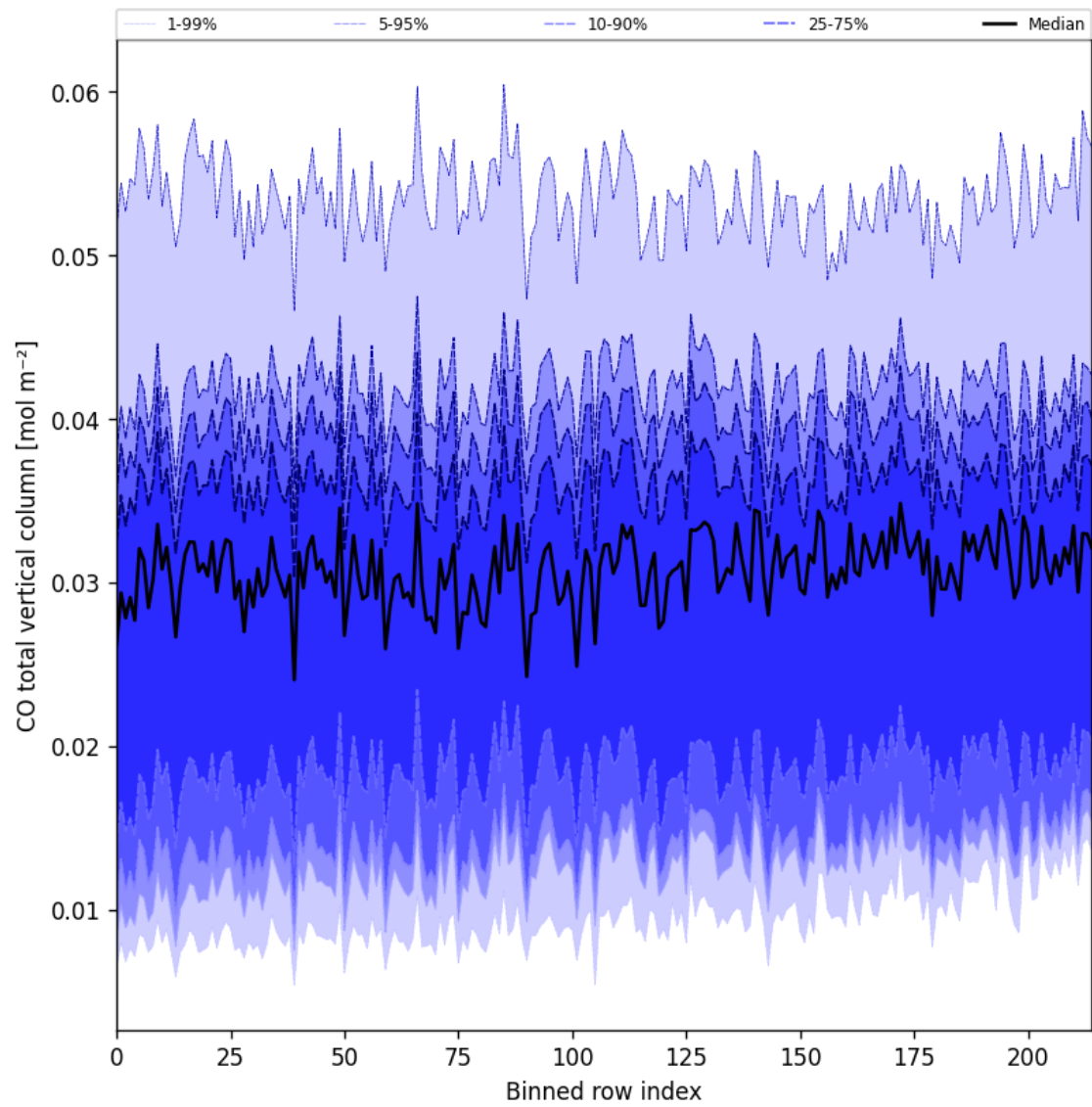
Figure 21: Along track statistics of “CO total vertical column” for 2025-03-27 to 2025-03-28
