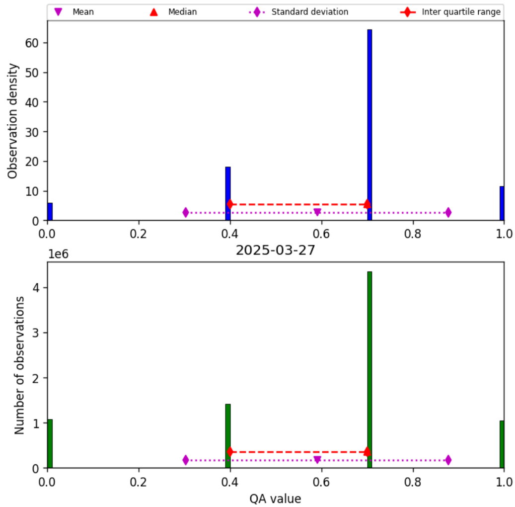
Figure 13: Histogram of “QA value” for 2025-03-27 to 2025-03-28
