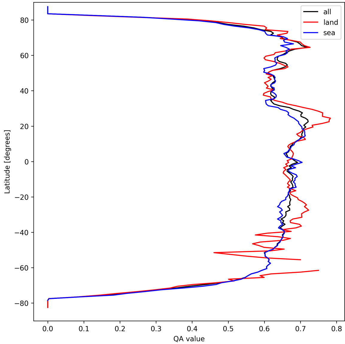
Figure 6: Zonal average of “QA value” for 2025-03-27 to 2025-03-28.
