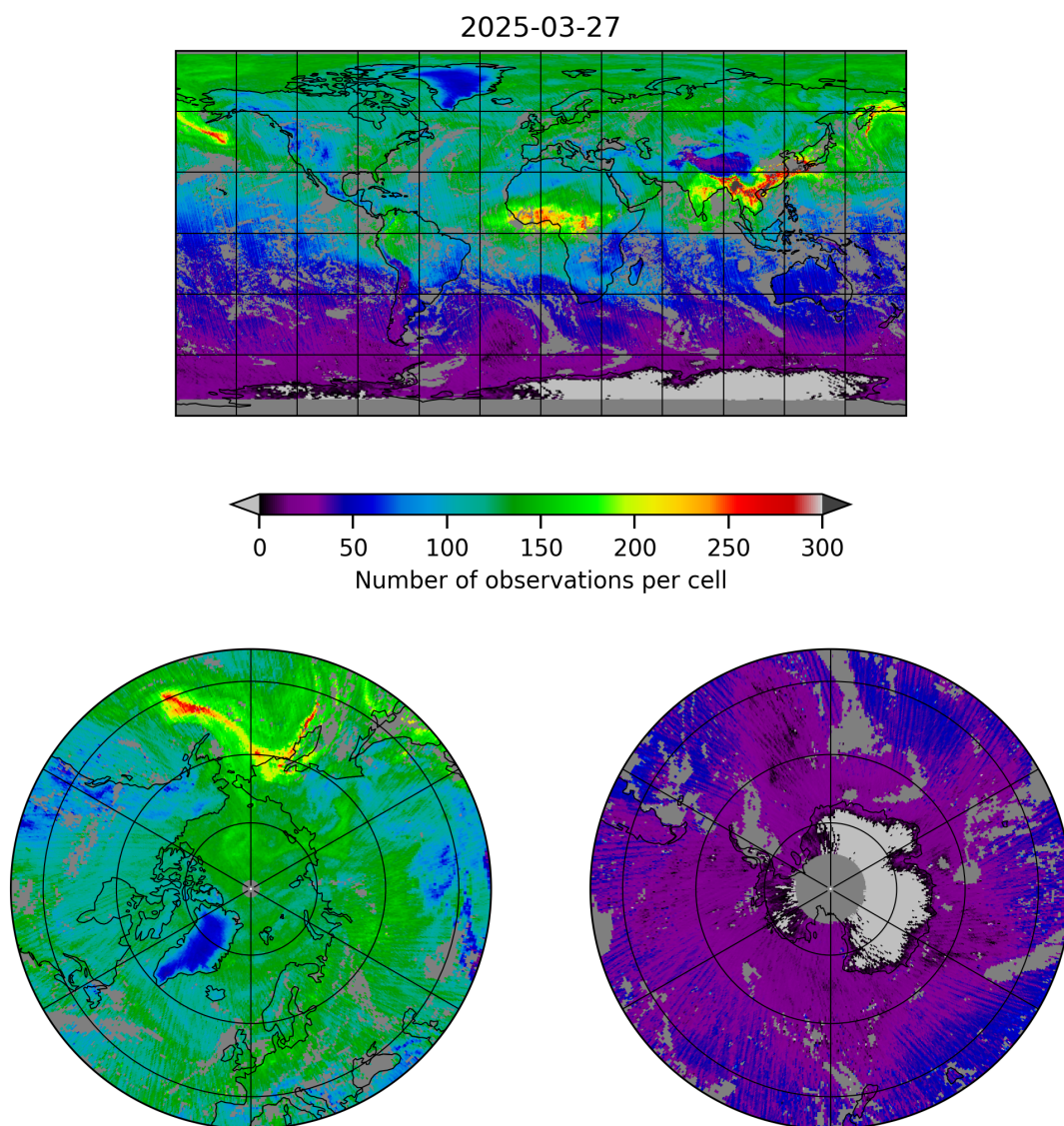
Figure 5: Map of the number of observations for 2025-03-27 to 2025-03-28
