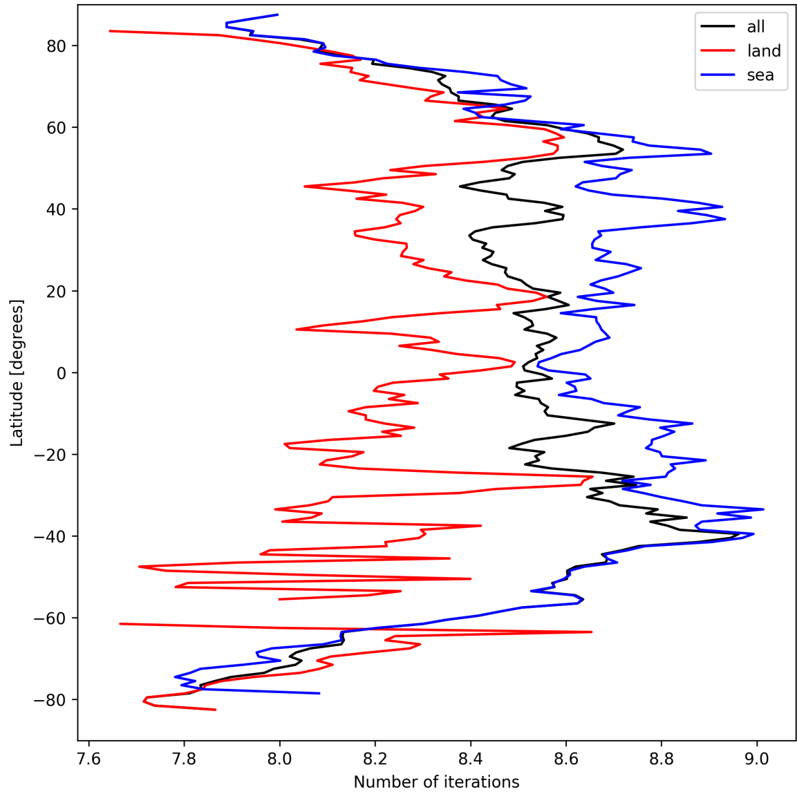
Figure 12: Zonal average of “Number of iterations” for 2025-03-27 to 2025-03-28.
