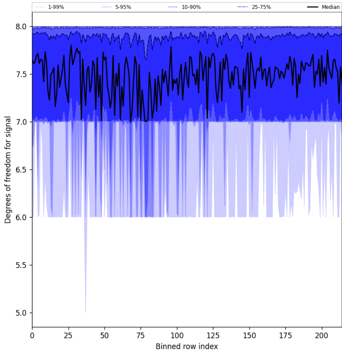
Figure 25: Along track statistics of “Degrees of freedom for signal” for 2025-03-27 to 2025-03-28
