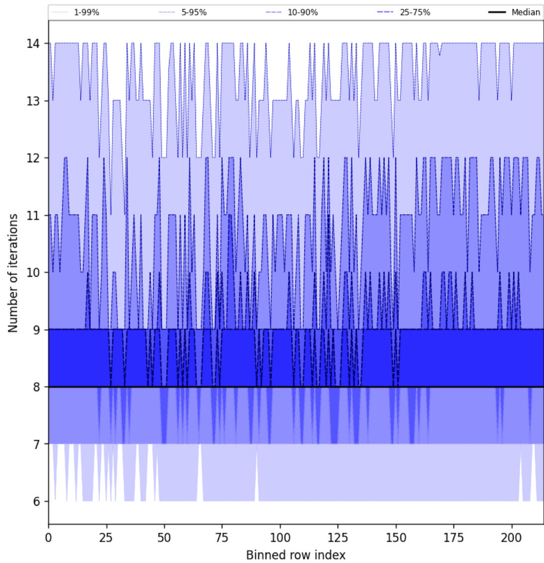
Figure 26: Along track statistics of “Number of iterations” for 2025-03-27 to 2025-03-28
