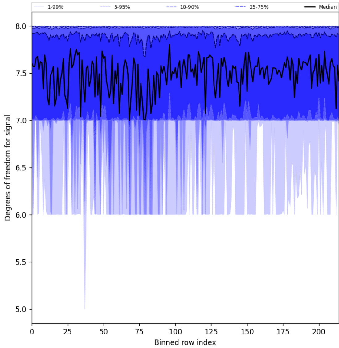
Figure 25: Along track statistics of “Degrees of freedom for signal” for 2025-03-28 to 2025-03-29
