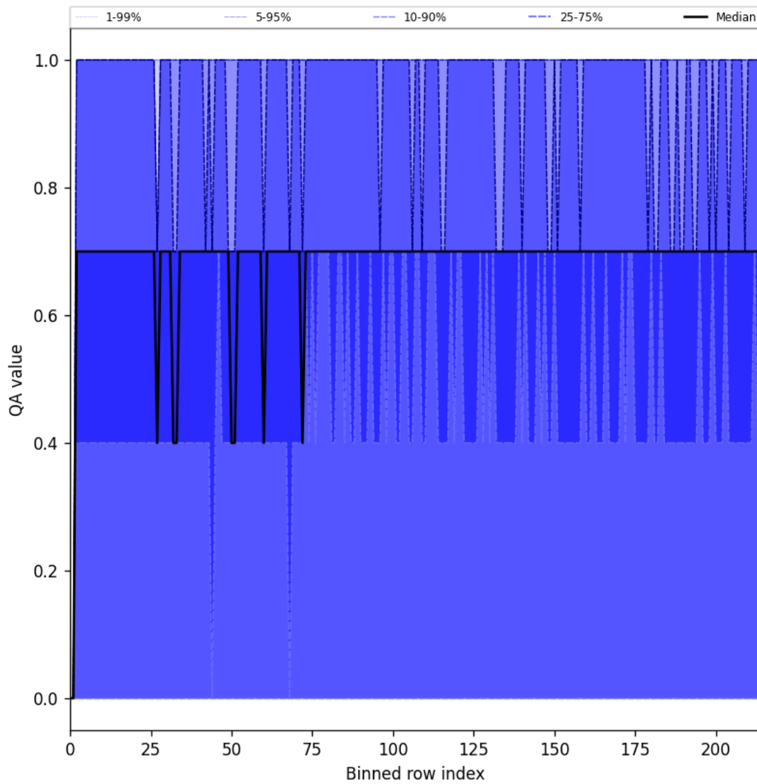
Figure 20: Along track statistics of “QA value” for 2025-03-28 to 2025-03-29
