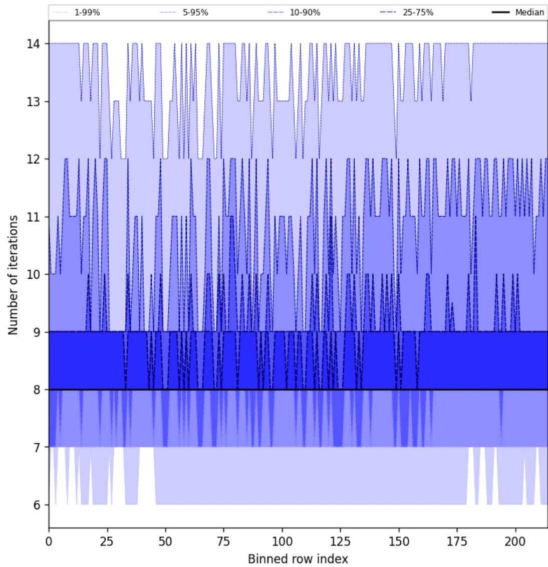
Figure 26: Along track statistics of “Number of iterations” for 2025-03-28 to 2025-03-29
