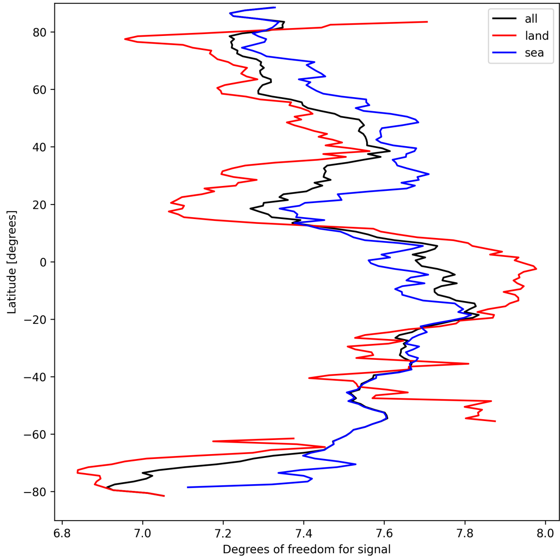
Figure 11: Zonal average of “Degrees of freedom for signal” for 2025-03-28 to 2025-03-29.
