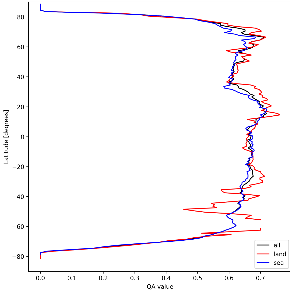
Figure 6: Zonal average of “QA value” for 2025-03-28 to 2025-03-29.
