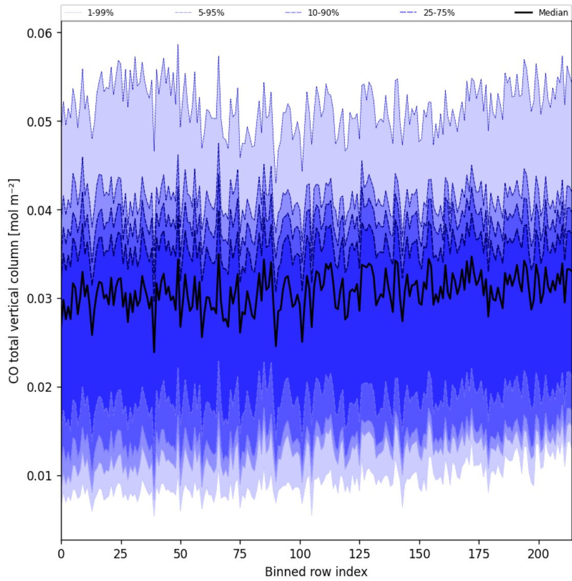
Figure 21: Along track statistics of “CO total vertical column” for 2025-03-28 to 2025-03-29
