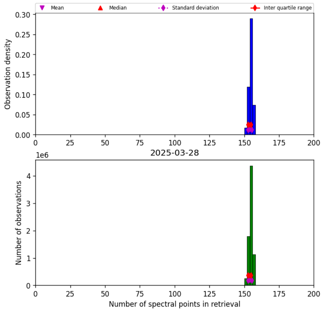
Figure 16: Histogram of “Number of spectral points in retrieval” for 2025-03-28 to 2025-03-29
