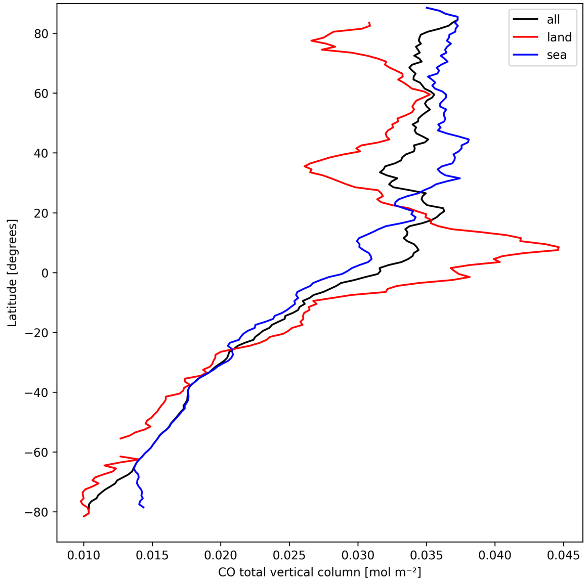
Figure 7: Zonal average of “CO total vertical column” for 2025-03-28 to 2025-03-29.
