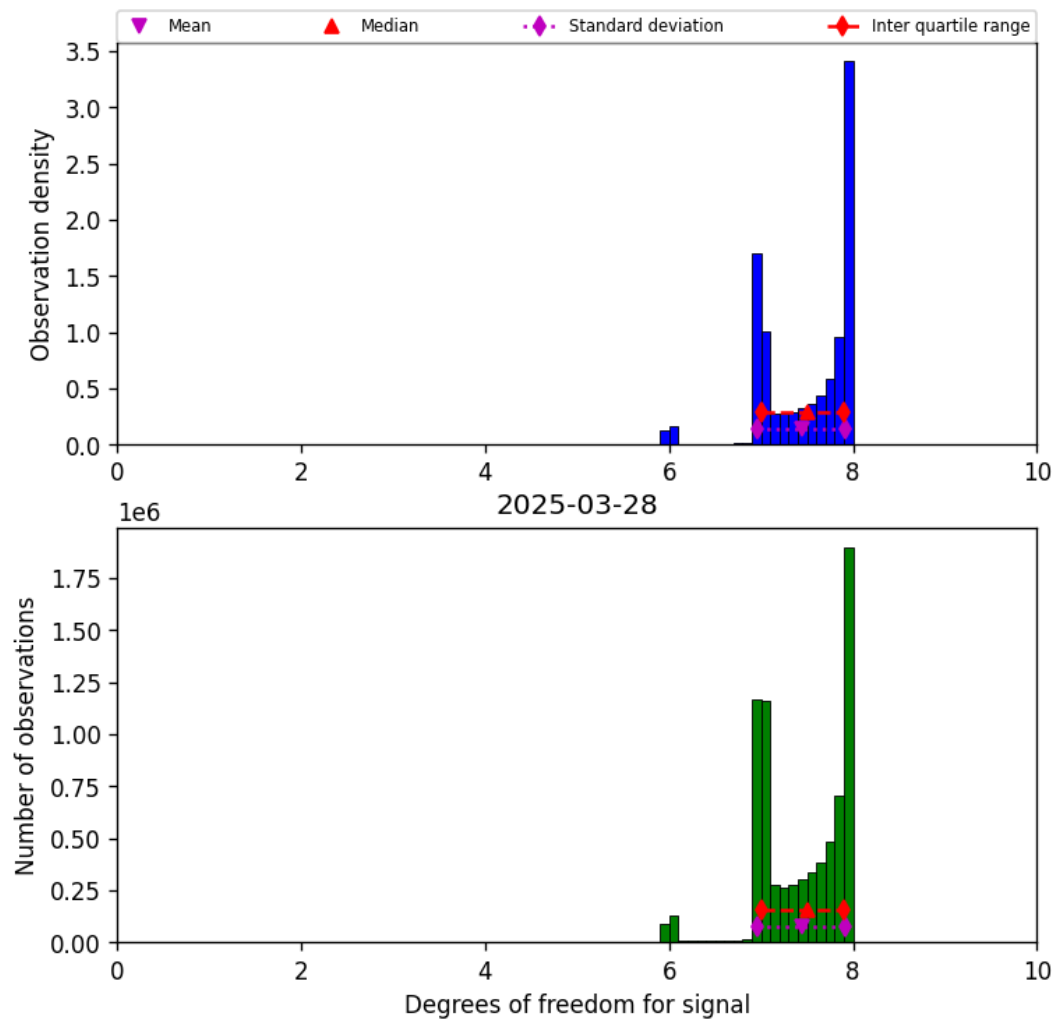
Figure 18: Histogram of “Degrees of freedom for signal” for 2025-03-28 to 2025-03-29
