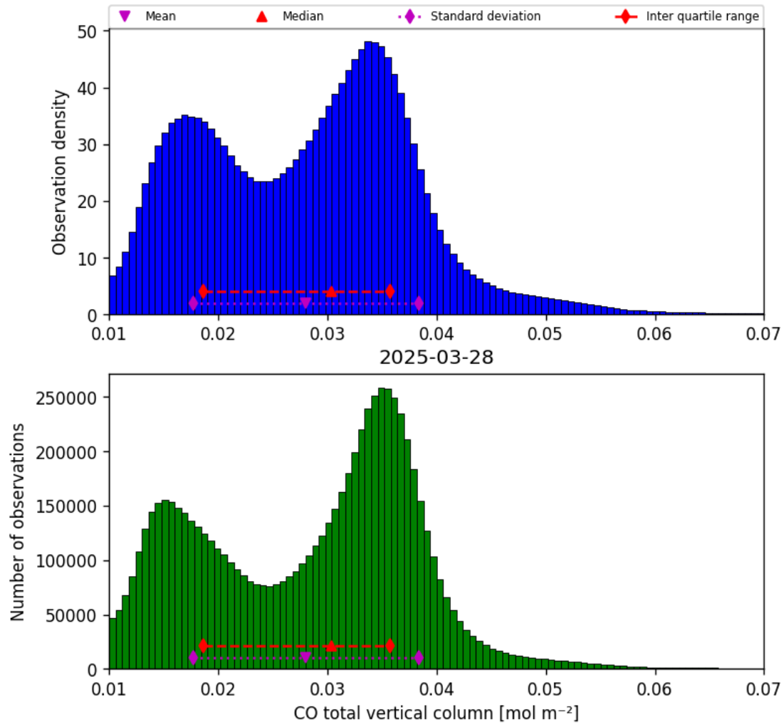
Figure 14: Histogram of “CO total vertical column” for 2025-03-28 to 2025-03-29
