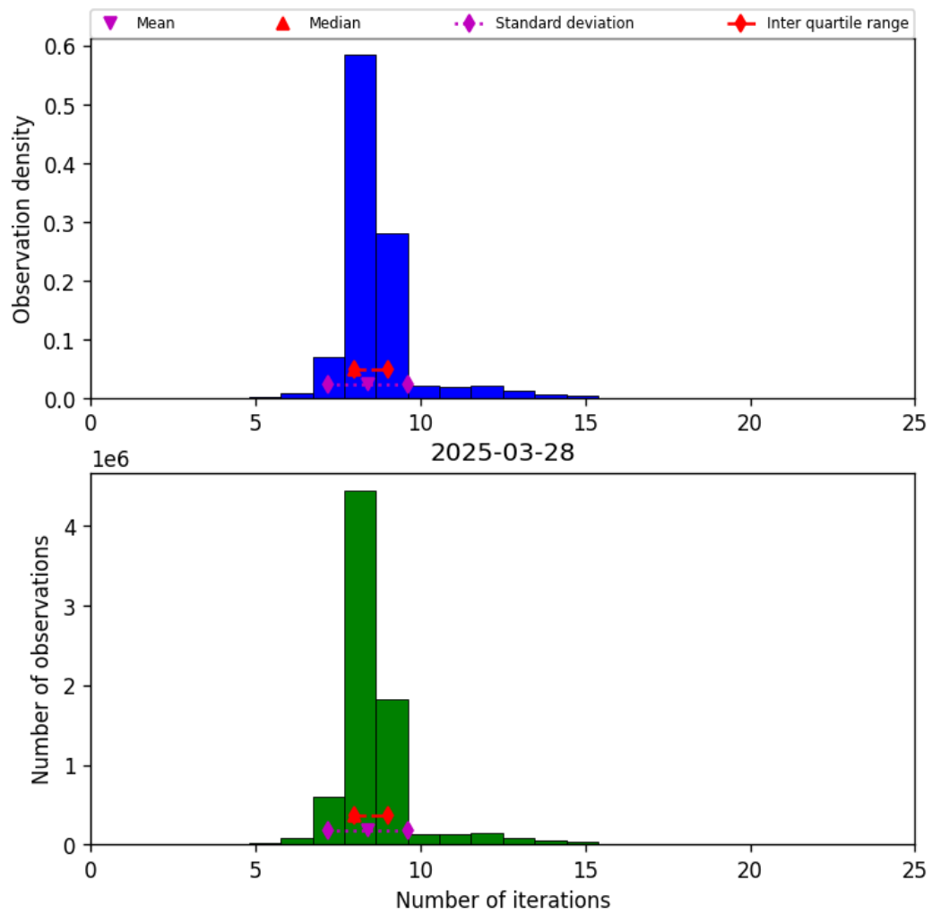
Figure 19: Histogram of “Number of iterations” for 2025-03-28 to 2025-03-29
