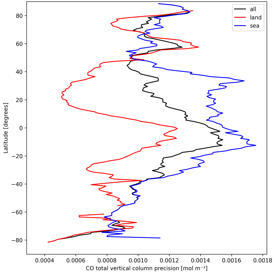
Figure 8: Zonal average of “CO total vertical column precision” for 2025-03-28 to 2025-03-29.
