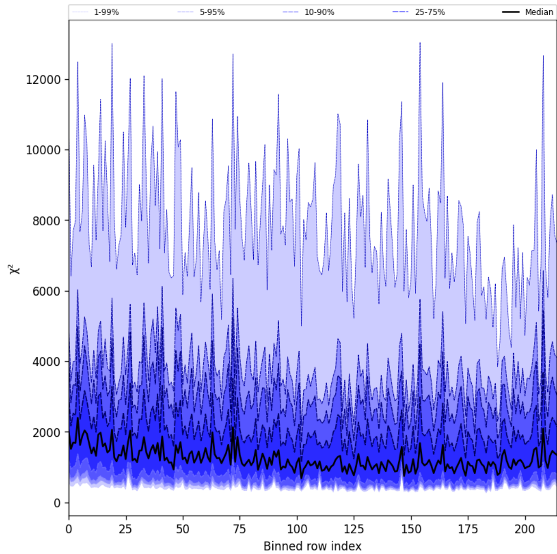
Figure 24: Along track statistics of “ \chi^2 ” for 2025-03-28 to 2025-03-29
