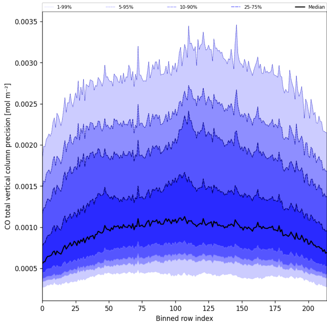
Figure 22: Along track statistics of “CO total vertical column precision” for 2025-03-28 to 2025-03-29
