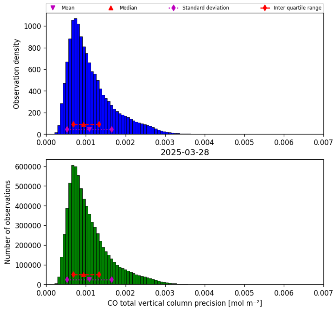
Figure 15: Histogram of “CO total vertical column precision” for 2025-03-28 to 2025-03-29
