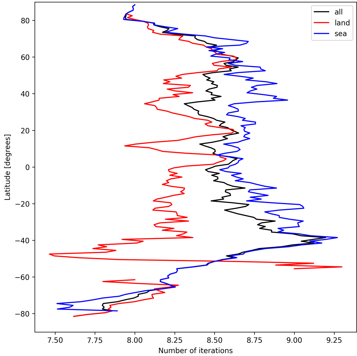
Figure 12: Zonal average of “Number of iterations” for 2025-03-28 to 2025-03-29.
