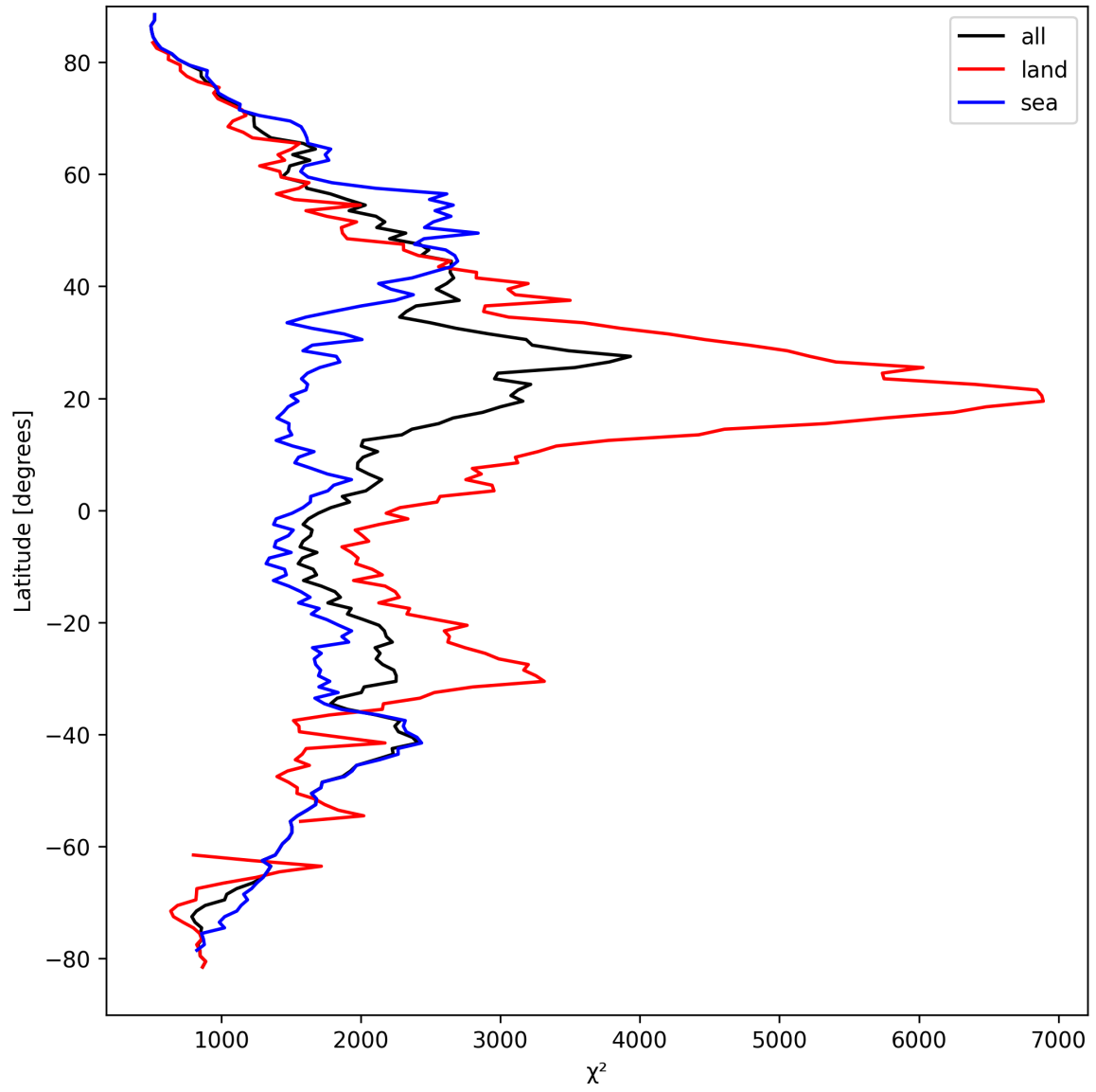
Figure 10: Zonal average of “ \chi^2 ” for 2025-03-28 to 2025-03-29.
