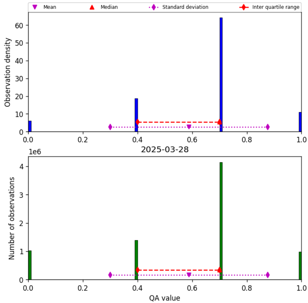
Figure 13: Histogram of “QA value” for 2025-03-28 to 2025-03-29
