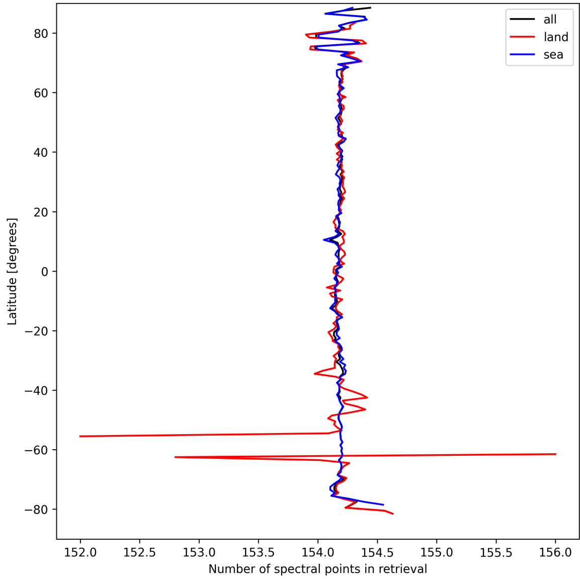
Figure 9: Zonal average of “Number of spectral points in retrieval” for 2025-03-28 to 2025-03-29.
