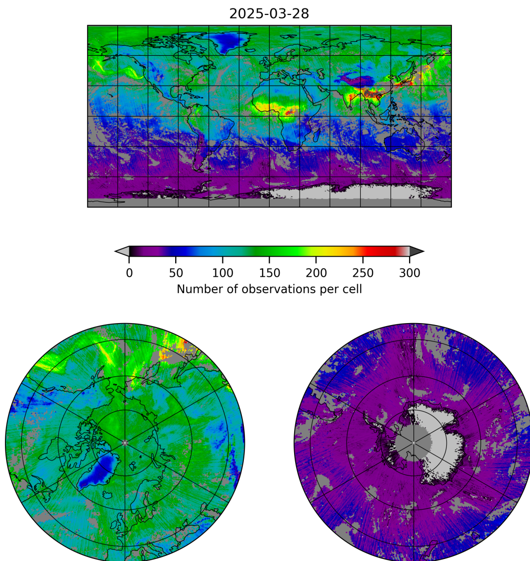
Figure 5: Map of the number of observations for 2025-03-28 to 2025-03-29
