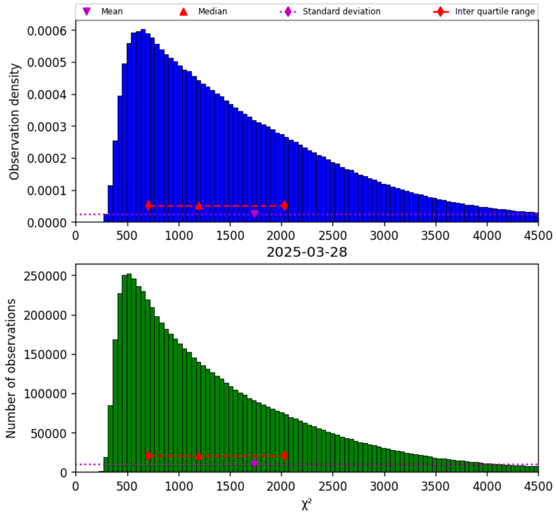
Figure 17: Histogram of “ \chi^2 ” for 2025-03-28 to 2025-03-29
