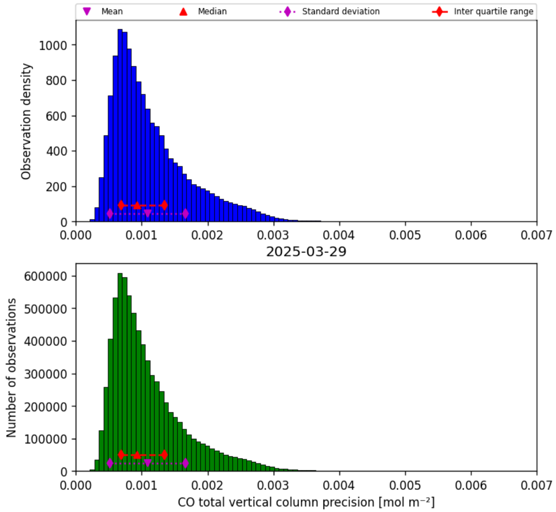
Figure 15: Histogram of “CO total vertical column precision” for 2025-03-29 to 2025-03-30
