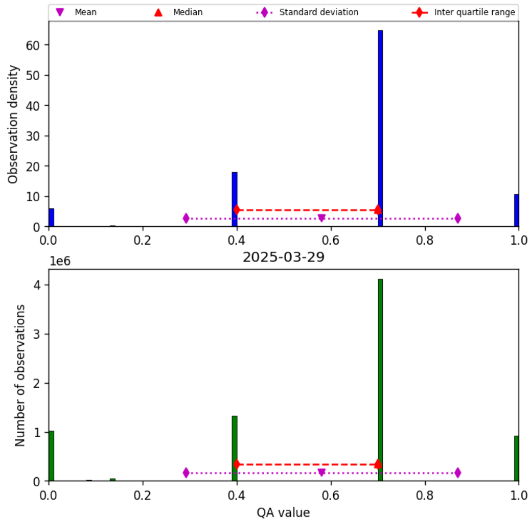
Figure 13: Histogram of “QA value” for 2025-03-29 to 2025-03-30
