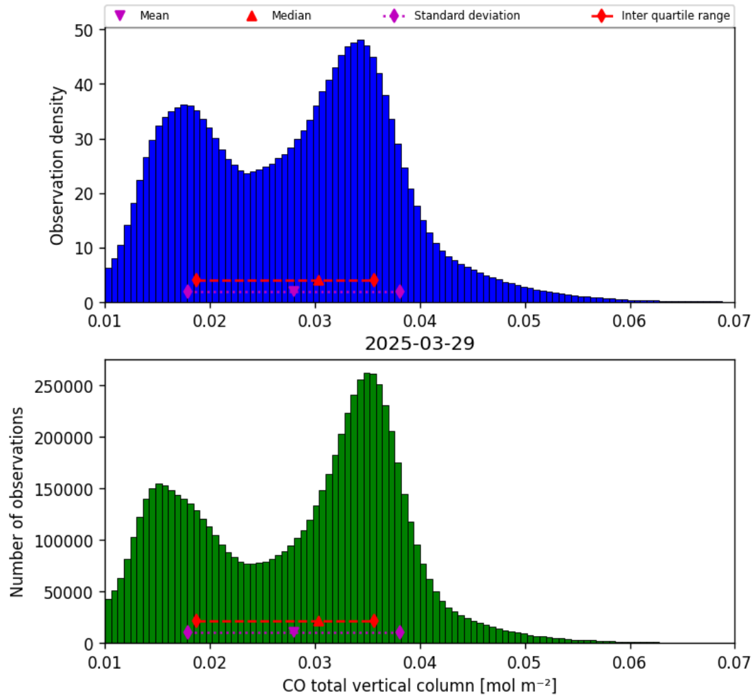
Figure 14: Histogram of “CO total vertical column” for 2025-03-29 to 2025-03-30
