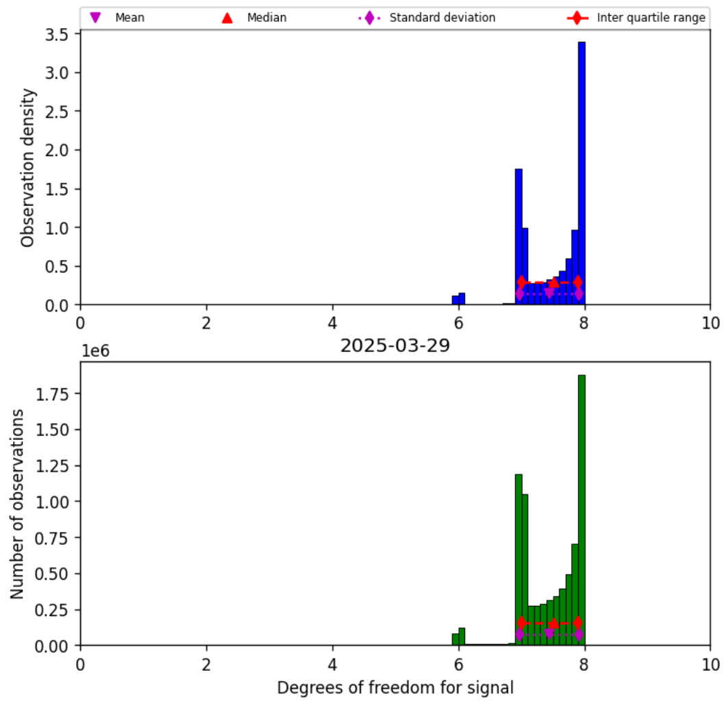
Figure 18: Histogram of “Degrees of freedom for signal” for 2025-03-29 to 2025-03-30
