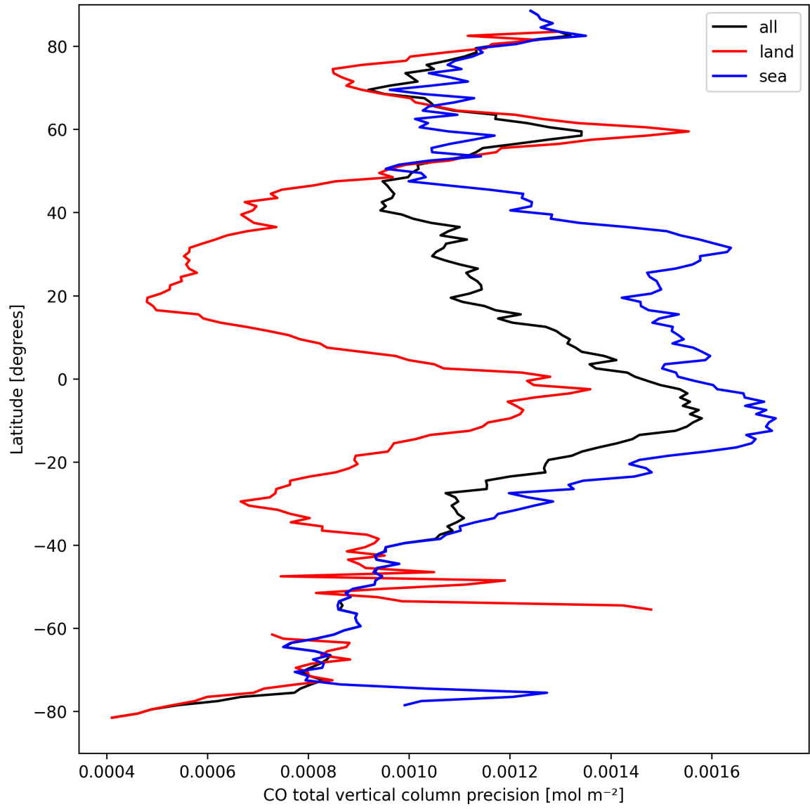
Figure 8: Zonal average of "CO total vertical column precision" for 2025-03-29 to 2025-03-30.
