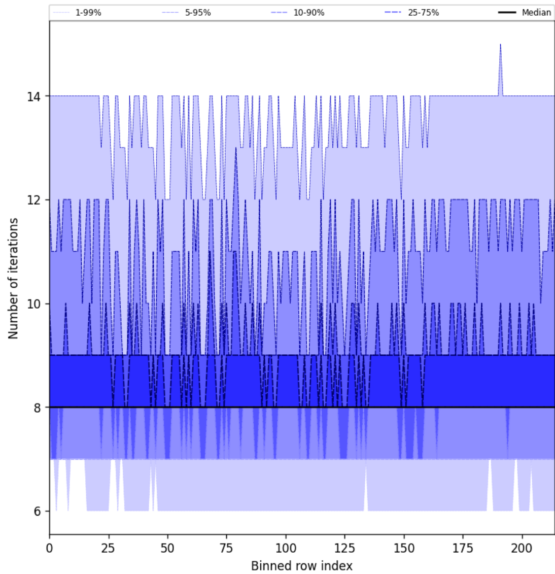
Figure 26: Along track statistics of “Number of iterations” for 2025-03-29 to 2025-03-30
