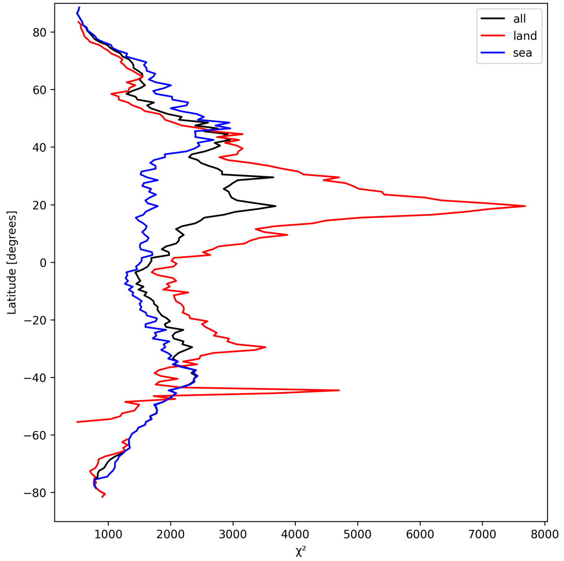
Figure 10: Zonal average of “ \chi^2 ” for 2025-03-29 to 2025-03-30.
