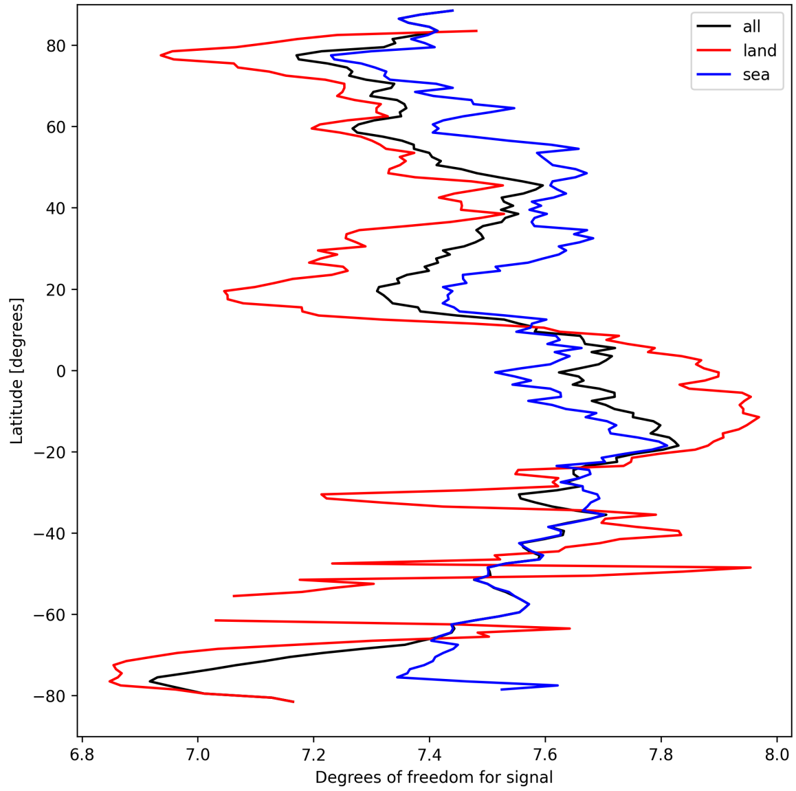
Figure 11: Zonal average of “Degrees of freedom for signal” for 2025-03-29 to 2025-03-30.
