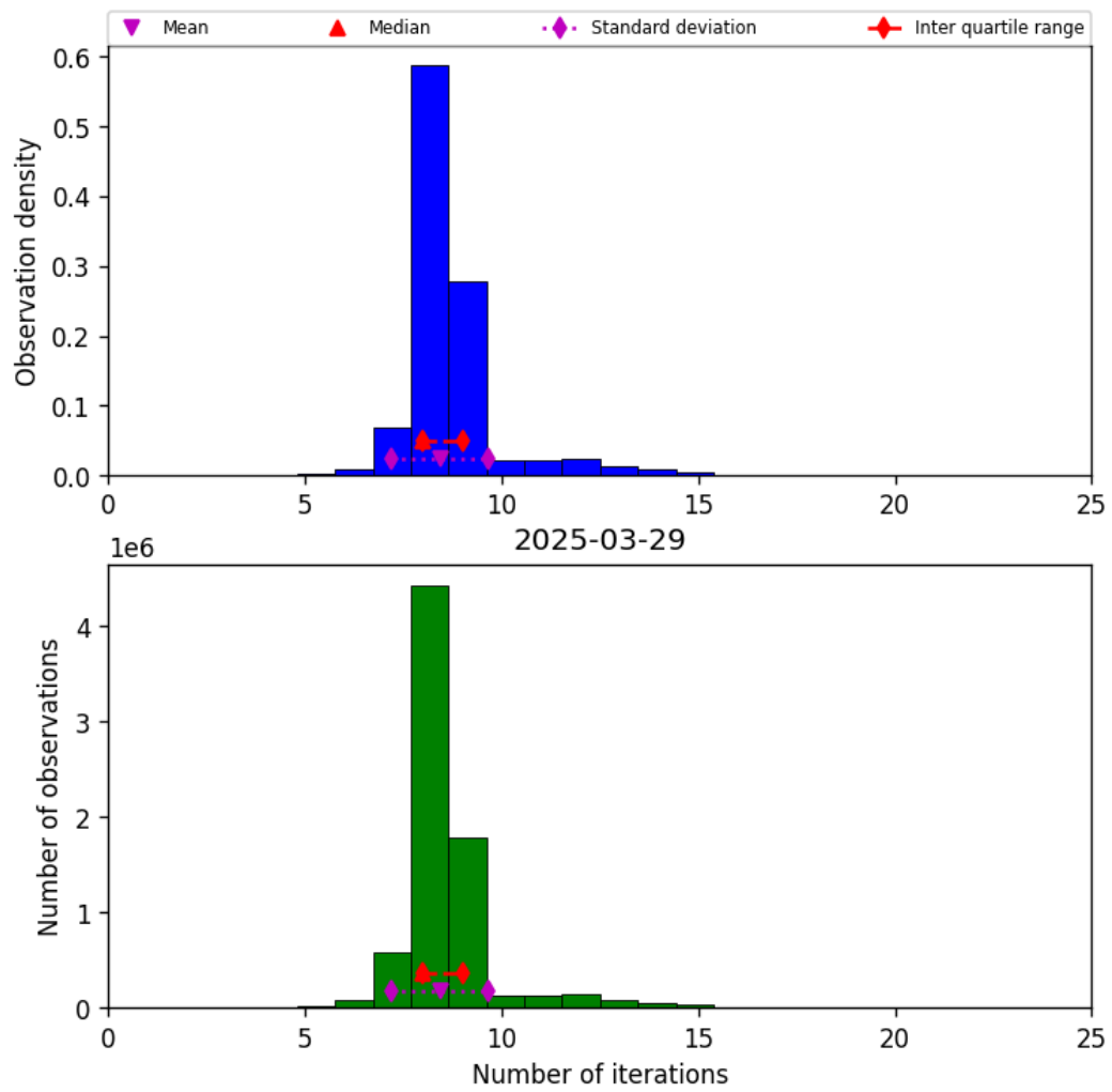
Figure 19: Histogram of “Number of iterations” for 2025-03-29 to 2025-03-30
