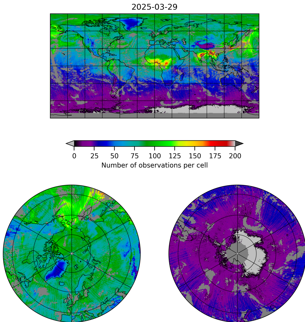
Figure 5: Map of the number of observations for 2025-03-29 to 2025-03-30
