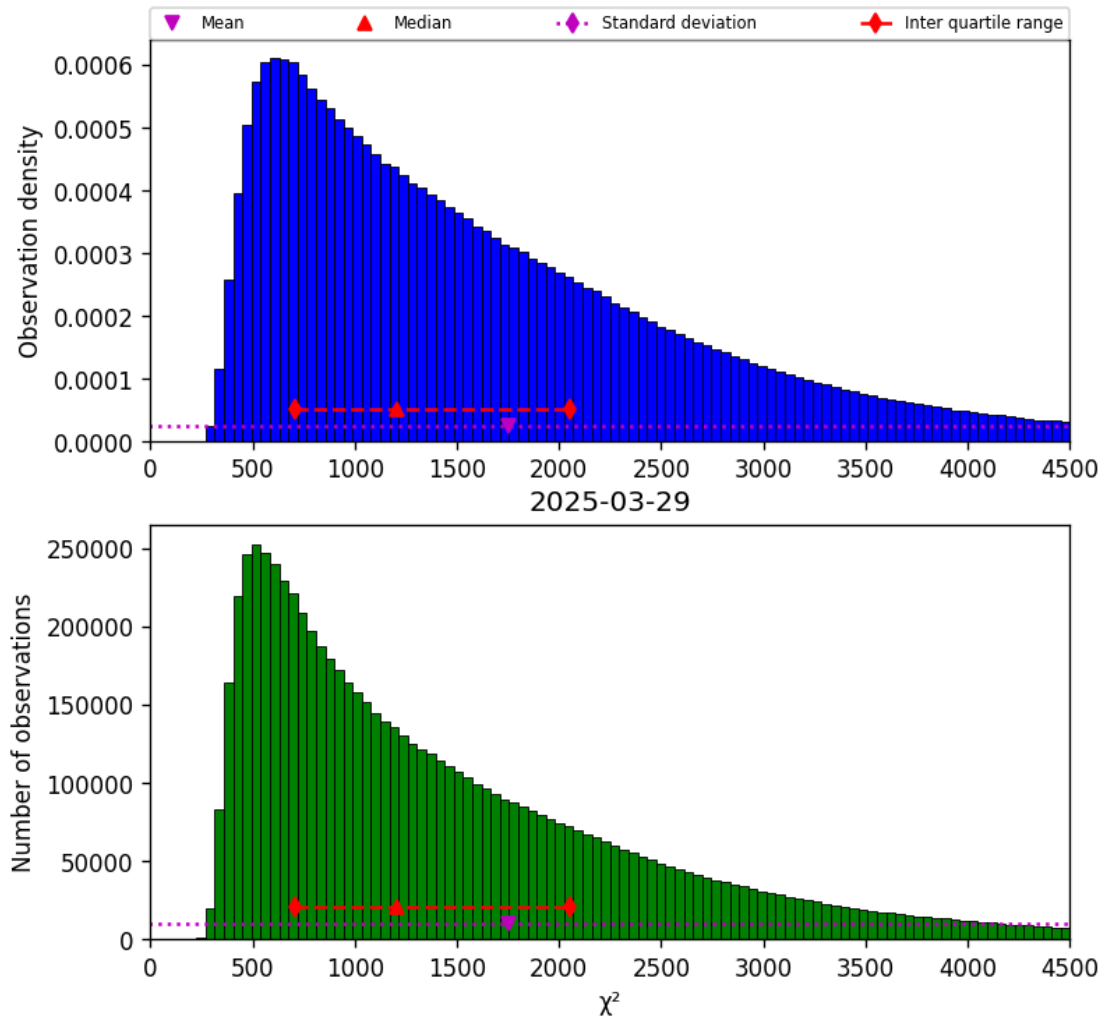
Figure 17: Histogram of “ \chi^2 ” for 2025-03-29 to 2025-03-30
