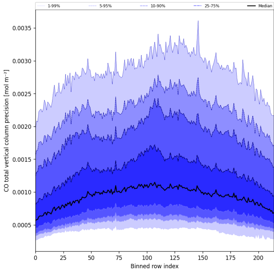
Figure 22: Along track statistics of “CO total vertical column precision” for 2025-03-29 to 2025-03-30
