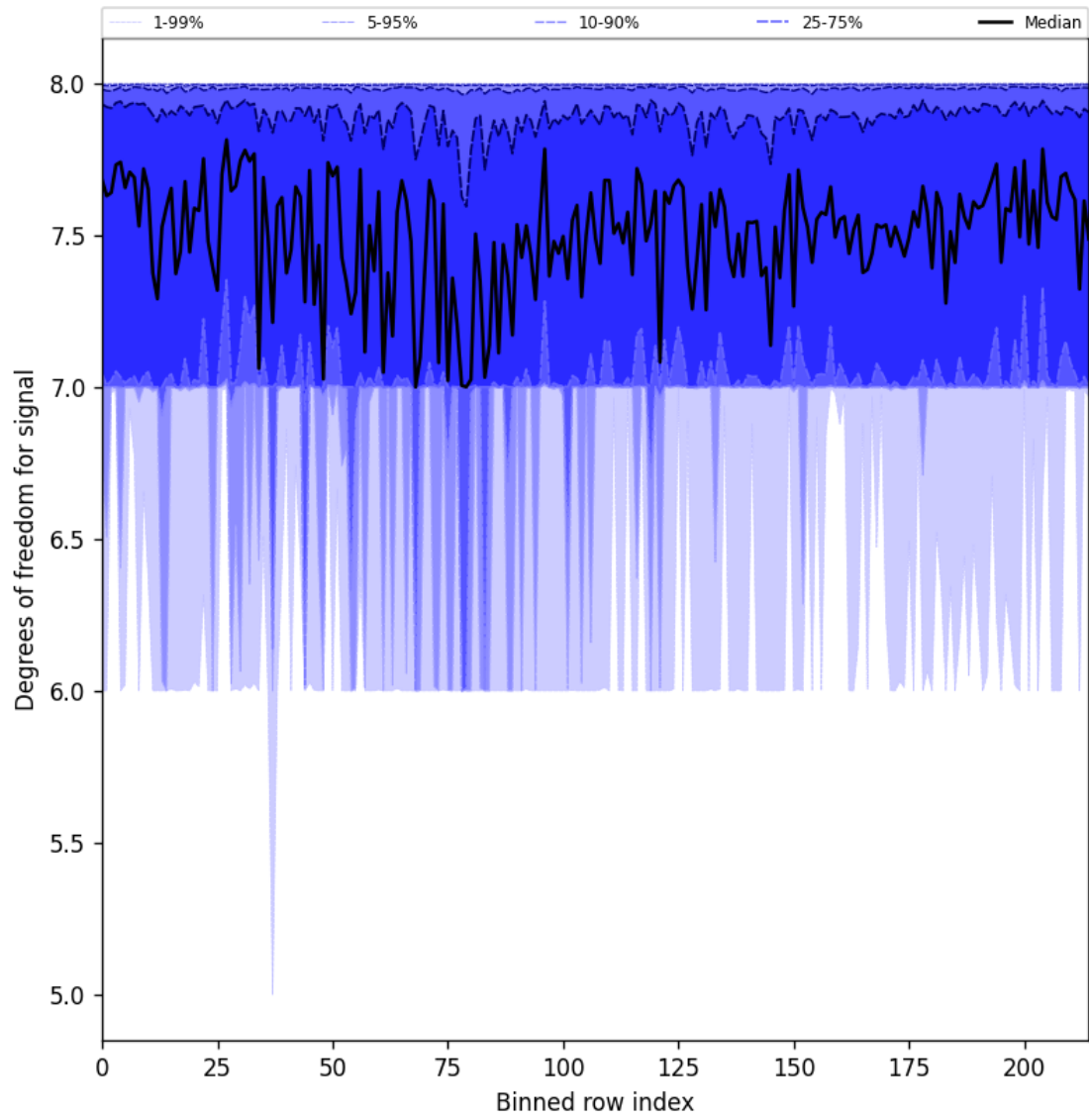
Figure 25: Along track statistics of “Degrees of freedom for signal” for 2025-03-29 to 2025-03-30
