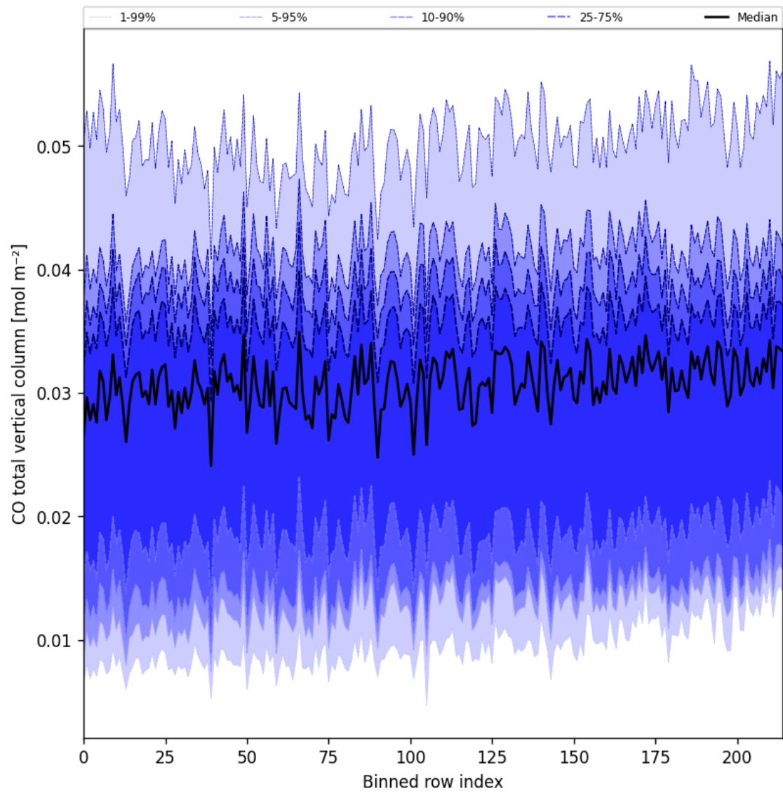
Figure 21: Along track statistics of “CO total vertical column” for 2025-03-29 to 2025-03-30
