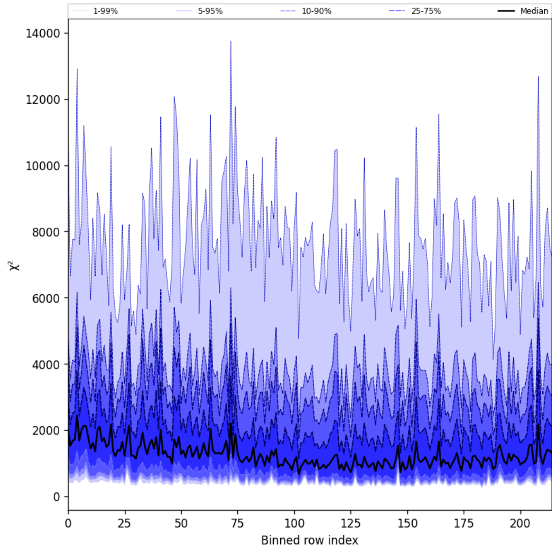
Figure 24: Along track statistics of “ \chi^2 ” for 2025-03-29 to 2025-03-30
