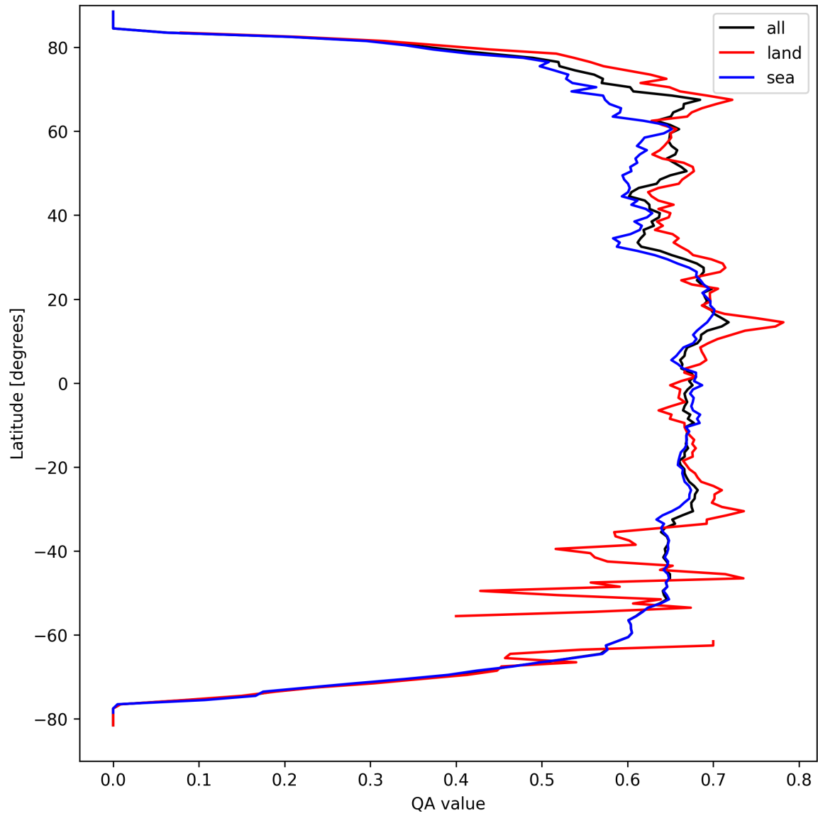
Figure 6: Zonal average of “QA value” for 2025-03-29 to 2025-03-30.
