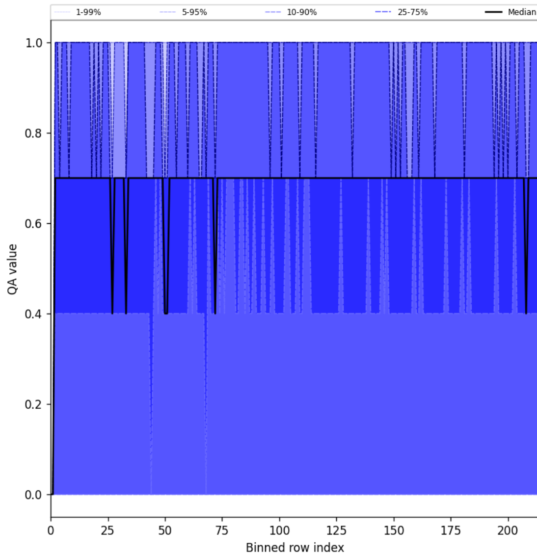
Figure 20: Along track statistics of “QA value” for 2025-03-29 to 2025-03-30
