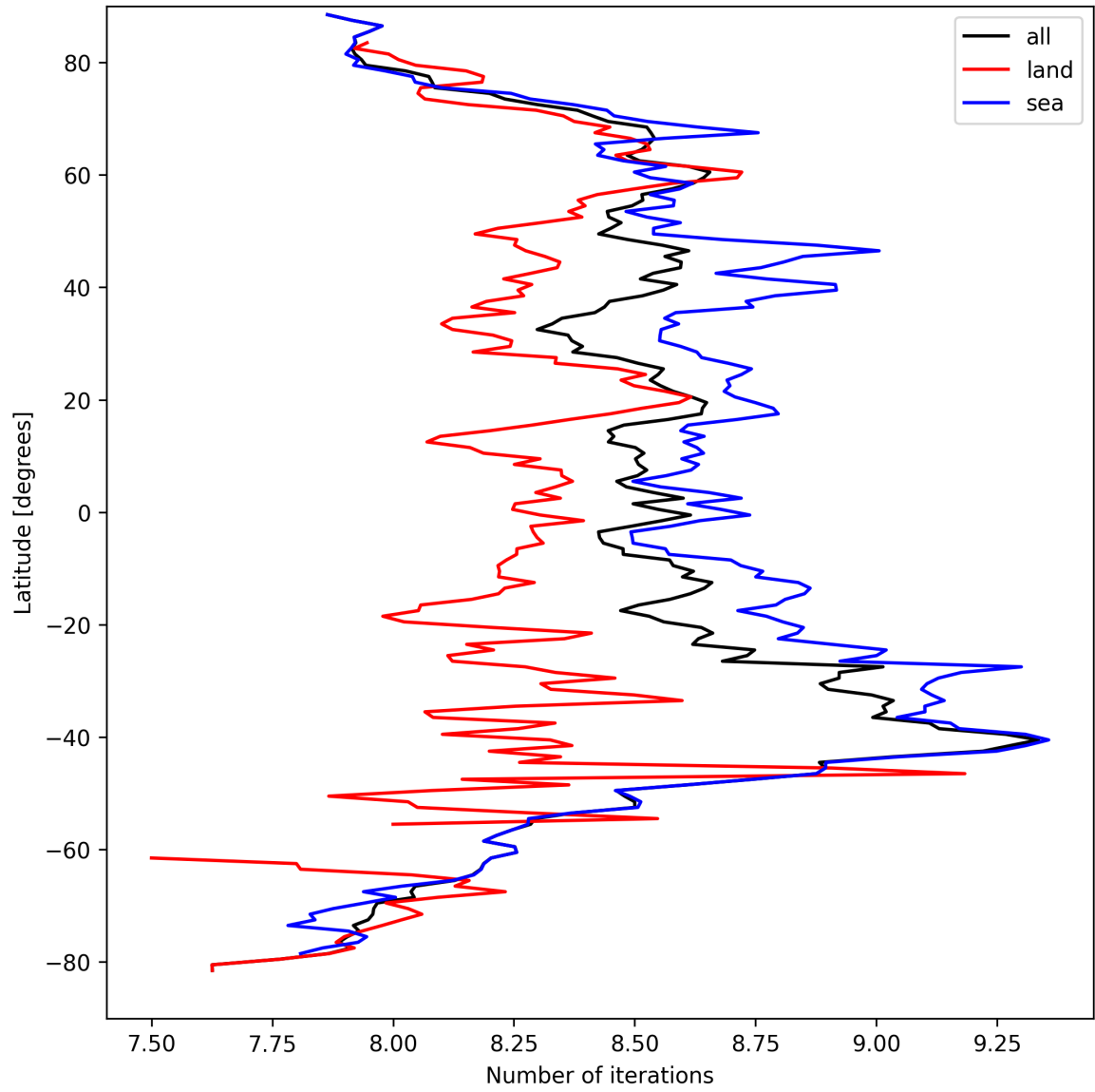
Figure 12: Zonal average of “Number of iterations” for 2025-03-29 to 2025-03-30.
