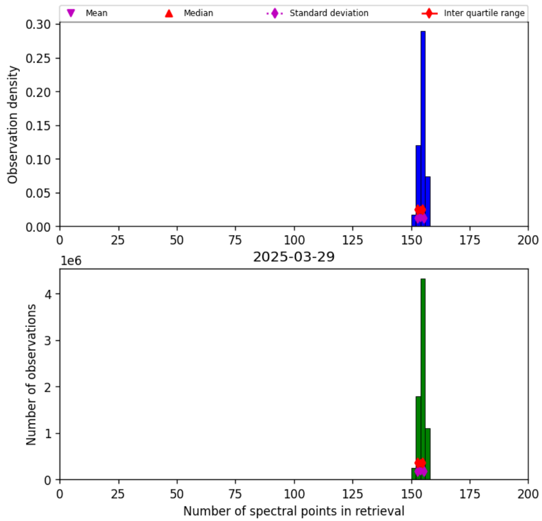
Figure 16: Histogram of “Number of spectral points in retrieval” for 2025-03-29 to 2025-03-30
