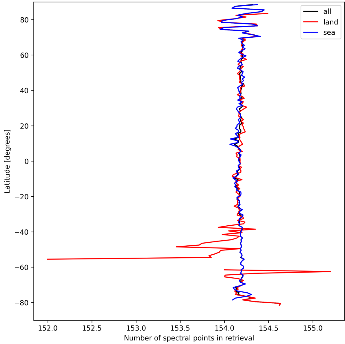
Figure 9: Zonal average of “Number of spectral points in retrieval” for 2025-03-29 to 2025-03-30.
