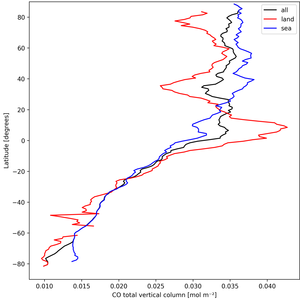
Figure 7: Zonal average of “CO total vertical column” for 2025-03-29 to 2025-03-30.
