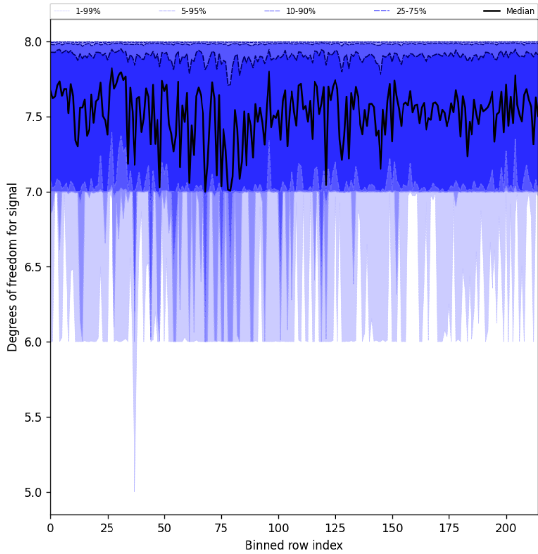
Figure 25: Along track statistics of “Degrees of freedom for signal” for 2025-03-30 to 2025-03-31
