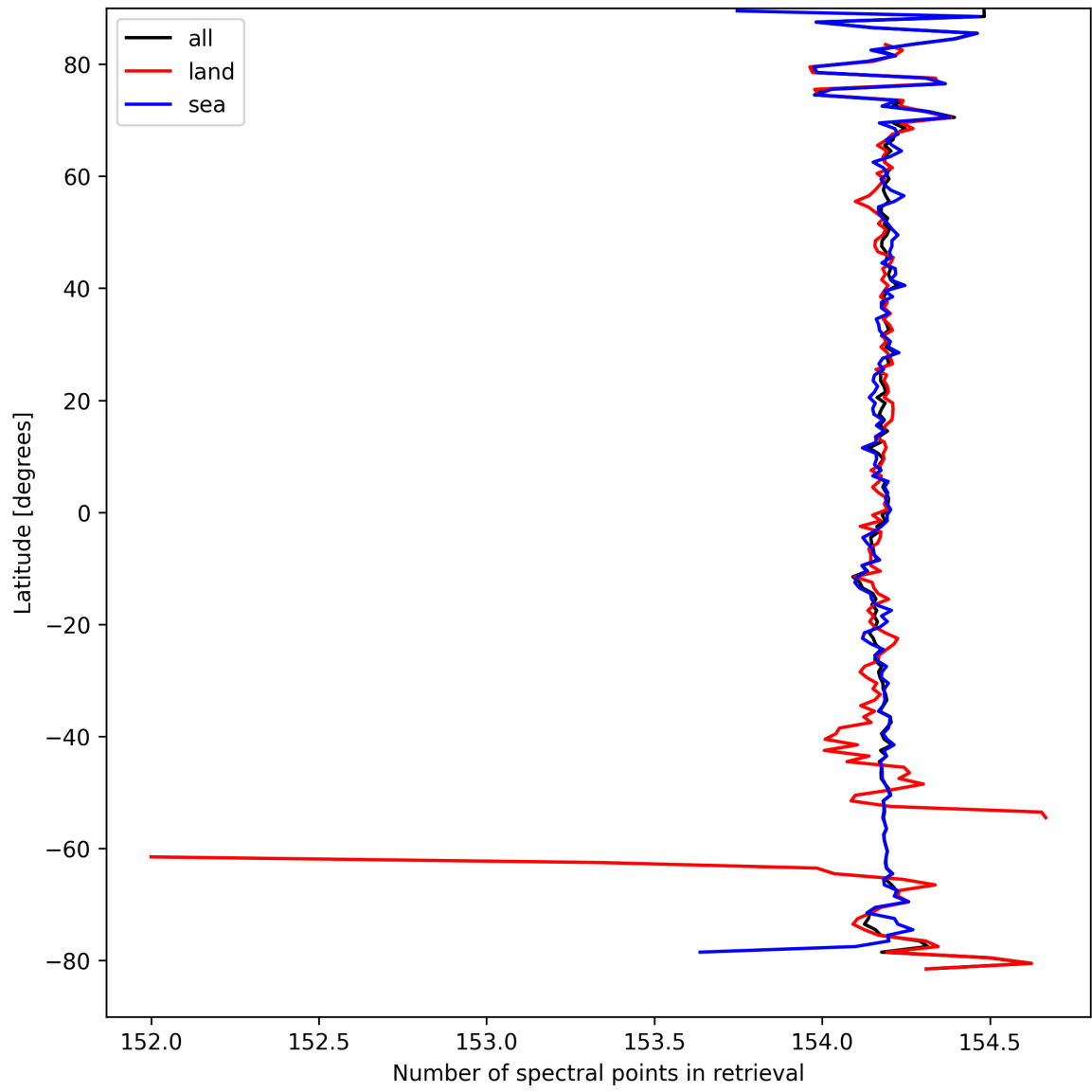
Figure 9: Zonal average of “Number of spectral points in retrieval” for 2025-03-30 to 2025-03-31.
