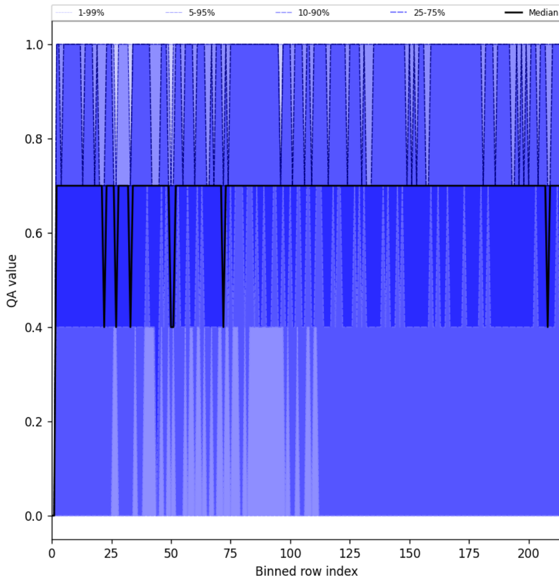
Figure 20: Along track statistics of “QA value” for 2025-03-30 to 2025-03-31
