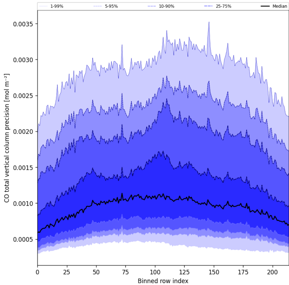
Figure 22: Along track statistics of “CO total vertical column precision” for 2025-03-30 to 2025-03-31
