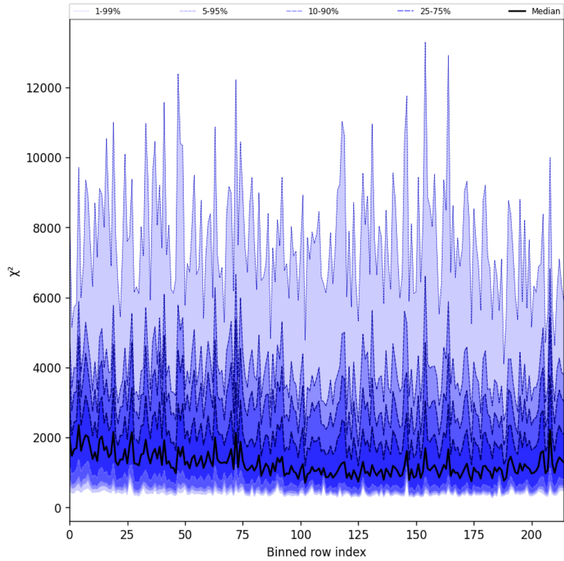
Figure 24: Along track statistics of “ \chi^2 ” for 2025-03-30 to 2025-03-31
