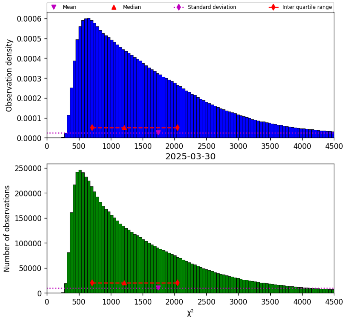
Figure 17: Histogram of " \chi^2 " for 2025-03-30 to 2025-03-31
