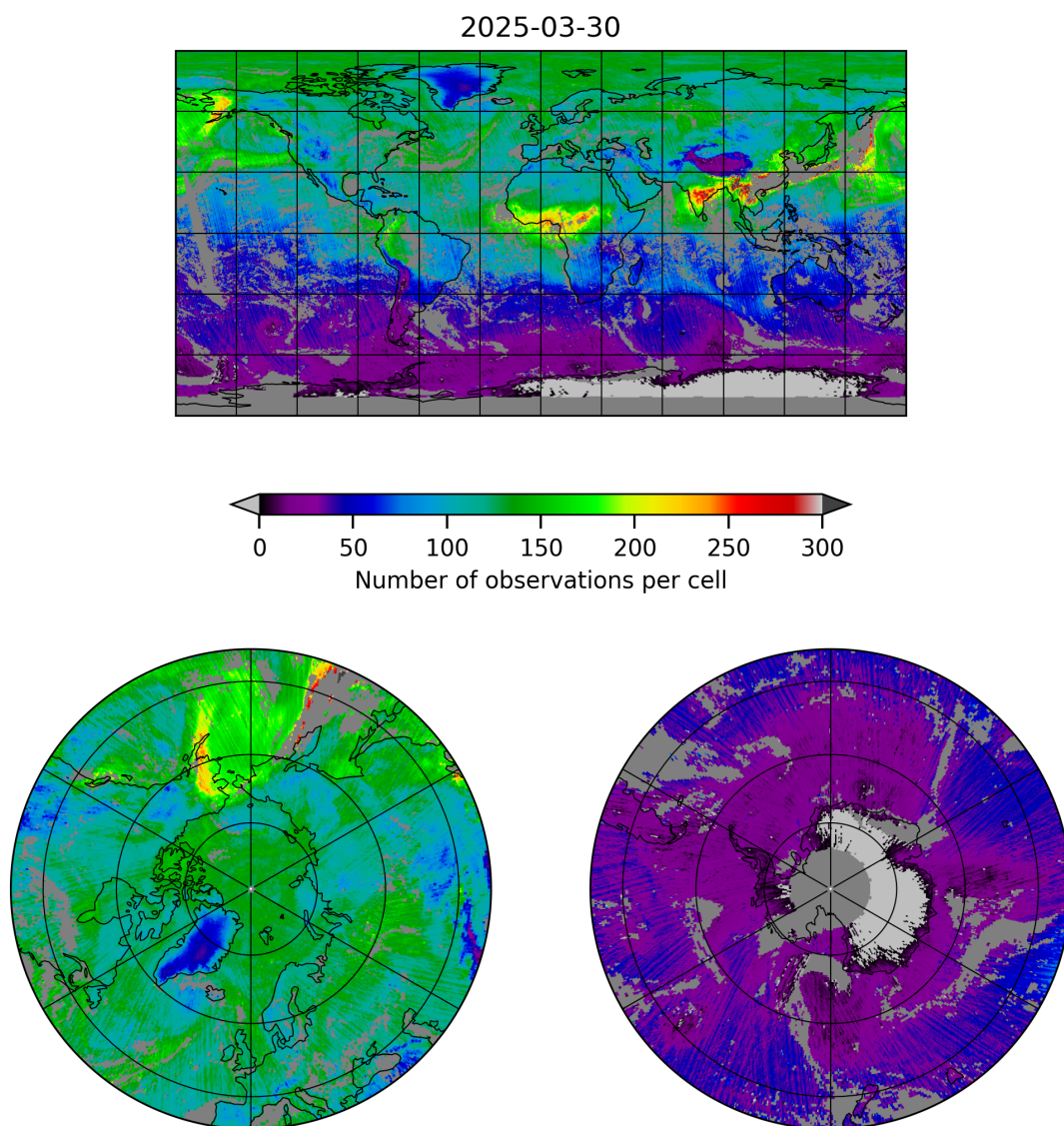
Figure 5: Map of the number of observations for 2025-03-30 to 2025-03-31
