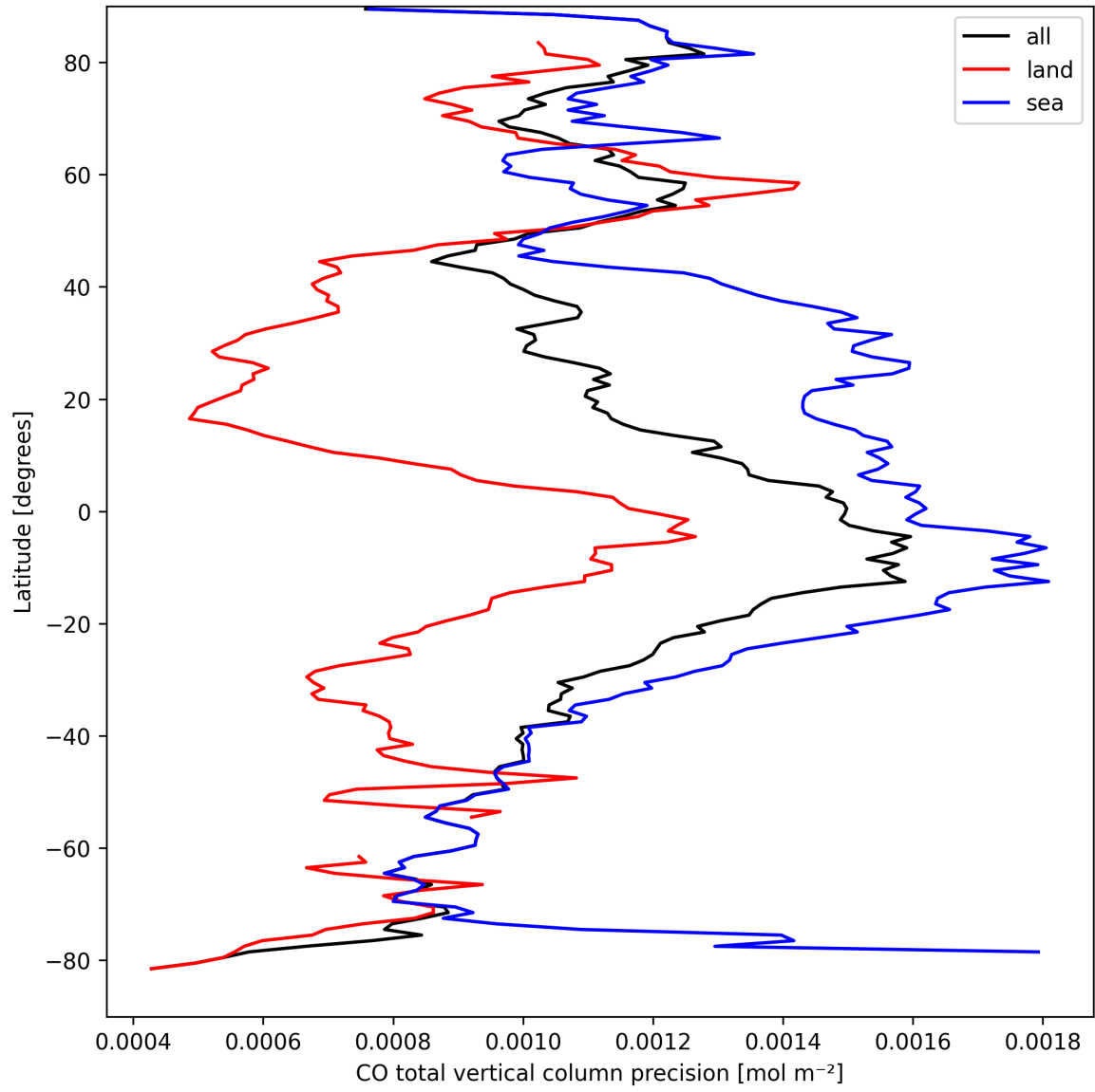
Figure 8: Zonal average of “CO total vertical column precision” for 2025-03-30 to 2025-03-31.
