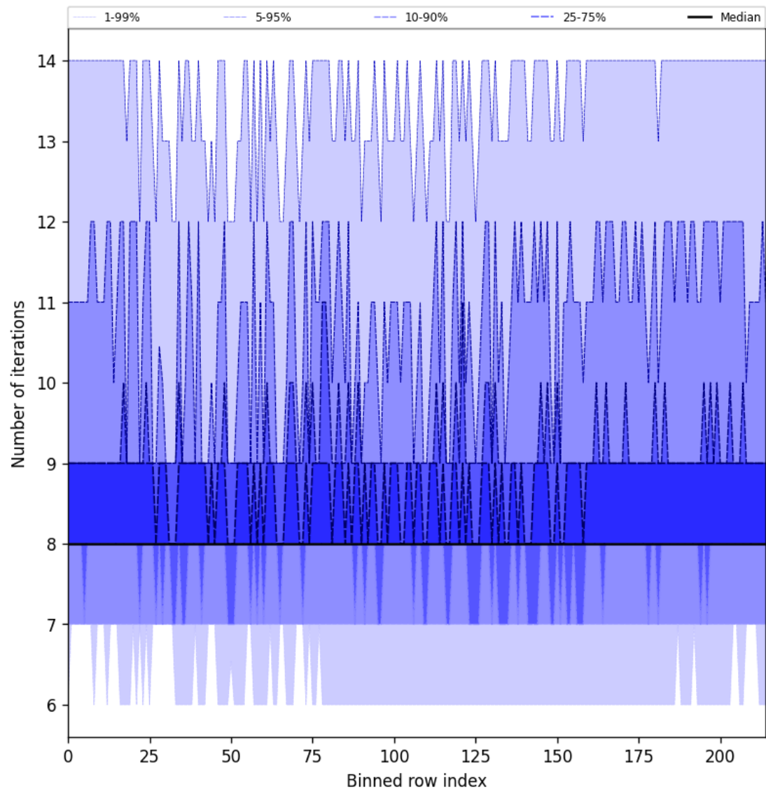
Figure 26: Along track statistics of “Number of iterations” for 2025-03-30 to 2025-03-31
