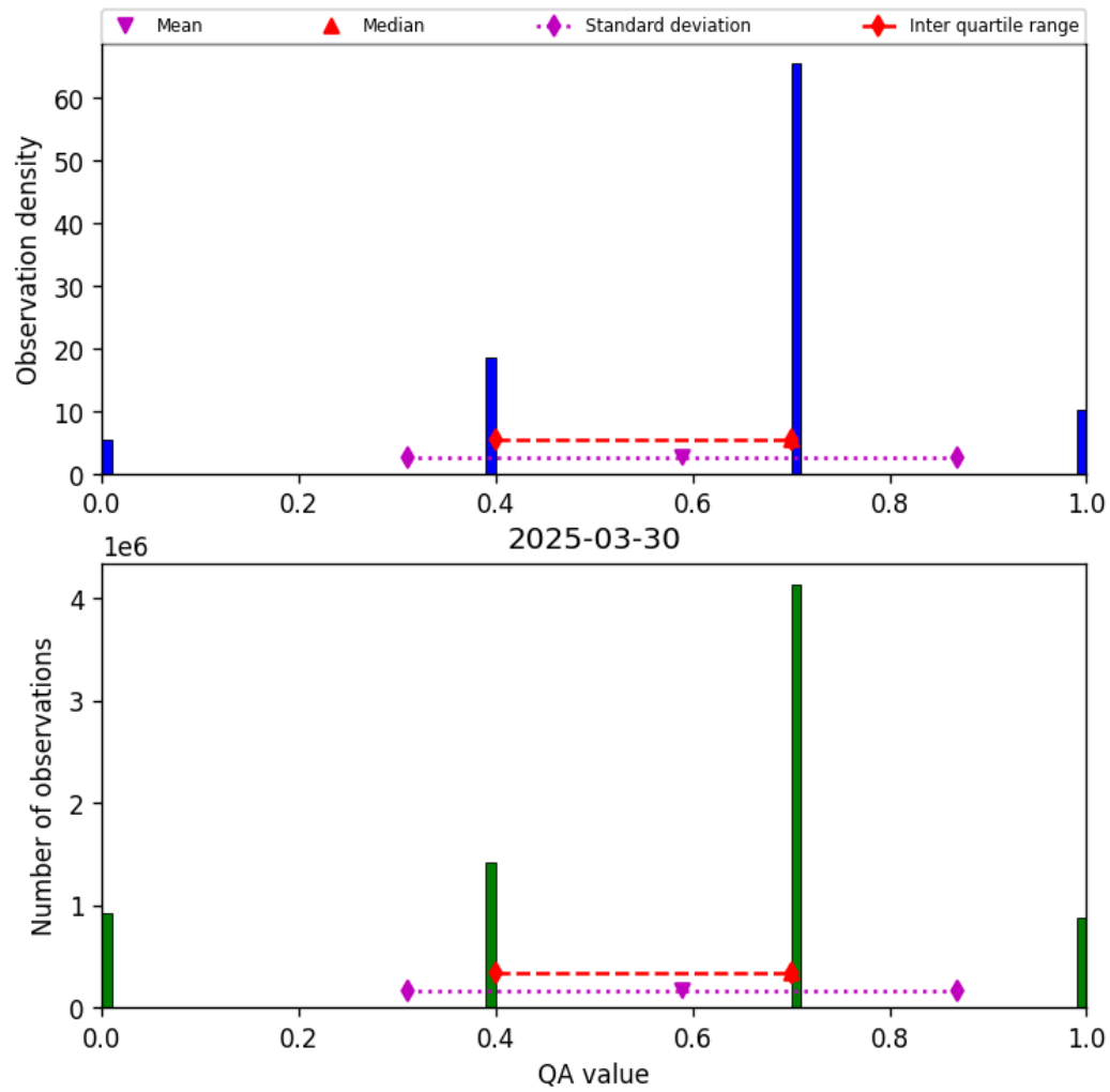
Figure 13: Histogram of “QA value” for 2025-03-30 to 2025-03-31
