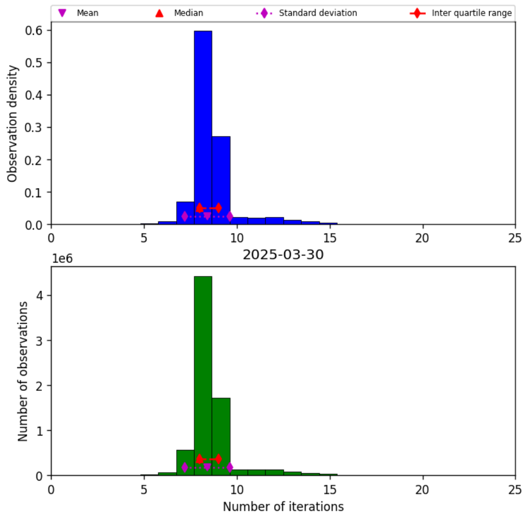
Figure 19: Histogram of “Number of iterations” for 2025-03-30 to 2025-03-31
