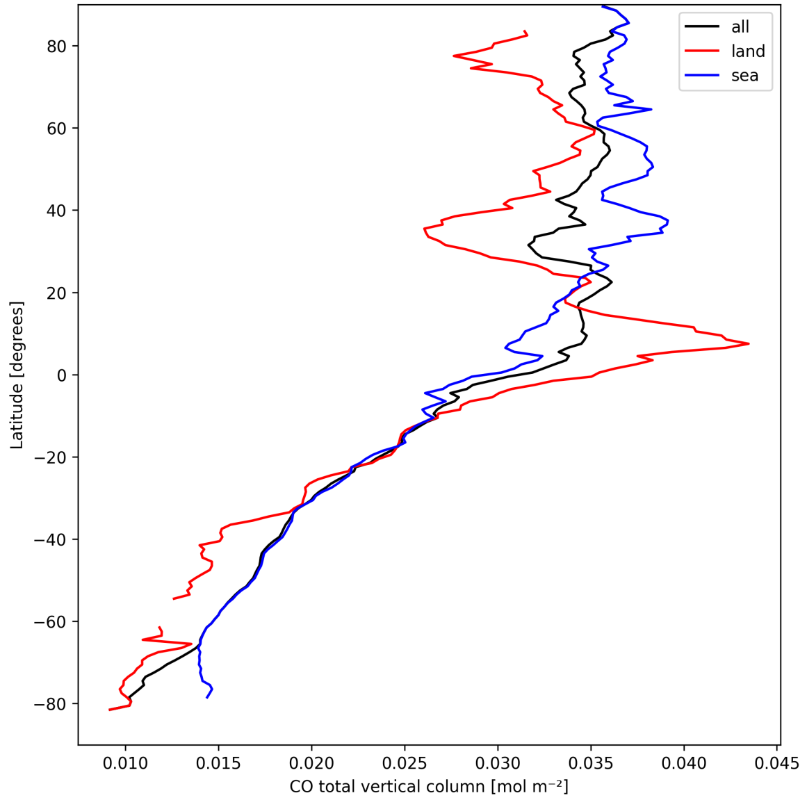
Figure 7: Zonal average of “CO total vertical column” for 2025-03-30 to 2025-03-31.
