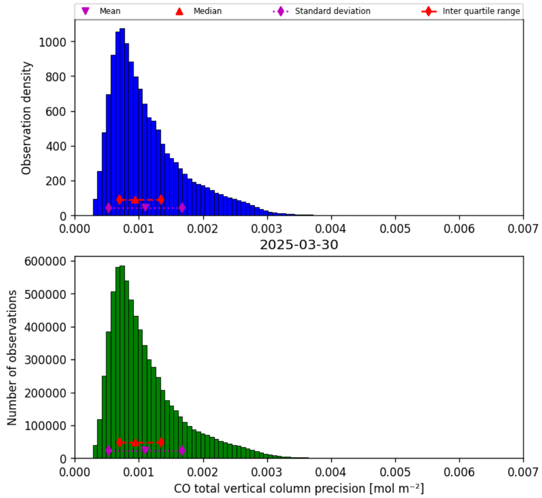
Figure 15: Histogram of “CO total vertical column precision” for 2025-03-30 to 2025-03-31
