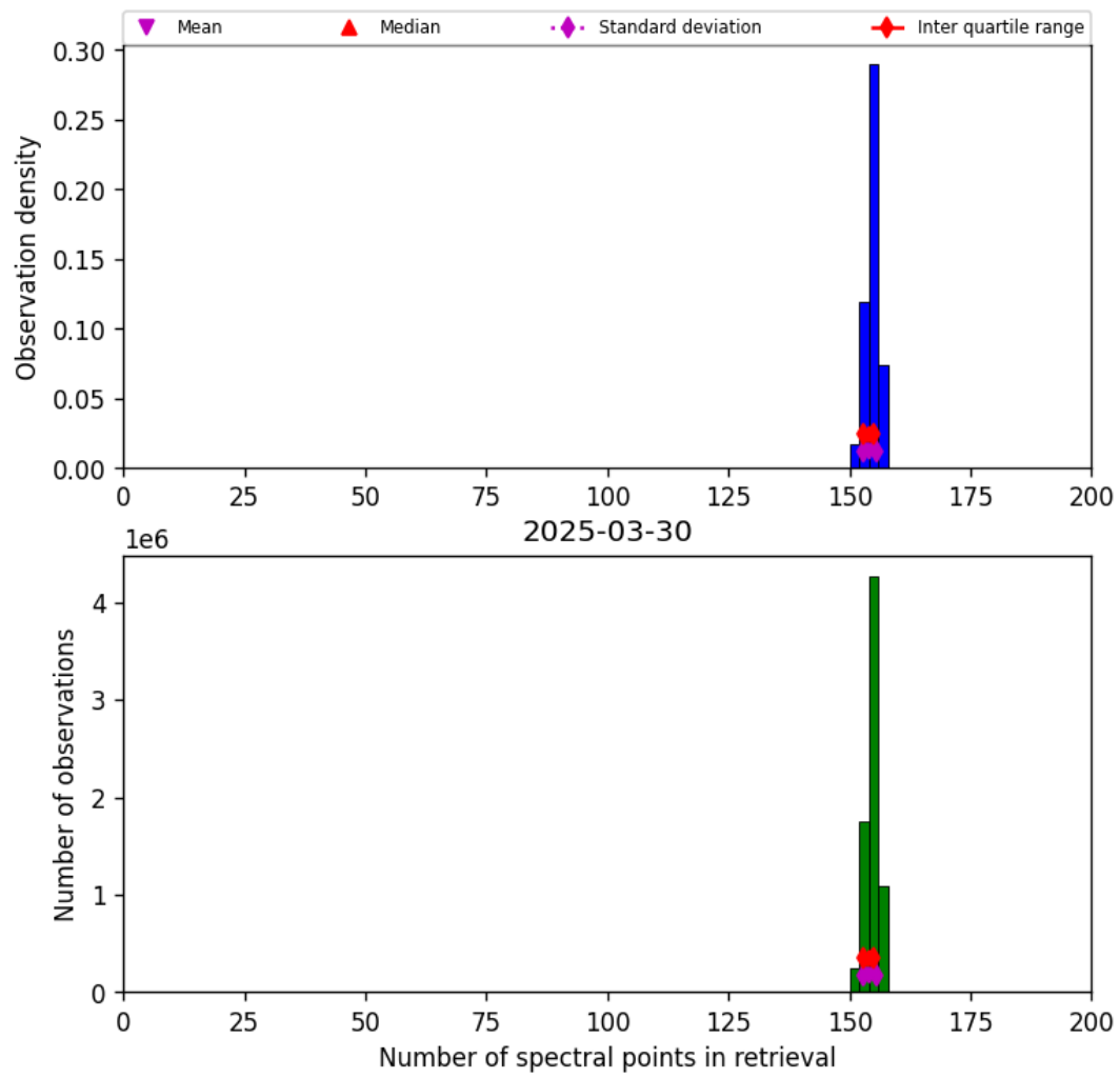
Figure 16: Histogram of “Number of spectral points in retrieval” for 2025-03-30 to 2025-03-31
