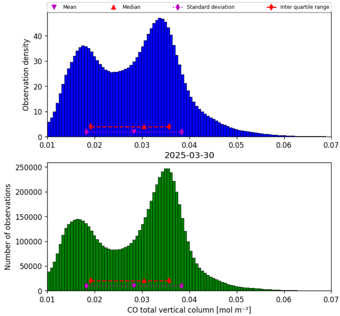
Figure 14: Histogram of “CO total vertical column” for 2025-03-30 to 2025-03-31
