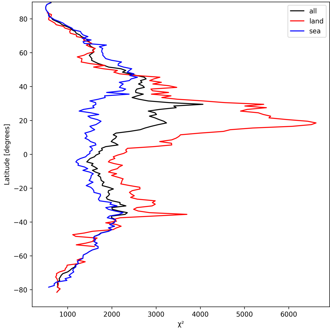
Figure 10: Zonal average of “ \chi^2 ” for 2025-03-30 to 2025-03-31.
