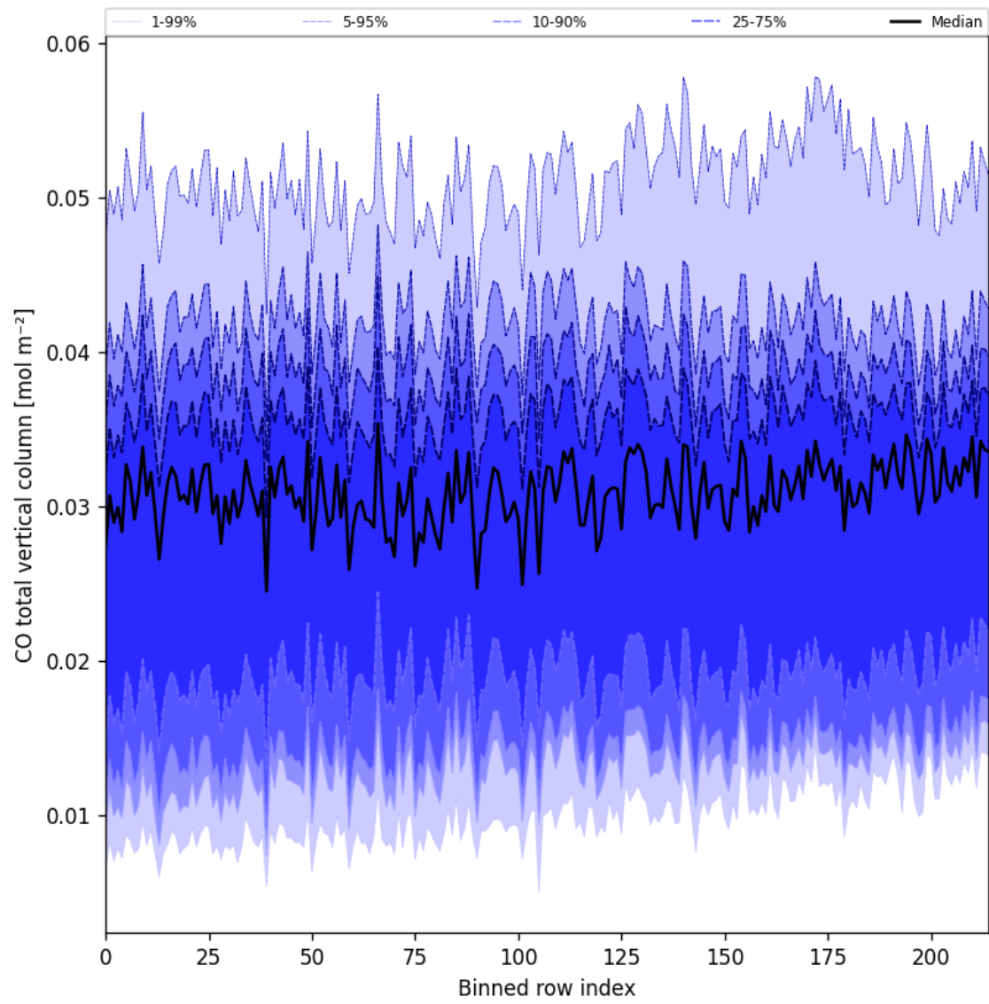
Figure 21: Along track statistics of “CO total vertical column” for 2025-03-30 to 2025-03-31
