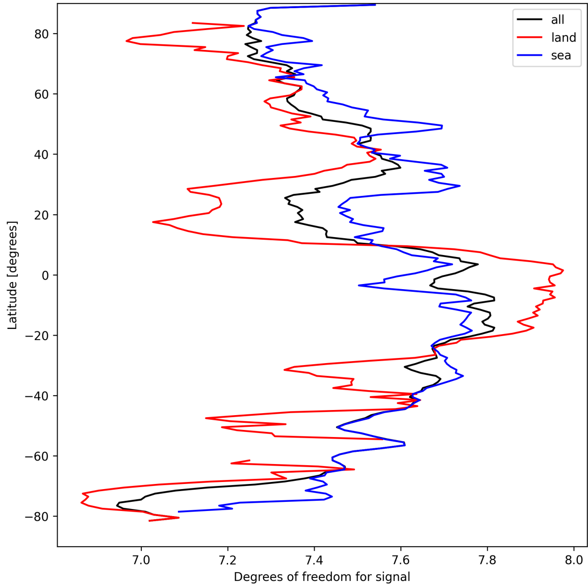
Figure 11: Zonal average of “Degrees of freedom for signal” for 2025-03-30 to 2025-03-31.
