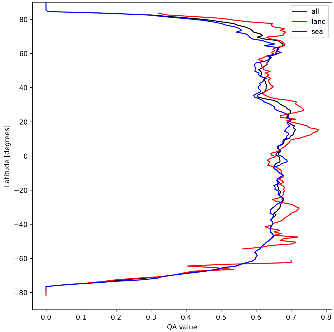
Figure 6: Zonal average of “QA value” for 2025-03-30 to 2025-03-31.
