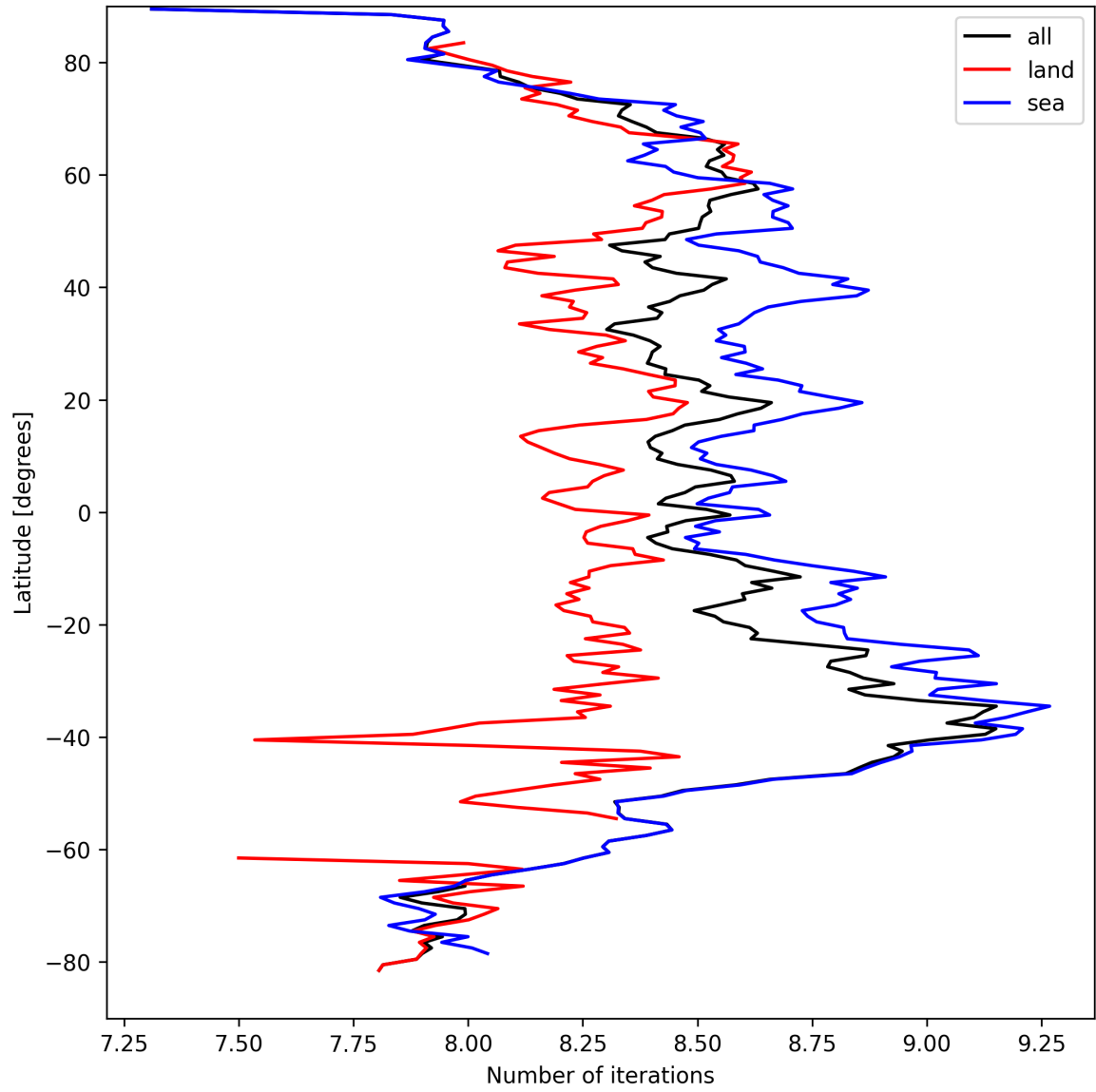
Figure 12: Zonal average of “Number of iterations” for 2025-03-30 to 2025-03-31.
