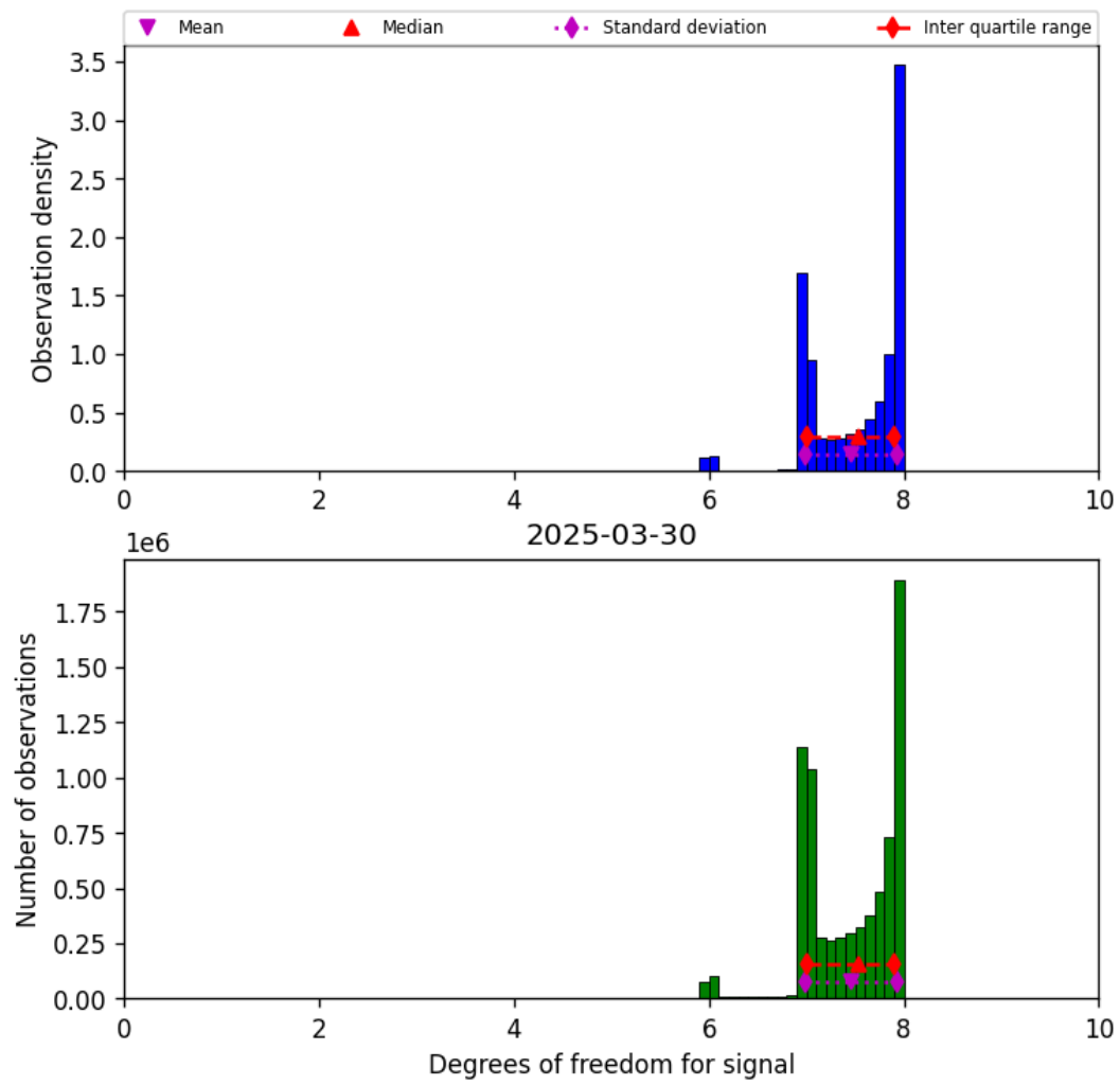
Figure 18: Histogram of “Degrees of freedom for signal” for 2025-03-30 to 2025-03-31
