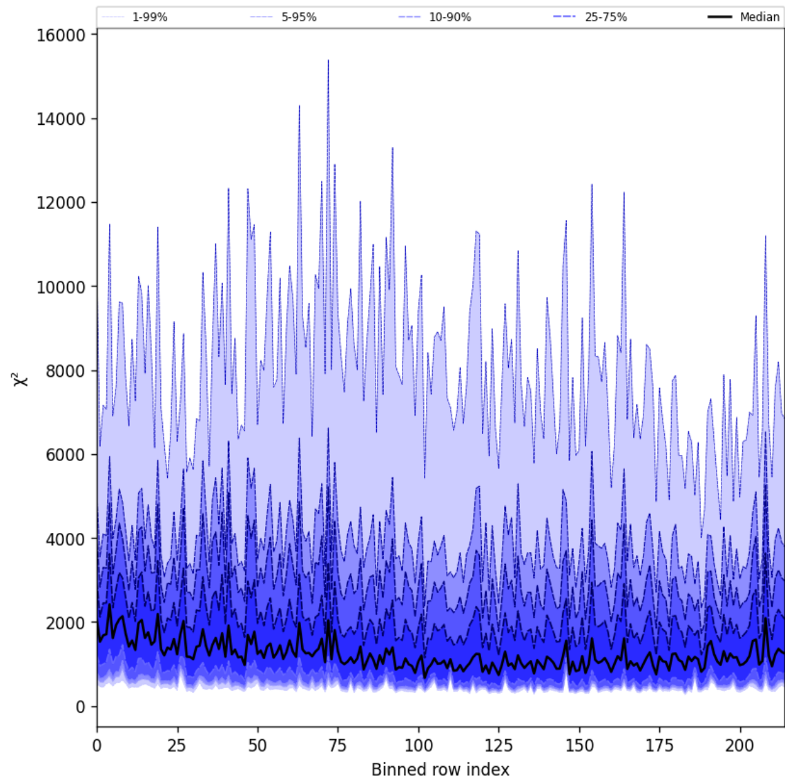
Figure 24: Along track statistics of “ \chi^2 ” for 2025-03-31 to 2025-03-31
