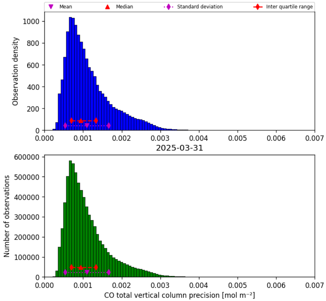
Figure 15: Histogram of “CO total vertical column precision” for 2025-03-31 to 2025-03-31
