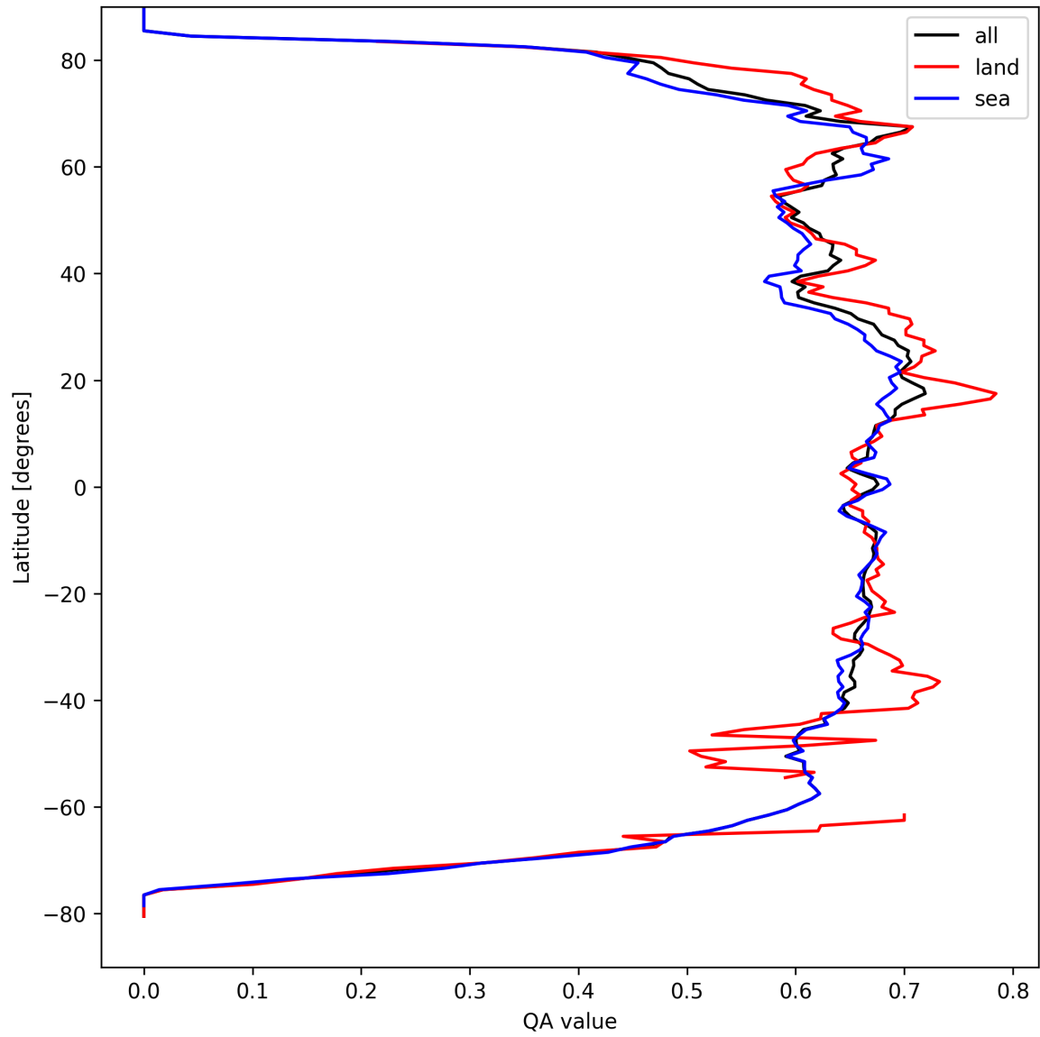
Figure 6: Zonal average of “QA value” for 2025-03-31 to 2025-03-31.
