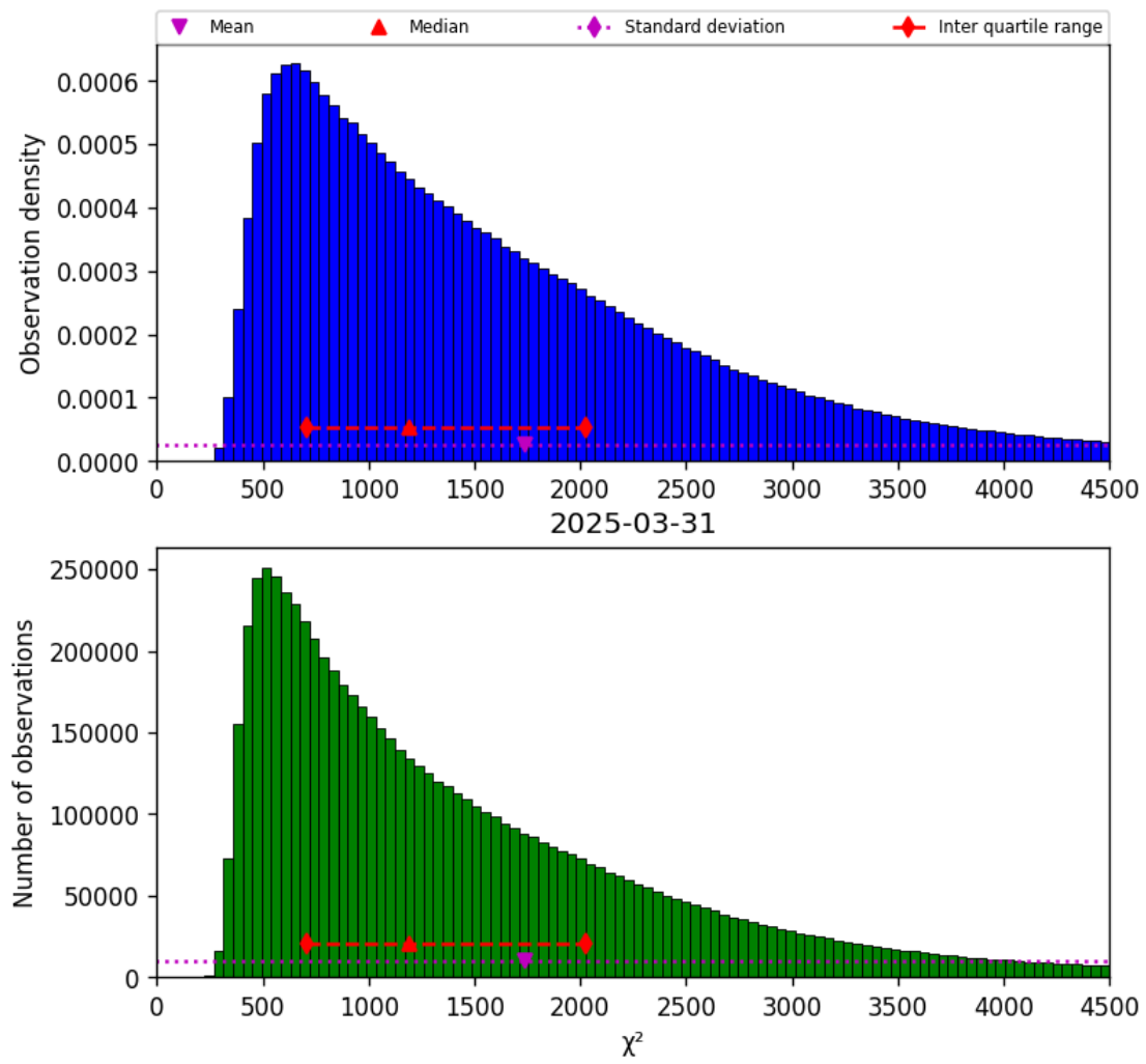
Figure 17: Histogram of " \chi^2 " for 2025-03-31 to 2025-03-31
