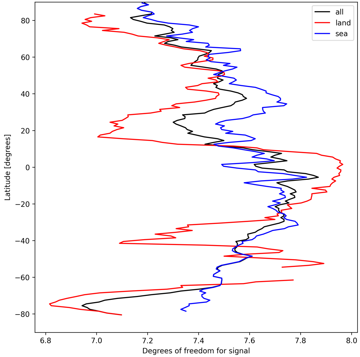
Figure 11: Zonal average of “Degrees of freedom for signal” for 2025-03-31 to 2025-03-31.
