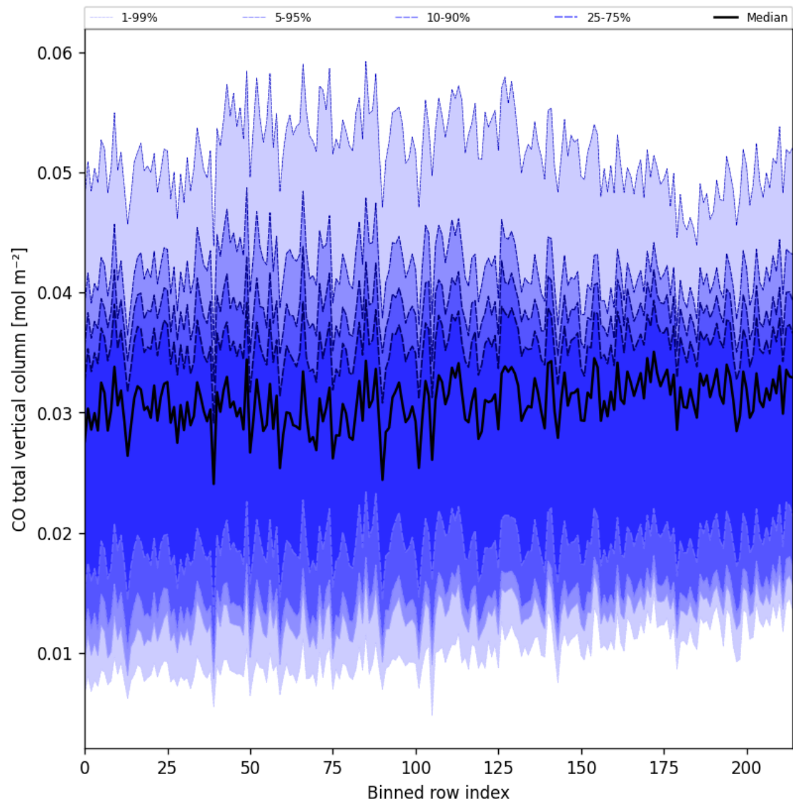
Figure 21: Along track statistics of “CO total vertical column” for 2025-03-31 to 2025-03-31
