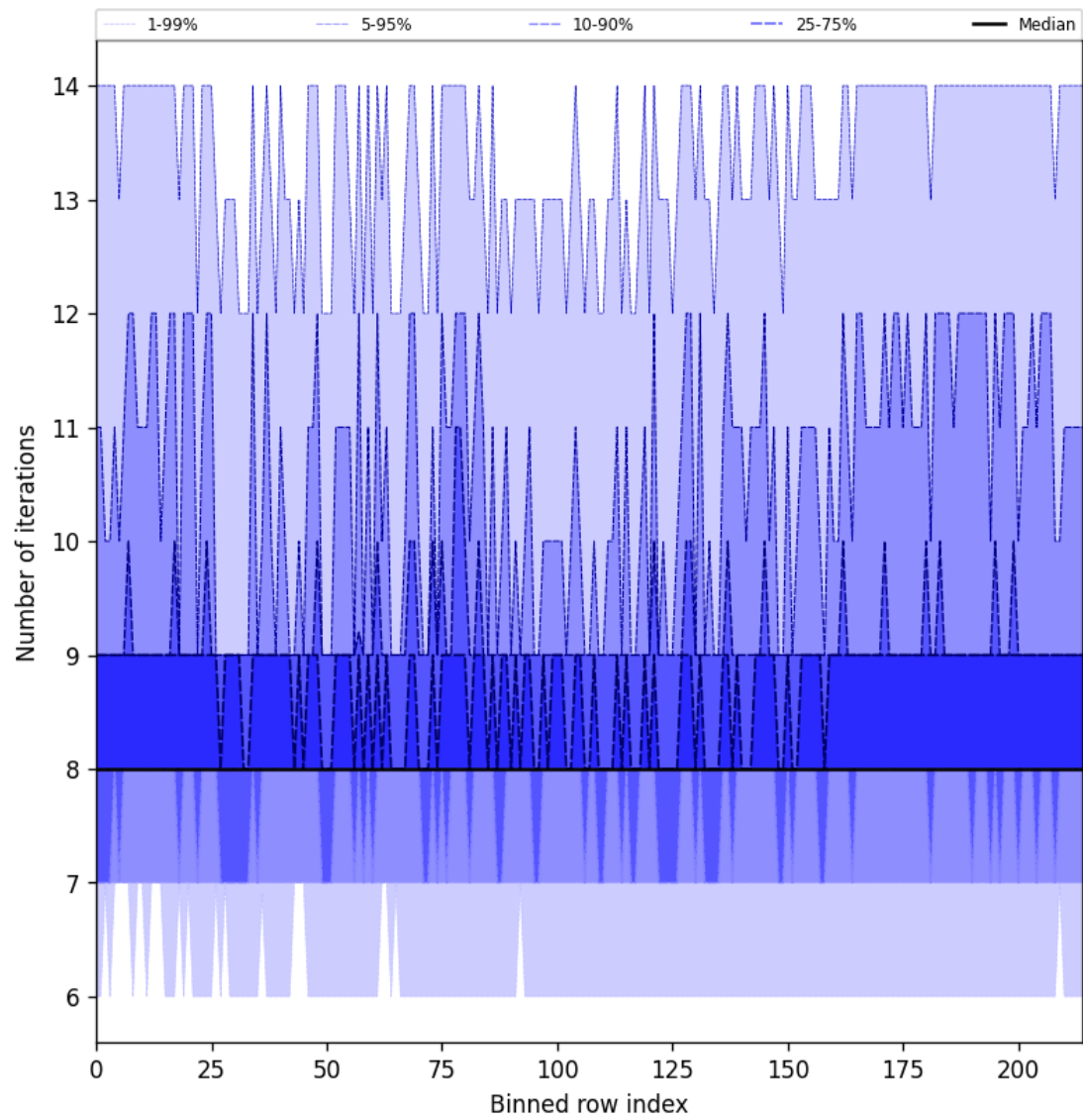
Figure 26: Along track statistics of “Number of iterations” for 2025-03-31 to 2025-03-31
