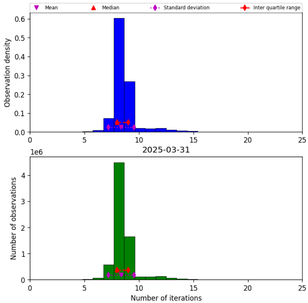
Figure 19: Histogram of “Number of iterations” for 2025-03-31 to 2025-03-31
