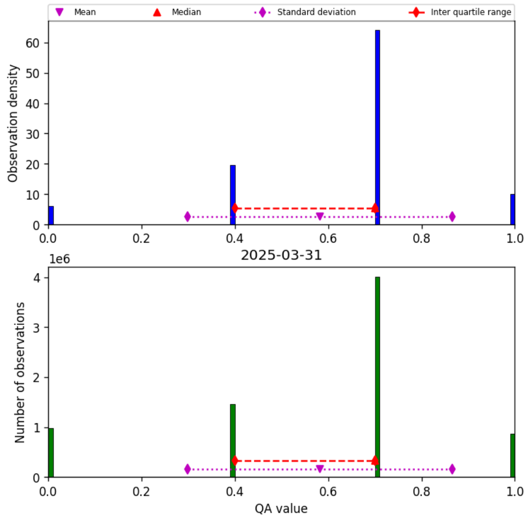
Figure 13: Histogram of “QA value” for 2025-03-31 to 2025-03-31
