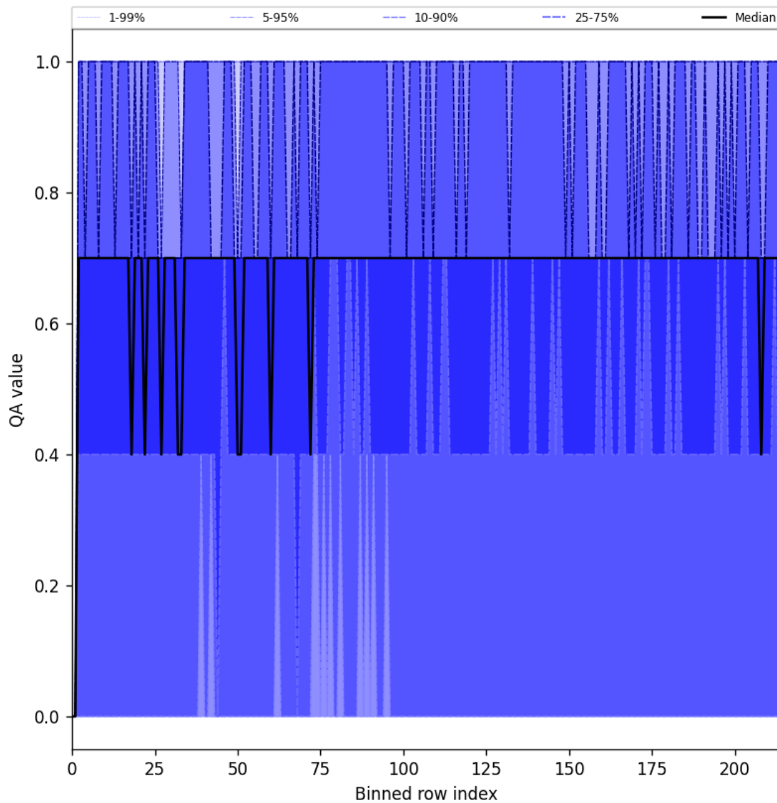
Figure 20: Along track statistics of “QA value” for 2025-03-31 to 2025-03-31
