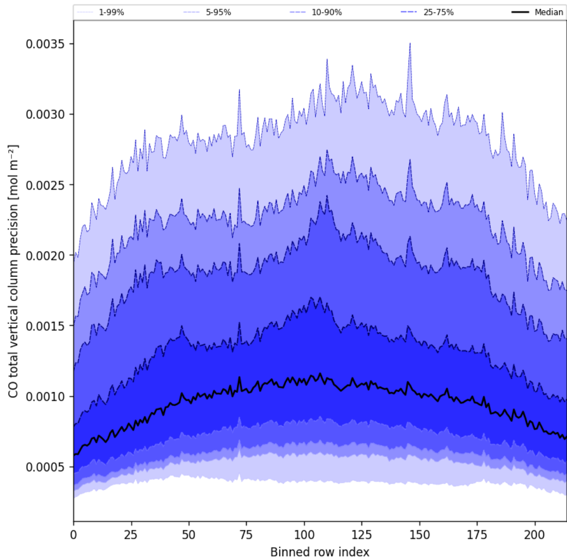
Figure 22: Along track statistics of “CO total vertical column precision” for 2025-03-31 to 2025-03-31
