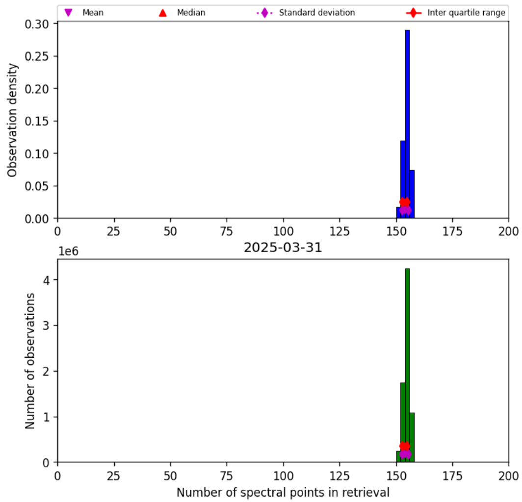
Figure 16: Histogram of “Number of spectral points in retrieval” for 2025-03-31 to 2025-03-31
