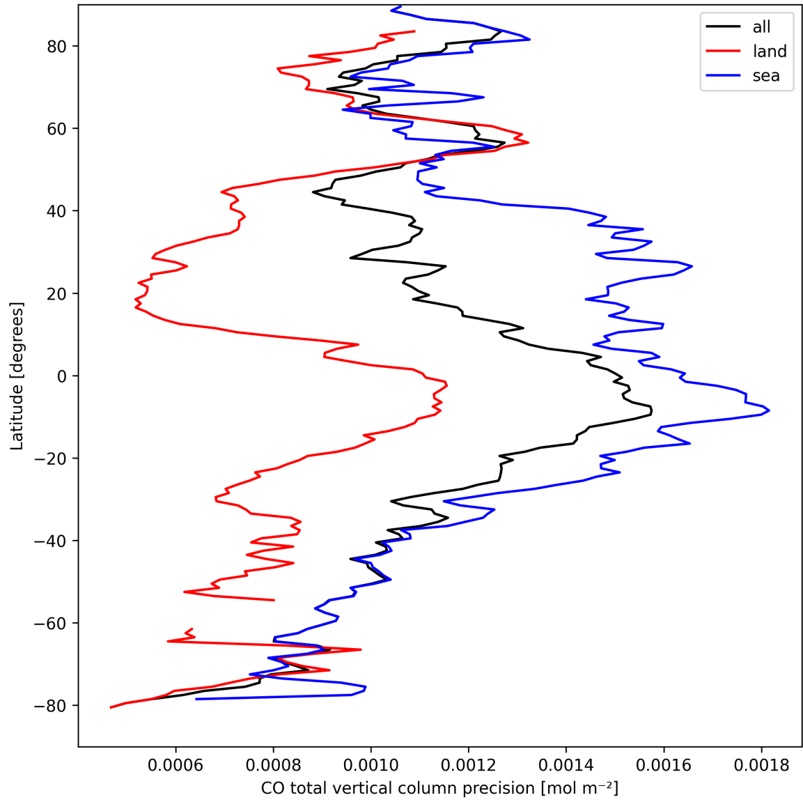
Figure 8: Zonal average of “CO total vertical column precision” for 2025-03-31 to 2025-03-31.
