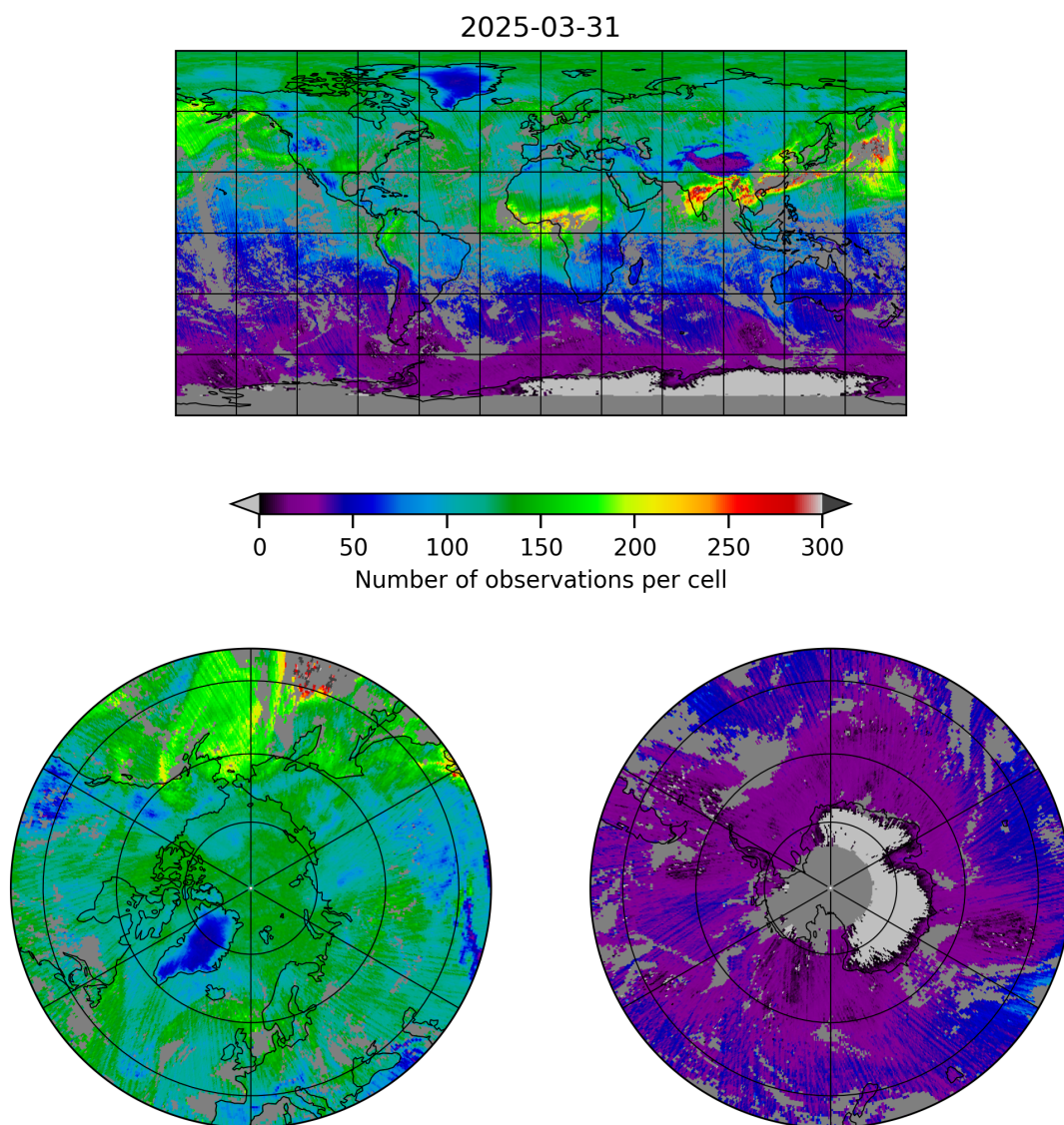
Figure 5: Map of the number of observations for 2025-03-31 to 2025-03-31
