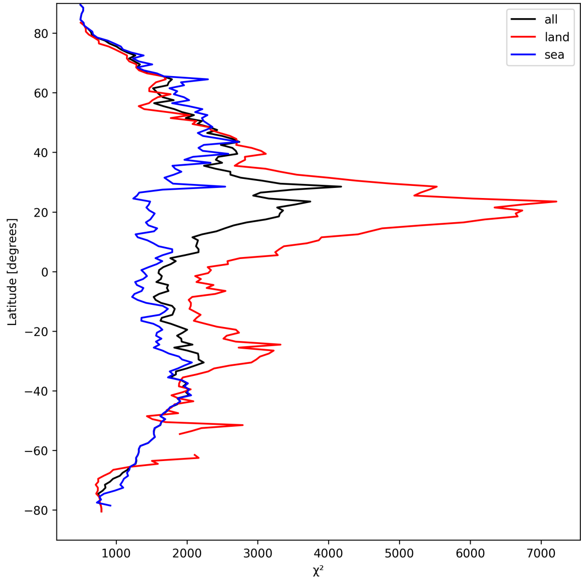
Figure 10: Zonal average of “ \chi^2 ” for 2025-03-31 to 2025-03-31.
