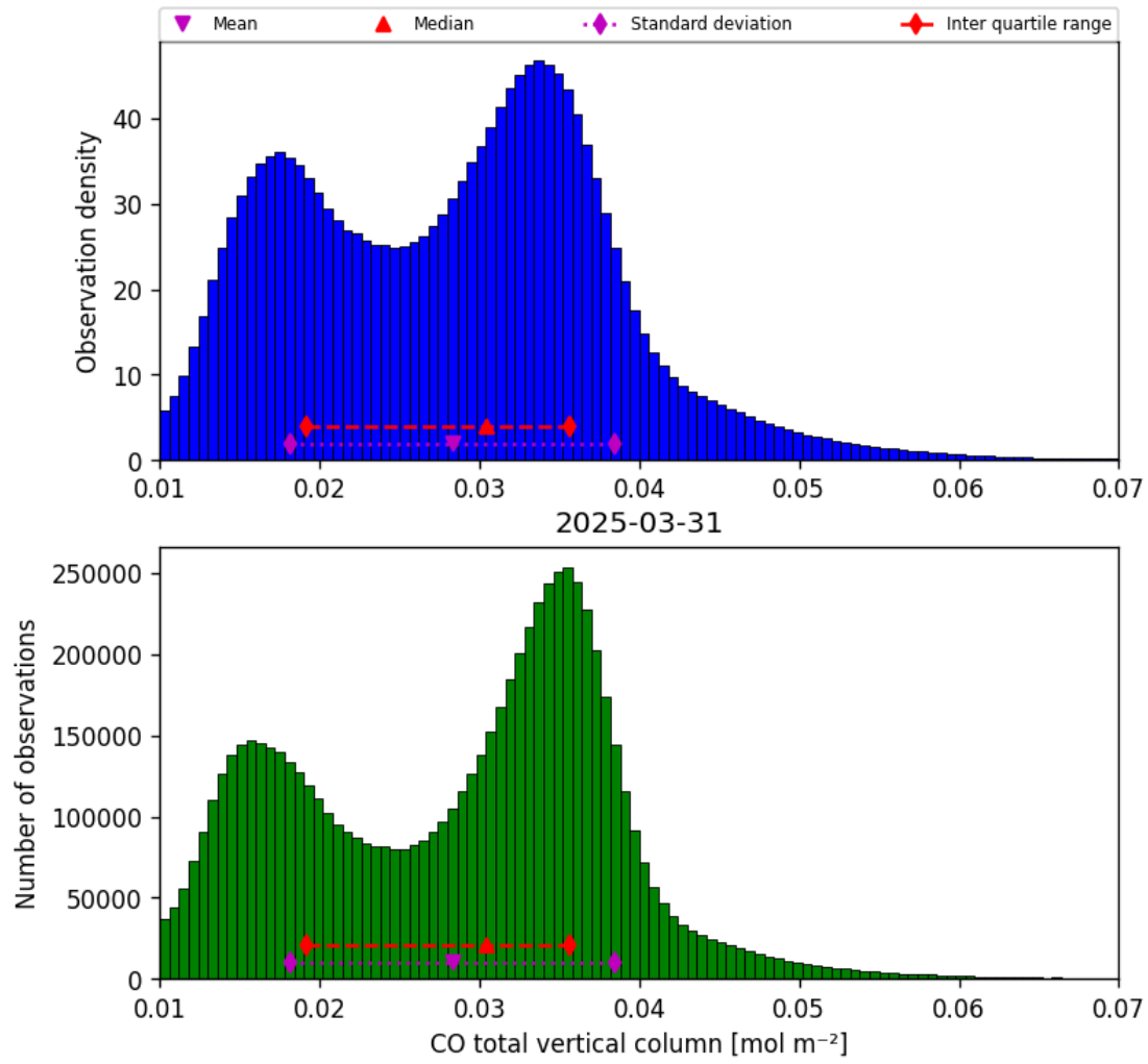
Figure 14: Histogram of “CO total vertical column” for 2025-03-31 to 2025-03-31
