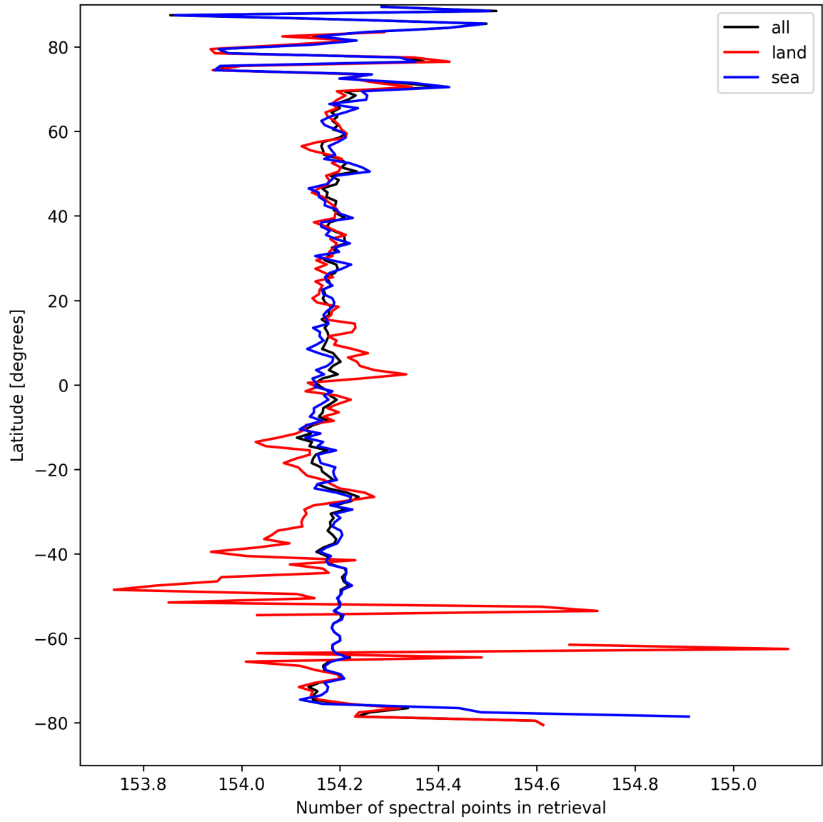
Figure 9: Zonal average of “Number of spectral points in retrieval” for 2025-03-31 to 2025-03-31.
