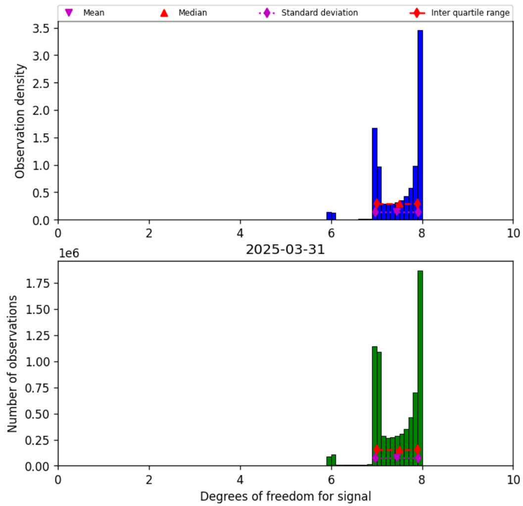
Figure 18: Histogram of “Degrees of freedom for signal” for 2025-03-31 to 2025-03-31
