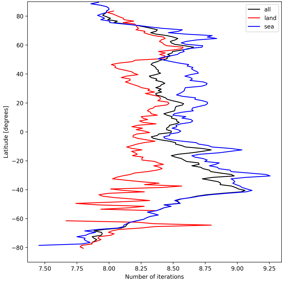
Figure 12: Zonal average of “Number of iterations” for 2025-03-31 to 2025-03-31.
