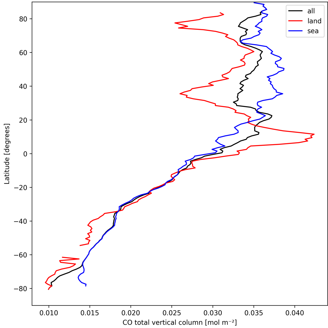
Figure 7: Zonal average of “CO total vertical column” for 2025-03-31 to 2025-03-31.
