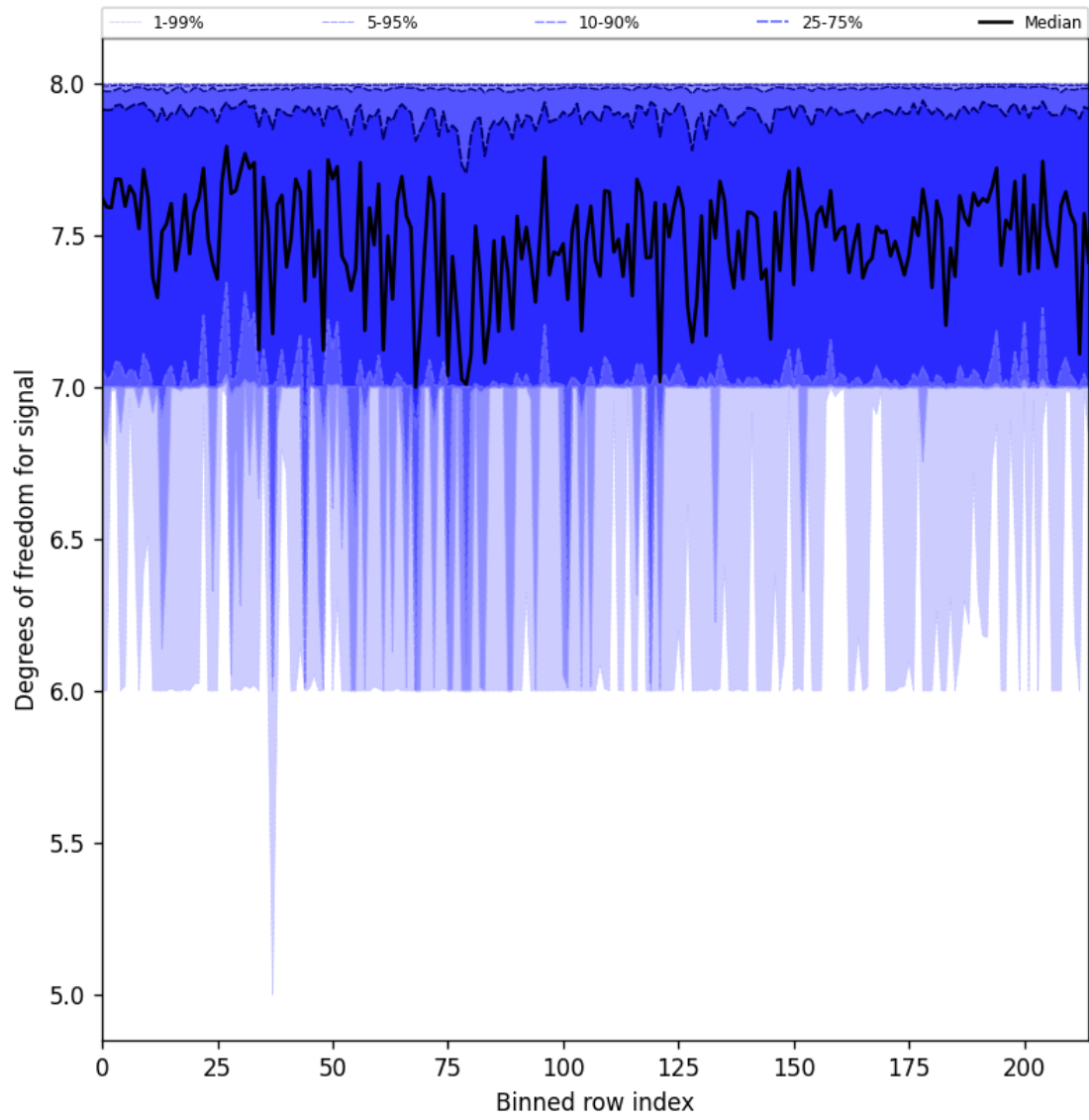
Figure 25: Along track statistics of “Degrees of freedom for signal” for 2025-03-31 to 2025-03-31
