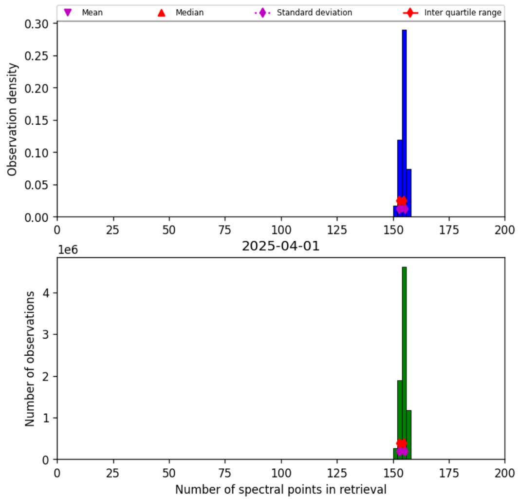
Figure 16: Histogram of “Number of spectral points in retrieval” for 2025-04-01 to 2025-04-02
