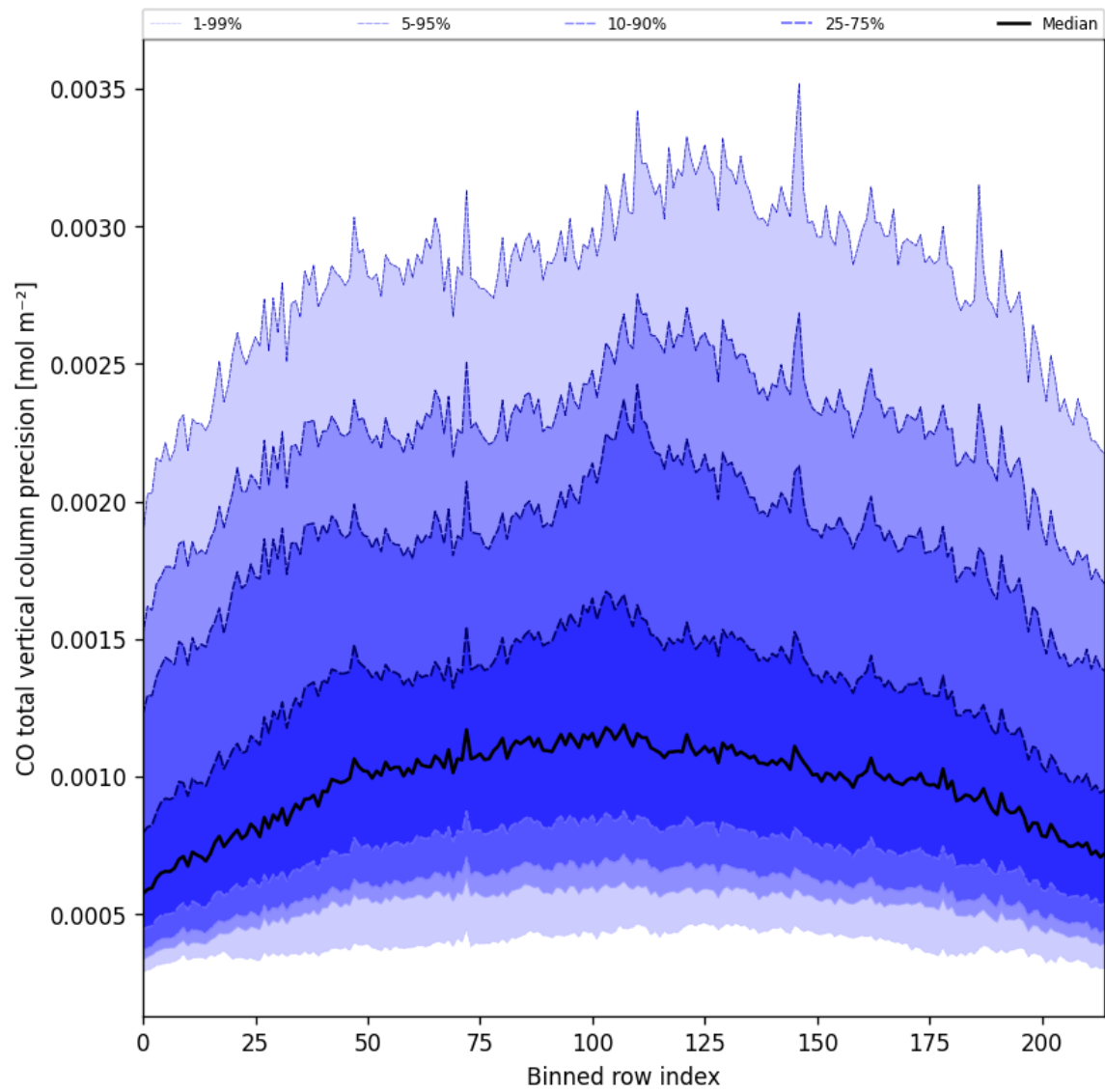
Figure 22: Along track statistics of “CO total vertical column precision” for 2025-04-01 to 2025-04-02
