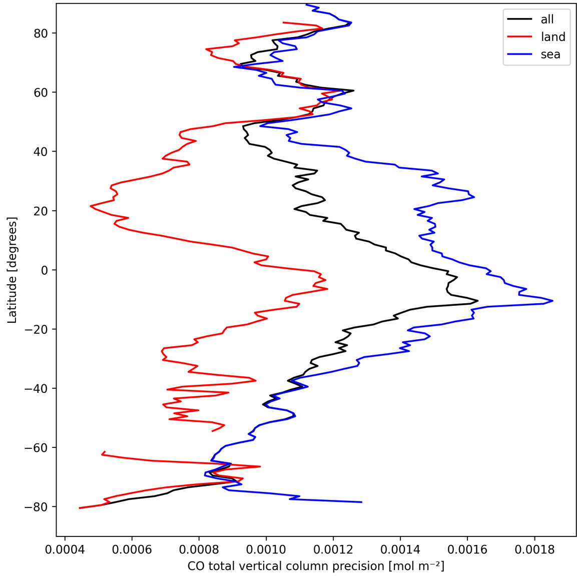
Figure 8: Zonal average of “CO total vertical column precision” for 2025-04-01 to 2025-04-02.
