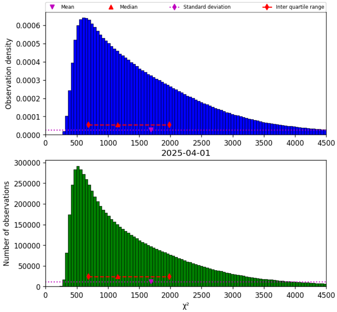
Figure 17: Histogram of “ \chi^2 ” for 2025-04-01 to 2025-04-02
