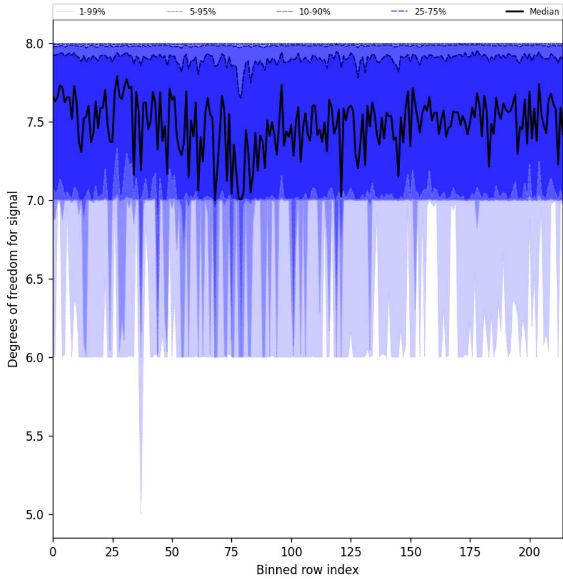
Figure 25: Along track statistics of “Degrees of freedom for signal” for 2025-04-01 to 2025-04-02
