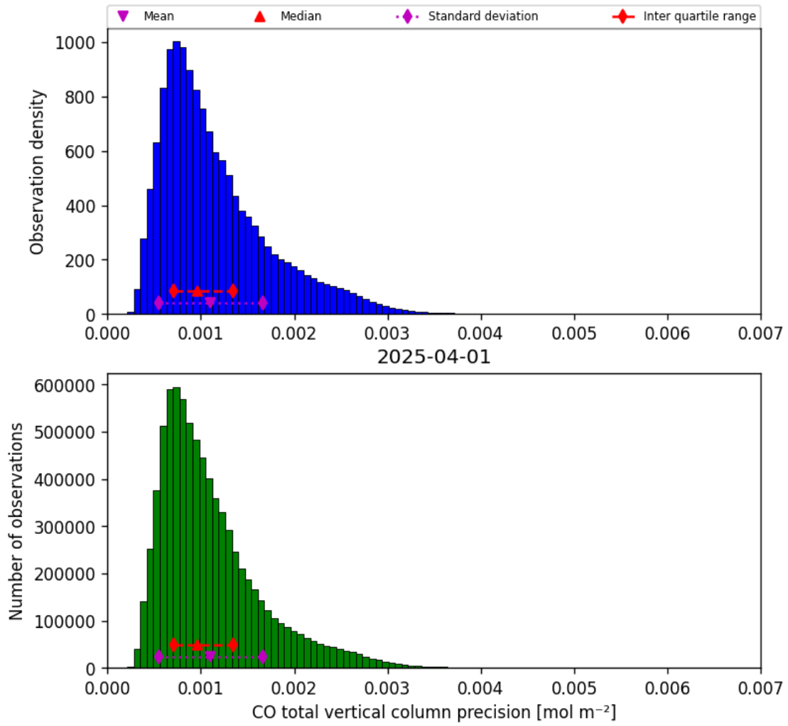
Figure 15: Histogram of “CO total vertical column precision” for 2025-04-01 to 2025-04-02
