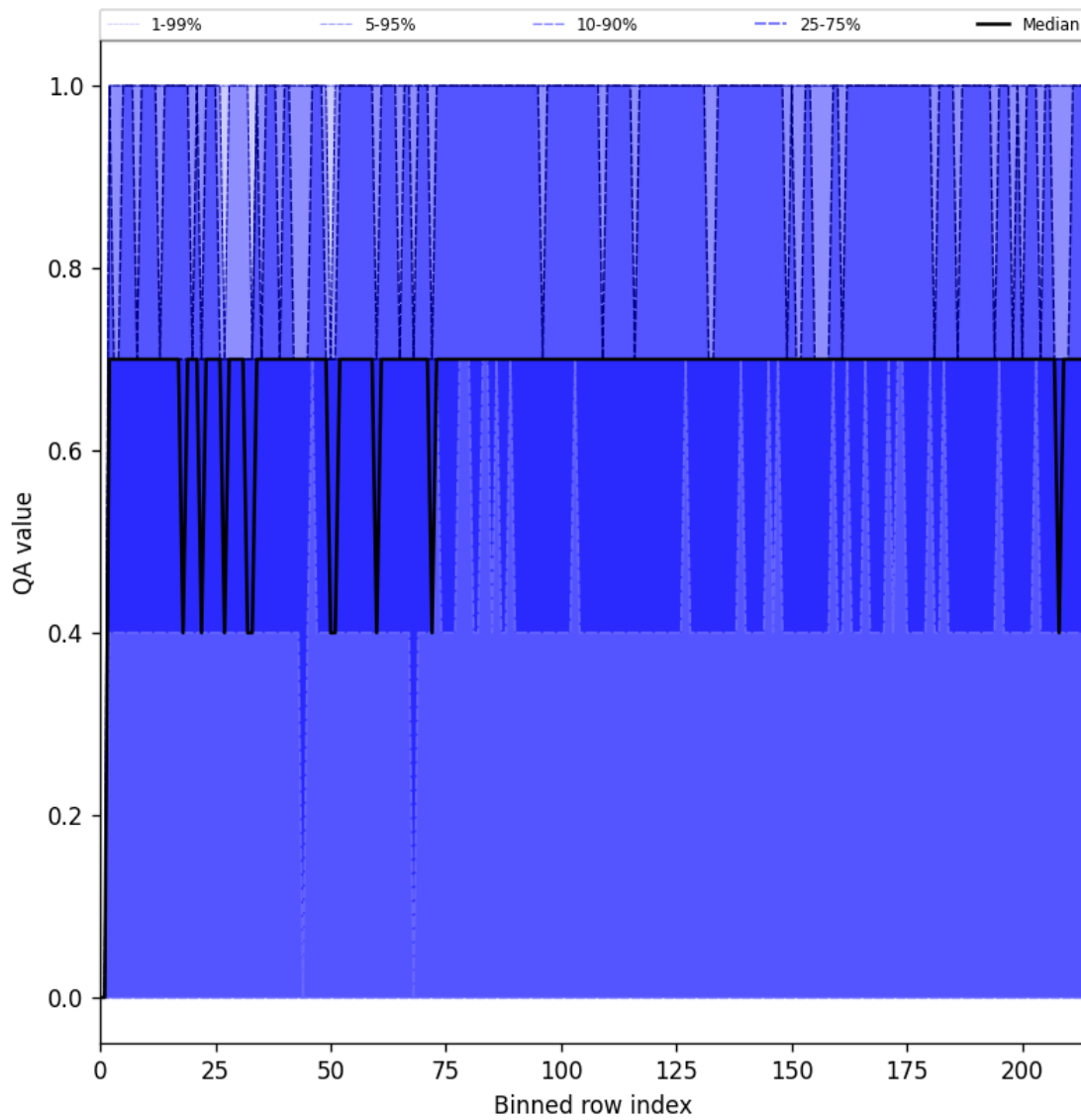
Figure 20: Along track statistics of “QA value” for 2025-04-01 to 2025-04-02
