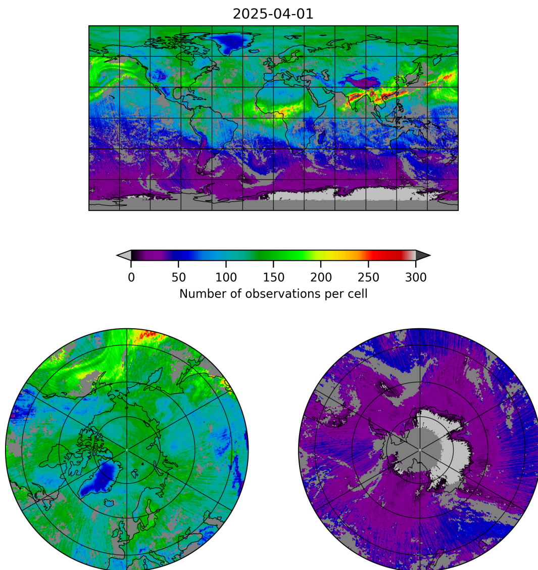
Figure 5: Map of the number of observations for 2025-04-01 to 2025-04-02
