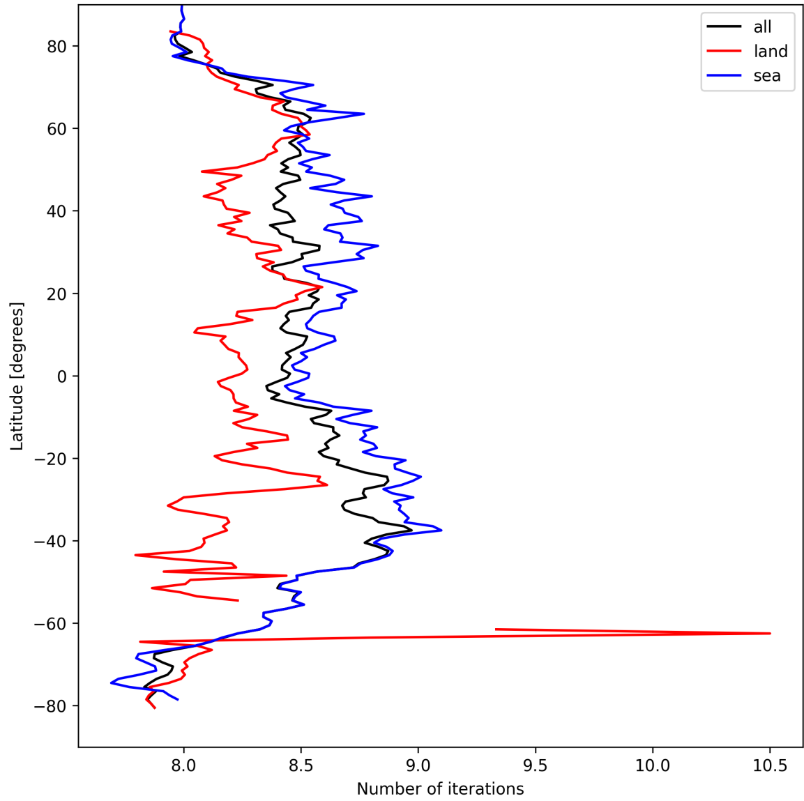
Figure 12: Zonal average of “Number of iterations” for 2025-04-01 to 2025-04-02.
