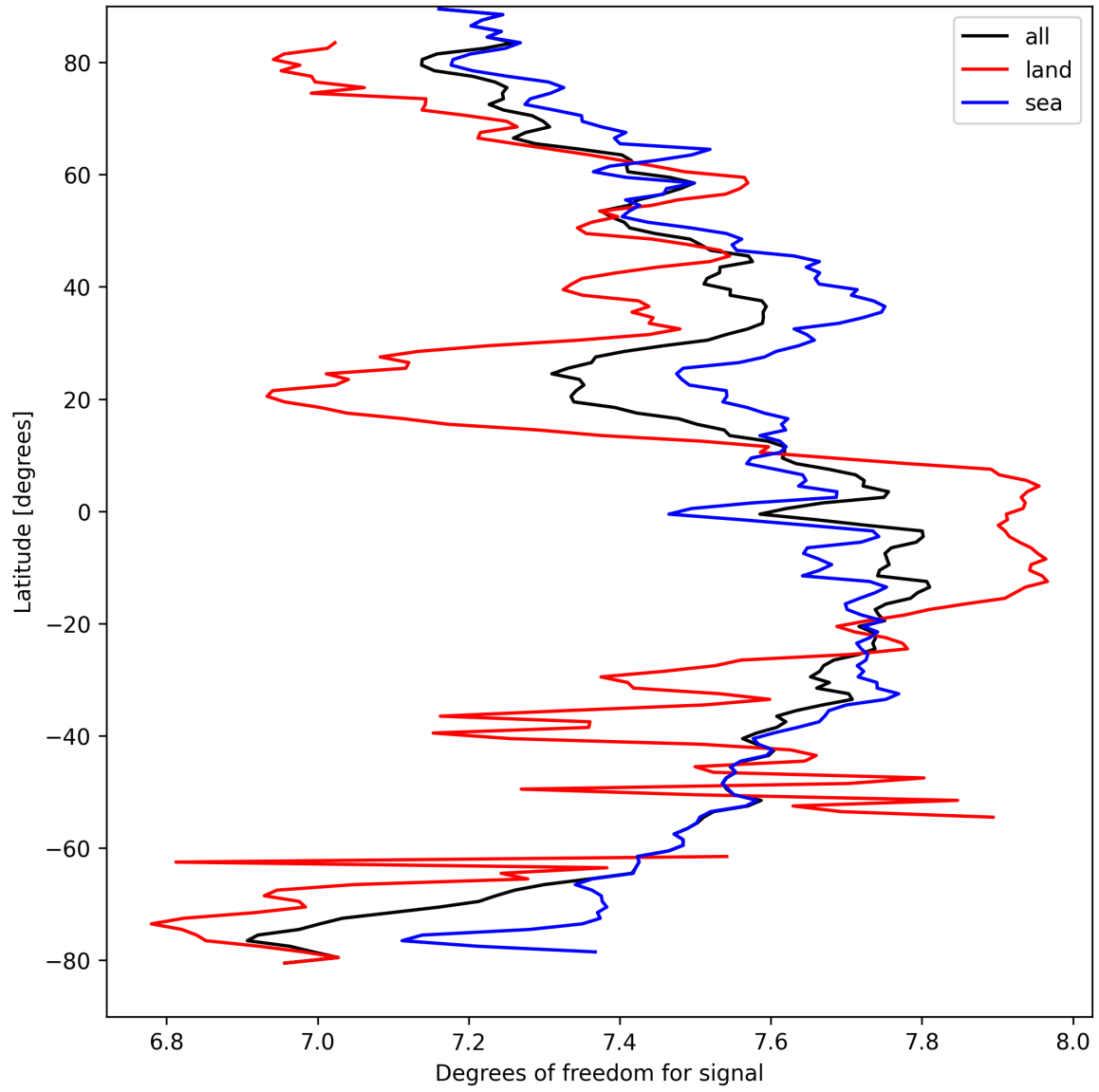
Figure 11: Zonal average of “Degrees of freedom for signal” for 2025-04-01 to 2025-04-02.
