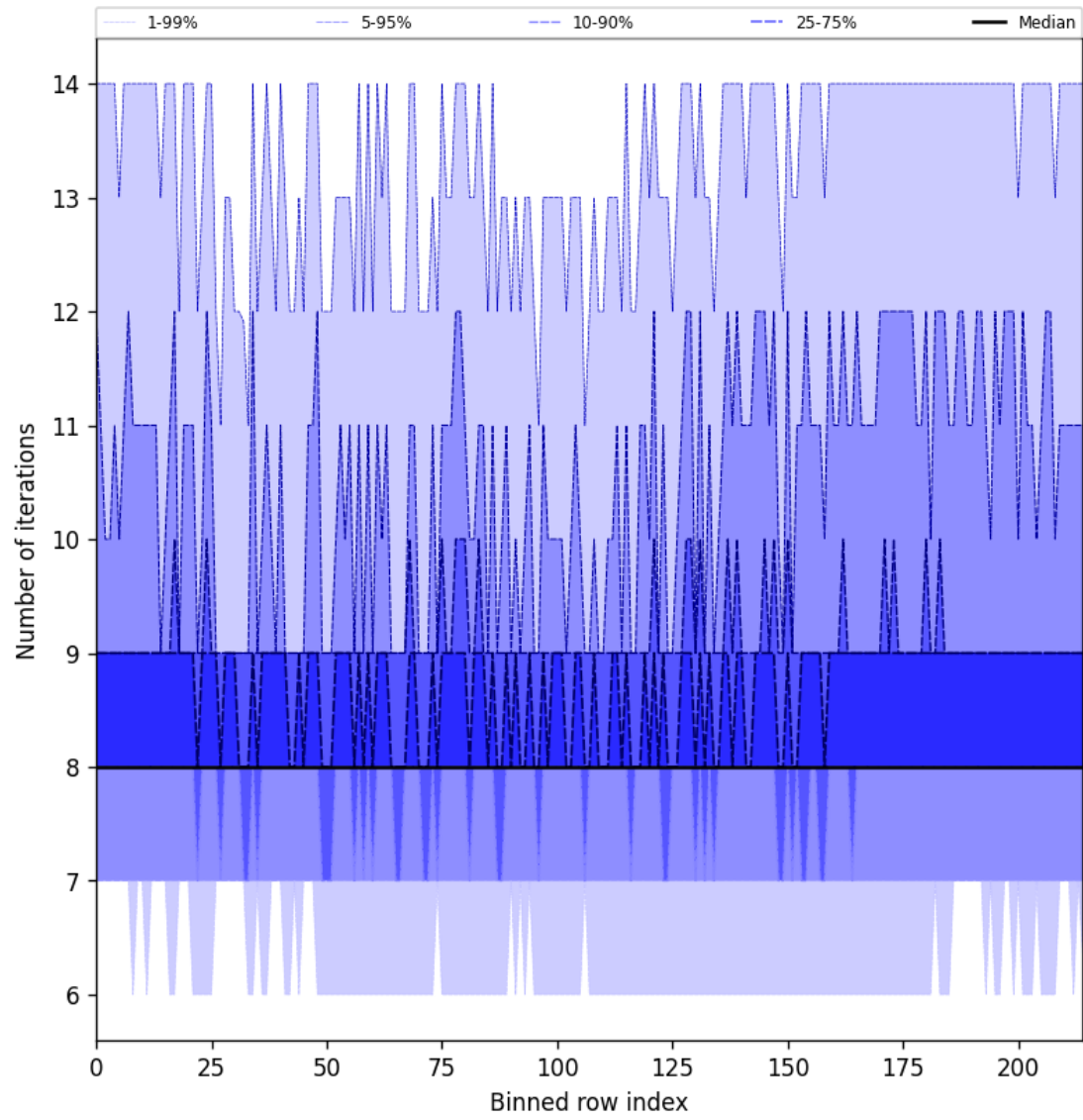
Figure 26: Along track statistics of “Number of iterations” for 2025-04-01 to 2025-04-02
