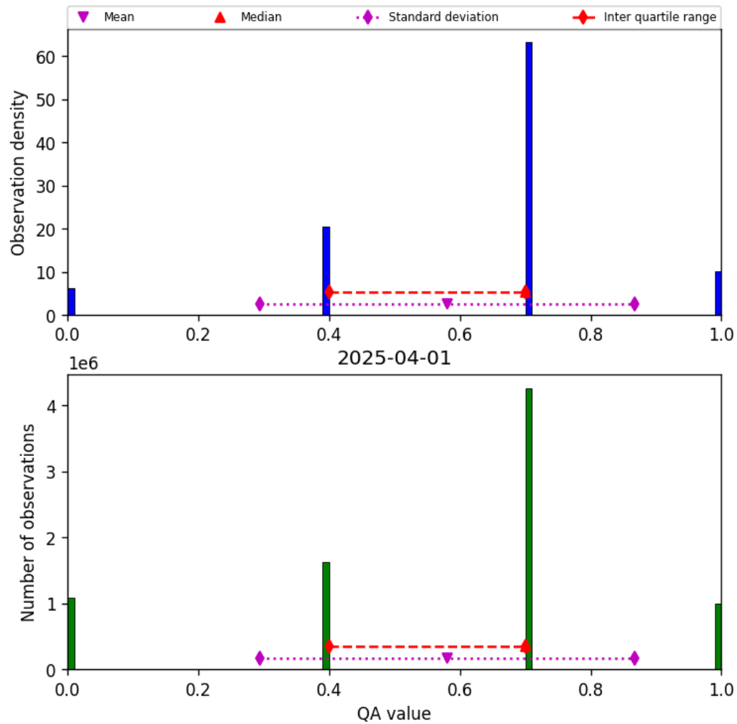
Figure 13: Histogram of “QA value” for 2025-04-01 to 2025-04-02
