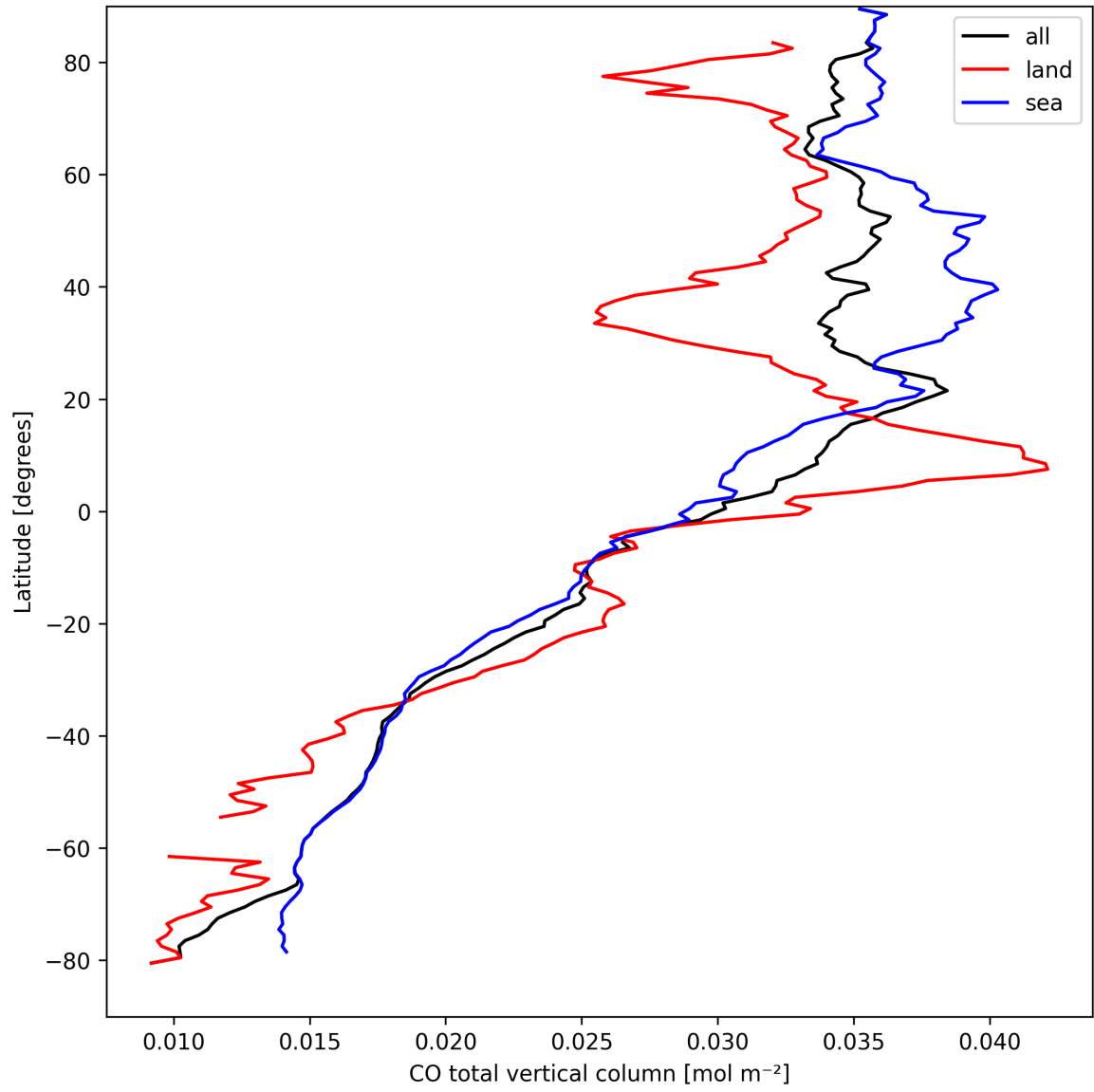
Figure 7: Zonal average of “CO total vertical column” for 2025-04-01 to 2025-04-02.
