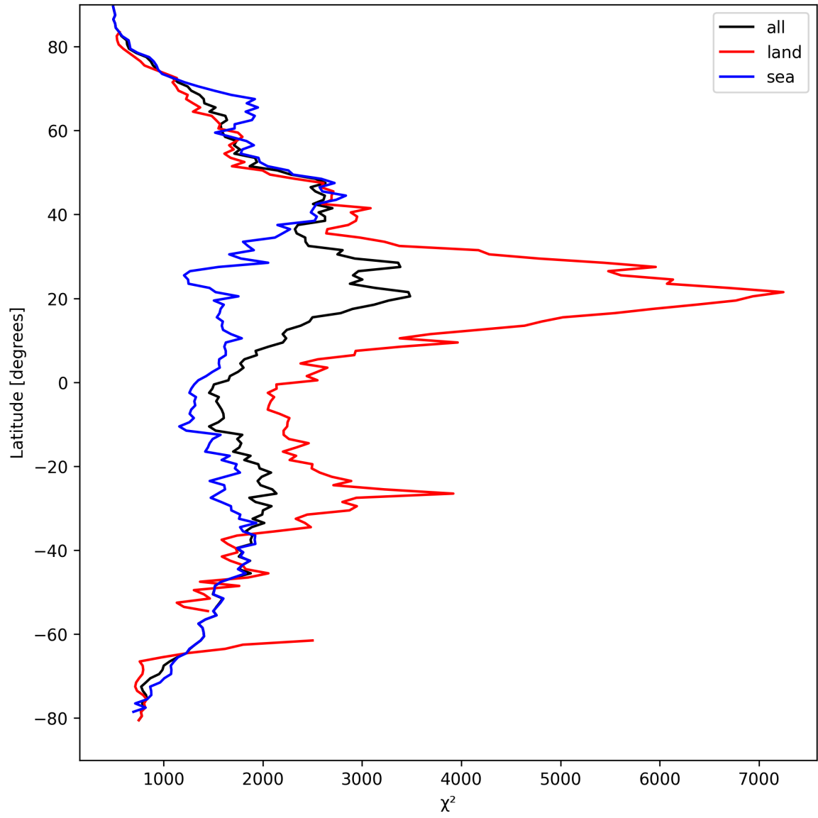
Figure 10: Zonal average of “ \chi^2 ” for 2025-04-01 to 2025-04-02.
