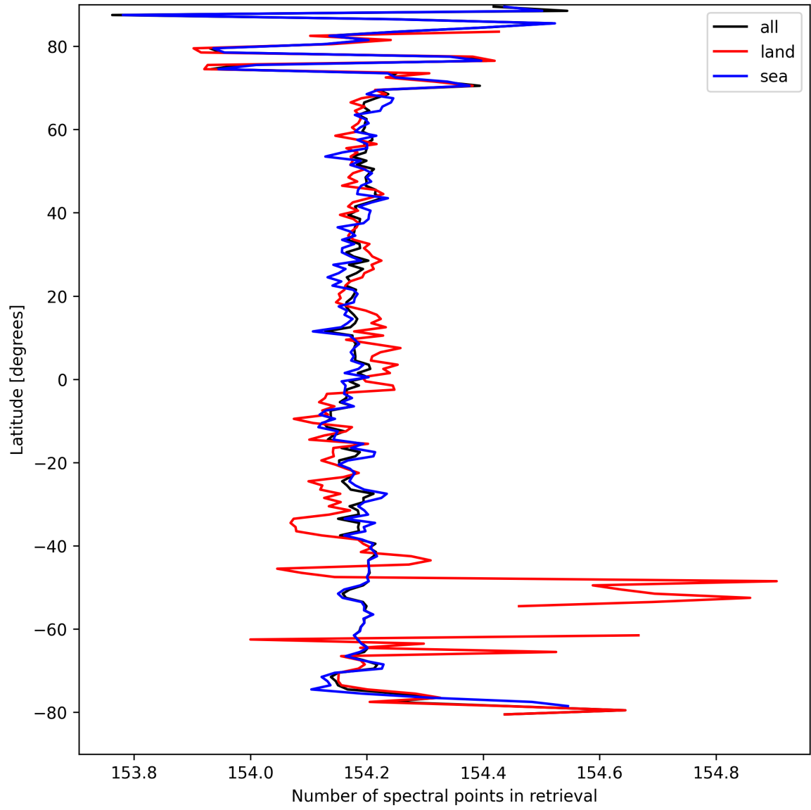
Figure 9: Zonal average of “Number of spectral points in retrieval” for 2025-04-01 to 2025-04-02.
