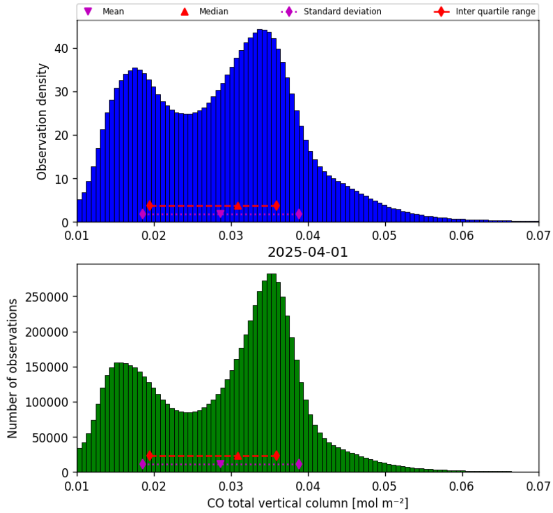
Figure 14: Histogram of “CO total vertical column” for 2025-04-01 to 2025-04-02
