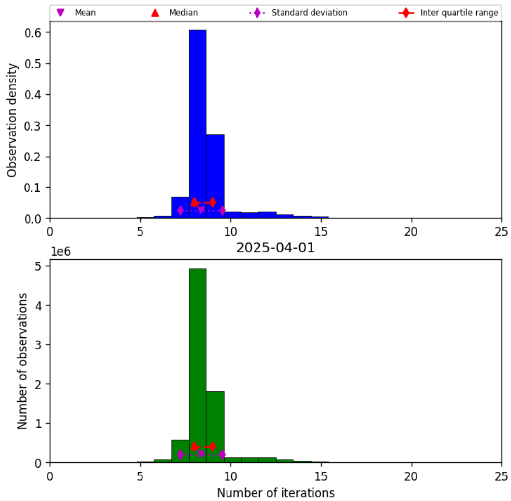
Figure 19: Histogram of “Number of iterations” for 2025-04-01 to 2025-04-02
