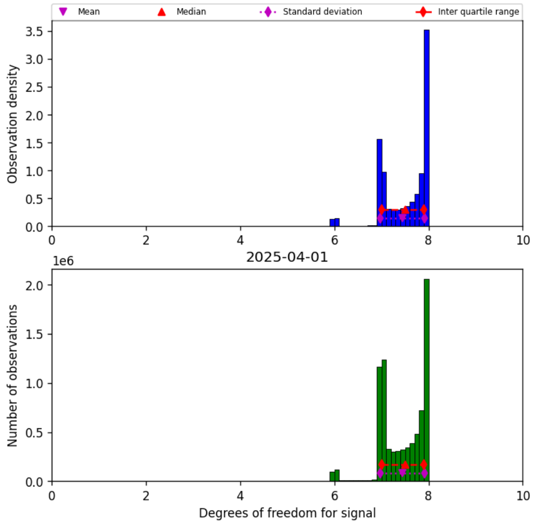
Figure 18: Histogram of “Degrees of freedom for signal” for 2025-04-01 to 2025-04-02
