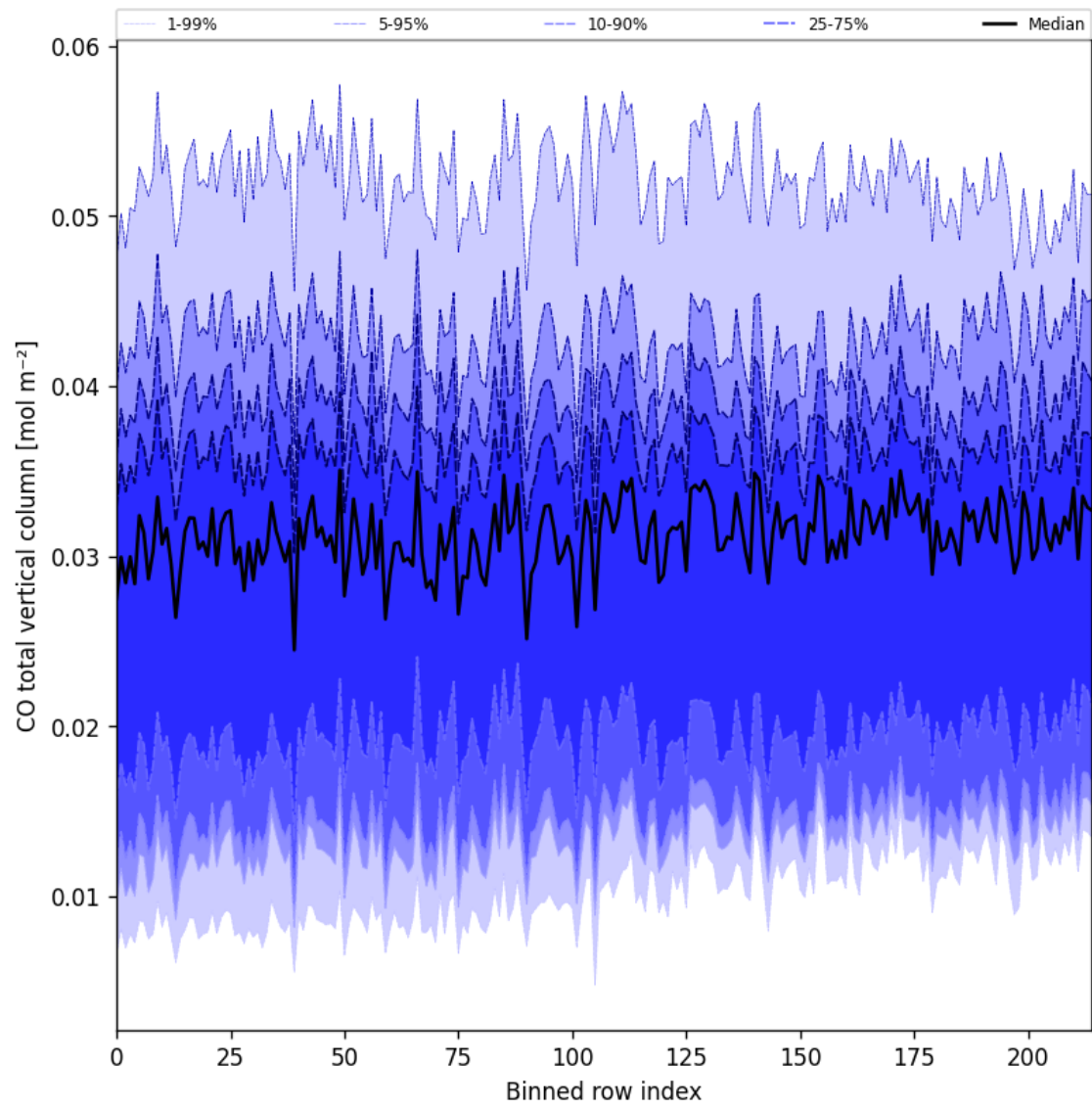
Figure 21: Along track statistics of “CO total vertical column” for 2025-04-01 to 2025-04-02
