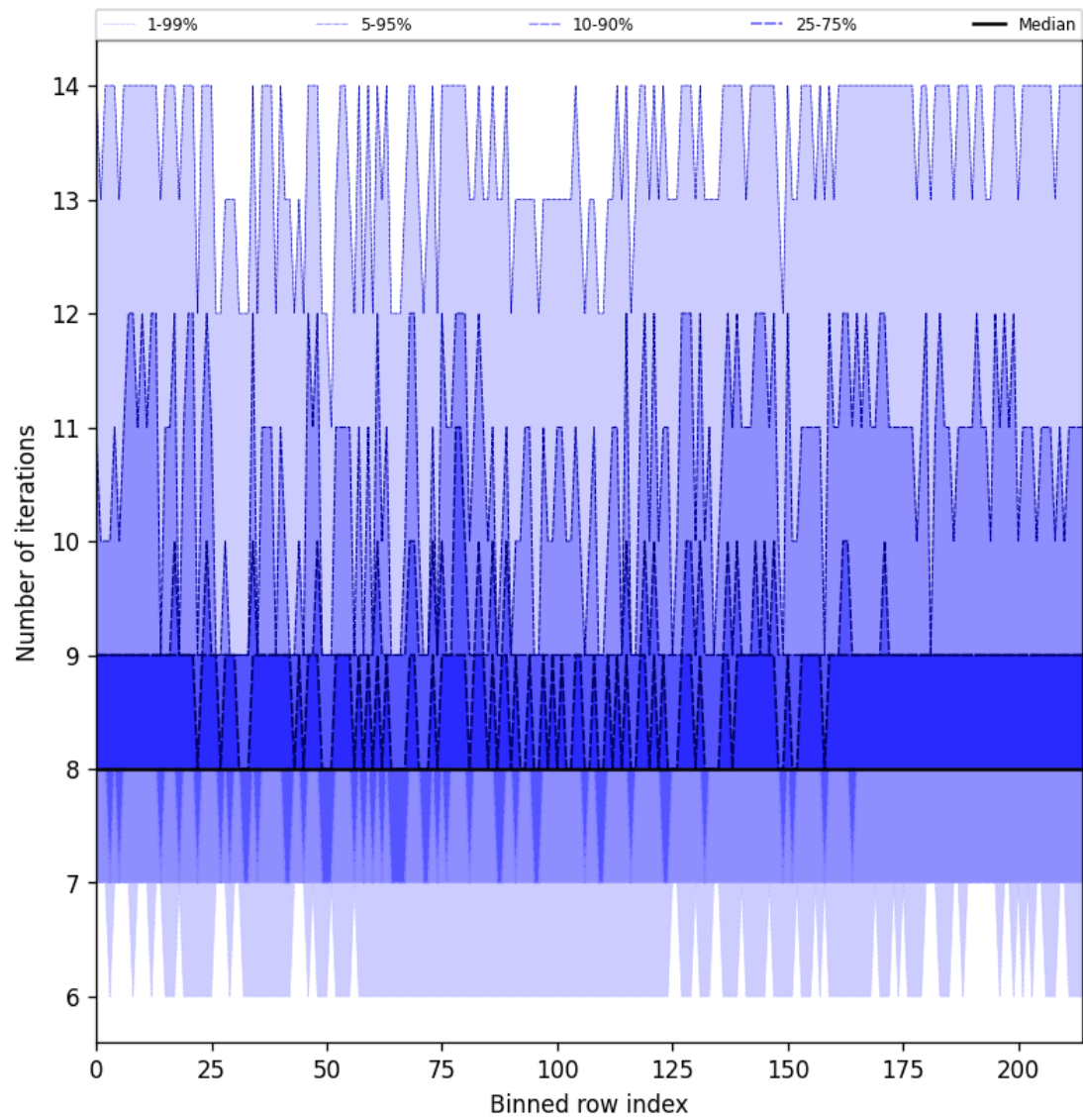
Figure 26: Along track statistics of “Number of iterations” for 2025-04-02 to 2025-04-03
