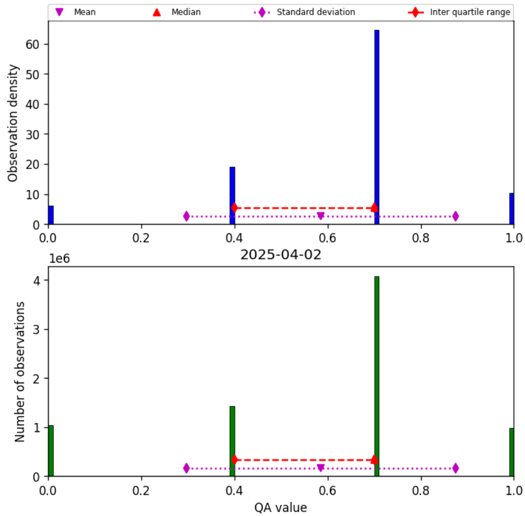
Figure 13: Histogram of “QA value” for 2025-04-02 to 2025-04-03
