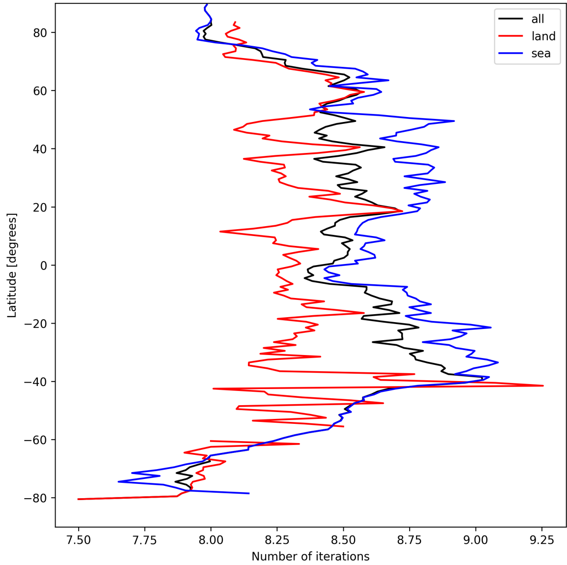
Figure 12: Zonal average of “Number of iterations” for 2025-04-02 to 2025-04-03.
