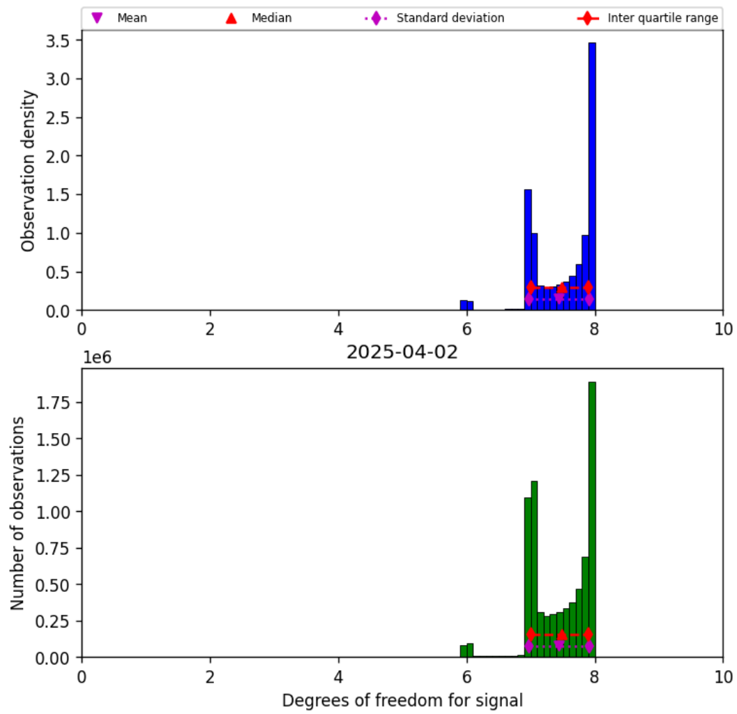
Figure 18: Histogram of “Degrees of freedom for signal” for 2025-04-02 to 2025-04-03
