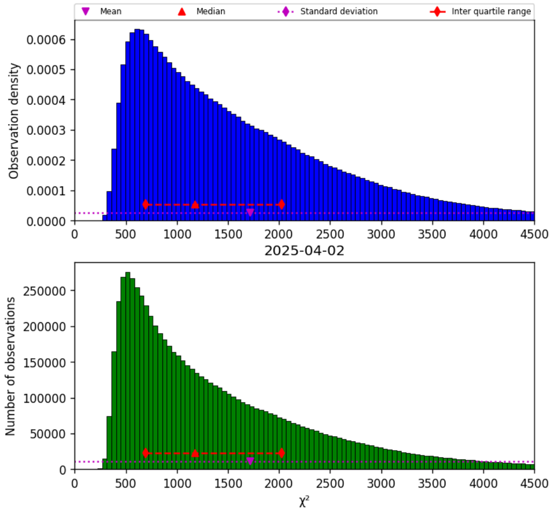
Figure 17: Histogram of “ \chi^2 ” for 2025-04-02 to 2025-04-03
