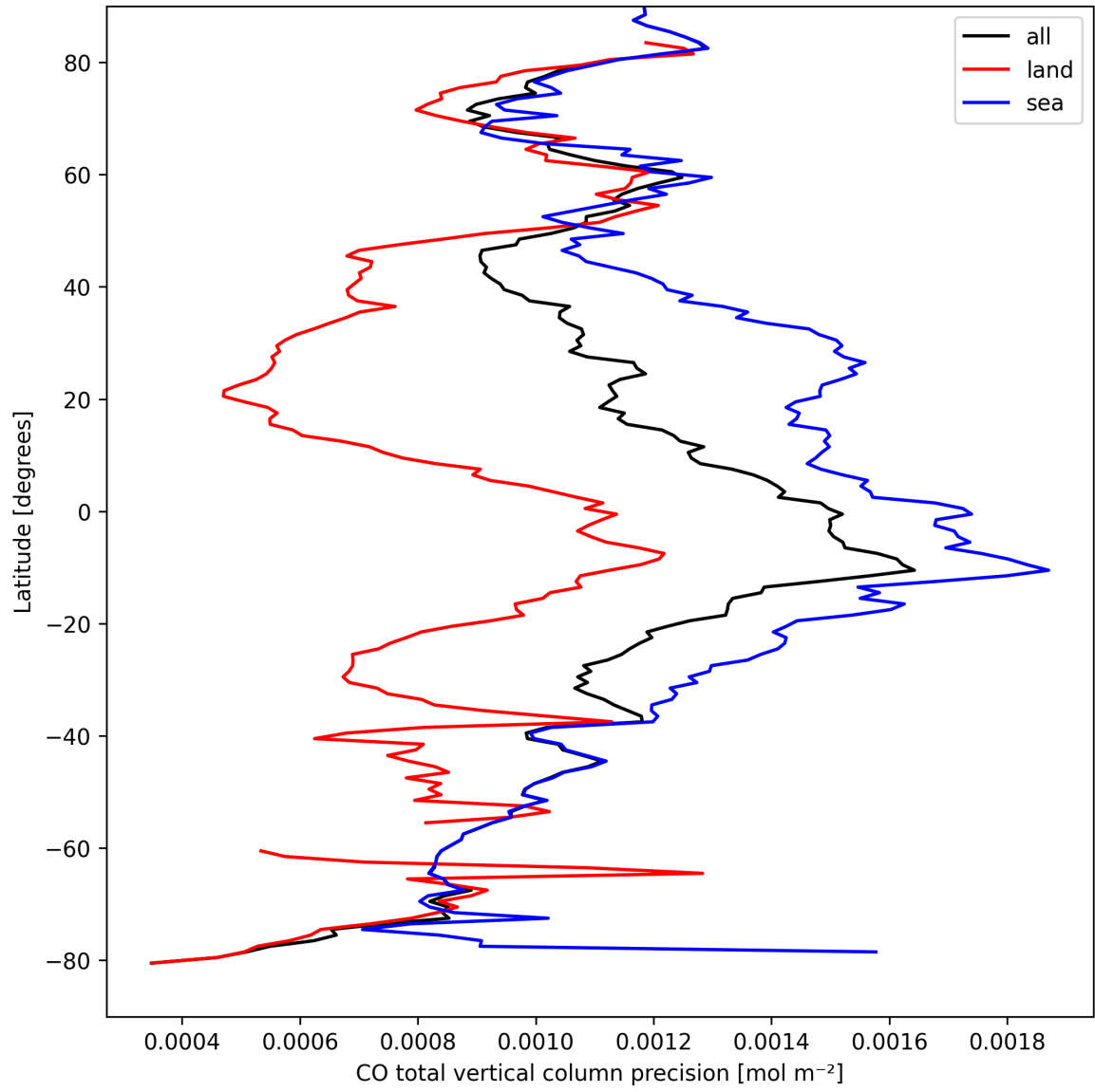
Figure 8: Zonal average of “CO total vertical column precision” for 2025-04-02 to 2025-04-03.
