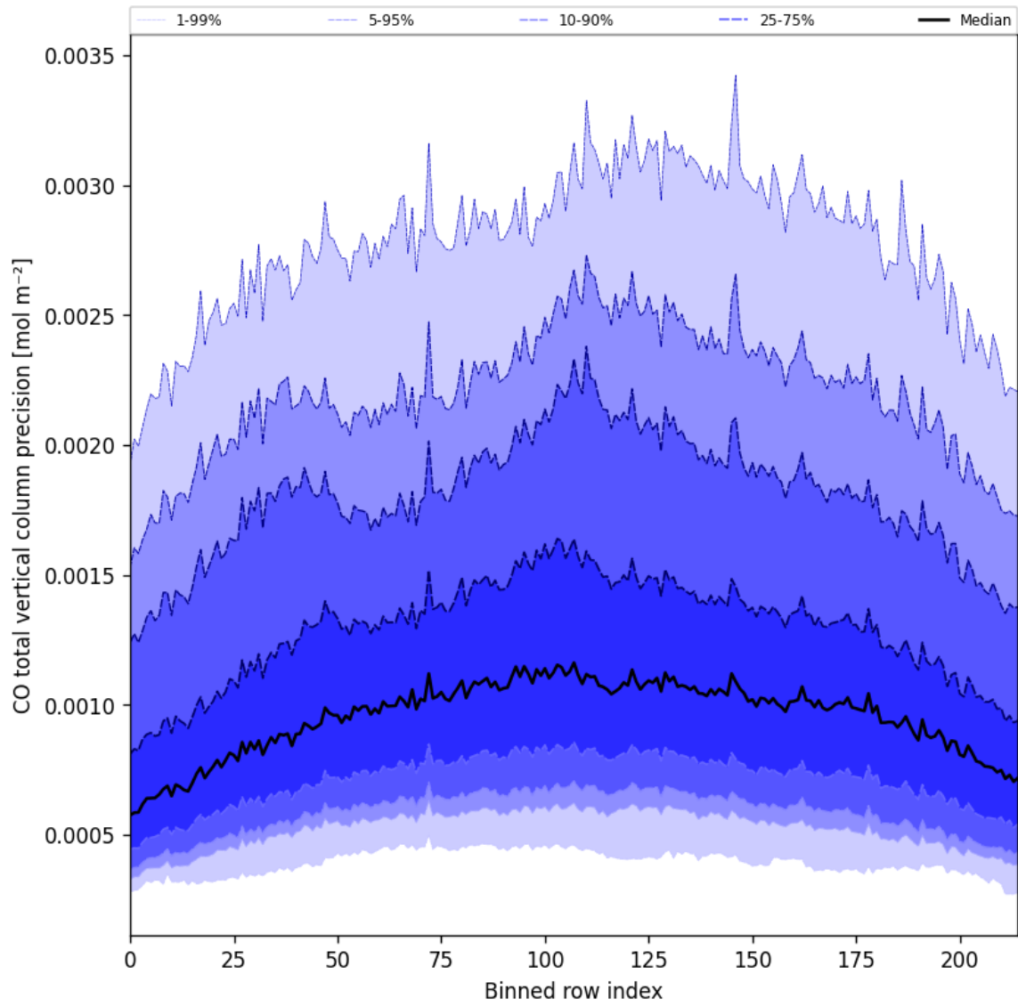
Figure 22: Along track statistics of “CO total vertical column precision” for 2025-04-02 to 2025-04-03
