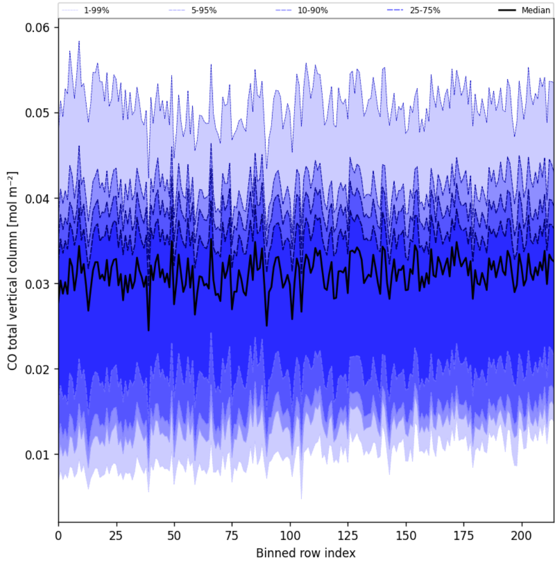
Figure 21: Along track statistics of “CO total vertical column” for 2025-04-02 to 2025-04-03
