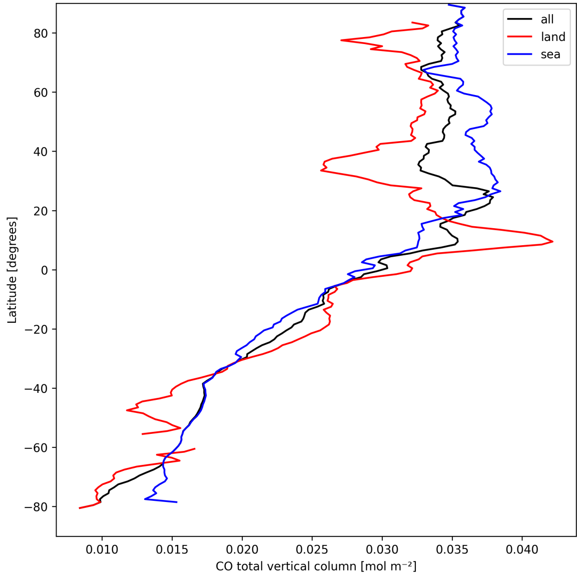
Figure 7: Zonal average of “CO total vertical column” for 2025-04-02 to 2025-04-03.
