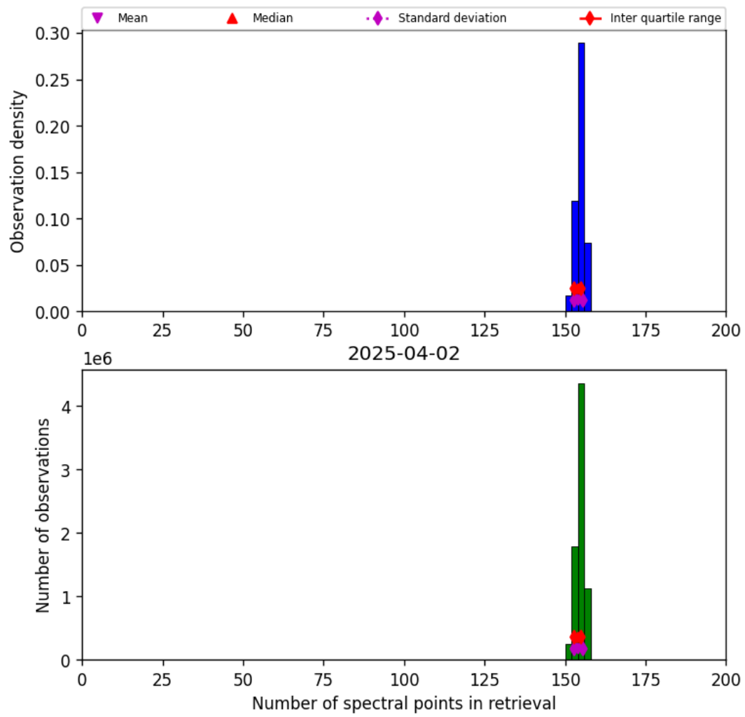
Figure 16: Histogram of “Number of spectral points in retrieval” for 2025-04-02 to 2025-04-03
