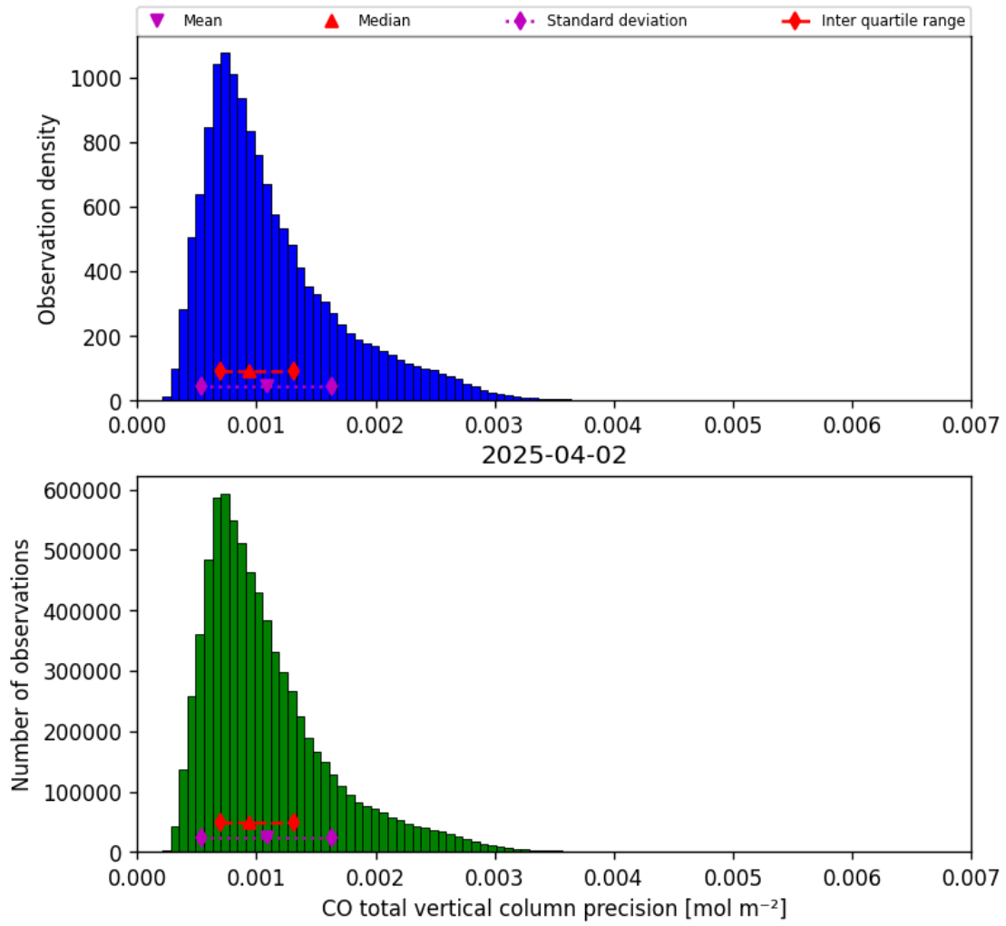
Figure 15: Histogram of “CO total vertical column precision” for 2025-04-02 to 2025-04-03
