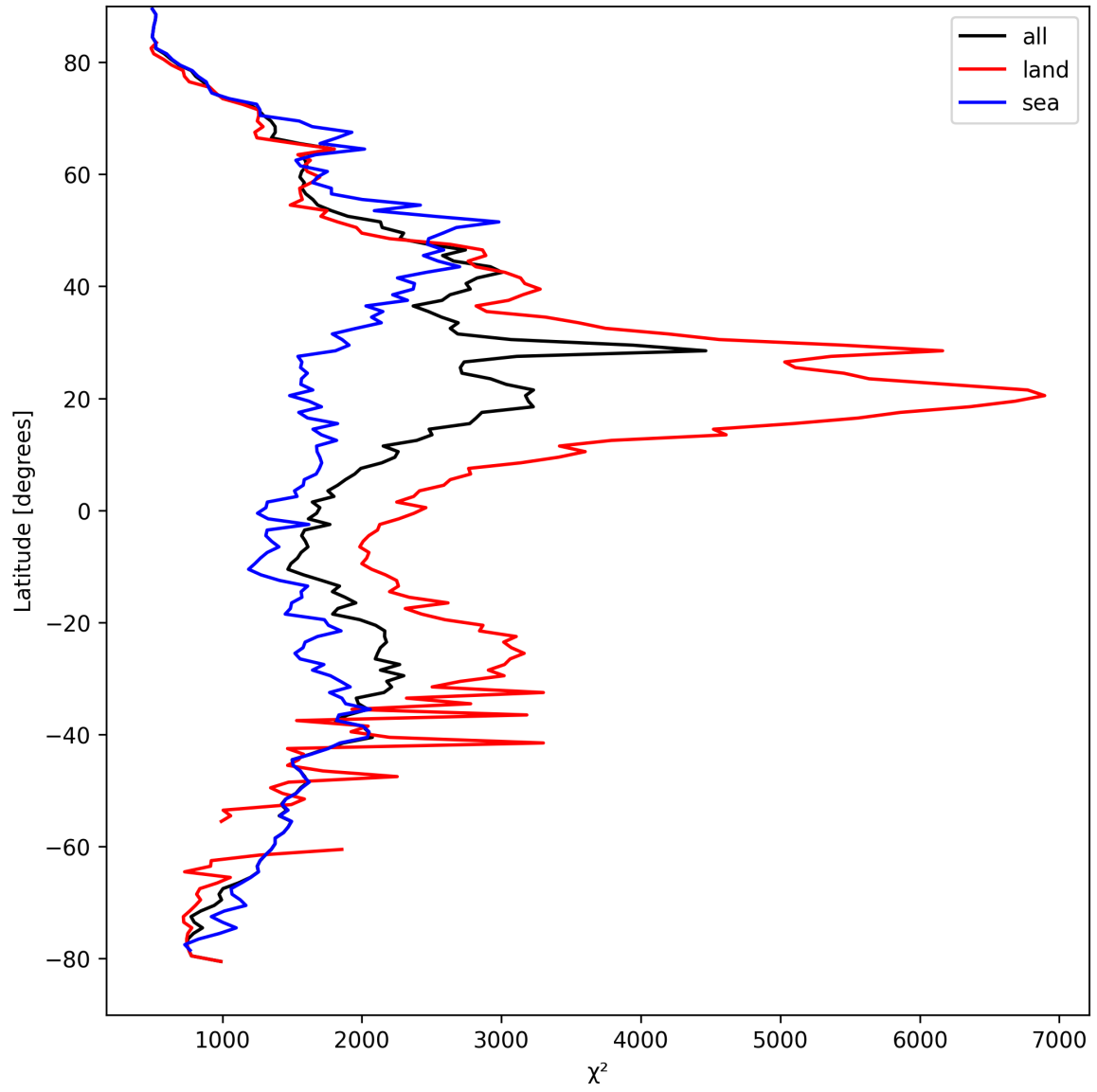
Figure 10: Zonal average of “ \chi^2 ” for 2025-04-02 to 2025-04-03.
