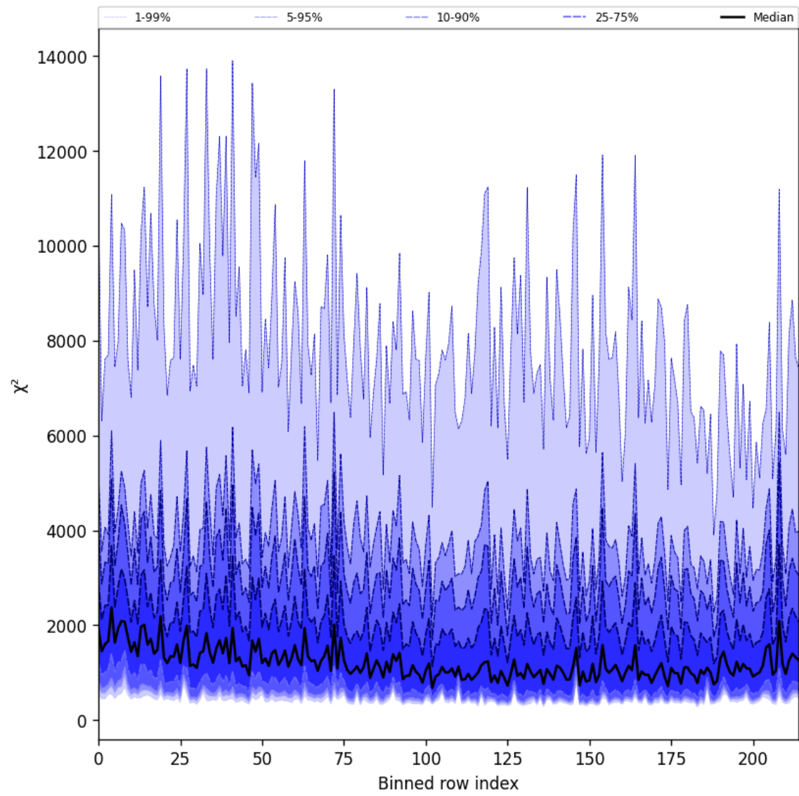
Figure 24: Along track statistics of “ \chi^2 ” for 2025-04-02 to 2025-04-03
