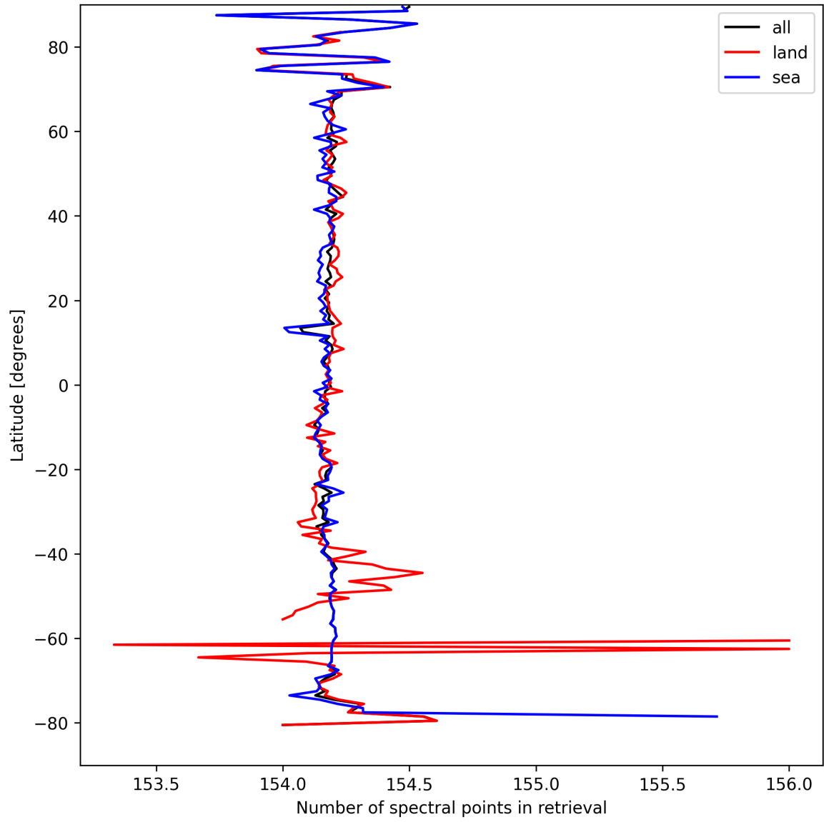
Figure 9: Zonal average of “Number of spectral points in retrieval” for 2025-04-02 to 2025-04-03.
