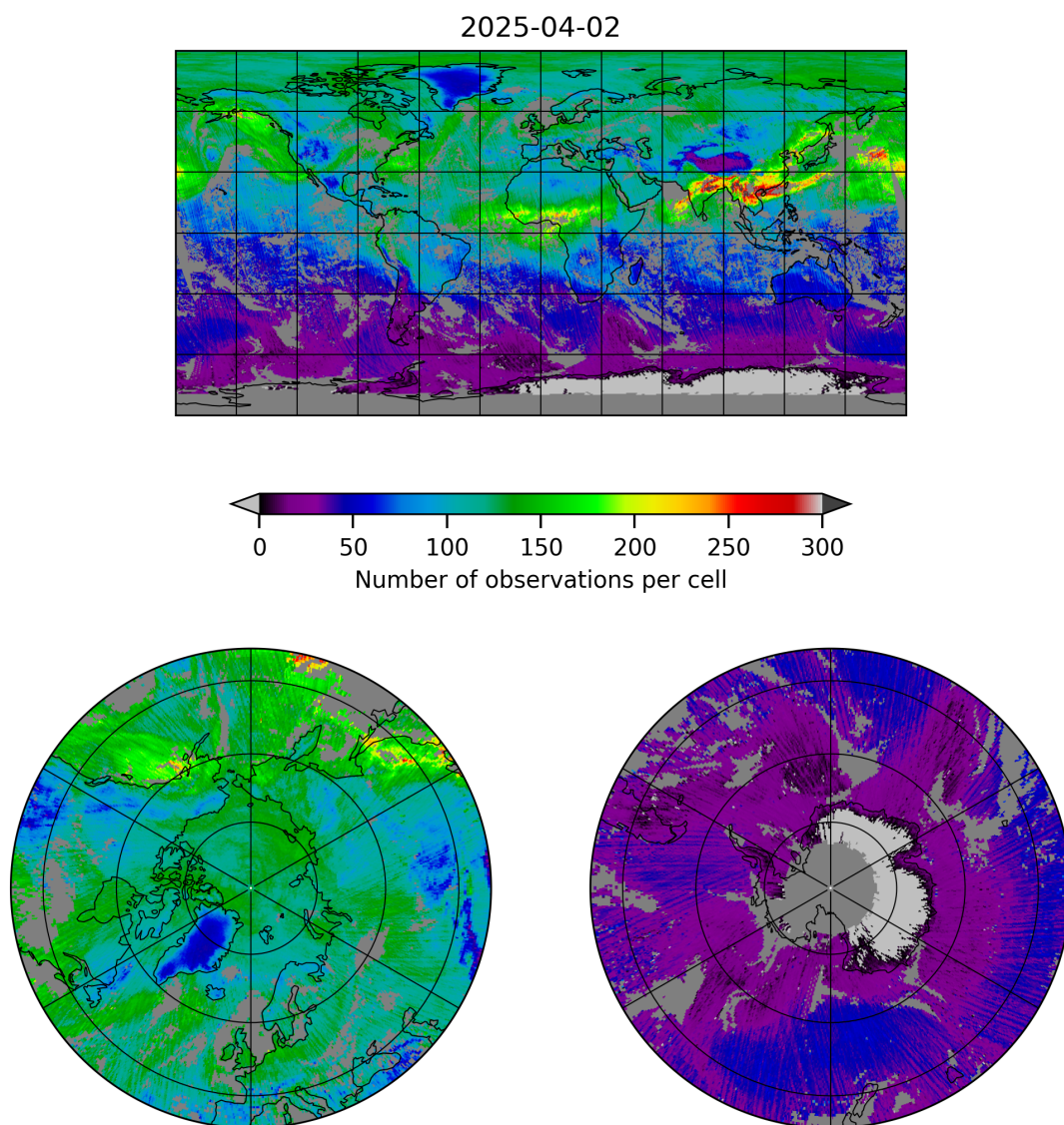
Figure 5: Map of the number of observations for 2025-04-02 to 2025-04-03
