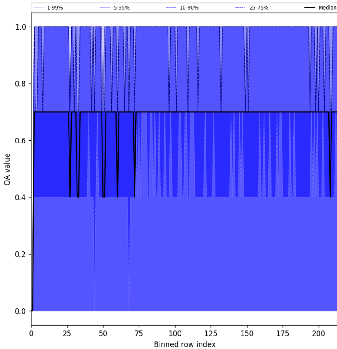
Figure 20: Along track statistics of “QA value” for 2025-04-02 to 2025-04-03
