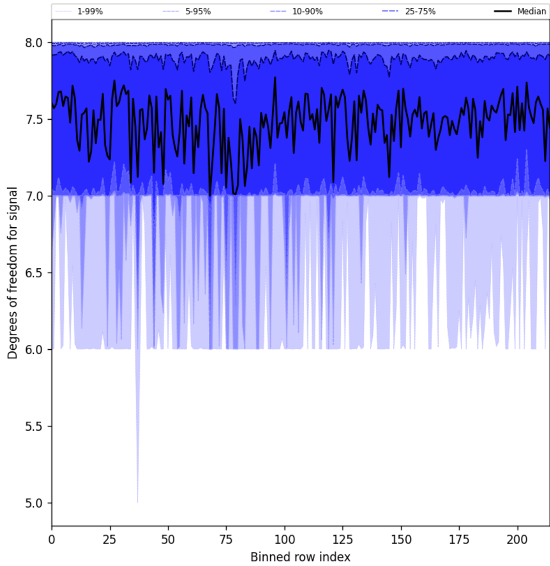
Figure 25: Along track statistics of “Degrees of freedom for signal” for 2025-04-02 to 2025-04-03
