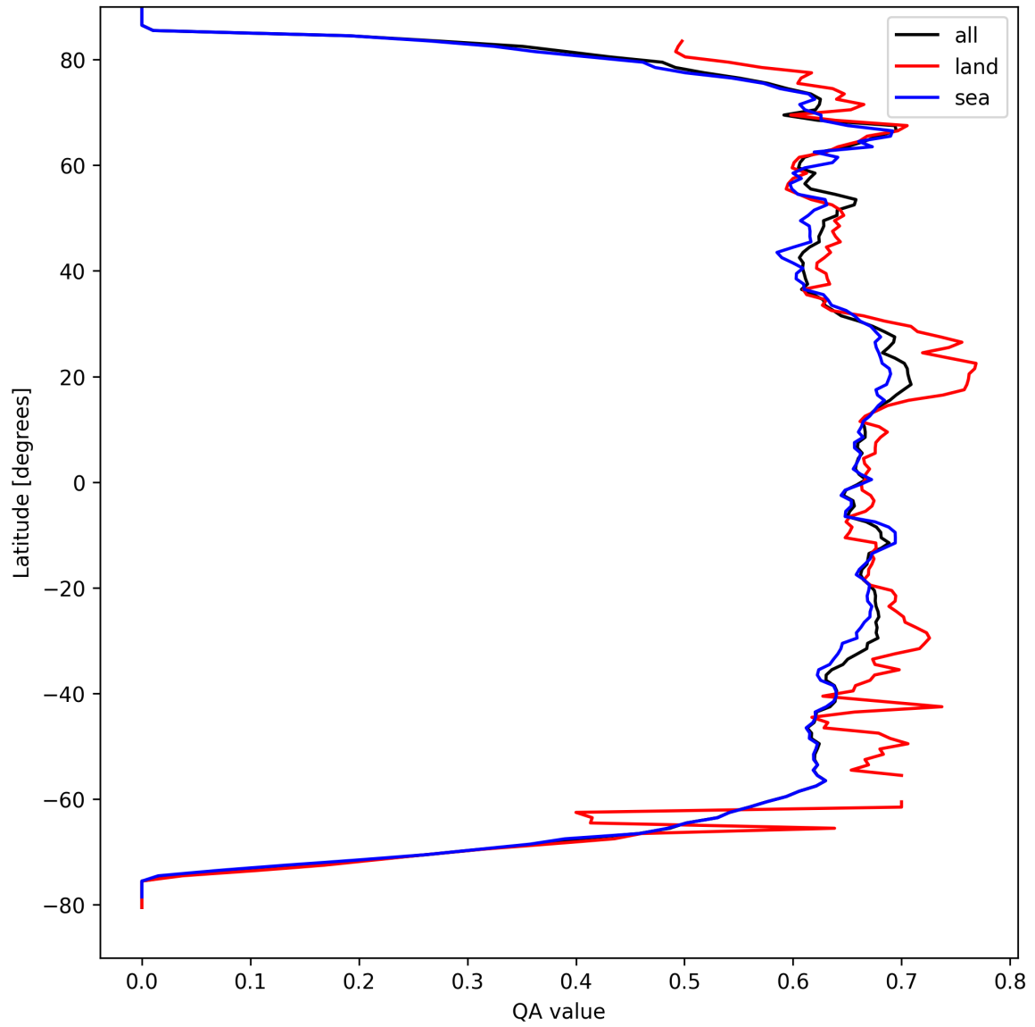
Figure 6: Zonal average of “QA value” for 2025-04-02 to 2025-04-03.
