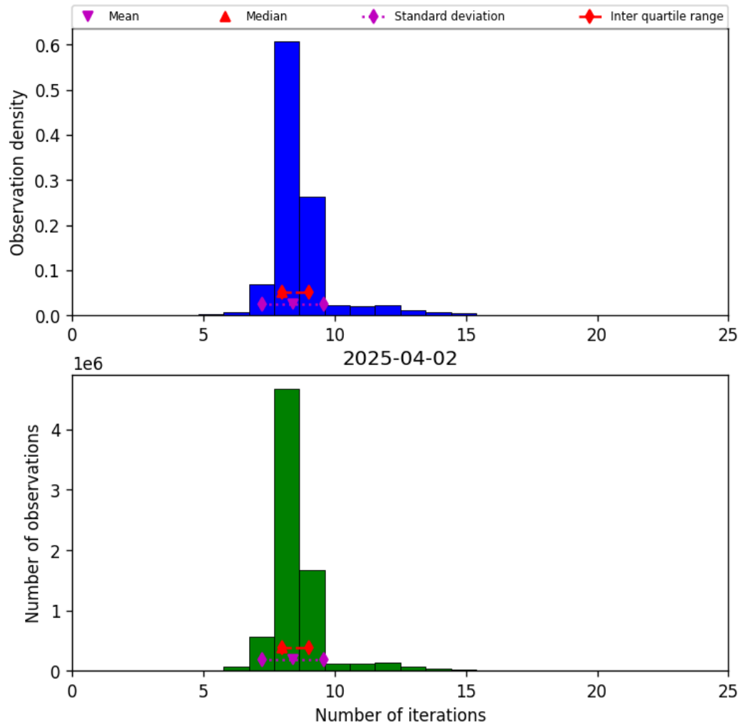
Figure 19: Histogram of “Number of iterations” for 2025-04-02 to 2025-04-03
