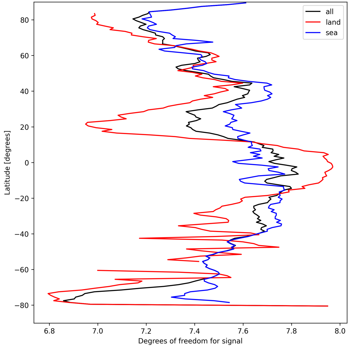
Figure 11: Zonal average of “Degrees of freedom for signal” for 2025-04-02 to 2025-04-03.
