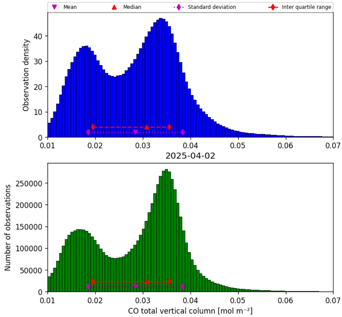
Figure 14: Histogram of “CO total vertical column” for 2025-04-02 to 2025-04-03
