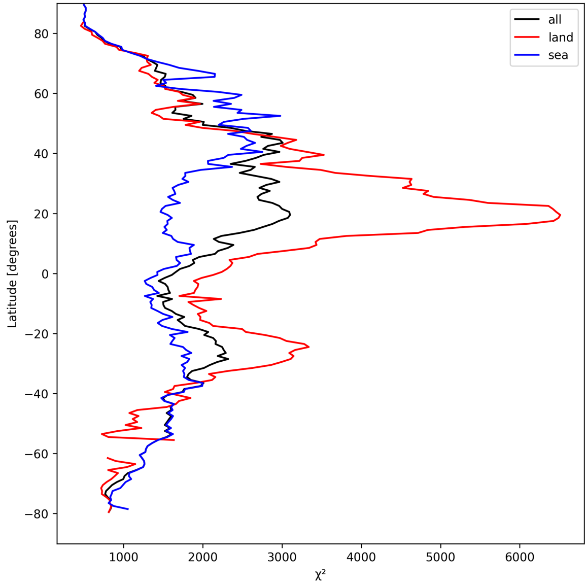
Figure 10: Zonal average of “ \chi^2 ” for 2025-04-03 to 2025-04-04.
