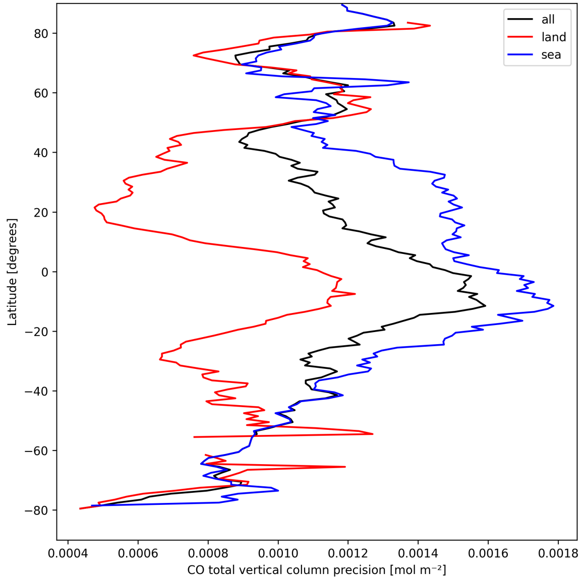
Figure 8: Zonal average of “CO total vertical column precision” for 2025-04-03 to 2025-04-04.
