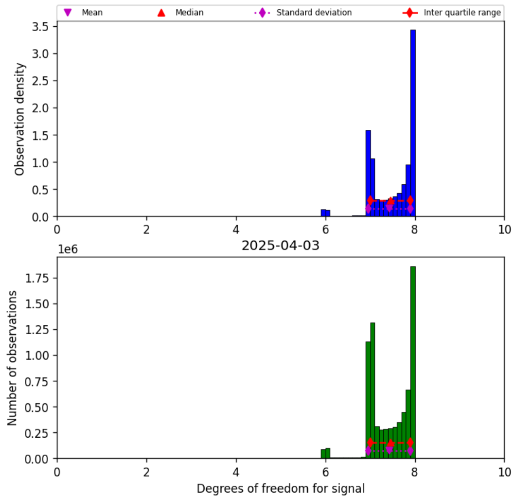
Figure 18: Histogram of “Degrees of freedom for signal” for 2025-04-03 to 2025-04-04
