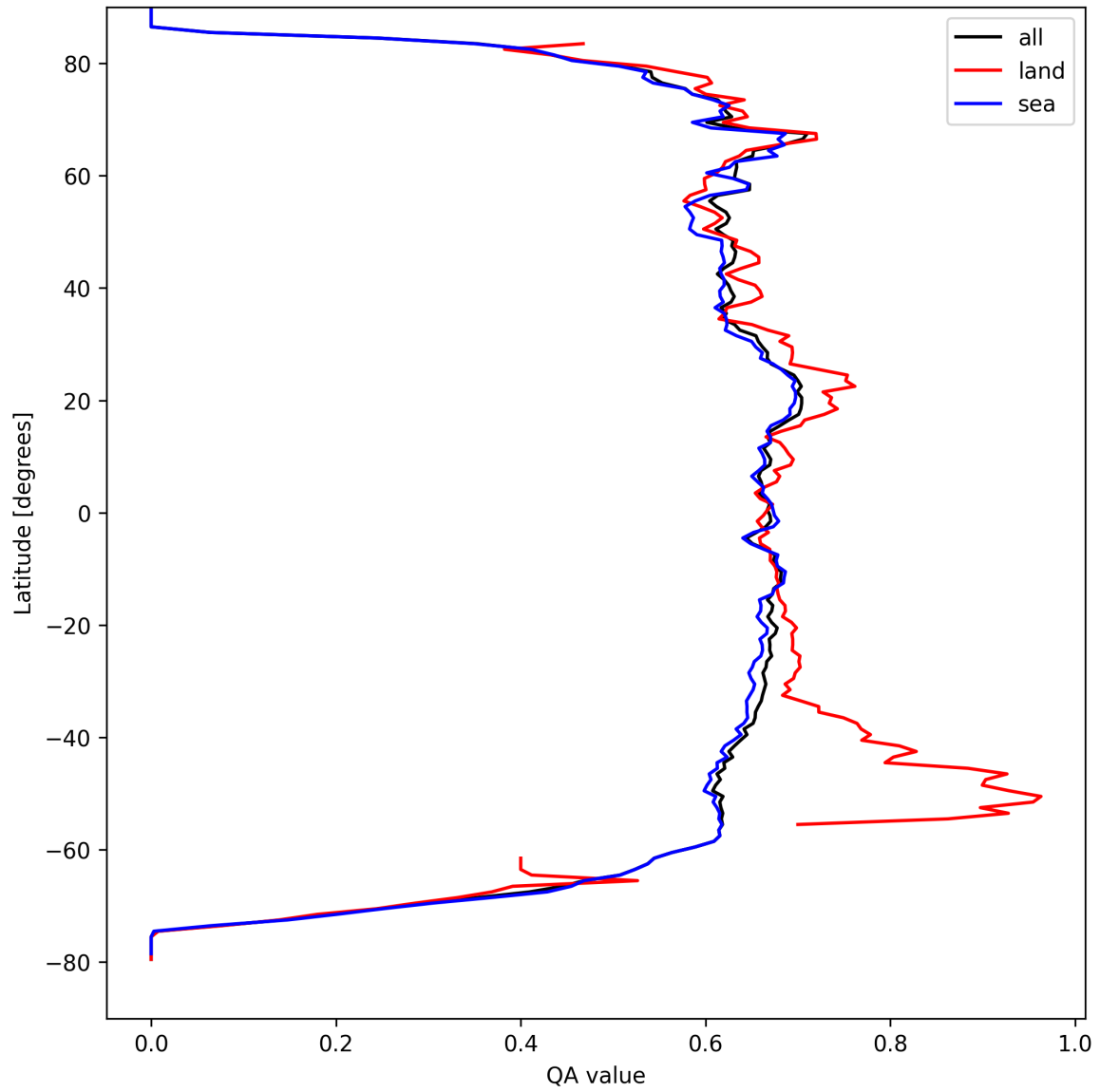
Figure 6: Zonal average of “QA value” for 2025-04-03 to 2025-04-04.
