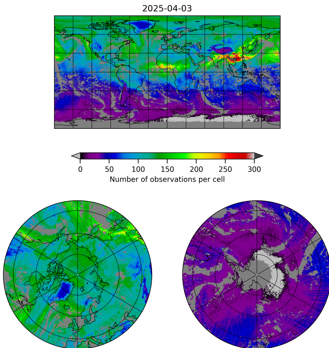
Figure 5: Map of the number of observations for 2025-04-03 to 2025-04-04
