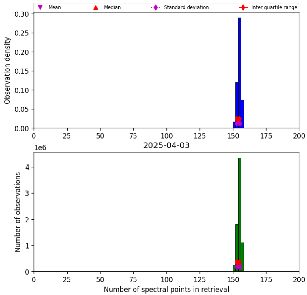
Figure 16: Histogram of “Number of spectral points in retrieval” for 2025-04-03 to 2025-04-04
