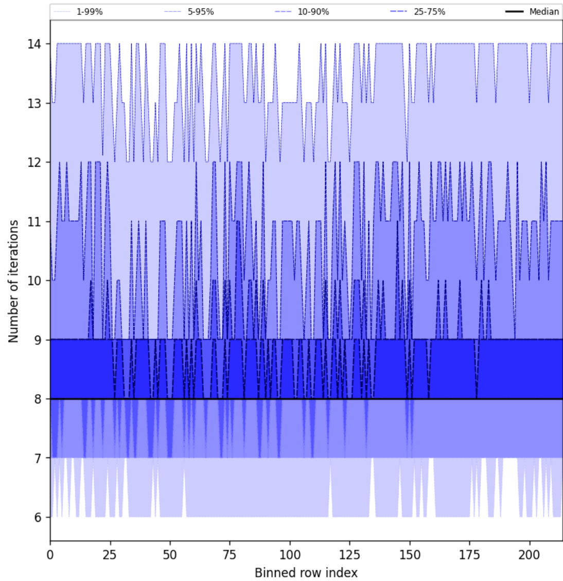
Figure 26: Along track statistics of “Number of iterations” for 2025-04-03 to 2025-04-04
