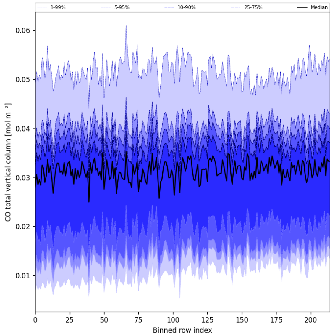
Figure 21: Along track statistics of “CO total vertical column” for 2025-04-03 to 2025-04-04
