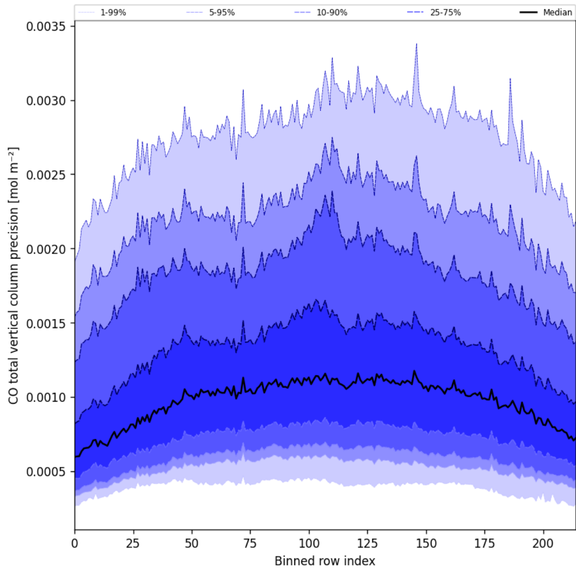
Figure 22: Along track statistics of “CO total vertical column precision” for 2025-04-03 to 2025-04-04
