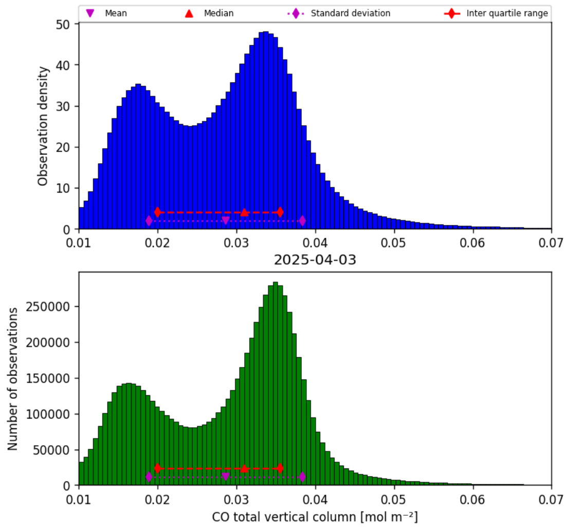
Figure 14: Histogram of “CO total vertical column” for 2025-04-03 to 2025-04-04
