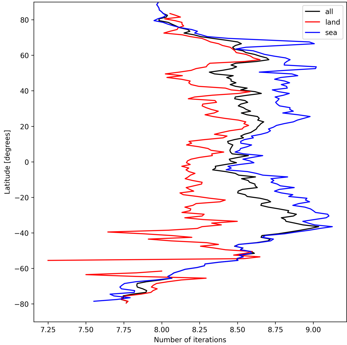
Figure 12: Zonal average of “Number of iterations” for 2025-04-03 to 2025-04-04.
