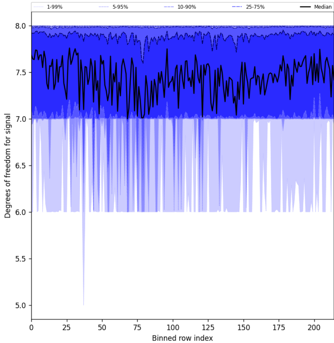
Figure 25: Along track statistics of “Degrees of freedom for signal” for 2025-04-03 to 2025-04-04
