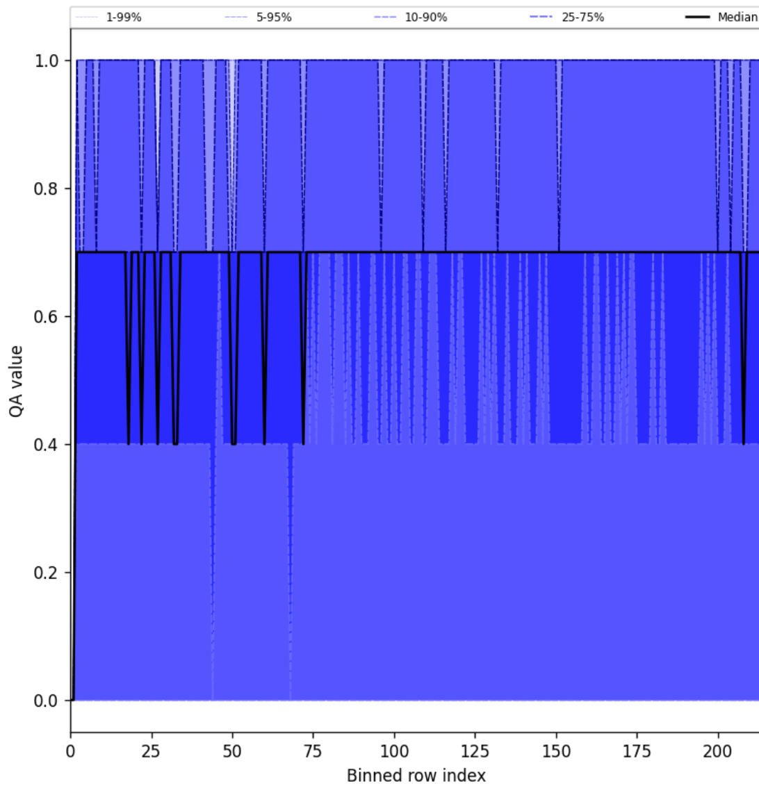
Figure 20: Along track statistics of “QA value” for 2025-04-03 to 2025-04-04
