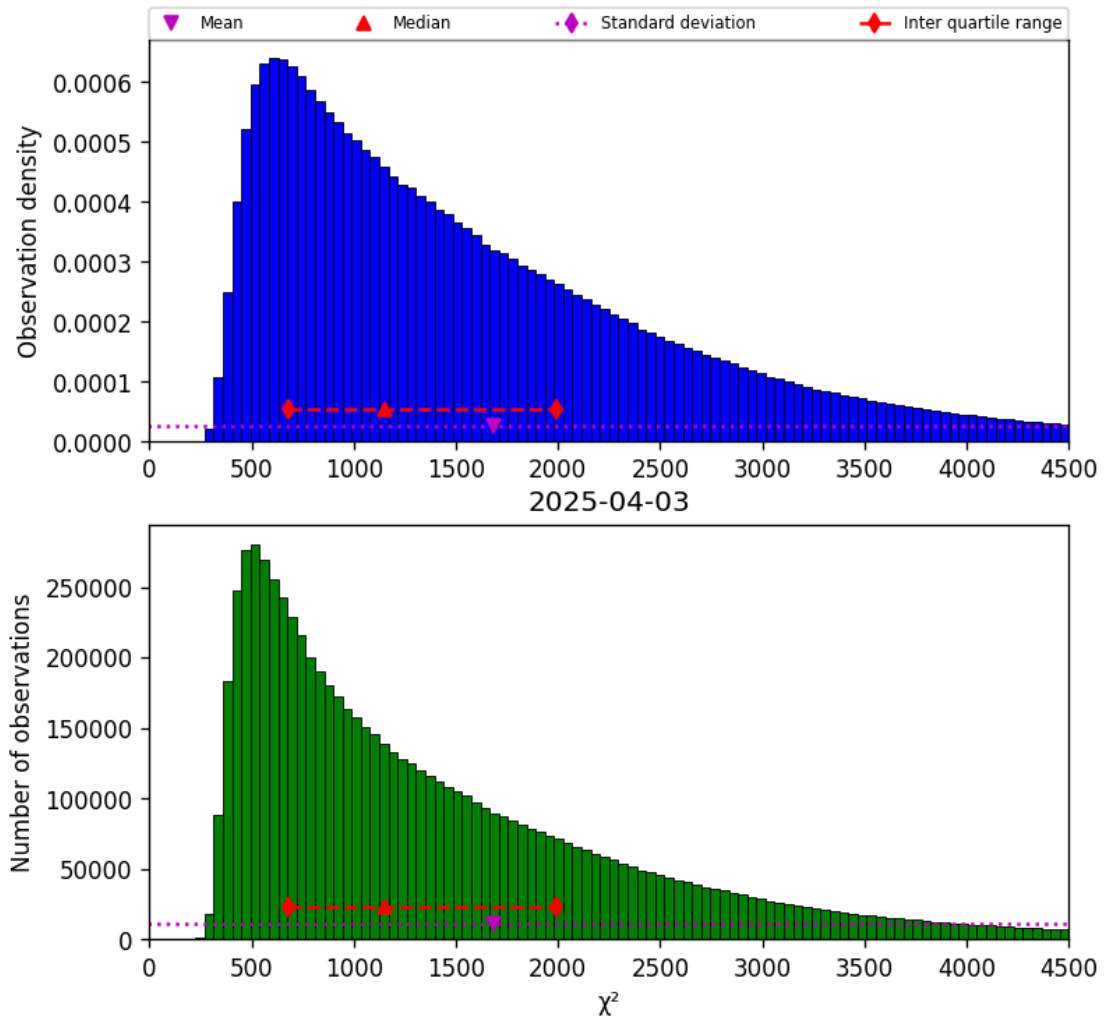
Figure 17: Histogram of “ \chi^2 ” for 2025-04-03 to 2025-04-04
