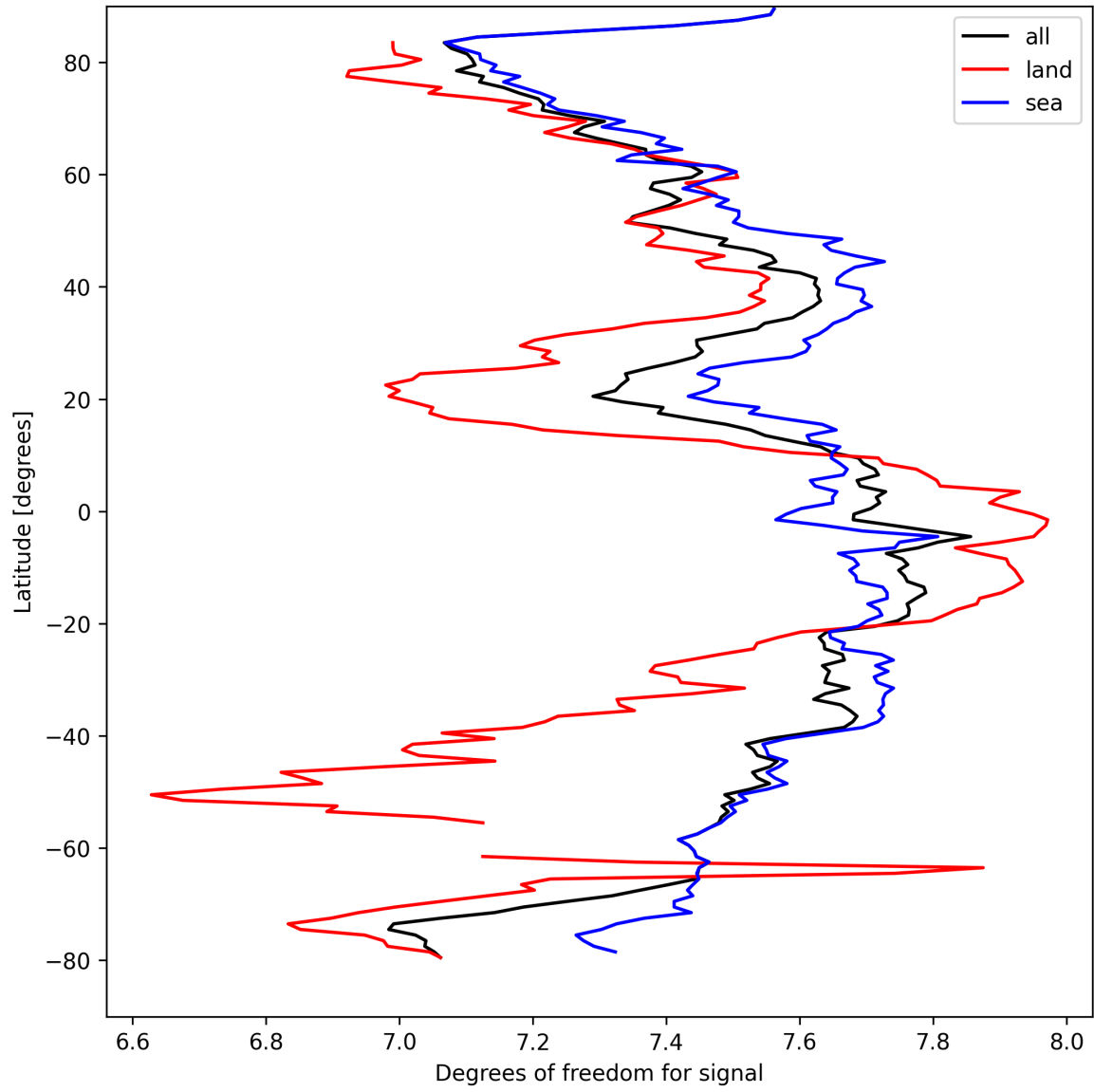
Figure 11: Zonal average of “Degrees of freedom for signal” for 2025-04-03 to 2025-04-04.
