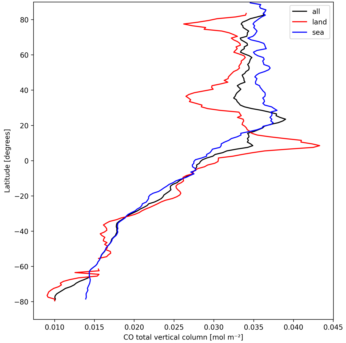
Figure 7: Zonal average of “CO total vertical column” for 2025-04-03 to 2025-04-04.
