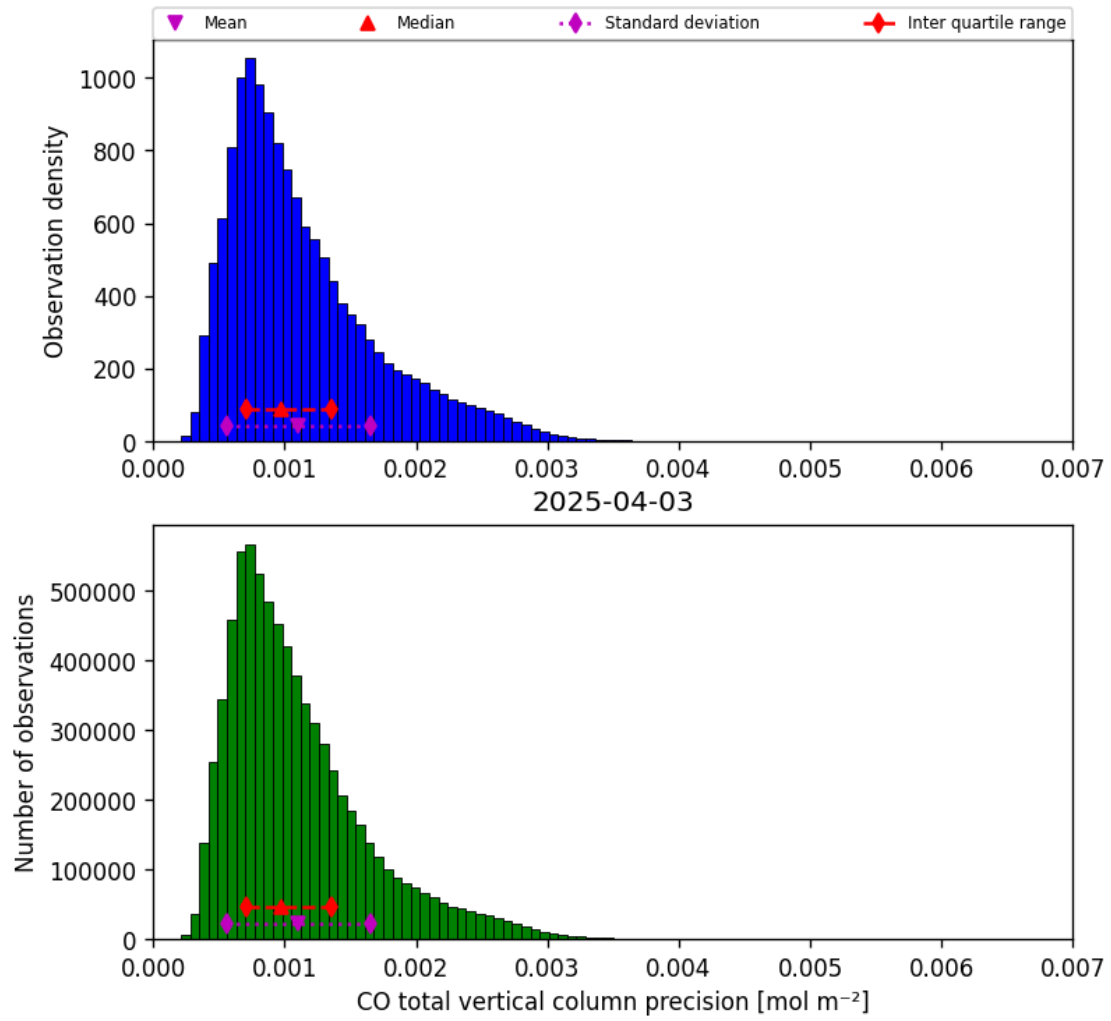
Figure 15: Histogram of “CO total vertical column precision” for 2025-04-03 to 2025-04-04
