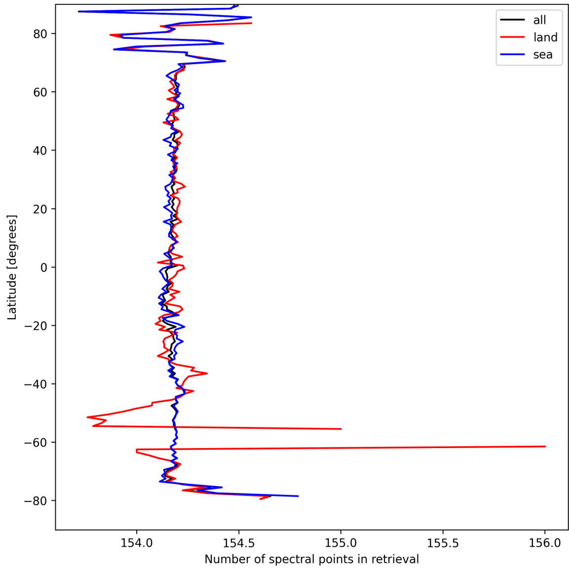
Figure 9: Zonal average of “Number of spectral points in retrieval” for 2025-04-03 to 2025-04-04.
