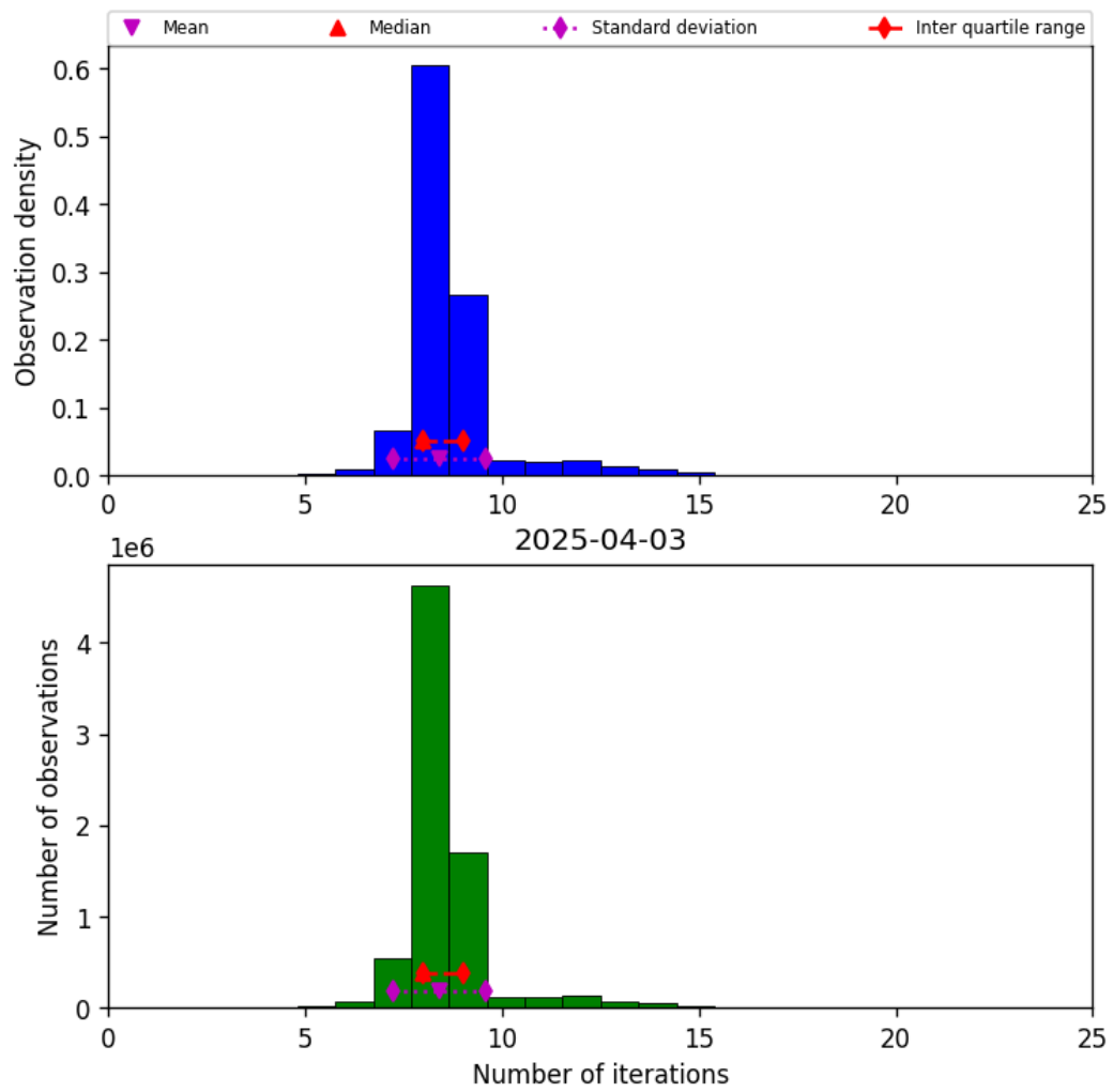
Figure 19: Histogram of “Number of iterations” for 2025-04-03 to 2025-04-04
