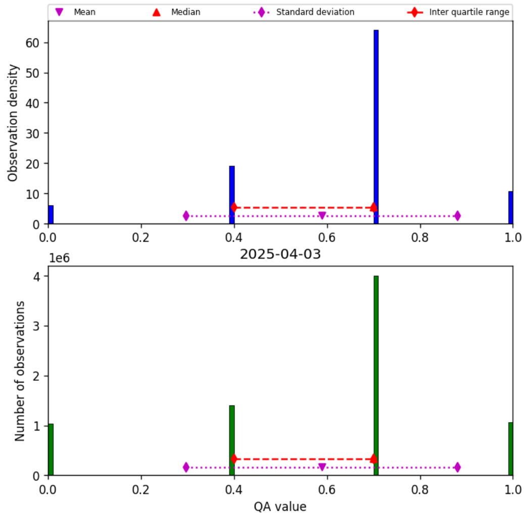
Figure 13: Histogram of “QA value” for 2025-04-03 to 2025-04-04
