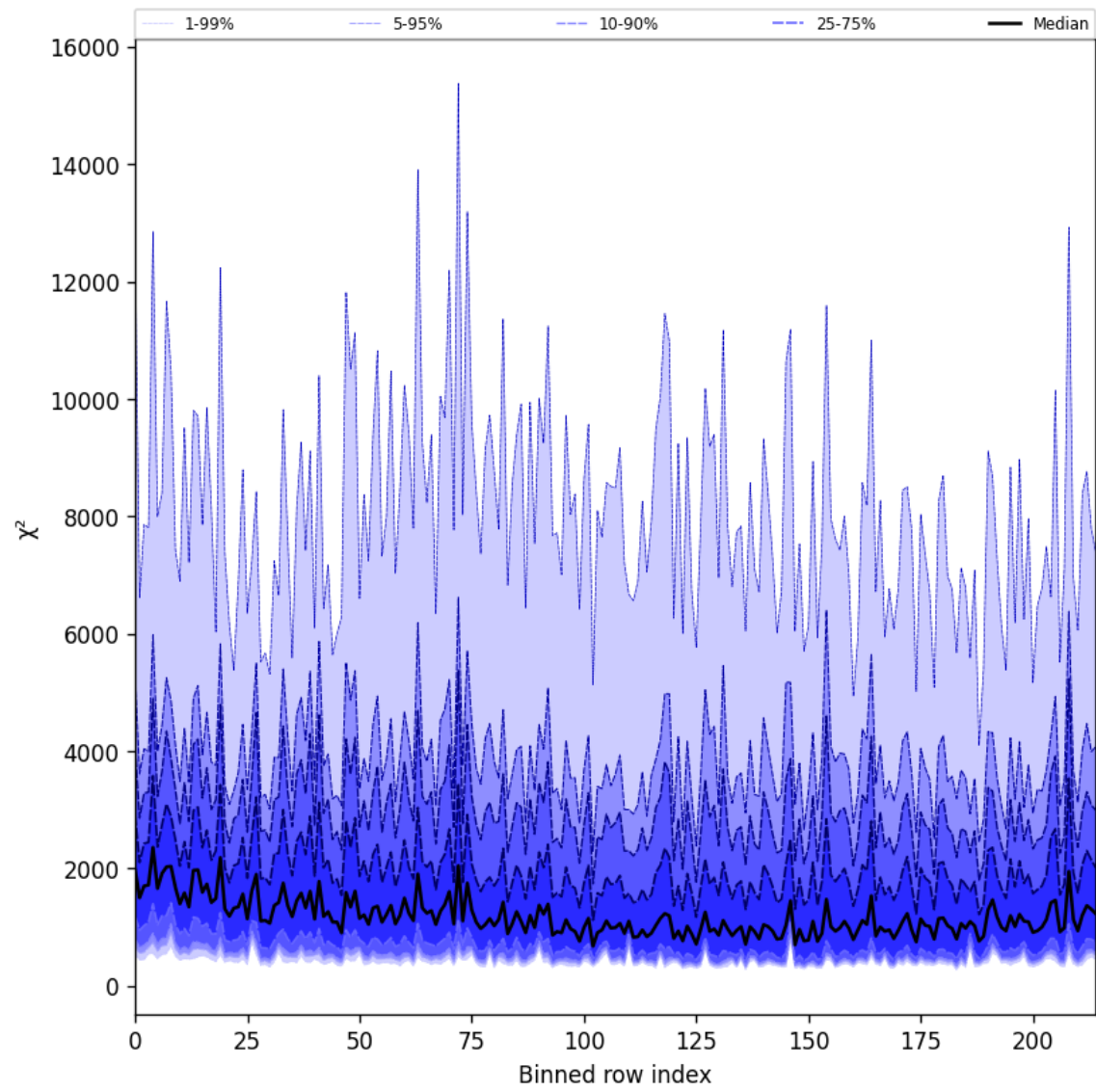
Figure 24: Along track statistics of “ \chi^2 ” for 2025-04-03 to 2025-04-04
