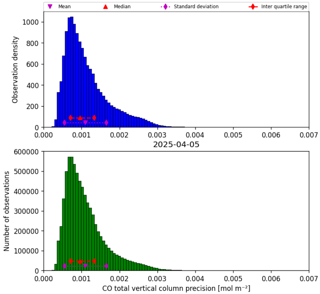
Figure 15: Histogram of “CO total vertical column precision” for 2025-04-05 to 2025-04-06
