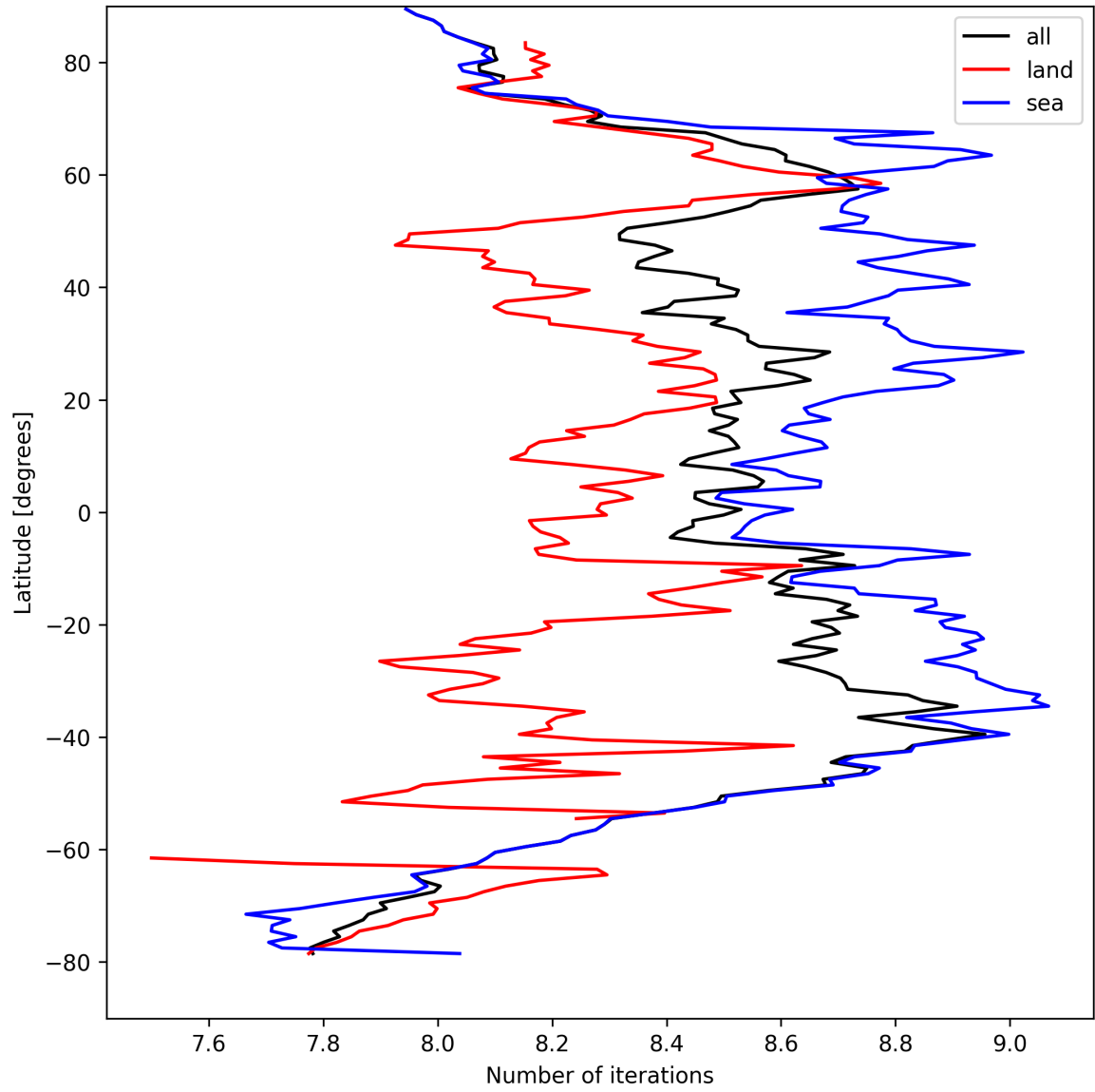
Figure 12: Zonal average of “Number of iterations” for 2025-04-05 to 2025-04-06.
