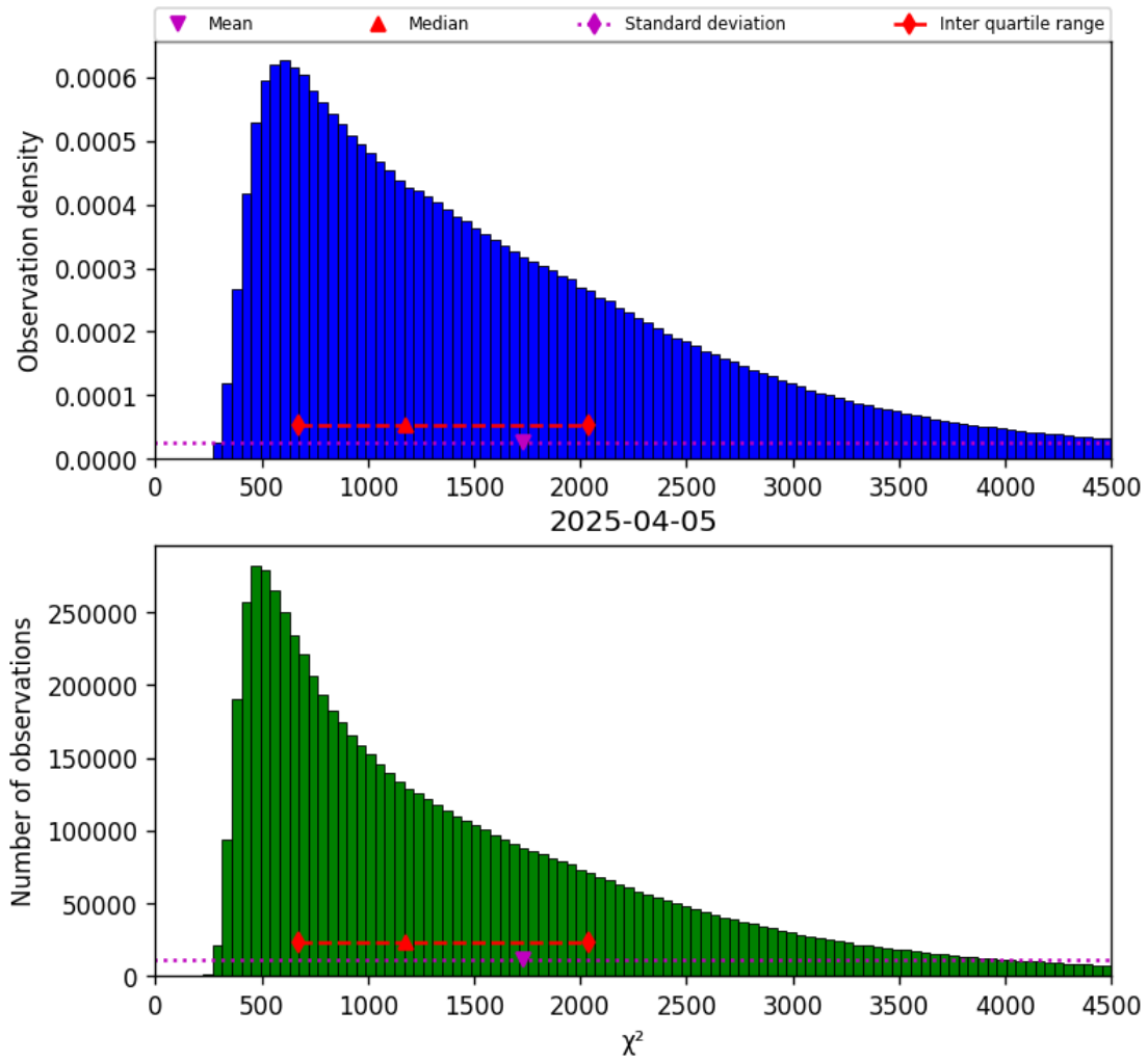
Figure 17: Histogram of " \chi^2 " for 2025-04-05 to 2025-04-06
