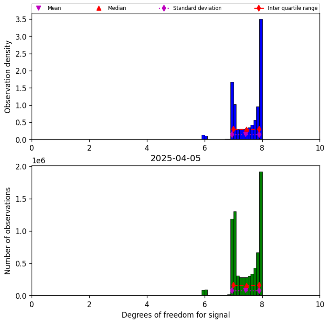
Figure 18: Histogram of “Degrees of freedom for signal” for 2025-04-05 to 2025-04-06
