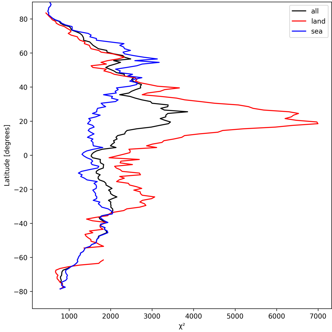
Figure 10: Zonal average of “ \chi^2 ” for 2025-04-05 to 2025-04-06.
