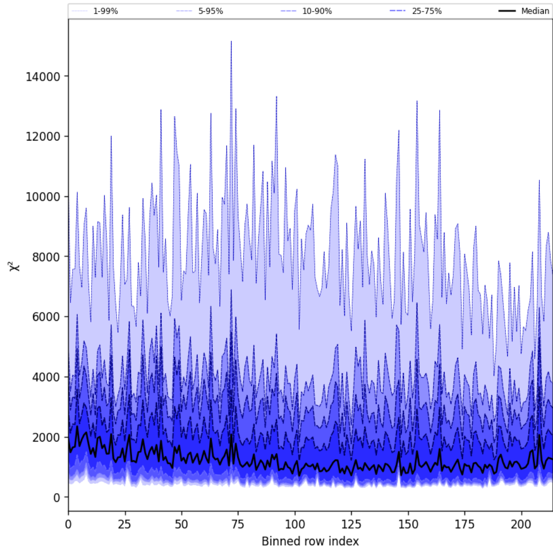
Figure 24: Along track statistics of “ \chi^2 ” for 2025-04-05 to 2025-04-06
