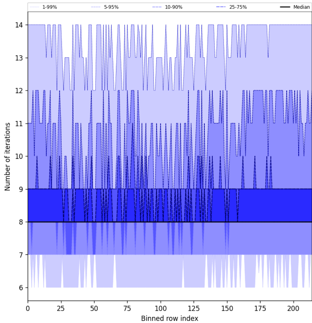
Figure 26: Along track statistics of “Number of iterations” for 2025-04-05 to 2025-04-06
