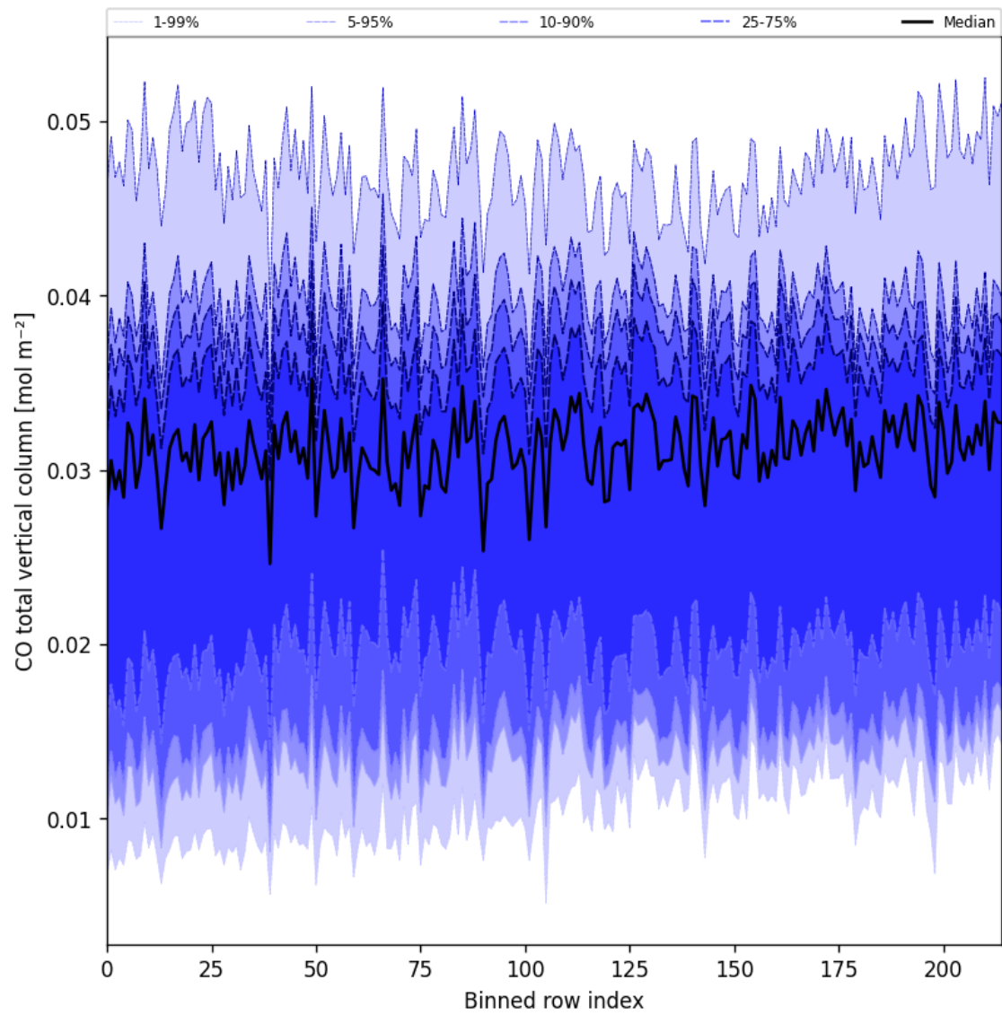
Figure 21: Along track statistics of “CO total vertical column” for 2025-04-05 to 2025-04-06
