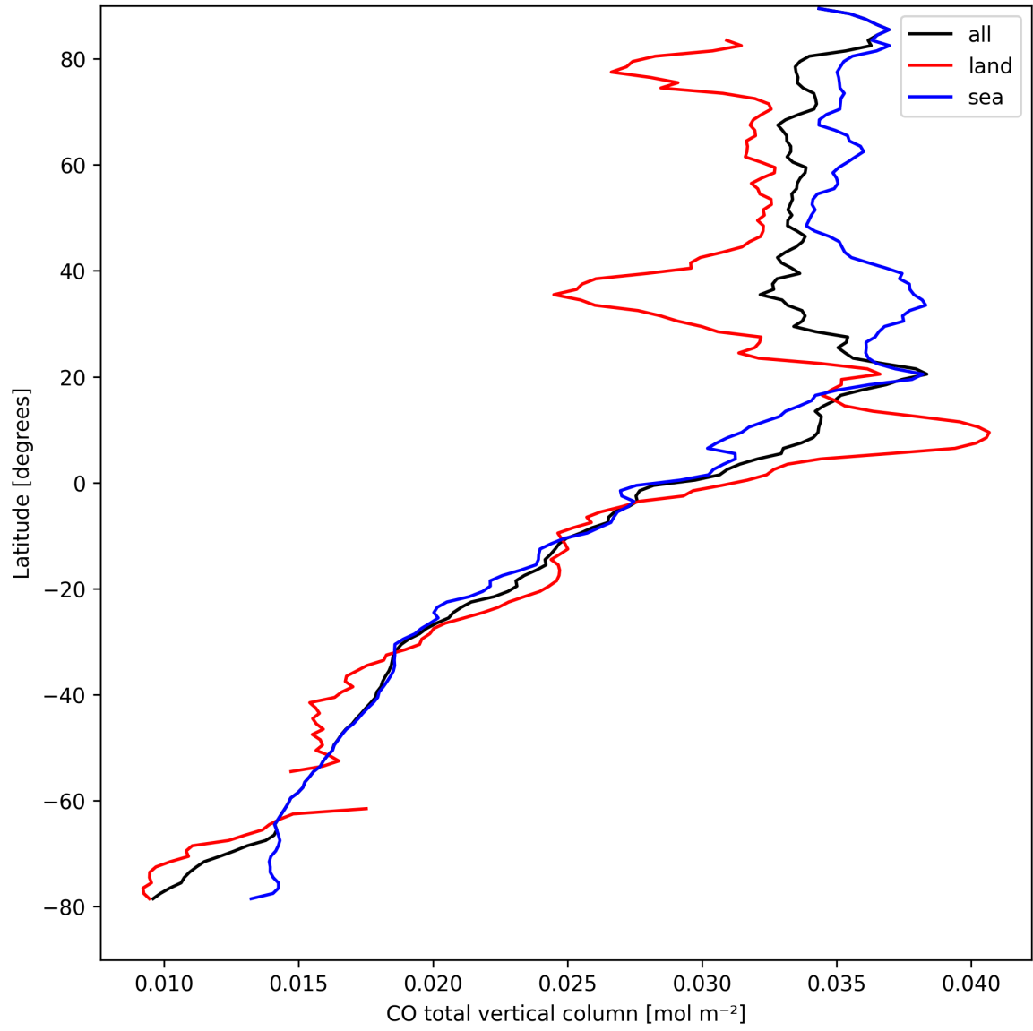
Figure 7: Zonal average of “CO total vertical column” for 2025-04-05 to 2025-04-06.
