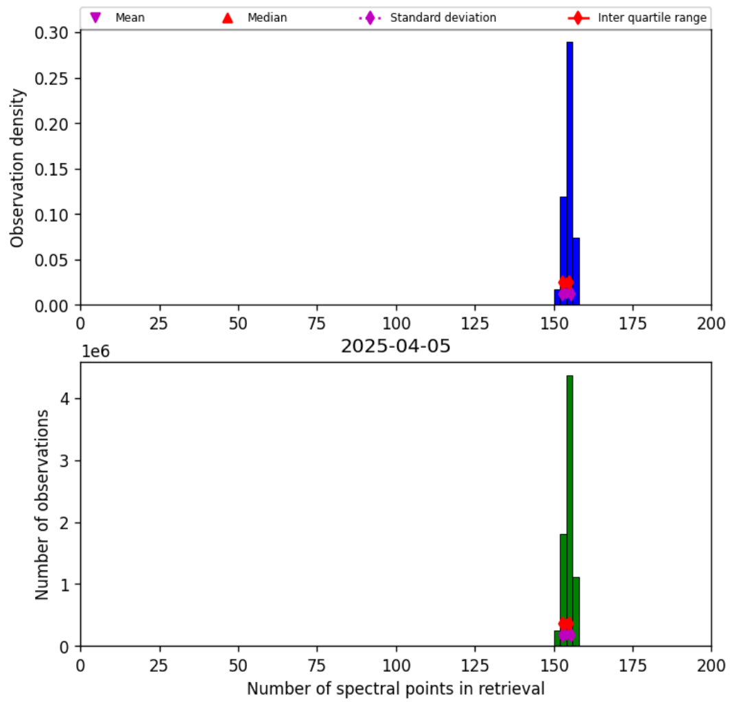
Figure 16: Histogram of “Number of spectral points in retrieval” for 2025-04-05 to 2025-04-06
