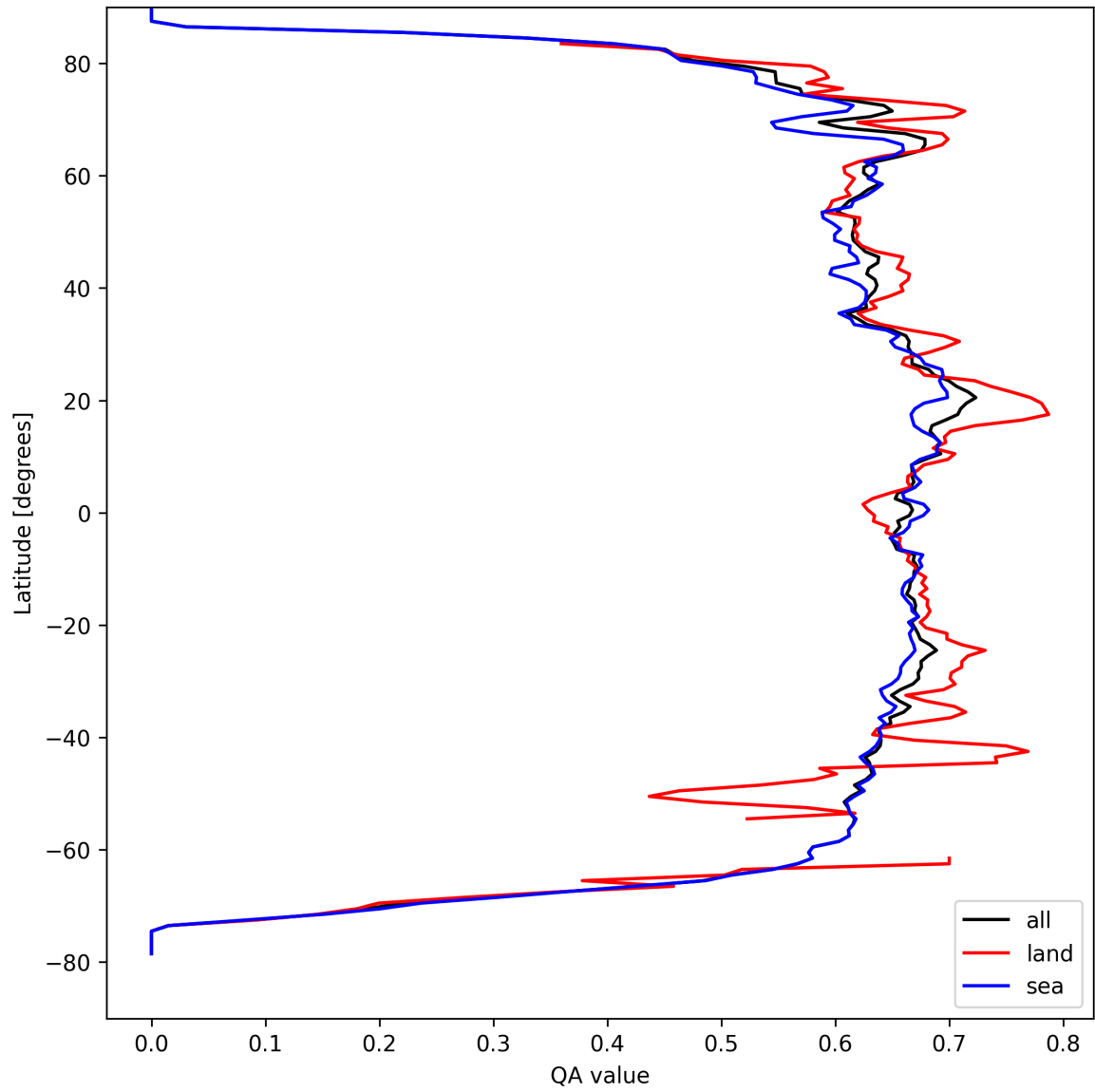
Figure 6: Zonal average of “QA value” for 2025-04-05 to 2025-04-06.
