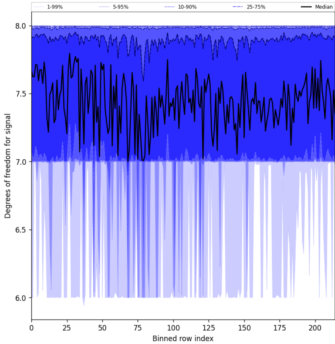
Figure 25: Along track statistics of “Degrees of freedom for signal” for 2025-04-05 to 2025-04-06
