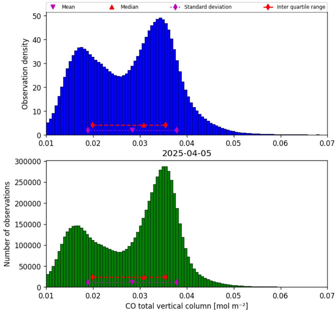
Figure 14: Histogram of “CO total vertical column” for 2025-04-05 to 2025-04-06
