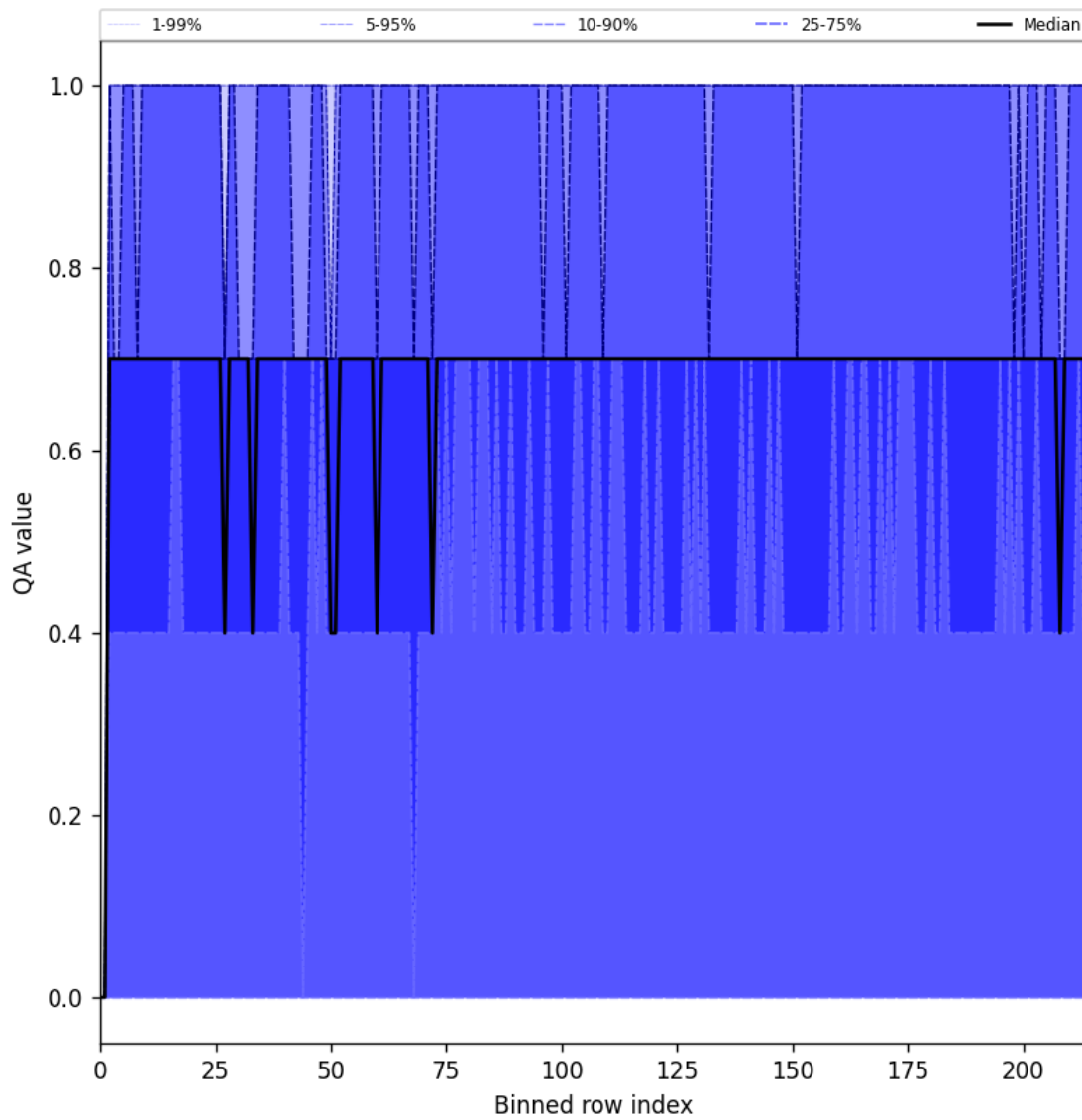
Figure 20: Along track statistics of “QA value” for 2025-04-05 to 2025-04-06
