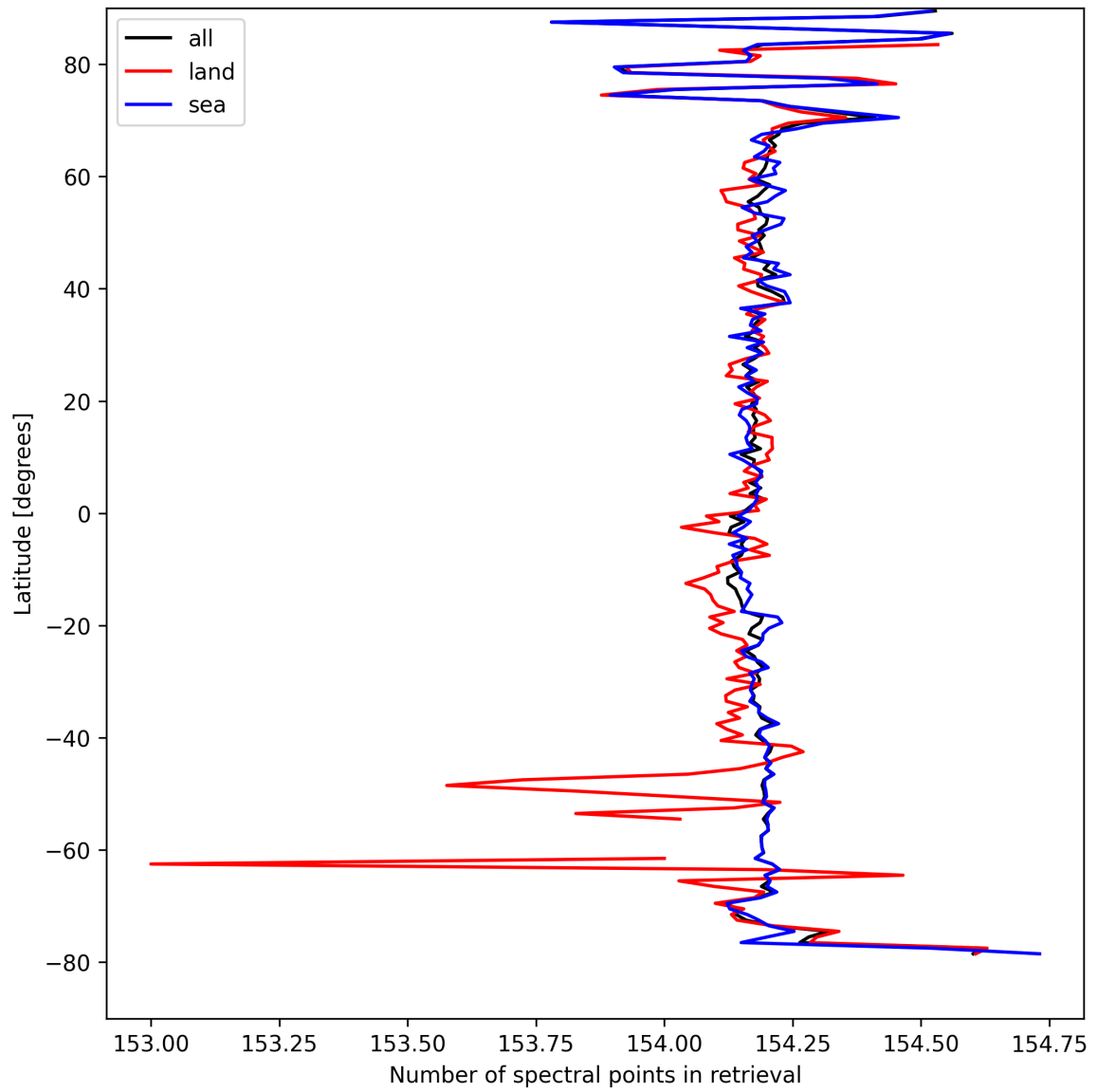
Figure 9: Zonal average of “Number of spectral points in retrieval” for 2025-04-05 to 2025-04-06.
