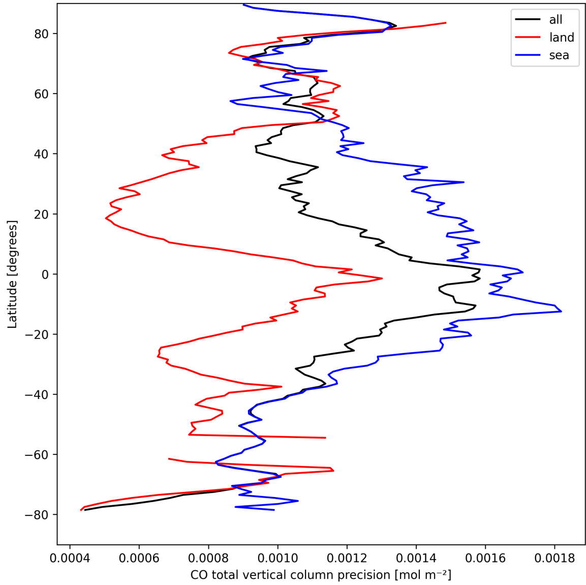
Figure 8: Zonal average of “CO total vertical column precision” for 2025-04-05 to 2025-04-06.
