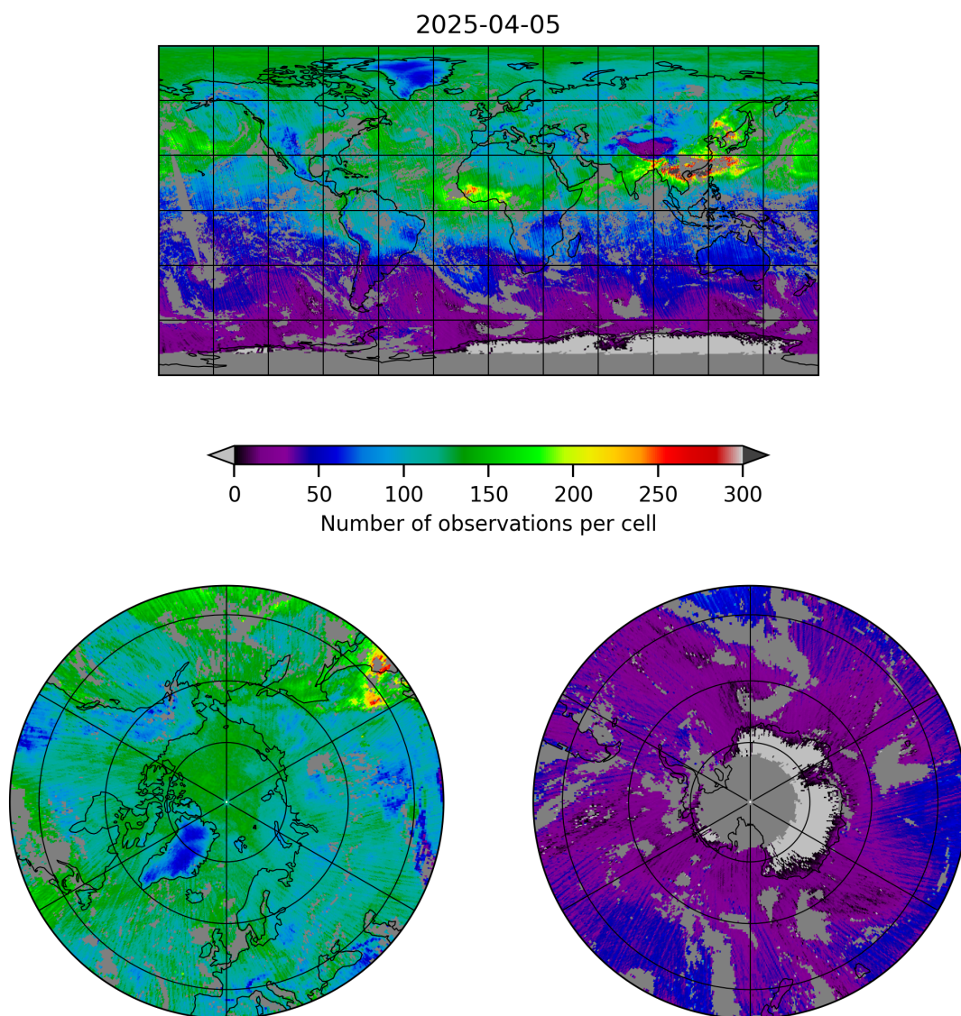
Figure 5: Map of the number of observations for 2025-04-05 to 2025-04-06
