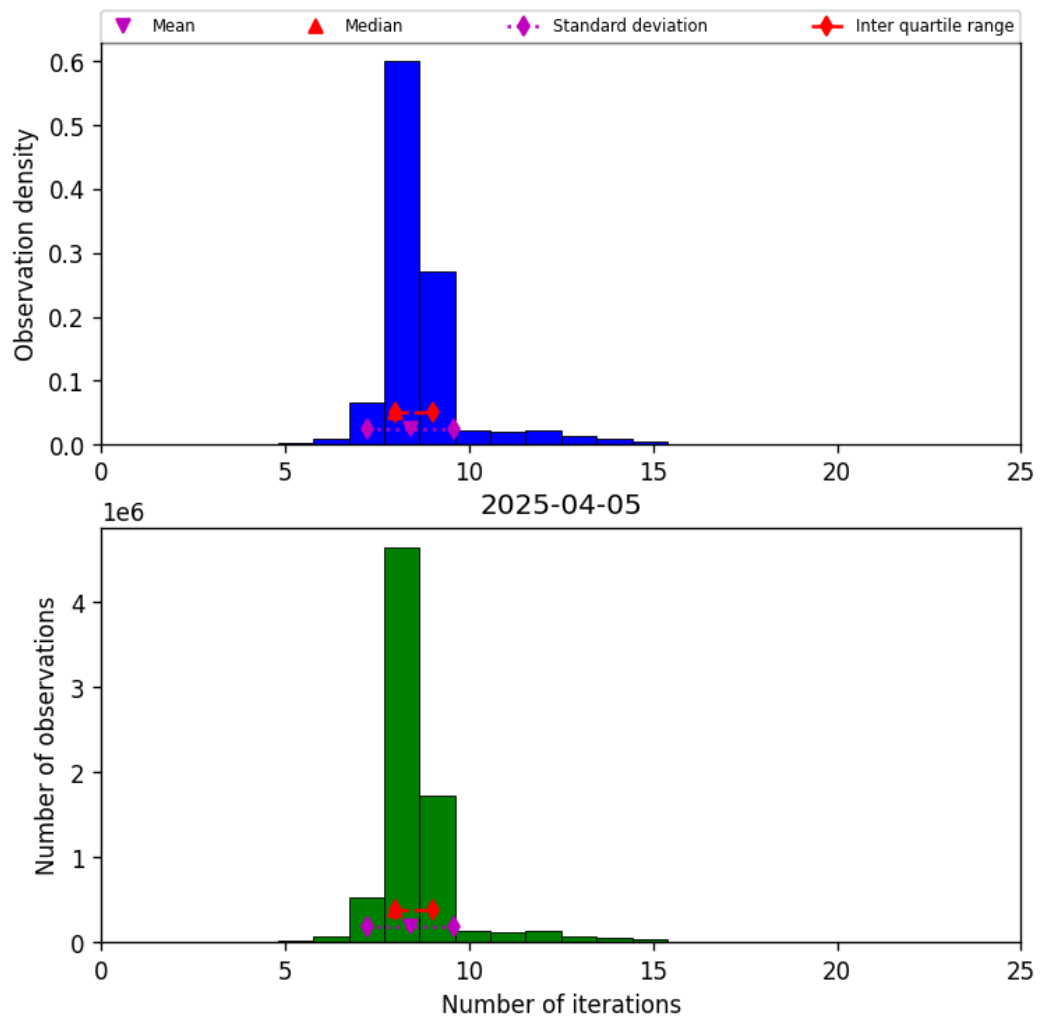
Figure 19: Histogram of “Number of iterations” for 2025-04-05 to 2025-04-06
