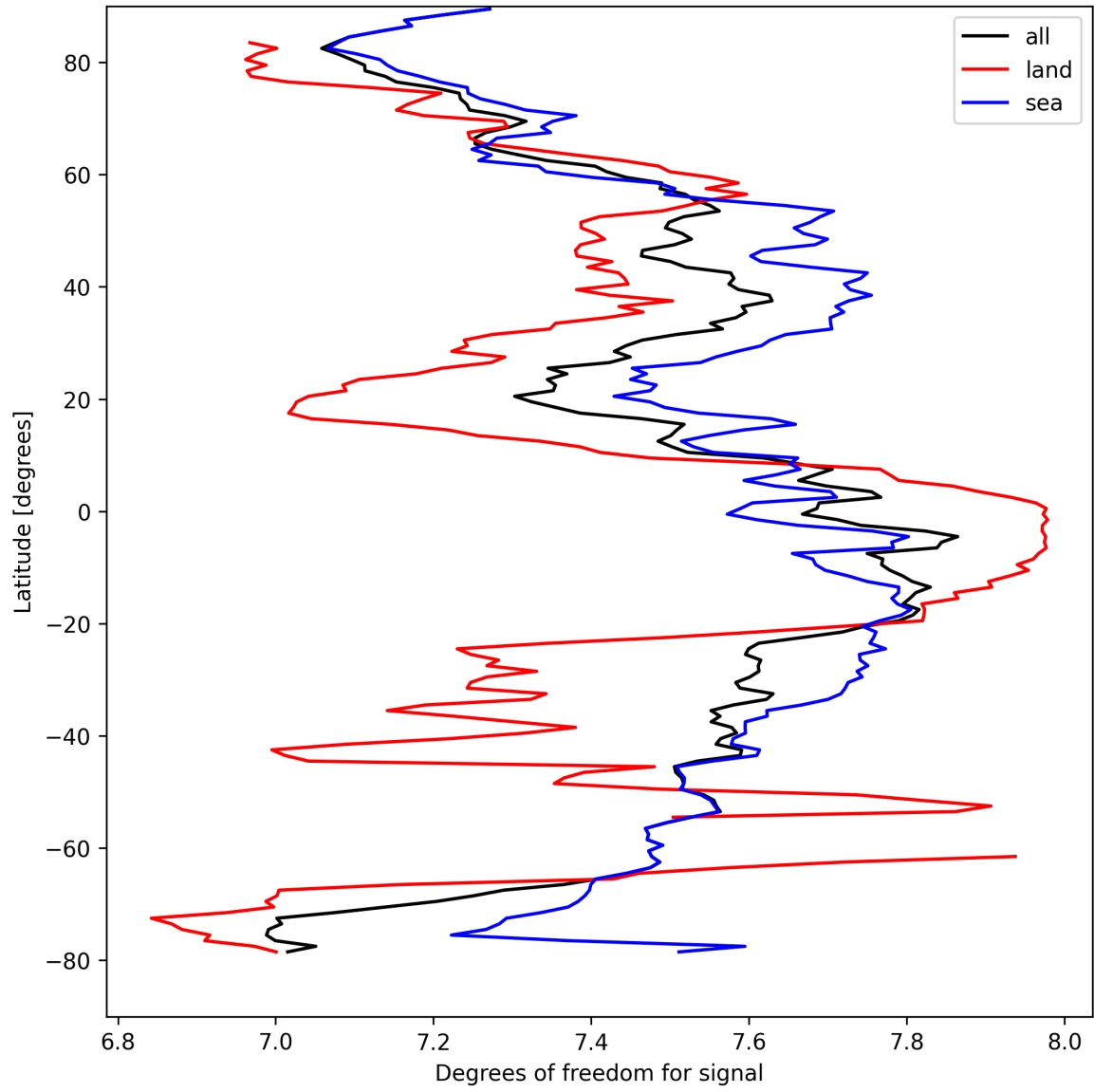
Figure 11: Zonal average of “Degrees of freedom for signal” for 2025-04-05 to 2025-04-06.
