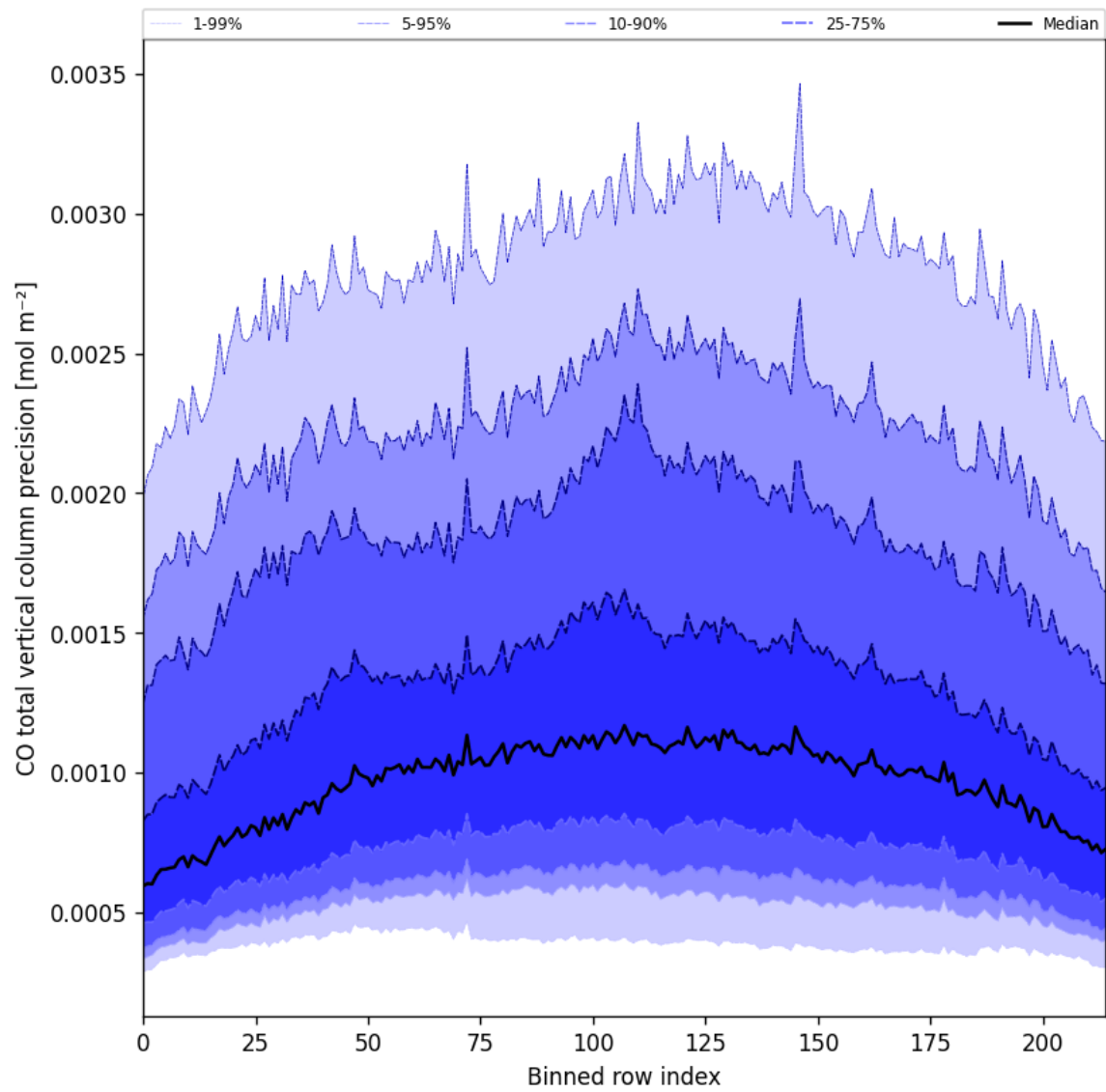
Figure 22: Along track statistics of “CO total vertical column precision” for 2025-04-05 to 2025-04-06
