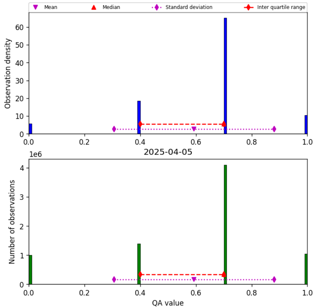
Figure 13: Histogram of “QA value” for 2025-04-05 to 2025-04-06
