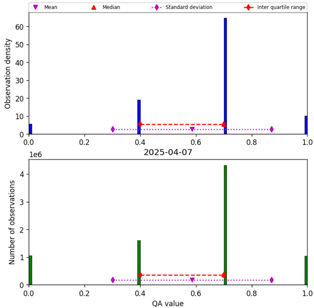
Figure 13: Histogram of “QA value” for 2025-04-07 to 2025-04-08
