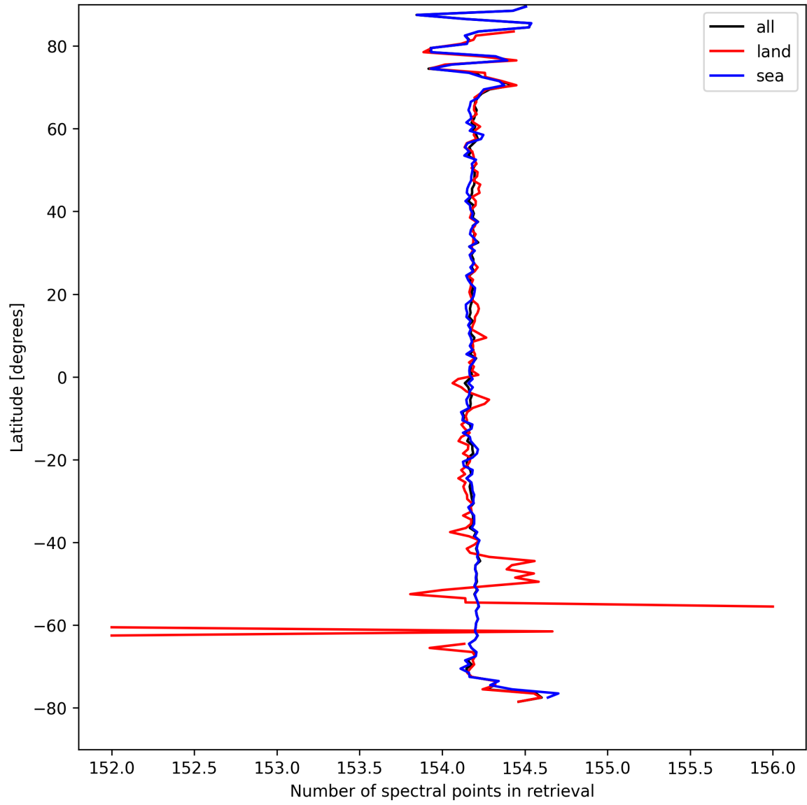
Figure 9: Zonal average of “Number of spectral points in retrieval” for 2025-04-07 to 2025-04-08.
