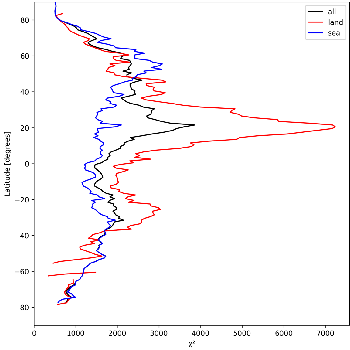
Figure 10: Zonal average of “ \chi^2 ” for 2025-04-07 to 2025-04-08.
