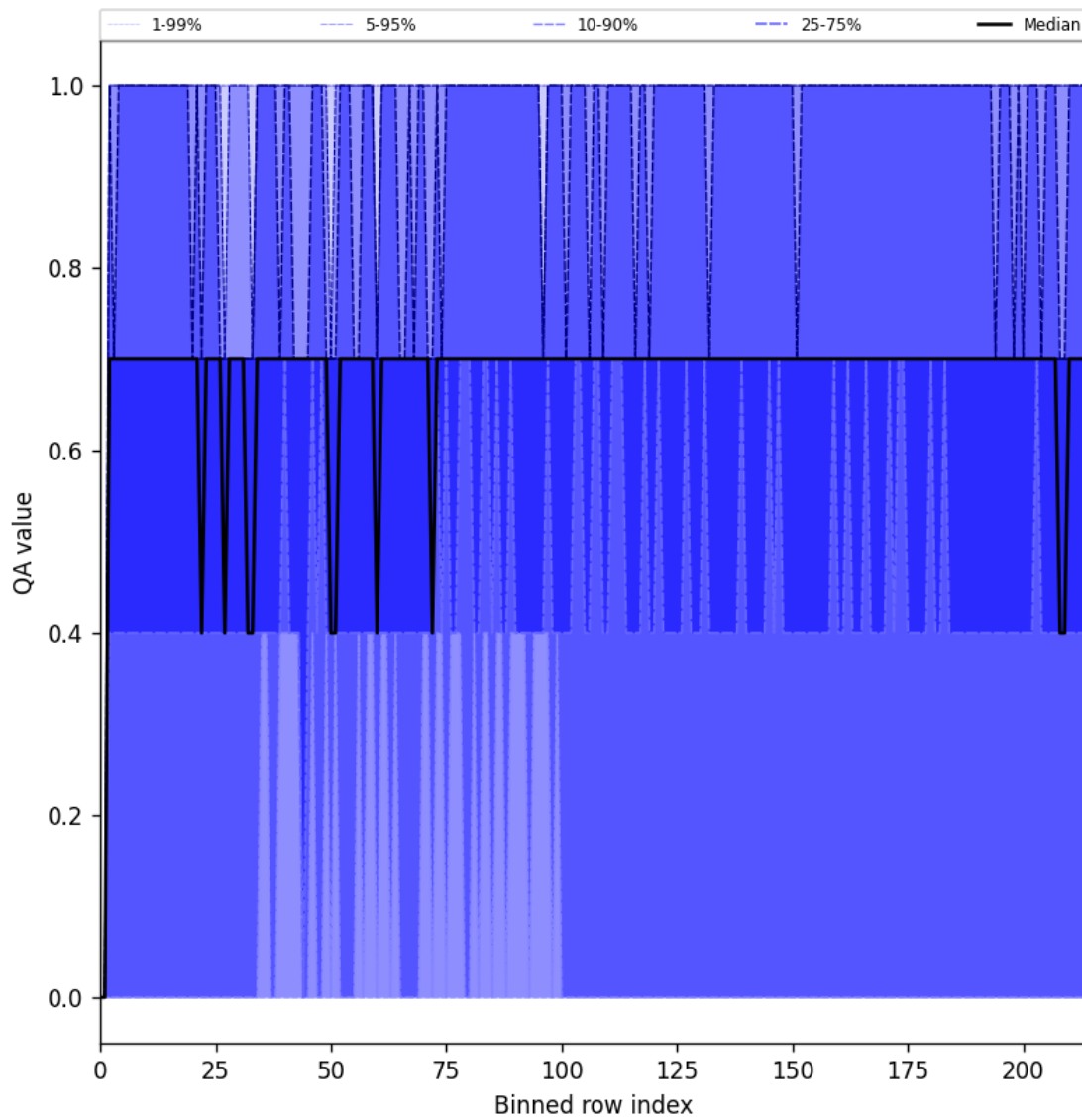
Figure 20: Along track statistics of “QA value” for 2025-04-07 to 2025-04-08
