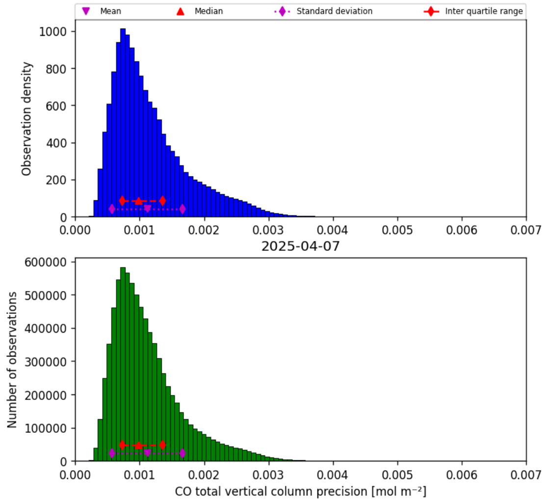
Figure 15: Histogram of “CO total vertical column precision” for 2025-04-07 to 2025-04-08
