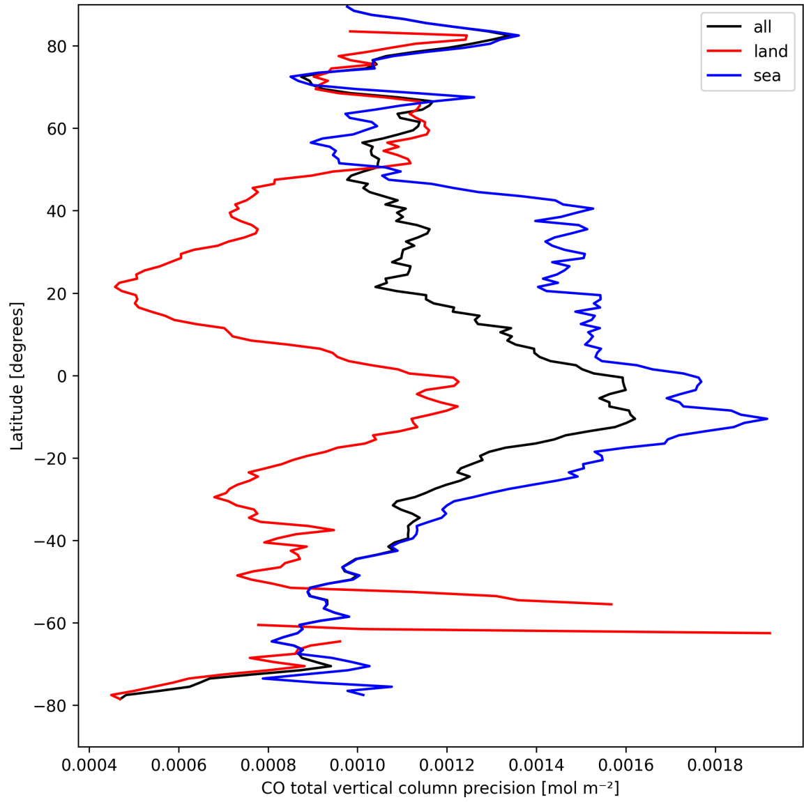
Figure 8: Zonal average of "CO total vertical column precision" for 2025-04-07 to 2025-04-08.
