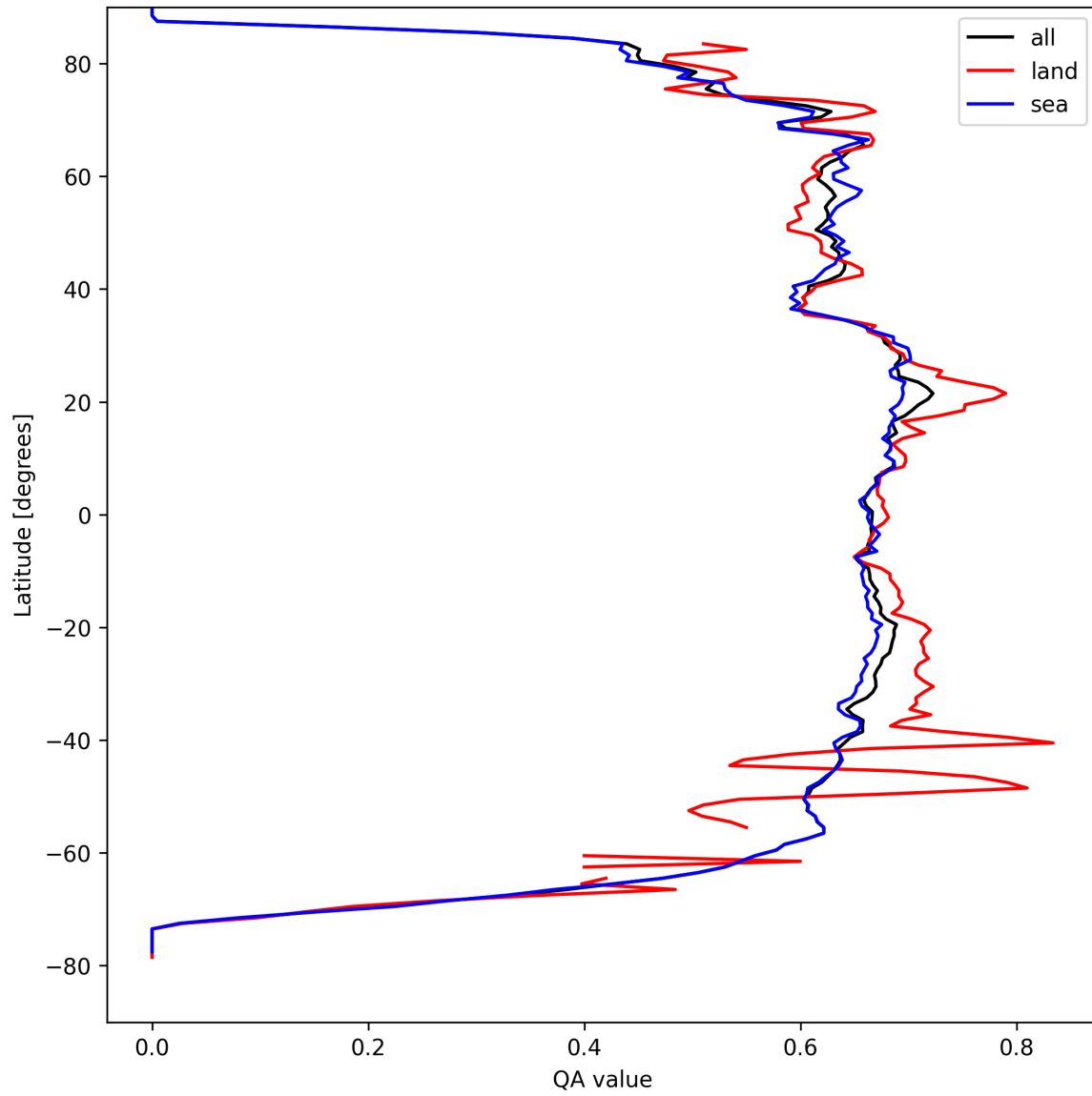
Figure 6: Zonal average of “QA value” for 2025-04-07 to 2025-04-08.
