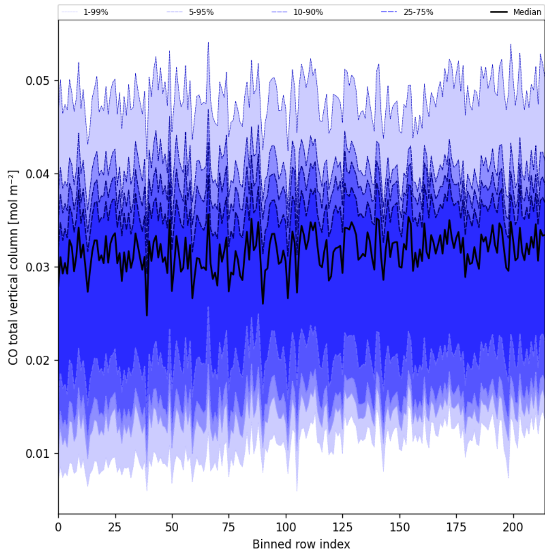
Figure 21: Along track statistics of “CO total vertical column” for 2025-04-07 to 2025-04-08
