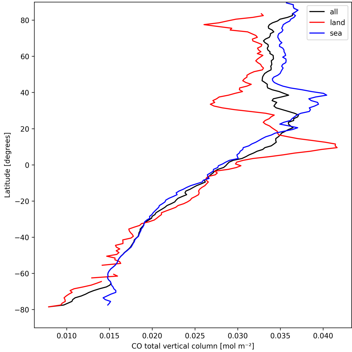
Figure 7: Zonal average of “CO total vertical column” for 2025-04-07 to 2025-04-08.
