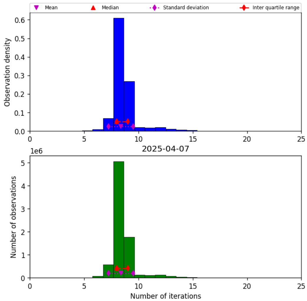
Figure 19: Histogram of “Number of iterations” for 2025-04-07 to 2025-04-08
