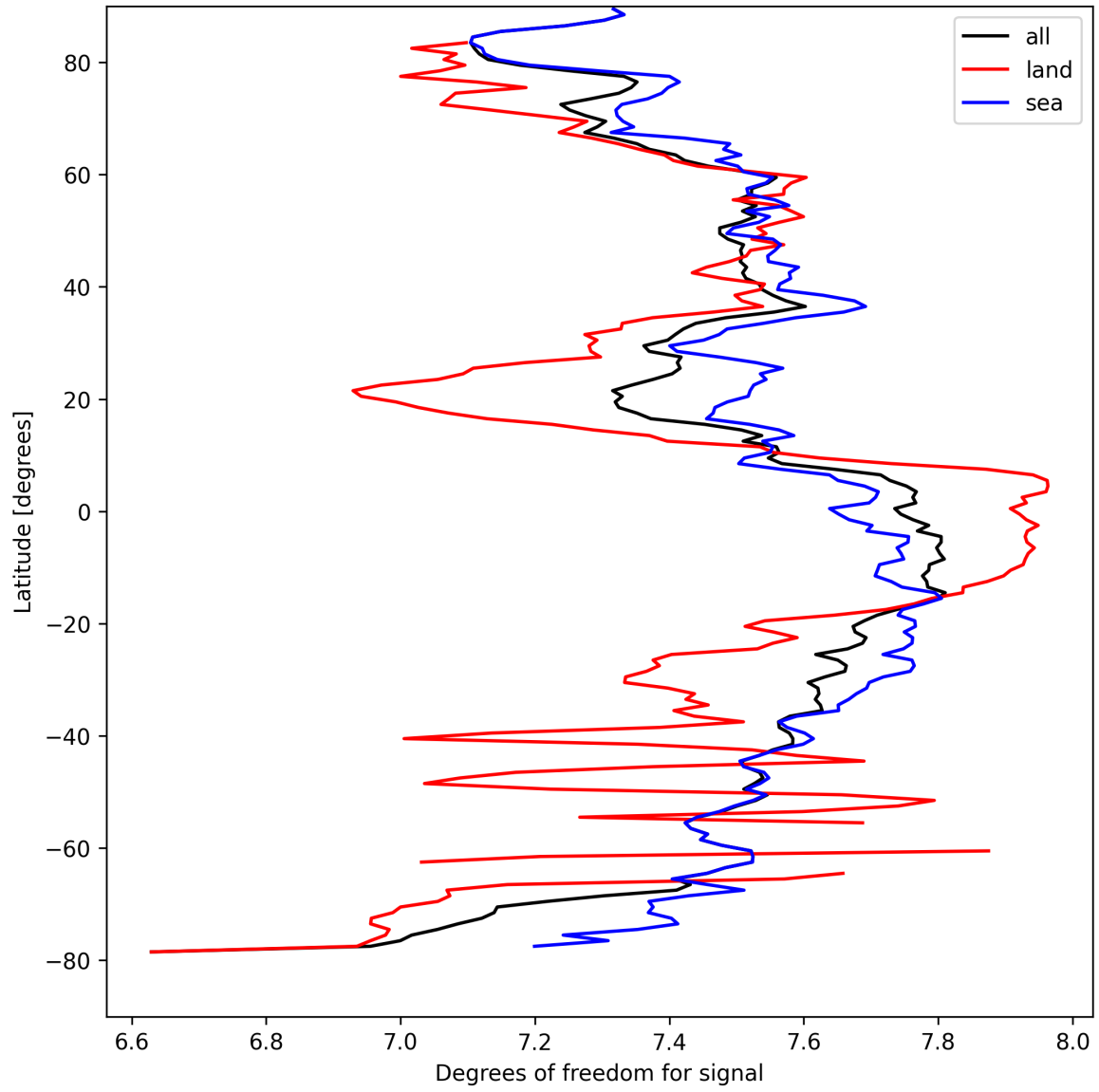
Figure 11: Zonal average of “Degrees of freedom for signal” for 2025-04-07 to 2025-04-08.
