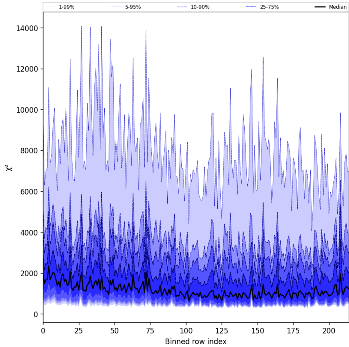
Figure 24: Along track statistics of “ \chi^2 ” for 2025-04-07 to 2025-04-08
