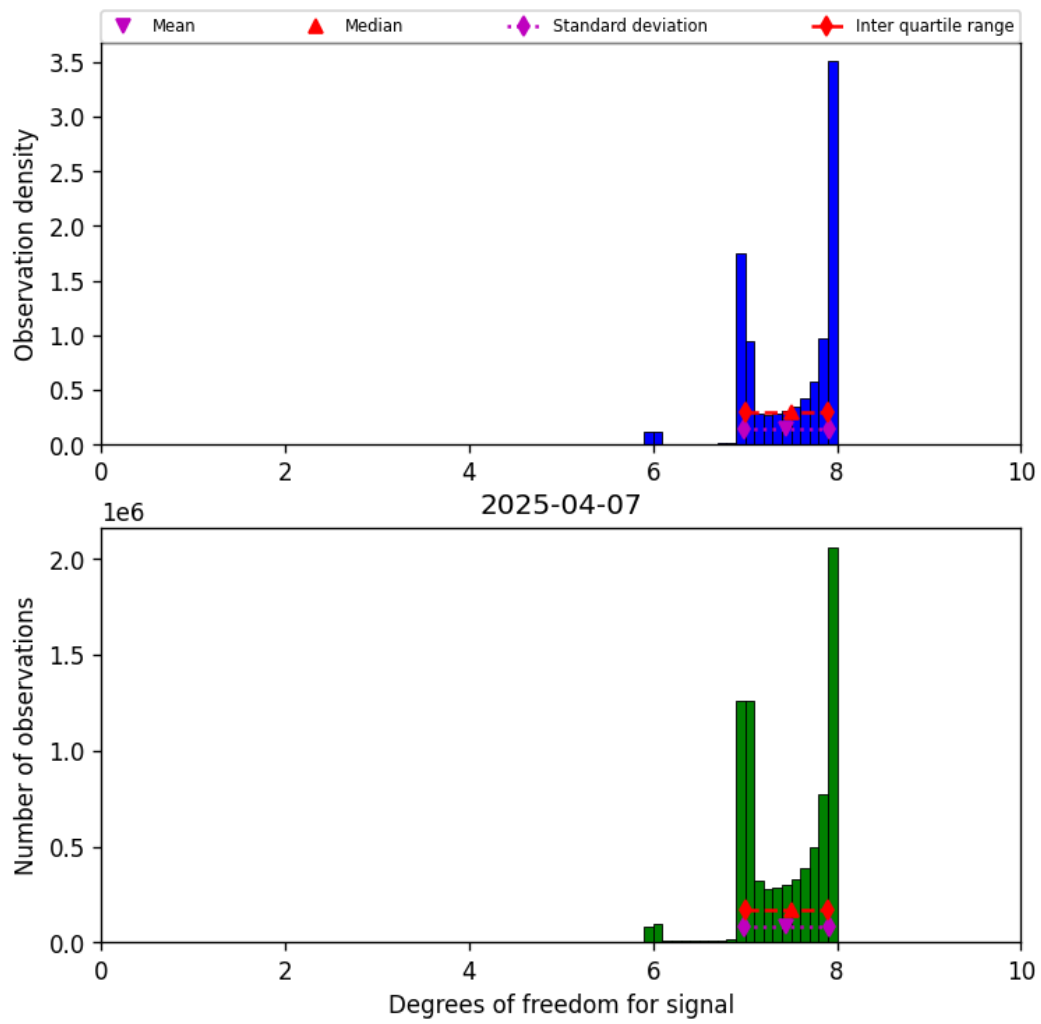
Figure 18: Histogram of “Degrees of freedom for signal” for 2025-04-07 to 2025-04-08
