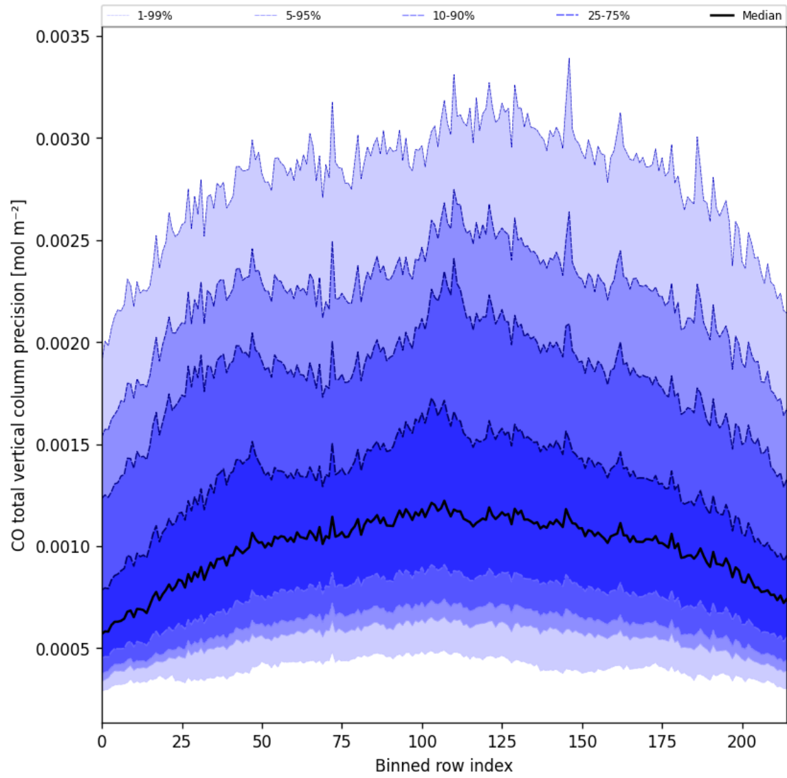
Figure 22: Along track statistics of “CO total vertical column precision” for 2025-04-07 to 2025-04-08
