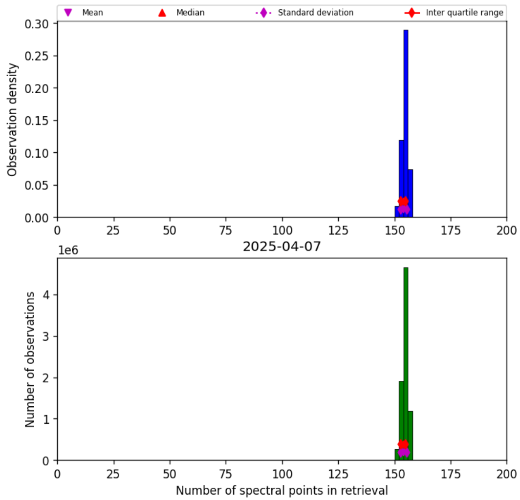
Figure 16: Histogram of “Number of spectral points in retrieval” for 2025-04-07 to 2025-04-08
