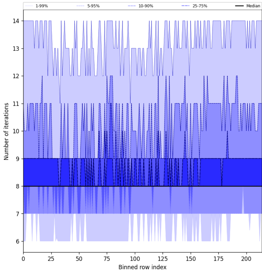
Figure 26: Along track statistics of “Number of iterations” for 2025-04-07 to 2025-04-08
