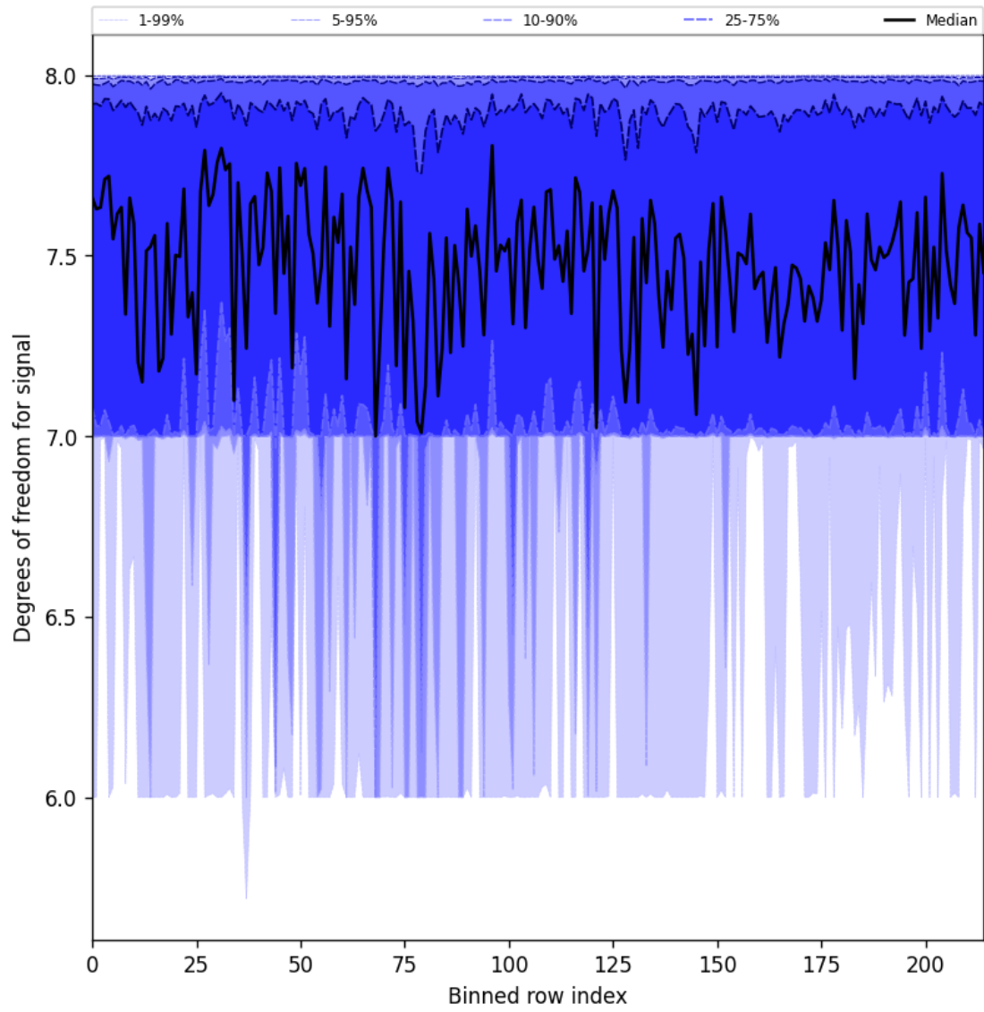
Figure 25: Along track statistics of “Degrees of freedom for signal” for 2025-04-07 to 2025-04-08
