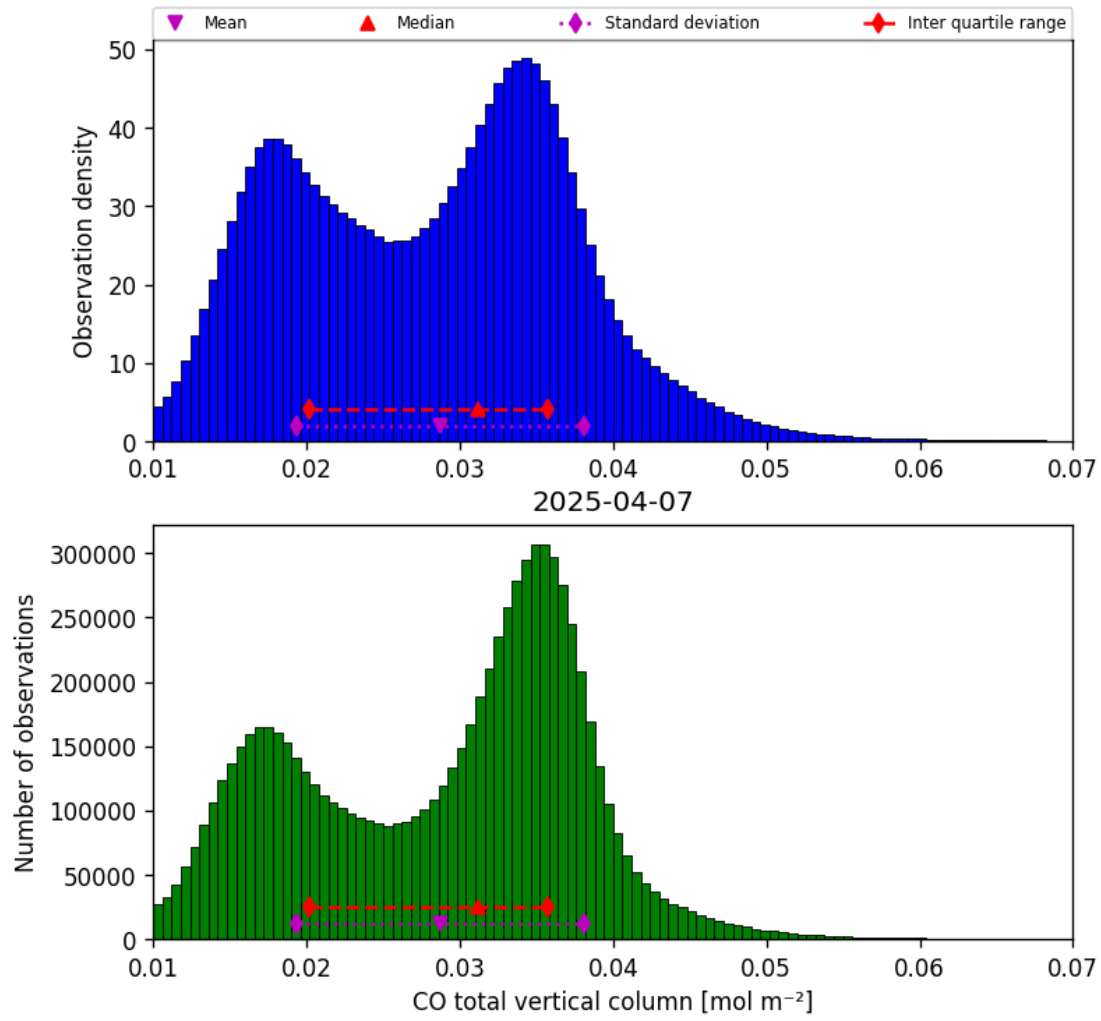
Figure 14: Histogram of “CO total vertical column” for 2025-04-07 to 2025-04-08
