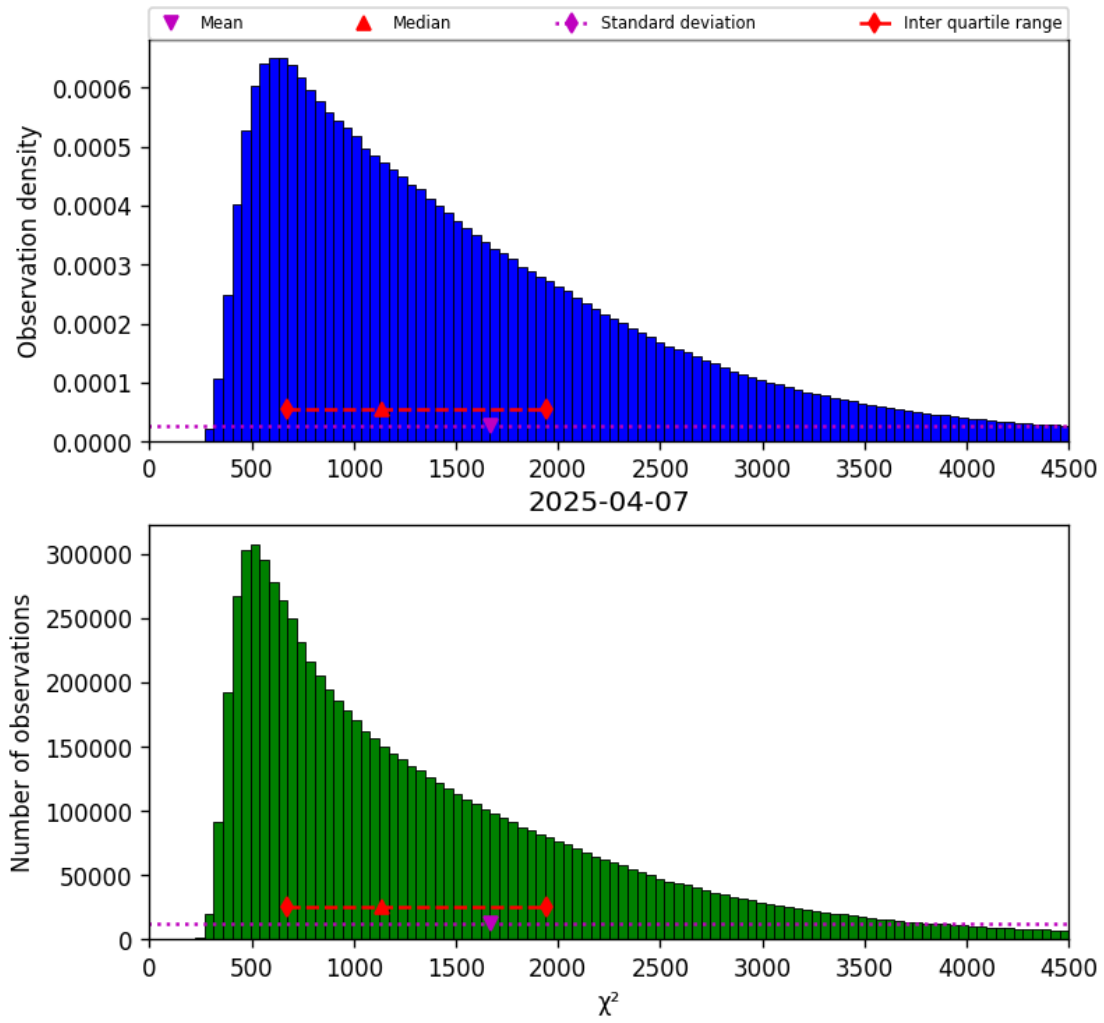
Figure 17: Histogram of “ \chi^2 ” for 2025-04-07 to 2025-04-08
