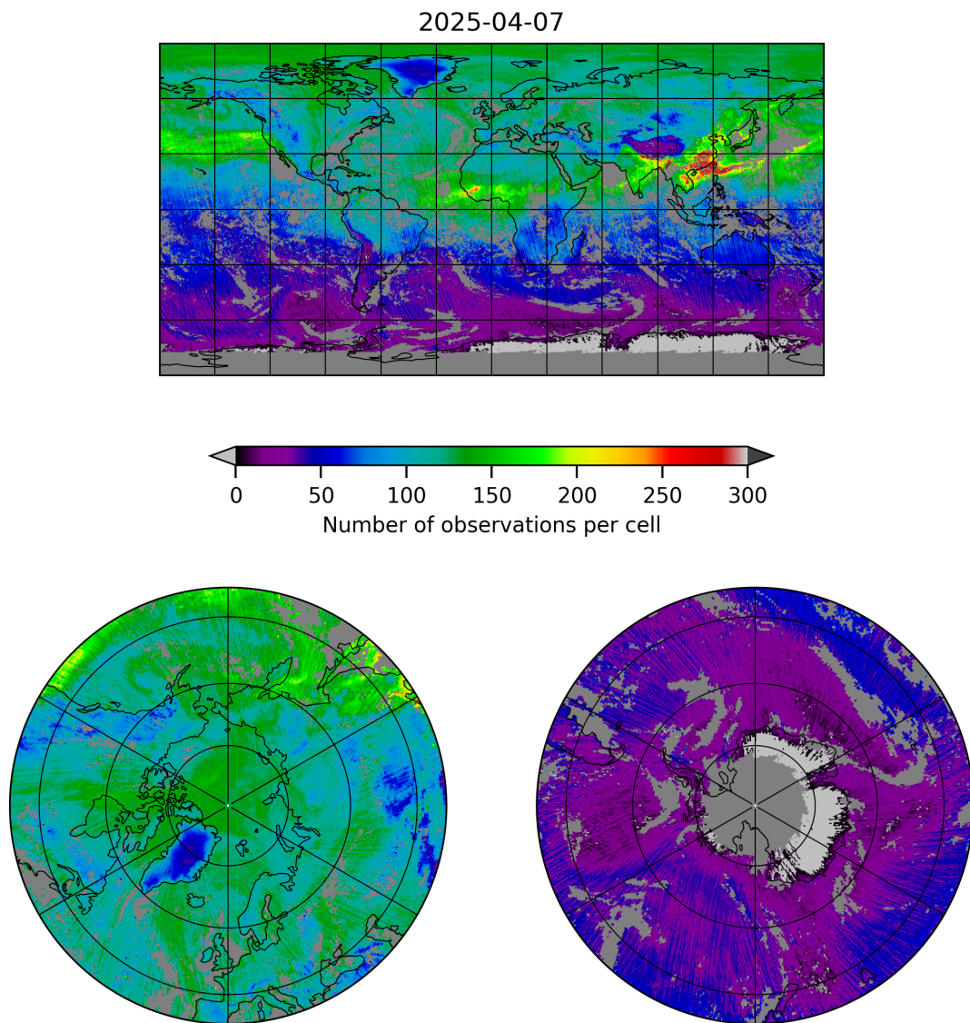
Figure 5: Map of the number of observations for 2025-04-07 to 2025-04-08
