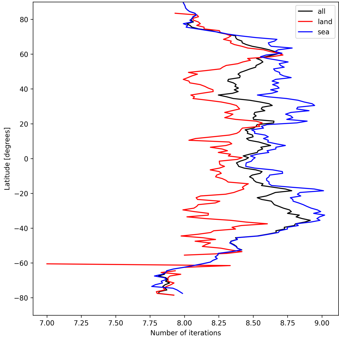
Figure 12: Zonal average of “Number of iterations” for 2025-04-07 to 2025-04-08.
