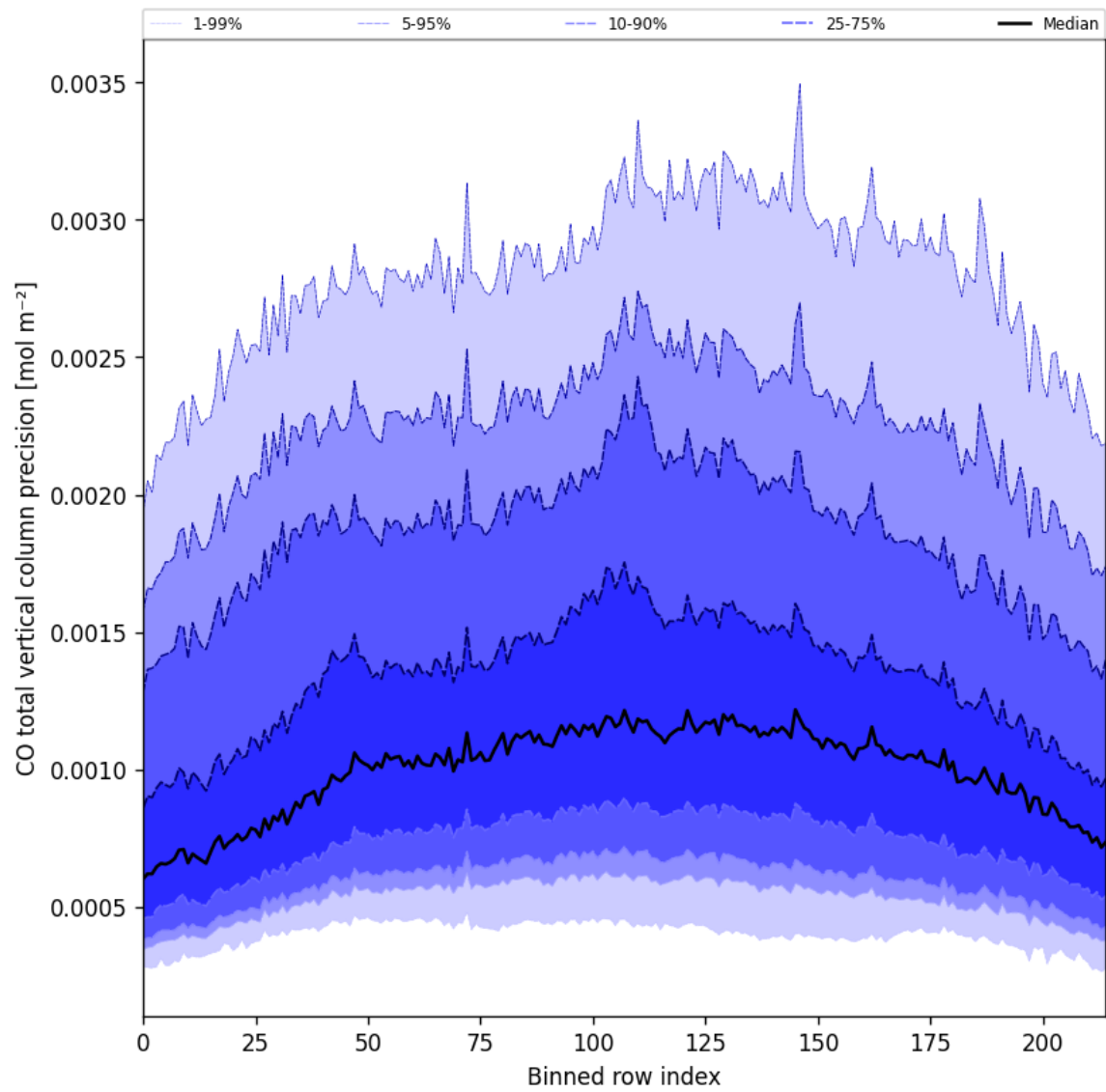
Figure 22: Along track statistics of “CO total vertical column precision” for 2025-04-08 to 2025-04-09
