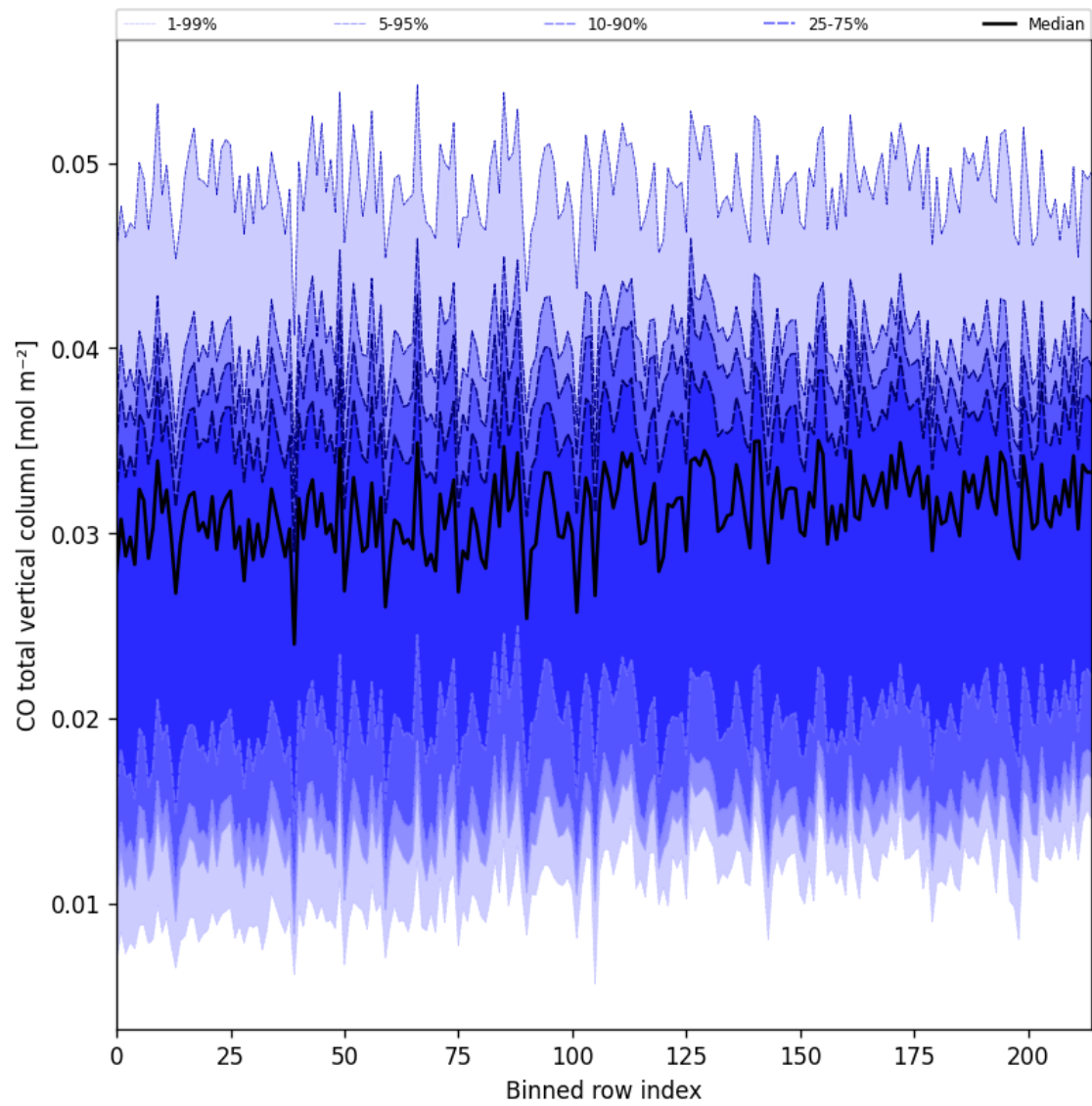
Figure 21: Along track statistics of “CO total vertical column” for 2025-04-08 to 2025-04-09
