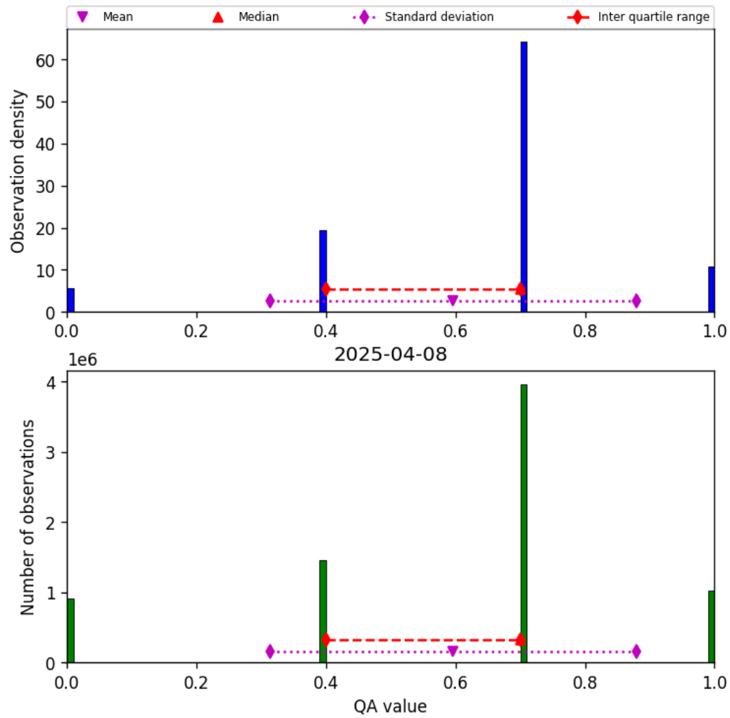
Figure 13: Histogram of “QA value” for 2025-04-08 to 2025-04-09
