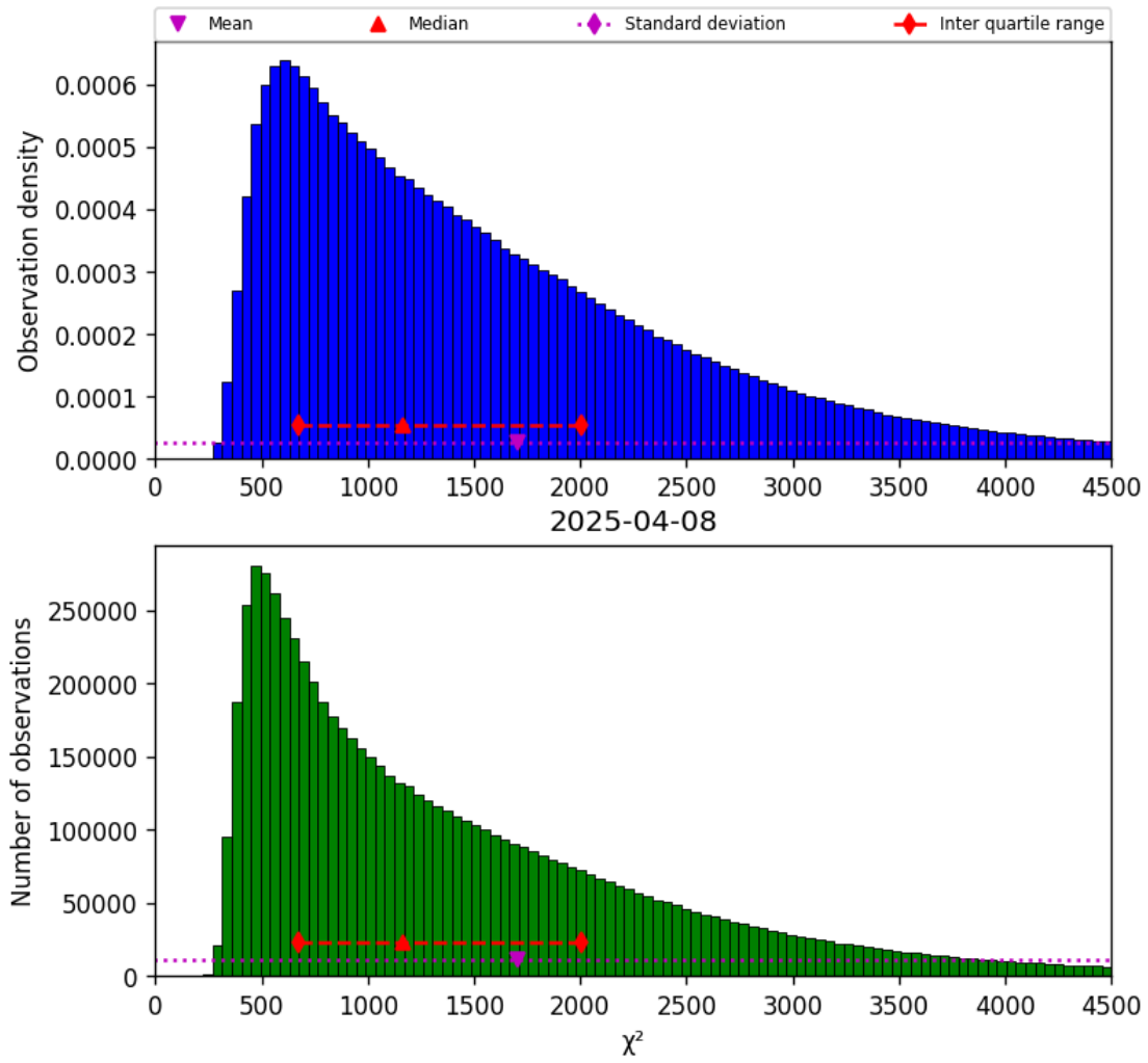
Figure 17: Histogram of " \chi^2 " for 2025-04-08 to 2025-04-09
