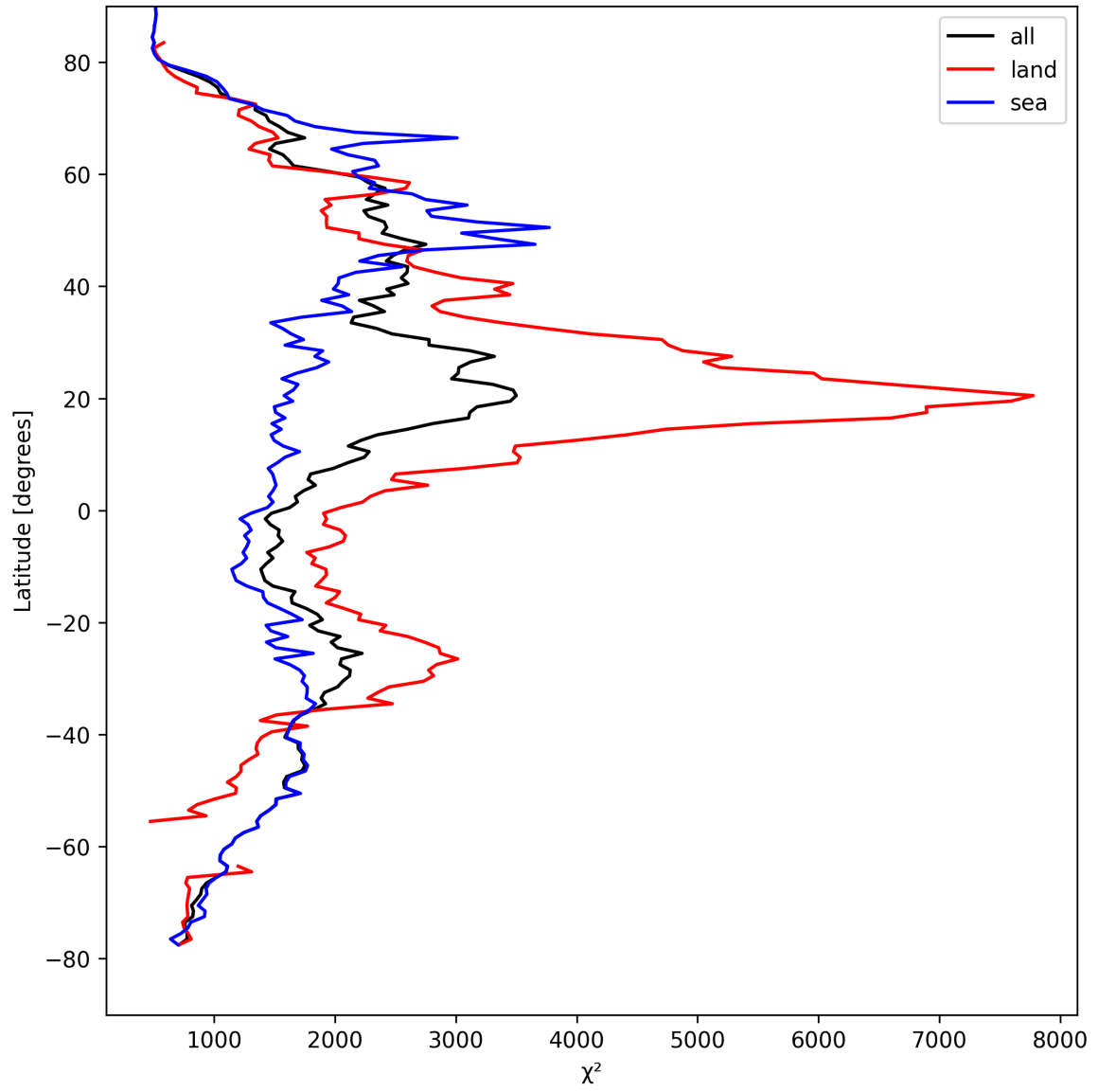
Figure 10: Zonal average of “ \chi^2 ” for 2025-04-08 to 2025-04-09.
