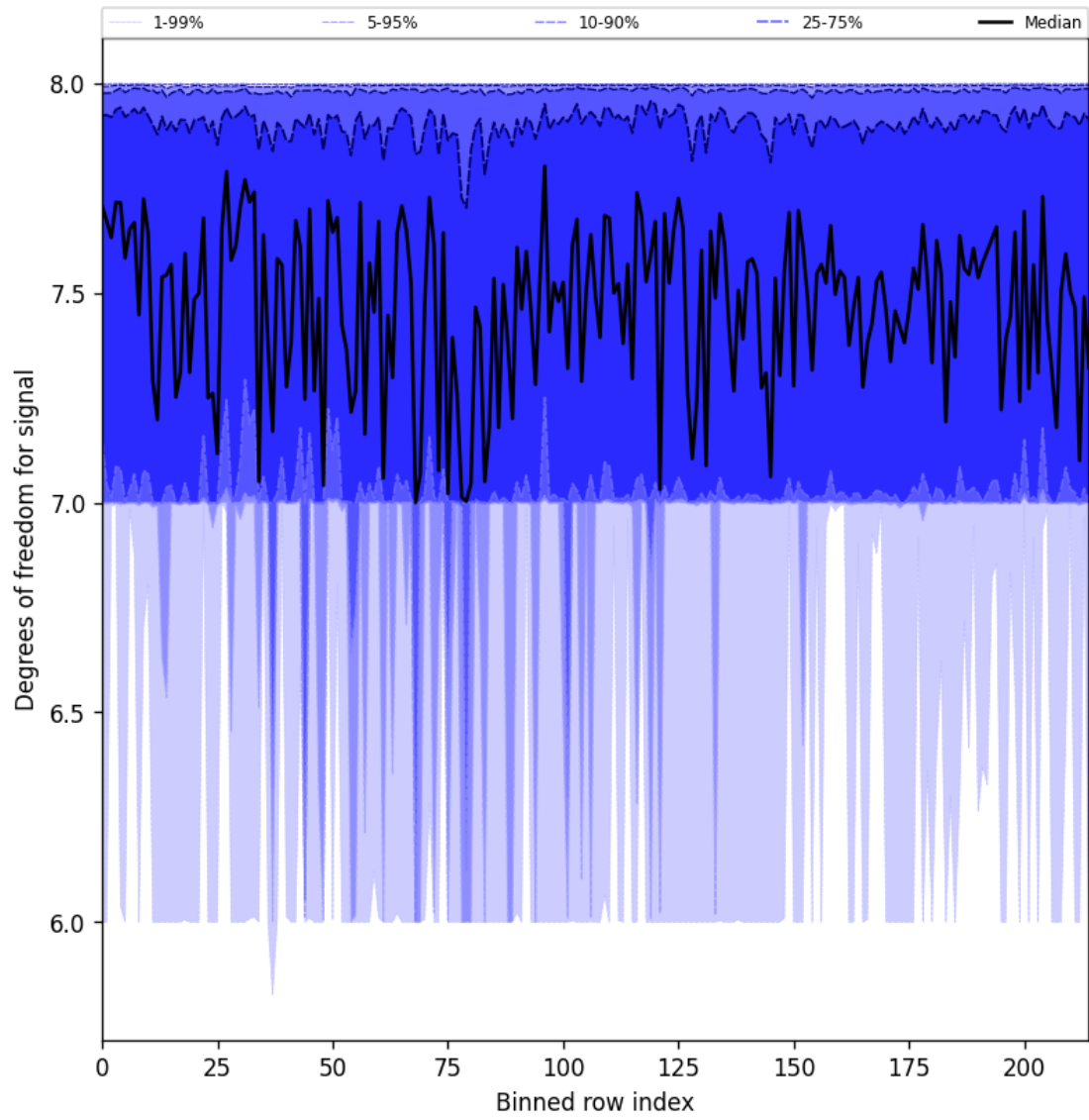
Figure 25: Along track statistics of “Degrees of freedom for signal” for 2025-04-08 to 2025-04-09
