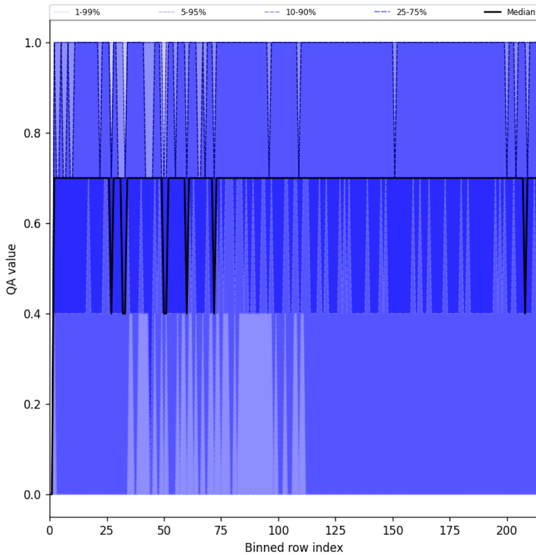
Figure 20: Along track statistics of “QA value” for 2025-04-08 to 2025-04-09
