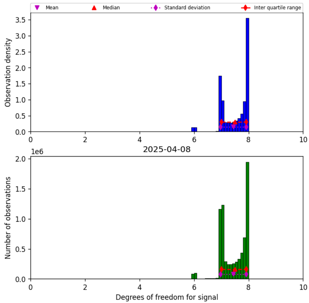
Figure 18: Histogram of “Degrees of freedom for signal” for 2025-04-08 to 2025-04-09
