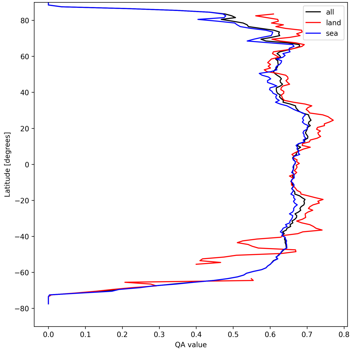
Figure 6: Zonal average of “QA value” for 2025-04-08 to 2025-04-09.
