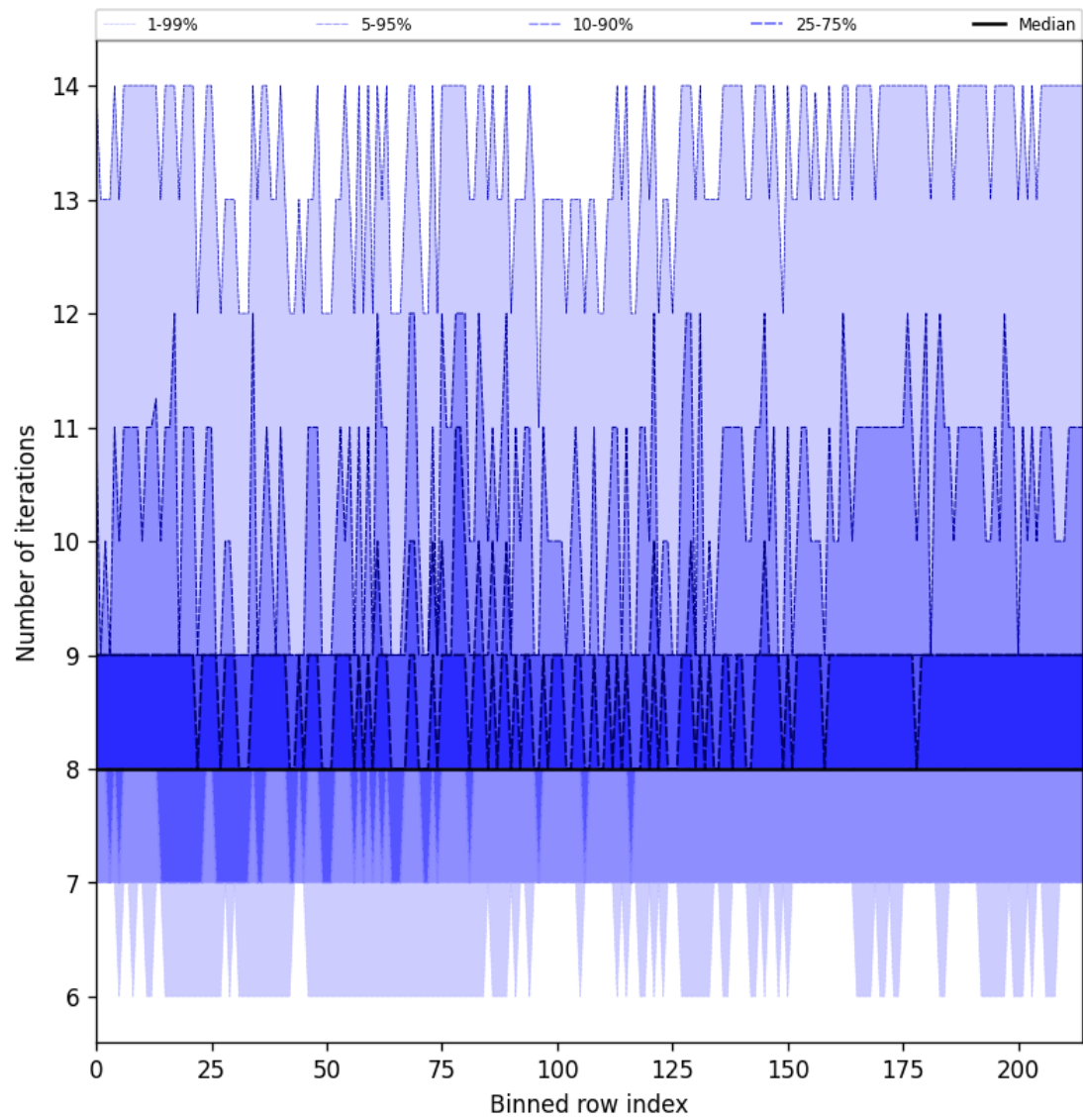
Figure 26: Along track statistics of “Number of iterations” for 2025-04-08 to 2025-04-09
