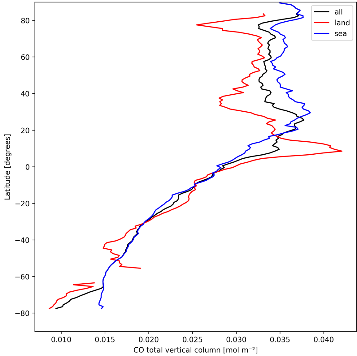
Figure 7: Zonal average of “CO total vertical column” for 2025-04-08 to 2025-04-09.
