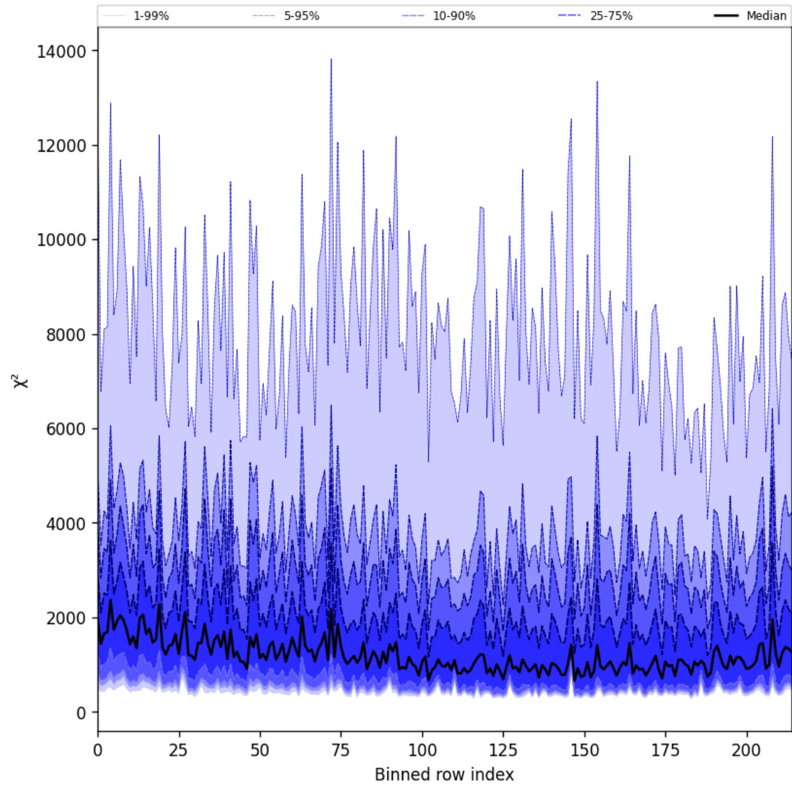
Figure 24: Along track statistics of “ \chi^2 ” for 2025-04-08 to 2025-04-09
