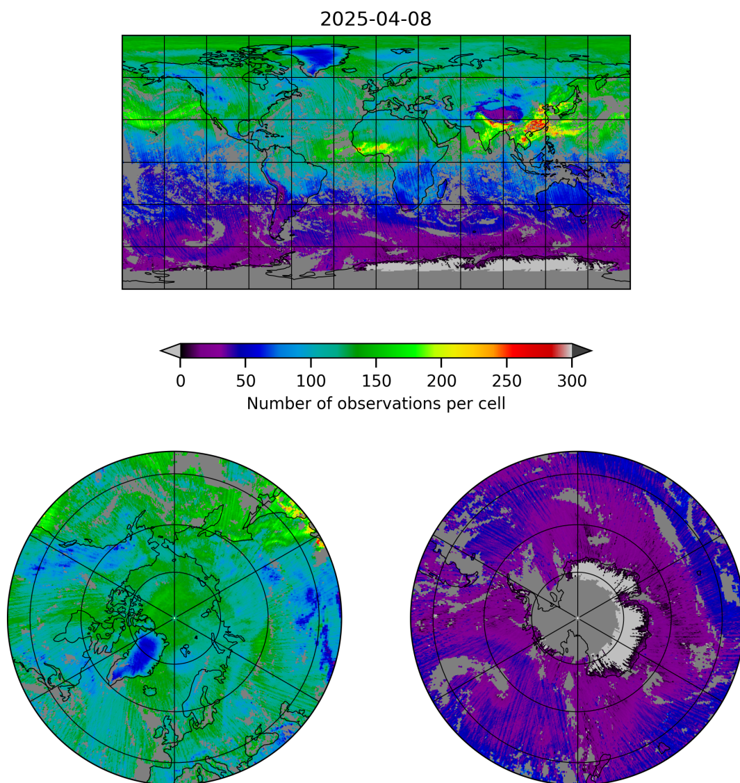
Figure 5: Map of the number of observations for 2025-04-08 to 2025-04-09
