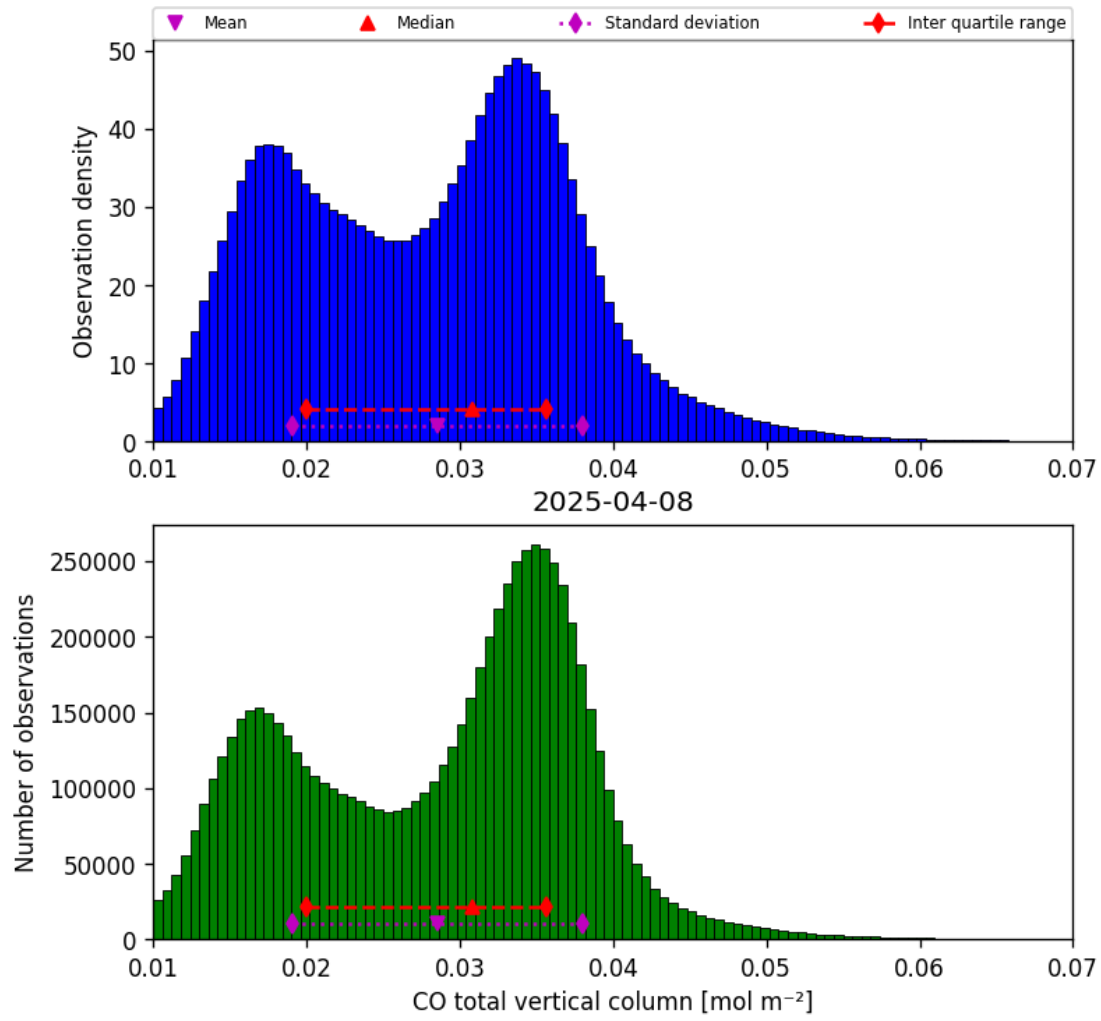
Figure 14: Histogram of “CO total vertical column” for 2025-04-08 to 2025-04-09
