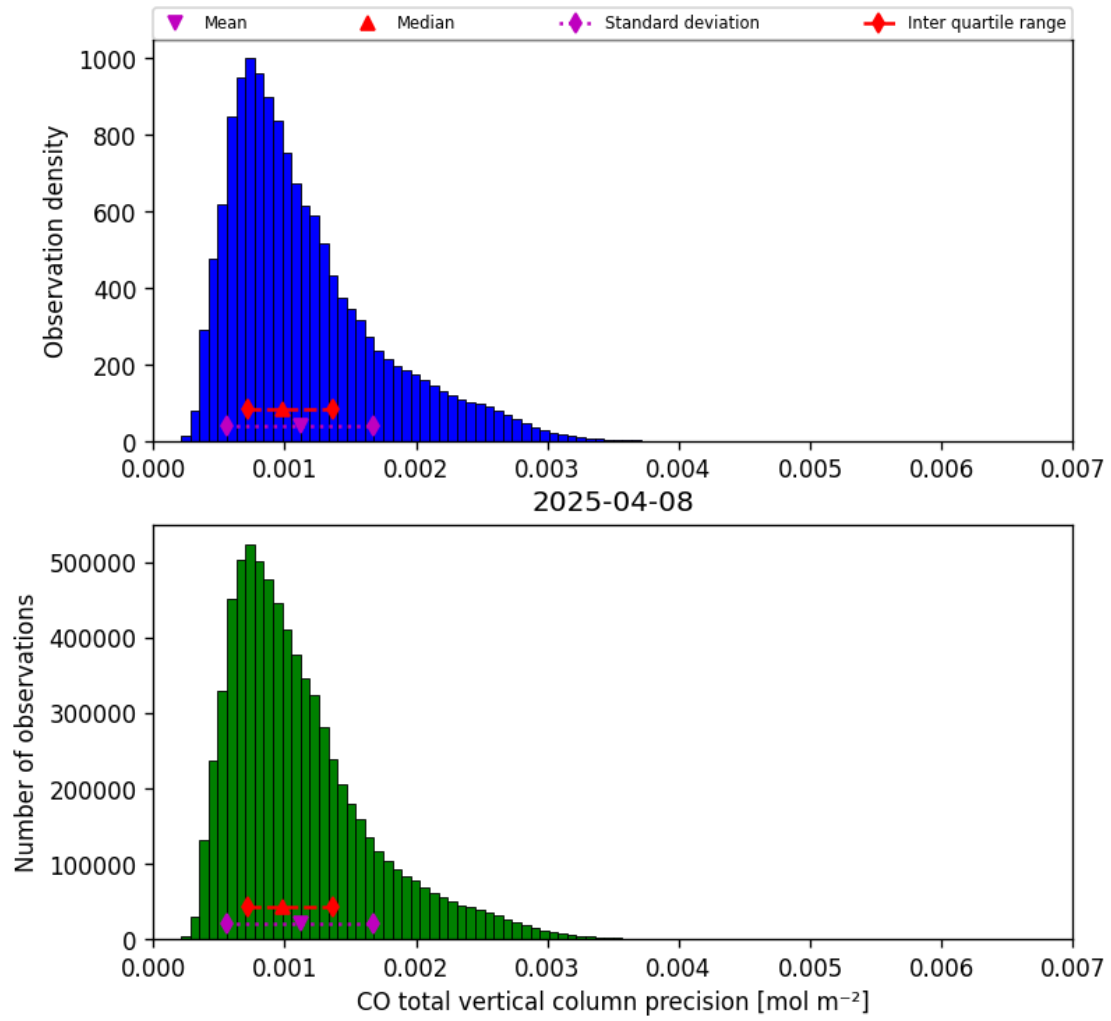
Figure 15: Histogram of “CO total vertical column precision” for 2025-04-08 to 2025-04-09
