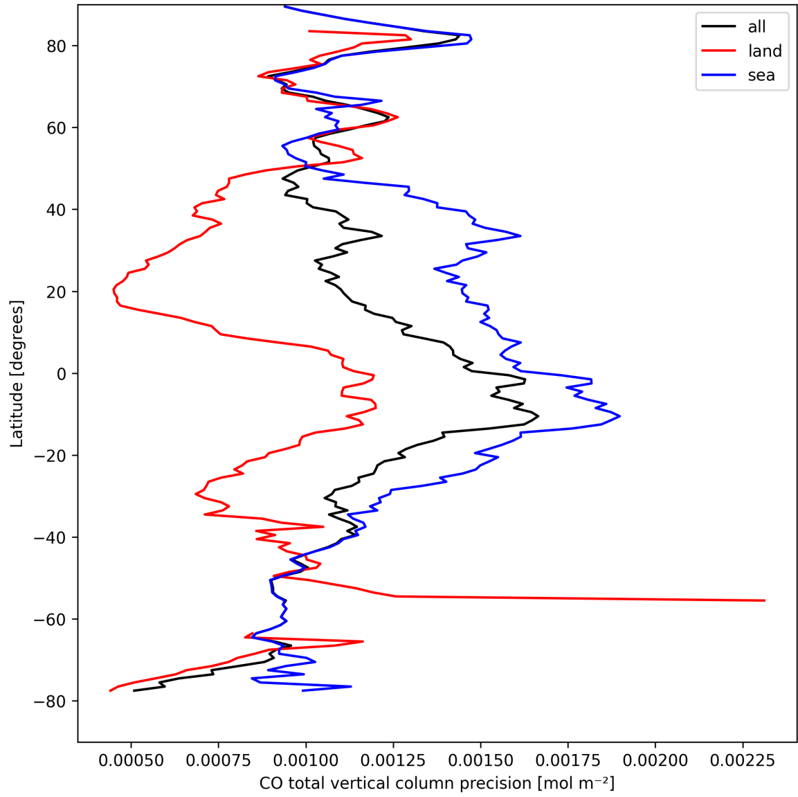
Figure 8: Zonal average of “CO total vertical column precision” for 2025-04-08 to 2025-04-09.
