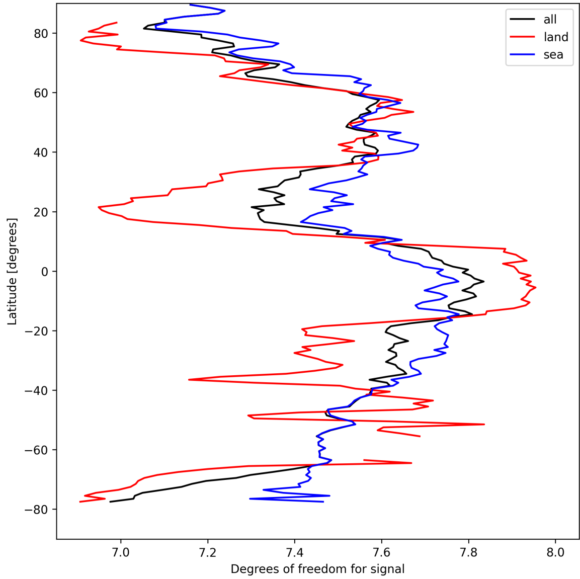
Figure 11: Zonal average of “Degrees of freedom for signal” for 2025-04-08 to 2025-04-09.
