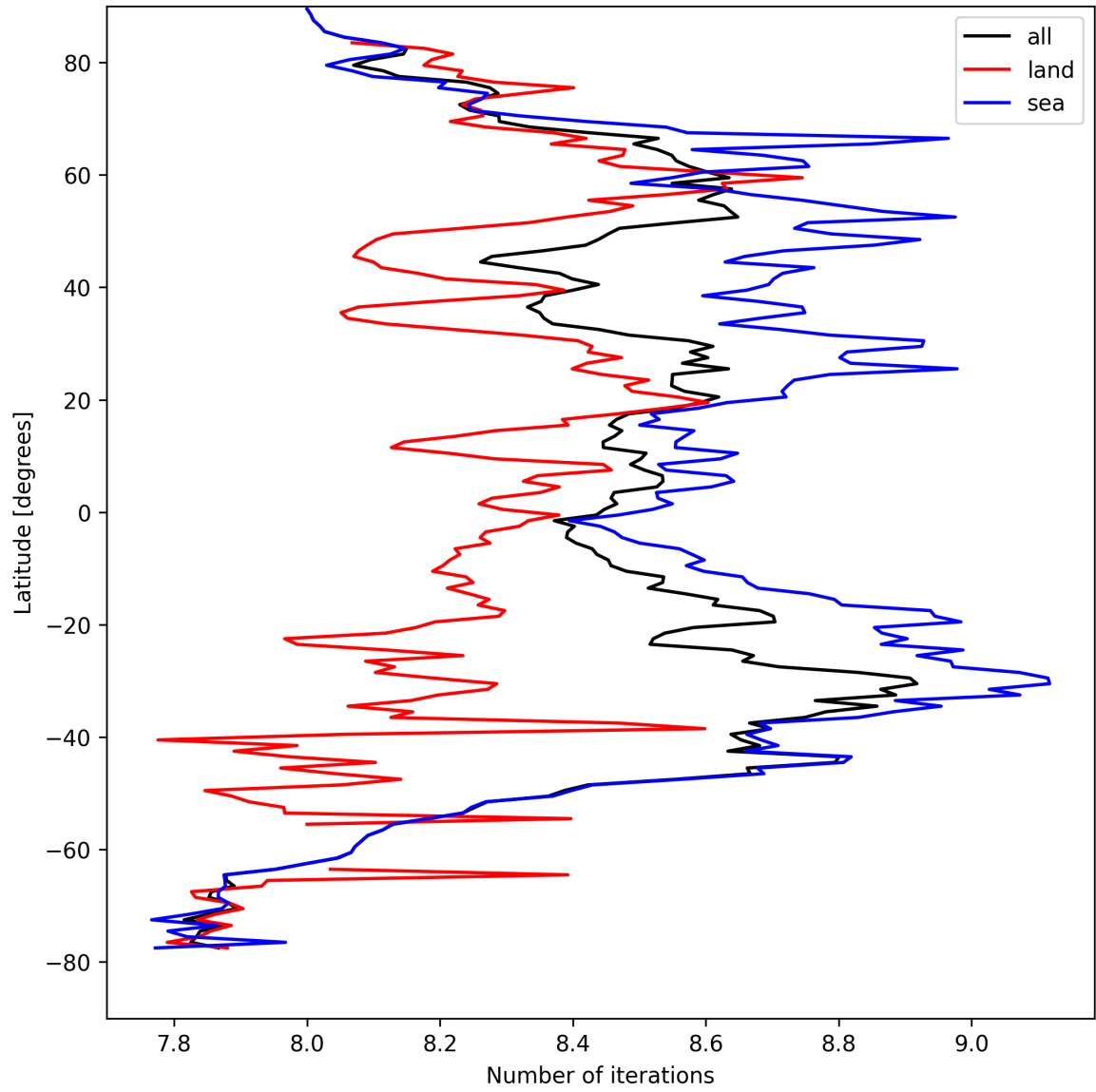
Figure 12: Zonal average of “Number of iterations” for 2025-04-08 to 2025-04-09.
