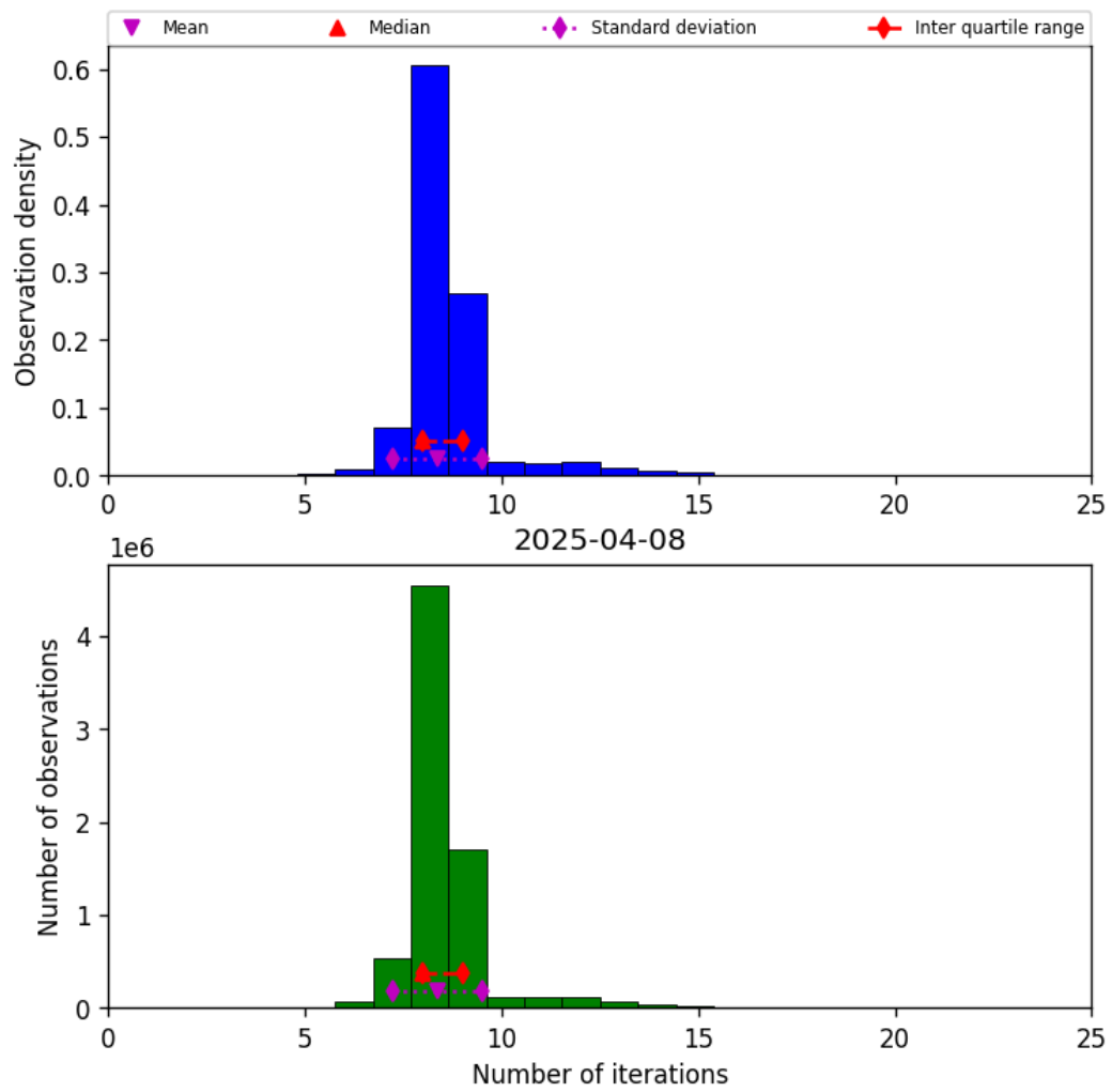
Figure 19: Histogram of “Number of iterations” for 2025-04-08 to 2025-04-09
