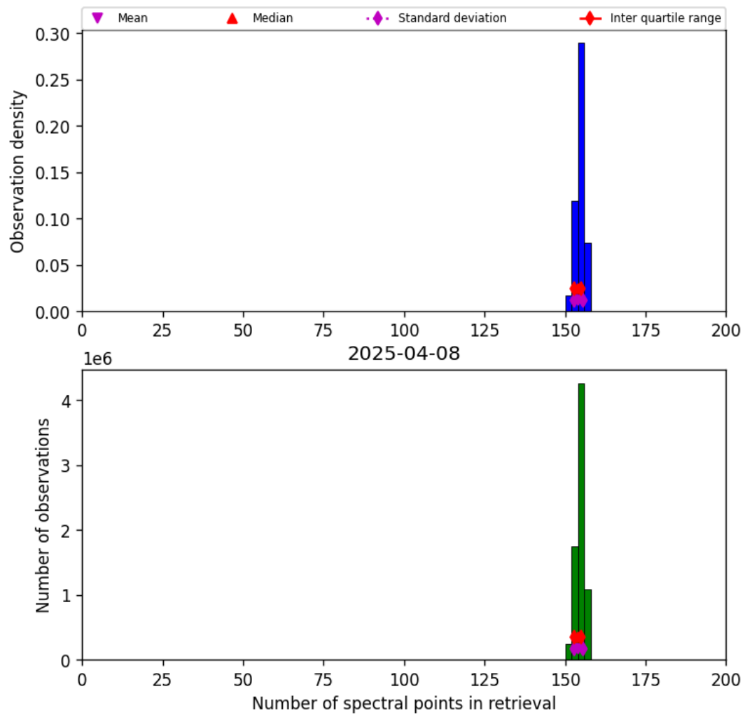
Figure 16: Histogram of “Number of spectral points in retrieval” for 2025-04-08 to 2025-04-09
