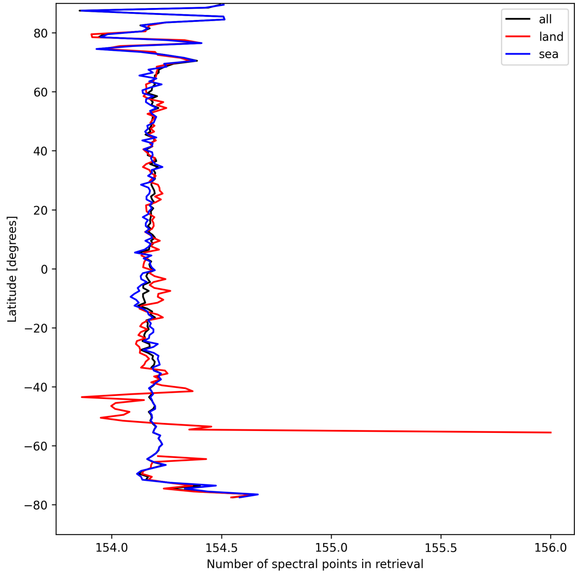
Figure 9: Zonal average of “Number of spectral points in retrieval” for 2025-04-08 to 2025-04-09.
