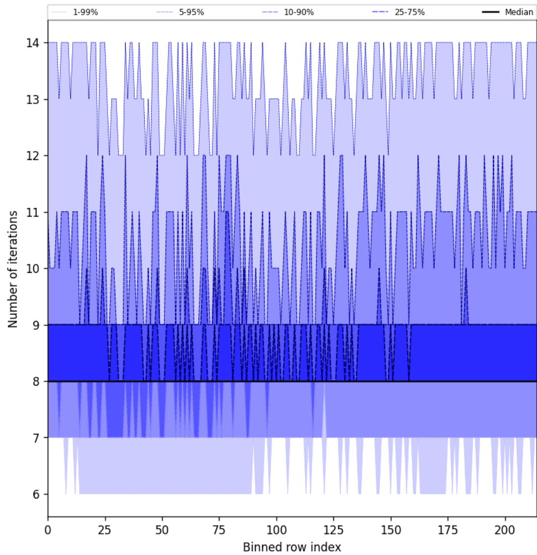
Figure 26: Along track statistics of “Number of iterations” for 2025-04-09 to 2025-04-10
