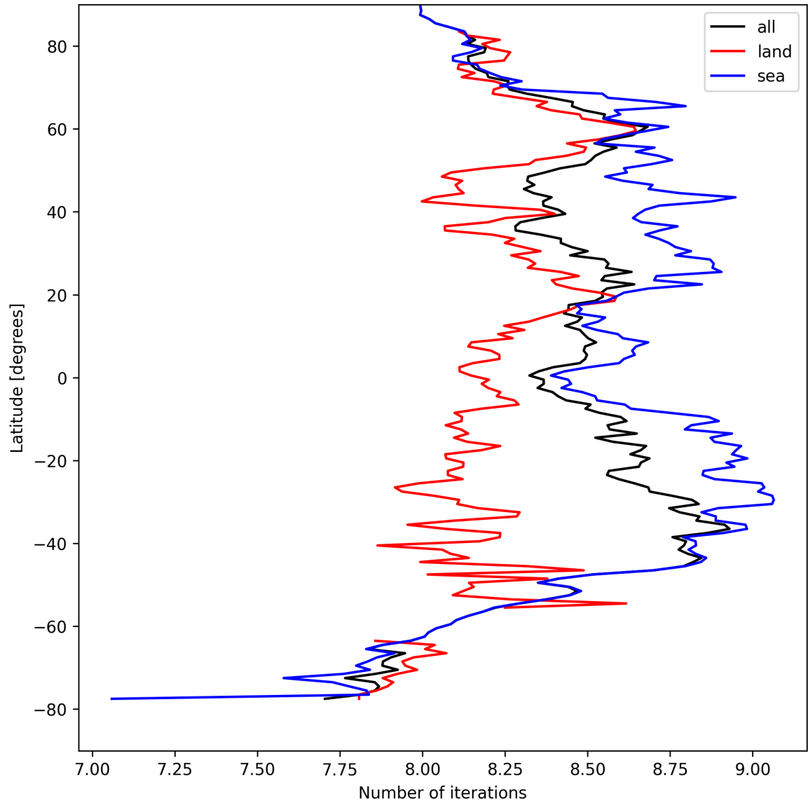
Figure 12: Zonal average of “Number of iterations” for 2025-04-09 to 2025-04-10.
