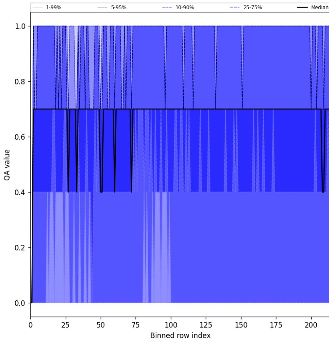
Figure 20: Along track statistics of “QA value” for 2025-04-09 to 2025-04-10
