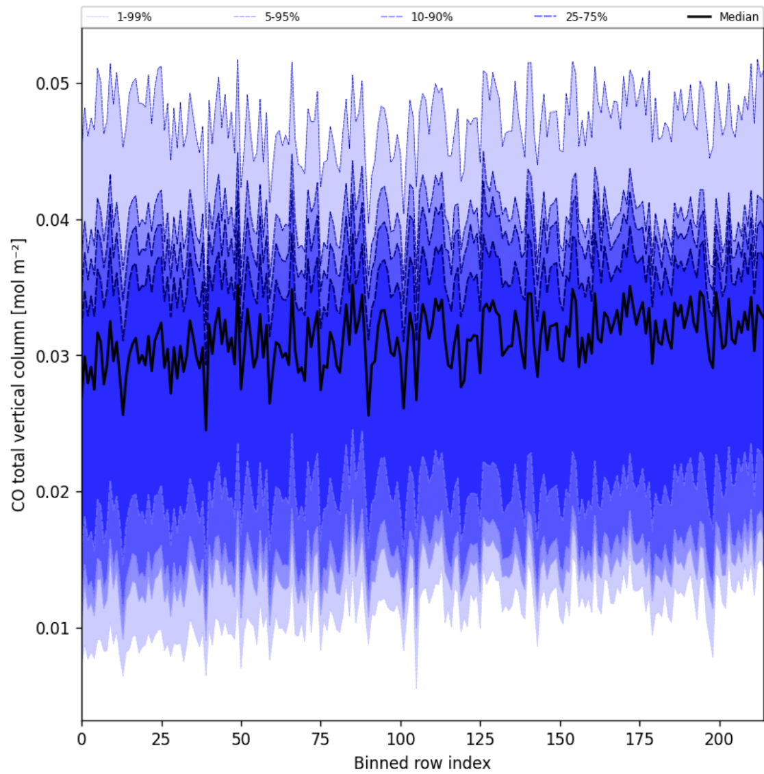
Figure 21: Along track statistics of “CO total vertical column” for 2025-04-09 to 2025-04-10
