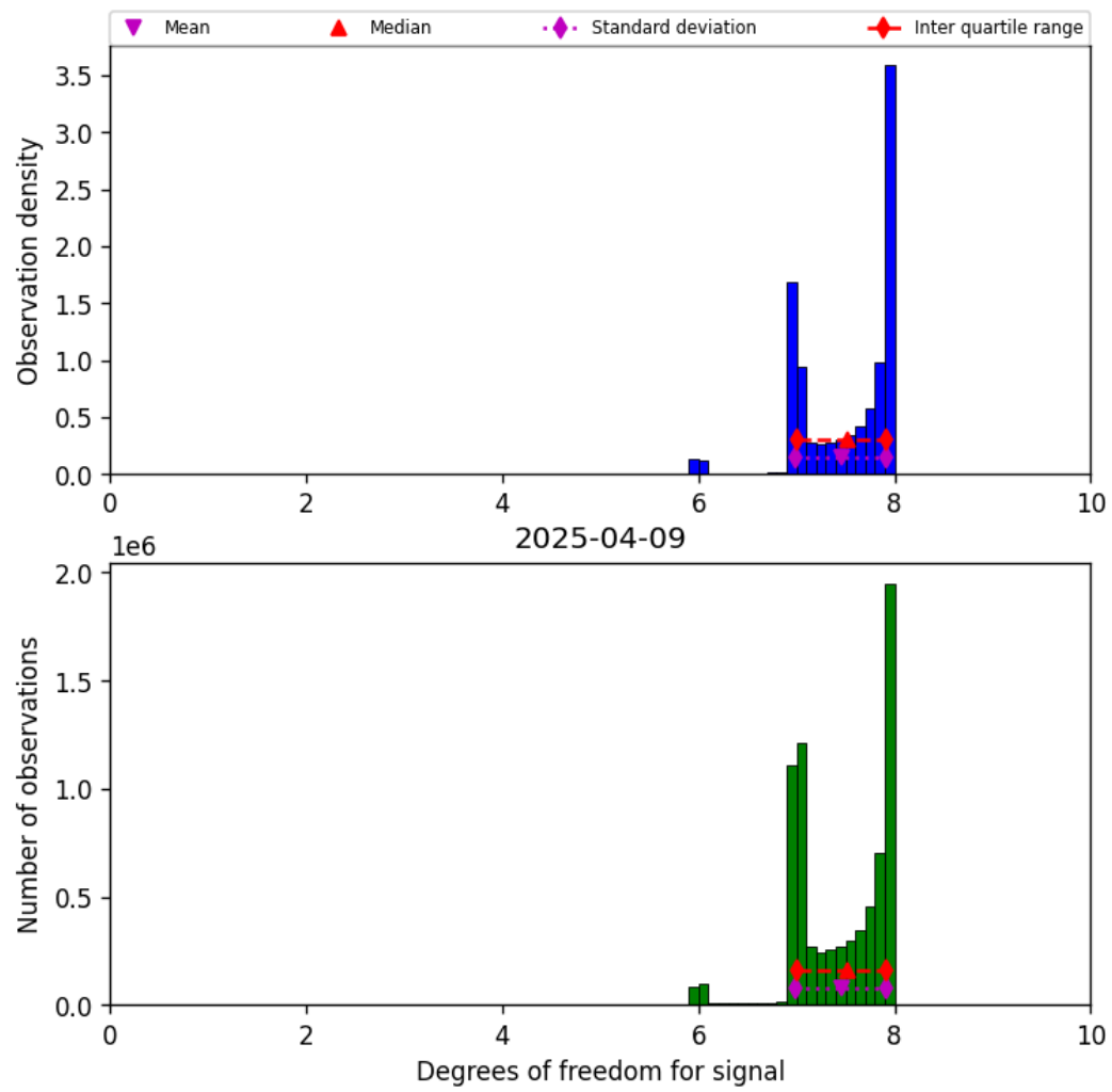
Figure 18: Histogram of “Degrees of freedom for signal” for 2025-04-09 to 2025-04-10
