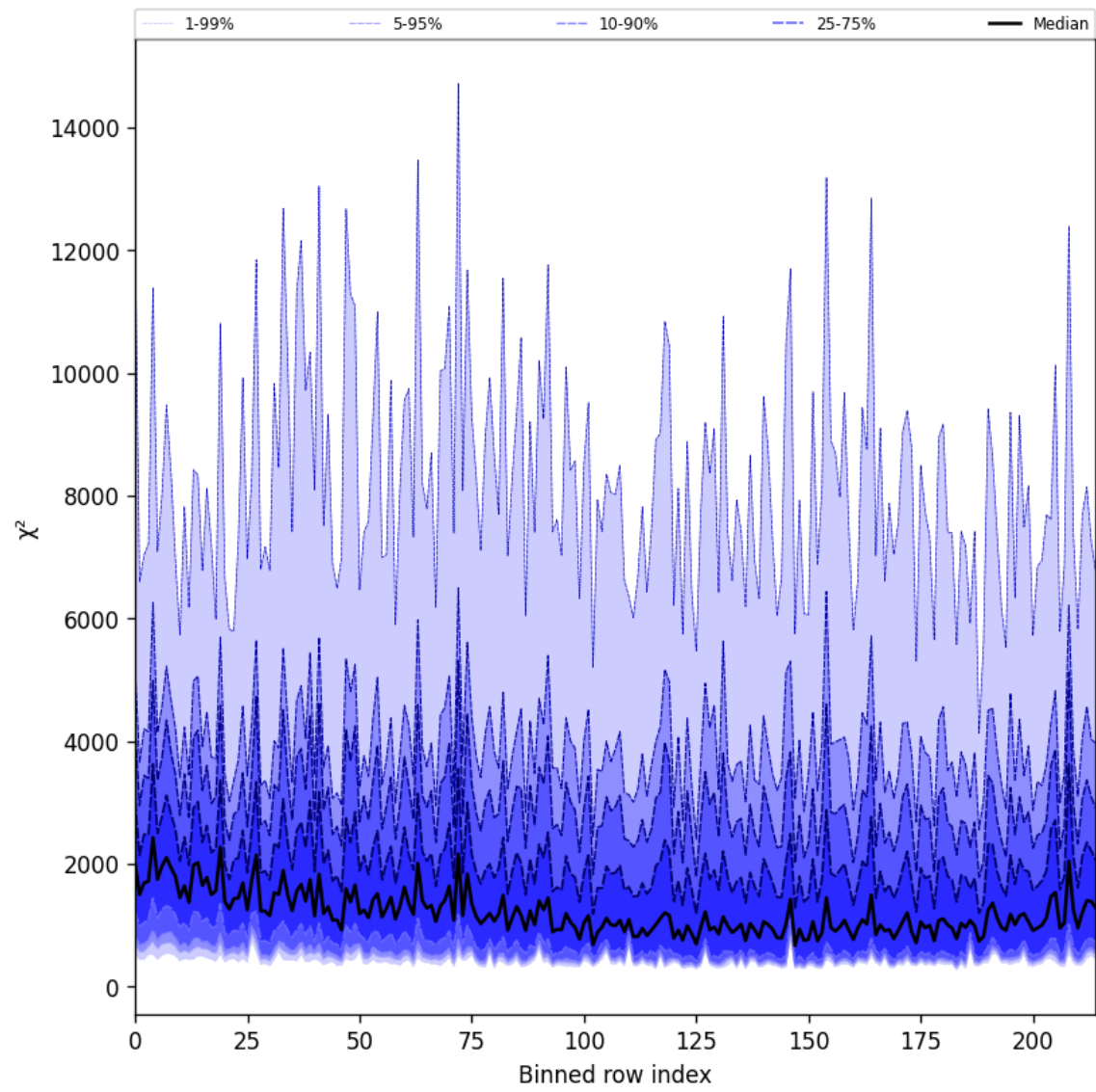
Figure 24: Along track statistics of “ \chi^2 ” for 2025-04-09 to 2025-04-10
