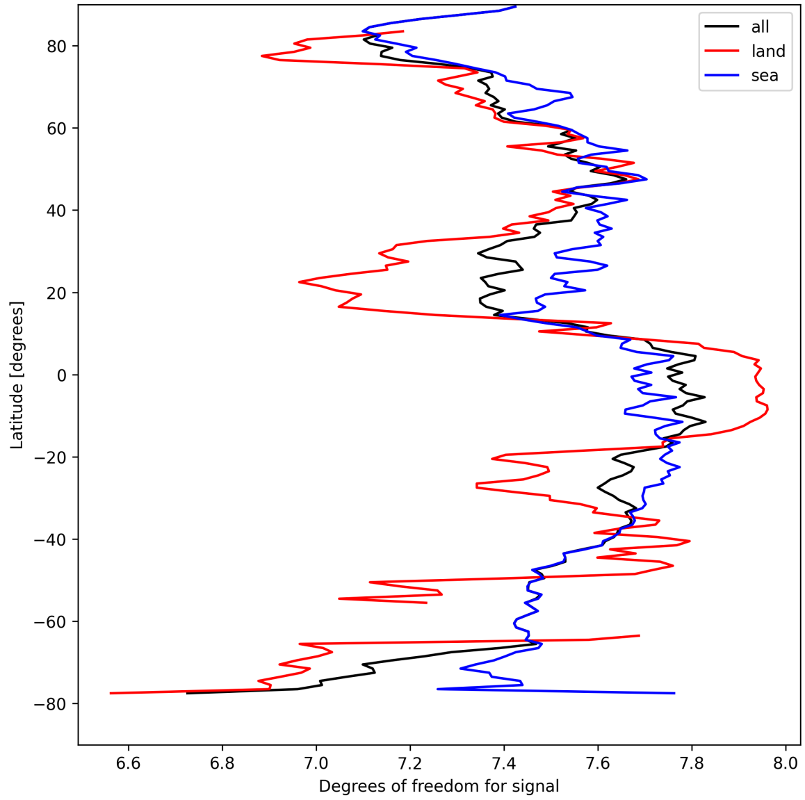
Figure 11: Zonal average of “Degrees of freedom for signal” for 2025-04-09 to 2025-04-10.
