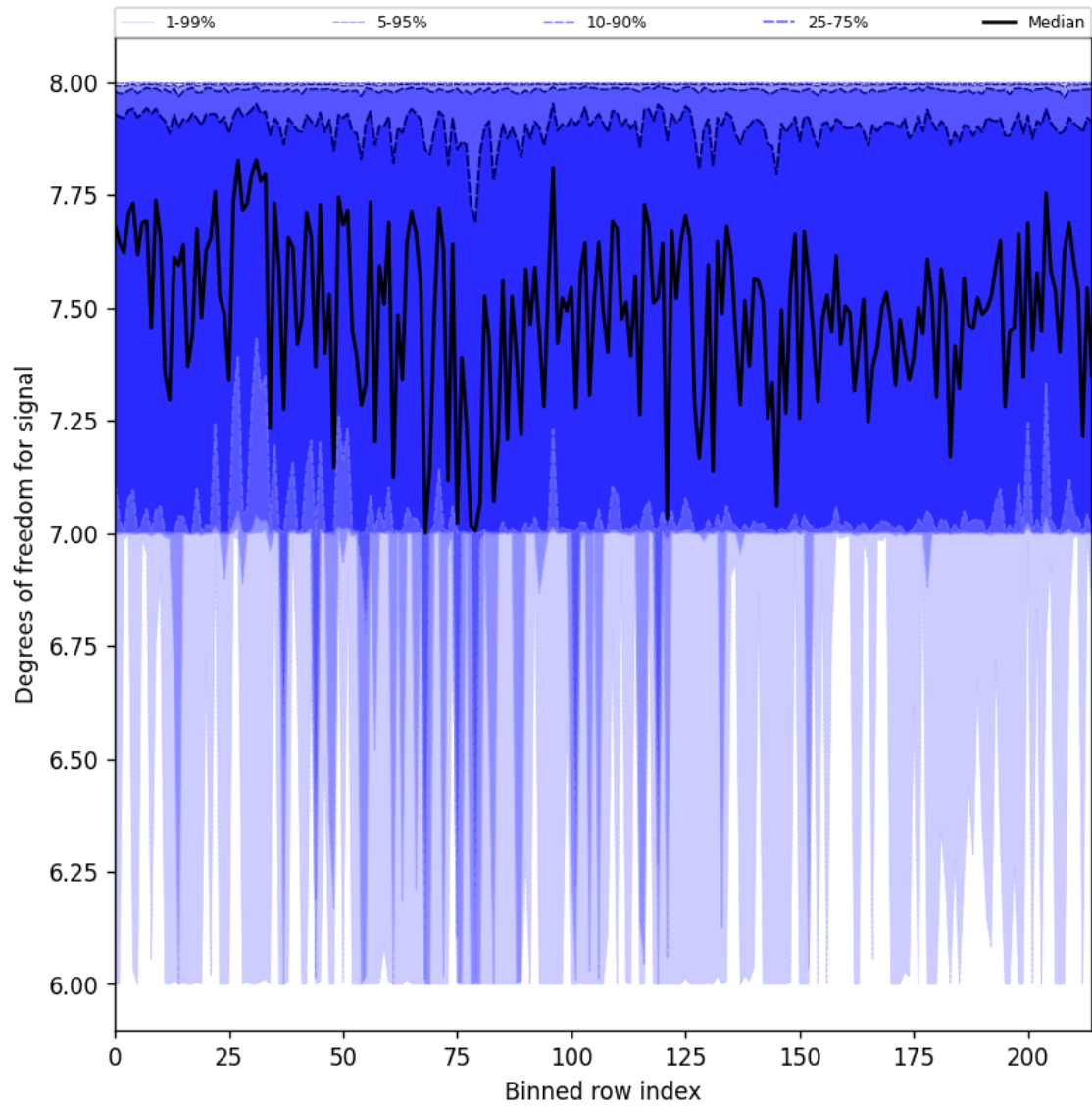
Figure 25: Along track statistics of “Degrees of freedom for signal” for 2025-04-09 to 2025-04-10
