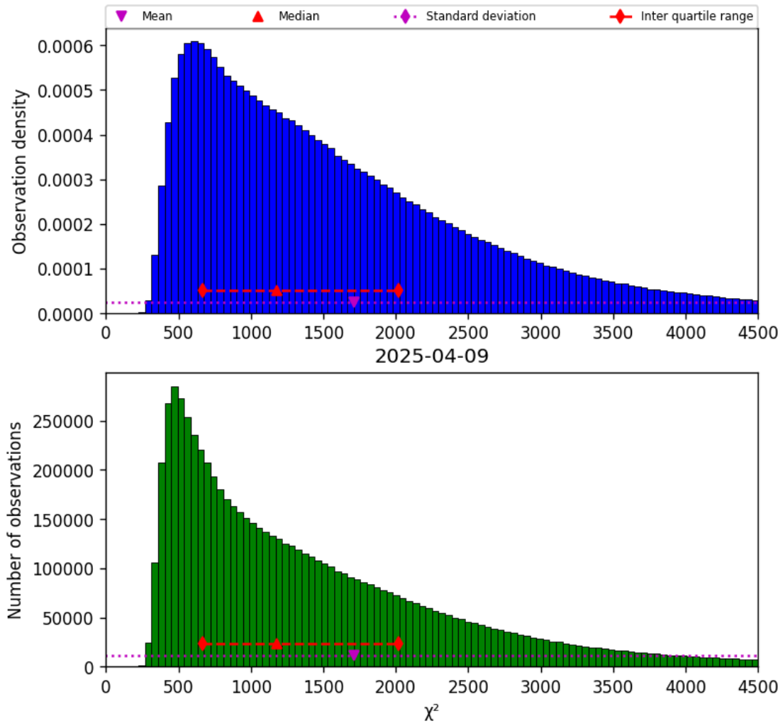
Figure 17: Histogram of “ \chi^2 ” for 2025-04-09 to 2025-04-10
