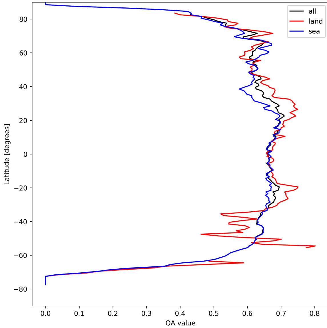
Figure 6: Zonal average of “QA value” for 2025-04-09 to 2025-04-10.
