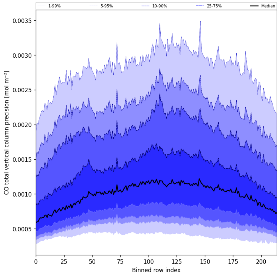
Figure 22: Along track statistics of “CO total vertical column precision” for 2025-04-09 to 2025-04-10
