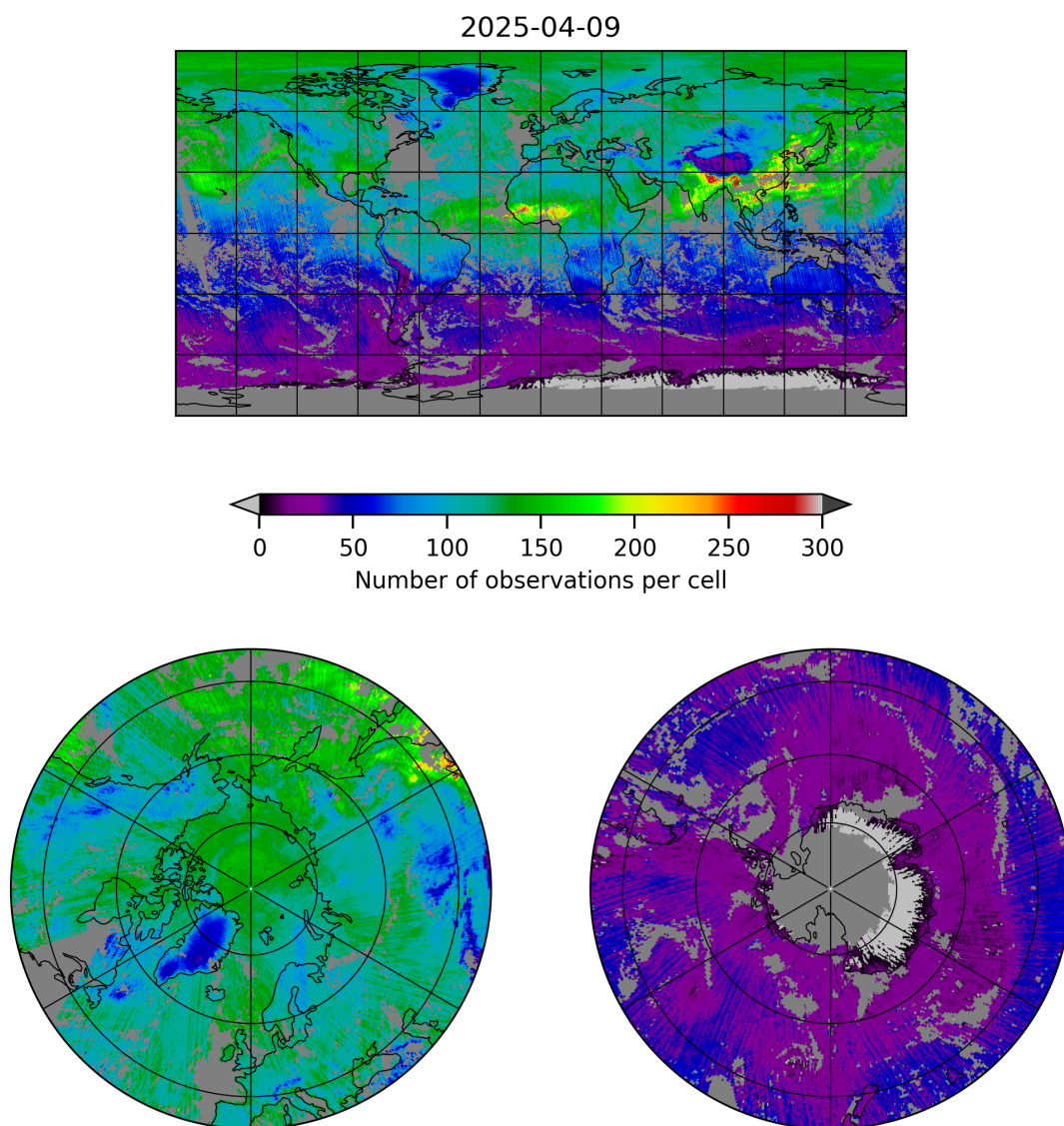
Figure 5: Map of the number of observations for 2025-04-09 to 2025-04-10
