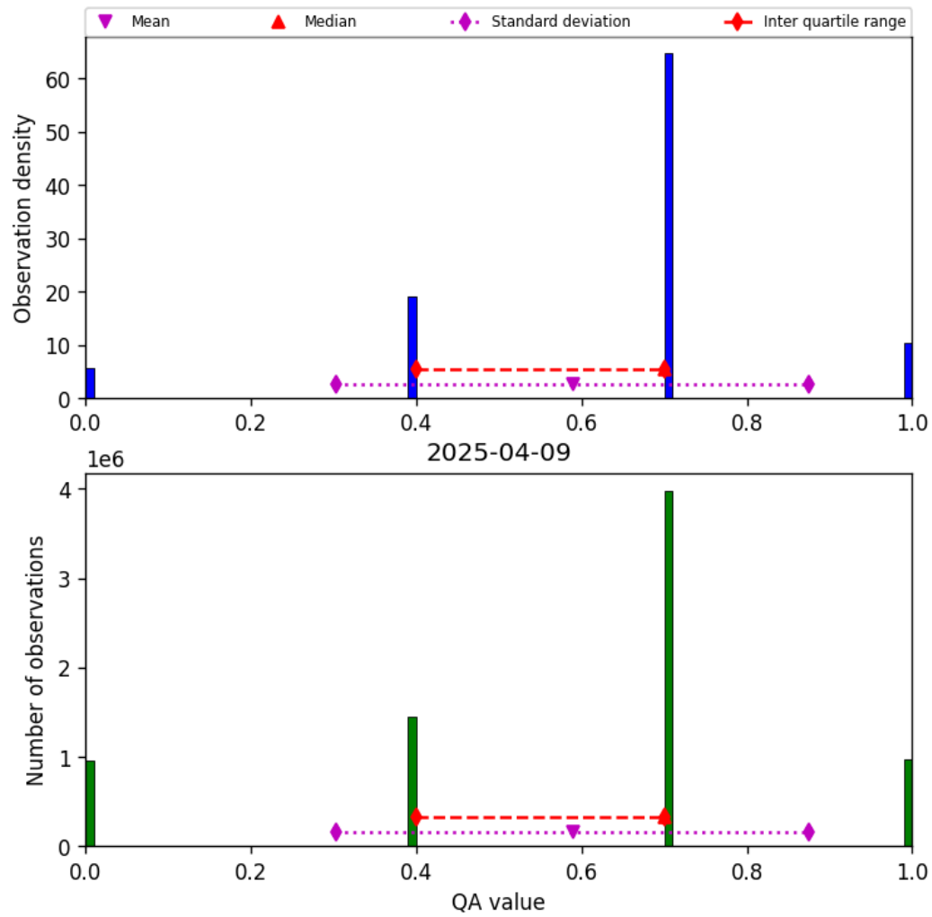
Figure 13: Histogram of “QA value” for 2025-04-09 to 2025-04-10
