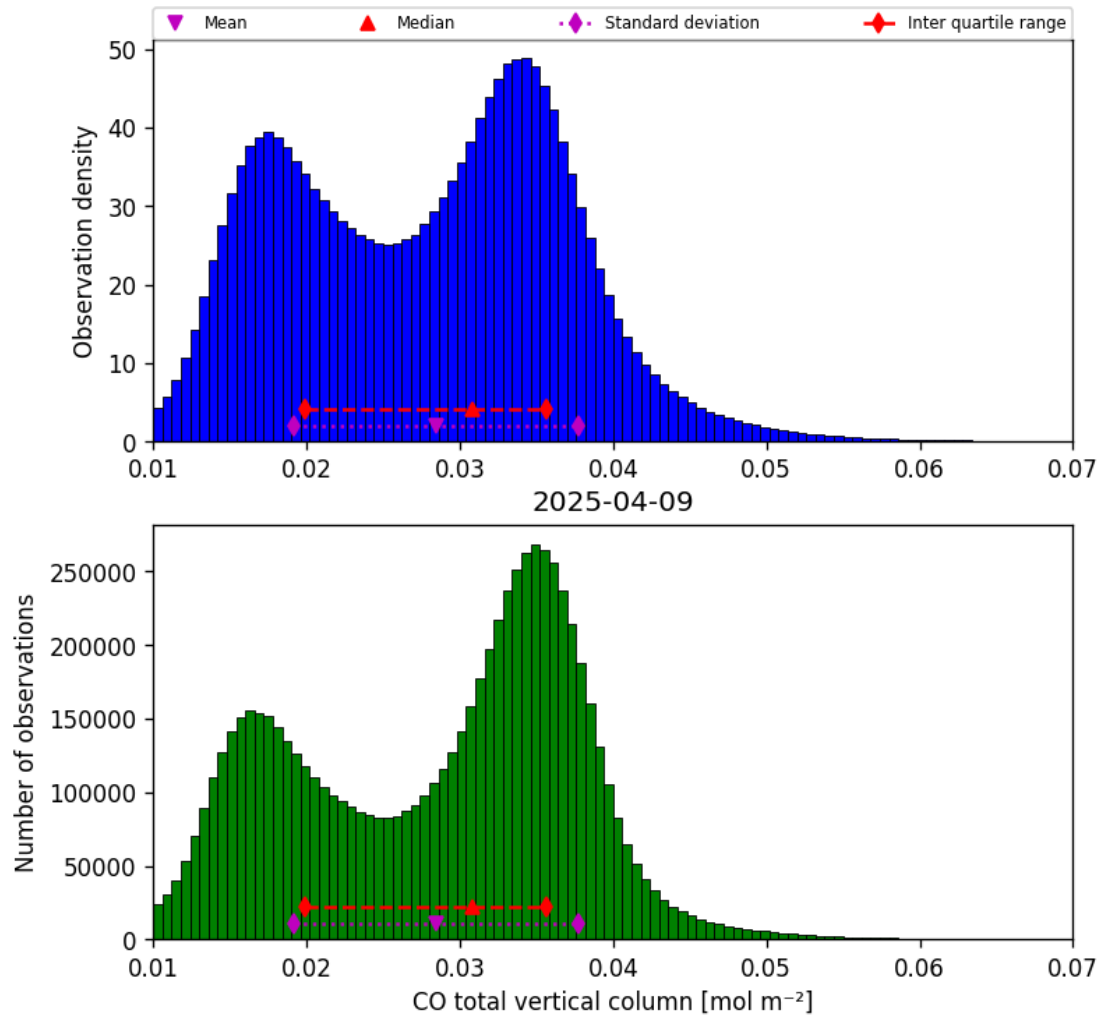
Figure 14: Histogram of “CO total vertical column” for 2025-04-09 to 2025-04-10
