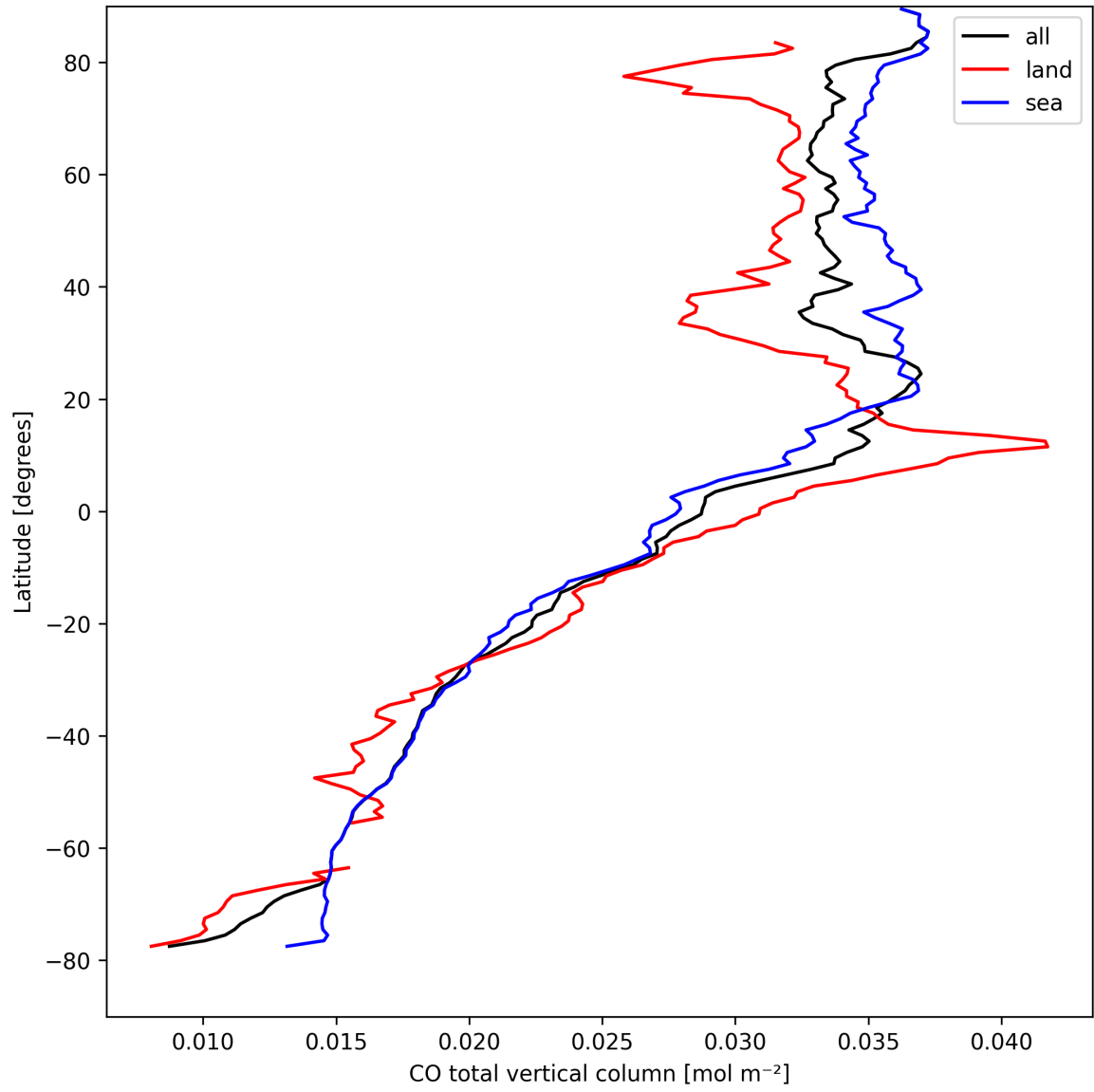
Figure 7: Zonal average of “CO total vertical column” for 2025-04-09 to 2025-04-10.
