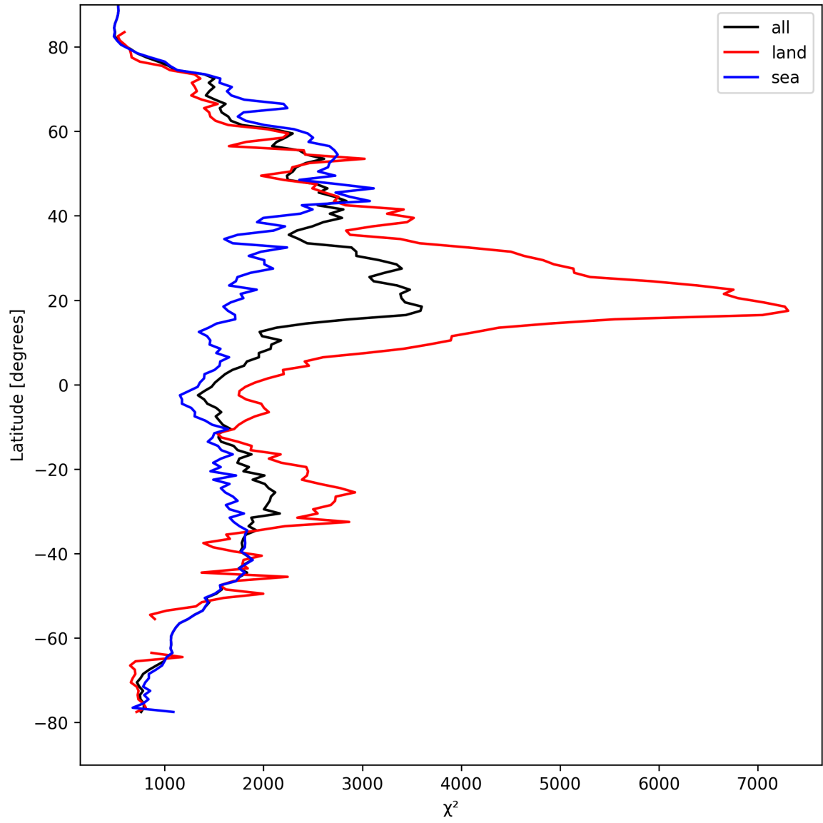
Figure 10: Zonal average of “ \chi^2 ” for 2025-04-09 to 2025-04-10.
