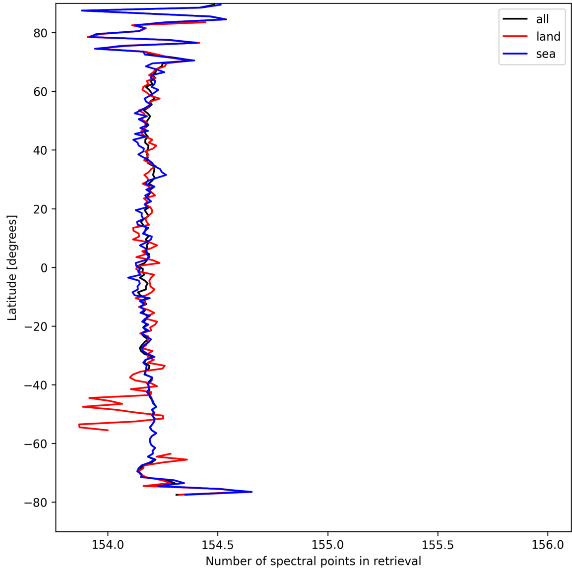
Figure 9: Zonal average of “Number of spectral points in retrieval” for 2025-04-09 to 2025-04-10.
