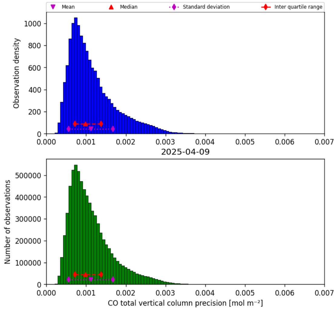
Figure 15: Histogram of “CO total vertical column precision” for 2025-04-09 to 2025-04-10
