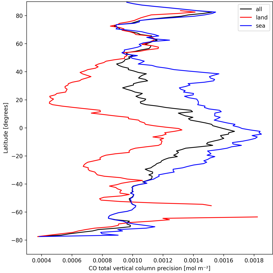
Figure 8: Zonal average of “CO total vertical column precision” for 2025-04-09 to 2025-04-10.
