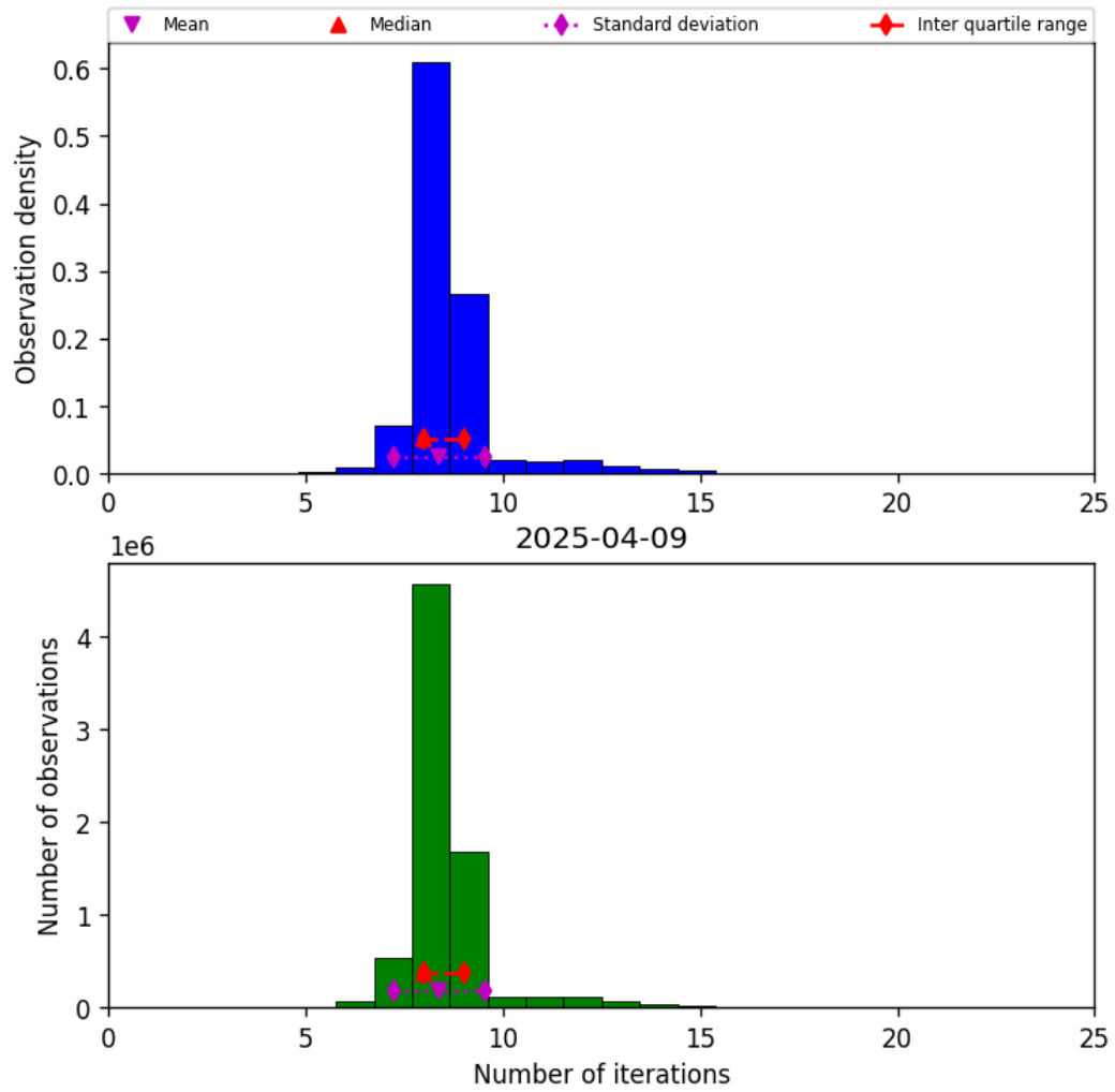
Figure 19: Histogram of “Number of iterations” for 2025-04-09 to 2025-04-10
