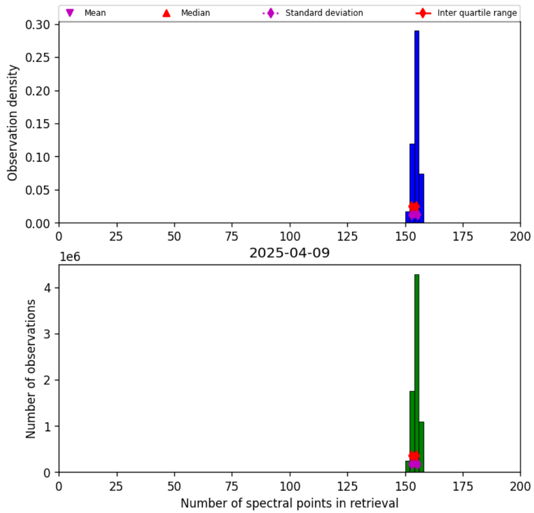
Figure 16: Histogram of “Number of spectral points in retrieval” for 2025-04-09 to 2025-04-10
