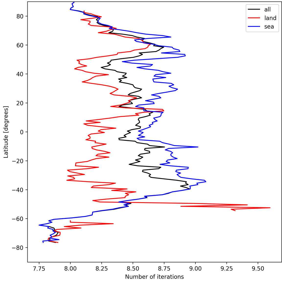
Figure 12: Zonal average of “Number of iterations” for 2025-04-11 to 2025-04-11.
