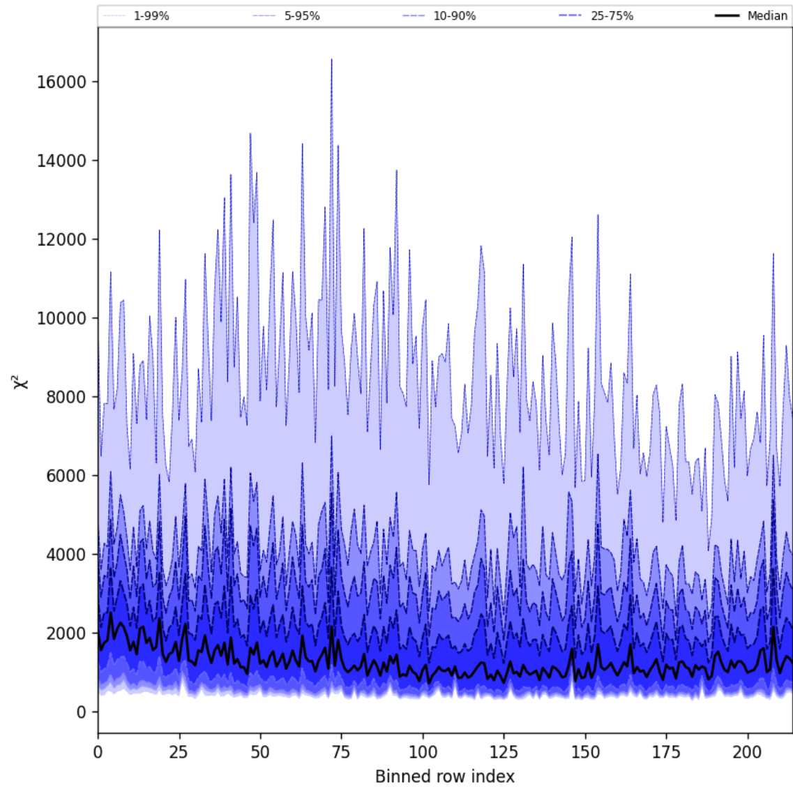
Figure 24: Along track statistics of “ \chi^2 ” for 2025-04-11 to 2025-04-11
