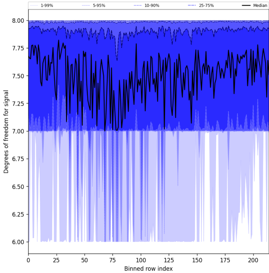
Figure 25: Along track statistics of “Degrees of freedom for signal” for 2025-04-11 to 2025-04-11
