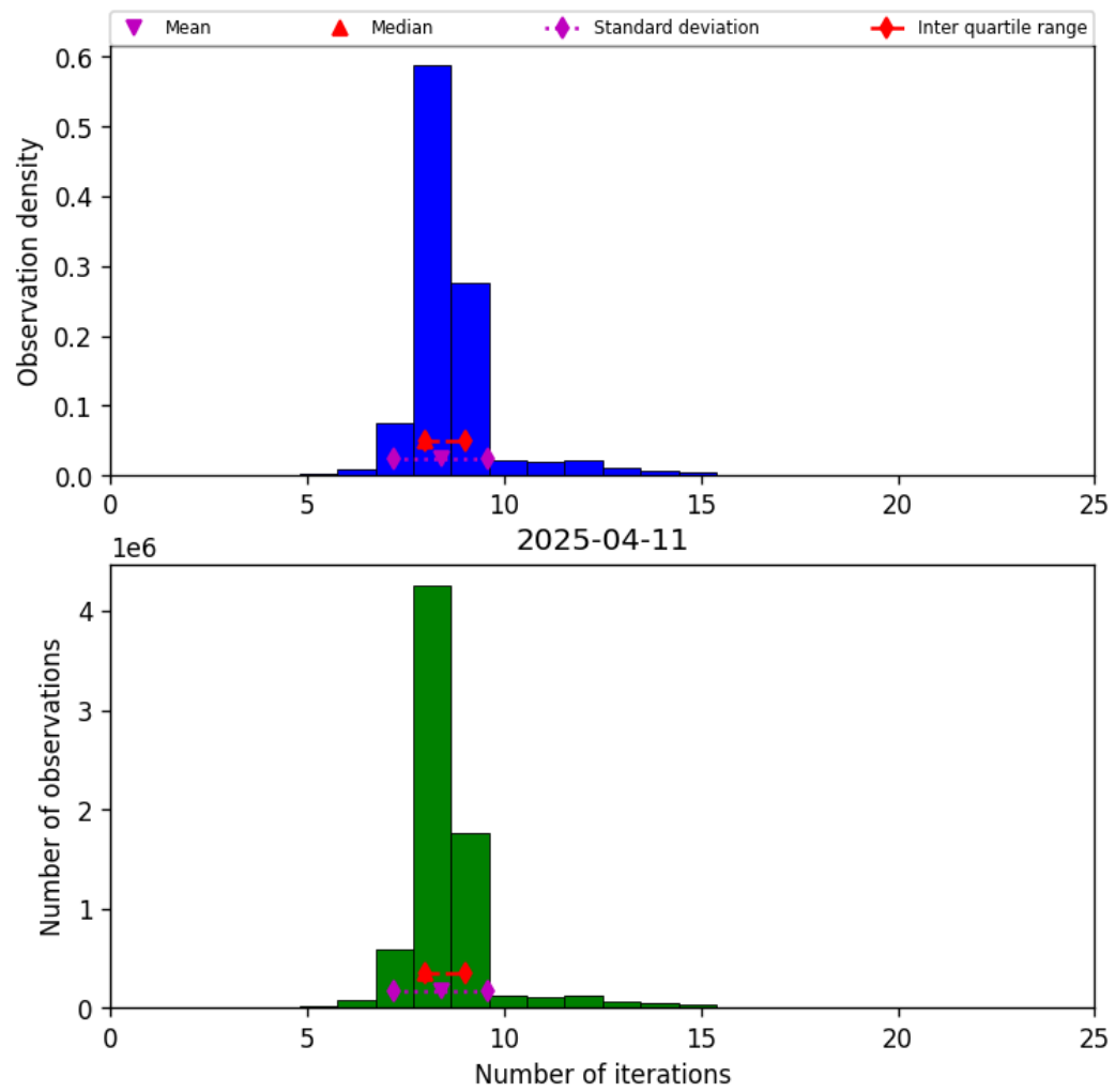
Figure 19: Histogram of “Number of iterations” for 2025-04-11 to 2025-04-11
