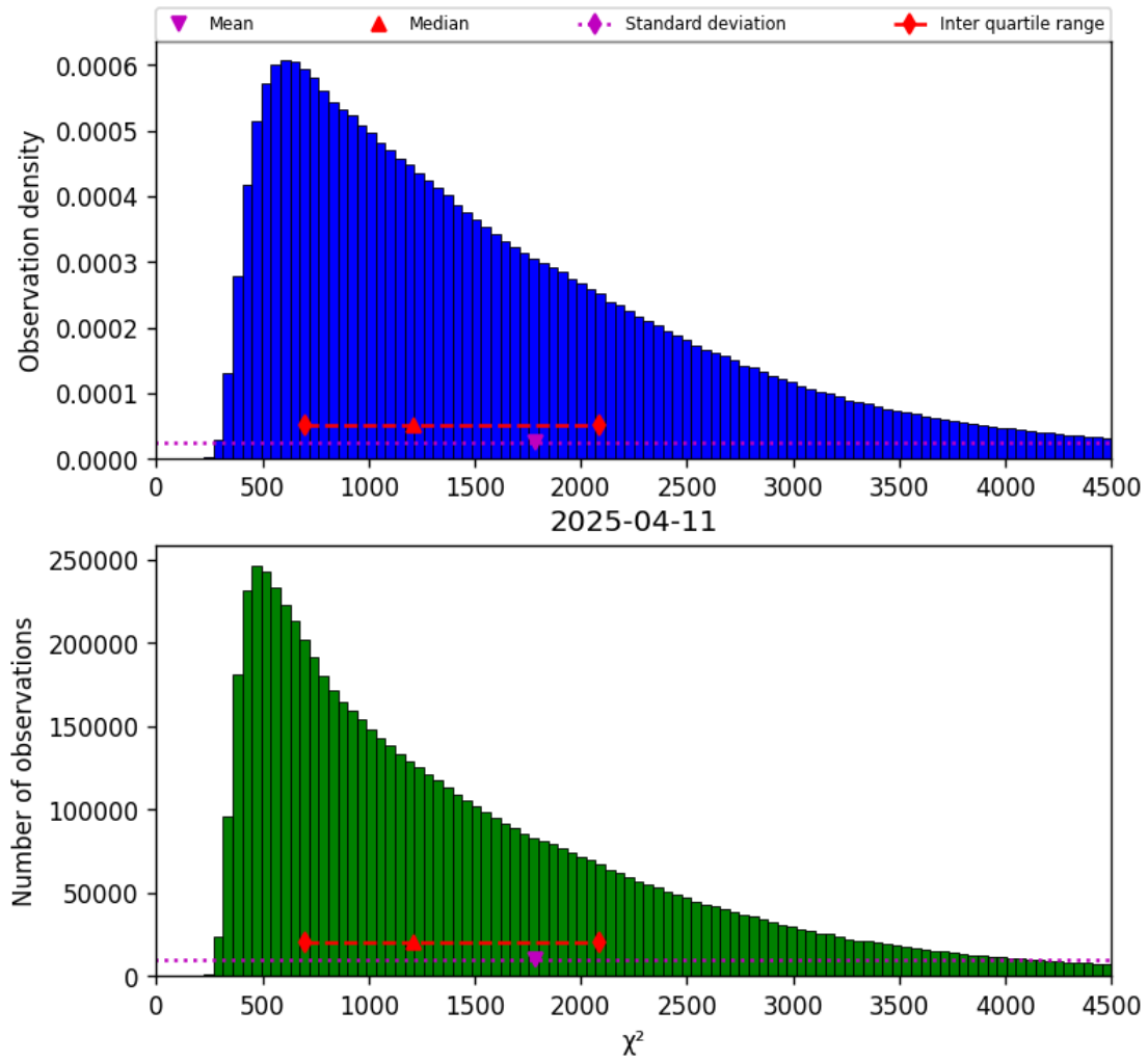
Figure 17: Histogram of " \chi^2 " for 2025-04-11 to 2025-04-11
