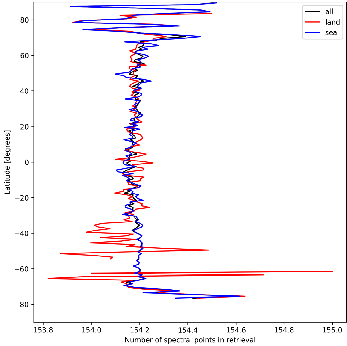
Figure 9: Zonal average of “Number of spectral points in retrieval” for 2025-04-11 to 2025-04-11.
