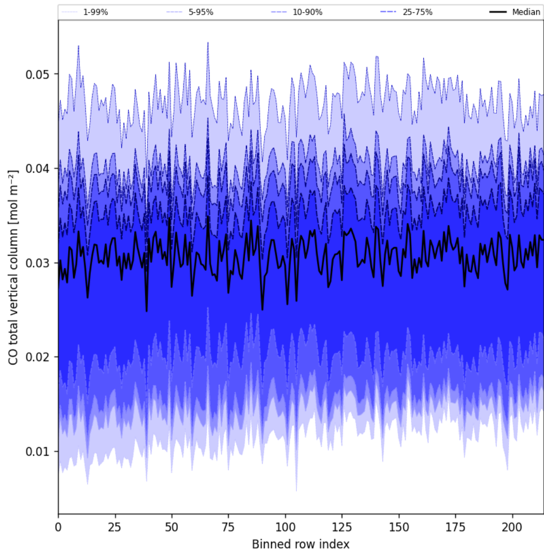
Figure 21: Along track statistics of “CO total vertical column” for 2025-04-11 to 2025-04-11
