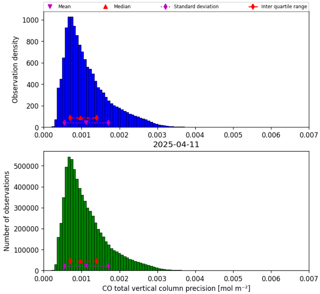
Figure 15: Histogram of “CO total vertical column precision” for 2025-04-11 to 2025-04-11
