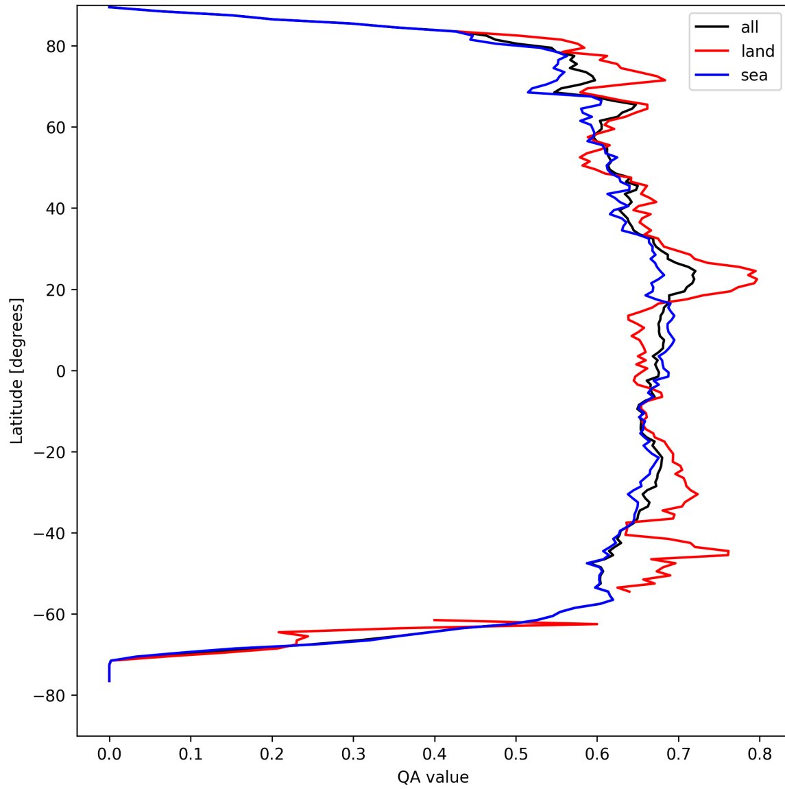
Figure 6: Zonal average of “QA value” for 2025-04-11 to 2025-04-11.
