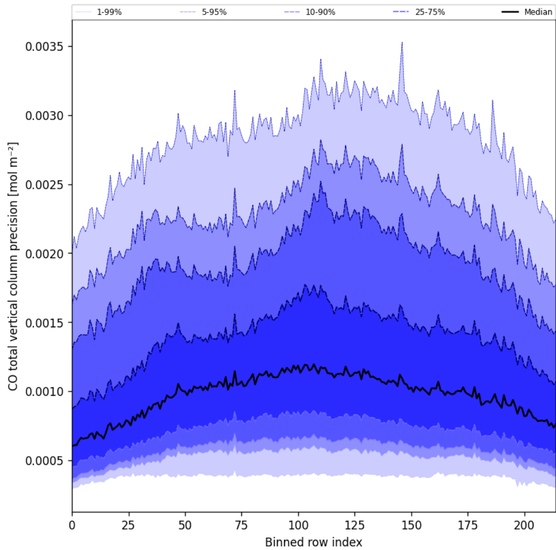
Figure 22: Along track statistics of “CO total vertical column precision” for 2025-04-11 to 2025-04-11
