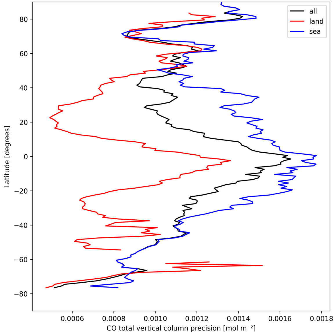
Figure 8: Zonal average of “CO total vertical column precision” for 2025-04-11 to 2025-04-11.
