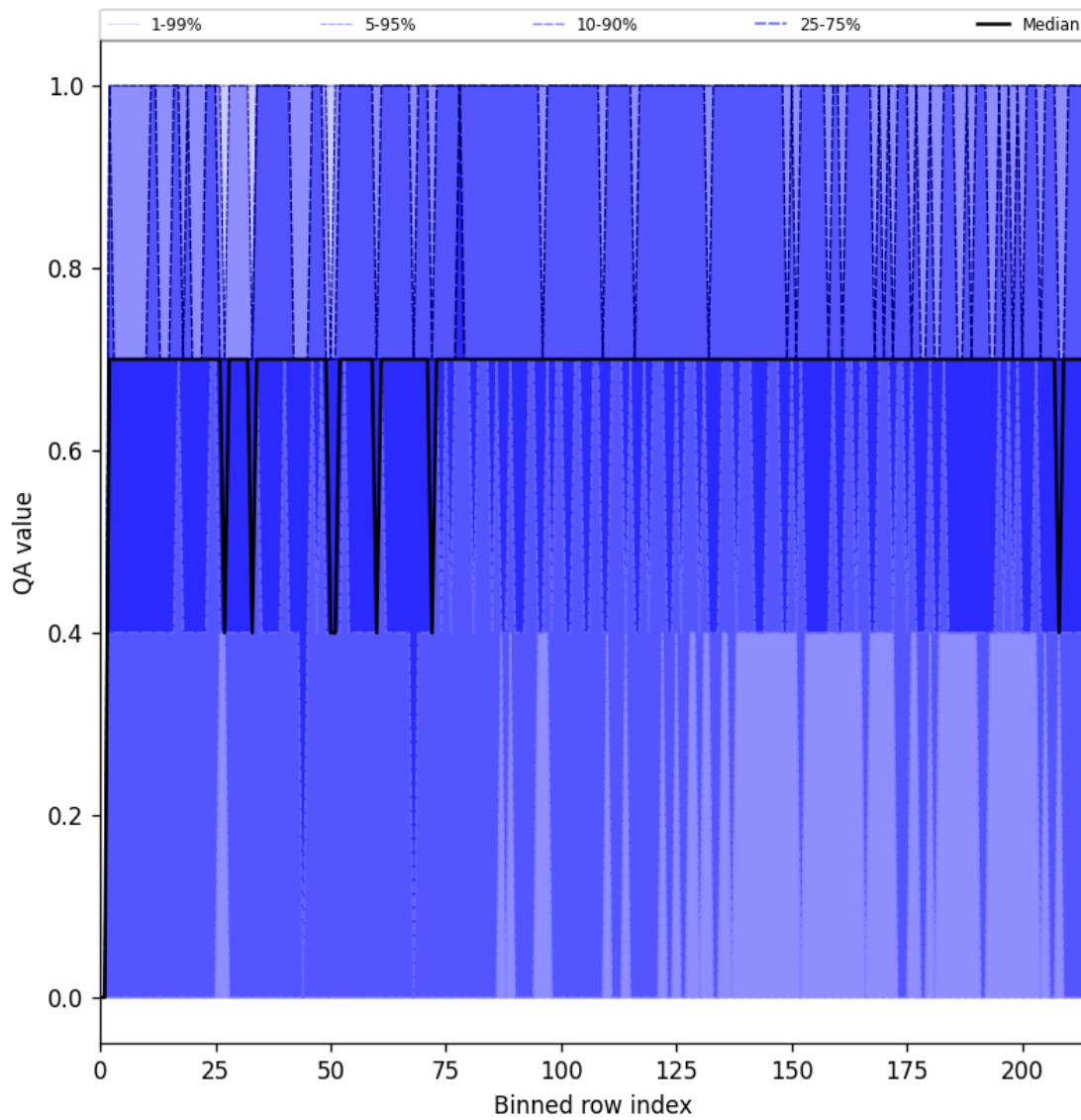
Figure 20: Along track statistics of “QA value” for 2025-04-11 to 2025-04-11
