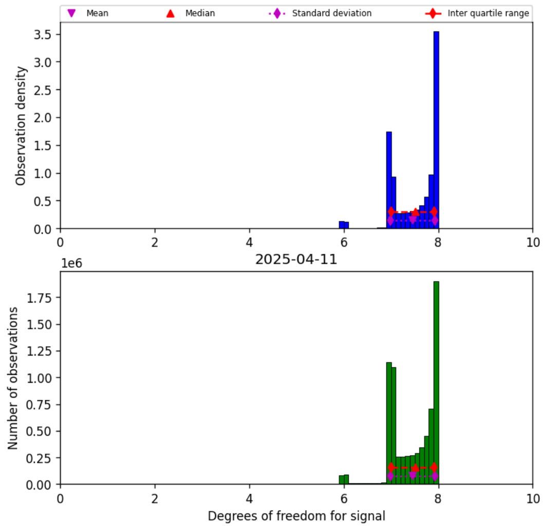
Figure 18: Histogram of “Degrees of freedom for signal” for 2025-04-11 to 2025-04-11
