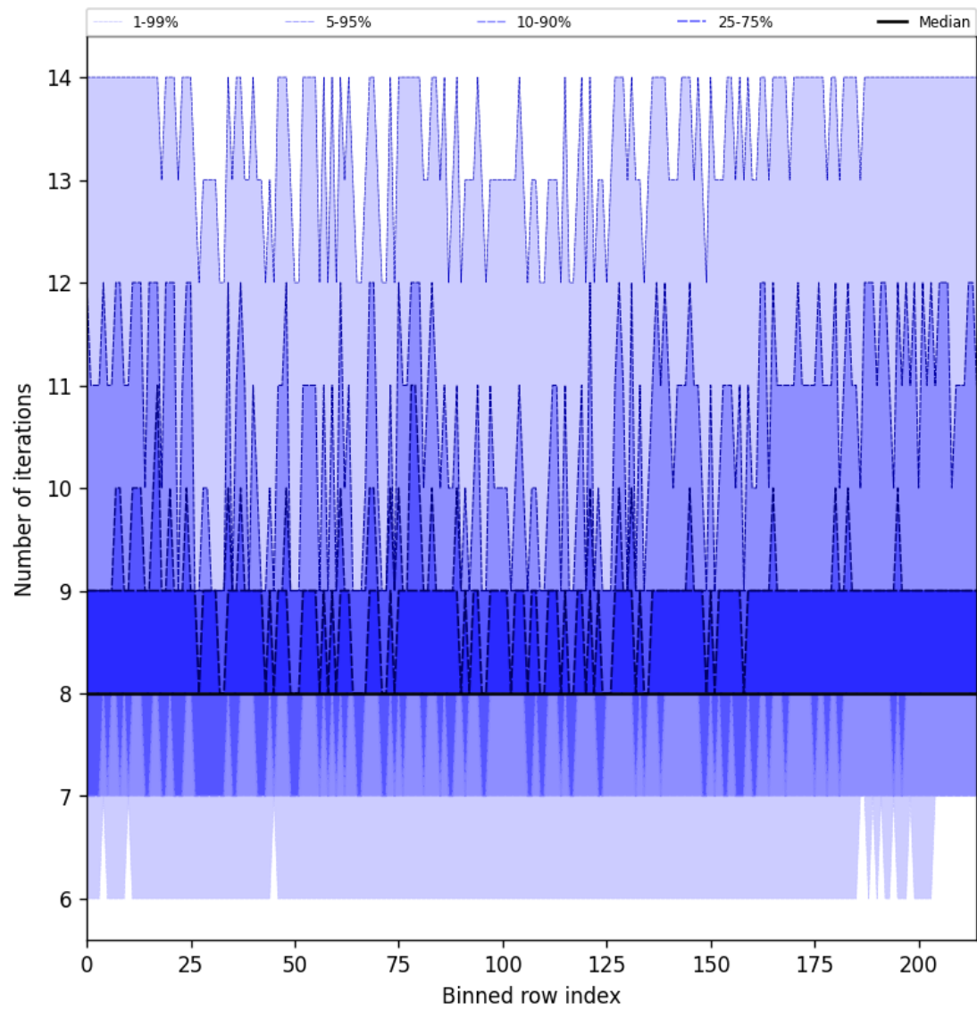
Figure 26: Along track statistics of “Number of iterations” for 2025-04-11 to 2025-04-11
