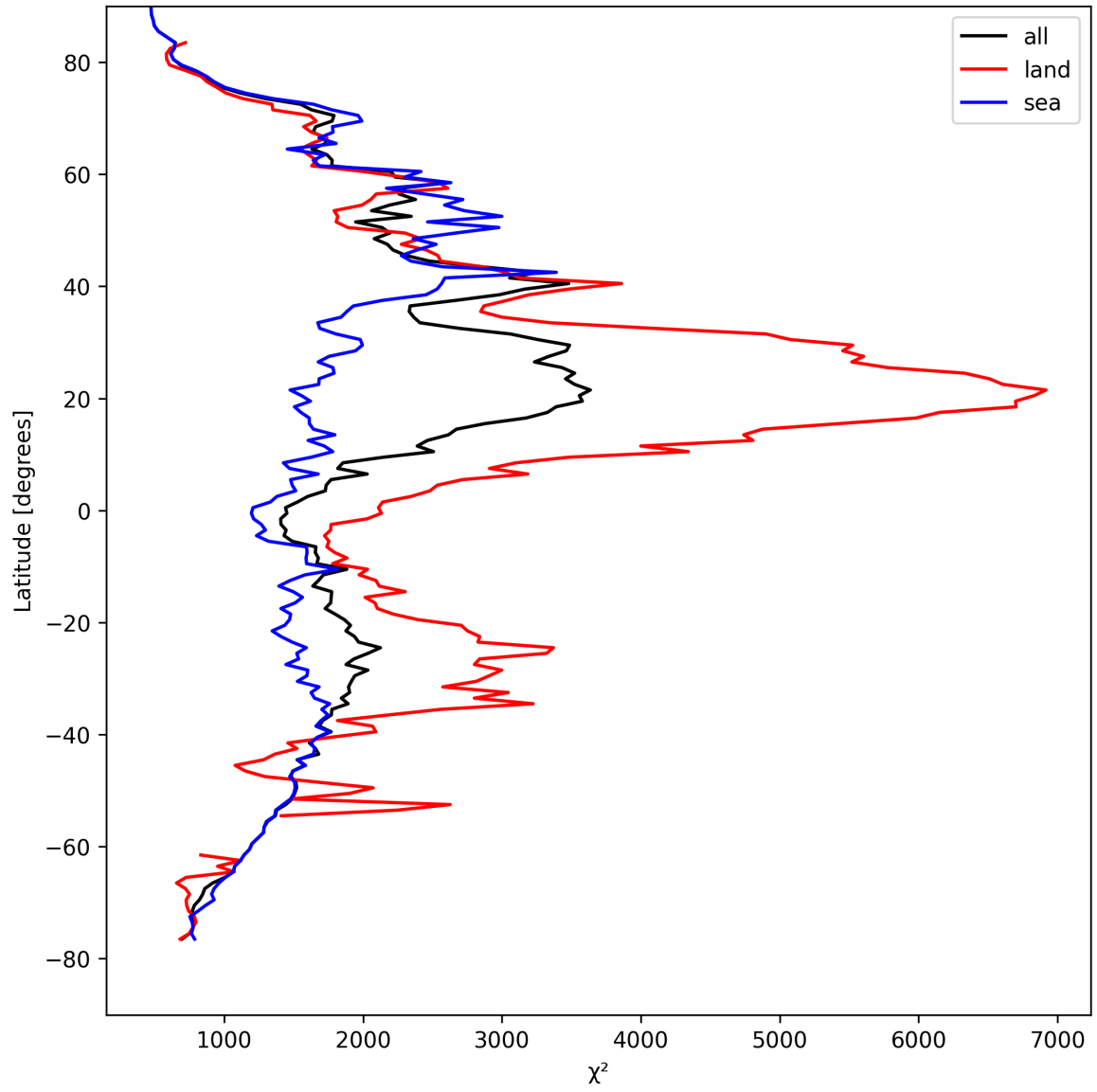
Figure 10: Zonal average of “ \chi^2 ” for 2025-04-11 to 2025-04-11.
