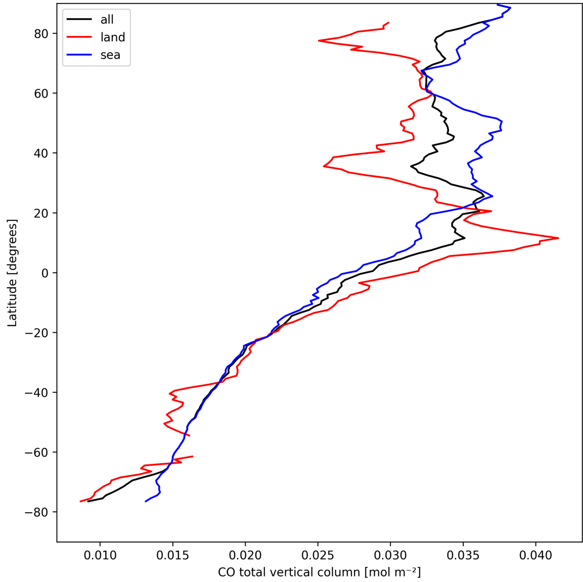
Figure 7: Zonal average of “CO total vertical column” for 2025-04-11 to 2025-04-11.
