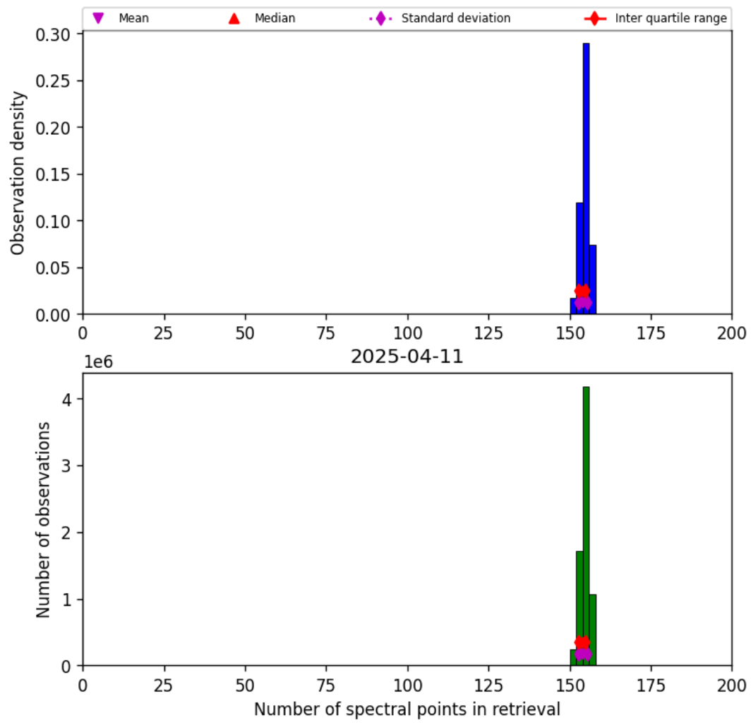
Figure 16: Histogram of “Number of spectral points in retrieval” for 2025-04-11 to 2025-04-11
