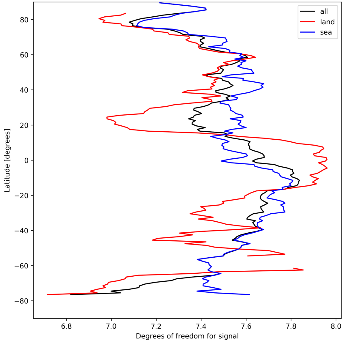
Figure 11: Zonal average of “Degrees of freedom for signal” for 2025-04-11 to 2025-04-11.
