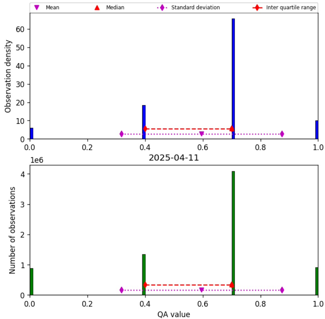
Figure 13: Histogram of “QA value” for 2025-04-11 to 2025-04-11
