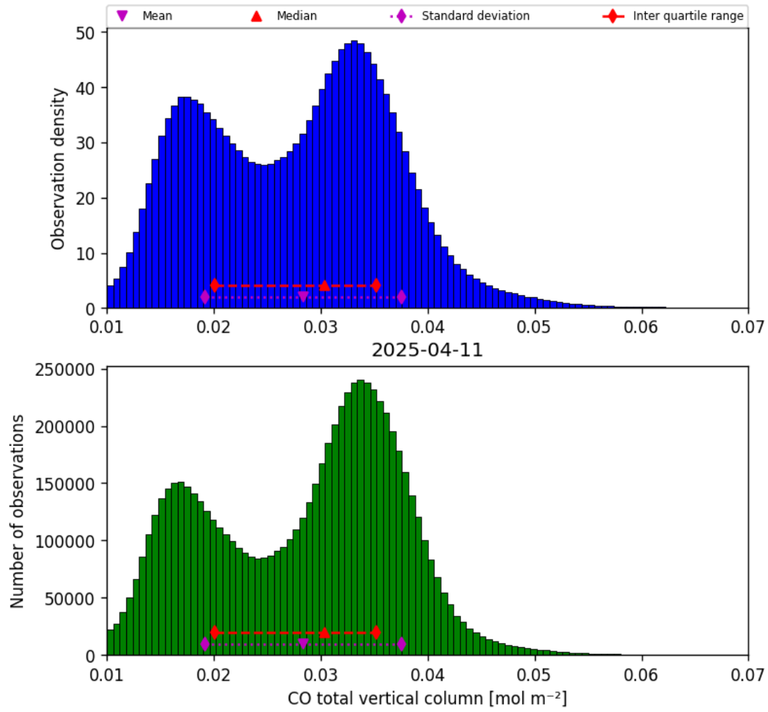
Figure 14: Histogram of “CO total vertical column” for 2025-04-11 to 2025-04-11
