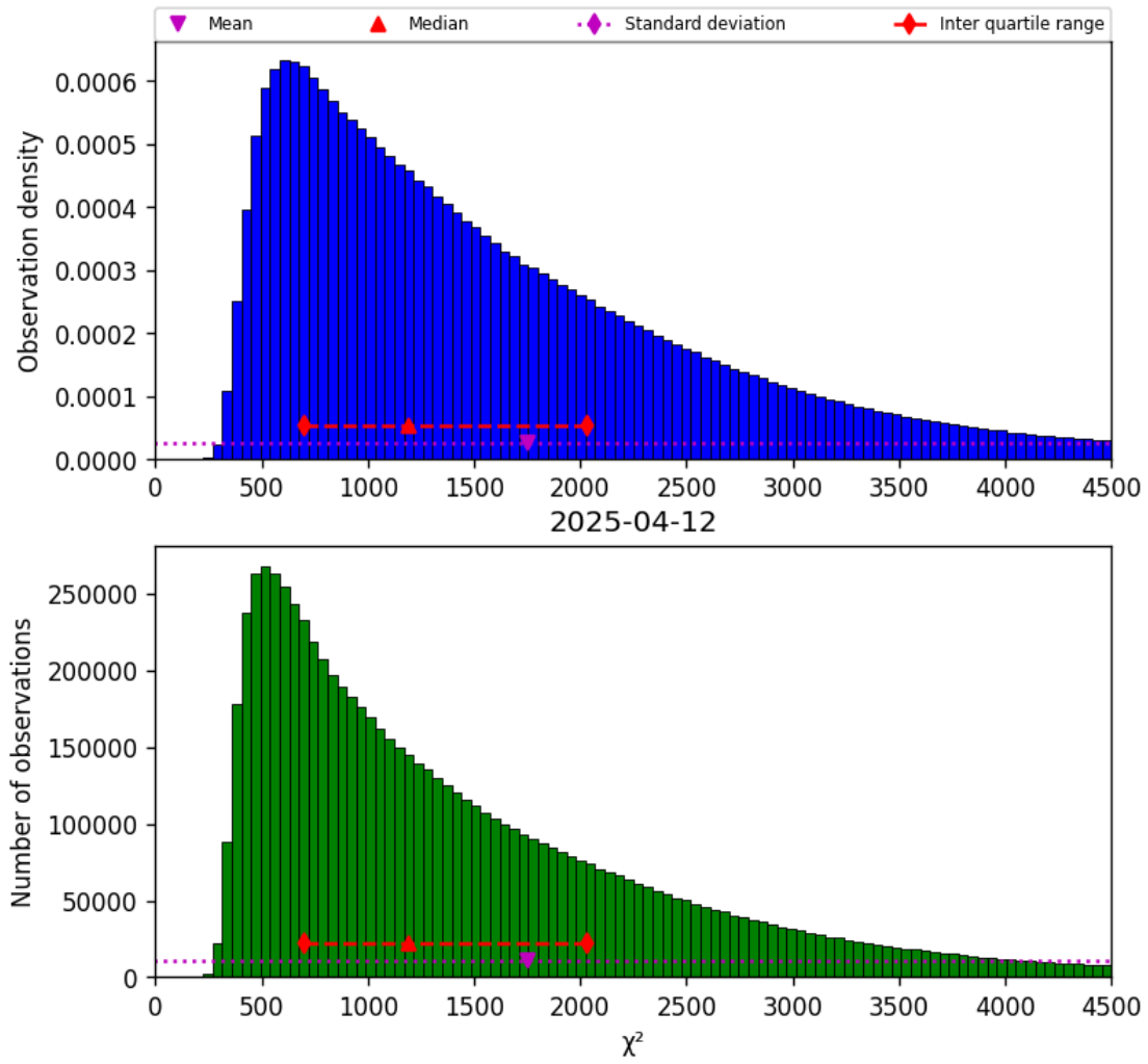
Figure 17: Histogram of “ \chi^2 ” for 2025-04-12 to 2025-04-13
