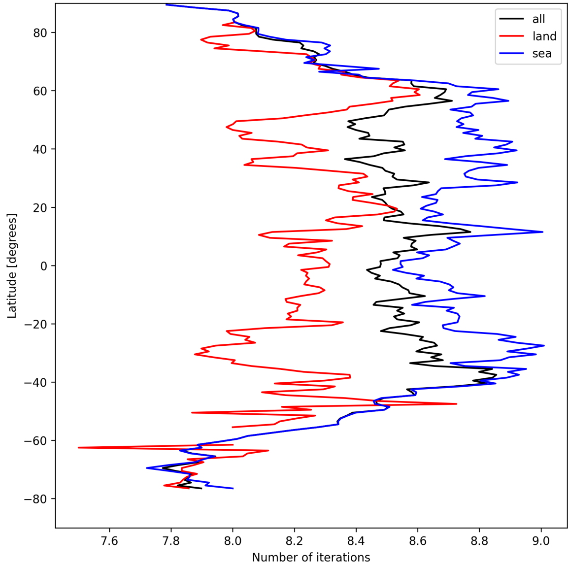
Figure 12: Zonal average of “Number of iterations” for 2025-04-12 to 2025-04-13.
