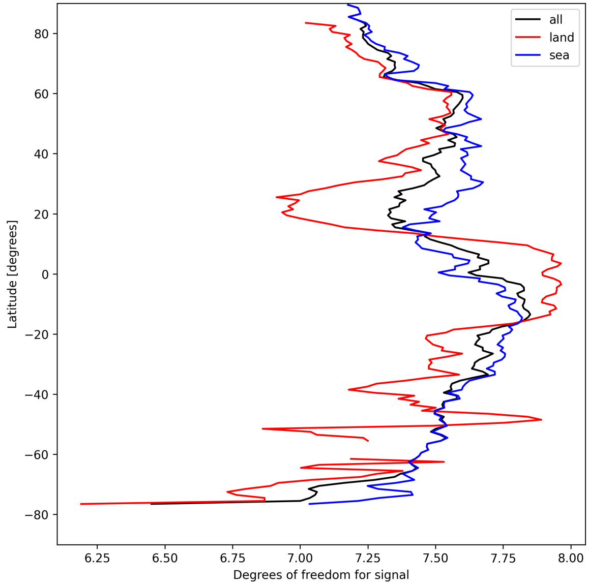
Figure 11: Zonal average of “Degrees of freedom for signal” for 2025-04-12 to 2025-04-13.
