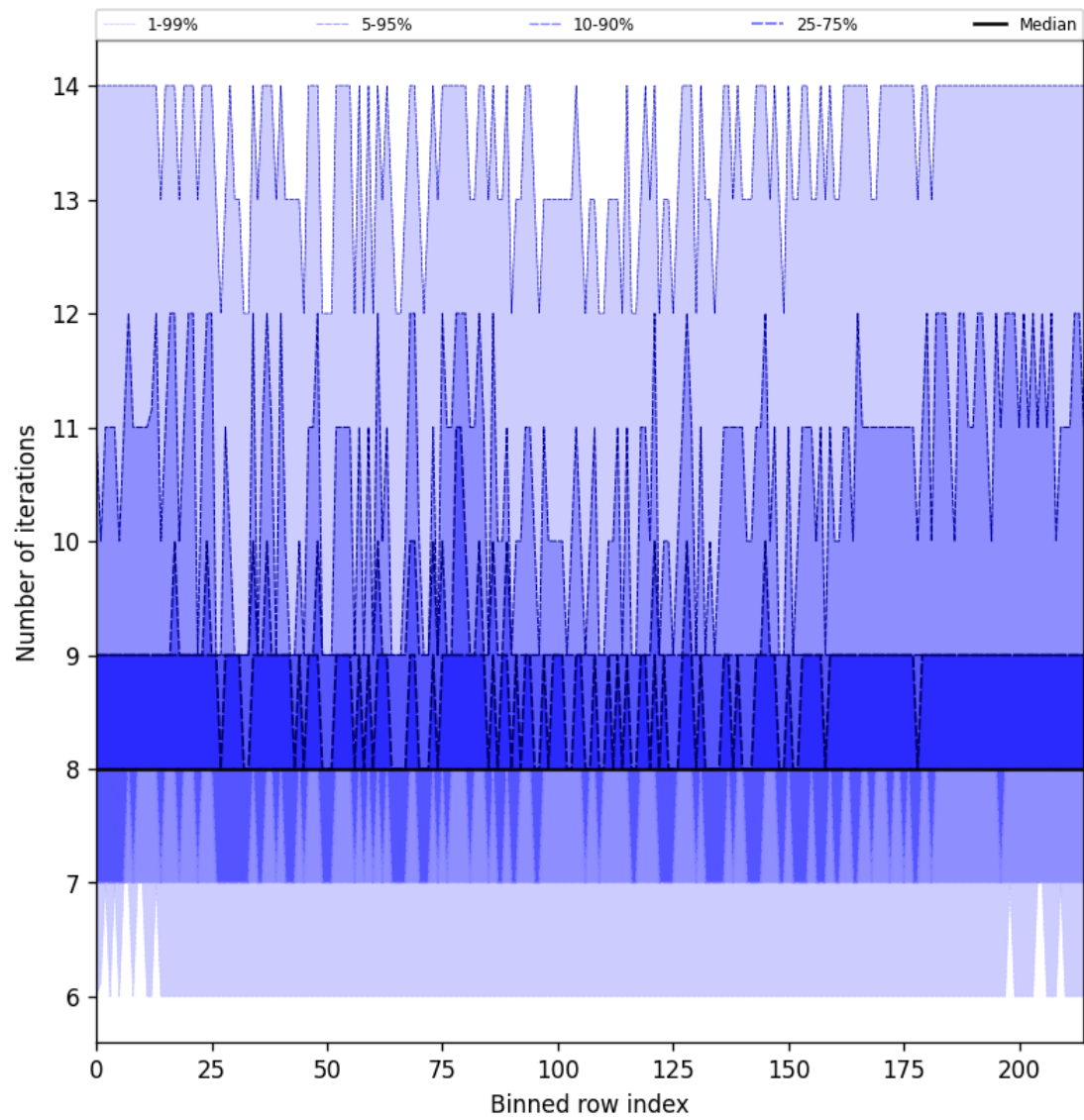
Figure 26: Along track statistics of “Number of iterations” for 2025-04-12 to 2025-04-13
