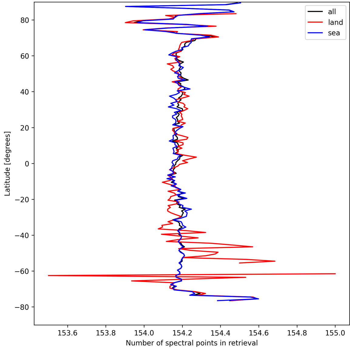
Figure 9: Zonal average of “Number of spectral points in retrieval” for 2025-04-12 to 2025-04-13.
