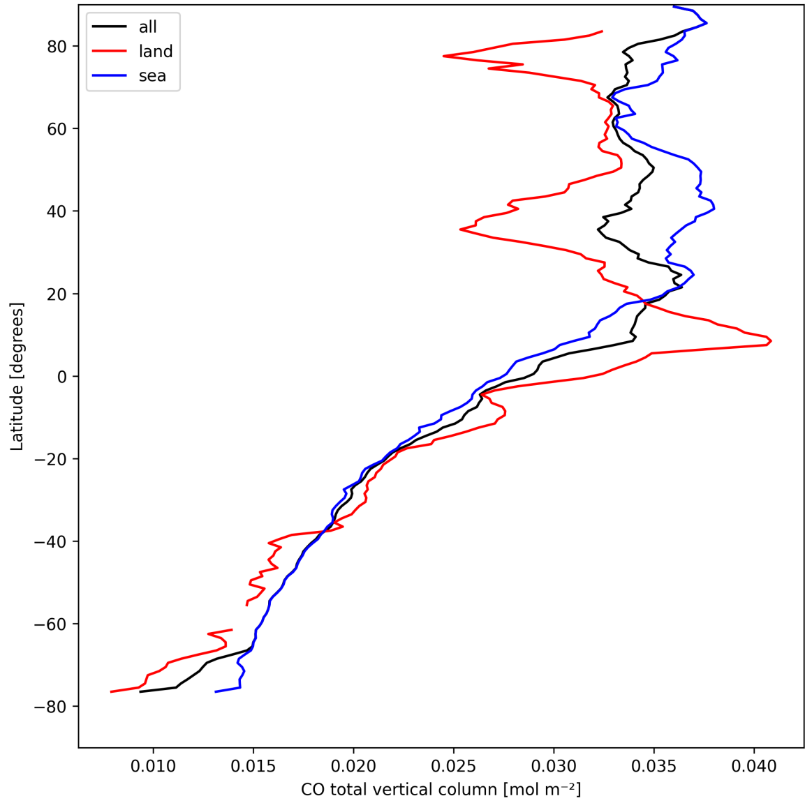
Figure 7: Zonal average of “CO total vertical column” for 2025-04-12 to 2025-04-13.
