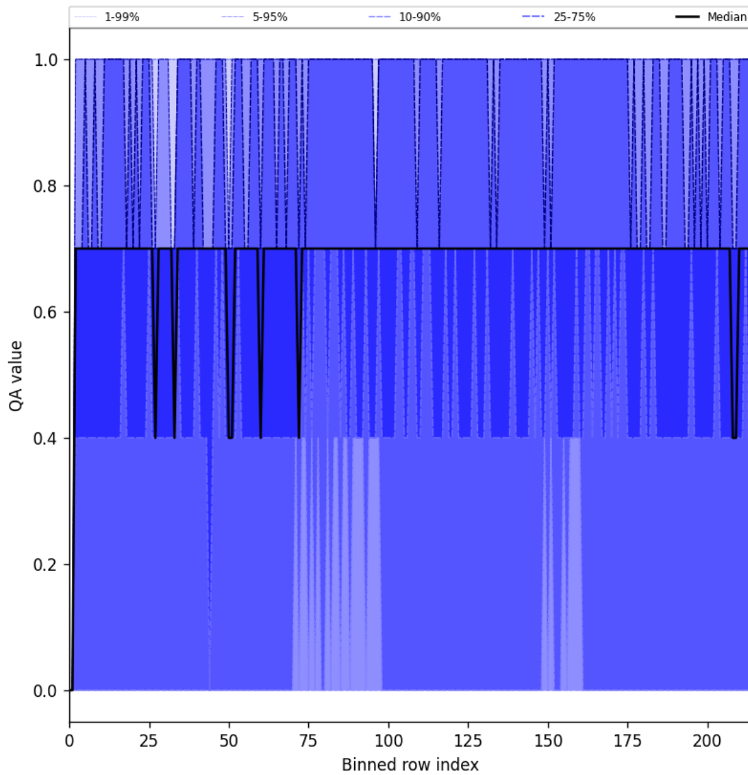
Figure 20: Along track statistics of “QA value” for 2025-04-12 to 2025-04-13
