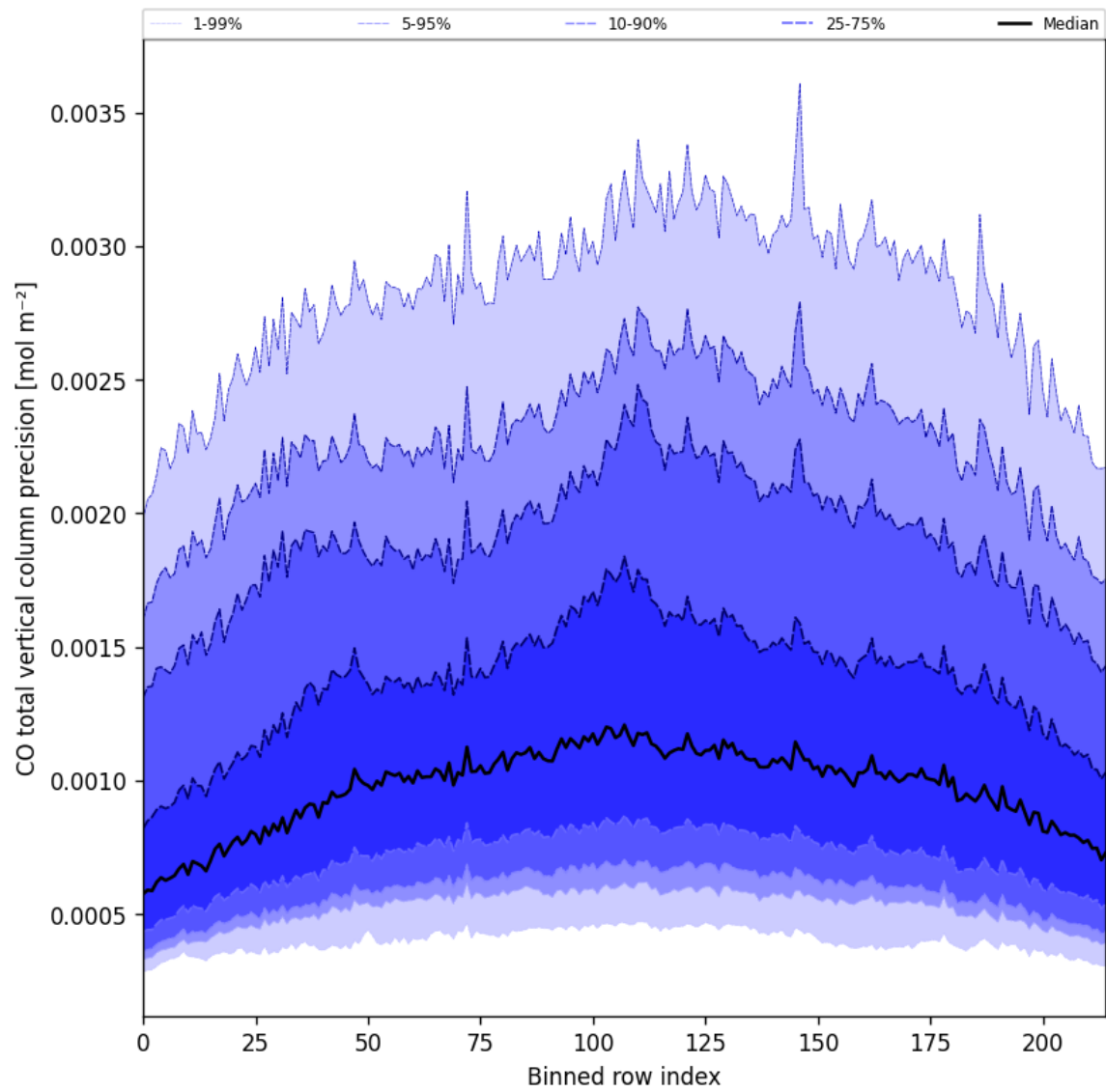
Figure 22: Along track statistics of “CO total vertical column precision” for 2025-04-12 to 2025-04-13
