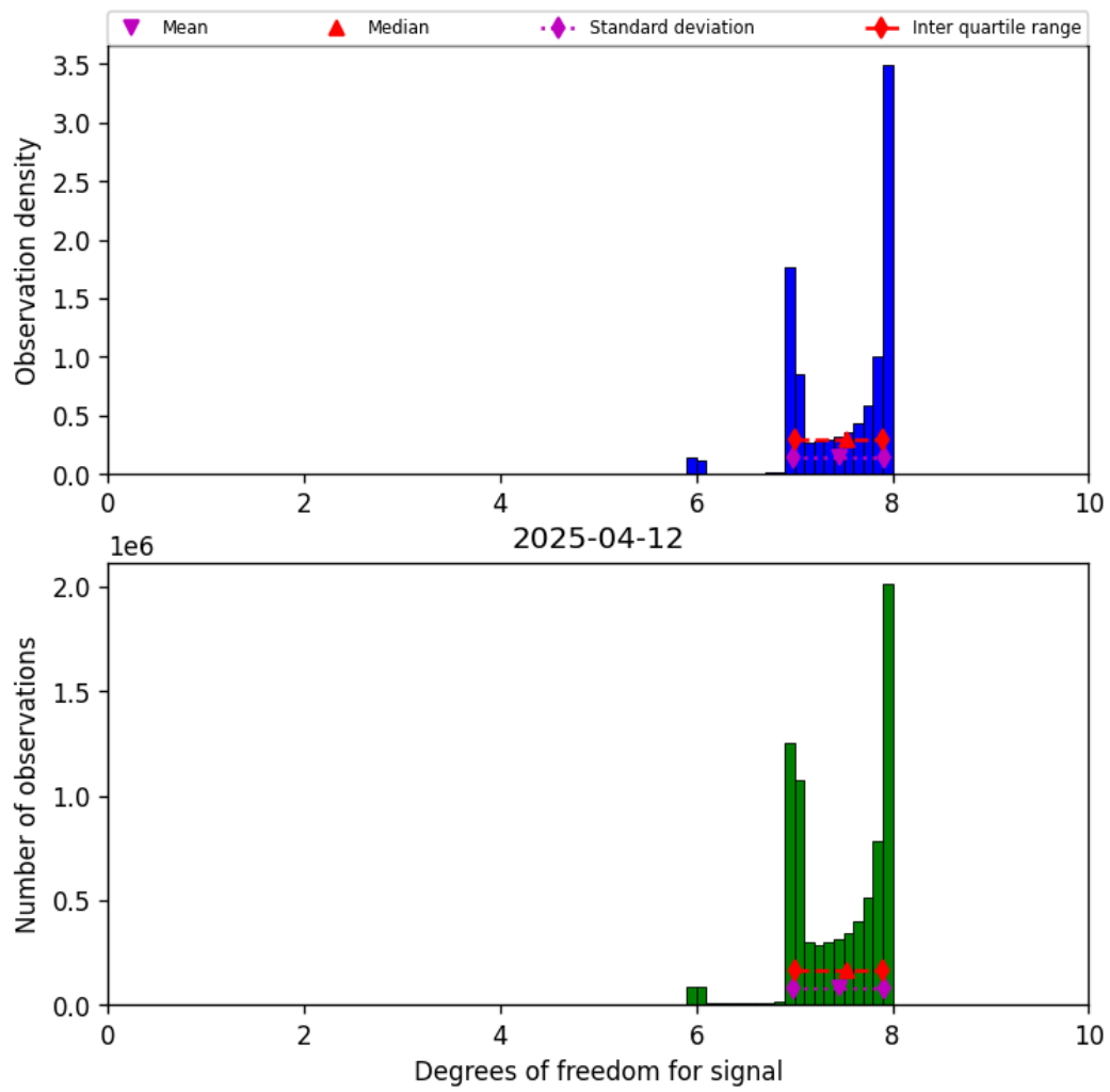
Figure 18: Histogram of “Degrees of freedom for signal” for 2025-04-12 to 2025-04-13
