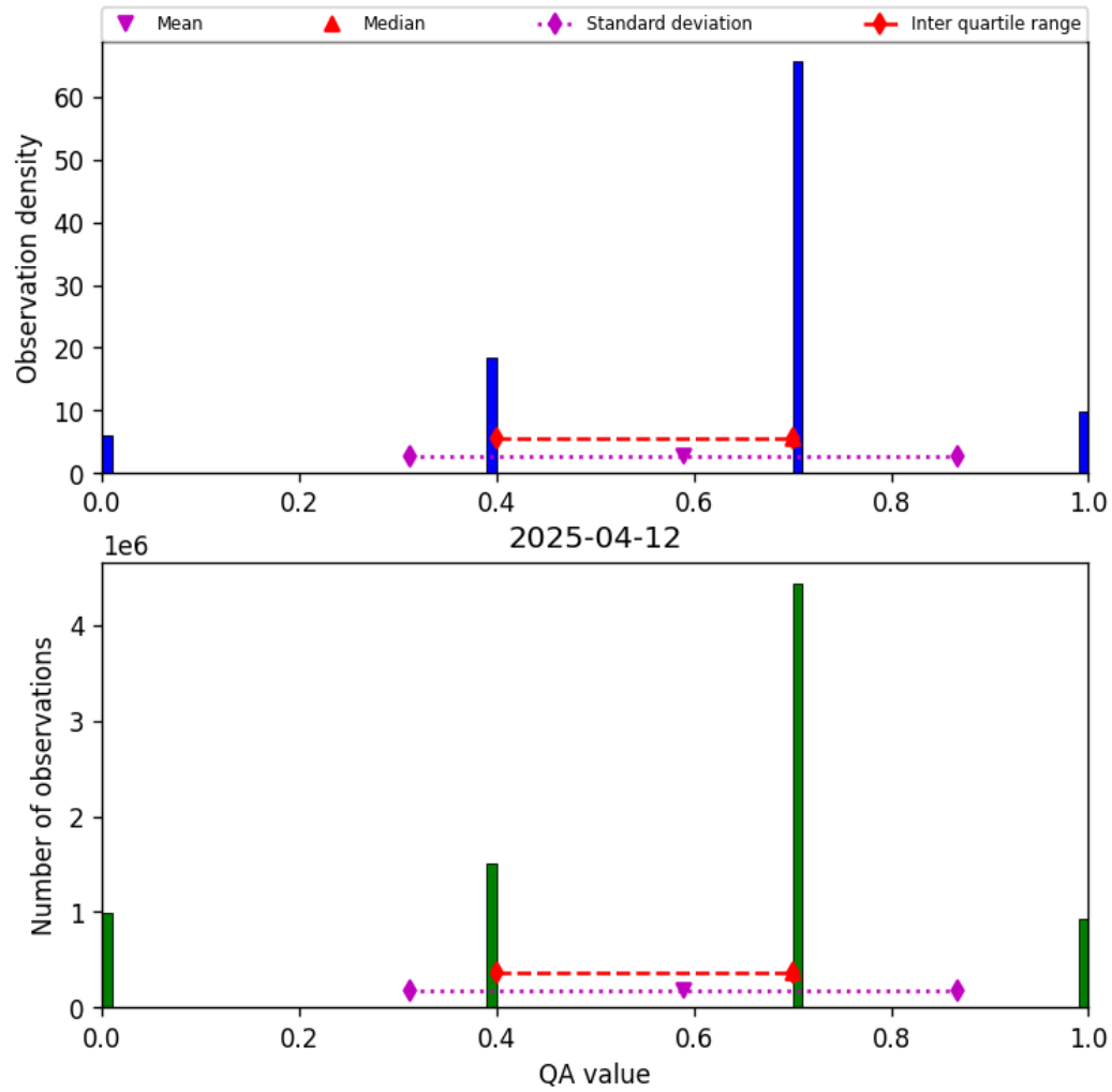
Figure 13: Histogram of “QA value” for 2025-04-12 to 2025-04-13
