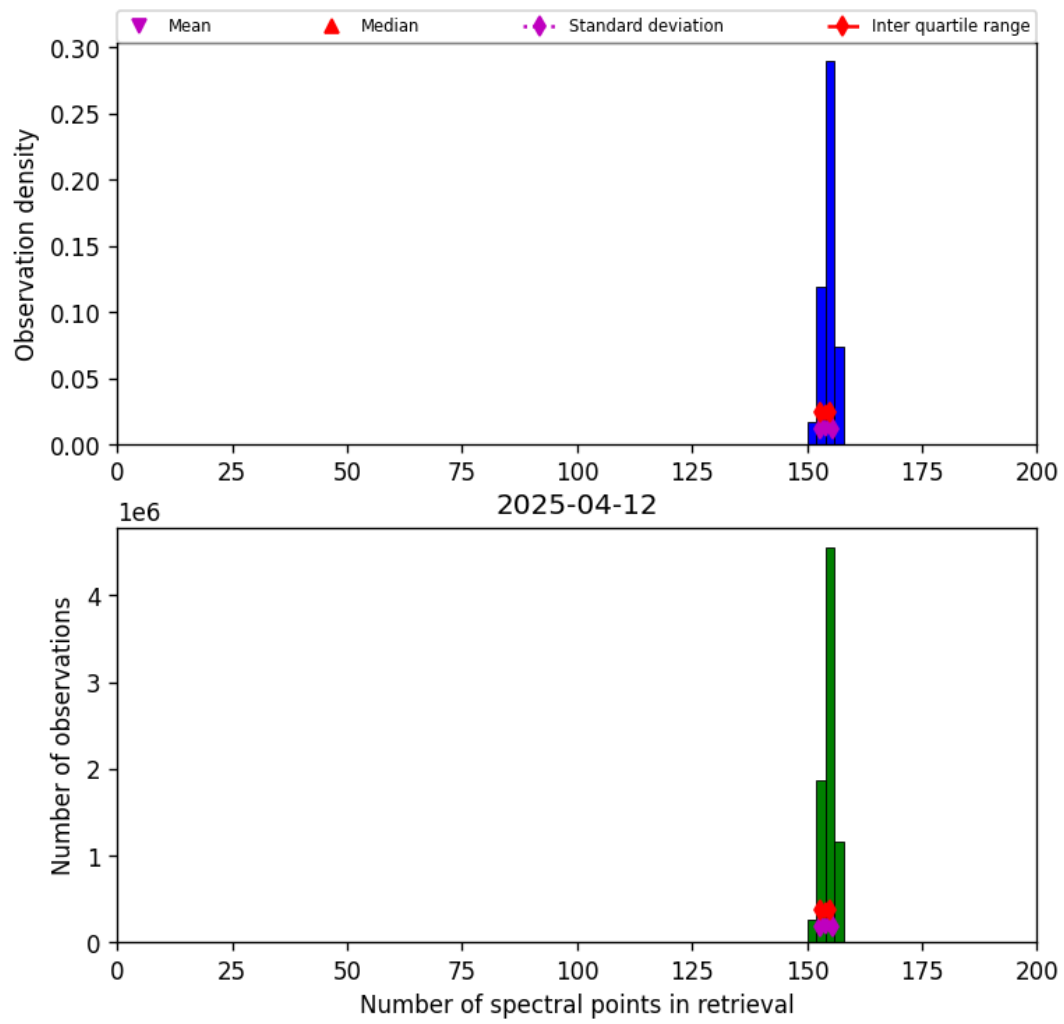
Figure 16: Histogram of “Number of spectral points in retrieval” for 2025-04-12 to 2025-04-13
