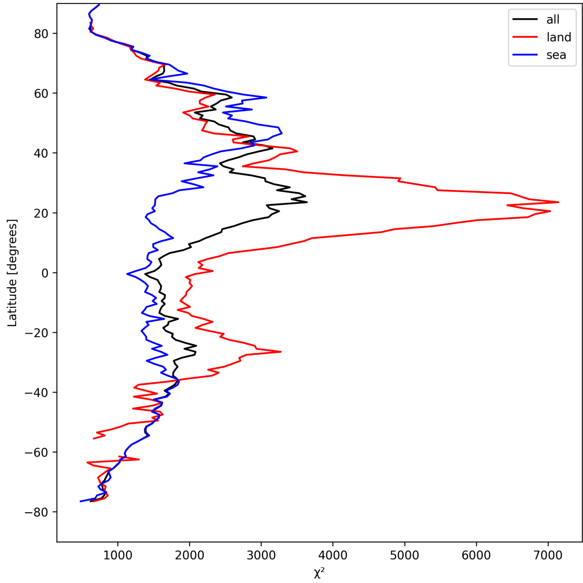
Figure 10: Zonal average of “ \chi^2 ” for 2025-04-12 to 2025-04-13.
