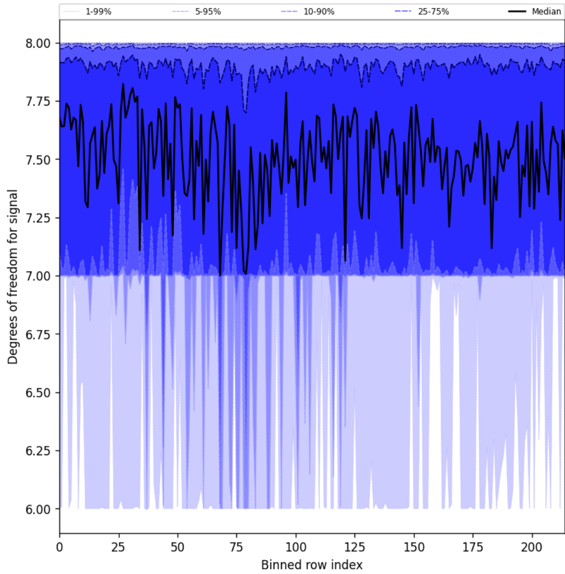
Figure 25: Along track statistics of “Degrees of freedom for signal” for 2025-04-12 to 2025-04-13
