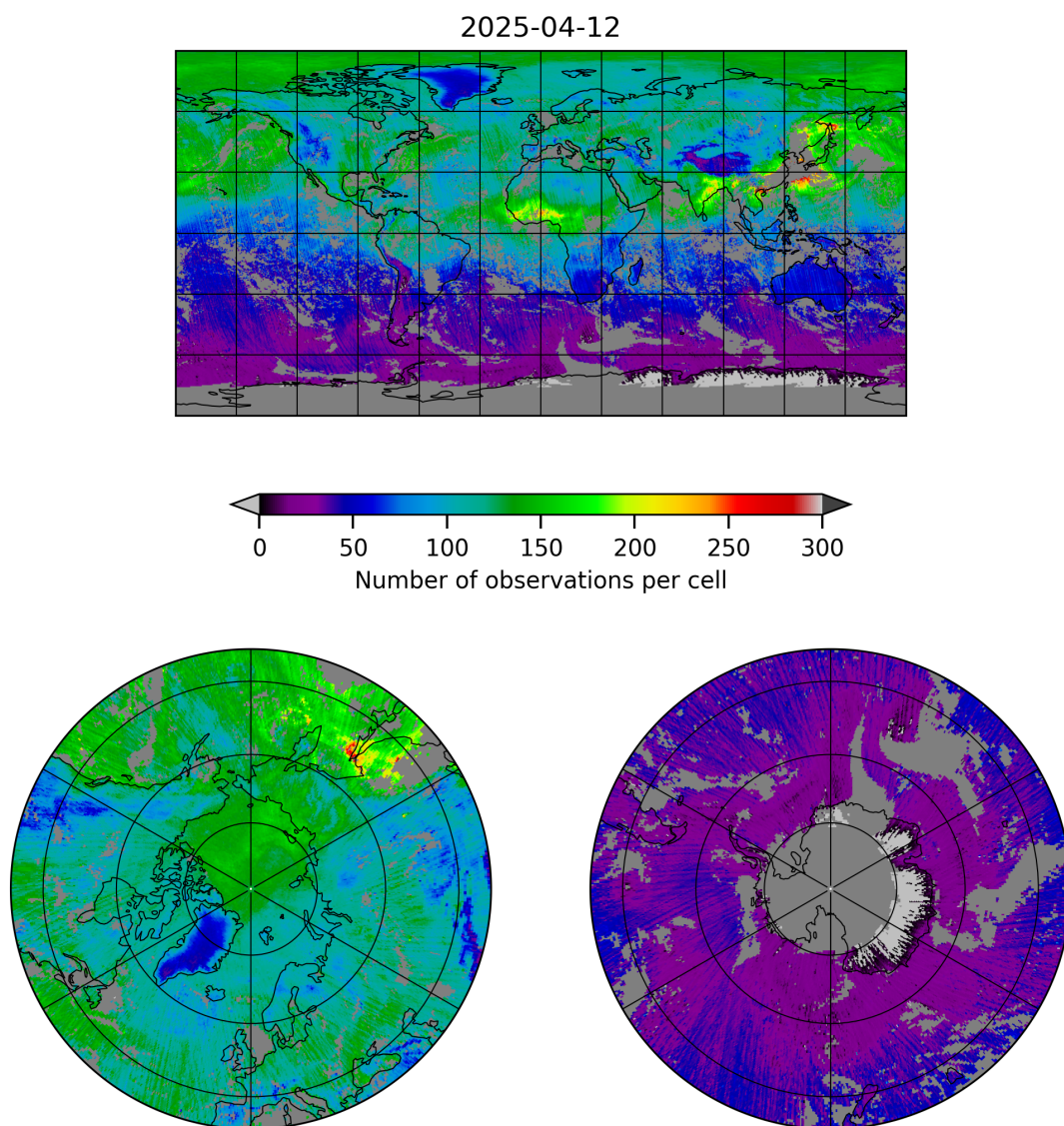
Figure 5: Map of the number of observations for 2025-04-12 to 2025-04-13
