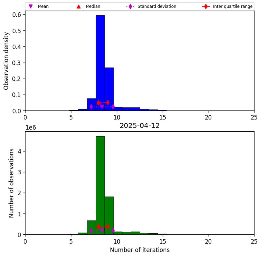
Figure 19: Histogram of “Number of iterations” for 2025-04-12 to 2025-04-13
