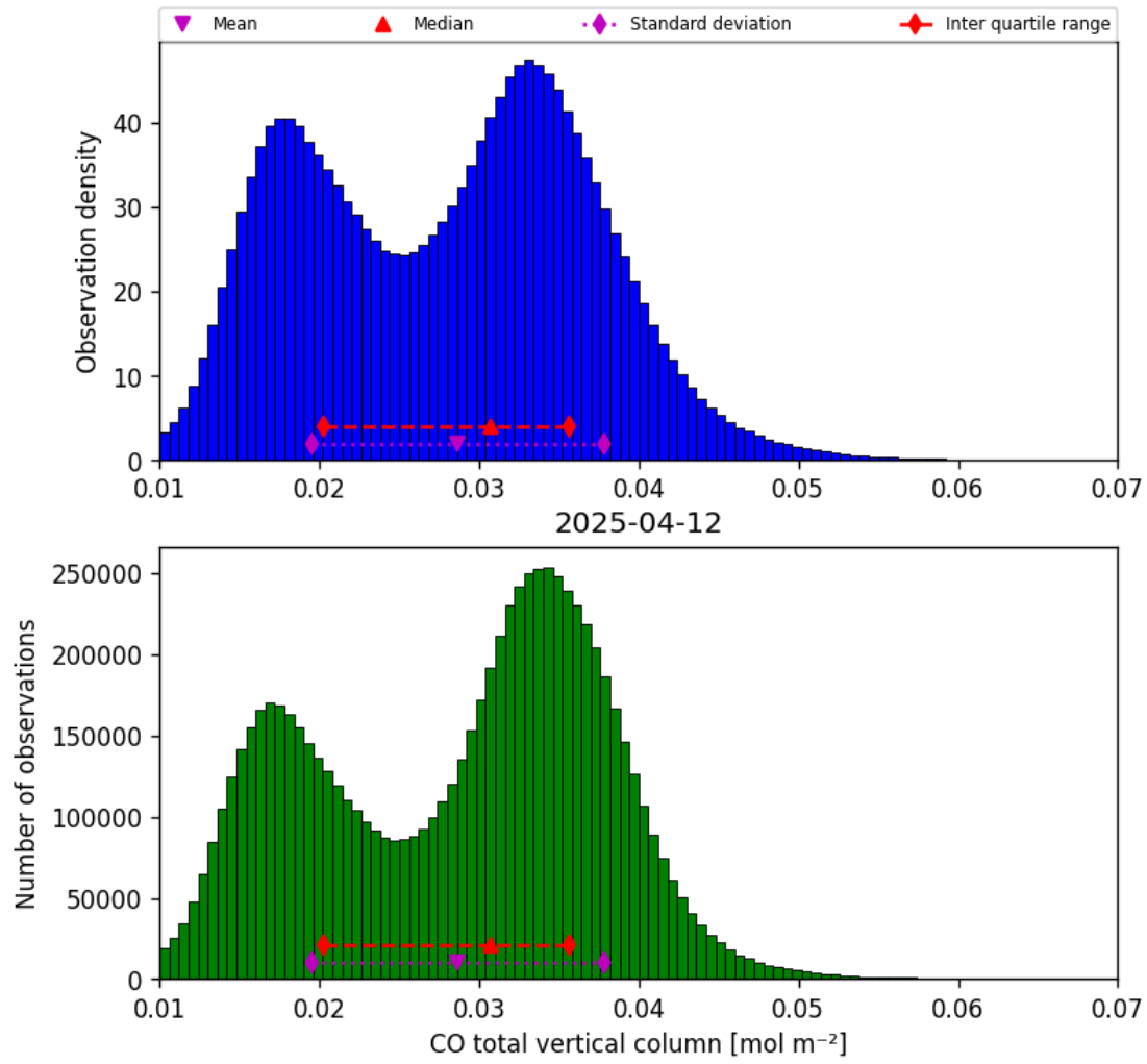
Figure 14: Histogram of “CO total vertical column” for 2025-04-12 to 2025-04-13
