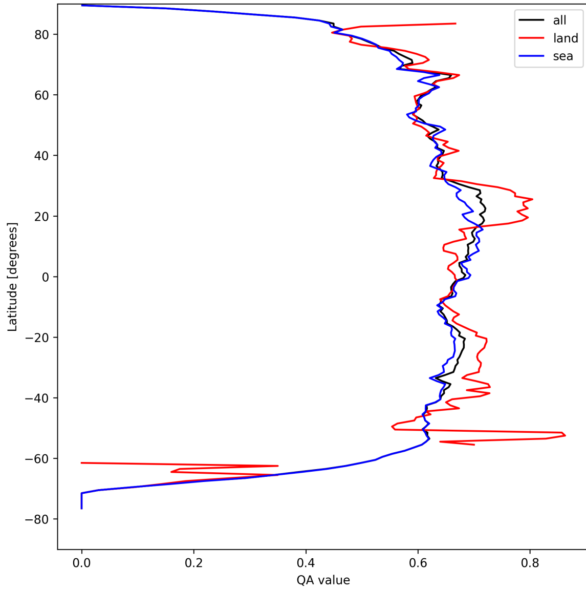
Figure 6: Zonal average of “QA value” for 2025-04-12 to 2025-04-13.
