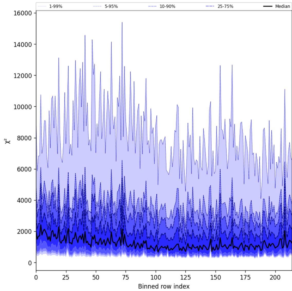
Figure 24: Along track statistics of “ \chi^2 ” for 2025-04-12 to 2025-04-13
