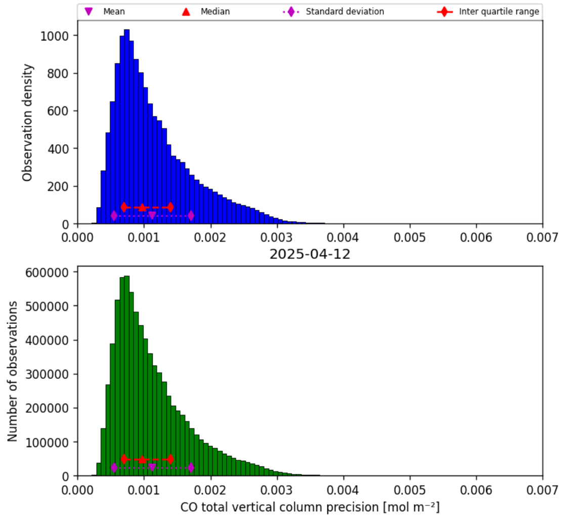
Figure 15: Histogram of “CO total vertical column precision” for 2025-04-12 to 2025-04-13
