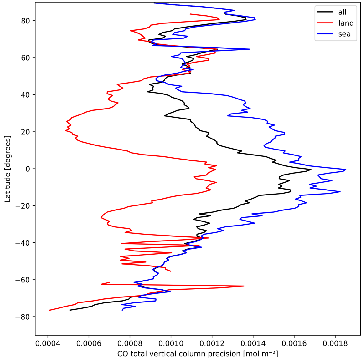
Figure 8: Zonal average of "CO total vertical column precision" for 2025-04-12 to 2025-04-13.
