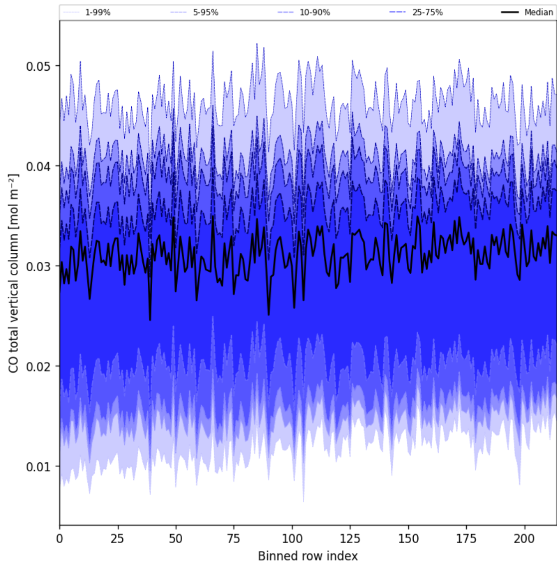
Figure 21: Along track statistics of “CO total vertical column” for 2025-04-12 to 2025-04-13
