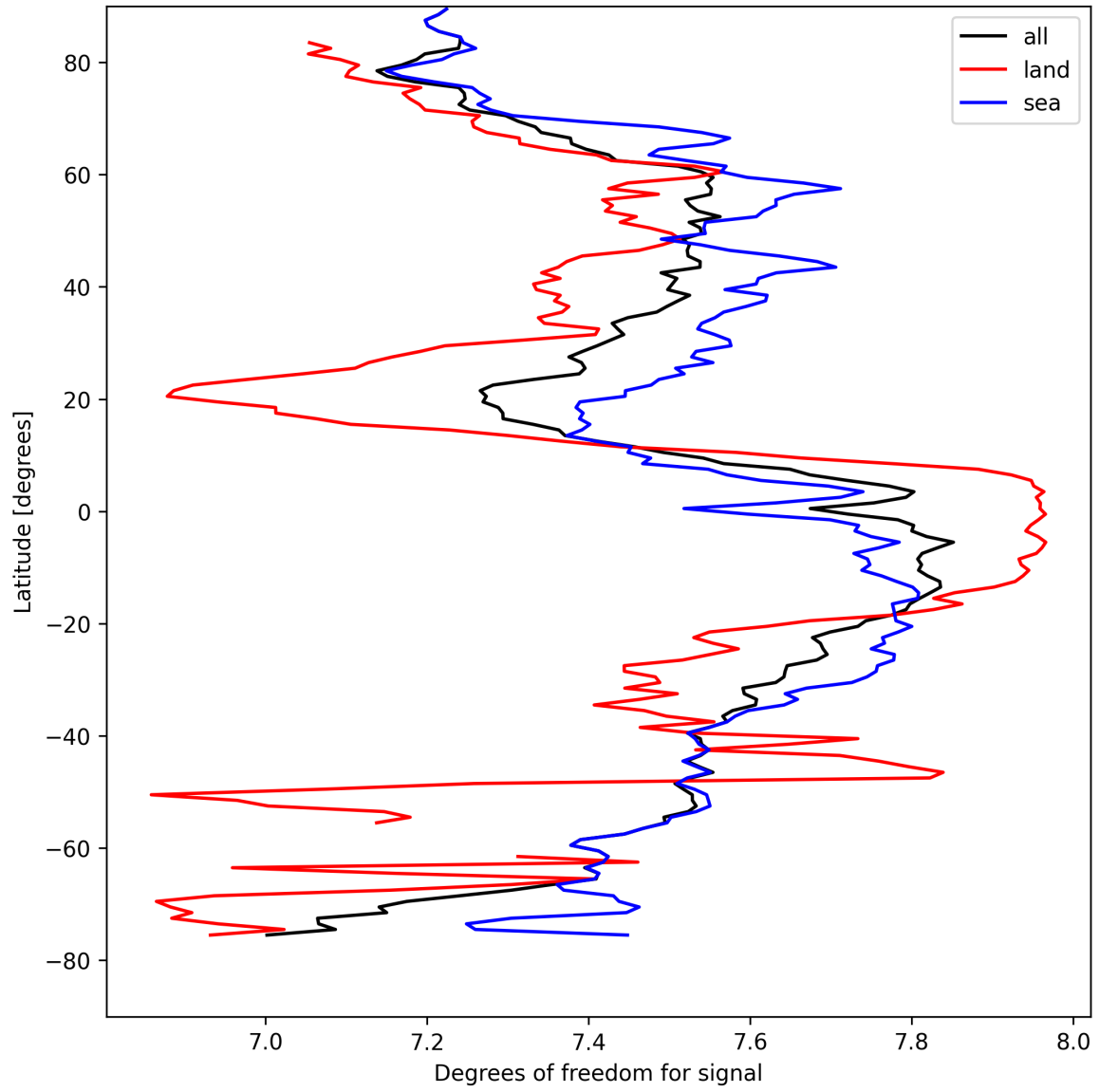
Figure 11: Zonal average of “Degrees of freedom for signal” for 2025-04-13 to 2025-04-14.
