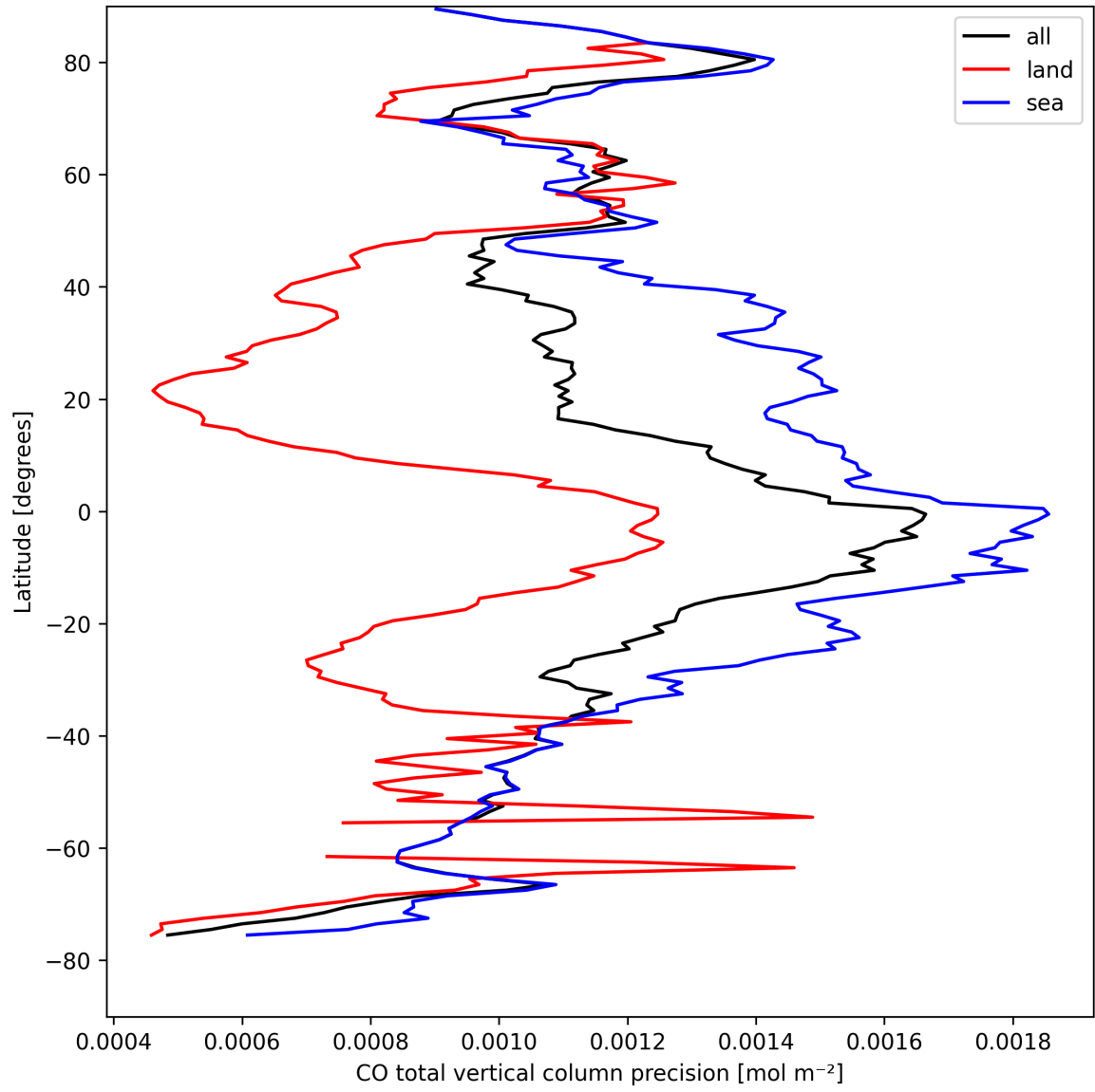
Figure 8: Zonal average of "CO total vertical column precision" for 2025-04-13 to 2025-04-14.
