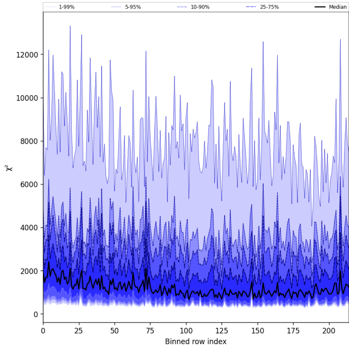
Figure 24: Along track statistics of “ \chi^2 ” for 2025-04-13 to 2025-04-14
