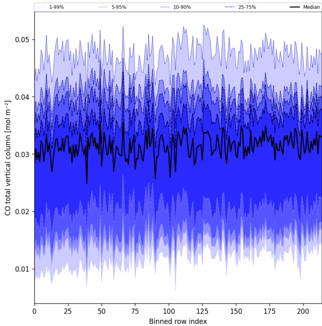
Figure 21: Along track statistics of “CO total vertical column” for 2025-04-13 to 2025-04-14
