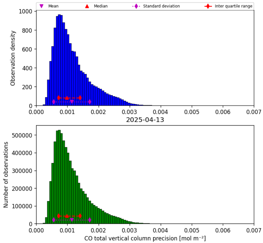
Figure 15: Histogram of “CO total vertical column precision” for 2025-04-13 to 2025-04-14
