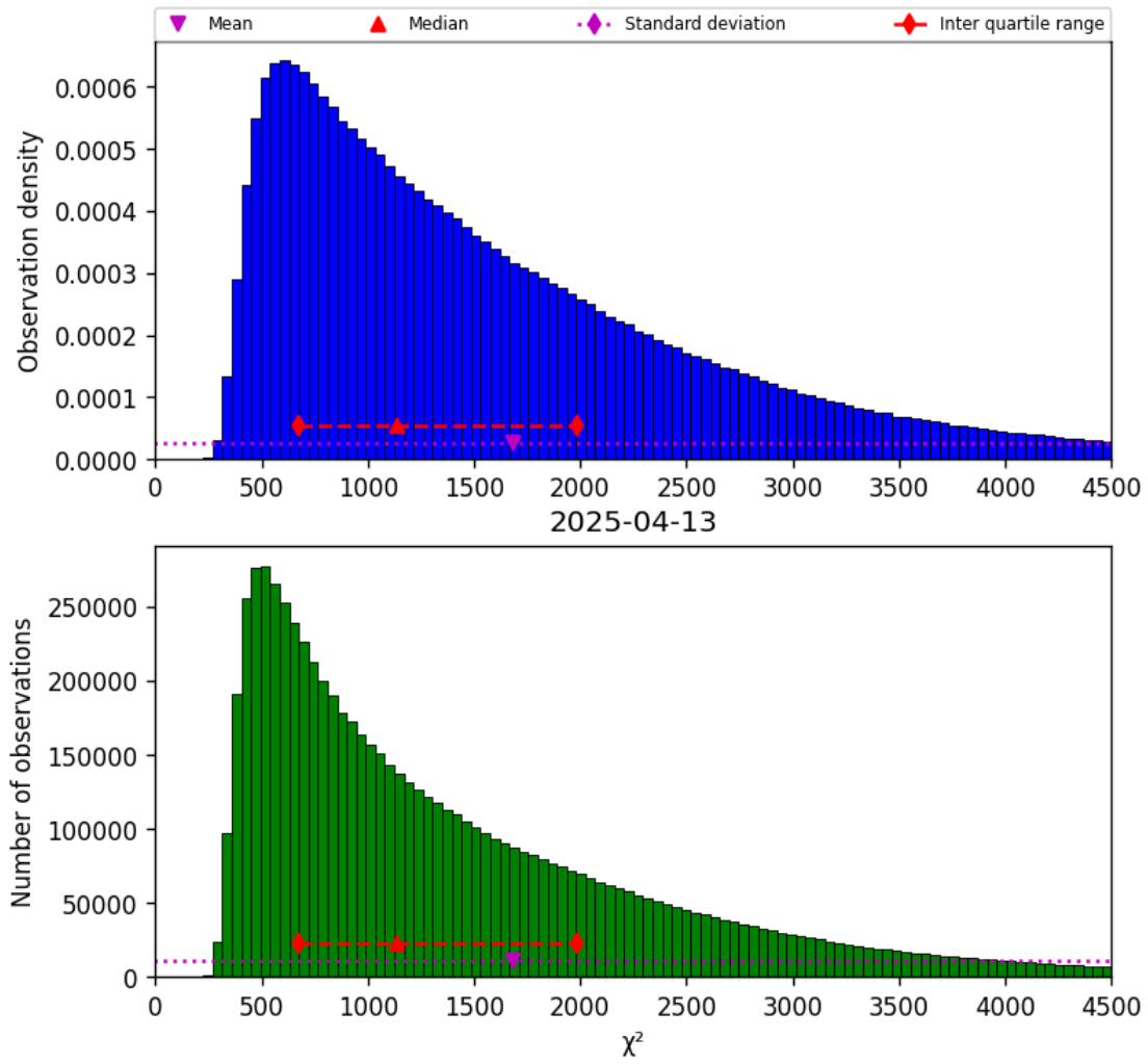
Figure 17: Histogram of “ \chi^2 ” for 2025-04-13 to 2025-04-14
