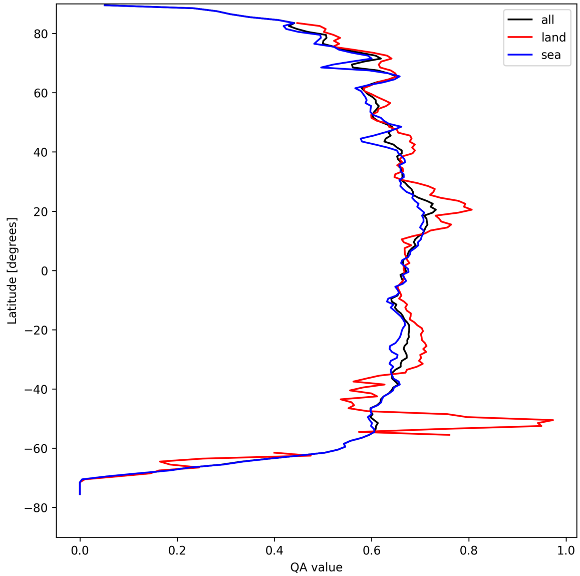
Figure 6: Zonal average of “QA value” for 2025-04-13 to 2025-04-14.
