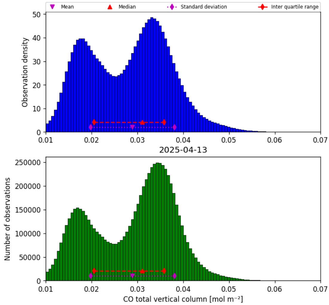
Figure 14: Histogram of “CO total vertical column” for 2025-04-13 to 2025-04-14
