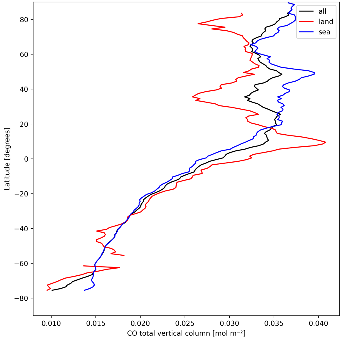
Figure 7: Zonal average of “CO total vertical column” for 2025-04-13 to 2025-04-14.
