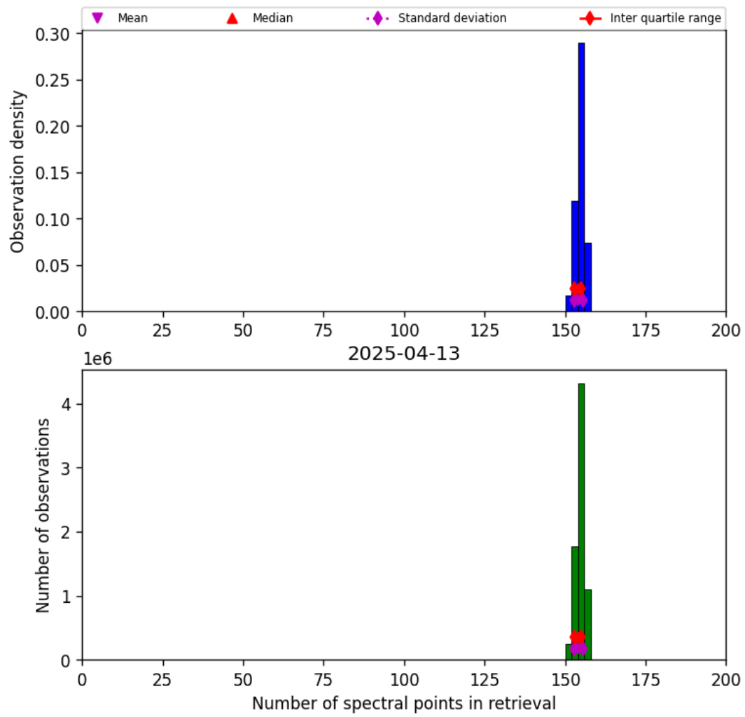
Figure 16: Histogram of “Number of spectral points in retrieval” for 2025-04-13 to 2025-04-14
