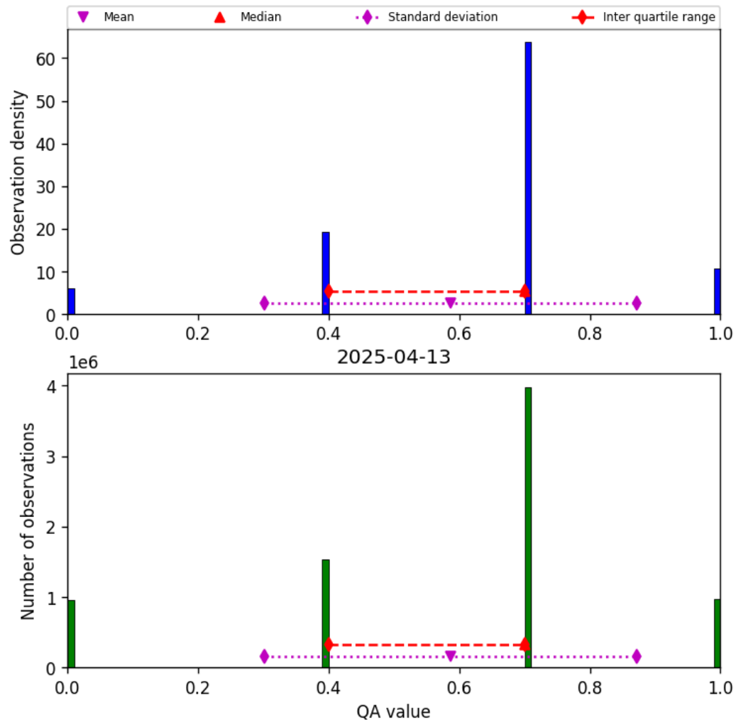
Figure 13: Histogram of "QA value" for 2025-04-13 to 2025-04-14
