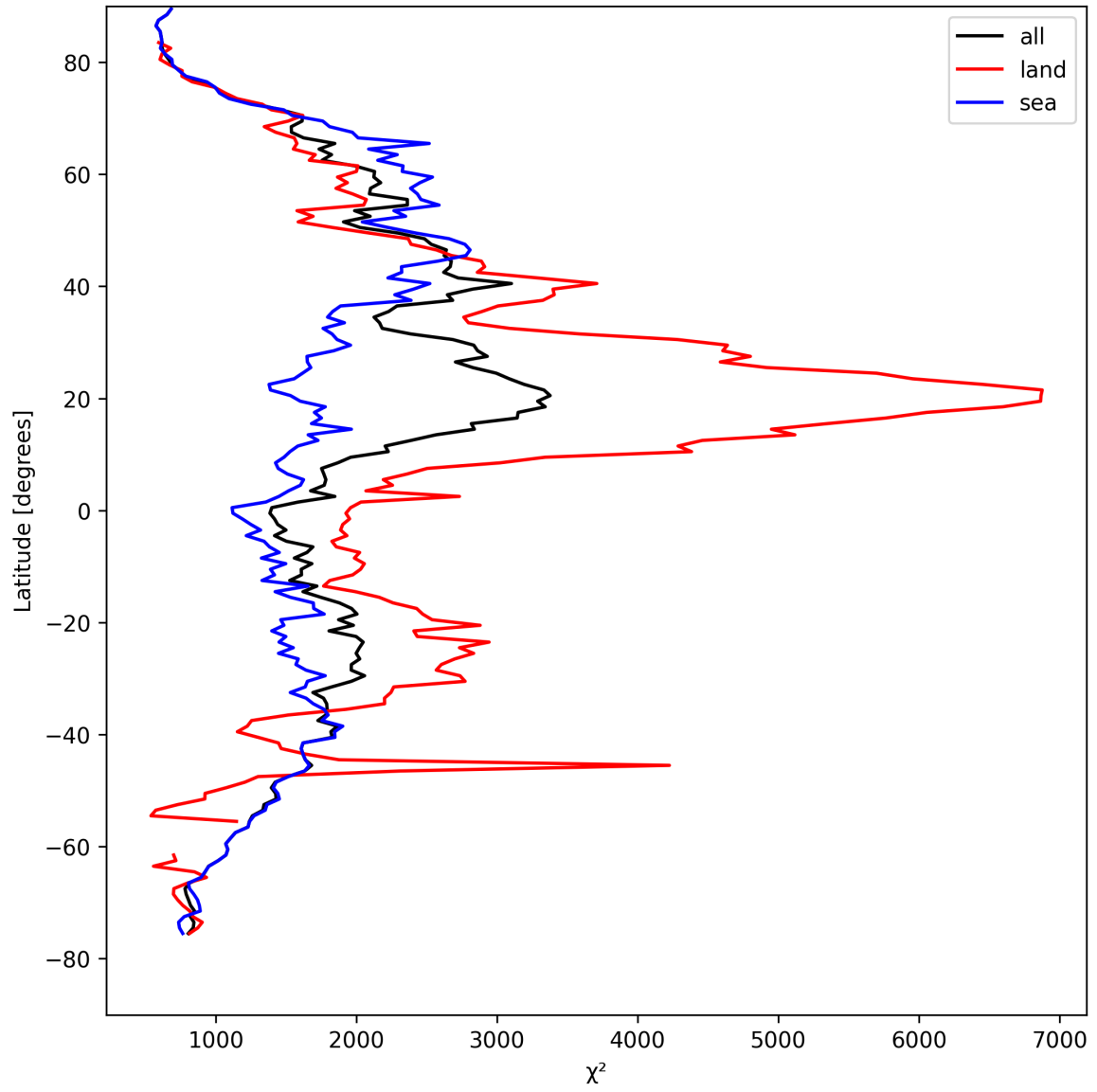
Figure 10: Zonal average of “ \chi^2 ” for 2025-04-13 to 2025-04-14.
