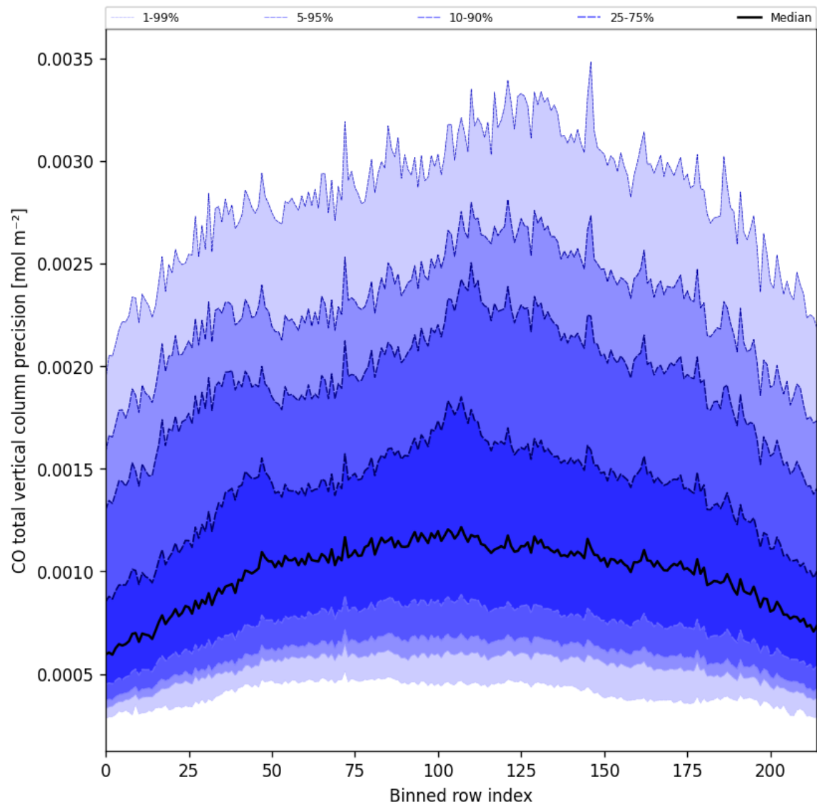
Figure 22: Along track statistics of “CO total vertical column precision” for 2025-04-13 to 2025-04-14
