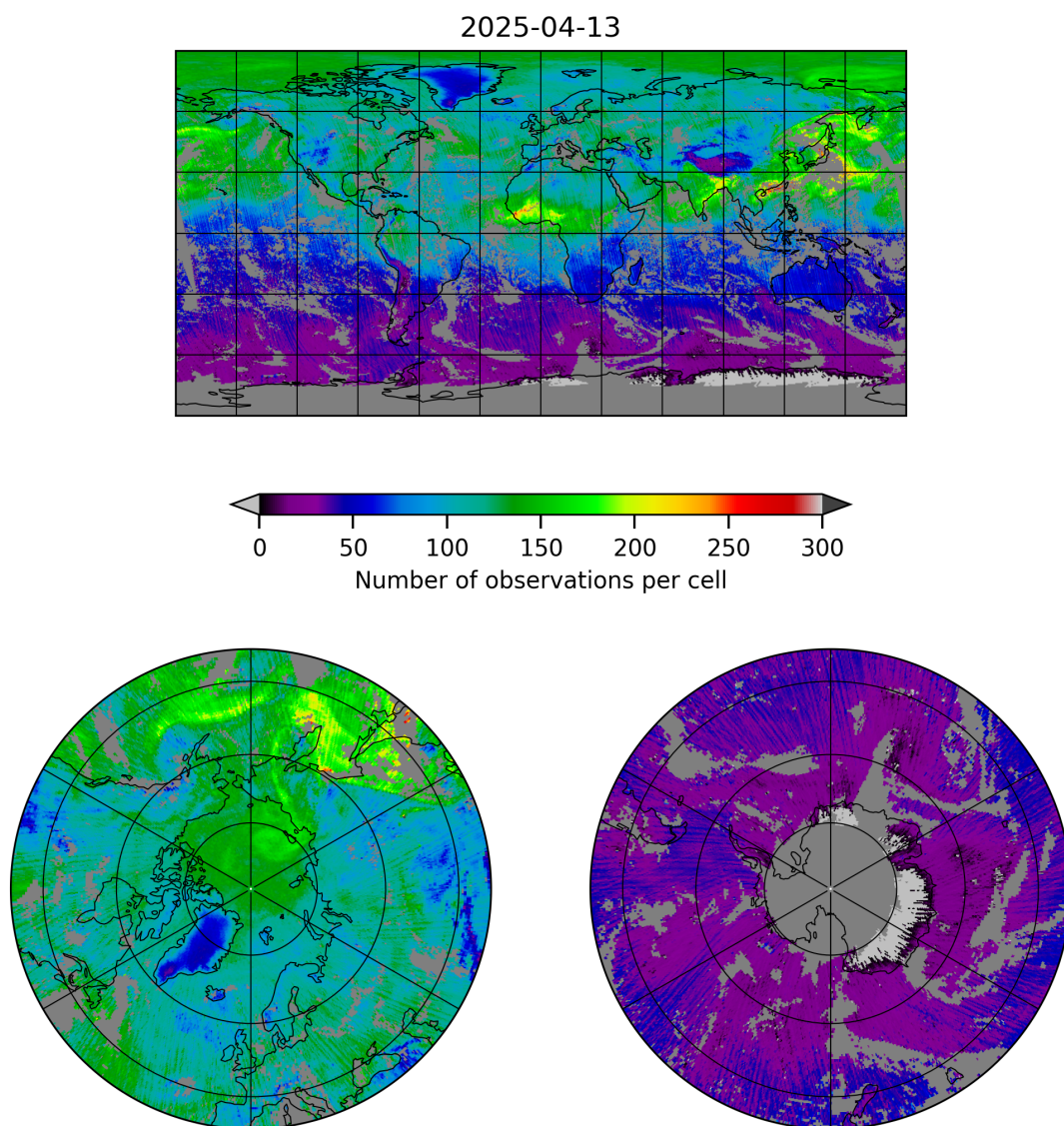
Figure 5: Map of the number of observations for 2025-04-13 to 2025-04-14
