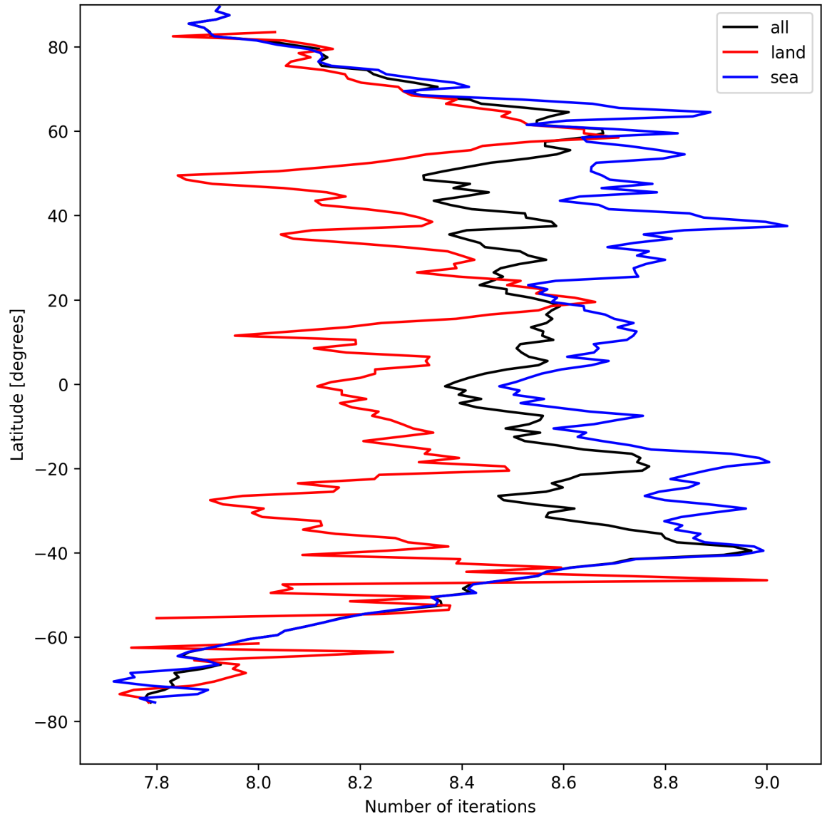
Figure 12: Zonal average of “Number of iterations” for 2025-04-13 to 2025-04-14.
