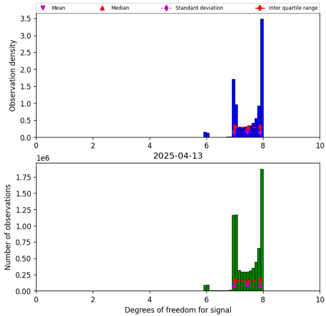
Figure 18: Histogram of “Degrees of freedom for signal” for 2025-04-13 to 2025-04-14
