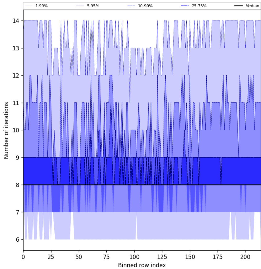
Figure 26: Along track statistics of “Number of iterations” for 2025-04-13 to 2025-04-14
