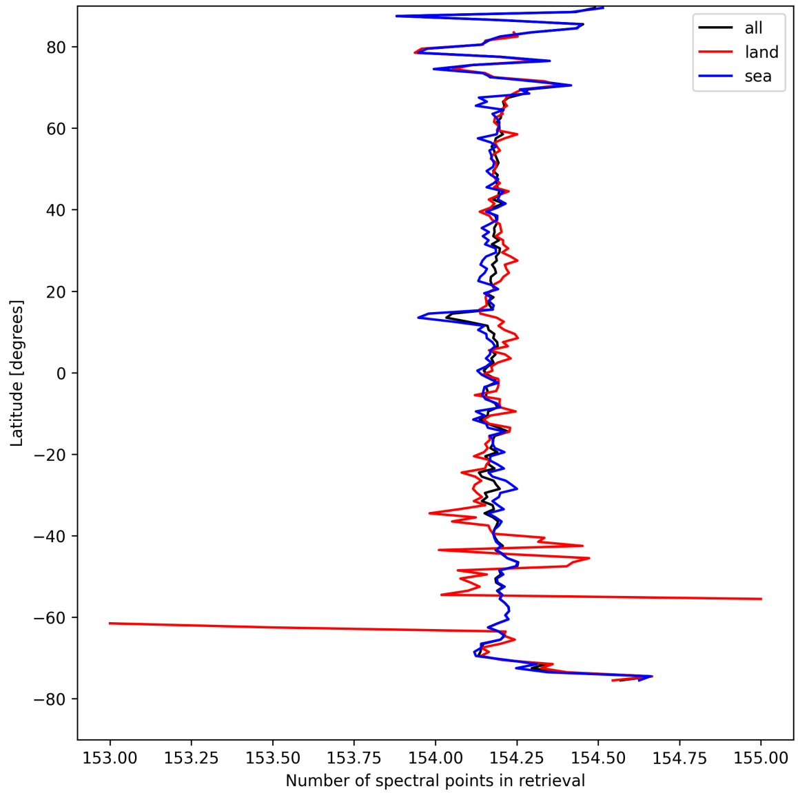
Figure 9: Zonal average of “Number of spectral points in retrieval” for 2025-04-13 to 2025-04-14.
