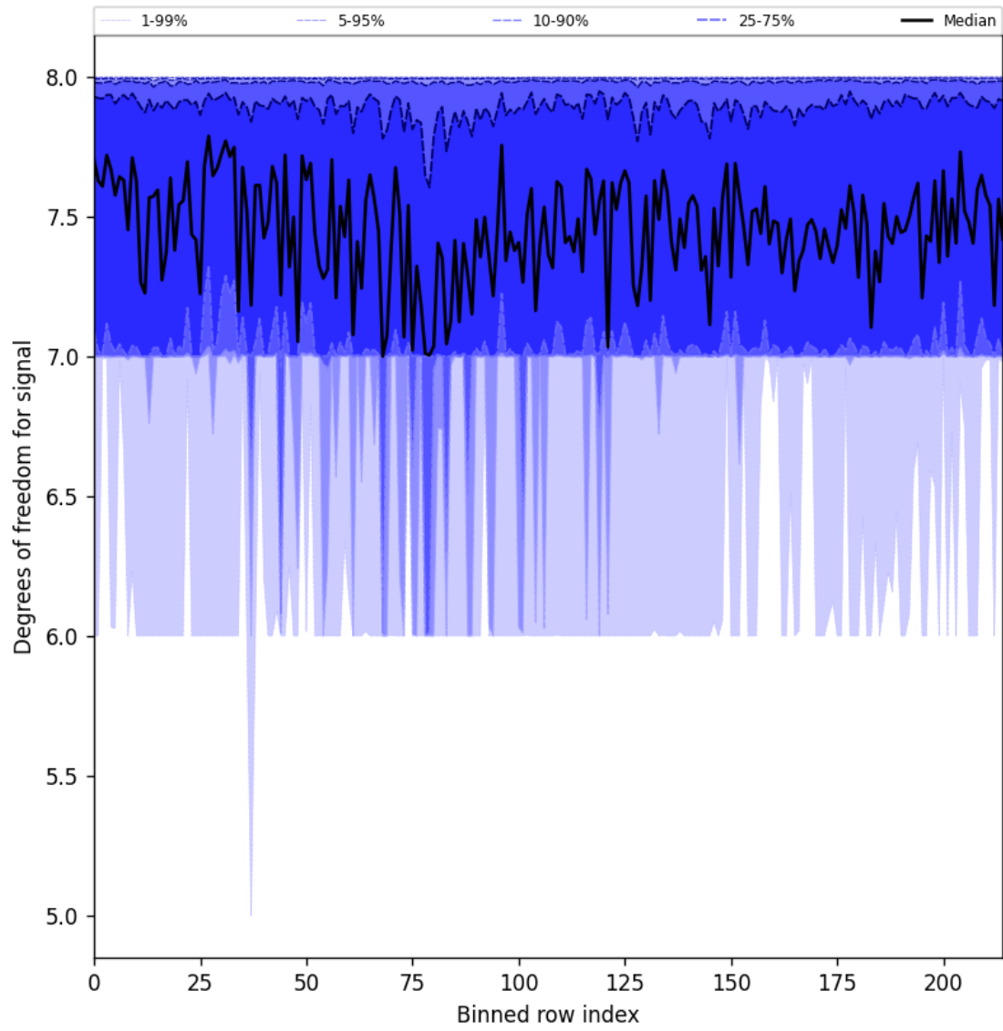
Figure 25: Along track statistics of “Degrees of freedom for signal” for 2025-04-13 to 2025-04-14
