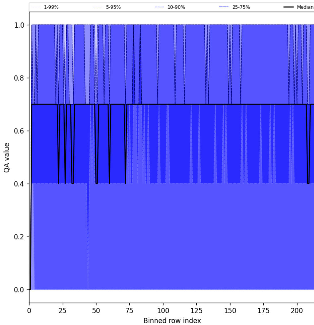
Figure 20: Along track statistics of “QA value” for 2025-04-13 to 2025-04-14
