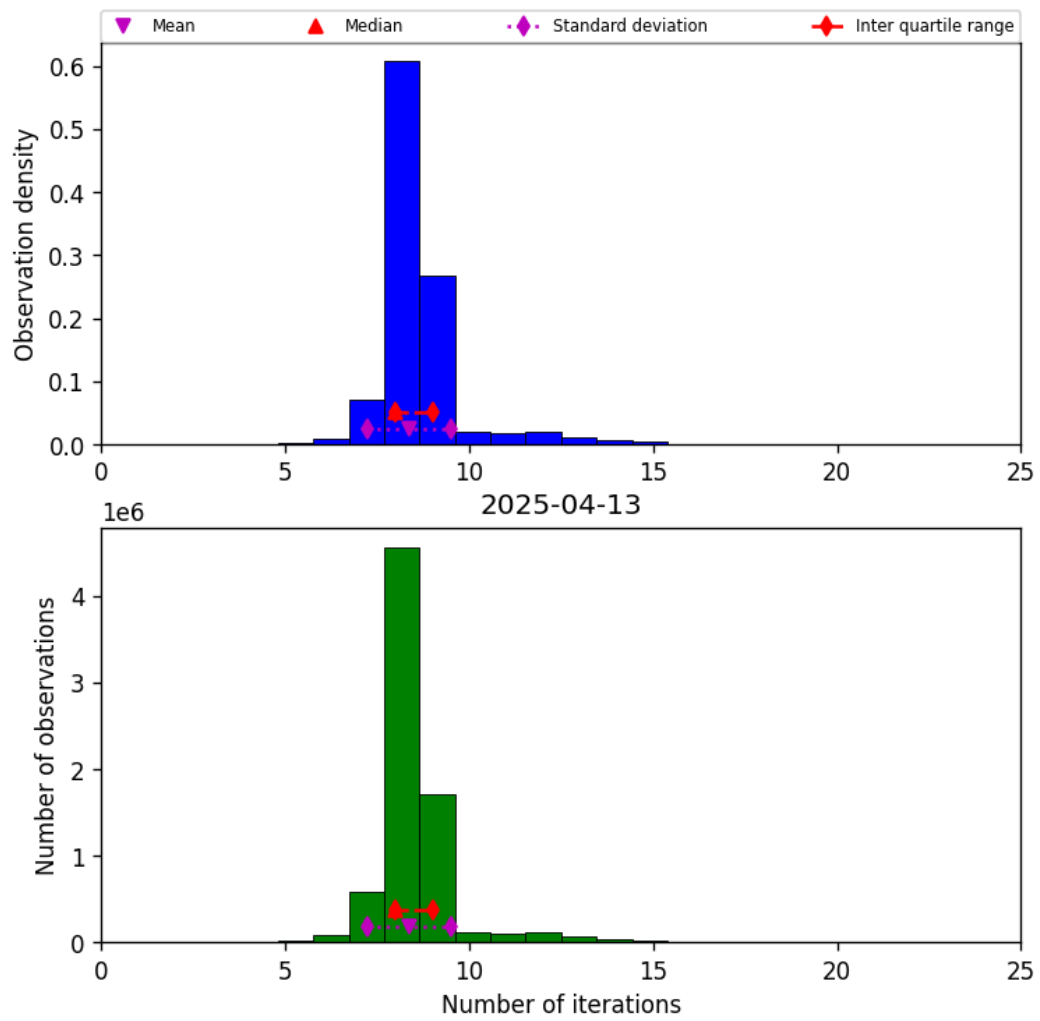
Figure 19: Histogram of “Number of iterations” for 2025-04-13 to 2025-04-14
