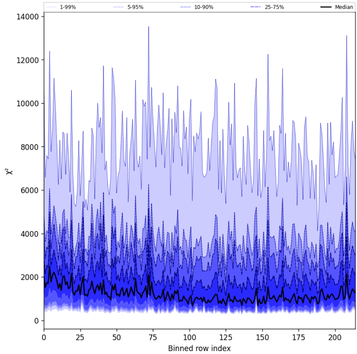
Figure 24: Along track statistics of “ \chi^2 ” for 2025-04-14 to 2025-04-15
