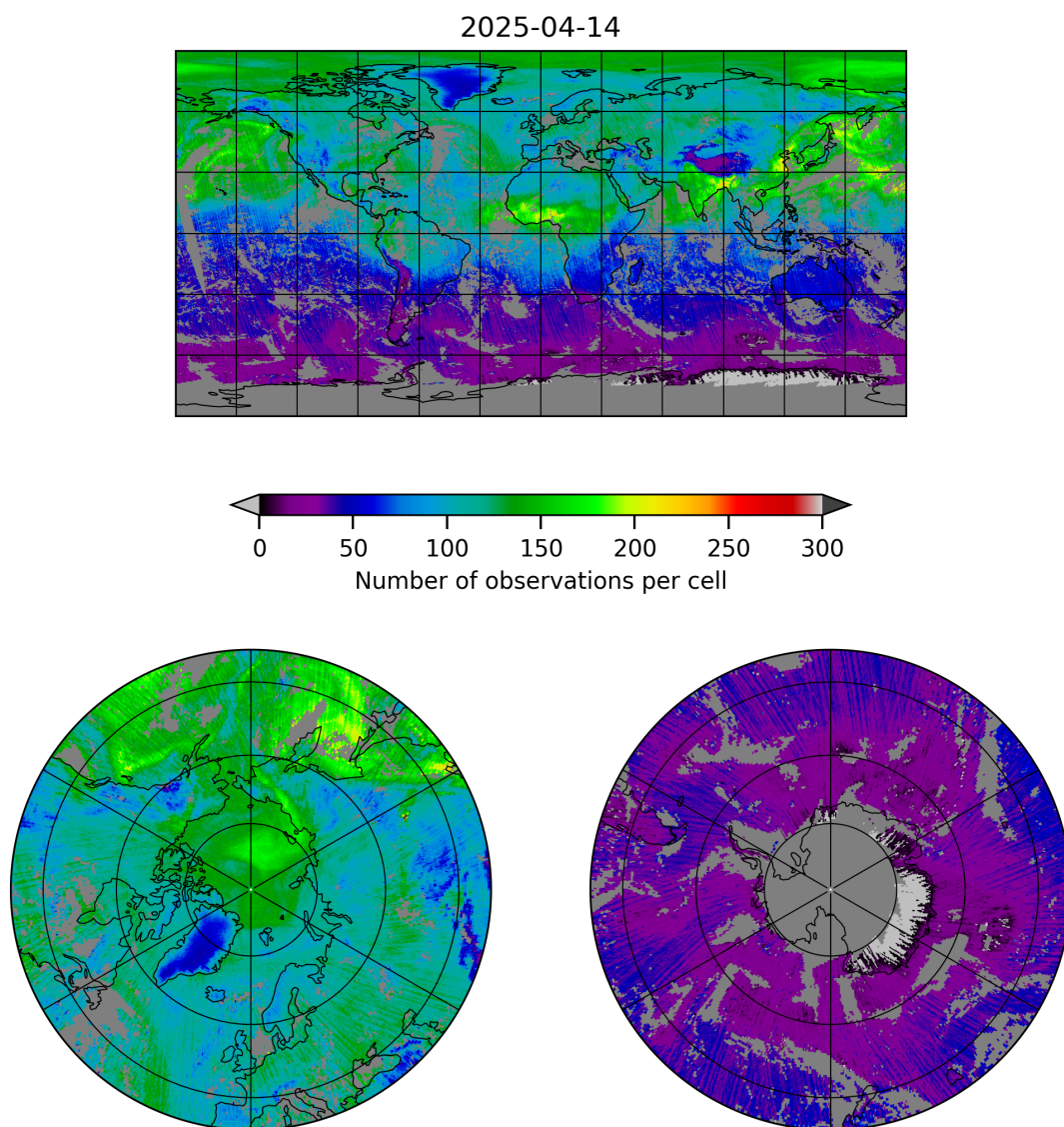
Figure 5: Map of the number of observations for 2025-04-14 to 2025-04-15
