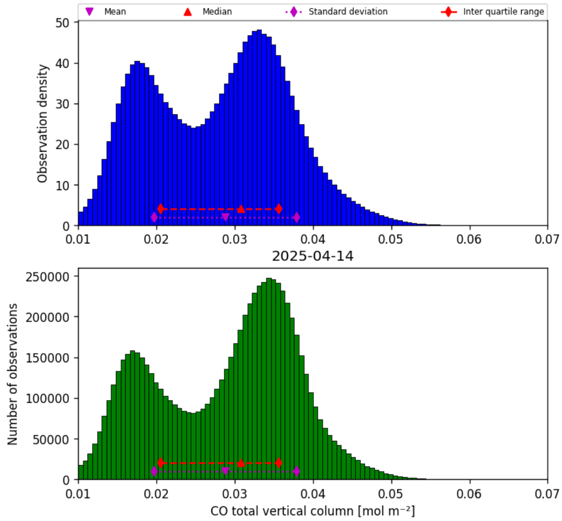
Figure 14: Histogram of “CO total vertical column” for 2025-04-14 to 2025-04-15
