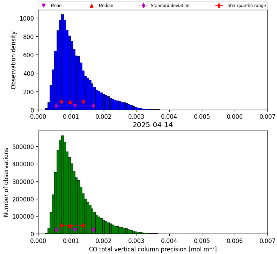
Figure 15: Histogram of “CO total vertical column precision” for 2025-04-14 to 2025-04-15
