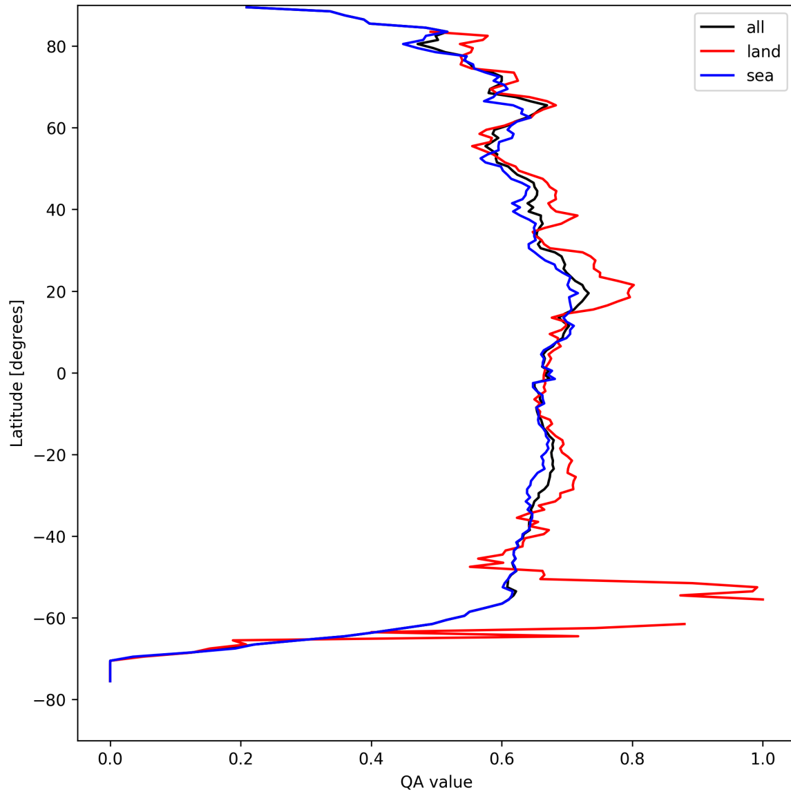
Figure 6: Zonal average of “QA value” for 2025-04-14 to 2025-04-15.
