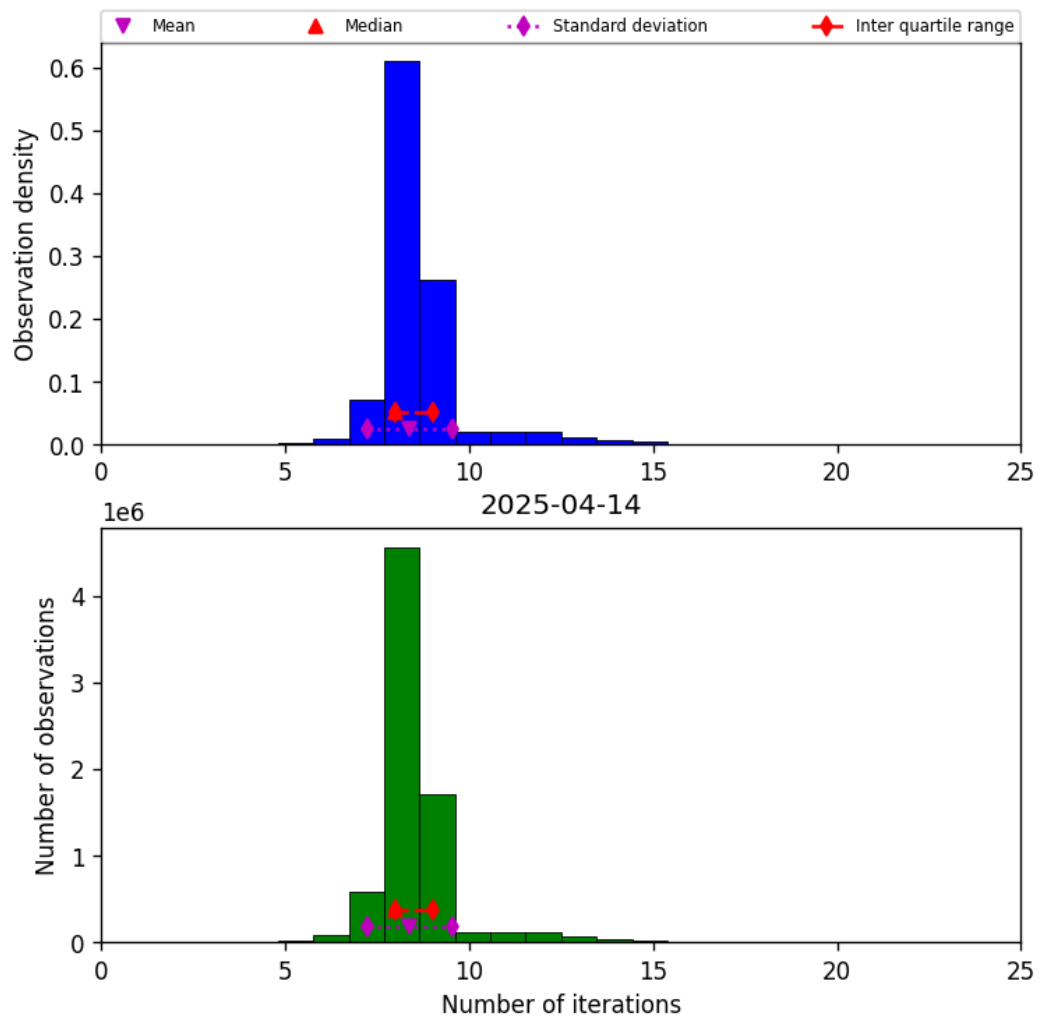
Figure 19: Histogram of “Number of iterations” for 2025-04-14 to 2025-04-15
