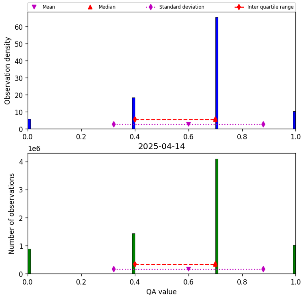
Figure 13: Histogram of “QA value” for 2025-04-14 to 2025-04-15
