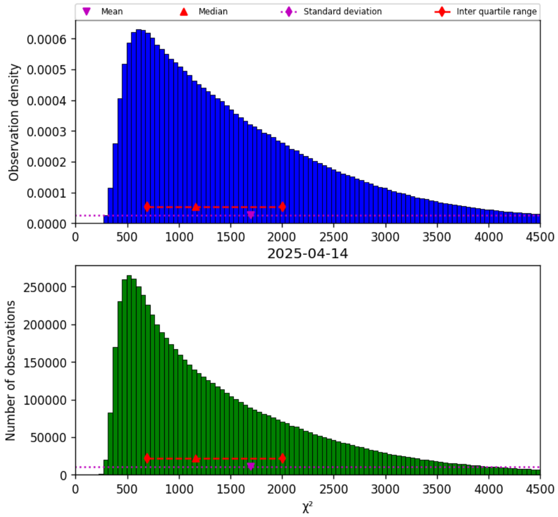
Figure 17: Histogram of “ \chi^2 ” for 2025-04-14 to 2025-04-15
