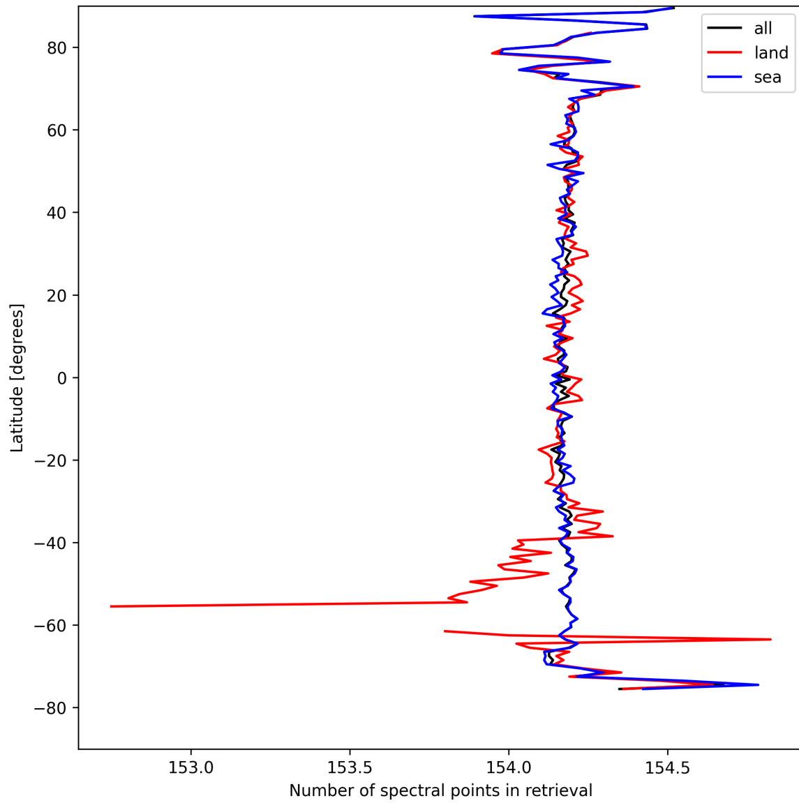
Figure 9: Zonal average of “Number of spectral points in retrieval” for 2025-04-14 to 2025-04-15.
