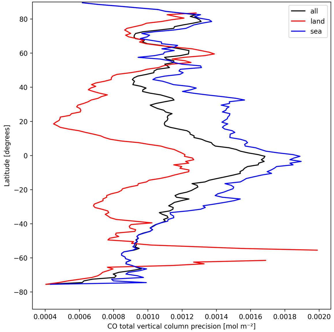
Figure 8: Zonal average of "CO total vertical column precision" for 2025-04-14 to 2025-04-15.
