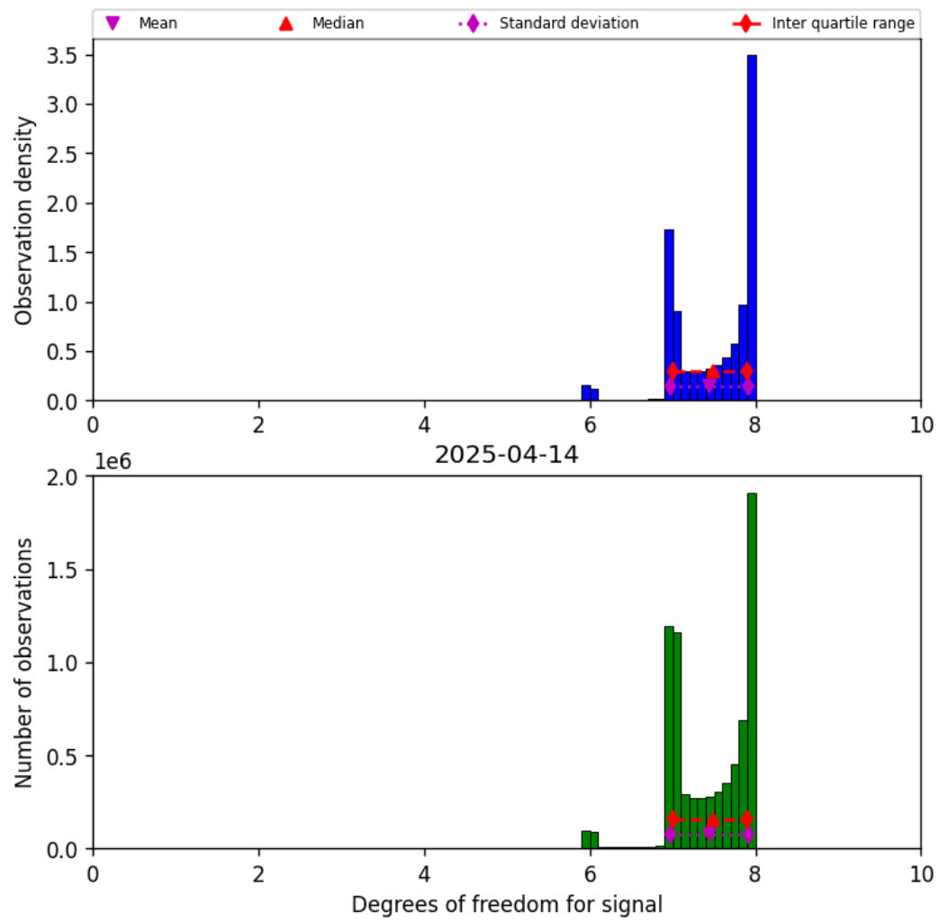
Figure 18: Histogram of “Degrees of freedom for signal” for 2025-04-14 to 2025-04-15
