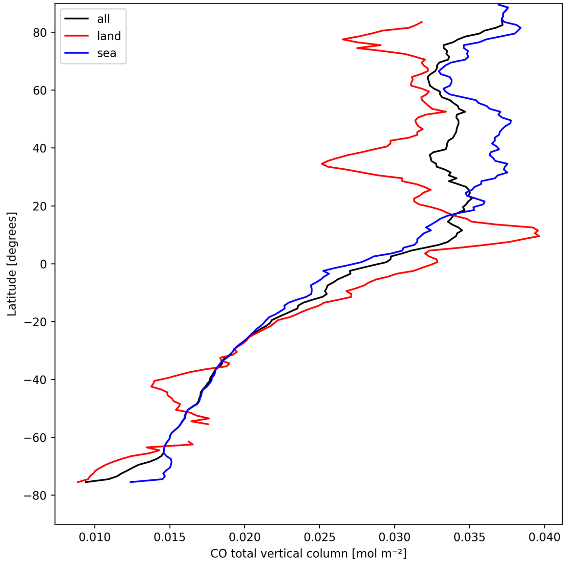
Figure 7: Zonal average of “CO total vertical column” for 2025-04-14 to 2025-04-15.
