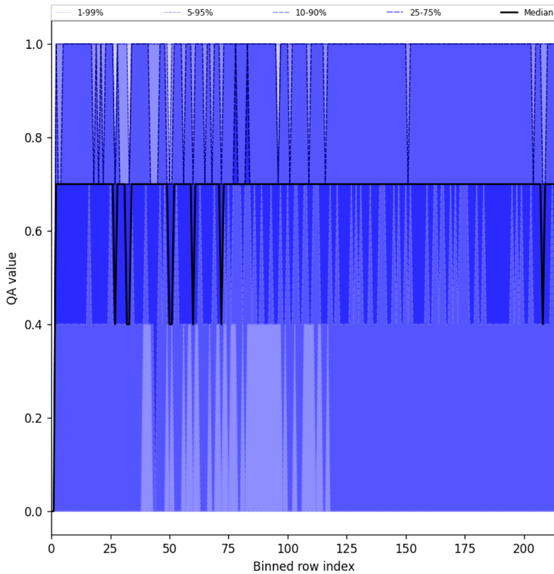
Figure 20: Along track statistics of “QA value” for 2025-04-14 to 2025-04-15
