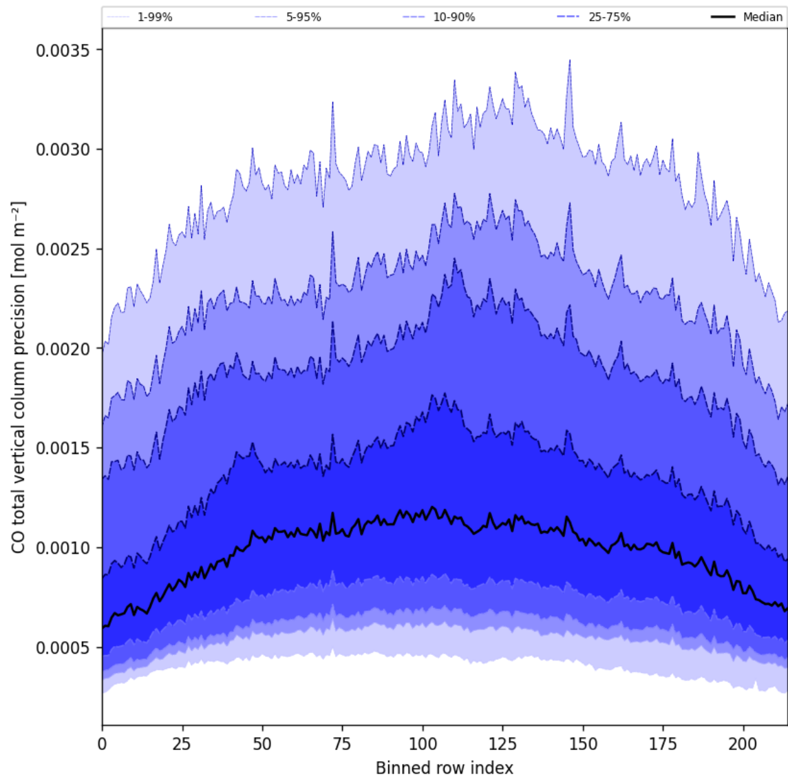
Figure 22: Along track statistics of “CO total vertical column precision” for 2025-04-14 to 2025-04-15
