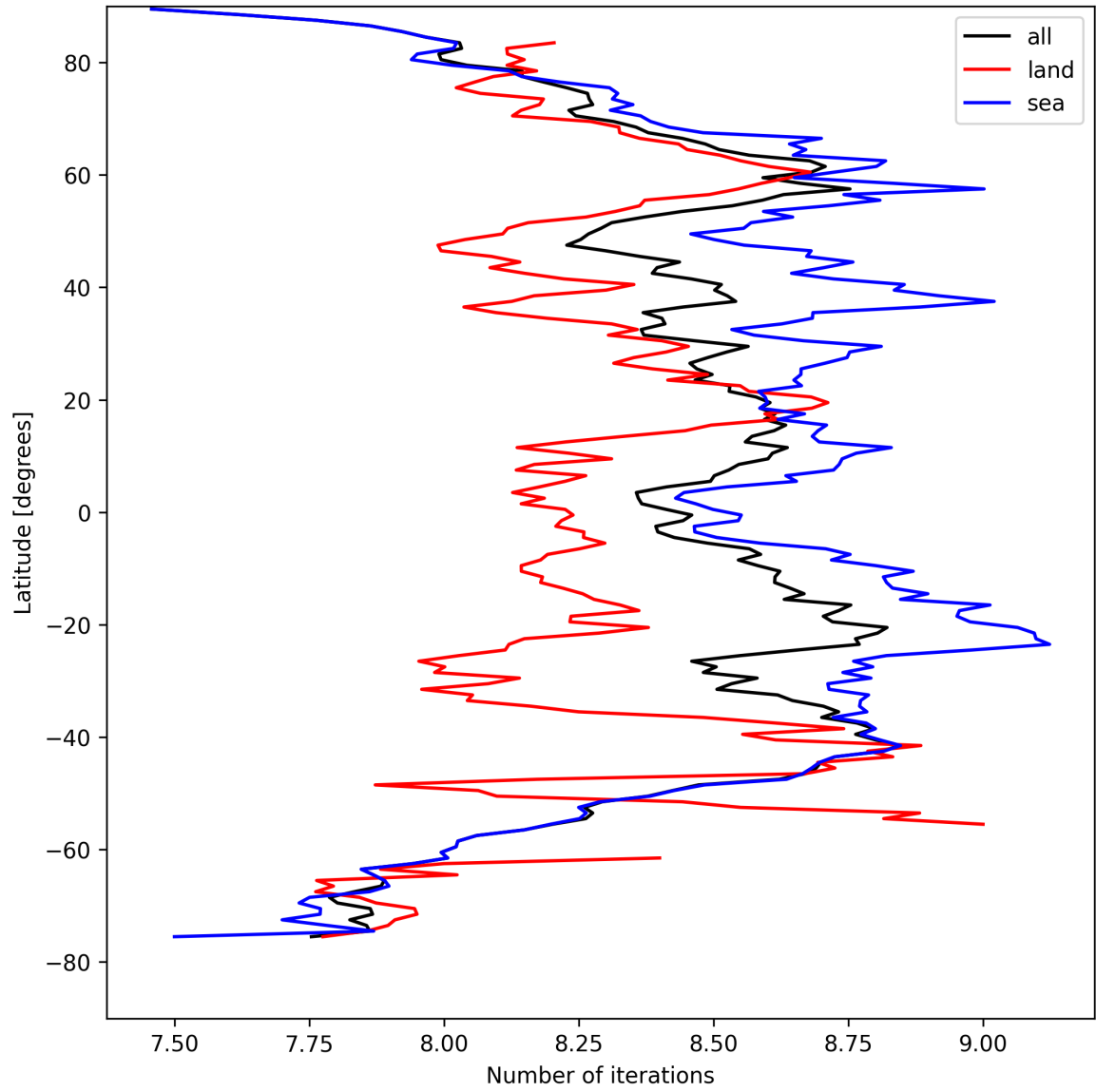
Figure 12: Zonal average of “Number of iterations” for 2025-04-14 to 2025-04-15.
