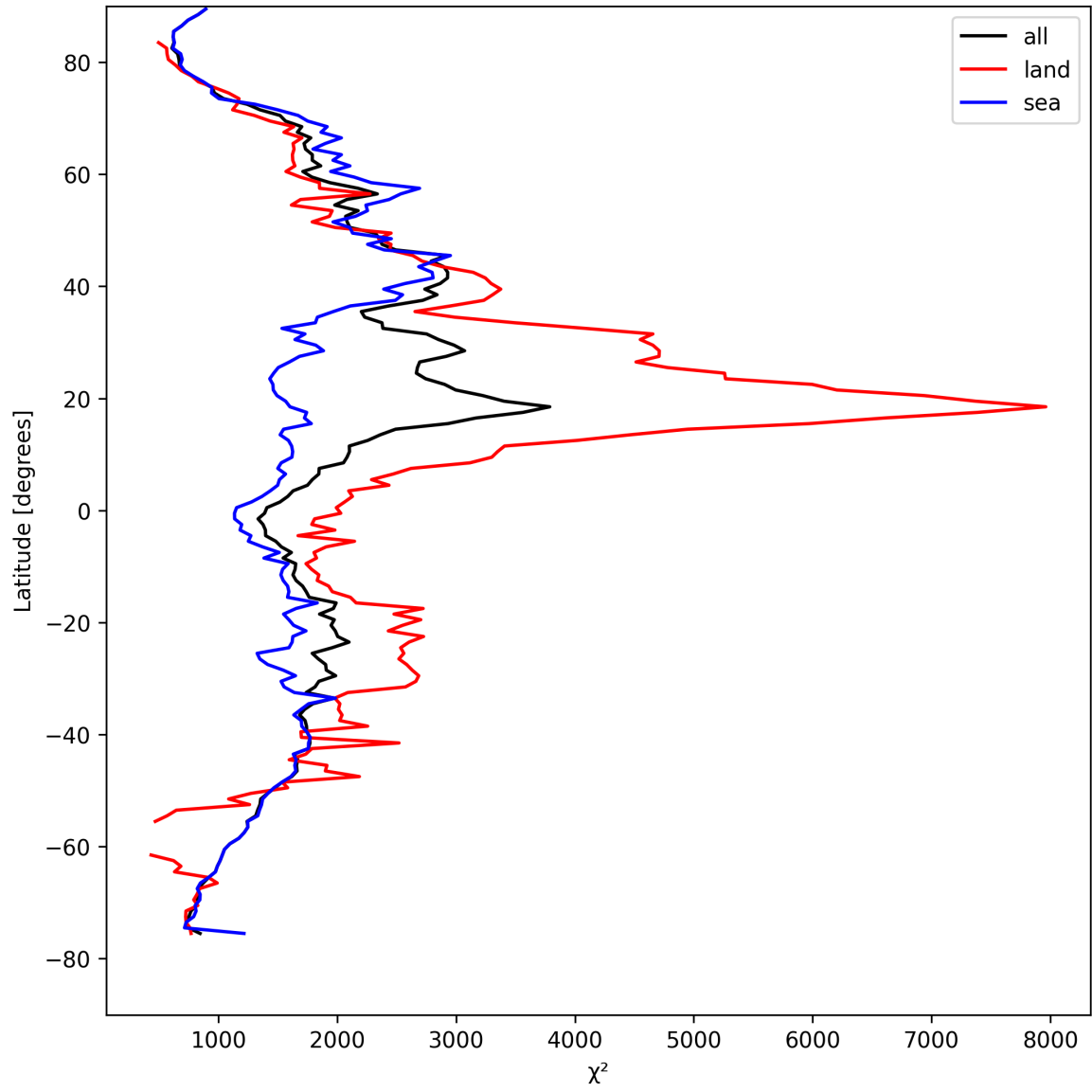
Figure 10: Zonal average of “ \chi^2 ” for 2025-04-14 to 2025-04-15.
