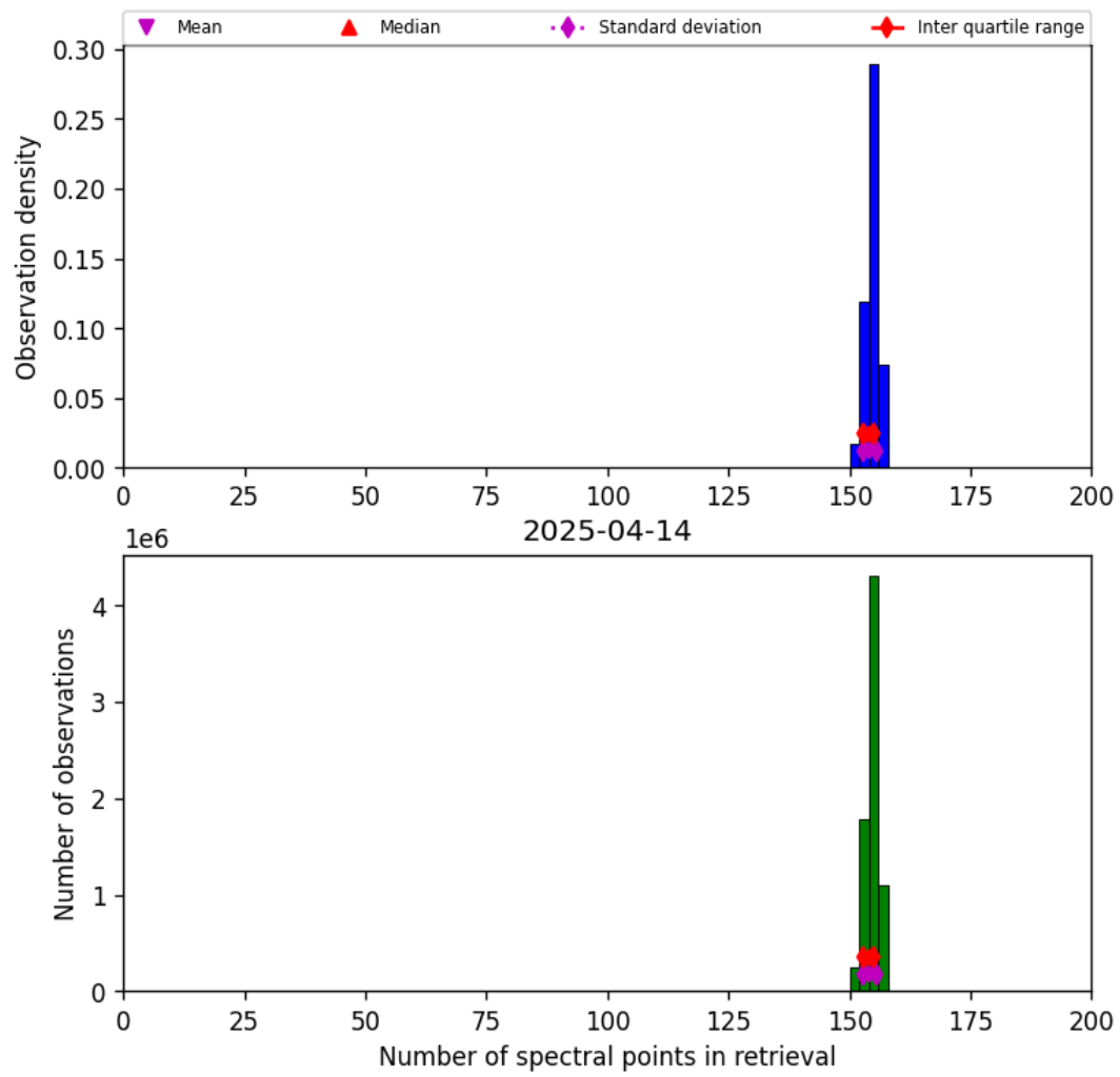
Figure 16: Histogram of “Number of spectral points in retrieval” for 2025-04-14 to 2025-04-15
