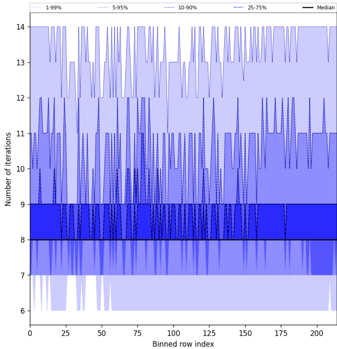
Figure 26: Along track statistics of “Number of iterations” for 2025-04-14 to 2025-04-15
