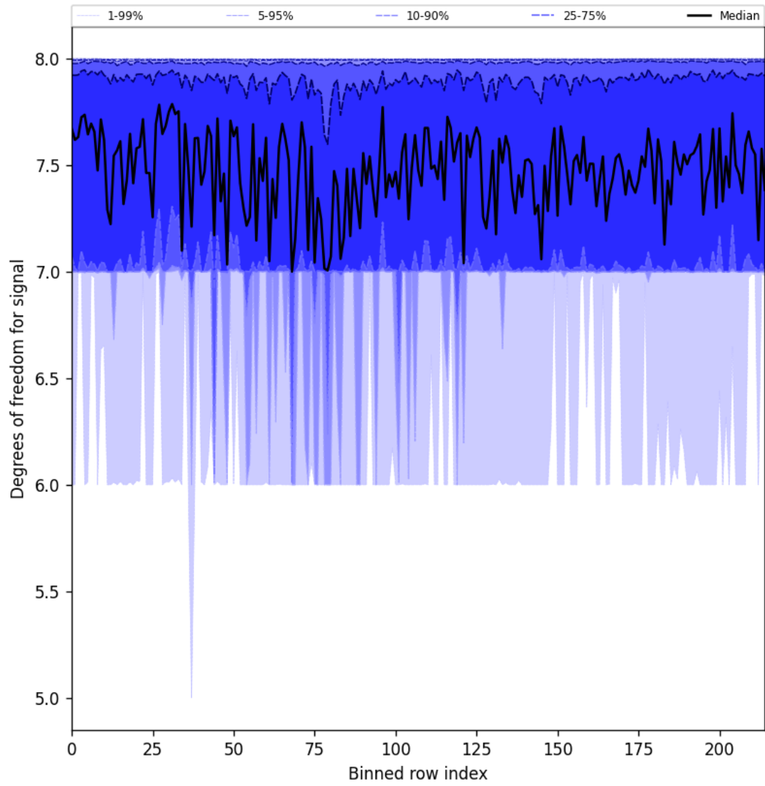
Figure 25: Along track statistics of “Degrees of freedom for signal” for 2025-04-14 to 2025-04-15
