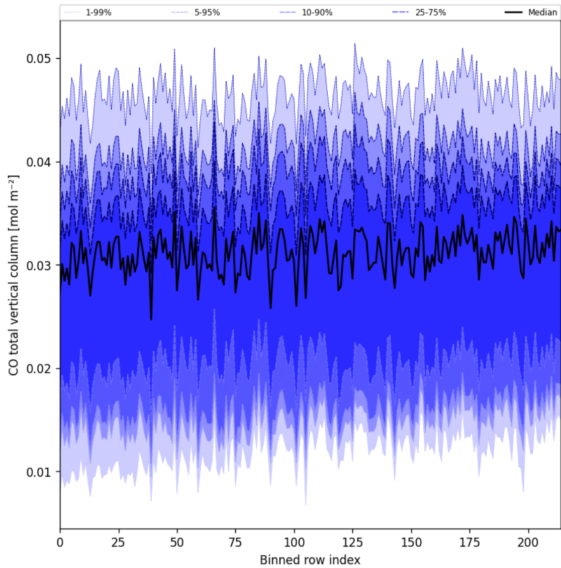
Figure 21: Along track statistics of “CO total vertical column” for 2025-04-14 to 2025-04-15
