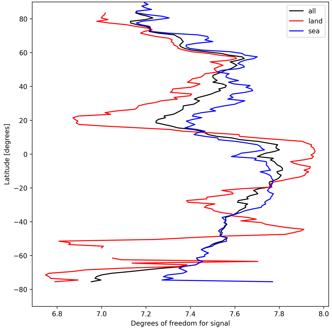
Figure 11: Zonal average of “Degrees of freedom for signal” for 2025-04-14 to 2025-04-15.
