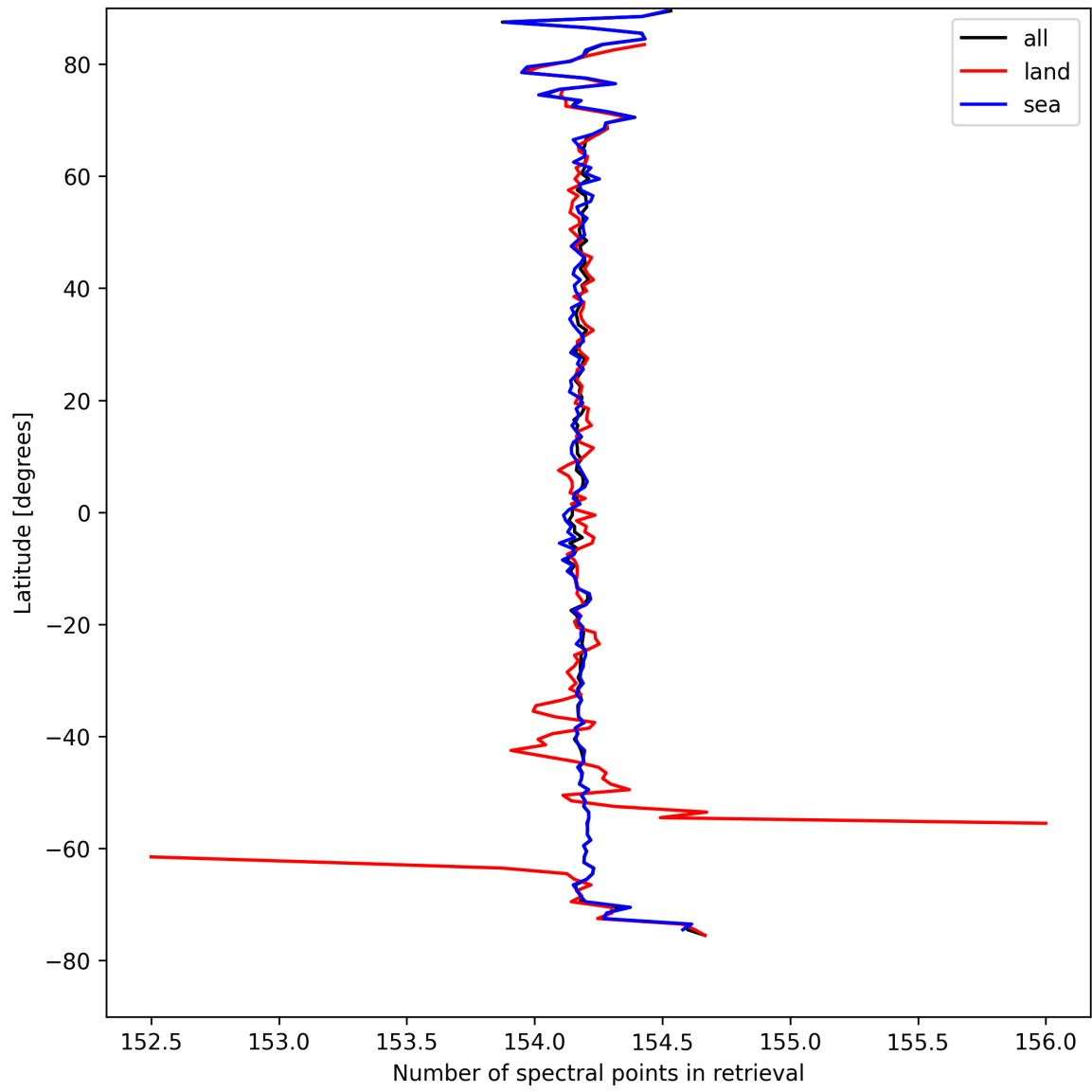
Figure 9: Zonal average of “Number of spectral points in retrieval” for 2025-04-15 to 2025-04-16.
