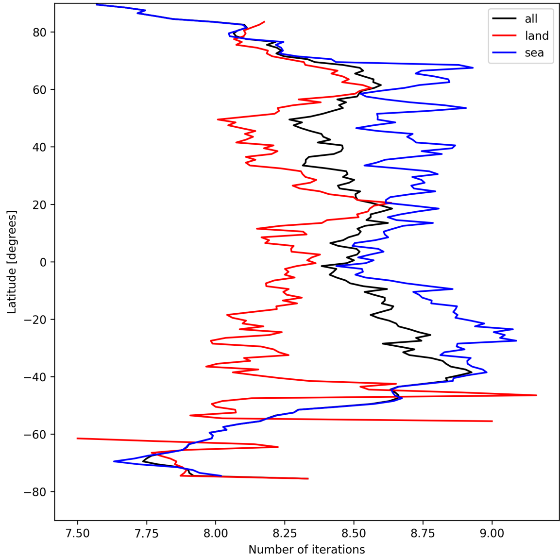
Figure 12: Zonal average of “Number of iterations” for 2025-04-15 to 2025-04-16.
