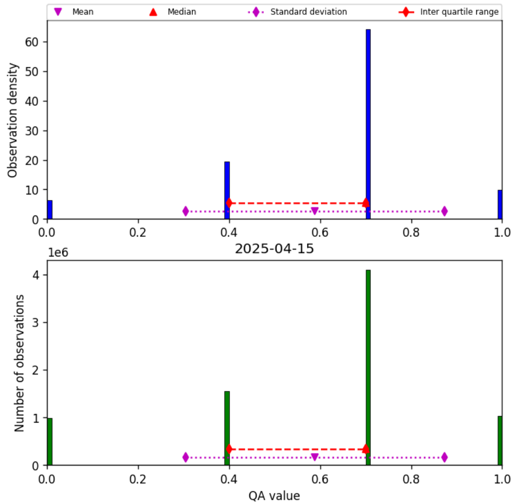
Figure 13: Histogram of “QA value” for 2025-04-15 to 2025-04-16
