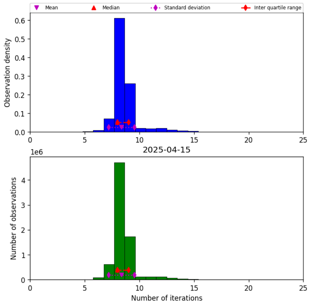
Figure 19: Histogram of “Number of iterations” for 2025-04-15 to 2025-04-16
