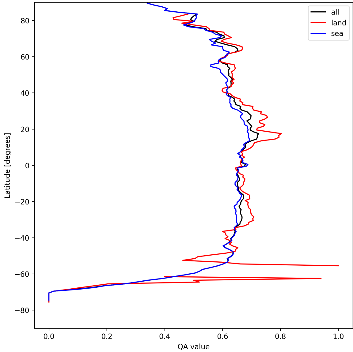
Figure 6: Zonal average of “QA value” for 2025-04-15 to 2025-04-16.
