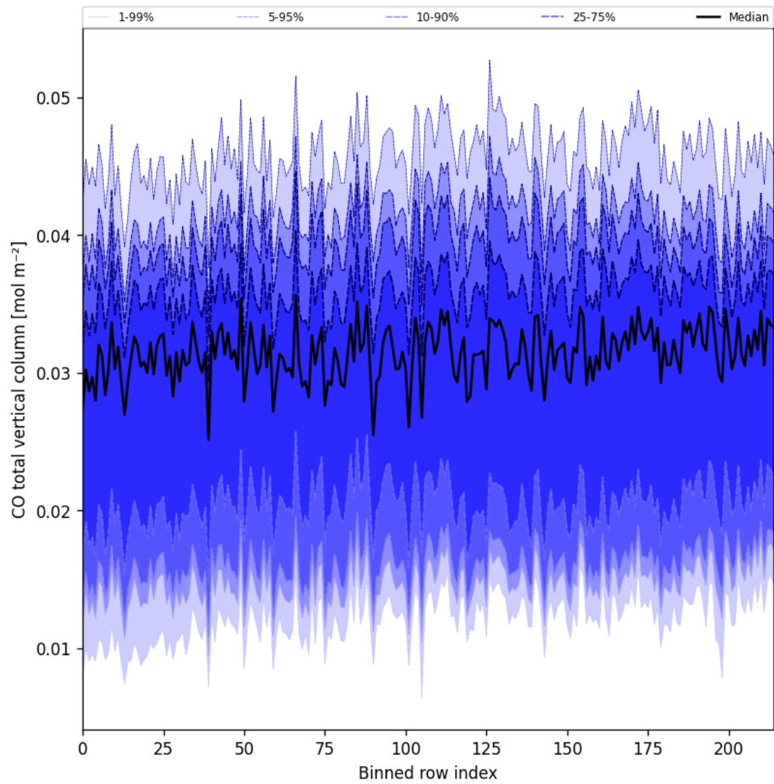
Figure 21: Along track statistics of “CO total vertical column” for 2025-04-15 to 2025-04-16
