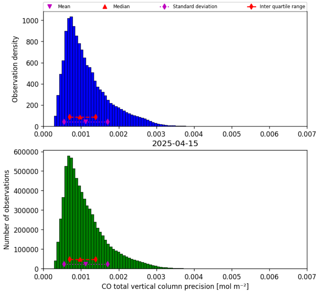
Figure 15: Histogram of “CO total vertical column precision” for 2025-04-15 to 2025-04-16
