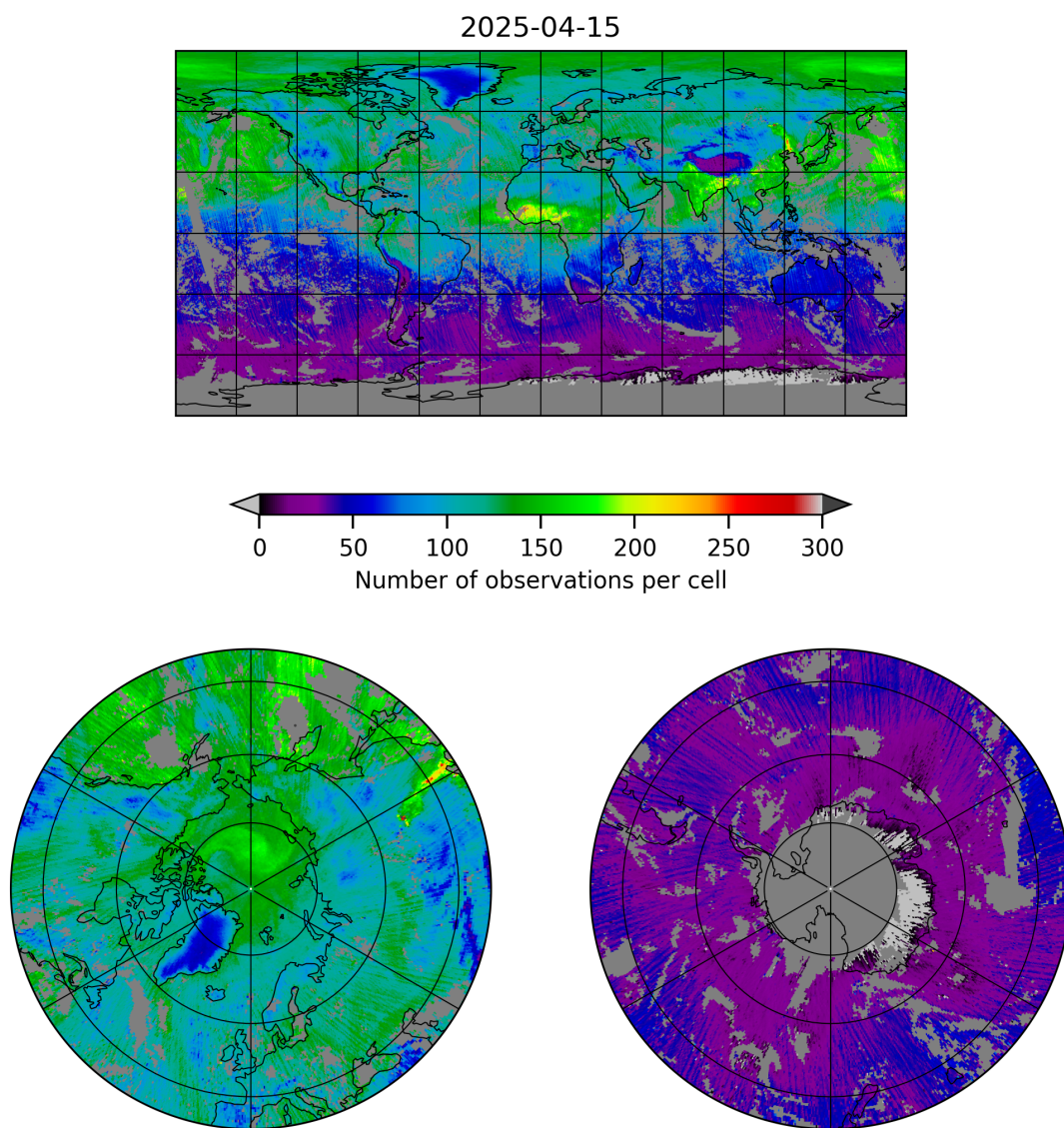
Figure 5: Map of the number of observations for 2025-04-15 to 2025-04-16
