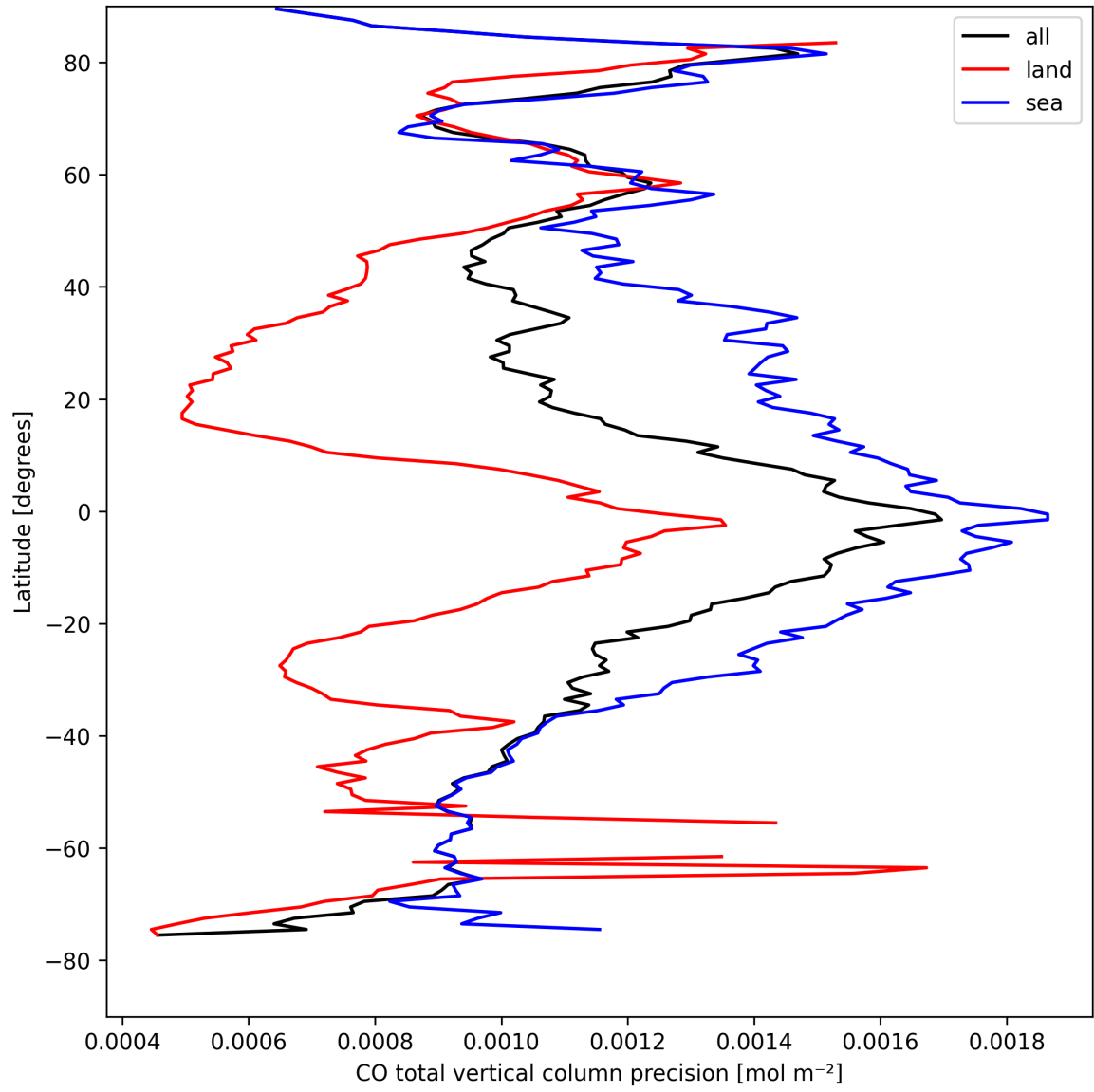
Figure 8: Zonal average of “CO total vertical column precision” for 2025-04-15 to 2025-04-16.
