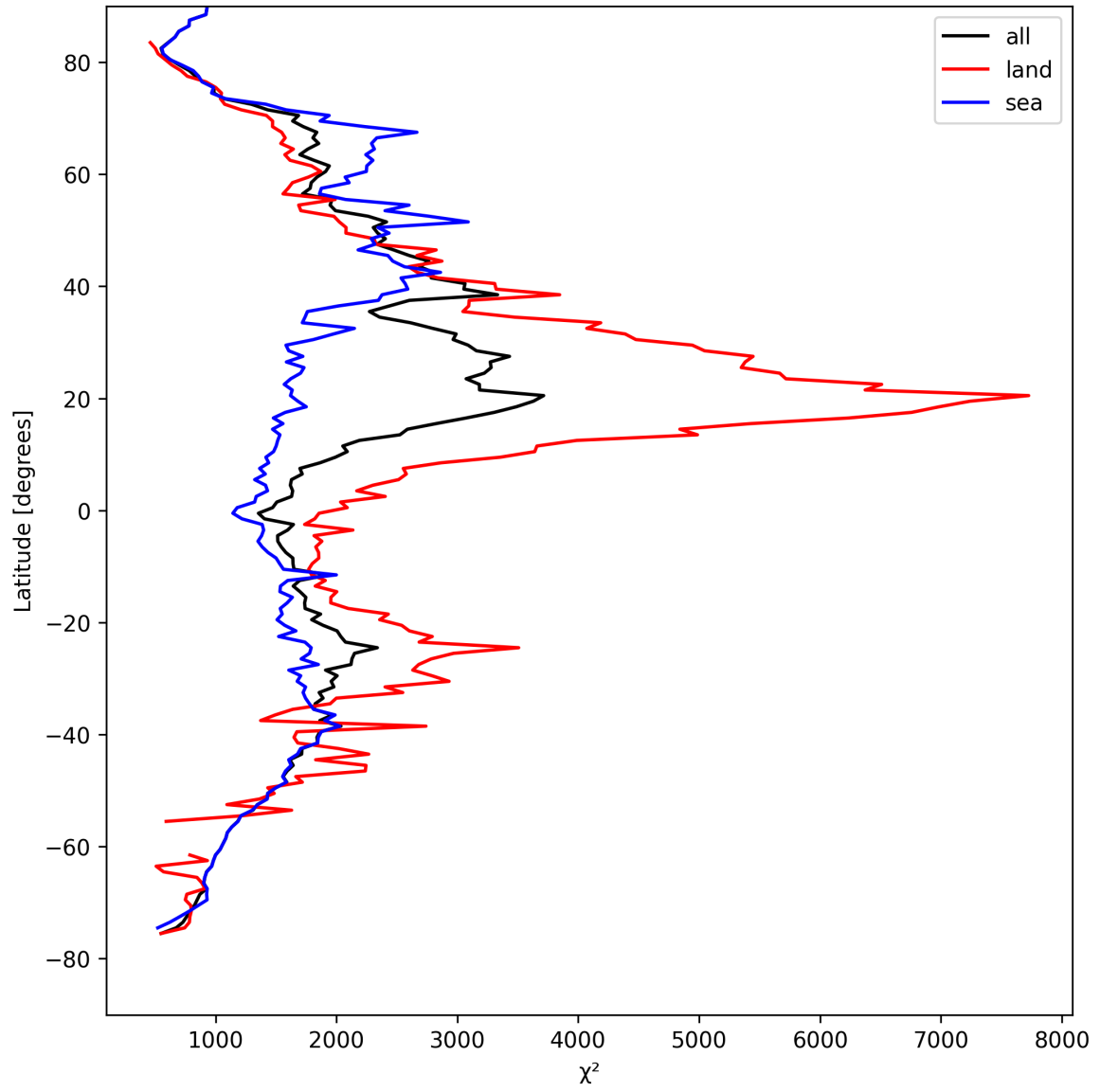
Figure 10: Zonal average of “ \chi^2 ” for 2025-04-15 to 2025-04-16.
