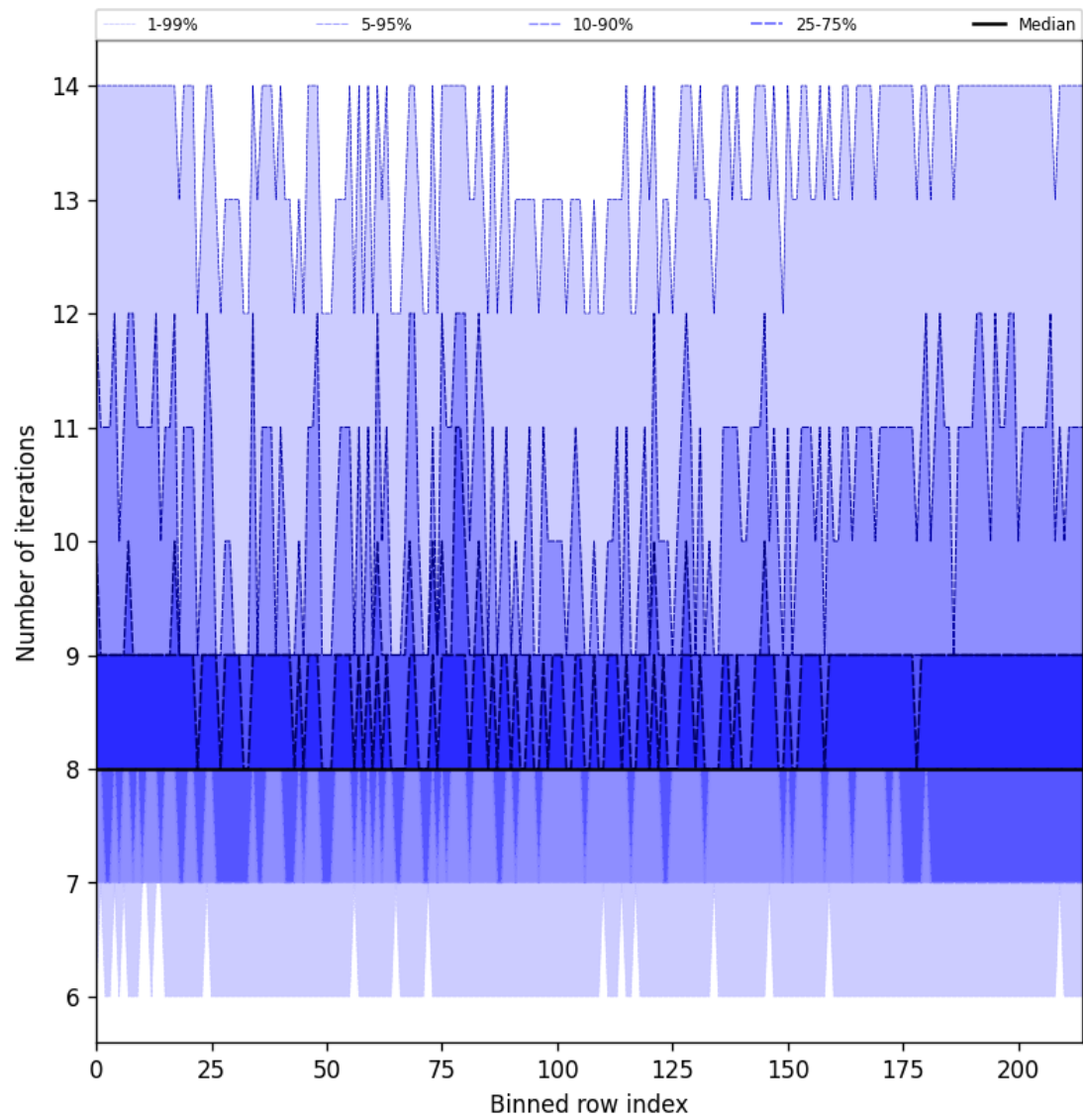
Figure 26: Along track statistics of “Number of iterations” for 2025-04-15 to 2025-04-16
