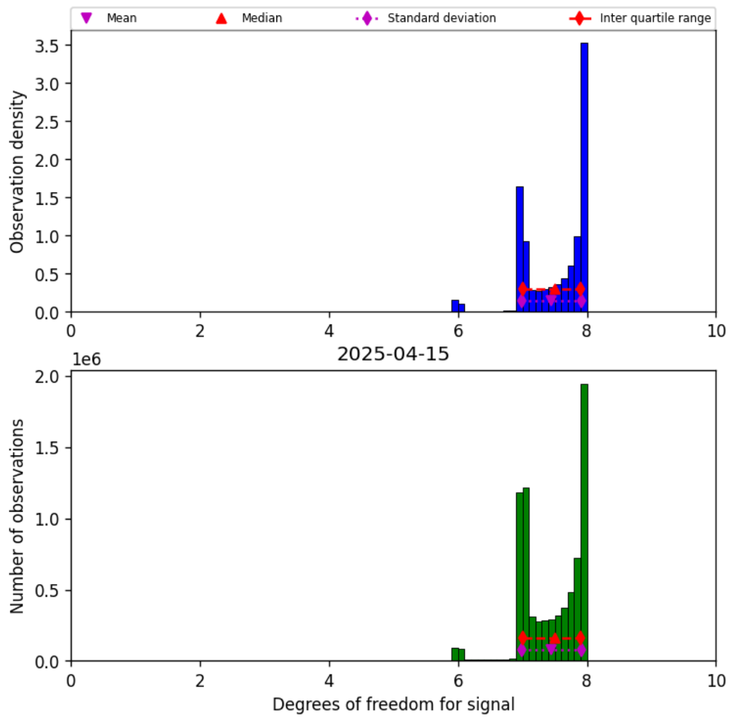
Figure 18: Histogram of “Degrees of freedom for signal” for 2025-04-15 to 2025-04-16
