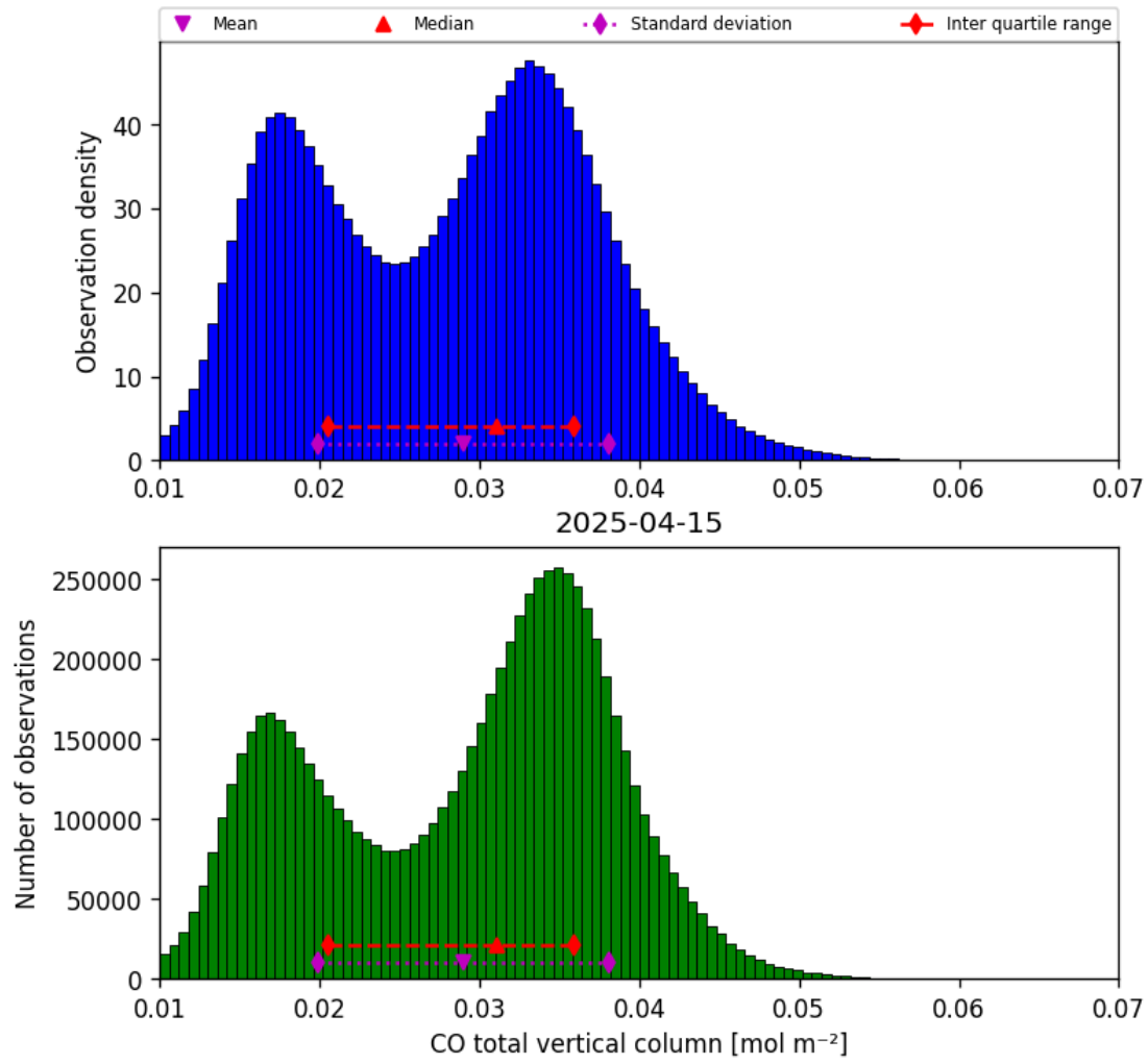
Figure 14: Histogram of “CO total vertical column” for 2025-04-15 to 2025-04-16
