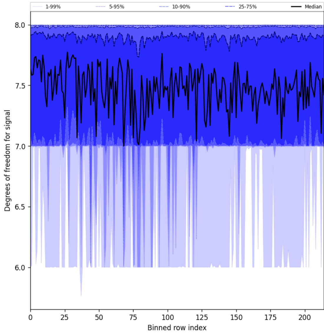
Figure 25: Along track statistics of “Degrees of freedom for signal” for 2025-04-15 to 2025-04-16
