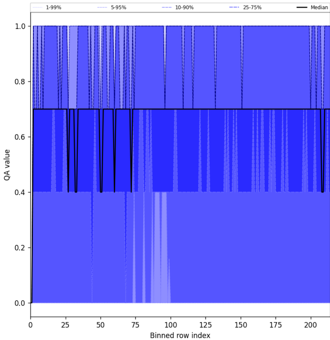
Figure 20: Along track statistics of “QA value” for 2025-04-15 to 2025-04-16
