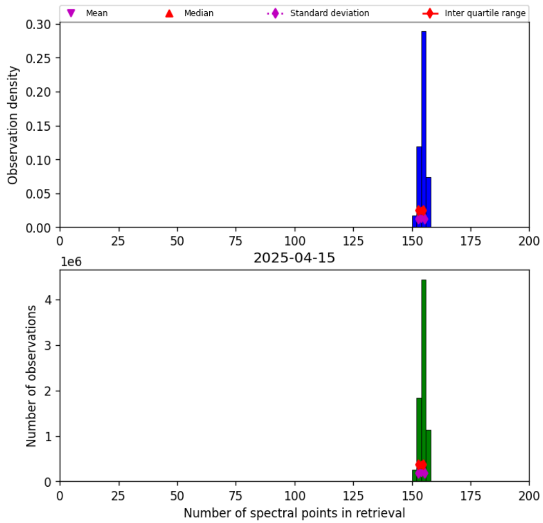
Figure 16: Histogram of “Number of spectral points in retrieval” for 2025-04-15 to 2025-04-16
