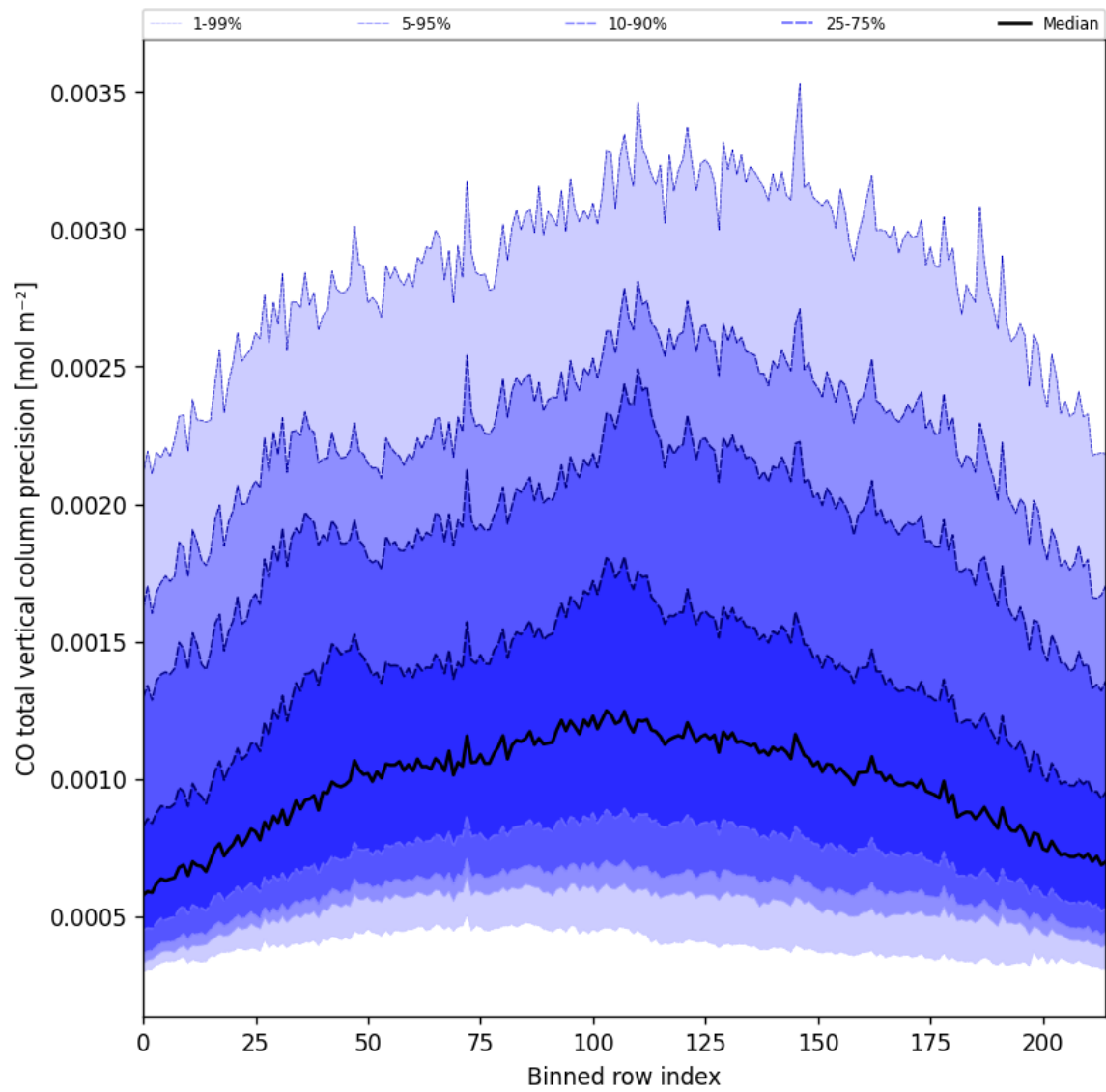
Figure 22: Along track statistics of “CO total vertical column precision” for 2025-04-15 to 2025-04-16
