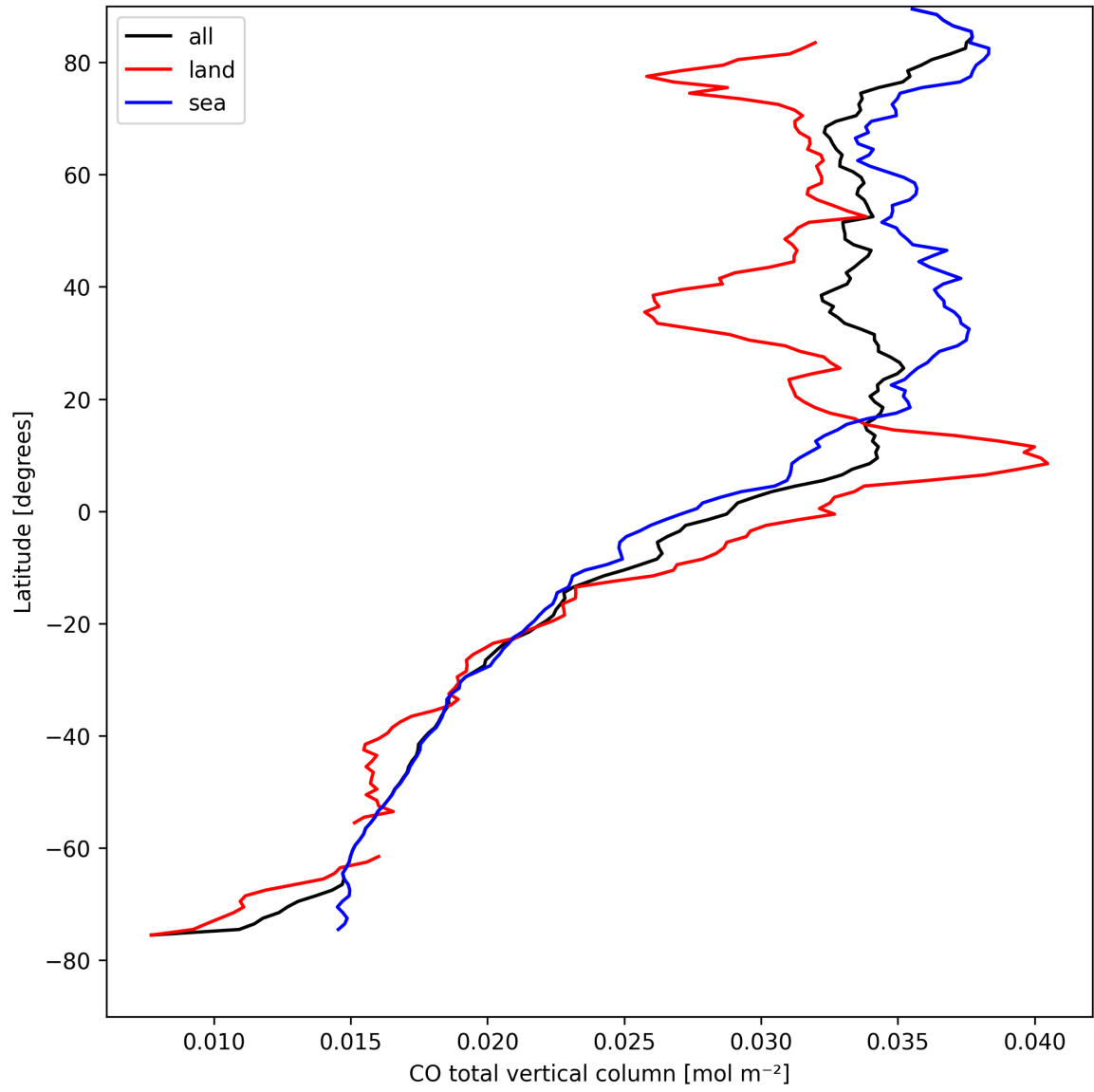
Figure 7: Zonal average of “CO total vertical column” for 2025-04-15 to 2025-04-16.
