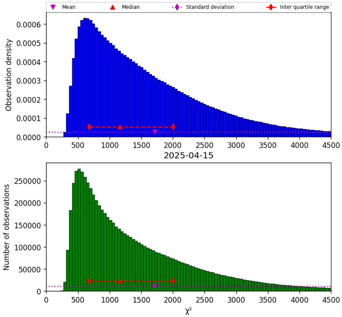
Figure 17: Histogram of “ \chi^2 ” for 2025-04-15 to 2025-04-16
