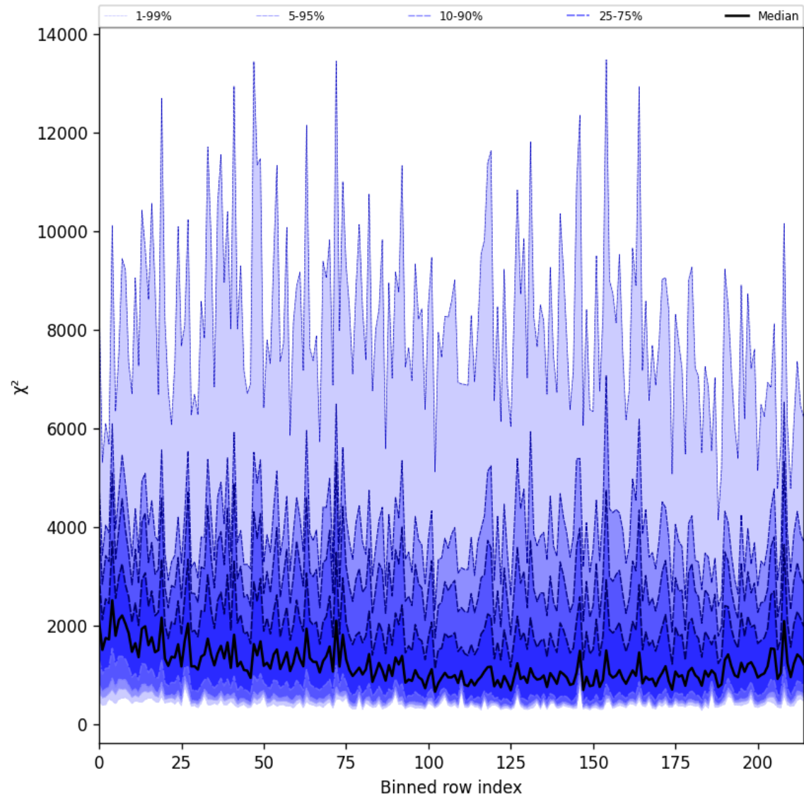
Figure 24: Along track statistics of “ \chi^2 ” for 2025-04-15 to 2025-04-16
