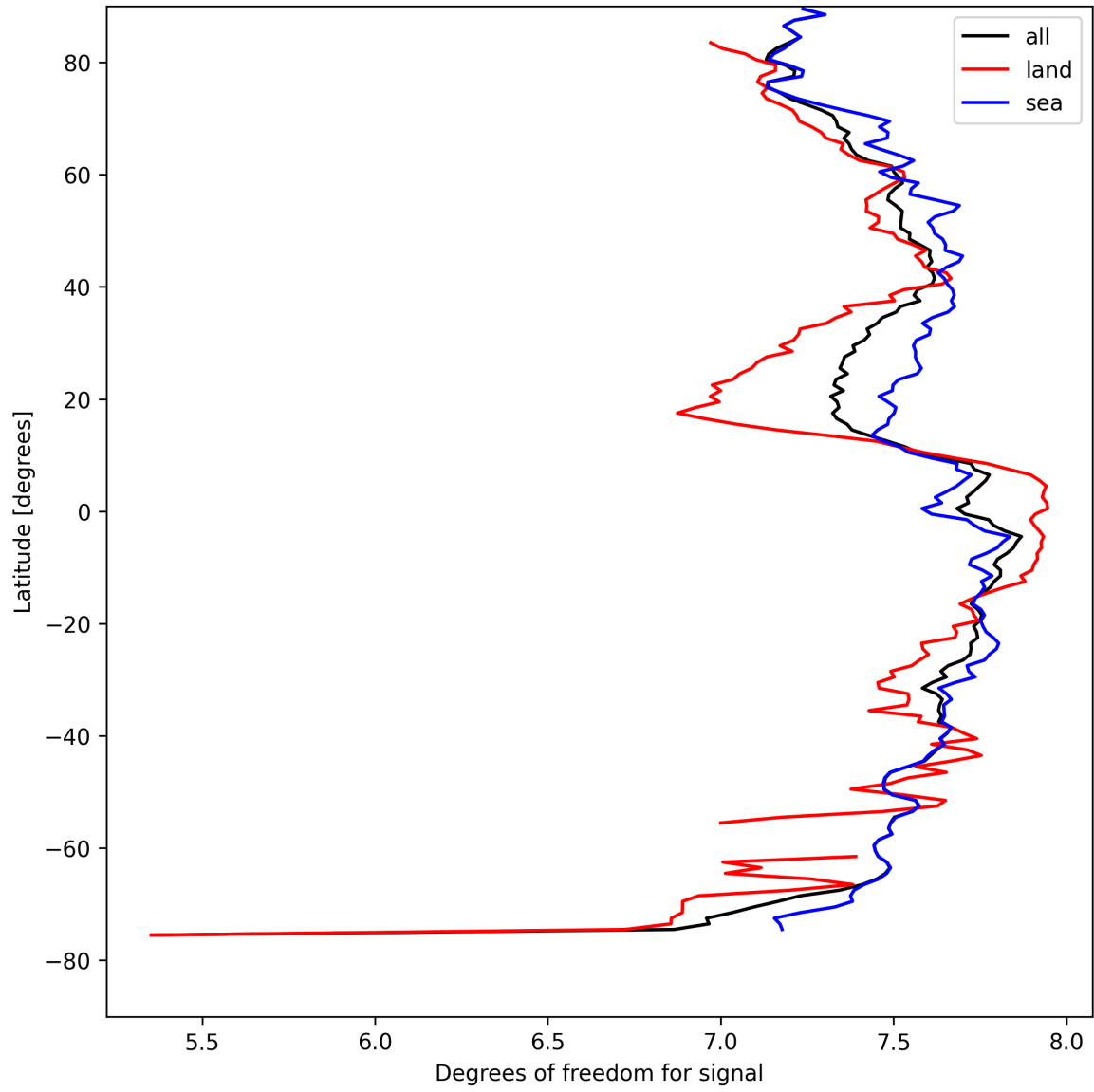
Figure 11: Zonal average of “Degrees of freedom for signal” for 2025-04-15 to 2025-04-16.
