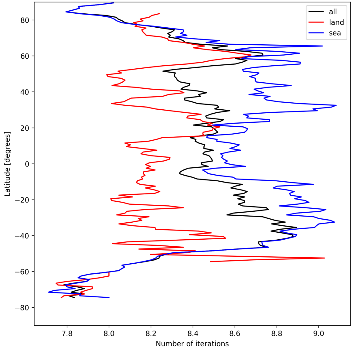
Figure 12: Zonal average of “Number of iterations” for 2025-04-16 to 2025-04-16.
