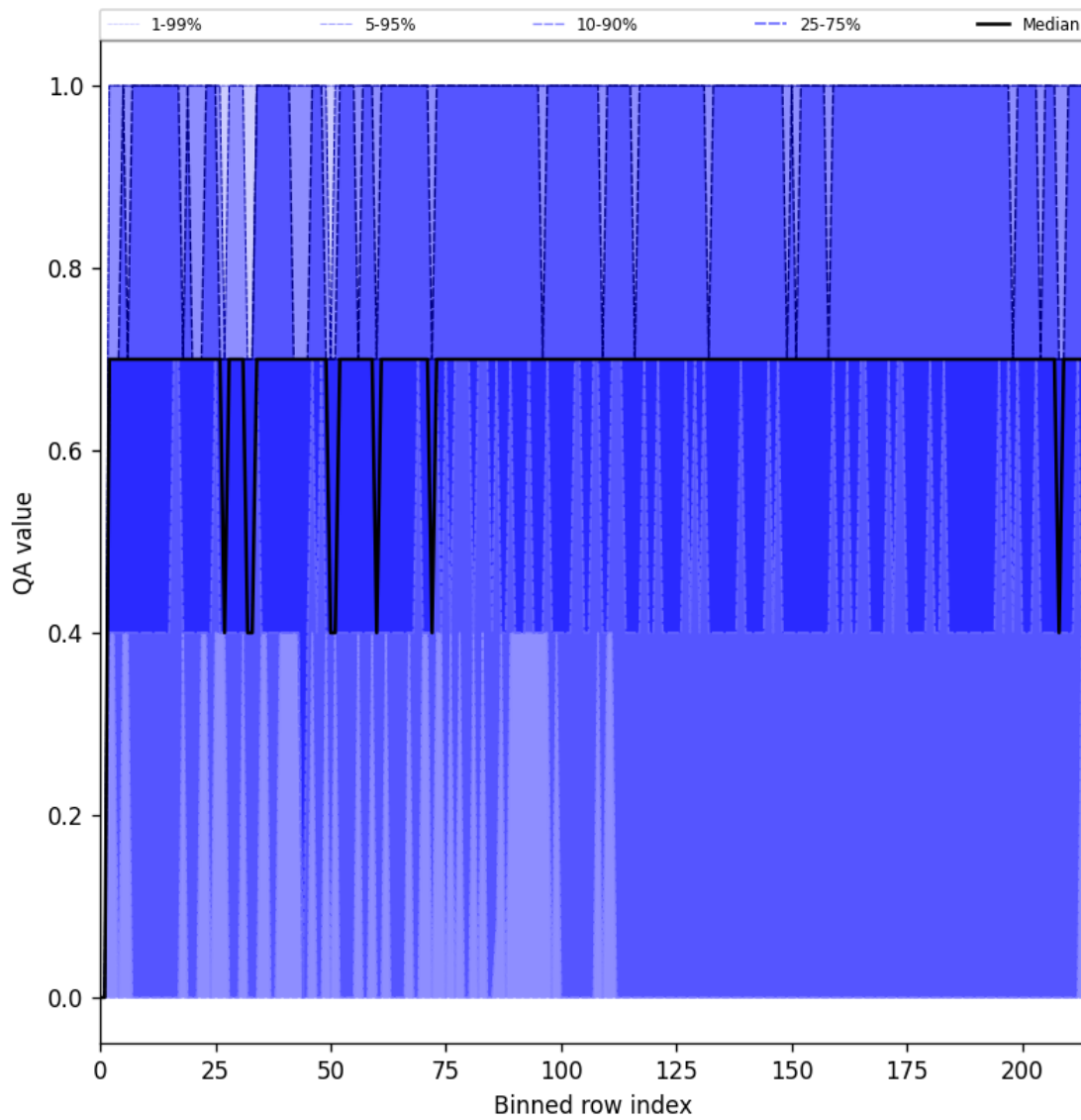
Figure 20: Along track statistics of “QA value” for 2025-04-16 to 2025-04-16
