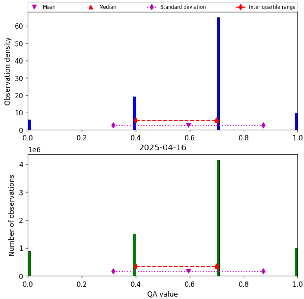
Figure 13: Histogram of “QA value” for 2025-04-16 to 2025-04-16
