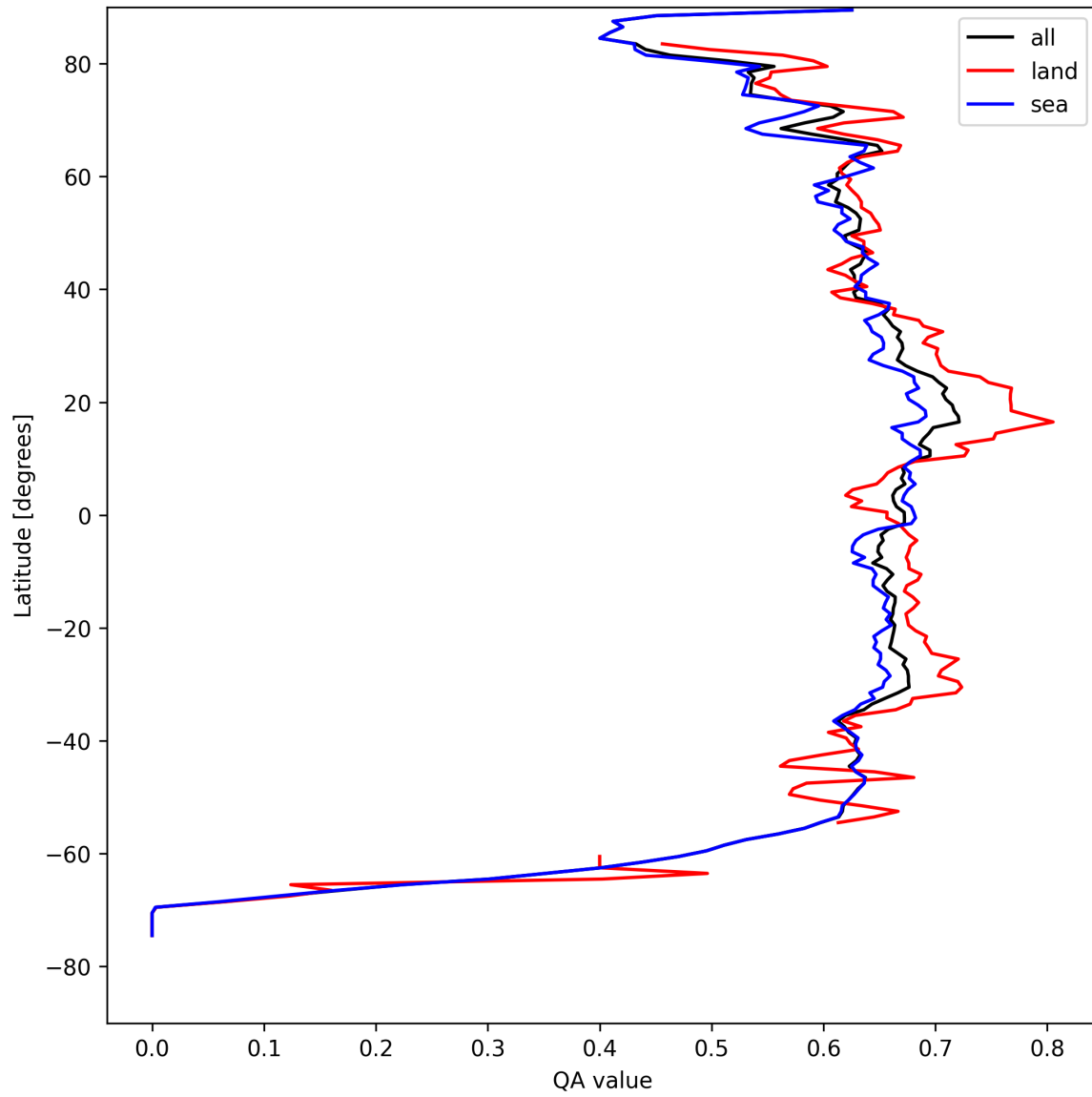
Figure 6: Zonal average of “QA value” for 2025-04-16 to 2025-04-16.
