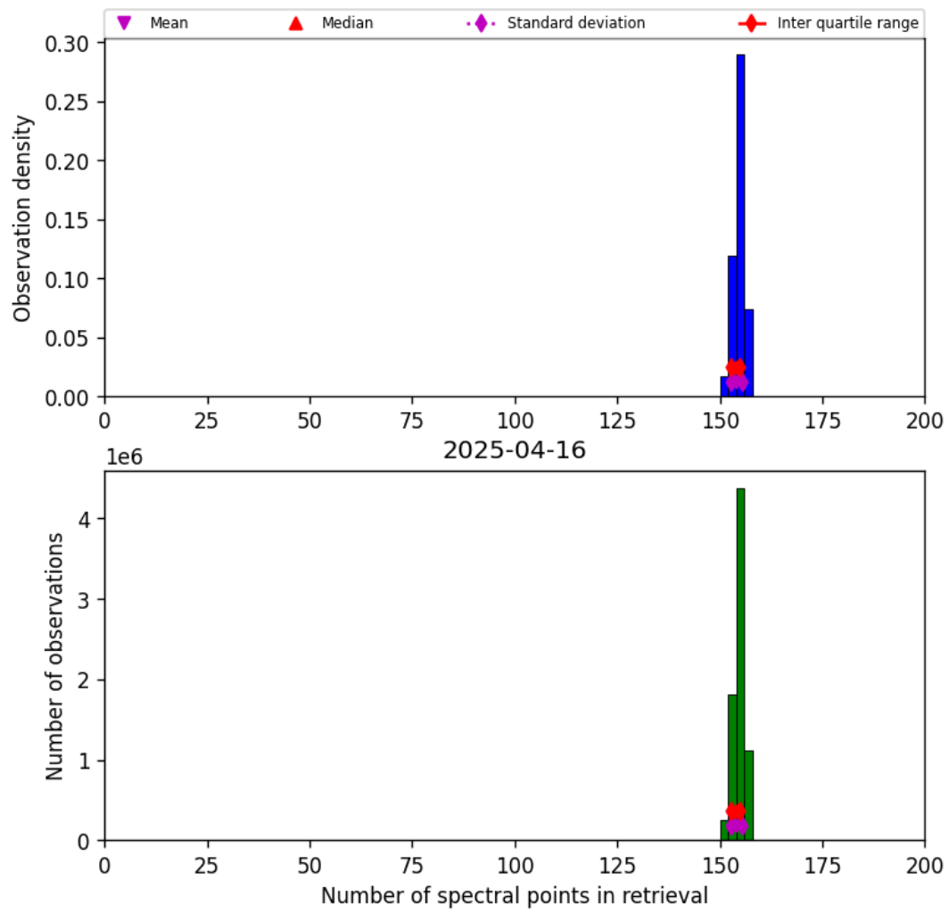
Figure 16: Histogram of “Number of spectral points in retrieval” for 2025-04-16 to 2025-04-16
