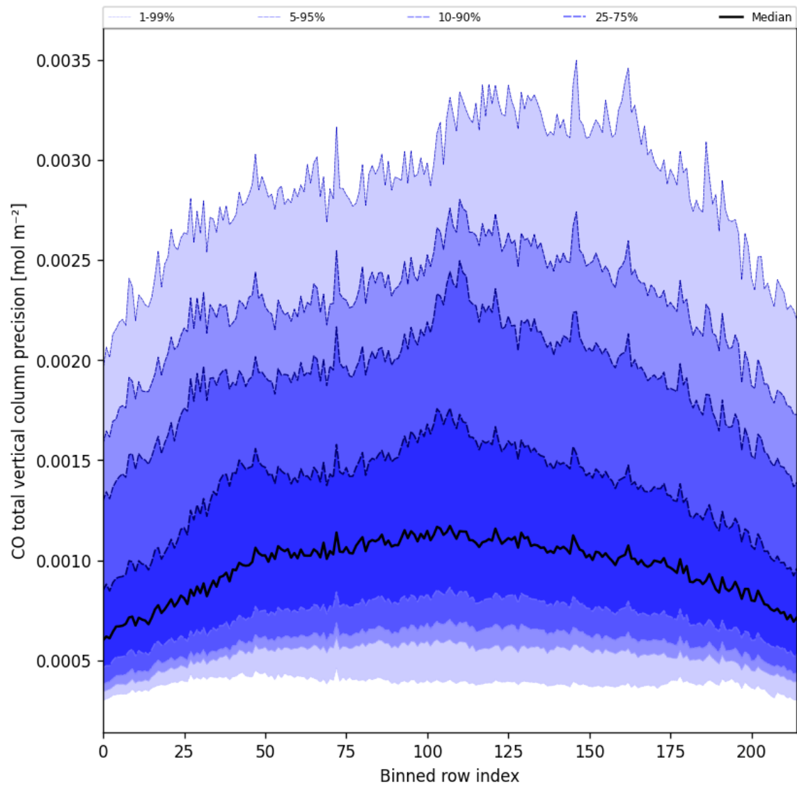
Figure 22: Along track statistics of “CO total vertical column precision” for 2025-04-16 to 2025-04-16
