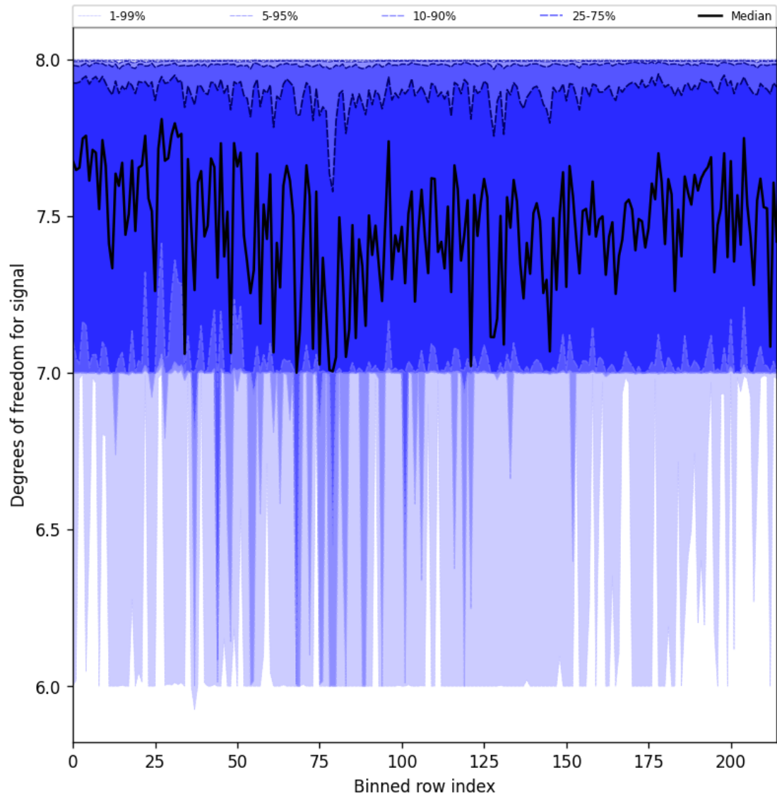
Figure 25: Along track statistics of “Degrees of freedom for signal” for 2025-04-16 to 2025-04-16
