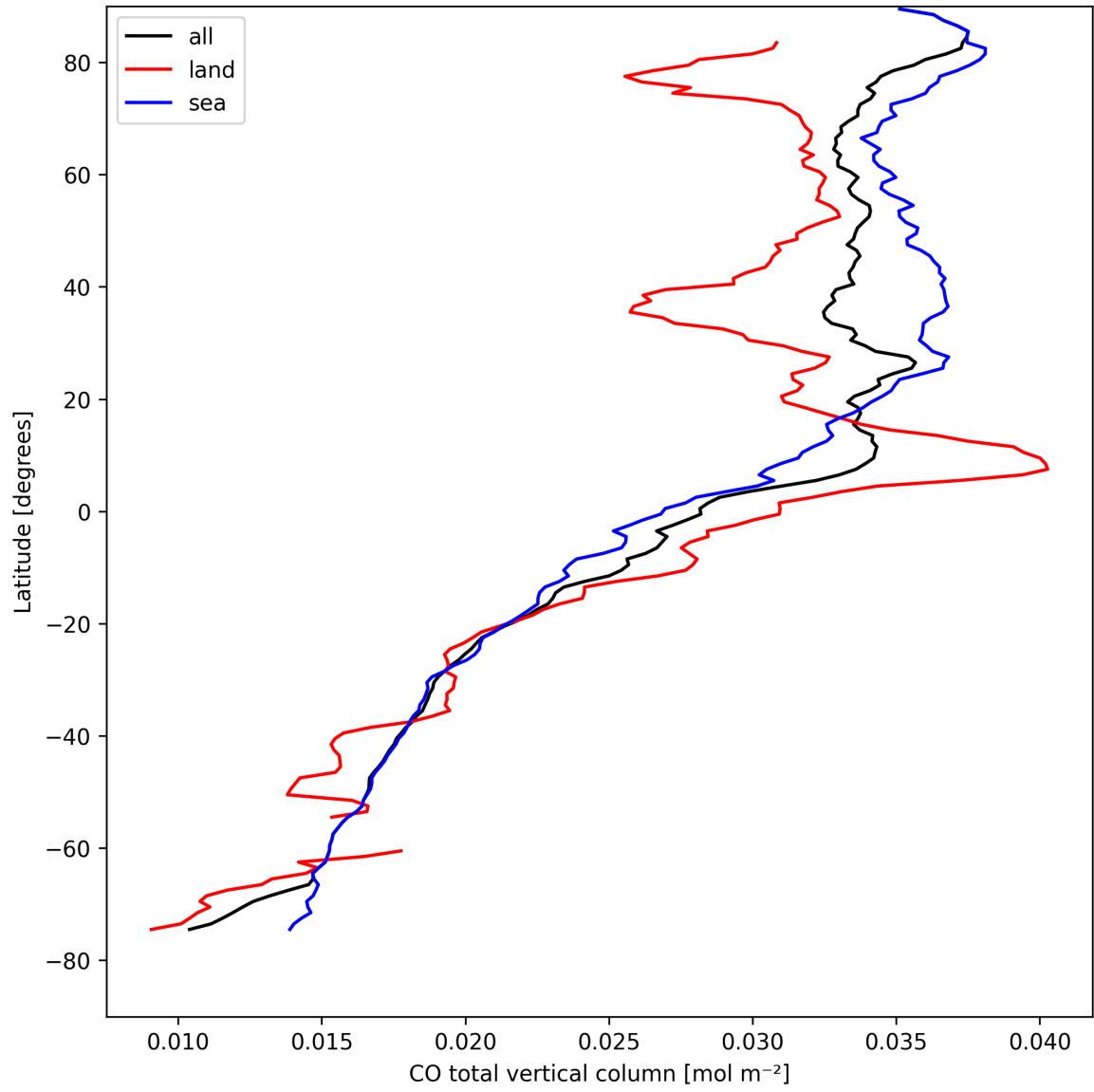
Figure 7: Zonal average of “CO total vertical column” for 2025-04-16 to 2025-04-16.
