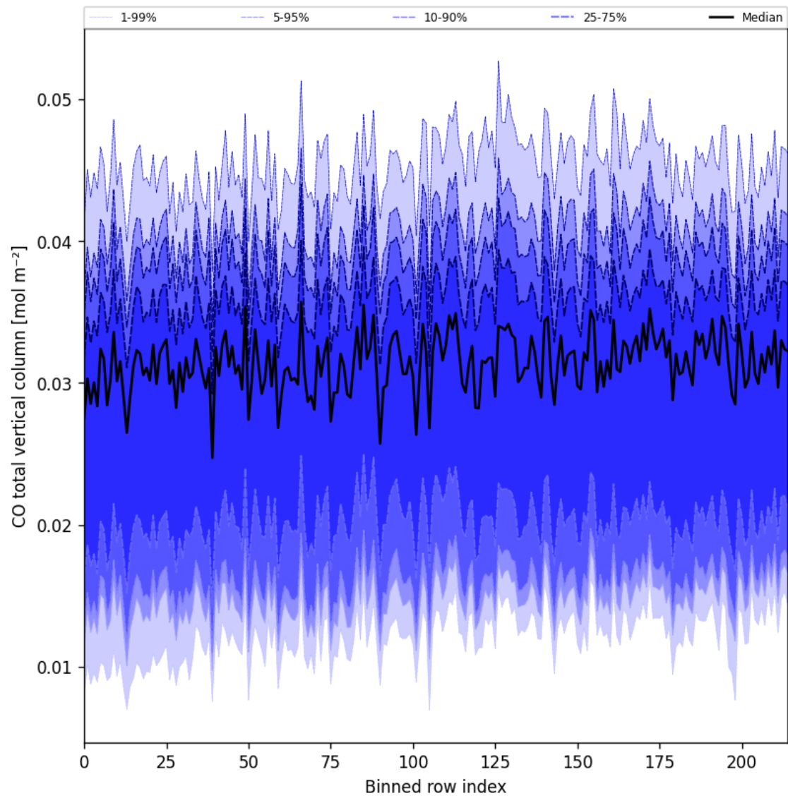
Figure 21: Along track statistics of “CO total vertical column” for 2025-04-16 to 2025-04-16
