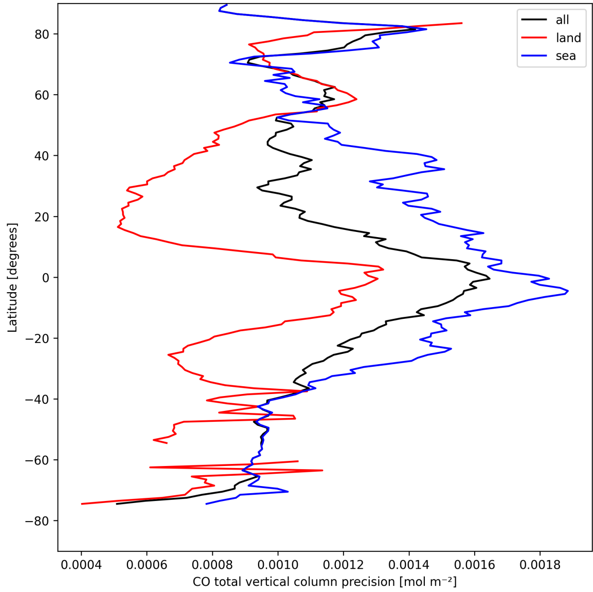
Figure 8: Zonal average of “CO total vertical column precision” for 2025-04-16 to 2025-04-16.
