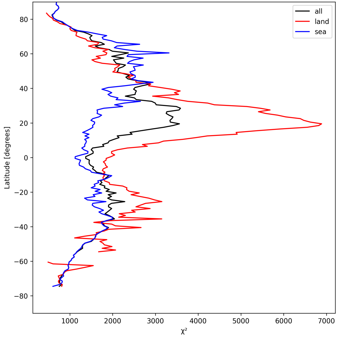
Figure 10: Zonal average of “ \chi^2 ” for 2025-04-16 to 2025-04-16.
