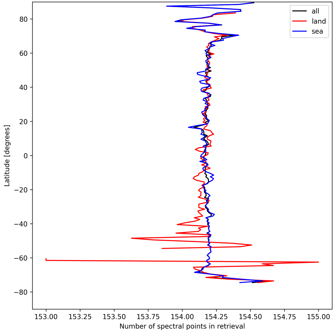
Figure 9: Zonal average of “Number of spectral points in retrieval” for 2025-04-16 to 2025-04-16.
