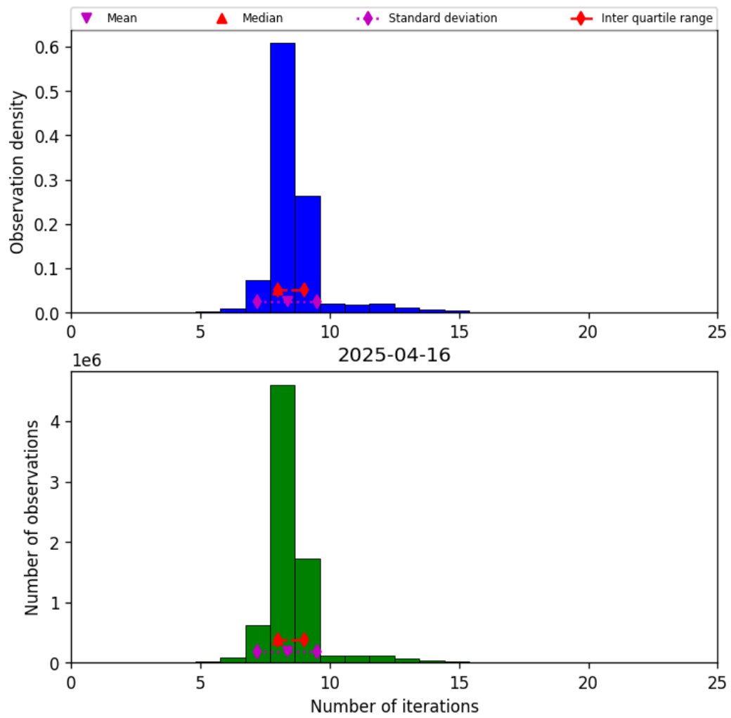
Figure 19: Histogram of “Number of iterations” for 2025-04-16 to 2025-04-16
