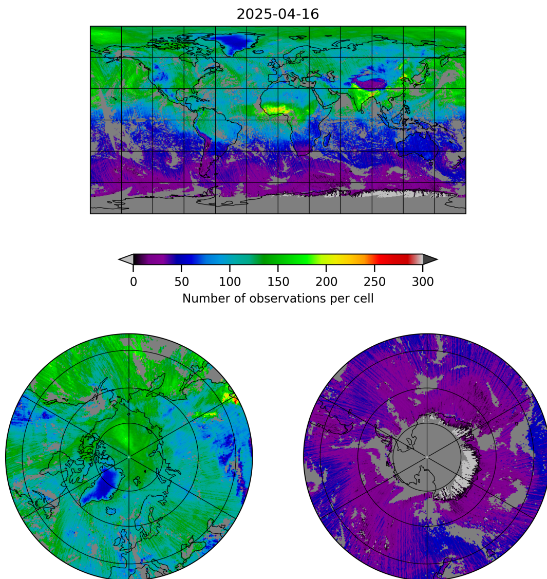
Figure 5: Map of the number of observations for 2025-04-16 to 2025-04-16
