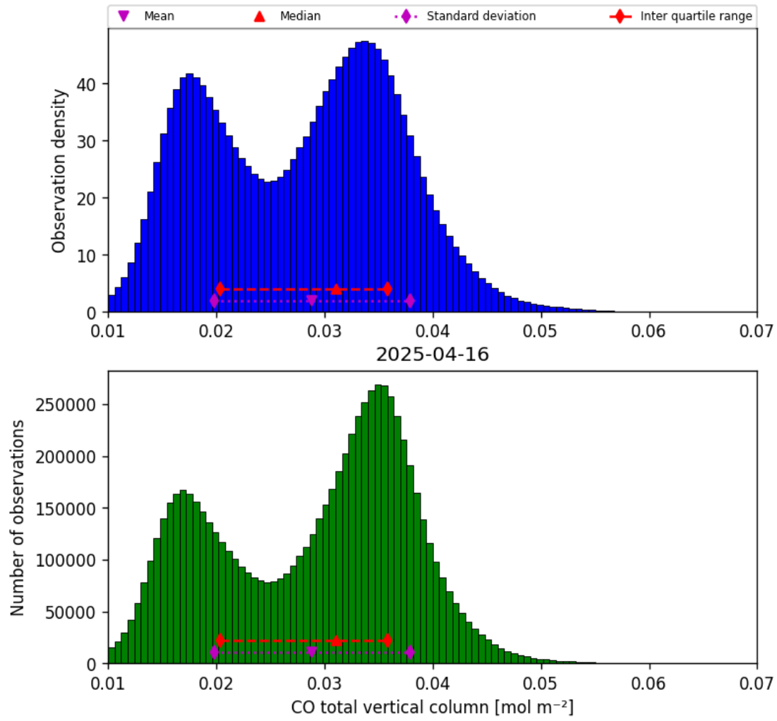
Figure 14: Histogram of “CO total vertical column” for 2025-04-16 to 2025-04-16
