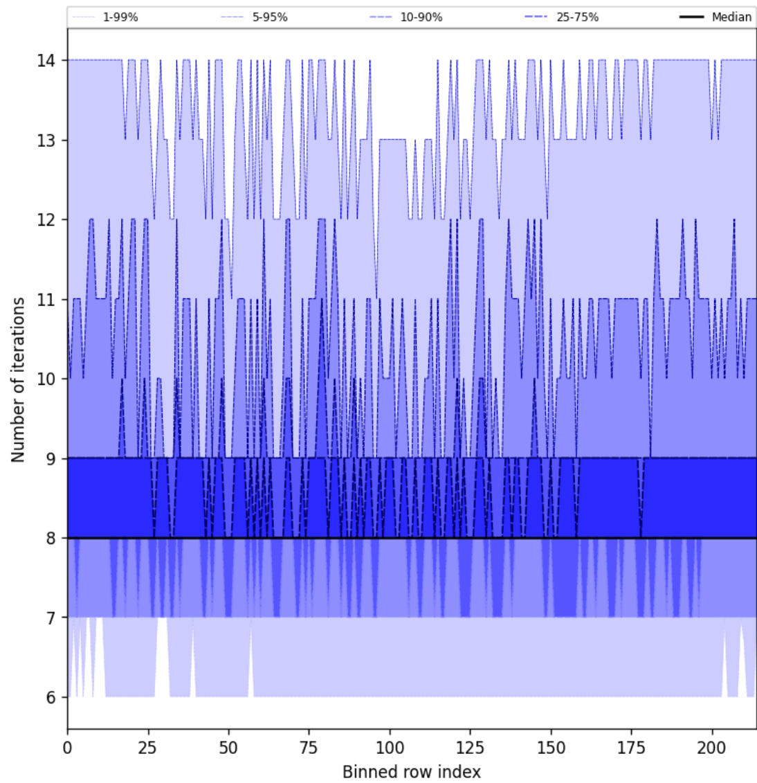
Figure 26: Along track statistics of “Number of iterations” for 2025-04-16 to 2025-04-16
