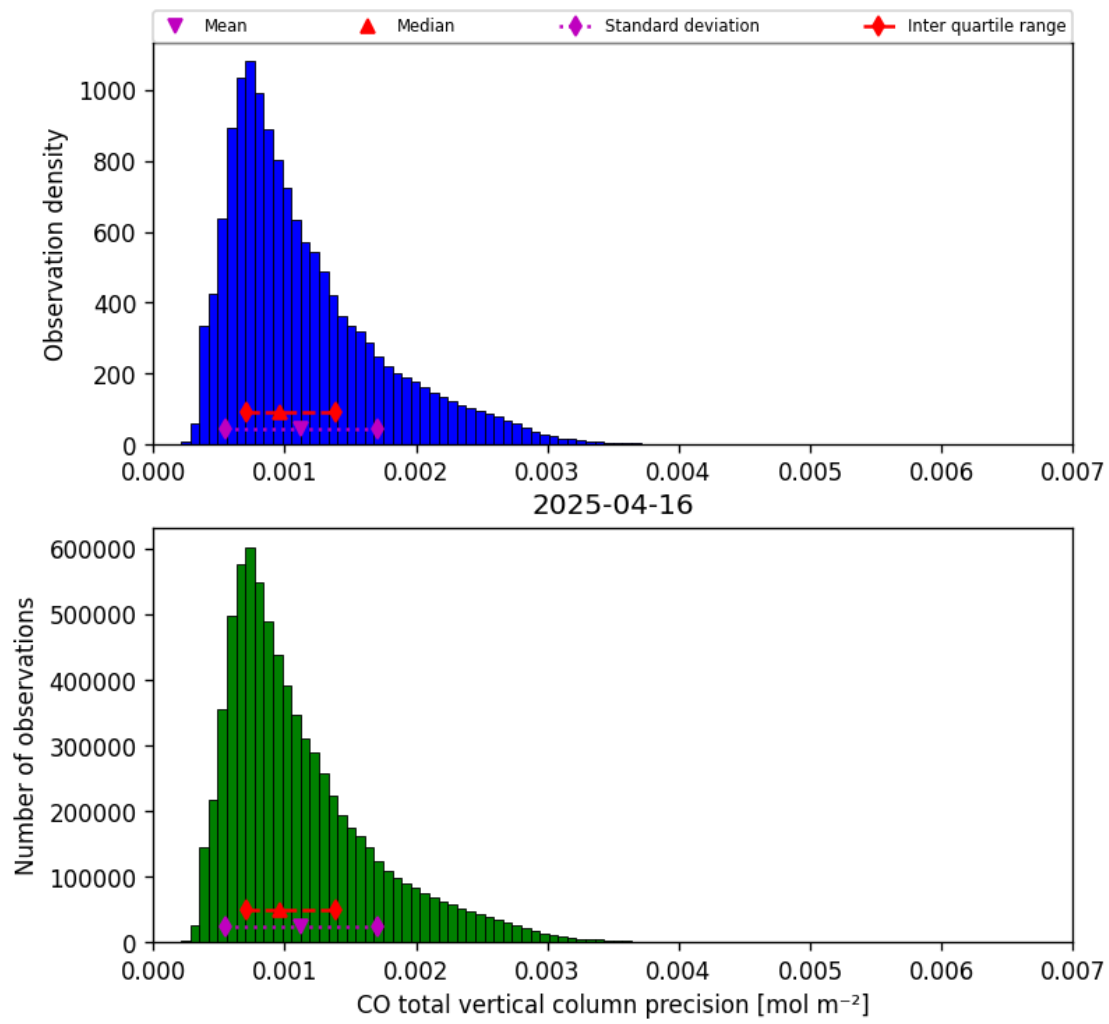
Figure 15: Histogram of “CO total vertical column precision” for 2025-04-16 to 2025-04-16
