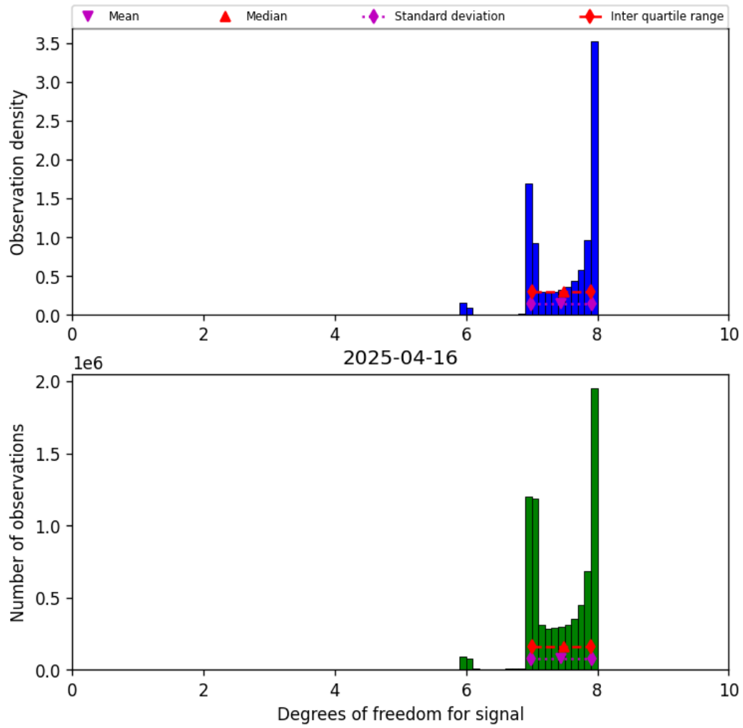
Figure 18: Histogram of “Degrees of freedom for signal” for 2025-04-16 to 2025-04-16
