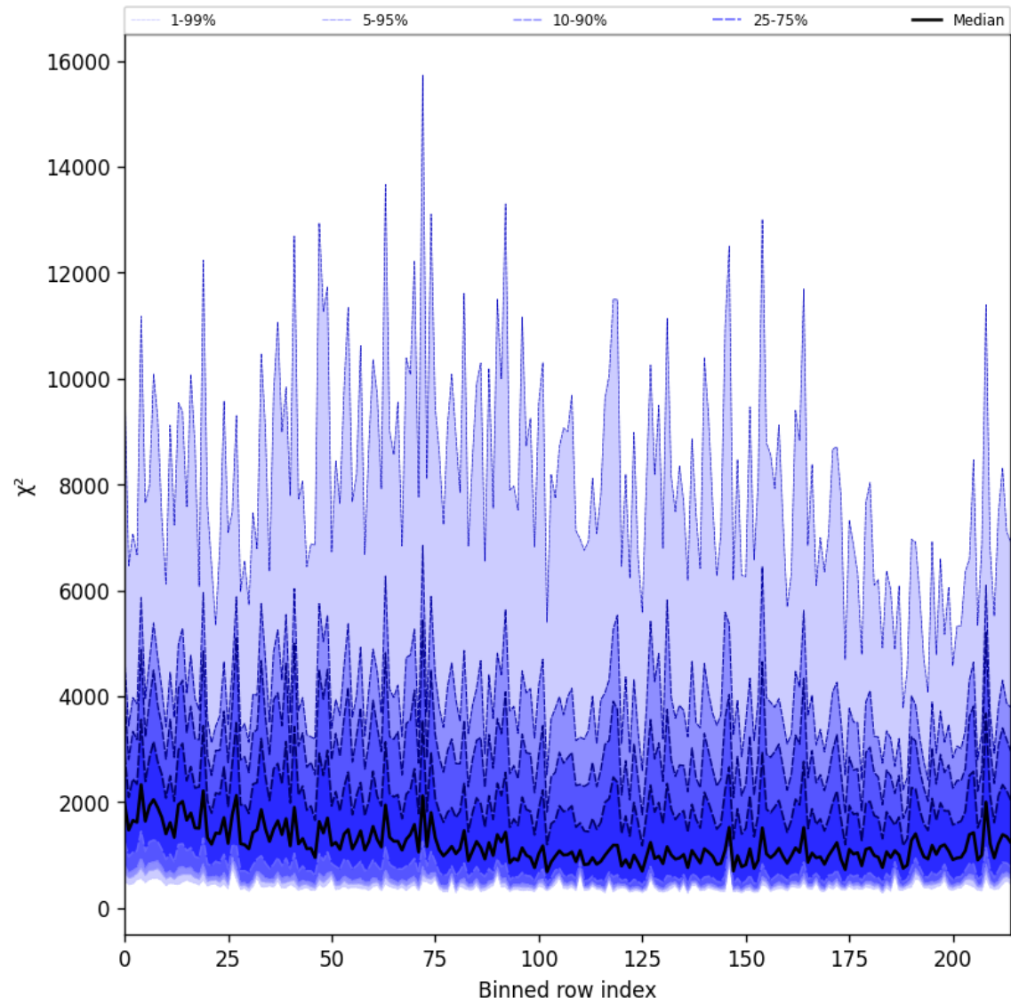
Figure 24: Along track statistics of “ \chi^2 ” for 2025-04-16 to 2025-04-16
