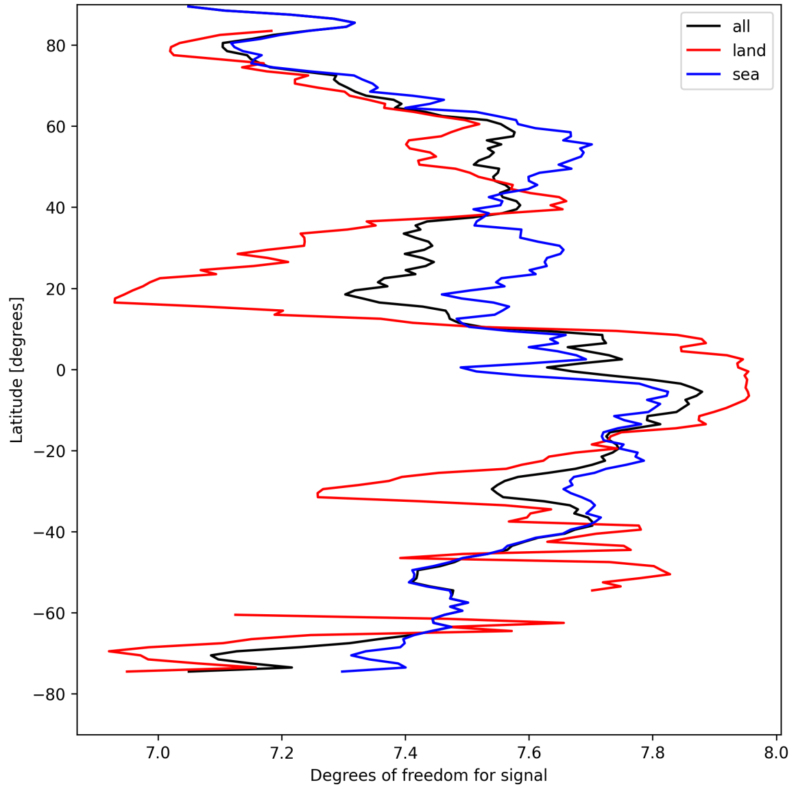
Figure 11: Zonal average of “Degrees of freedom for signal” for 2025-04-16 to 2025-04-16.
