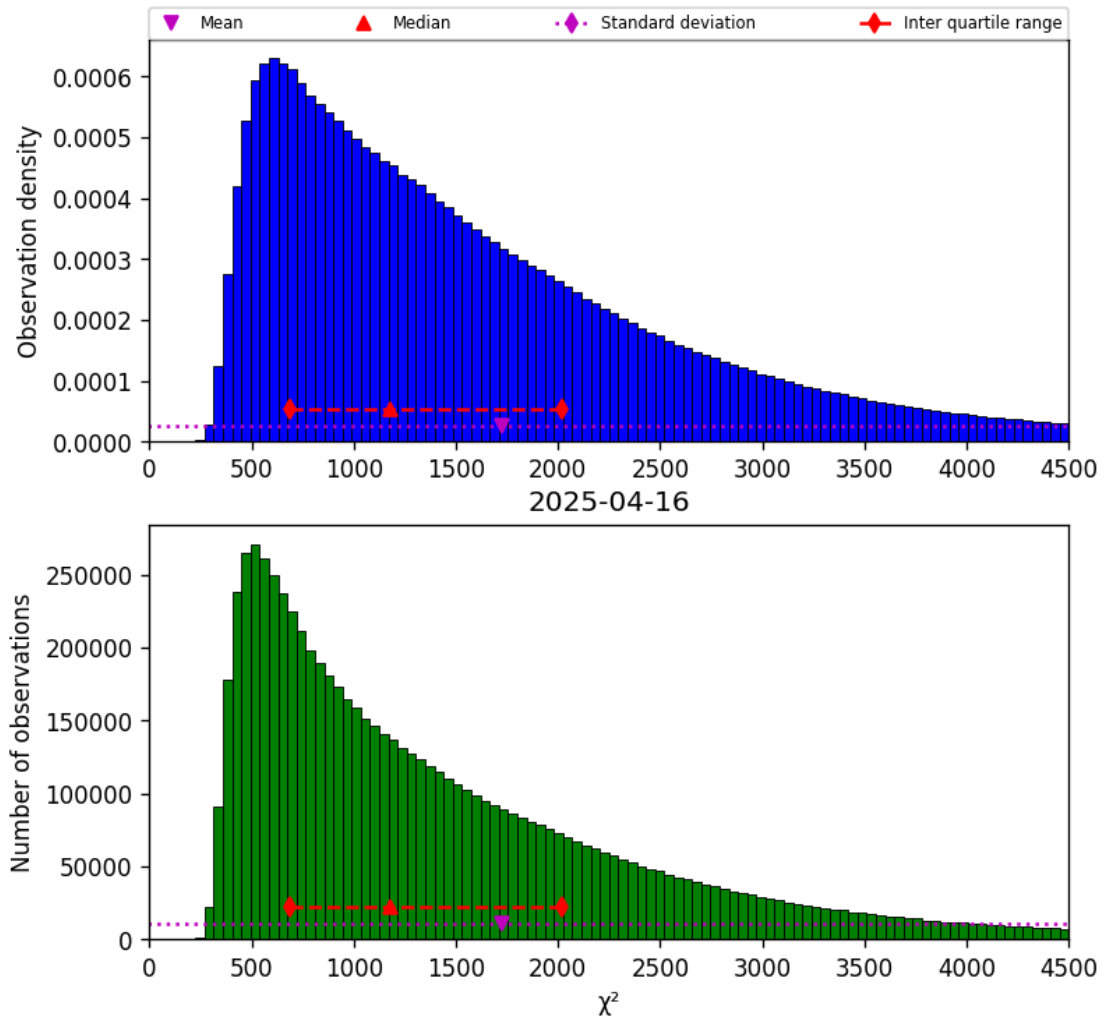
Figure 17: Histogram of " \chi^2 " for 2025-04-16 to 2025-04-16
