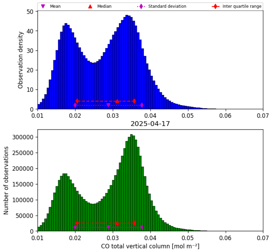
Figure 14: Histogram of “CO total vertical column” for 2025-04-17 to 2025-04-18
