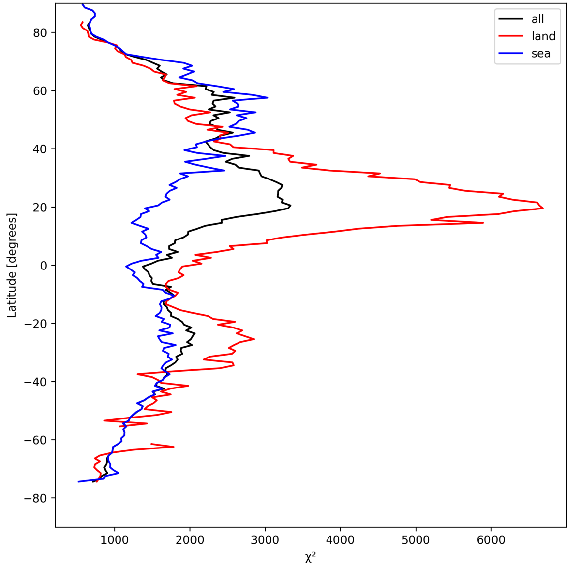
Figure 10: Zonal average of “ \chi^2 ” for 2025-04-17 to 2025-04-18.
