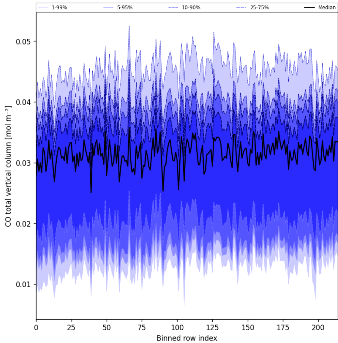
Figure 21: Along track statistics of “CO total vertical column” for 2025-04-17 to 2025-04-18
