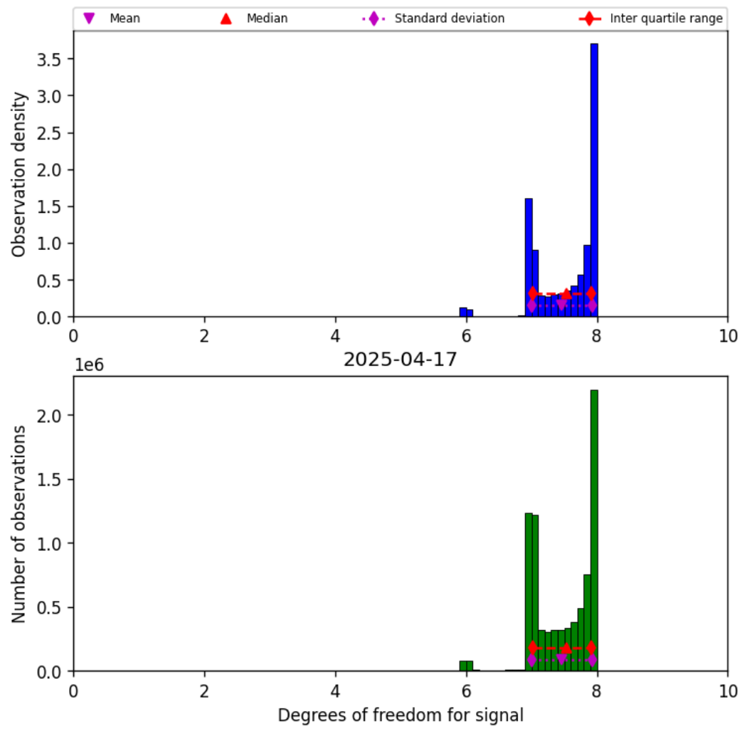
Figure 18: Histogram of “Degrees of freedom for signal” for 2025-04-17 to 2025-04-18
