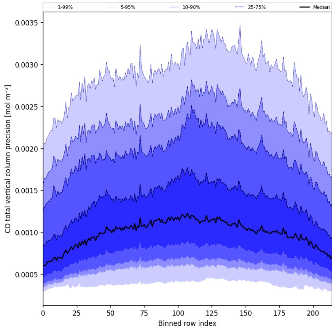
Figure 22: Along track statistics of “CO total vertical column precision” for 2025-04-17 to 2025-04-18
