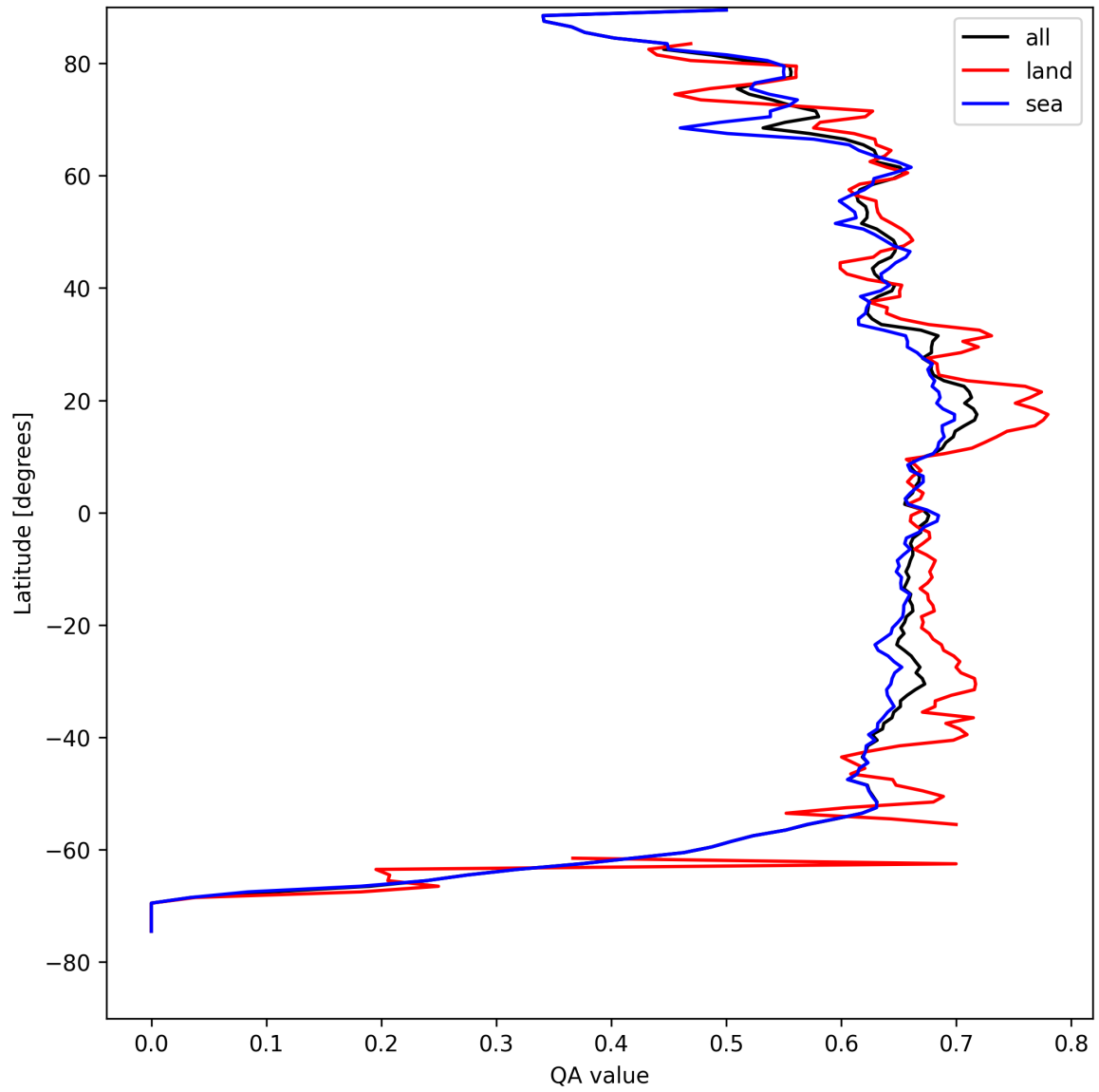
Figure 6: Zonal average of “QA value” for 2025-04-17 to 2025-04-18.
