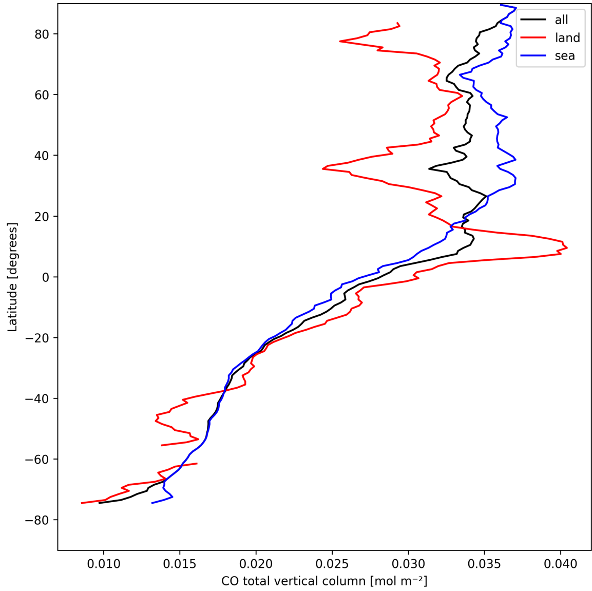
Figure 7: Zonal average of “CO total vertical column” for 2025-04-17 to 2025-04-18.
