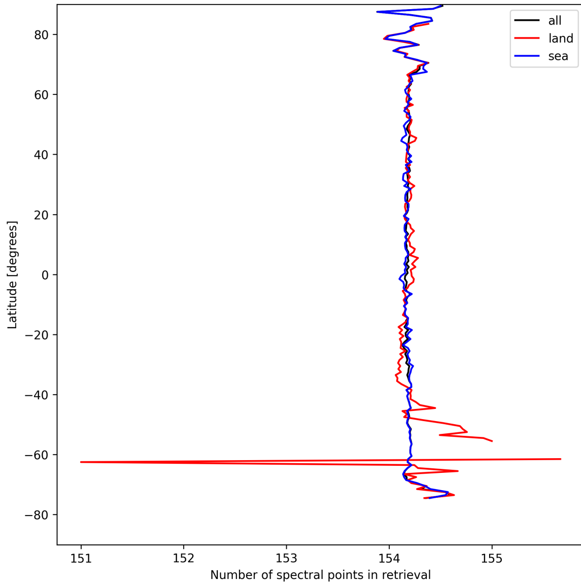
Figure 9: Zonal average of “Number of spectral points in retrieval” for 2025-04-17 to 2025-04-18.
