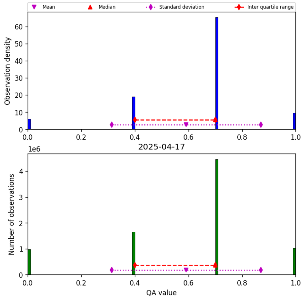
Figure 13: Histogram of “QA value” for 2025-04-17 to 2025-04-18
