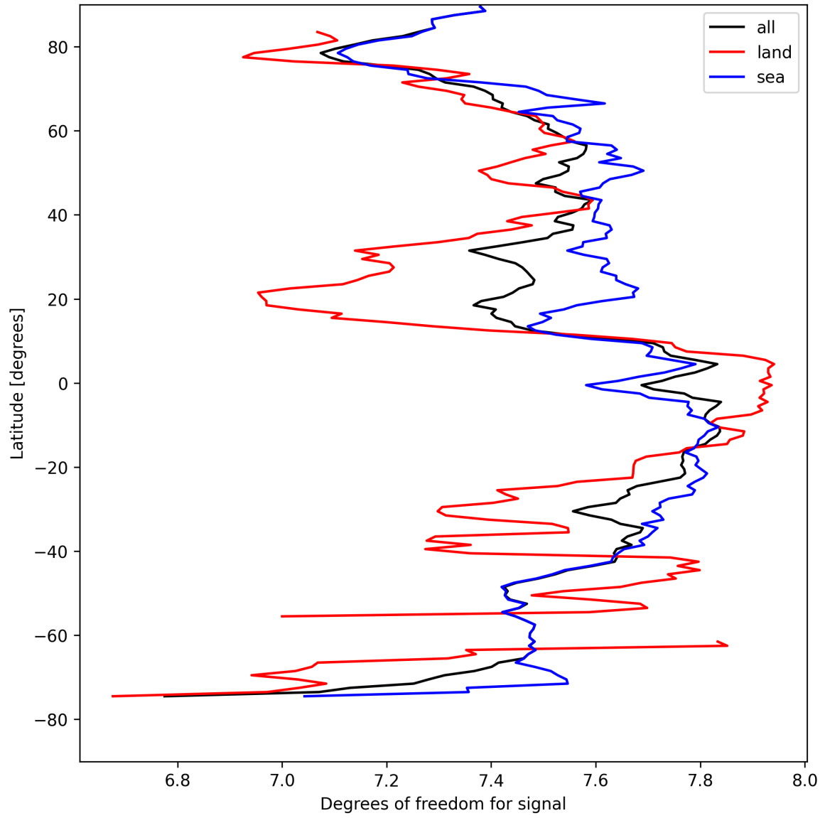
Figure 11: Zonal average of “Degrees of freedom for signal” for 2025-04-17 to 2025-04-18.
