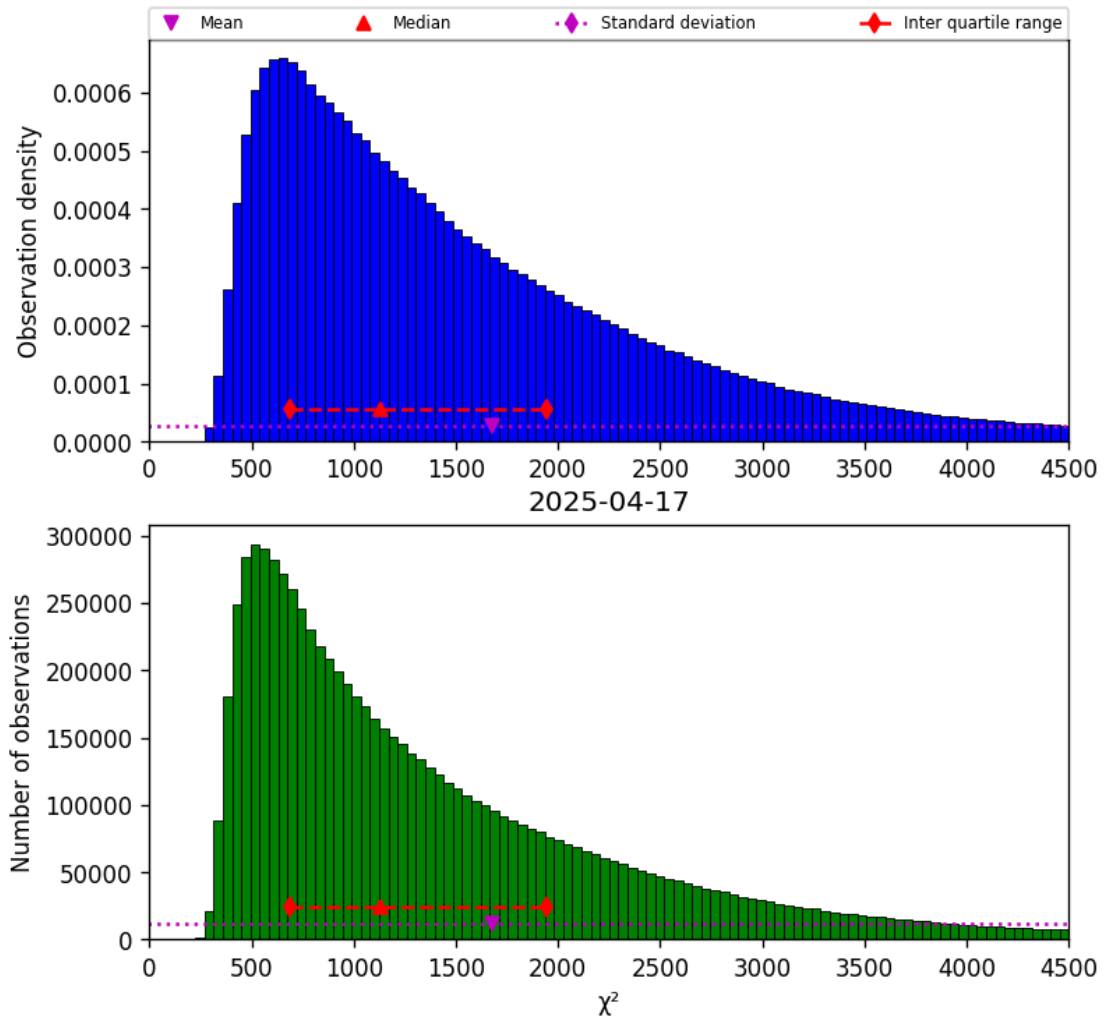
Figure 17: Histogram of “ \chi^2 ” for 2025-04-17 to 2025-04-18
