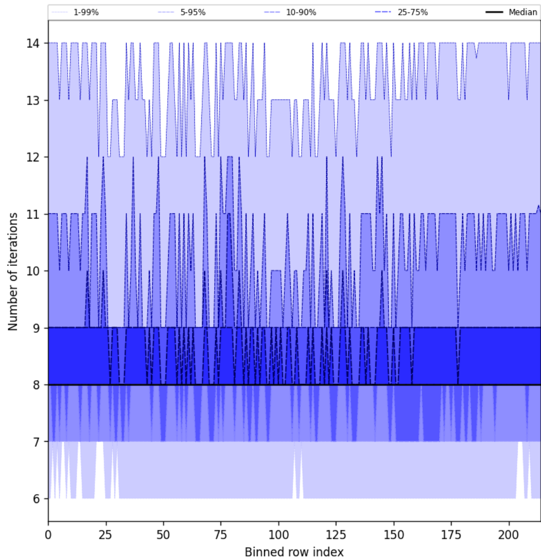
Figure 26: Along track statistics of “Number of iterations” for 2025-04-17 to 2025-04-18
