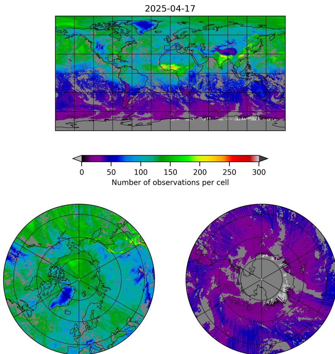
Figure 5: Map of the number of observations for 2025-04-17 to 2025-04-18
