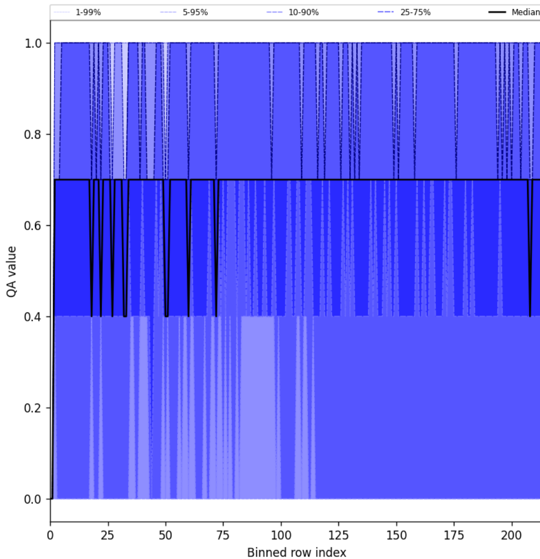
Figure 20: Along track statistics of “QA value” for 2025-04-17 to 2025-04-18
