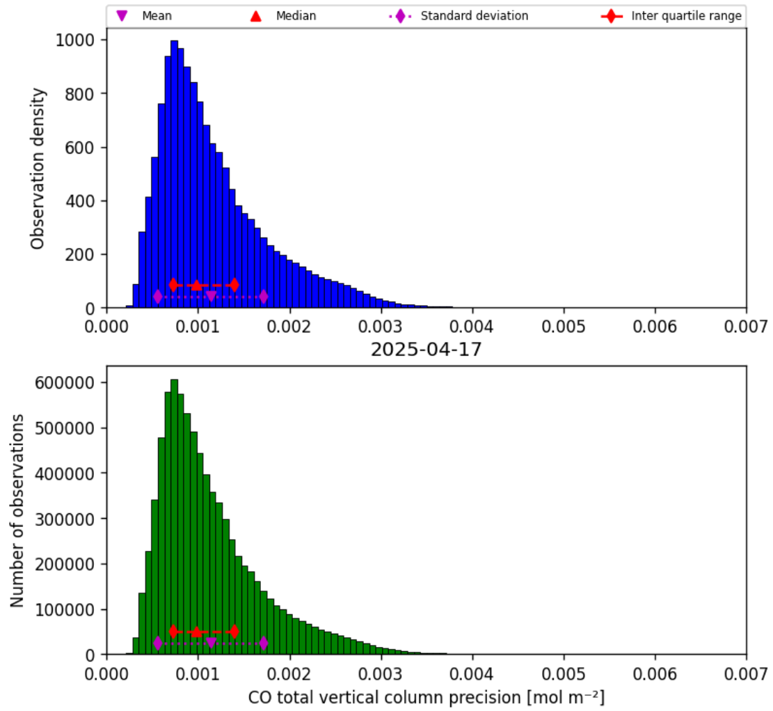
Figure 15: Histogram of “CO total vertical column precision” for 2025-04-17 to 2025-04-18
