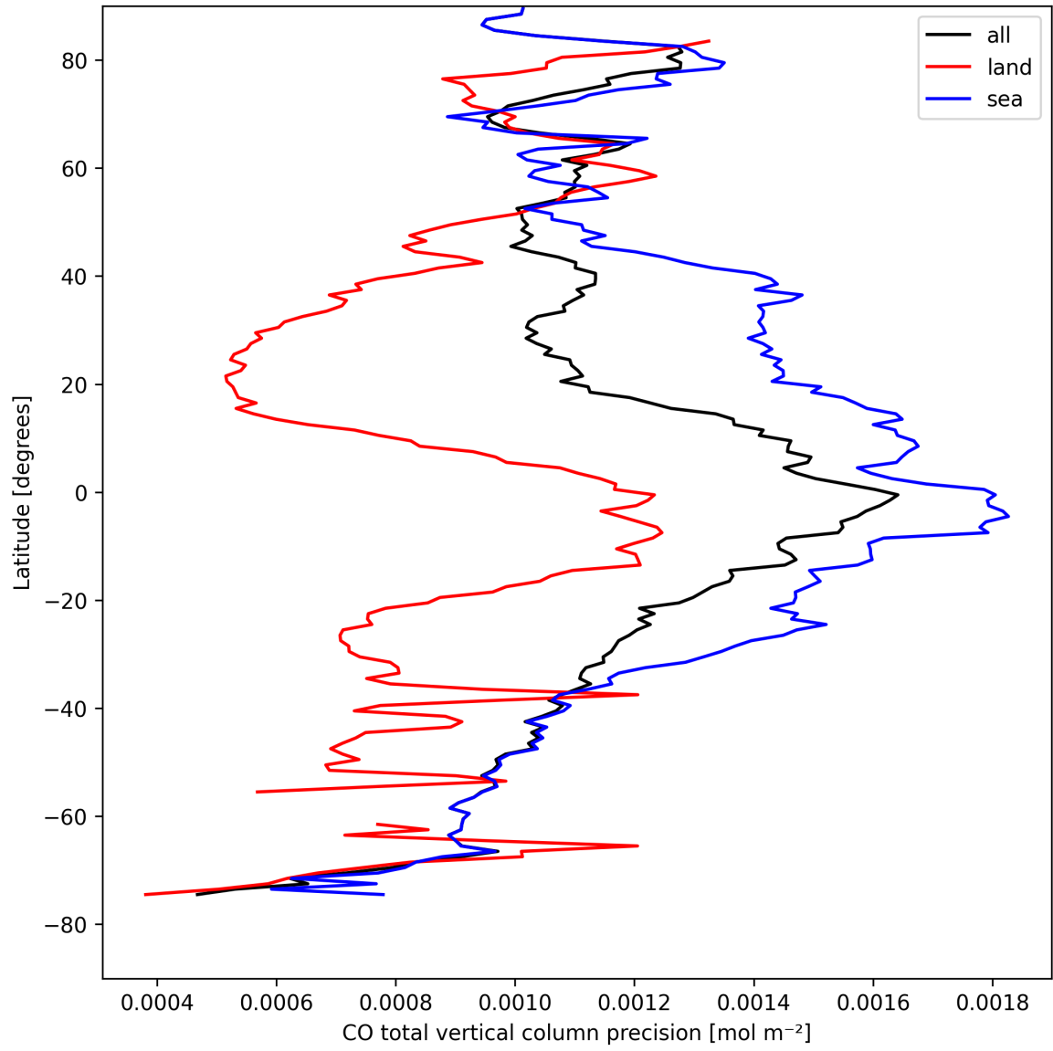
Figure 8: Zonal average of “CO total vertical column precision” for 2025-04-17 to 2025-04-18.
