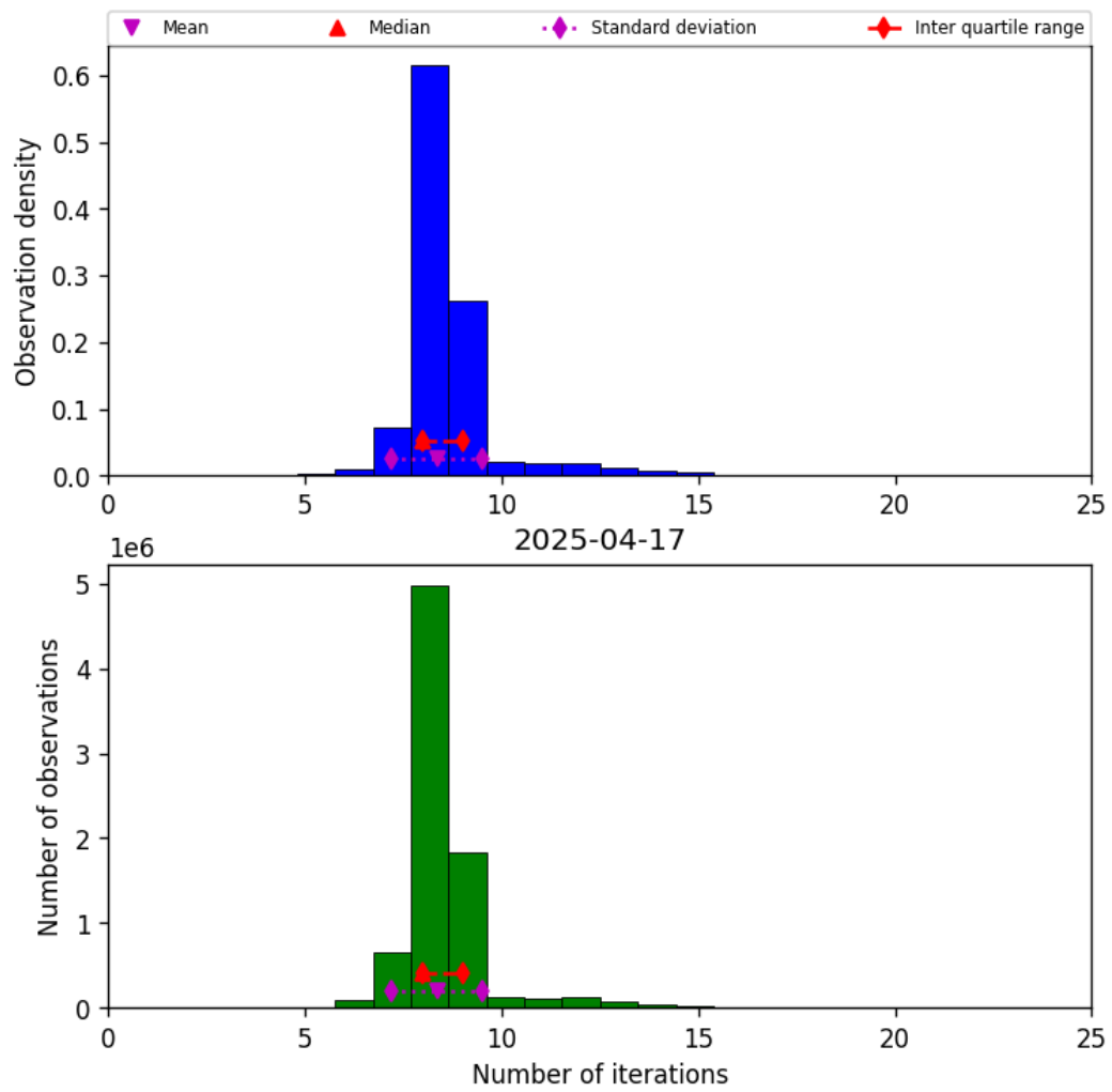
Figure 19: Histogram of “Number of iterations” for 2025-04-17 to 2025-04-18
