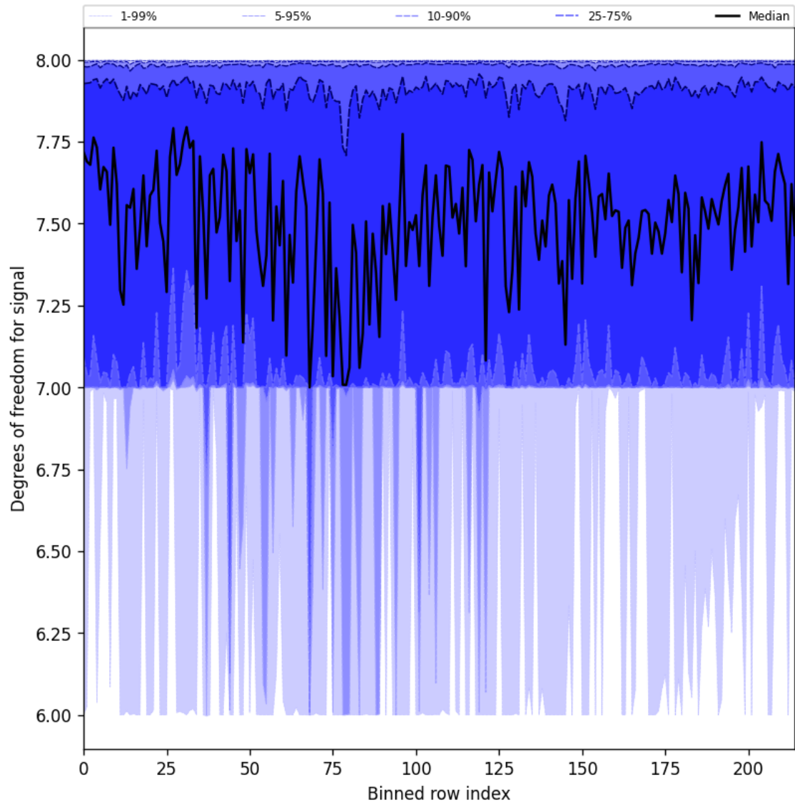
Figure 25: Along track statistics of “Degrees of freedom for signal” for 2025-04-17 to 2025-04-18
