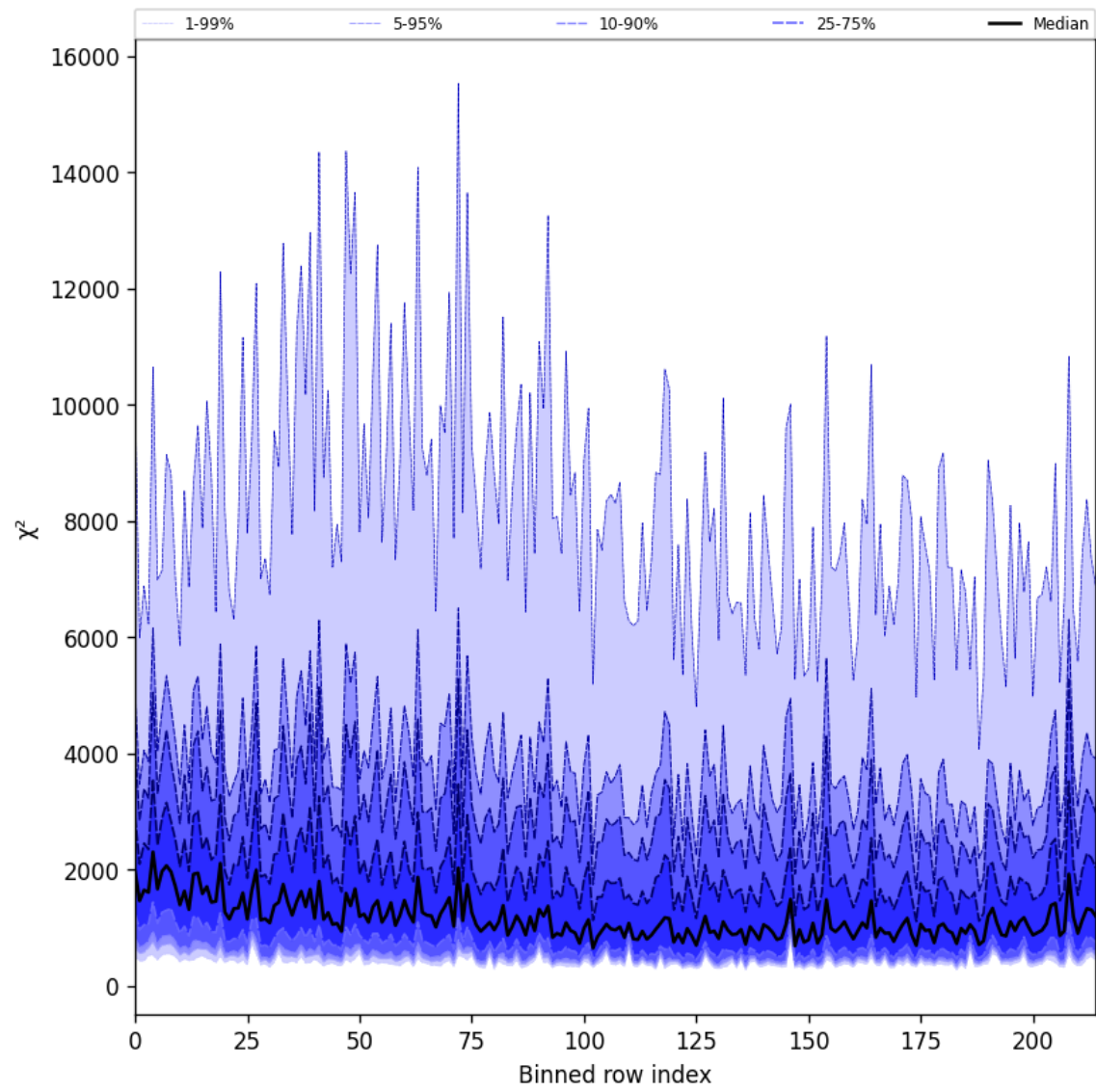
Figure 24: Along track statistics of “ \chi^2 ” for 2025-04-17 to 2025-04-18
