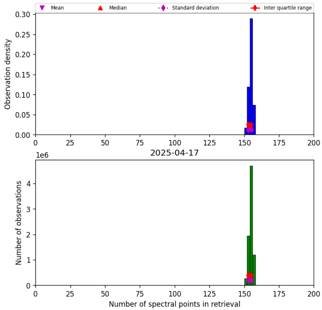
Figure 16: Histogram of “Number of spectral points in retrieval” for 2025-04-17 to 2025-04-18
