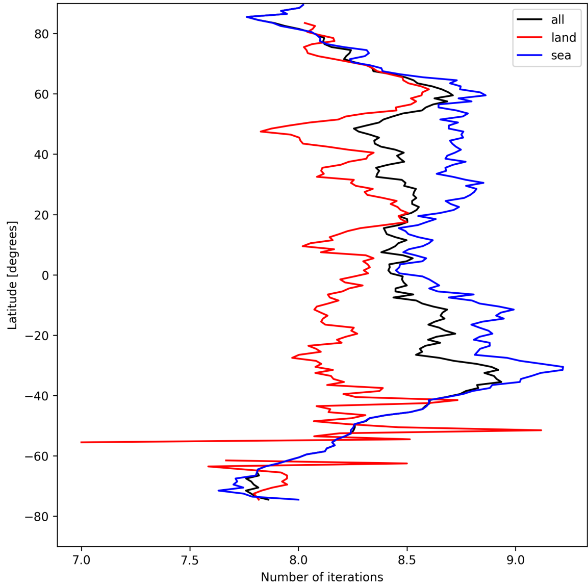
Figure 12: Zonal average of “Number of iterations” for 2025-04-17 to 2025-04-18.
