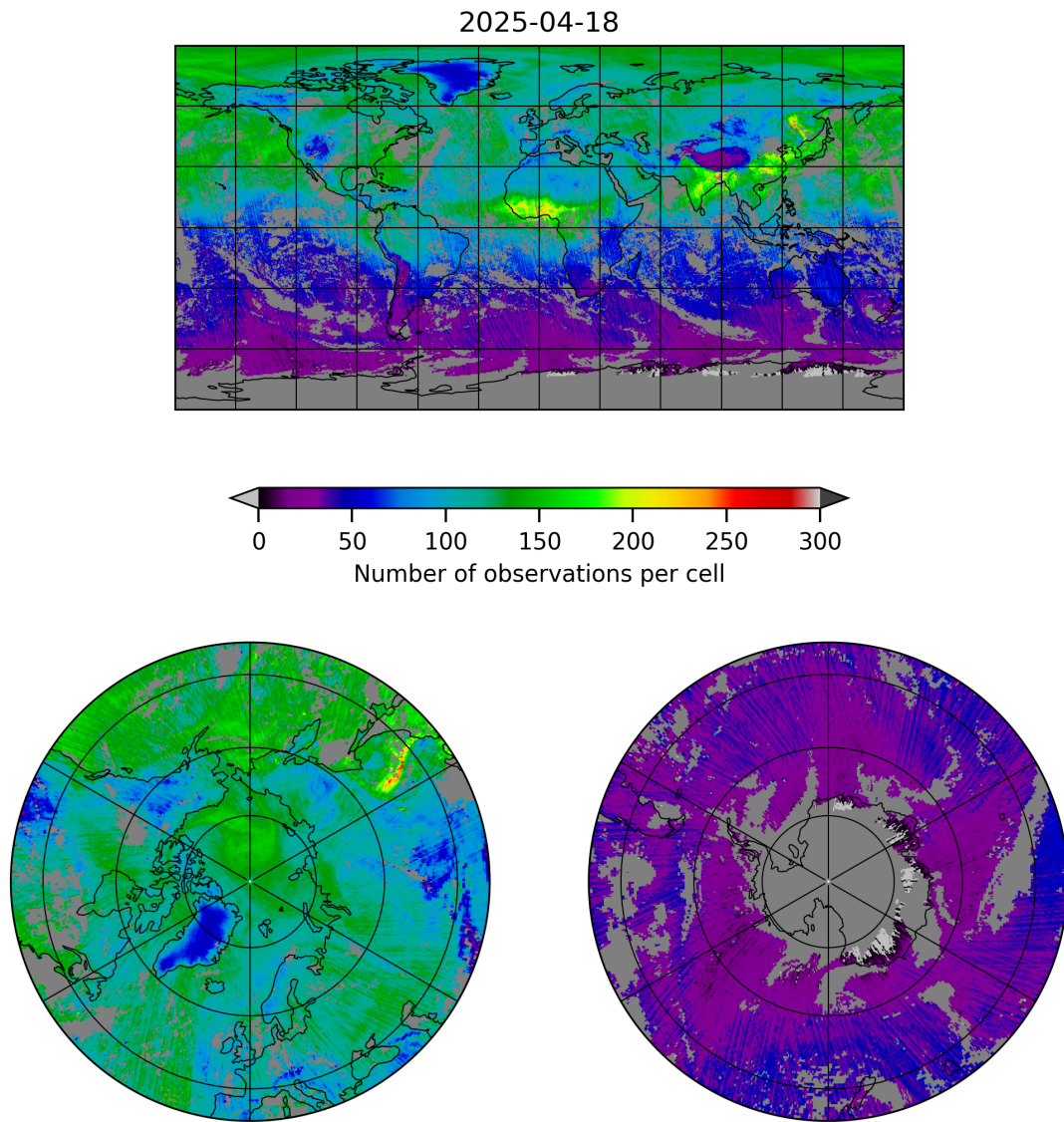
Figure 5: Map of the number of observations for 2025-04-18 to 2025-04-19
