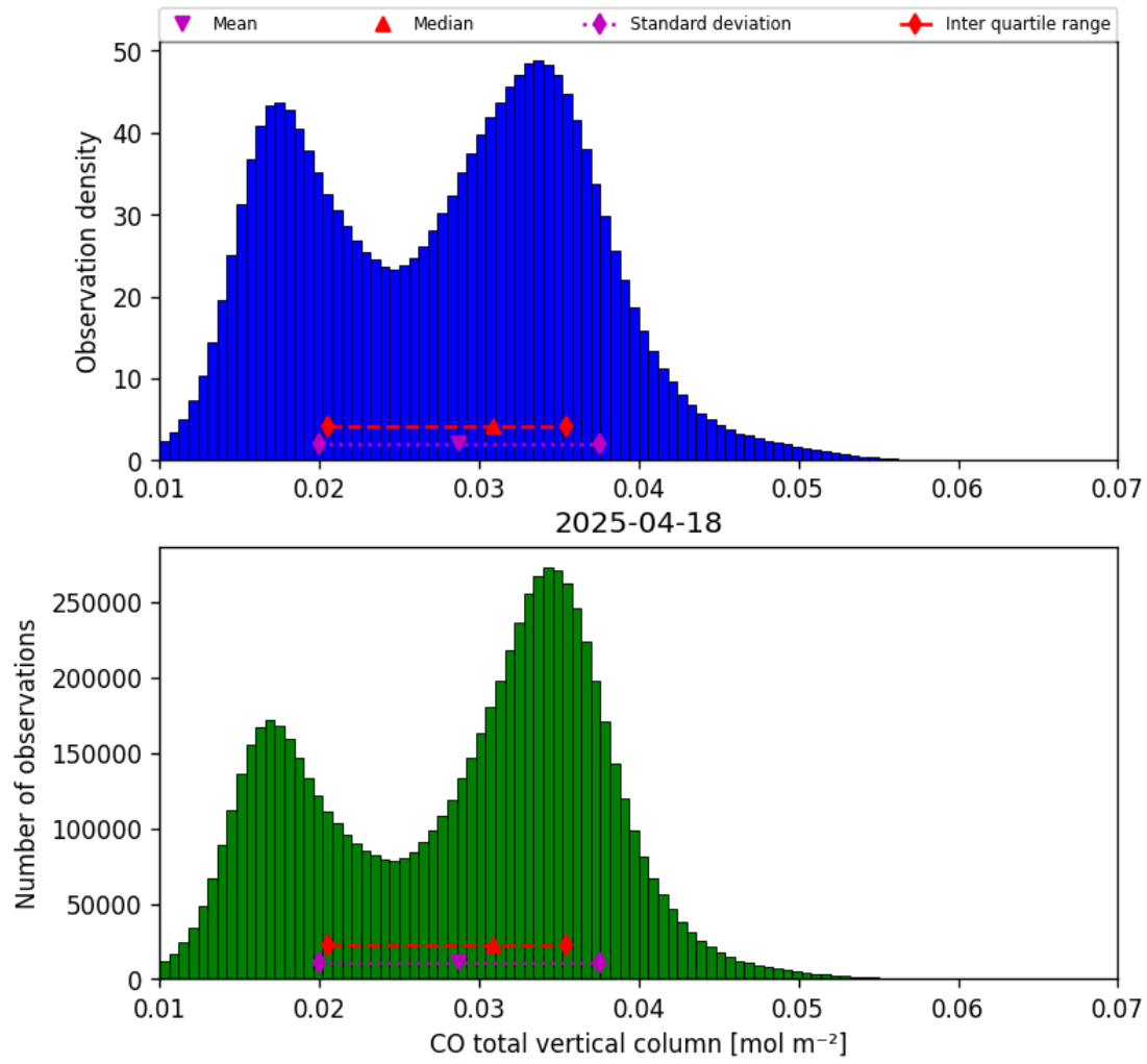
Figure 14: Histogram of “CO total vertical column” for 2025-04-18 to 2025-04-19
