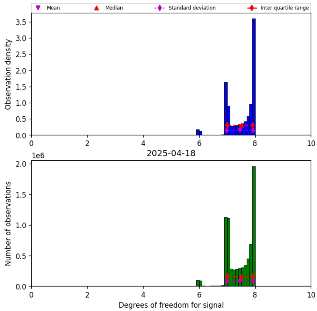
Figure 18: Histogram of “Degrees of freedom for signal” for 2025-04-18 to 2025-04-19
