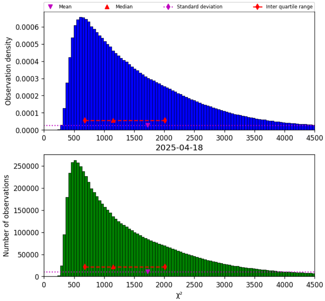
Figure 17: Histogram of “ \chi^2 ” for 2025-04-18 to 2025-04-19
