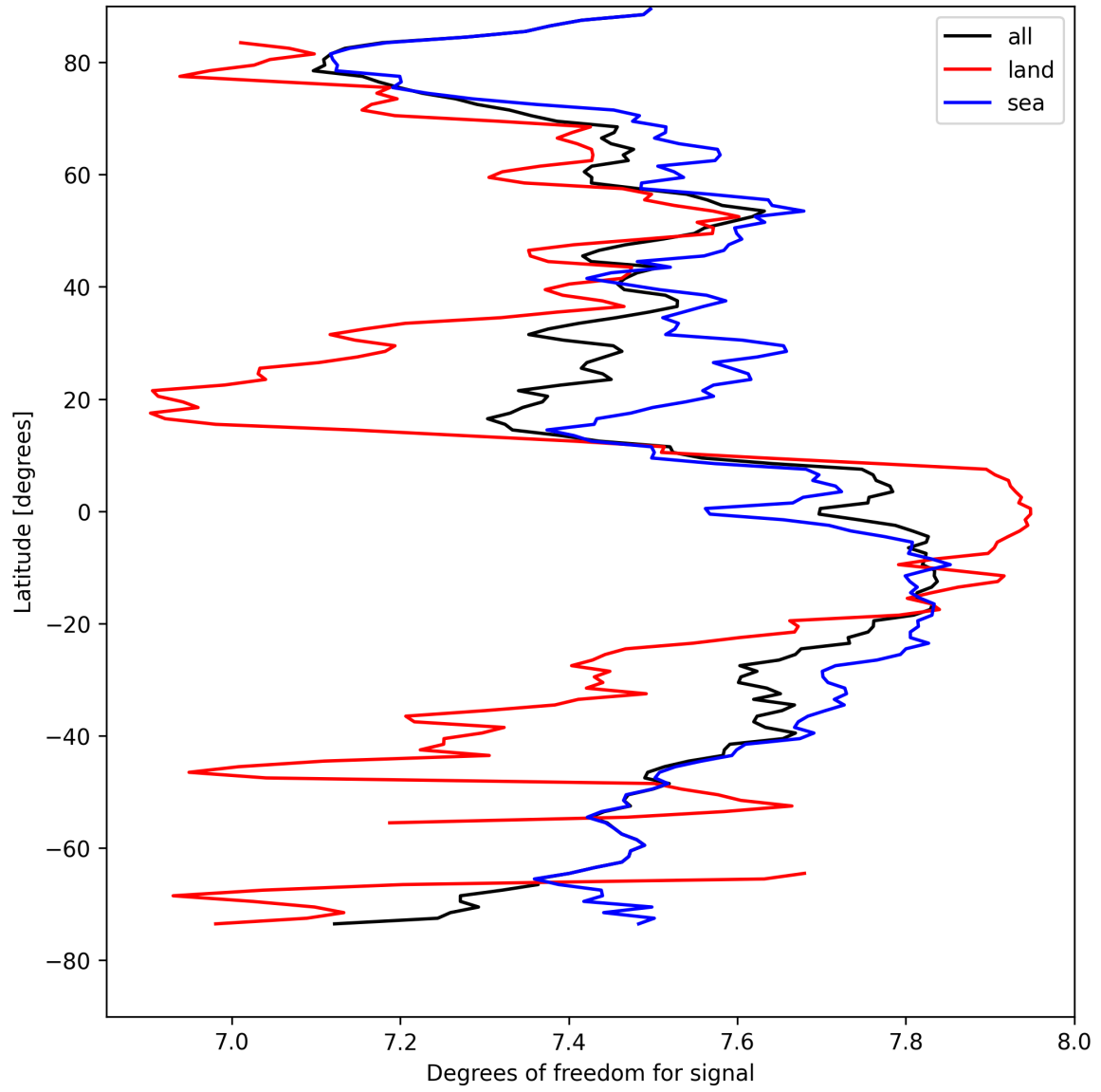
Figure 11: Zonal average of “Degrees of freedom for signal” for 2025-04-18 to 2025-04-19.
