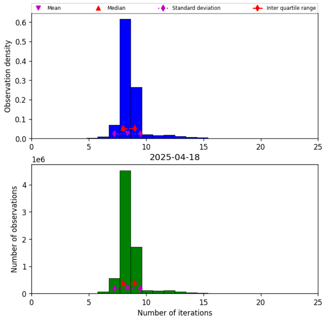
Figure 19: Histogram of “Number of iterations” for 2025-04-18 to 2025-04-19
