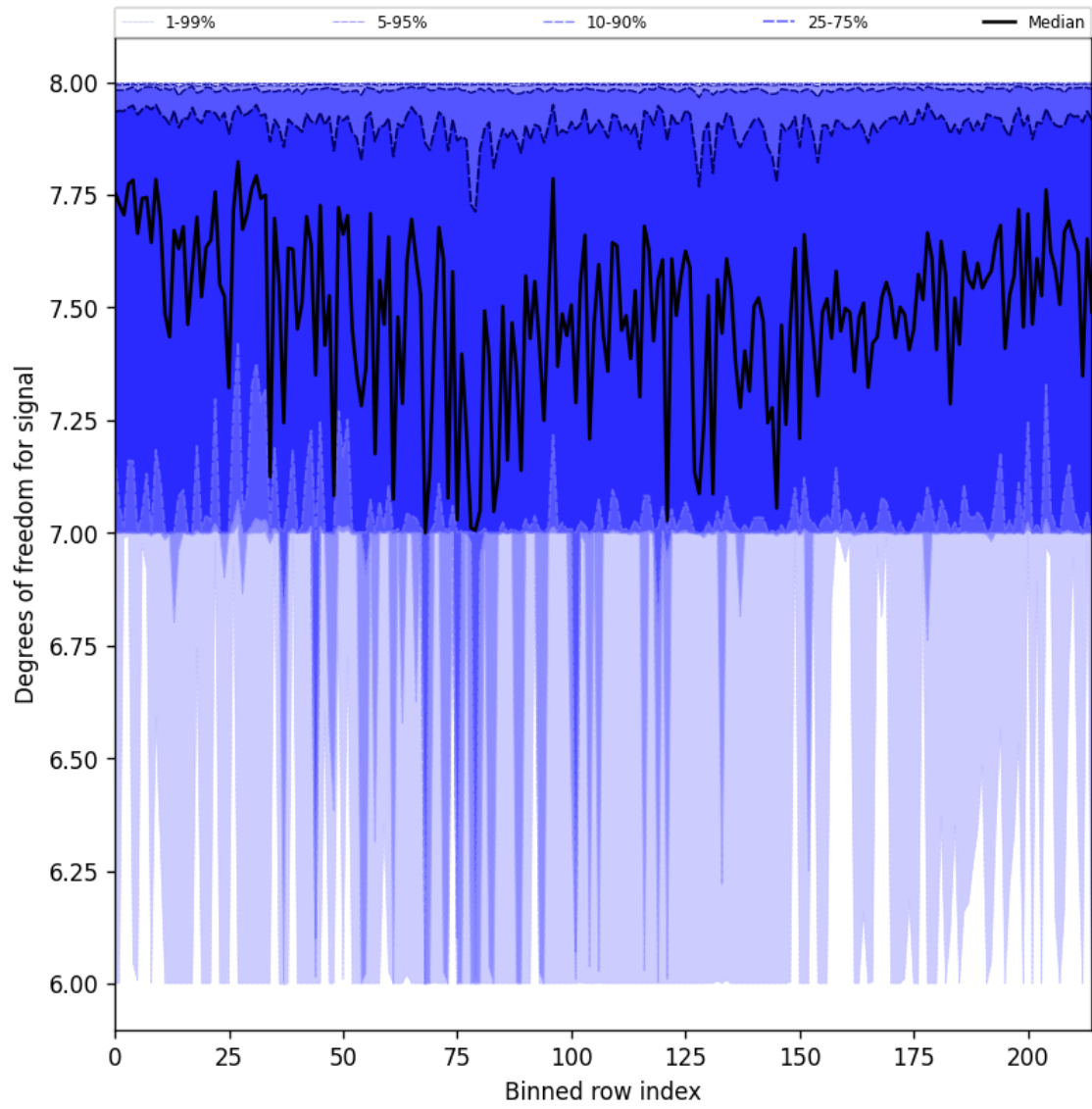
Figure 25: Along track statistics of “Degrees of freedom for signal” for 2025-04-18 to 2025-04-19
