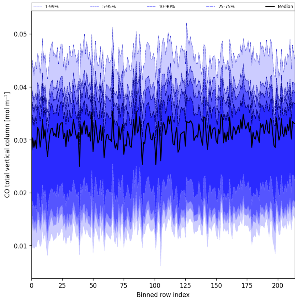
Figure 21: Along track statistics of “CO total vertical column” for 2025-04-18 to 2025-04-19
