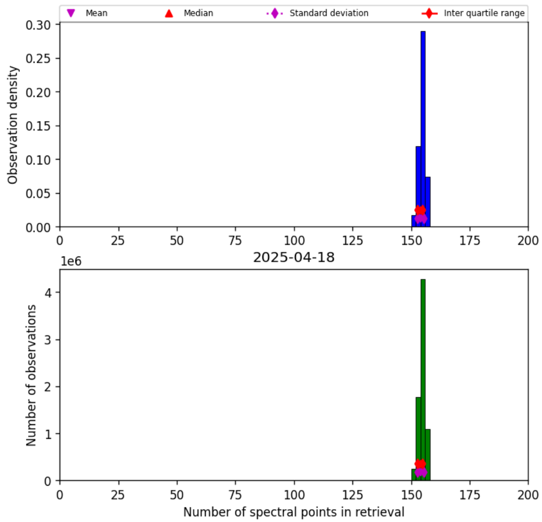
Figure 16: Histogram of “Number of spectral points in retrieval” for 2025-04-18 to 2025-04-19
