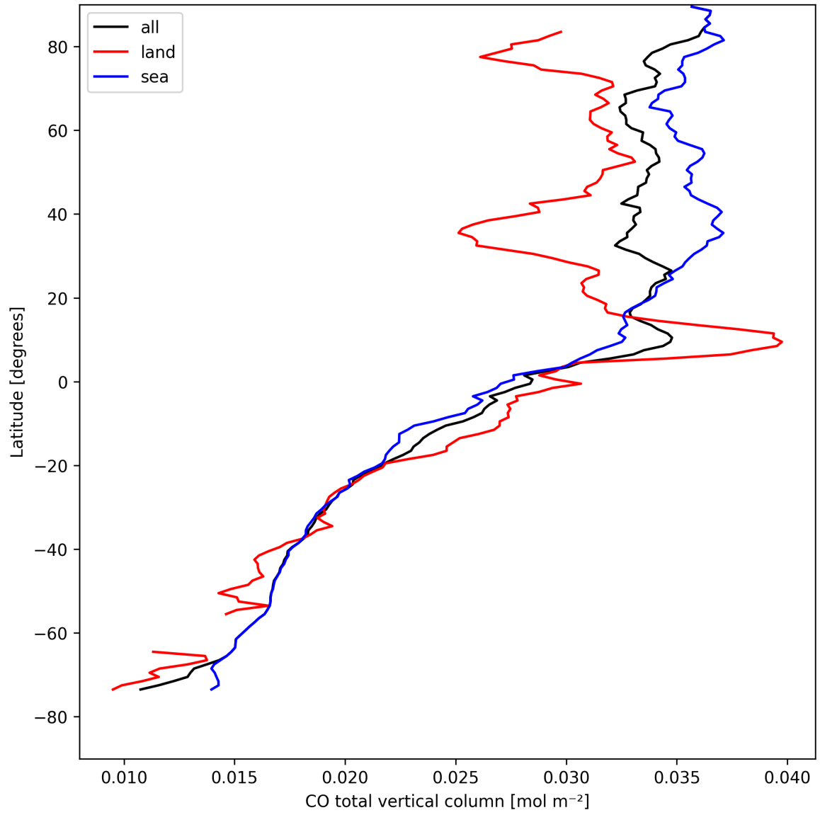
Figure 7: Zonal average of “CO total vertical column” for 2025-04-18 to 2025-04-19.
