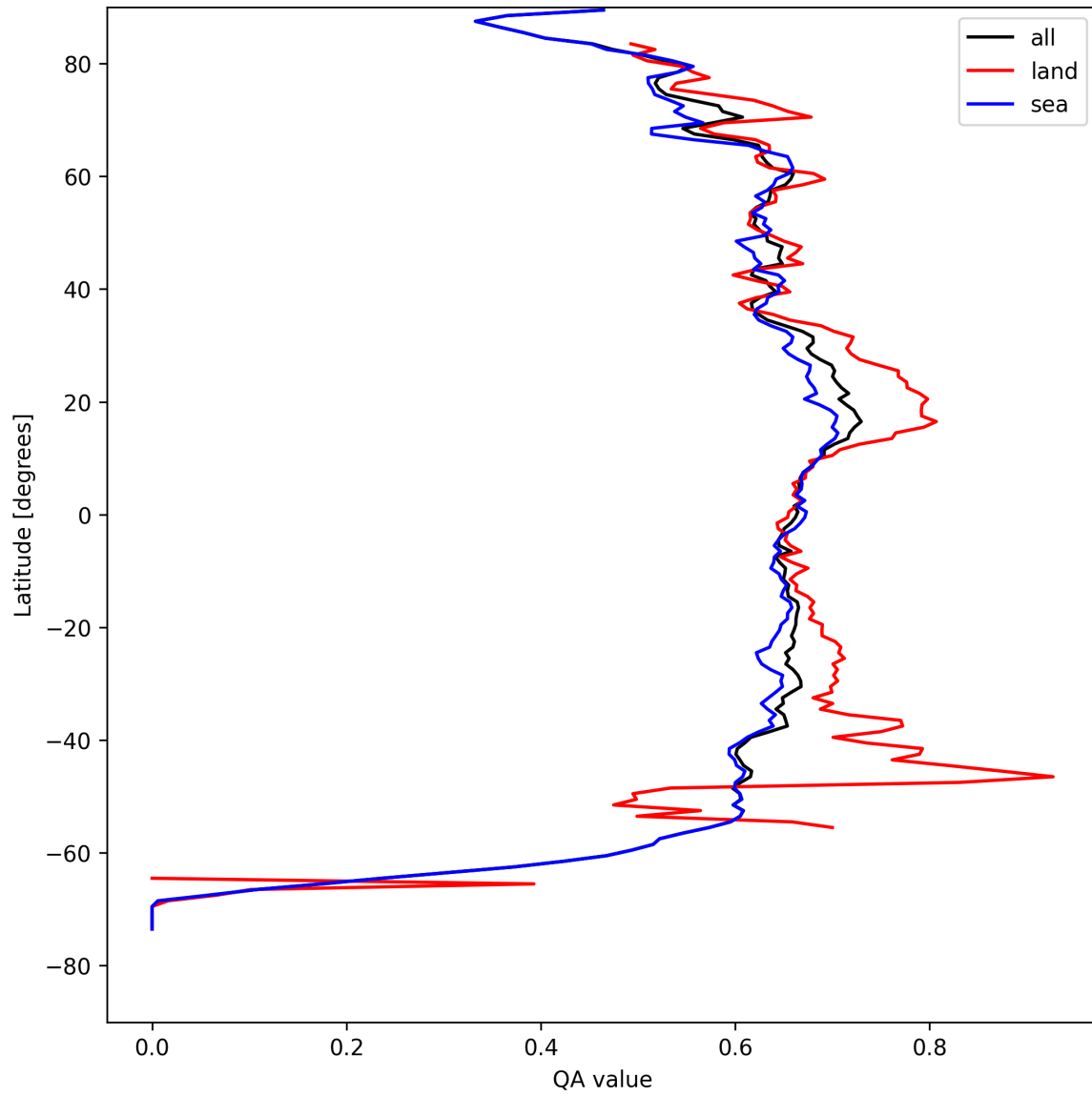
Figure 6: Zonal average of “QA value” for 2025-04-18 to 2025-04-19.
