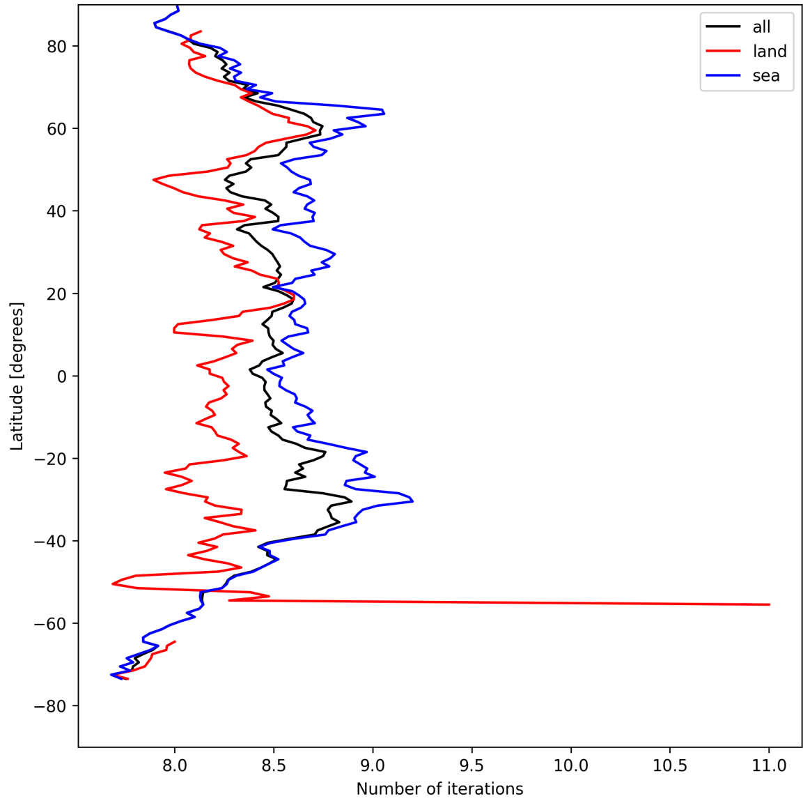
Figure 12: Zonal average of “Number of iterations” for 2025-04-18 to 2025-04-19.
