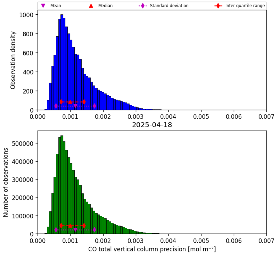
Figure 15: Histogram of “CO total vertical column precision” for 2025-04-18 to 2025-04-19
