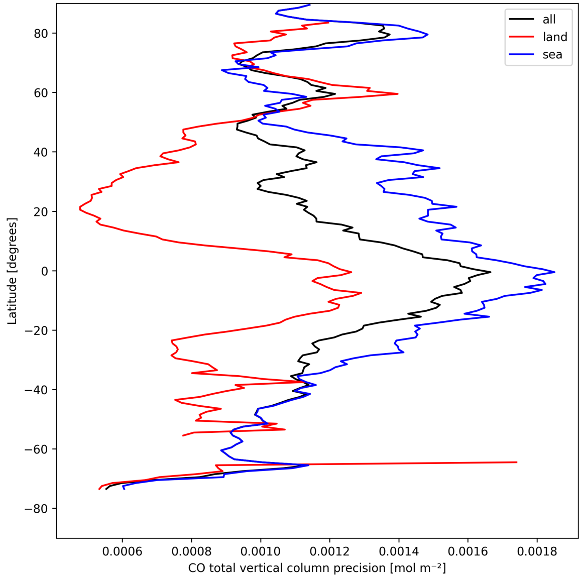
Figure 8: Zonal average of "CO total vertical column precision" for 2025-04-18 to 2025-04-19.
