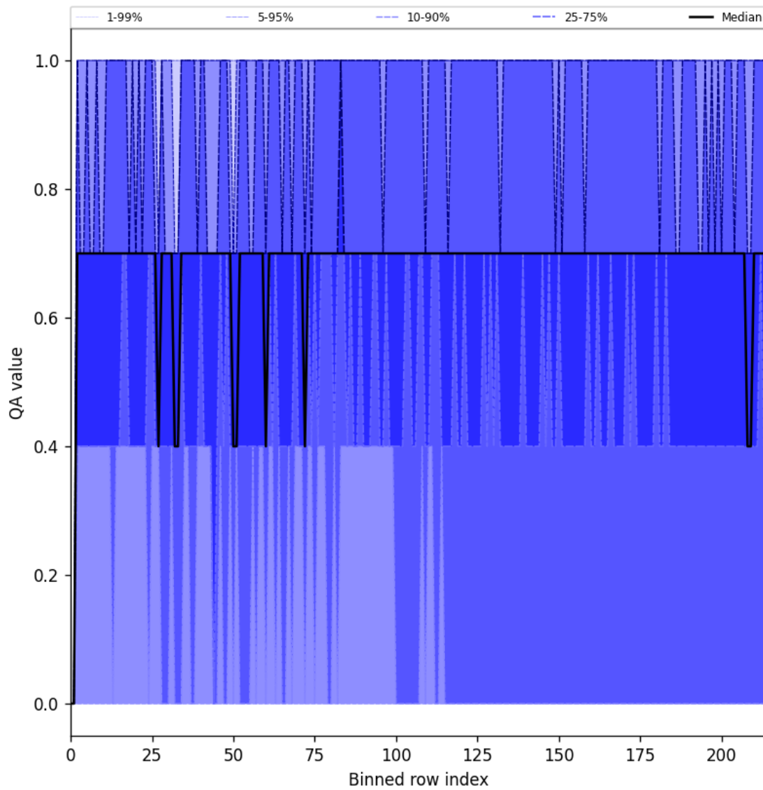
Figure 20: Along track statistics of “QA value” for 2025-04-18 to 2025-04-19
