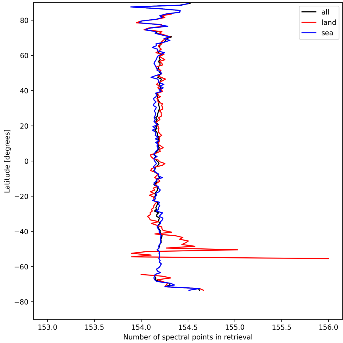
Figure 9: Zonal average of “Number of spectral points in retrieval” for 2025-04-18 to 2025-04-19.
