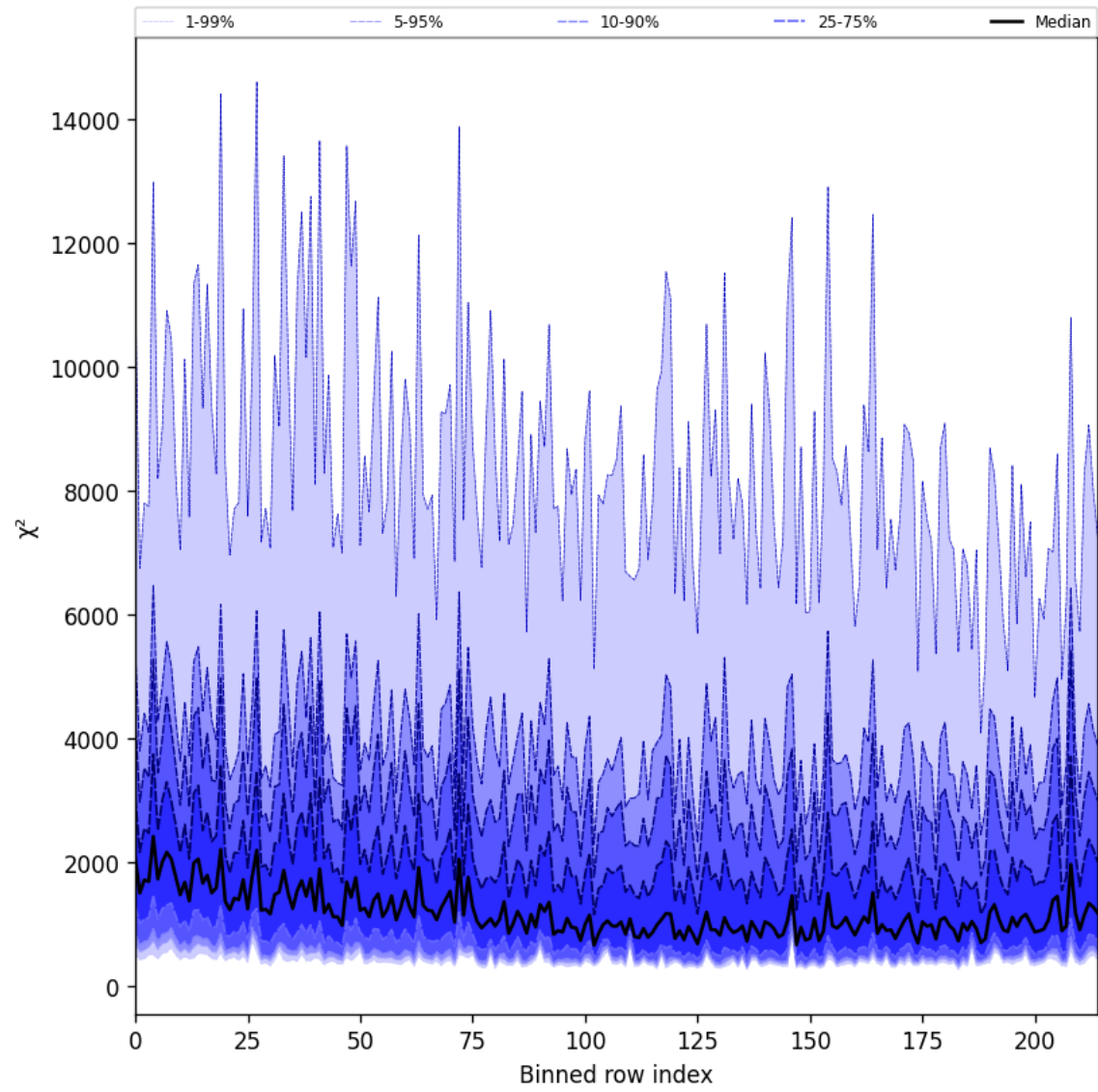
Figure 24: Along track statistics of “ \chi^2 ” for 2025-04-18 to 2025-04-19
