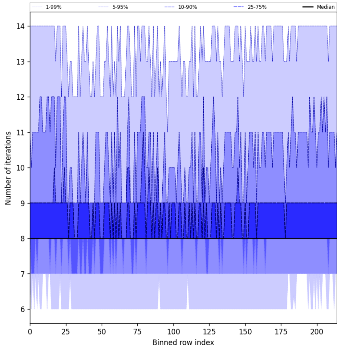
Figure 26: Along track statistics of “Number of iterations” for 2025-04-18 to 2025-04-19
