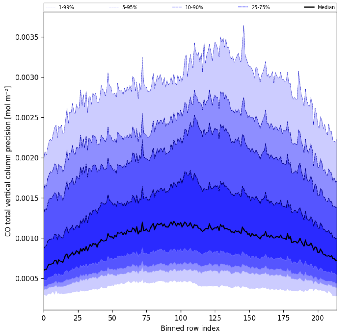
Figure 22: Along track statistics of “CO total vertical column precision” for 2025-04-18 to 2025-04-19
