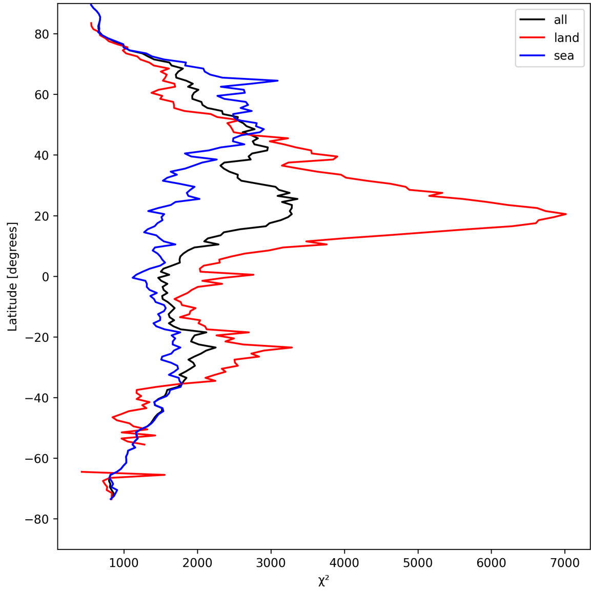
Figure 10: Zonal average of “ \chi^2 ” for 2025-04-18 to 2025-04-19.
