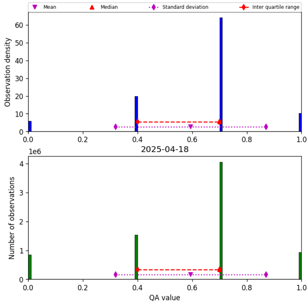
Figure 13: Histogram of “QA value” for 2025-04-18 to 2025-04-19
