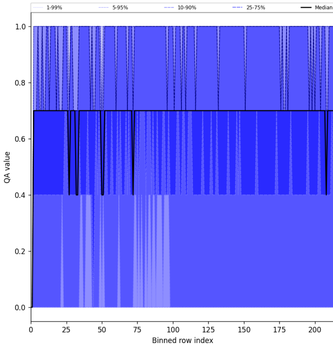
Figure 20: Along track statistics of “QA value” for 2025-04-19 to 2025-04-20
