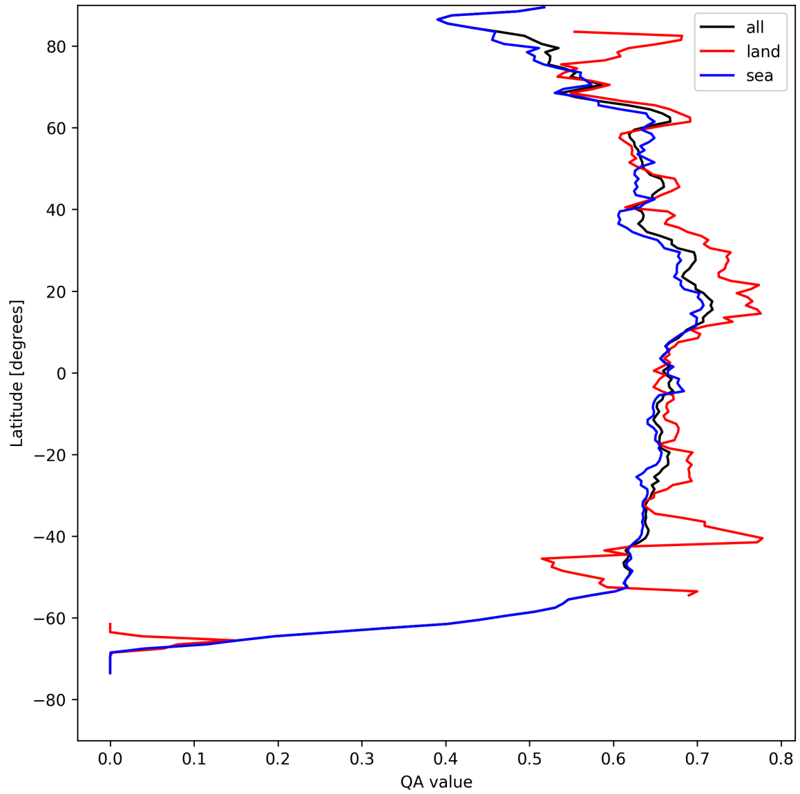
Figure 6: Zonal average of “QA value” for 2025-04-19 to 2025-04-20.
