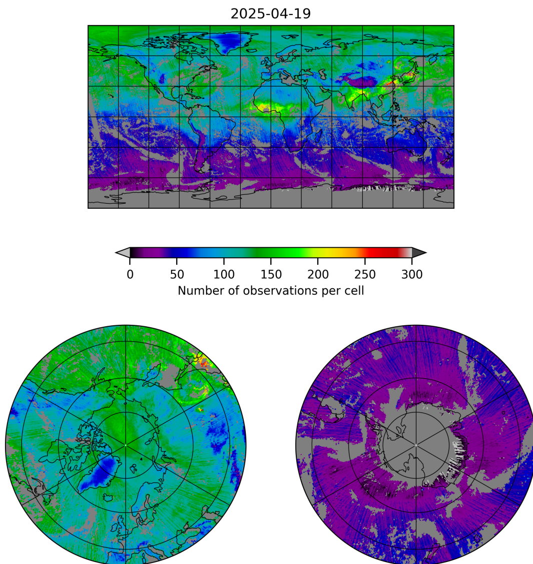
Figure 5: Map of the number of observations for 2025-04-19 to 2025-04-20
