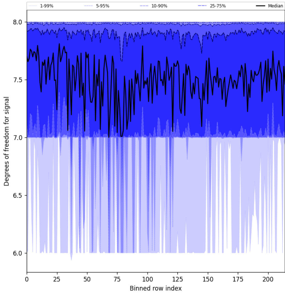
Figure 25: Along track statistics of “Degrees of freedom for signal” for 2025-04-19 to 2025-04-20
