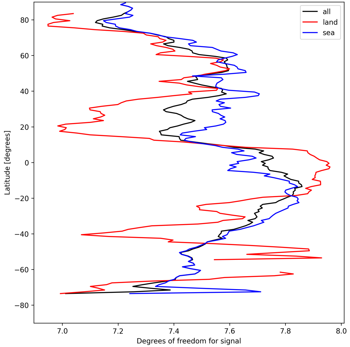
Figure 11: Zonal average of “Degrees of freedom for signal” for 2025-04-19 to 2025-04-20.
