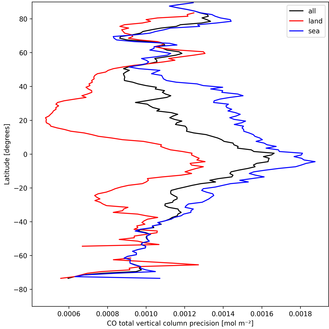
Figure 8: Zonal average of “CO total vertical column precision” for 2025-04-19 to 2025-04-20.
