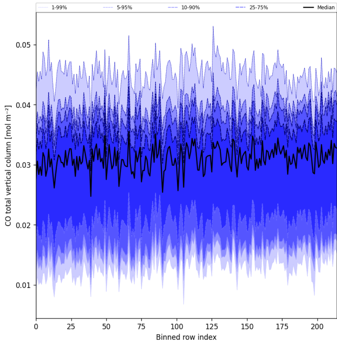
Figure 21: Along track statistics of “CO total vertical column” for 2025-04-19 to 2025-04-20
