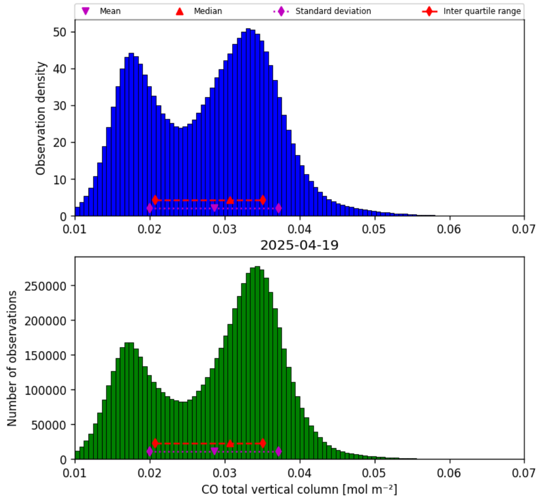
Figure 14: Histogram of “CO total vertical column” for 2025-04-19 to 2025-04-20
