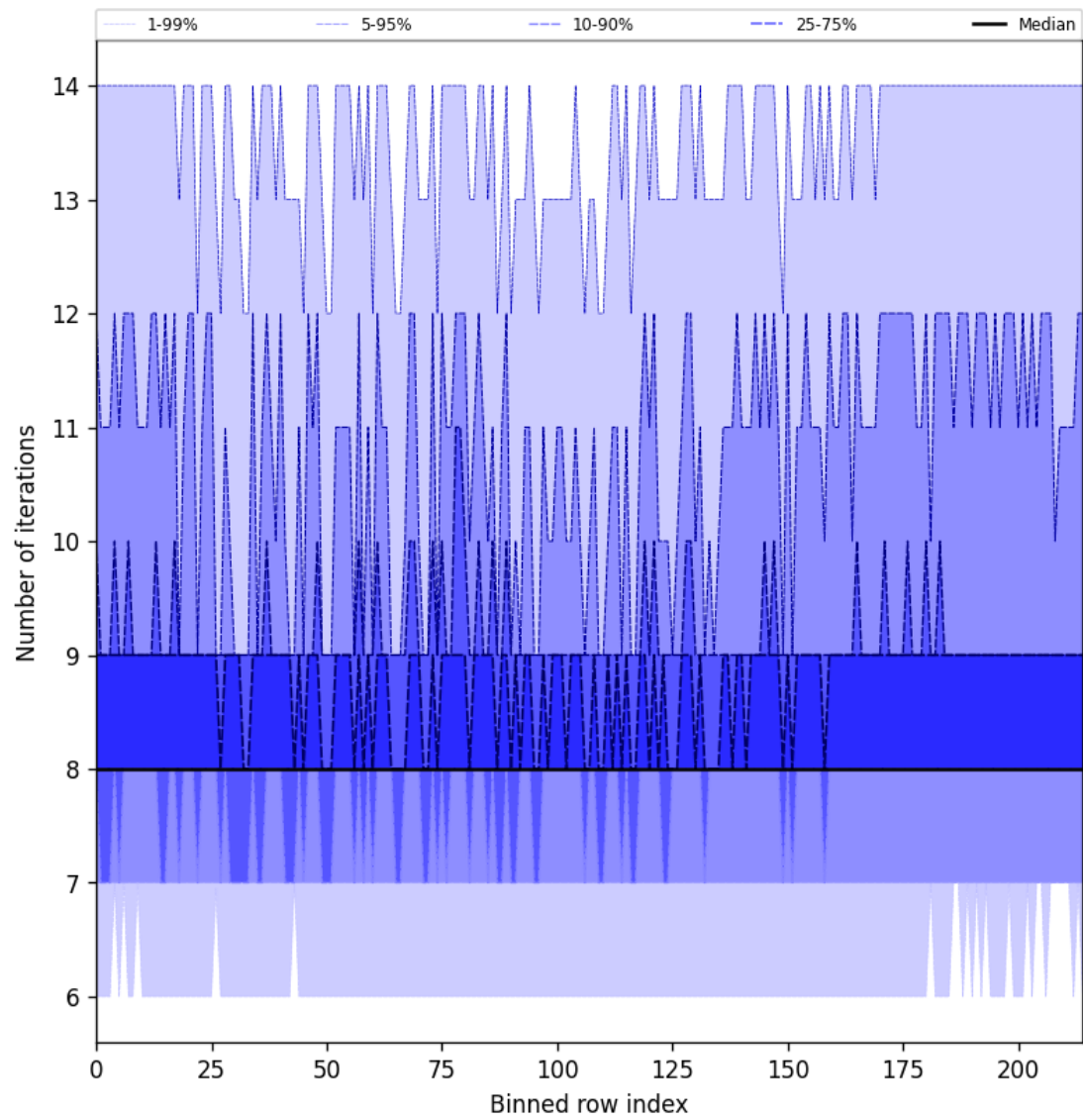
Figure 26: Along track statistics of “Number of iterations” for 2025-04-19 to 2025-04-20
