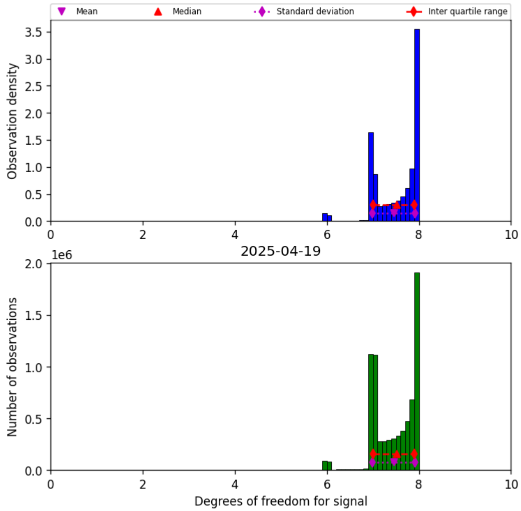
Figure 18: Histogram of “Degrees of freedom for signal” for 2025-04-19 to 2025-04-20
