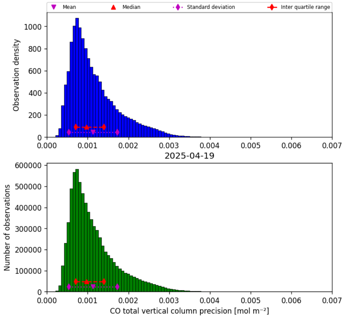
Figure 15: Histogram of “CO total vertical column precision” for 2025-04-19 to 2025-04-20
