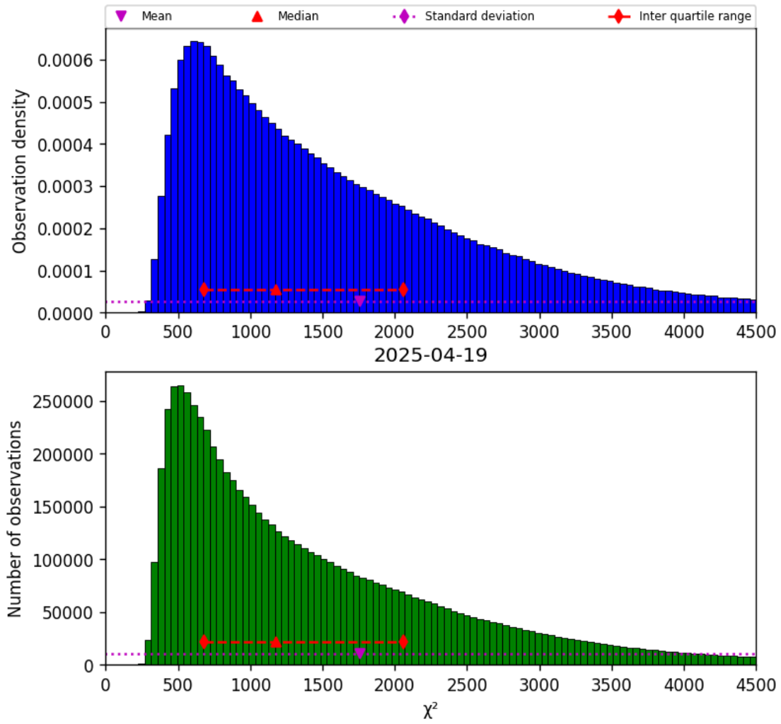
Figure 17: Histogram of “ \chi^2 ” for 2025-04-19 to 2025-04-20
