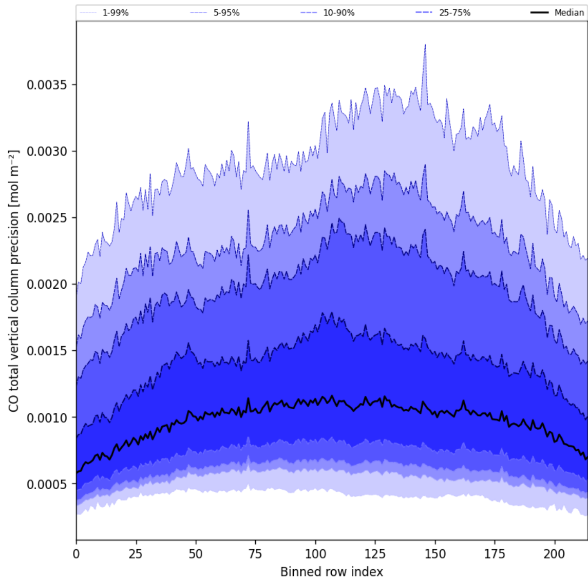
Figure 22: Along track statistics of “CO total vertical column precision” for 2025-04-19 to 2025-04-20
