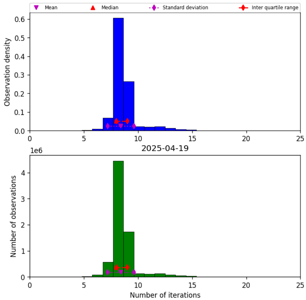
Figure 19: Histogram of “Number of iterations” for 2025-04-19 to 2025-04-20
