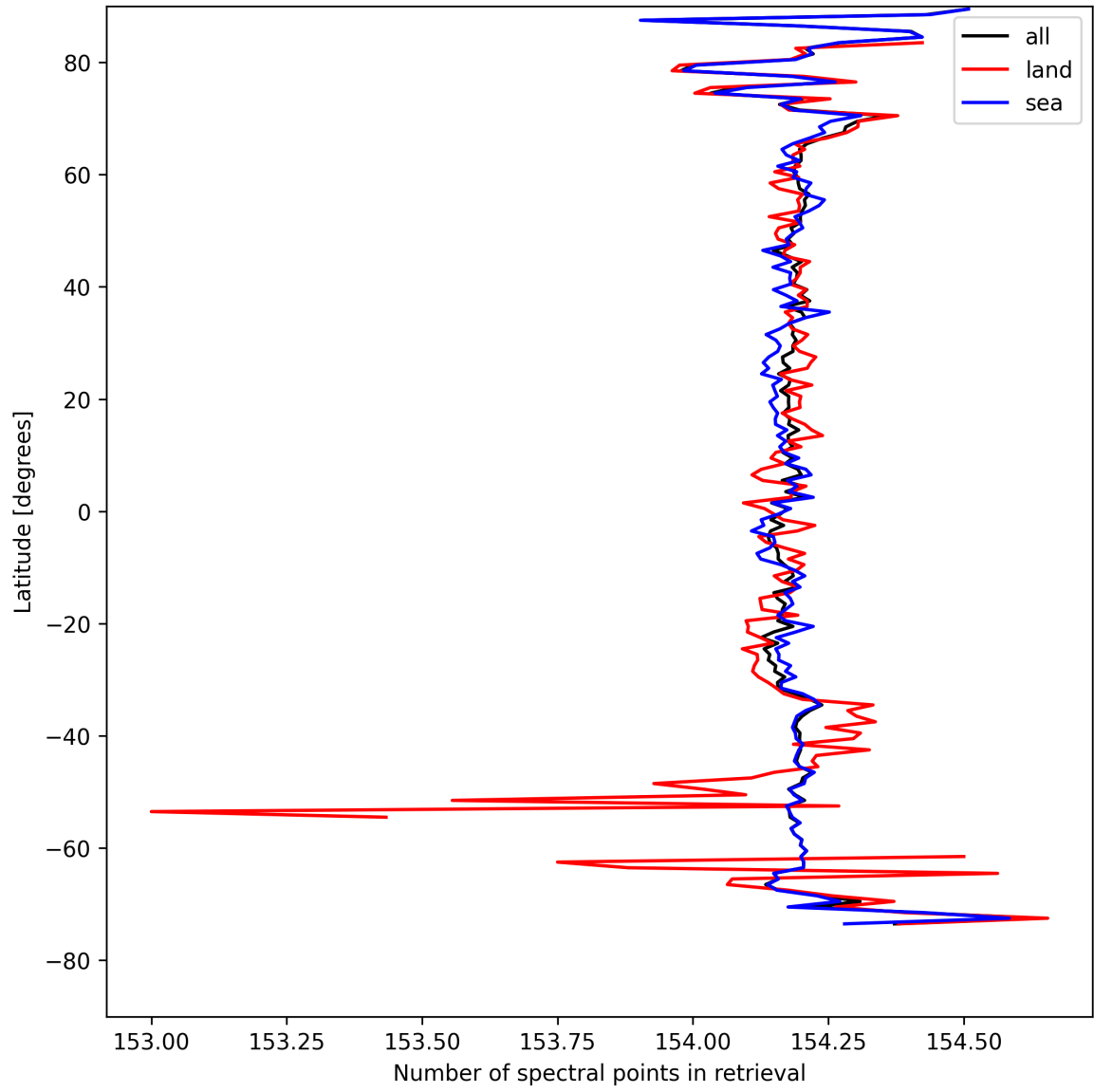
Figure 9: Zonal average of “Number of spectral points in retrieval” for 2025-04-19 to 2025-04-20.
