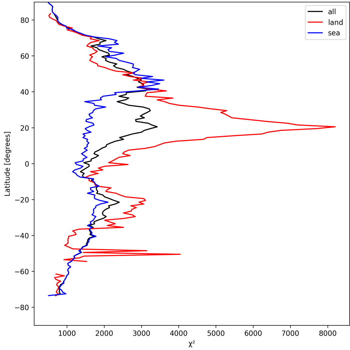
Figure 10: Zonal average of “ \chi^2 ” for 2025-04-19 to 2025-04-20.
