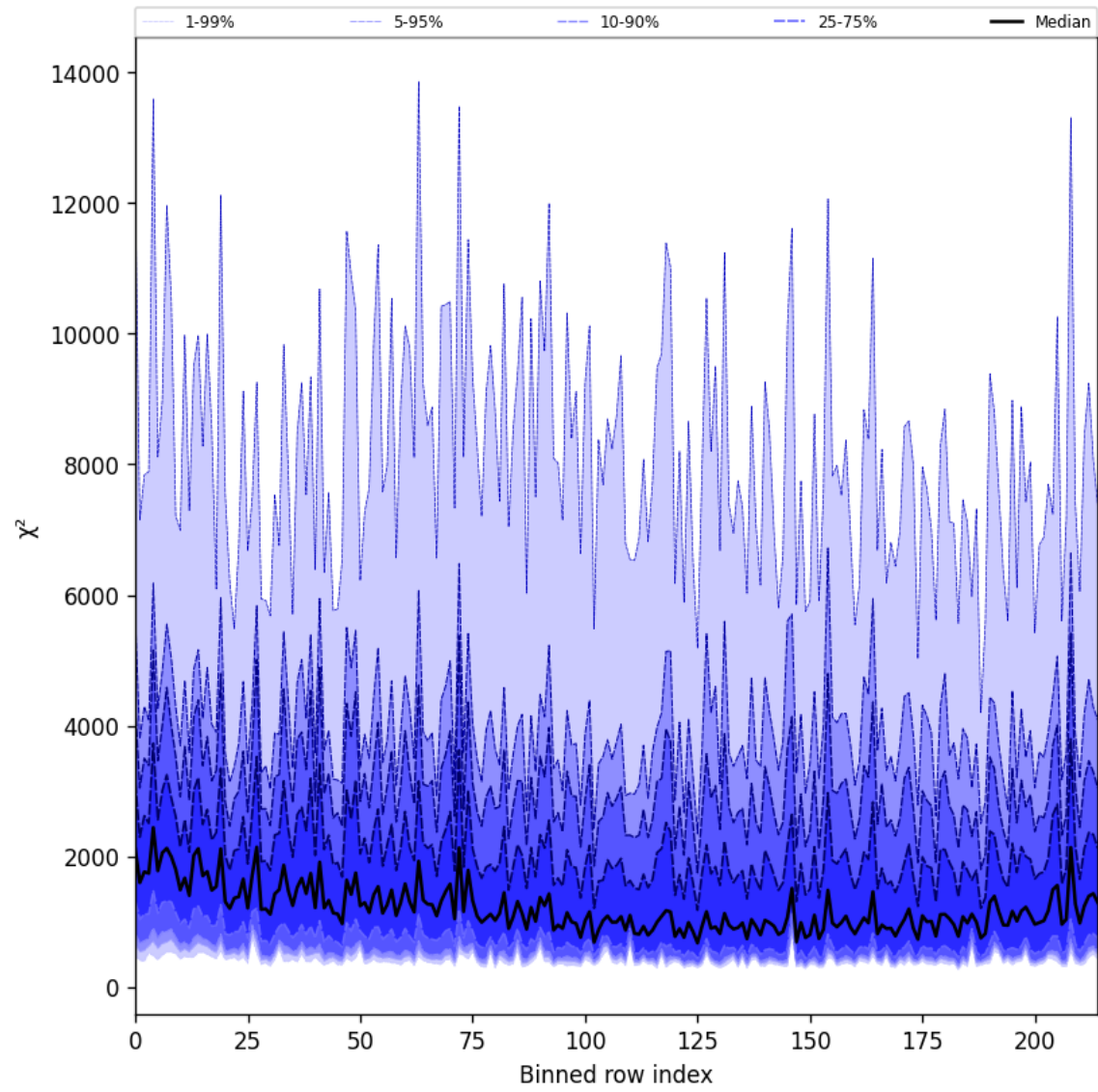
Figure 24: Along track statistics of “ \chi^2 ” for 2025-04-19 to 2025-04-20
