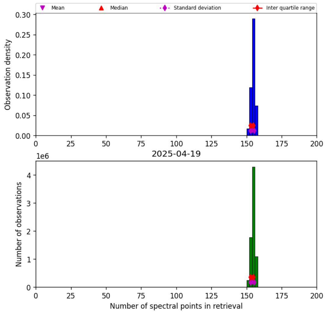
Figure 16: Histogram of “Number of spectral points in retrieval” for 2025-04-19 to 2025-04-20
