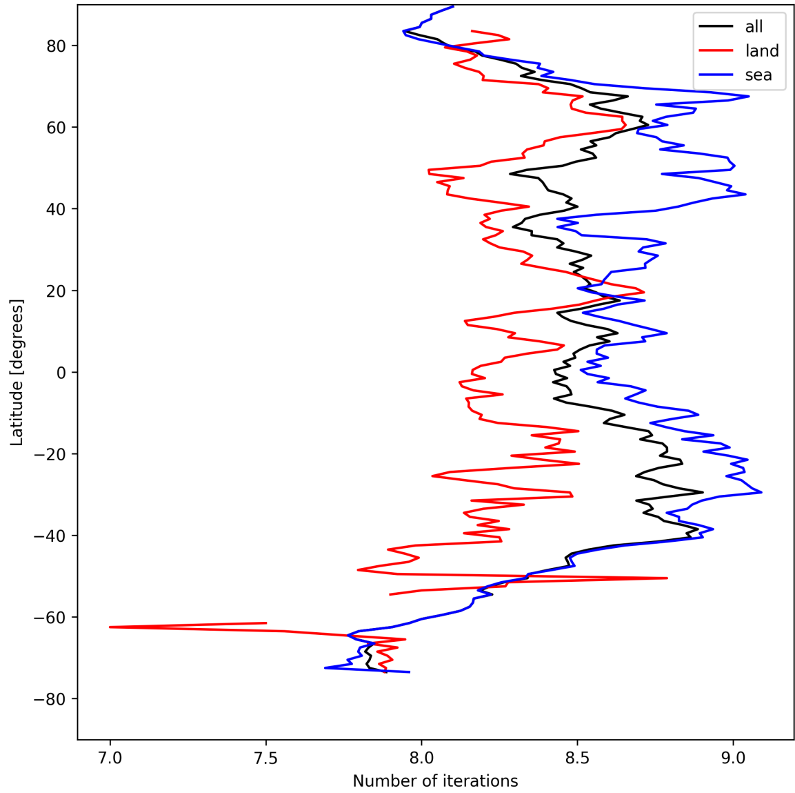
Figure 12: Zonal average of “Number of iterations” for 2025-04-19 to 2025-04-20.
