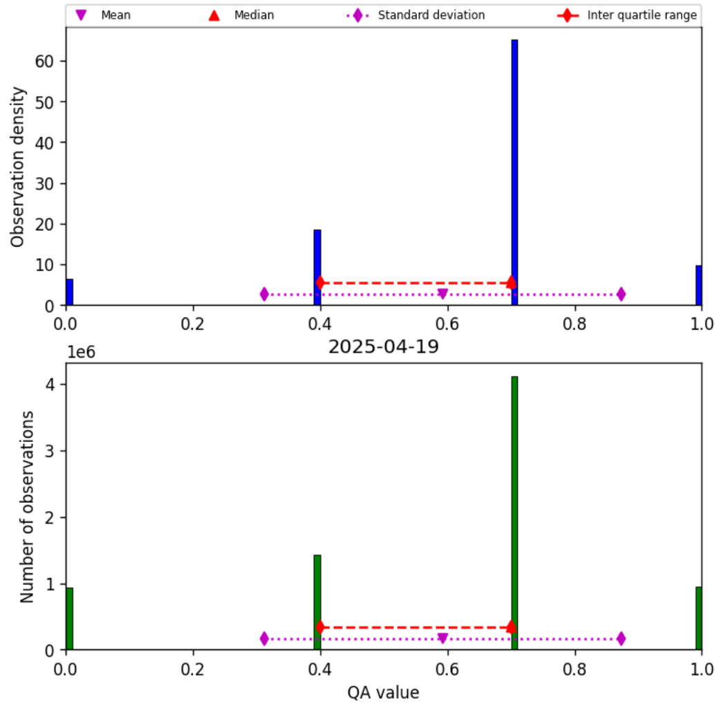
Figure 13: Histogram of “QA value” for 2025-04-19 to 2025-04-20
