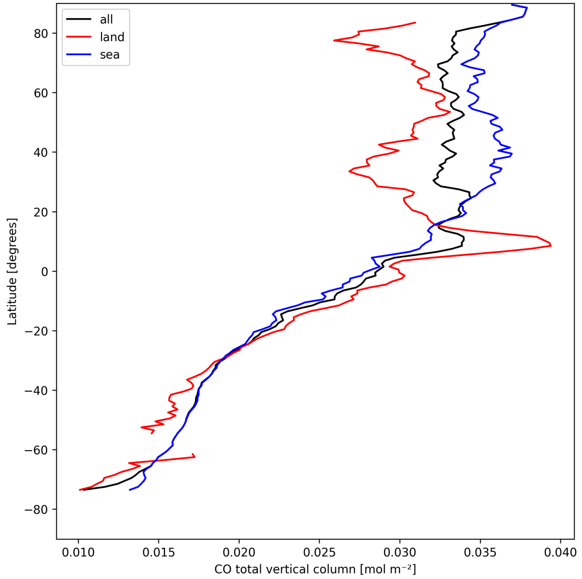
Figure 7: Zonal average of “CO total vertical column” for 2025-04-19 to 2025-04-20.
