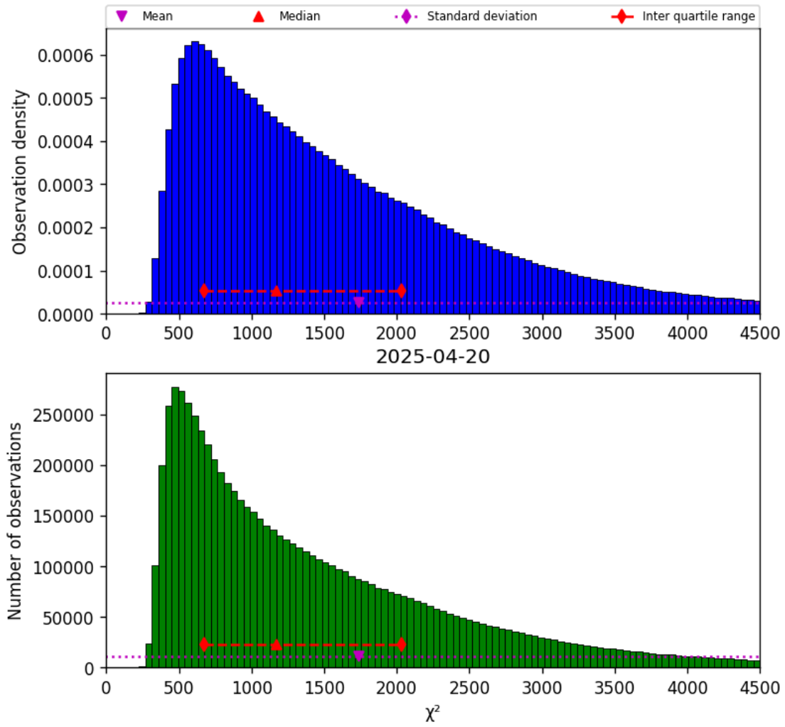
Figure 17: Histogram of “ \chi^2 ” for 2025-04-20 to 2025-04-21
