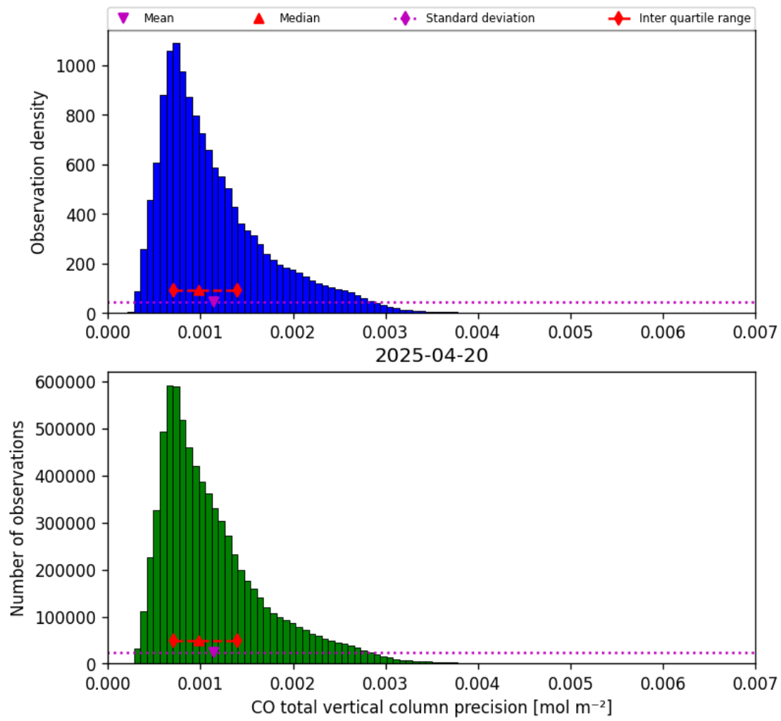
Figure 15: Histogram of “CO total vertical column precision” for 2025-04-20 to 2025-04-21
