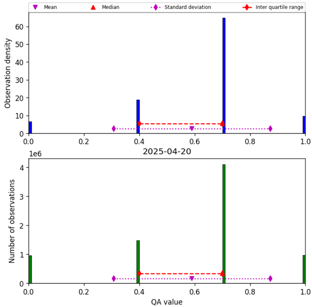
Figure 13: Histogram of “QA value” for 2025-04-20 to 2025-04-21
