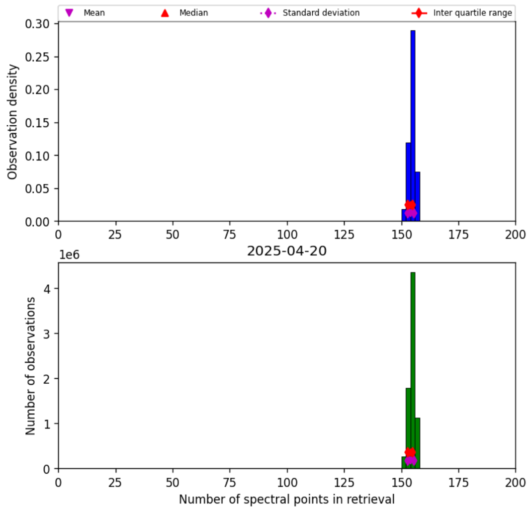
Figure 16: Histogram of “Number of spectral points in retrieval” for 2025-04-20 to 2025-04-21
