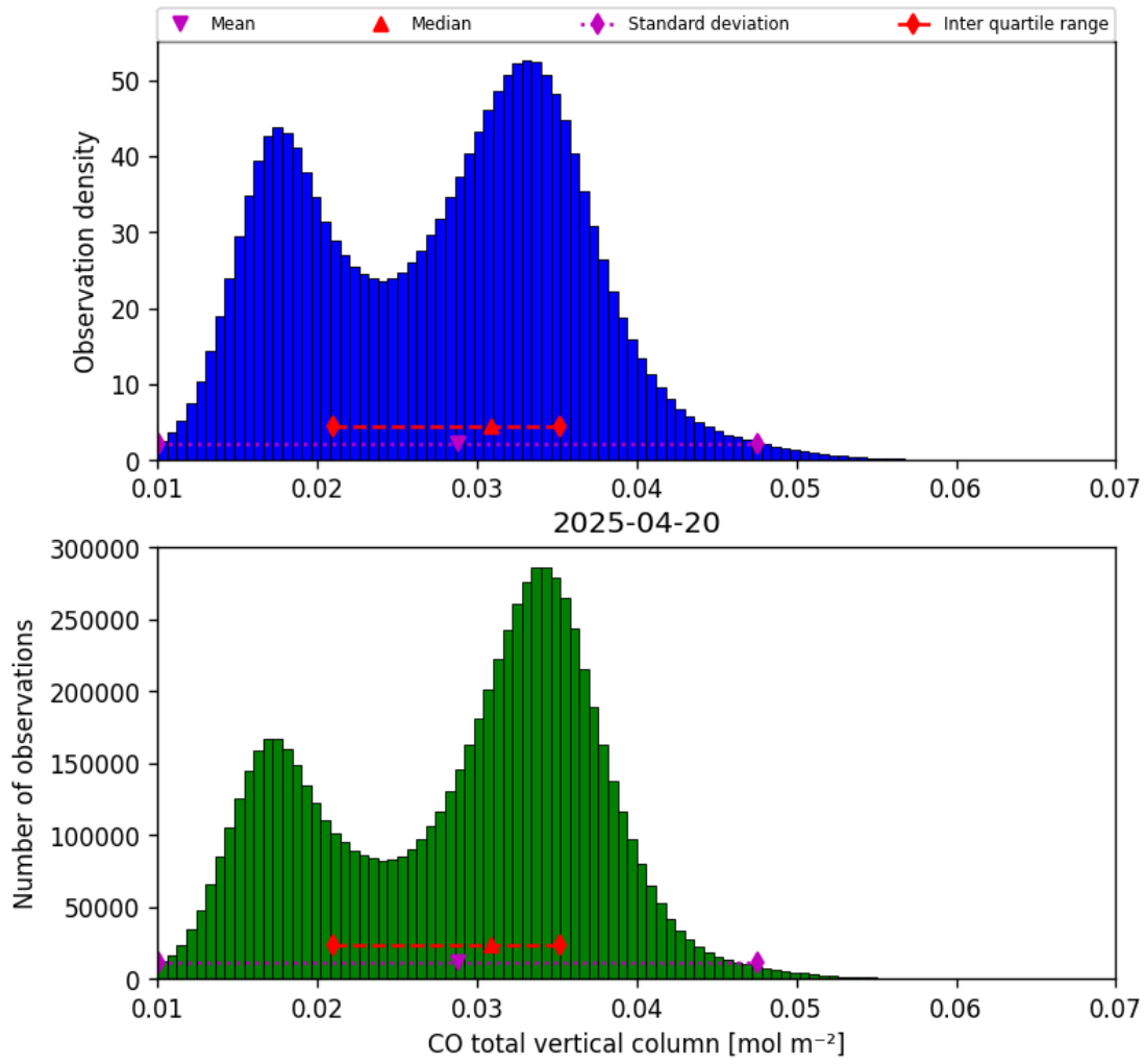
Figure 14: Histogram of “CO total vertical column” for 2025-04-20 to 2025-04-21
