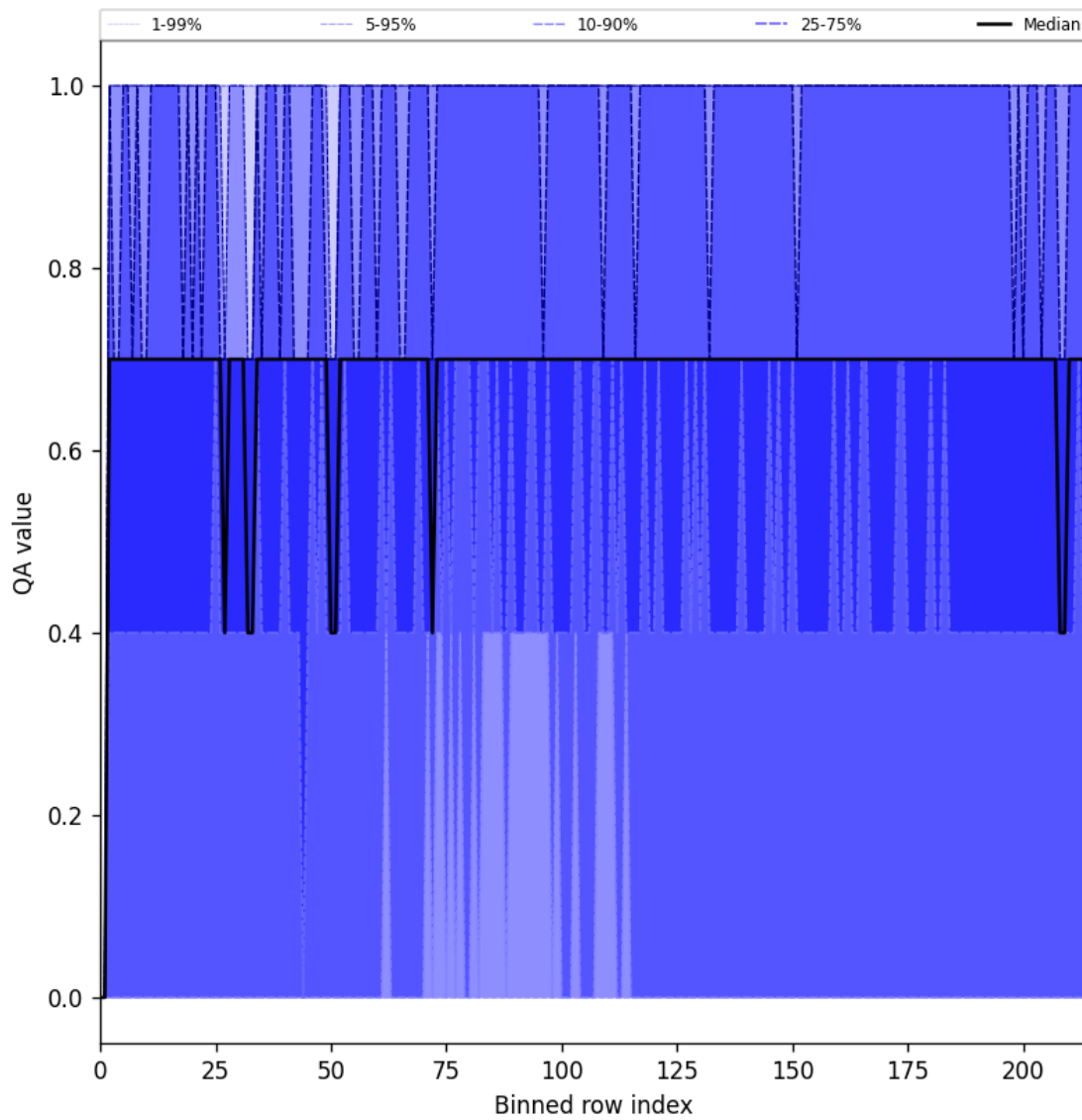
Figure 20: Along track statistics of “QA value” for 2025-04-20 to 2025-04-21
