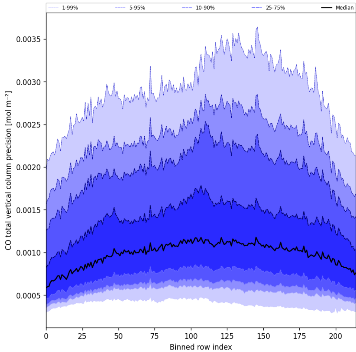
Figure 22: Along track statistics of “CO total vertical column precision” for 2025-04-20 to 2025-04-21
