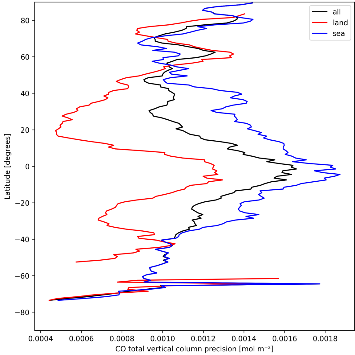
Figure 8: Zonal average of “CO total vertical column precision” for 2025-04-20 to 2025-04-21.
