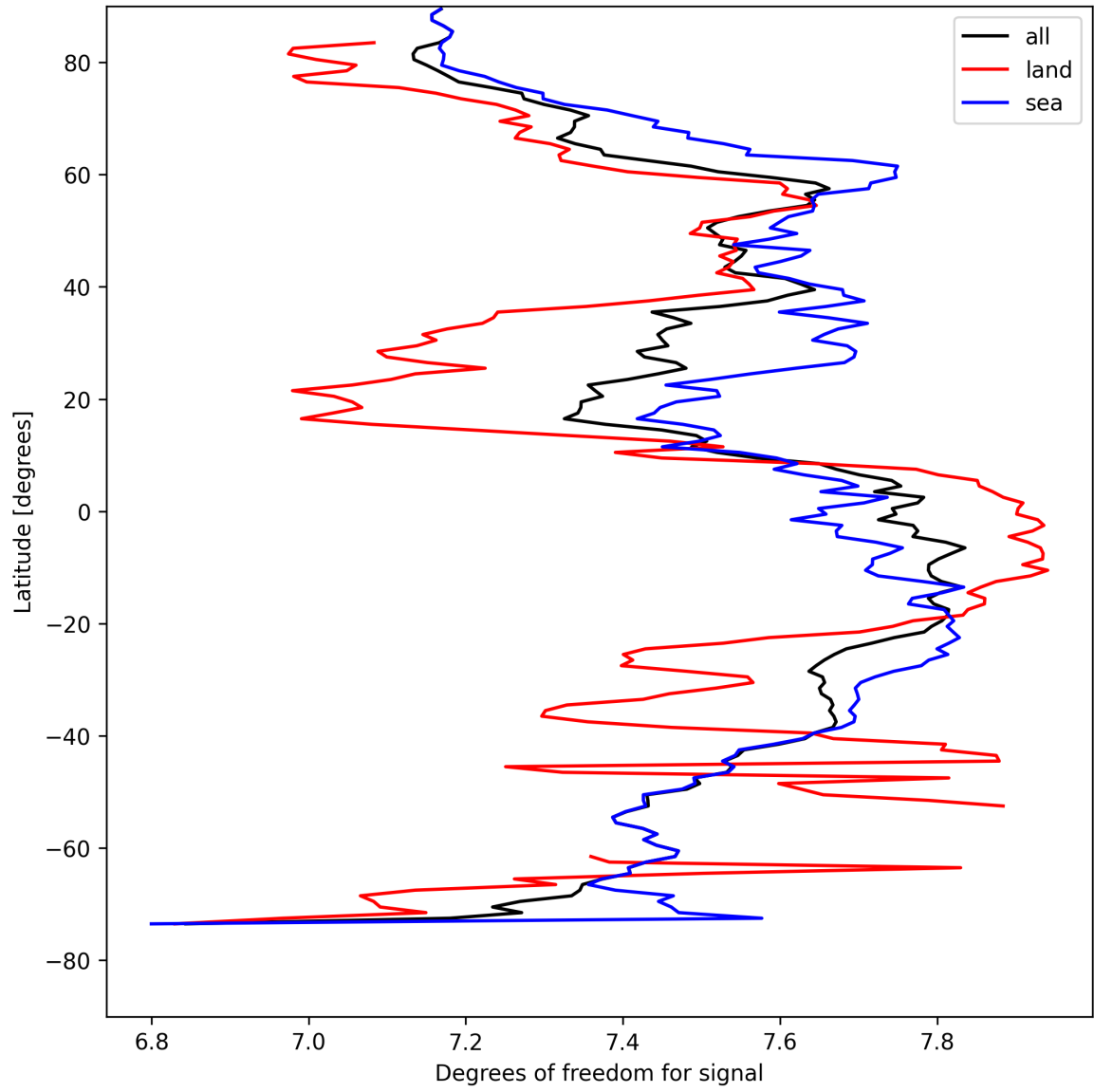
Figure 11: Zonal average of “Degrees of freedom for signal” for 2025-04-20 to 2025-04-21.
