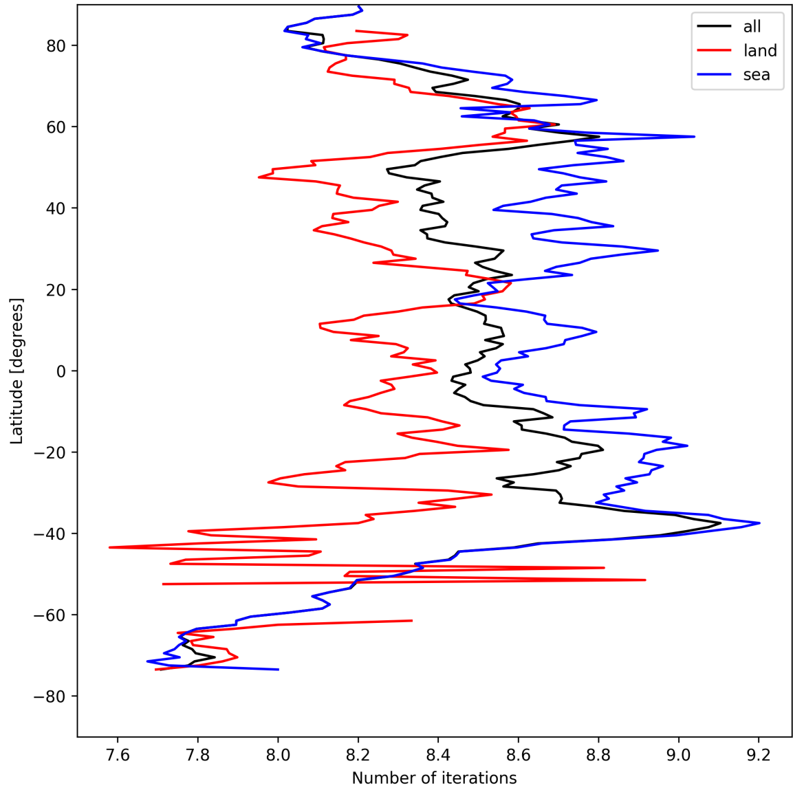
Figure 12: Zonal average of “Number of iterations” for 2025-04-20 to 2025-04-21.
