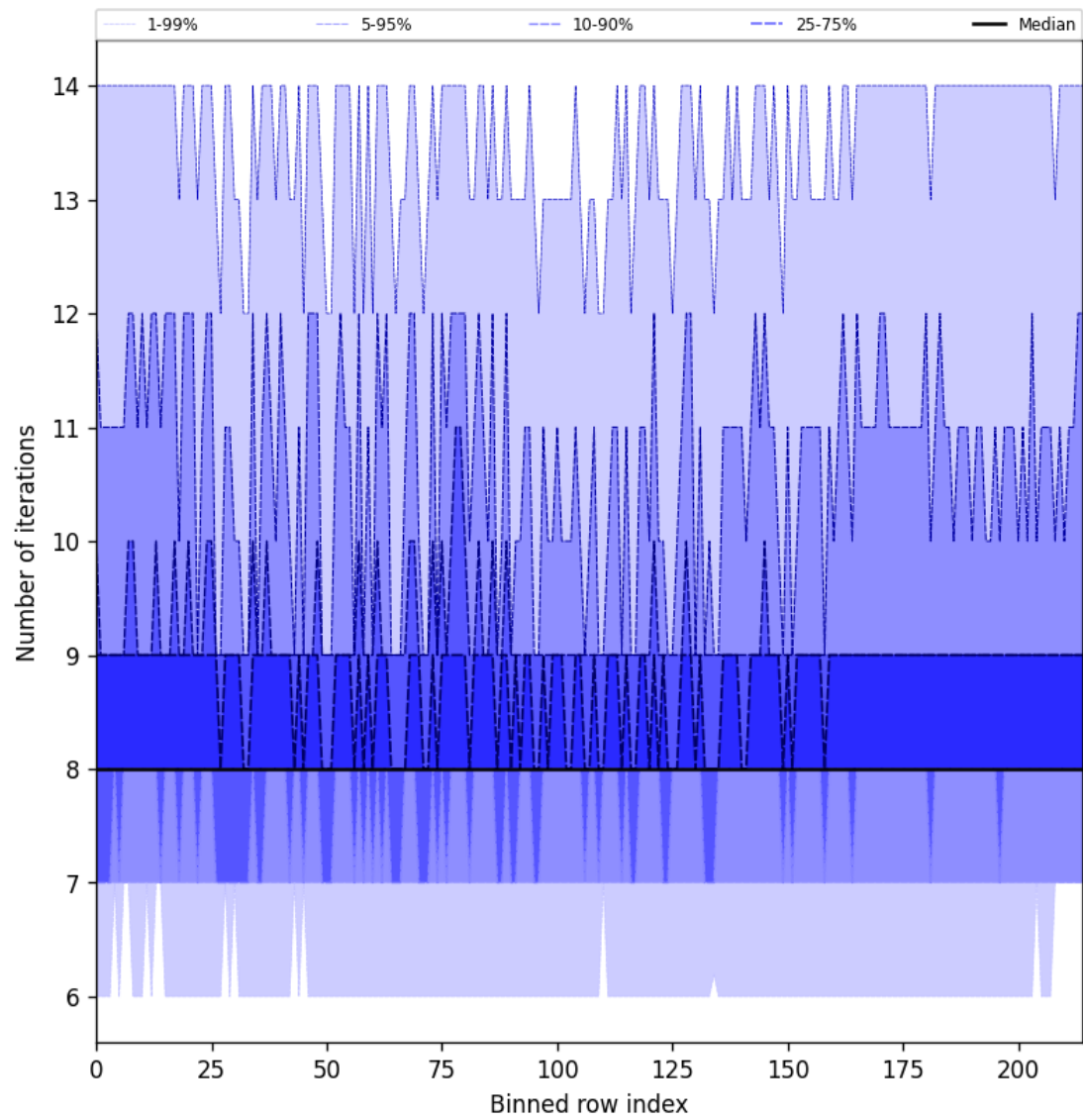
Figure 26: Along track statistics of “Number of iterations” for 2025-04-20 to 2025-04-21
