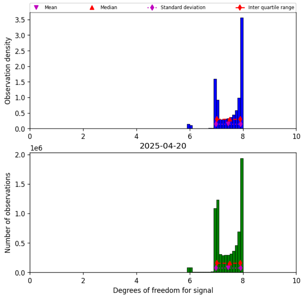
Figure 18: Histogram of “Degrees of freedom for signal” for 2025-04-20 to 2025-04-21
