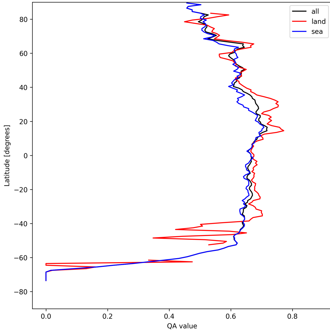
Figure 6: Zonal average of “QA value” for 2025-04-20 to 2025-04-21.
