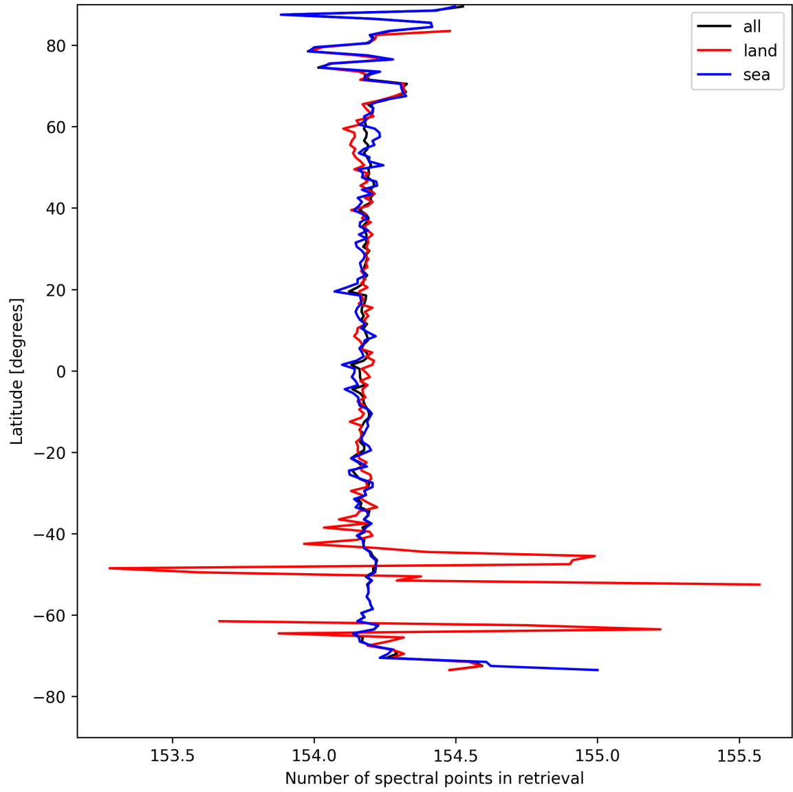
Figure 9: Zonal average of “Number of spectral points in retrieval” for 2025-04-20 to 2025-04-21.
