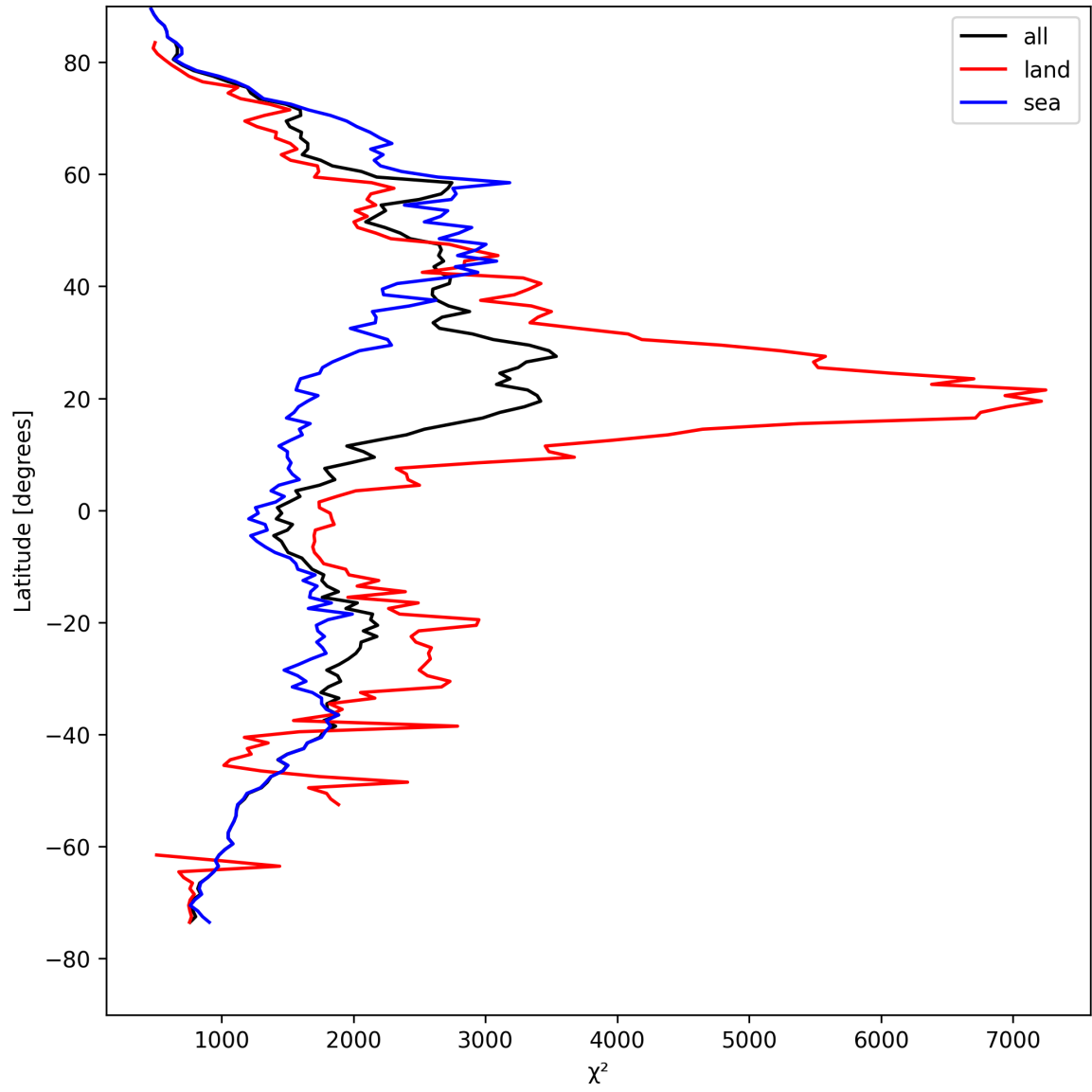
Figure 10: Zonal average of “ \chi^2 ” for 2025-04-20 to 2025-04-21.
