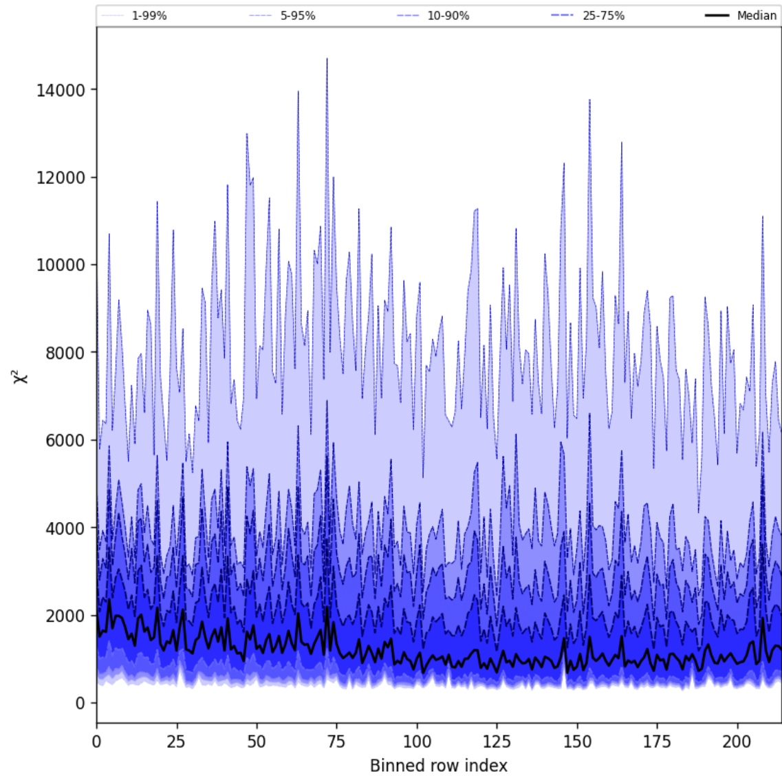
Figure 24: Along track statistics of “ \chi^2 ” for 2025-04-20 to 2025-04-21
