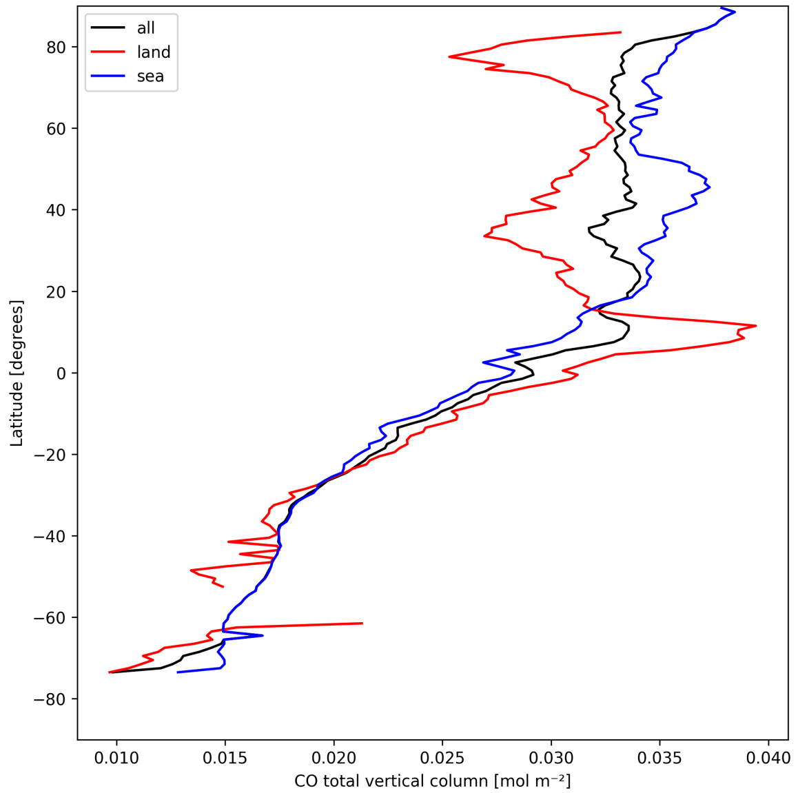
Figure 7: Zonal average of “CO total vertical column” for 2025-04-20 to 2025-04-21.
