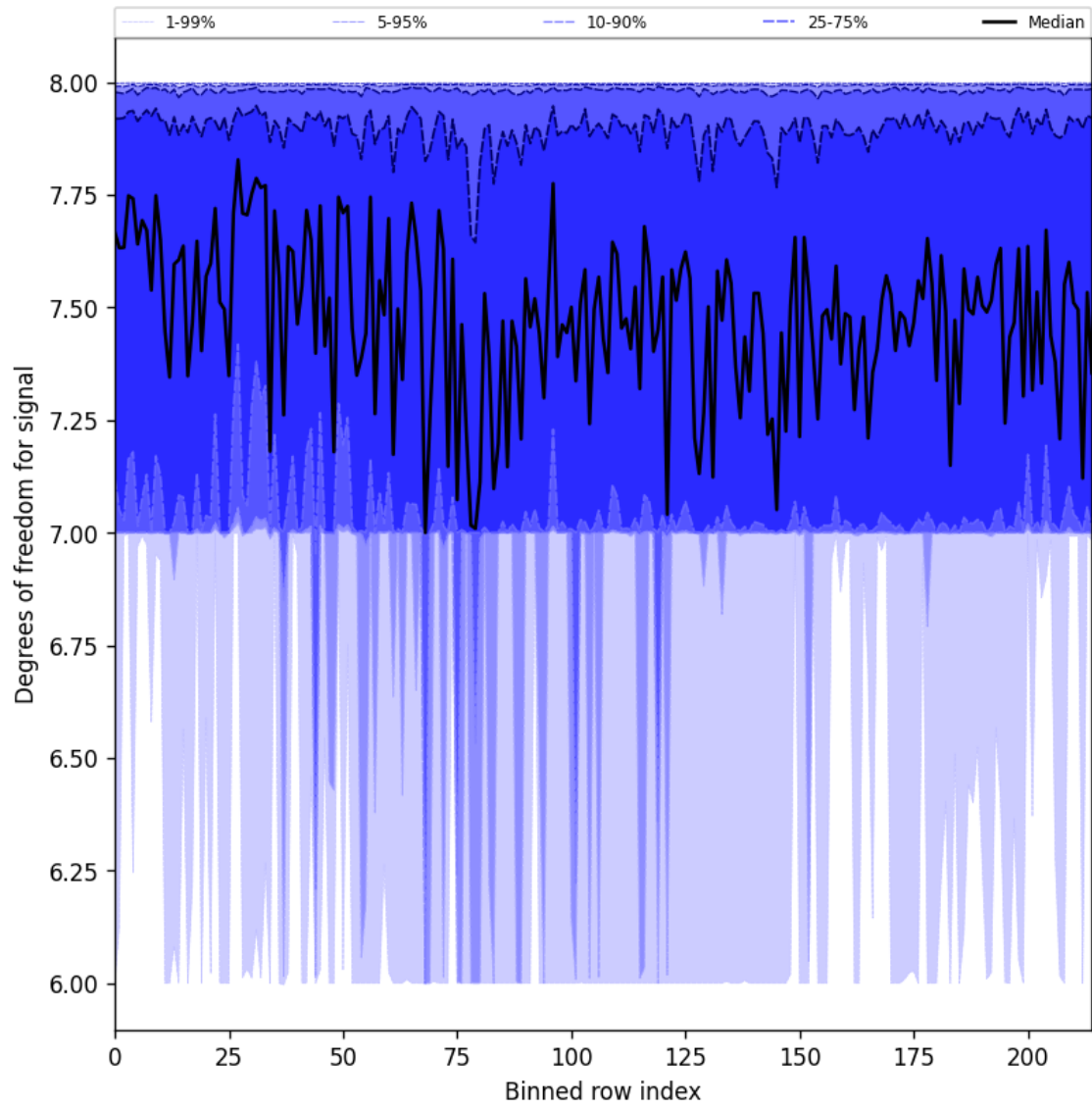
Figure 25: Along track statistics of “Degrees of freedom for signal” for 2025-04-20 to 2025-04-21
