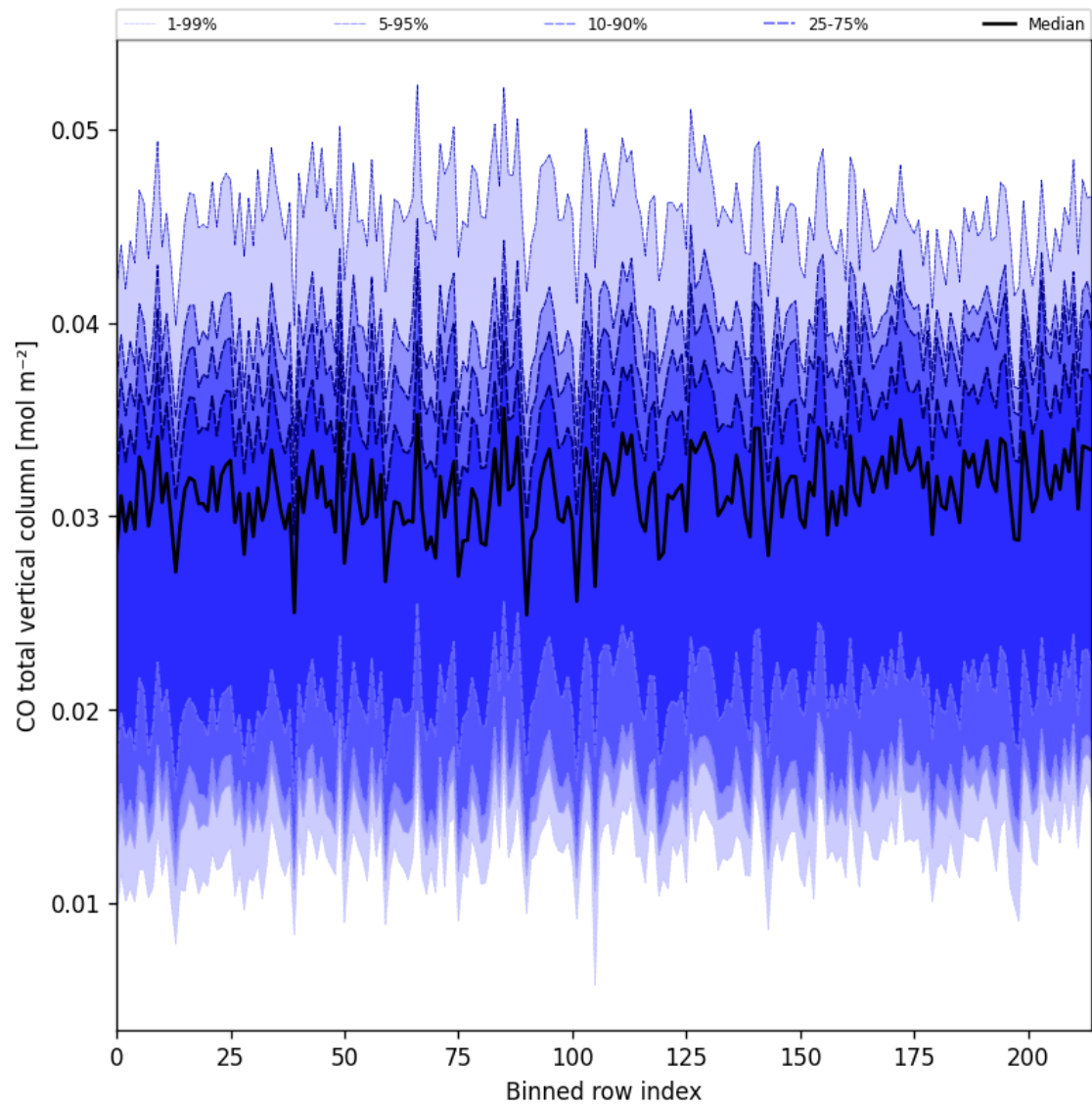
Figure 21: Along track statistics of “CO total vertical column” for 2025-04-20 to 2025-04-21
