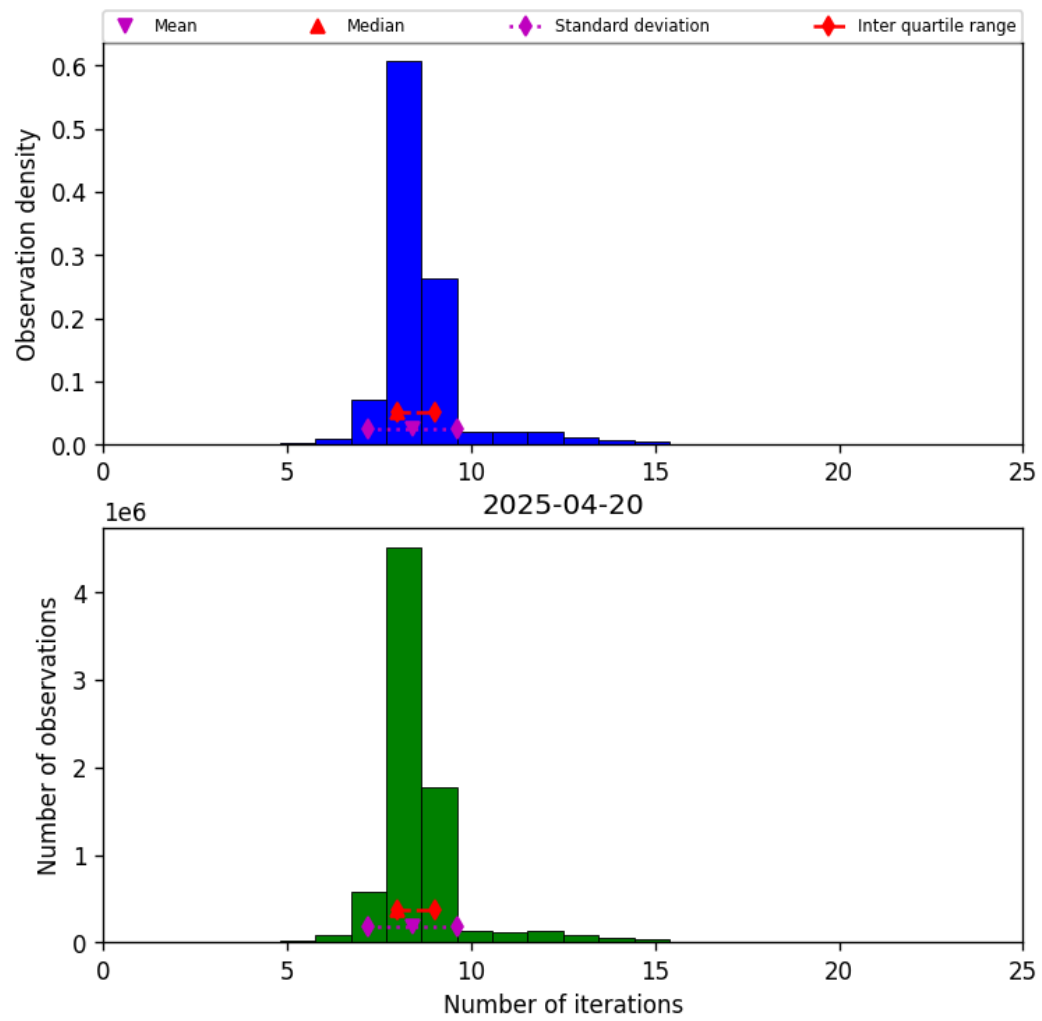
Figure 19: Histogram of “Number of iterations” for 2025-04-20 to 2025-04-21
