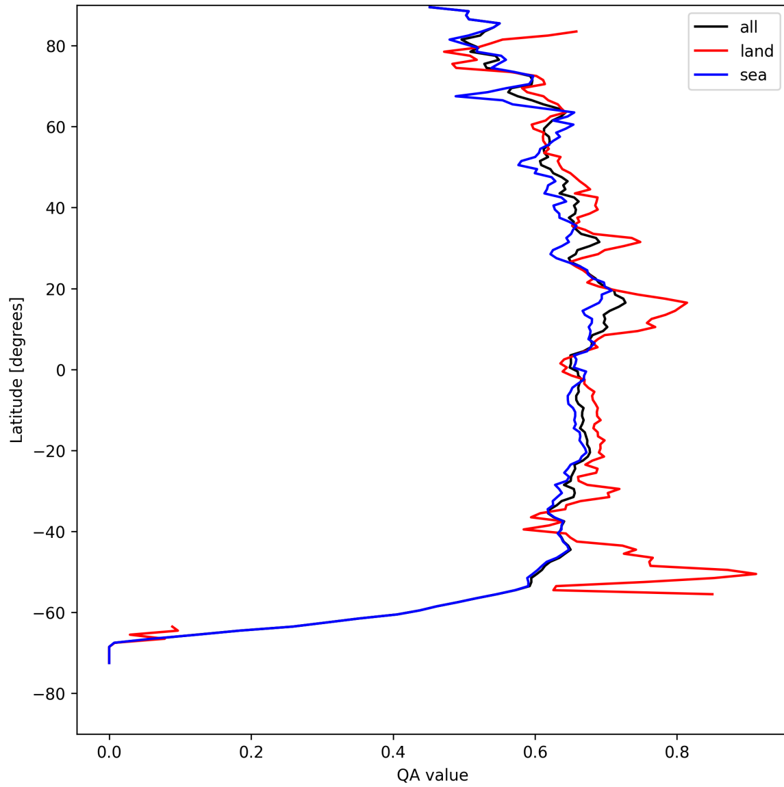
Figure 6: Zonal average of “QA value” for 2025-04-21 to 2025-04-22.
