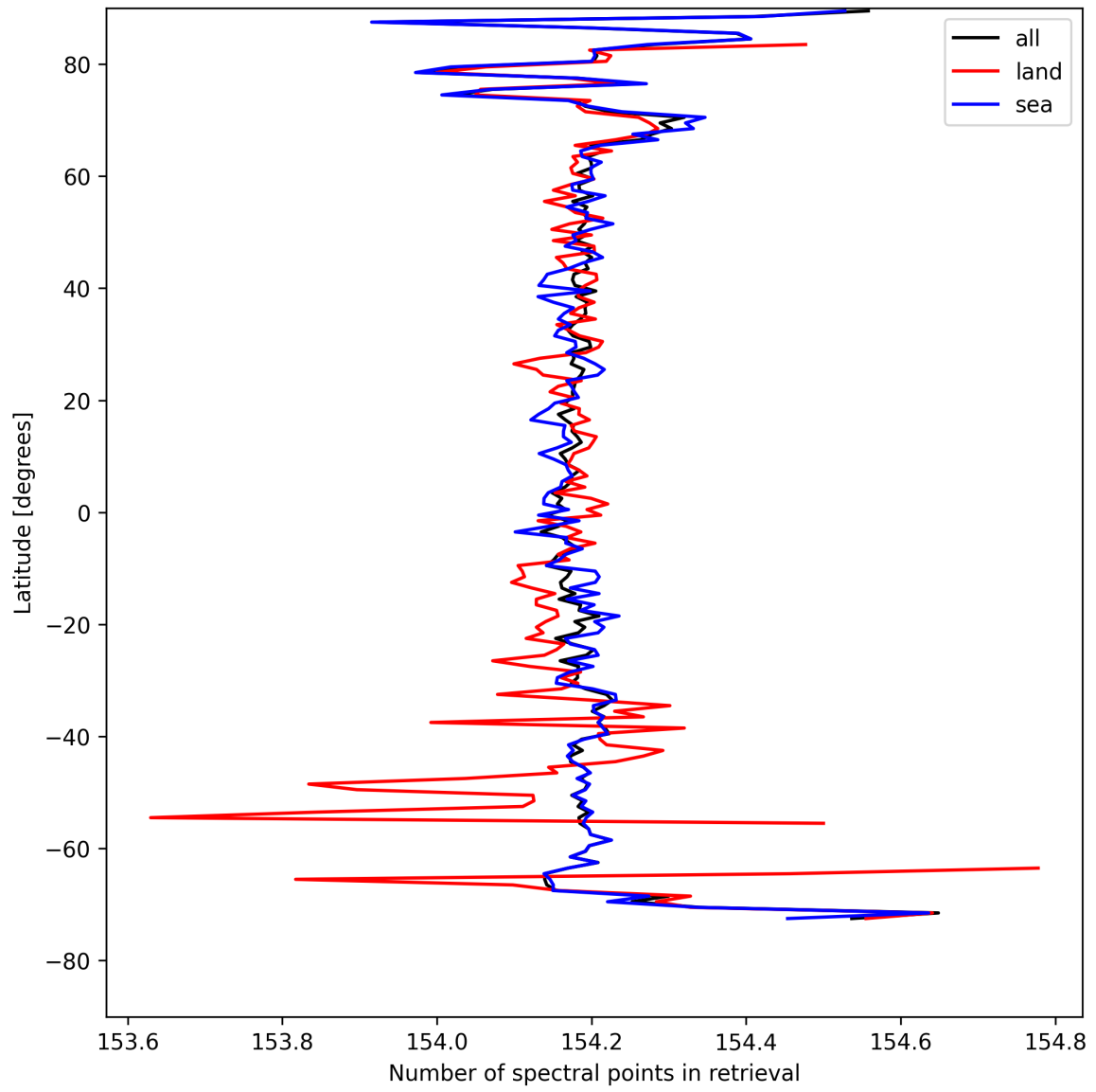
Figure 9: Zonal average of “Number of spectral points in retrieval” for 2025-04-21 to 2025-04-22.
