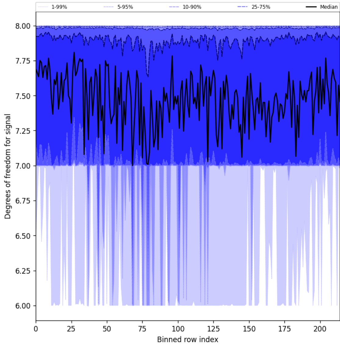
Figure 25: Along track statistics of “Degrees of freedom for signal” for 2025-04-21 to 2025-04-22
