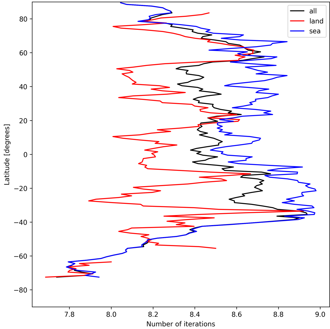
Figure 12: Zonal average of “Number of iterations” for 2025-04-21 to 2025-04-22.
