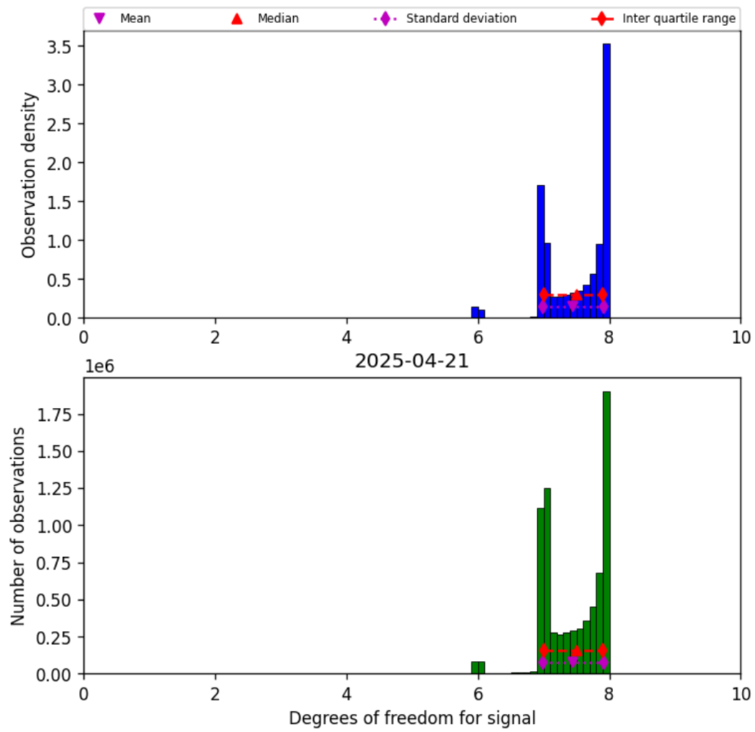
Figure 18: Histogram of “Degrees of freedom for signal” for 2025-04-21 to 2025-04-22
