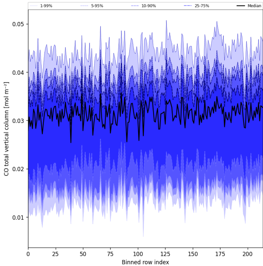
Figure 21: Along track statistics of "CO total vertical column" for 2025-04-21 to 2025-04-22
