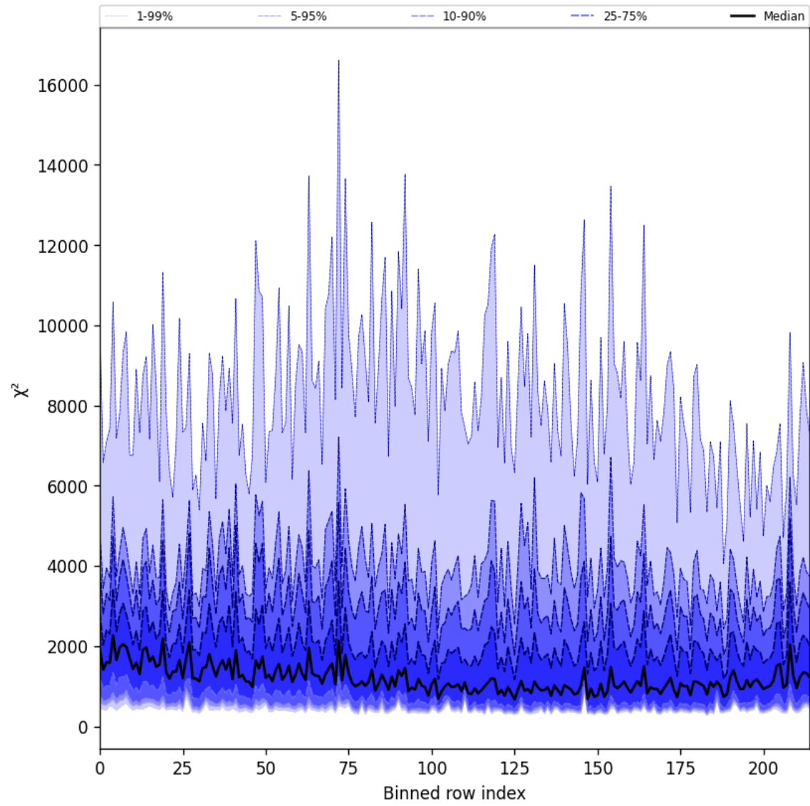
Figure 24: Along track statistics of “ \chi^2 ” for 2025-04-21 to 2025-04-22
