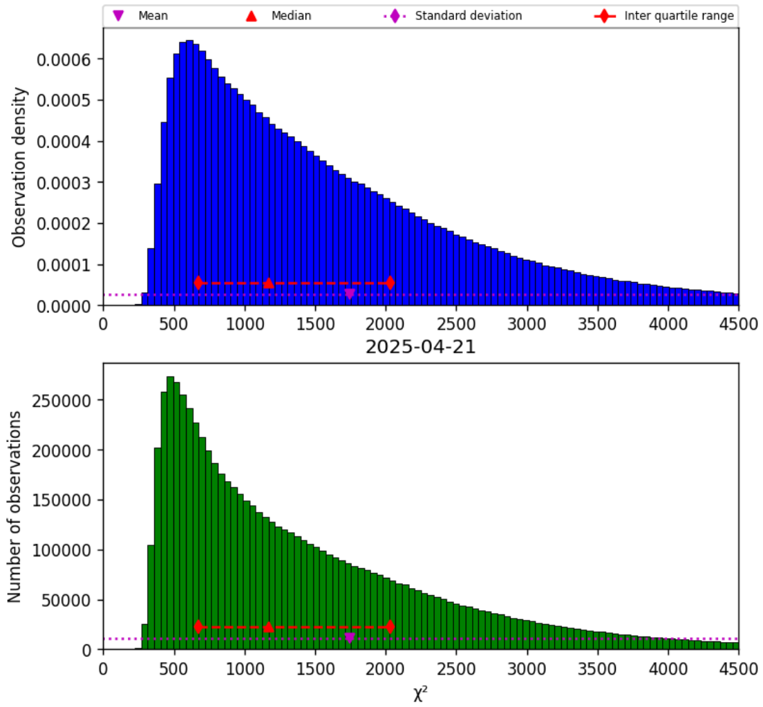
Figure 17: Histogram of “ \chi^2 ” for 2025-04-21 to 2025-04-22
