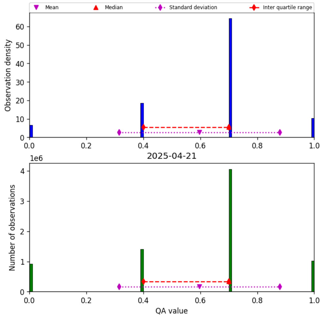
Figure 13: Histogram of “QA value” for 2025-04-21 to 2025-04-22
