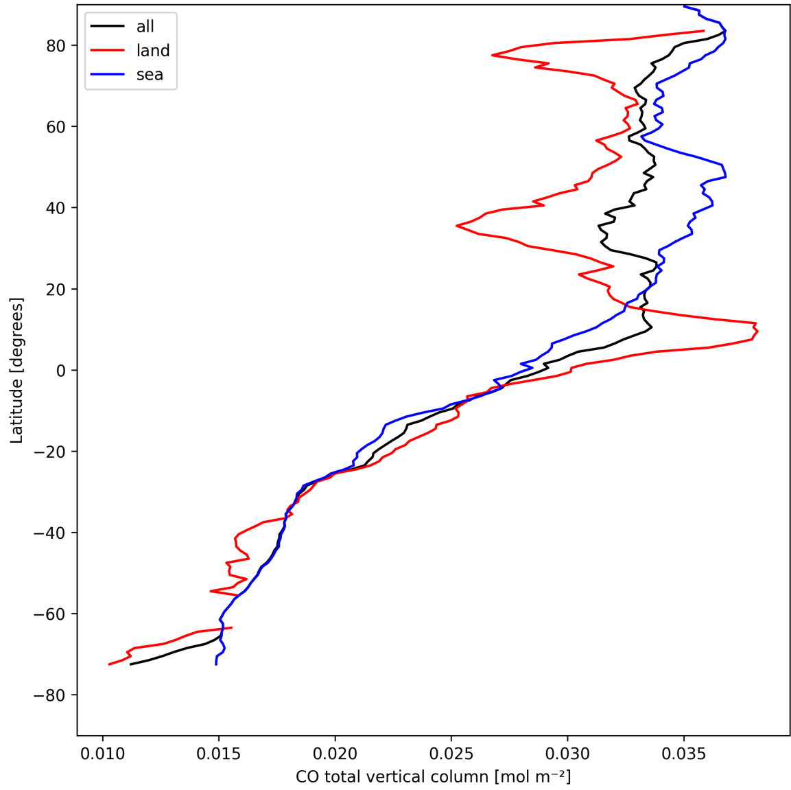
Figure 7: Zonal average of “CO total vertical column” for 2025-04-21 to 2025-04-22.
