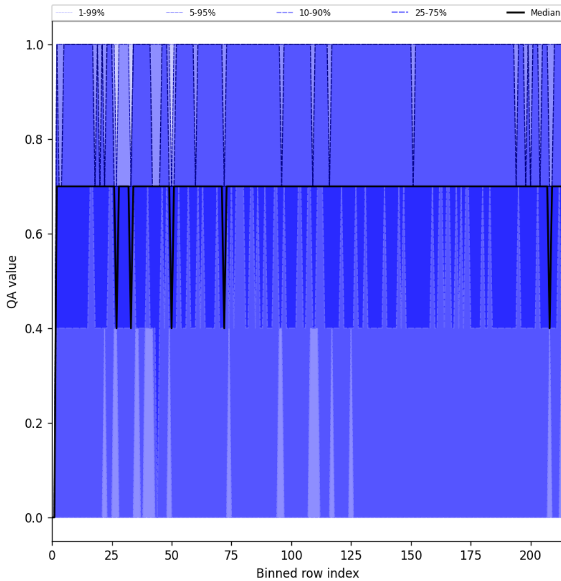
Figure 20: Along track statistics of “QA value” for 2025-04-21 to 2025-04-22
