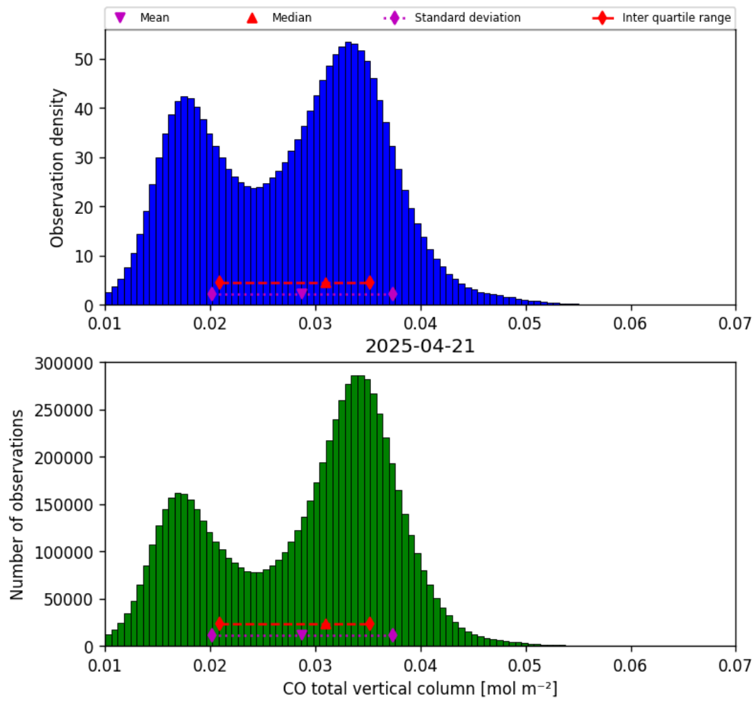
Figure 14: Histogram of “CO total vertical column” for 2025-04-21 to 2025-04-22
