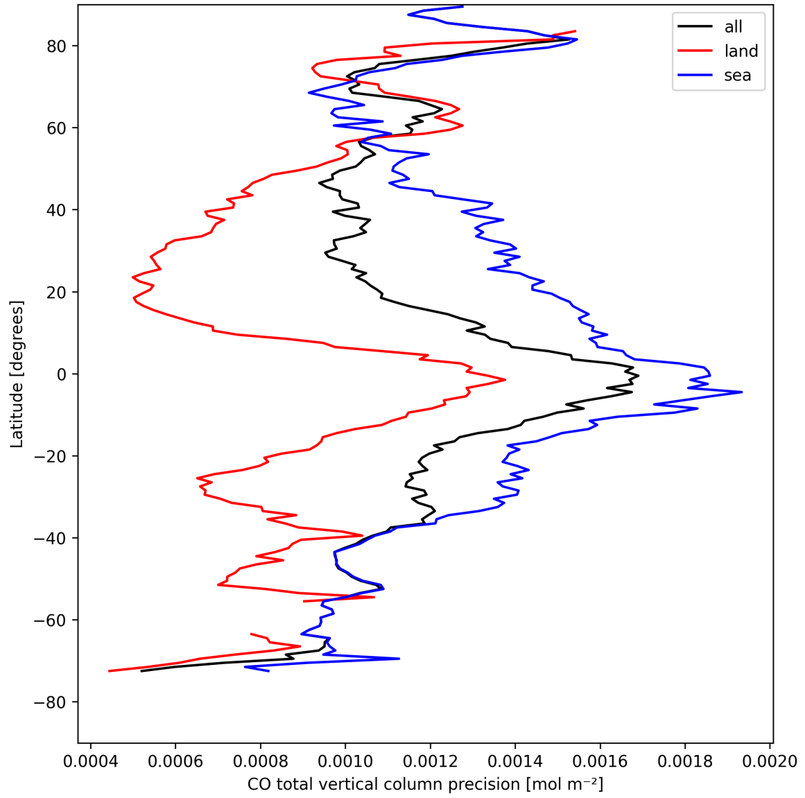
Figure 8: Zonal average of “CO total vertical column precision” for 2025-04-21 to 2025-04-22.
