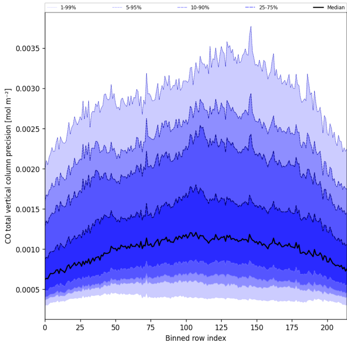
Figure 22: Along track statistics of “CO total vertical column precision” for 2025-04-21 to 2025-04-22
