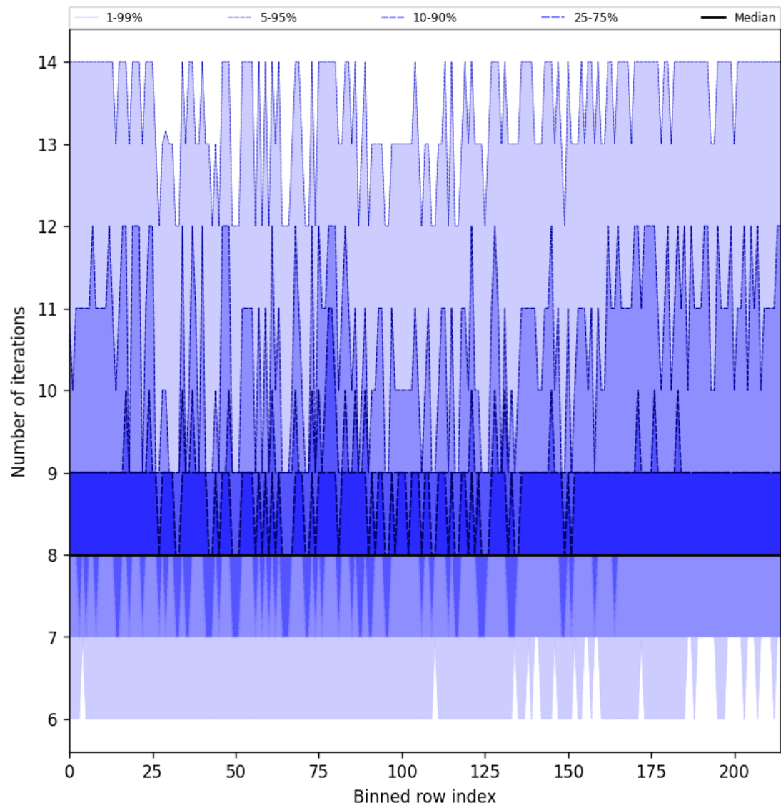
Figure 26: Along track statistics of “Number of iterations” for 2025-04-21 to 2025-04-22
