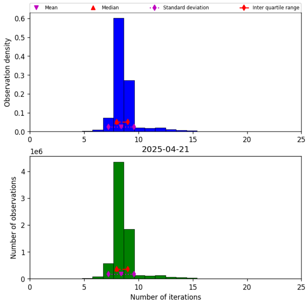
Figure 19: Histogram of “Number of iterations” for 2025-04-21 to 2025-04-22
