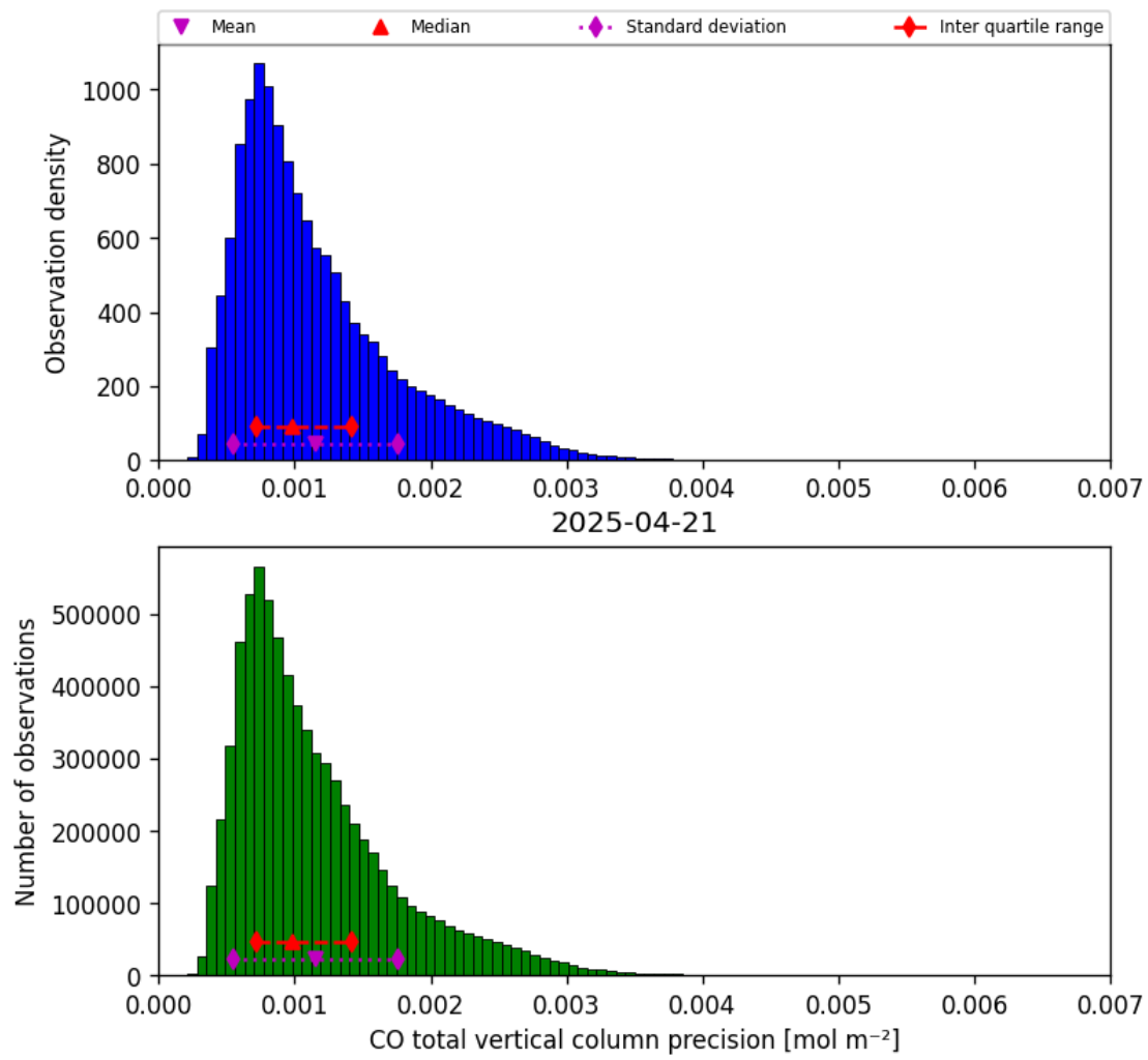
Figure 15: Histogram of “CO total vertical column precision” for 2025-04-21 to 2025-04-22
