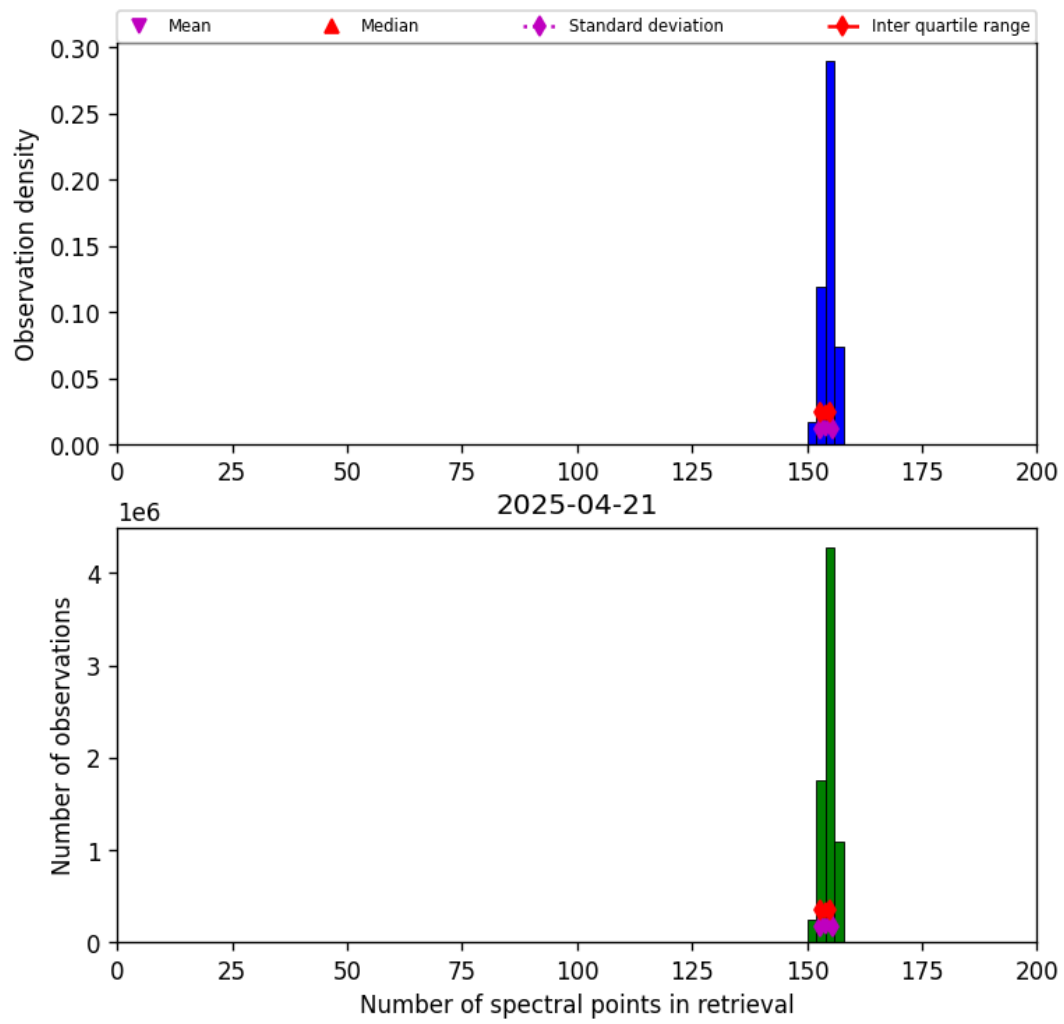
Figure 16: Histogram of “Number of spectral points in retrieval” for 2025-04-21 to 2025-04-22
