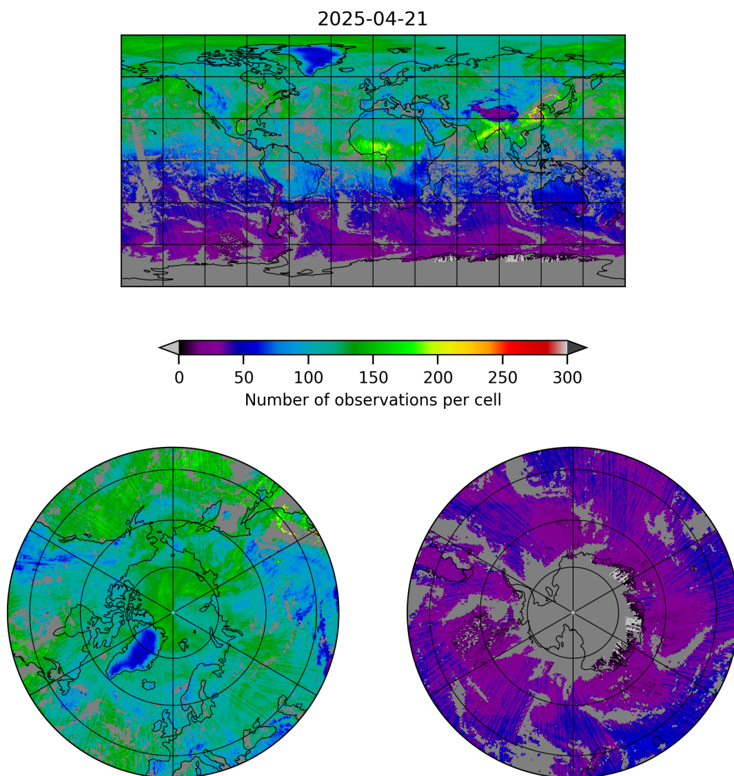
Figure 5: Map of the number of observations for 2025-04-21 to 2025-04-22
