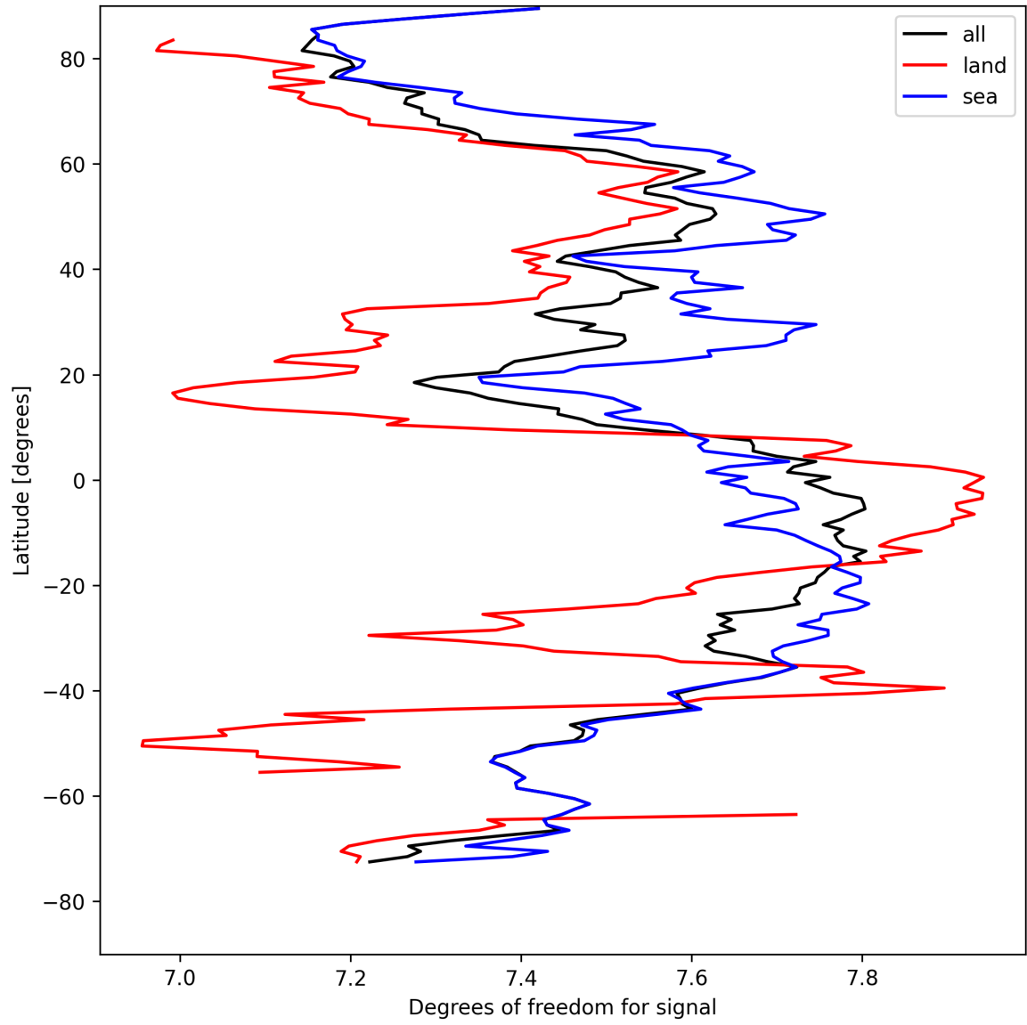
Figure 11: Zonal average of “Degrees of freedom for signal” for 2025-04-21 to 2025-04-22.
