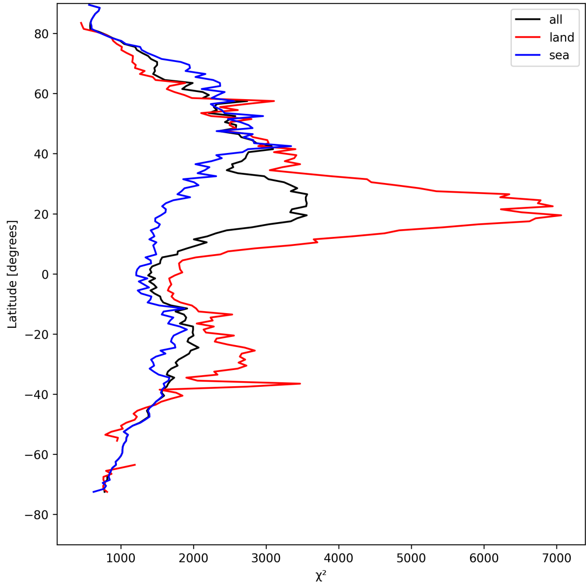
Figure 10: Zonal average of “ \chi^2 ” for 2025-04-21 to 2025-04-22.
