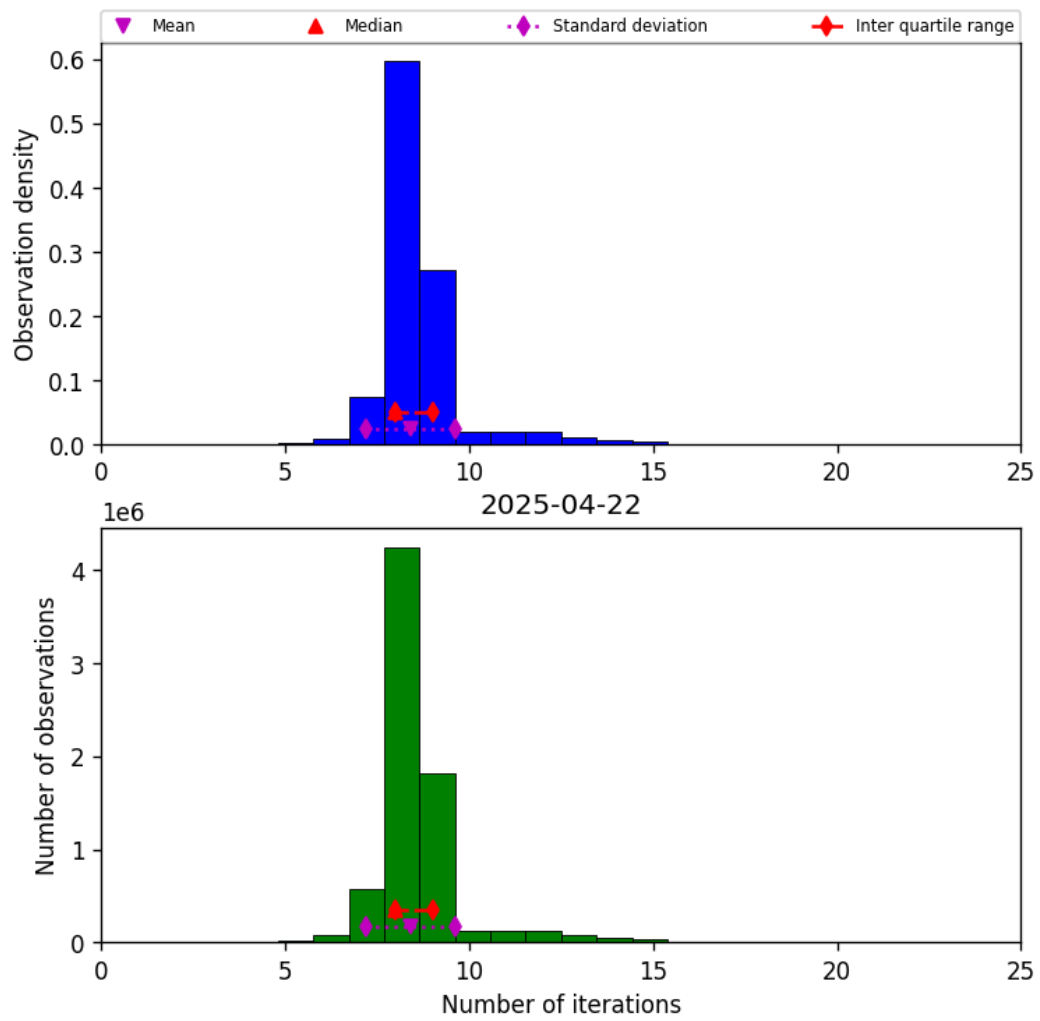
Figure 19: Histogram of “Number of iterations” for 2025-04-22 to 2025-04-22
