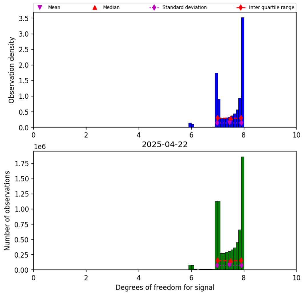
Figure 18: Histogram of “Degrees of freedom for signal” for 2025-04-22 to 2025-04-22
