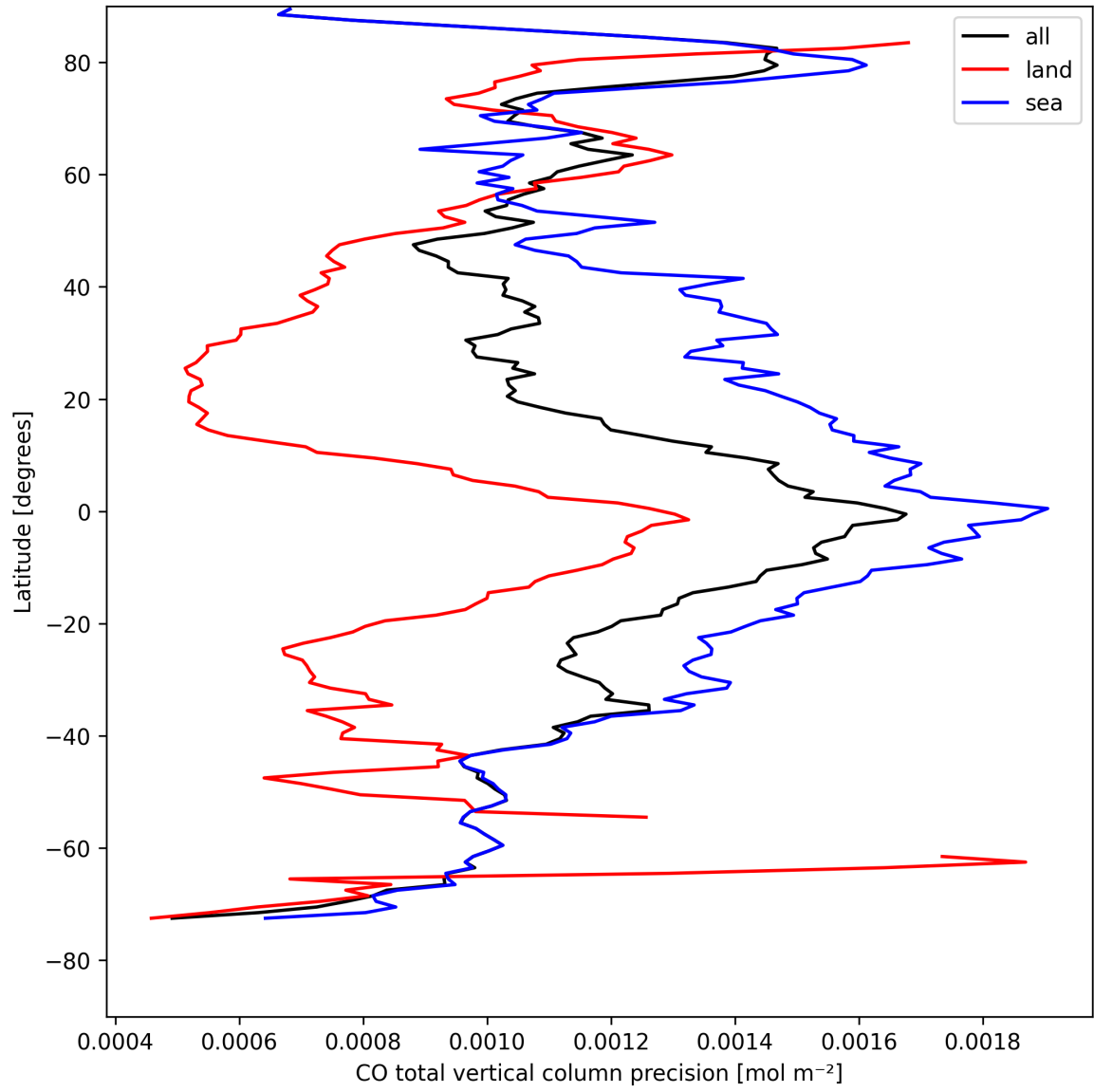
Figure 8: Zonal average of “CO total vertical column precision” for 2025-04-22 to 2025-04-22.
