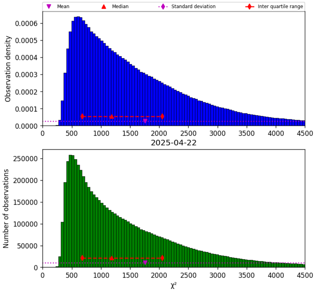
Figure 17: Histogram of " \chi^2 " for 2025-04-22 to 2025-04-22
