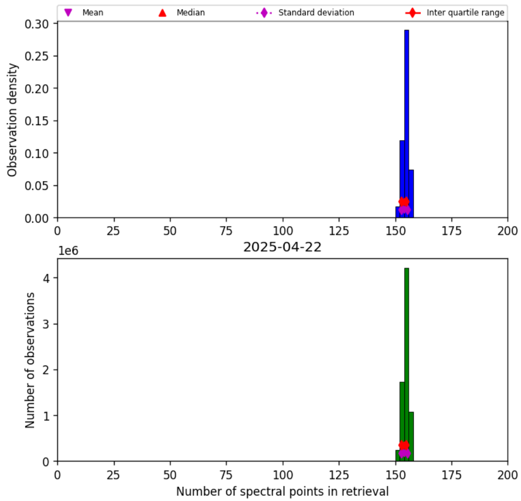
Figure 16: Histogram of “Number of spectral points in retrieval” for 2025-04-22 to 2025-04-22
