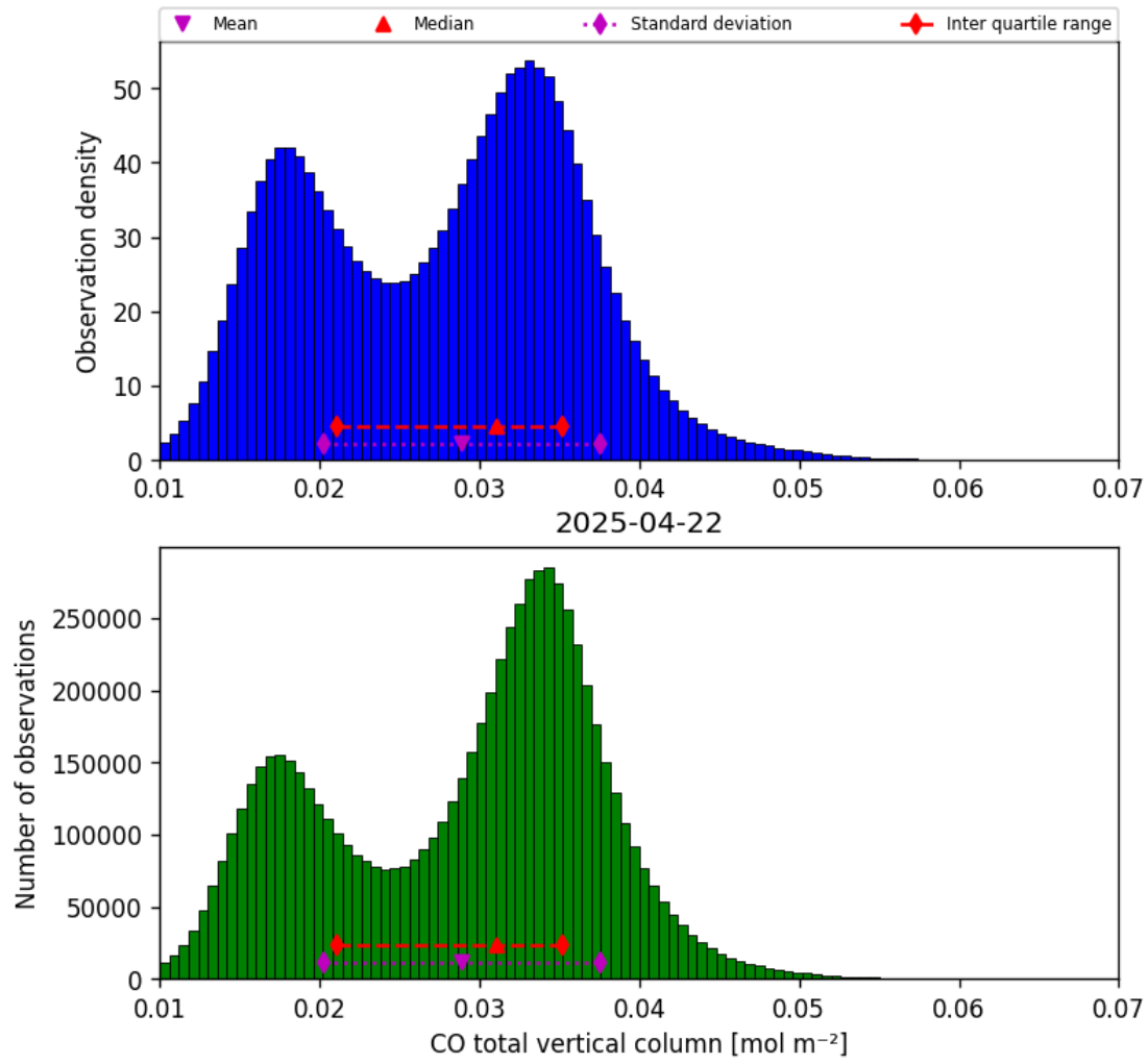
Figure 14: Histogram of “CO total vertical column” for 2025-04-22 to 2025-04-22
