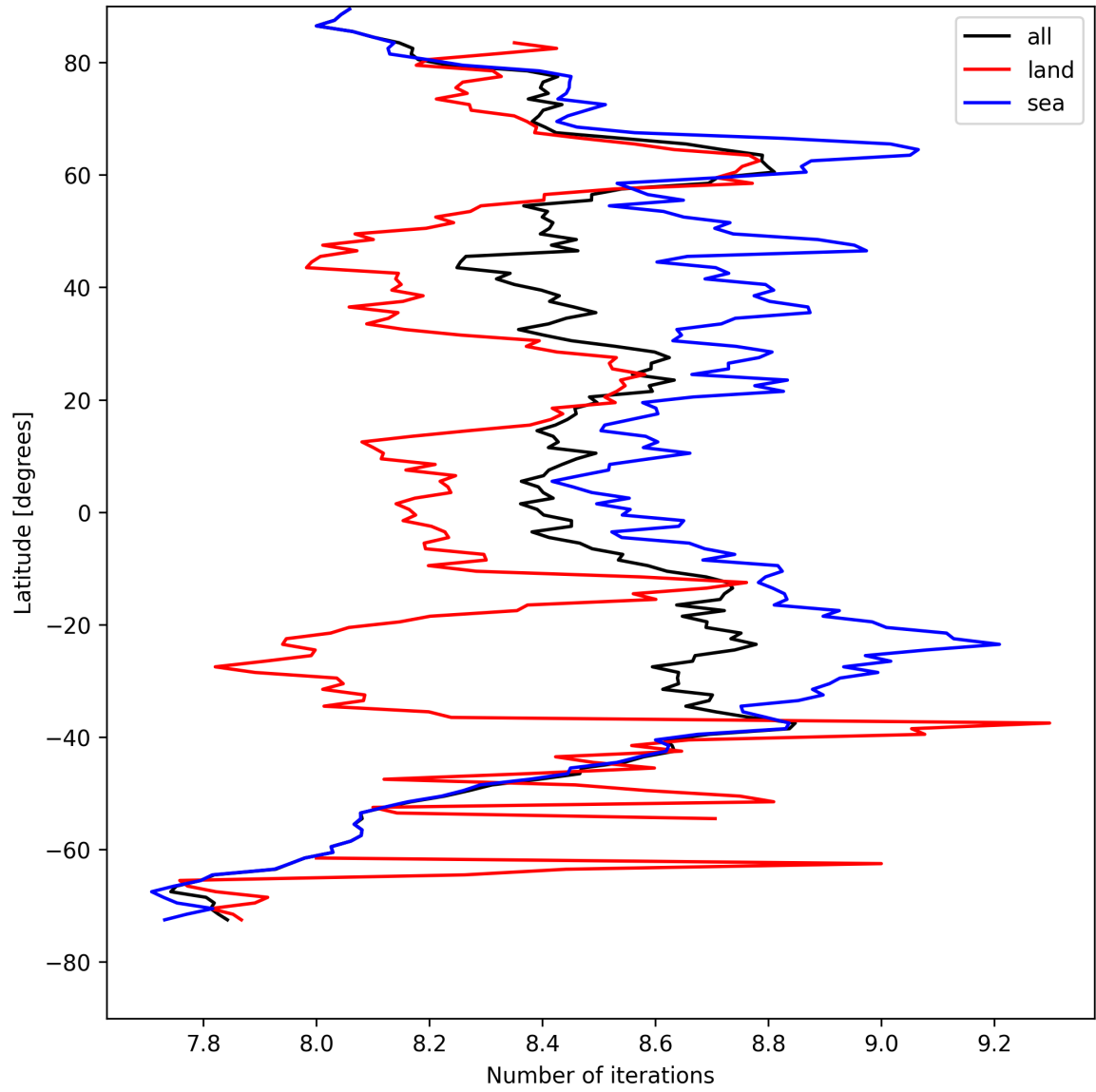
Figure 12: Zonal average of “Number of iterations” for 2025-04-22 to 2025-04-22.
