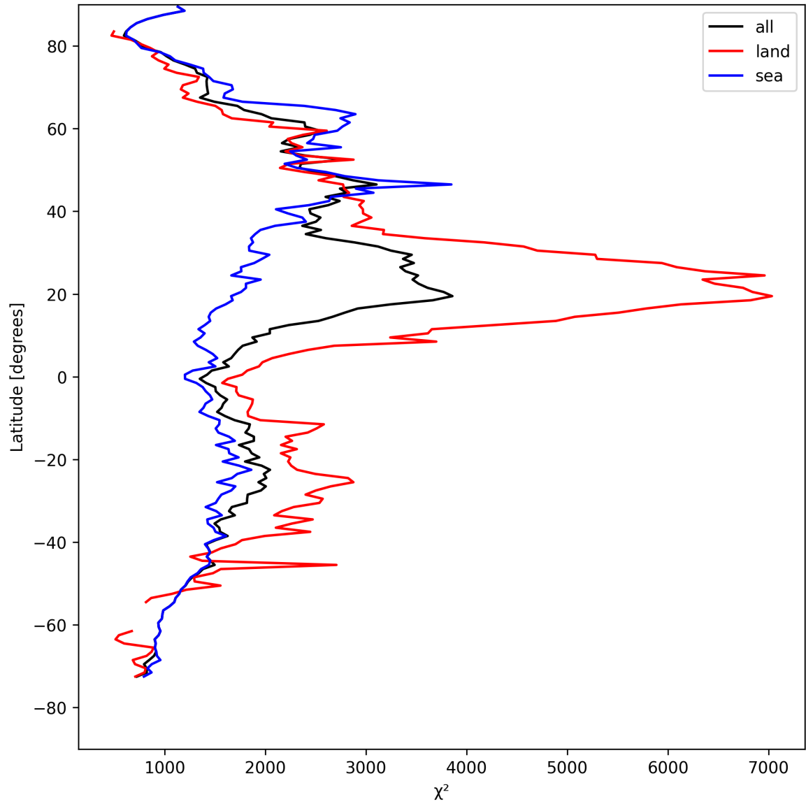
Figure 10: Zonal average of “ \chi^2 ” for 2025-04-22 to 2025-04-22.
