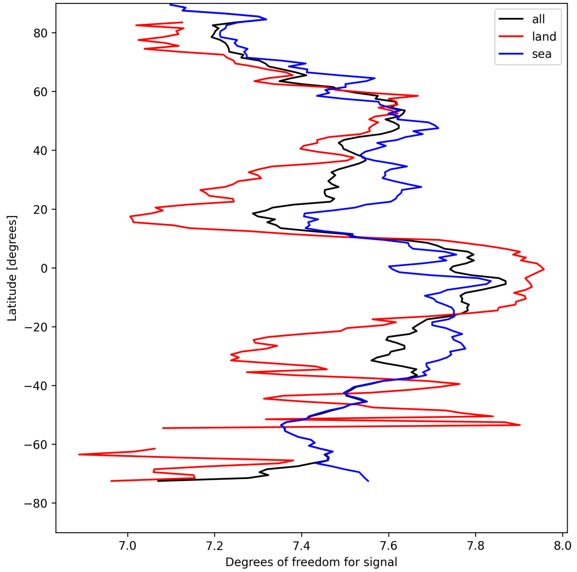
Figure 11: Zonal average of “Degrees of freedom for signal” for 2025-04-22 to 2025-04-22.
