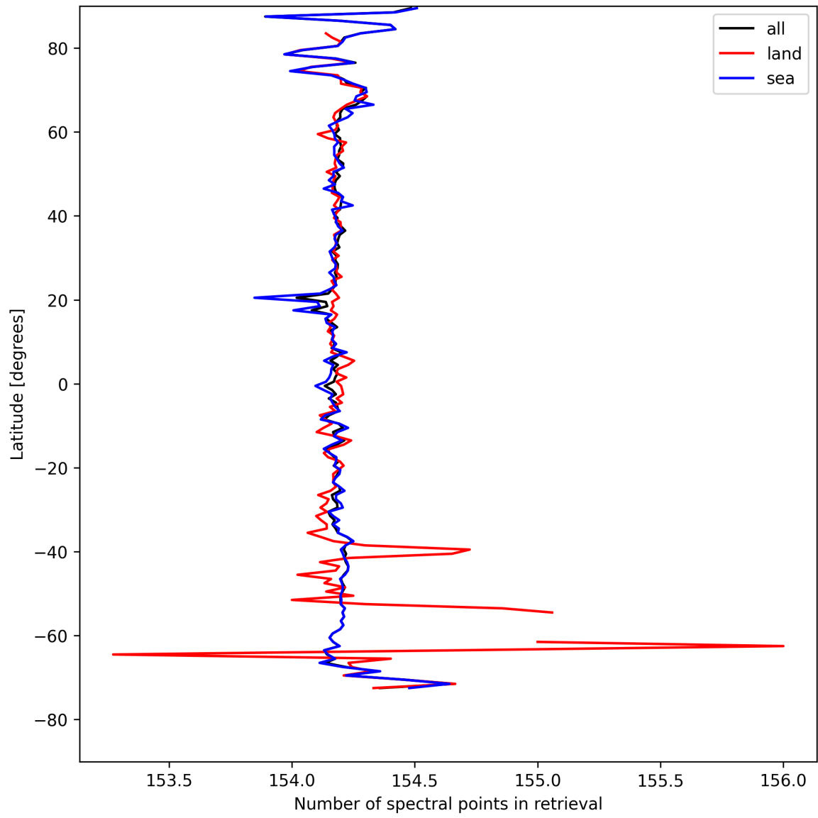
Figure 9: Zonal average of “Number of spectral points in retrieval” for 2025-04-22 to 2025-04-22.
