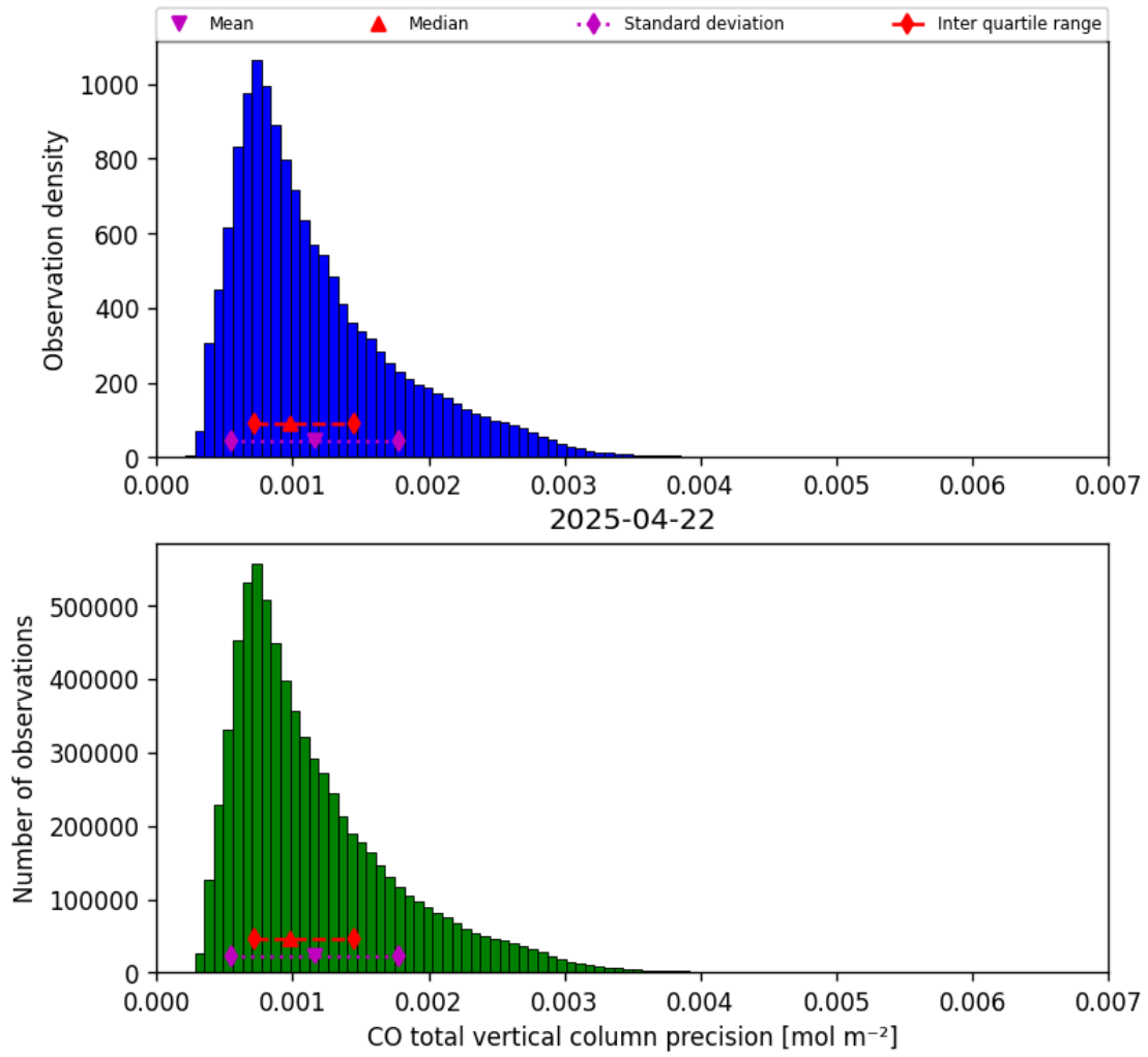
Figure 15: Histogram of “CO total vertical column precision” for 2025-04-22 to 2025-04-22
