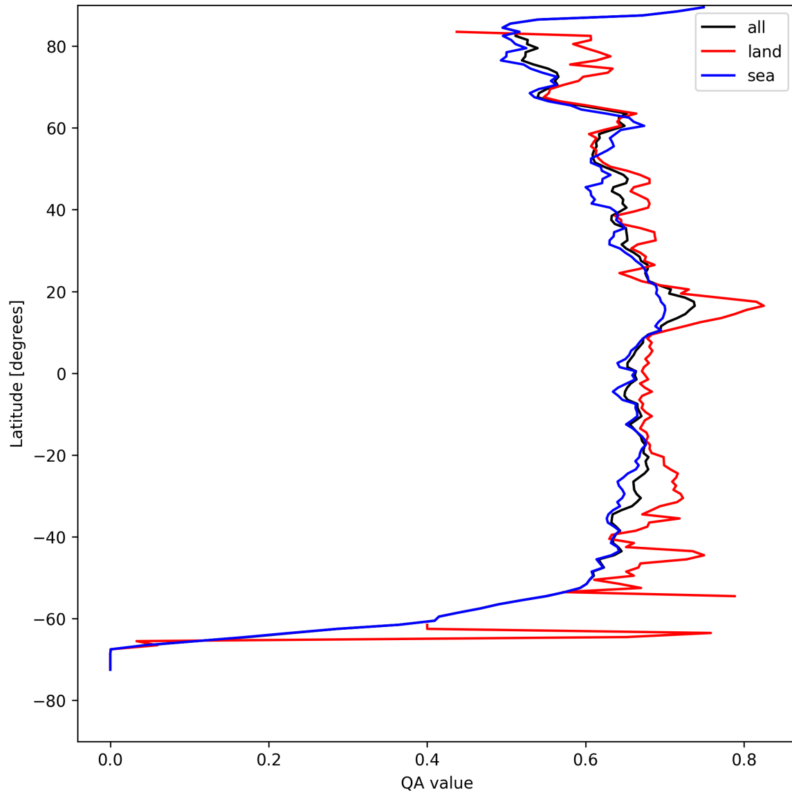
Figure 6: Zonal average of “QA value” for 2025-04-22 to 2025-04-22.
