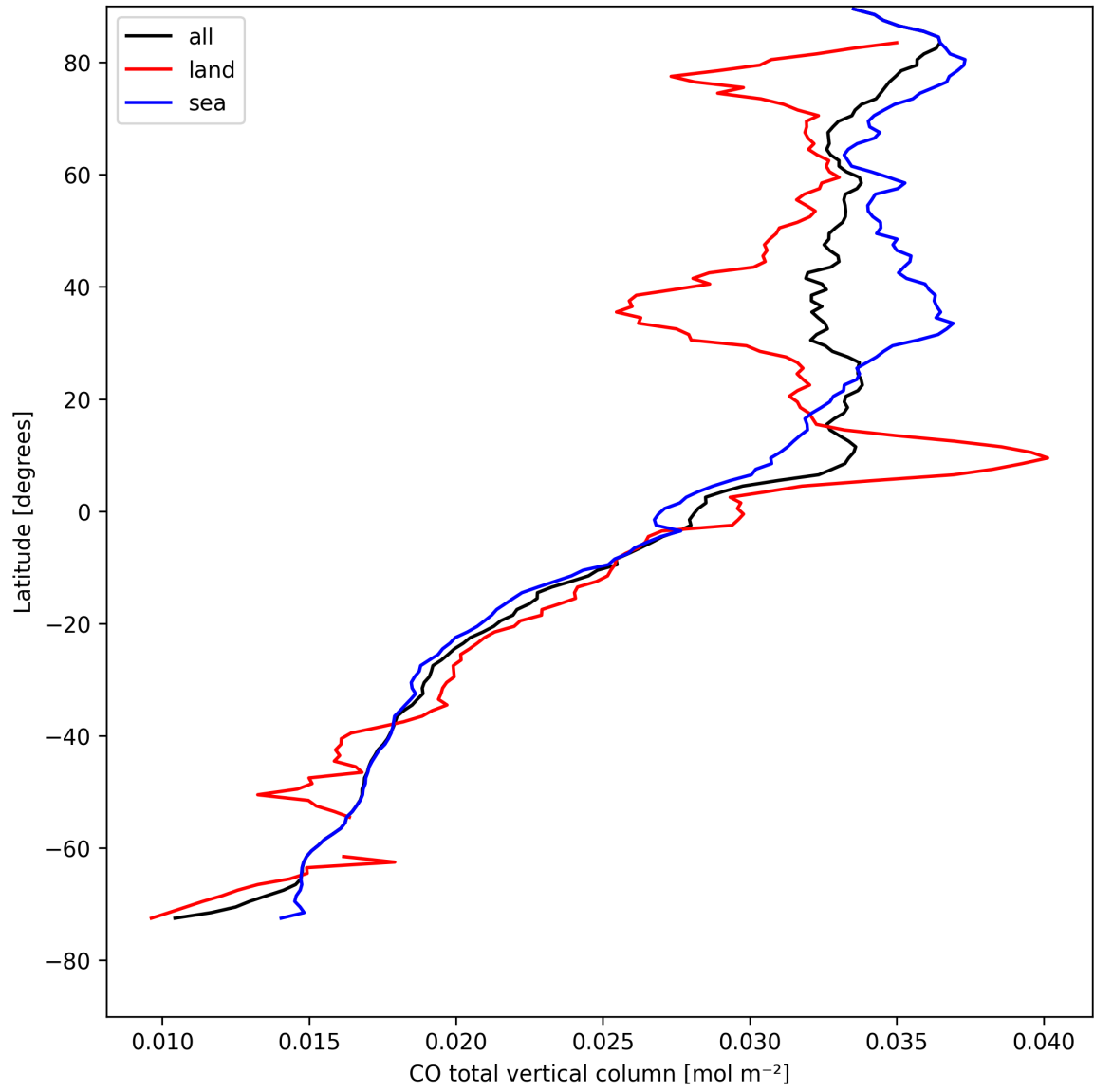
Figure 7: Zonal average of “CO total vertical column” for 2025-04-22 to 2025-04-22.
