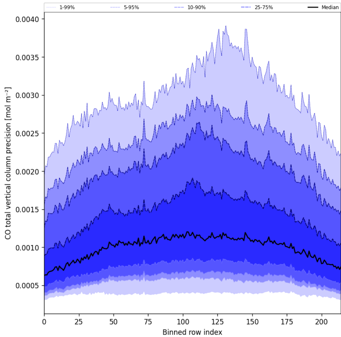
Figure 22: Along track statistics of “CO total vertical column precision” for 2025-04-22 to 2025-04-22
