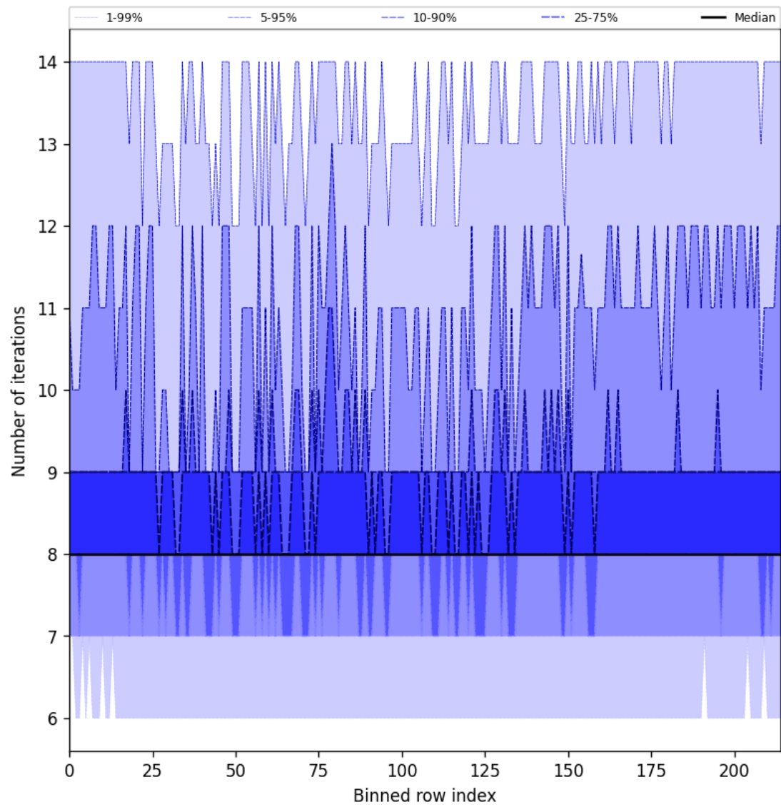
Figure 26: Along track statistics of “Number of iterations” for 2025-04-22 to 2025-04-22
