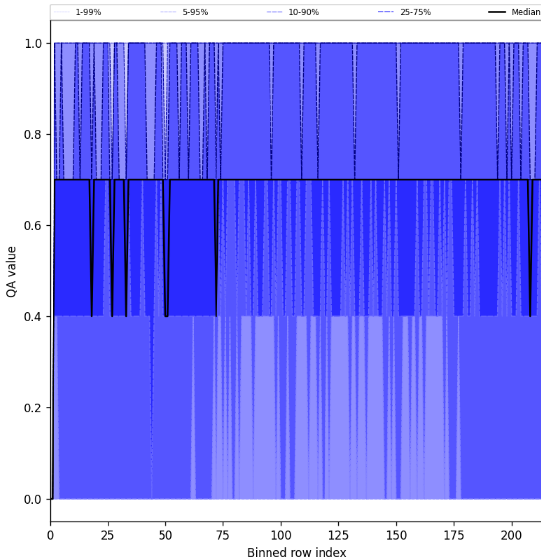
Figure 20: Along track statistics of “QA value” for 2025-04-22 to 2025-04-22
