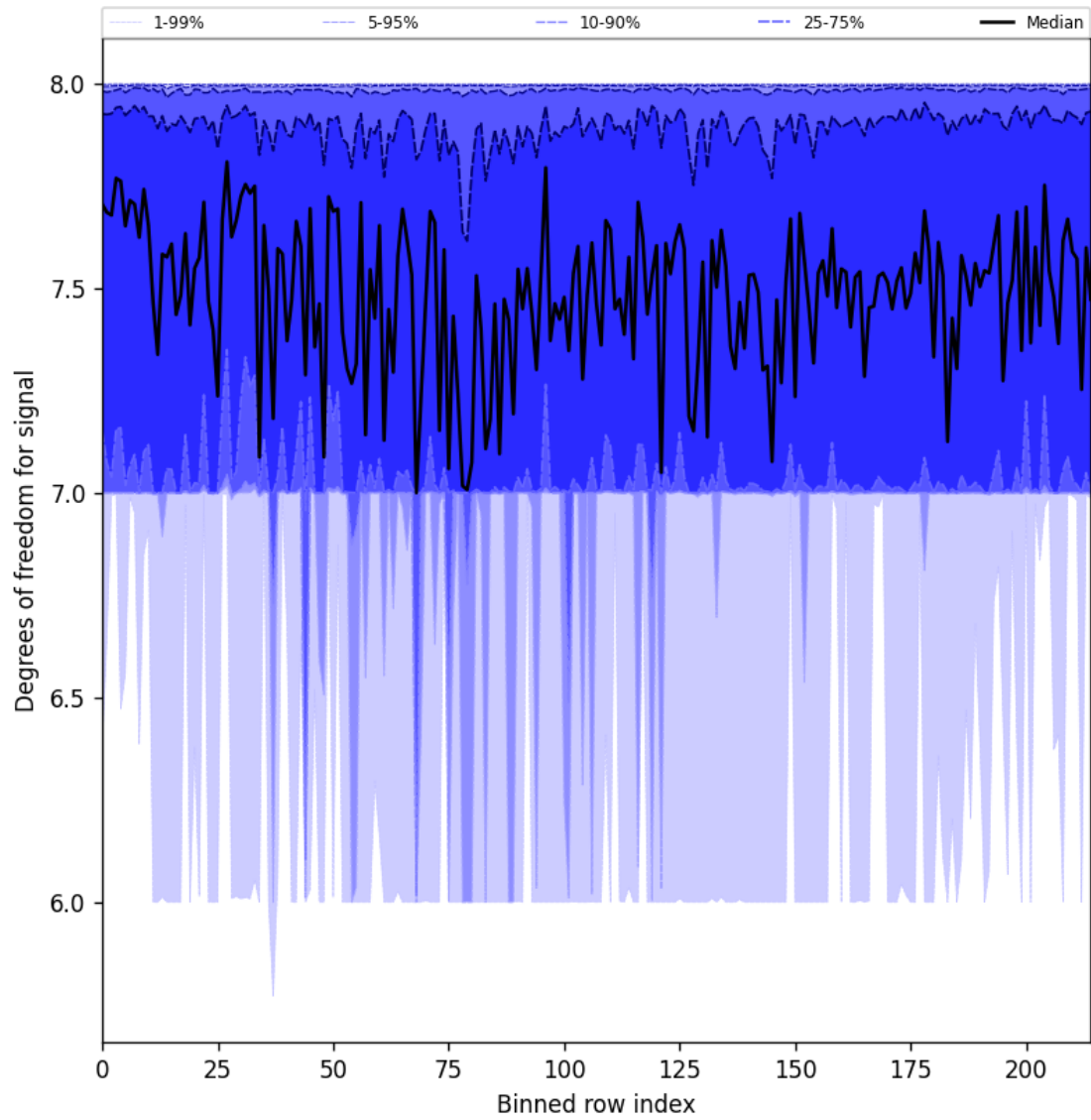
Figure 25: Along track statistics of “Degrees of freedom for signal” for 2025-04-22 to 2025-04-22
