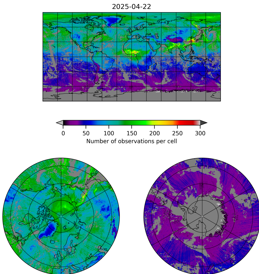
Figure 5: Map of the number of observations for 2025-04-22 to 2025-04-22
