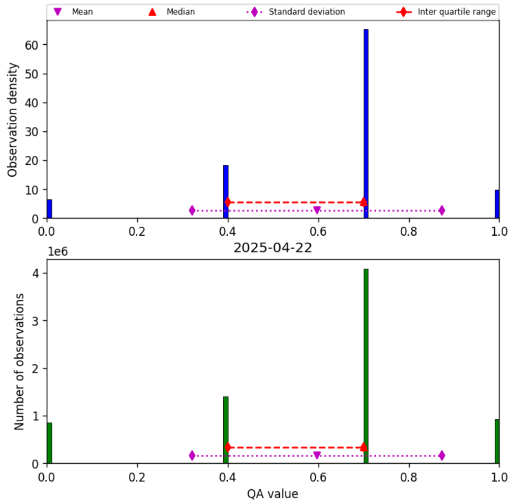
Figure 13: Histogram of “QA value” for 2025-04-22 to 2025-04-22
