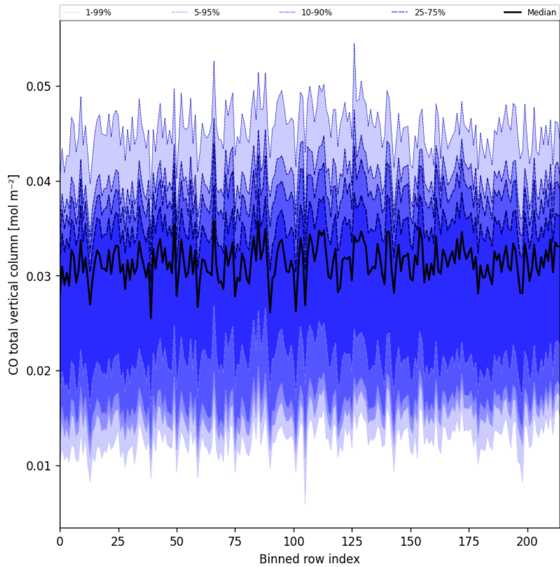
Figure 21: Along track statistics of “CO total vertical column” for 2025-04-22 to 2025-04-22
