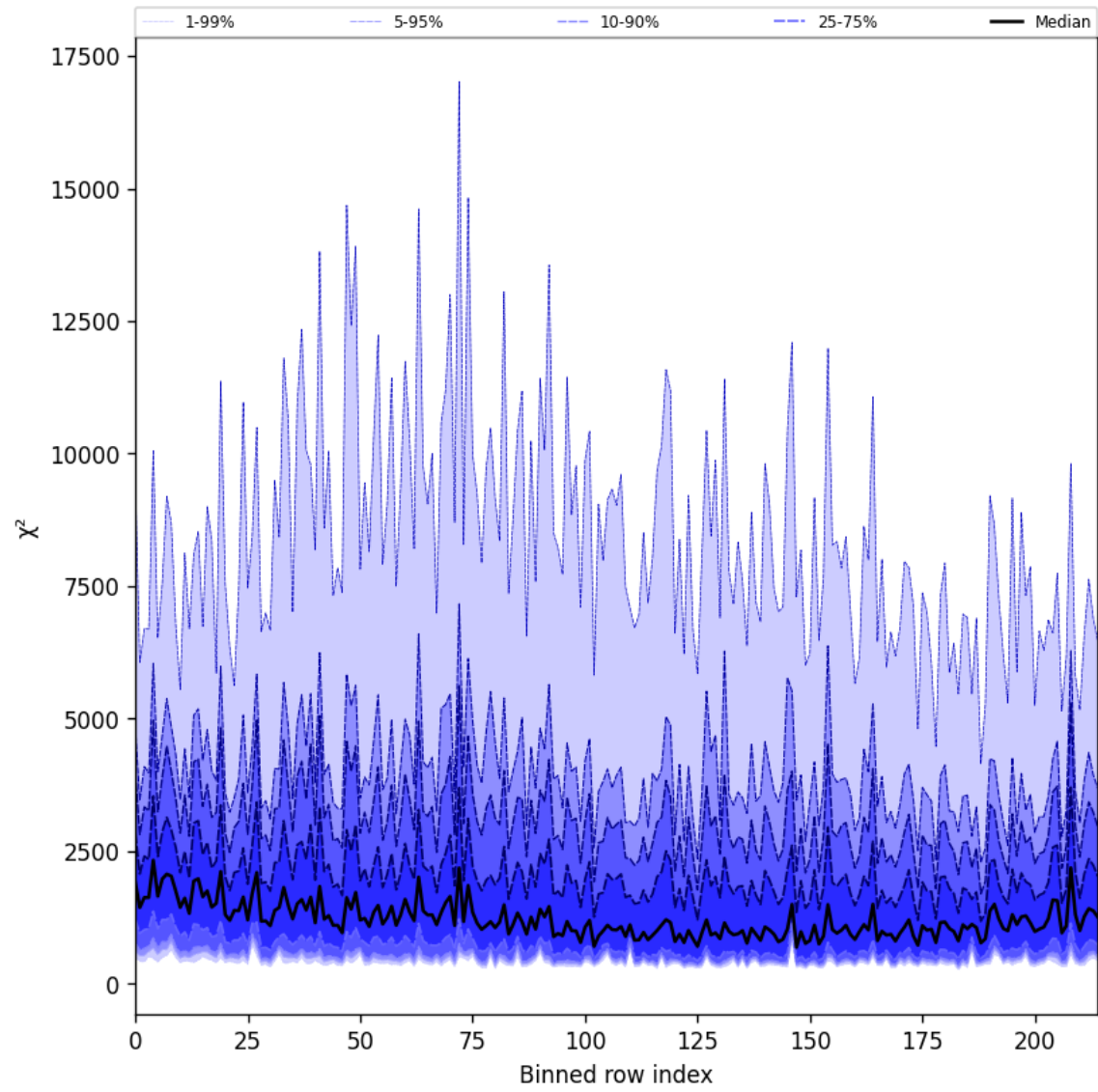
Figure 24: Along track statistics of “ \chi^2 ” for 2025-04-22 to 2025-04-22
