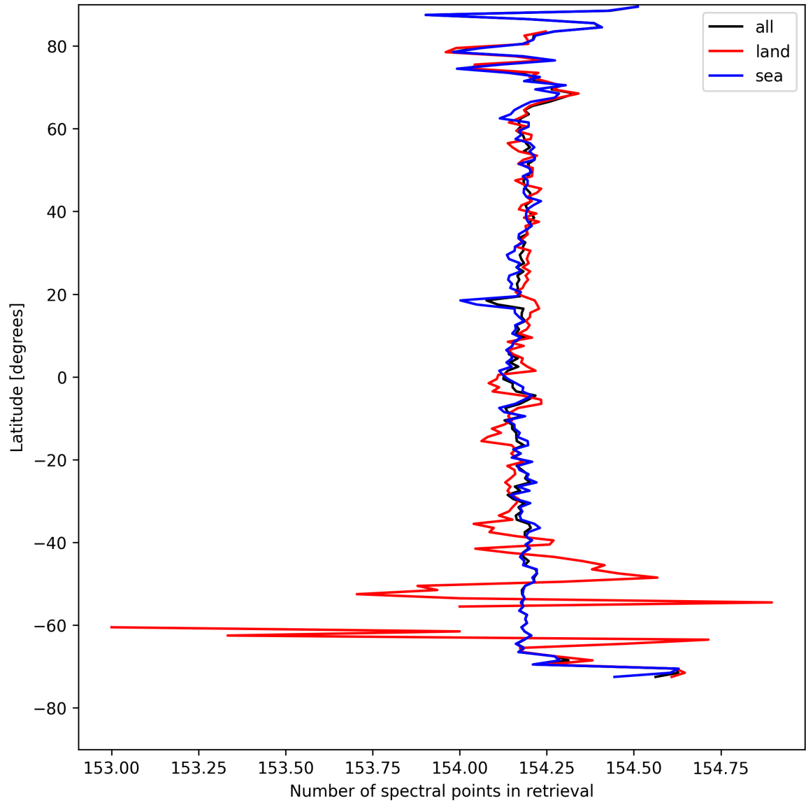
Figure 9: Zonal average of “Number of spectral points in retrieval” for 2025-04-23 to 2025-04-24.
