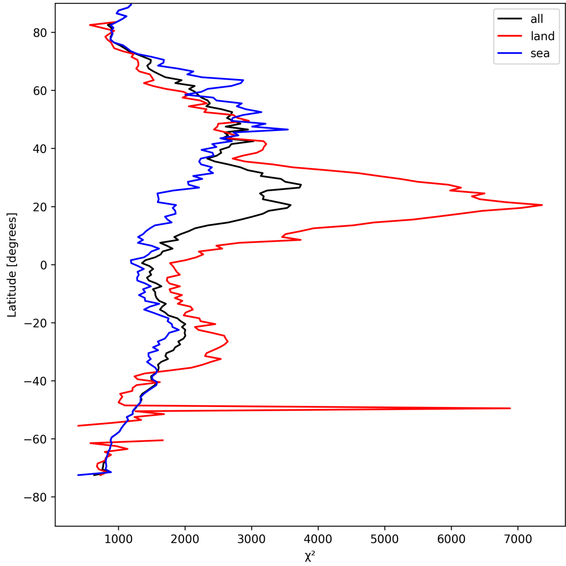
Figure 10: Zonal average of “ \chi^2 ” for 2025-04-23 to 2025-04-24.
