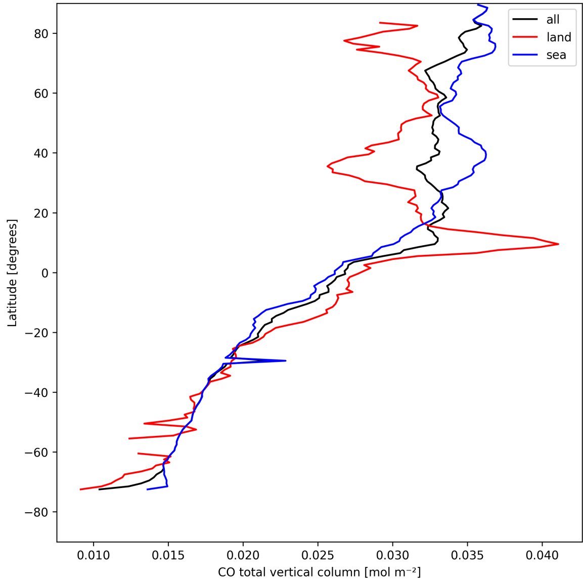
Figure 7: Zonal average of “CO total vertical column” for 2025-04-23 to 2025-04-24.
