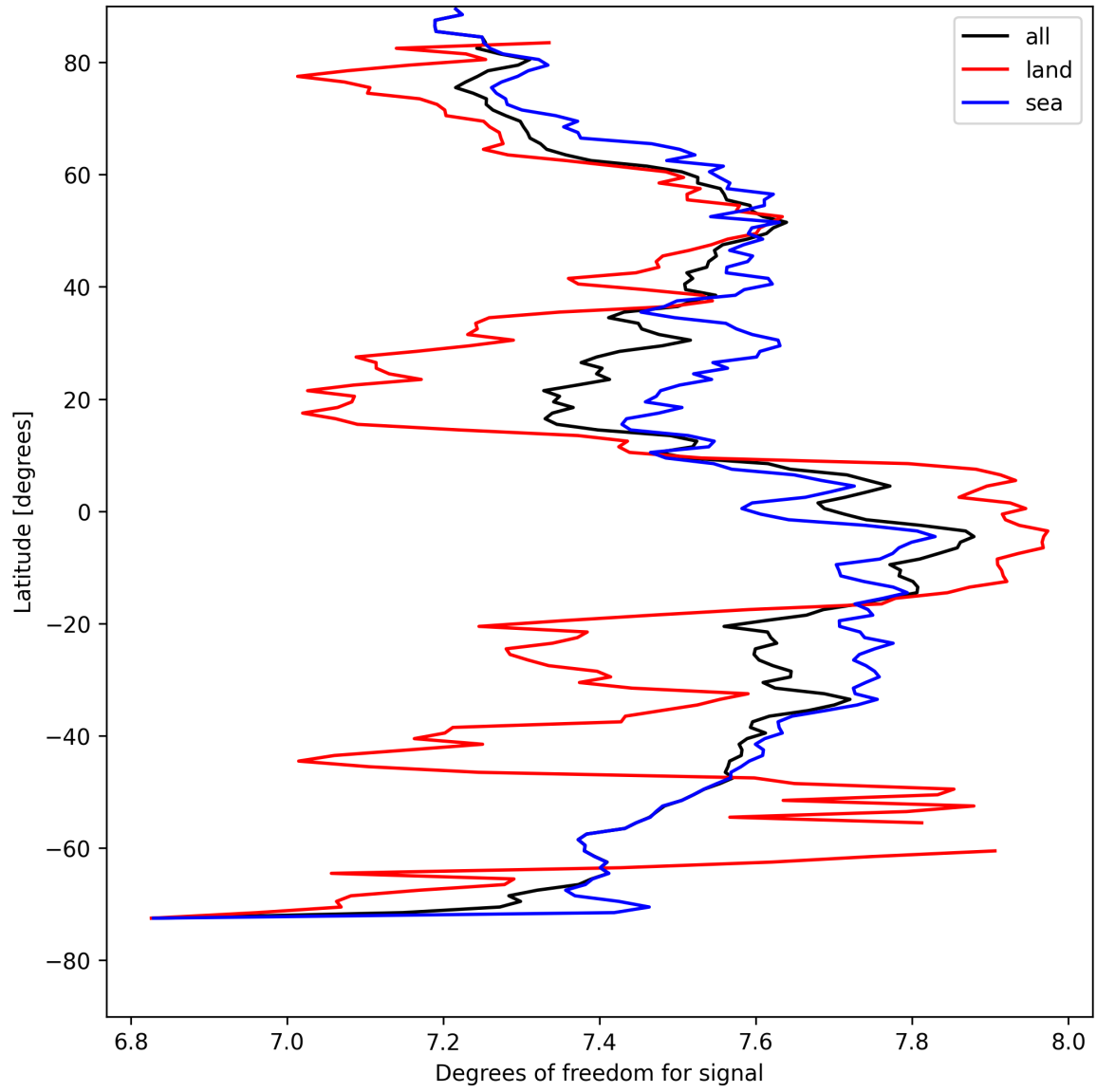
Figure 11: Zonal average of “Degrees of freedom for signal” for 2025-04-23 to 2025-04-24.
