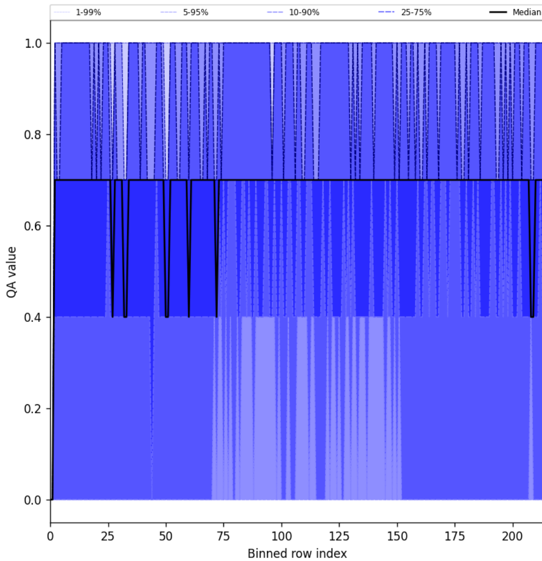
Figure 20: Along track statistics of “QA value” for 2025-04-23 to 2025-04-24
