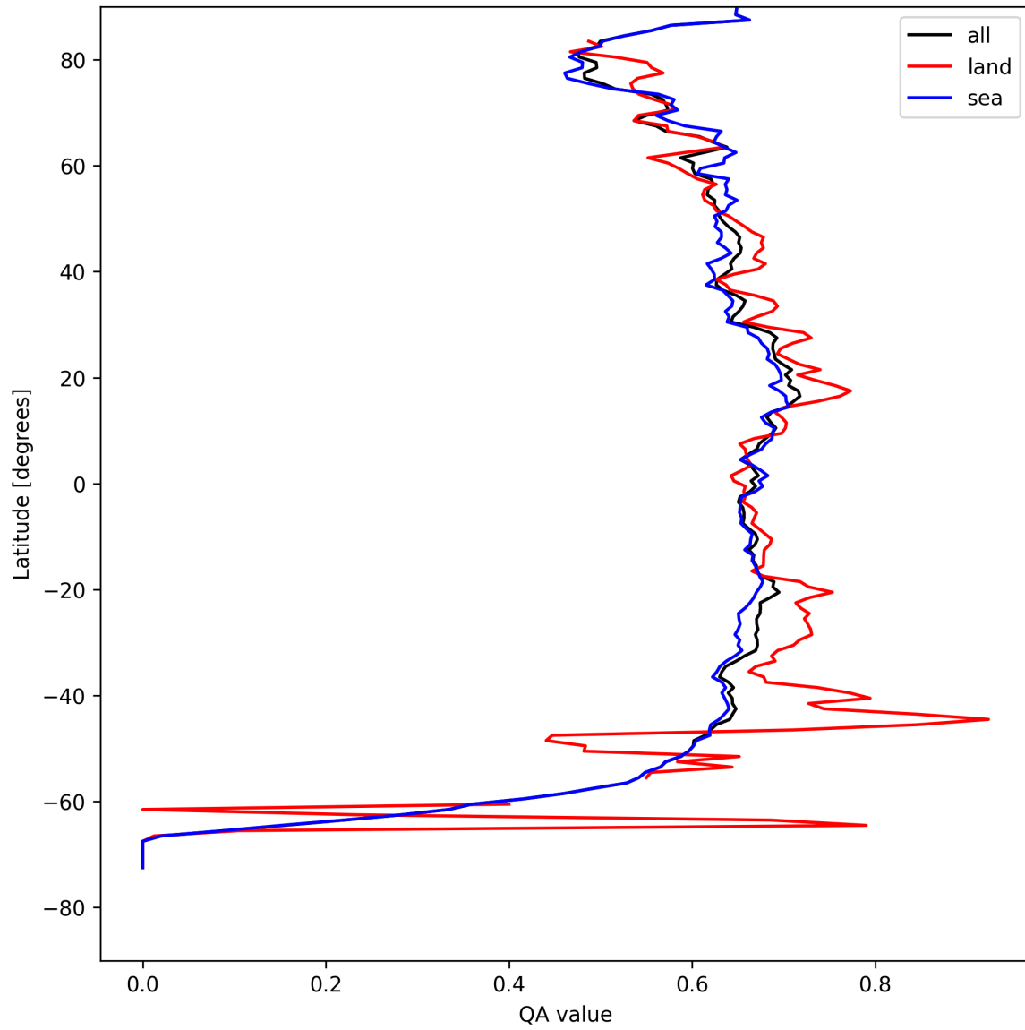
Figure 6: Zonal average of “QA value” for 2025-04-23 to 2025-04-24.
