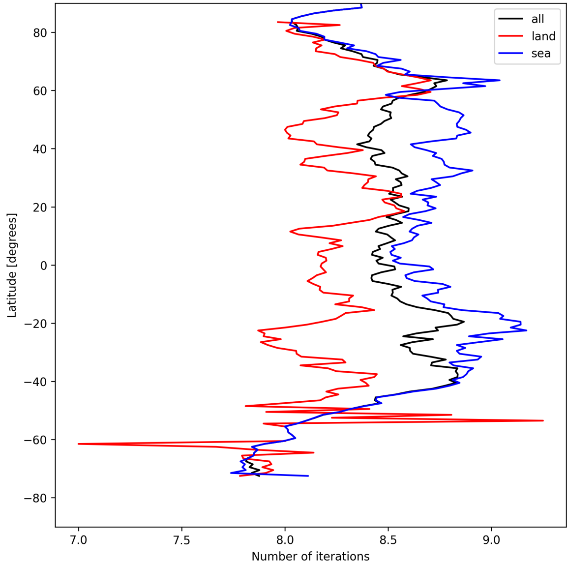
Figure 12: Zonal average of “Number of iterations” for 2025-04-23 to 2025-04-24.
