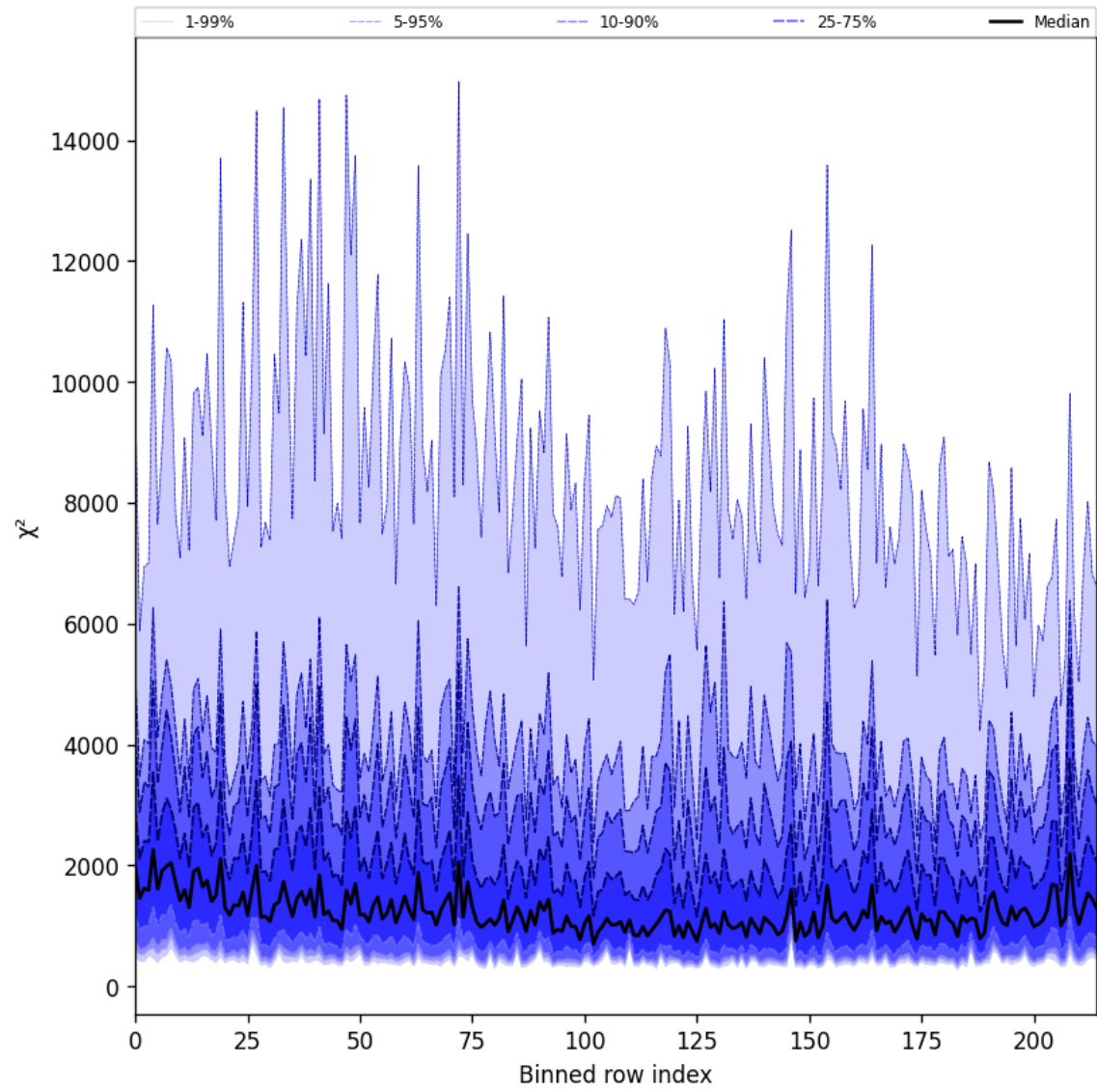
Figure 24: Along track statistics of “ \chi^2 ” for 2025-04-23 to 2025-04-24
