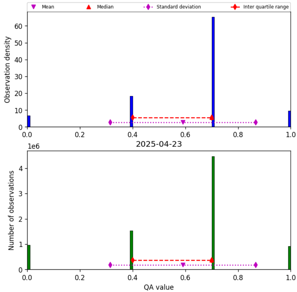
Figure 13: Histogram of “QA value” for 2025-04-23 to 2025-04-24
