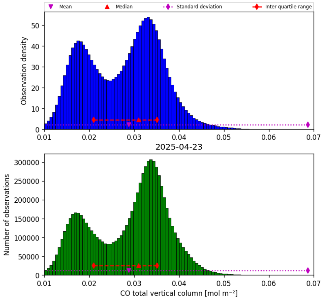
Figure 14: Histogram of “CO total vertical column” for 2025-04-23 to 2025-04-24
