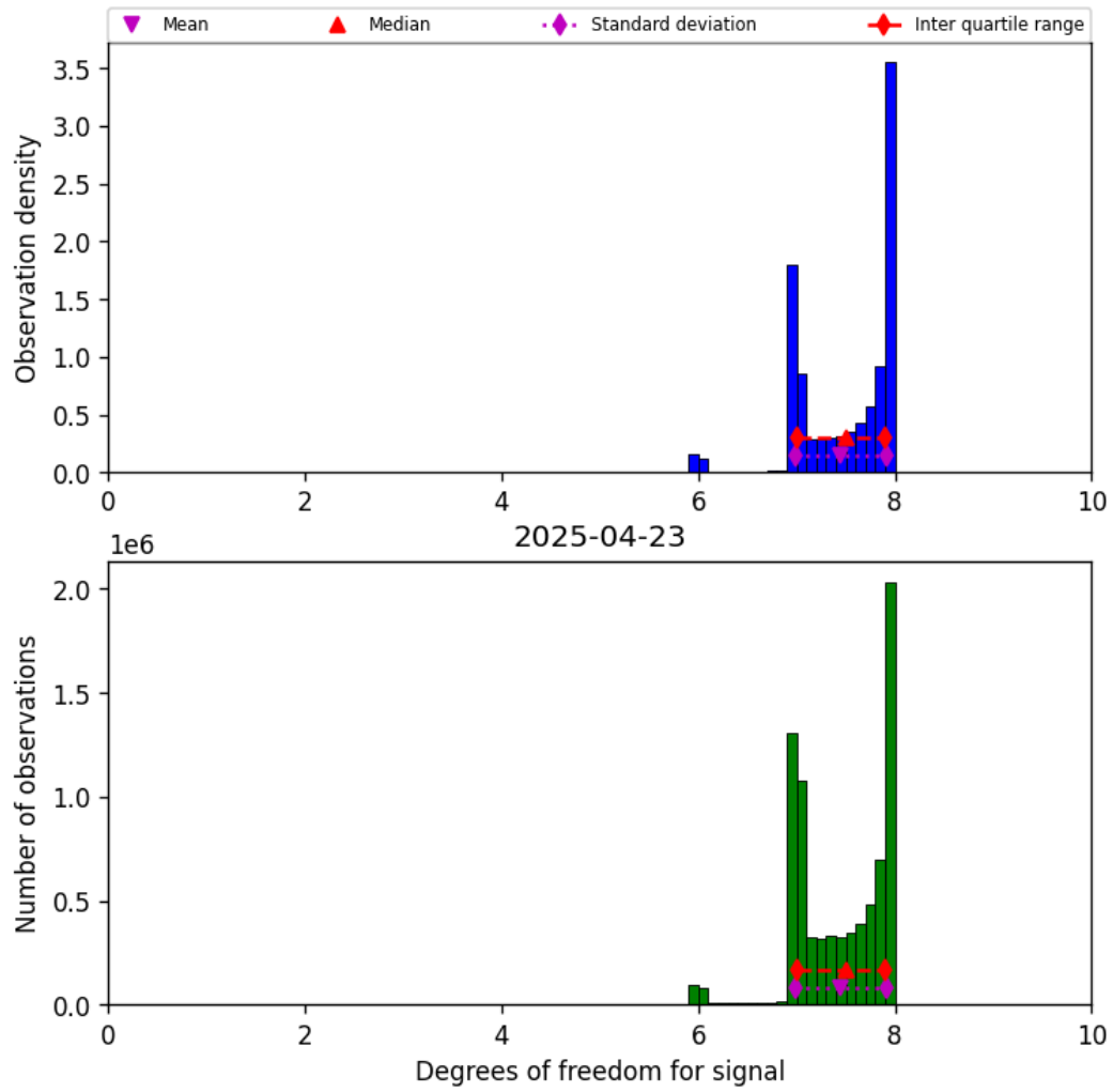
Figure 18: Histogram of “Degrees of freedom for signal” for 2025-04-23 to 2025-04-24
