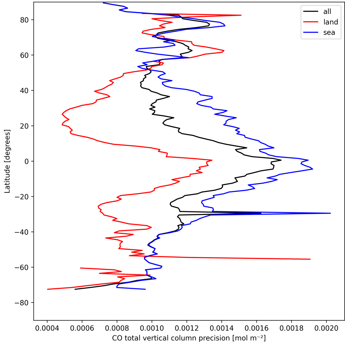
Figure 8: Zonal average of “CO total vertical column precision” for 2025-04-23 to 2025-04-24.
