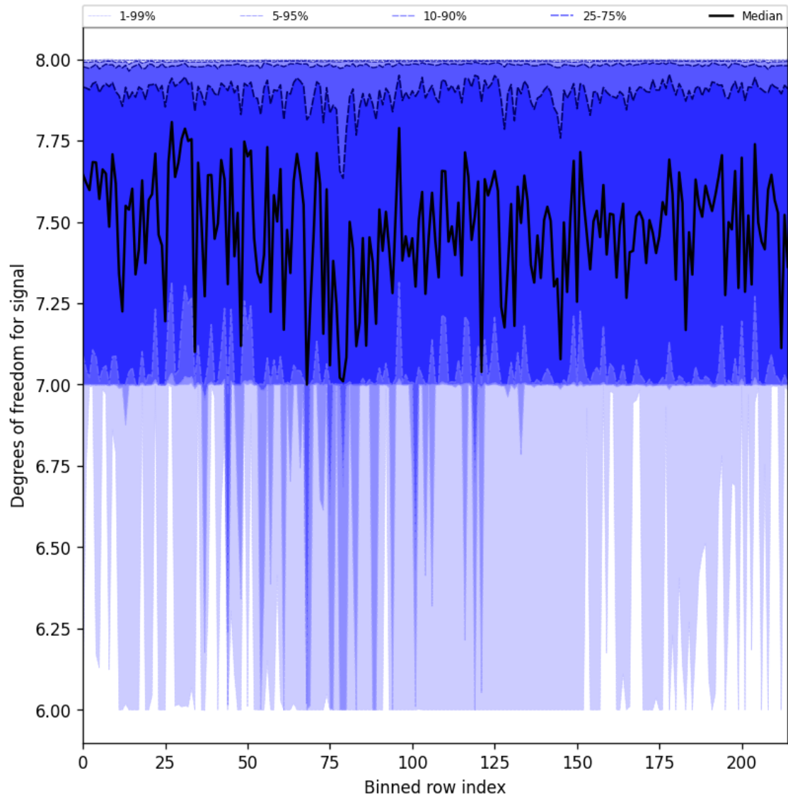
Figure 25: Along track statistics of “Degrees of freedom for signal” for 2025-04-23 to 2025-04-24
