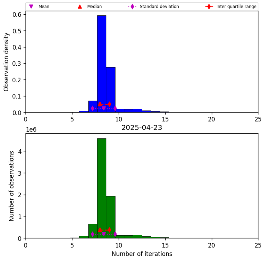
Figure 19: Histogram of “Number of iterations” for 2025-04-23 to 2025-04-24
