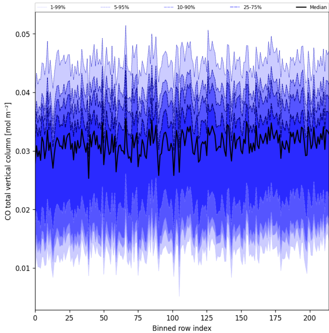
Figure 21: Along track statistics of "CO total vertical column" for 2025-04-23 to 2025-04-24
