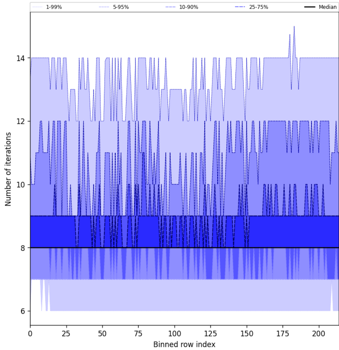
Figure 26: Along track statistics of “Number of iterations” for 2025-04-23 to 2025-04-24
