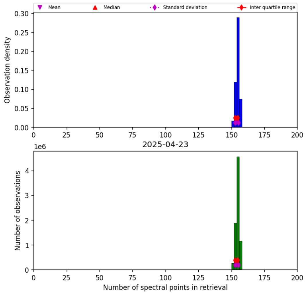
Figure 16: Histogram of “Number of spectral points in retrieval” for 2025-04-23 to 2025-04-24
