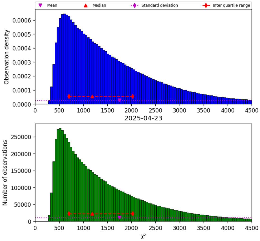
Figure 17: Histogram of “ \chi^2 ” for 2025-04-23 to 2025-04-24
