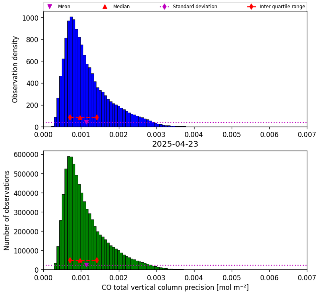
Figure 15: Histogram of “CO total vertical column precision” for 2025-04-23 to 2025-04-24
