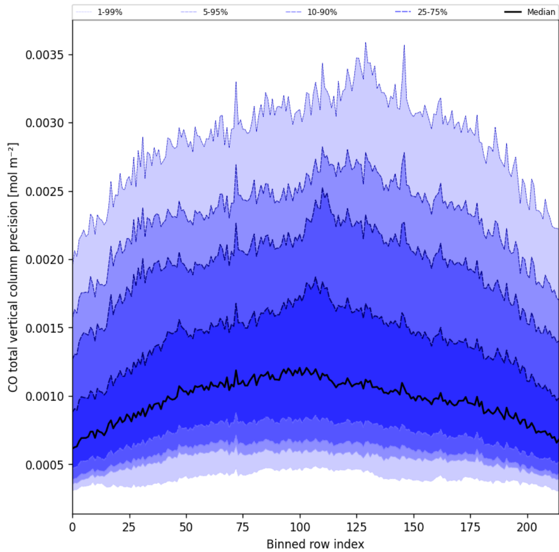
Figure 22: Along track statistics of “CO total vertical column precision” for 2025-04-23 to 2025-04-24
