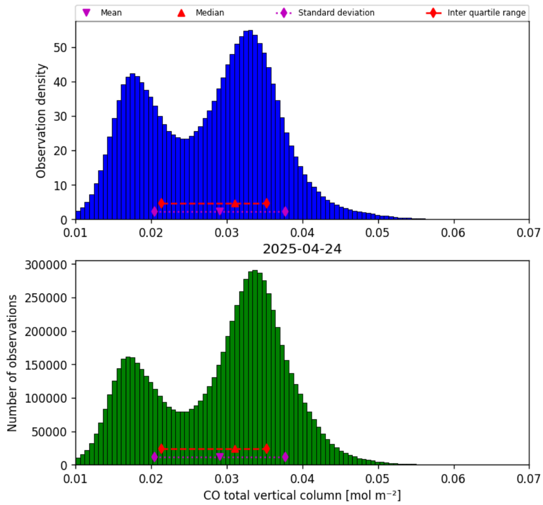
Figure 14: Histogram of “CO total vertical column” for 2025-04-24 to 2025-04-25
