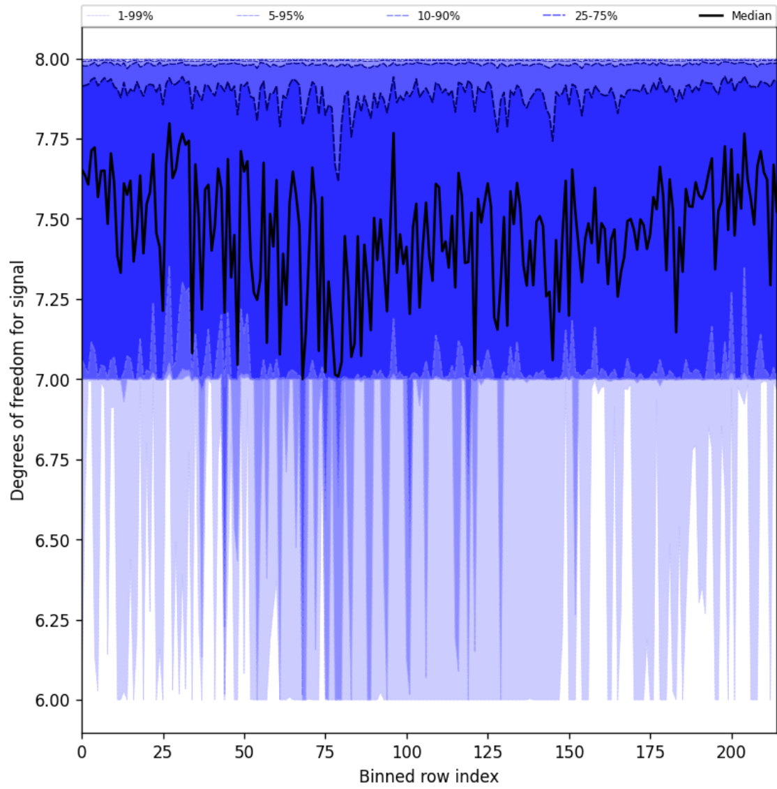
Figure 25: Along track statistics of “Degrees of freedom for signal” for 2025-04-24 to 2025-04-25
