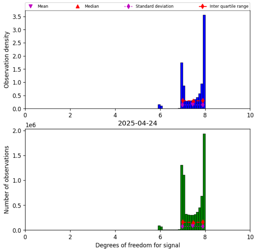
Figure 18: Histogram of “Degrees of freedom for signal” for 2025-04-24 to 2025-04-25
