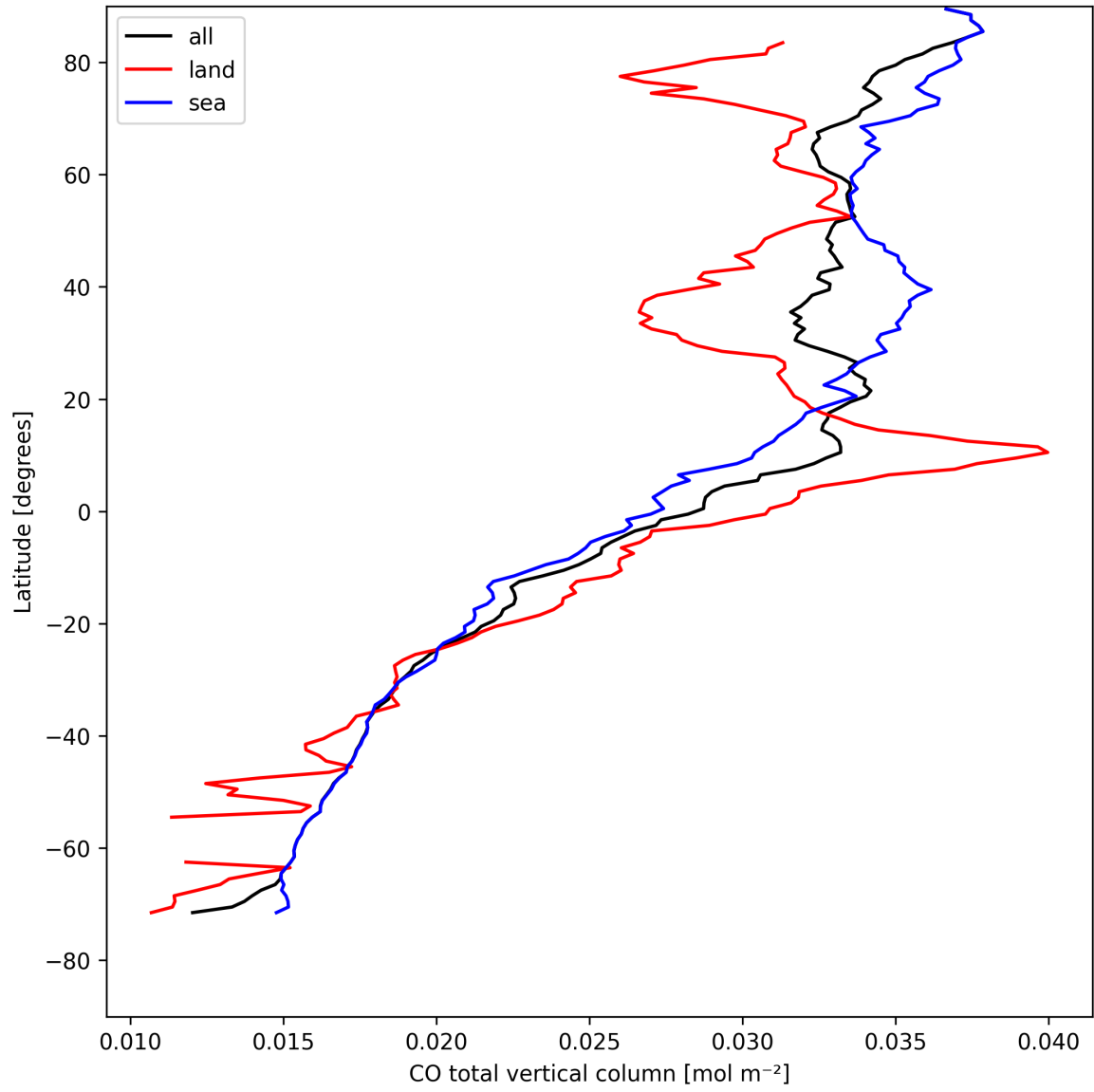
Figure 7: Zonal average of “CO total vertical column” for 2025-04-24 to 2025-04-25.
