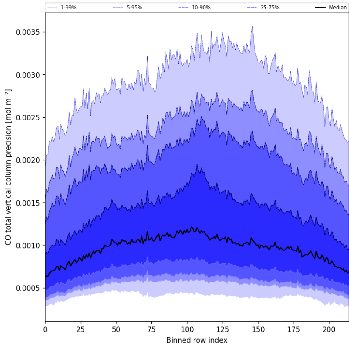
Figure 22: Along track statistics of “CO total vertical column precision” for 2025-04-24 to 2025-04-25
