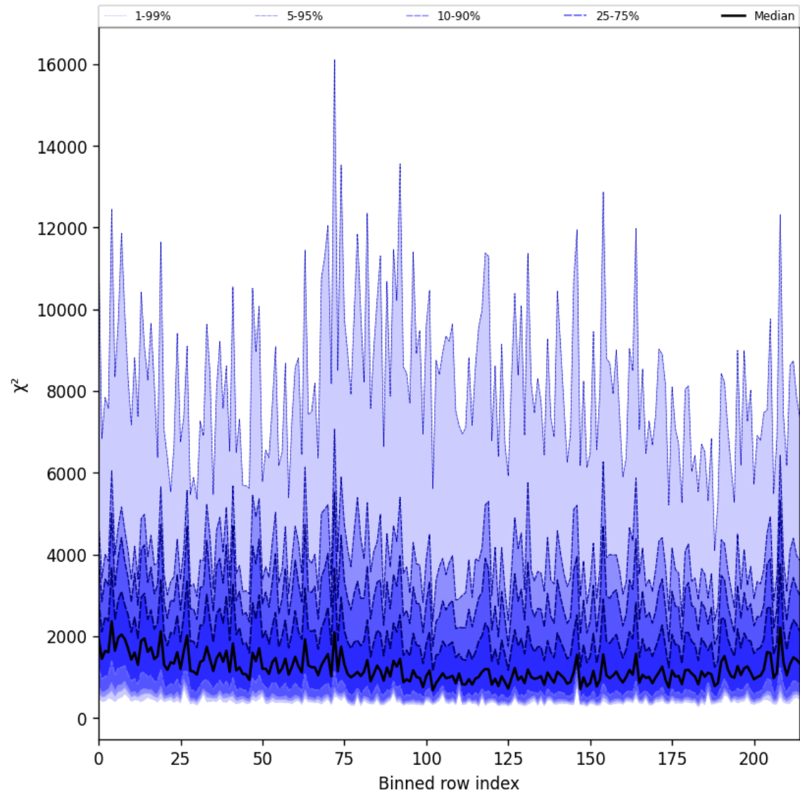
Figure 24: Along track statistics of “ \chi^2 ” for 2025-04-24 to 2025-04-25
