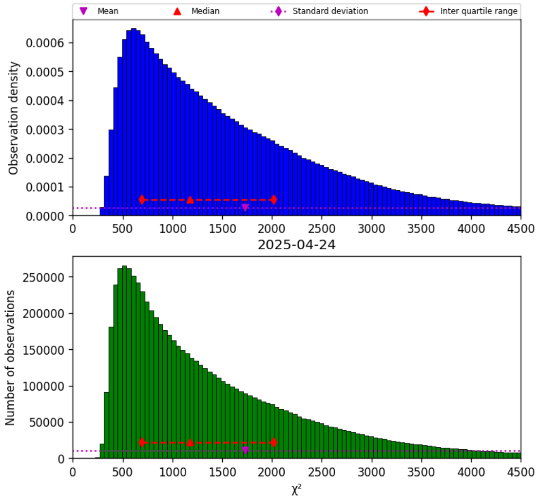
Figure 17: Histogram of “ \chi^2 ” for 2025-04-24 to 2025-04-25
