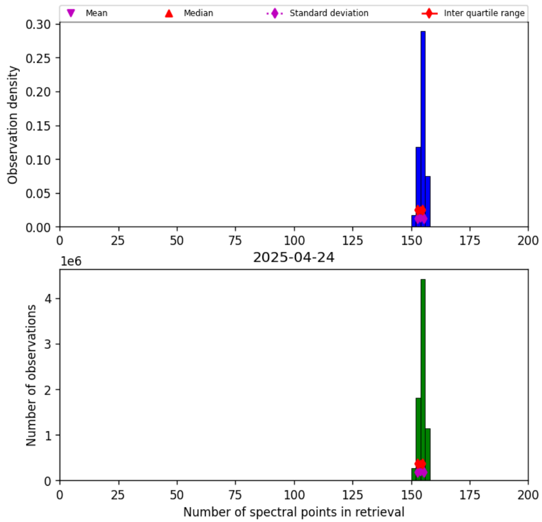
Figure 16: Histogram of “Number of spectral points in retrieval” for 2025-04-24 to 2025-04-25
