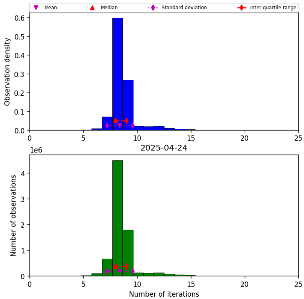
Figure 19: Histogram of “Number of iterations” for 2025-04-24 to 2025-04-25
