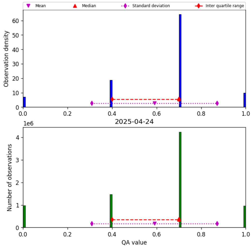
Figure 13: Histogram of “QA value” for 2025-04-24 to 2025-04-25
