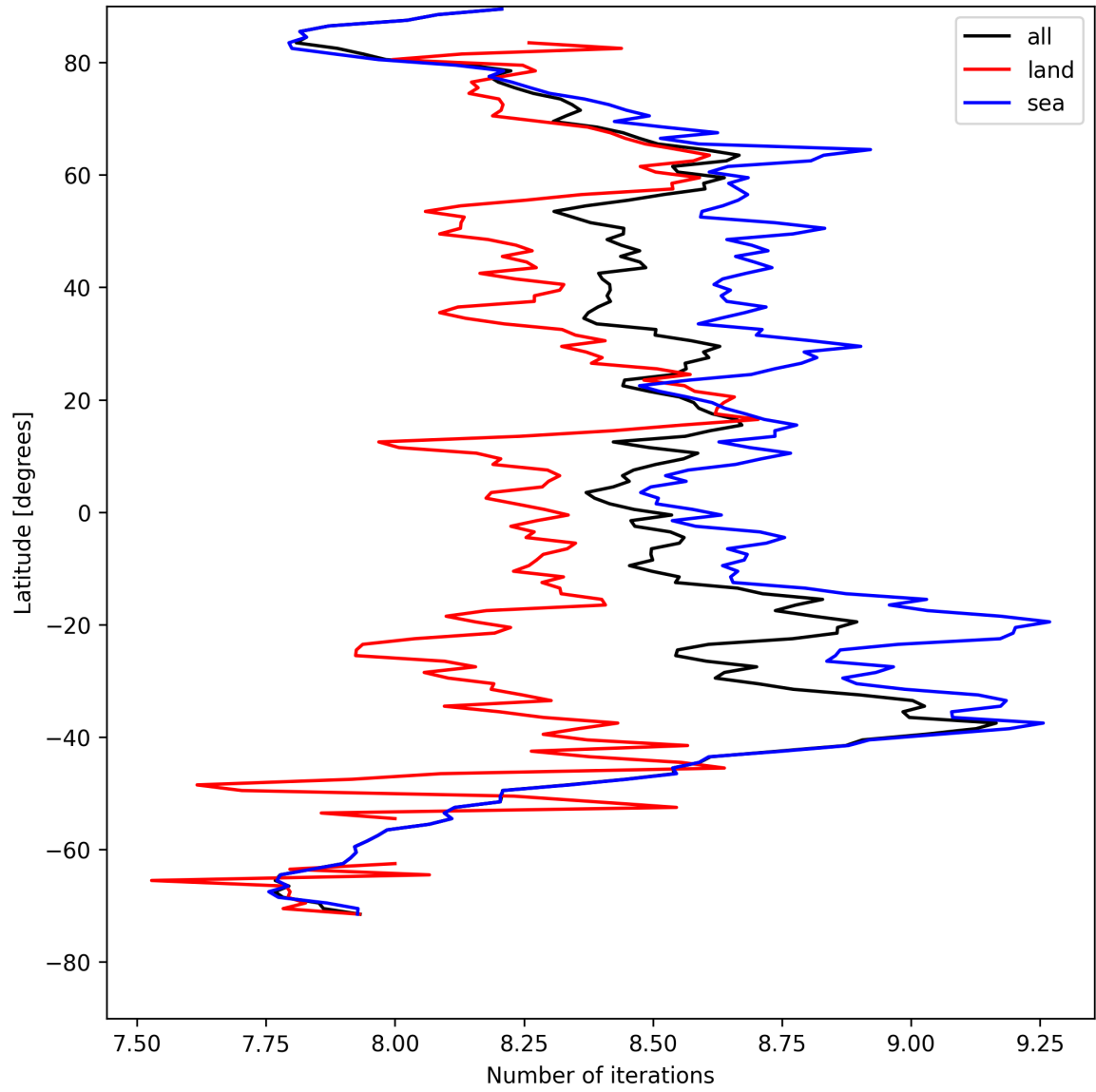
Figure 12: Zonal average of “Number of iterations” for 2025-04-24 to 2025-04-25.
