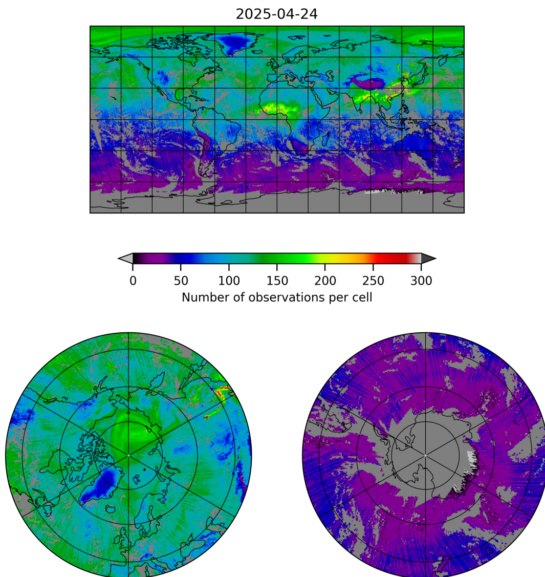
Figure 5: Map of the number of observations for 2025-04-24 to 2025-04-25
