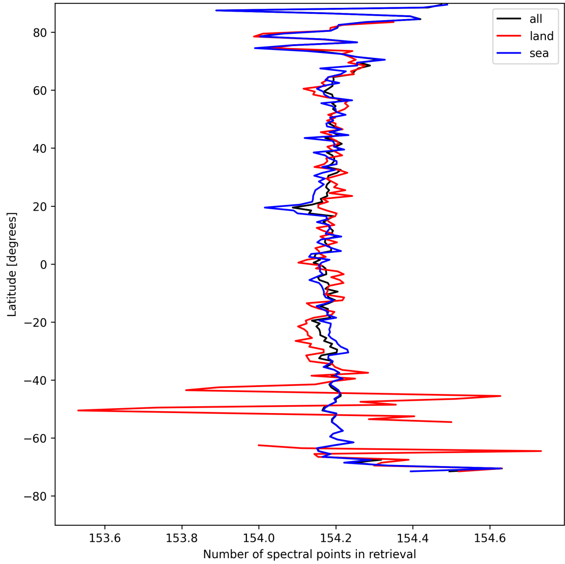
Figure 9: Zonal average of “Number of spectral points in retrieval” for 2025-04-24 to 2025-04-25.
