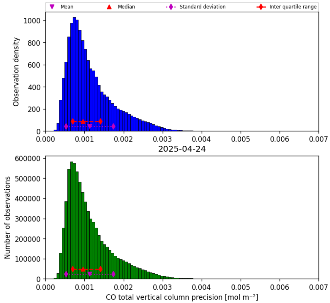
Figure 15: Histogram of “CO total vertical column precision” for 2025-04-24 to 2025-04-25
