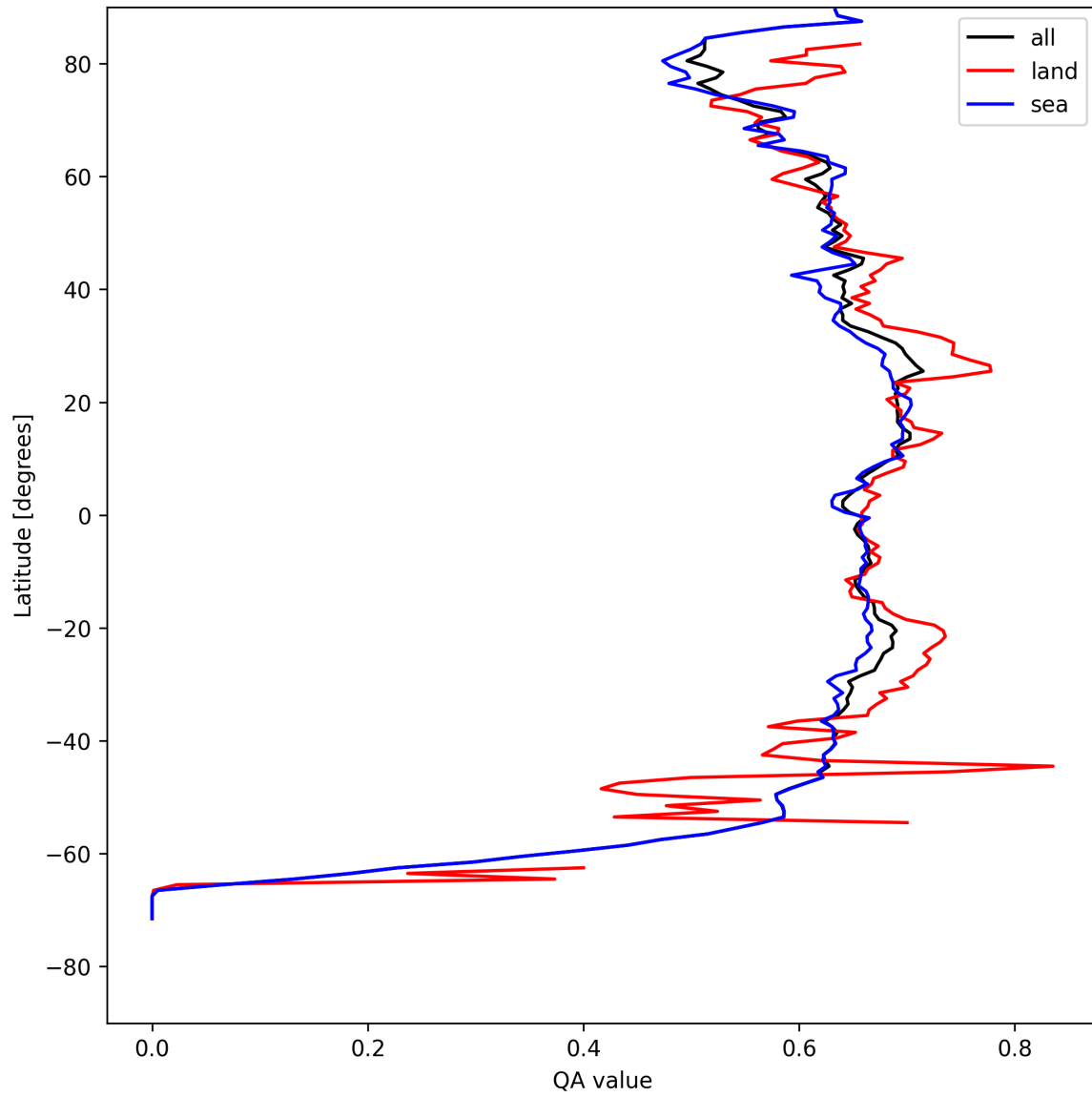
Figure 6: Zonal average of “QA value” for 2025-04-24 to 2025-04-25.
