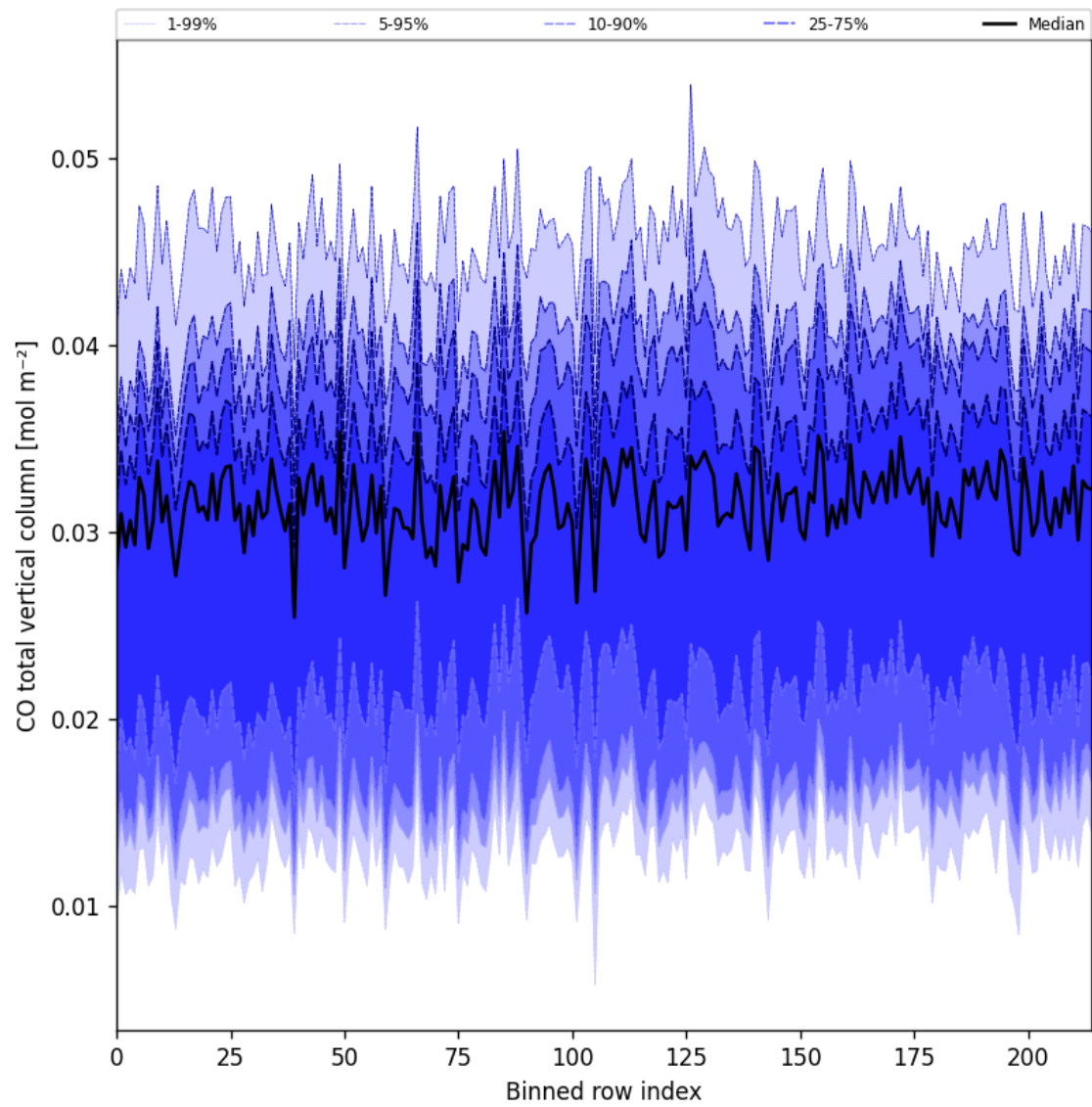
Figure 21: Along track statistics of “CO total vertical column” for 2025-04-24 to 2025-04-25
