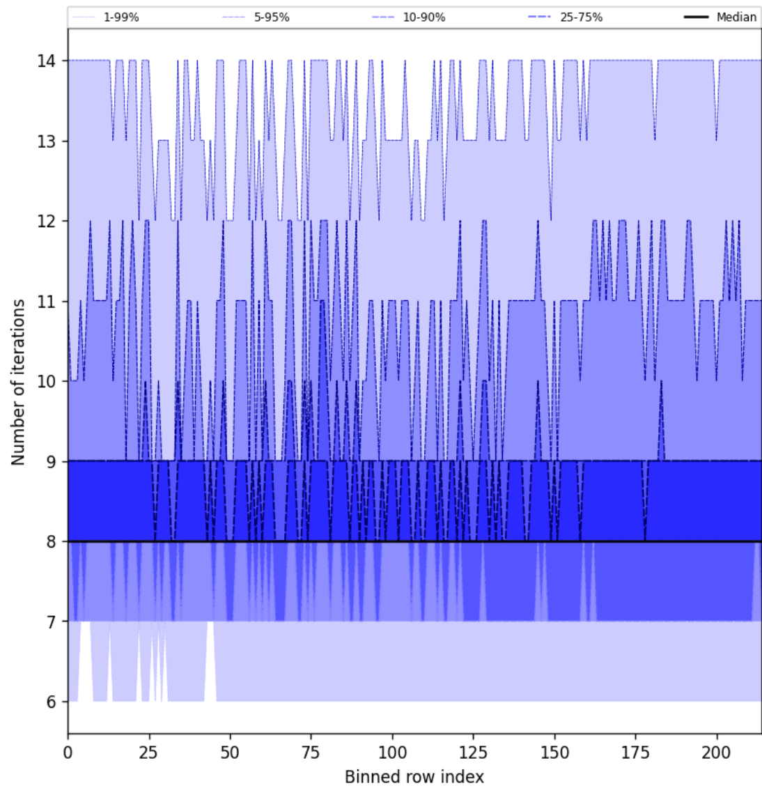
Figure 26: Along track statistics of “Number of iterations” for 2025-04-24 to 2025-04-25
