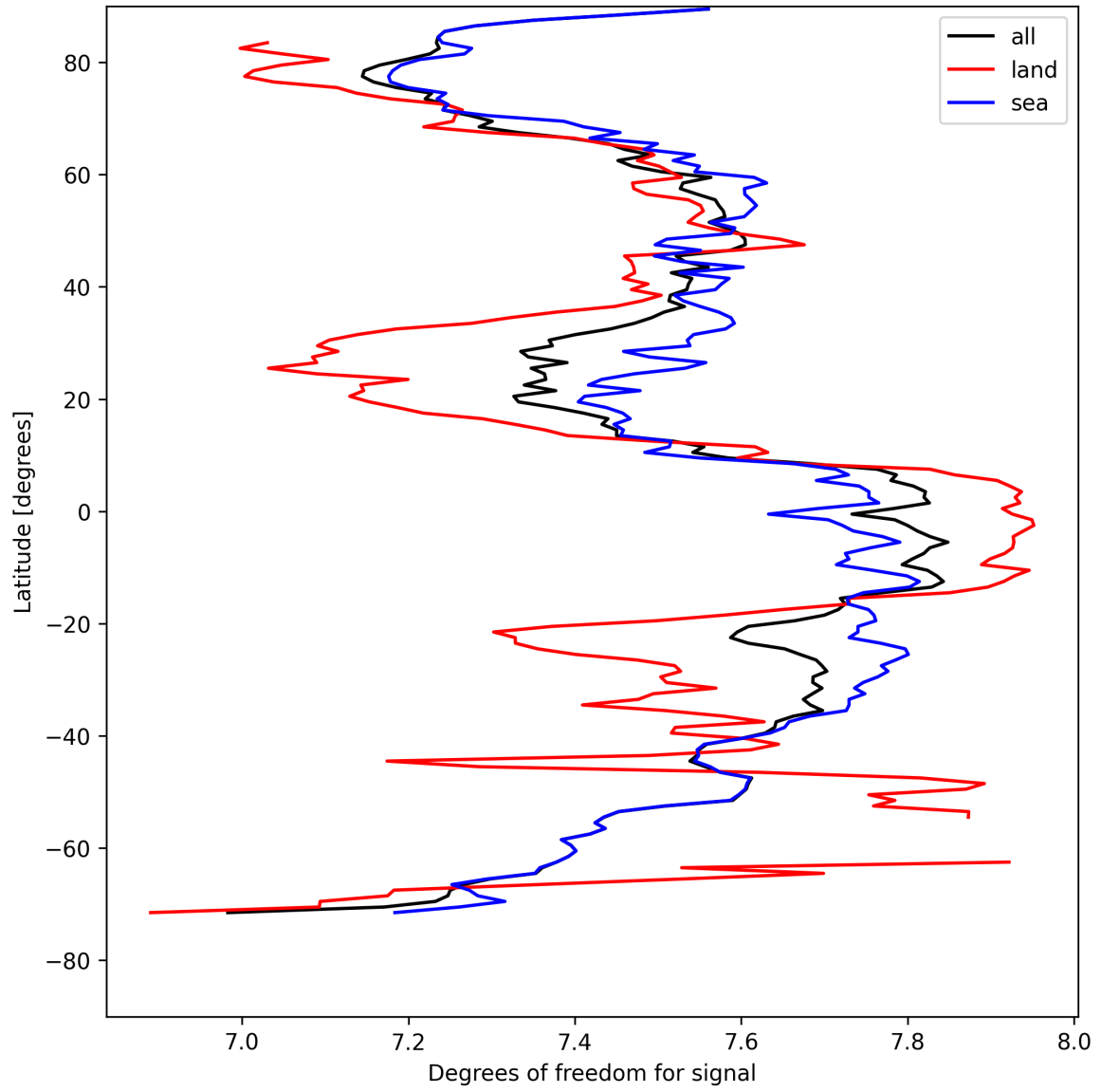
Figure 11: Zonal average of “Degrees of freedom for signal” for 2025-04-24 to 2025-04-25.
