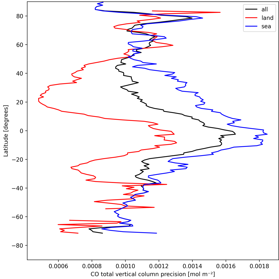
Figure 8: Zonal average of "CO total vertical column precision" for 2025-04-24 to 2025-04-25.
