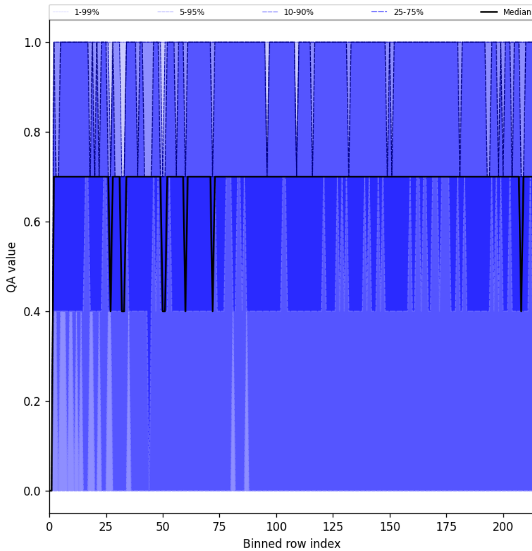
Figure 20: Along track statistics of “QA value” for 2025-04-24 to 2025-04-25
