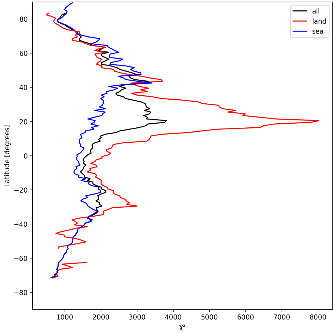
Figure 10: Zonal average of “ \chi^2 ” for 2025-04-24 to 2025-04-25.
