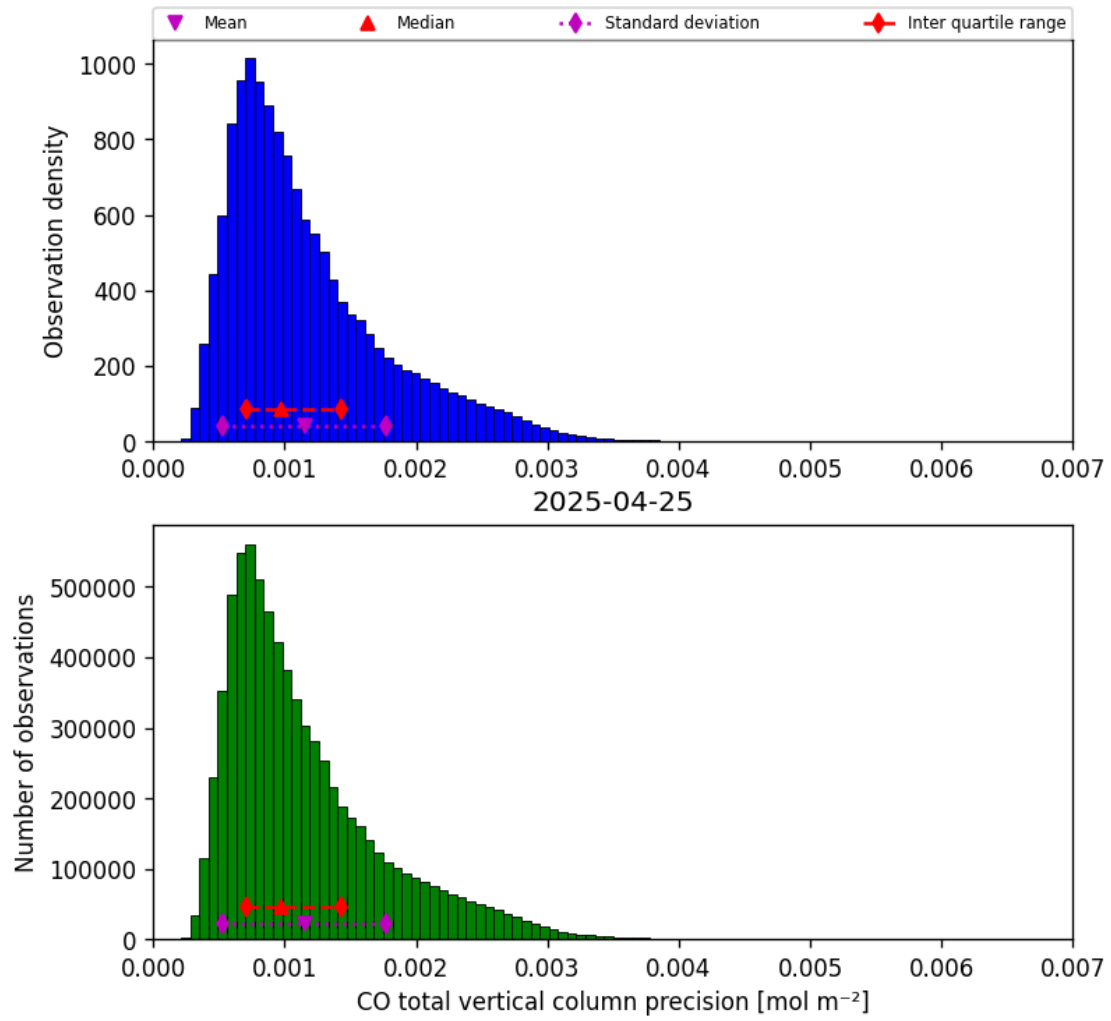
Figure 15: Histogram of “CO total vertical column precision” for 2025-04-25 to 2025-04-26
