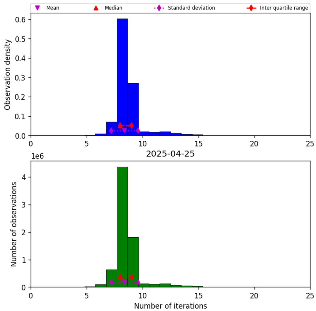
Figure 19: Histogram of “Number of iterations” for 2025-04-25 to 2025-04-26
