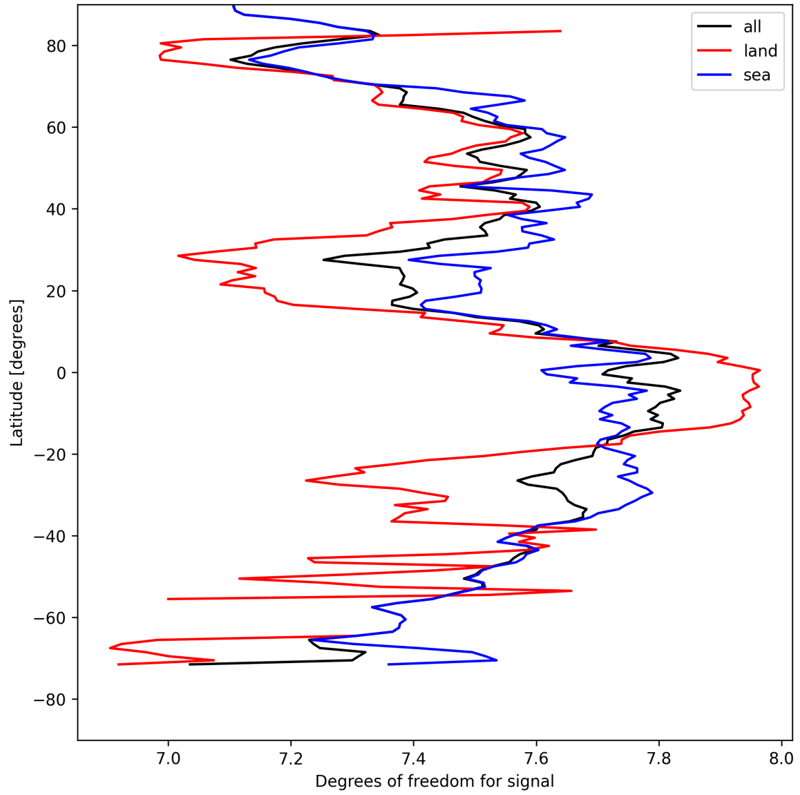
Figure 11: Zonal average of “Degrees of freedom for signal” for 2025-04-25 to 2025-04-26.
