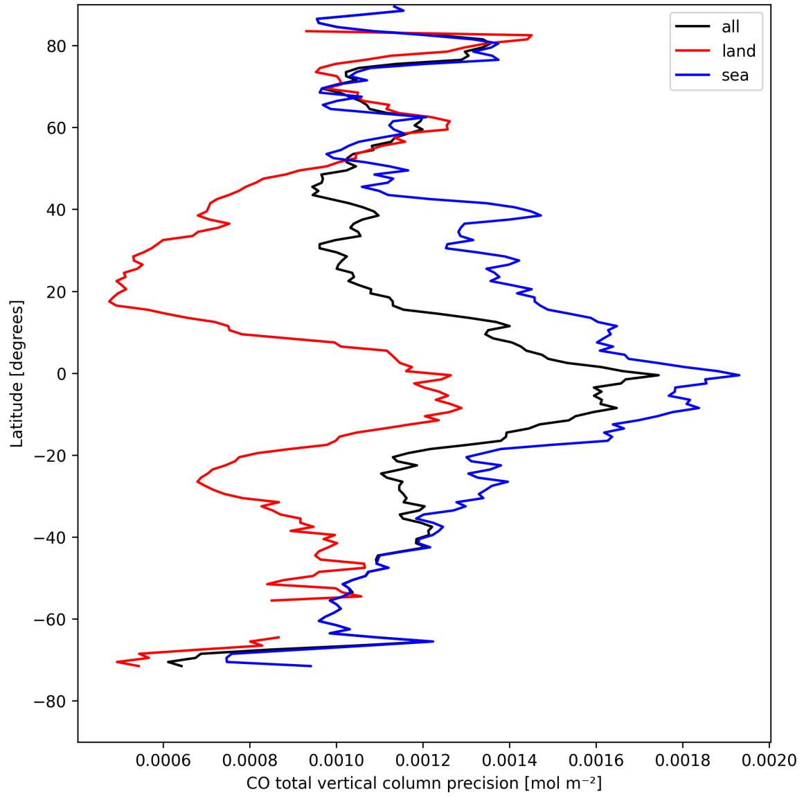
Figure 8: Zonal average of “CO total vertical column precision” for 2025-04-25 to 2025-04-26.
