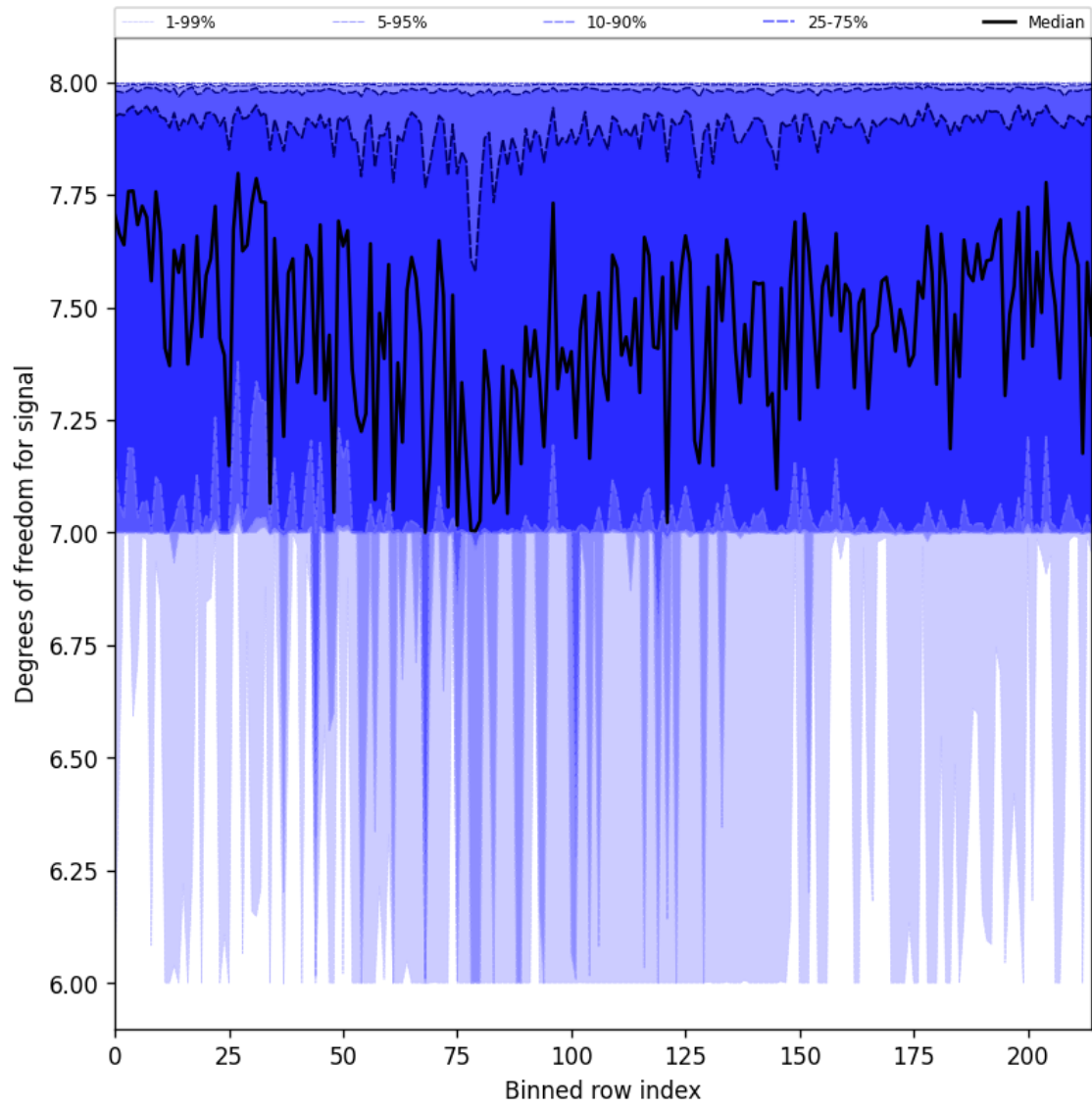
Figure 25: Along track statistics of “Degrees of freedom for signal” for 2025-04-25 to 2025-04-26
