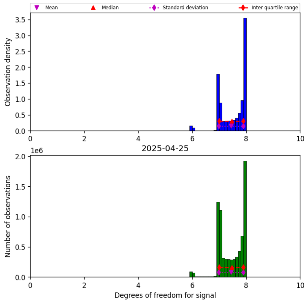
Figure 18: Histogram of “Degrees of freedom for signal” for 2025-04-25 to 2025-04-26
