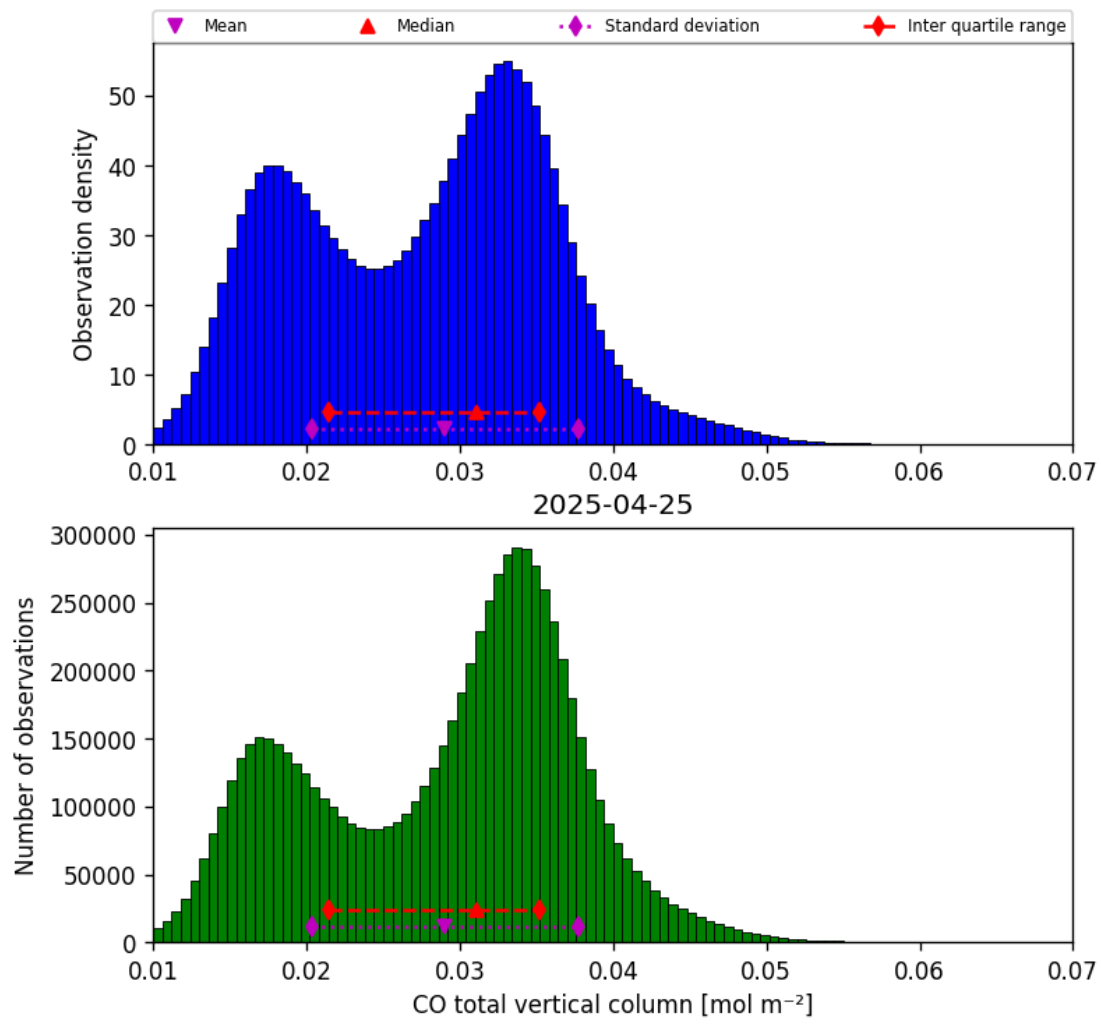
Figure 14: Histogram of “CO total vertical column” for 2025-04-25 to 2025-04-26
