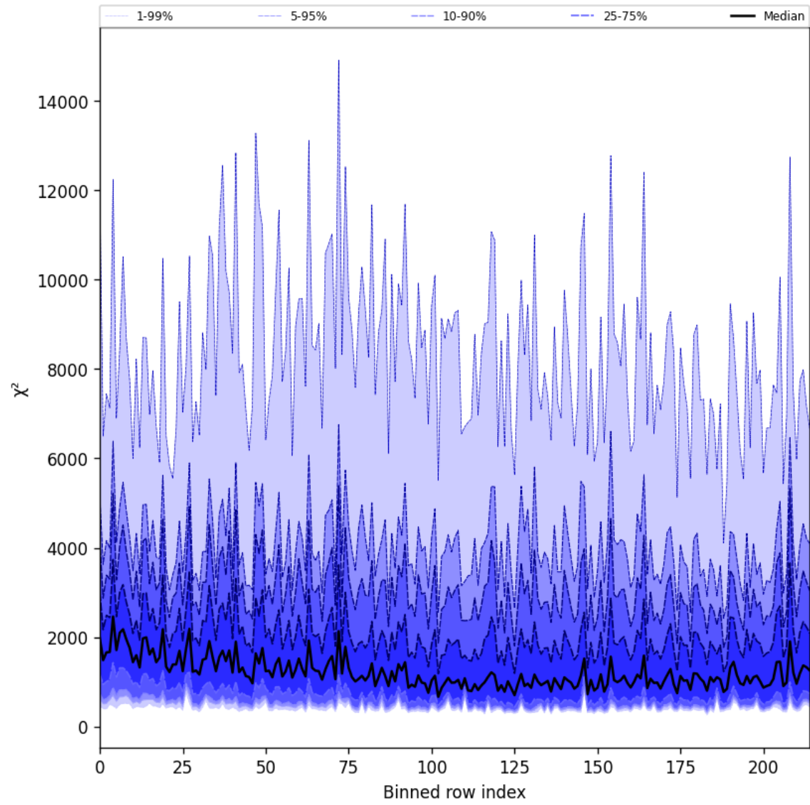
Figure 24: Along track statistics of “ \chi^2 ” for 2025-04-25 to 2025-04-26
