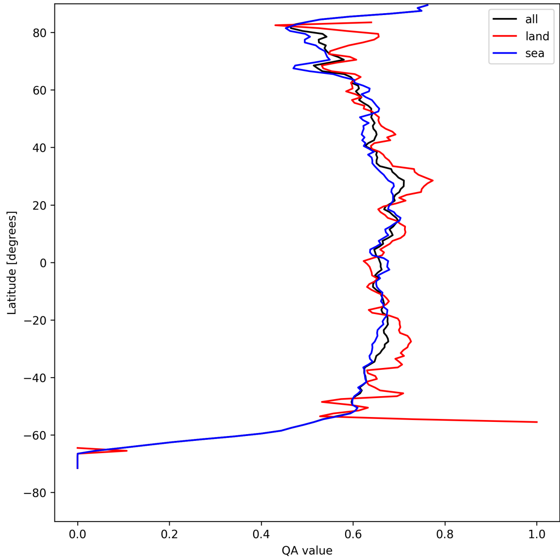
Figure 6: Zonal average of “QA value” for 2025-04-25 to 2025-04-26.
