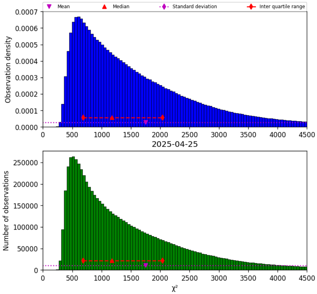
Figure 17: Histogram of “ \chi^2 ” for 2025-04-25 to 2025-04-26
