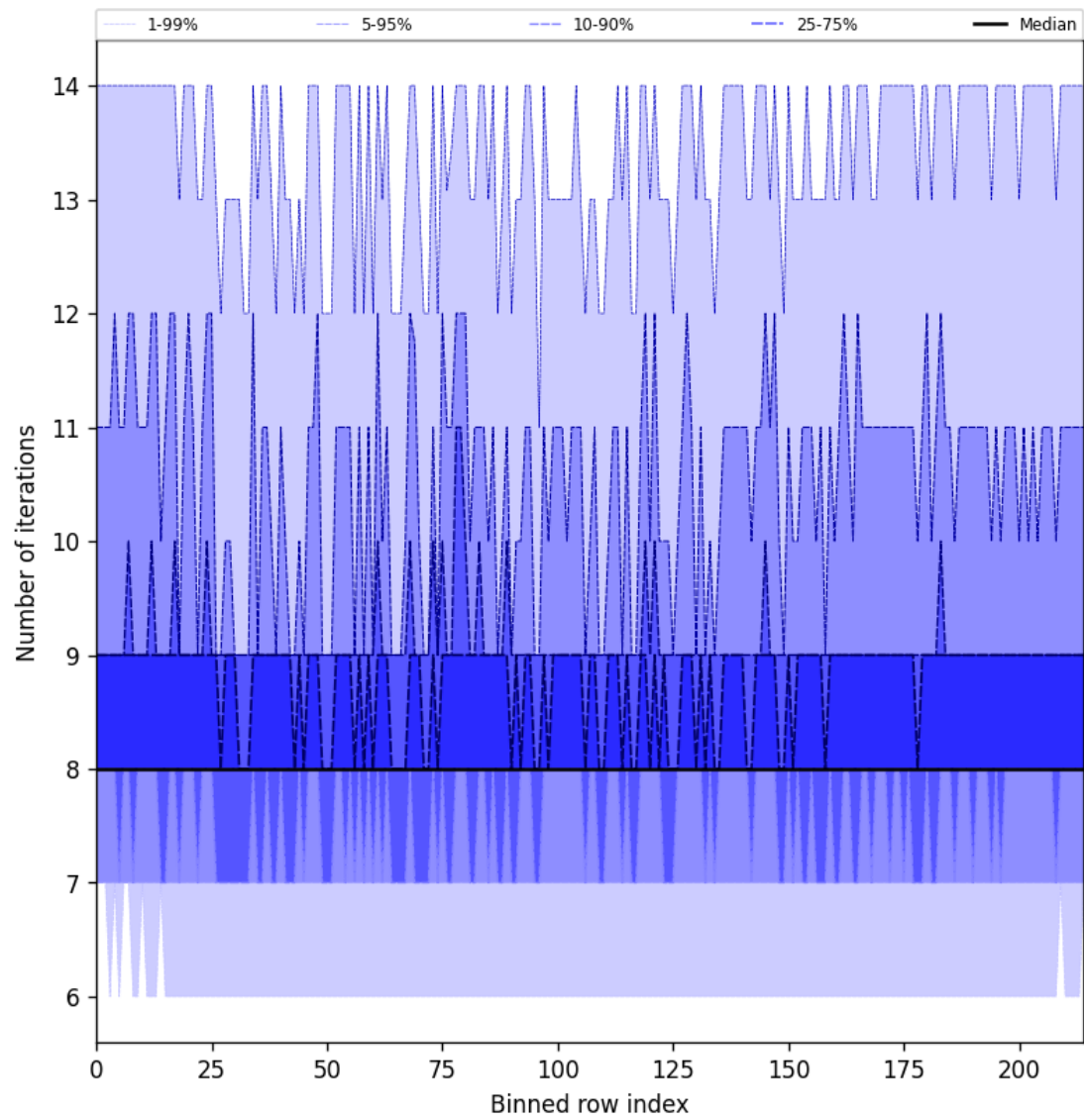
Figure 26: Along track statistics of “Number of iterations” for 2025-04-25 to 2025-04-26
