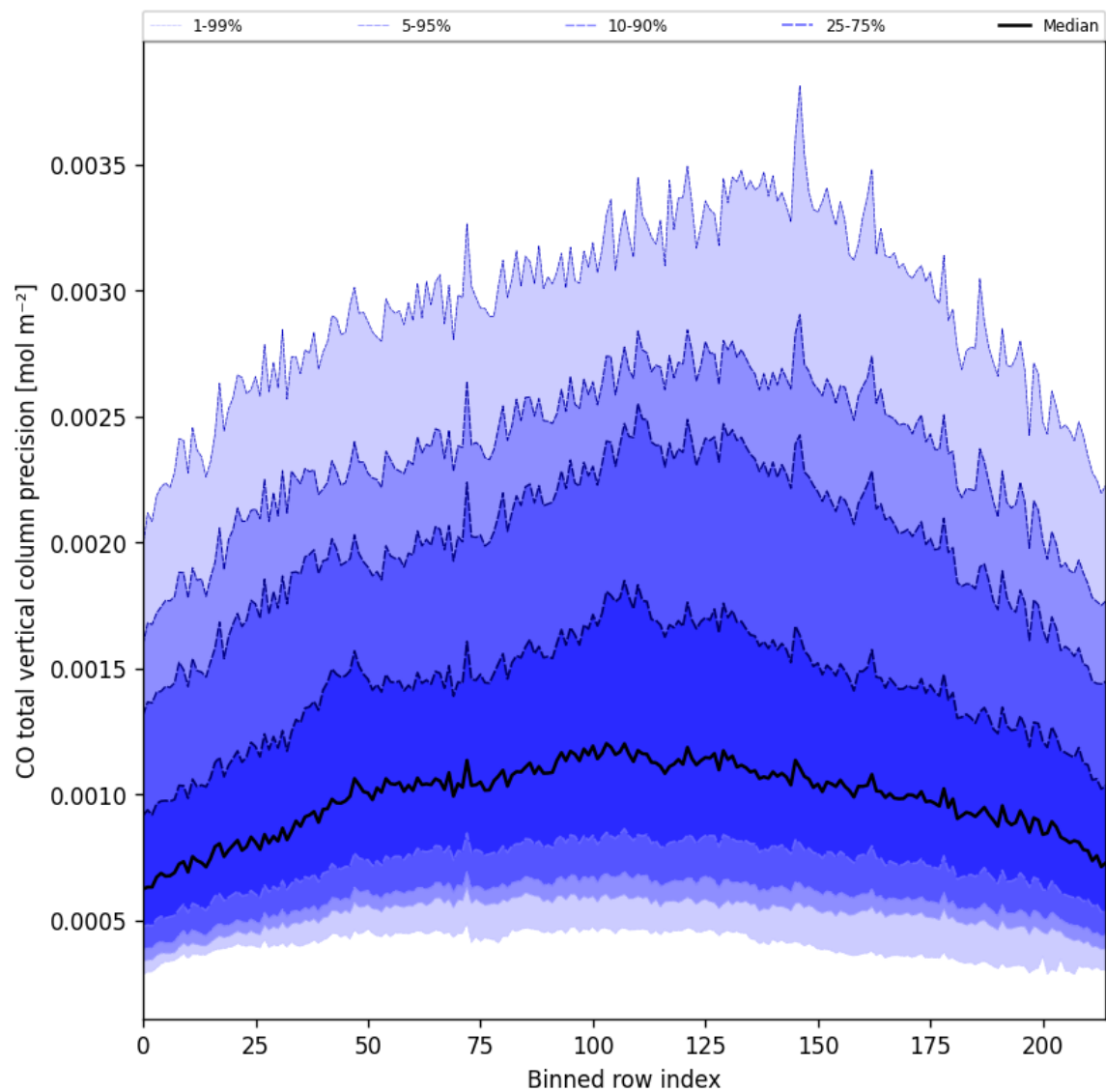
Figure 22: Along track statistics of “CO total vertical column precision” for 2025-04-25 to 2025-04-26
