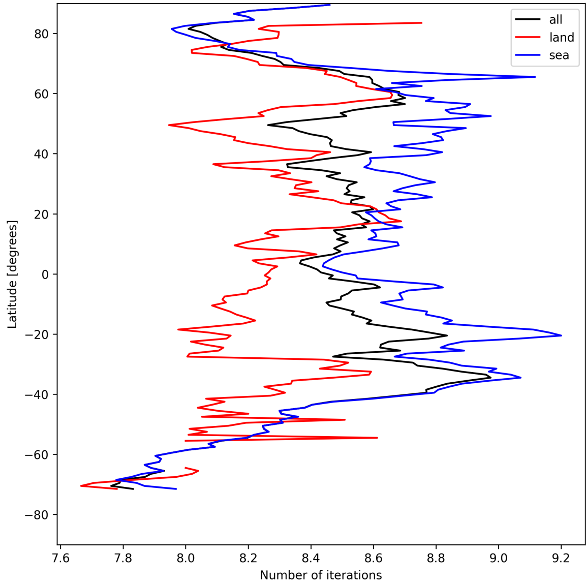
Figure 12: Zonal average of “Number of iterations” for 2025-04-25 to 2025-04-26.
