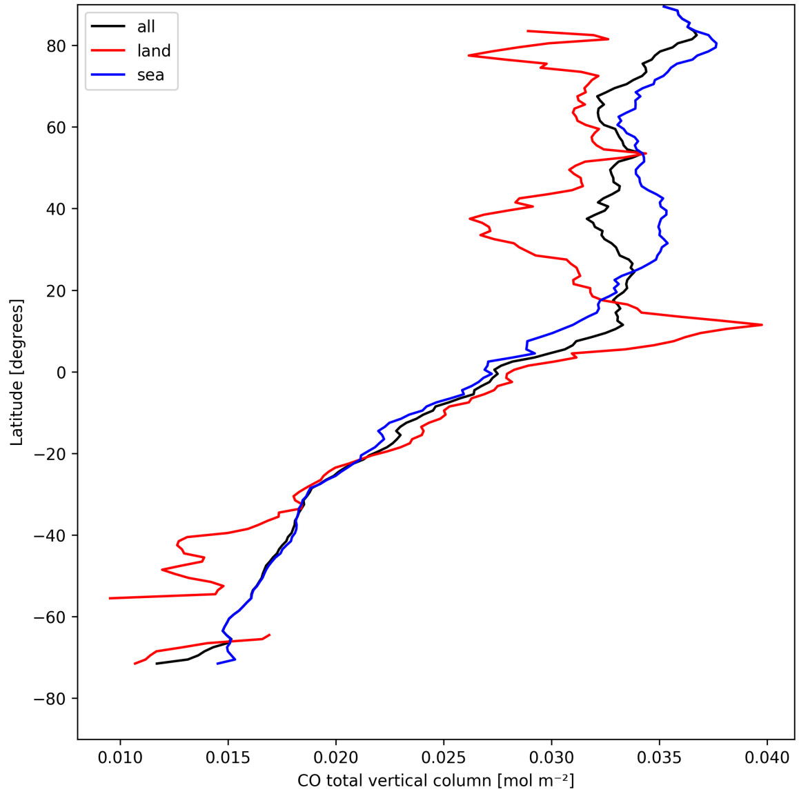
Figure 7: Zonal average of “CO total vertical column” for 2025-04-25 to 2025-04-26.
