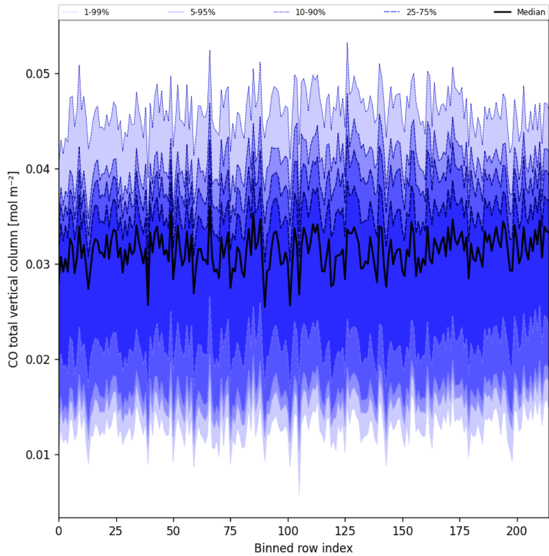
Figure 21: Along track statistics of “CO total vertical column” for 2025-04-25 to 2025-04-26
