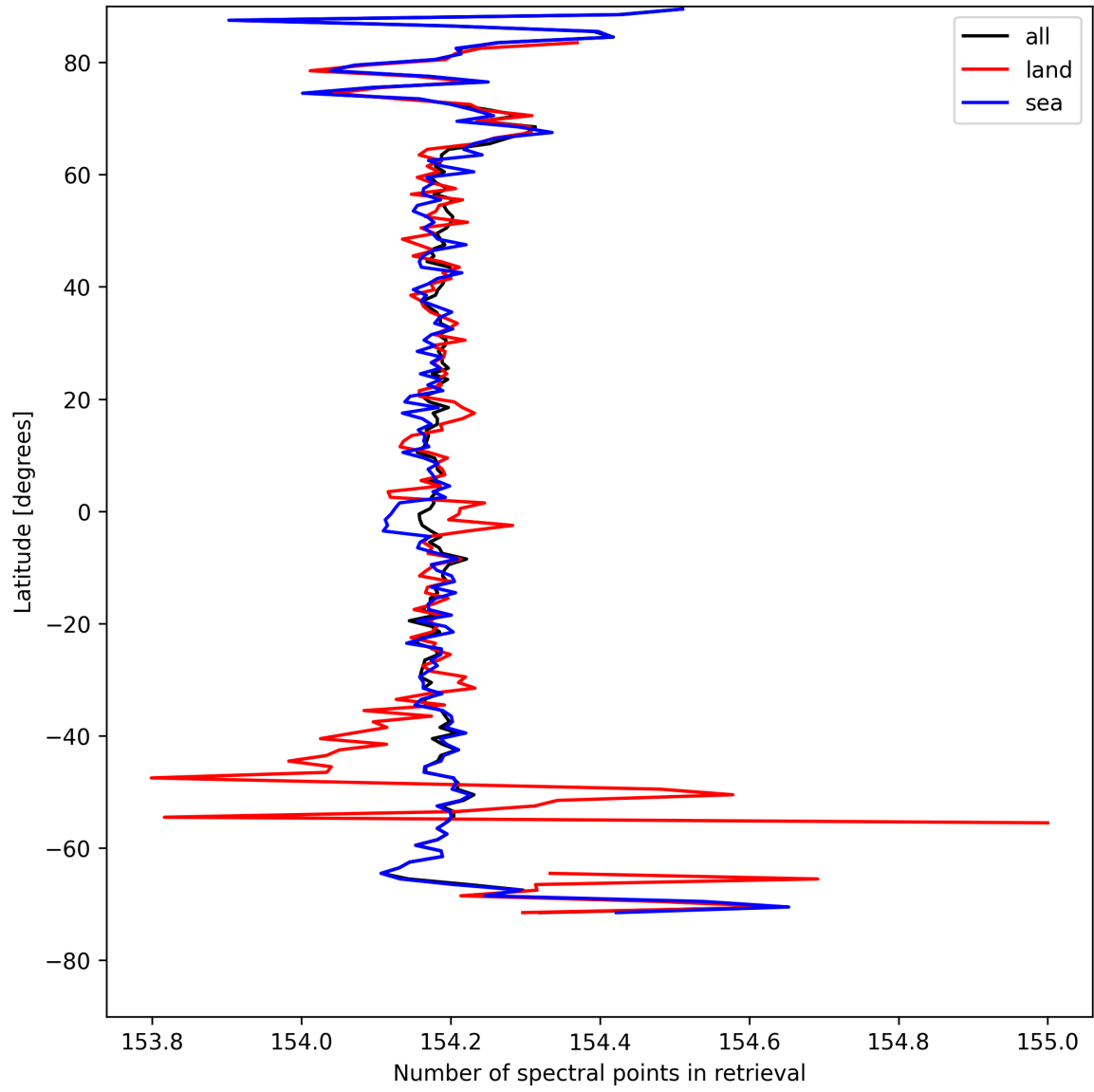
Figure 9: Zonal average of “Number of spectral points in retrieval” for 2025-04-25 to 2025-04-26.
