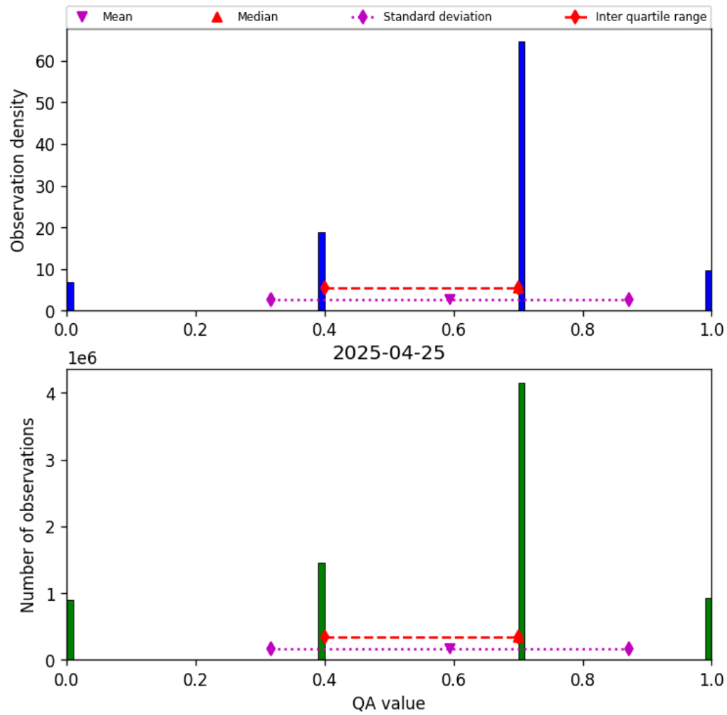
Figure 13: Histogram of “QA value” for 2025-04-25 to 2025-04-26
