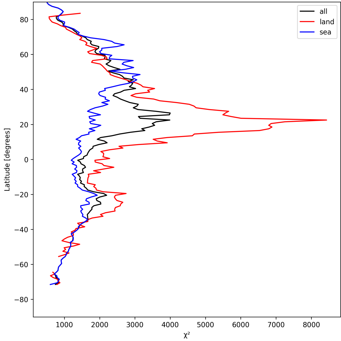
Figure 10: Zonal average of “ \chi^2 ” for 2025-04-25 to 2025-04-26.
