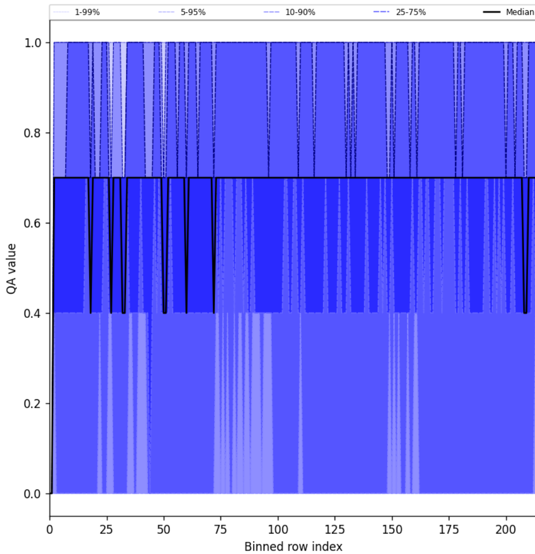
Figure 20: Along track statistics of “QA value” for 2025-04-25 to 2025-04-26
