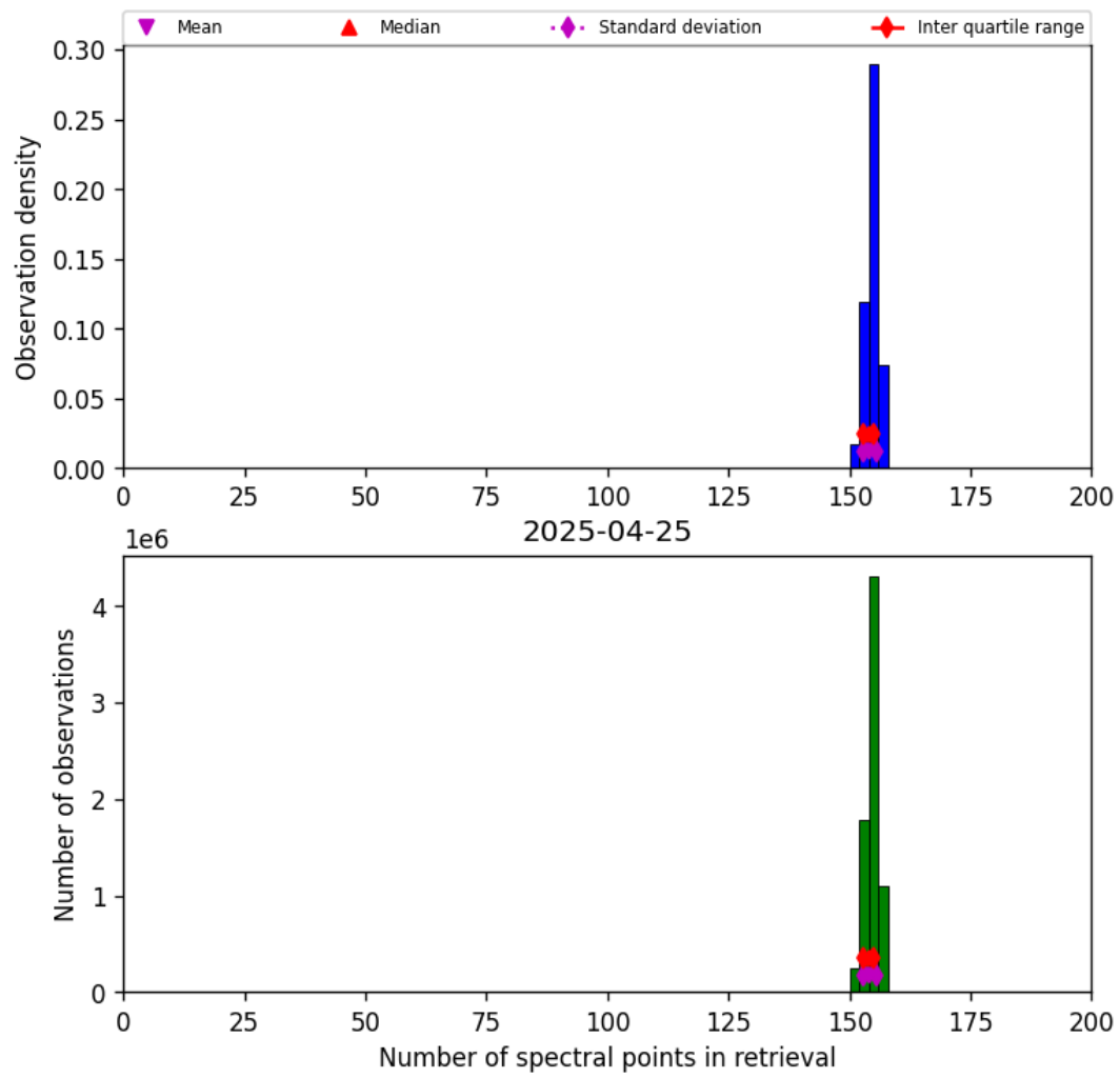
Figure 16: Histogram of “Number of spectral points in retrieval” for 2025-04-25 to 2025-04-26
