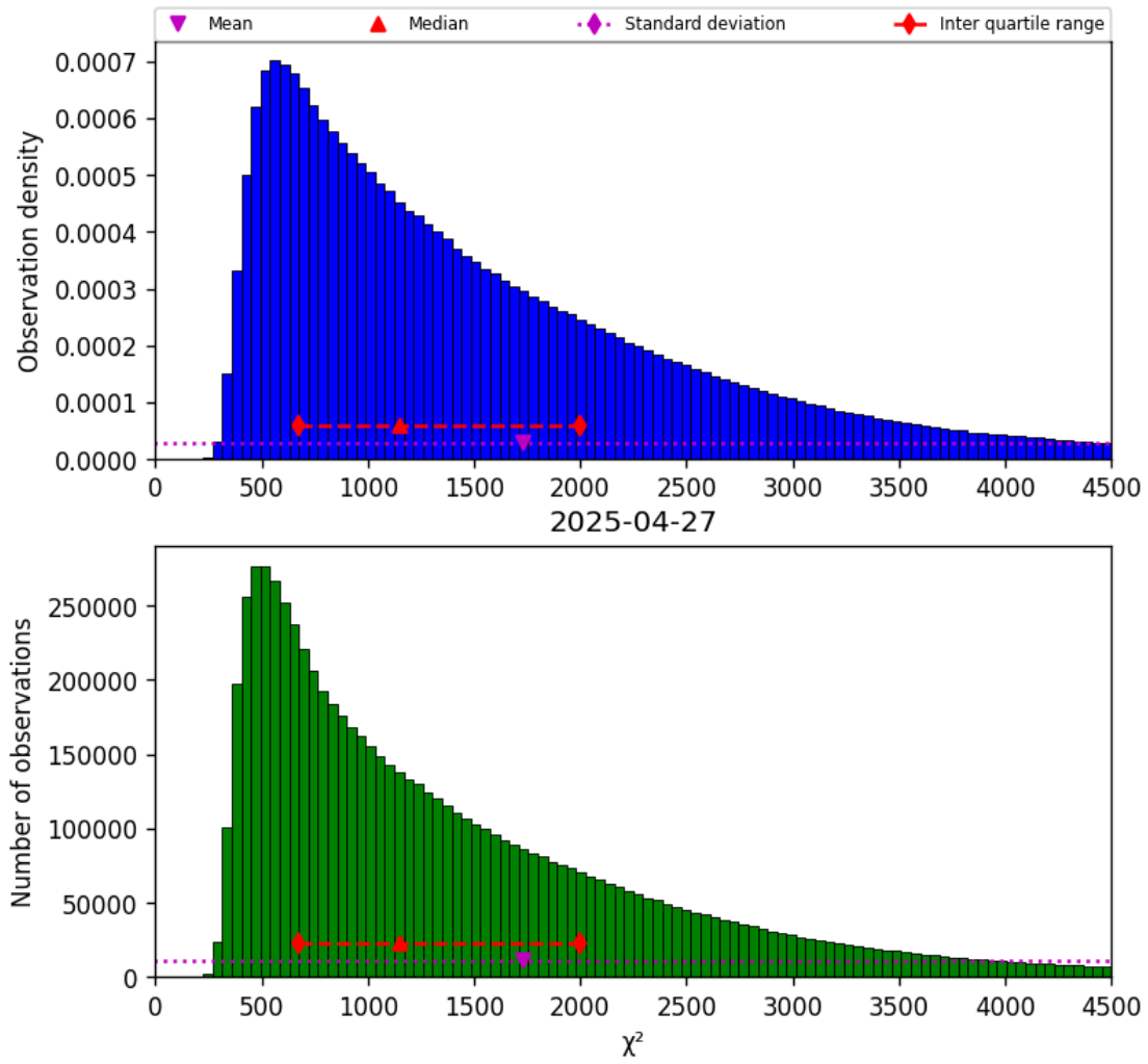
Figure 17: Histogram of “ \chi^2 ” for 2025-04-27 to 2025-04-27
