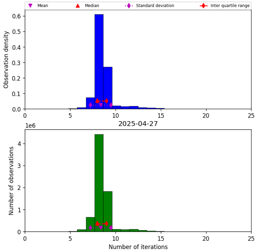
Figure 19: Histogram of “Number of iterations” for 2025-04-27 to 2025-04-27
