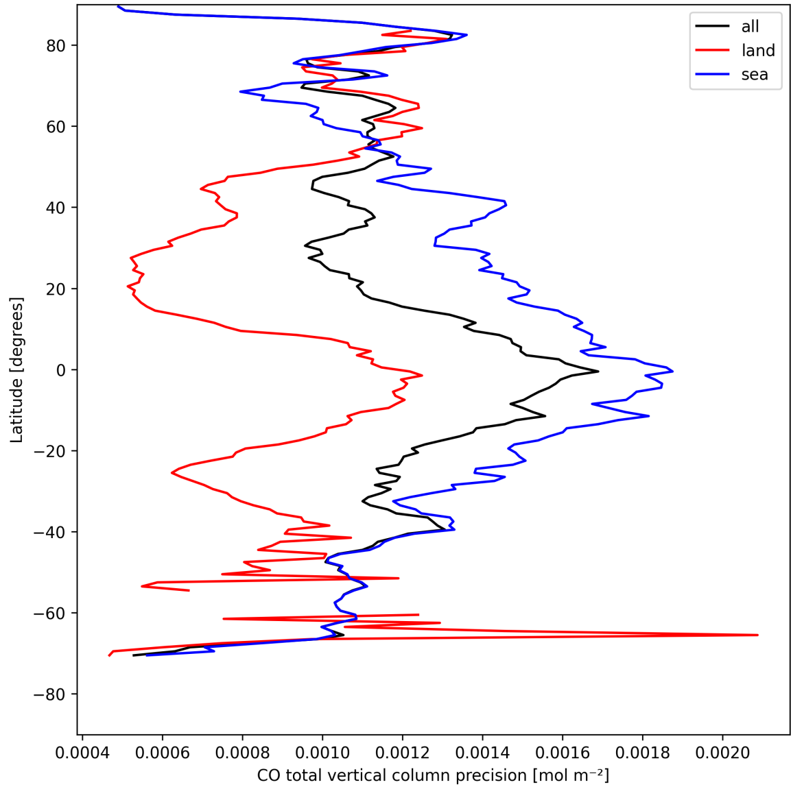
Figure 8: Zonal average of “CO total vertical column precision” for 2025-04-27 to 2025-04-27.
