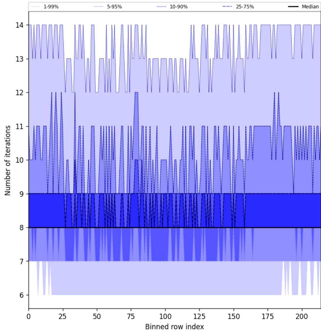
Figure 26: Along track statistics of “Number of iterations” for 2025-04-27 to 2025-04-27
