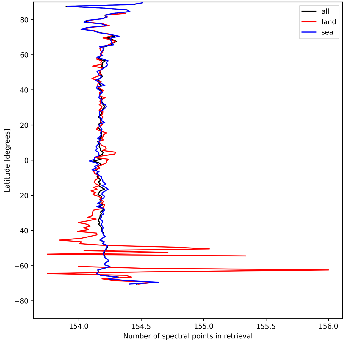
Figure 9: Zonal average of “Number of spectral points in retrieval” for 2025-04-27 to 2025-04-27.
