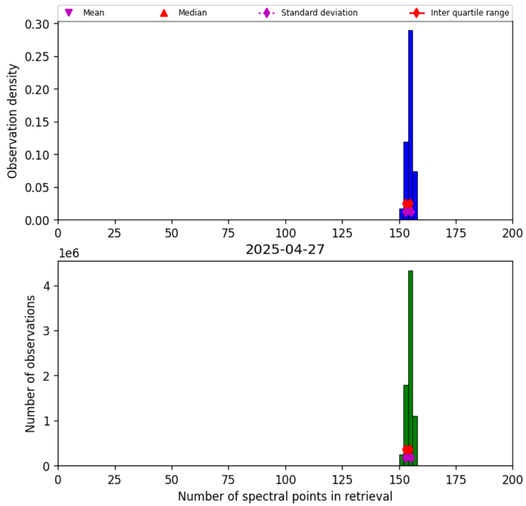
Figure 16: Histogram of “Number of spectral points in retrieval” for 2025-04-27 to 2025-04-27
