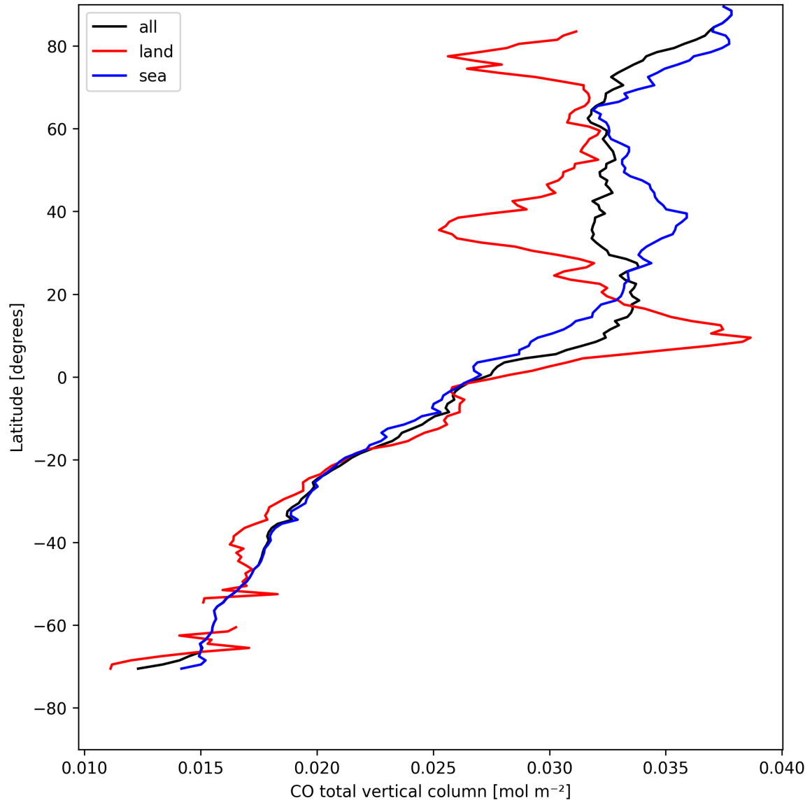
Figure 7: Zonal average of “CO total vertical column” for 2025-04-27 to 2025-04-27.
