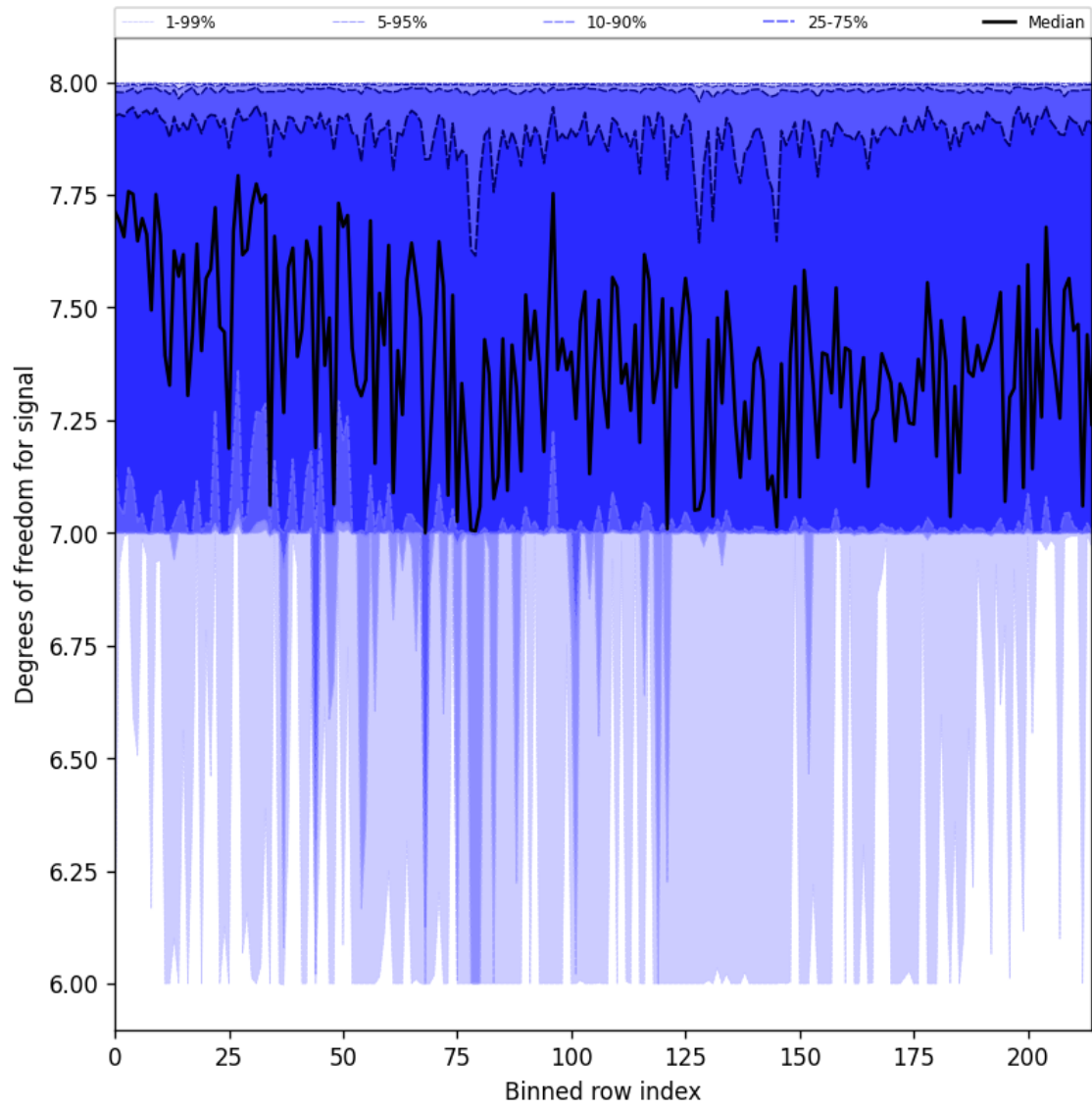
Figure 25: Along track statistics of “Degrees of freedom for signal” for 2025-04-27 to 2025-04-27
