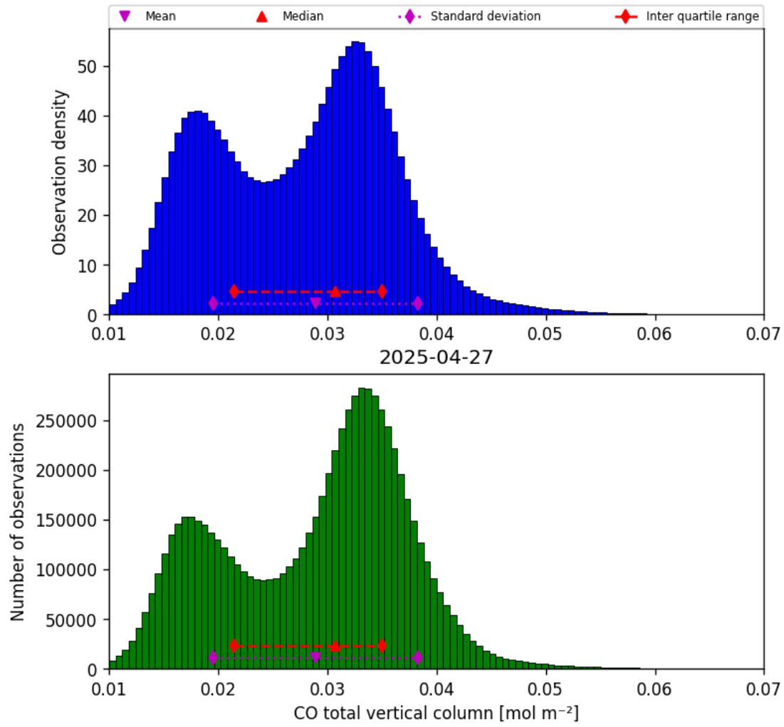
Figure 14: Histogram of “CO total vertical column” for 2025-04-27 to 2025-04-27
