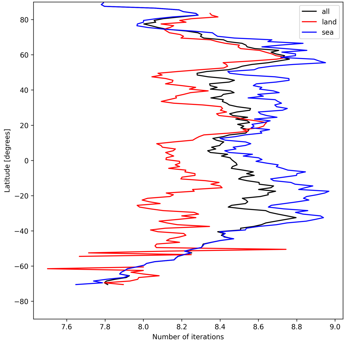
Figure 12: Zonal average of “Number of iterations” for 2025-04-27 to 2025-04-27.
