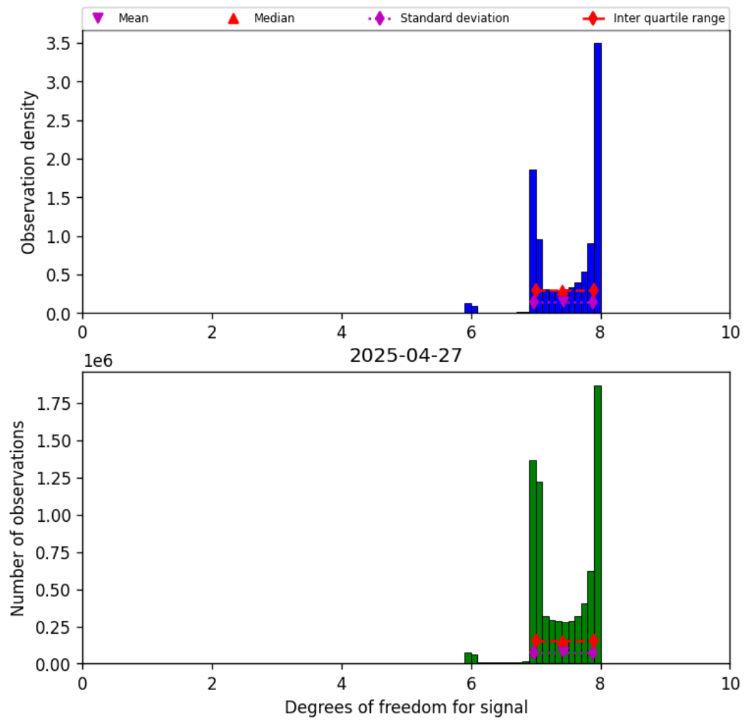
Figure 18: Histogram of “Degrees of freedom for signal” for 2025-04-27 to 2025-04-27
