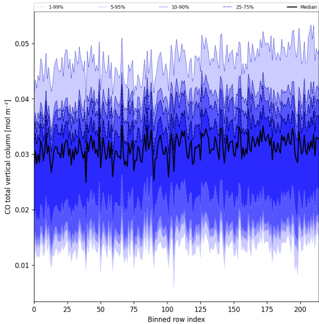
Figure 21: Along track statistics of “CO total vertical column” for 2025-04-27 to 2025-04-27
