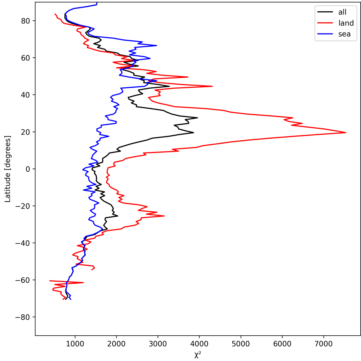
Figure 10: Zonal average of “ \chi^2 ” for 2025-04-27 to 2025-04-27.
