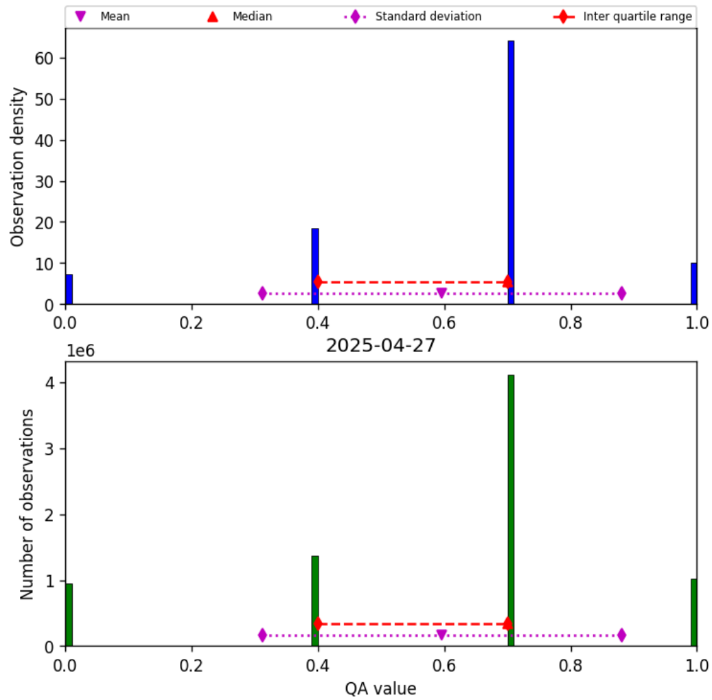
Figure 13: Histogram of “QA value” for 2025-04-27 to 2025-04-27
