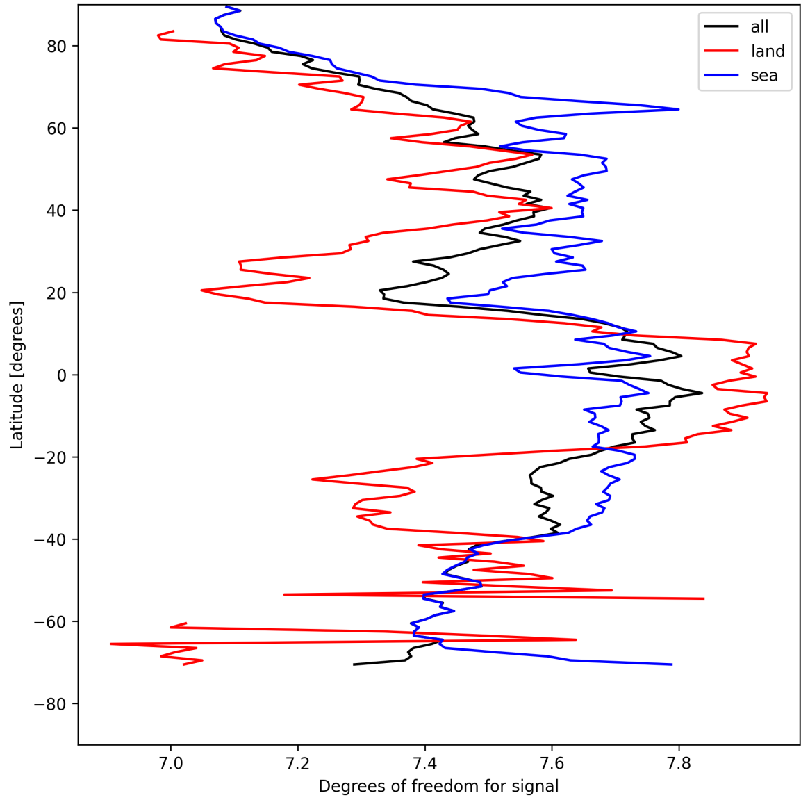
Figure 11: Zonal average of “Degrees of freedom for signal” for 2025-04-27 to 2025-04-27.
