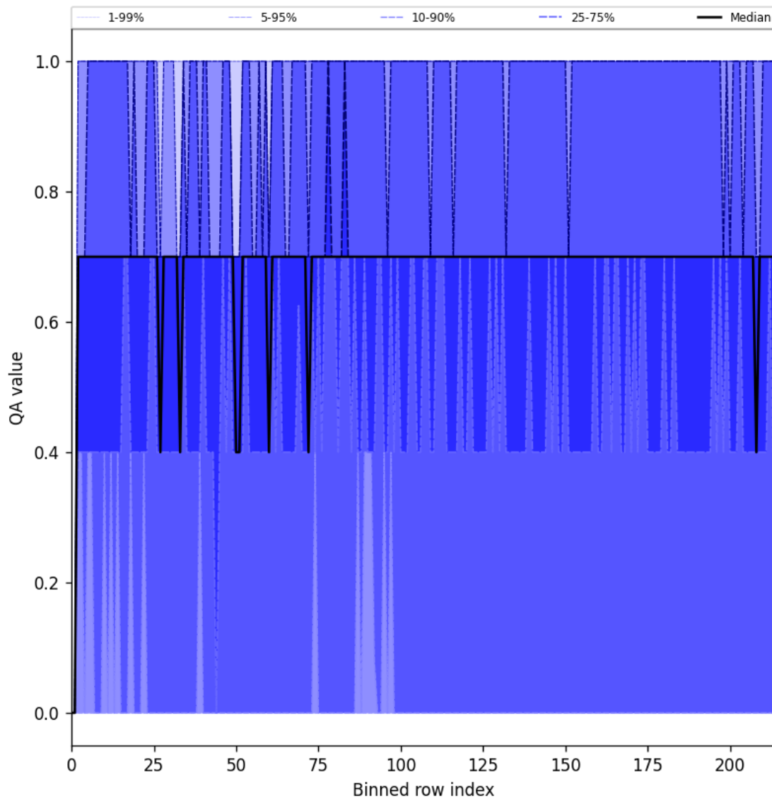
Figure 20: Along track statistics of “QA value” for 2025-04-27 to 2025-04-27
