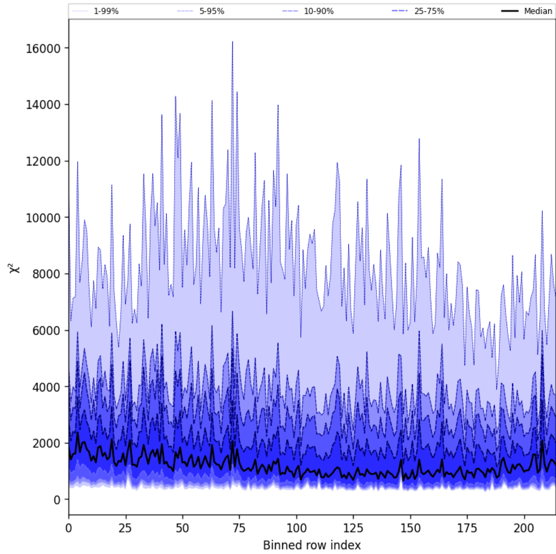
Figure 24: Along track statistics of “ \chi^2 ” for 2025-04-27 to 2025-04-27
