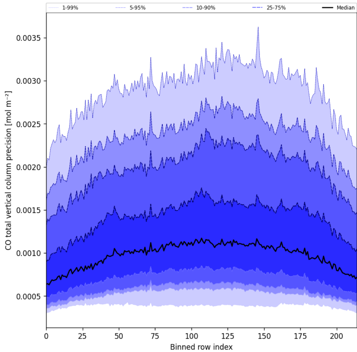
Figure 22: Along track statistics of “CO total vertical column precision” for 2025-04-27 to 2025-04-27
