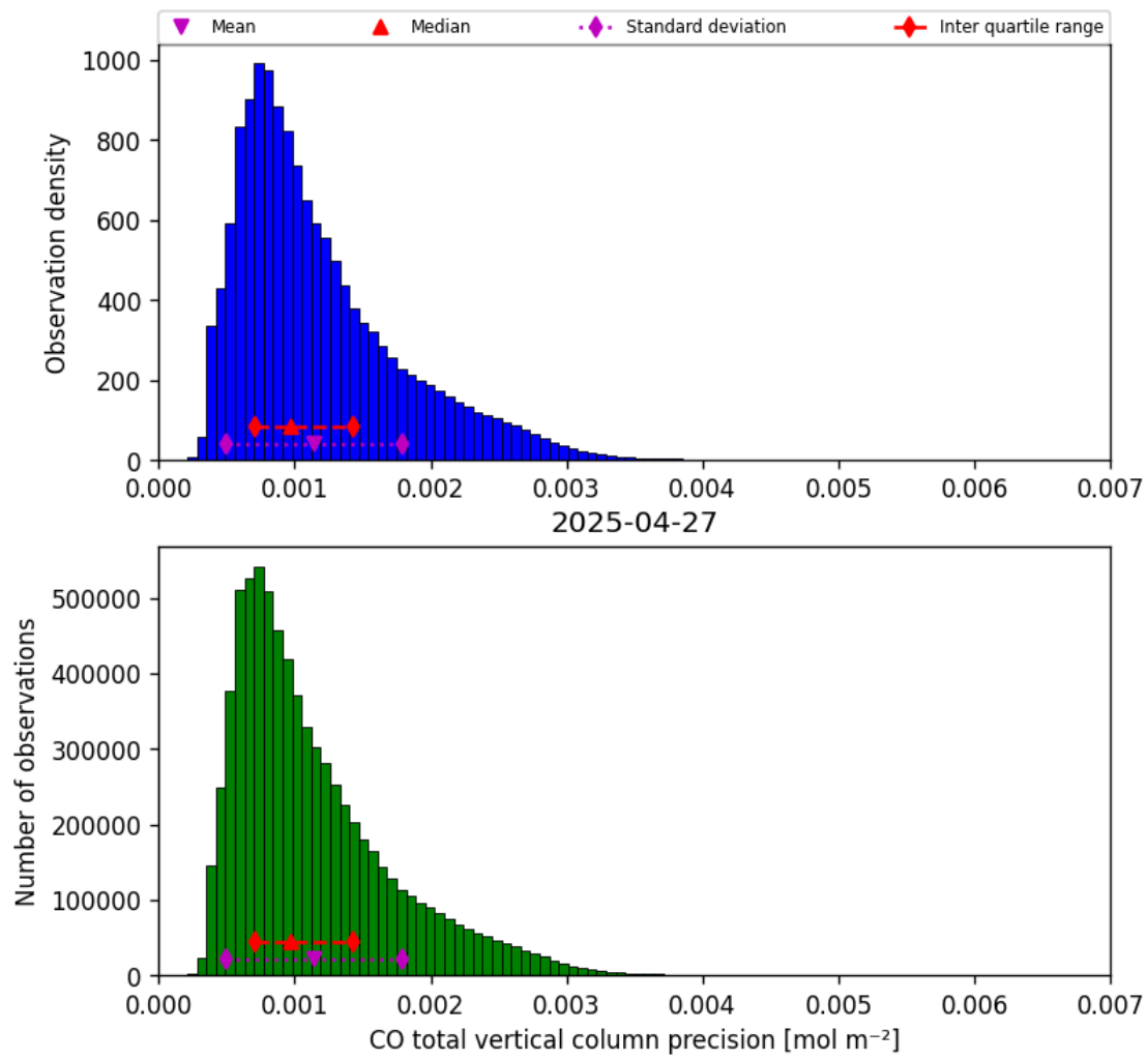
Figure 15: Histogram of “CO total vertical column precision” for 2025-04-27 to 2025-04-27
