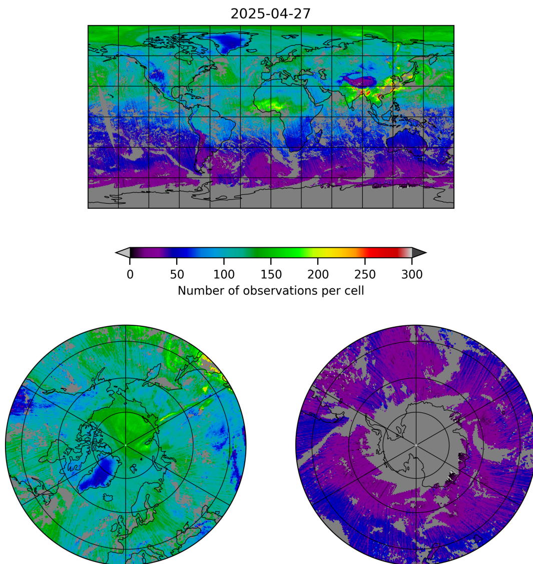
Figure 5: Map of the number of observations for 2025-04-27 to 2025-04-27
