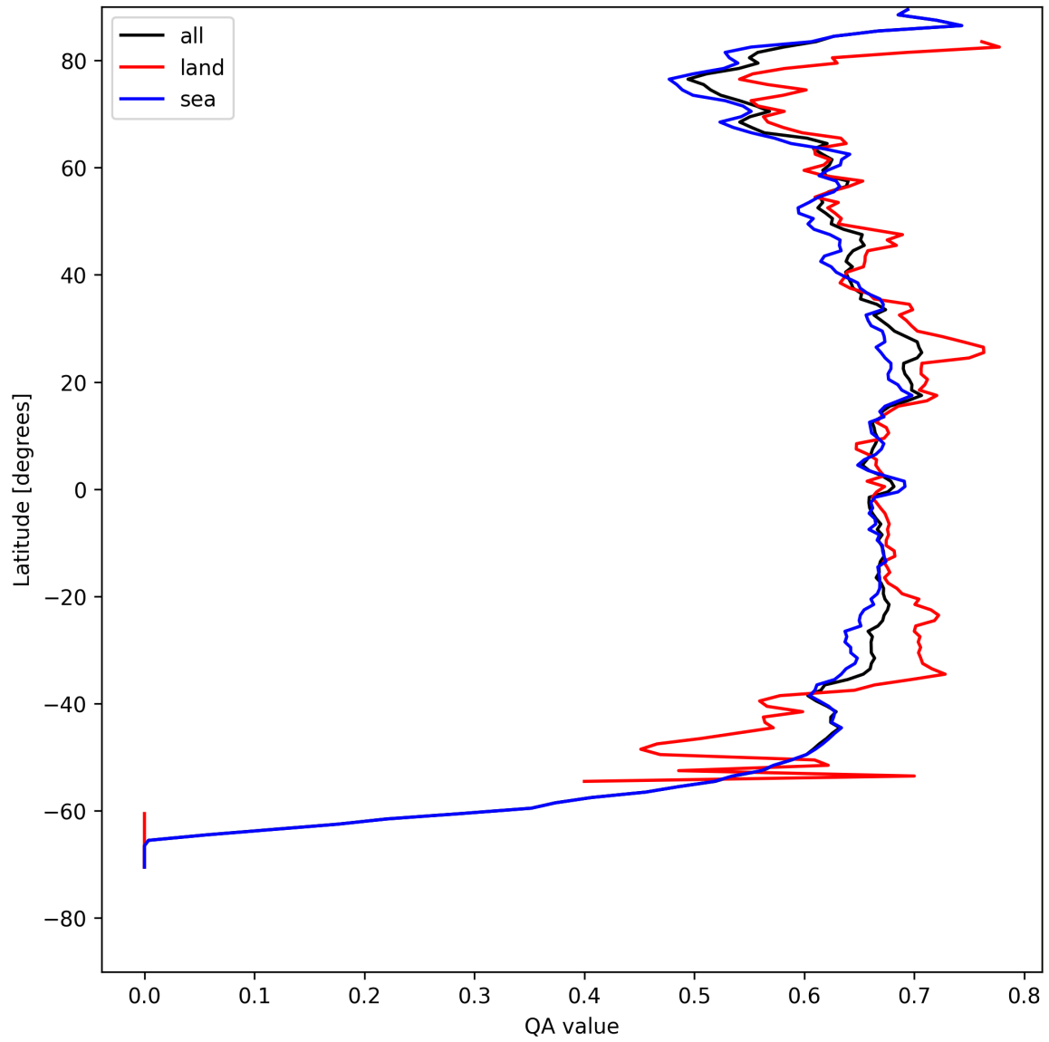
Figure 6: Zonal average of “QA value” for 2025-04-27 to 2025-04-27.
