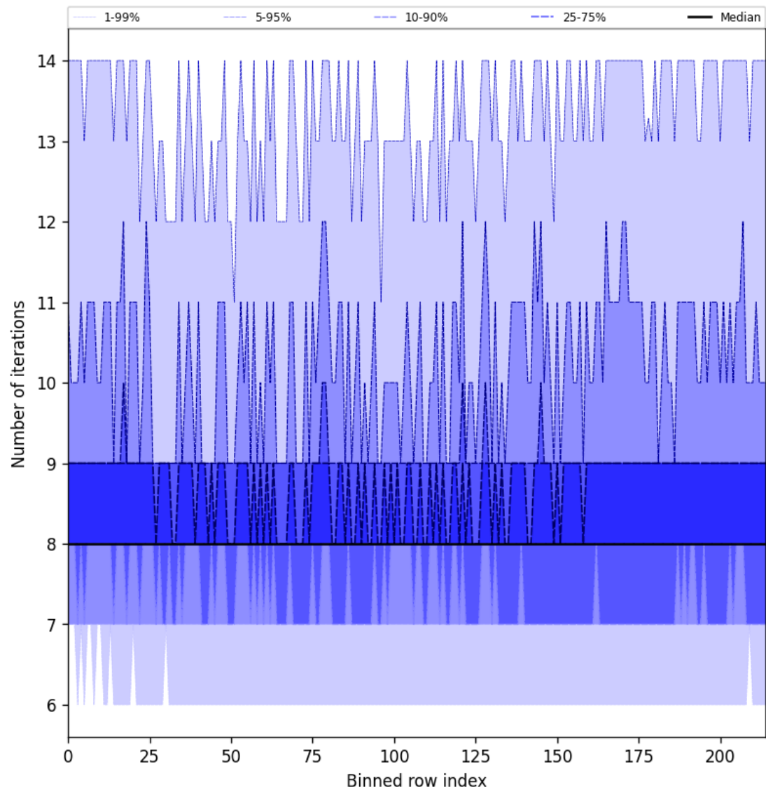
Figure 26: Along track statistics of “Number of iterations” for 2025-04-28 to 2025-04-29
