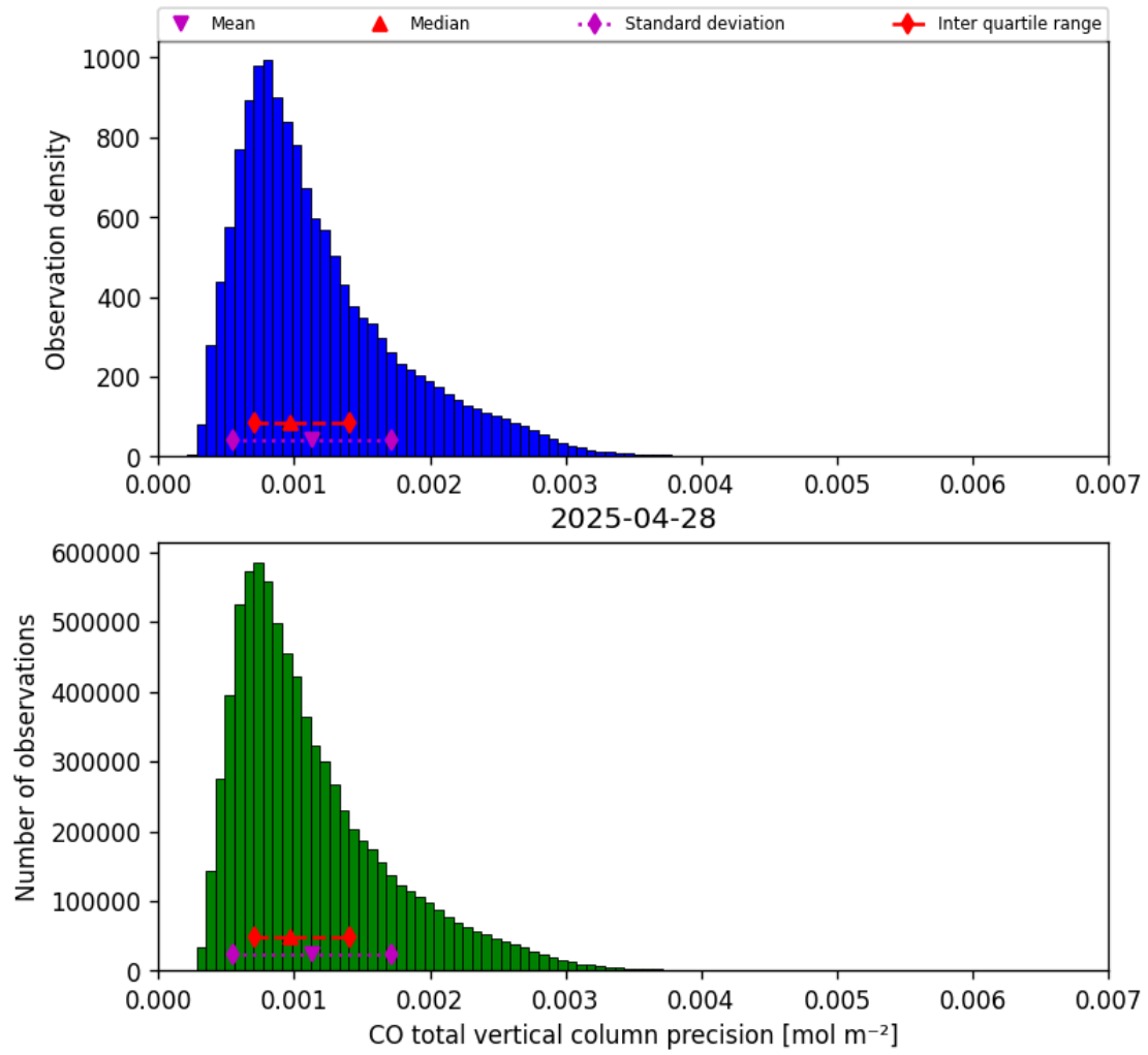
Figure 15: Histogram of “CO total vertical column precision” for 2025-04-28 to 2025-04-29
