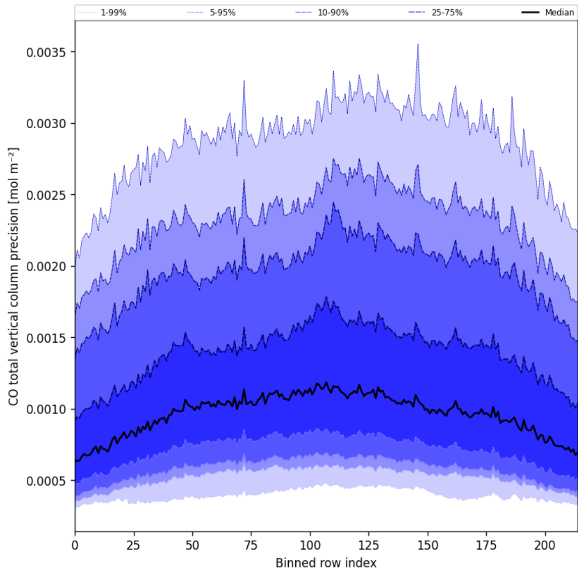
Figure 22: Along track statistics of “CO total vertical column precision” for 2025-04-28 to 2025-04-29
