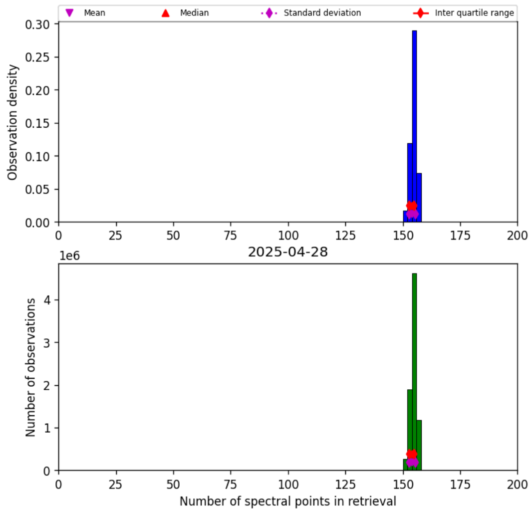
Figure 16: Histogram of “Number of spectral points in retrieval” for 2025-04-28 to 2025-04-29
