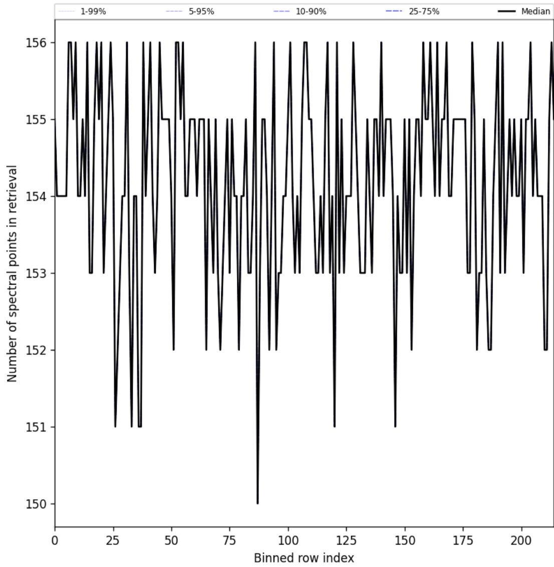
Figure 23: Along track statistics of “Number of spectral points in retrieval” for 2025-04-28 to 2025-04-29
