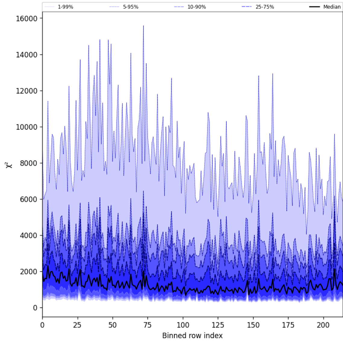
Figure 24: Along track statistics of “ \chi^2 ” for 2025-04-28 to 2025-04-29
