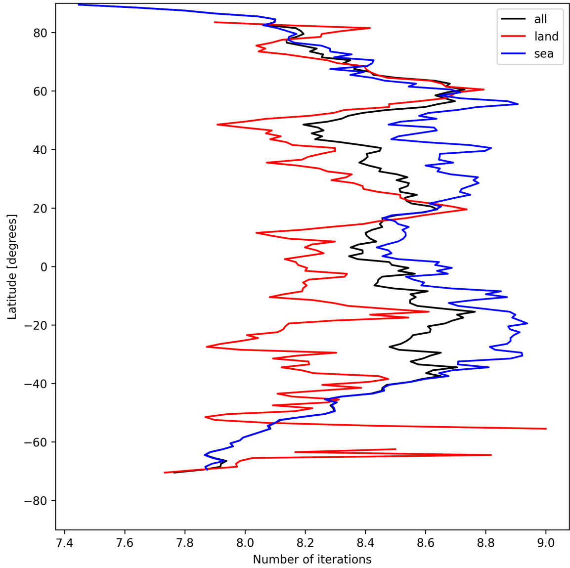
Figure 12: Zonal average of “Number of iterations” for 2025-04-29 to 2025-04-30.
