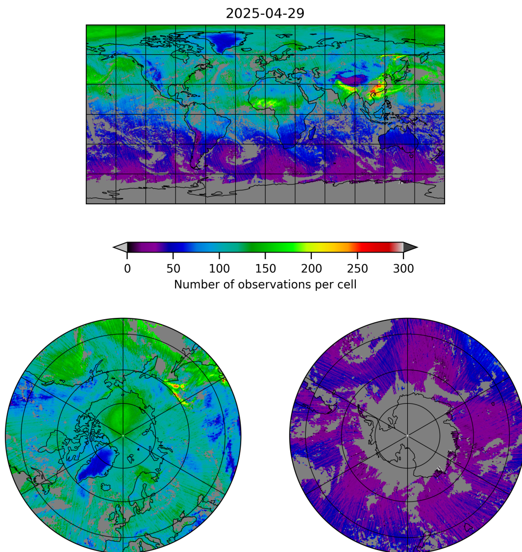
Figure 5: Map of the number of observations for 2025-04-29 to 2025-04-30
