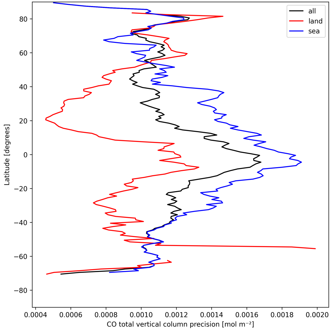
Figure 8: Zonal average of “CO total vertical column precision” for 2025-04-29 to 2025-04-30.
