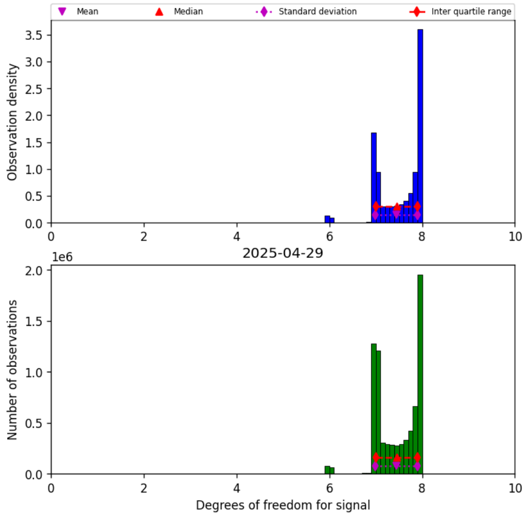
Figure 18: Histogram of “Degrees of freedom for signal” for 2025-04-29 to 2025-04-30
