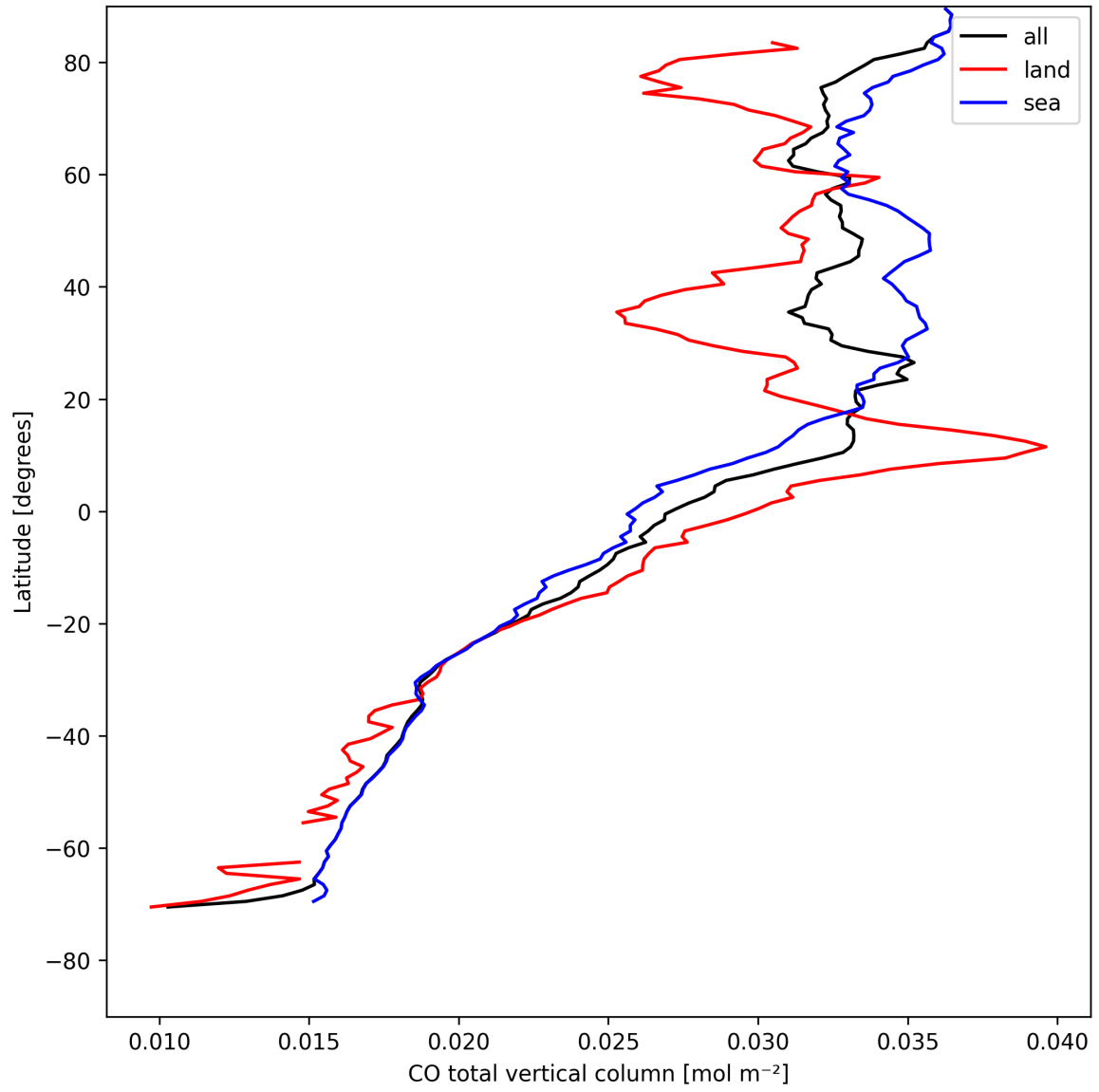
Figure 7: Zonal average of “CO total vertical column” for 2025-04-29 to 2025-04-30.
