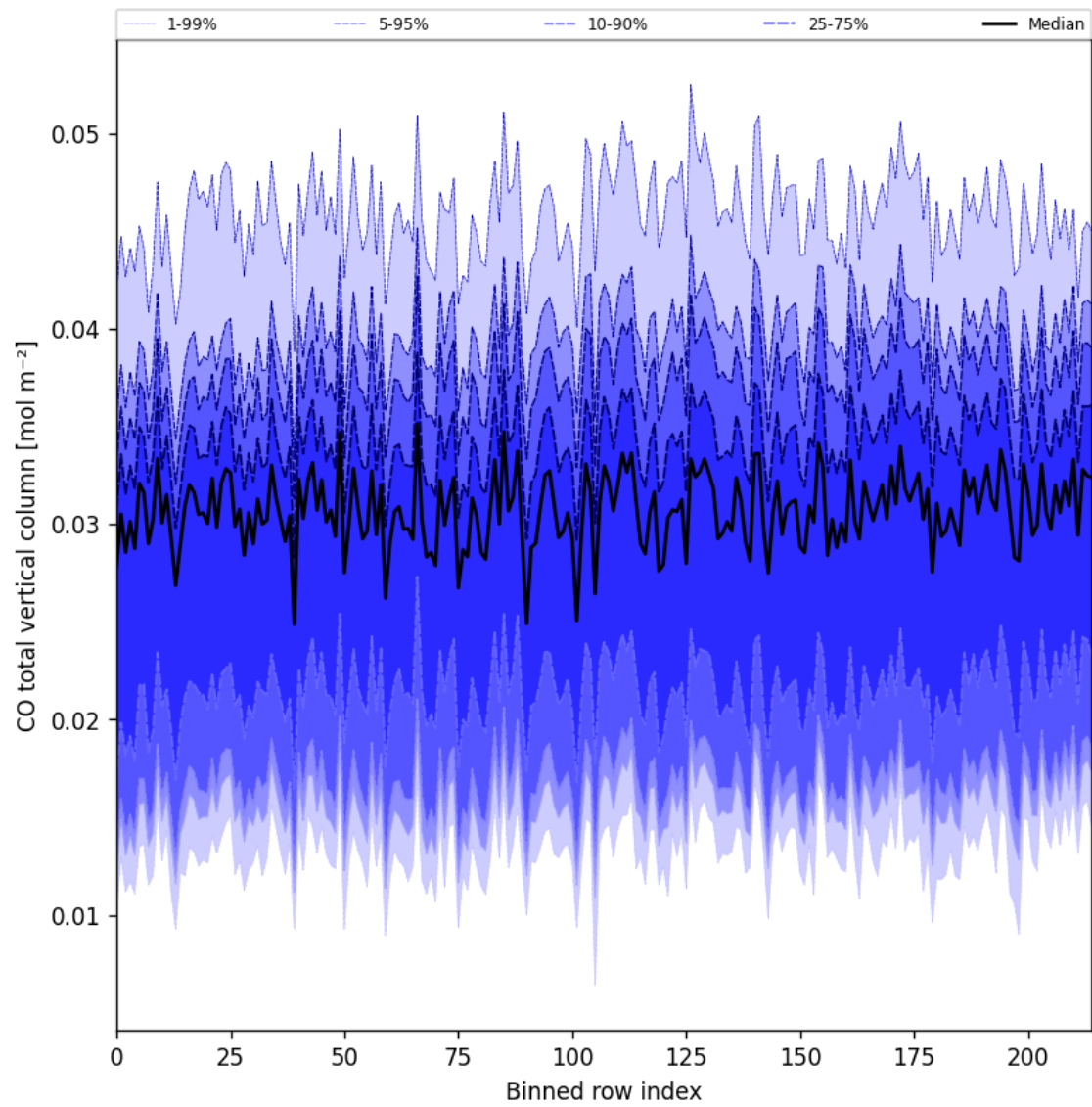
Figure 21: Along track statistics of “CO total vertical column” for 2025-04-29 to 2025-04-30
