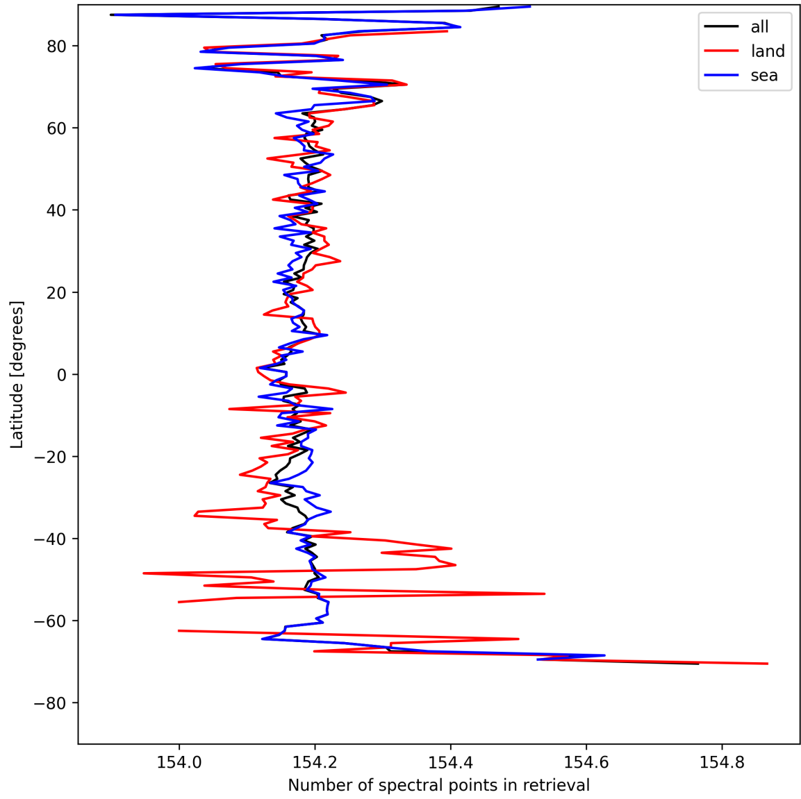
Figure 9: Zonal average of “Number of spectral points in retrieval” for 2025-04-29 to 2025-04-30.
