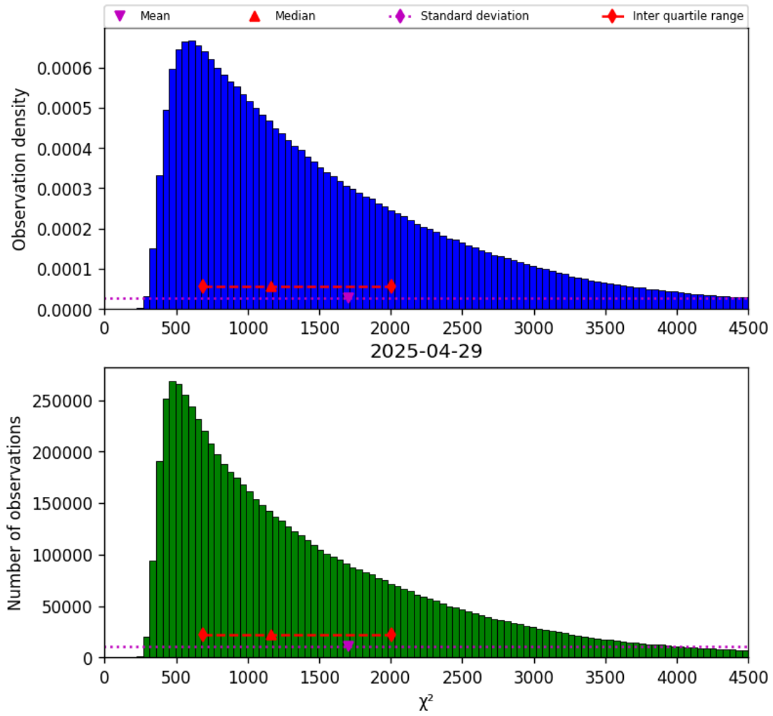
Figure 17: Histogram of “ \chi^2 ” for 2025-04-29 to 2025-04-30
