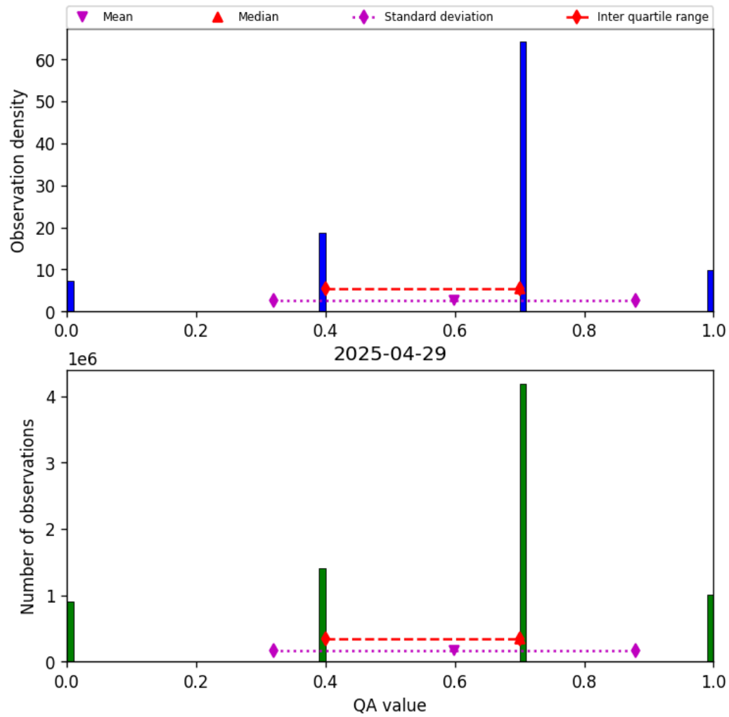
Figure 13: Histogram of “QA value” for 2025-04-29 to 2025-04-30
