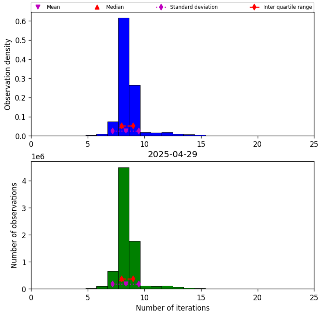
Figure 19: Histogram of “Number of iterations” for 2025-04-29 to 2025-04-30
