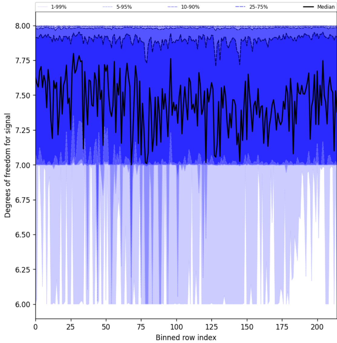
Figure 25: Along track statistics of “Degrees of freedom for signal” for 2025-04-29 to 2025-04-30
