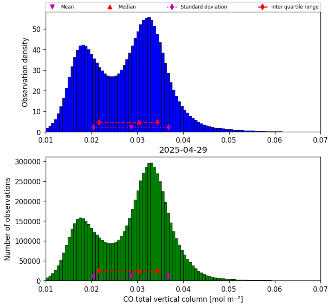
Figure 14: Histogram of “CO total vertical column” for 2025-04-29 to 2025-04-30
