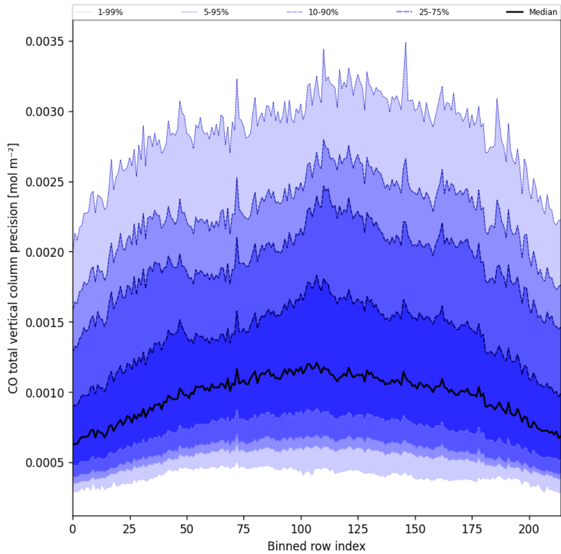
Figure 22: Along track statistics of “CO total vertical column precision” for 2025-04-29 to 2025-04-30
