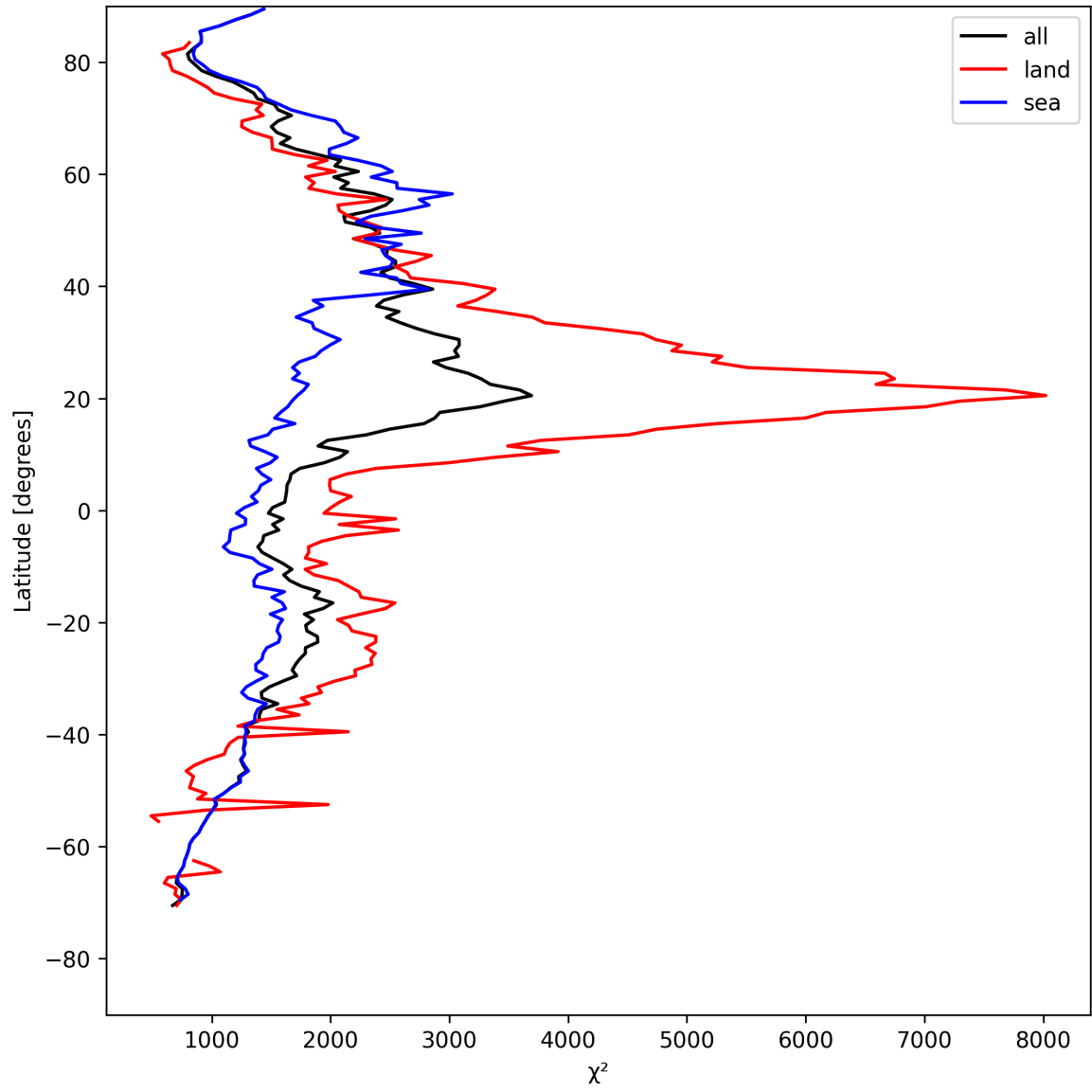
Figure 10: Zonal average of “ \chi^2 ” for 2025-04-29 to 2025-04-30.
