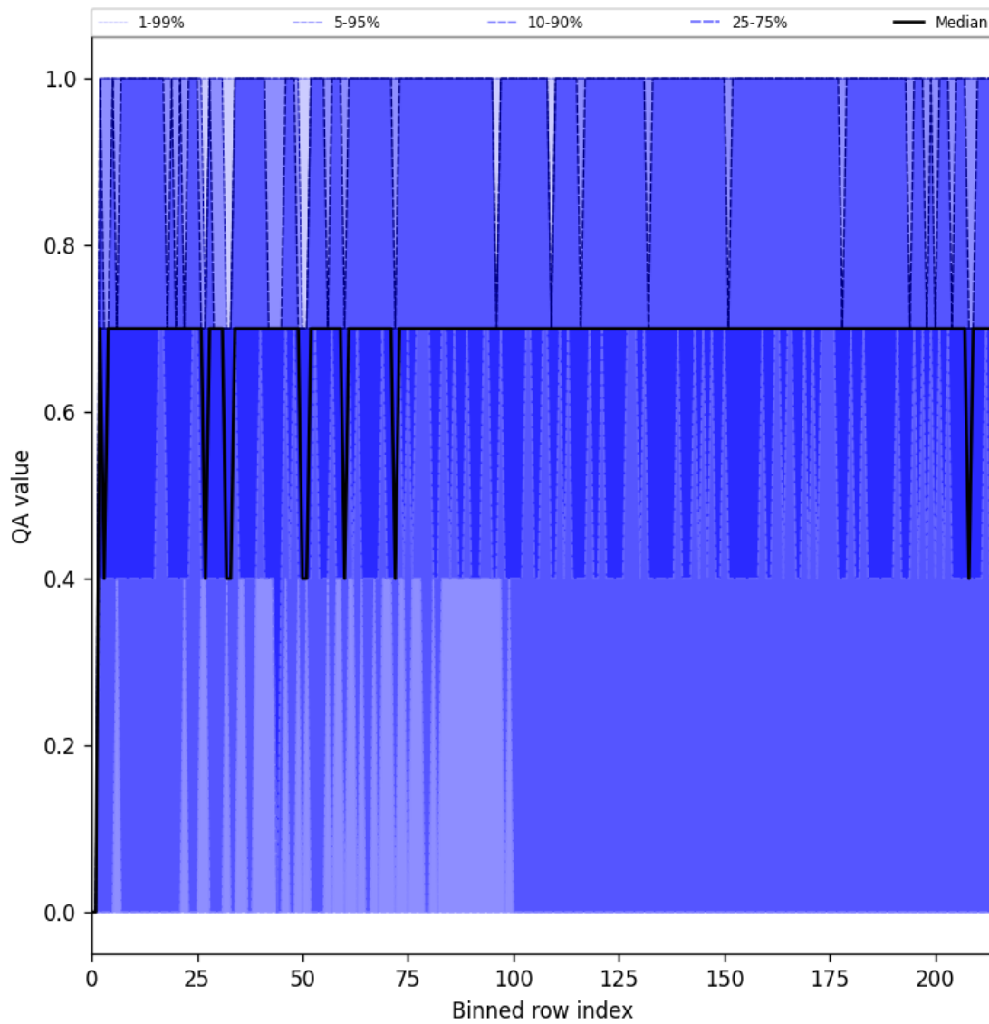
Figure 20: Along track statistics of “QA value” for 2025-04-29 to 2025-04-30
