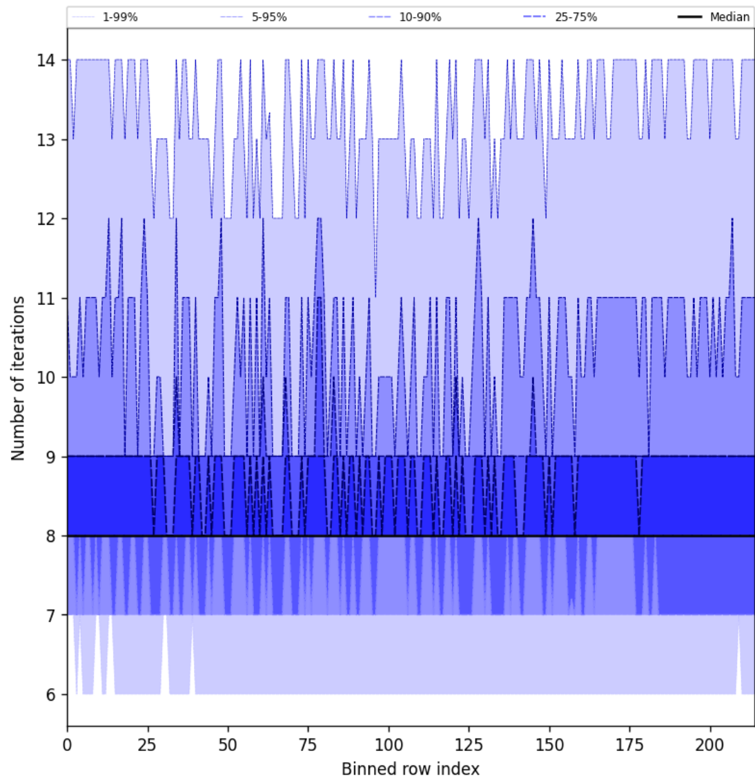
Figure 26: Along track statistics of “Number of iterations” for 2025-04-29 to 2025-04-30
