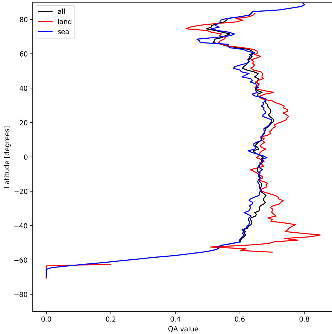
Figure 6: Zonal average of “QA value” for 2025-04-29 to 2025-04-30.
