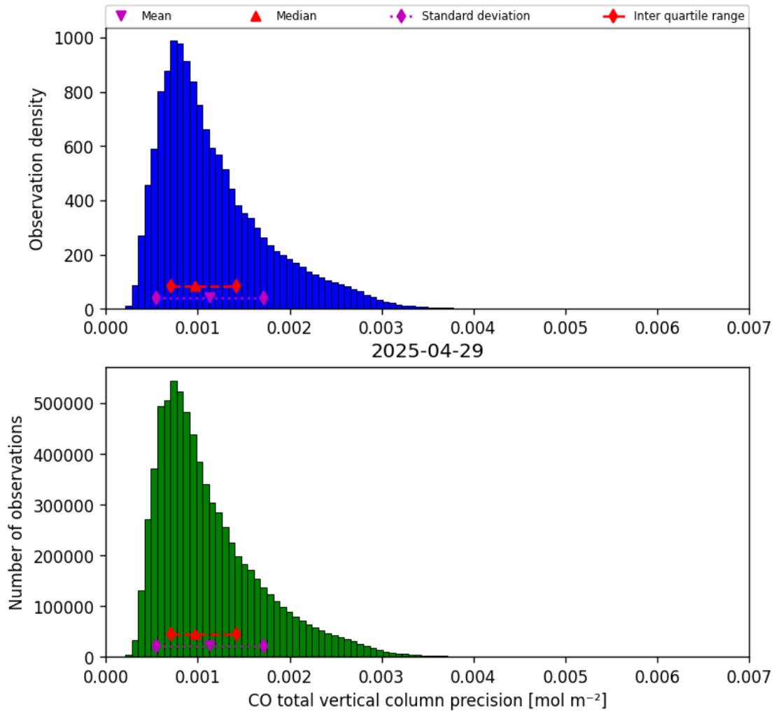
Figure 15: Histogram of “CO total vertical column precision” for 2025-04-29 to 2025-04-30
