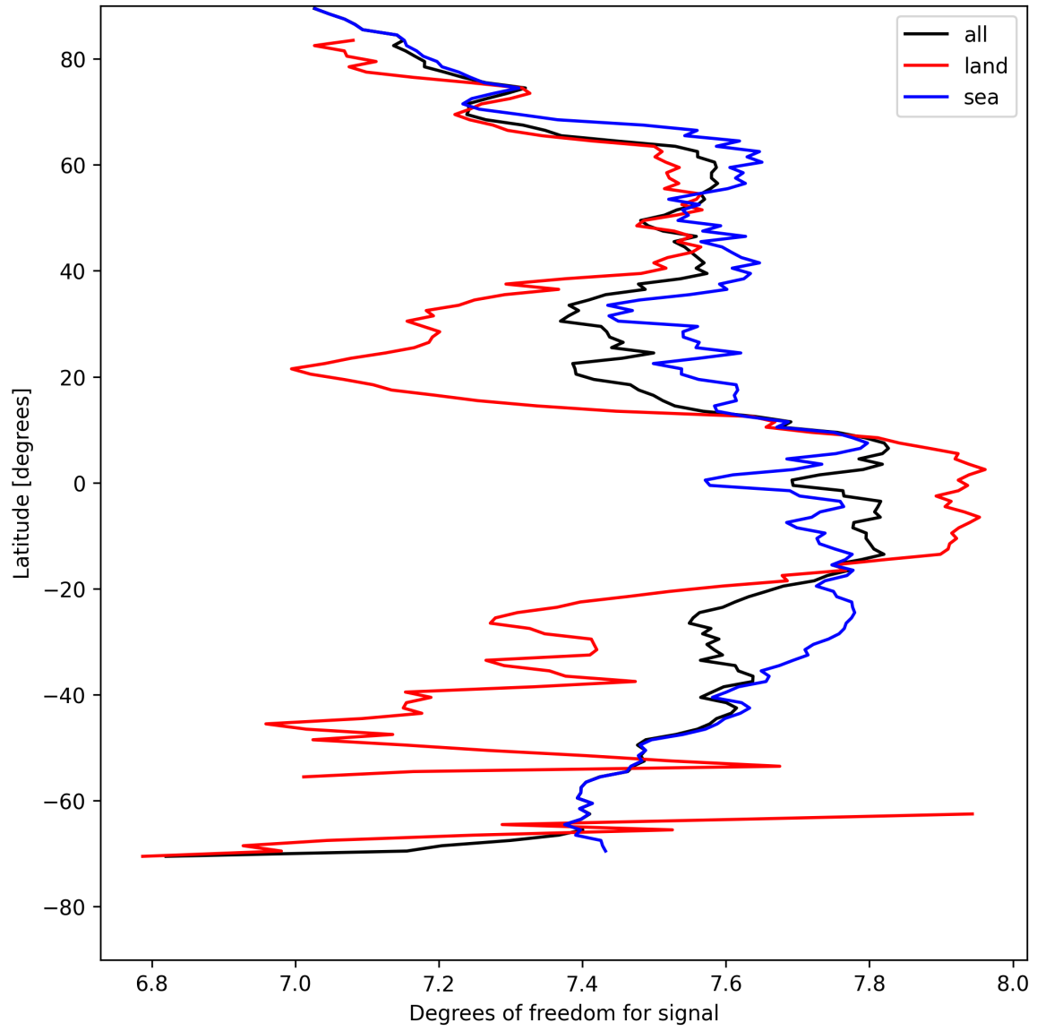
Figure 11: Zonal average of “Degrees of freedom for signal” for 2025-04-29 to 2025-04-30.
