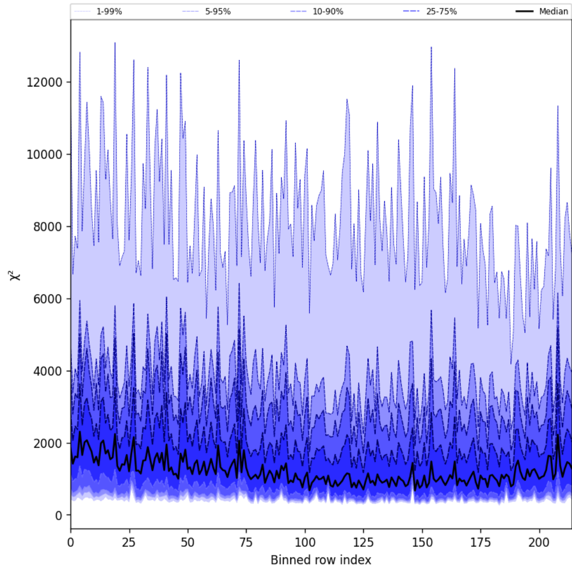
Figure 24: Along track statistics of “ \chi^2 ” for 2025-04-29 to 2025-04-30
