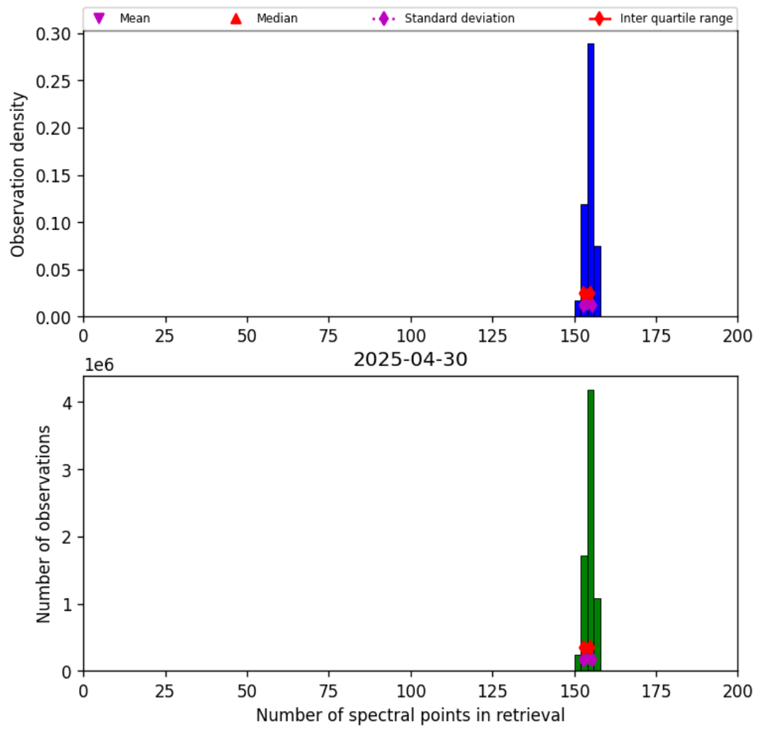
Figure 16: Histogram of “Number of spectral points in retrieval” for 2025-04-30 to 2025-05-01
