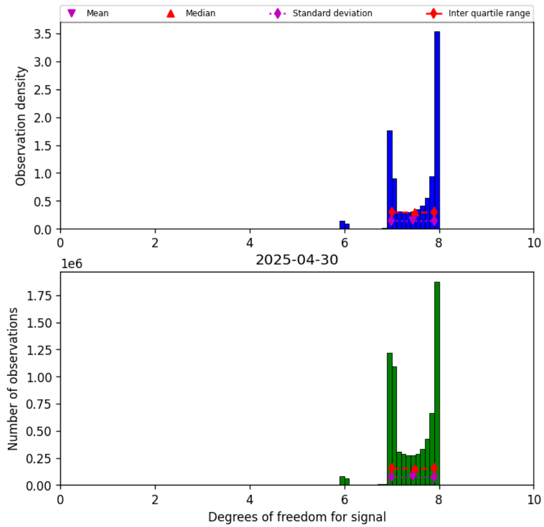
Figure 18: Histogram of “Degrees of freedom for signal” for 2025-04-30 to 2025-05-01
