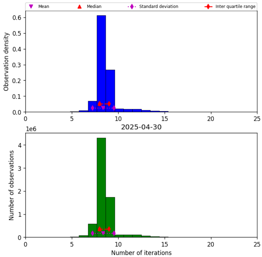
Figure 19: Histogram of “Number of iterations” for 2025-04-30 to 2025-05-01
