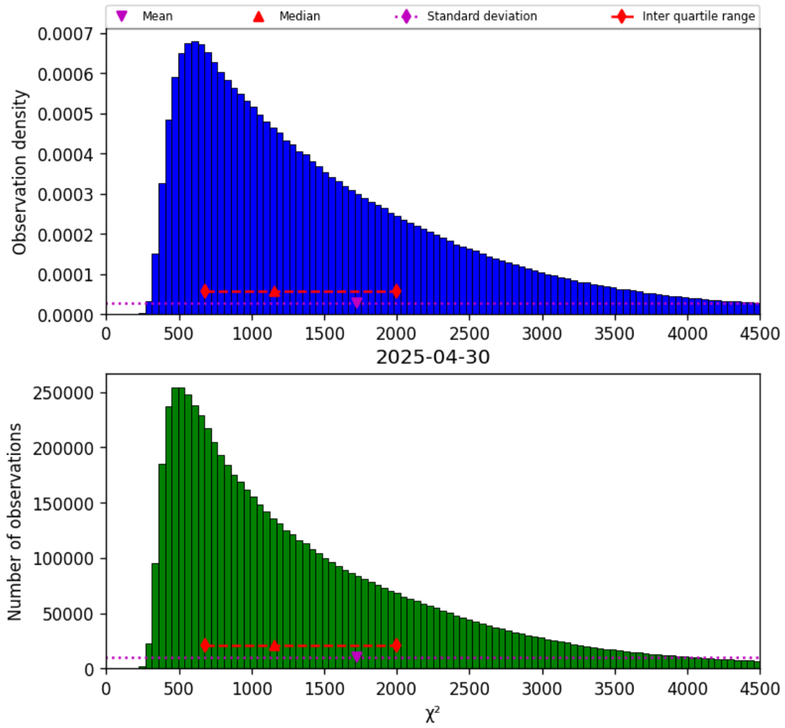
Figure 17: Histogram of " \chi^2 " for 2025-04-30 to 2025-05-01
