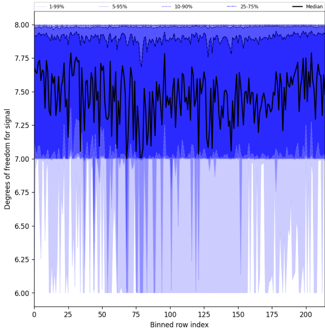
Figure 25: Along track statistics of “Degrees of freedom for signal” for 2025-04-30 to 2025-05-01
