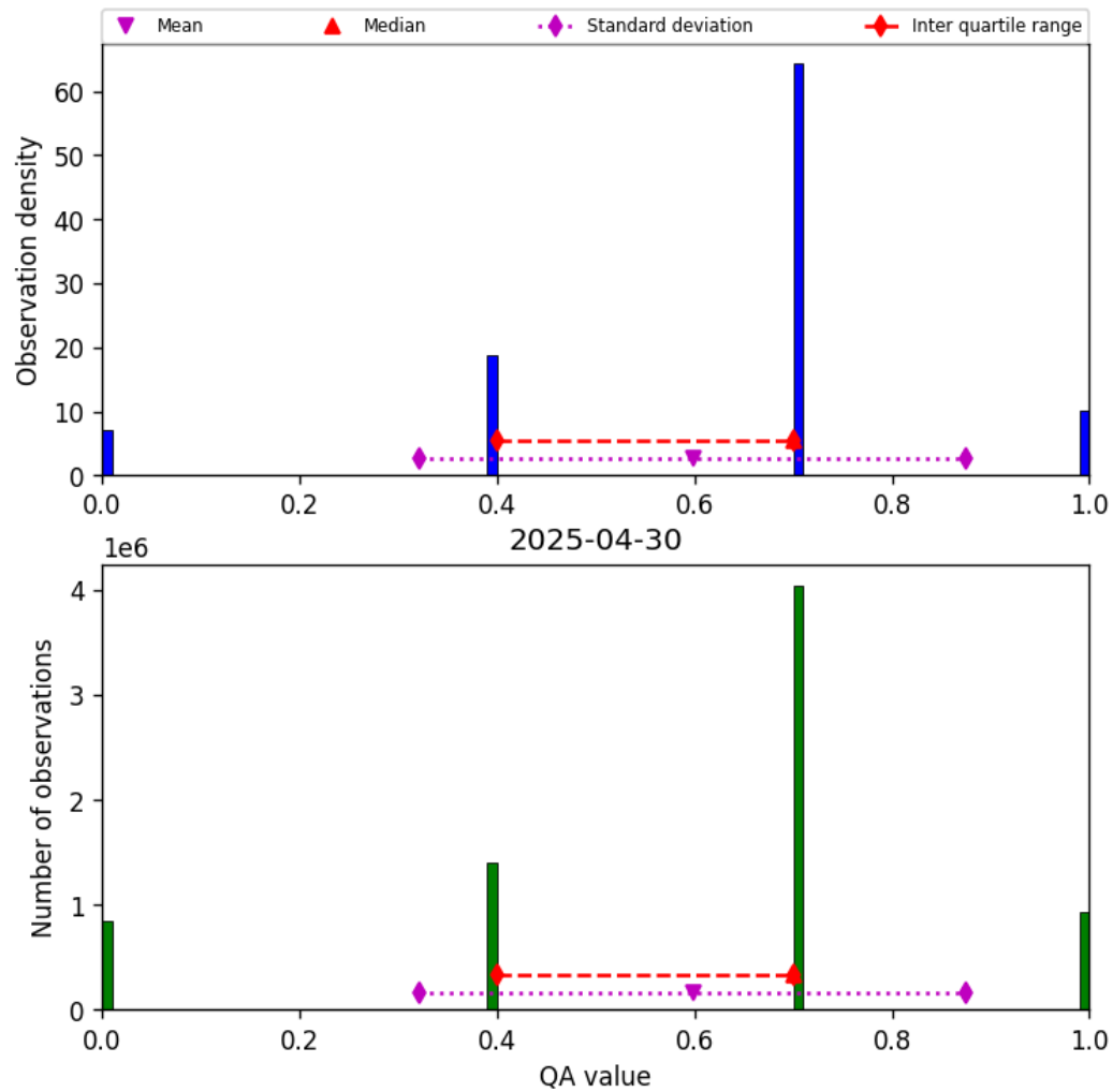
Figure 13: Histogram of “QA value” for 2025-04-30 to 2025-05-01
