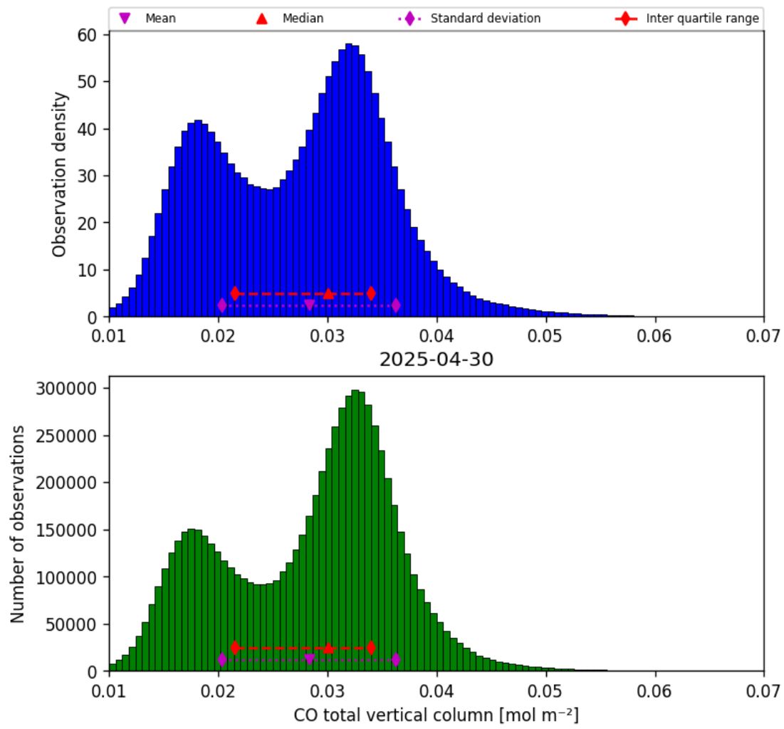
Figure 14: Histogram of “CO total vertical column” for 2025-04-30 to 2025-05-01
