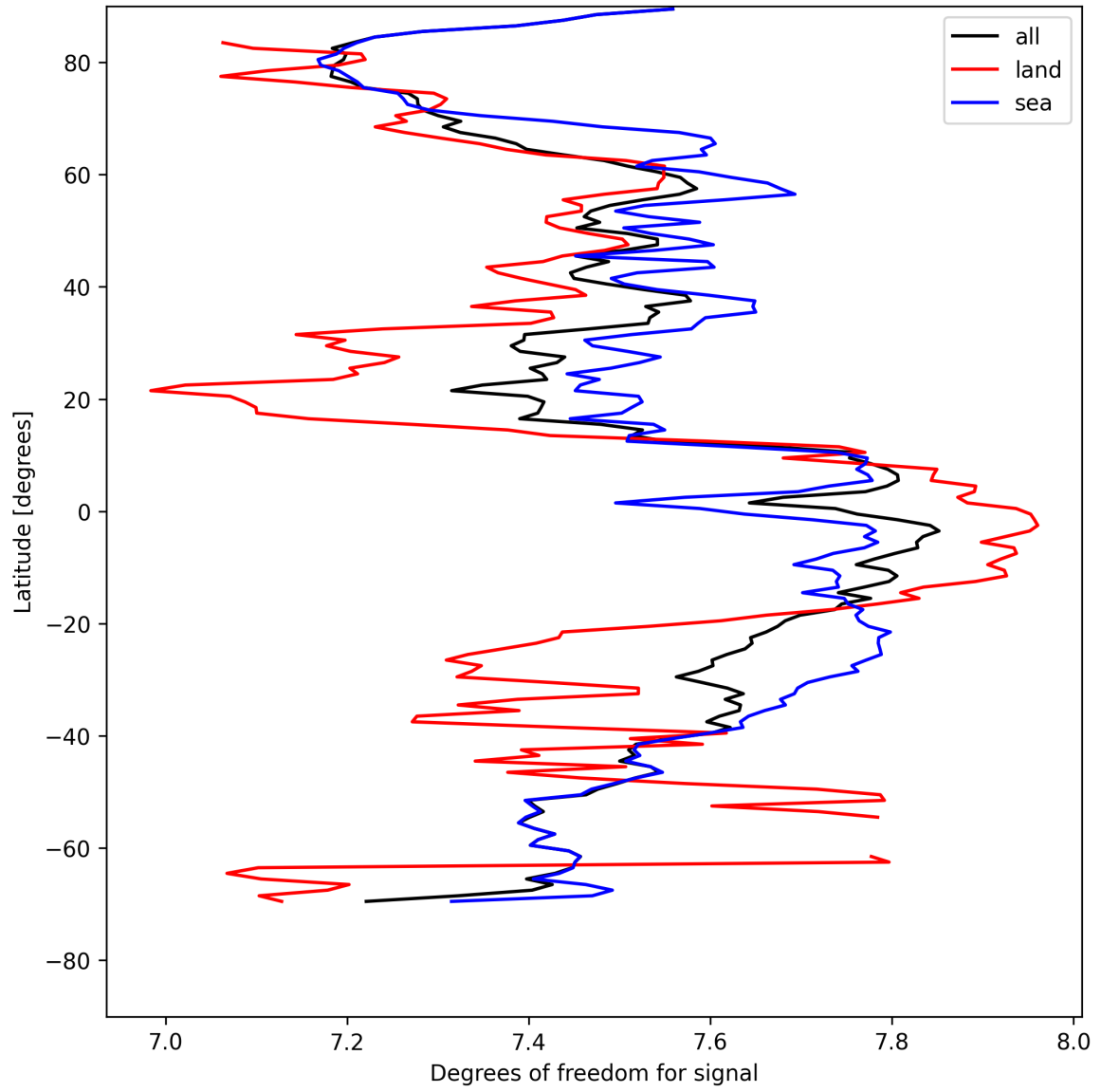
Figure 11: Zonal average of “Degrees of freedom for signal” for 2025-04-30 to 2025-05-01.
