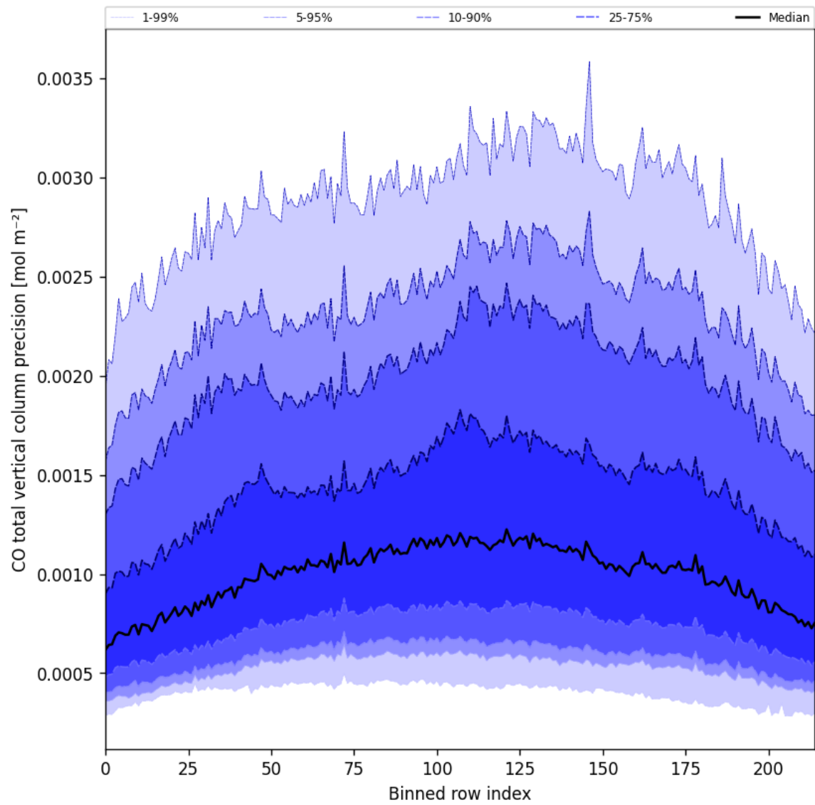
Figure 22: Along track statistics of “CO total vertical column precision” for 2025-04-30 to 2025-05-01
