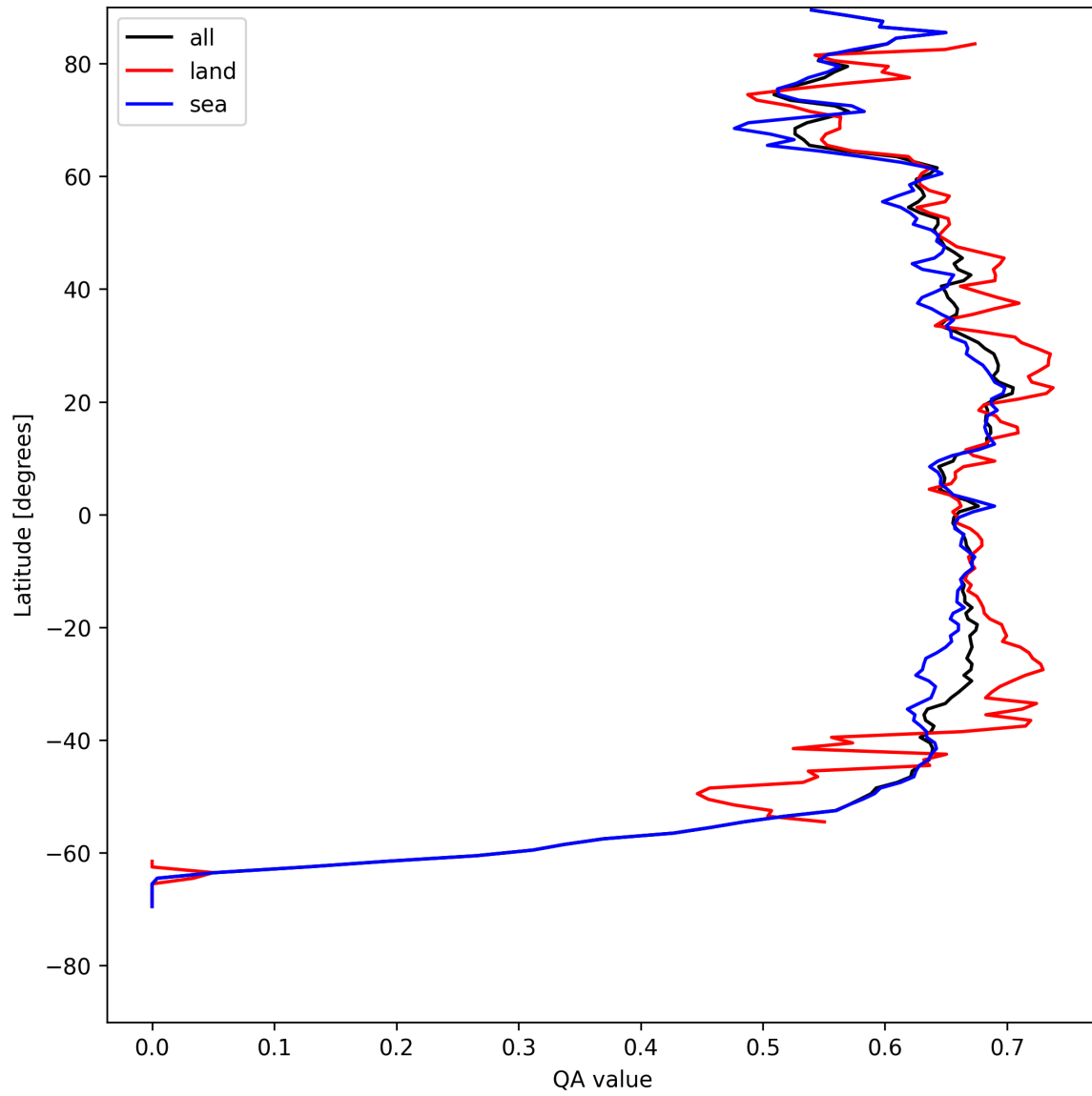
Figure 6: Zonal average of “QA value” for 2025-04-30 to 2025-05-01.
