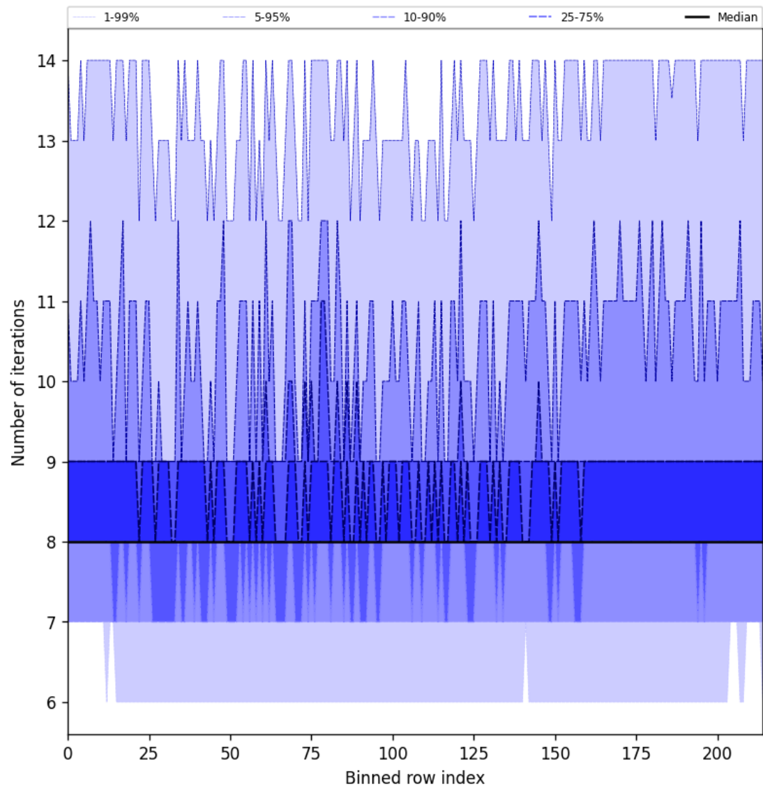
Figure 26: Along track statistics of “Number of iterations” for 2025-04-30 to 2025-05-01
