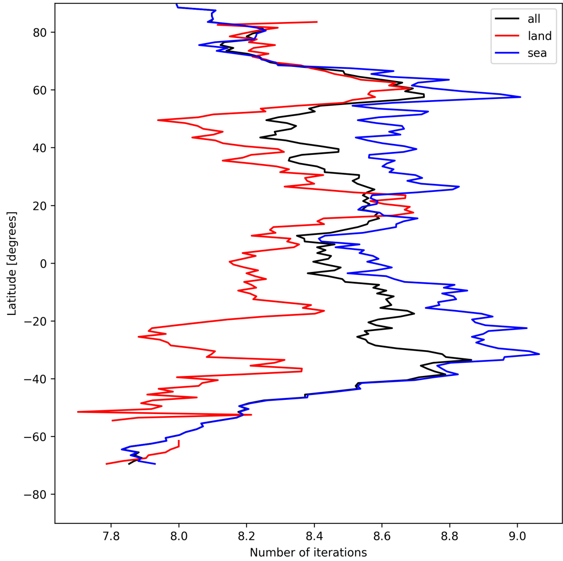
Figure 12: Zonal average of “Number of iterations” for 2025-04-30 to 2025-05-01.
