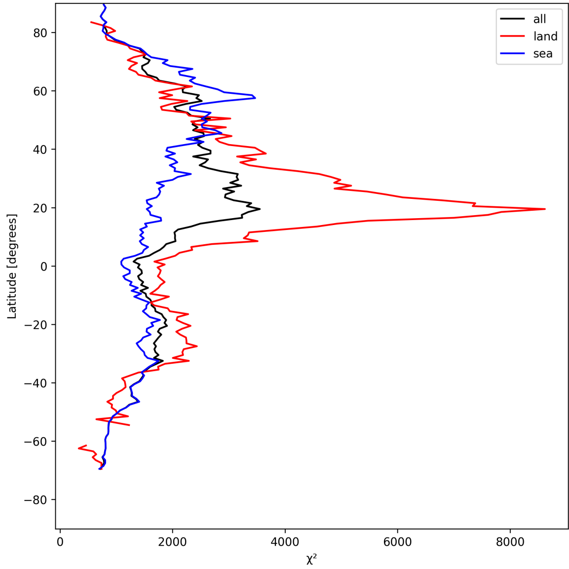
Figure 10: Zonal average of “ \chi^2 ” for 2025-04-30 to 2025-05-01.
