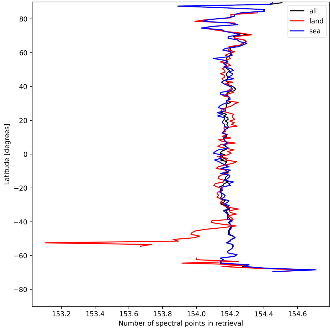
Figure 9: Zonal average of “Number of spectral points in retrieval” for 2025-04-30 to 2025-05-01.
