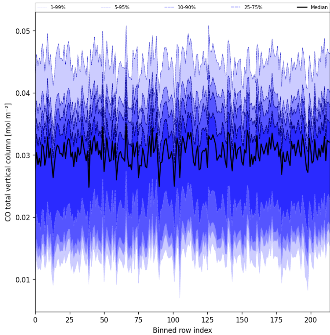
Figure 21: Along track statistics of “CO total vertical column” for 2025-04-30 to 2025-05-01
