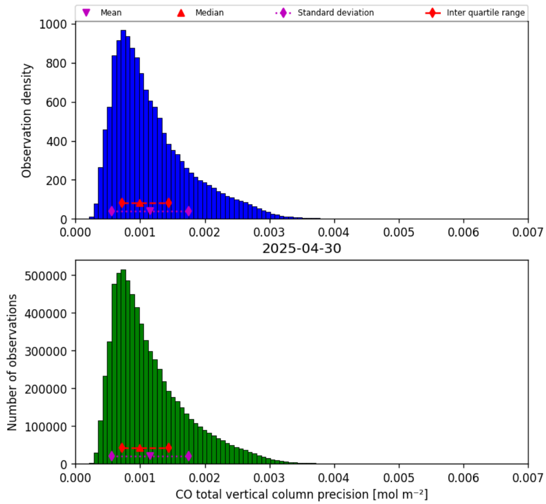
Figure 15: Histogram of “CO total vertical column precision” for 2025-04-30 to 2025-05-01
