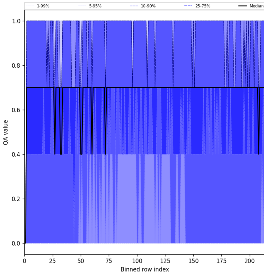
Figure 20: Along track statistics of “QA value” for 2025-04-30 to 2025-05-01
