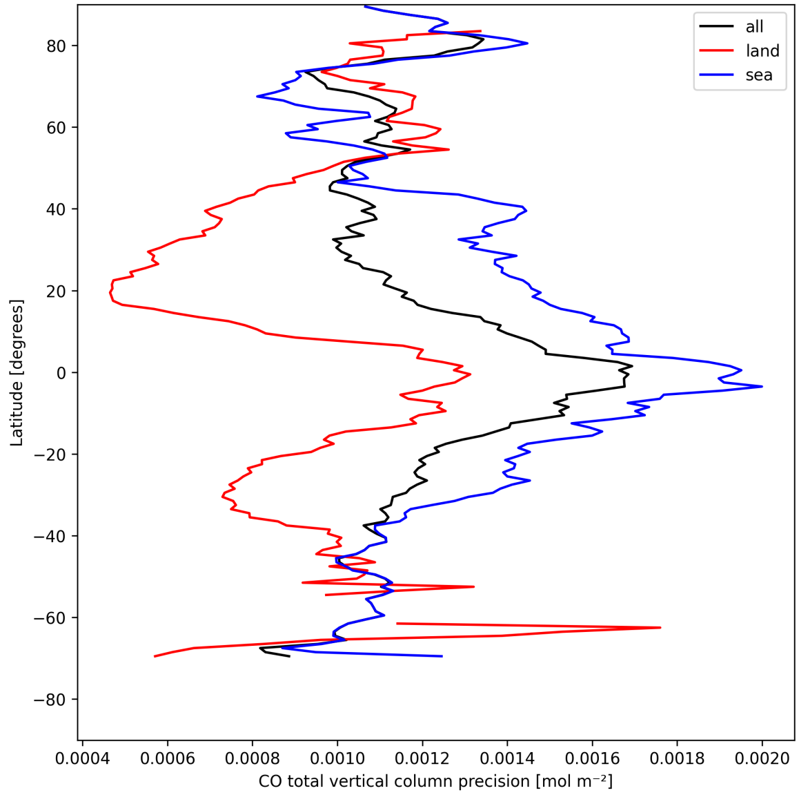
Figure 8: Zonal average of "CO total vertical column precision" for 2025-04-30 to 2025-05-01.
