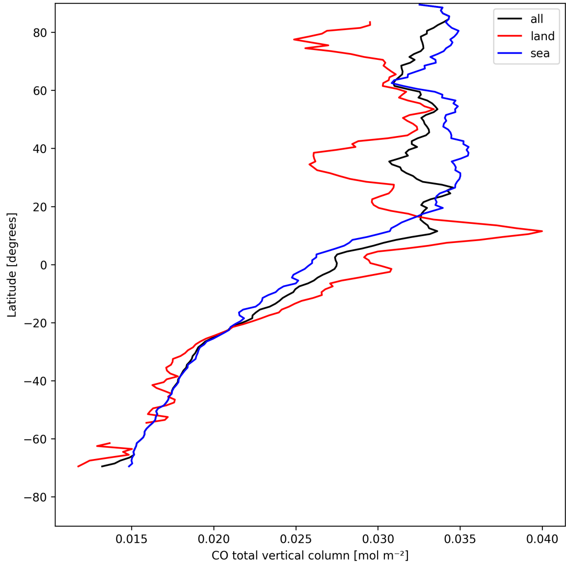
Figure 7: Zonal average of “CO total vertical column” for 2025-04-30 to 2025-05-01.
