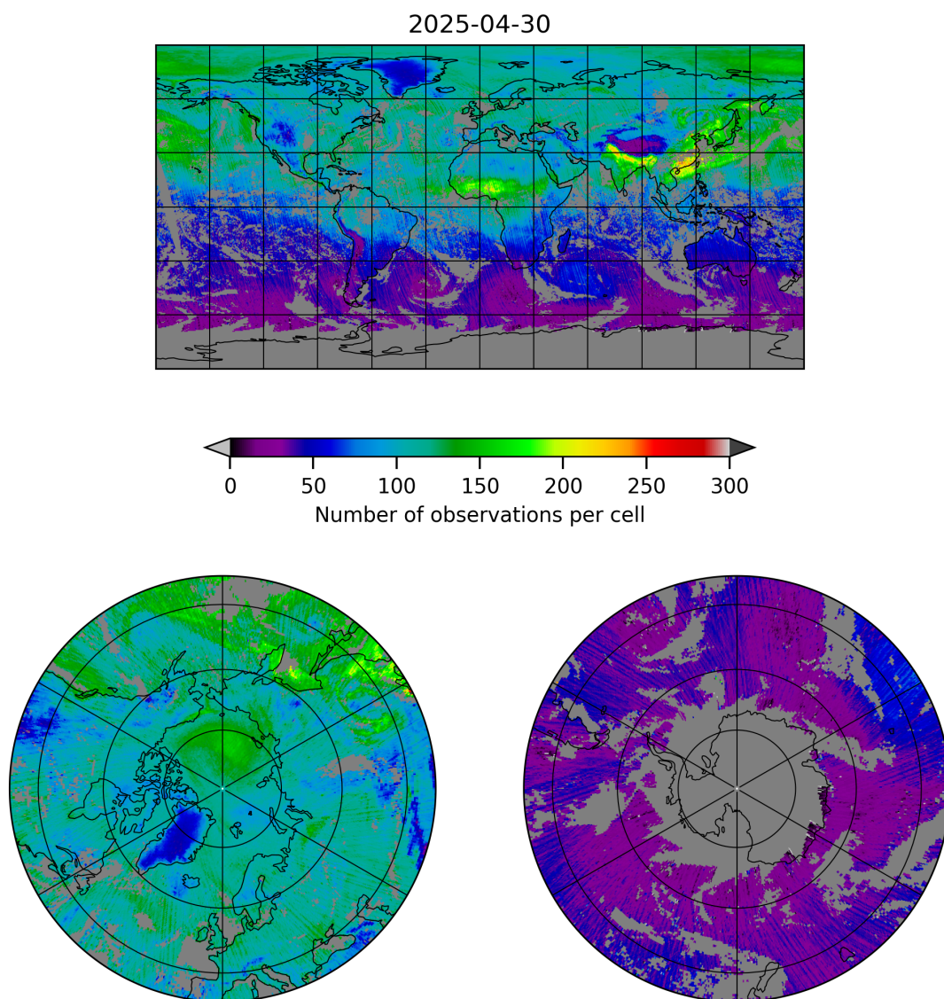
Figure 5: Map of the number of observations for 2025-04-30 to 2025-05-01
