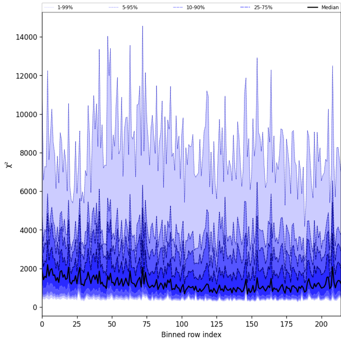
Figure 24: Along track statistics of “ \chi^2 ” for 2025-04-30 to 2025-05-01
