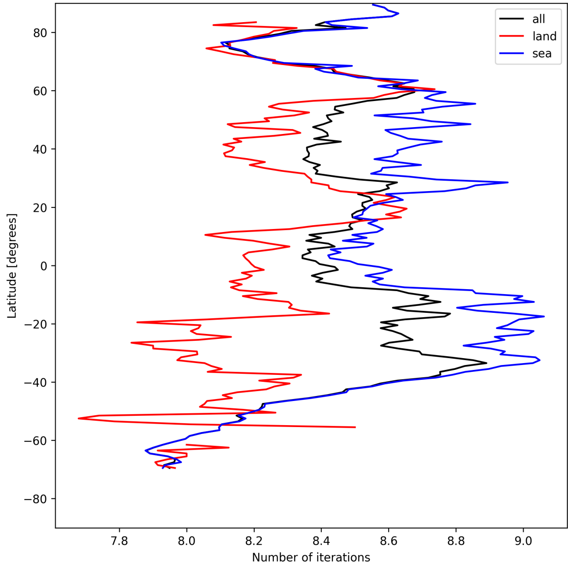
Figure 12: Zonal average of “Number of iterations” for 2025-05-01 to 2025-05-02.
