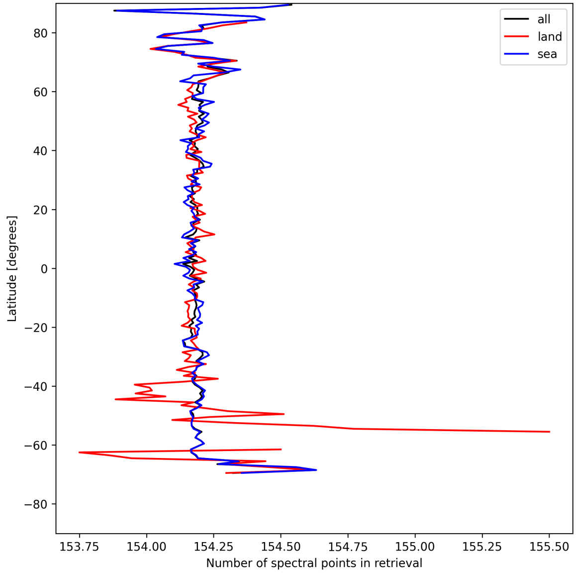
Figure 9: Zonal average of “Number of spectral points in retrieval” for 2025-05-01 to 2025-05-02.
