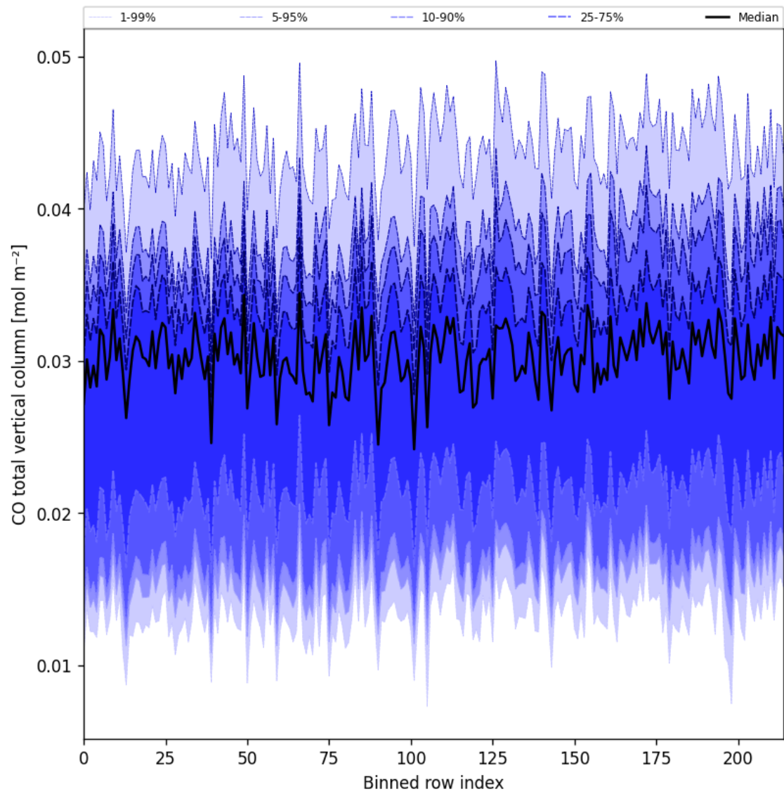
Figure 21: Along track statistics of “CO total vertical column” for 2025-05-01 to 2025-05-02
