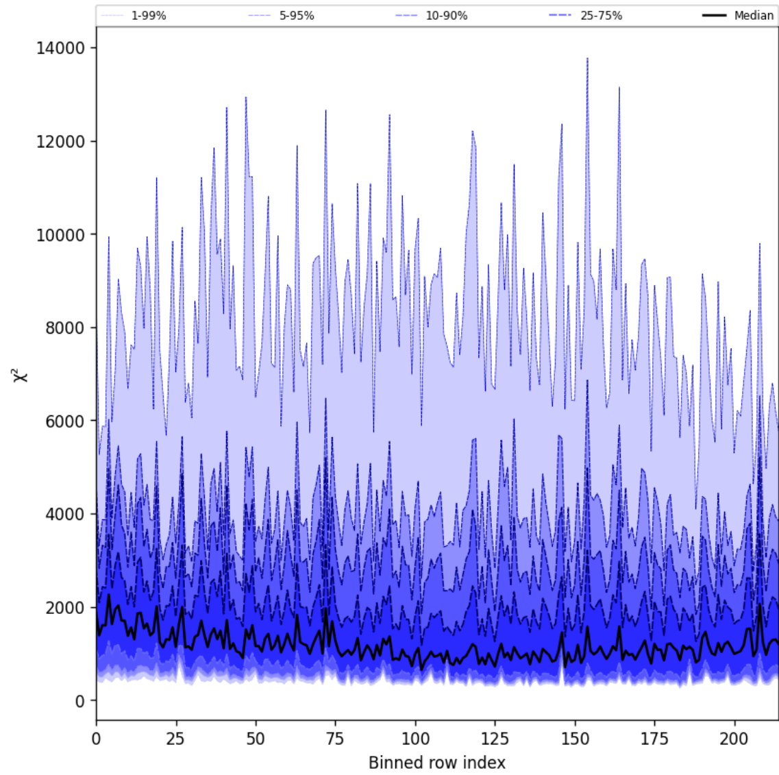
Figure 24: Along track statistics of “ \chi^2 ” for 2025-05-01 to 2025-05-02
