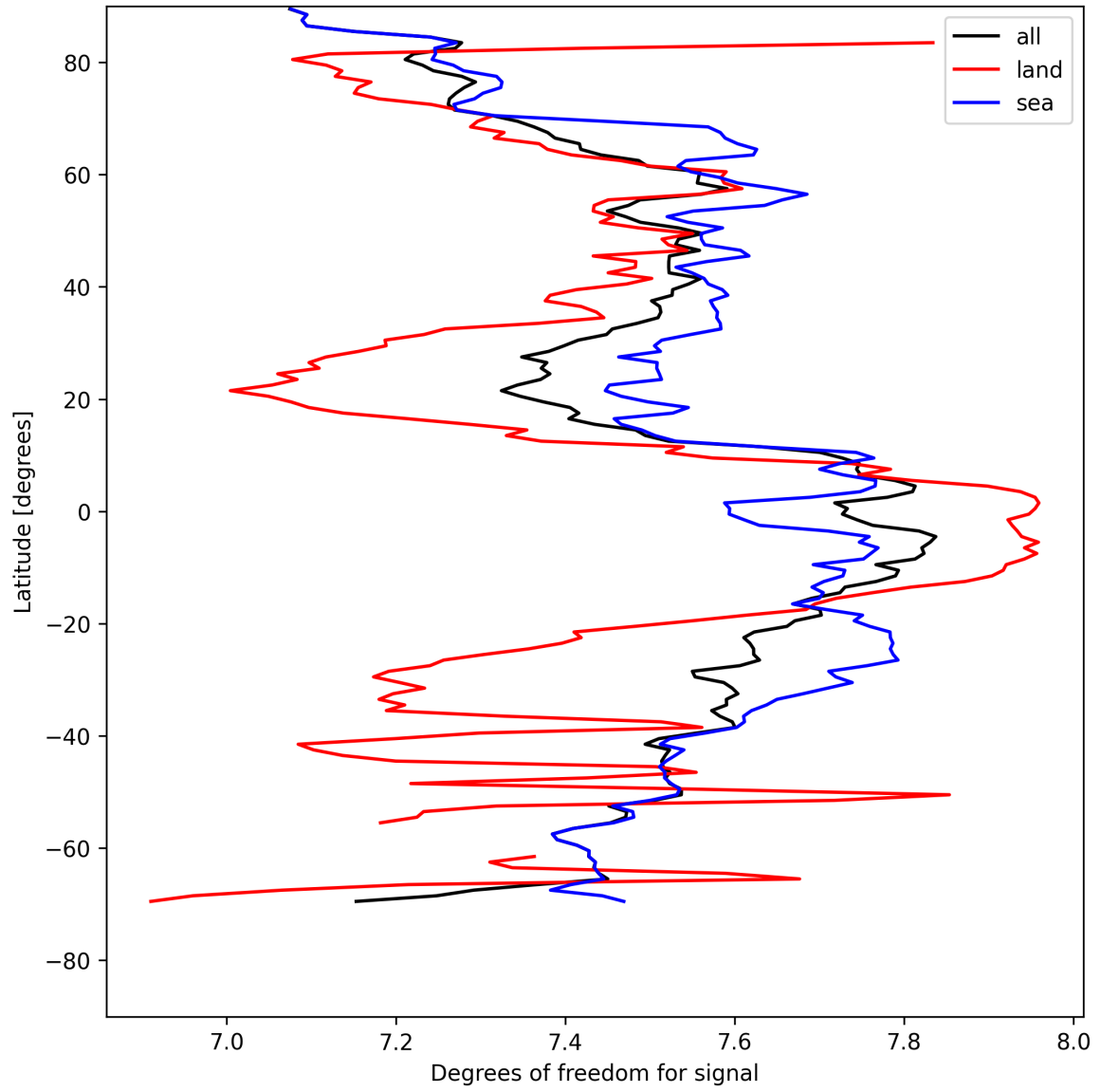
Figure 11: Zonal average of “Degrees of freedom for signal” for 2025-05-01 to 2025-05-02.
