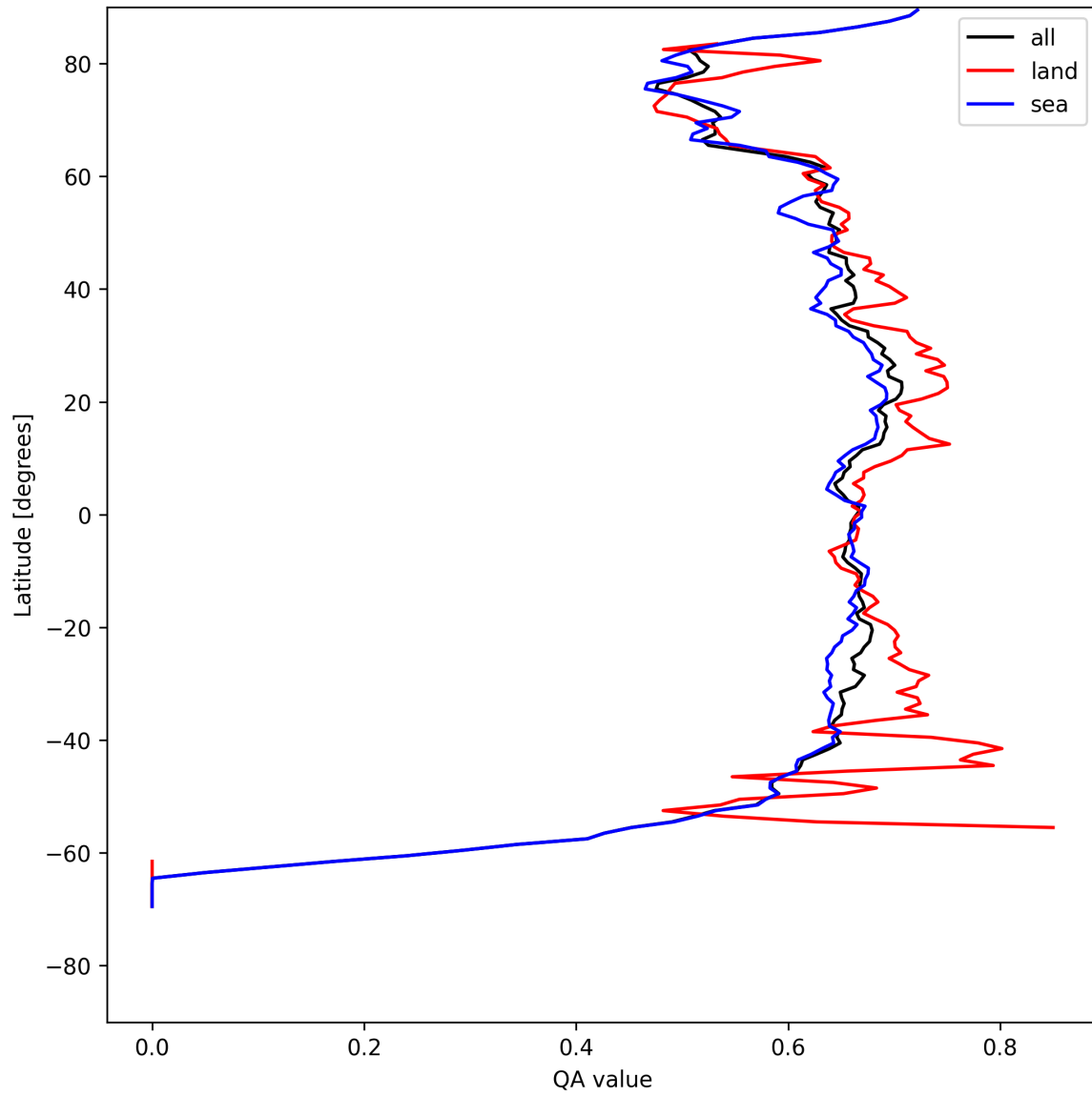
Figure 6: Zonal average of “QA value” for 2025-05-01 to 2025-05-02.
