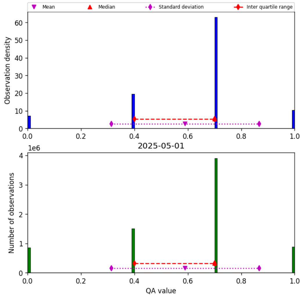
Figure 13: Histogram of “QA value” for 2025-05-01 to 2025-05-02
