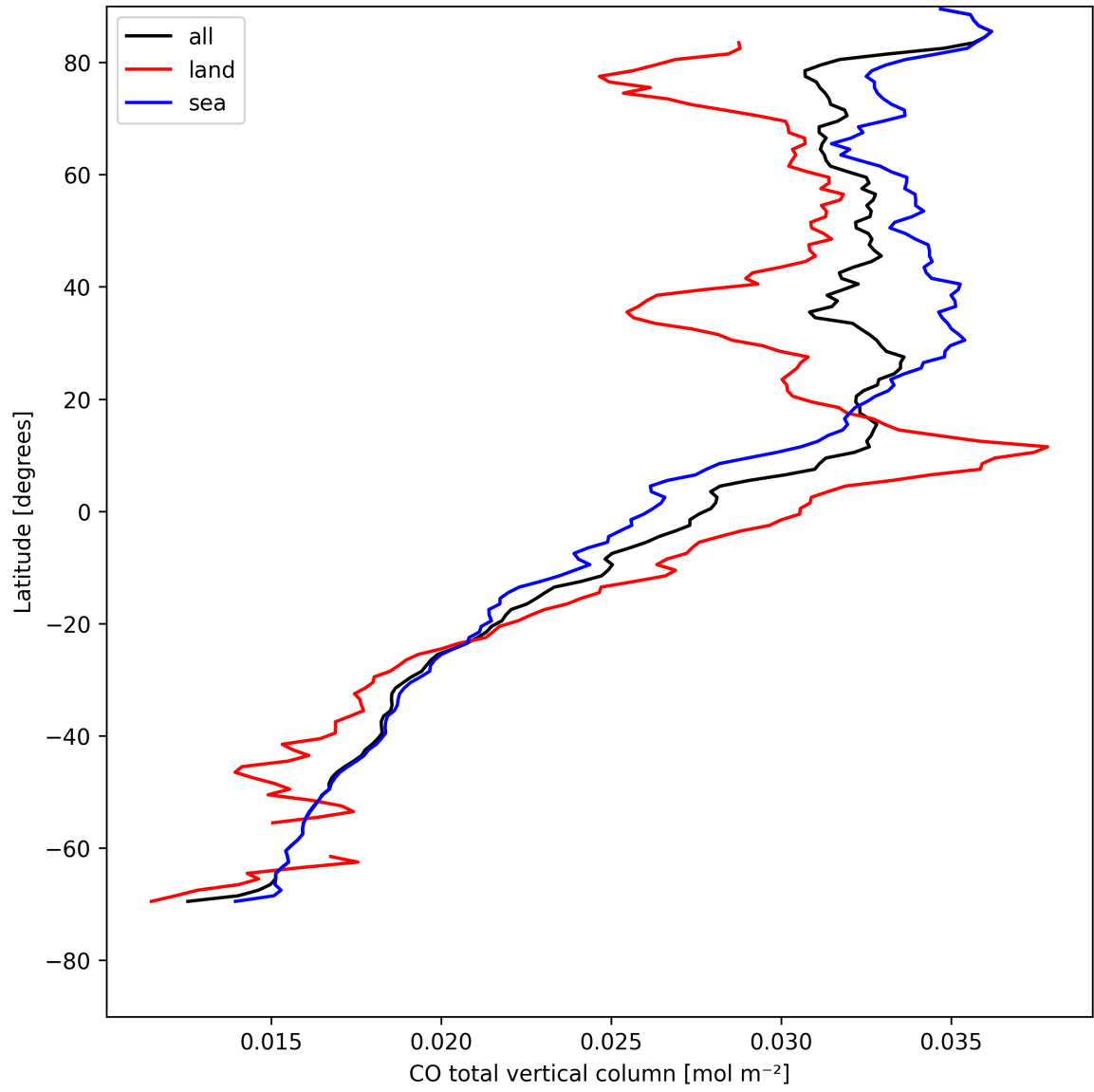
Figure 7: Zonal average of “CO total vertical column” for 2025-05-01 to 2025-05-02.
