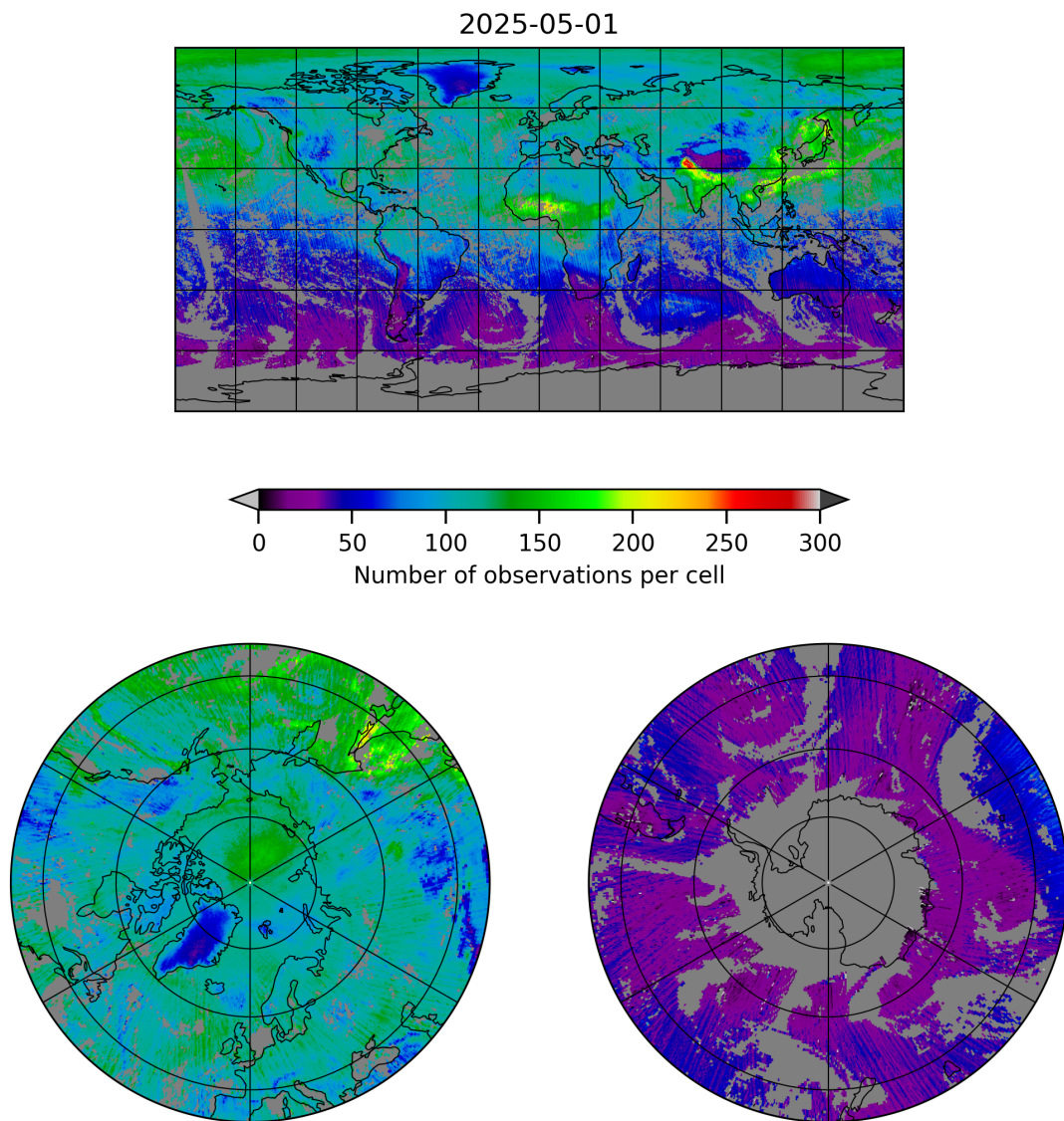
Figure 5: Map of the number of observations for 2025-05-01 to 2025-05-02
