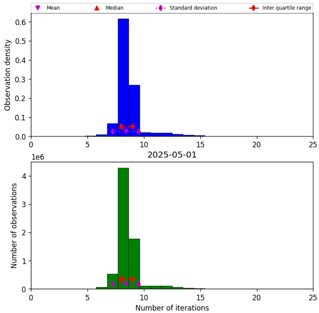
Figure 19: Histogram of “Number of iterations” for 2025-05-01 to 2025-05-02
