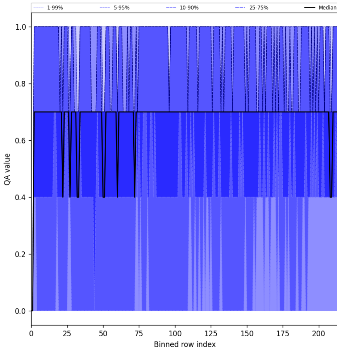
Figure 20: Along track statistics of “QA value” for 2025-05-01 to 2025-05-02
