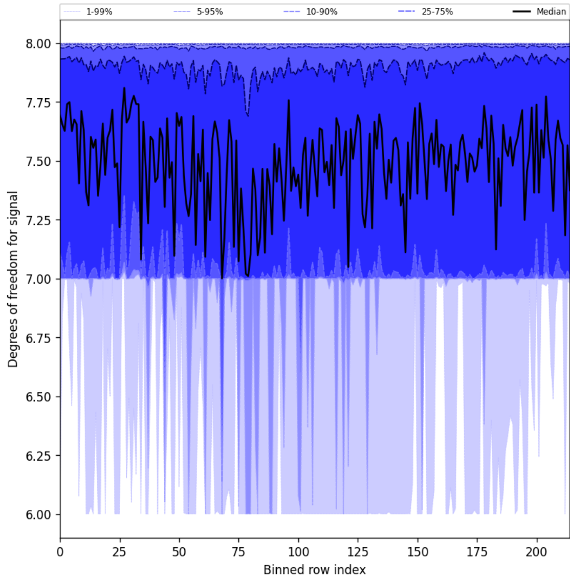
Figure 25: Along track statistics of “Degrees of freedom for signal” for 2025-05-01 to 2025-05-02
