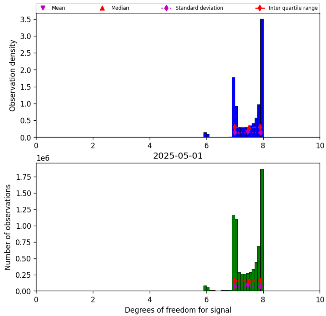
Figure 18: Histogram of “Degrees of freedom for signal” for 2025-05-01 to 2025-05-02
