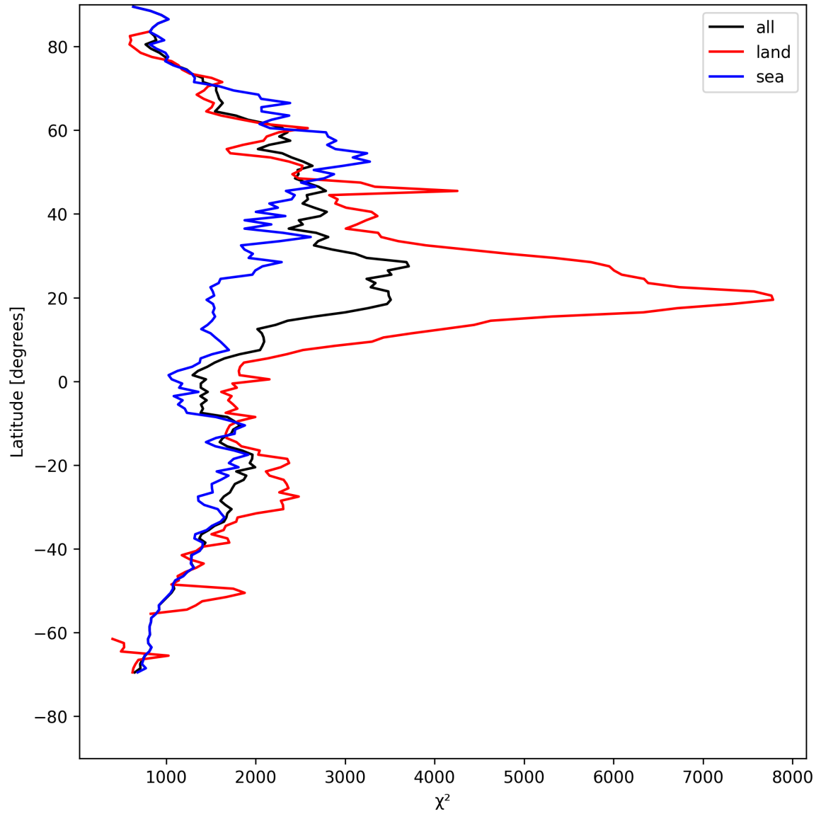
Figure 10: Zonal average of “ \chi^2 ” for 2025-05-01 to 2025-05-02.
