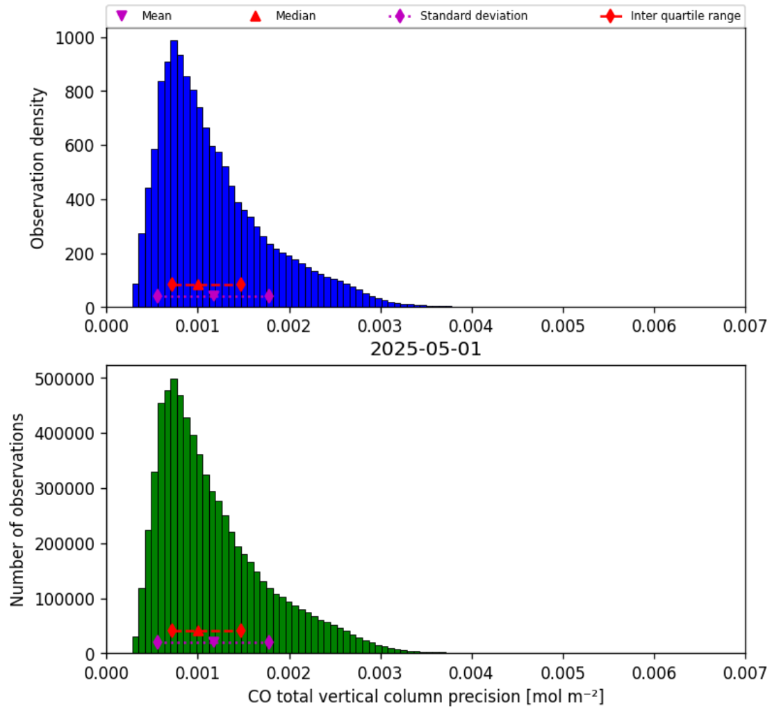
Figure 15: Histogram of “CO total vertical column precision” for 2025-05-01 to 2025-05-02
