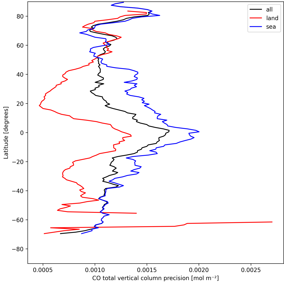
Figure 8: Zonal average of “CO total vertical column precision” for 2025-05-01 to 2025-05-02.
