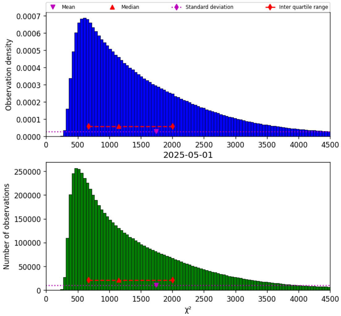
Figure 17: Histogram of “ \chi^2 ” for 2025-05-01 to 2025-05-02
