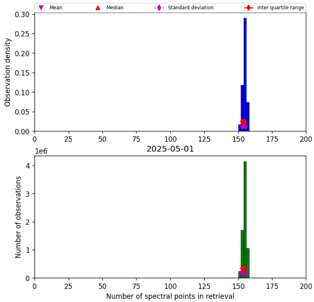
Figure 16: Histogram of “Number of spectral points in retrieval” for 2025-05-01 to 2025-05-02
