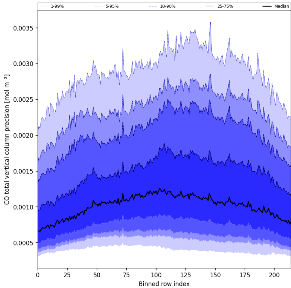
Figure 22: Along track statistics of “CO total vertical column precision” for 2025-05-01 to 2025-05-02
