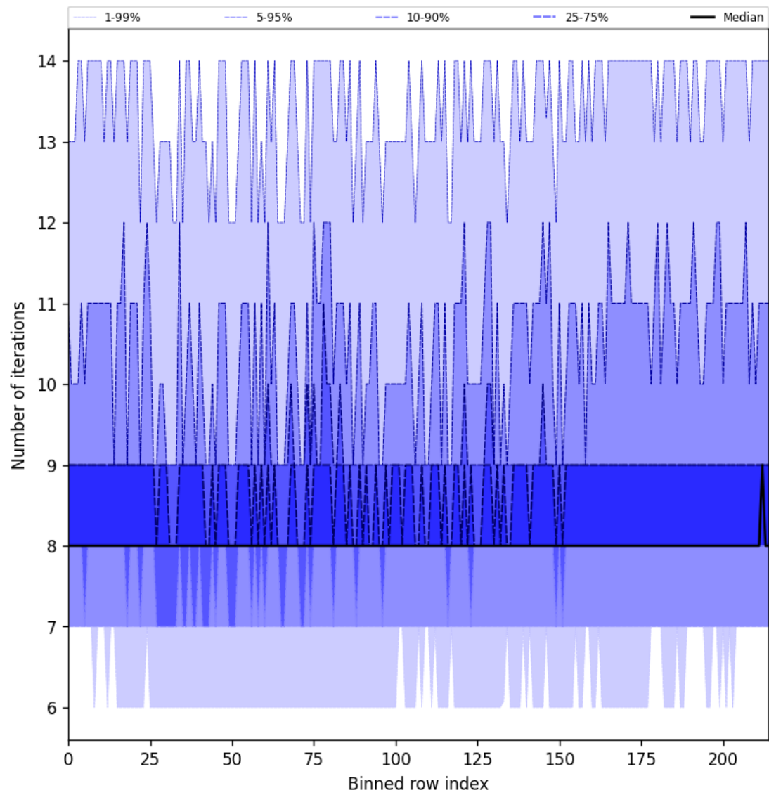
Figure 26: Along track statistics of “Number of iterations” for 2025-05-01 to 2025-05-02
