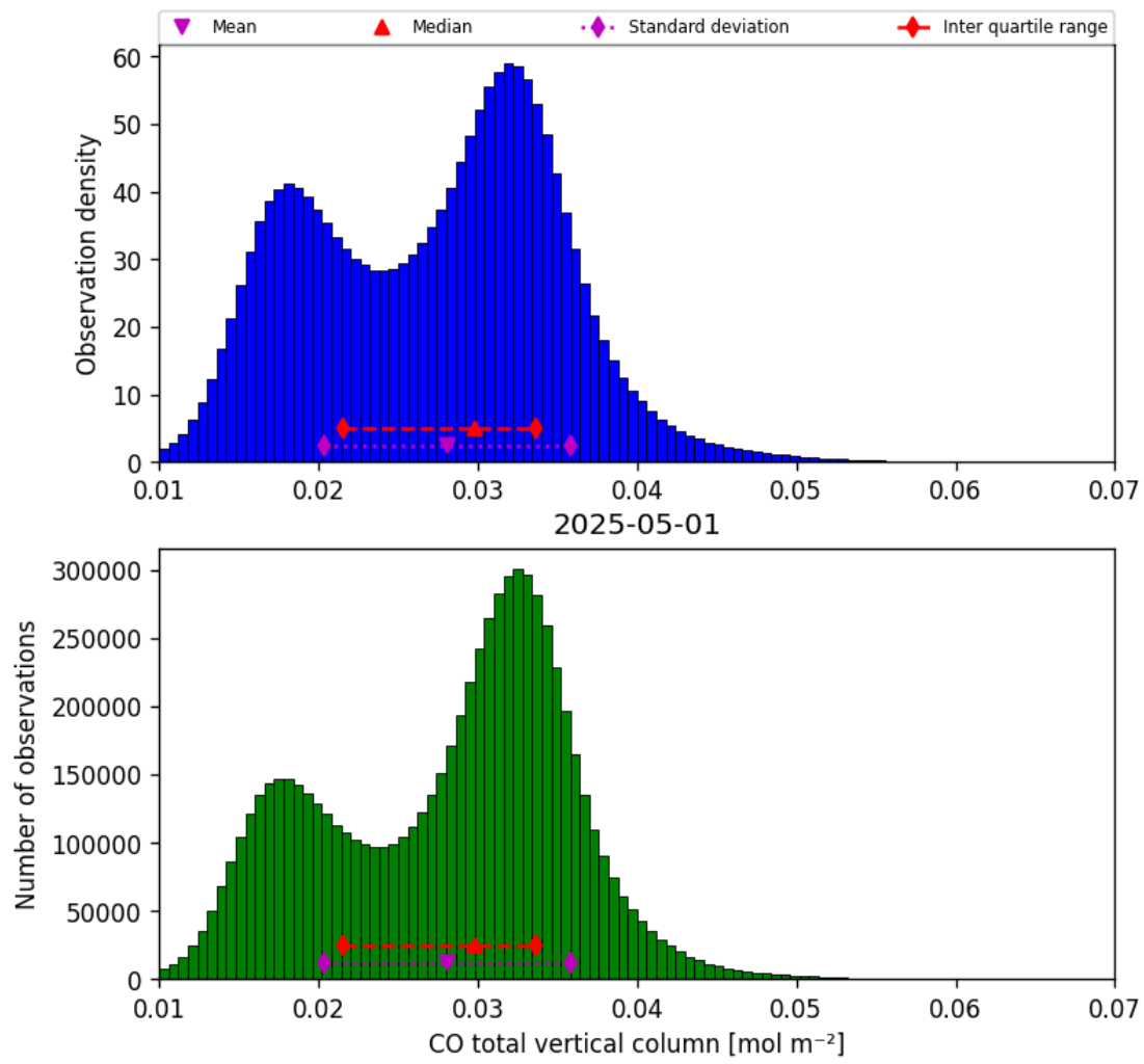
Figure 14: Histogram of “CO total vertical column” for 2025-05-01 to 2025-05-02
