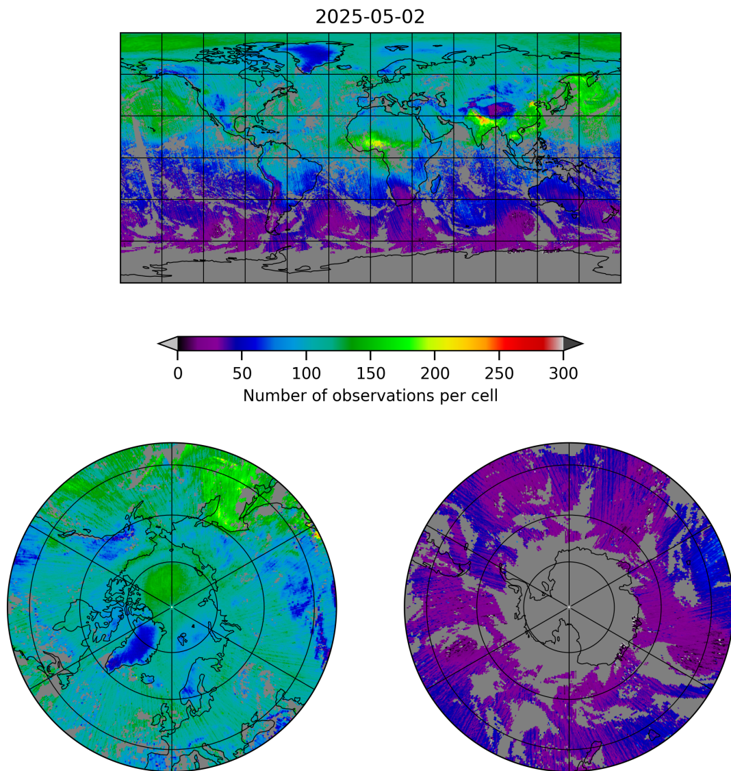
Figure 5: Map of the number of observations for 2025-05-02 to 2025-05-02
