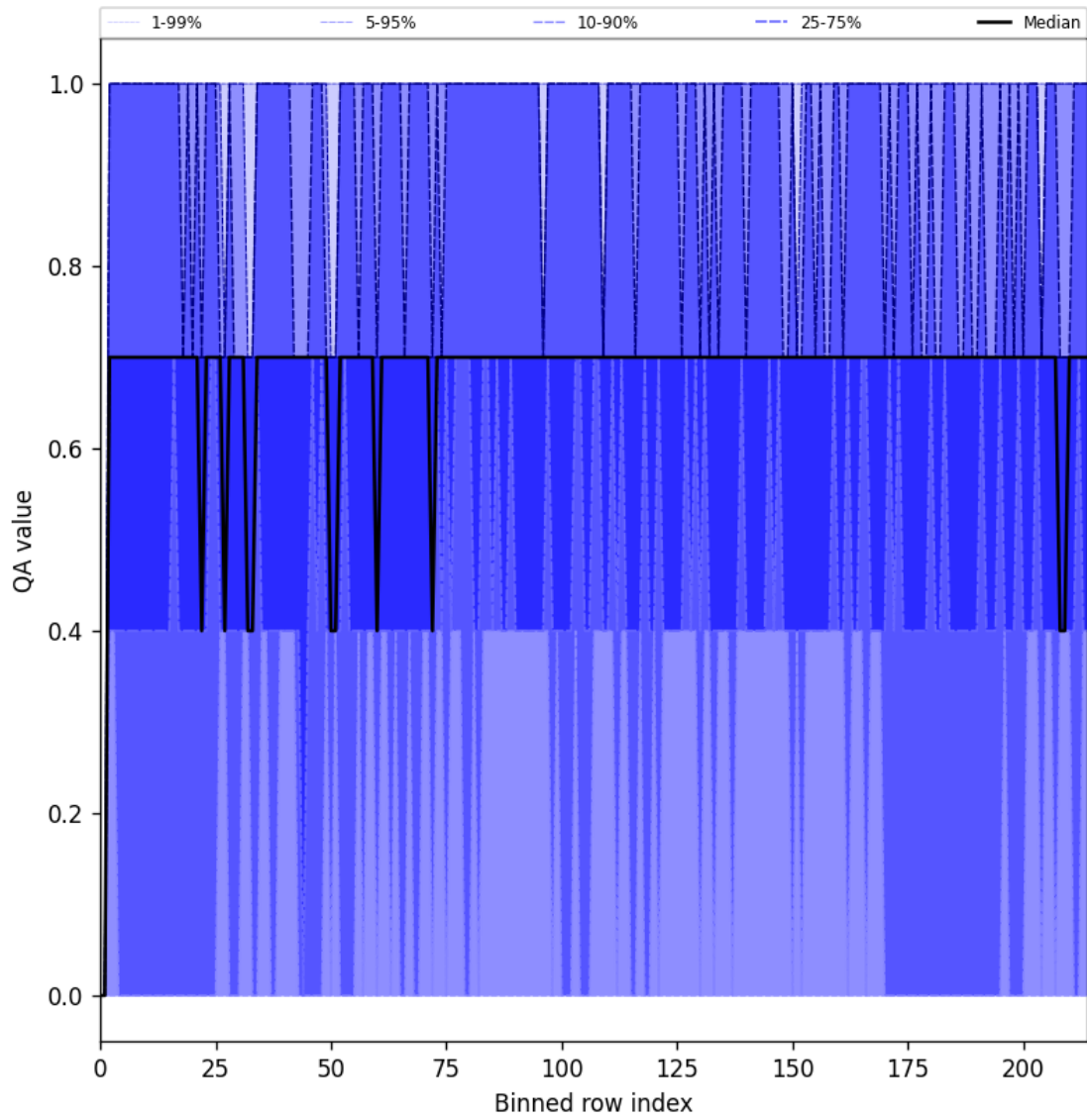
Figure 20: Along track statistics of “QA value” for 2025-05-02 to 2025-05-02
