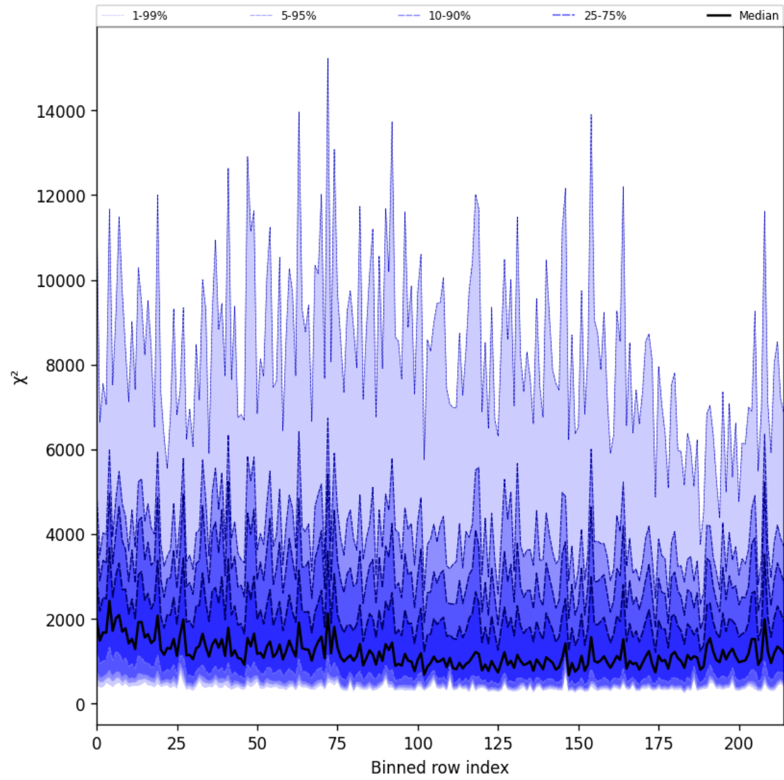
Figure 24: Along track statistics of “ \chi^2 ” for 2025-05-02 to 2025-05-02
