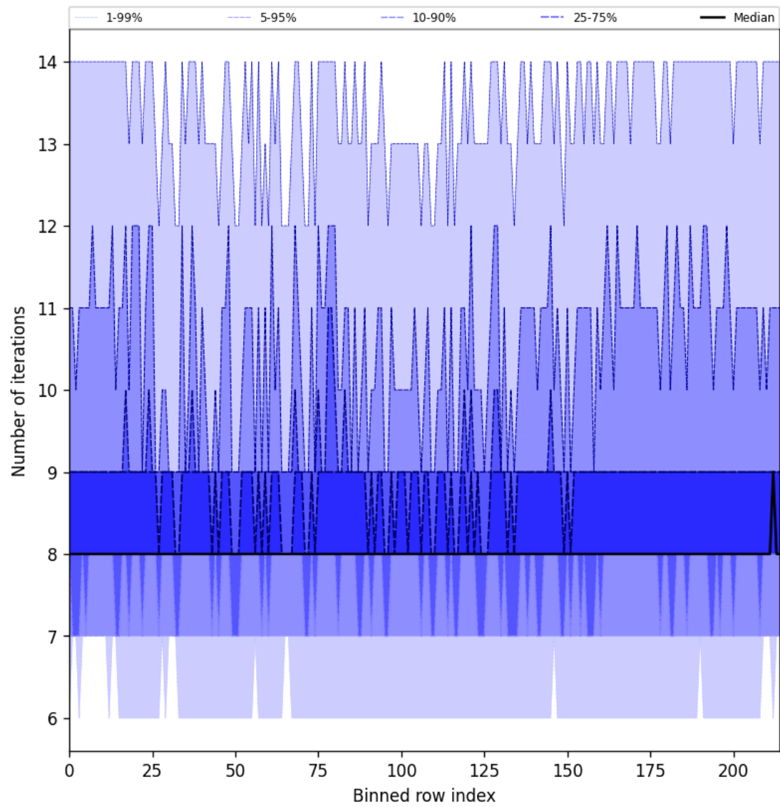
Figure 26: Along track statistics of “Number of iterations” for 2025-05-02 to 2025-05-02
