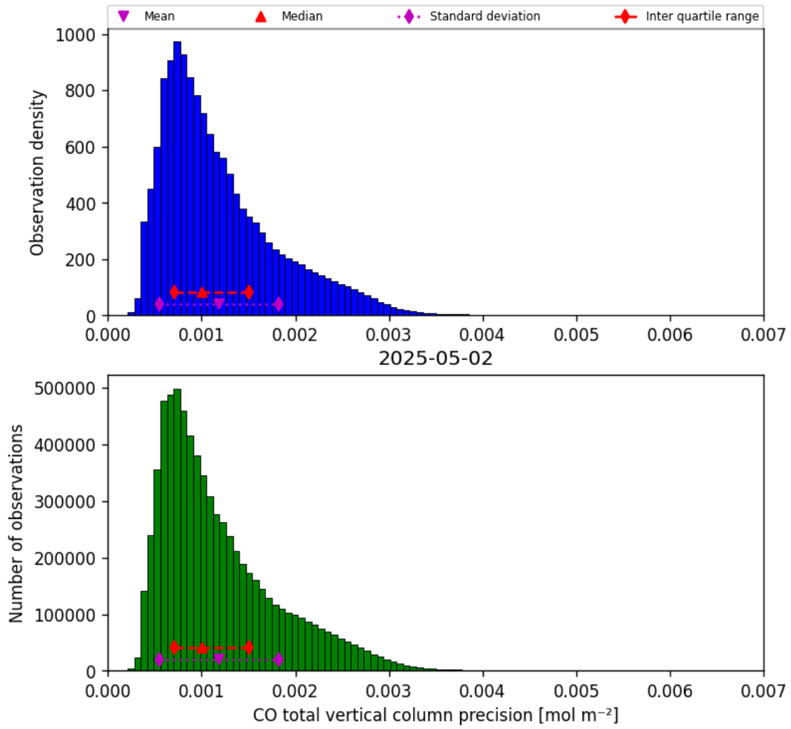
Figure 15: Histogram of “CO total vertical column precision” for 2025-05-02 to 2025-05-02
