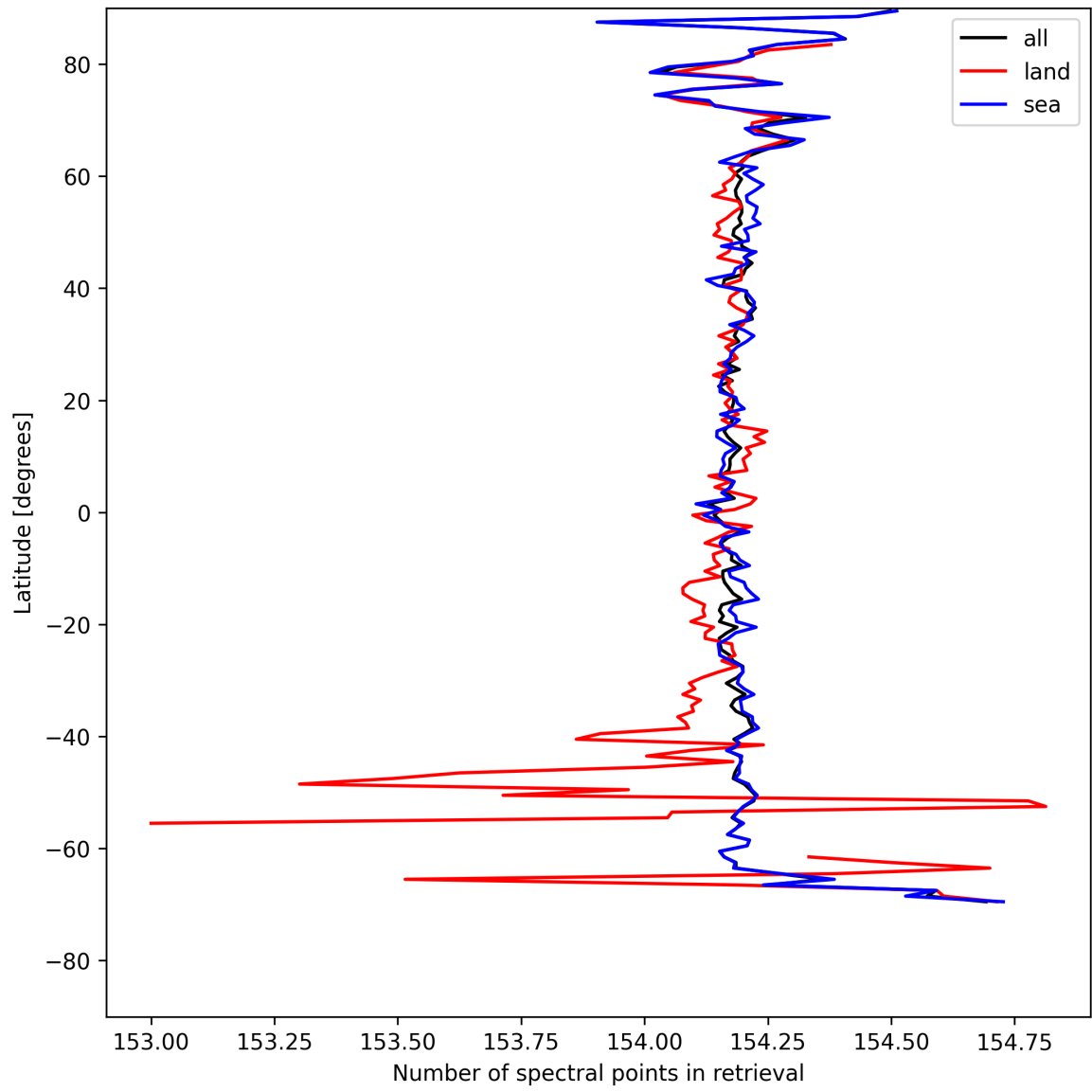
Figure 9: Zonal average of “Number of spectral points in retrieval” for 2025-05-02 to 2025-05-02.
