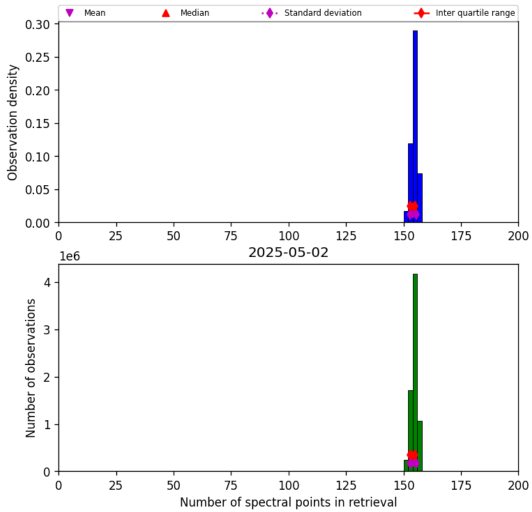
Figure 16: Histogram of “Number of spectral points in retrieval” for 2025-05-02 to 2025-05-02
