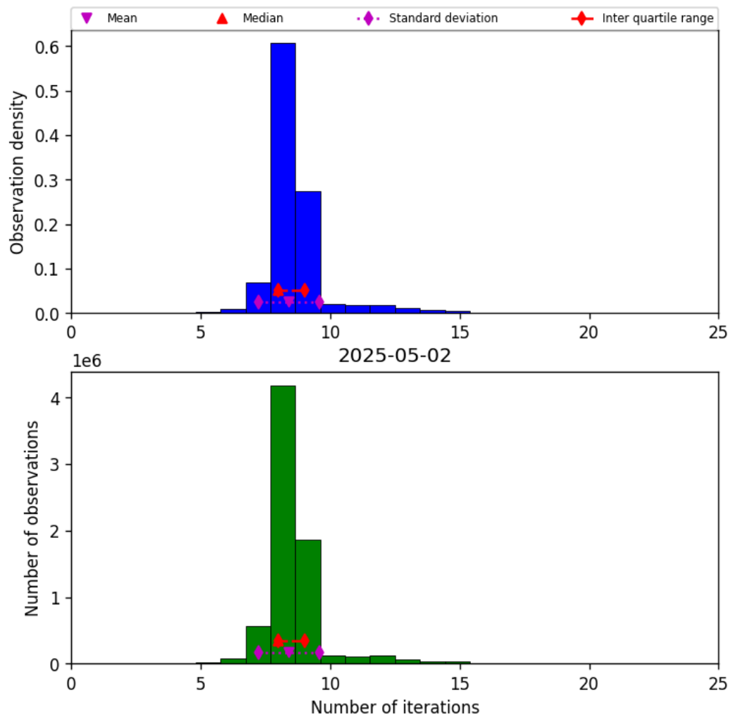
Figure 19: Histogram of “Number of iterations” for 2025-05-02 to 2025-05-02
