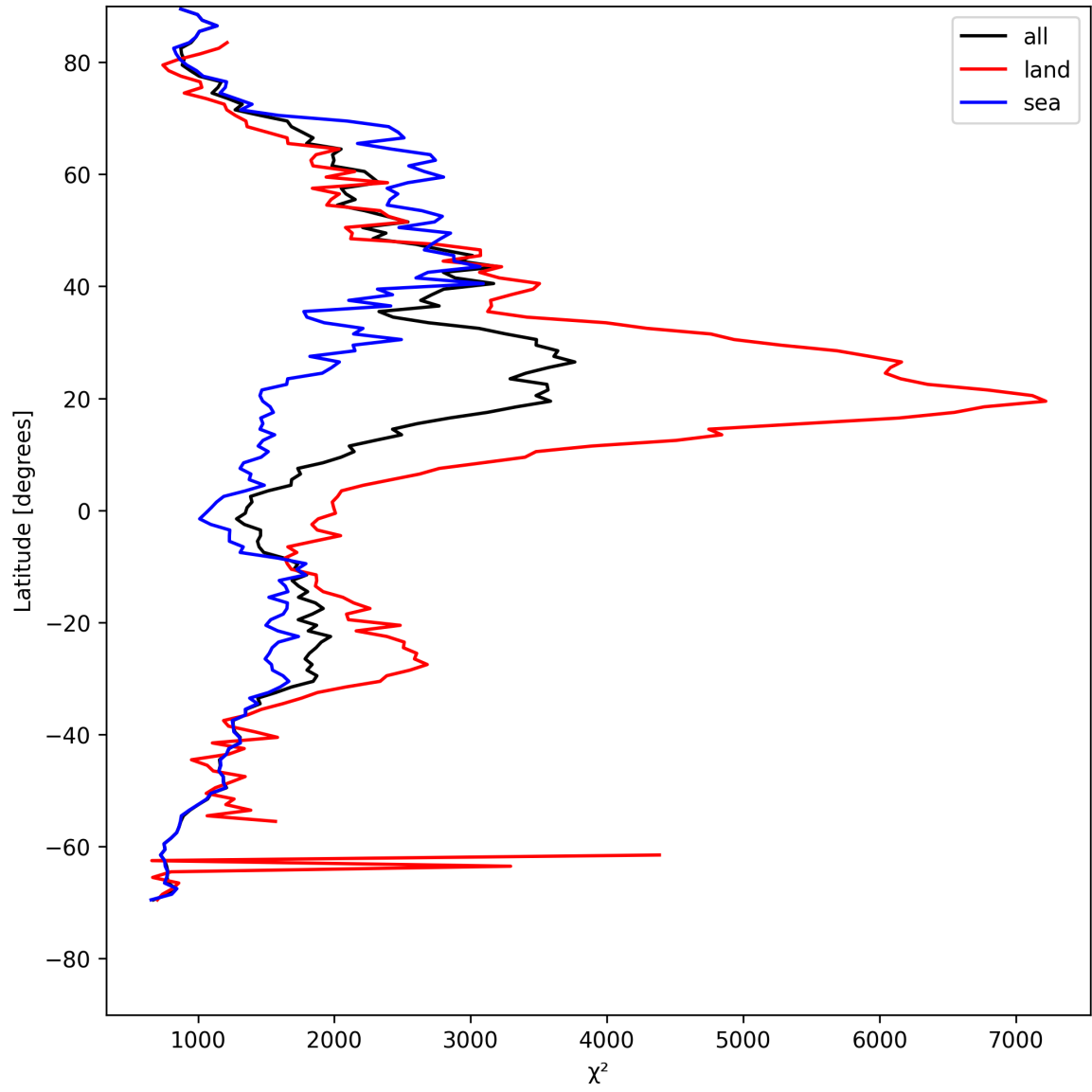
Figure 10: Zonal average of “ \chi^2 ” for 2025-05-02 to 2025-05-02.
