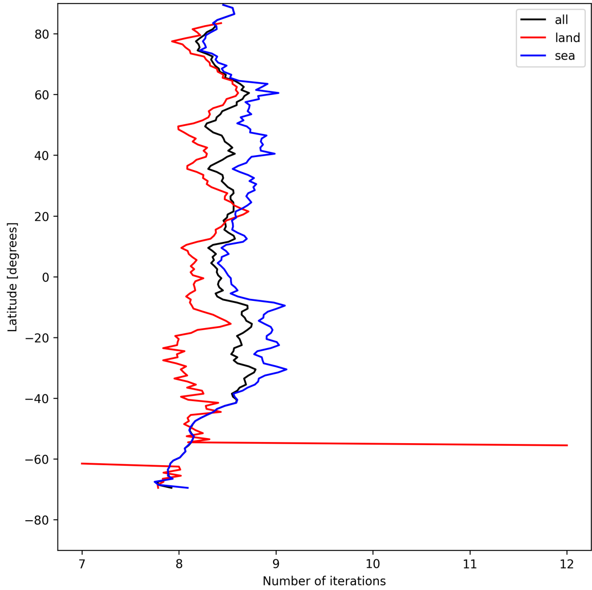
Figure 12: Zonal average of “Number of iterations” for 2025-05-02 to 2025-05-02.
