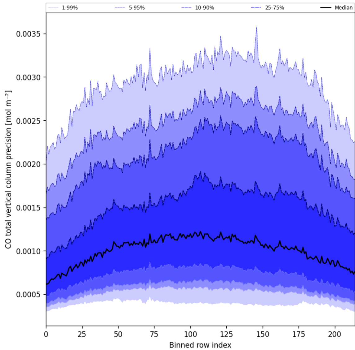
Figure 22: Along track statistics of “CO total vertical column precision” for 2025-05-02 to 2025-05-02
