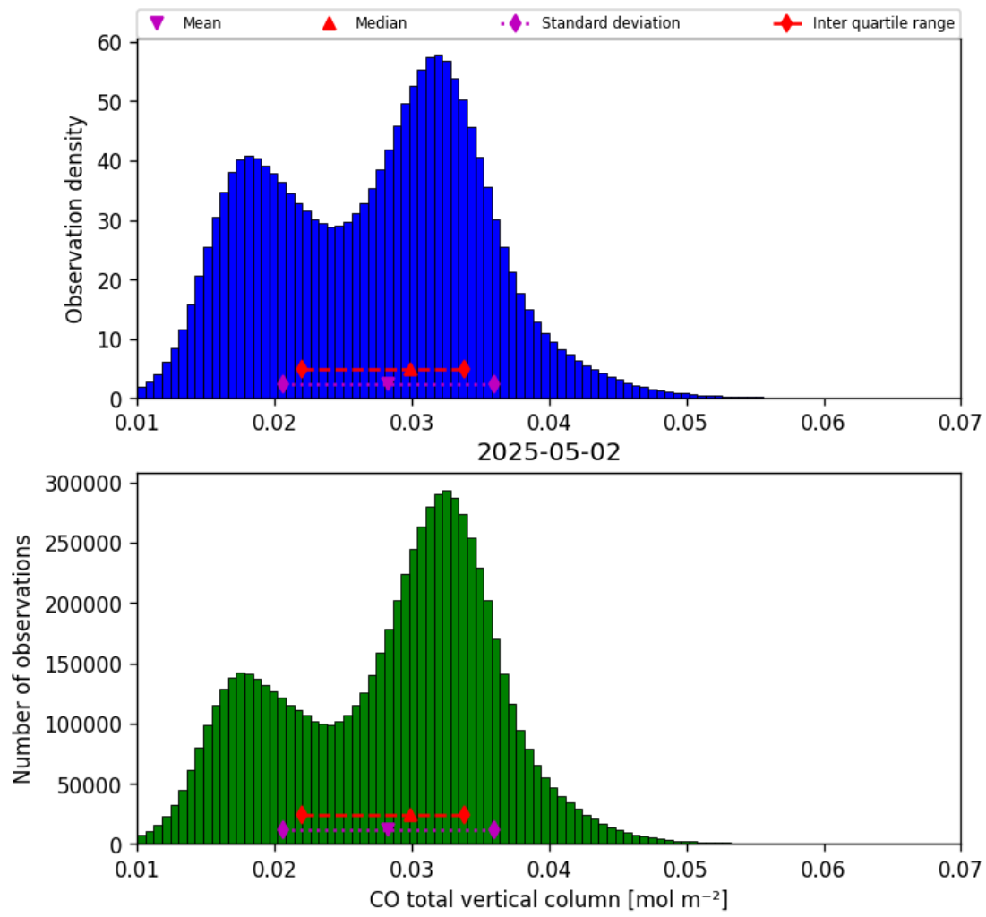
Figure 14: Histogram of “CO total vertical column” for 2025-05-02 to 2025-05-02
