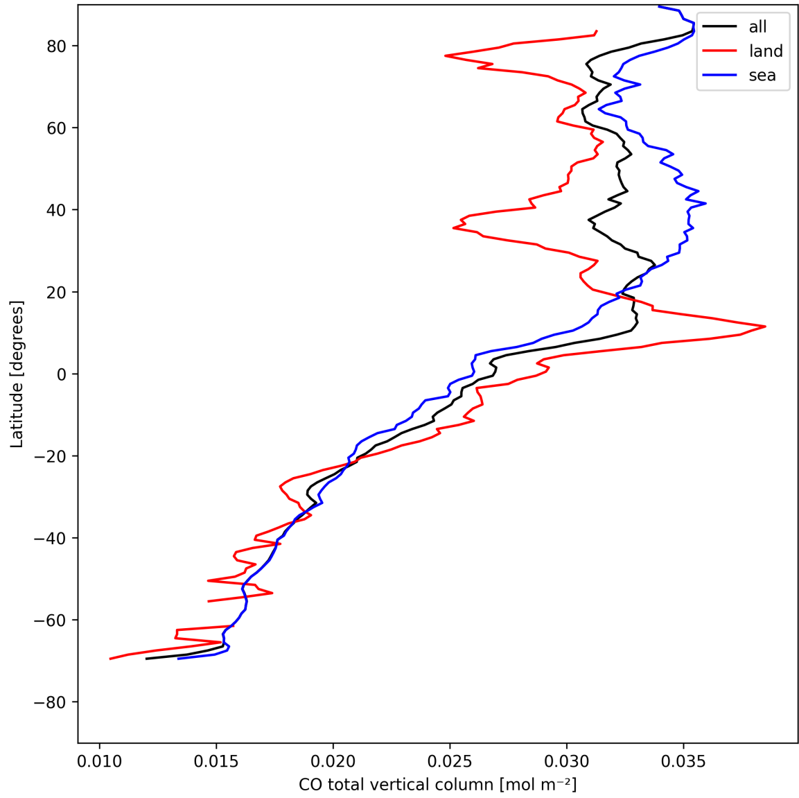
Figure 7: Zonal average of “CO total vertical column” for 2025-05-02 to 2025-05-02.
