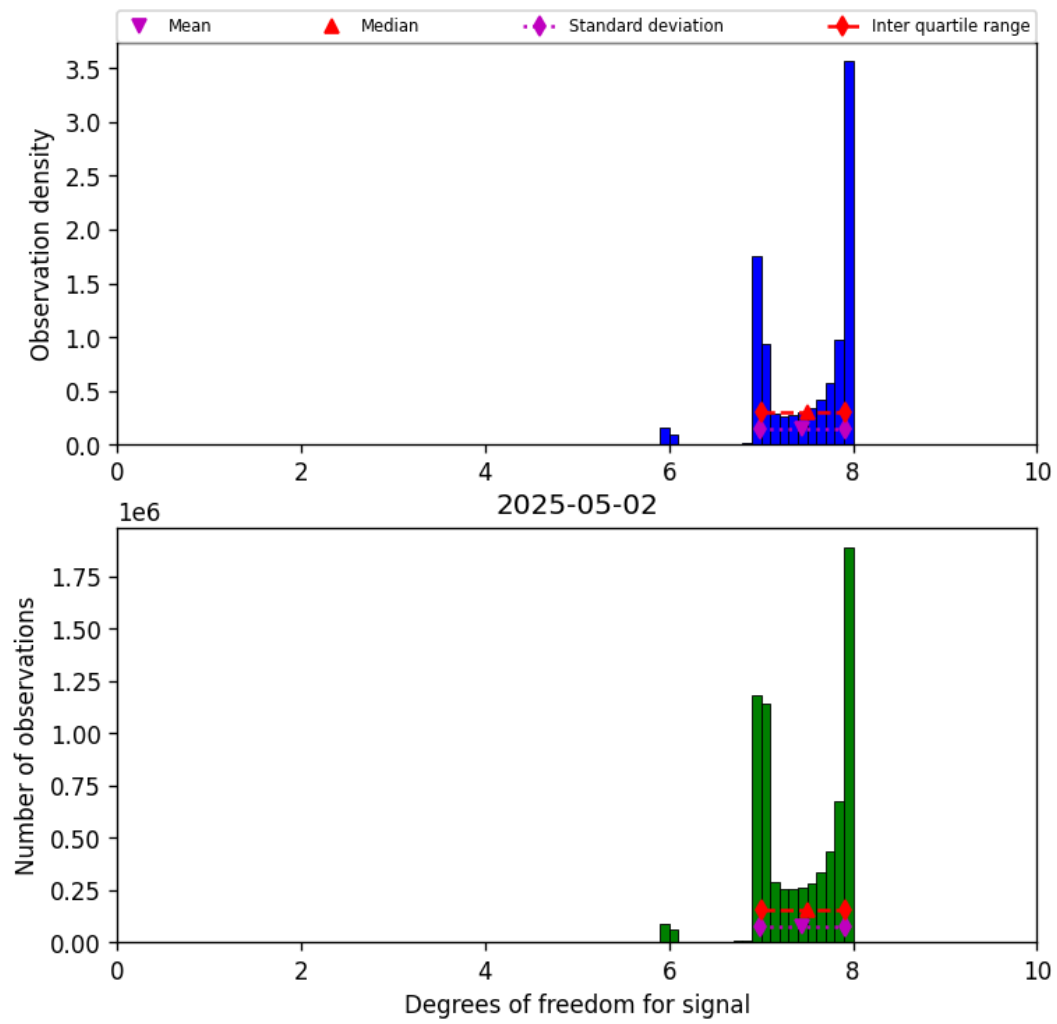
Figure 18: Histogram of “Degrees of freedom for signal” for 2025-05-02 to 2025-05-02
