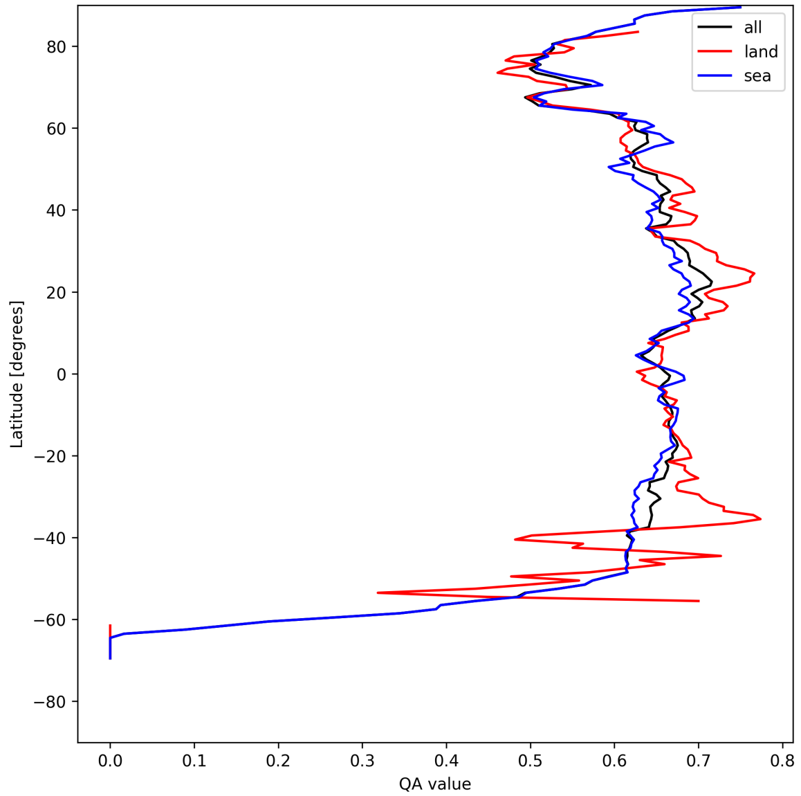
Figure 6: Zonal average of “QA value” for 2025-05-02 to 2025-05-02.
