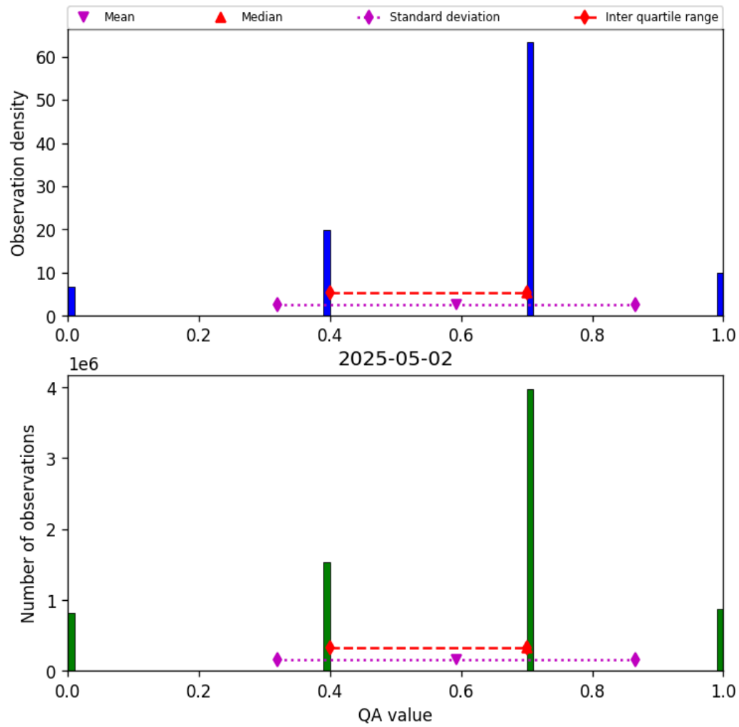
Figure 13: Histogram of "QA value" for 2025-05-02 to 2025-05-02
