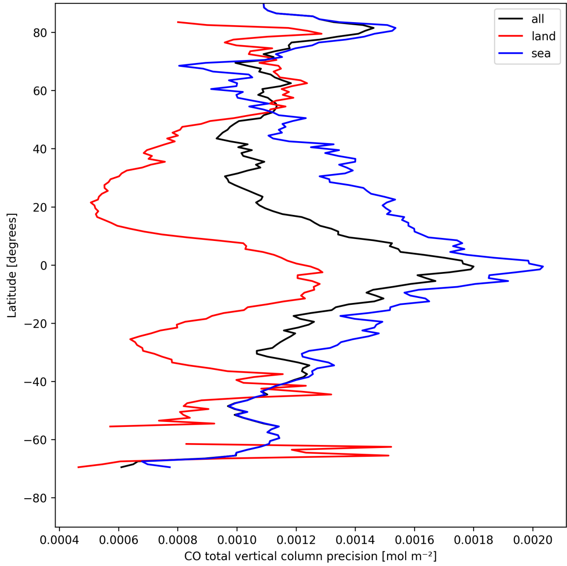
Figure 8: Zonal average of “CO total vertical column precision” for 2025-05-02 to 2025-05-02.
