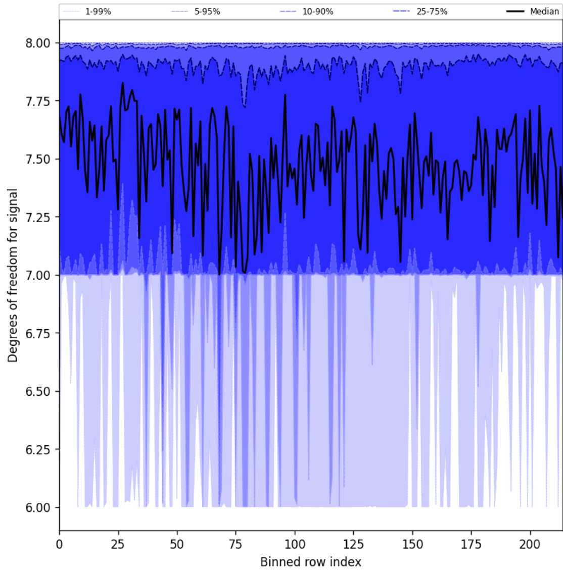
Figure 25: Along track statistics of “Degrees of freedom for signal” for 2025-05-02 to 2025-05-02
