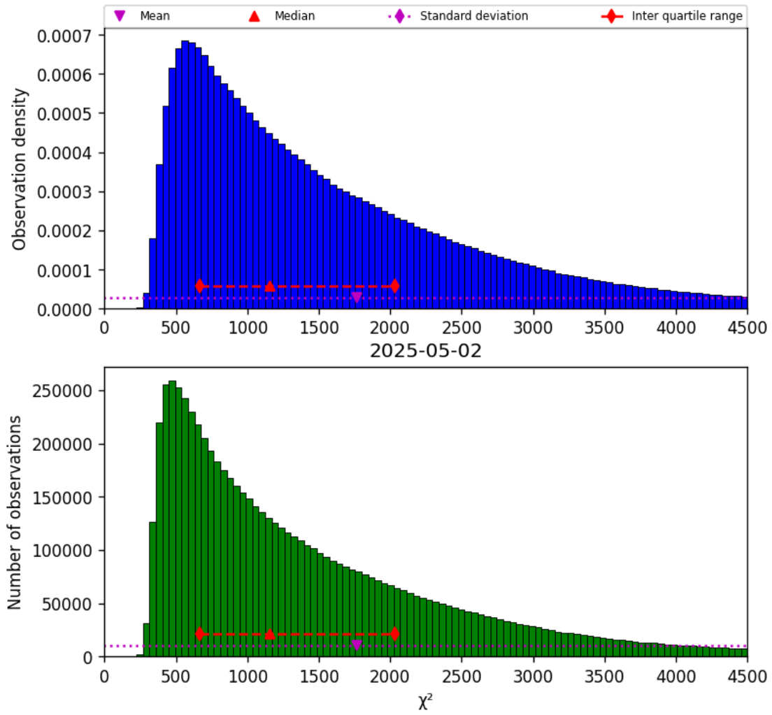
Figure 17: Histogram of " \chi^2 " for 2025-05-02 to 2025-05-02
