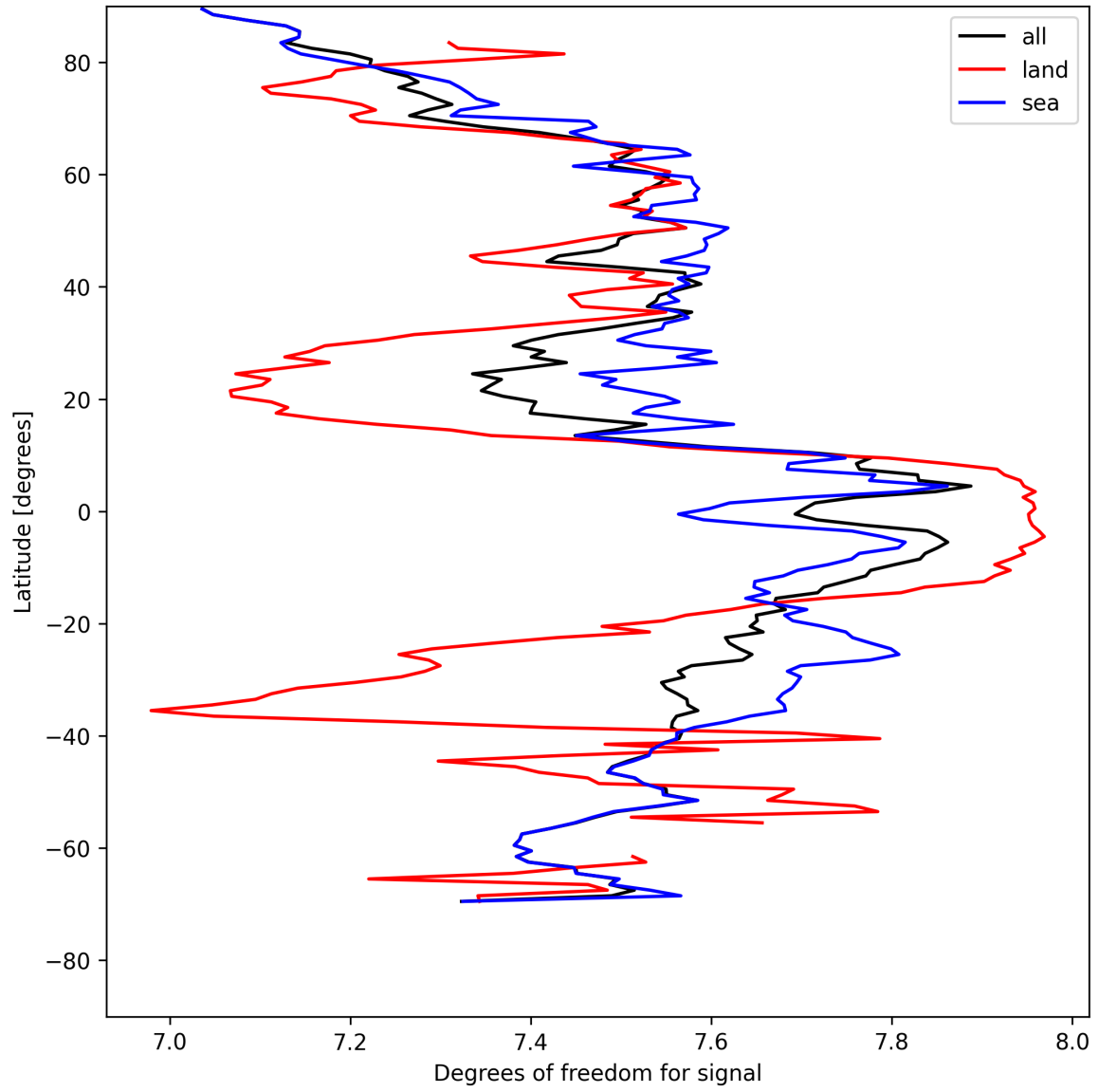
Figure 11: Zonal average of “Degrees of freedom for signal” for 2025-05-02 to 2025-05-02.
