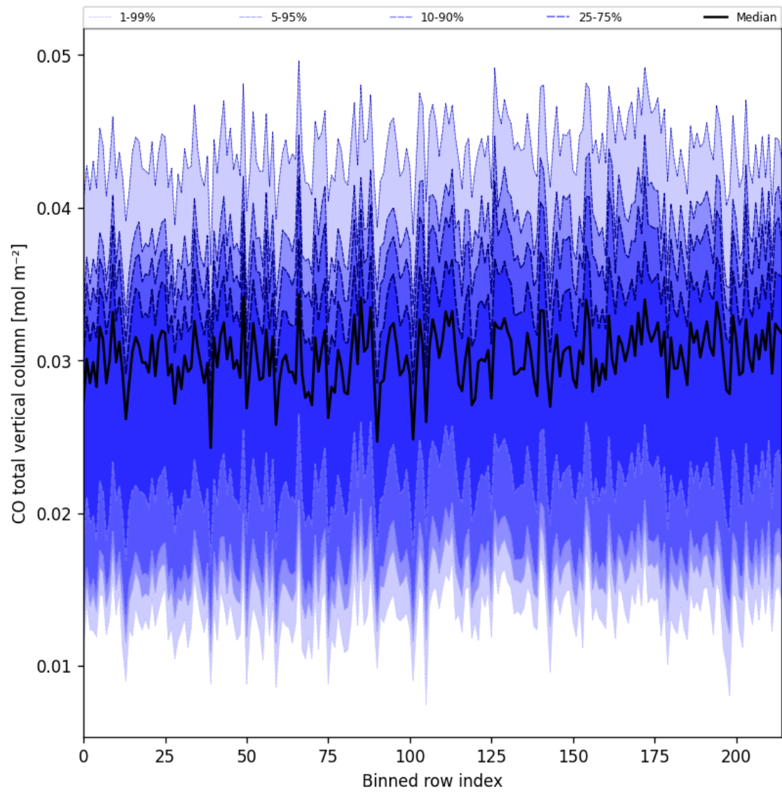
Figure 21: Along track statistics of “CO total vertical column” for 2025-05-02 to 2025-05-02
