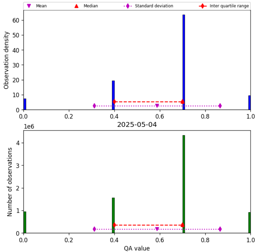
Figure 13: Histogram of “QA value” for 2025-05-04 to 2025-05-05
