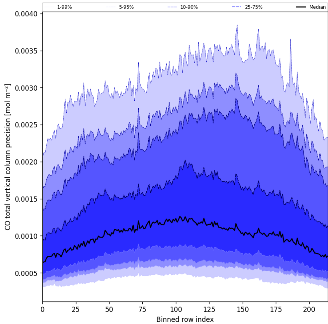
Figure 22: Along track statistics of “CO total vertical column precision” for 2025-05-04 to 2025-05-05
