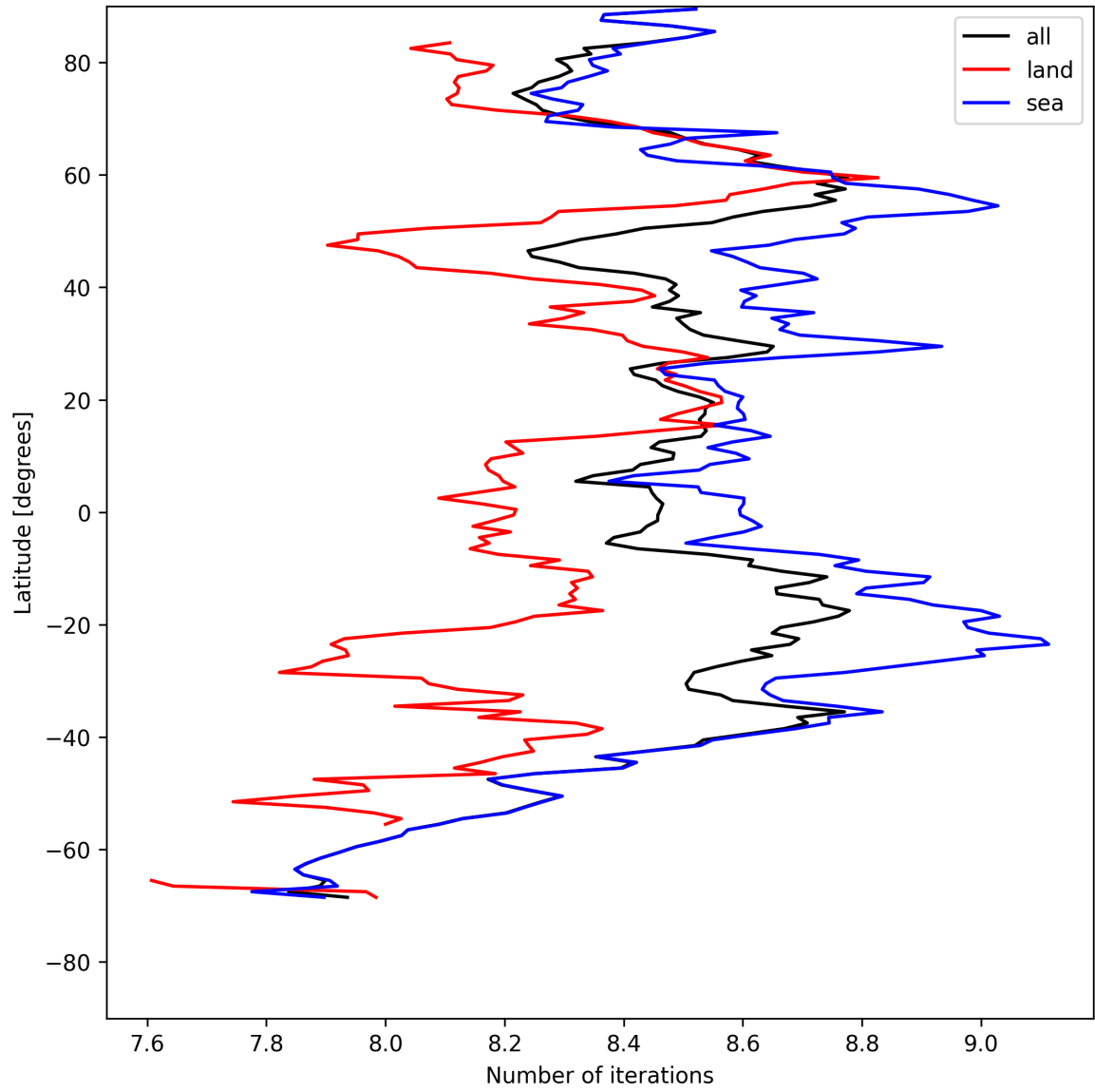
Figure 12: Zonal average of “Number of iterations” for 2025-05-04 to 2025-05-05.
