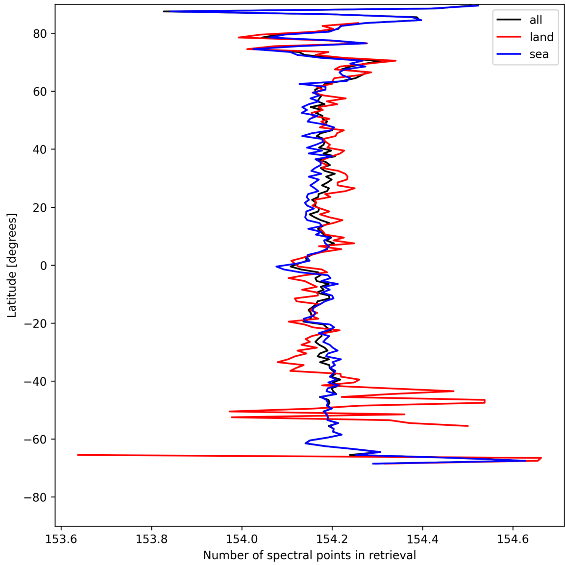
Figure 9: Zonal average of “Number of spectral points in retrieval” for 2025-05-04 to 2025-05-05.
