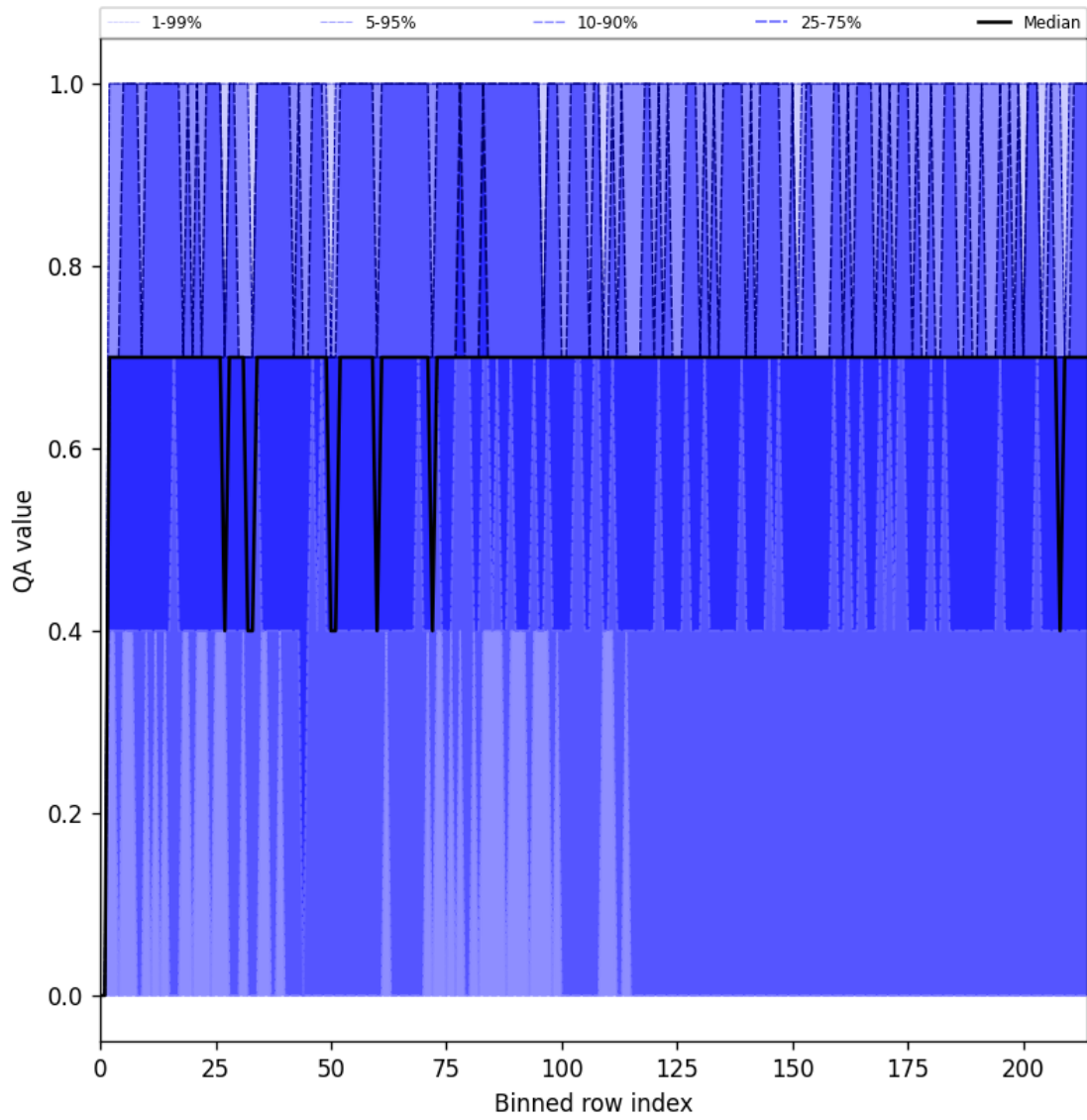
Figure 20: Along track statistics of “QA value” for 2025-05-04 to 2025-05-05
