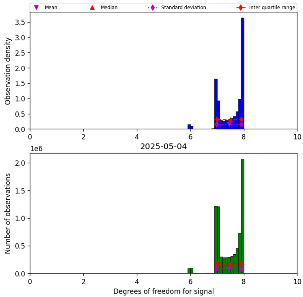
Figure 18: Histogram of “Degrees of freedom for signal” for 2025-05-04 to 2025-05-05
