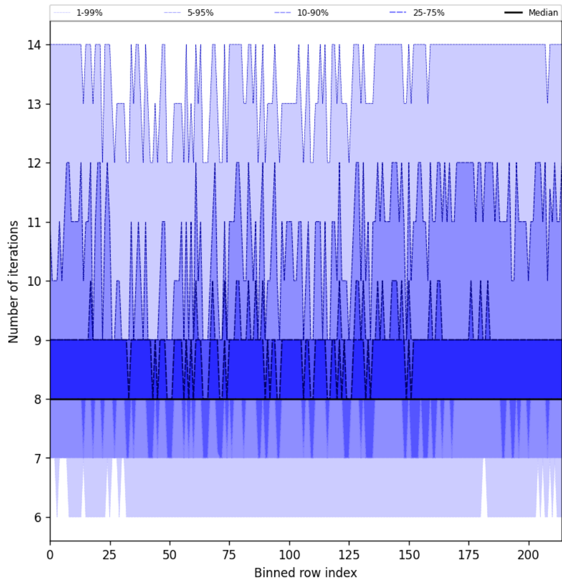
Figure 26: Along track statistics of “Number of iterations” for 2025-05-04 to 2025-05-05
