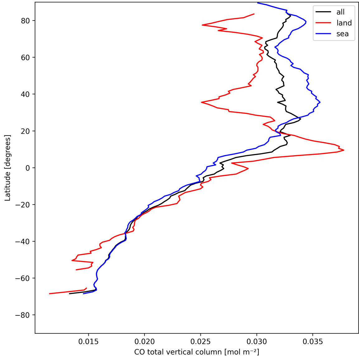
Figure 7: Zonal average of “CO total vertical column” for 2025-05-04 to 2025-05-05.
