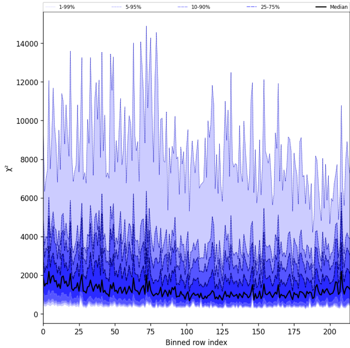
Figure 24: Along track statistics of “ \chi^2 ” for 2025-05-04 to 2025-05-05
