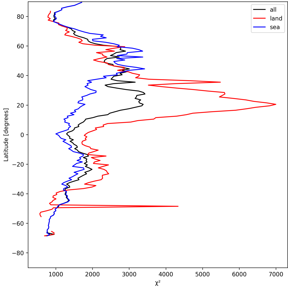
Figure 10: Zonal average of “ \chi^2 ” for 2025-05-04 to 2025-05-05.
