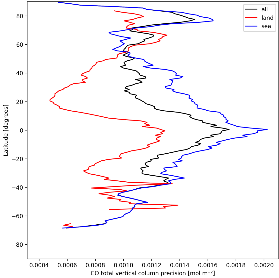
Figure 8: Zonal average of “CO total vertical column precision” for 2025-05-04 to 2025-05-05.
