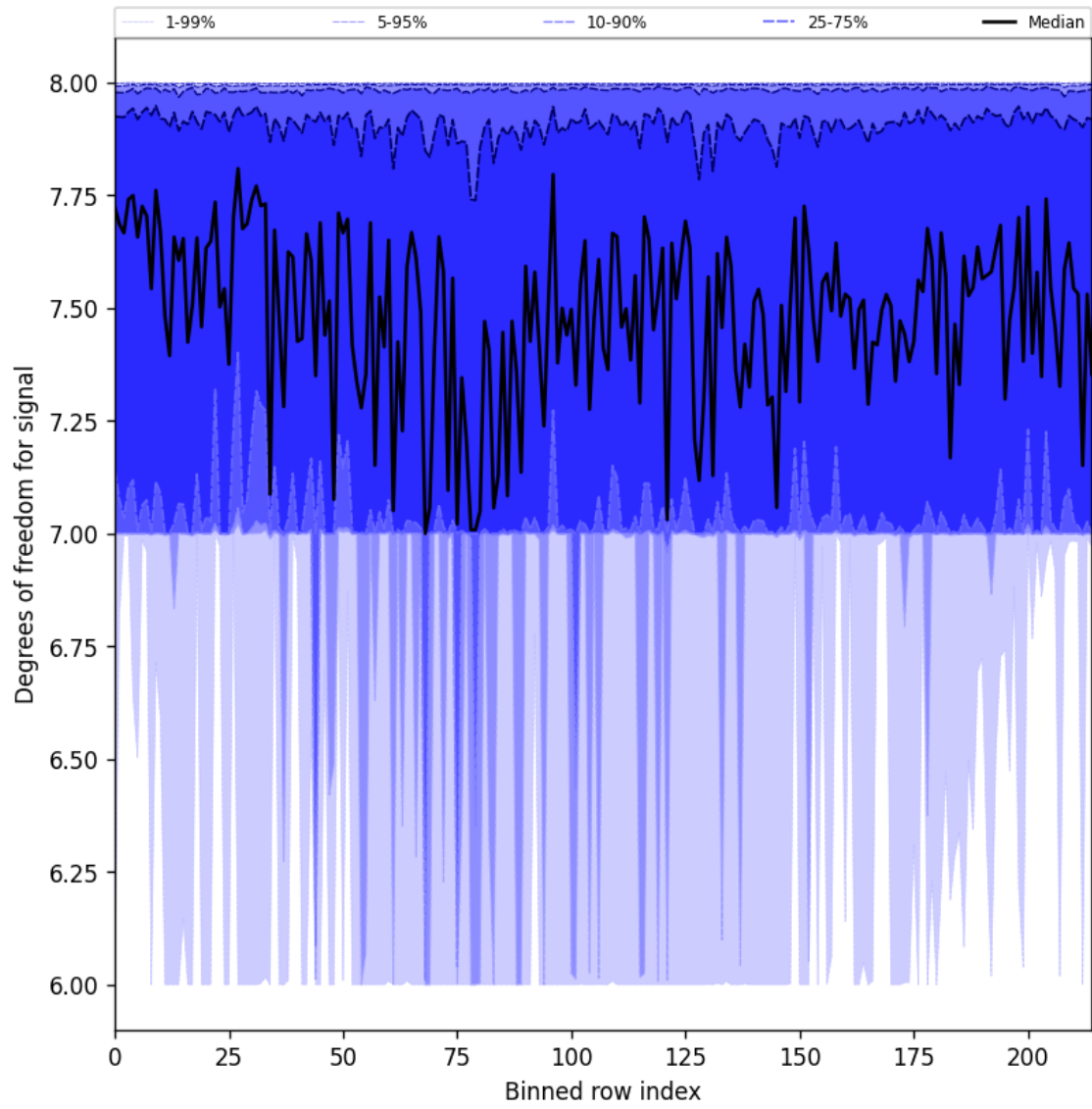
Figure 25: Along track statistics of “Degrees of freedom for signal” for 2025-05-04 to 2025-05-05
