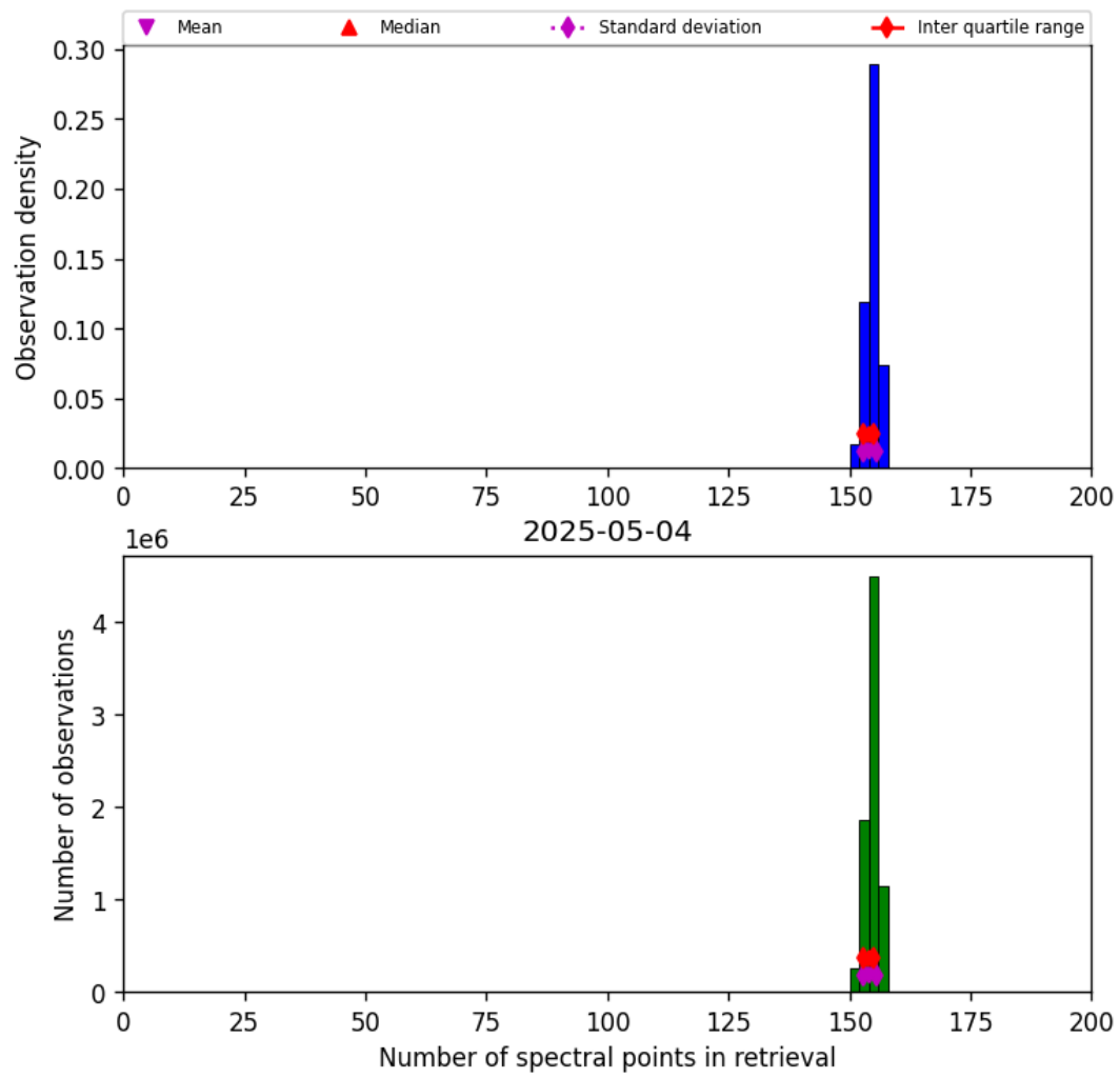
Figure 16: Histogram of “Number of spectral points in retrieval” for 2025-05-04 to 2025-05-05
