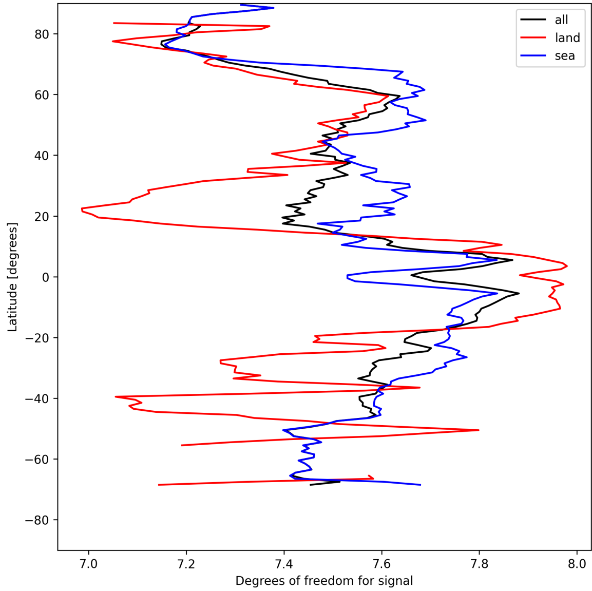
Figure 11: Zonal average of “Degrees of freedom for signal” for 2025-05-04 to 2025-05-05.
