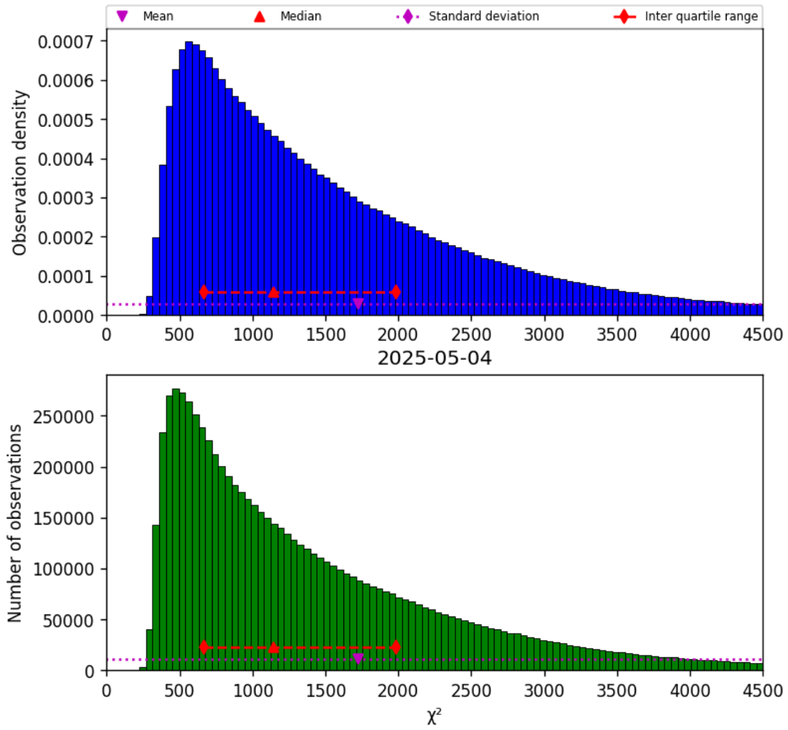
Figure 17: Histogram of " \chi^2 " for 2025-05-04 to 2025-05-05
