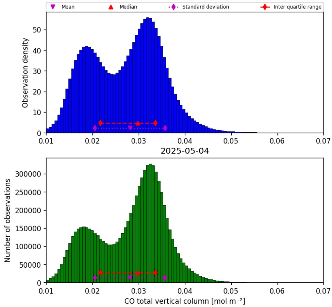
Figure 14: Histogram of “CO total vertical column” for 2025-05-04 to 2025-05-05
