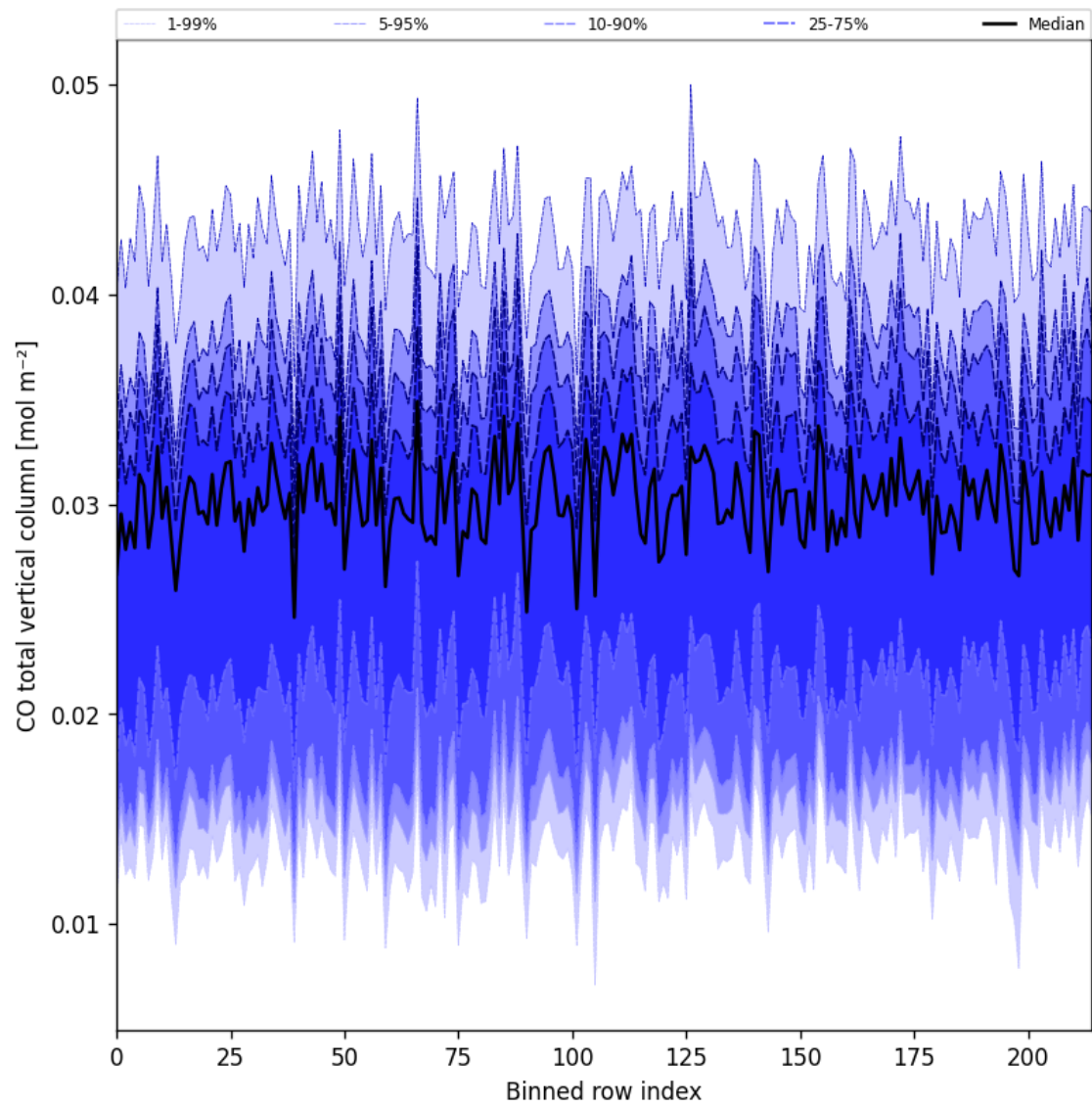
Figure 21: Along track statistics of “CO total vertical column” for 2025-05-04 to 2025-05-05
