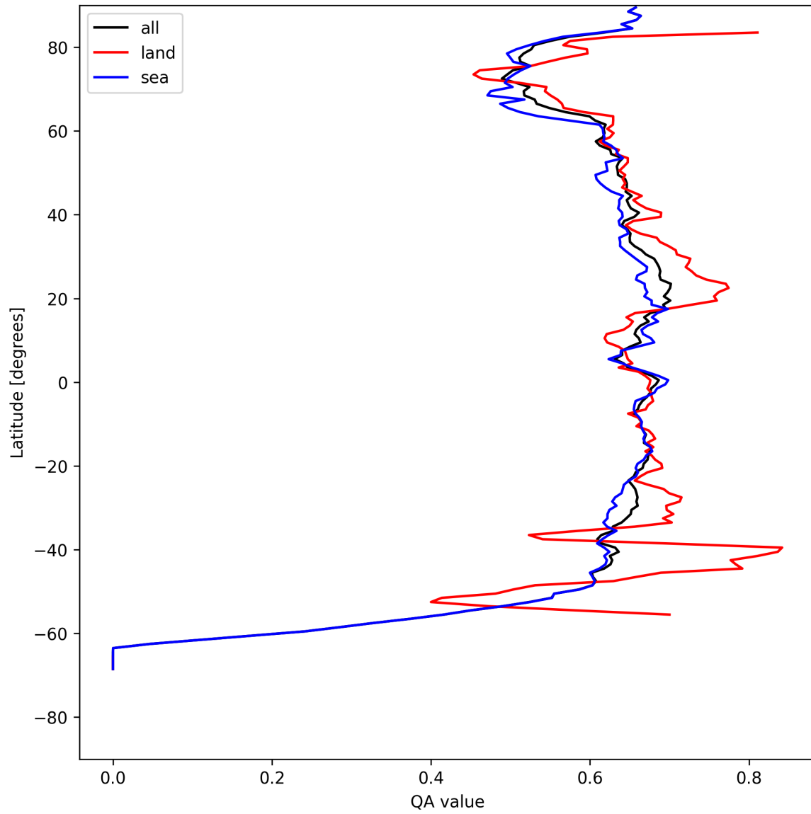
Figure 6: Zonal average of “QA value” for 2025-05-04 to 2025-05-05.
