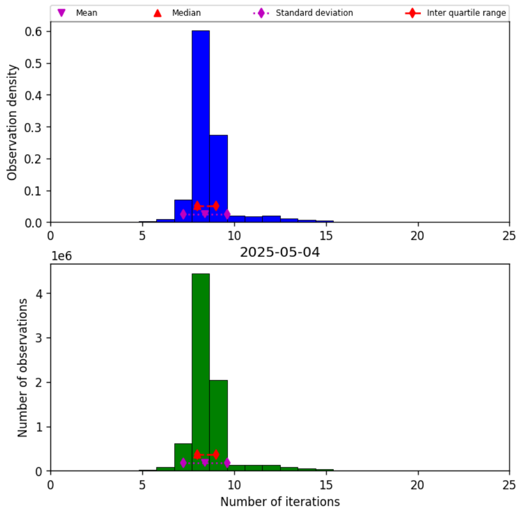
Figure 19: Histogram of “Number of iterations” for 2025-05-04 to 2025-05-05
