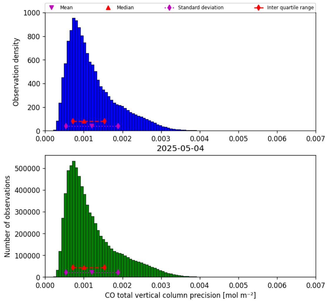
Figure 15: Histogram of “CO total vertical column precision” for 2025-05-04 to 2025-05-05
